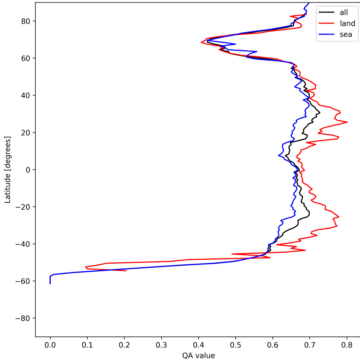
Figure 6: Zonal average of “QA value” for 2025-07-06 to 2025-07-06.
