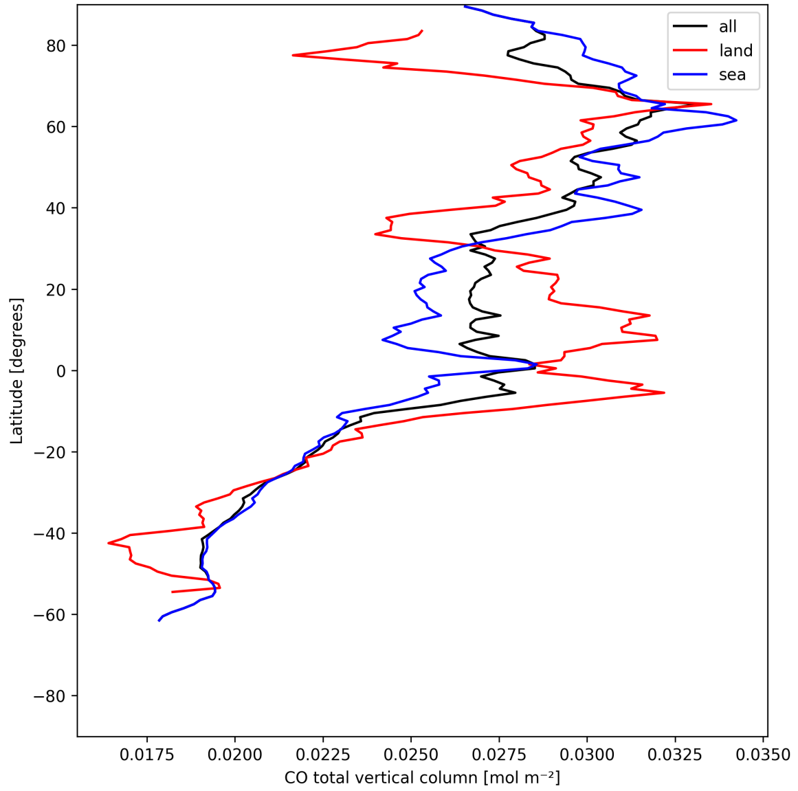
Figure 7: Zonal average of “CO total vertical column” for 2025-07-06 to 2025-07-06.
