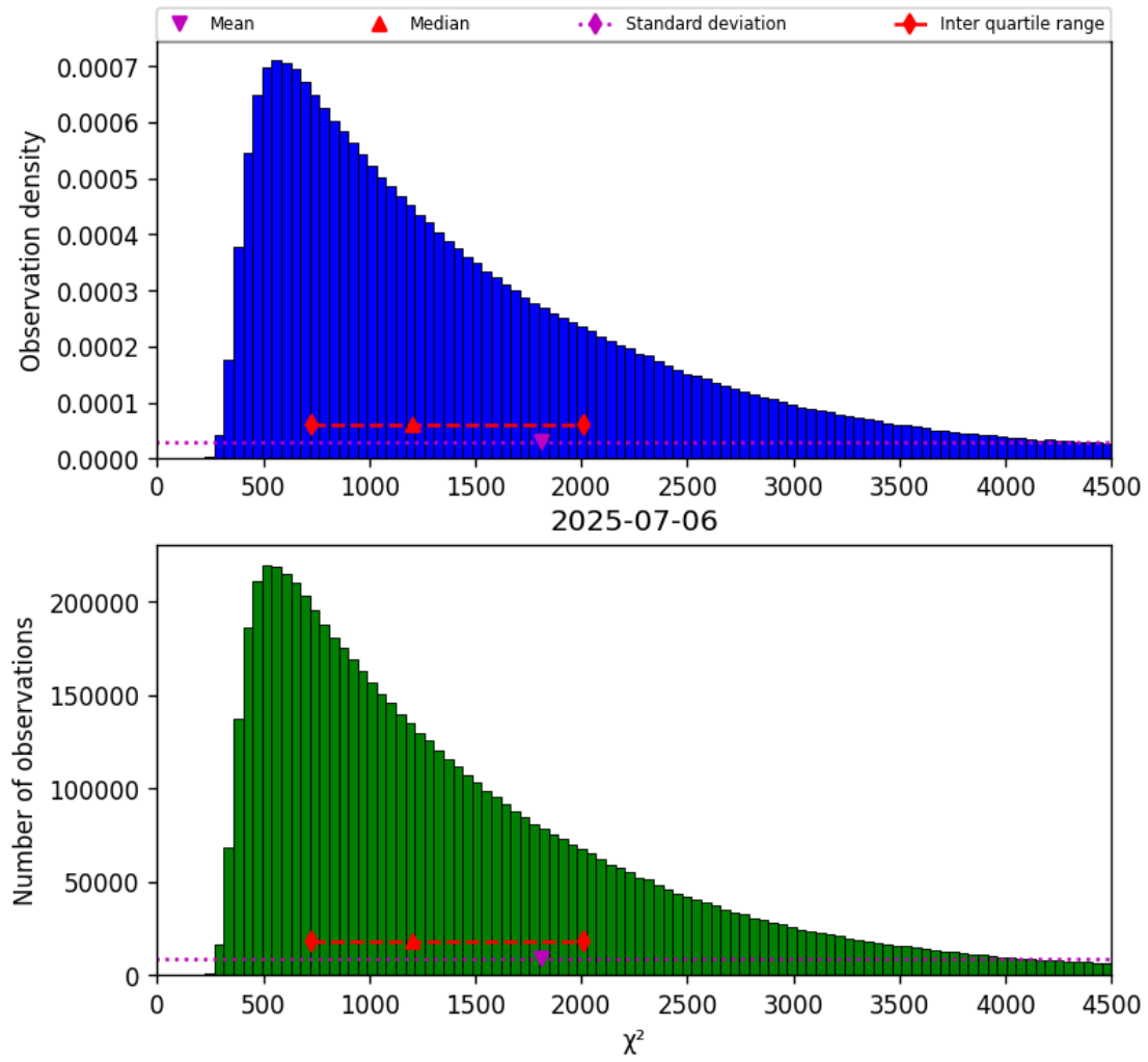
Figure 17: Histogram of “ \chi^2 ” for 2025-07-06 to 2025-07-06
