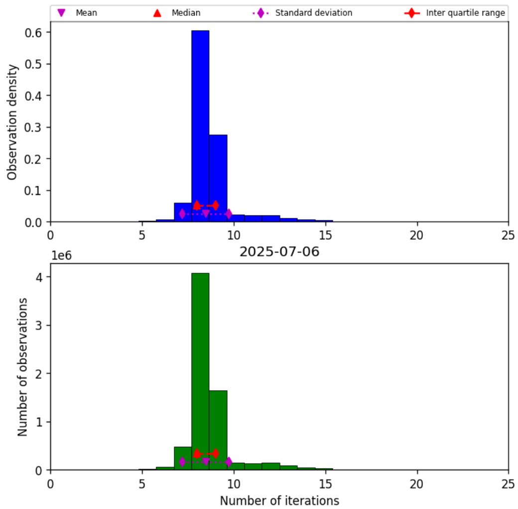
Figure 19: Histogram of “Number of iterations” for 2025-07-06 to 2025-07-06
