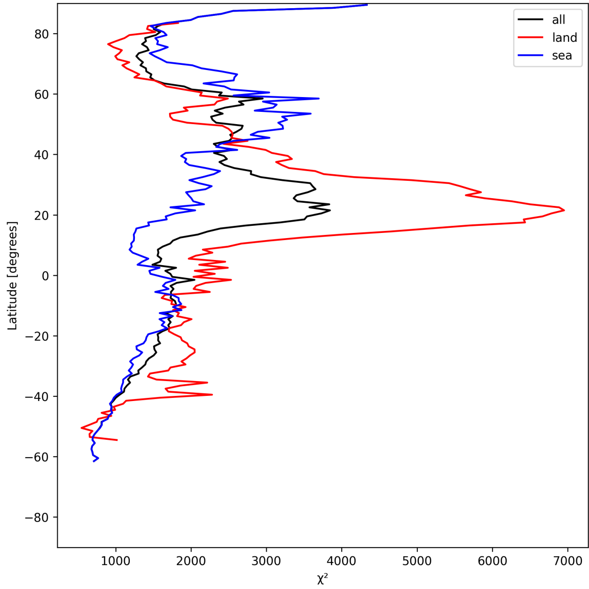
Figure 10: Zonal average of “ \chi^2 ” for 2025-07-06 to 2025-07-06.
