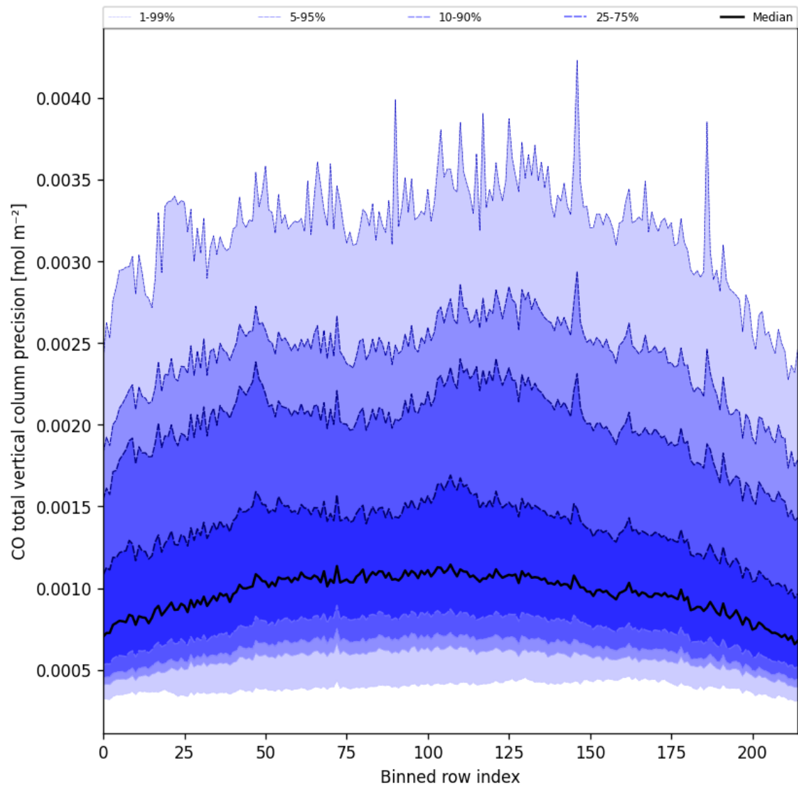
Figure 22: Along track statistics of “CO total vertical column precision” for 2025-07-06 to 2025-07-06
