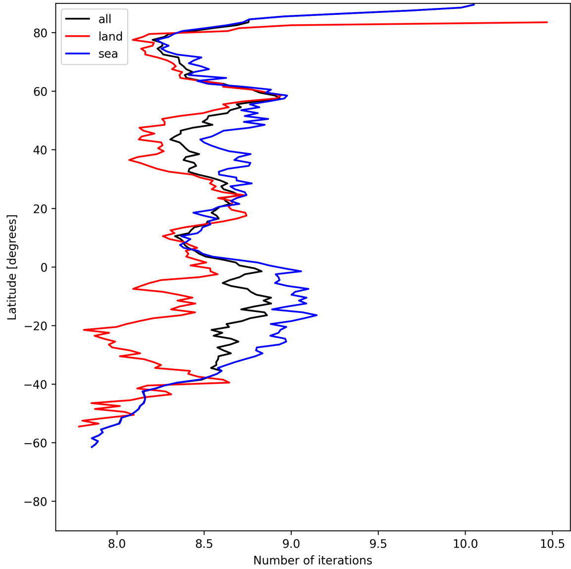
Figure 12: Zonal average of “Number of iterations” for 2025-07-06 to 2025-07-06.
