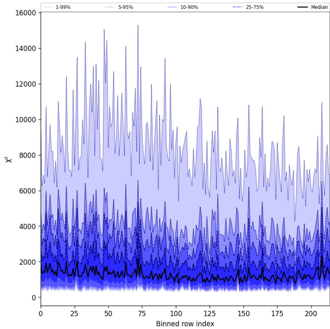
Figure 24: Along track statistics of “ \chi^2 ” for 2025-07-06 to 2025-07-06
