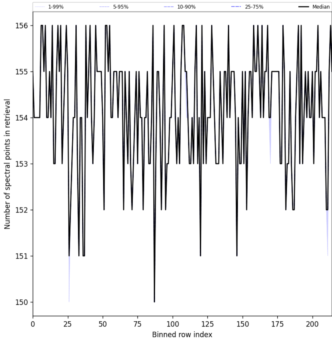
Figure 23: Along track statistics of “Number of spectral points in retrieval” for 2025-07-06 to 2025-07-06
