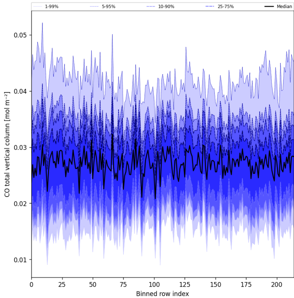
Figure 21: Along track statistics of “CO total vertical column” for 2025-07-06 to 2025-07-06
