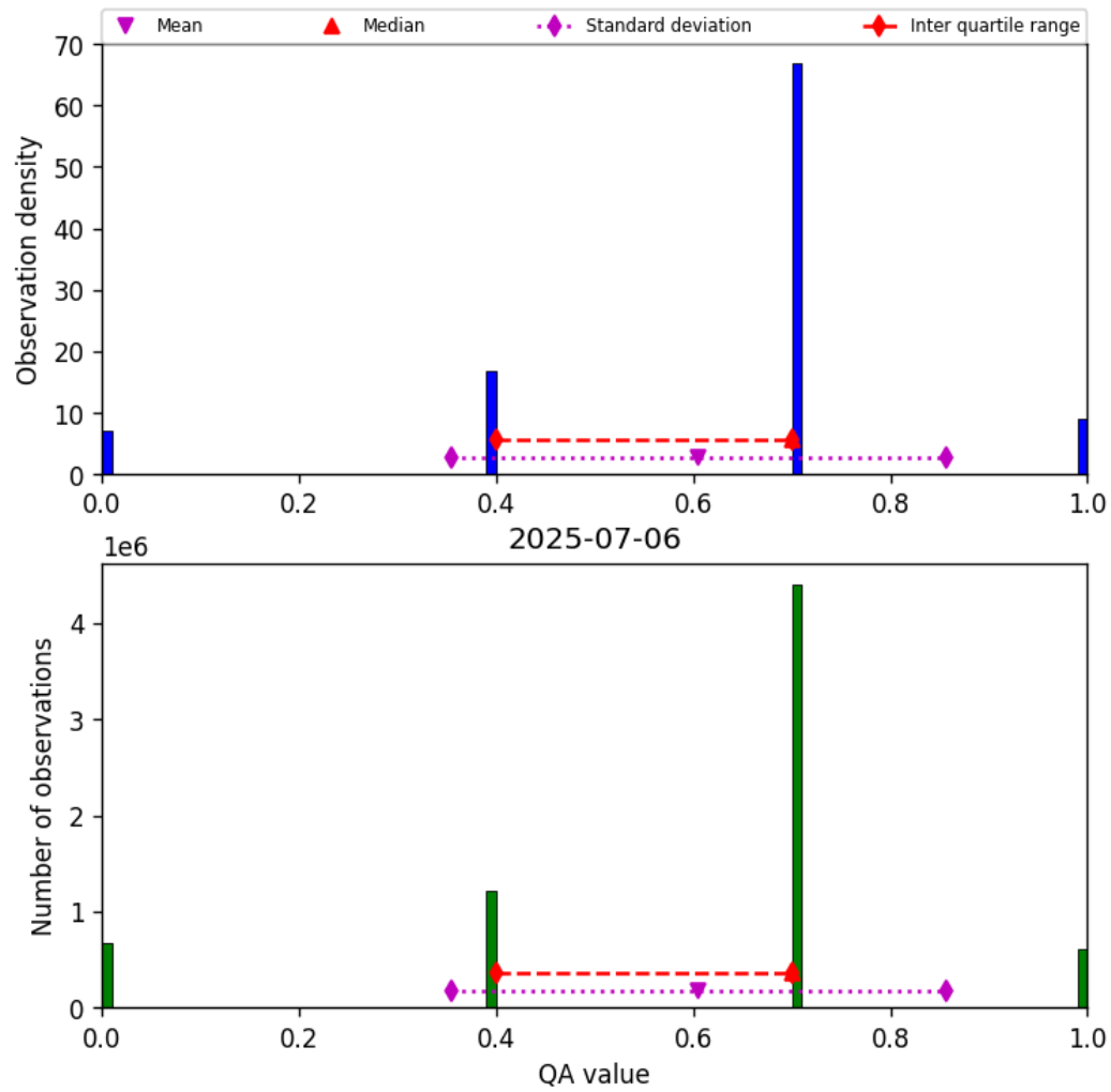
Figure 13: Histogram of “QA value” for 2025-07-06 to 2025-07-06
