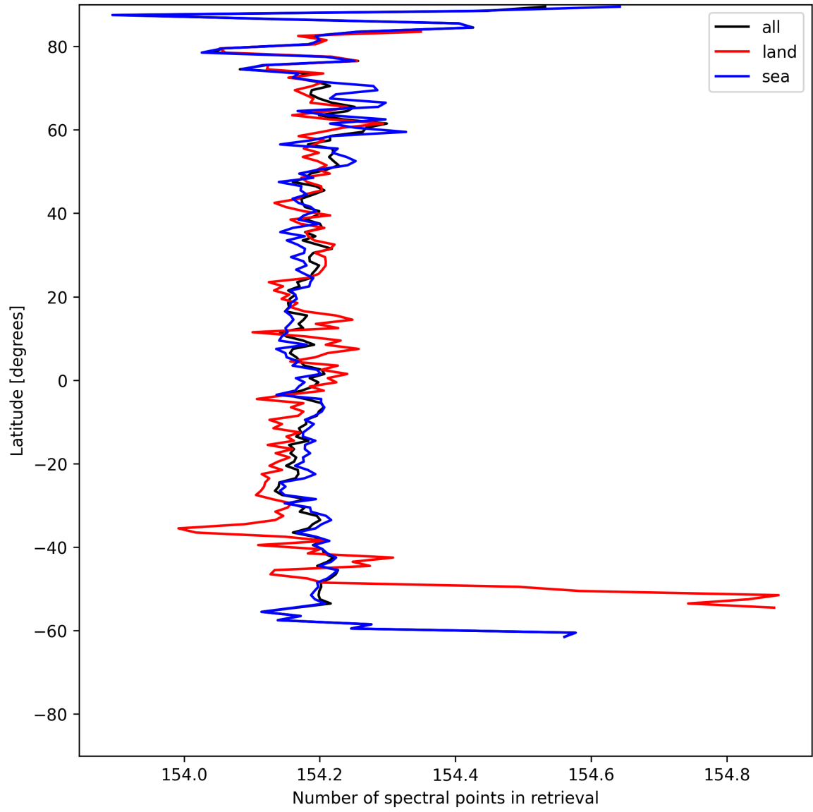
Figure 9: Zonal average of “Number of spectral points in retrieval” for 2025-07-06 to 2025-07-06.
