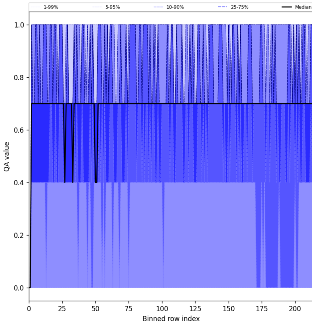
Figure 20: Along track statistics of “QA value” for 2025-07-06 to 2025-07-06
