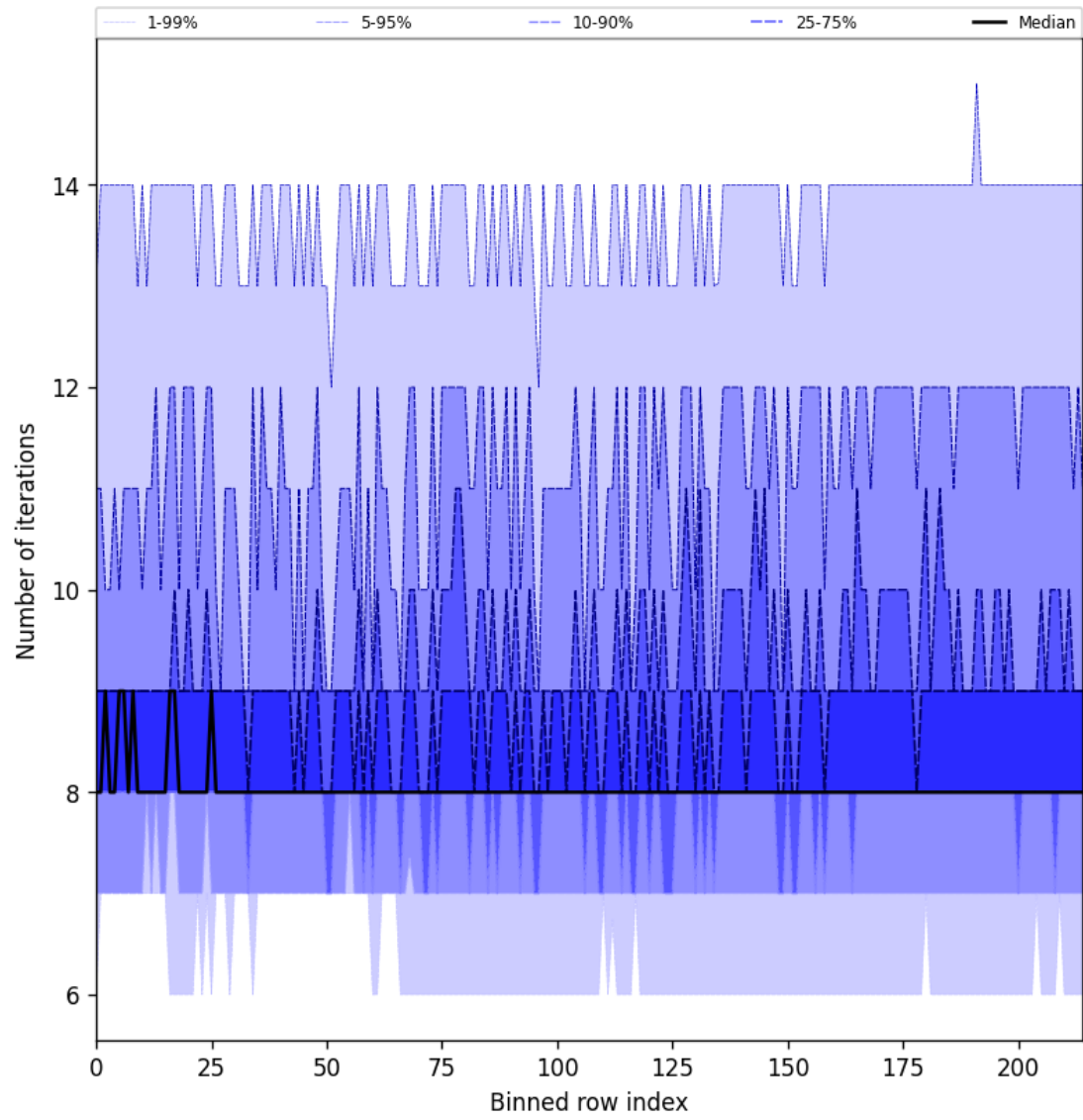
Figure 26: Along track statistics of “Number of iterations” for 2025-07-06 to 2025-07-06
