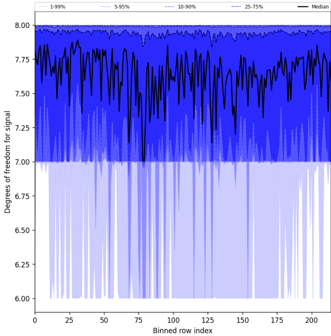
Figure 25: Along track statistics of “Degrees of freedom for signal” for 2025-07-06 to 2025-07-06
