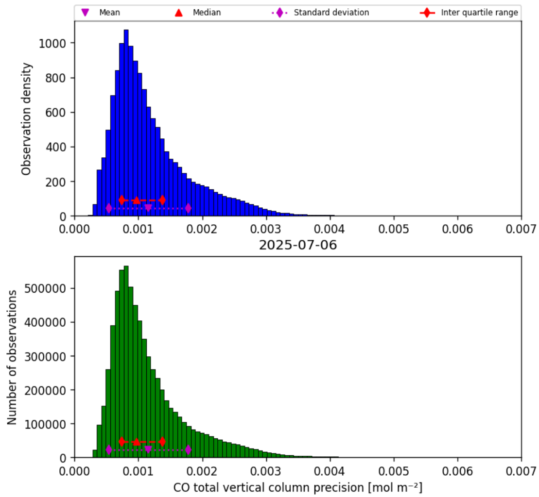
Figure 15: Histogram of “CO total vertical column precision” for 2025-07-06 to 2025-07-06
