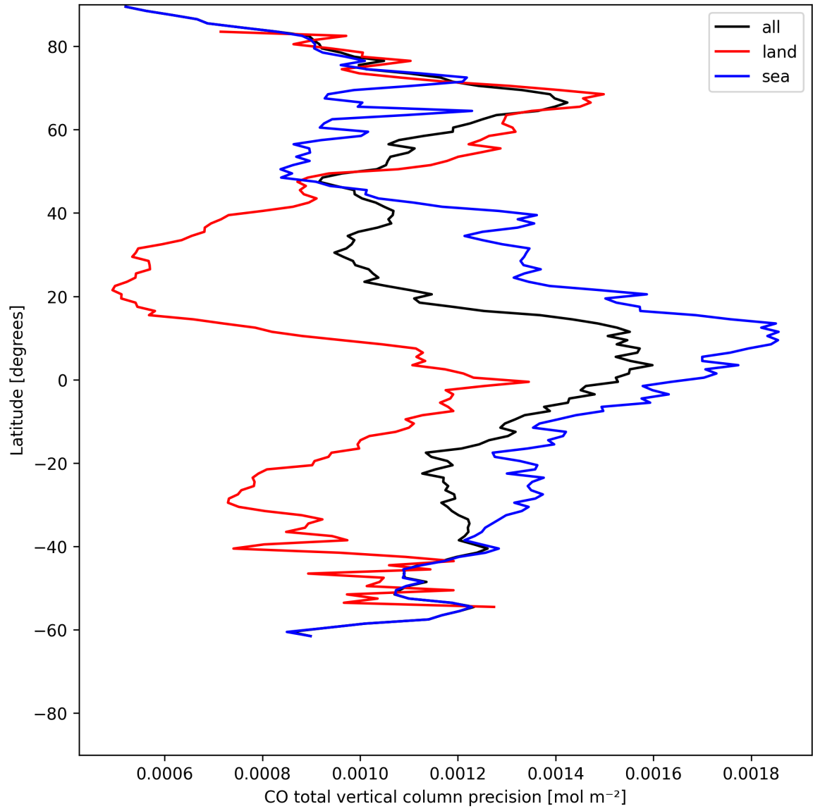
Figure 8: Zonal average of "CO total vertical column precision" for 2025-07-06 to 2025-07-06.
