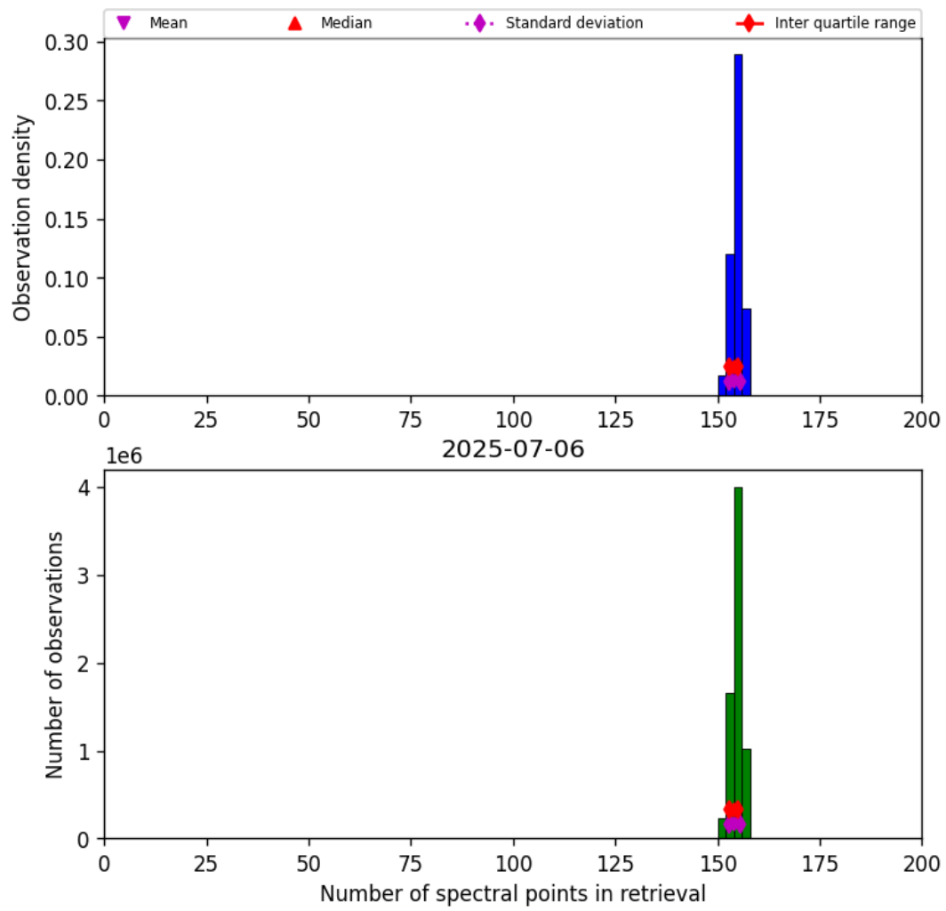
Figure 16: Histogram of “Number of spectral points in retrieval” for 2025-07-06 to 2025-07-06
