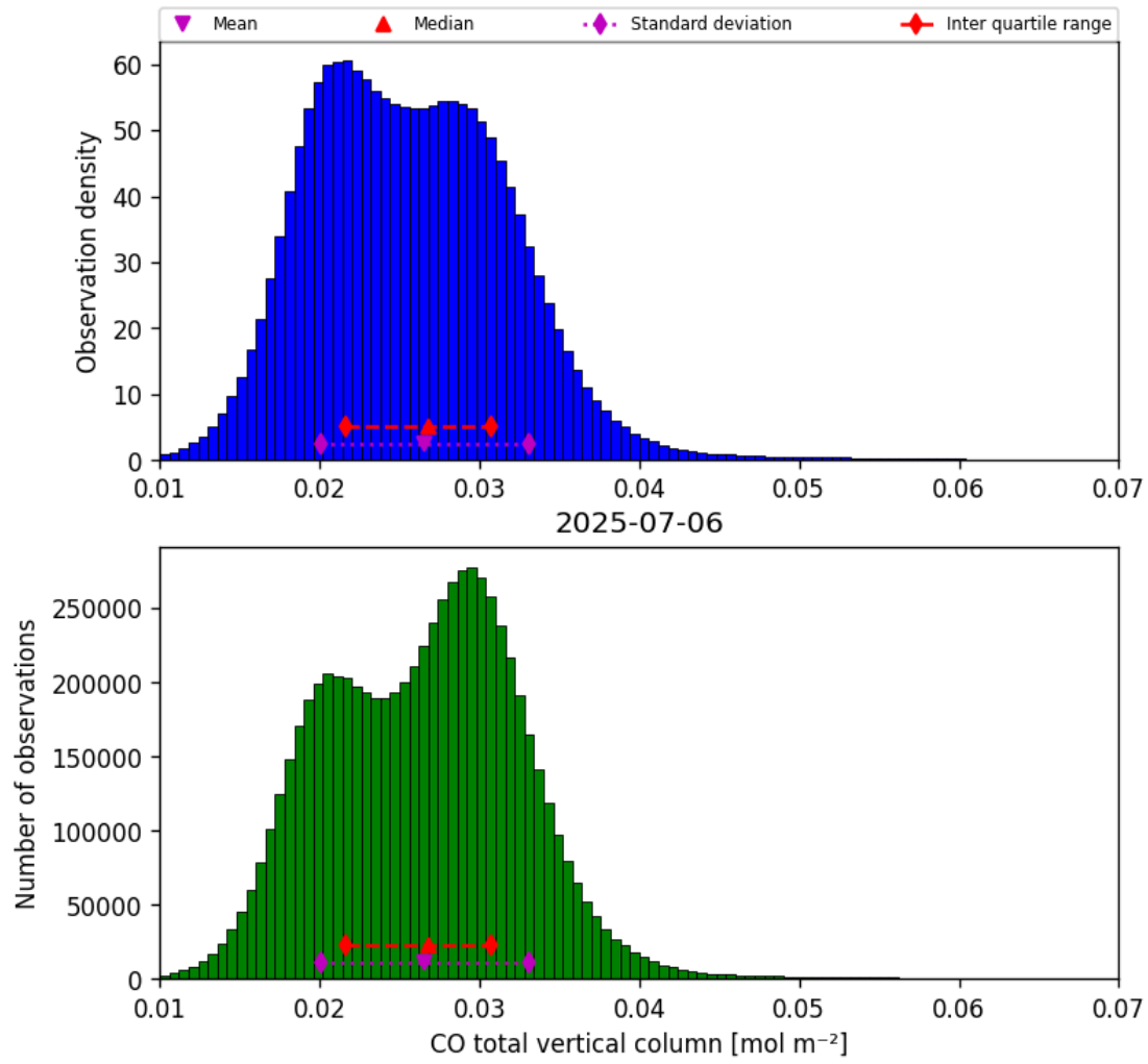
Figure 14: Histogram of “CO total vertical column” for 2025-07-06 to 2025-07-06
