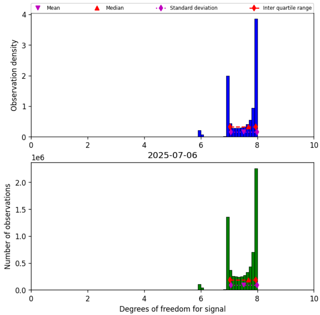
Figure 18: Histogram of “Degrees of freedom for signal” for 2025-07-06 to 2025-07-06
