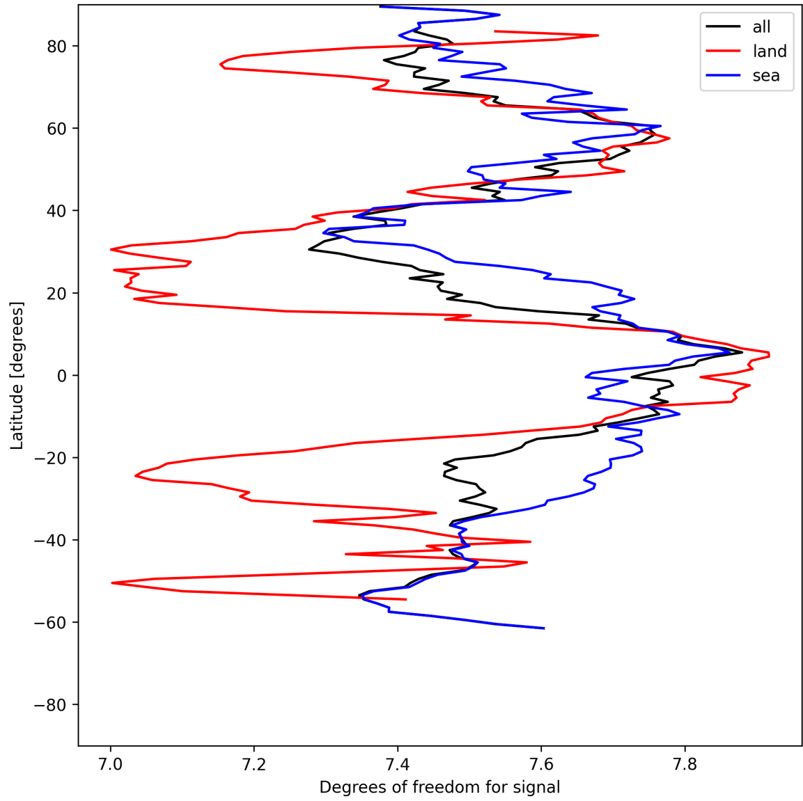
Figure 11: Zonal average of “Degrees of freedom for signal” for 2025-07-06 to 2025-07-06.
