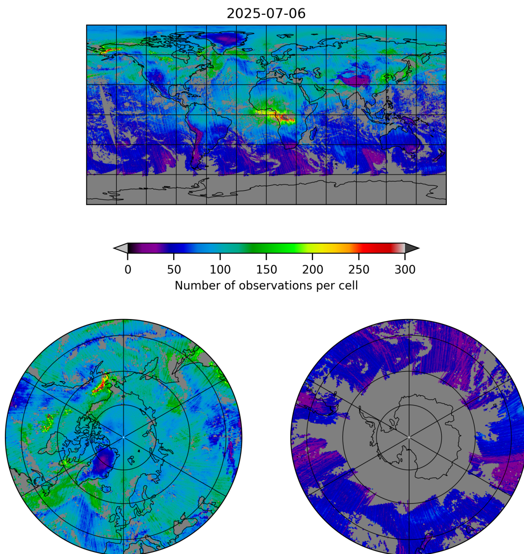
Figure 5: Map of the number of observations for 2025-07-06 to 2025-07-06
