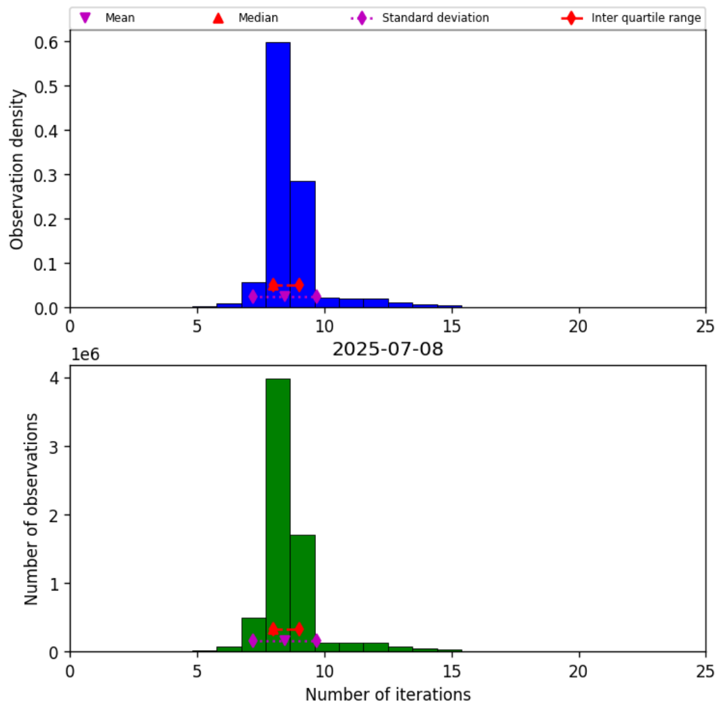
Figure 19: Histogram of “Number of iterations” for 2025-07-08 to 2025-07-09
