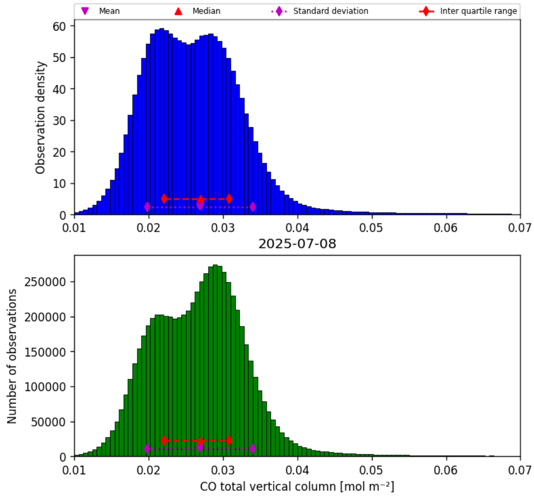
Figure 14: Histogram of “CO total vertical column” for 2025-07-08 to 2025-07-09
