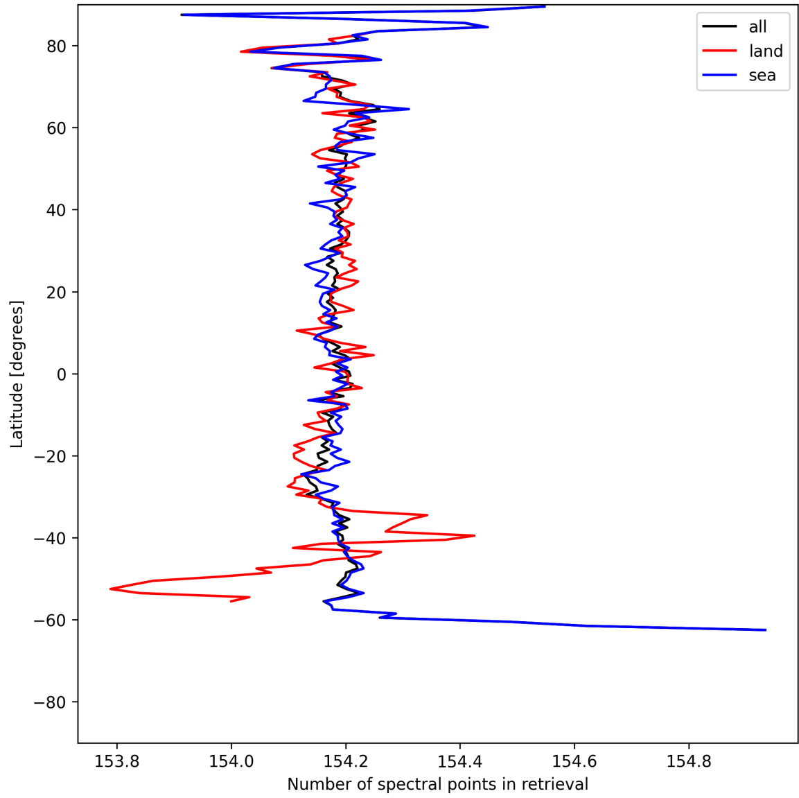
Figure 9: Zonal average of “Number of spectral points in retrieval” for 2025-07-08 to 2025-07-09.
