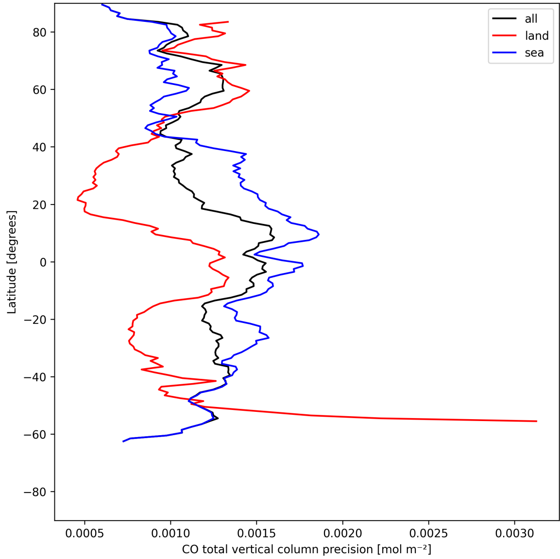
Figure 8: Zonal average of “CO total vertical column precision” for 2025-07-08 to 2025-07-09.
