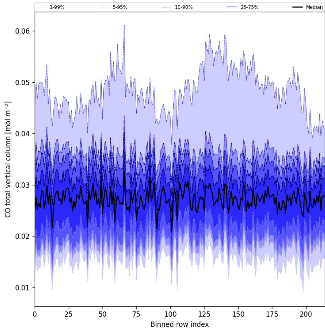
Figure 21: Along track statistics of “CO total vertical column” for 2025-07-08 to 2025-07-09
