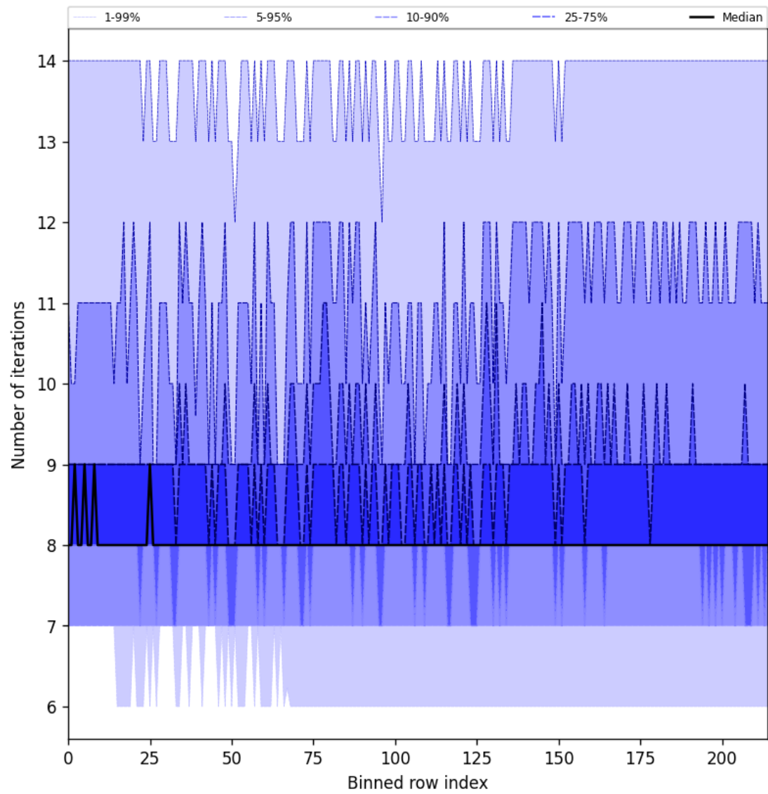
Figure 26: Along track statistics of “Number of iterations” for 2025-07-08 to 2025-07-09
