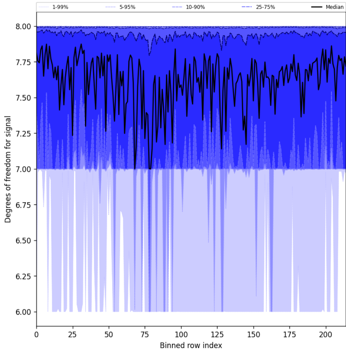
Figure 25: Along track statistics of “Degrees of freedom for signal” for 2025-07-08 to 2025-07-09
