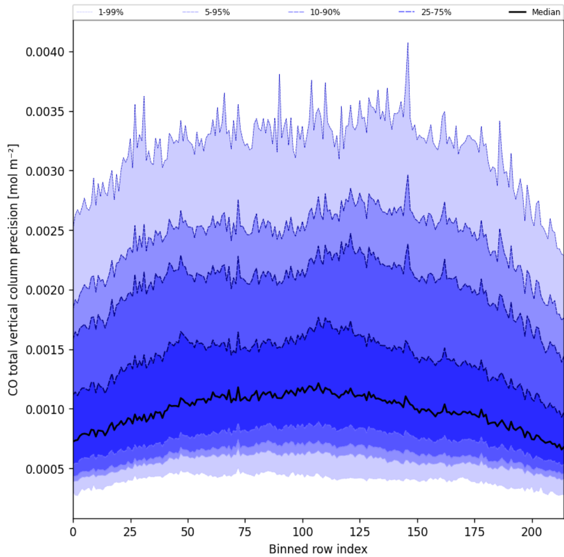
Figure 22: Along track statistics of “CO total vertical column precision” for 2025-07-08 to 2025-07-09
