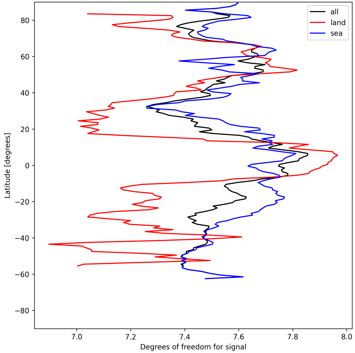
Figure 11: Zonal average of “Degrees of freedom for signal” for 2025-07-08 to 2025-07-09.
