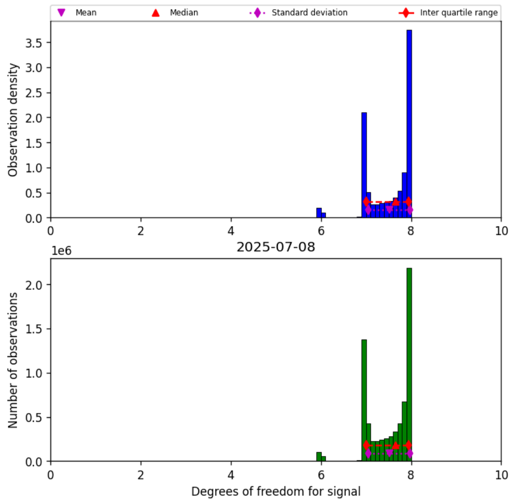
Figure 18: Histogram of “Degrees of freedom for signal” for 2025-07-08 to 2025-07-09
