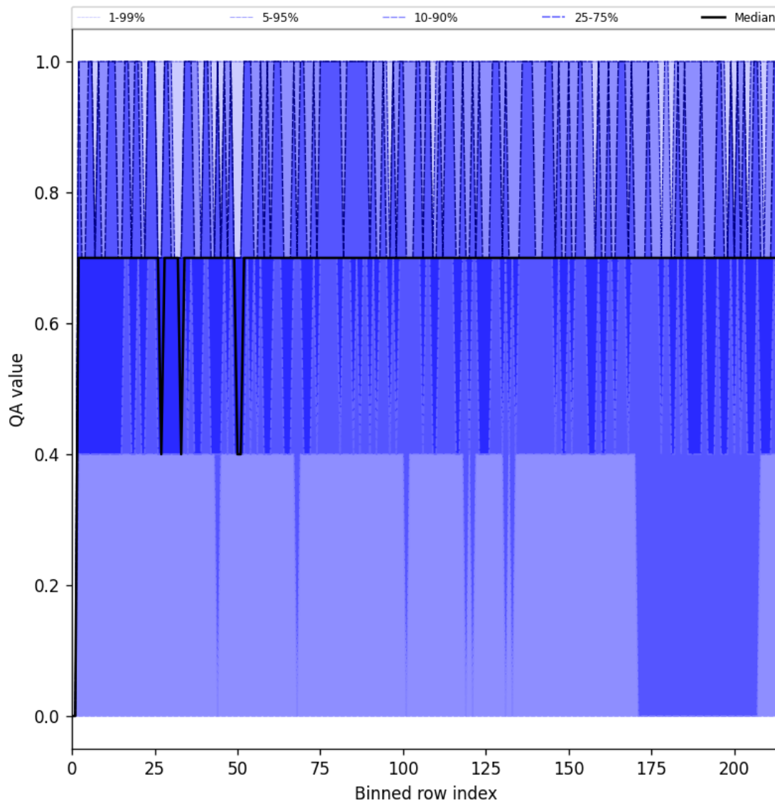
Figure 20: Along track statistics of “QA value” for 2025-07-08 to 2025-07-09
