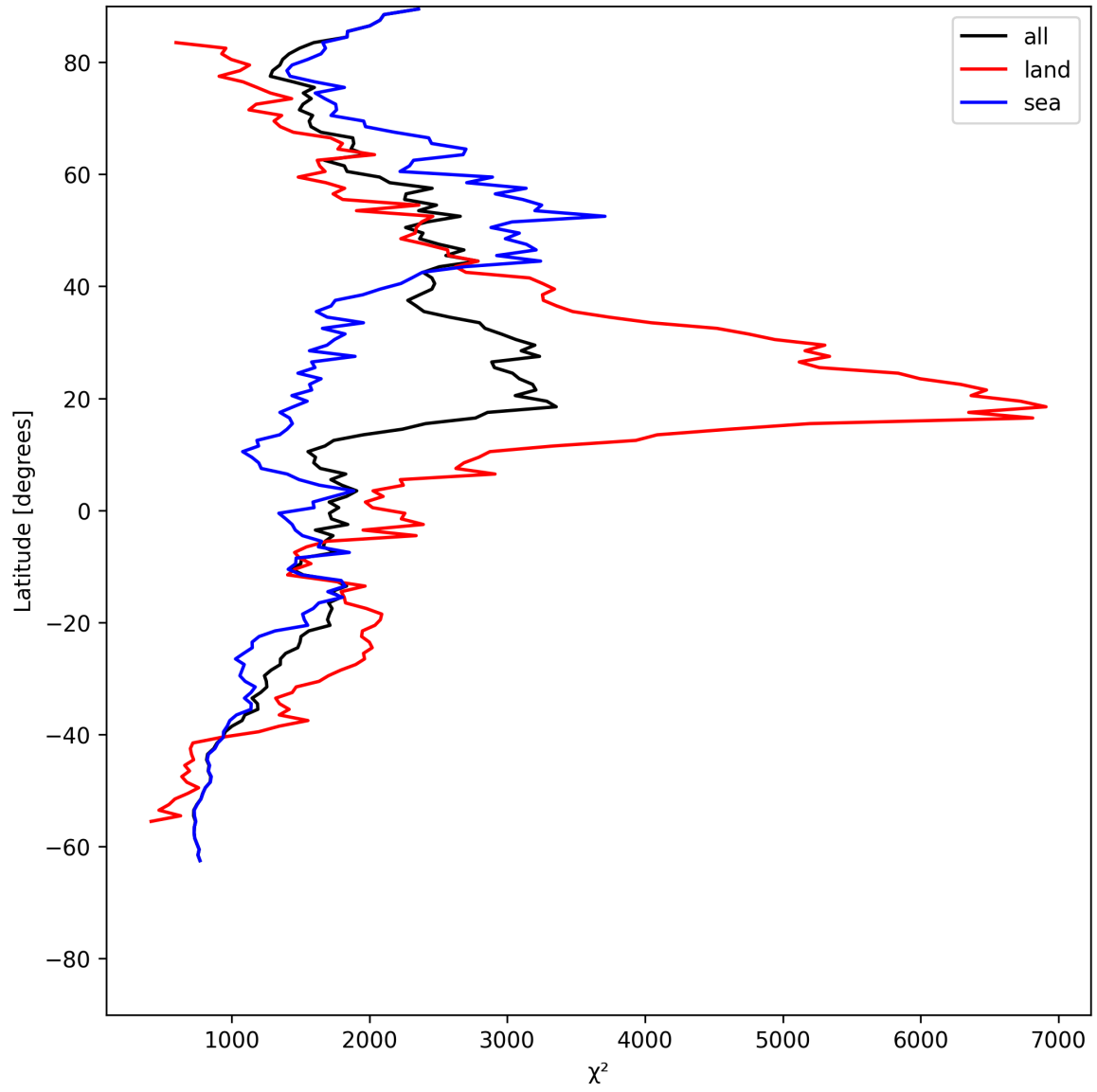
Figure 10: Zonal average of “ \chi^2 ” for 2025-07-08 to 2025-07-09.
