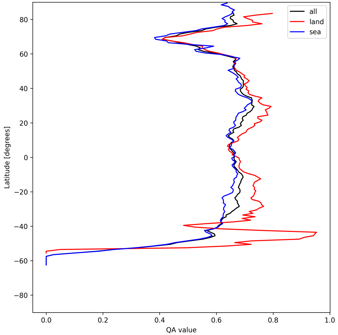
Figure 6: Zonal average of “QA value” for 2025-07-08 to 2025-07-09.
