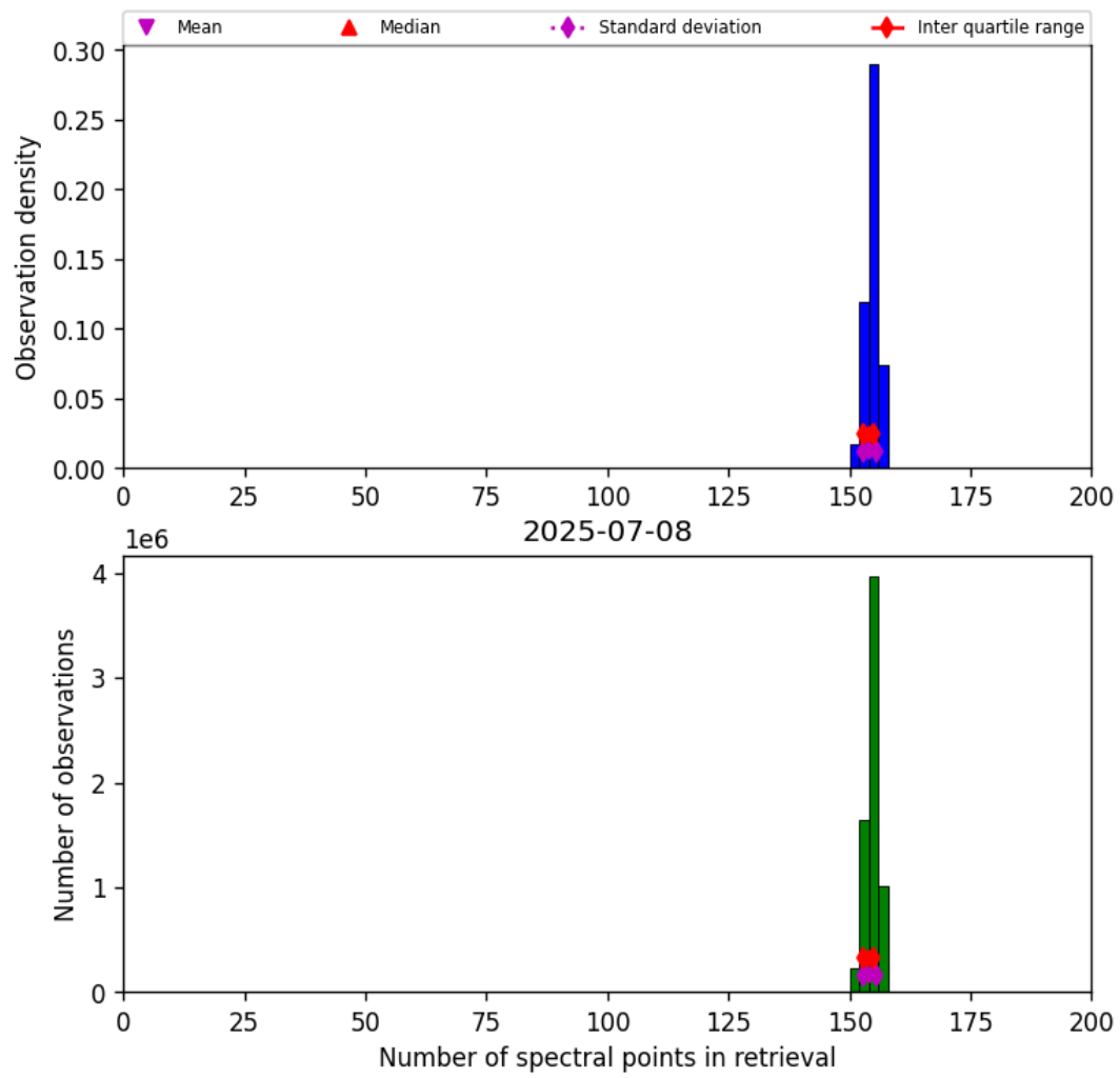
Figure 16: Histogram of “Number of spectral points in retrieval” for 2025-07-08 to 2025-07-09
