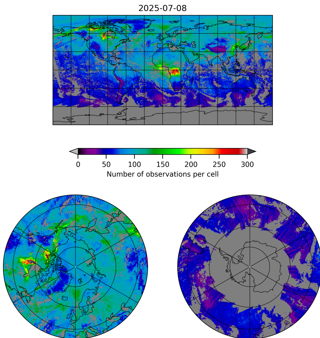
Figure 5: Map of the number of observations for 2025-07-08 to 2025-07-09
