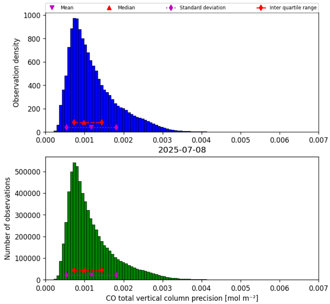
Figure 15: Histogram of “CO total vertical column precision” for 2025-07-08 to 2025-07-09
