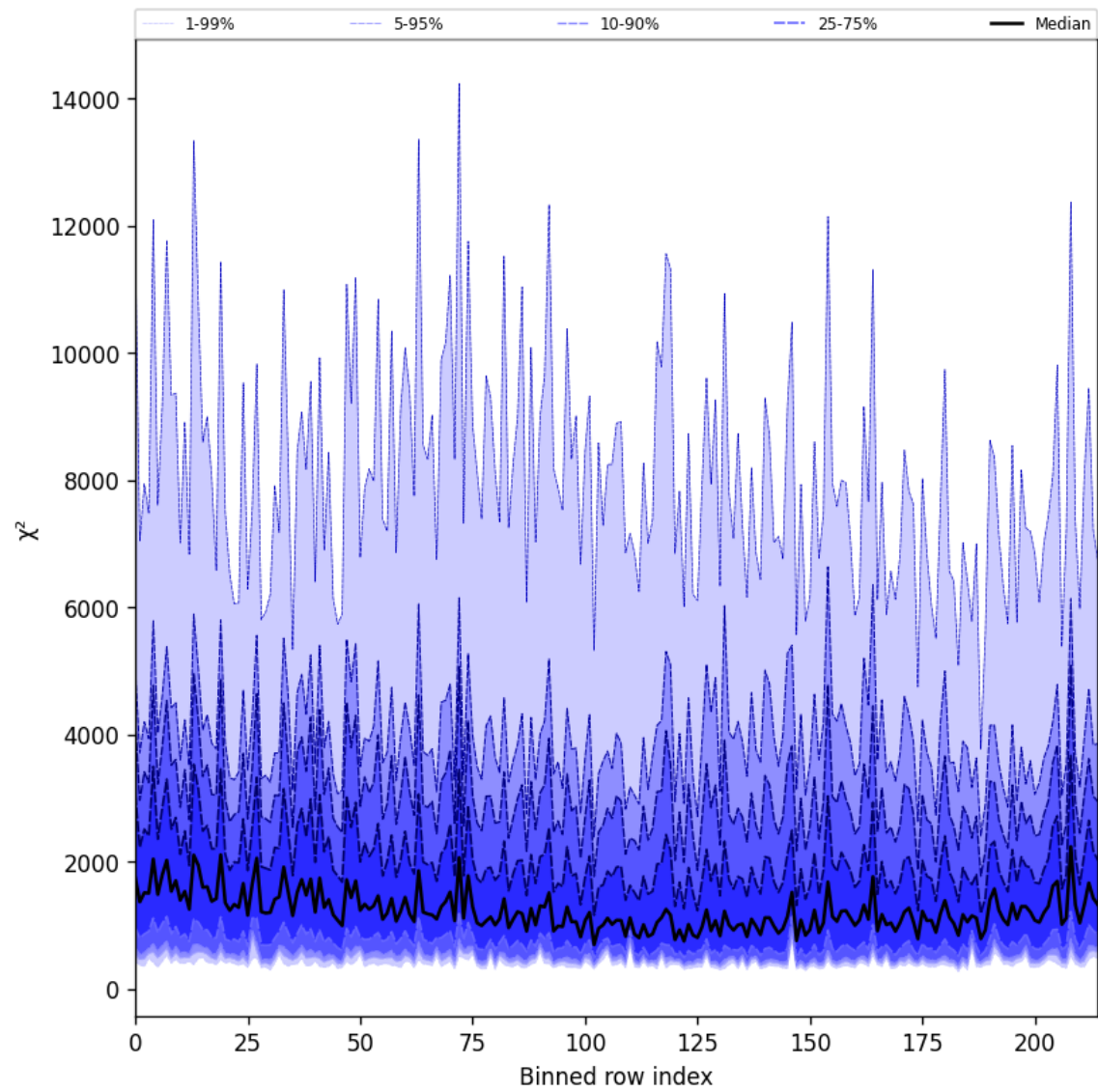
Figure 24: Along track statistics of “ \chi^2 ” for 2025-07-08 to 2025-07-09
