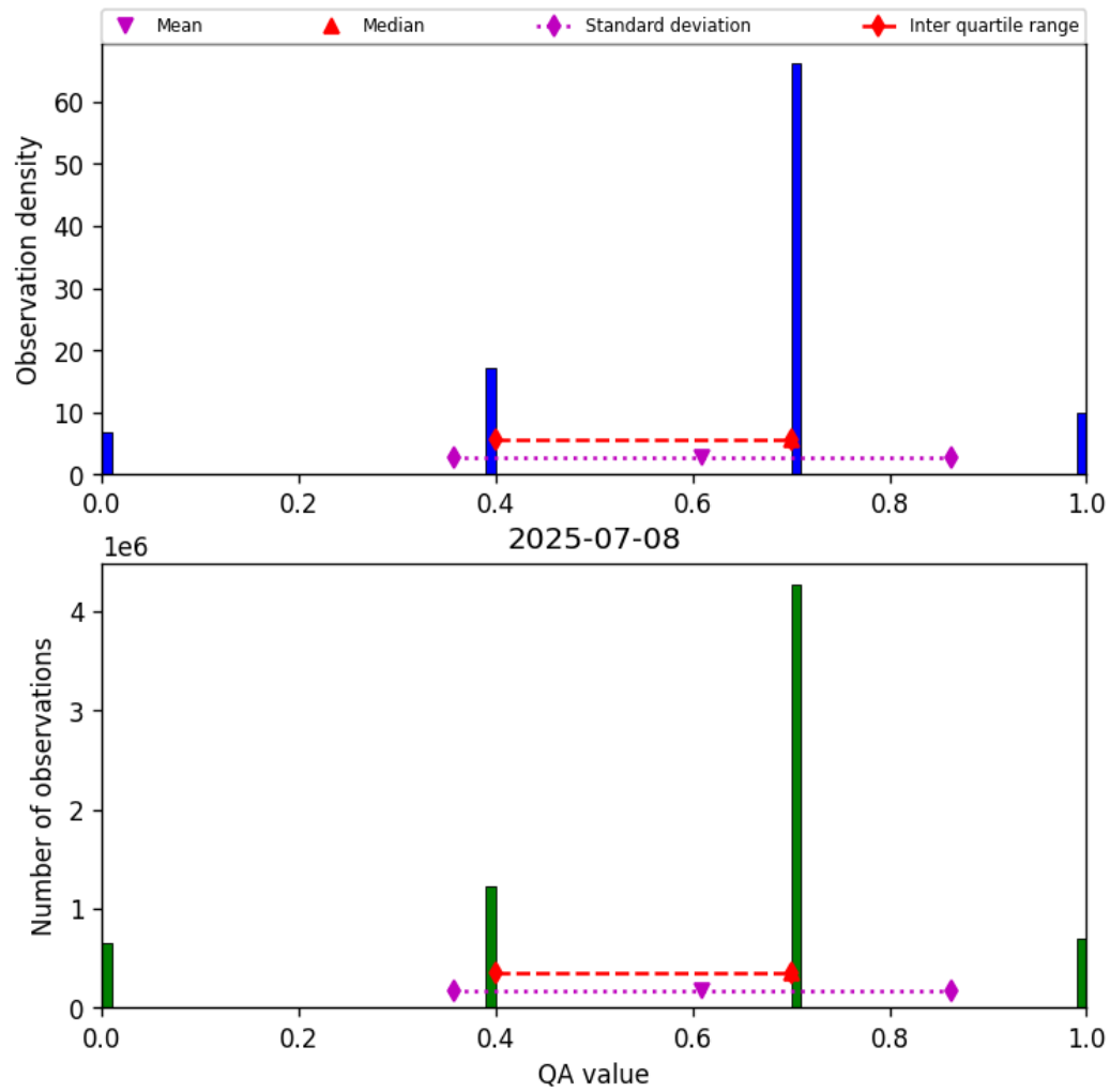
Figure 13: Histogram of “QA value” for 2025-07-08 to 2025-07-09
