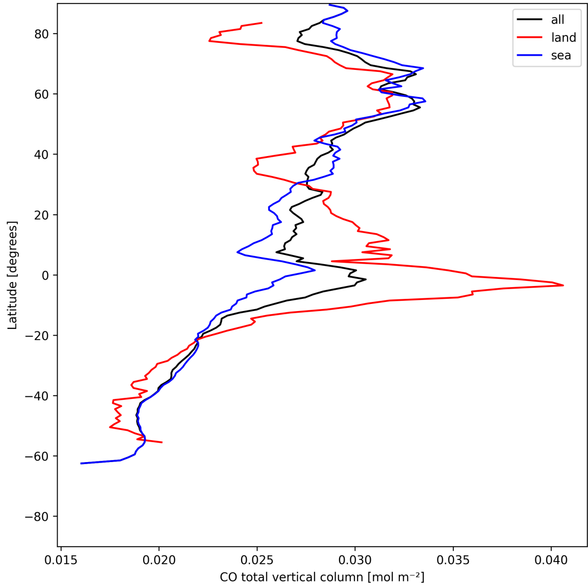
Figure 7: Zonal average of “CO total vertical column” for 2025-07-08 to 2025-07-09.
