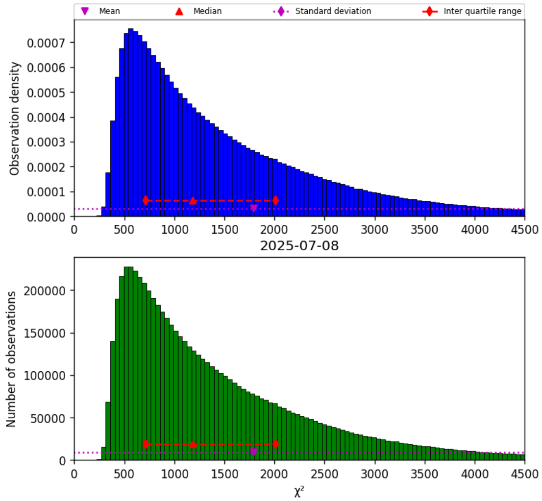
Figure 17: Histogram of “ \chi^2 ” for 2025-07-08 to 2025-07-09
