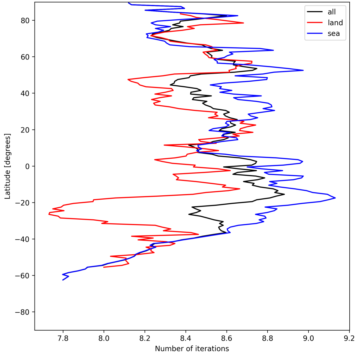
Figure 12: Zonal average of “Number of iterations” for 2025-07-08 to 2025-07-09.
