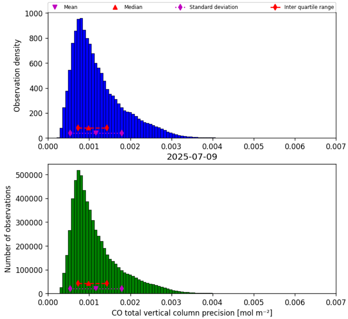
Figure 15: Histogram of “CO total vertical column precision” for 2025-07-09 to 2025-07-10
