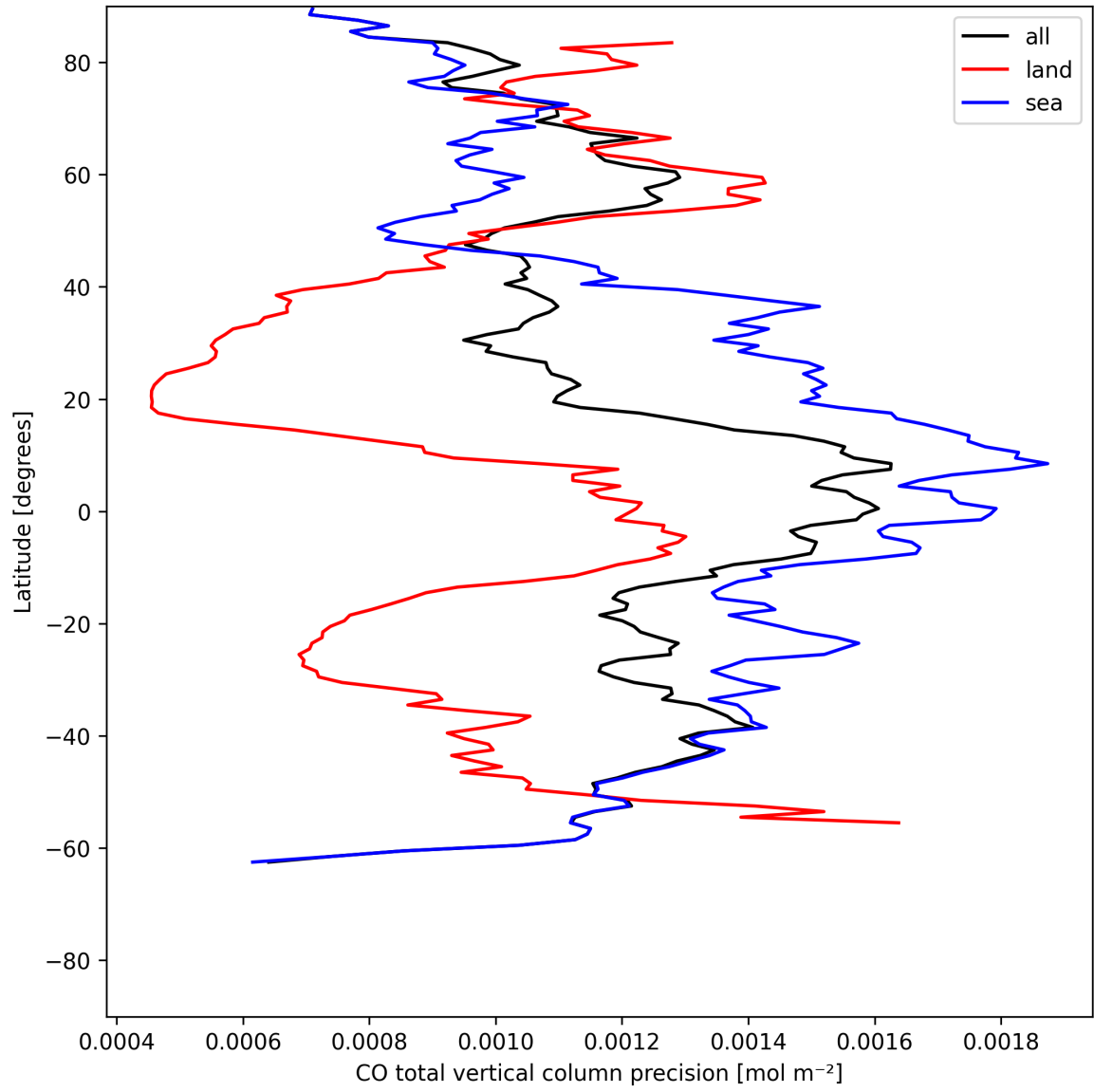
Figure 8: Zonal average of “CO total vertical column precision” for 2025-07-09 to 2025-07-10.
