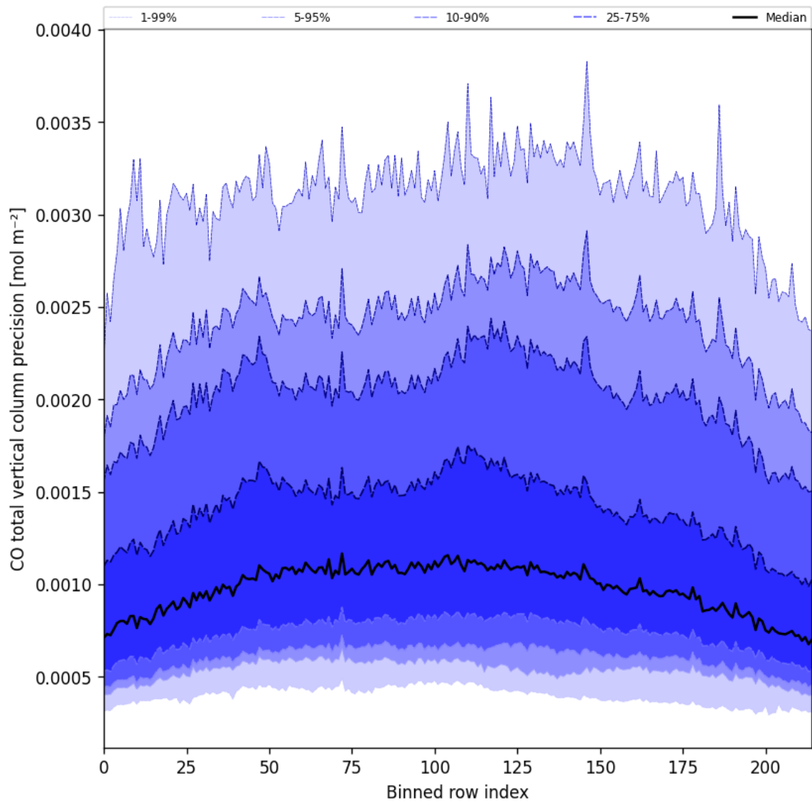
Figure 22: Along track statistics of “CO total vertical column precision” for 2025-07-09 to 2025-07-10
