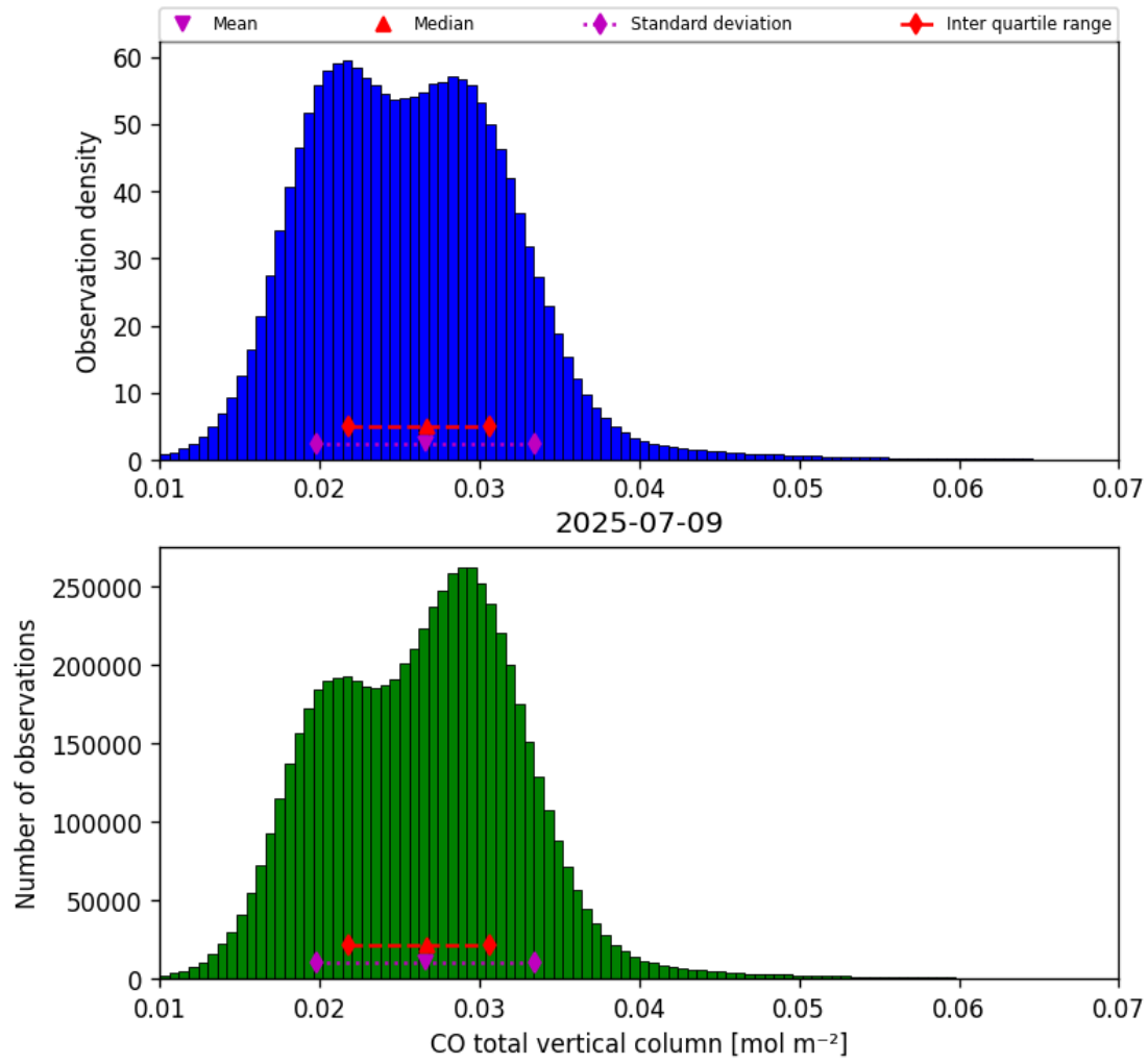
Figure 14: Histogram of “CO total vertical column” for 2025-07-09 to 2025-07-10
