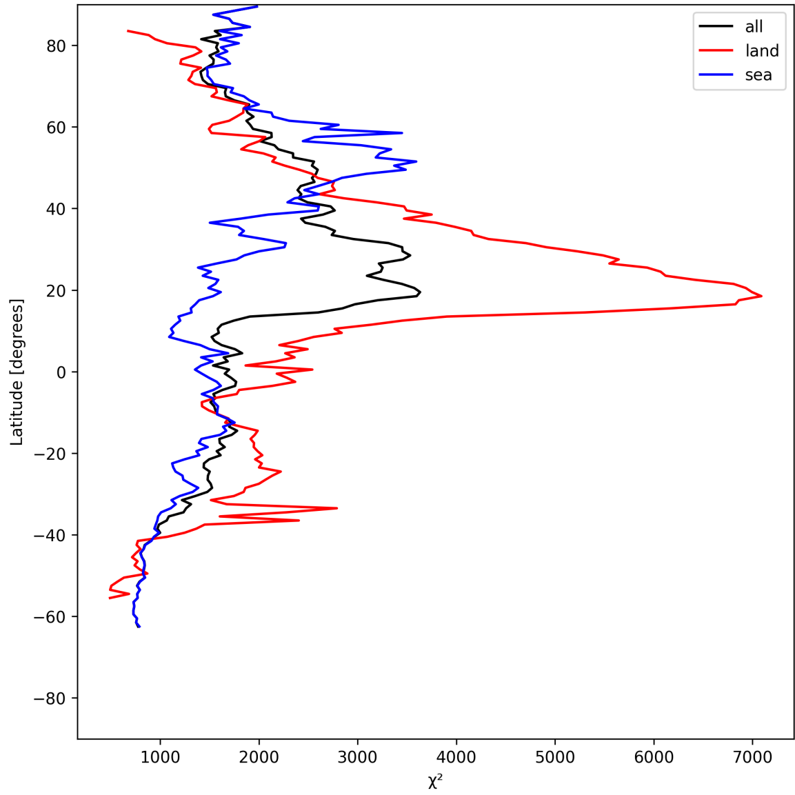
Figure 10: Zonal average of “ \chi^2 ” for 2025-07-09 to 2025-07-10.
