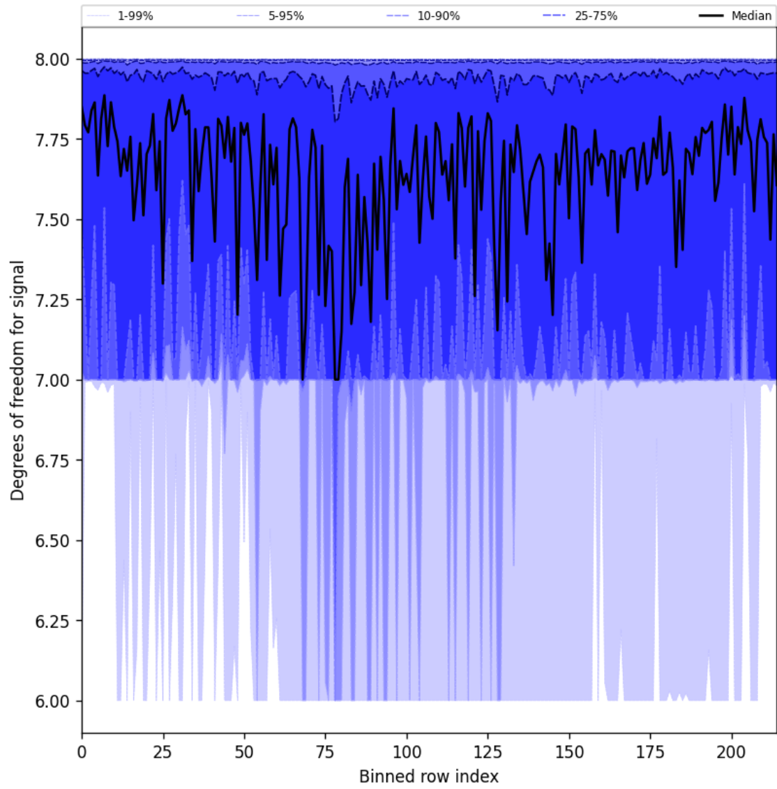
Figure 25: Along track statistics of “Degrees of freedom for signal” for 2025-07-09 to 2025-07-10
