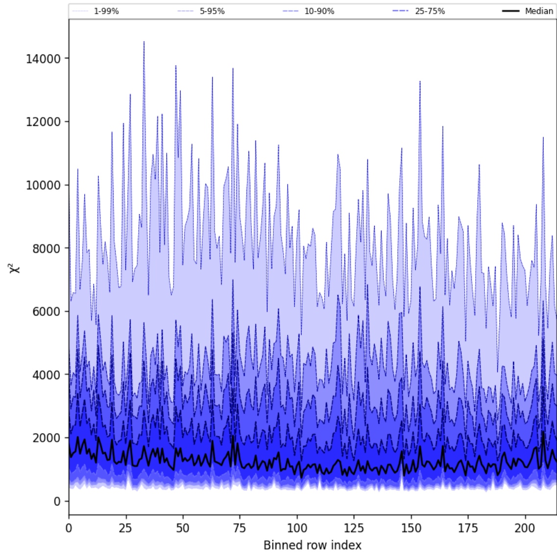
Figure 24: Along track statistics of “ \chi^2 ” for 2025-07-09 to 2025-07-10
