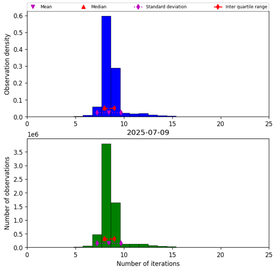
Figure 19: Histogram of “Number of iterations” for 2025-07-09 to 2025-07-10
