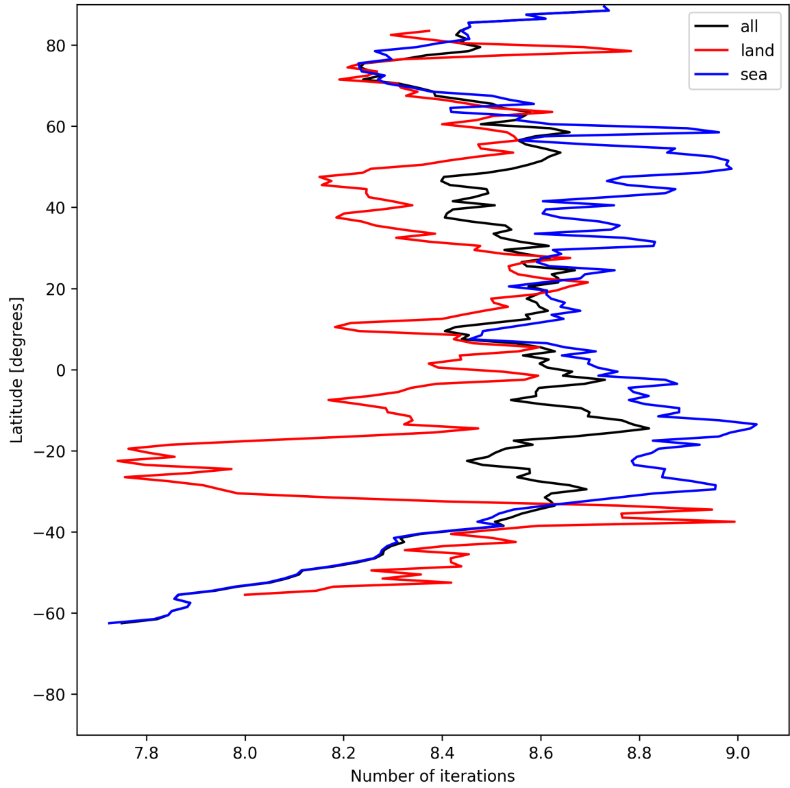
Figure 12: Zonal average of “Number of iterations” for 2025-07-09 to 2025-07-10.
