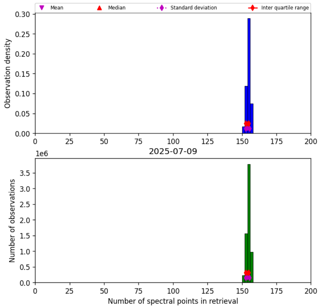
Figure 16: Histogram of “Number of spectral points in retrieval” for 2025-07-09 to 2025-07-10
