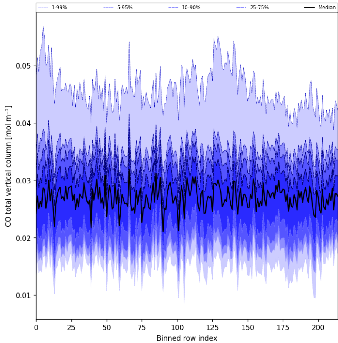
Figure 21: Along track statistics of “CO total vertical column” for 2025-07-09 to 2025-07-10
