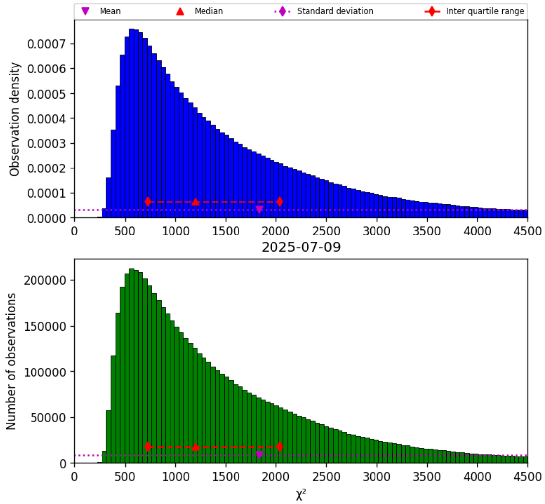
Figure 17: Histogram of “ \chi^2 ” for 2025-07-09 to 2025-07-10
