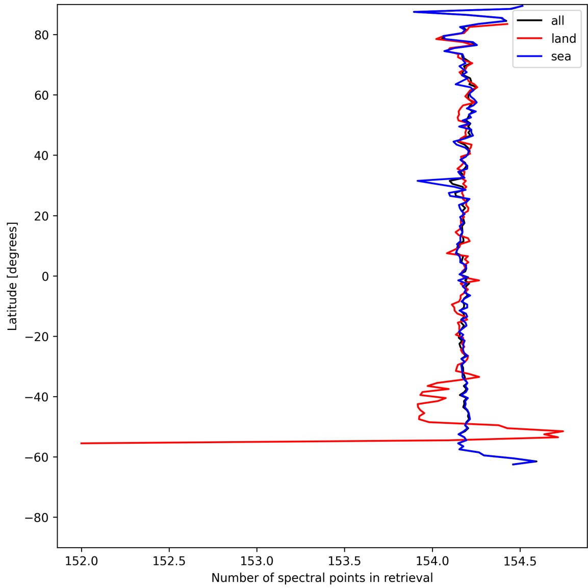
Figure 9: Zonal average of “Number of spectral points in retrieval” for 2025-07-09 to 2025-07-10.
