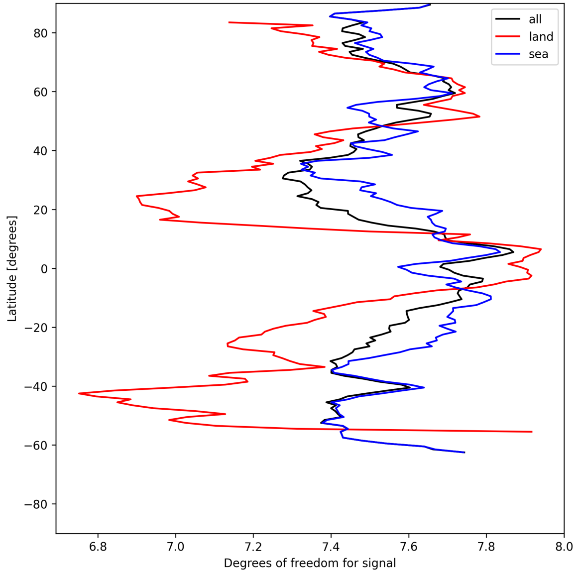
Figure 11: Zonal average of “Degrees of freedom for signal” for 2025-07-09 to 2025-07-10.
