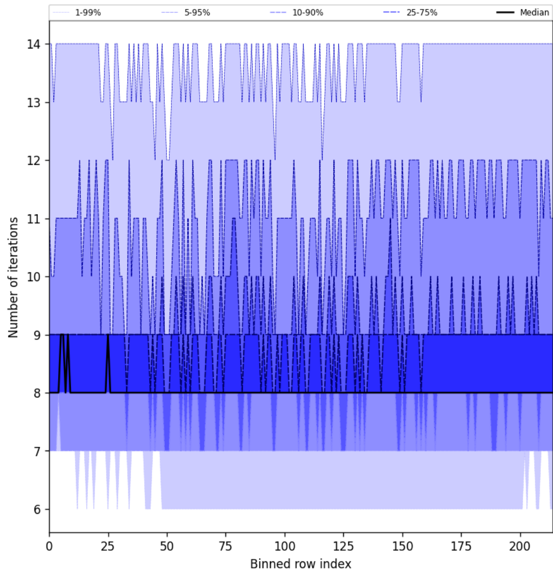
Figure 26: Along track statistics of “Number of iterations” for 2025-07-09 to 2025-07-10
