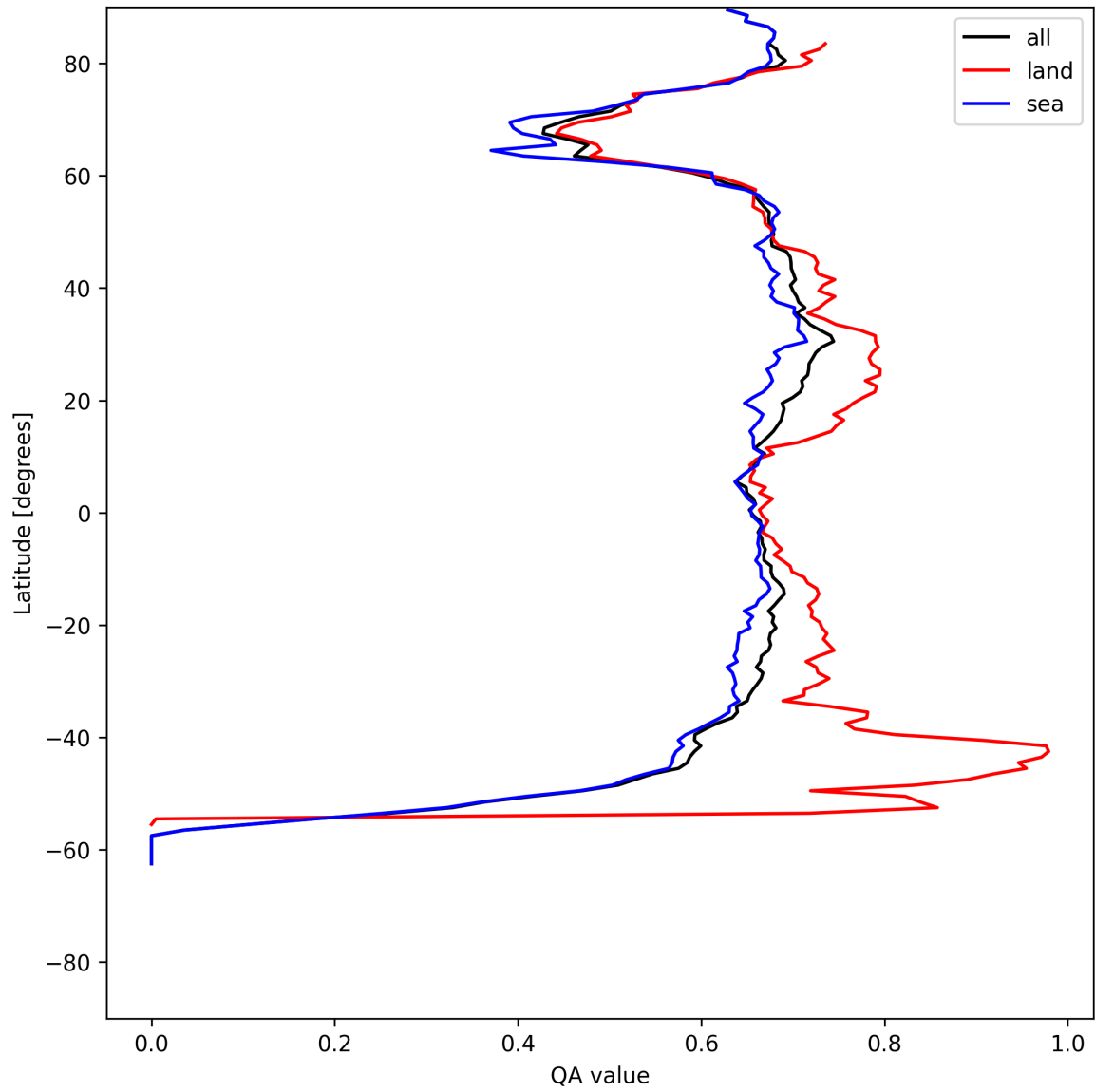
Figure 6: Zonal average of “QA value” for 2025-07-09 to 2025-07-10.
