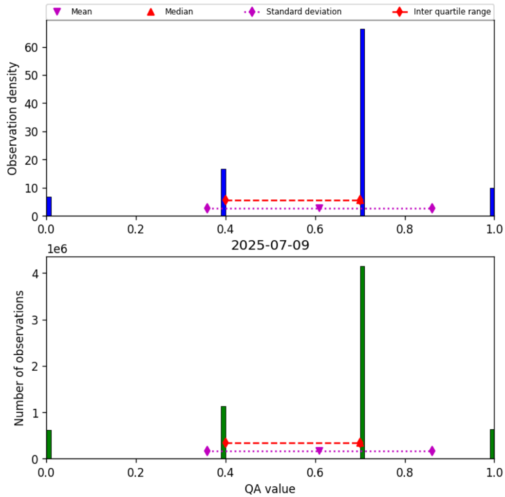
Figure 13: Histogram of “QA value” for 2025-07-09 to 2025-07-10
