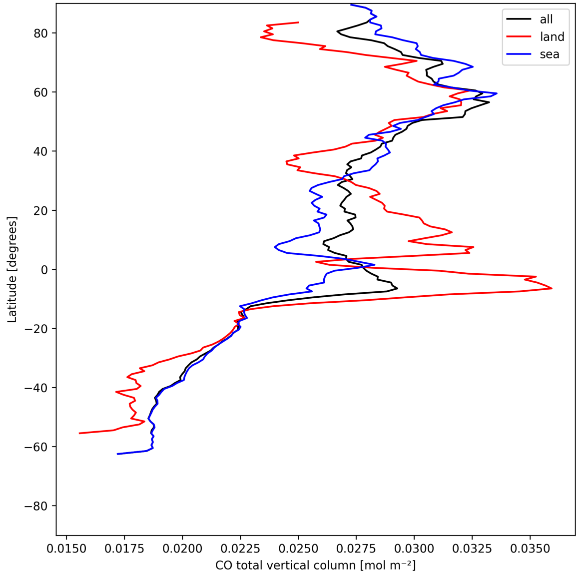
Figure 7: Zonal average of “CO total vertical column” for 2025-07-09 to 2025-07-10.
