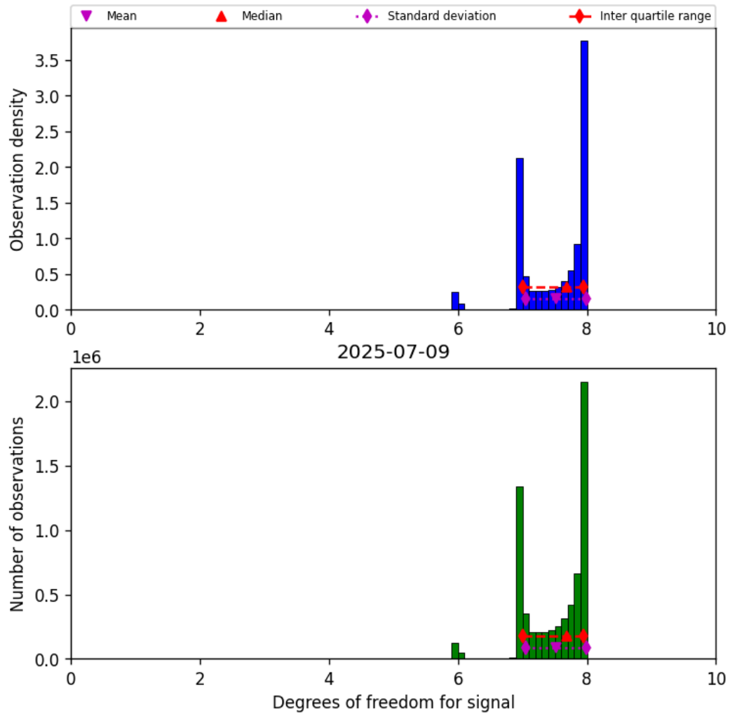
Figure 18: Histogram of “Degrees of freedom for signal” for 2025-07-09 to 2025-07-10
