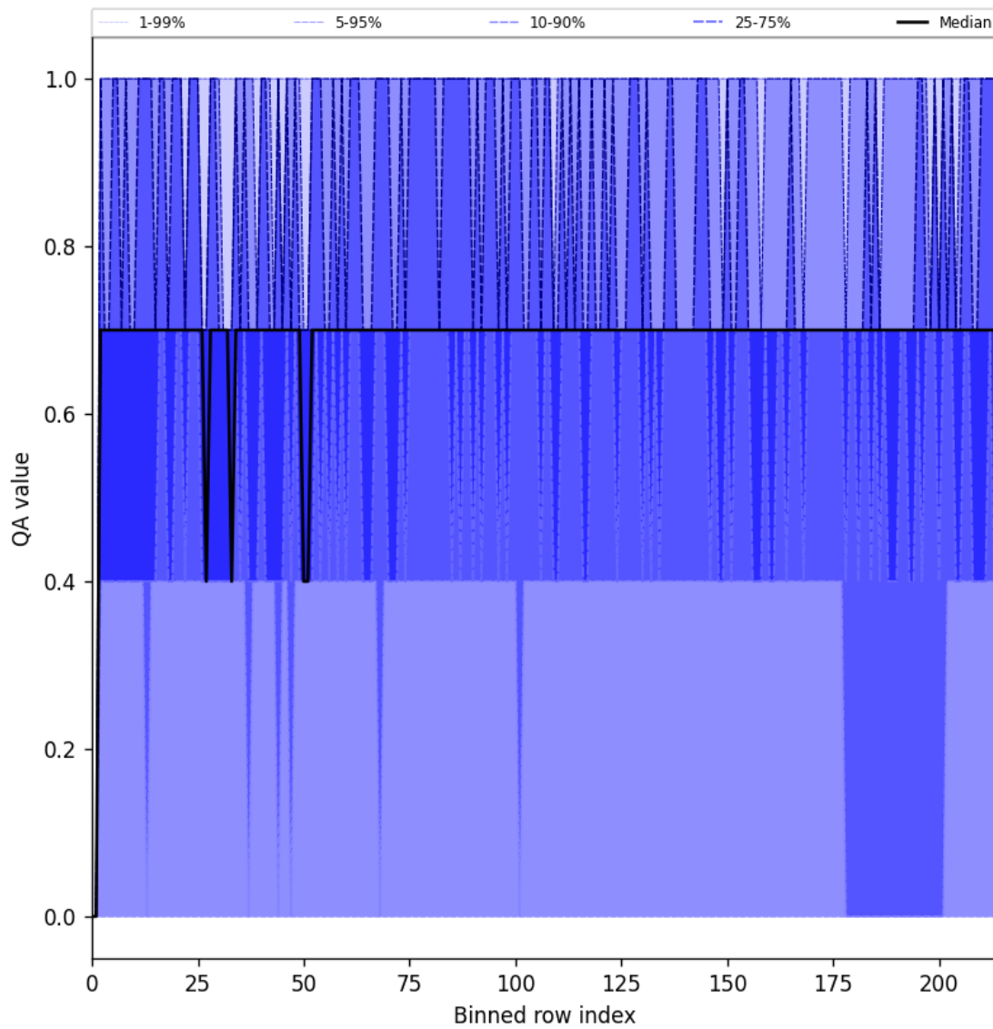
Figure 20: Along track statistics of “QA value” for 2025-07-09 to 2025-07-10
