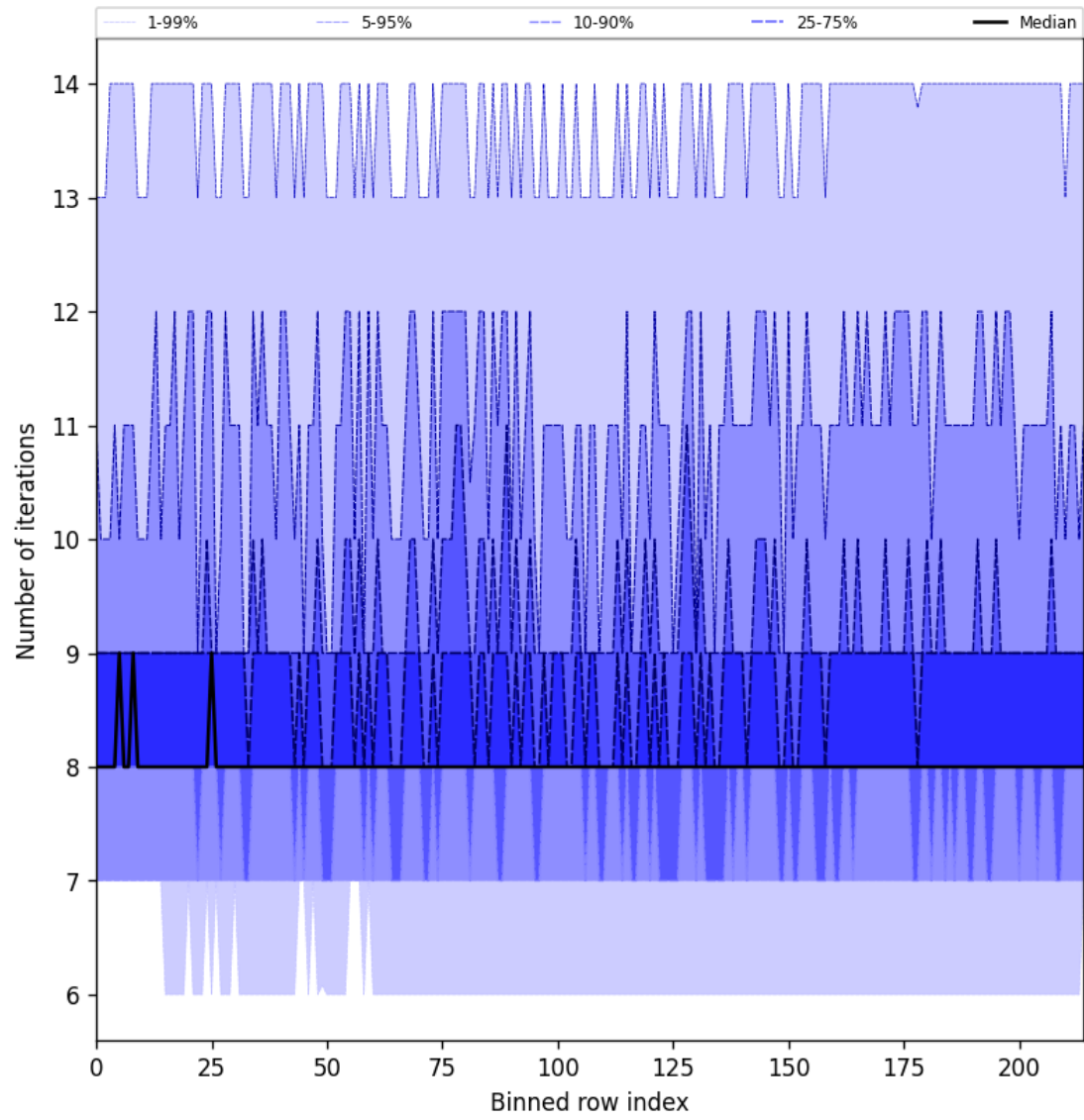
Figure 26: Along track statistics of “Number of iterations” for 2025-07-10 to 2025-07-11
