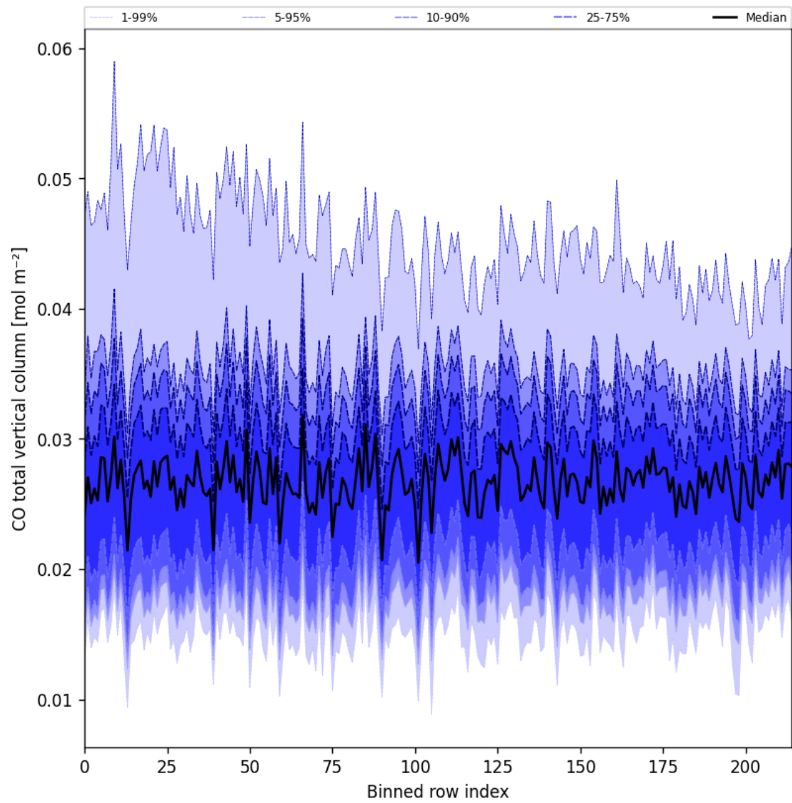
Figure 21: Along track statistics of “CO total vertical column” for 2025-07-10 to 2025-07-11
