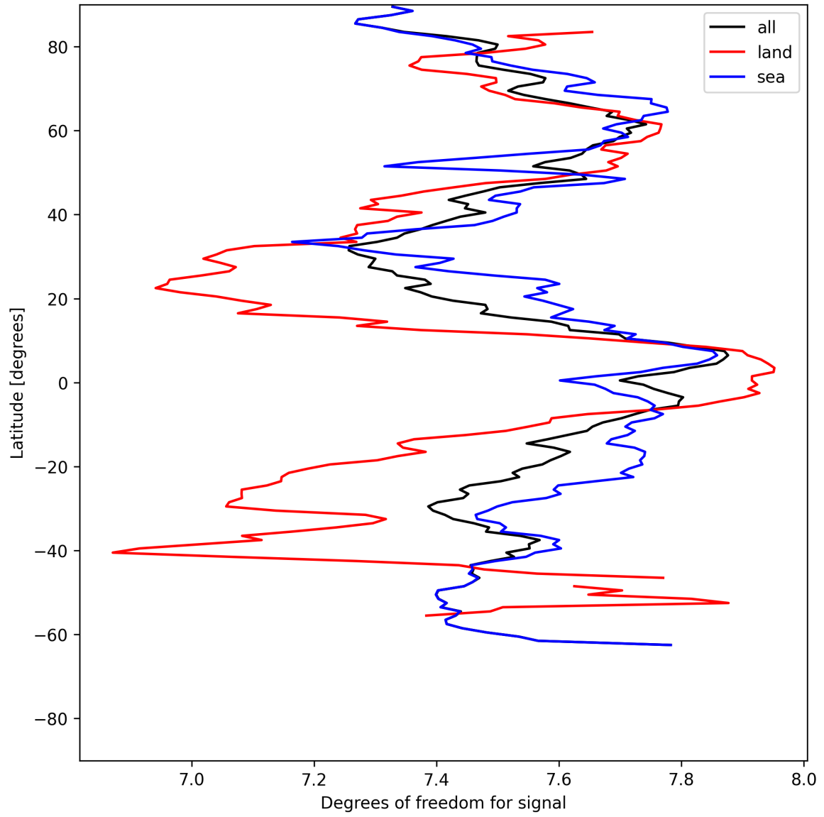
Figure 11: Zonal average of “Degrees of freedom for signal” for 2025-07-10 to 2025-07-11.
