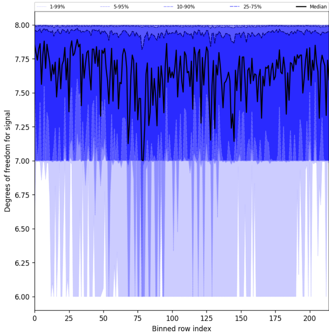
Figure 25: Along track statistics of “Degrees of freedom for signal” for 2025-07-10 to 2025-07-11
