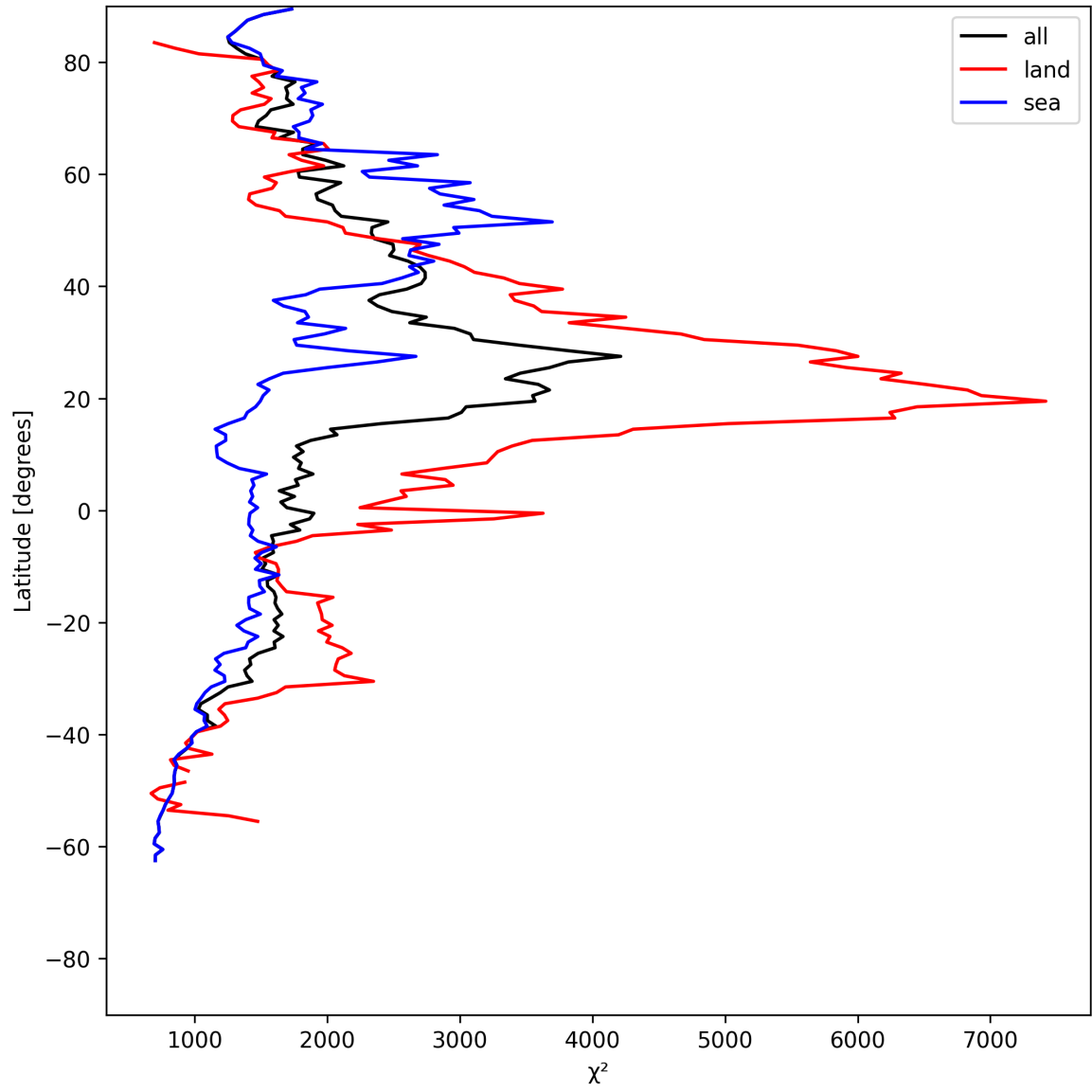
Figure 10: Zonal average of “ \chi^2 ” for 2025-07-10 to 2025-07-11.
