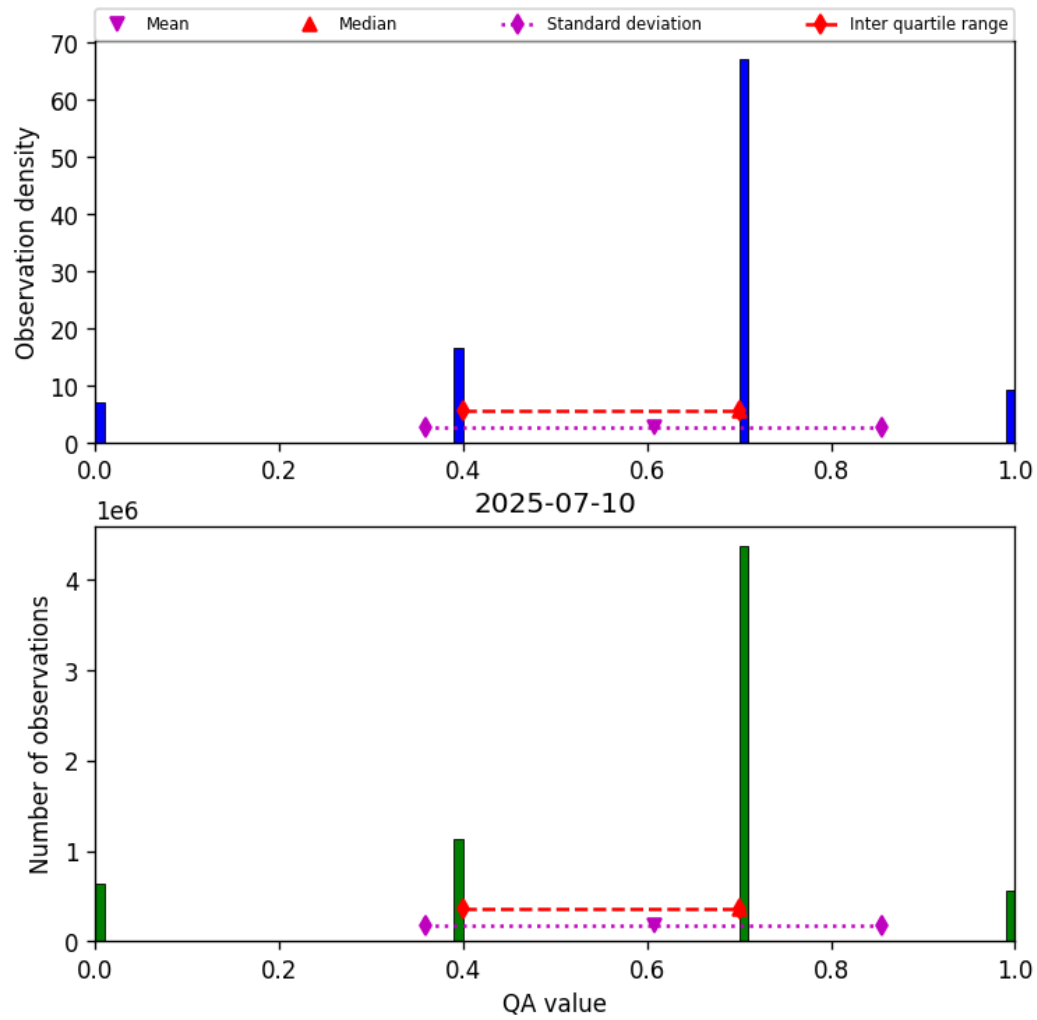
Figure 13: Histogram of “QA value” for 2025-07-10 to 2025-07-11
