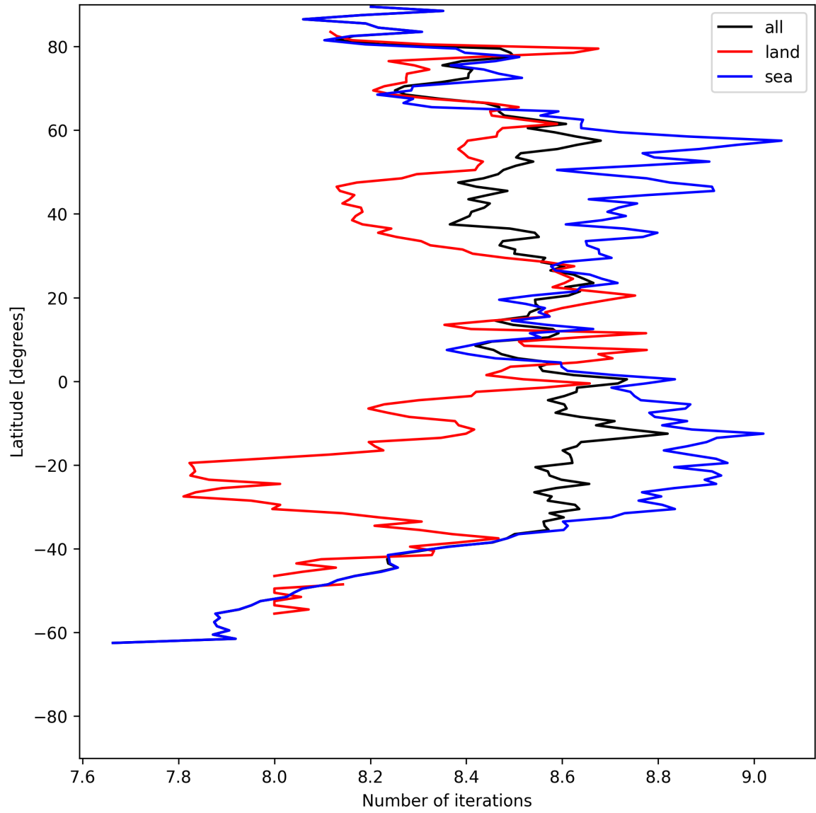
Figure 12: Zonal average of “Number of iterations” for 2025-07-10 to 2025-07-11.
