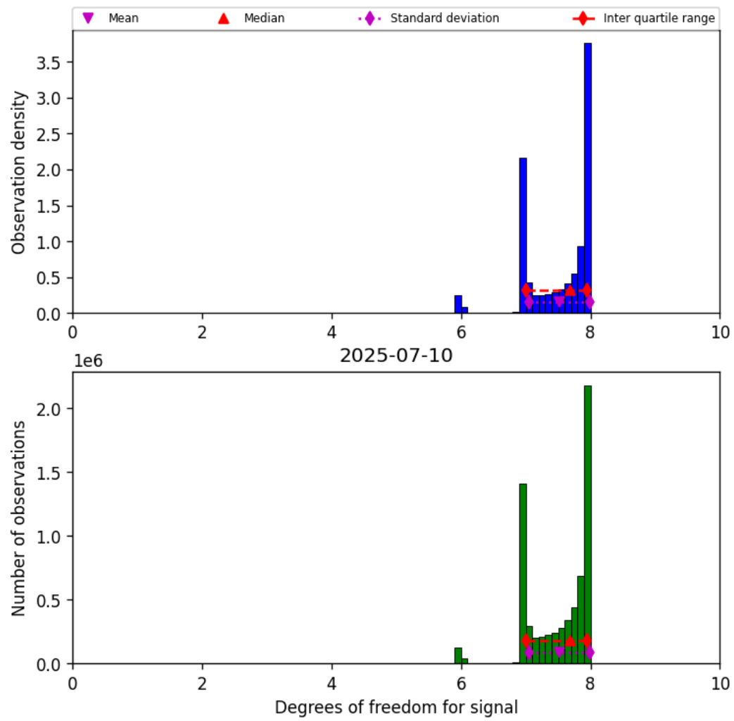
Figure 18: Histogram of “Degrees of freedom for signal” for 2025-07-10 to 2025-07-11
