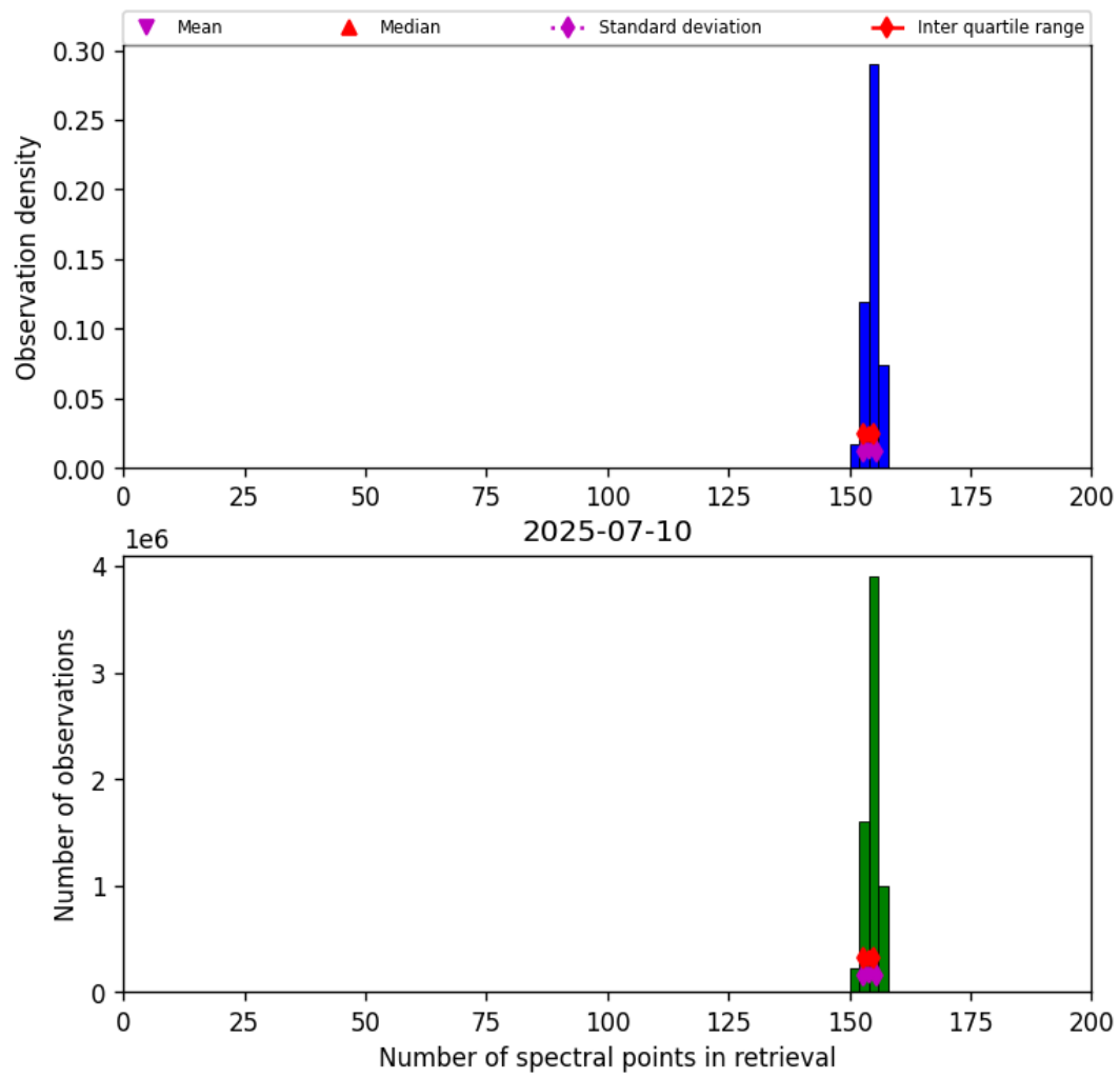
Figure 16: Histogram of “Number of spectral points in retrieval” for 2025-07-10 to 2025-07-11
