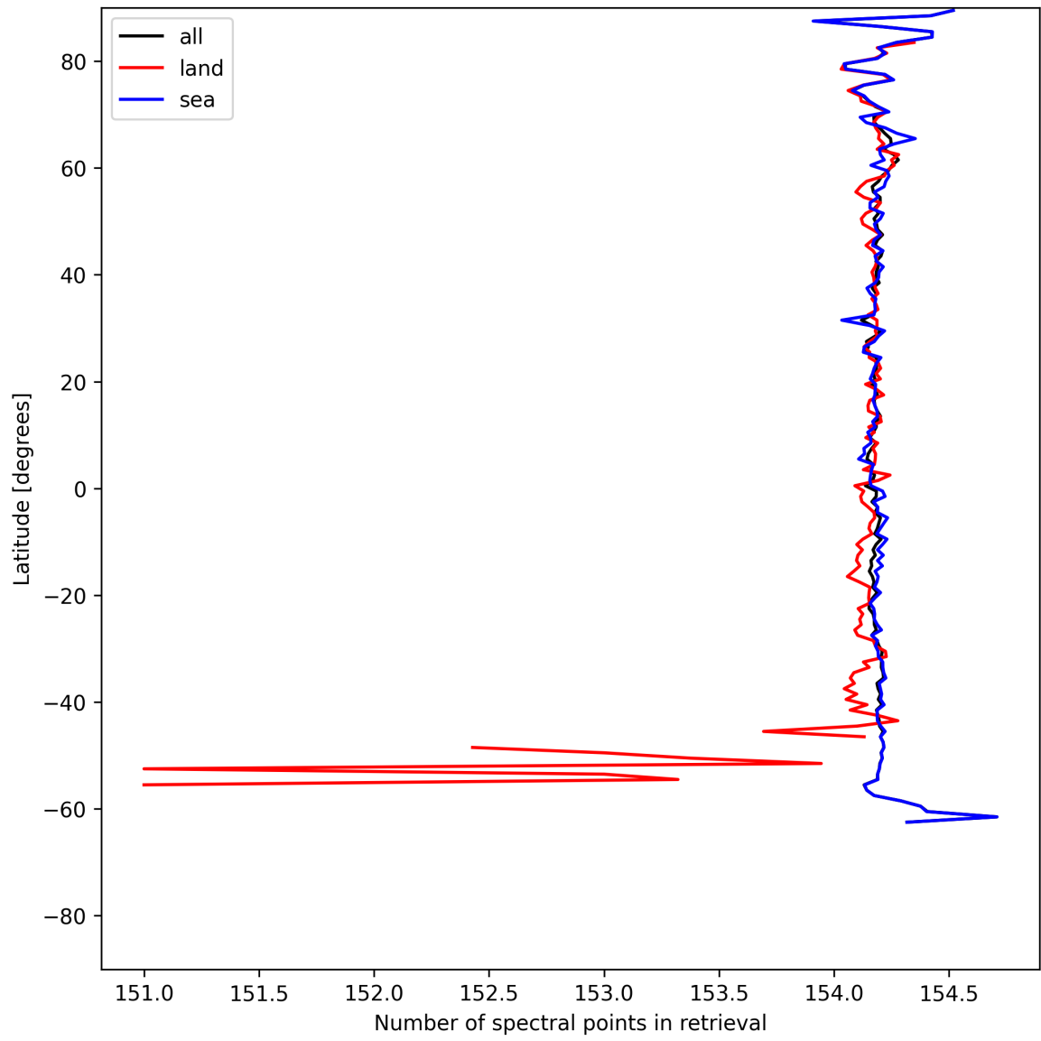
Figure 9: Zonal average of “Number of spectral points in retrieval” for 2025-07-10 to 2025-07-11.
