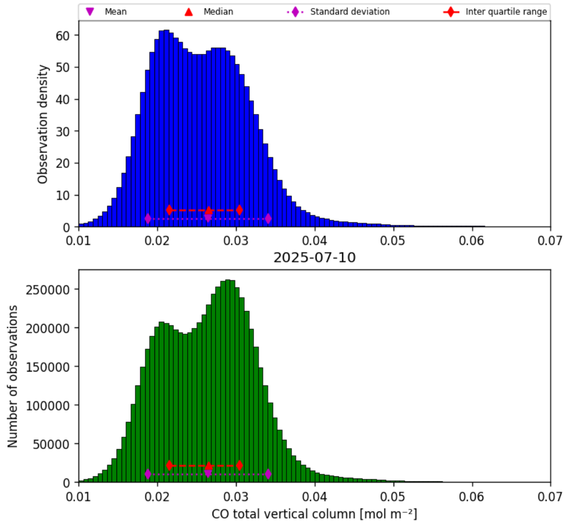
Figure 14: Histogram of “CO total vertical column” for 2025-07-10 to 2025-07-11
