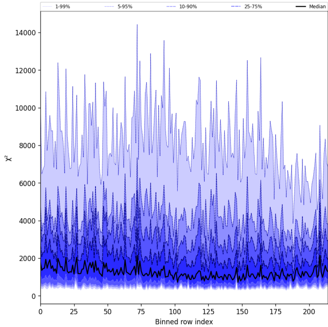
Figure 24: Along track statistics of “ \chi^2 ” for 2025-07-10 to 2025-07-11
