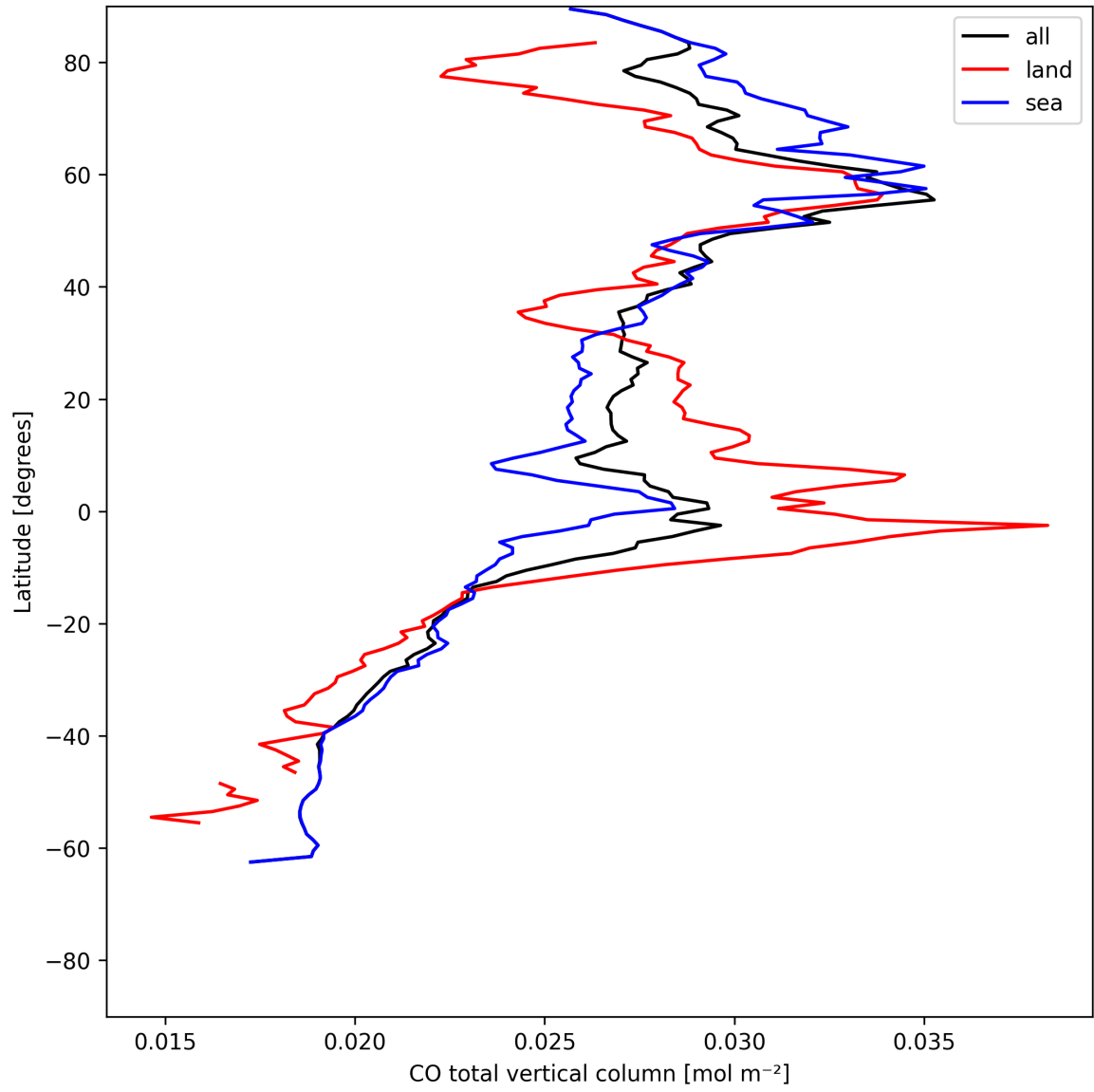
Figure 7: Zonal average of “CO total vertical column” for 2025-07-10 to 2025-07-11.
