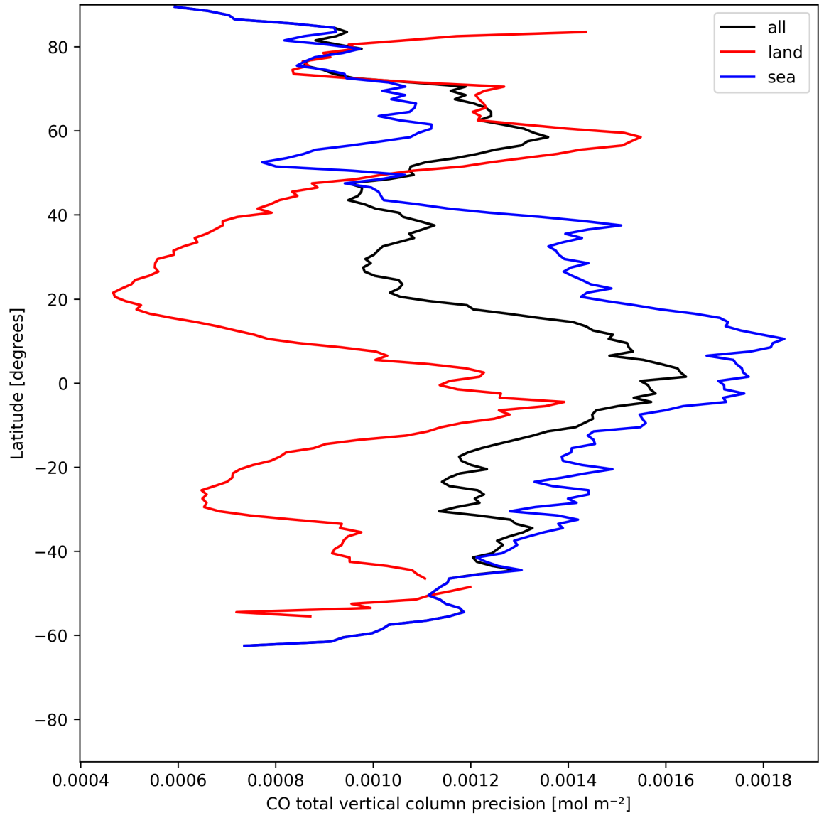
Figure 8: Zonal average of “CO total vertical column precision” for 2025-07-10 to 2025-07-11.
