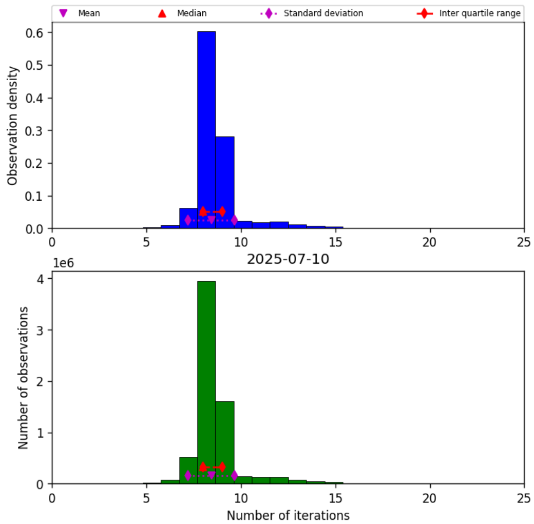
Figure 19: Histogram of “Number of iterations” for 2025-07-10 to 2025-07-11
