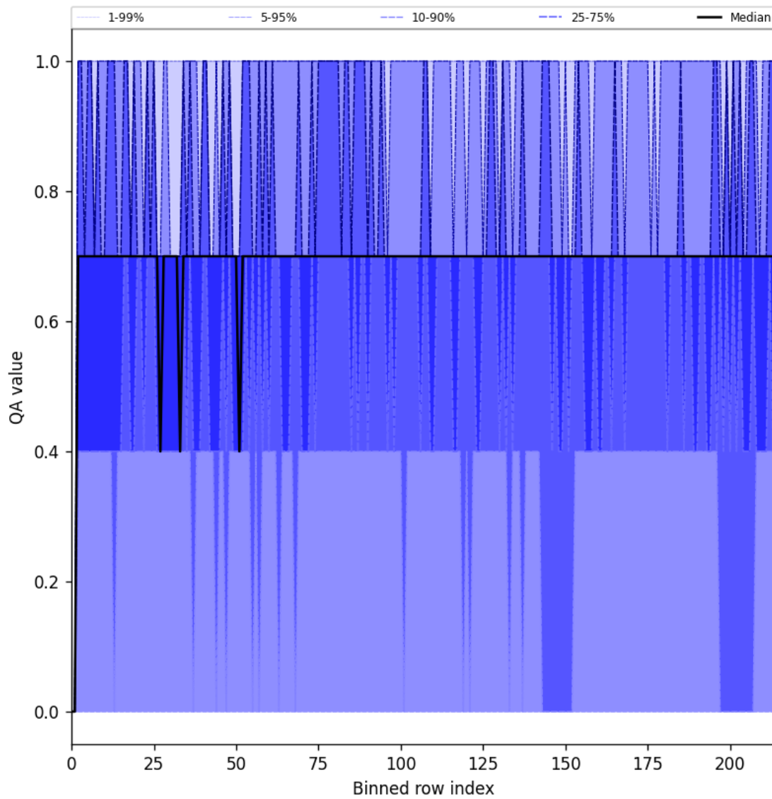
Figure 20: Along track statistics of “QA value” for 2025-07-10 to 2025-07-11
