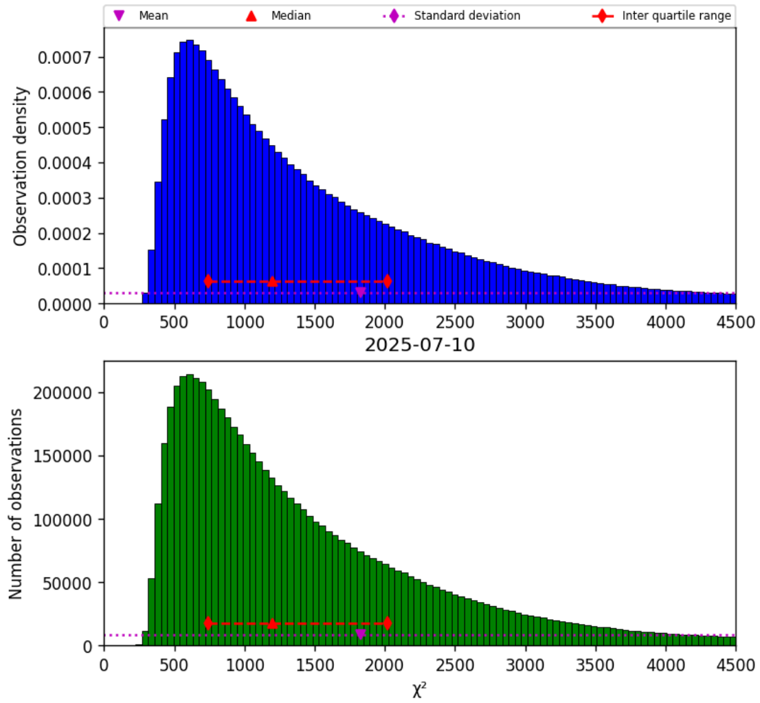
Figure 17: Histogram of “ \chi^2 ” for 2025-07-10 to 2025-07-11
