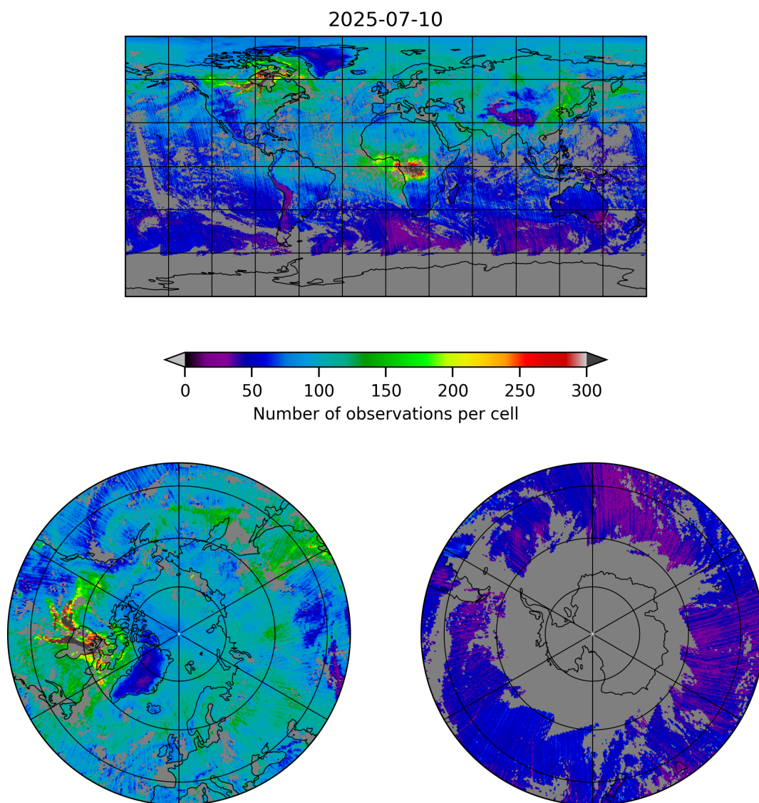
Figure 5: Map of the number of observations for 2025-07-10 to 2025-07-11
