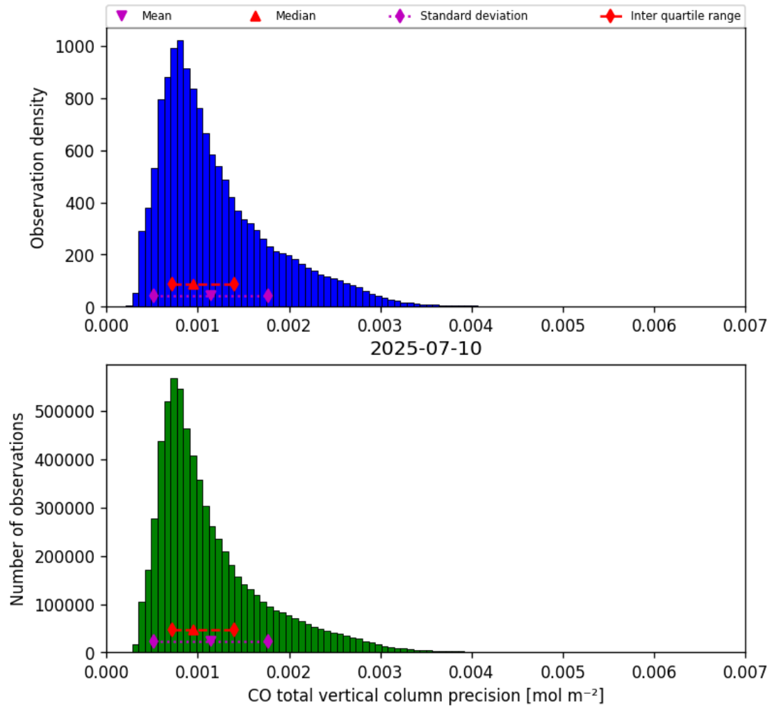
Figure 15: Histogram of “CO total vertical column precision” for 2025-07-10 to 2025-07-11
