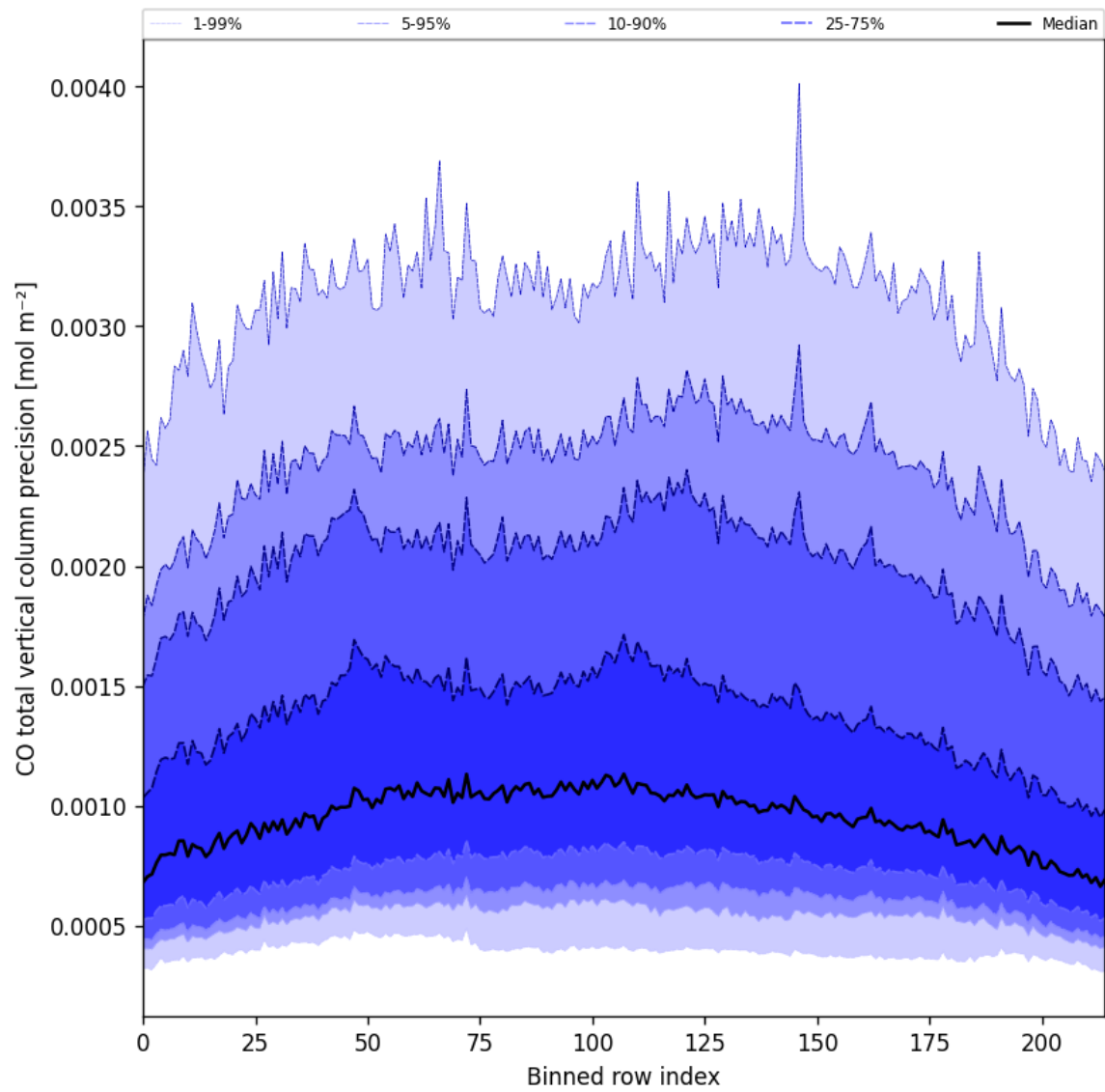
Figure 22: Along track statistics of “CO total vertical column precision” for 2025-07-10 to 2025-07-11
