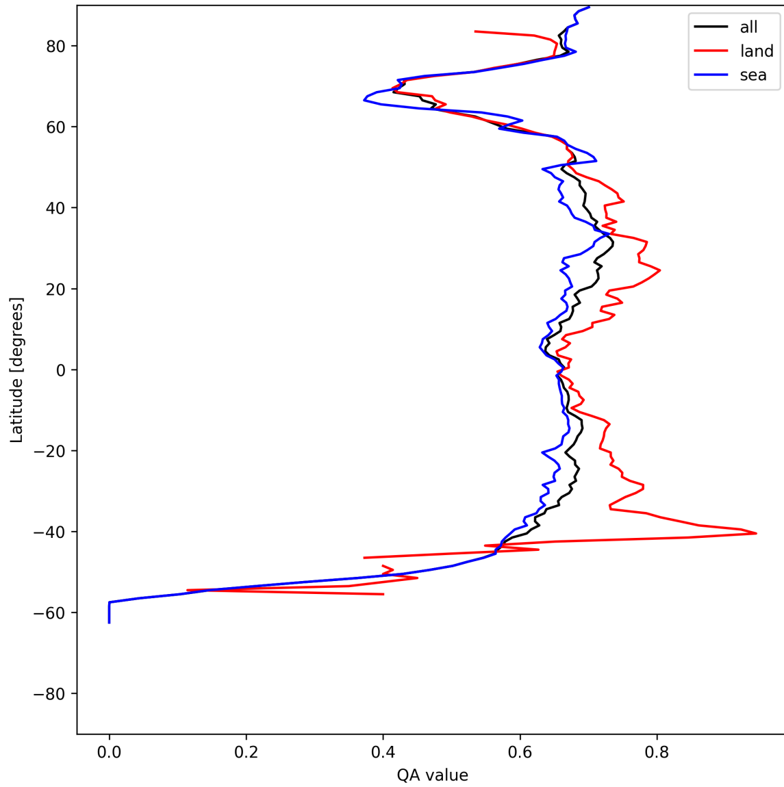
Figure 6: Zonal average of “QA value” for 2025-07-10 to 2025-07-11.
