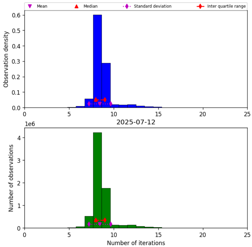
Figure 19: Histogram of “Number of iterations” for 2025-07-12 to 2025-07-13
