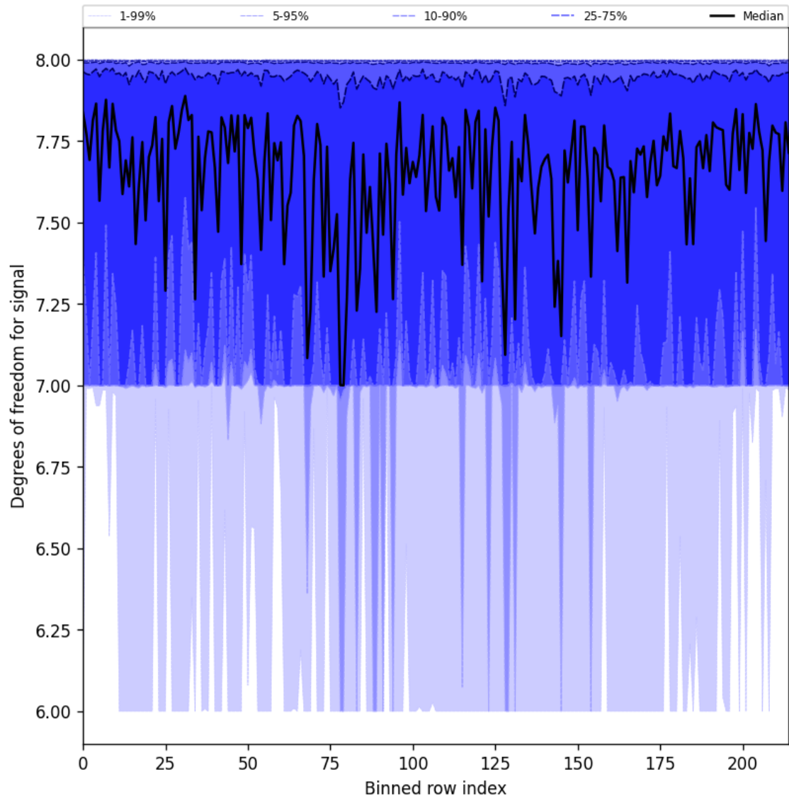
Figure 25: Along track statistics of “Degrees of freedom for signal” for 2025-07-12 to 2025-07-13
