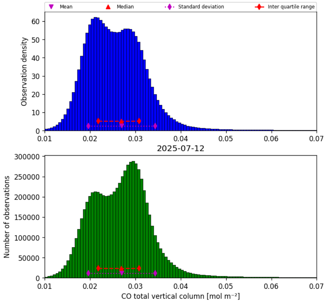
Figure 14: Histogram of “CO total vertical column” for 2025-07-12 to 2025-07-13
