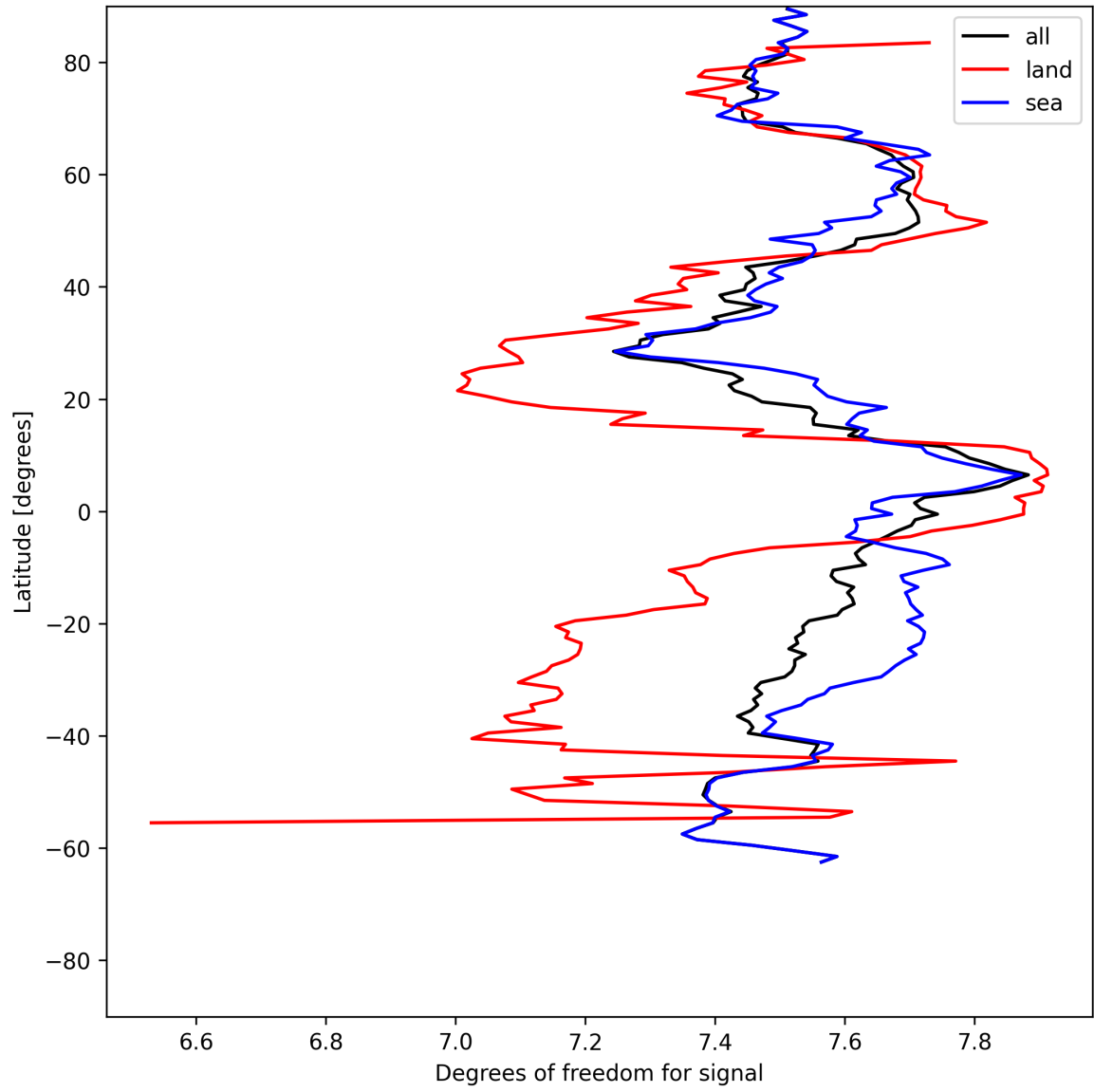
Figure 11: Zonal average of “Degrees of freedom for signal” for 2025-07-12 to 2025-07-13.
