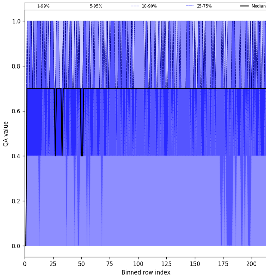
Figure 20: Along track statistics of “QA value” for 2025-07-12 to 2025-07-13
