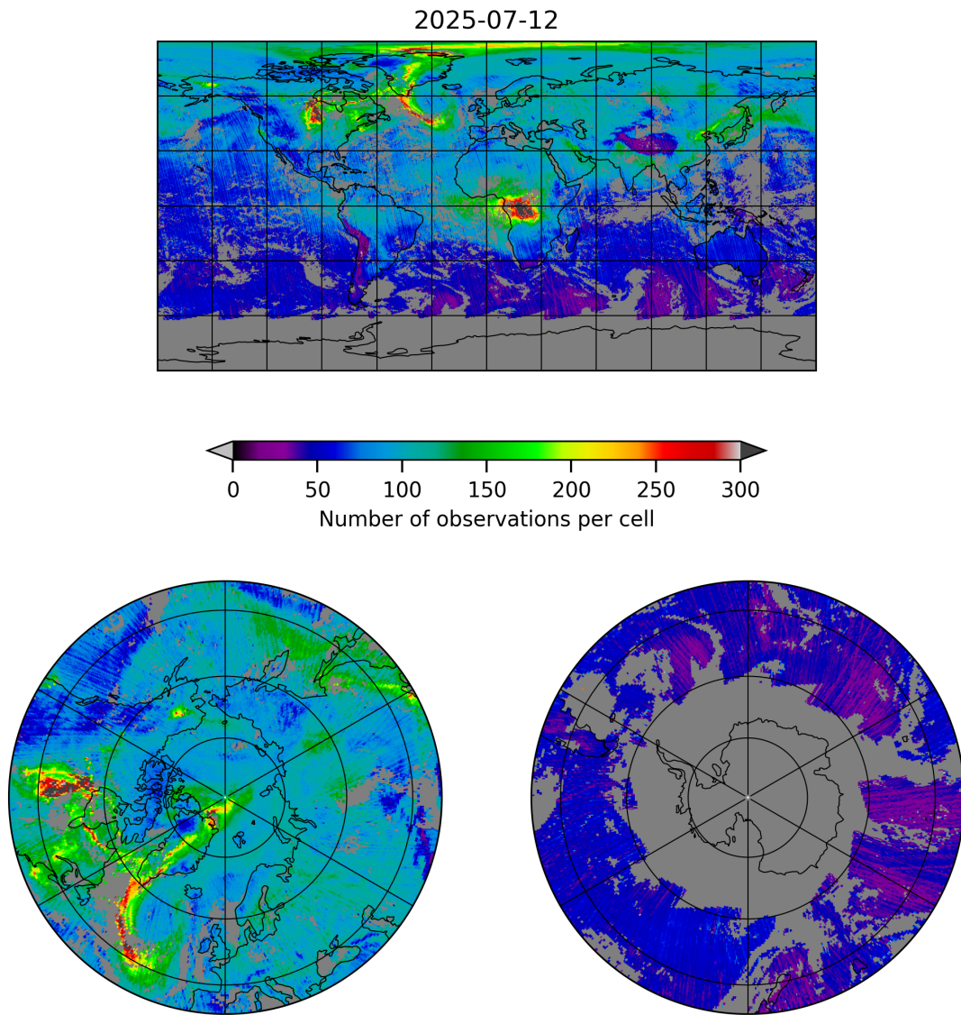
Figure 5: Map of the number of observations for 2025-07-12 to 2025-07-13
