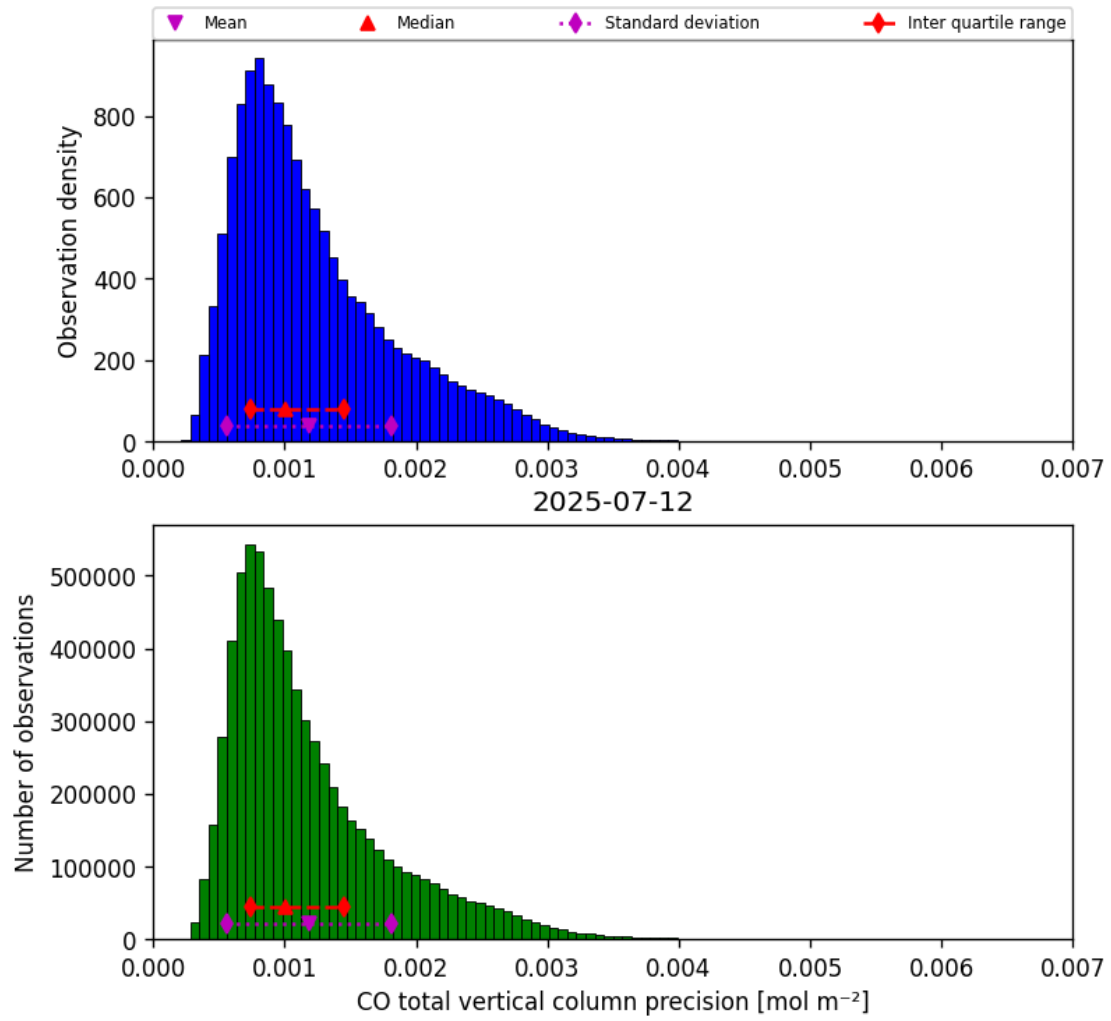
Figure 15: Histogram of “CO total vertical column precision” for 2025-07-12 to 2025-07-13
