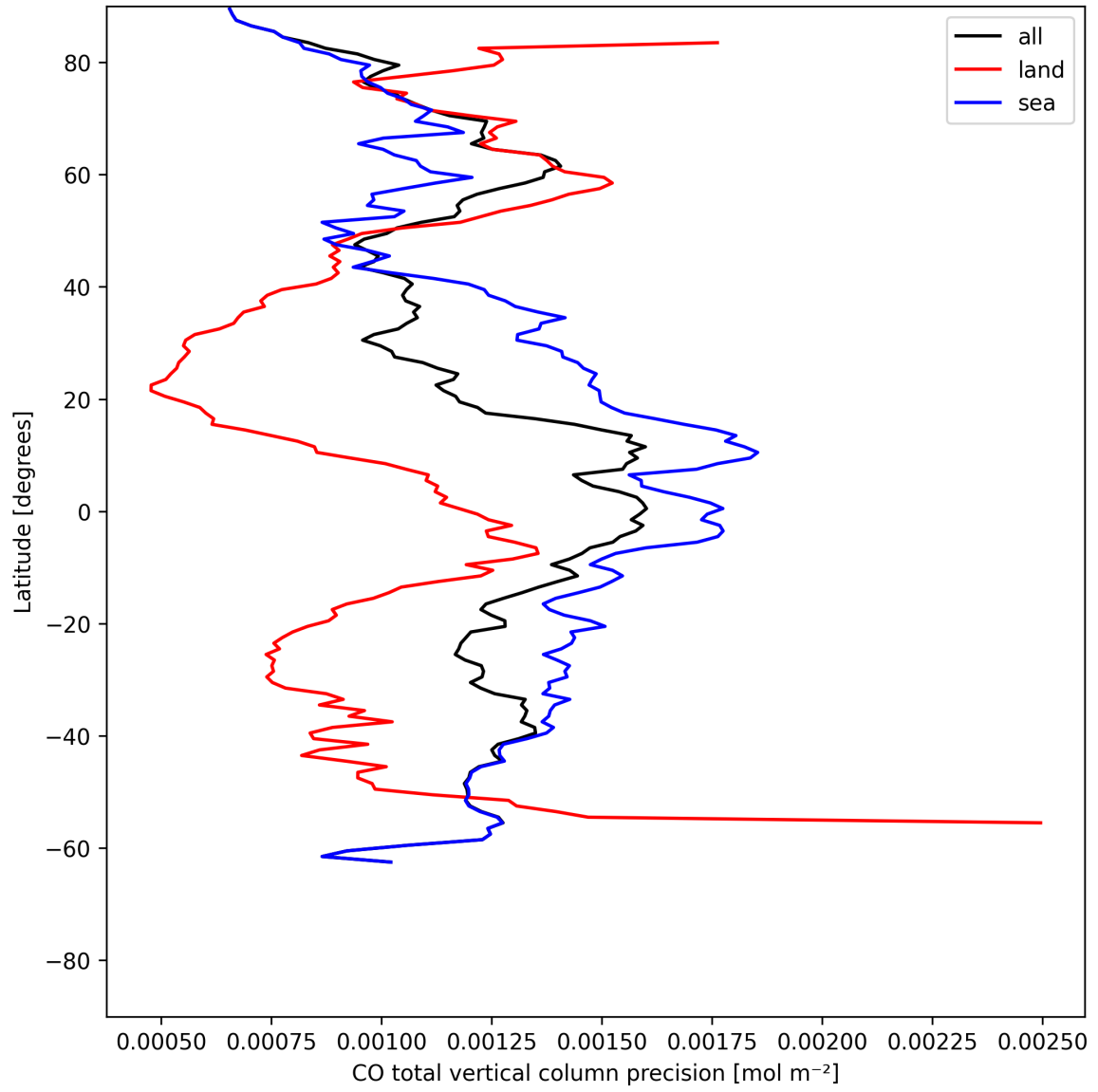
Figure 8: Zonal average of “CO total vertical column precision” for 2025-07-12 to 2025-07-13.
