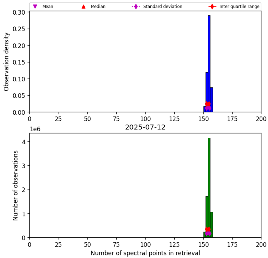
Figure 16: Histogram of “Number of spectral points in retrieval” for 2025-07-12 to 2025-07-13
