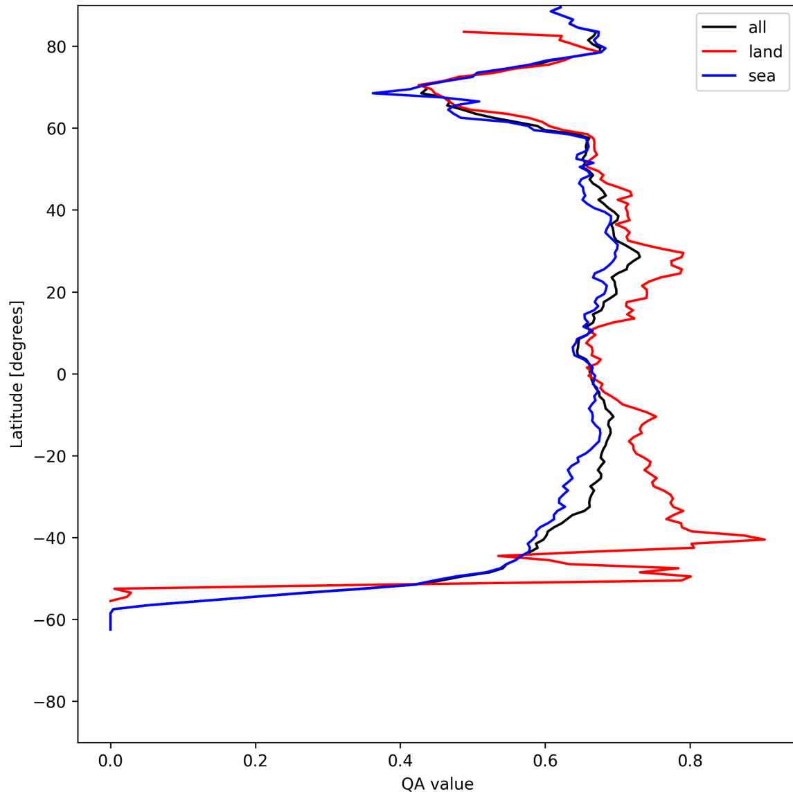
Figure 6: Zonal average of “QA value” for 2025-07-12 to 2025-07-13.
