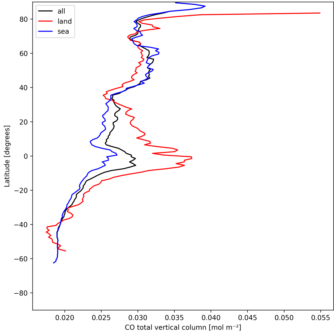
Figure 7: Zonal average of “CO total vertical column” for 2025-07-12 to 2025-07-13.
