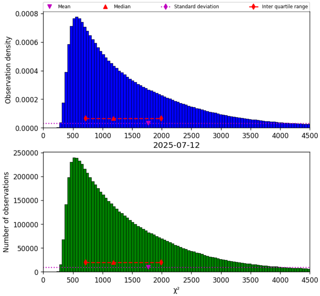
Figure 17: Histogram of “ \chi^2 ” for 2025-07-12 to 2025-07-13
