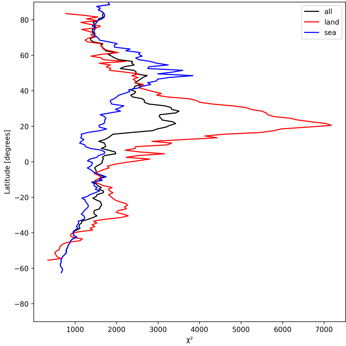
Figure 10: Zonal average of “ \chi^2 ” for 2025-07-12 to 2025-07-13.
