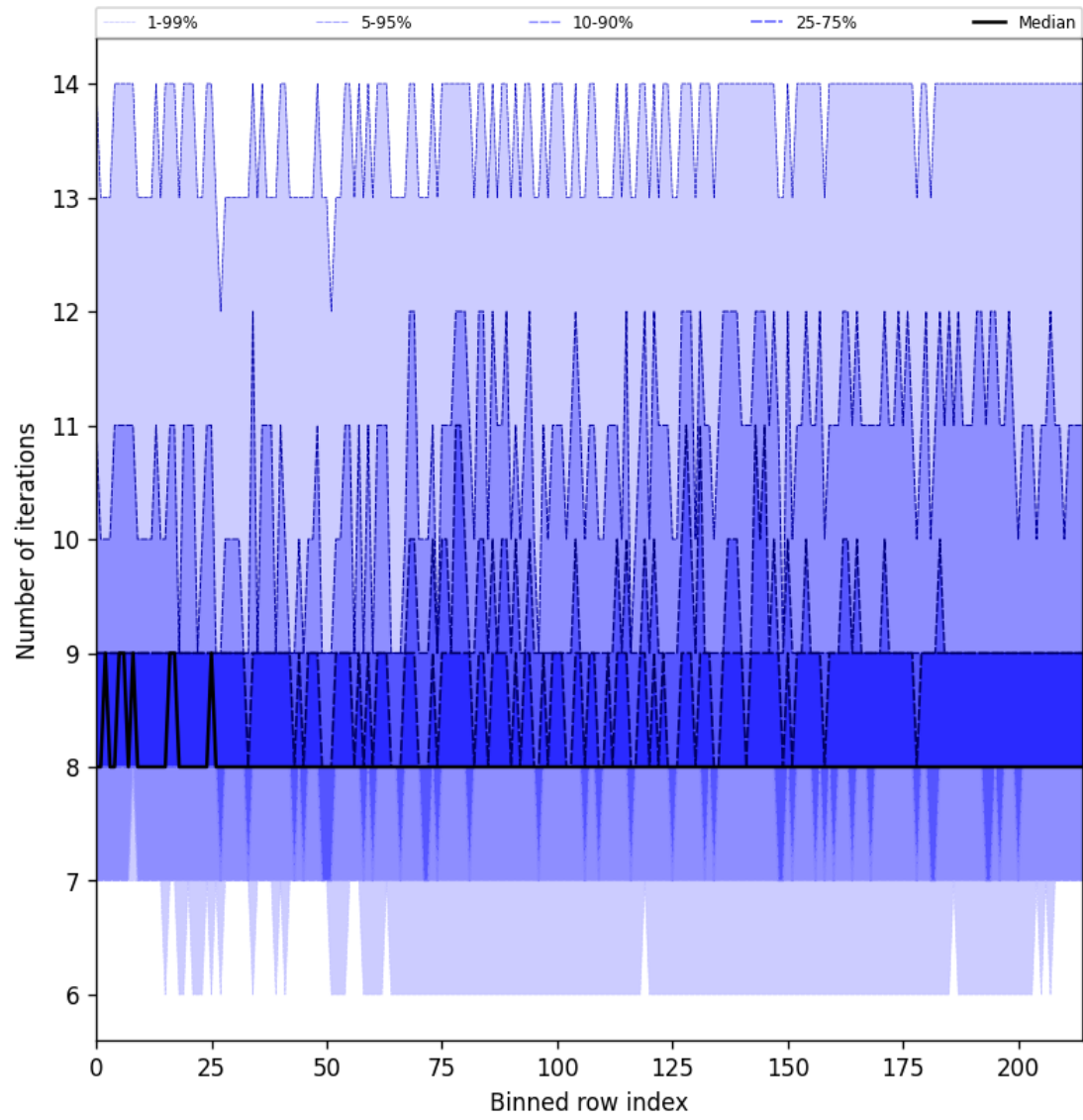
Figure 26: Along track statistics of “Number of iterations” for 2025-07-12 to 2025-07-13
