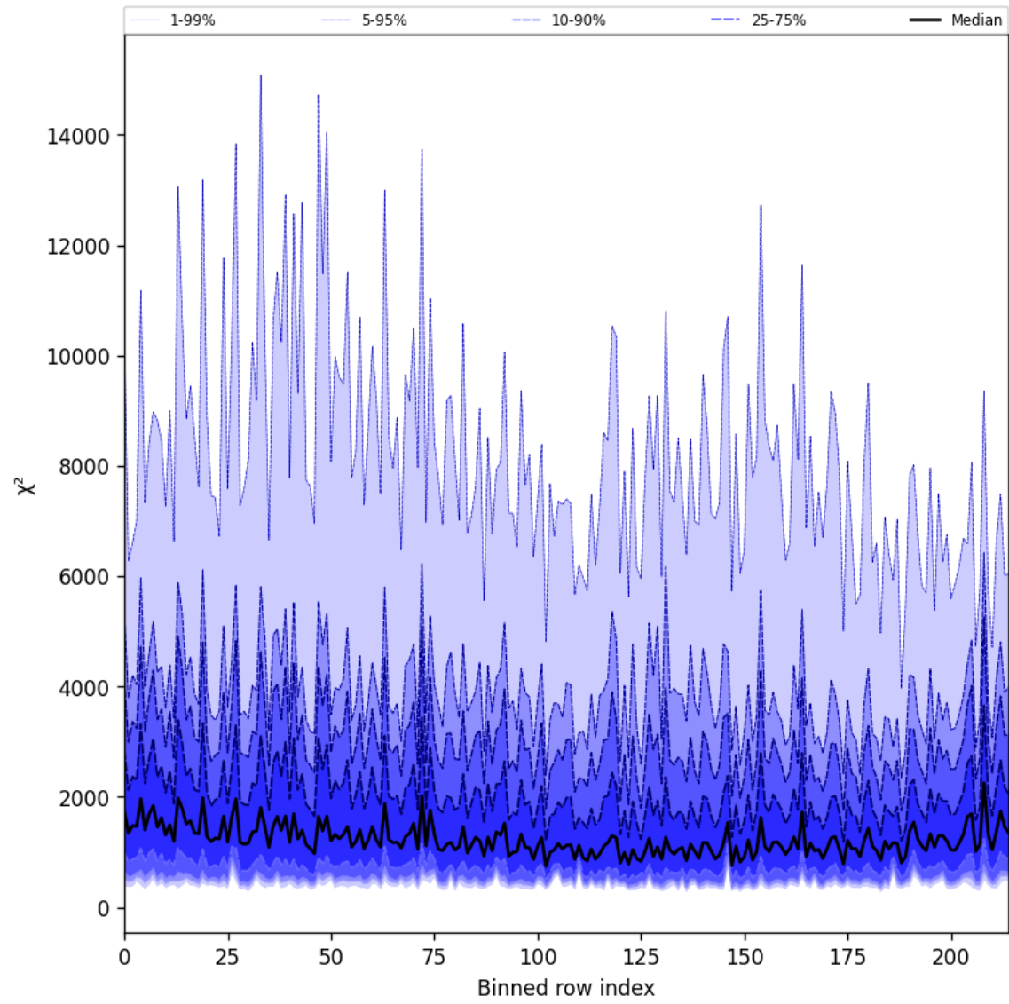
Figure 24: Along track statistics of “ \chi^2 ” for 2025-07-12 to 2025-07-13
