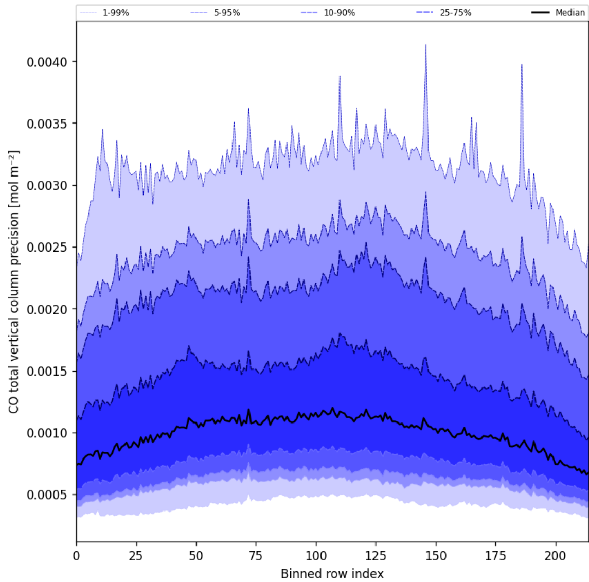
Figure 22: Along track statistics of “CO total vertical column precision” for 2025-07-12 to 2025-07-13
