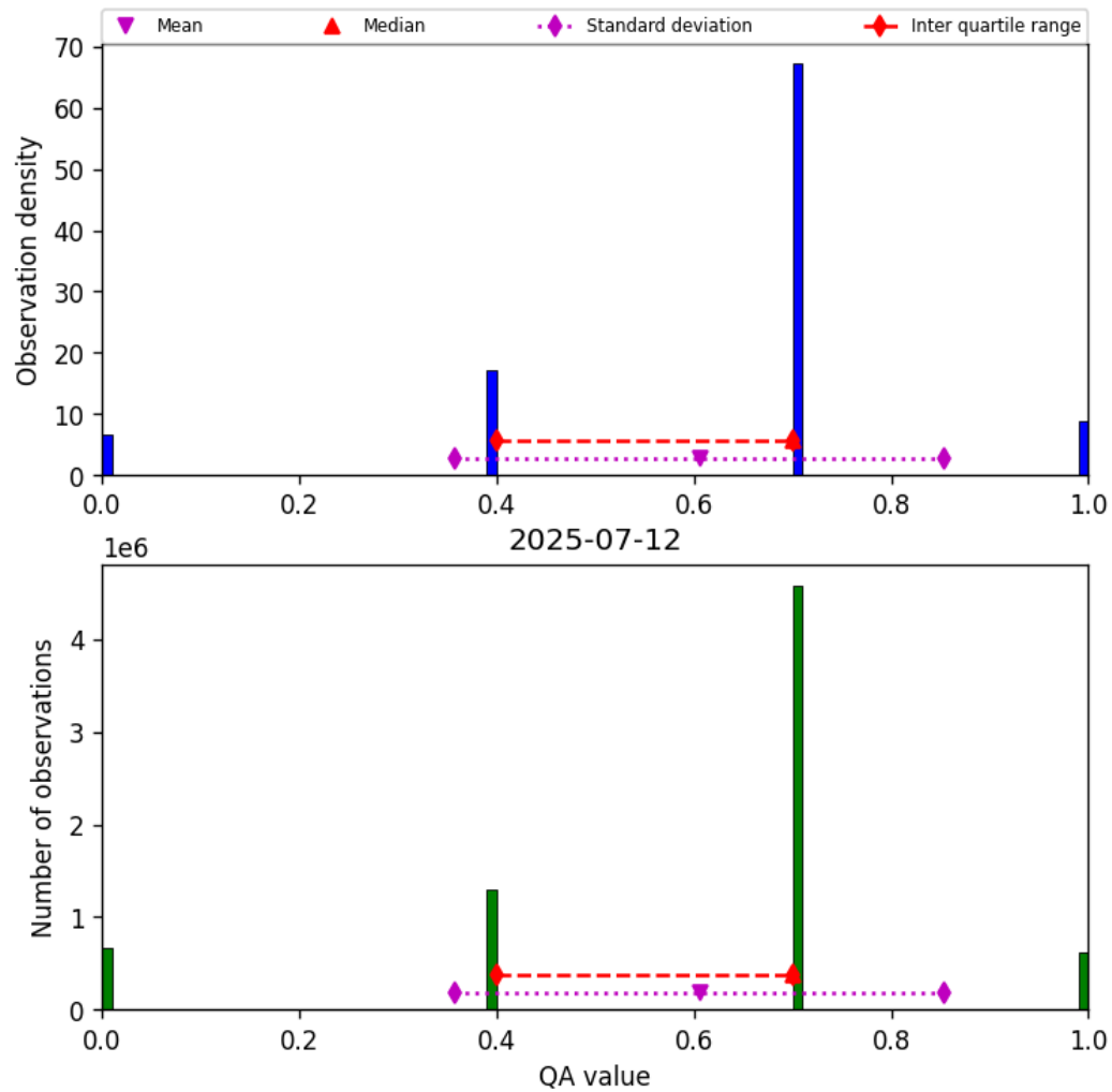
Figure 13: Histogram of “QA value” for 2025-07-12 to 2025-07-13
