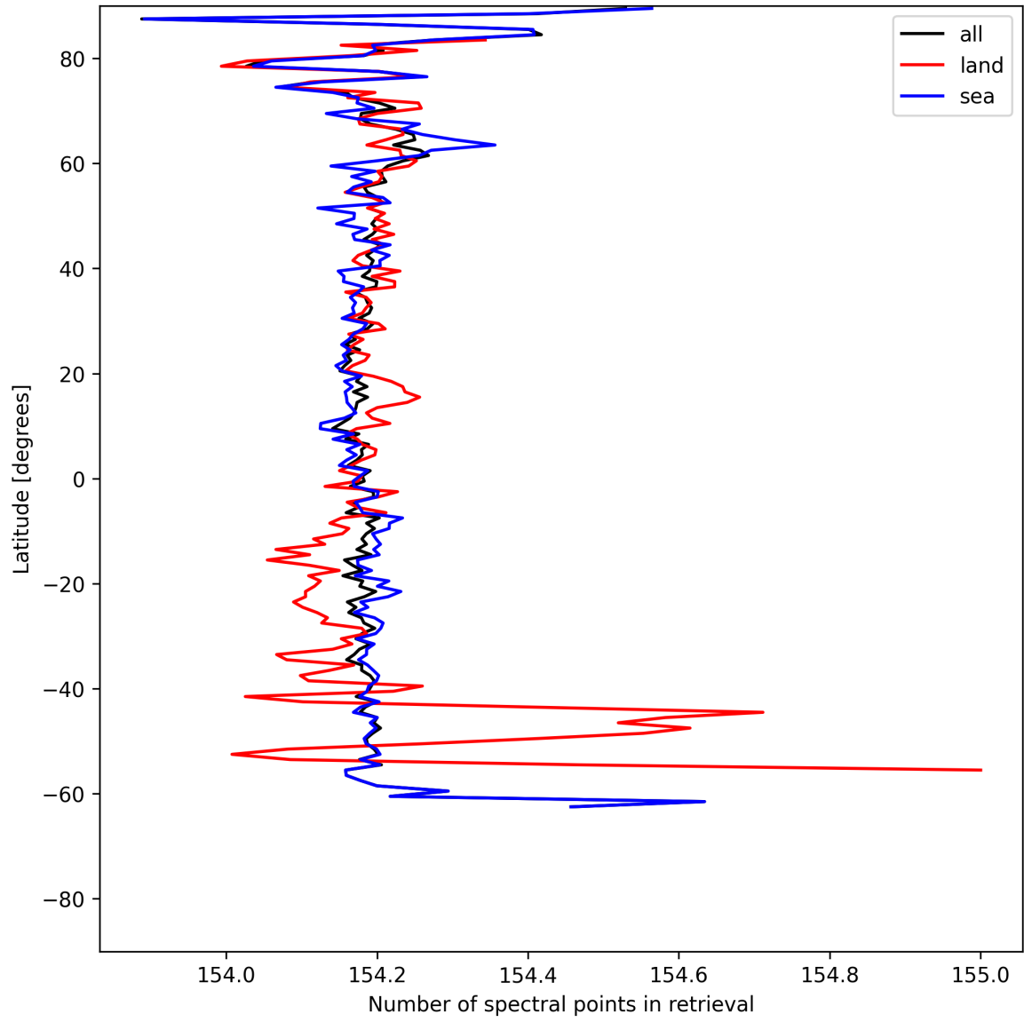
Figure 9: Zonal average of “Number of spectral points in retrieval” for 2025-07-12 to 2025-07-13.
