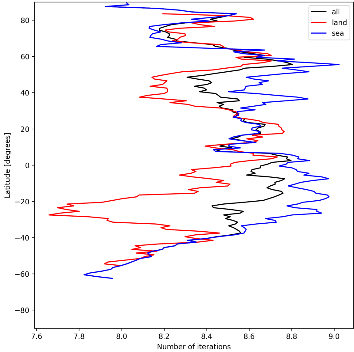
Figure 12: Zonal average of “Number of iterations” for 2025-07-12 to 2025-07-13.
