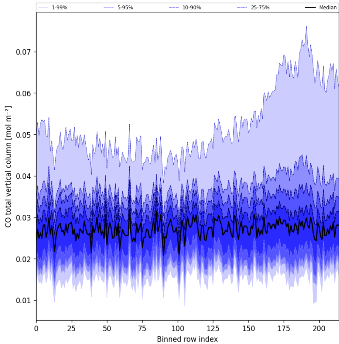
Figure 21: Along track statistics of “CO total vertical column” for 2025-07-12 to 2025-07-13
