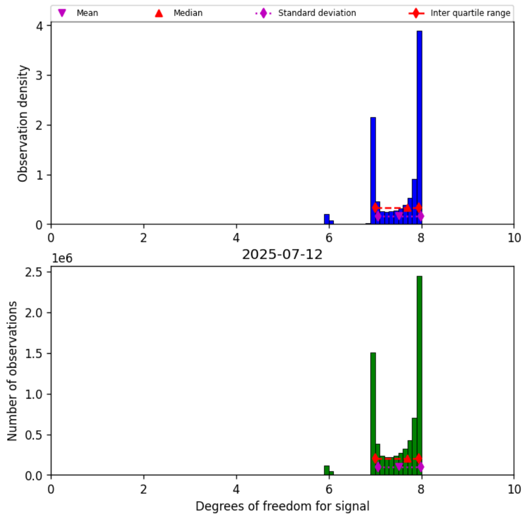
Figure 18: Histogram of “Degrees of freedom for signal” for 2025-07-12 to 2025-07-13
