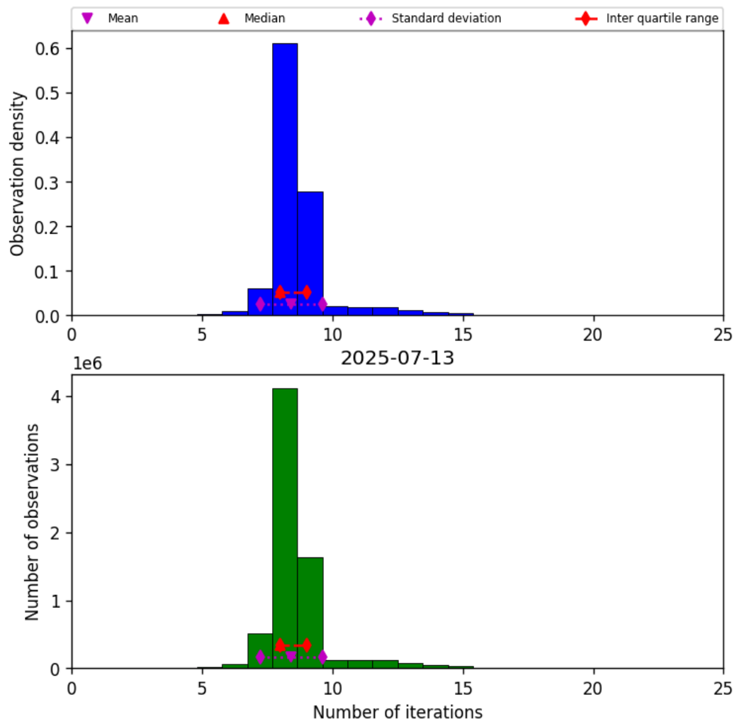
Figure 19: Histogram of “Number of iterations” for 2025-07-13 to 2025-07-14
