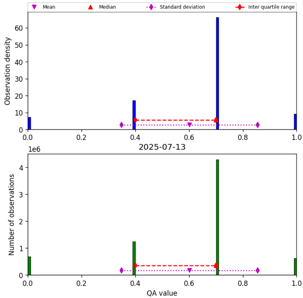
Figure 13: Histogram of “QA value” for 2025-07-13 to 2025-07-14
