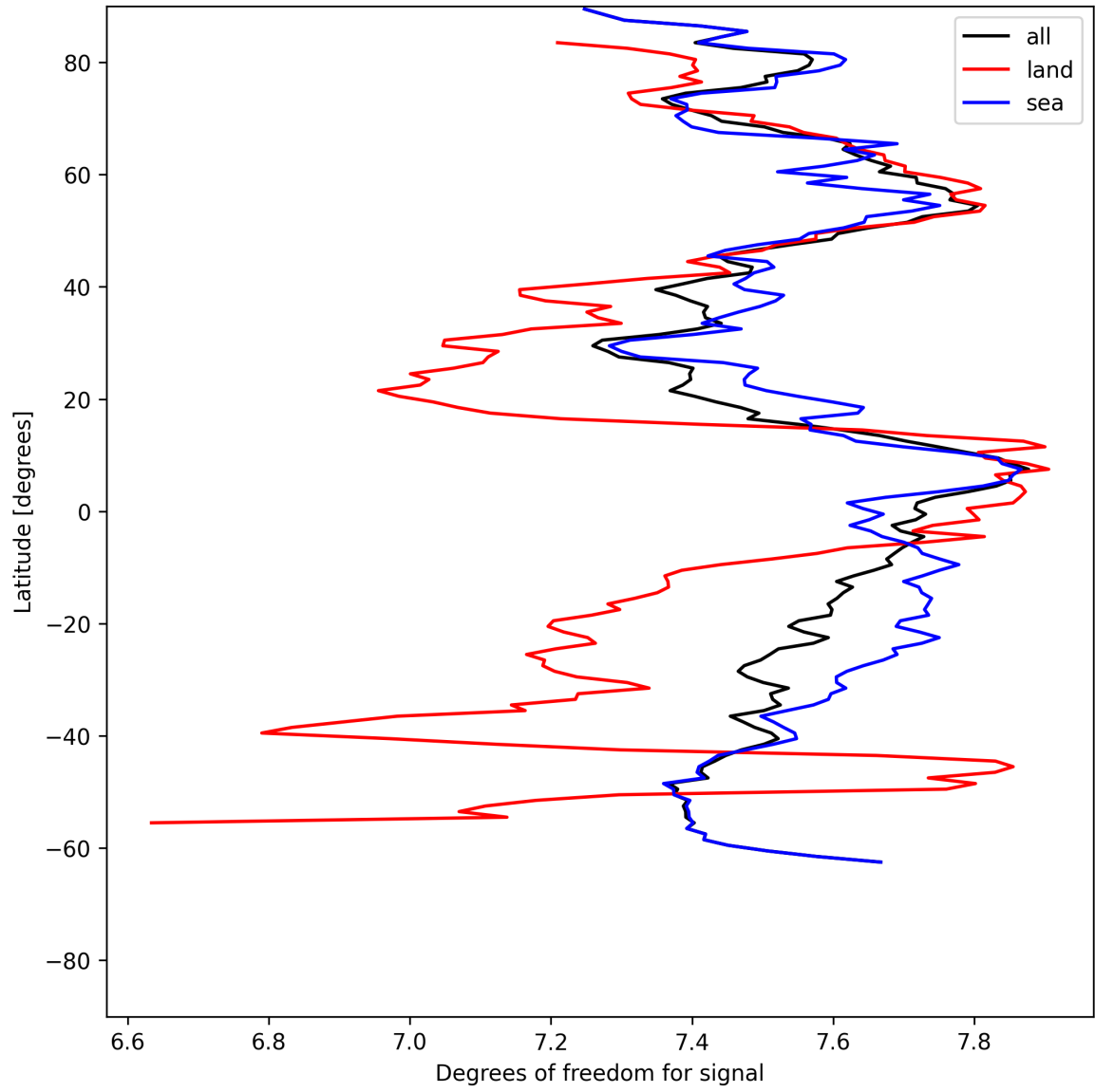
Figure 11: Zonal average of “Degrees of freedom for signal” for 2025-07-13 to 2025-07-14.
