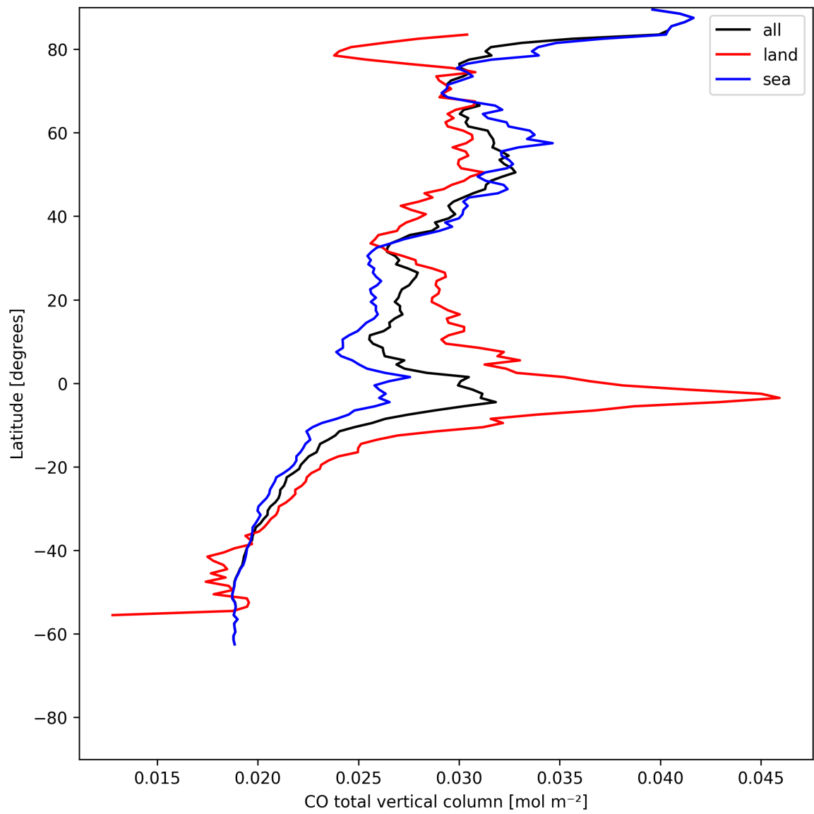
Figure 7: Zonal average of “CO total vertical column” for 2025-07-13 to 2025-07-14.
