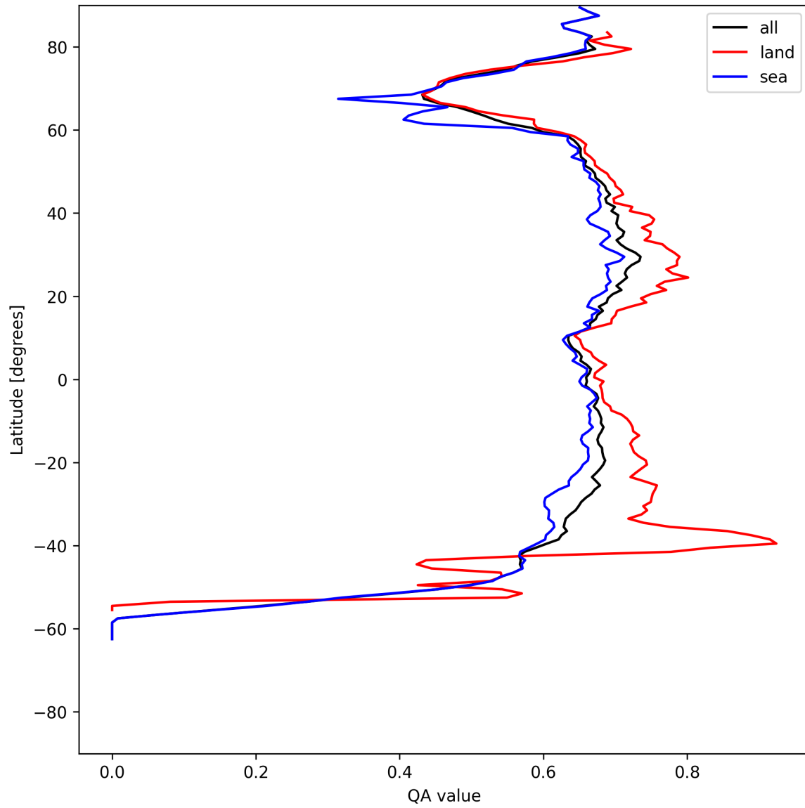
Figure 6: Zonal average of “QA value” for 2025-07-13 to 2025-07-14.
