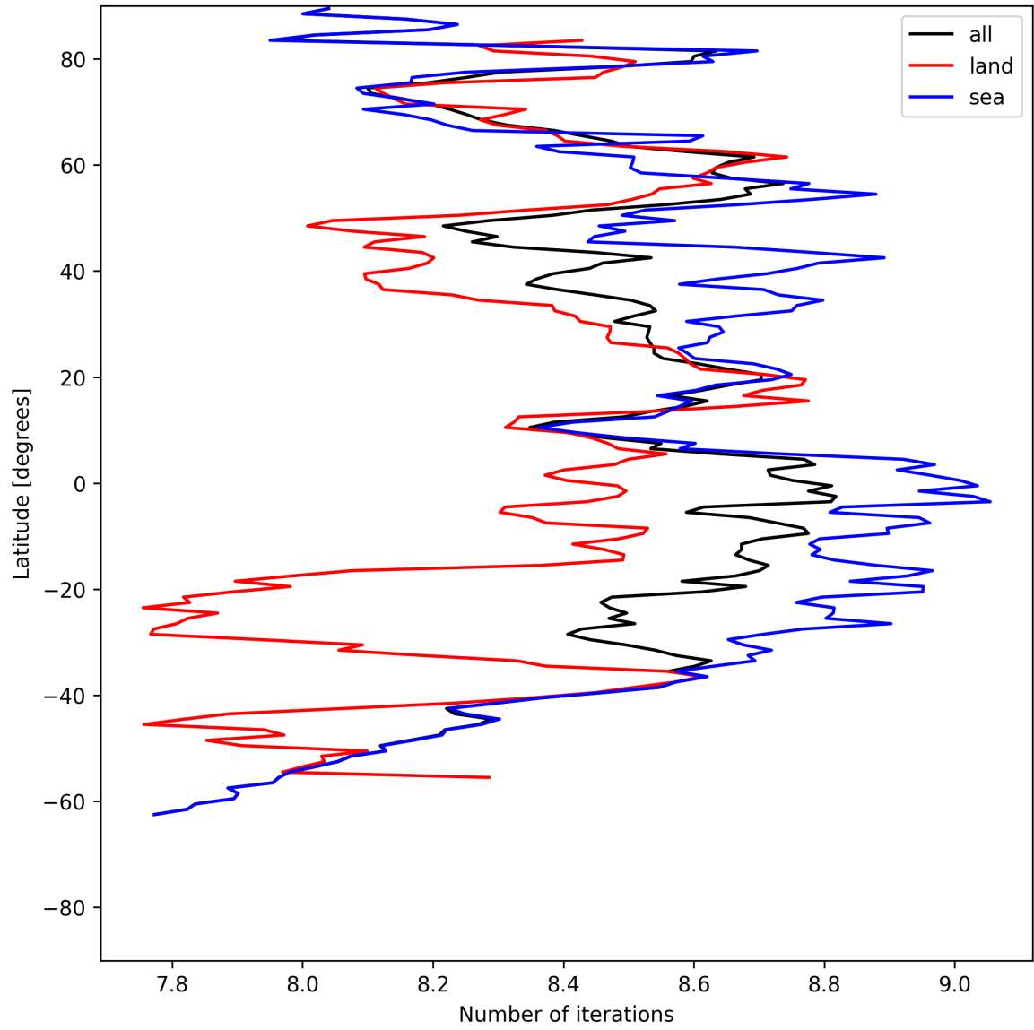
Figure 12: Zonal average of “Number of iterations” for 2025-07-13 to 2025-07-14.
