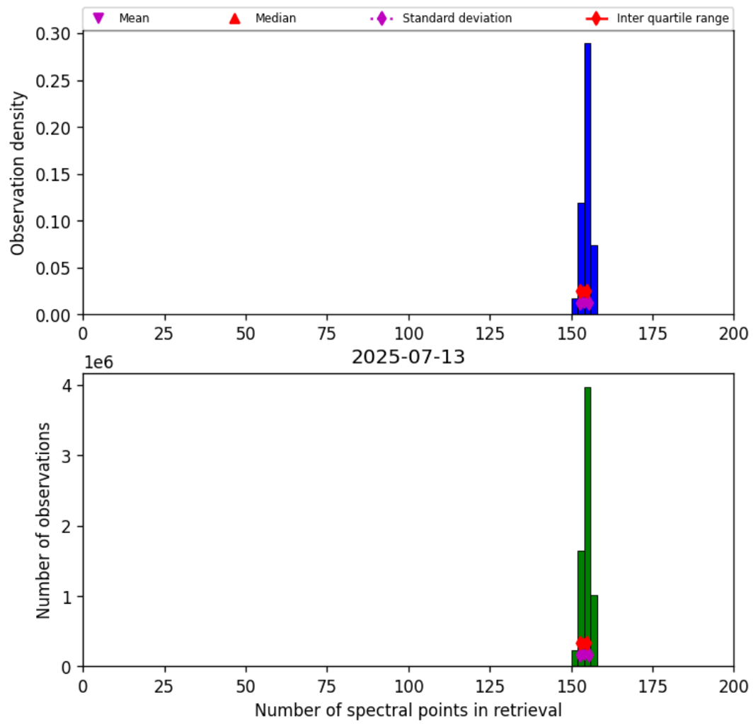
Figure 16: Histogram of “Number of spectral points in retrieval” for 2025-07-13 to 2025-07-14
