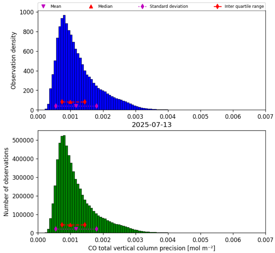
Figure 15: Histogram of “CO total vertical column precision” for 2025-07-13 to 2025-07-14
