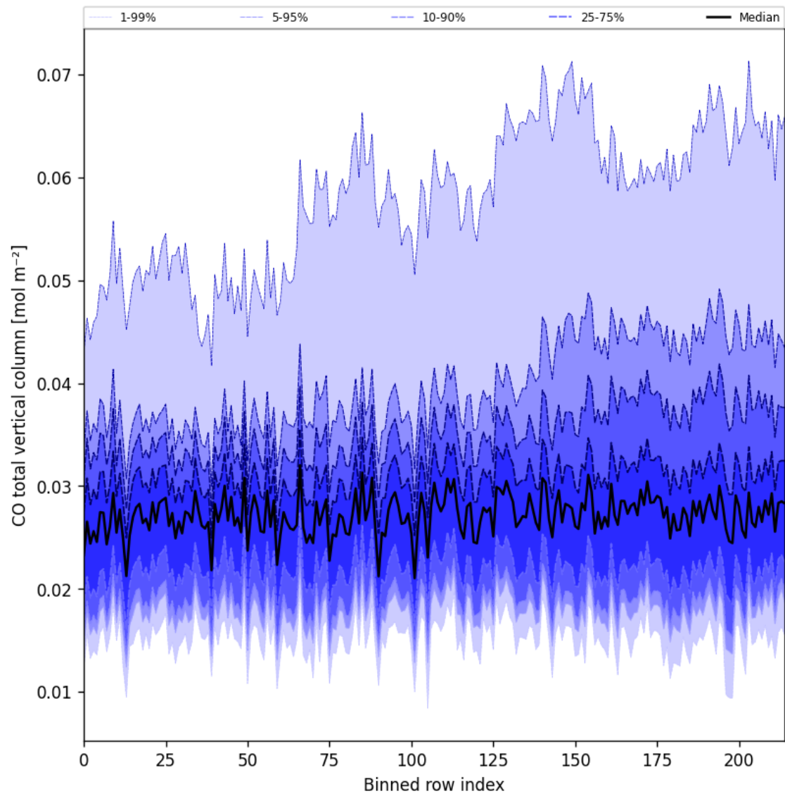
Figure 21: Along track statistics of “CO total vertical column” for 2025-07-13 to 2025-07-14
