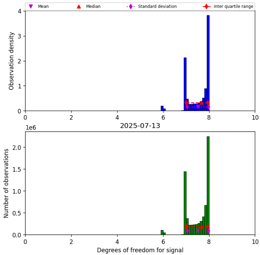
Figure 18: Histogram of “Degrees of freedom for signal” for 2025-07-13 to 2025-07-14
