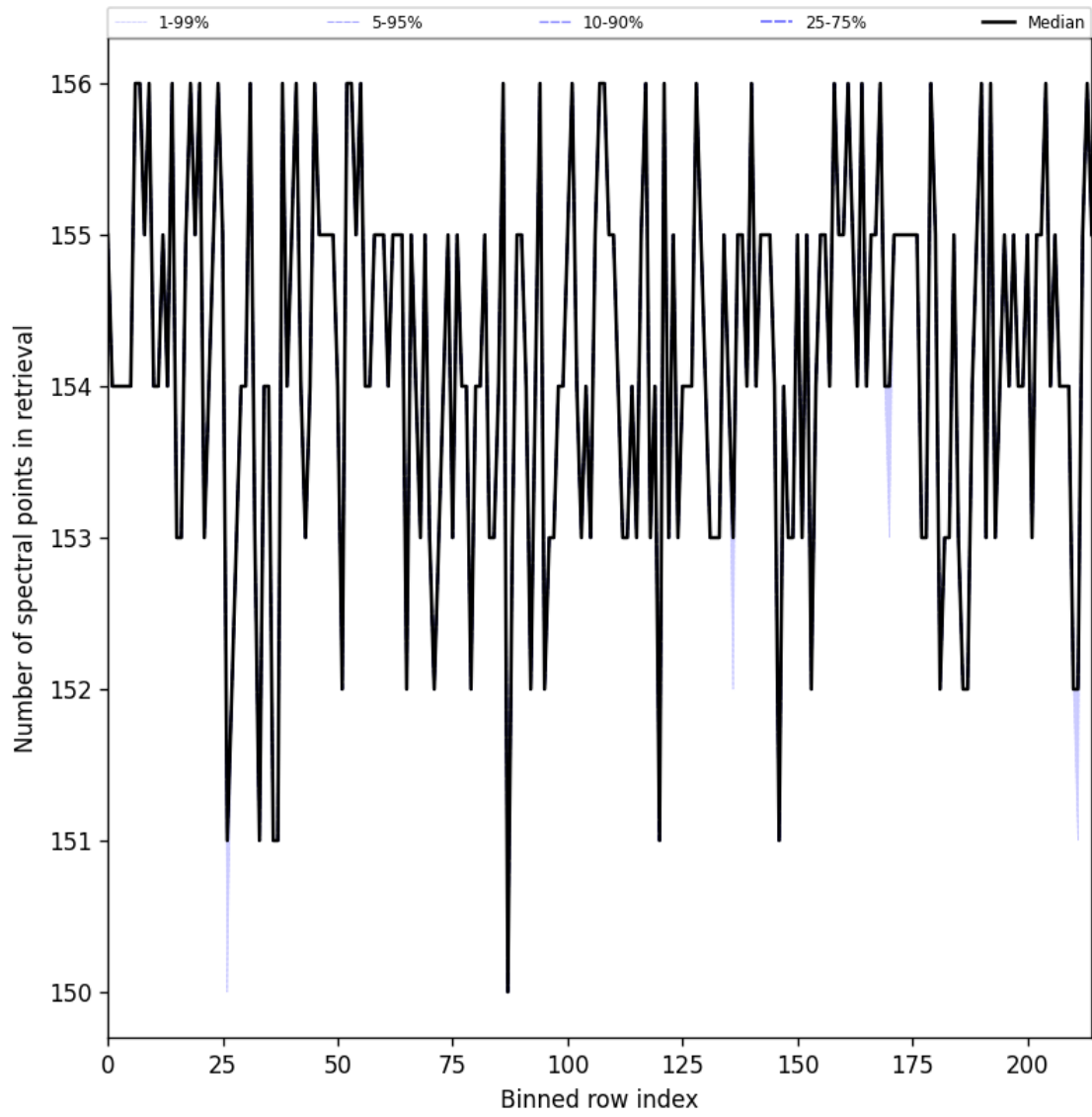
Figure 23: Along track statistics of “Number of spectral points in retrieval” for 2025-07-13 to 2025-07-14
