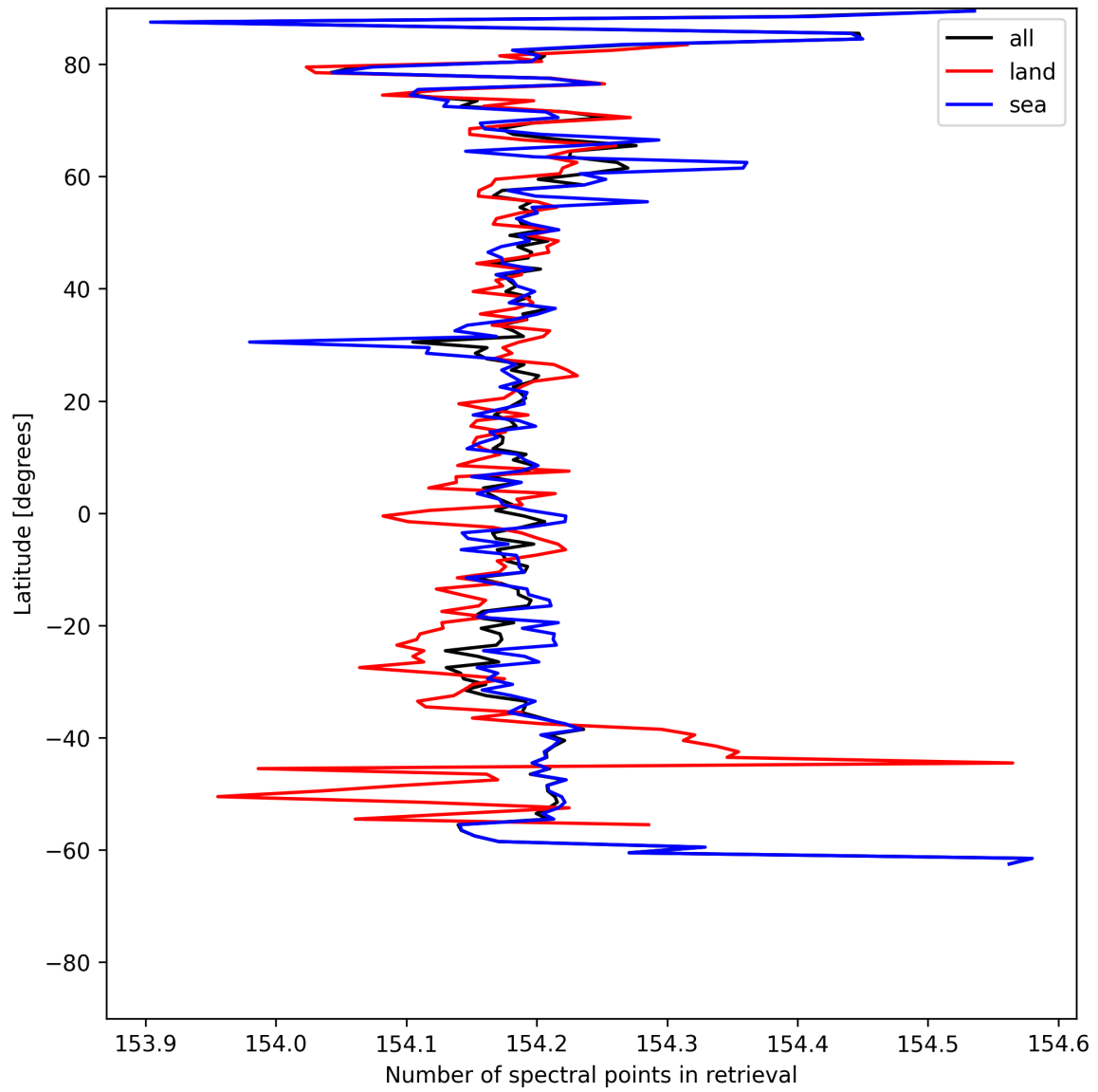
Figure 9: Zonal average of “Number of spectral points in retrieval” for 2025-07-13 to 2025-07-14.
