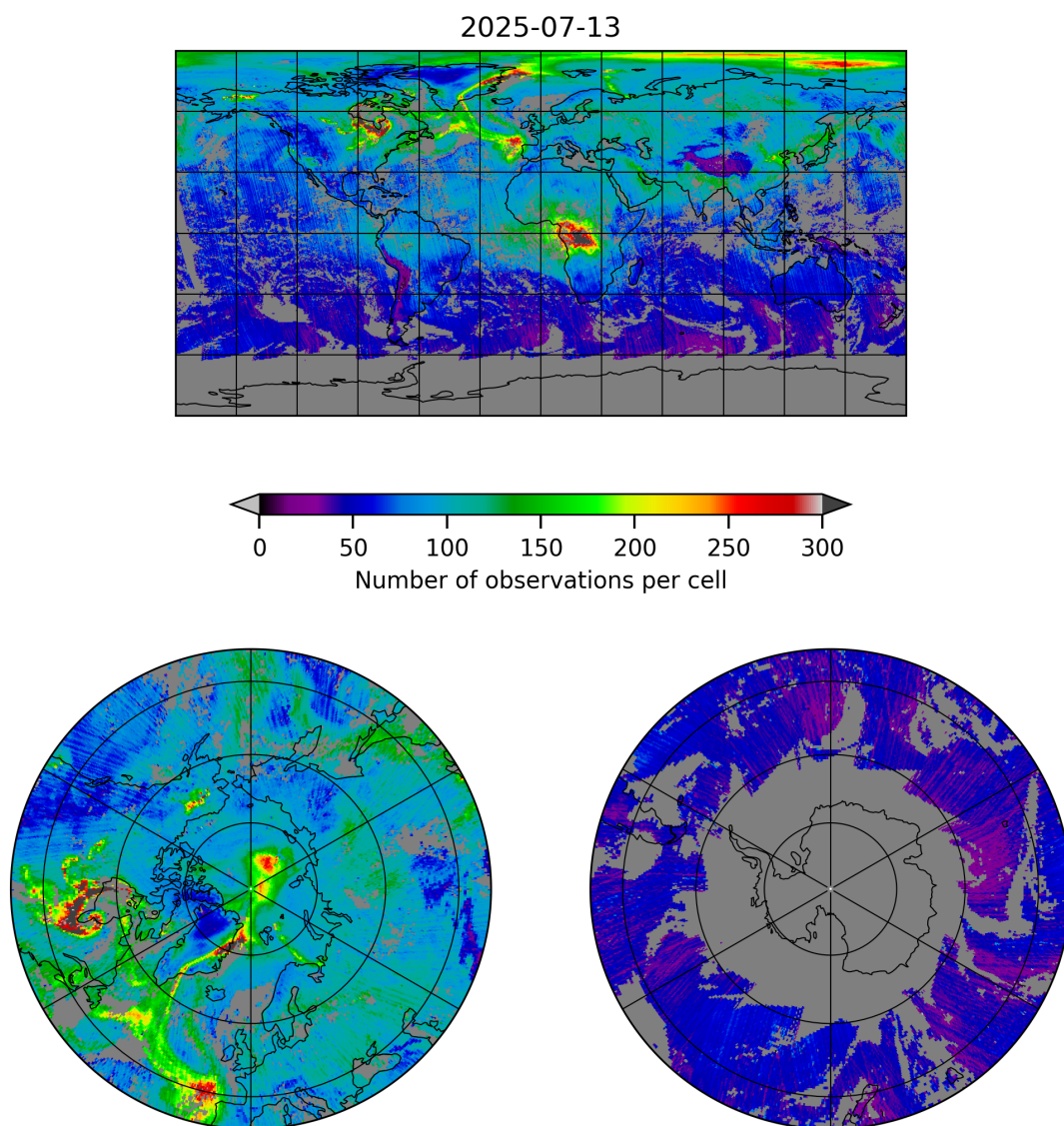
Figure 5: Map of the number of observations for 2025-07-13 to 2025-07-14
