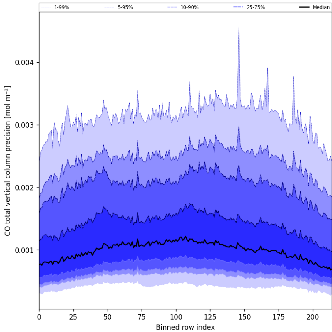
Figure 22: Along track statistics of “CO total vertical column precision” for 2025-07-13 to 2025-07-14
