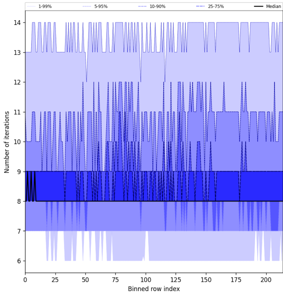
Figure 26: Along track statistics of “Number of iterations” for 2025-07-13 to 2025-07-14
