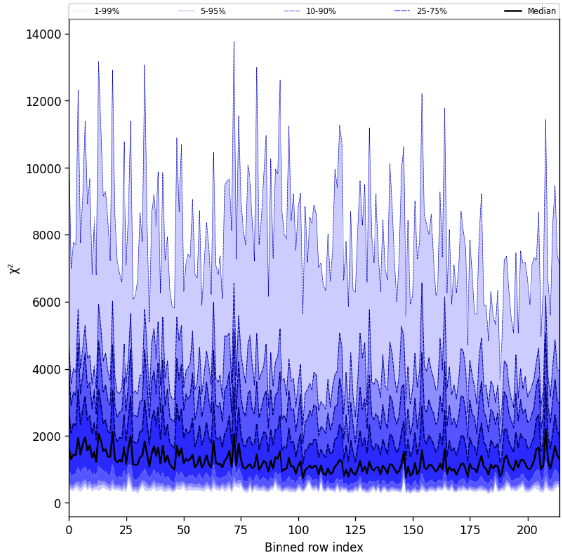
Figure 24: Along track statistics of “ \chi^2 ” for 2025-07-13 to 2025-07-14
