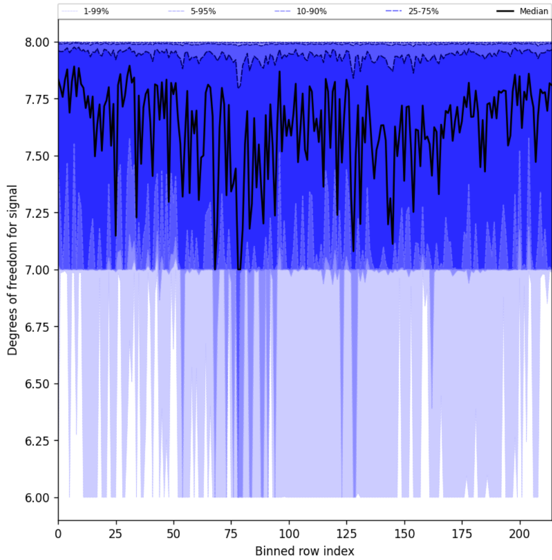
Figure 25: Along track statistics of “Degrees of freedom for signal” for 2025-07-13 to 2025-07-14
