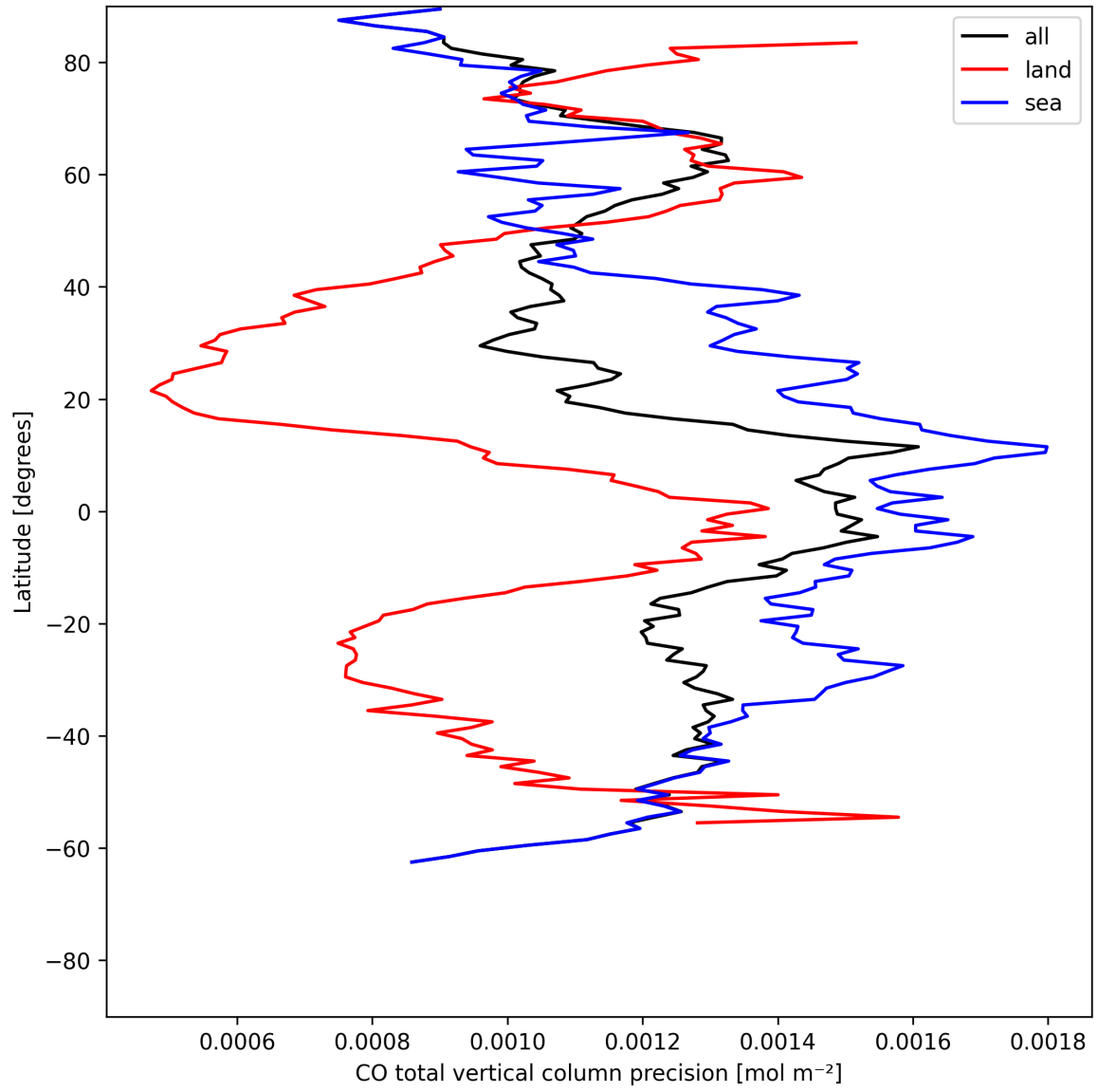
Figure 8: Zonal average of “CO total vertical column precision” for 2025-07-13 to 2025-07-14.
