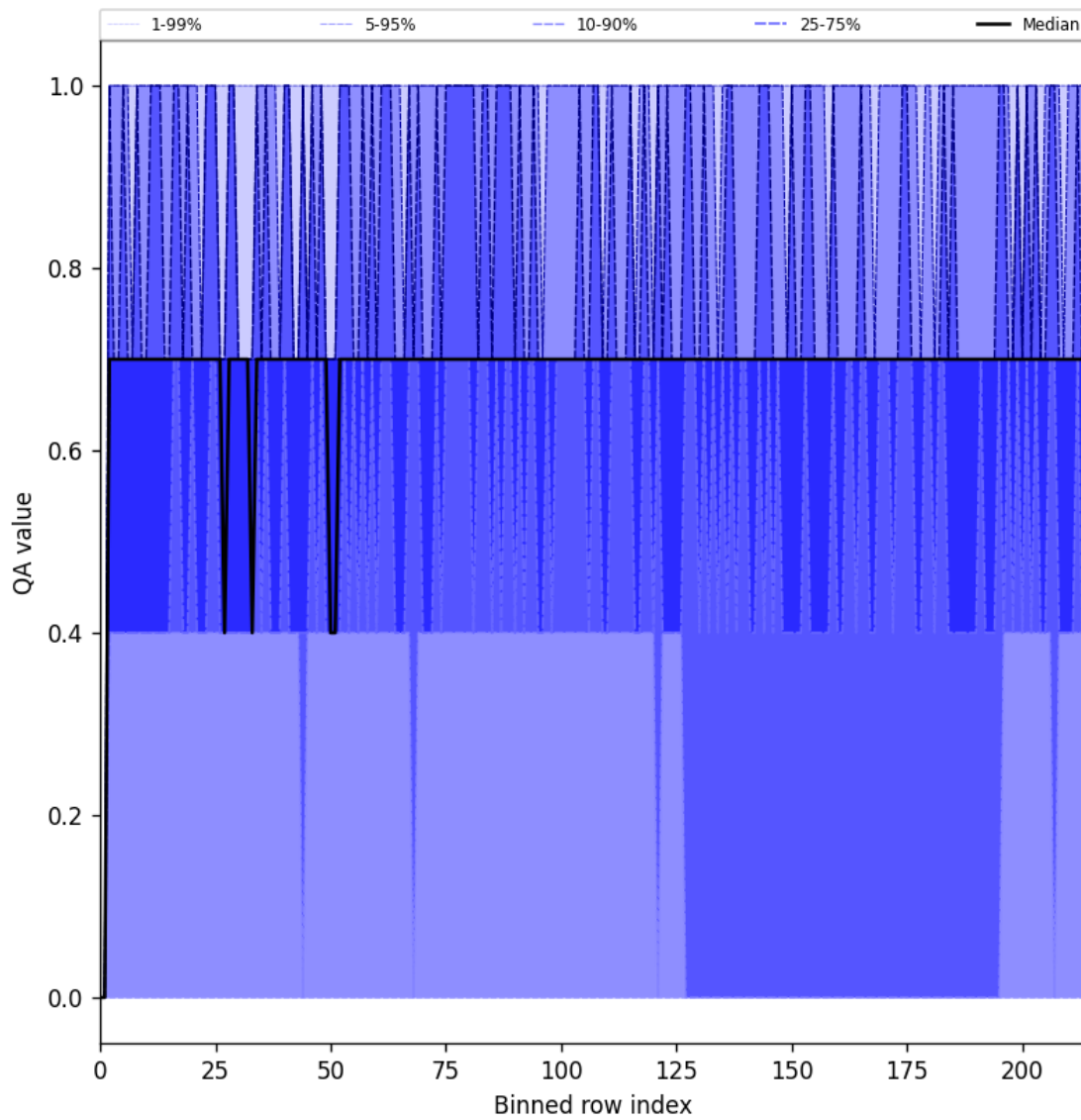
Figure 20: Along track statistics of “QA value” for 2025-07-13 to 2025-07-14
