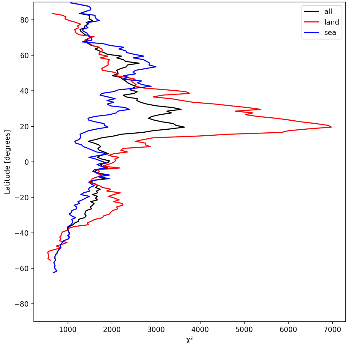
Figure 10: Zonal average of “ \chi^2 ” for 2025-07-13 to 2025-07-14.
