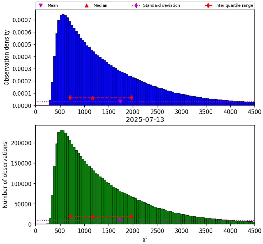
Figure 17: Histogram of " \chi^2 " for 2025-07-13 to 2025-07-14
