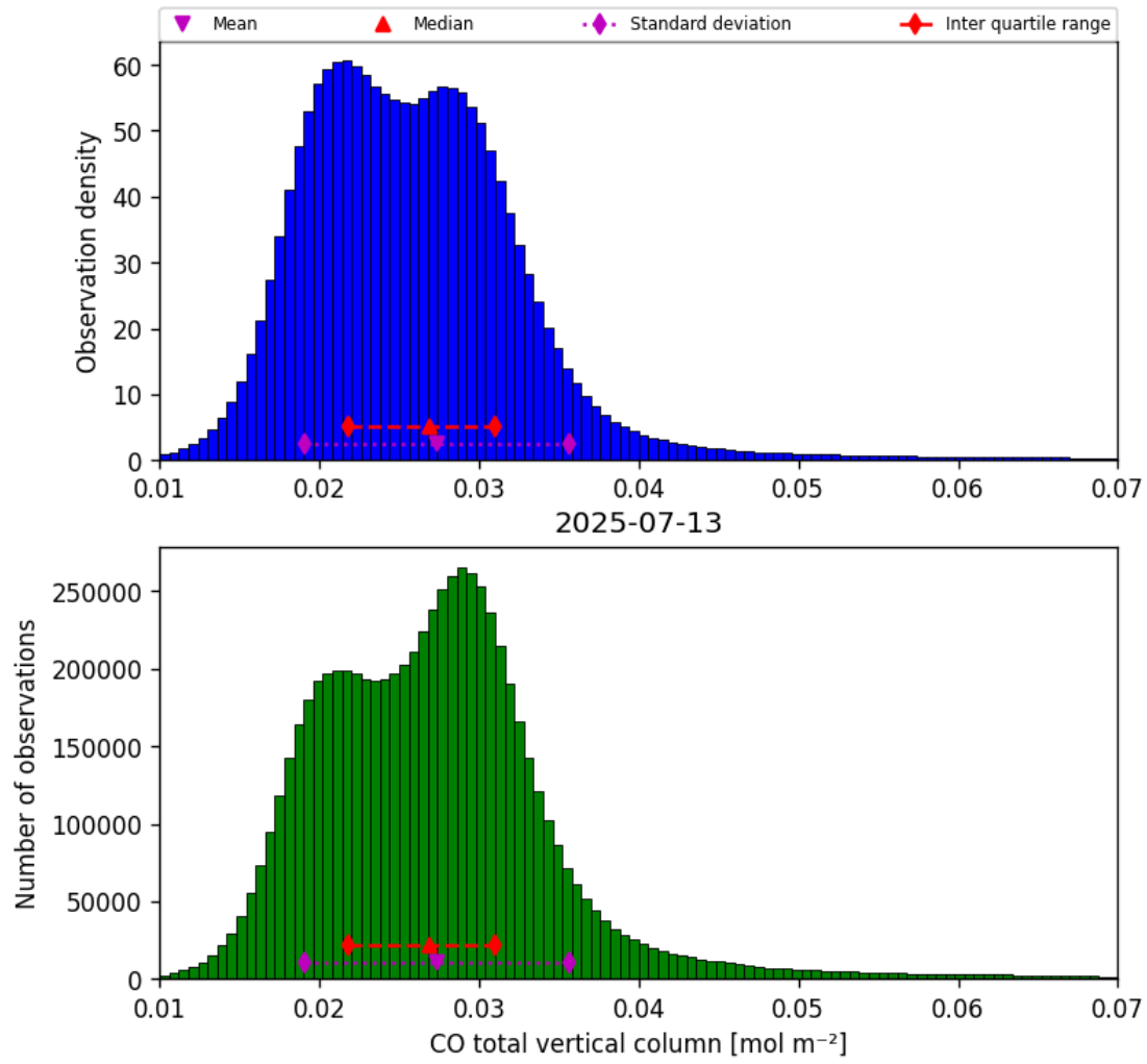
Figure 14: Histogram of “CO total vertical column” for 2025-07-13 to 2025-07-14
