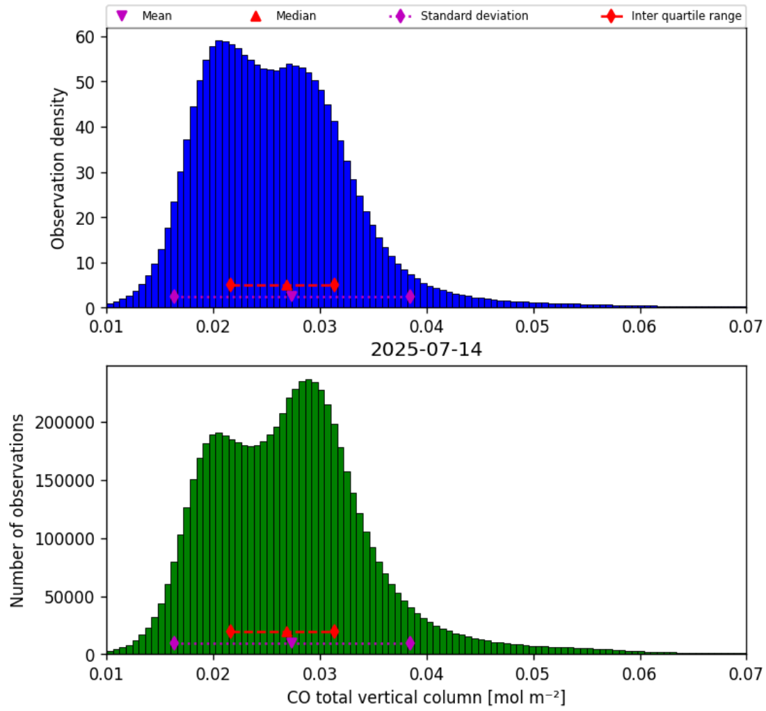
Figure 14: Histogram of “CO total vertical column” for 2025-07-14 to 2025-07-15
