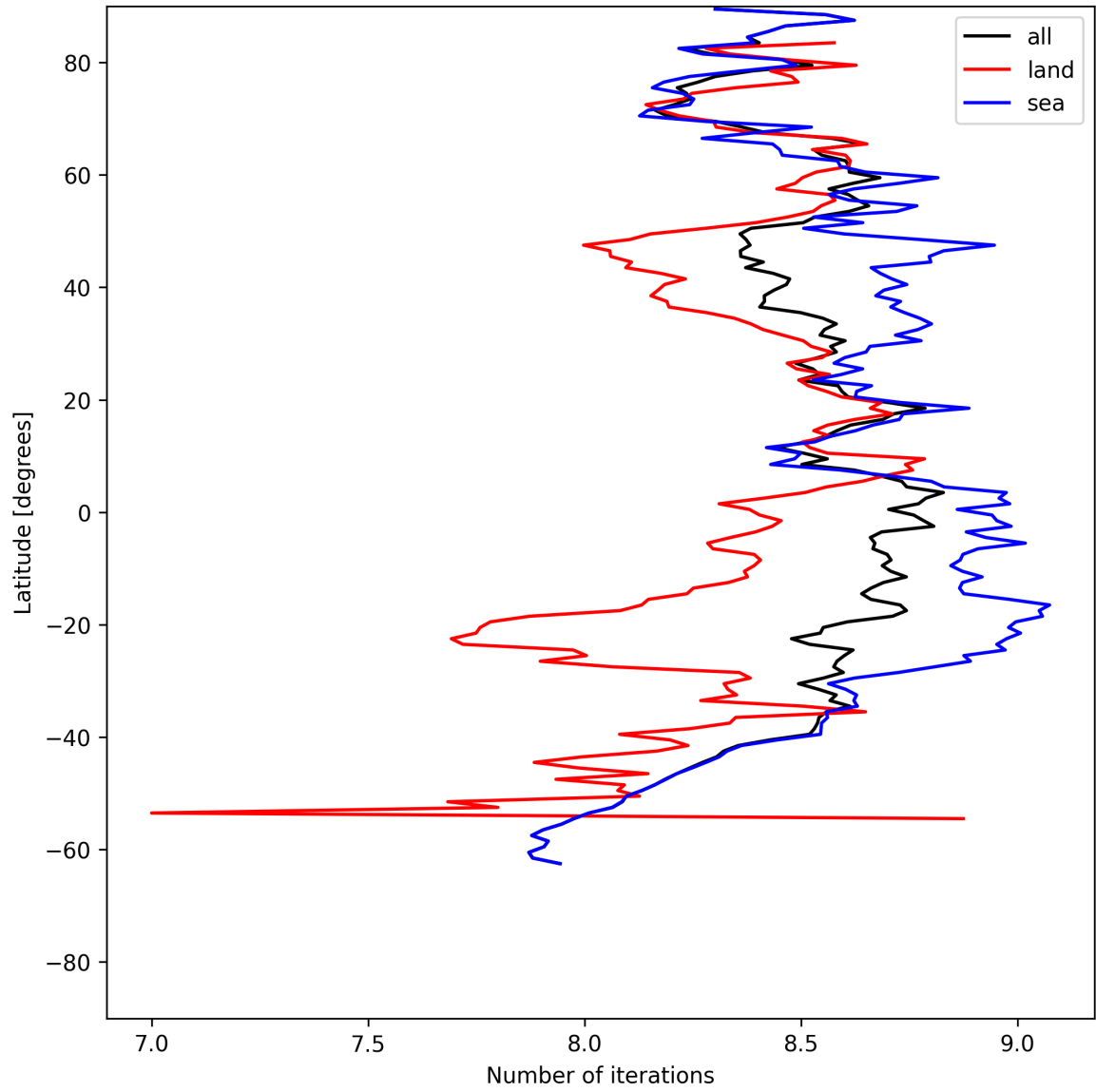
Figure 12: Zonal average of “Number of iterations” for 2025-07-14 to 2025-07-15.
