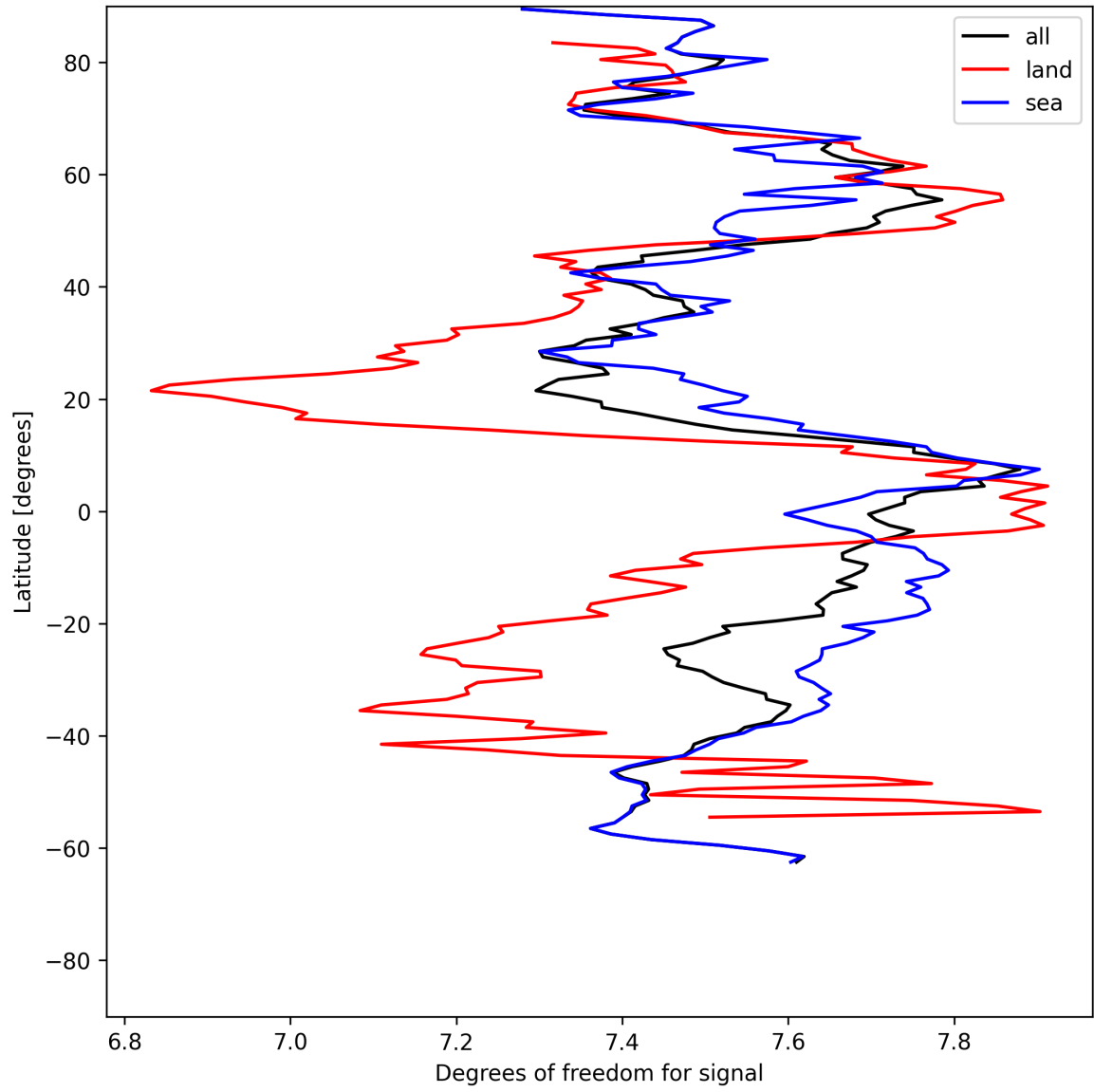
Figure 11: Zonal average of “Degrees of freedom for signal” for 2025-07-14 to 2025-07-15.
