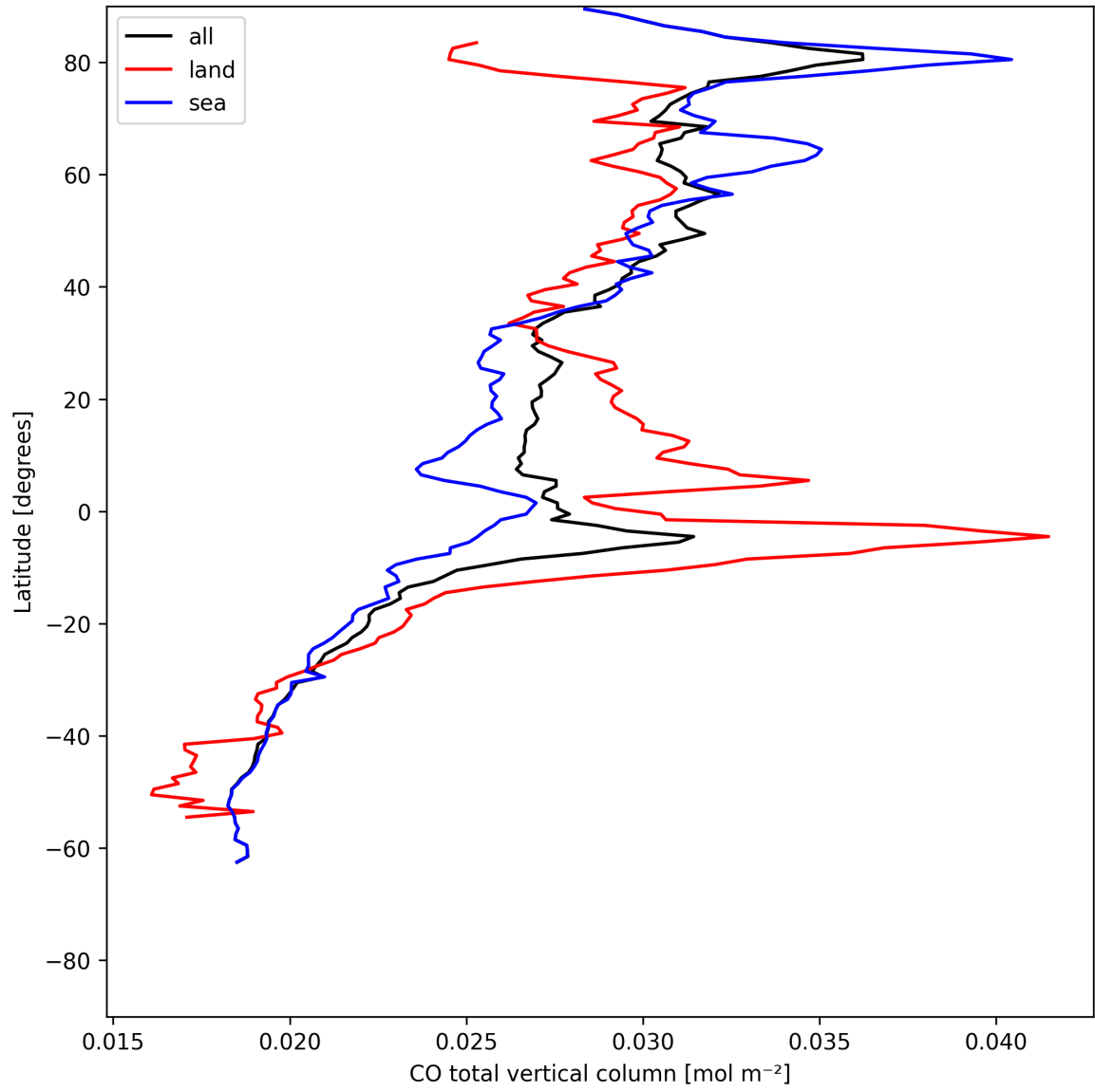
Figure 7: Zonal average of “CO total vertical column” for 2025-07-14 to 2025-07-15.
