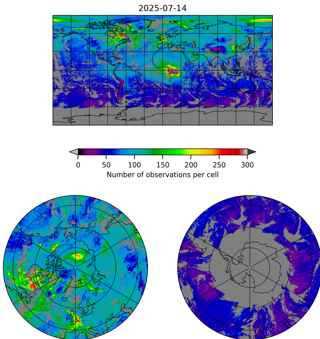
Figure 5: Map of the number of observations for 2025-07-14 to 2025-07-15
