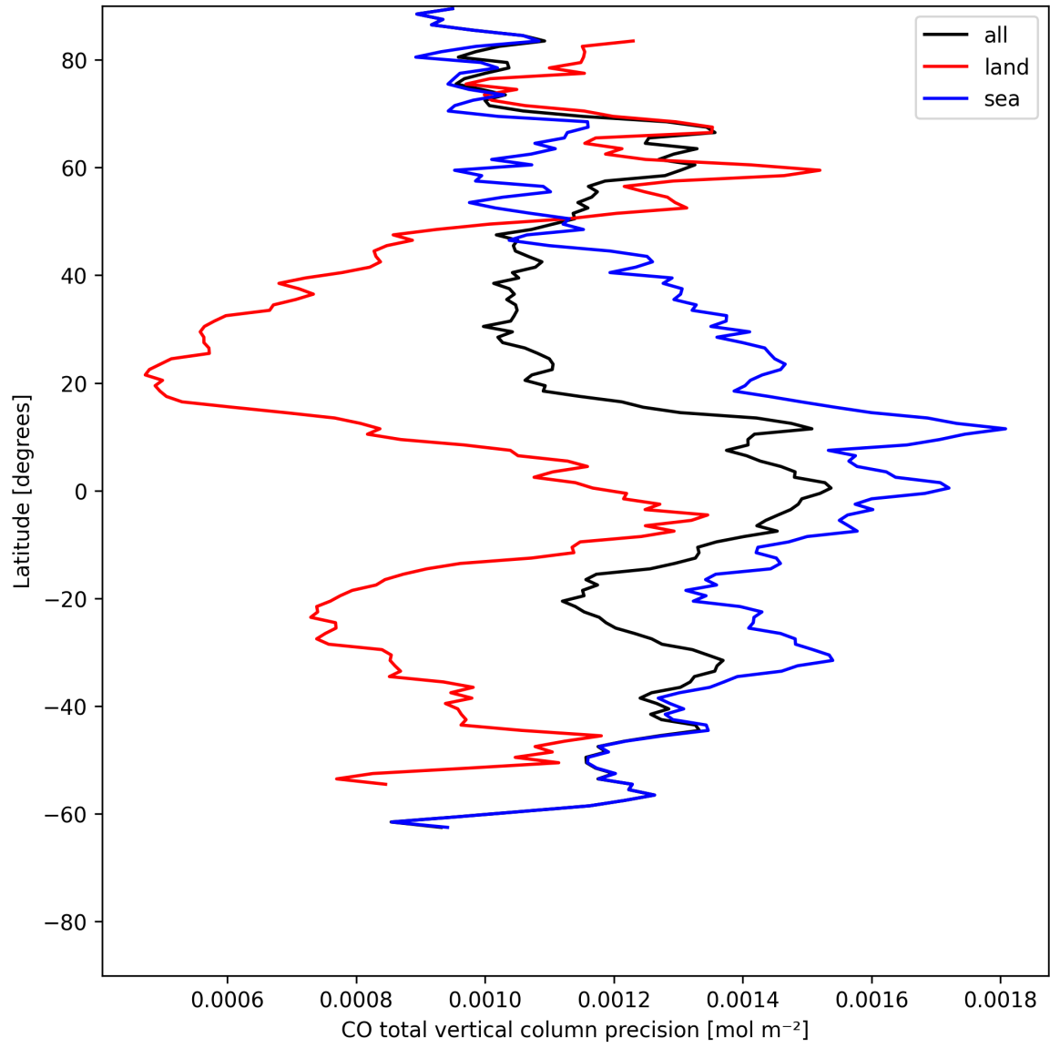
Figure 8: Zonal average of "CO total vertical column precision" for 2025-07-14 to 2025-07-15.
