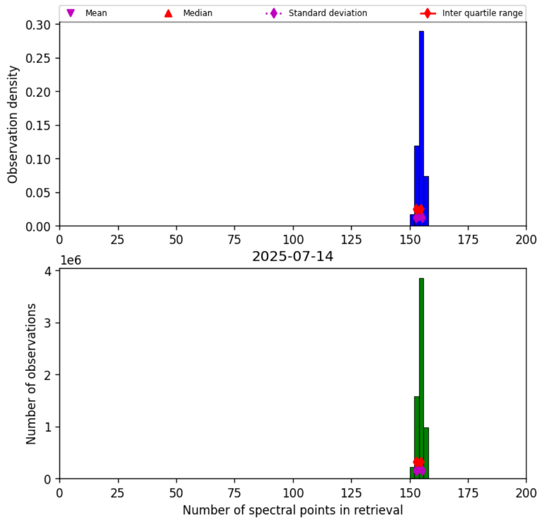
Figure 16: Histogram of “Number of spectral points in retrieval” for 2025-07-14 to 2025-07-15
