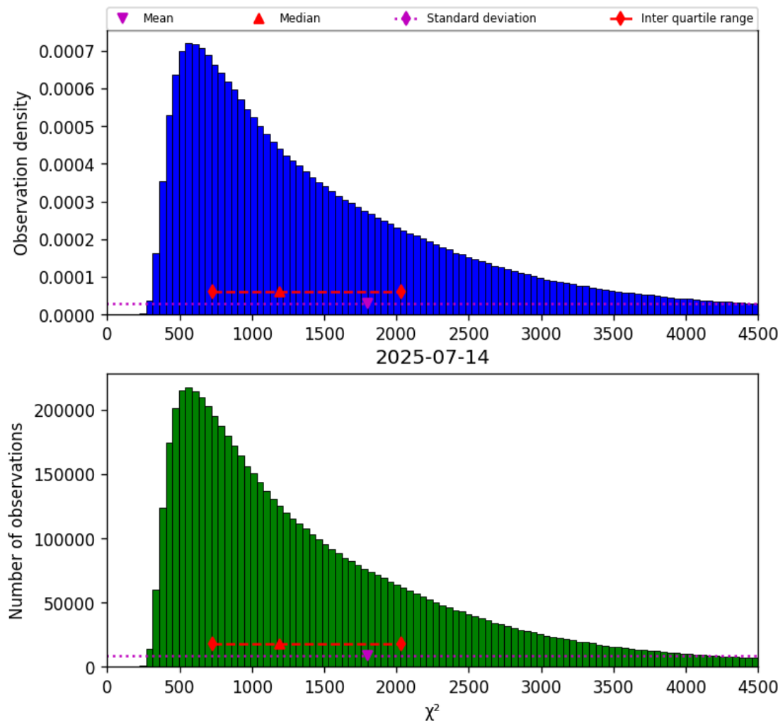
Figure 17: Histogram of “ \chi^2 ” for 2025-07-14 to 2025-07-15
