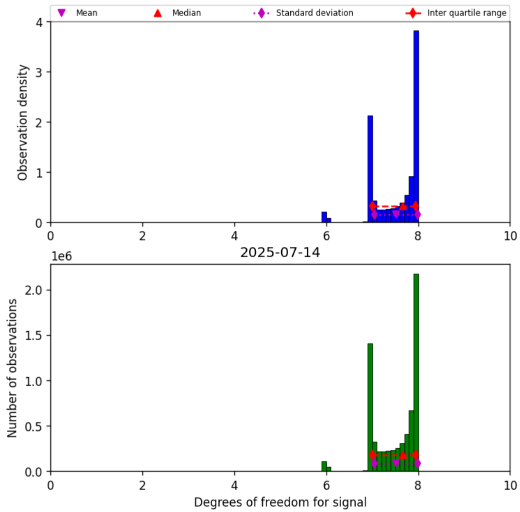
Figure 18: Histogram of “Degrees of freedom for signal” for 2025-07-14 to 2025-07-15
