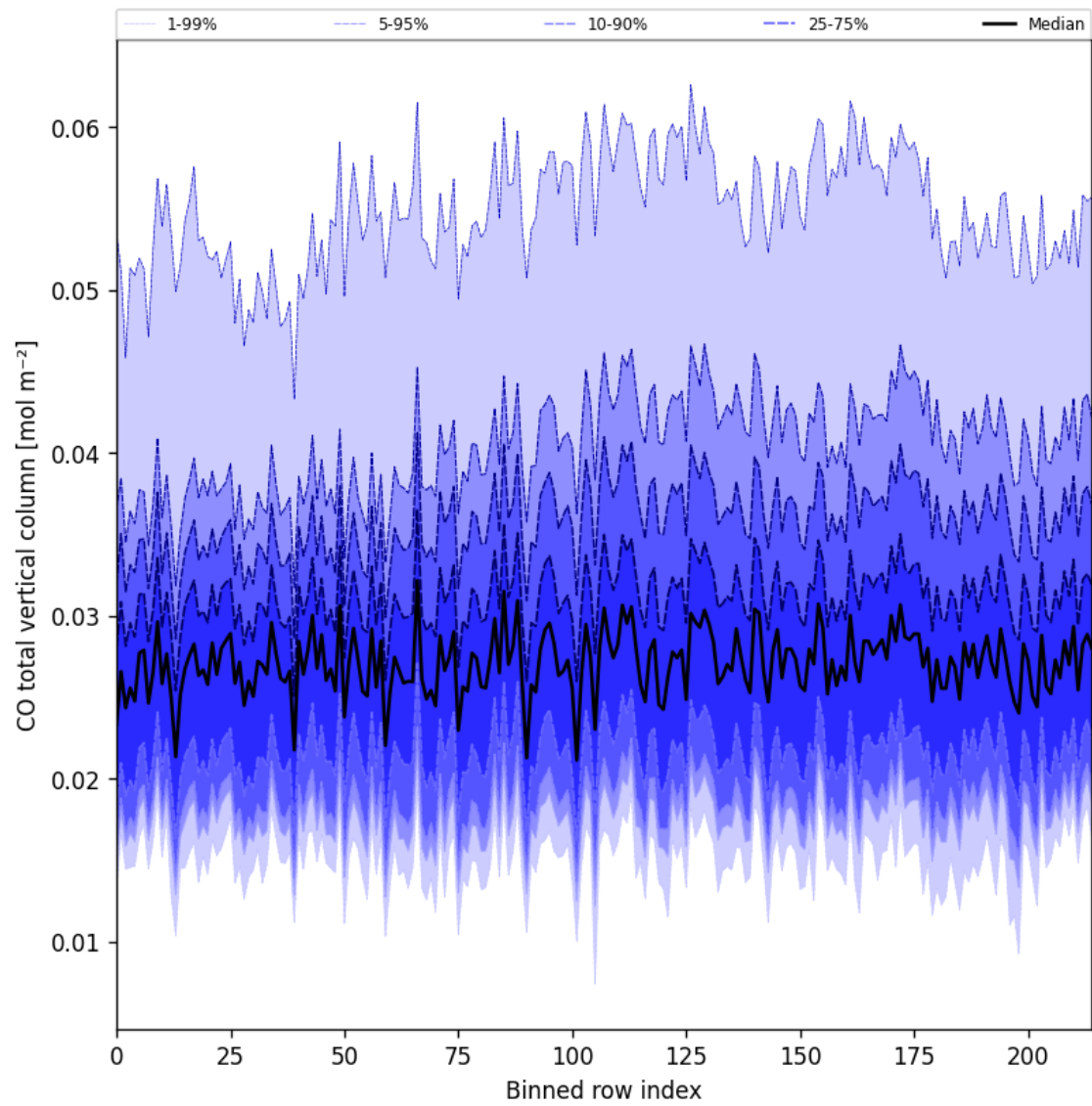
Figure 21: Along track statistics of “CO total vertical column” for 2025-07-14 to 2025-07-15
