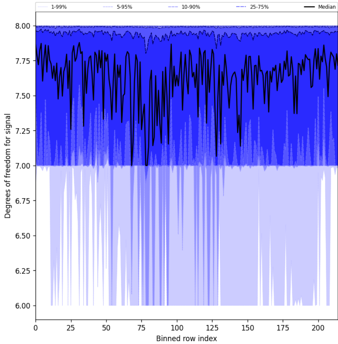
Figure 25: Along track statistics of “Degrees of freedom for signal” for 2025-07-14 to 2025-07-15
