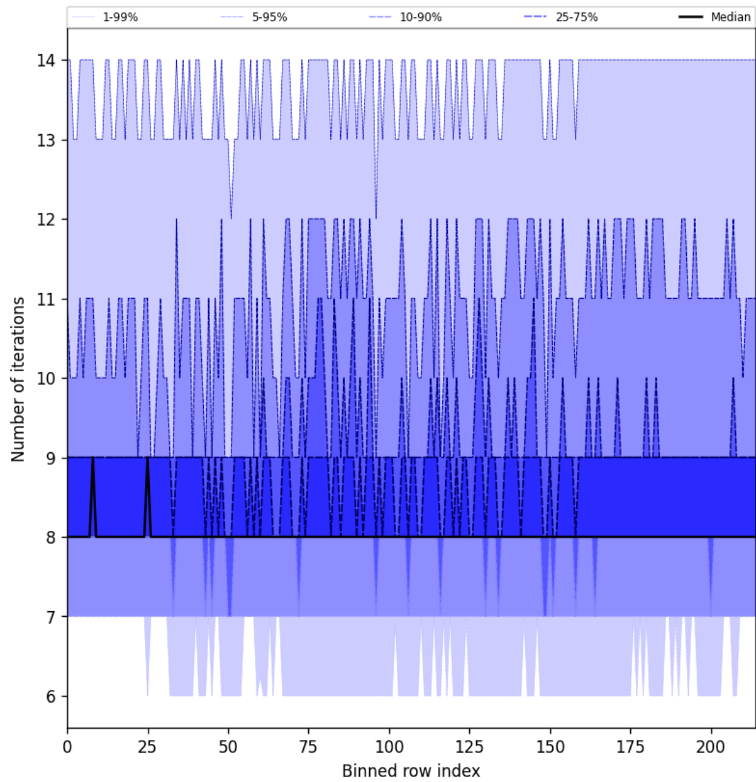
Figure 26: Along track statistics of “Number of iterations” for 2025-07-14 to 2025-07-15
