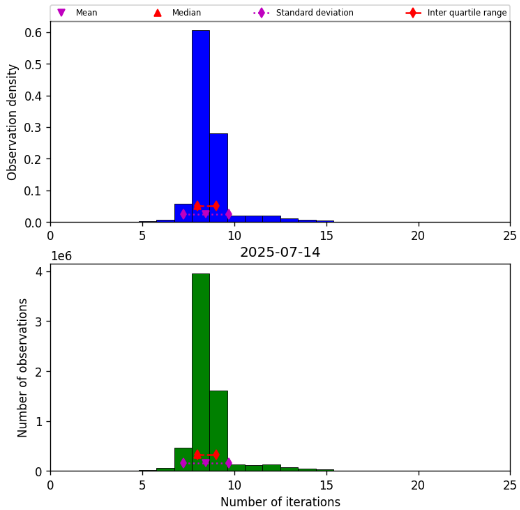
Figure 19: Histogram of “Number of iterations” for 2025-07-14 to 2025-07-15
