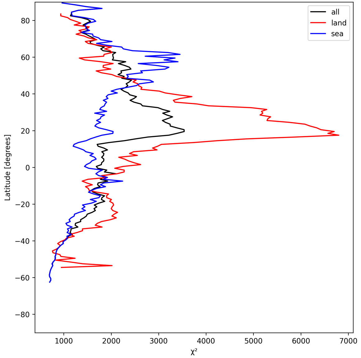
Figure 10: Zonal average of “ \chi^2 ” for 2025-07-14 to 2025-07-15.
