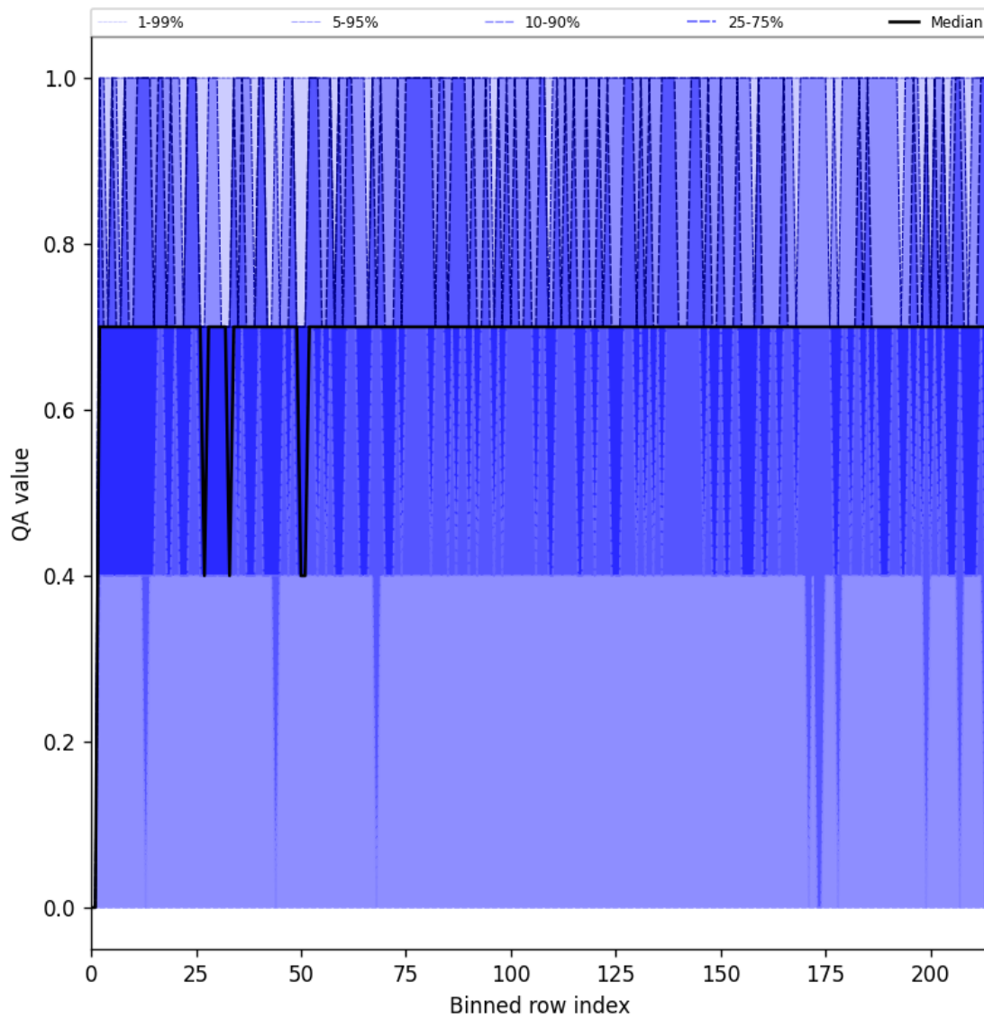
Figure 20: Along track statistics of “QA value” for 2025-07-14 to 2025-07-15
