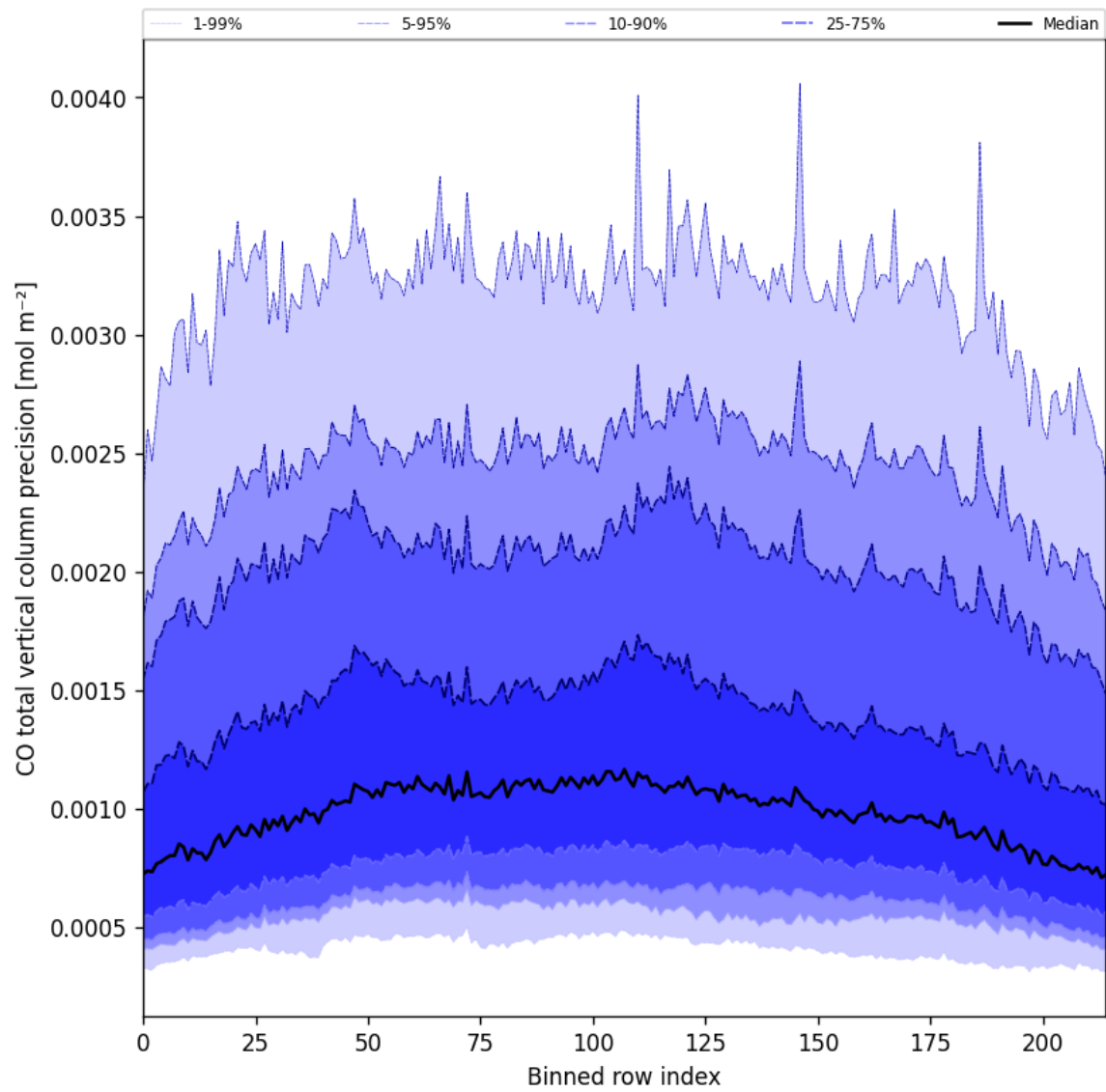
Figure 22: Along track statistics of “CO total vertical column precision” for 2025-07-14 to 2025-07-15
