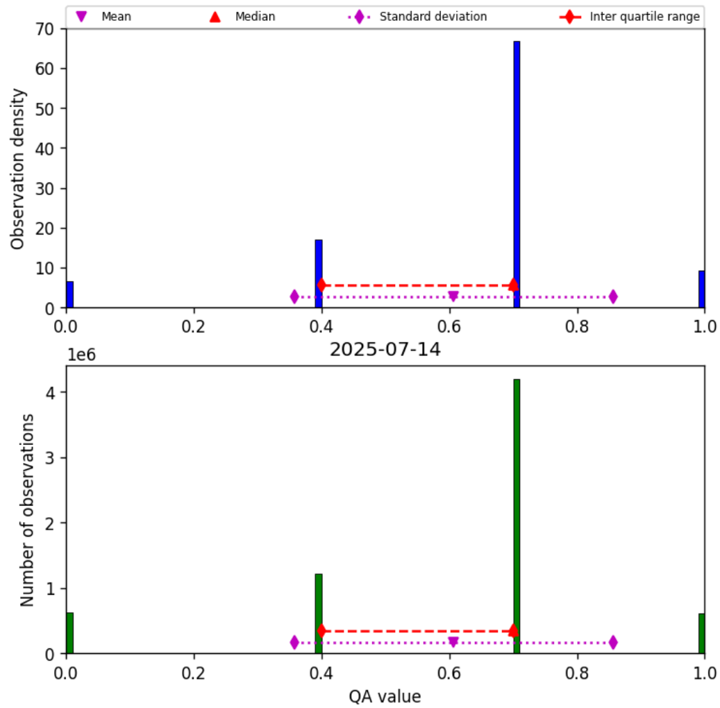
Figure 13: Histogram of “QA value” for 2025-07-14 to 2025-07-15
