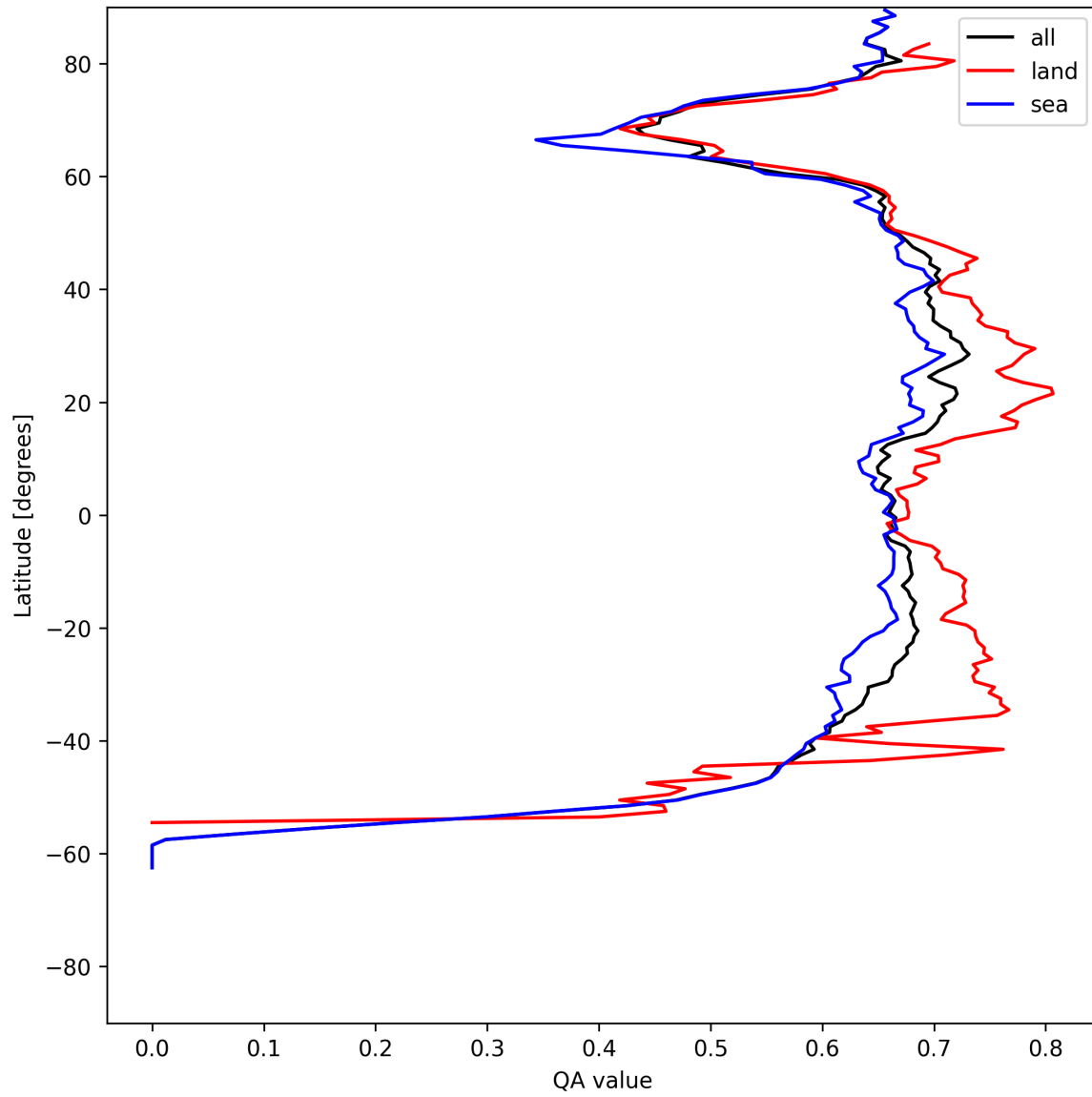
Figure 6: Zonal average of “QA value” for 2025-07-14 to 2025-07-15.
