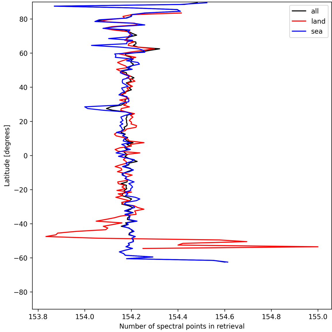
Figure 9: Zonal average of “Number of spectral points in retrieval” for 2025-07-14 to 2025-07-15.
