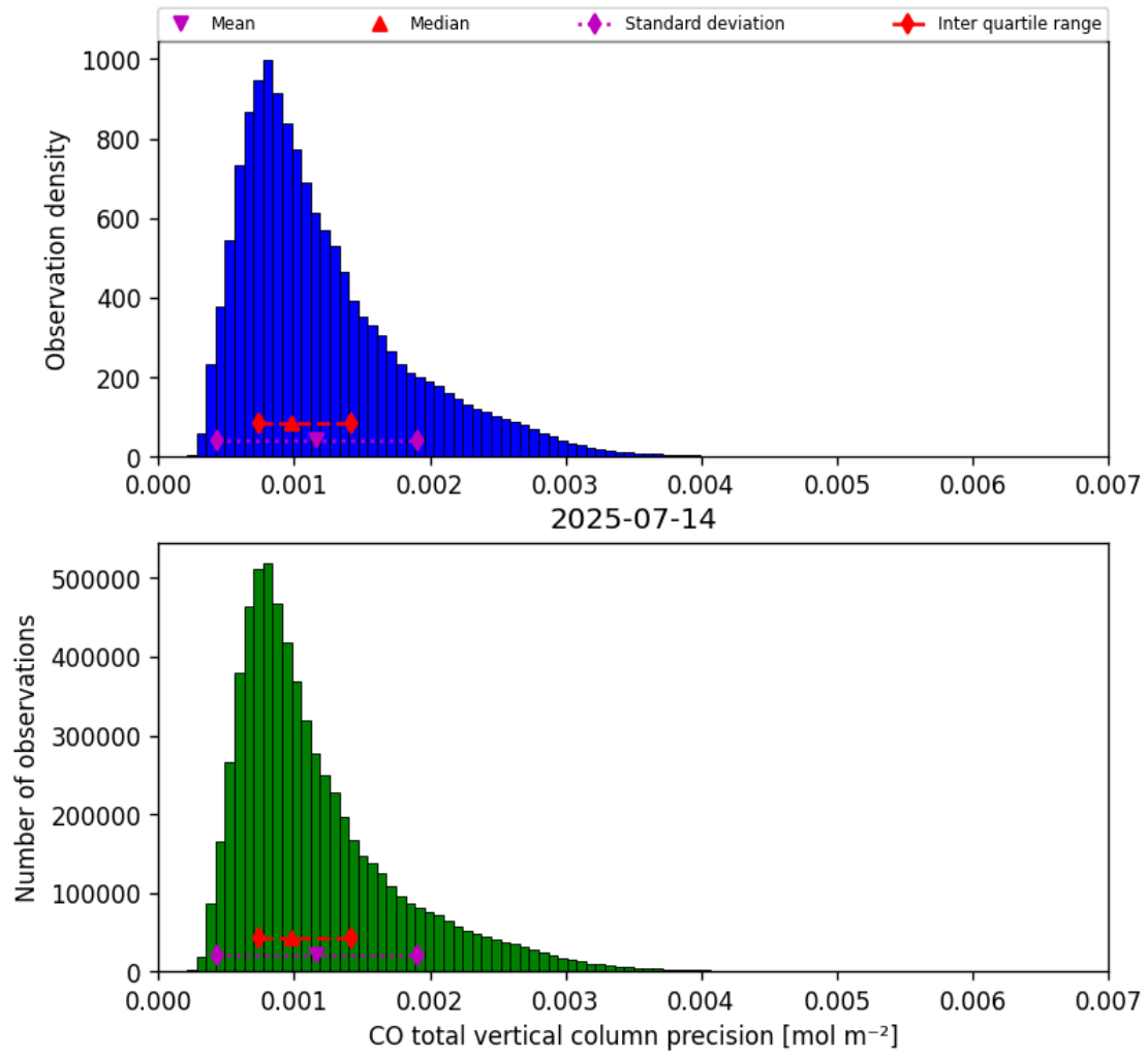
Figure 15: Histogram of “CO total vertical column precision” for 2025-07-14 to 2025-07-15
