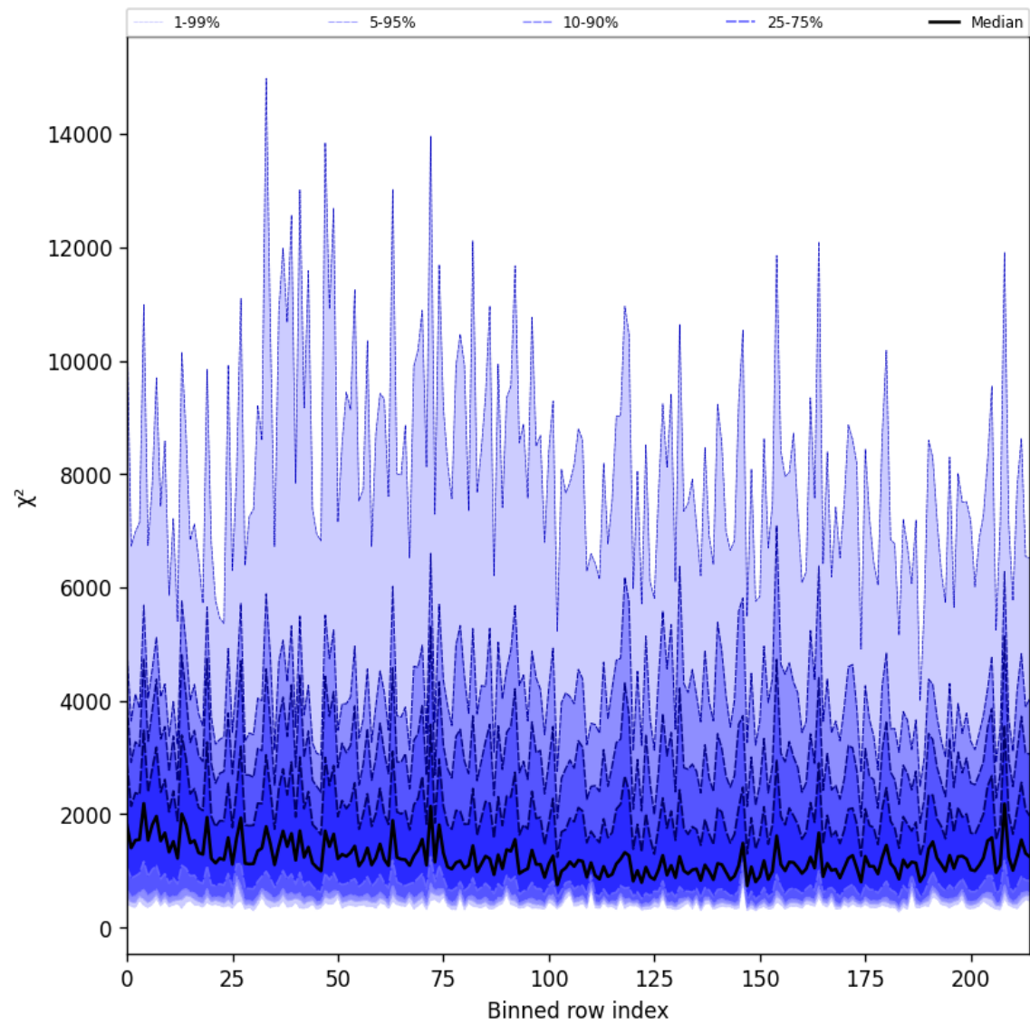
Figure 24: Along track statistics of “ \chi^2 ” for 2025-07-14 to 2025-07-15
