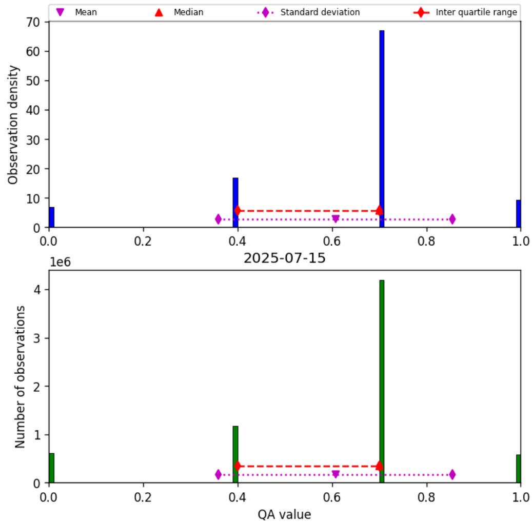
Figure 13: Histogram of “QA value” for 2025-07-15 to 2025-07-16
