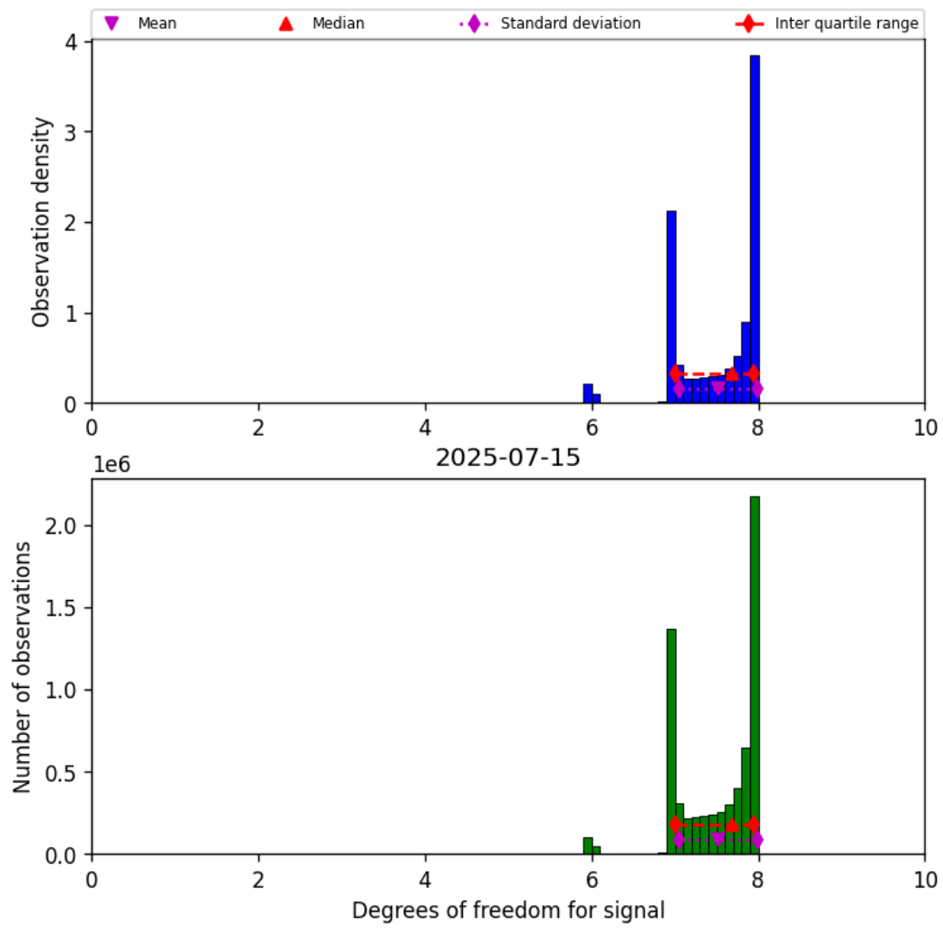
Figure 18: Histogram of “Degrees of freedom for signal” for 2025-07-15 to 2025-07-16
