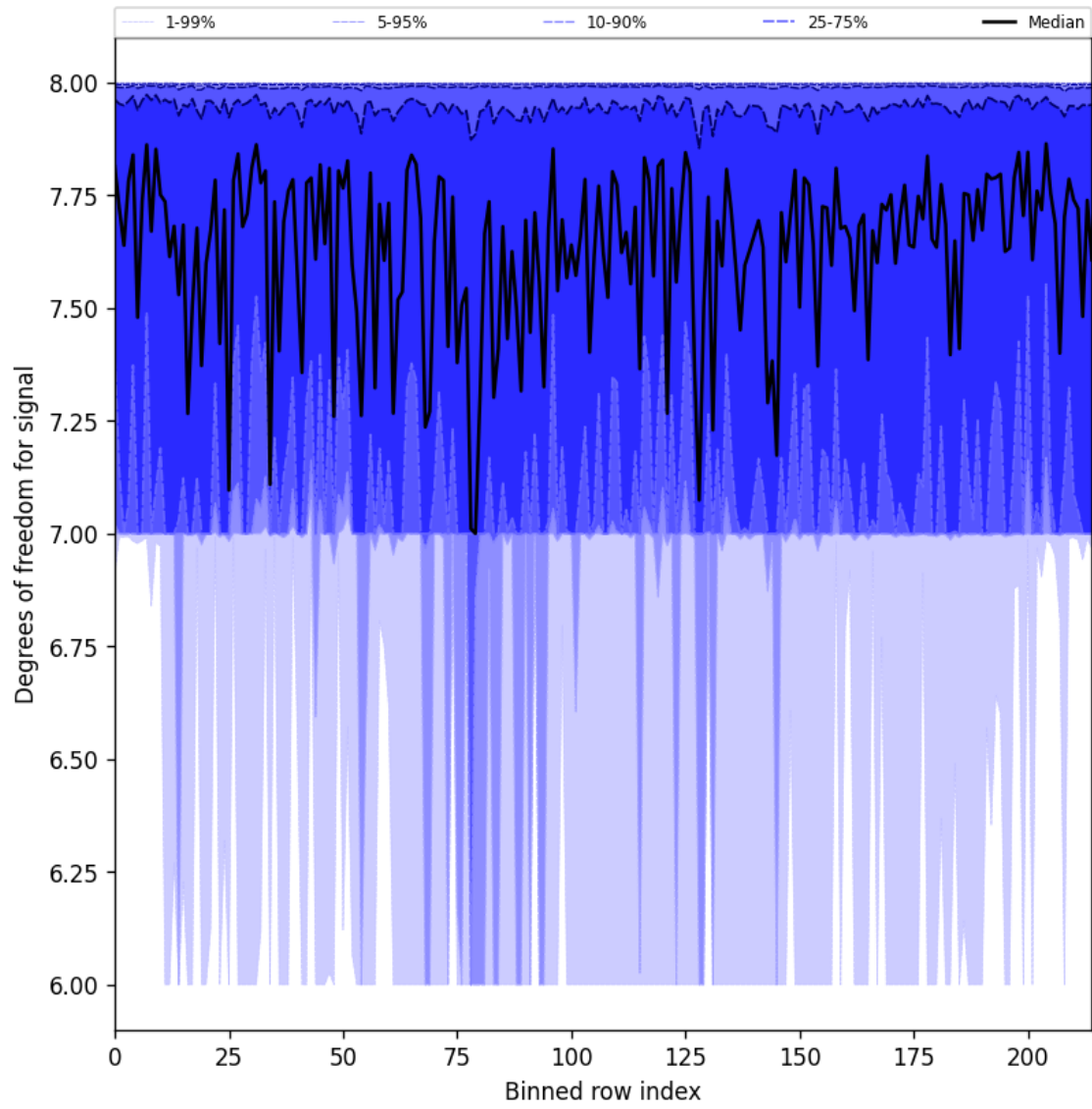
Figure 25: Along track statistics of “Degrees of freedom for signal” for 2025-07-15 to 2025-07-16
