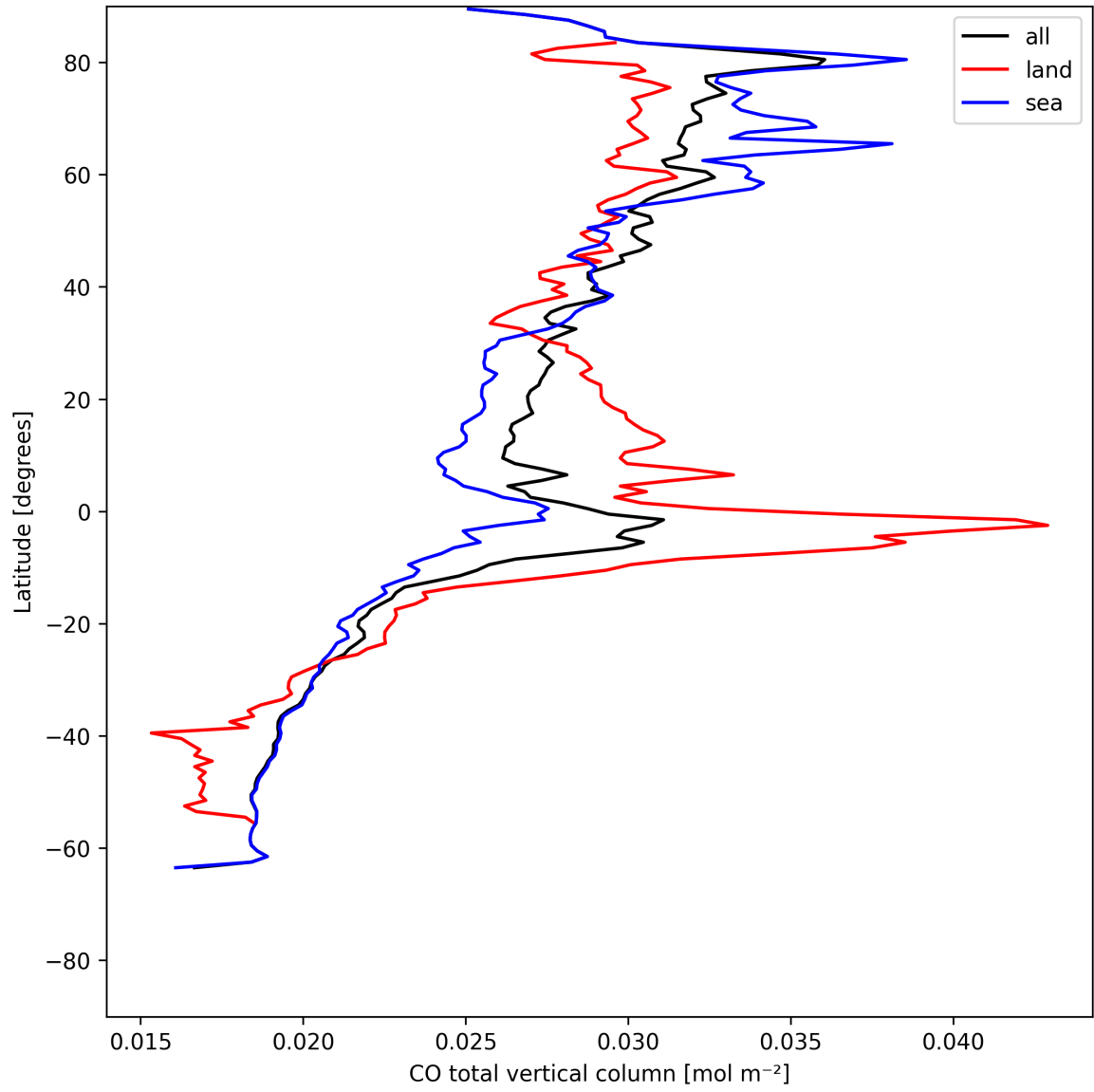
Figure 7: Zonal average of “CO total vertical column” for 2025-07-15 to 2025-07-16.
