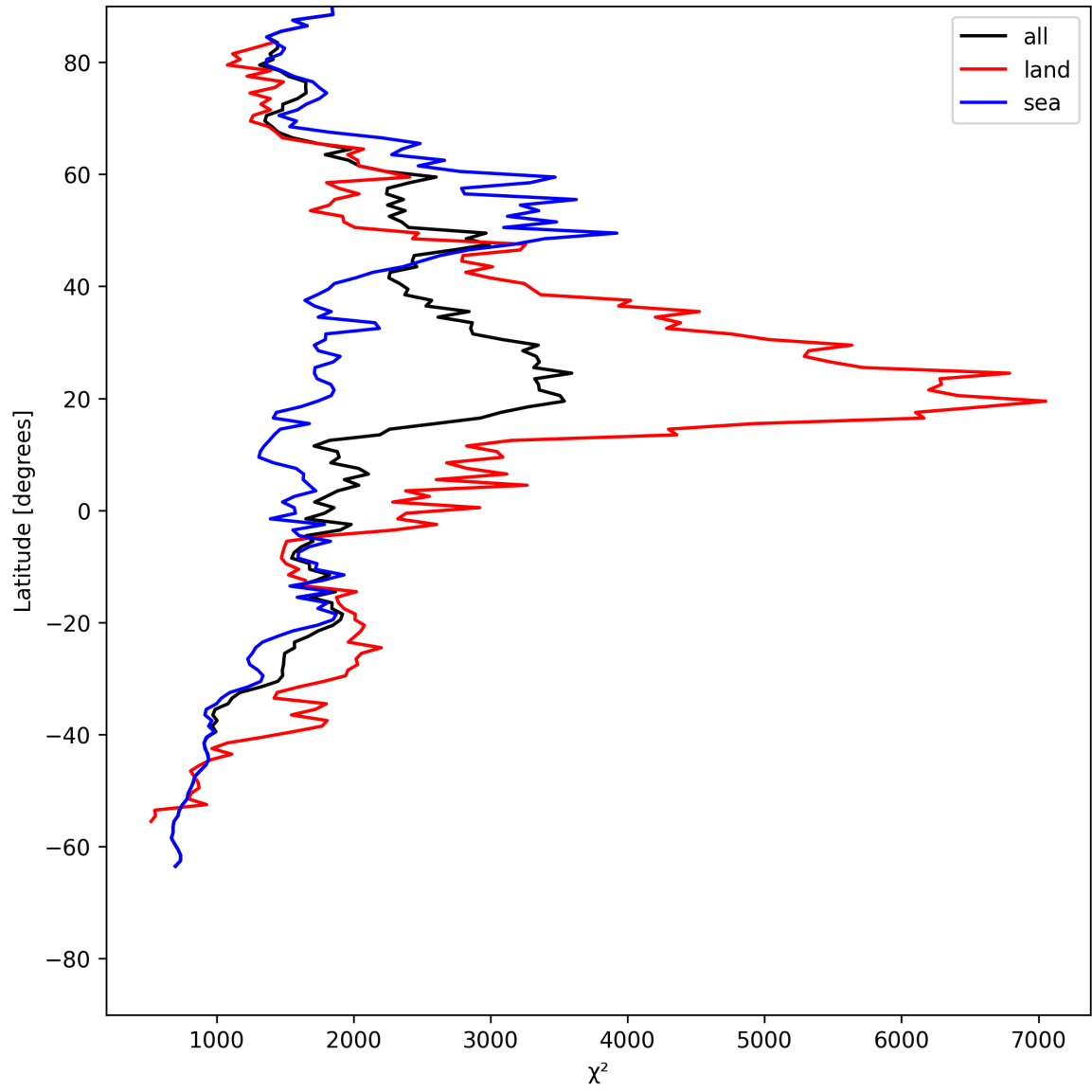
Figure 10: Zonal average of “ \chi^2 ” for 2025-07-15 to 2025-07-16.
