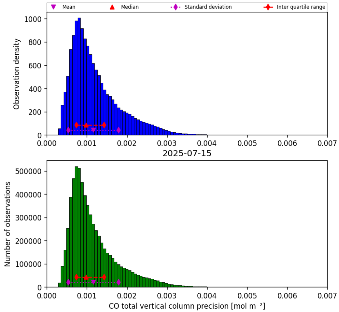
Figure 15: Histogram of “CO total vertical column precision” for 2025-07-15 to 2025-07-16
