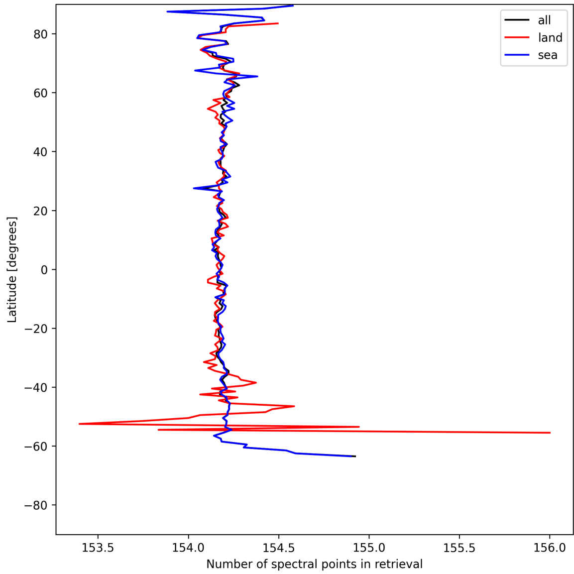
Figure 9: Zonal average of “Number of spectral points in retrieval” for 2025-07-15 to 2025-07-16.
