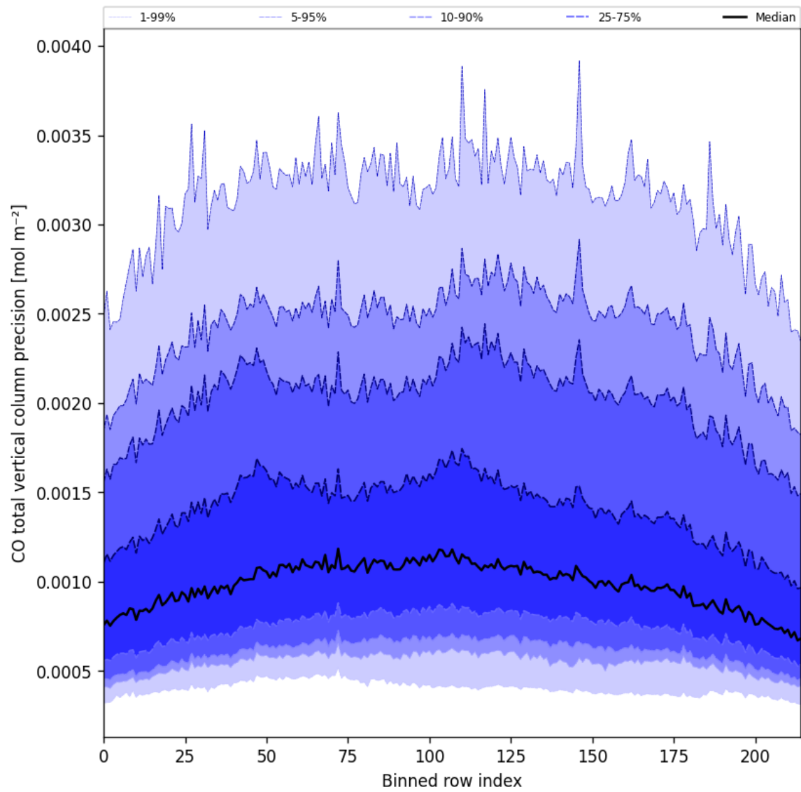
Figure 22: Along track statistics of “CO total vertical column precision” for 2025-07-15 to 2025-07-16
