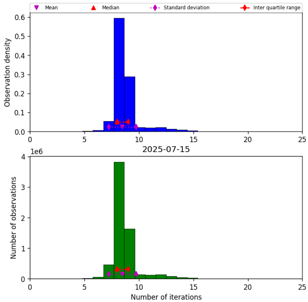
Figure 19: Histogram of “Number of iterations” for 2025-07-15 to 2025-07-16
