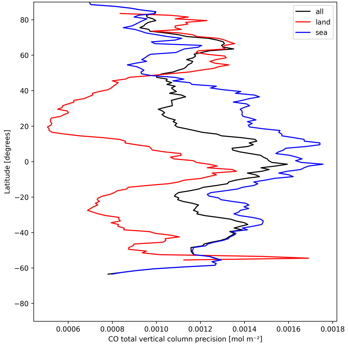
Figure 8: Zonal average of “CO total vertical column precision” for 2025-07-15 to 2025-07-16.
