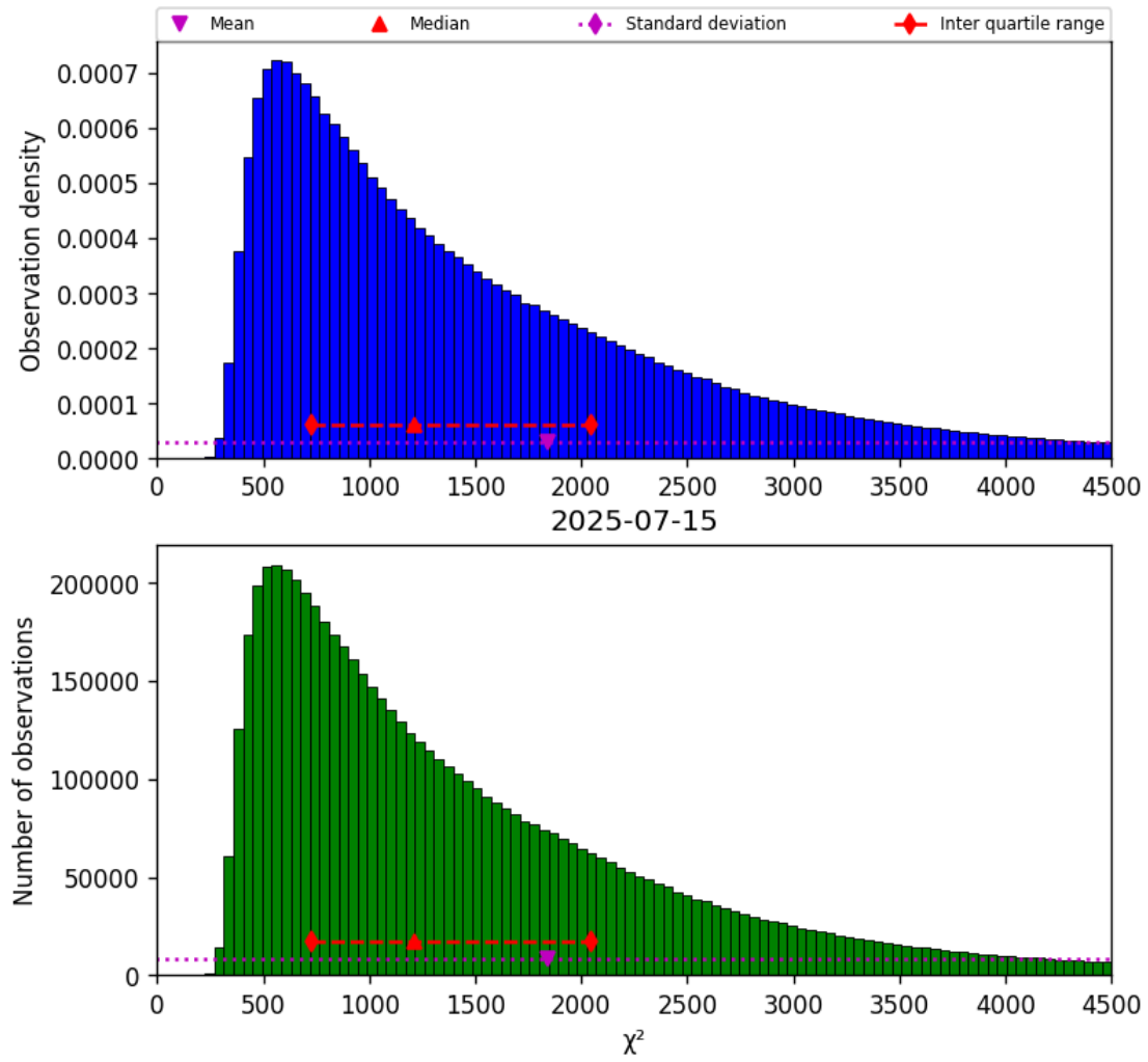
Figure 17: Histogram of “ \chi^2 ” for 2025-07-15 to 2025-07-16
