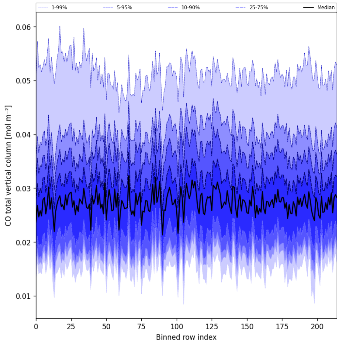
Figure 21: Along track statistics of “CO total vertical column” for 2025-07-15 to 2025-07-16
