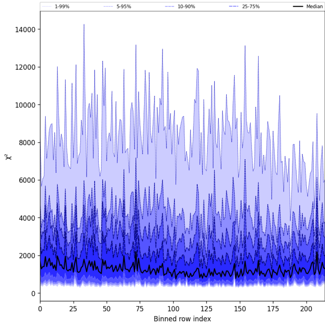
Figure 24: Along track statistics of “ \chi^2 ” for 2025-07-15 to 2025-07-16
