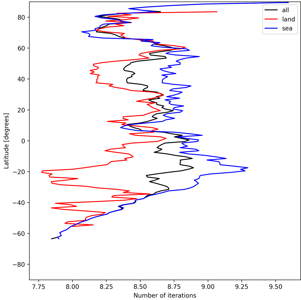
Figure 12: Zonal average of “Number of iterations” for 2025-07-15 to 2025-07-16.
