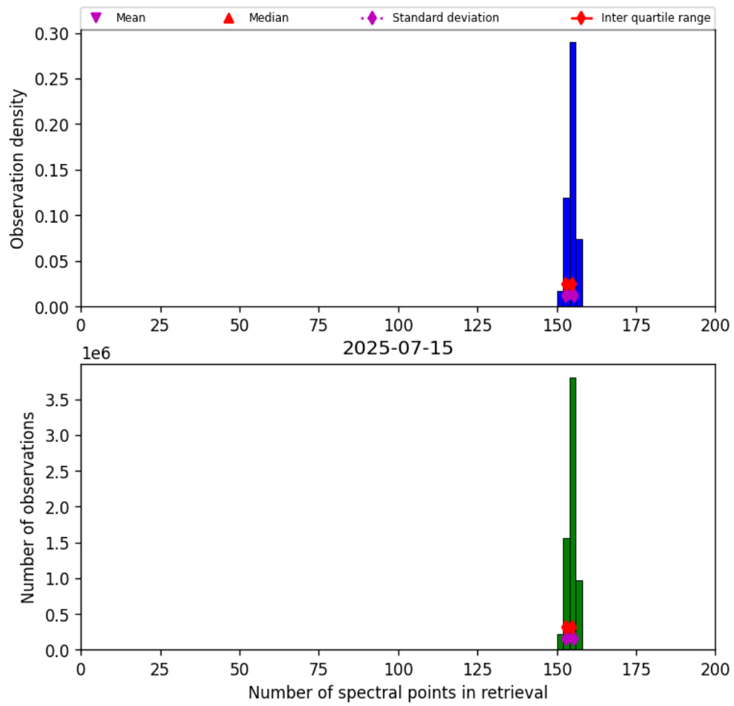
Figure 16: Histogram of “Number of spectral points in retrieval” for 2025-07-15 to 2025-07-16
