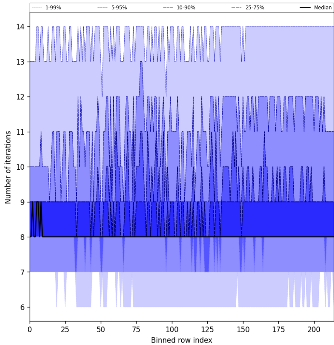
Figure 26: Along track statistics of “Number of iterations” for 2025-07-15 to 2025-07-16
