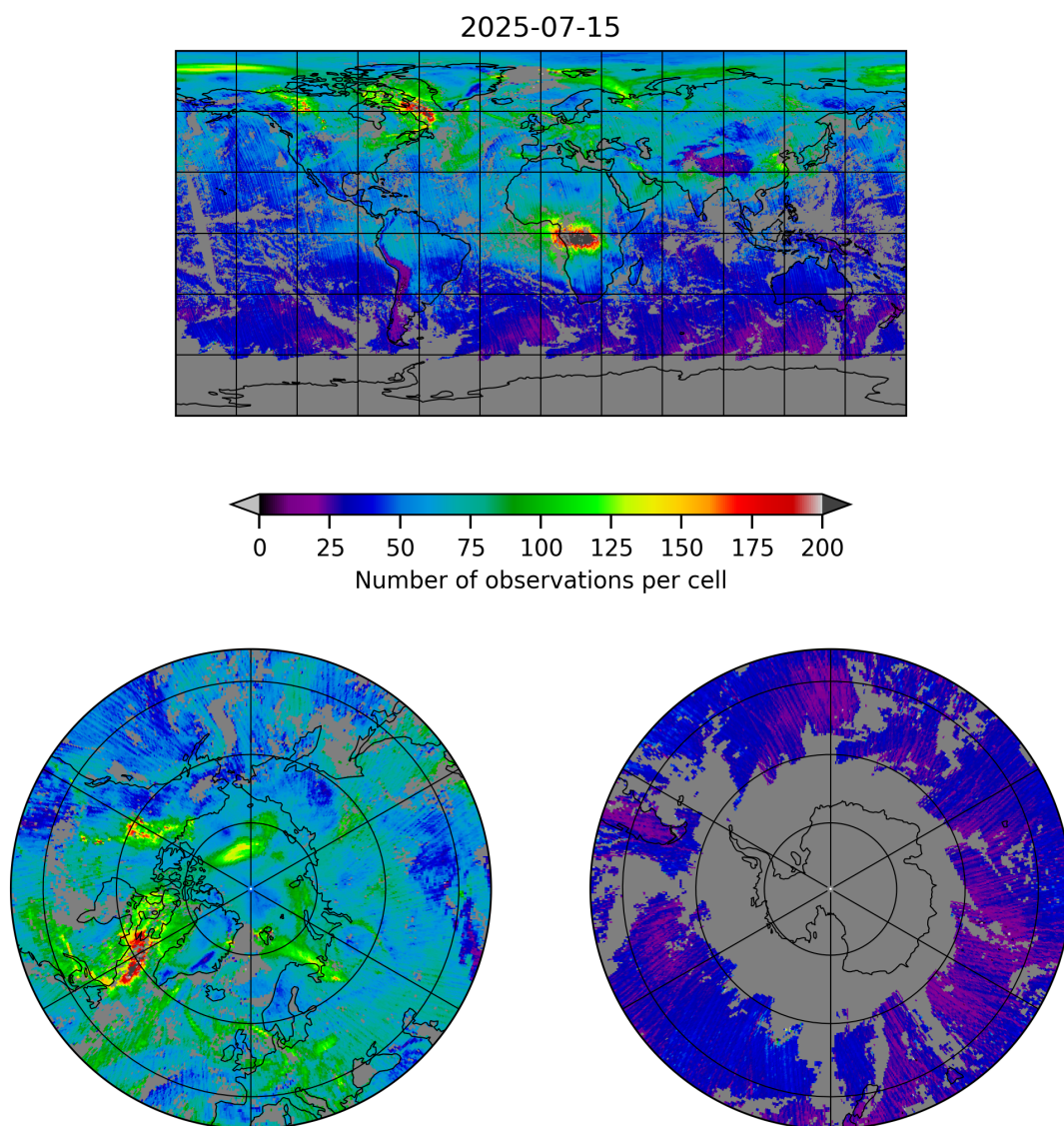
Figure 5: Map of the number of observations for 2025-07-15 to 2025-07-16
