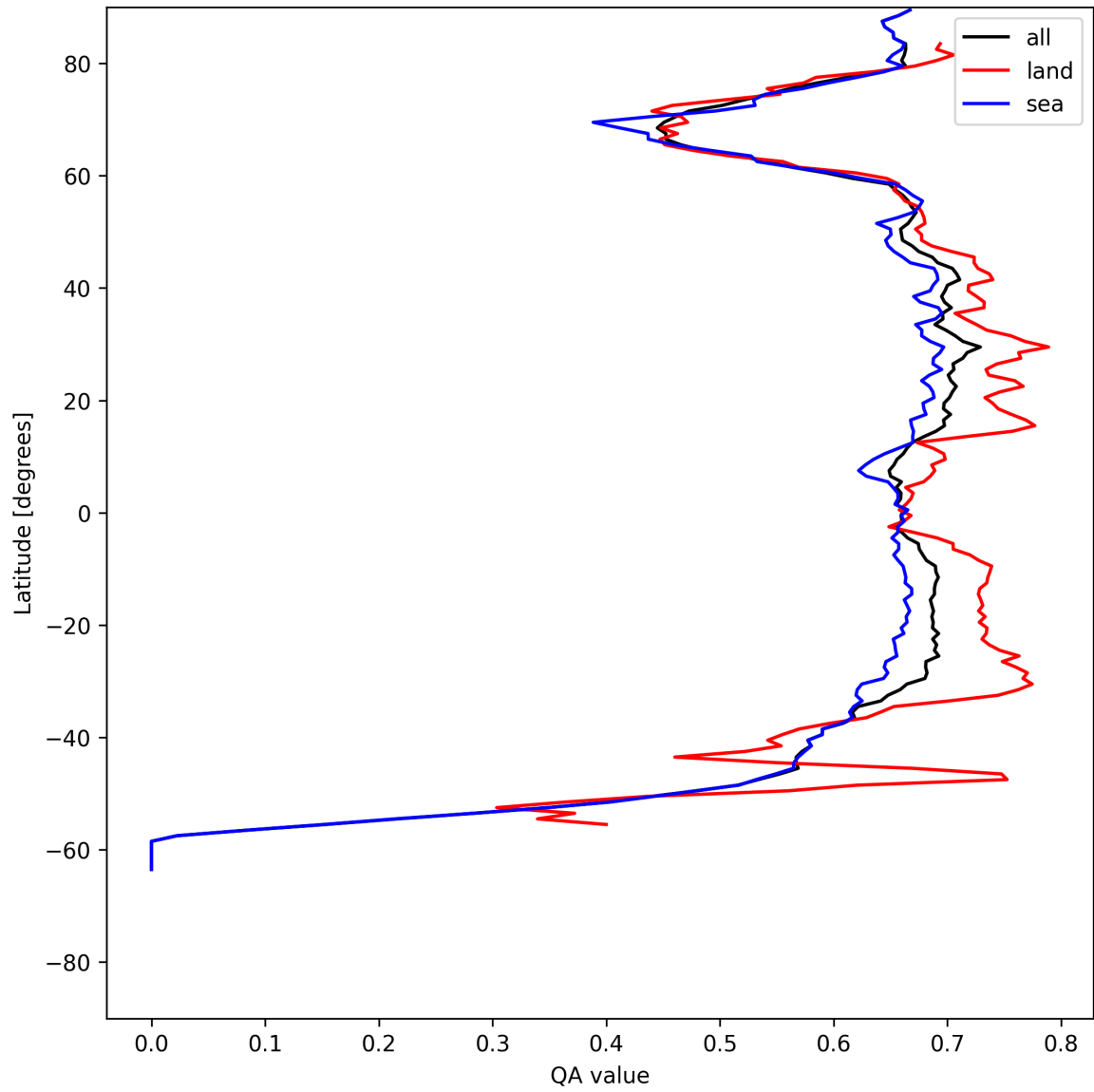
Figure 6: Zonal average of “QA value” for 2025-07-15 to 2025-07-16.
