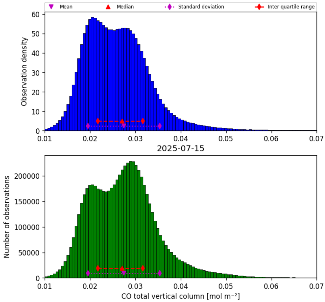
Figure 14: Histogram of “CO total vertical column” for 2025-07-15 to 2025-07-16
