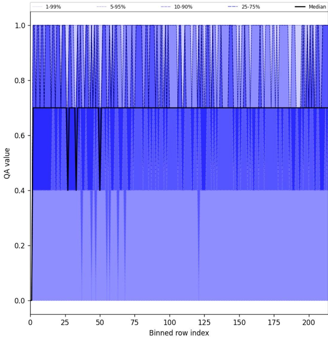
Figure 20: Along track statistics of “QA value” for 2025-07-15 to 2025-07-16
