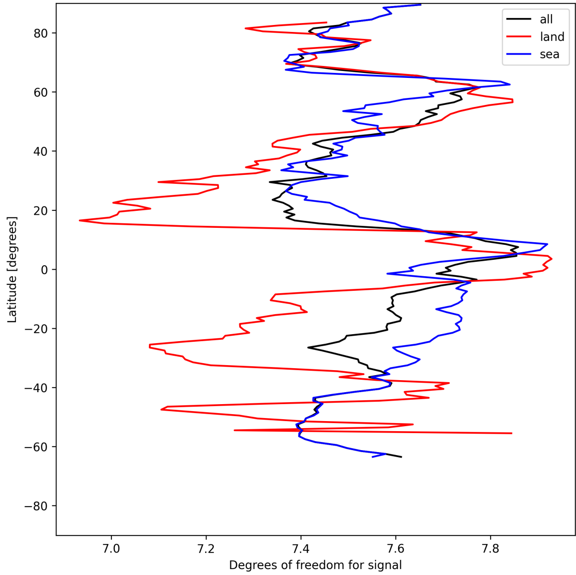
Figure 11: Zonal average of “Degrees of freedom for signal” for 2025-07-15 to 2025-07-16.
