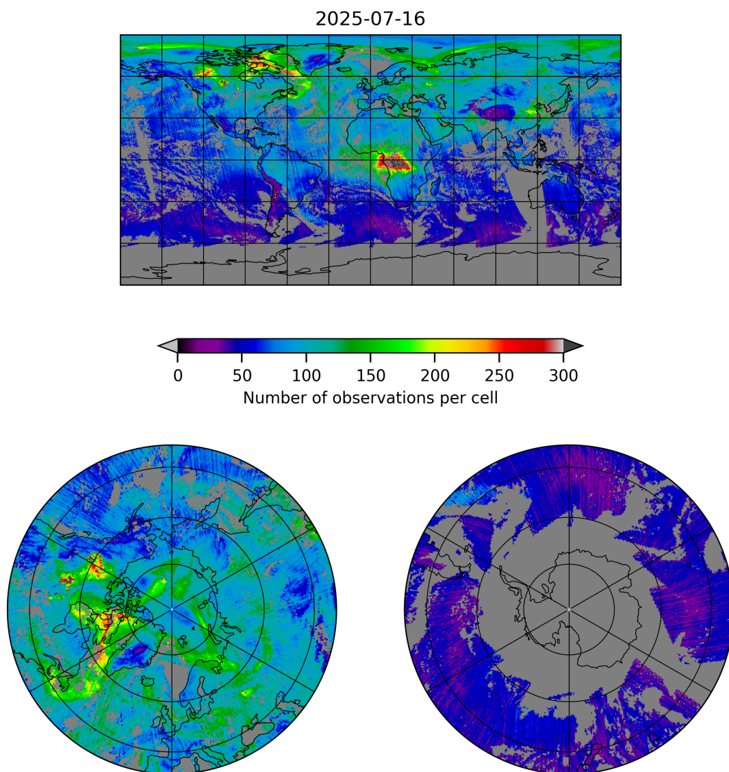
Figure 5: Map of the number of observations for 2025-07-16 to 2025-07-16
