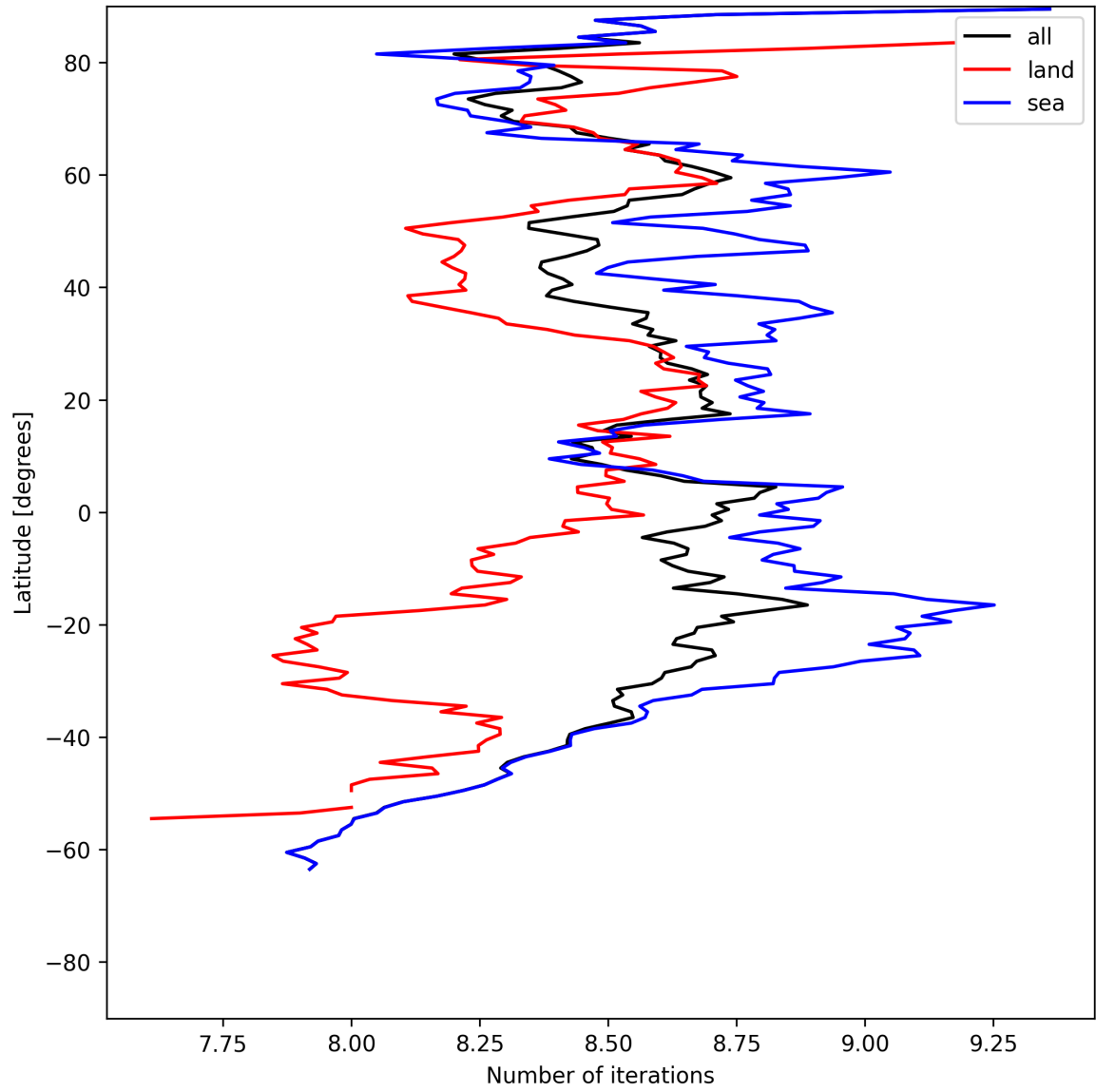
Figure 12: Zonal average of “Number of iterations” for 2025-07-16 to 2025-07-16.
