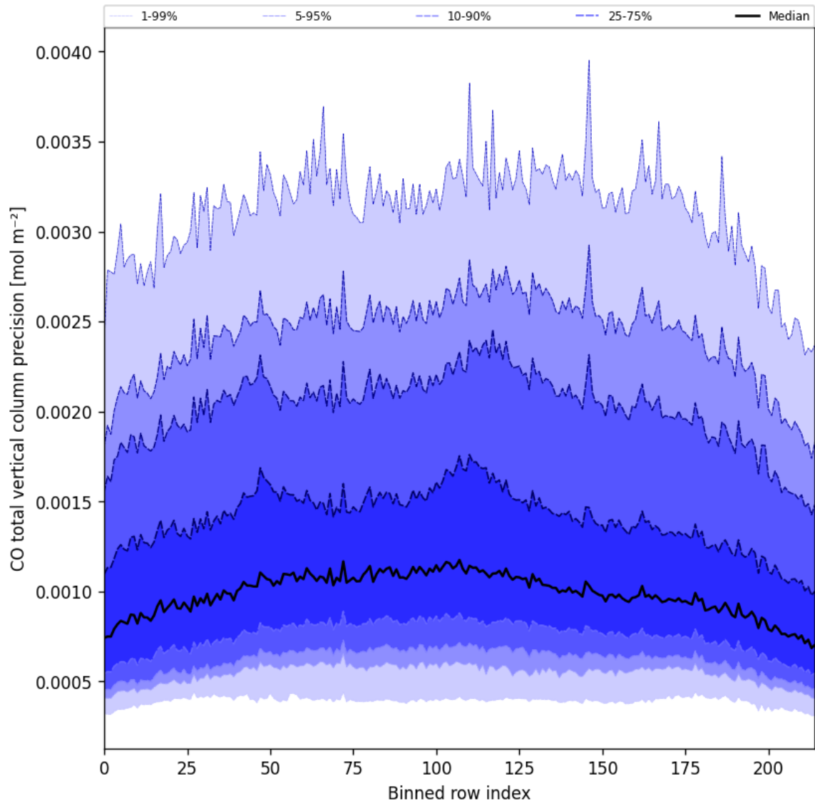
Figure 22: Along track statistics of “CO total vertical column precision” for 2025-07-16 to 2025-07-16
