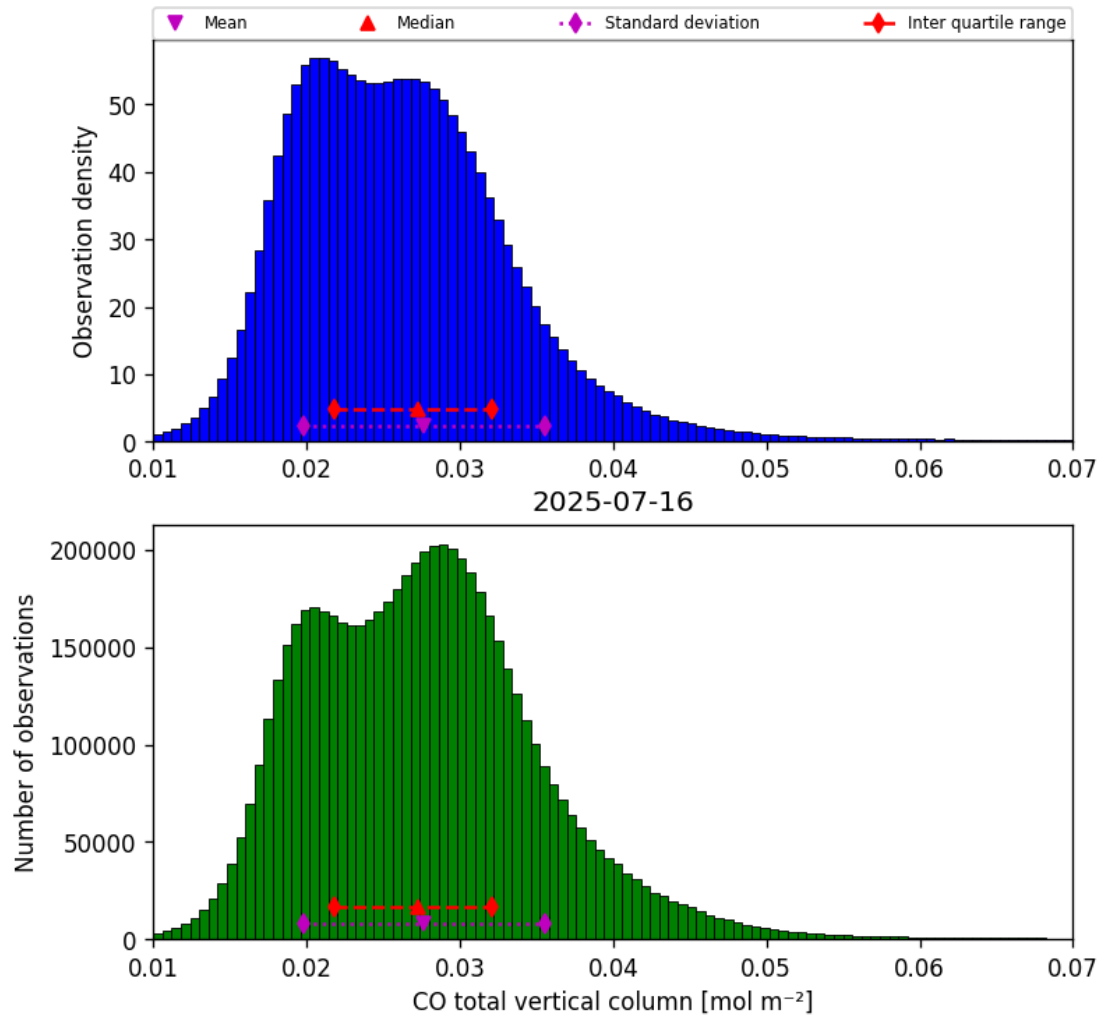
Figure 14: Histogram of “CO total vertical column” for 2025-07-16 to 2025-07-16
