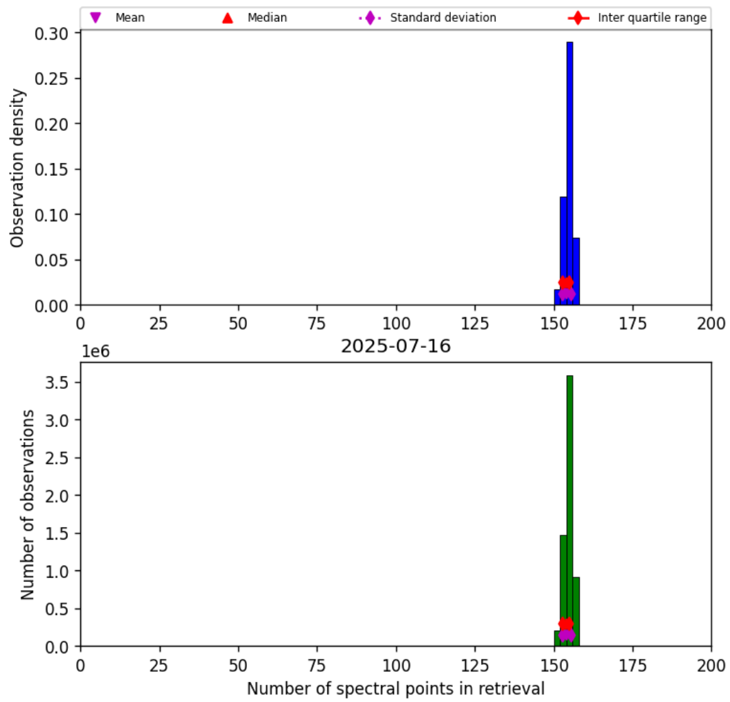
Figure 16: Histogram of “Number of spectral points in retrieval” for 2025-07-16 to 2025-07-16
