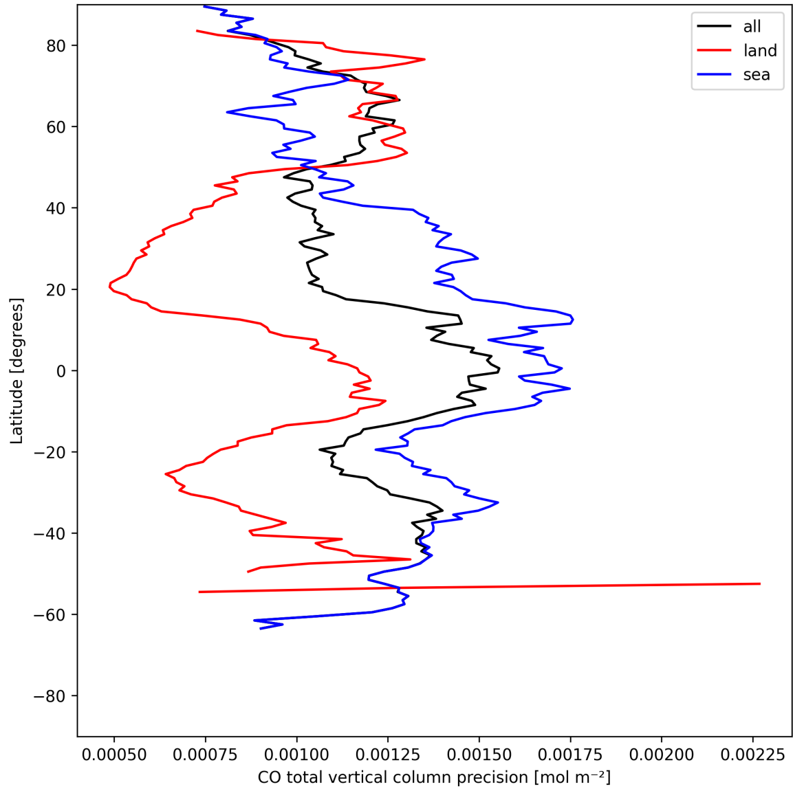
Figure 8: Zonal average of “CO total vertical column precision” for 2025-07-16 to 2025-07-16.
