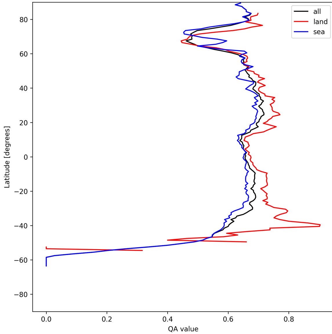
Figure 6: Zonal average of “QA value” for 2025-07-16 to 2025-07-16.
