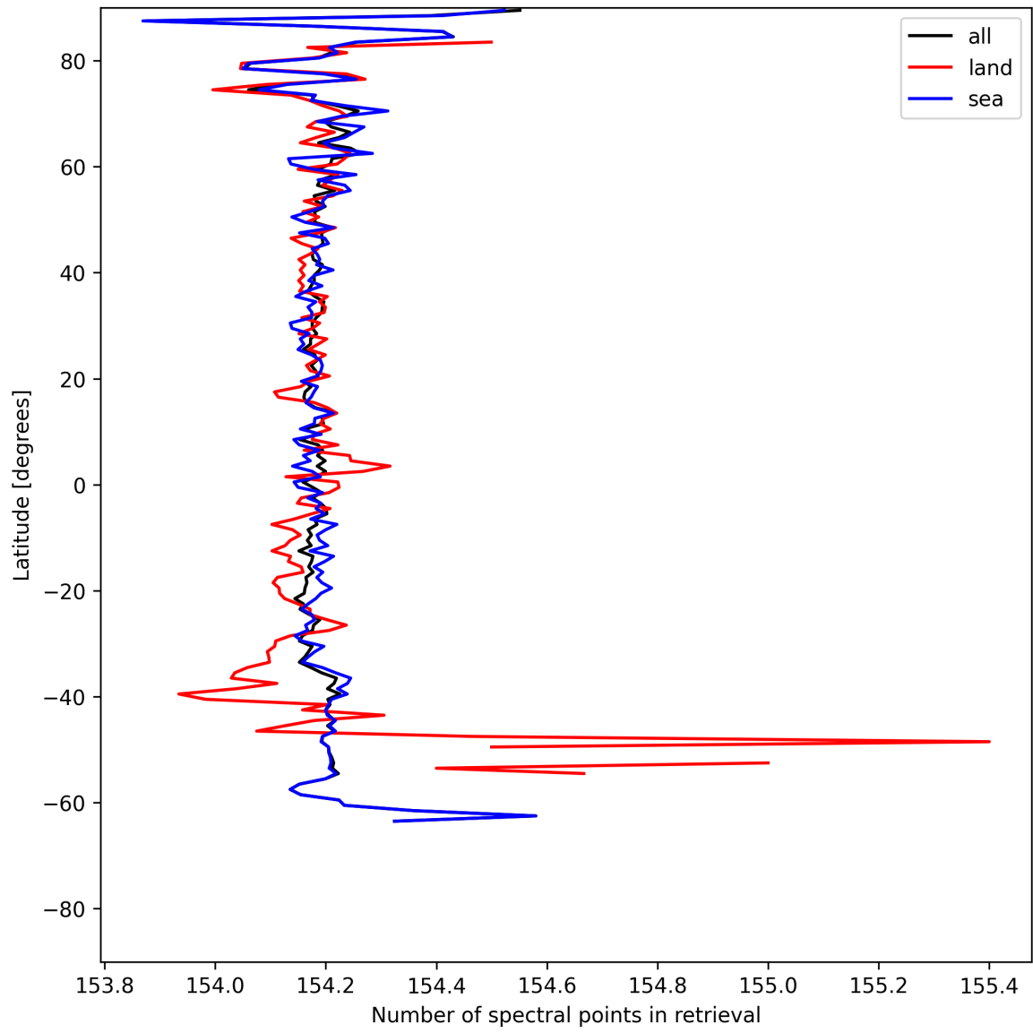
Figure 9: Zonal average of “Number of spectral points in retrieval” for 2025-07-16 to 2025-07-16.
