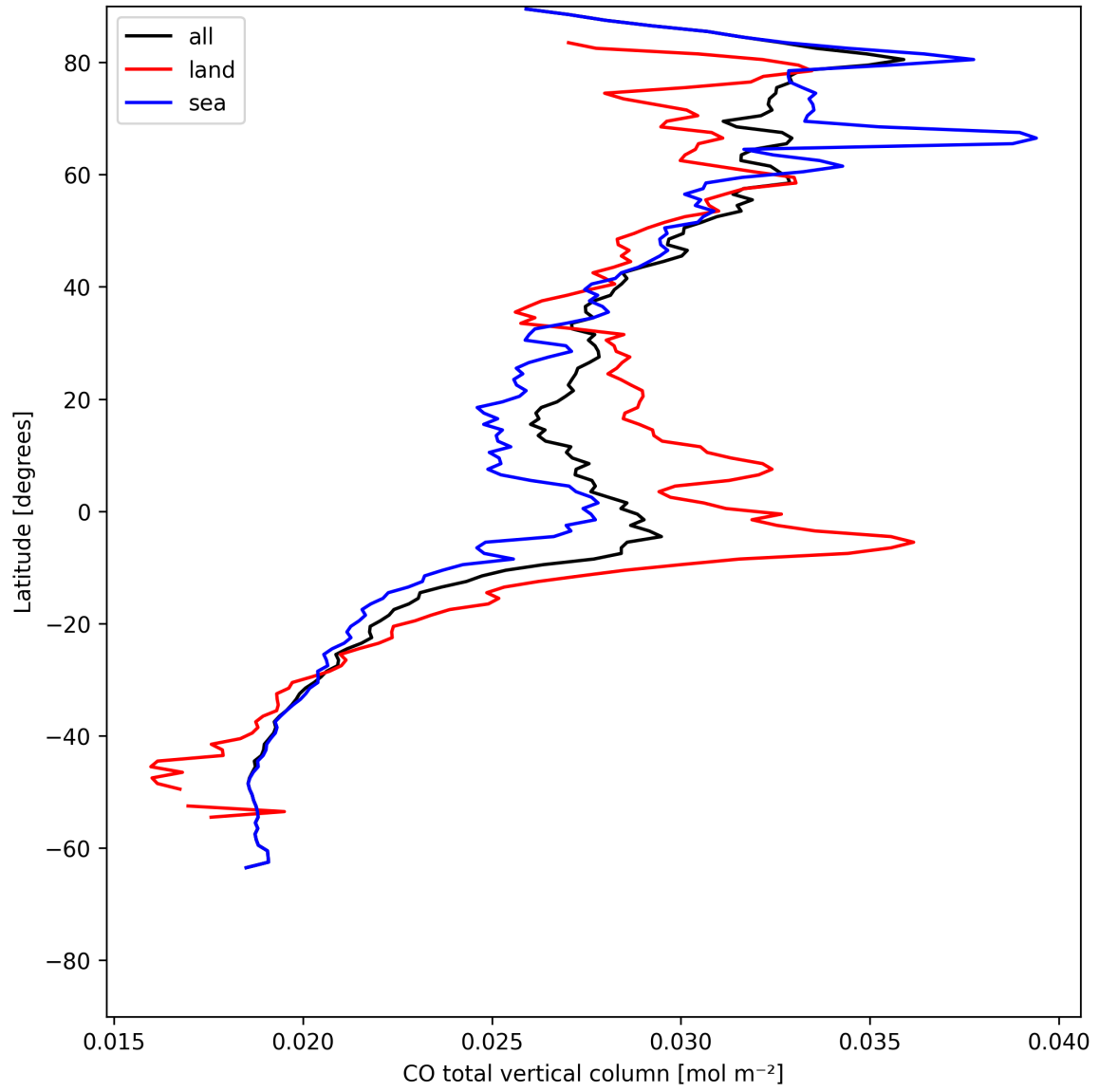
Figure 7: Zonal average of “CO total vertical column” for 2025-07-16 to 2025-07-16.
