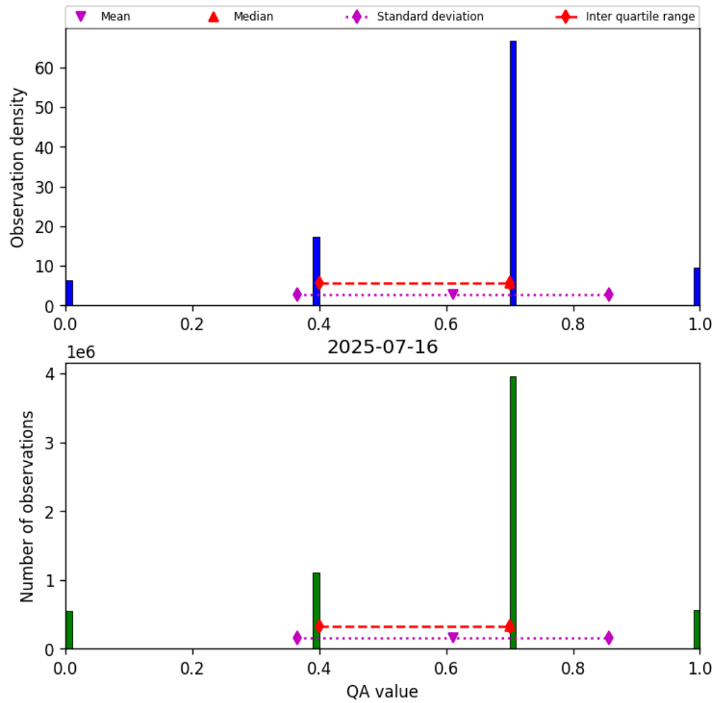
Figure 13: Histogram of “QA value” for 2025-07-16 to 2025-07-16
