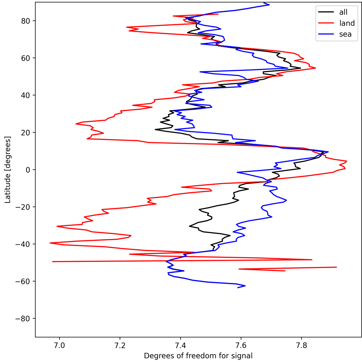
Figure 11: Zonal average of “Degrees of freedom for signal” for 2025-07-16 to 2025-07-16.
