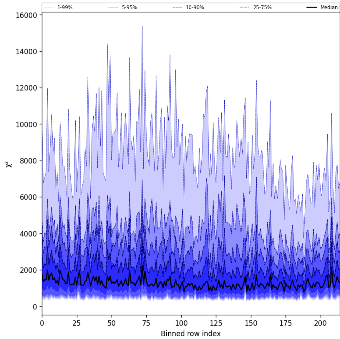
Figure 24: Along track statistics of “ \chi^2 ” for 2025-07-16 to 2025-07-16
