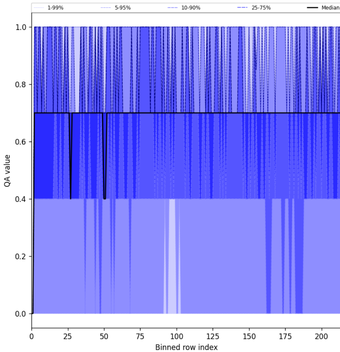
Figure 20: Along track statistics of “QA value” for 2025-07-16 to 2025-07-16
