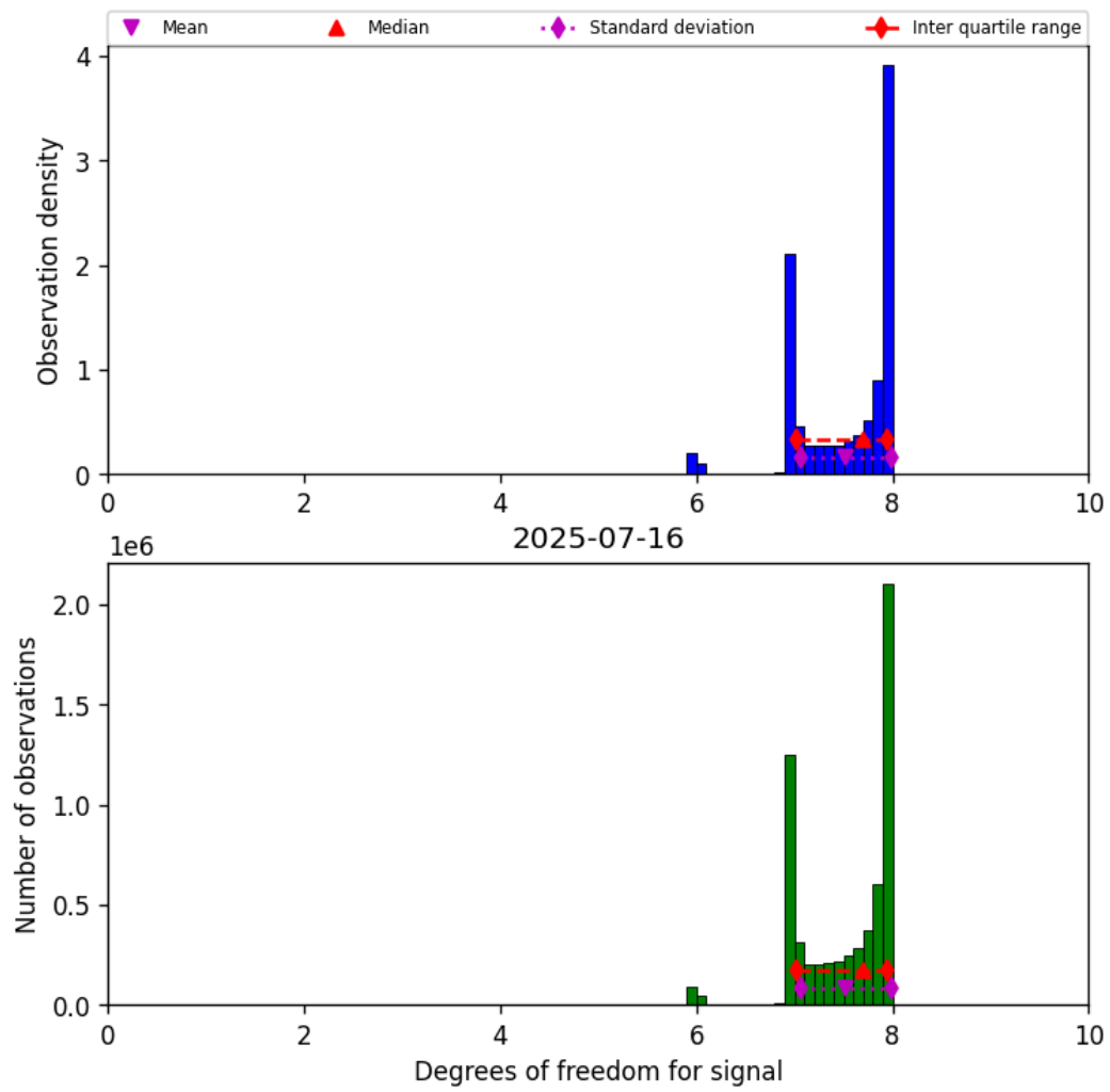
Figure 18: Histogram of “Degrees of freedom for signal” for 2025-07-16 to 2025-07-16
