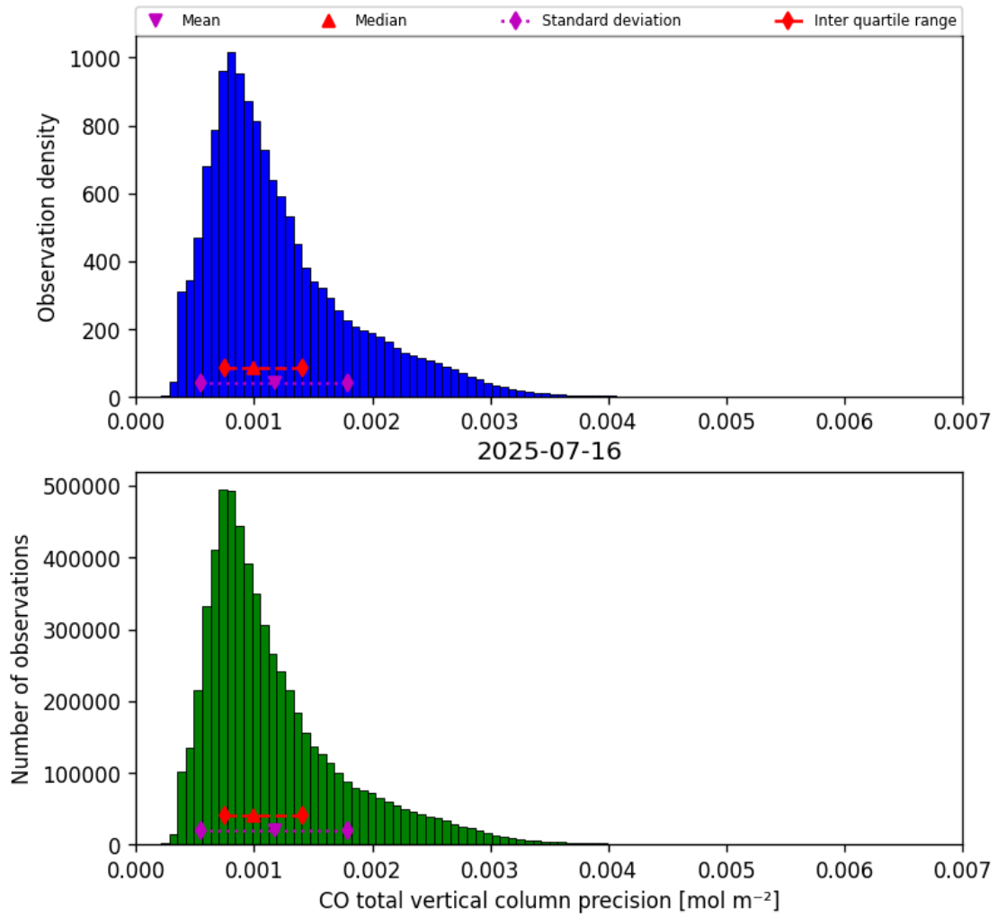
Figure 15: Histogram of “CO total vertical column precision” for 2025-07-16 to 2025-07-16
