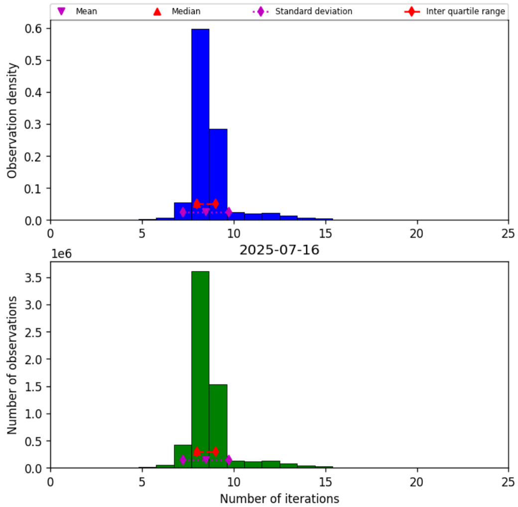
Figure 19: Histogram of “Number of iterations” for 2025-07-16 to 2025-07-16
