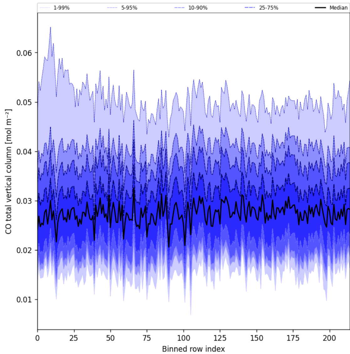
Figure 21: Along track statistics of “CO total vertical column” for 2025-07-16 to 2025-07-16
