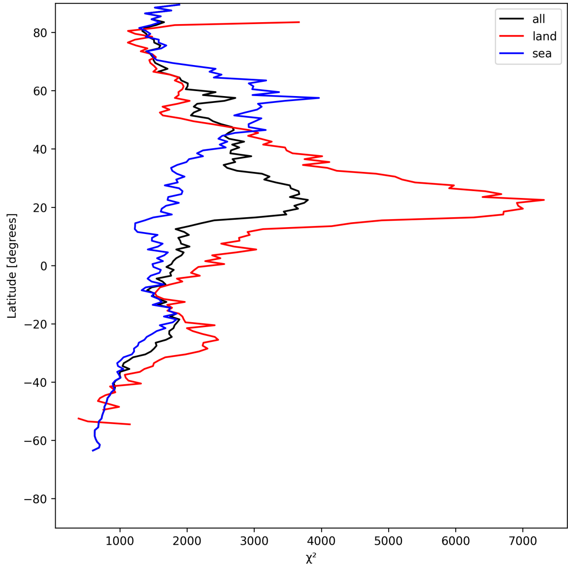
Figure 10: Zonal average of “ \chi^2 ” for 2025-07-16 to 2025-07-16.
