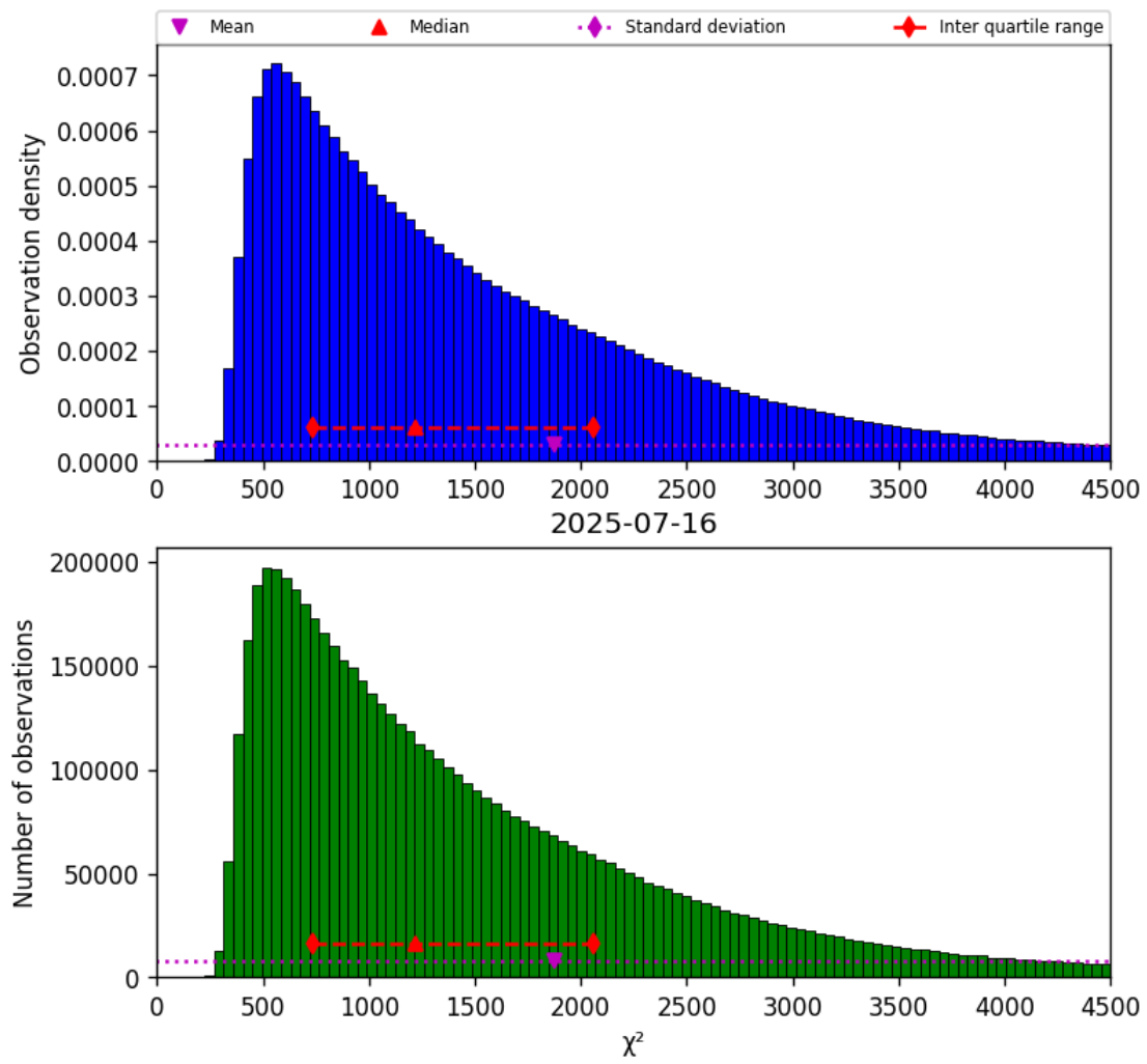
Figure 17: Histogram of “ \chi^2 ” for 2025-07-16 to 2025-07-16
