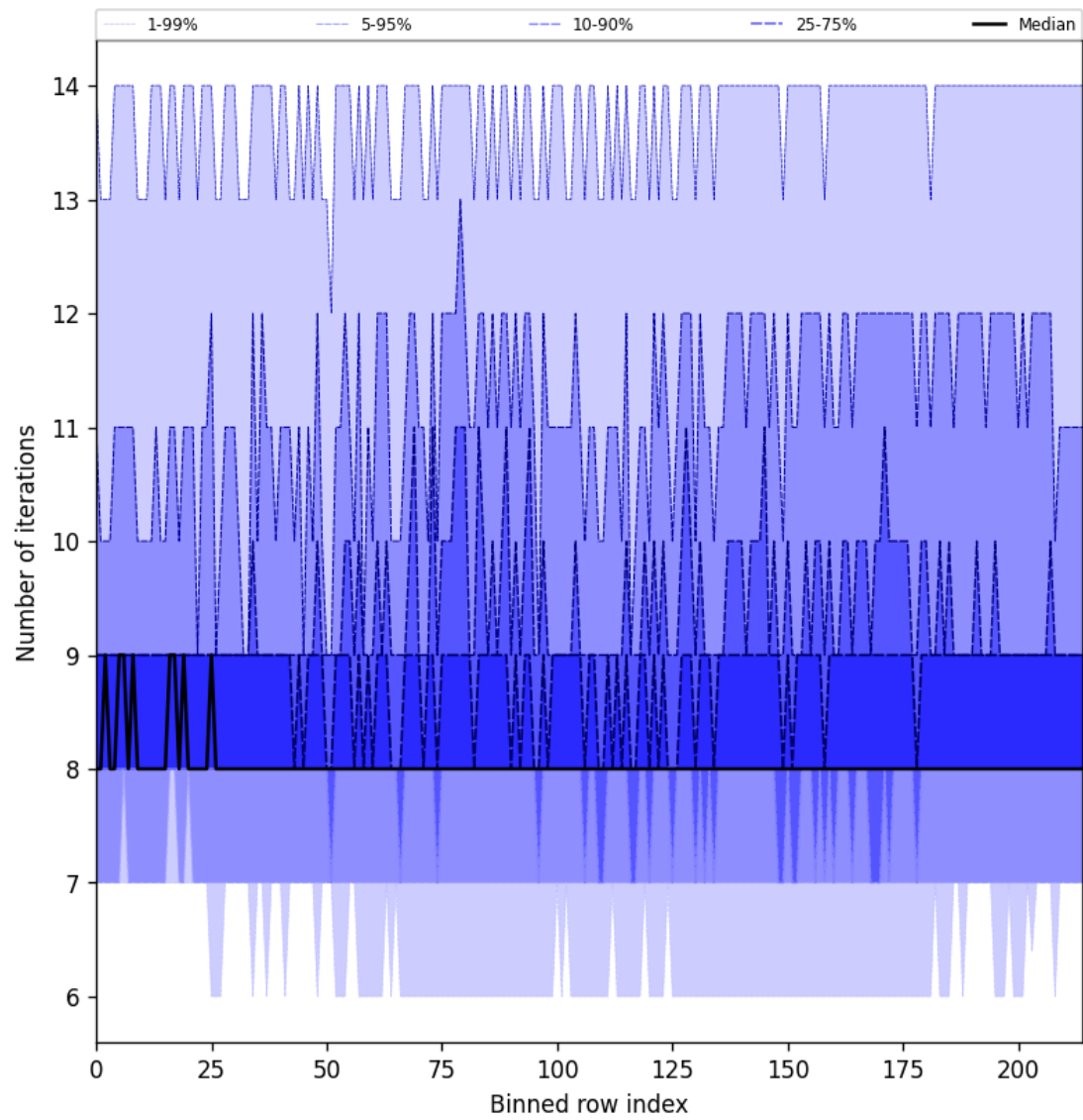
Figure 26: Along track statistics of “Number of iterations” for 2025-07-16 to 2025-07-16
