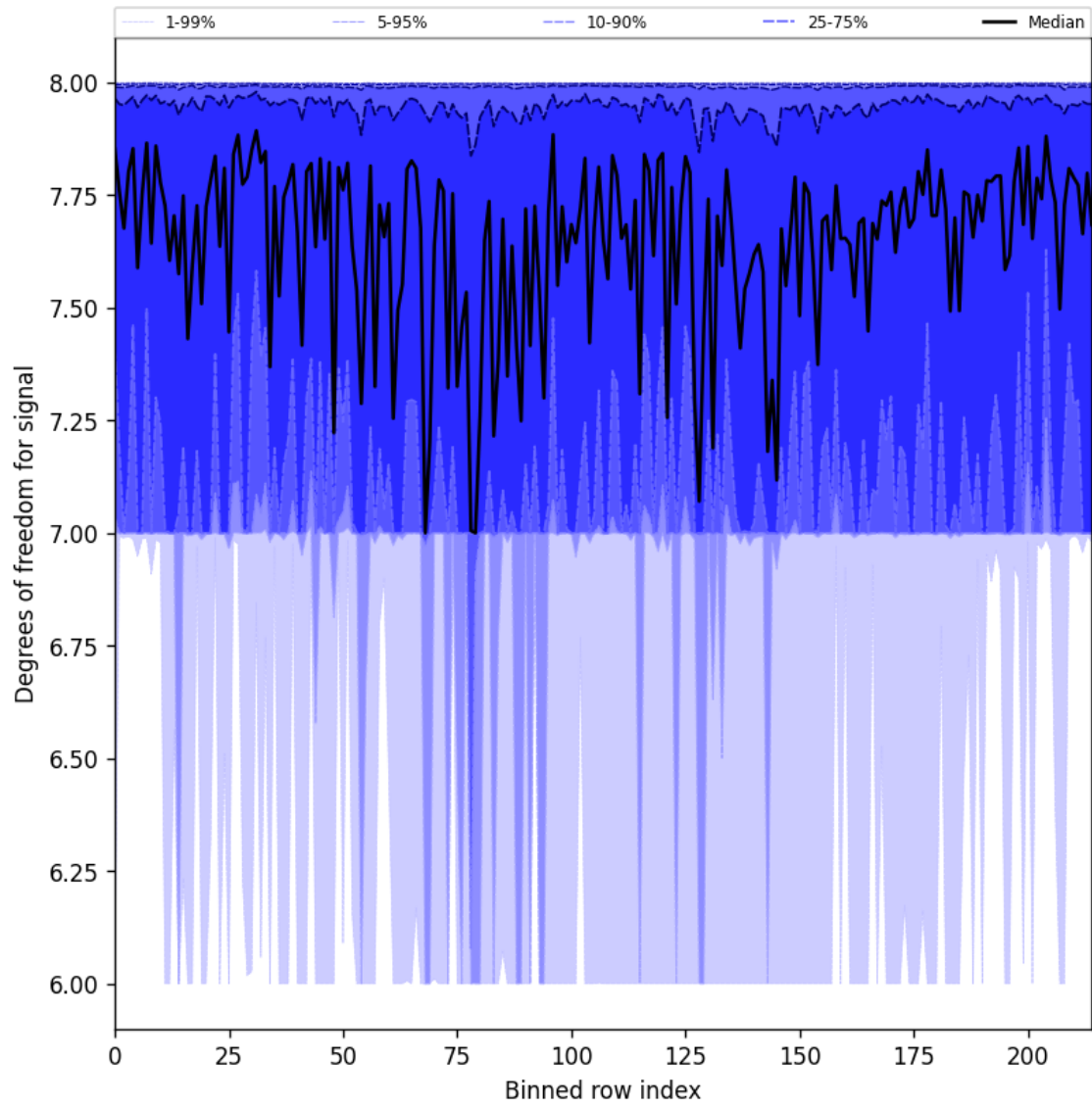
Figure 25: Along track statistics of “Degrees of freedom for signal” for 2025-07-16 to 2025-07-16
