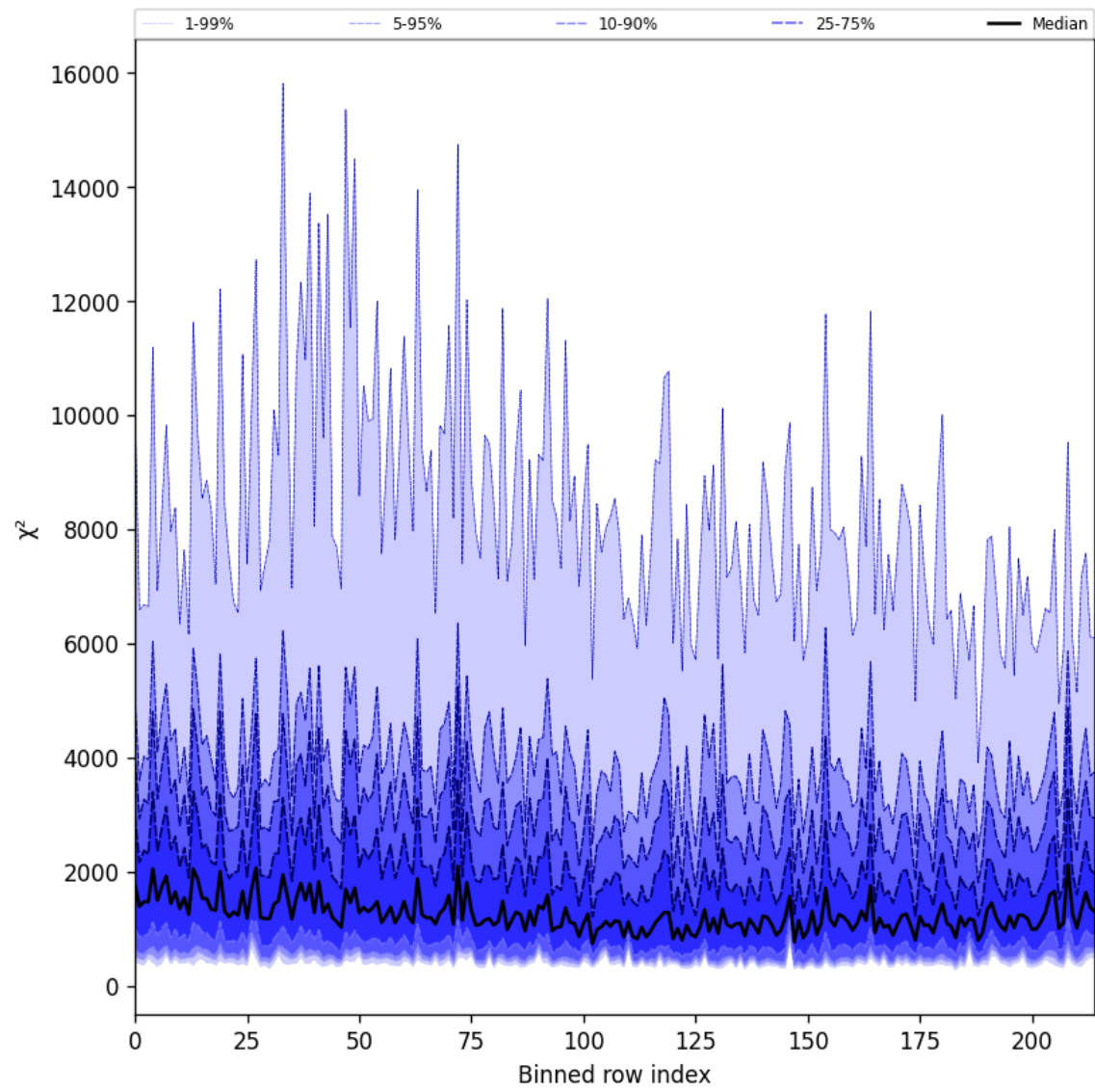
Figure 24: Along track statistics of “ \chi^2 ” for 2025-07-17 to 2025-07-18
