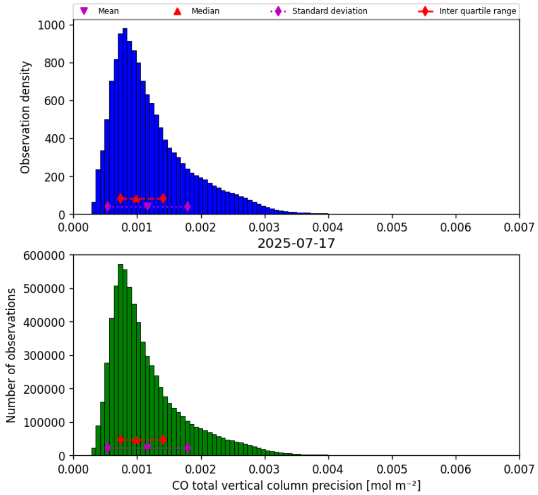
Figure 15: Histogram of “CO total vertical column precision” for 2025-07-17 to 2025-07-18
