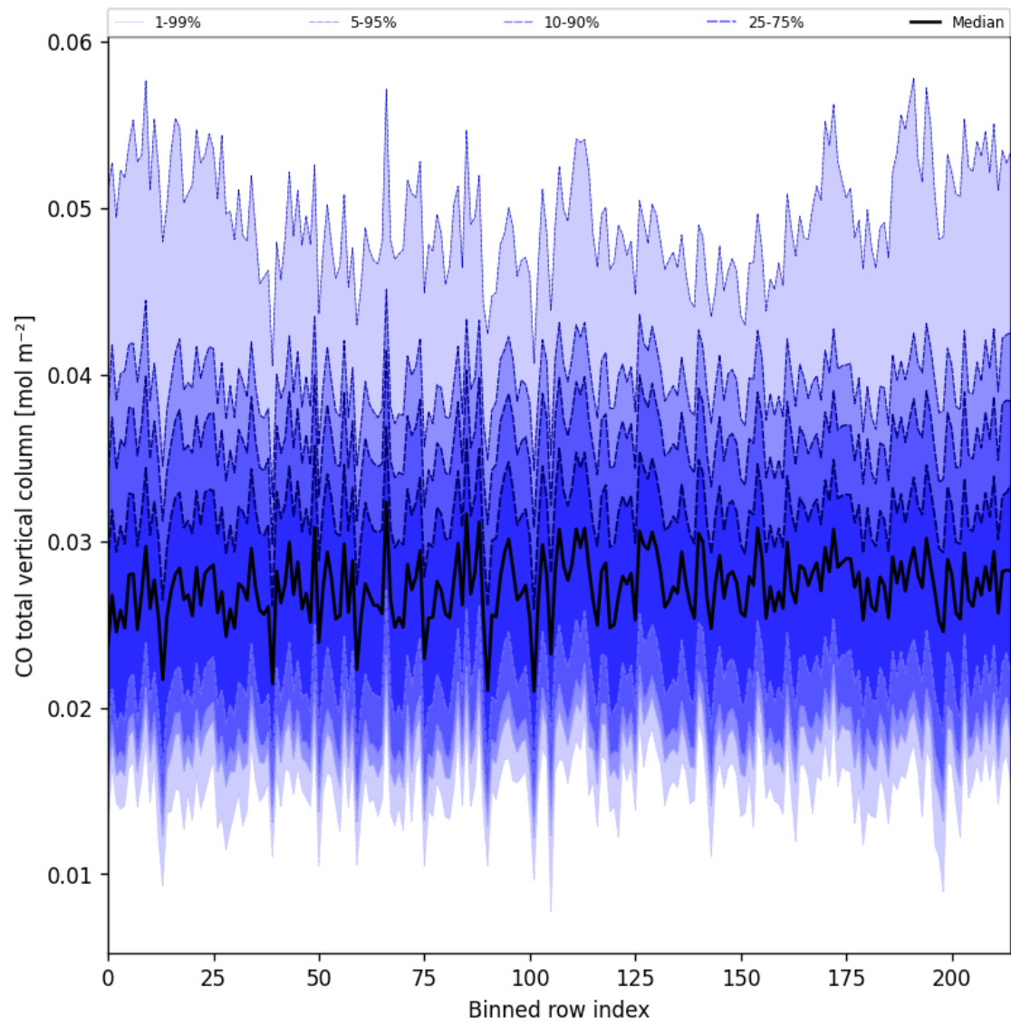
Figure 21: Along track statistics of “CO total vertical column” for 2025-07-17 to 2025-07-18
