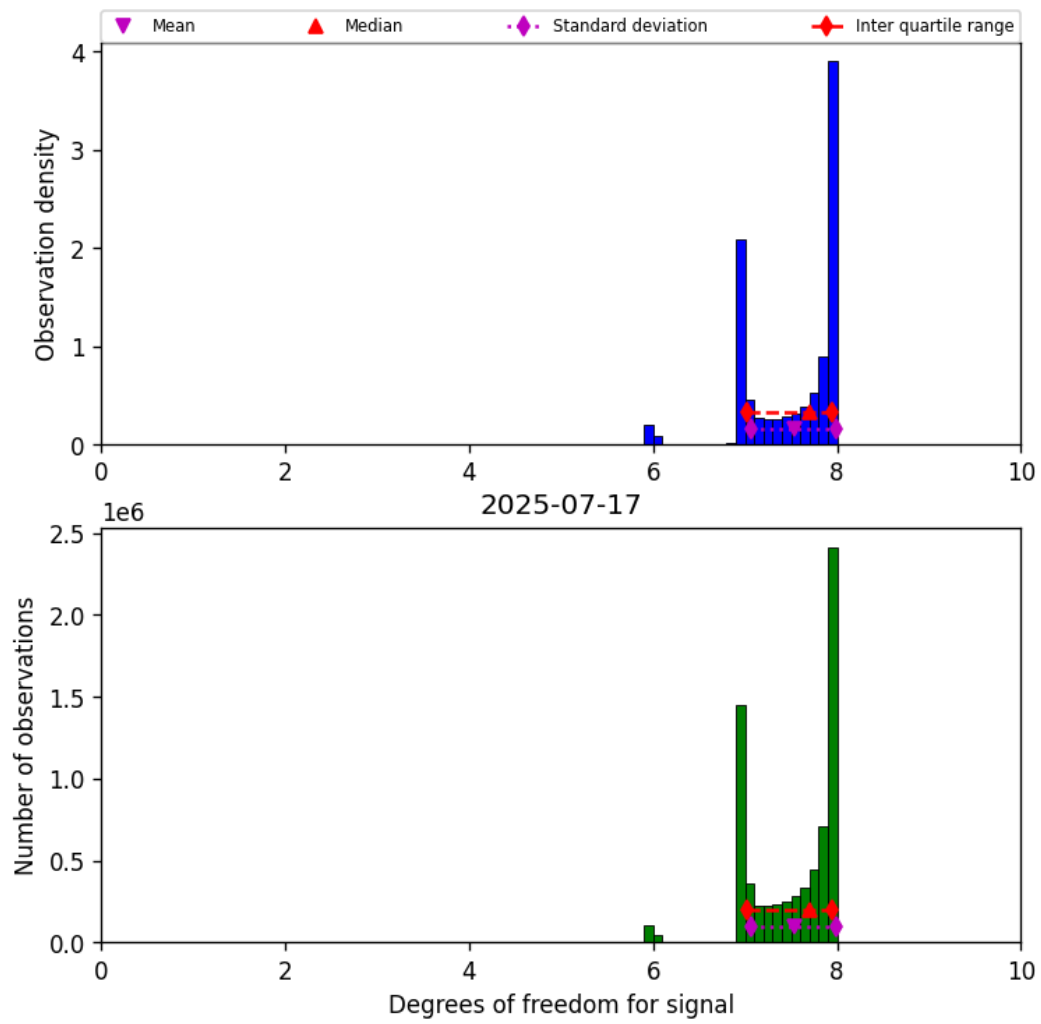
Figure 18: Histogram of “Degrees of freedom for signal” for 2025-07-17 to 2025-07-18
