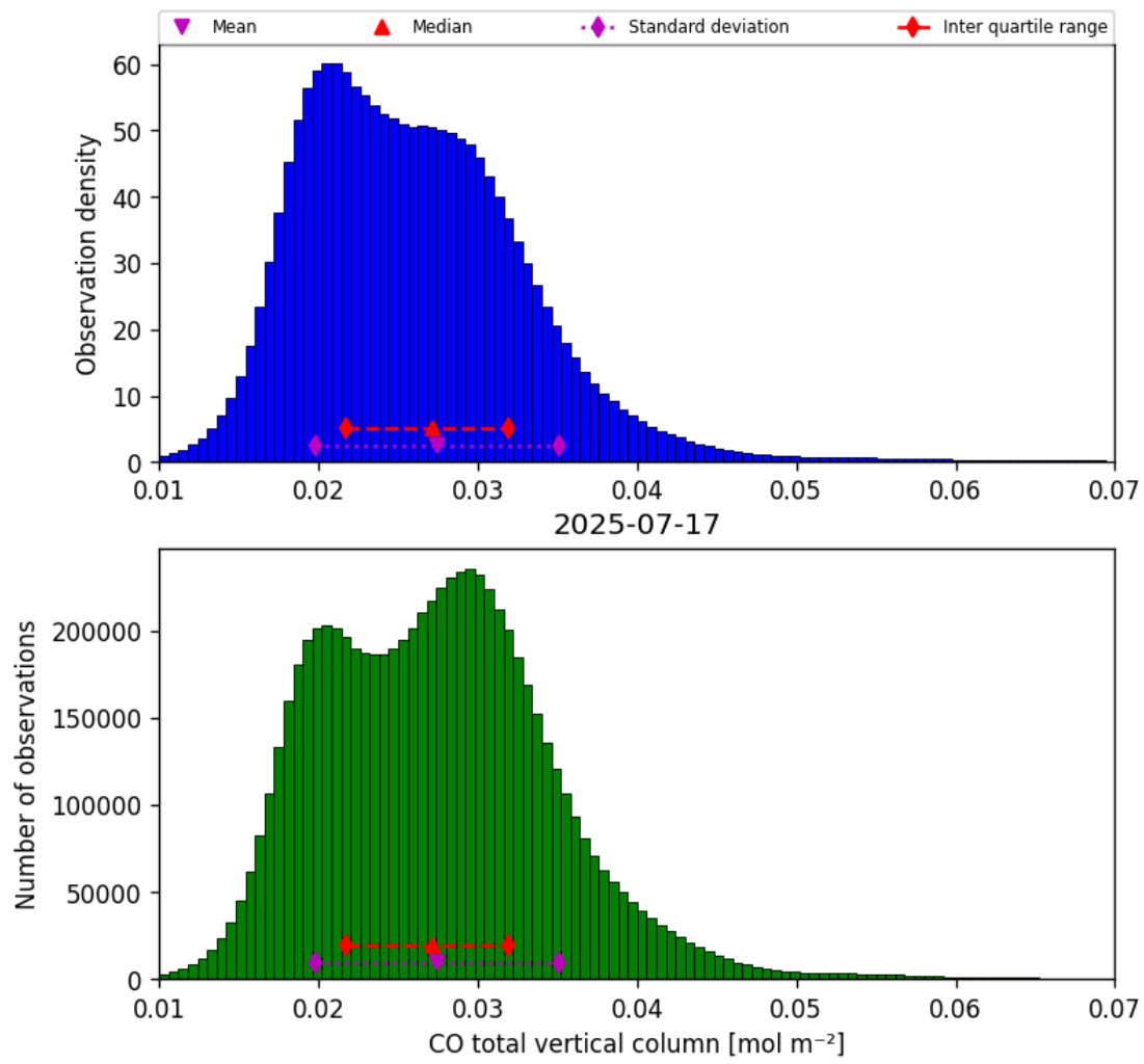
Figure 14: Histogram of “CO total vertical column” for 2025-07-17 to 2025-07-18
