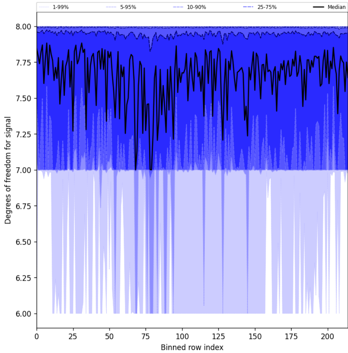
Figure 25: Along track statistics of “Degrees of freedom for signal” for 2025-07-17 to 2025-07-18
