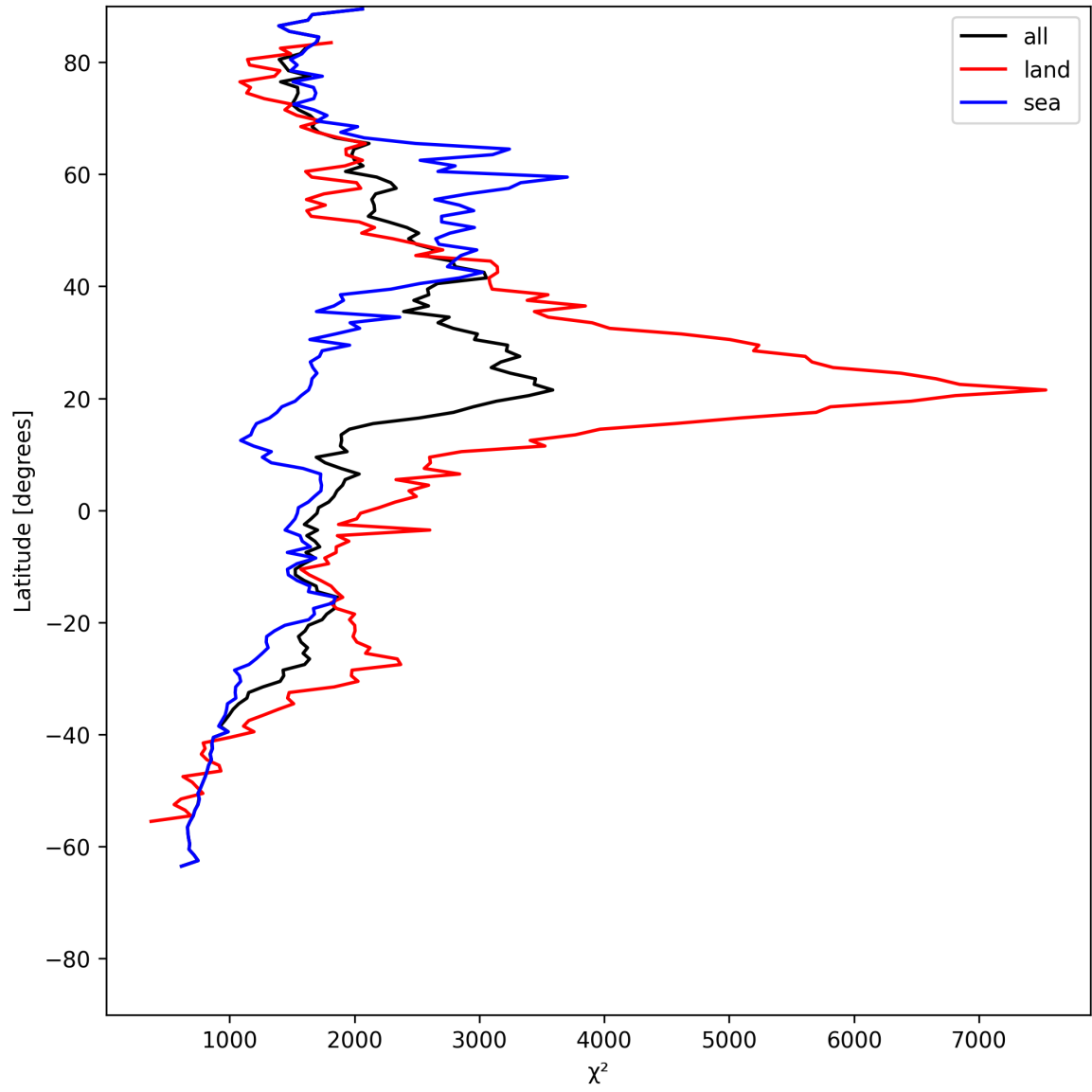
Figure 10: Zonal average of “ \chi^2 ” for 2025-07-17 to 2025-07-18.
