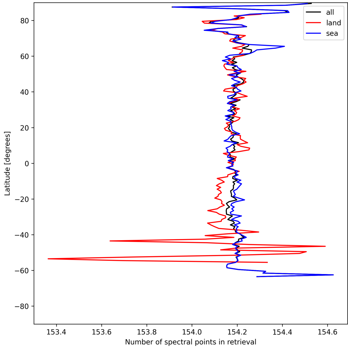
Figure 9: Zonal average of “Number of spectral points in retrieval” for 2025-07-17 to 2025-07-18.
