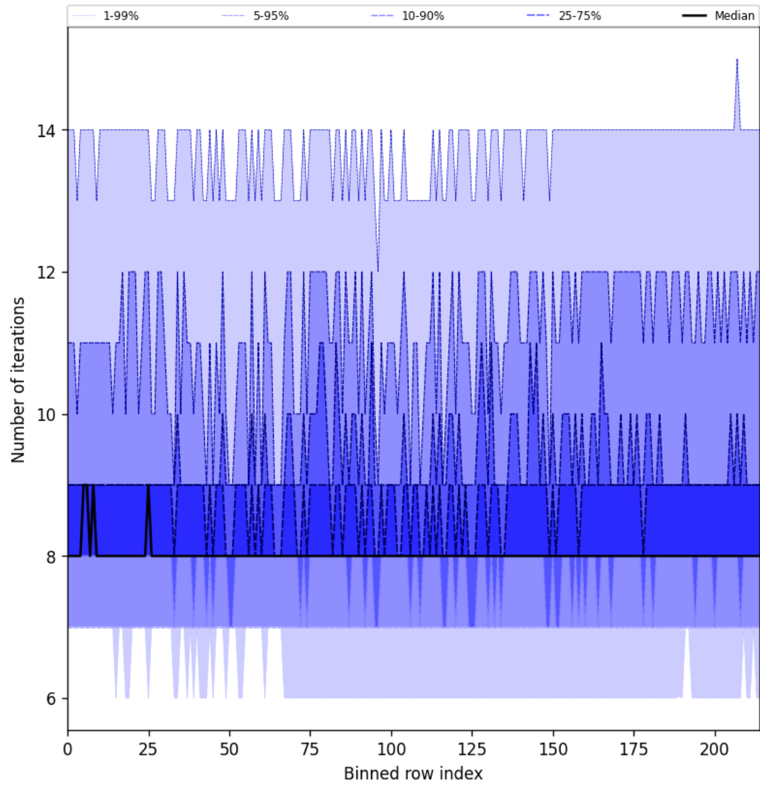
Figure 26: Along track statistics of “Number of iterations” for 2025-07-17 to 2025-07-18
