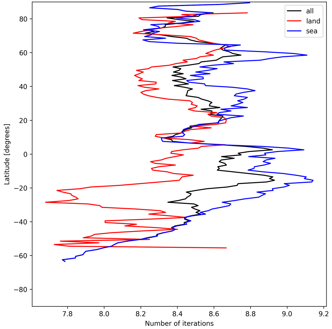
Figure 12: Zonal average of “Number of iterations” for 2025-07-17 to 2025-07-18.
