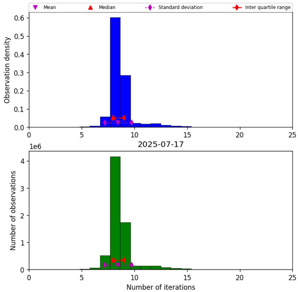
Figure 19: Histogram of “Number of iterations” for 2025-07-17 to 2025-07-18
