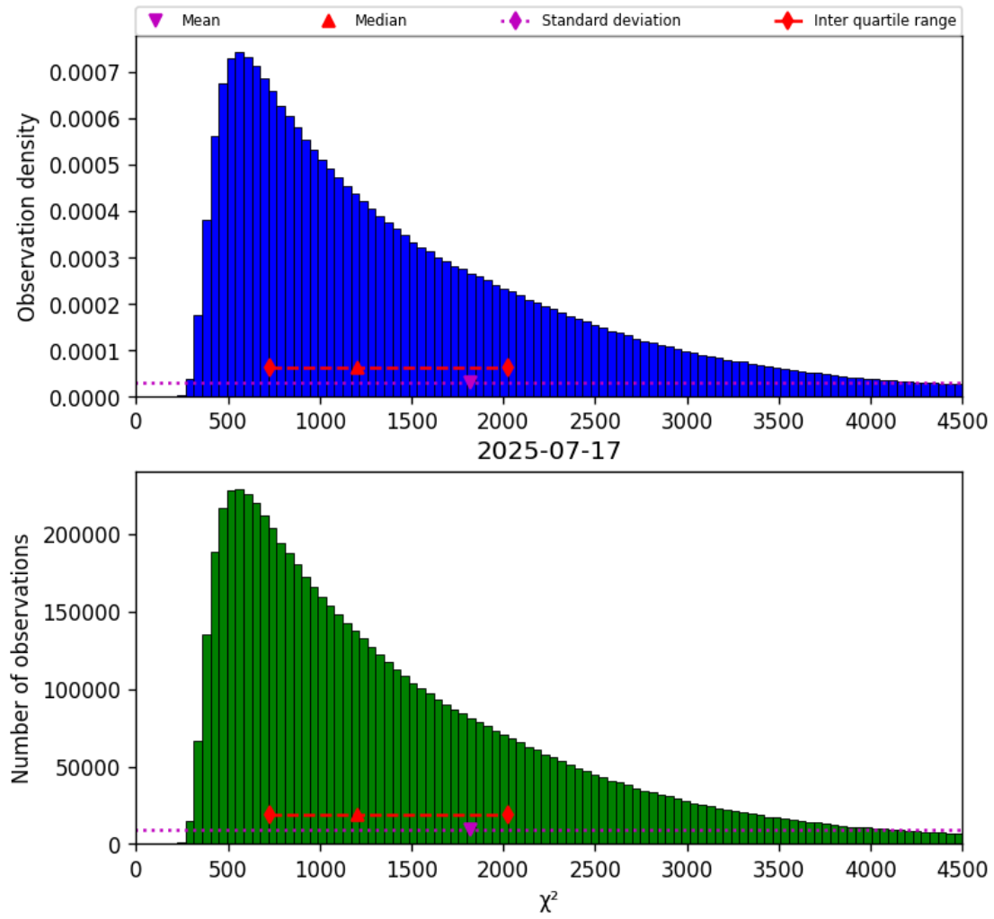
Figure 17: Histogram of “ \chi^2 ” for 2025-07-17 to 2025-07-18
