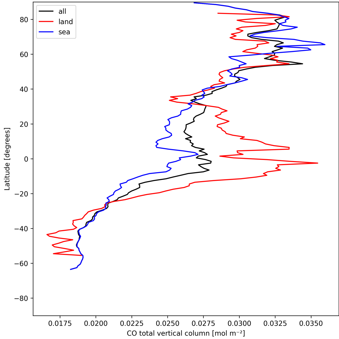
Figure 7: Zonal average of “CO total vertical column” for 2025-07-17 to 2025-07-18.
