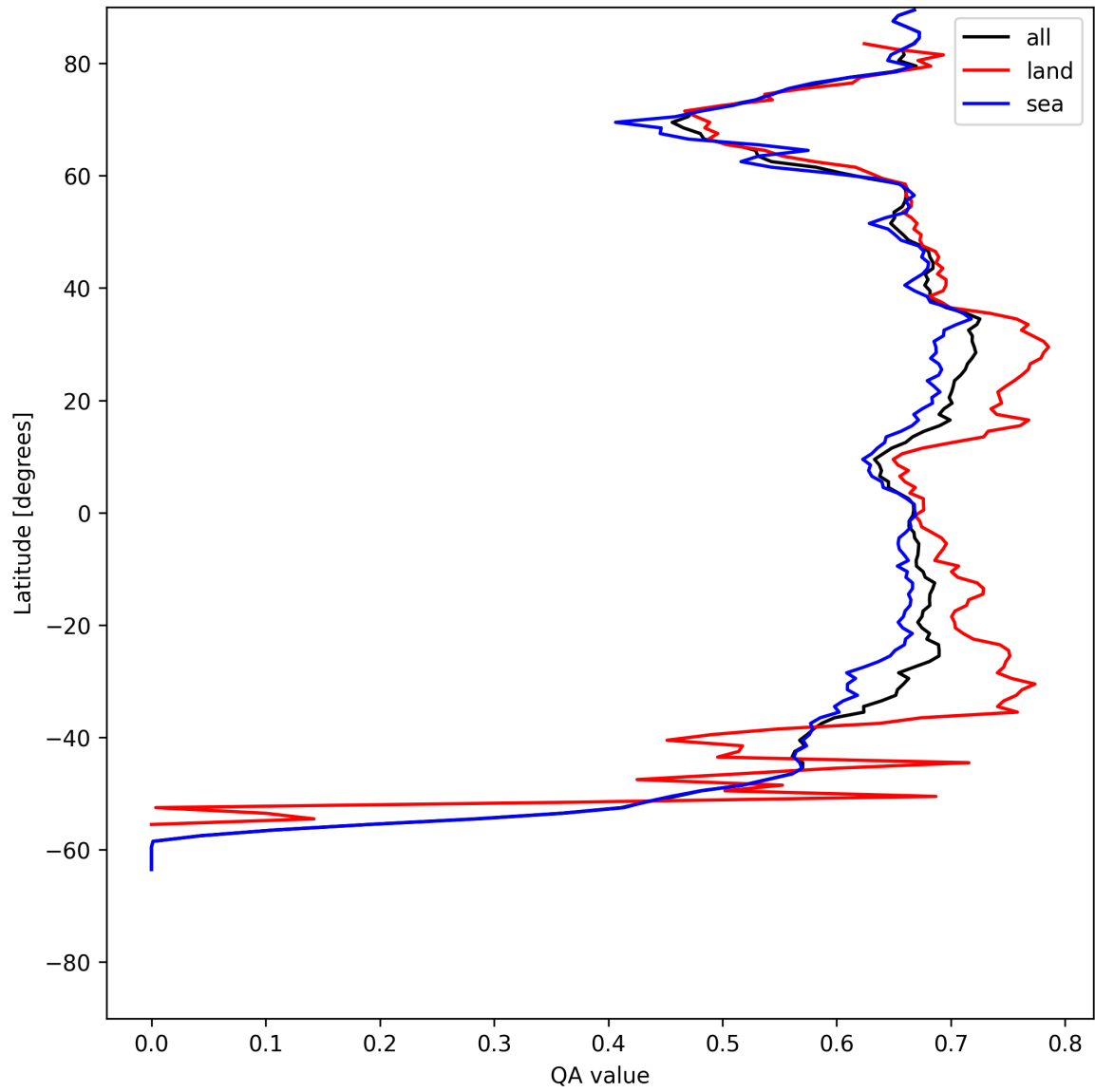
Figure 6: Zonal average of “QA value” for 2025-07-17 to 2025-07-18.
