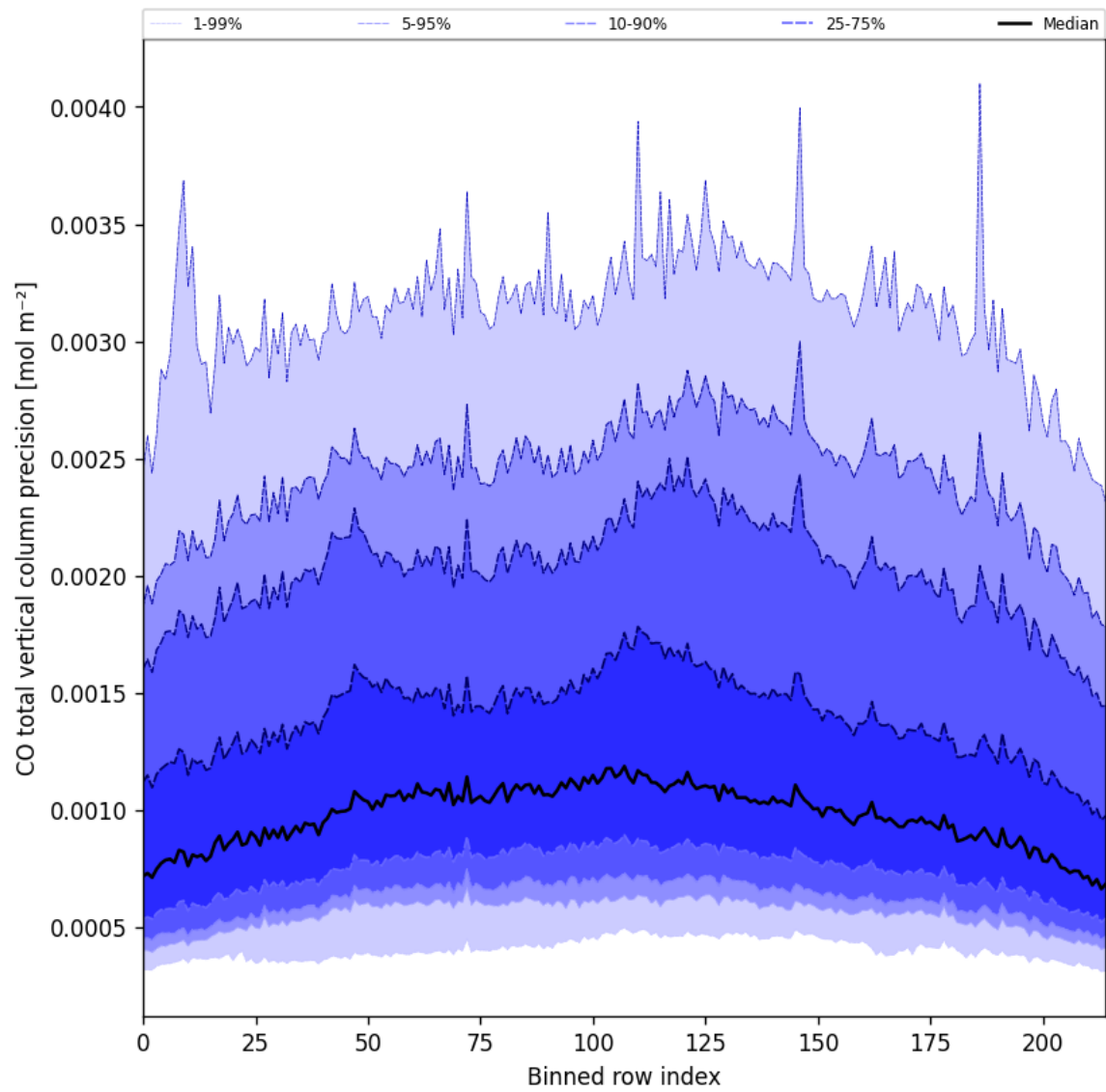
Figure 22: Along track statistics of “CO total vertical column precision” for 2025-07-17 to 2025-07-18
