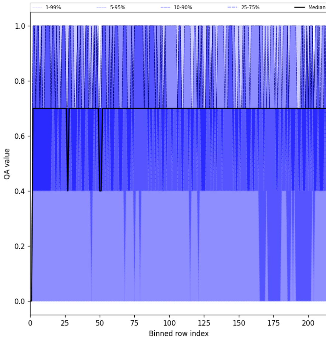
Figure 20: Along track statistics of “QA value” for 2025-07-17 to 2025-07-18
