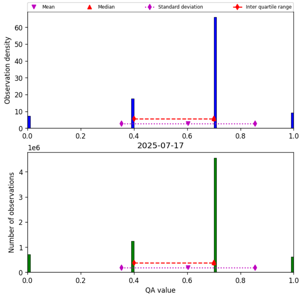
Figure 13: Histogram of “QA value” for 2025-07-17 to 2025-07-18
