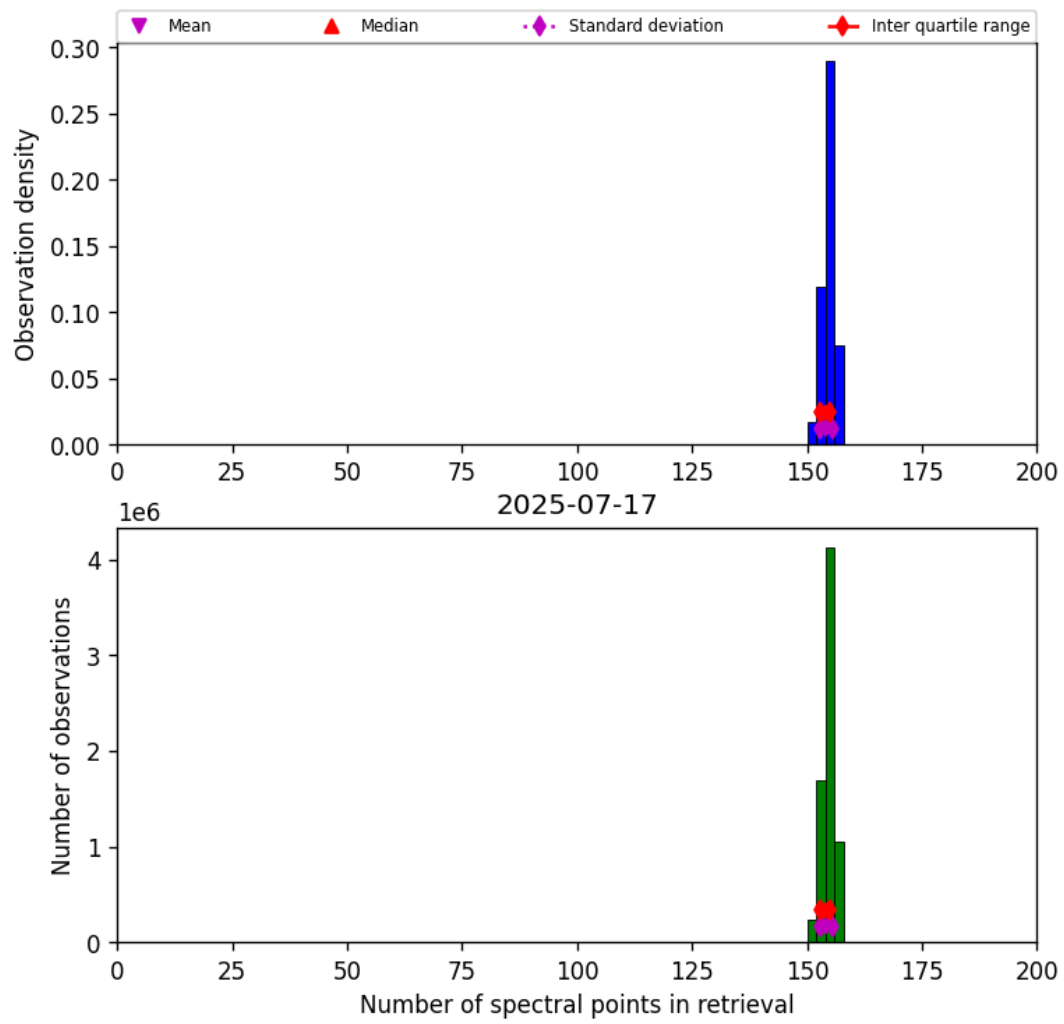
Figure 16: Histogram of “Number of spectral points in retrieval” for 2025-07-17 to 2025-07-18
