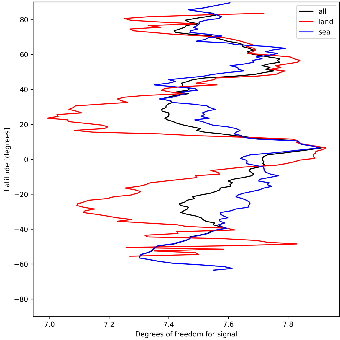
Figure 11: Zonal average of “Degrees of freedom for signal” for 2025-07-17 to 2025-07-18.
