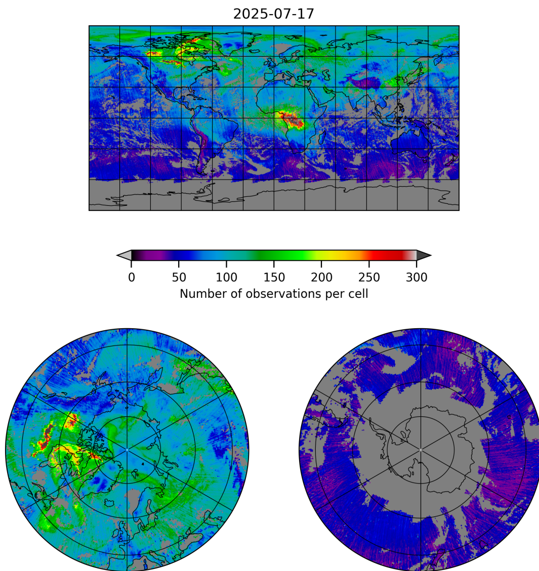
Figure 5: Map of the number of observations for 2025-07-17 to 2025-07-18
