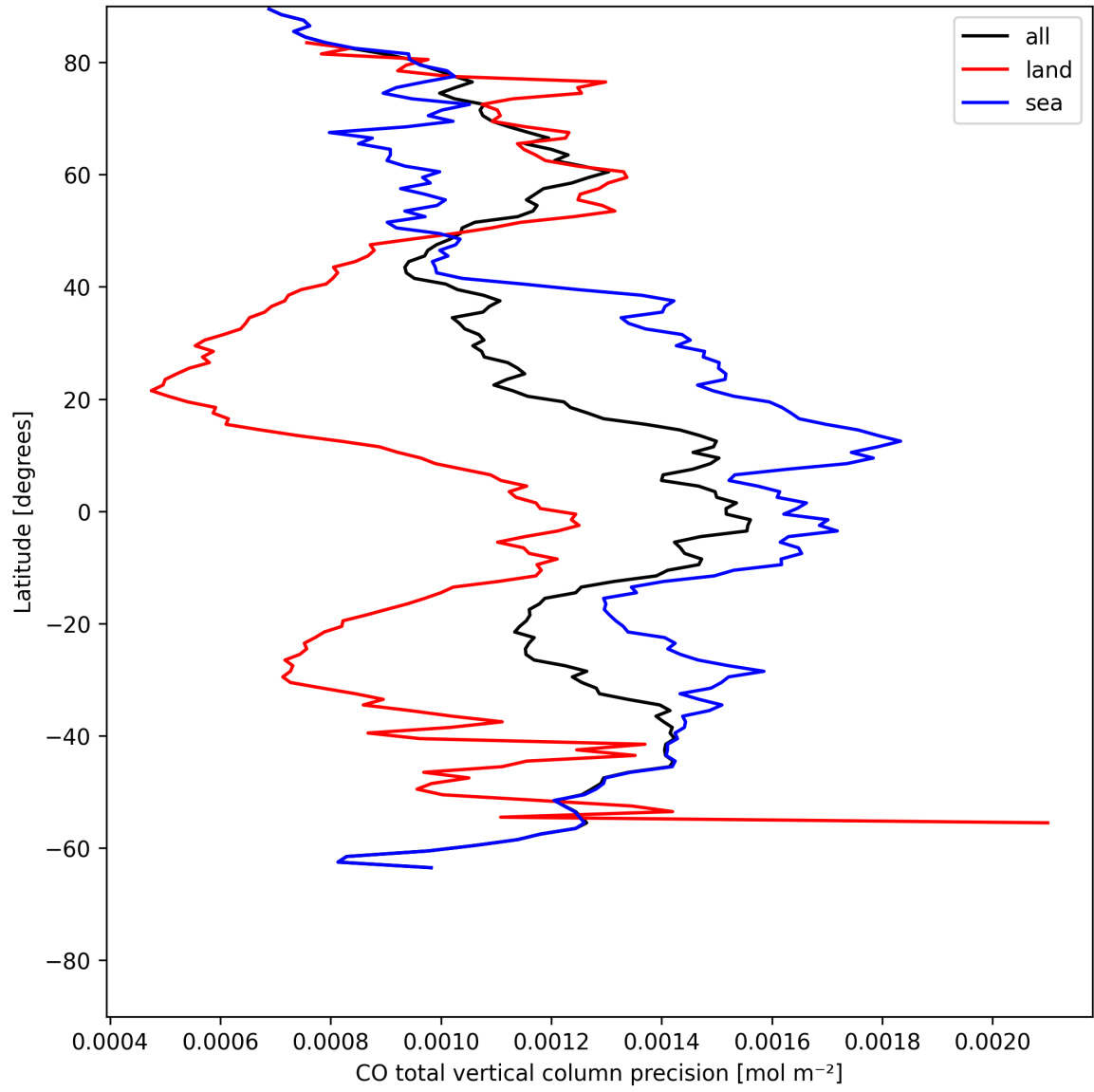
Figure 8: Zonal average of “CO total vertical column precision” for 2025-07-17 to 2025-07-18.
