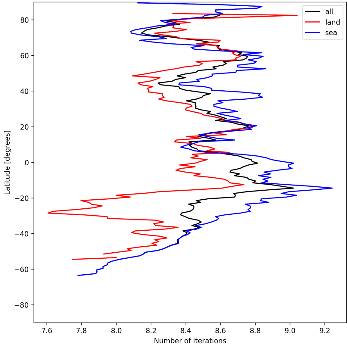
Figure 12: Zonal average of “Number of iterations” for 2025-07-18 to 2025-07-19.
