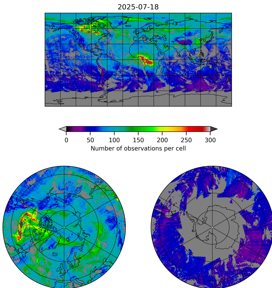
Figure 5: Map of the number of observations for 2025-07-18 to 2025-07-19
