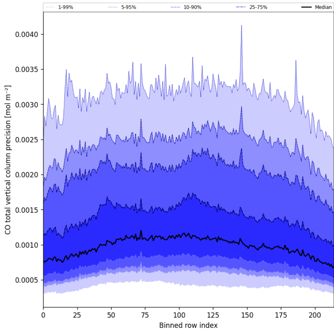
Figure 22: Along track statistics of “CO total vertical column precision” for 2025-07-18 to 2025-07-19
