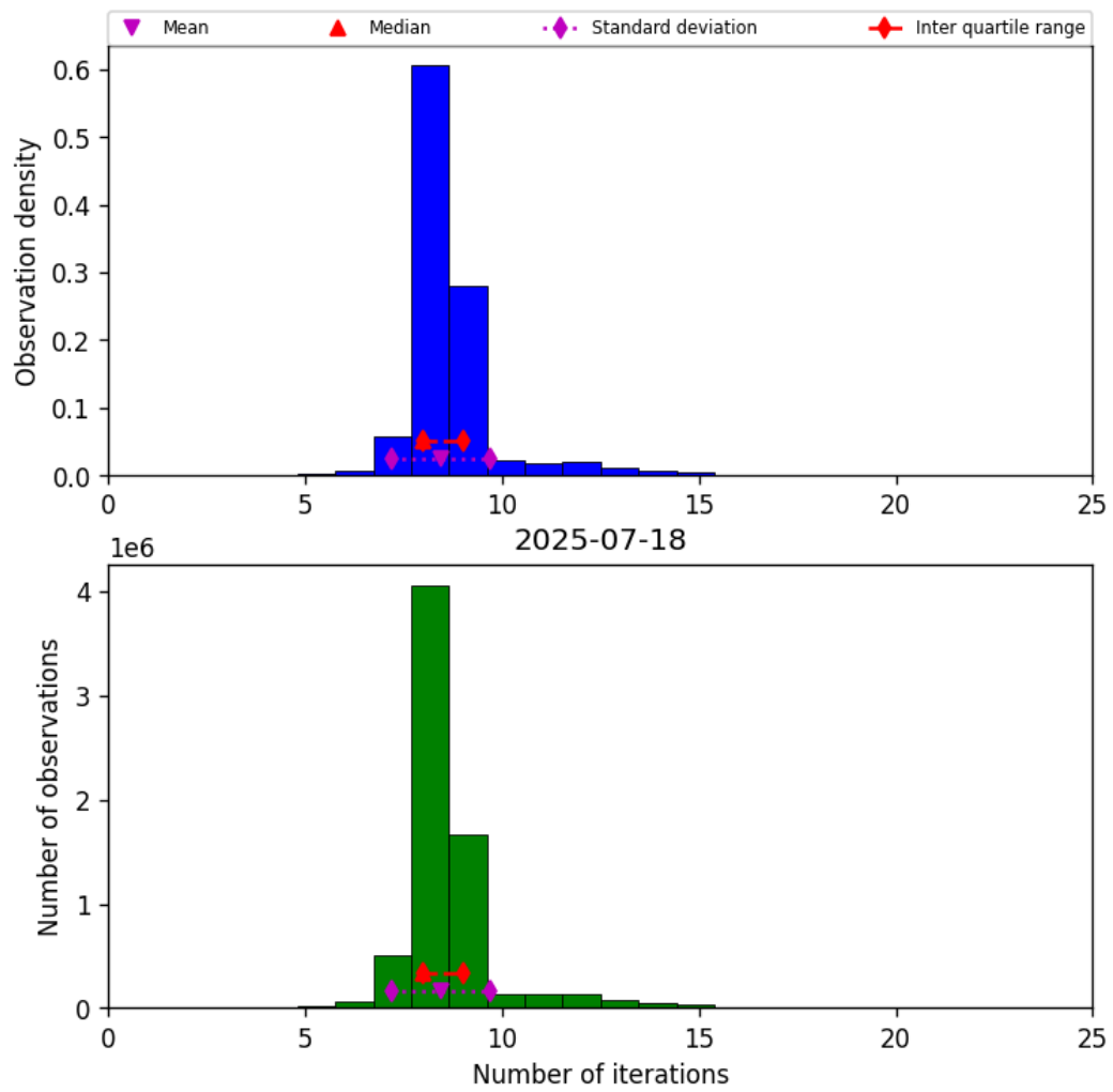
Figure 19: Histogram of “Number of iterations” for 2025-07-18 to 2025-07-19
