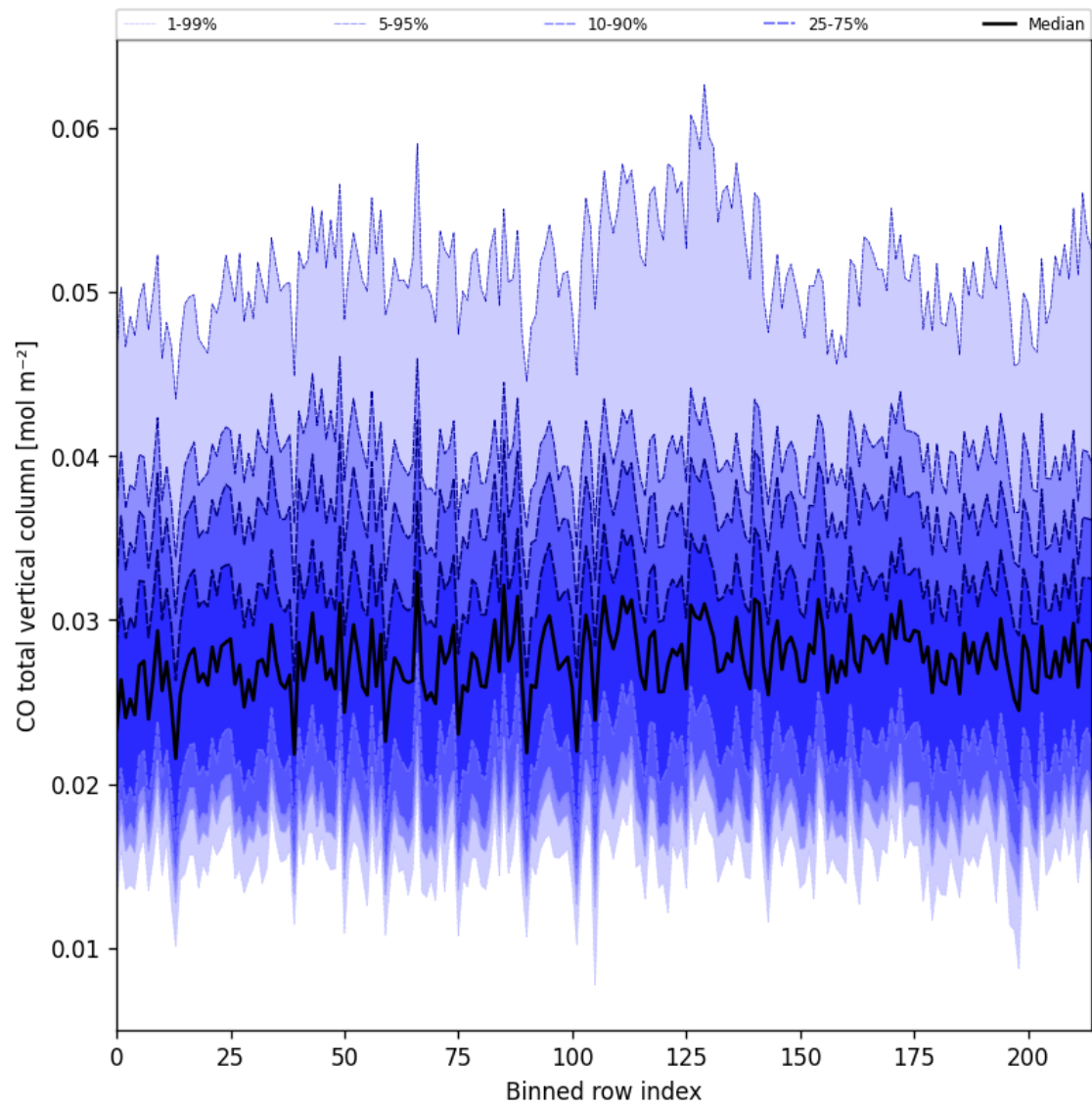
Figure 21: Along track statistics of “CO total vertical column” for 2025-07-18 to 2025-07-19
