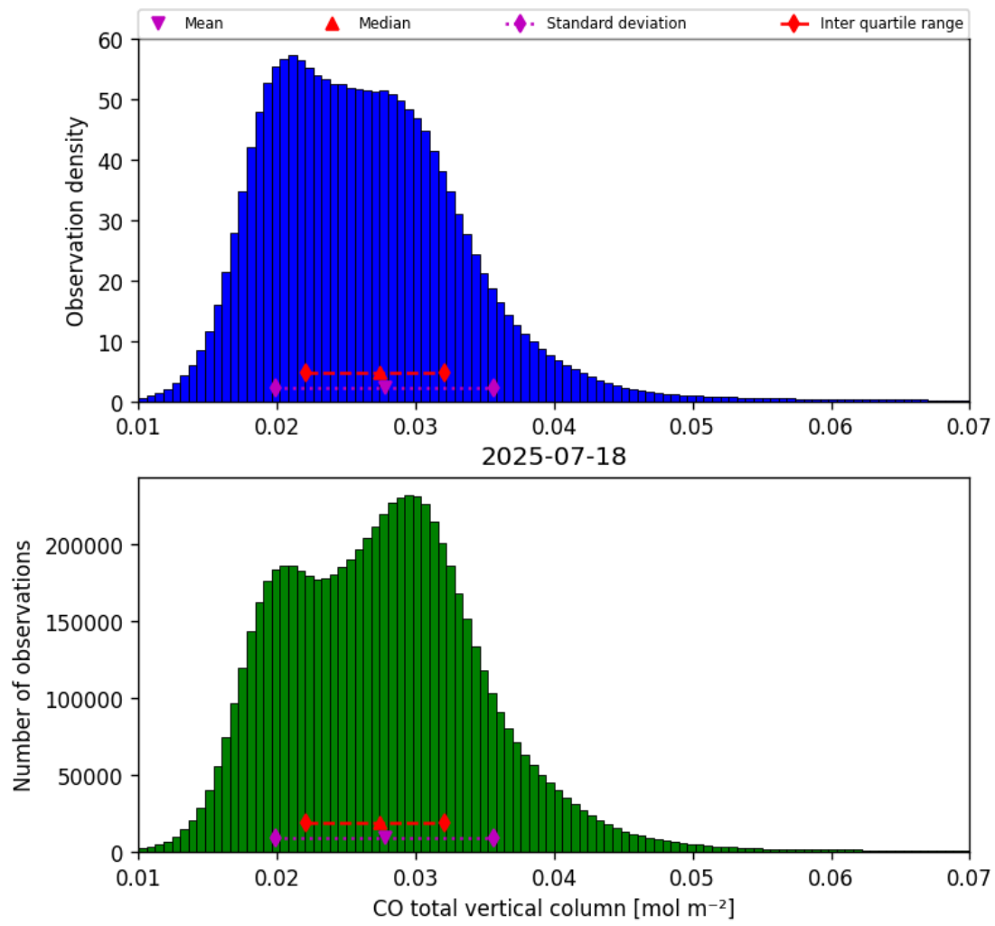
Figure 14: Histogram of “CO total vertical column” for 2025-07-18 to 2025-07-19
