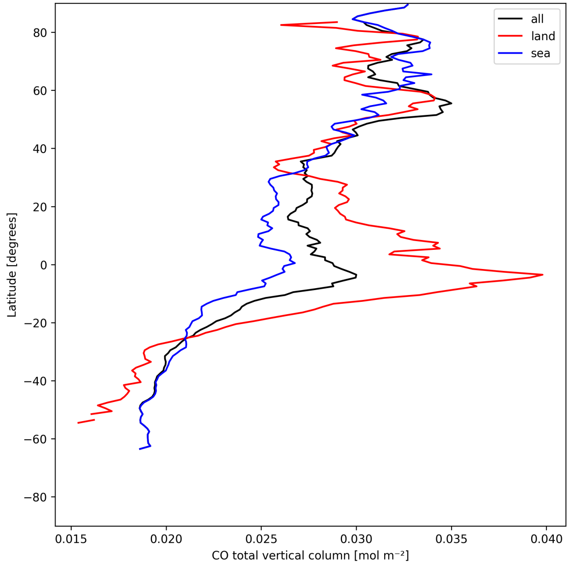
Figure 7: Zonal average of “CO total vertical column” for 2025-07-18 to 2025-07-19.
