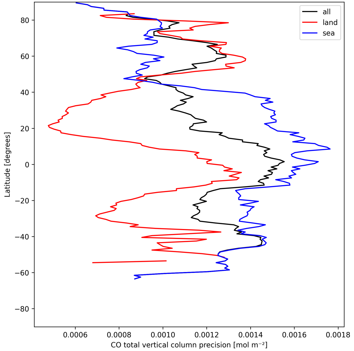
Figure 8: Zonal average of “CO total vertical column precision” for 2025-07-18 to 2025-07-19.
