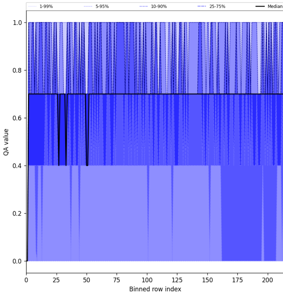
Figure 20: Along track statistics of “QA value” for 2025-07-18 to 2025-07-19
