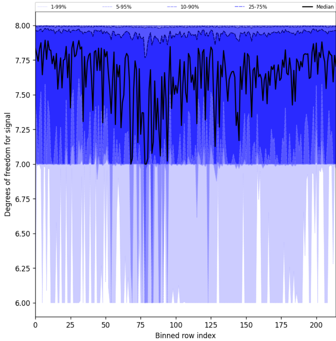
Figure 25: Along track statistics of “Degrees of freedom for signal” for 2025-07-18 to 2025-07-19
