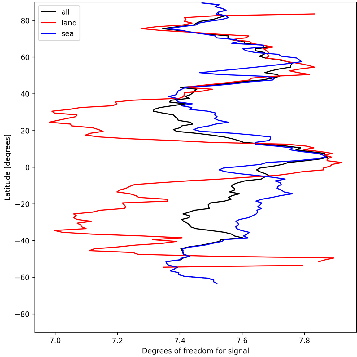
Figure 11: Zonal average of “Degrees of freedom for signal” for 2025-07-18 to 2025-07-19.
