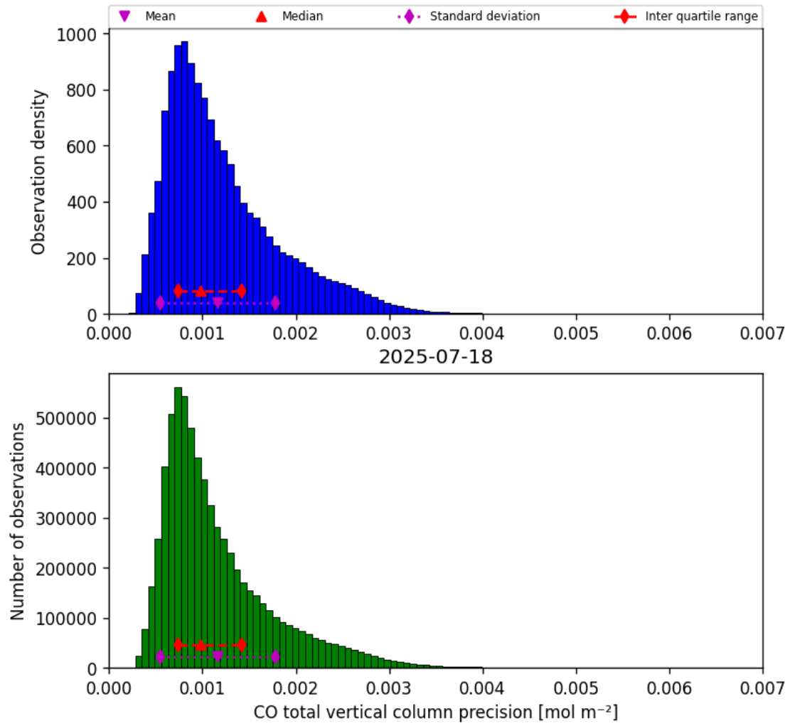
Figure 15: Histogram of “CO total vertical column precision” for 2025-07-18 to 2025-07-19
