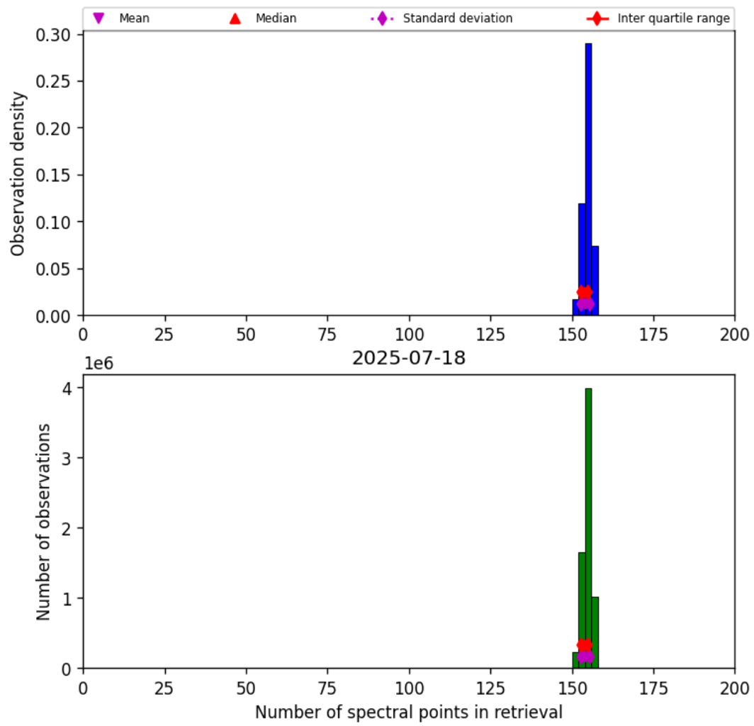
Figure 16: Histogram of “Number of spectral points in retrieval” for 2025-07-18 to 2025-07-19
