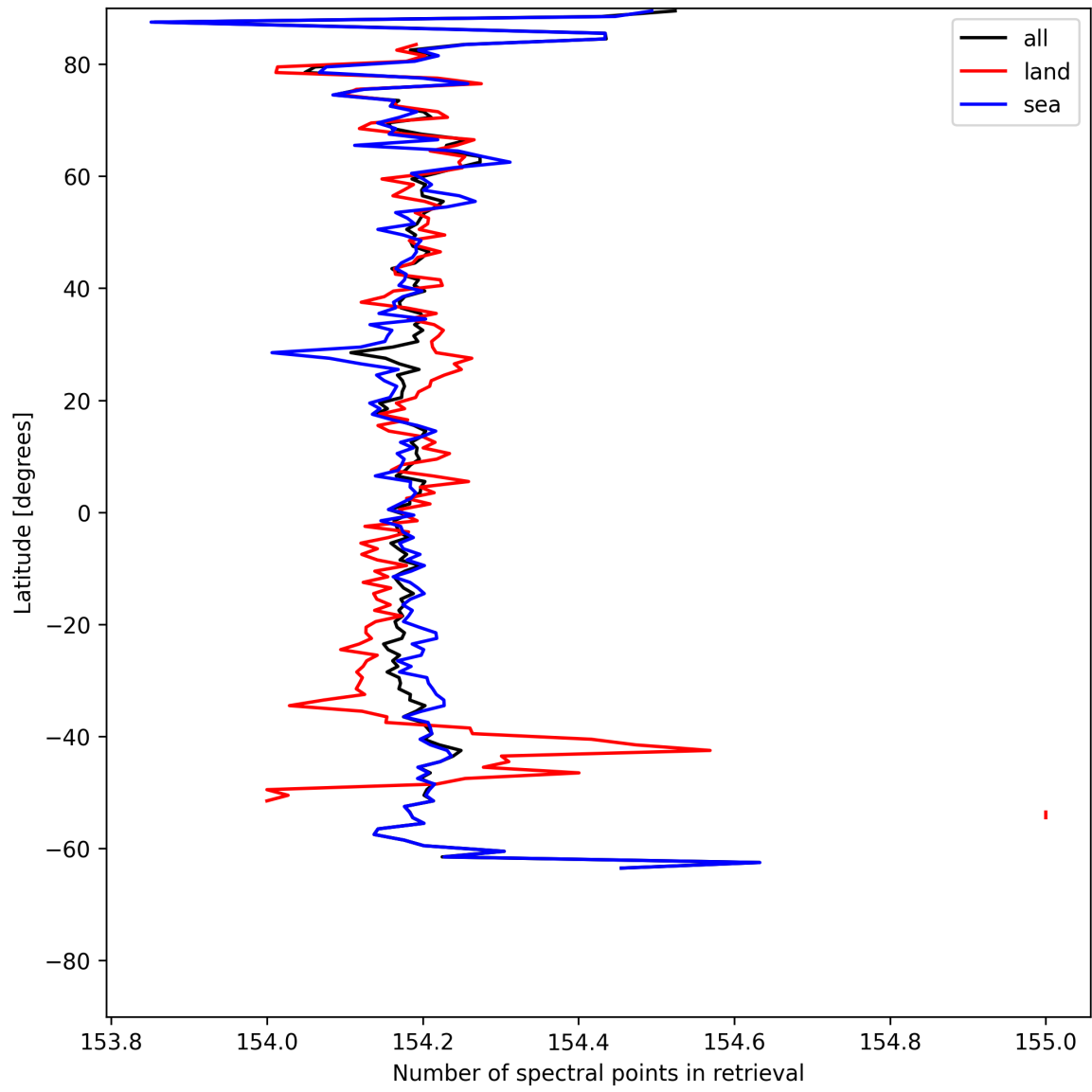
Figure 9: Zonal average of “Number of spectral points in retrieval” for 2025-07-18 to 2025-07-19.
