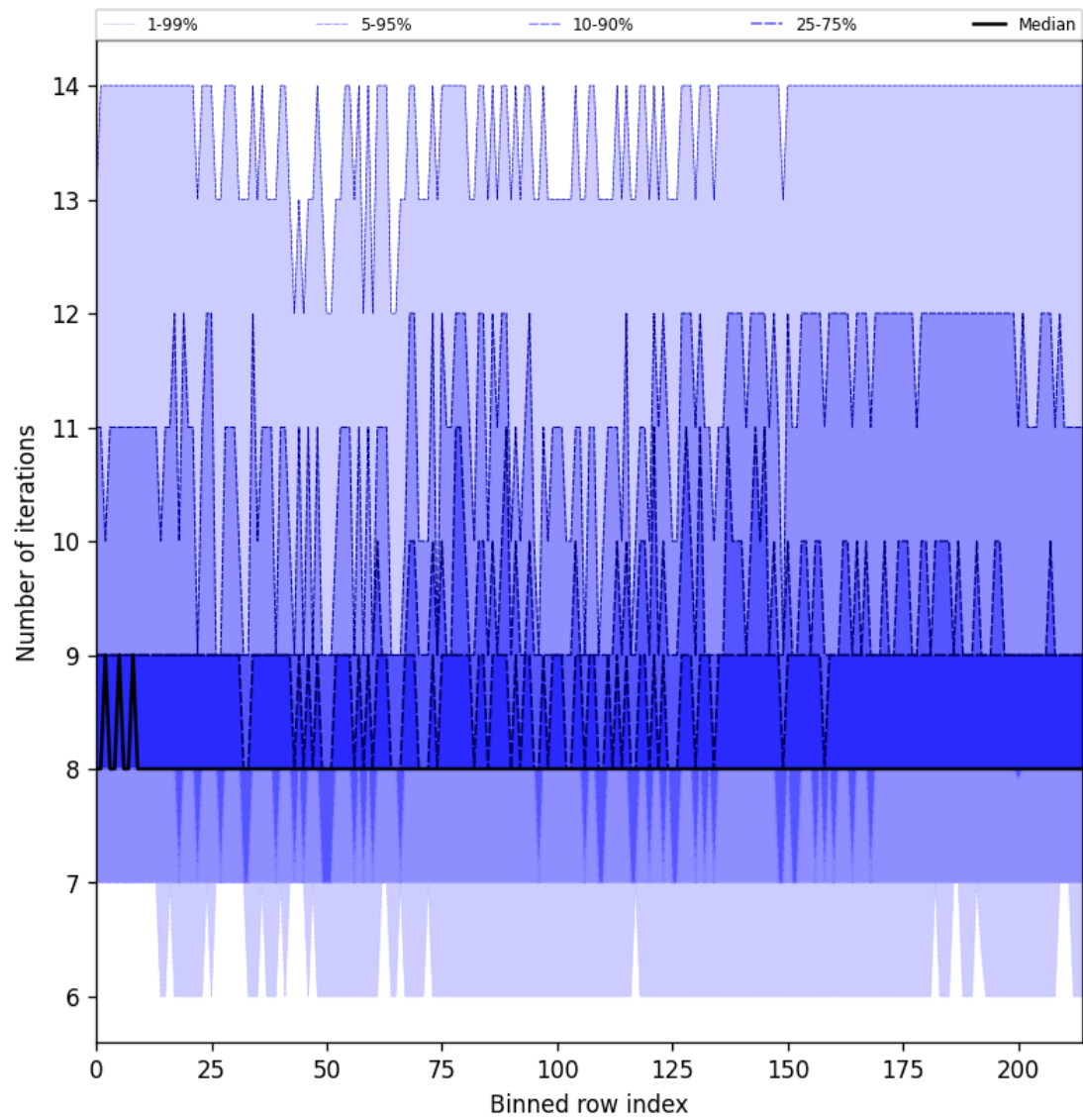
Figure 26: Along track statistics of “Number of iterations” for 2025-07-18 to 2025-07-19
