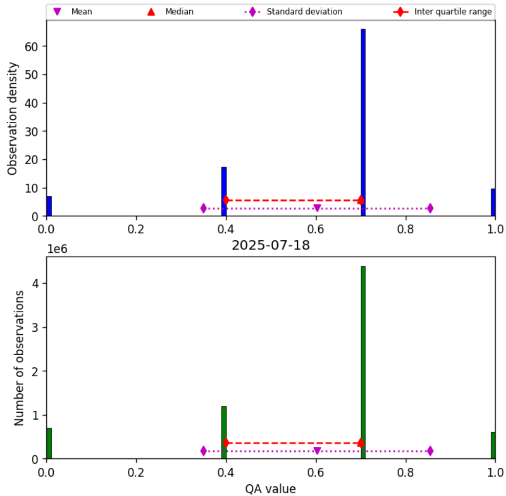
Figure 13: Histogram of “QA value” for 2025-07-18 to 2025-07-19
