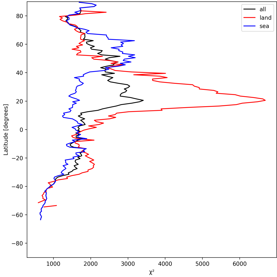
Figure 10: Zonal average of “ \chi^2 ” for 2025-07-18 to 2025-07-19.
