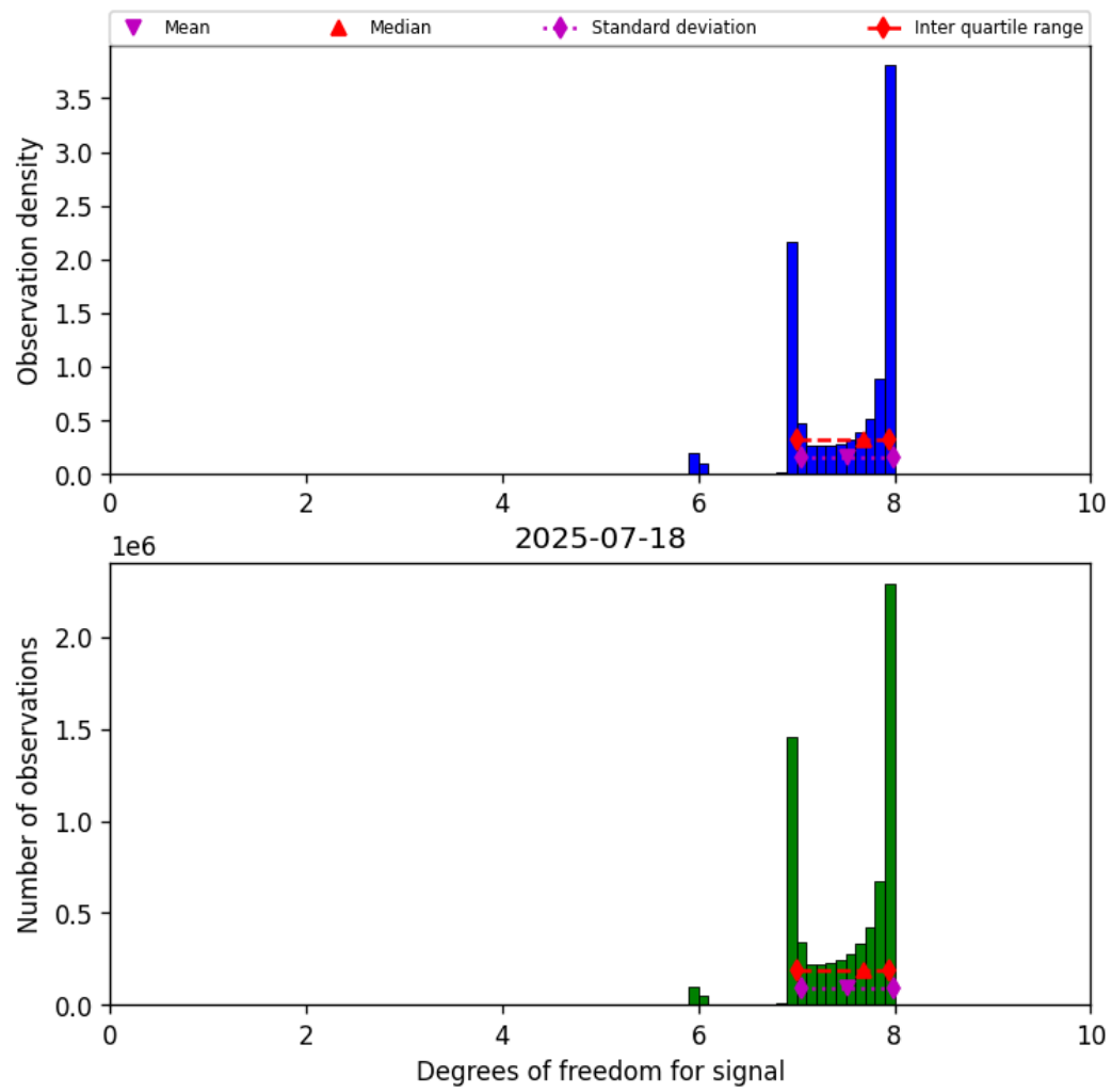
Figure 18: Histogram of “Degrees of freedom for signal” for 2025-07-18 to 2025-07-19
