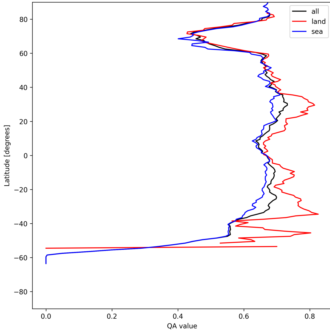
Figure 6: Zonal average of “QA value” for 2025-07-18 to 2025-07-19.
