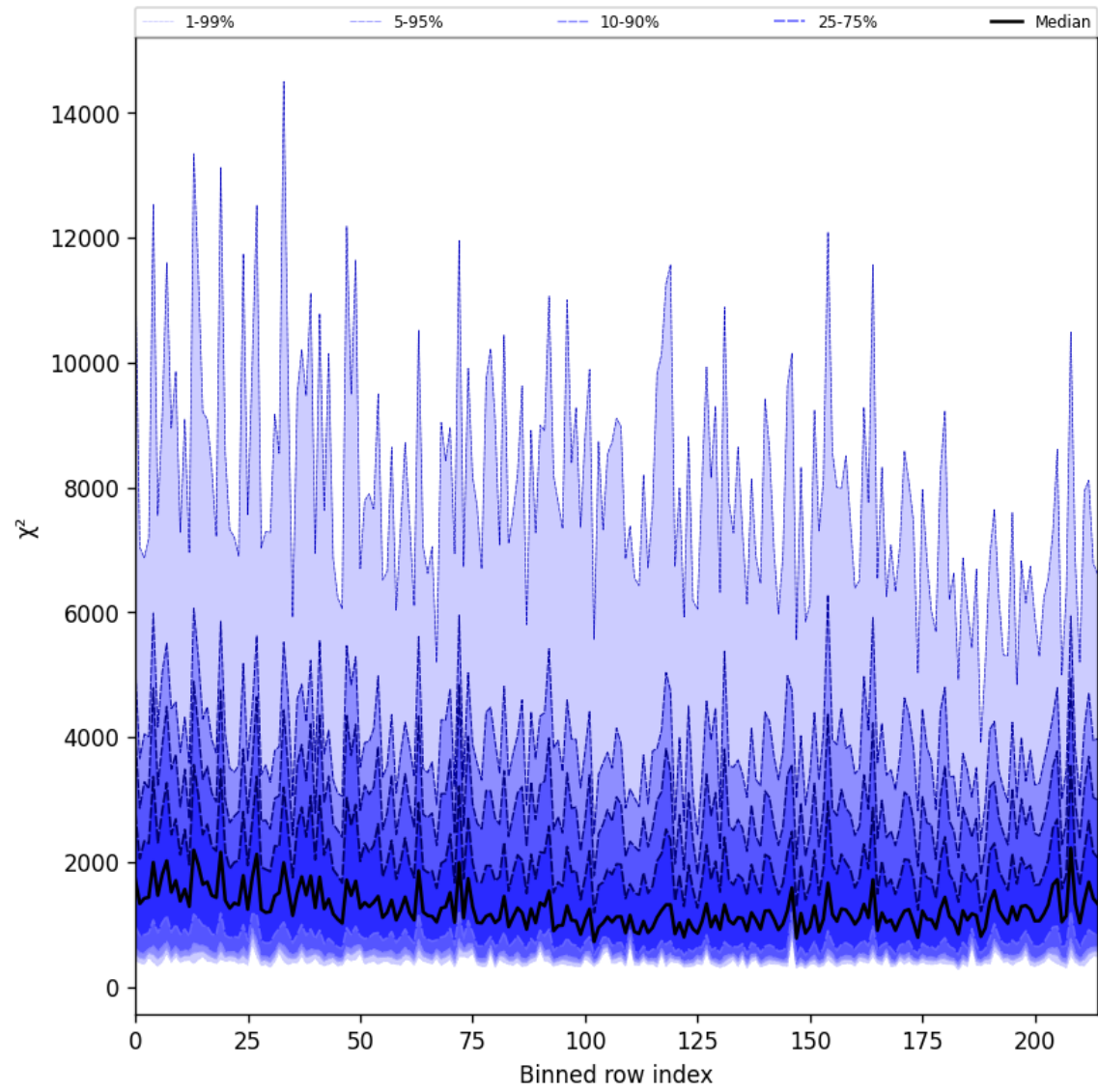
Figure 24: Along track statistics of “ \chi^2 ” for 2025-07-18 to 2025-07-19
