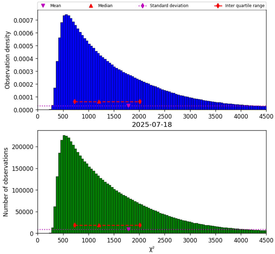
Figure 17: Histogram of “ \chi^2 ” for 2025-07-18 to 2025-07-19
