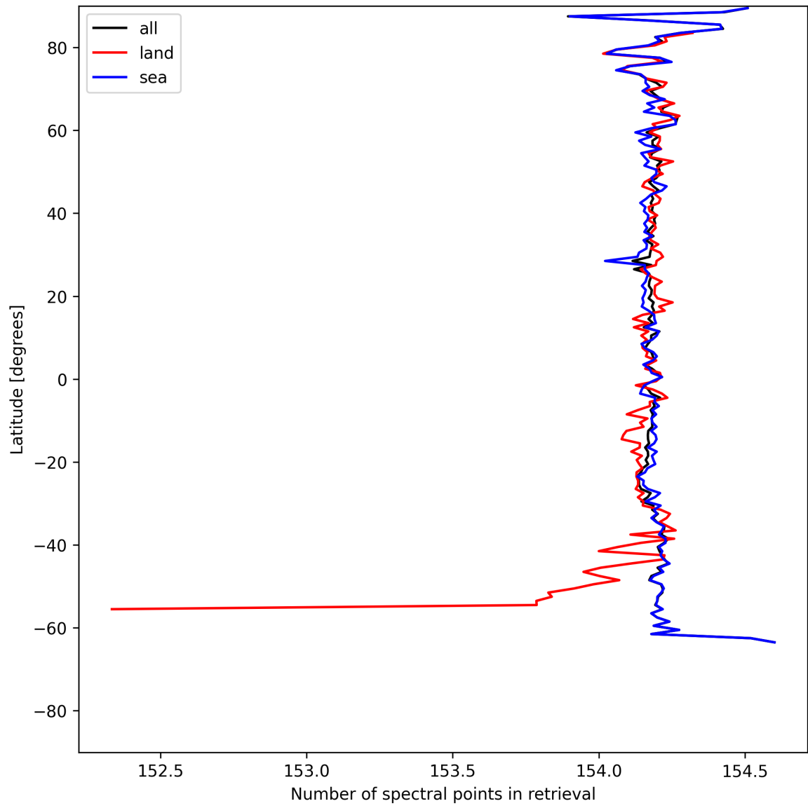
Figure 9: Zonal average of “Number of spectral points in retrieval” for 2025-07-19 to 2025-07-20.
