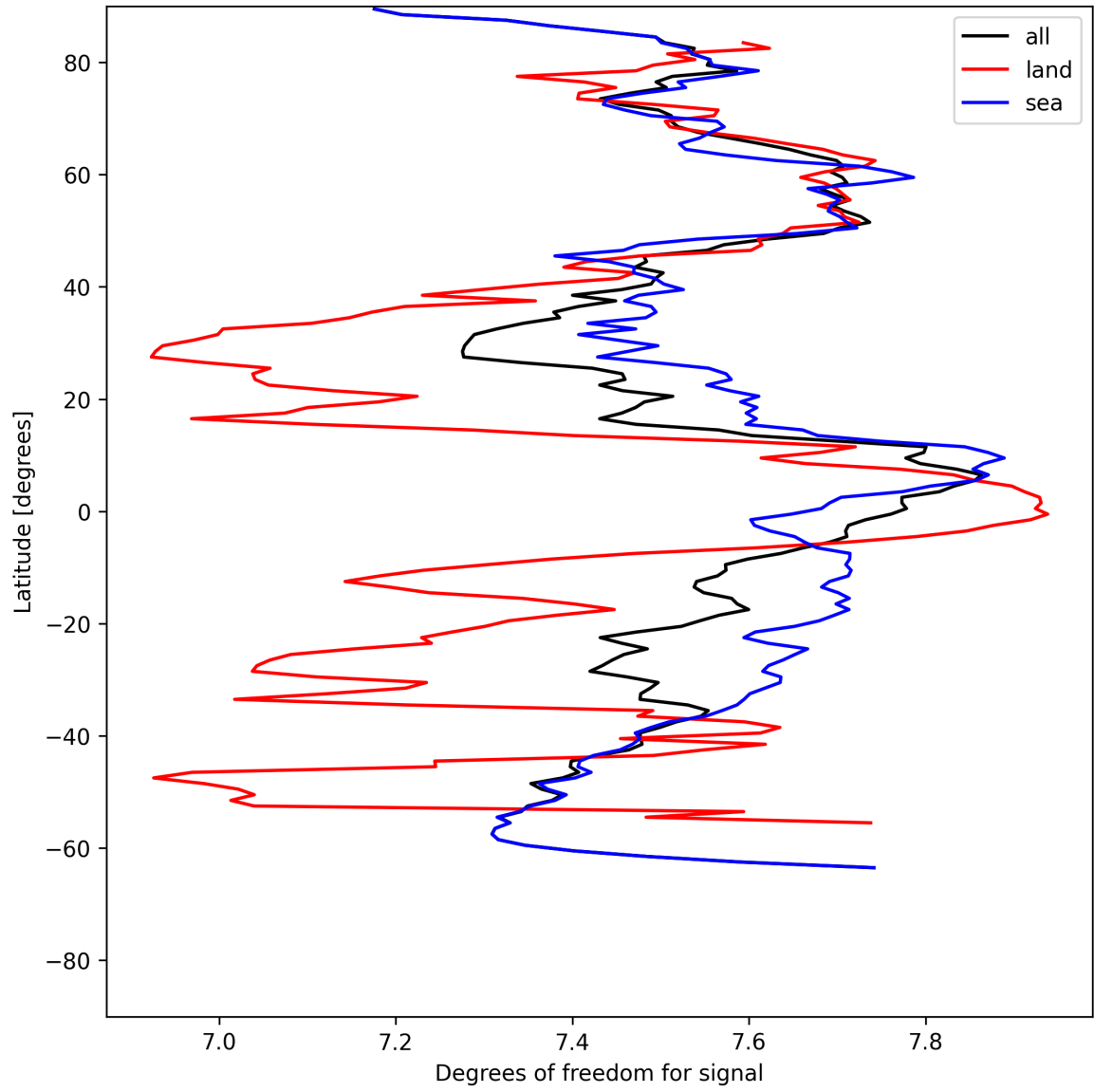
Figure 11: Zonal average of “Degrees of freedom for signal” for 2025-07-19 to 2025-07-20.
