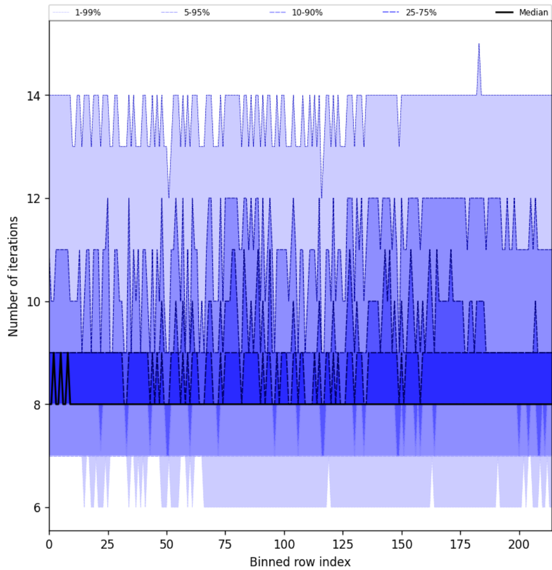
Figure 26: Along track statistics of “Number of iterations” for 2025-07-19 to 2025-07-20
