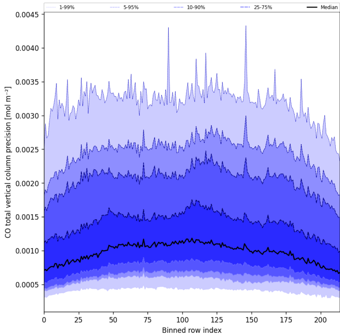
Figure 22: Along track statistics of “CO total vertical column precision” for 2025-07-19 to 2025-07-20
