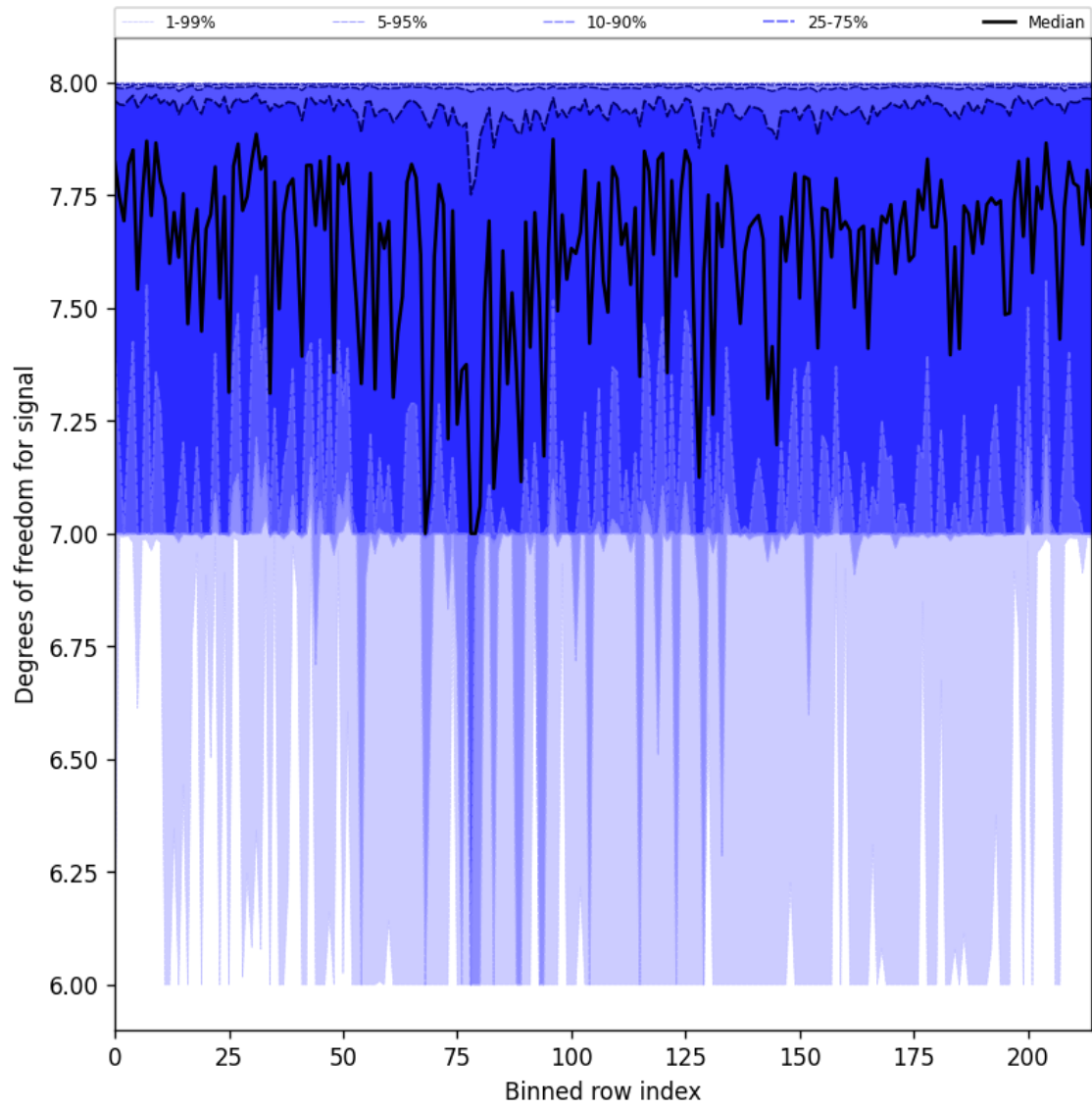
Figure 25: Along track statistics of “Degrees of freedom for signal” for 2025-07-19 to 2025-07-20
