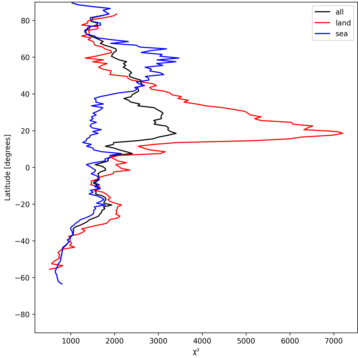
Figure 10: Zonal average of “ \chi^2 ” for 2025-07-19 to 2025-07-20.
