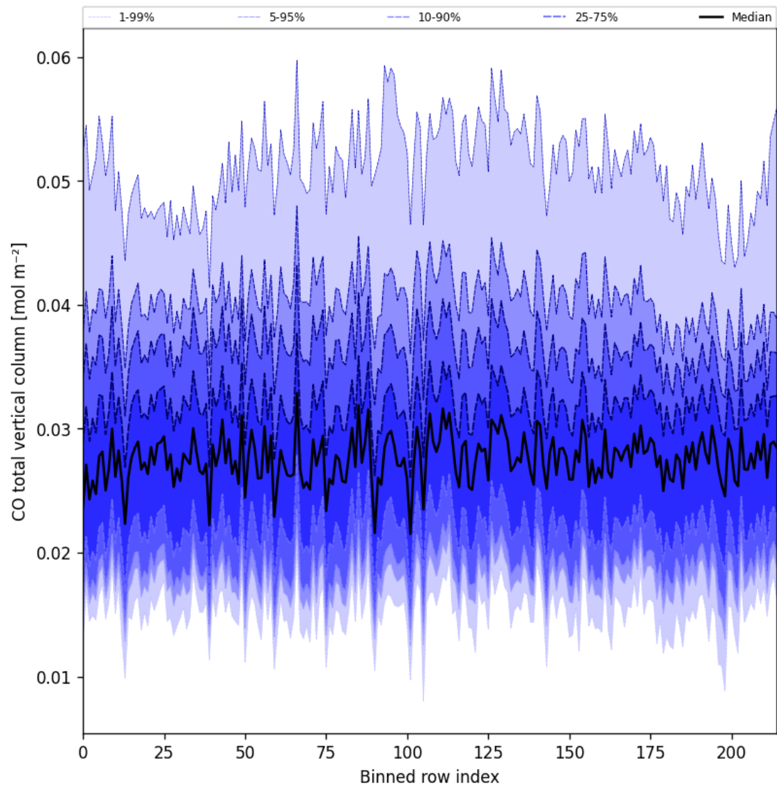
Figure 21: Along track statistics of “CO total vertical column” for 2025-07-19 to 2025-07-20
