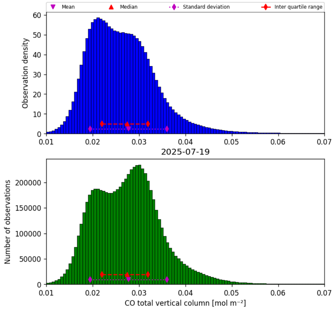
Figure 14: Histogram of “CO total vertical column” for 2025-07-19 to 2025-07-20
