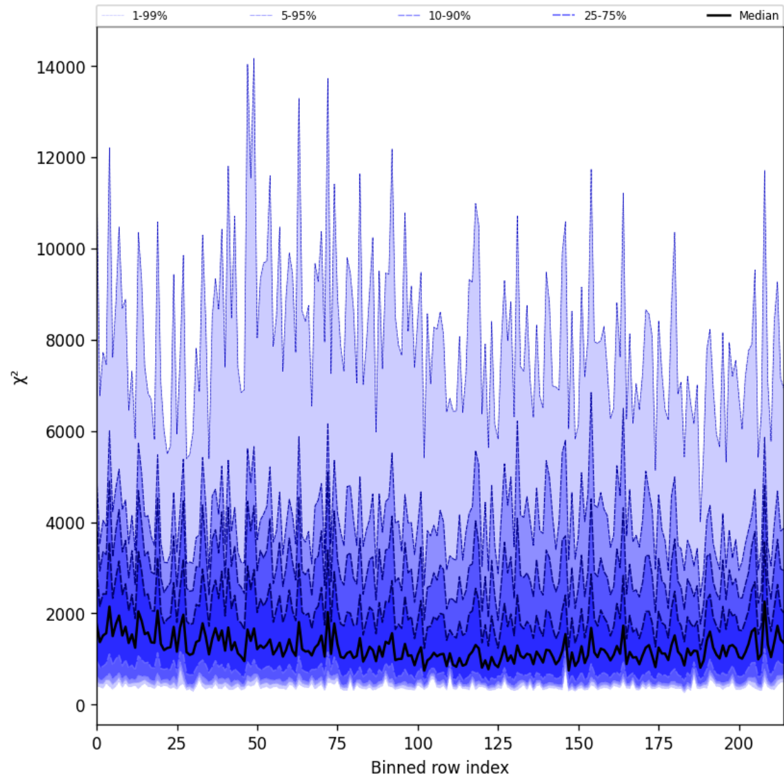
Figure 24: Along track statistics of “ \chi^2 ” for 2025-07-19 to 2025-07-20
