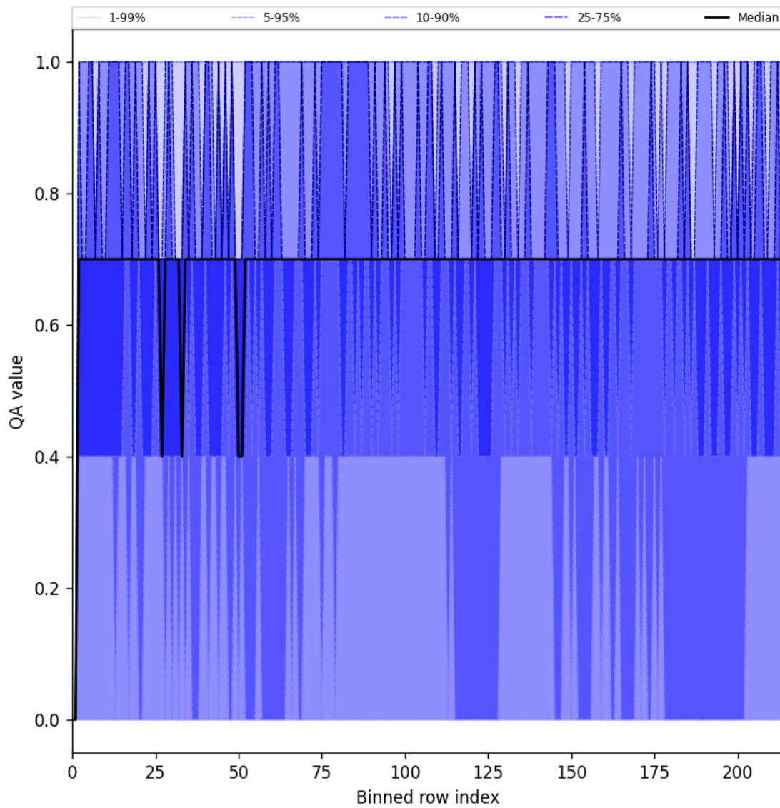
Figure 20: Along track statistics of “QA value” for 2025-07-19 to 2025-07-20
