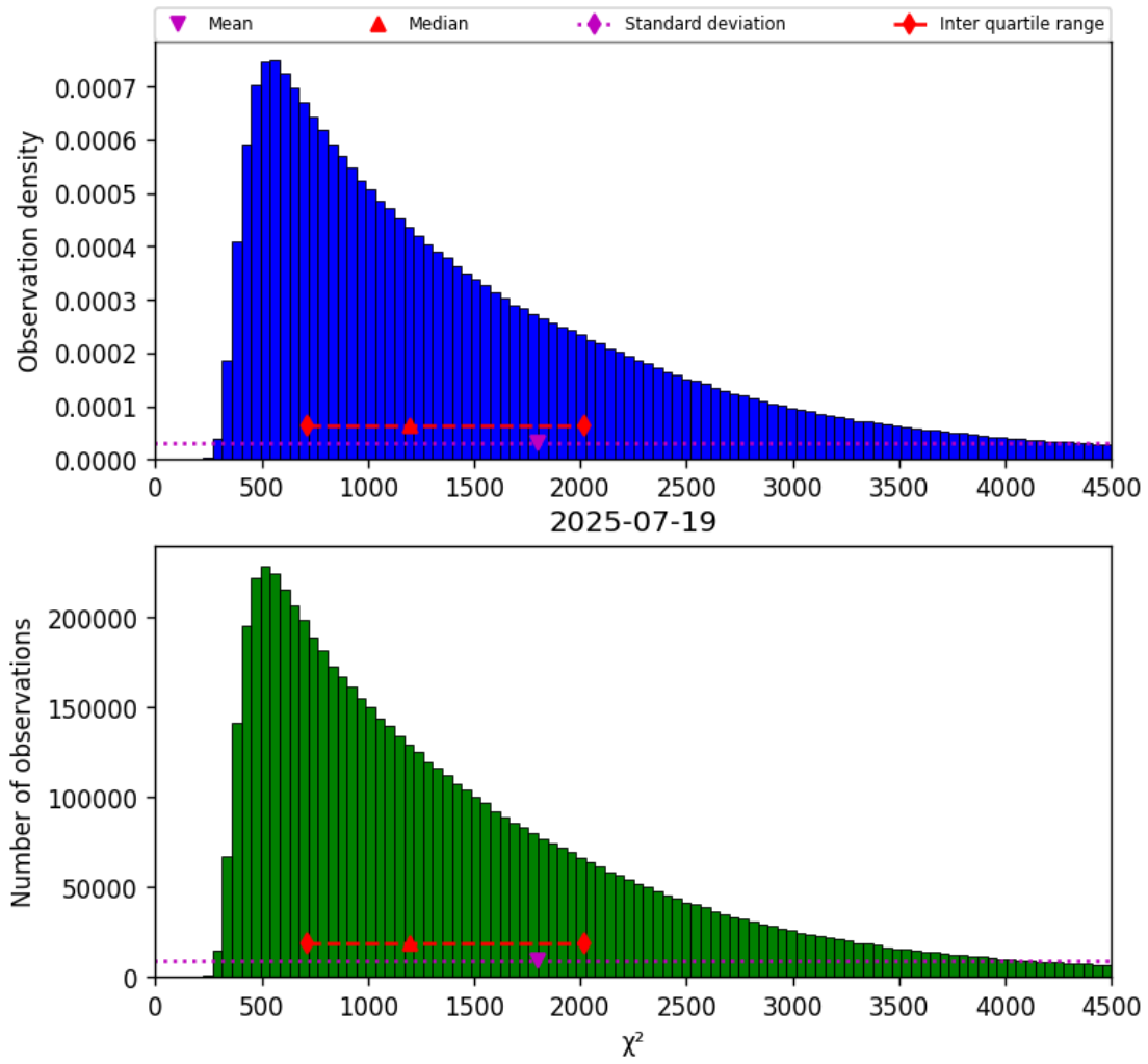
Figure 17: Histogram of “ \chi^2 ” for 2025-07-19 to 2025-07-20
