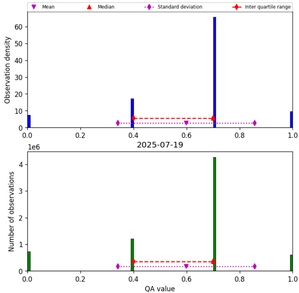
Figure 13: Histogram of “QA value” for 2025-07-19 to 2025-07-20
