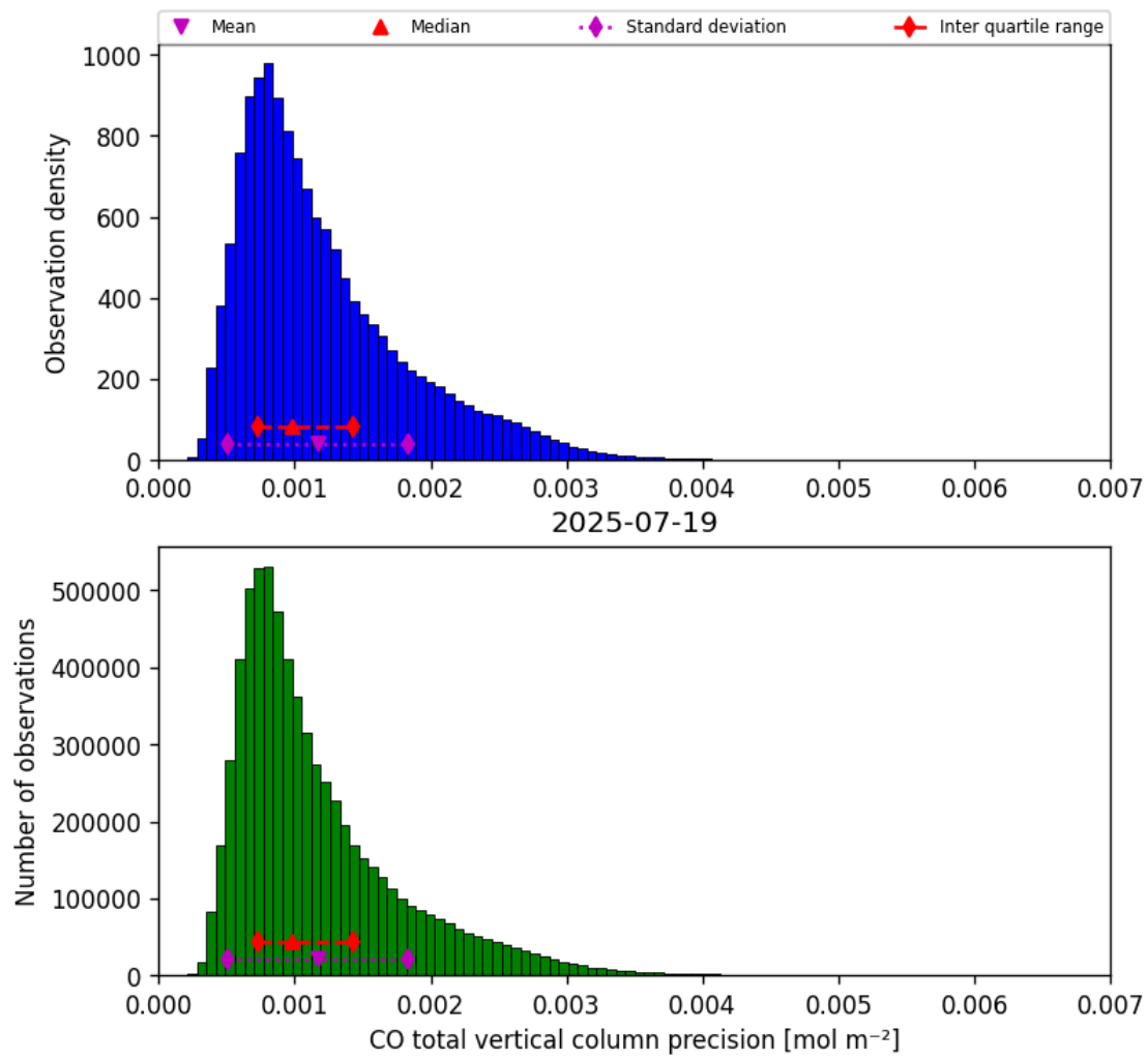
Figure 15: Histogram of “CO total vertical column precision” for 2025-07-19 to 2025-07-20
