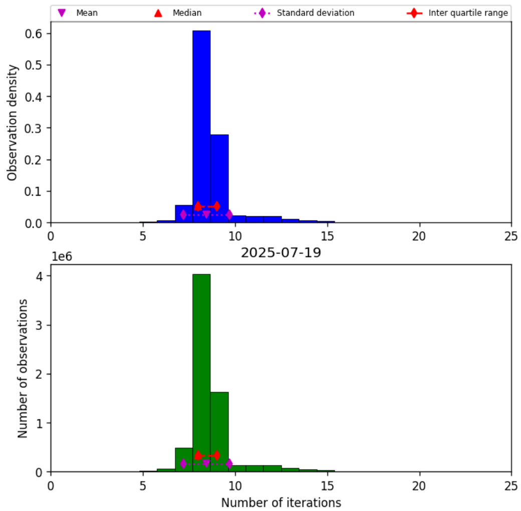
Figure 19: Histogram of “Number of iterations” for 2025-07-19 to 2025-07-20
