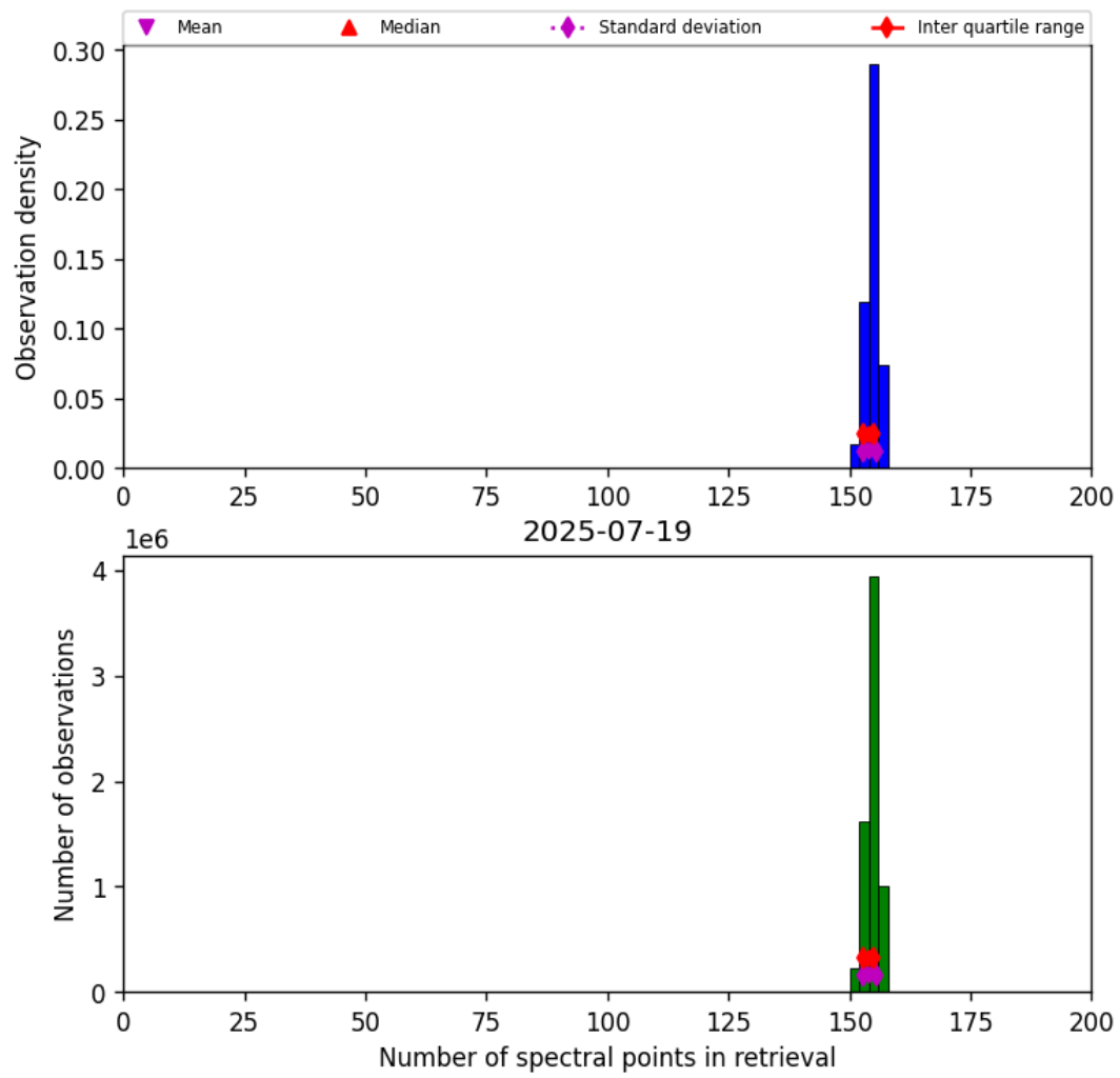
Figure 16: Histogram of “Number of spectral points in retrieval” for 2025-07-19 to 2025-07-20
