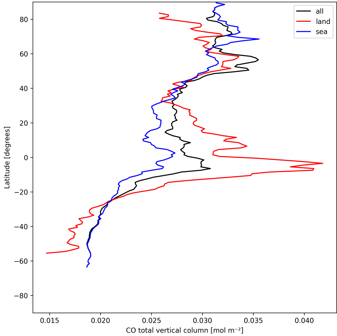
Figure 7: Zonal average of “CO total vertical column” for 2025-07-19 to 2025-07-20.
