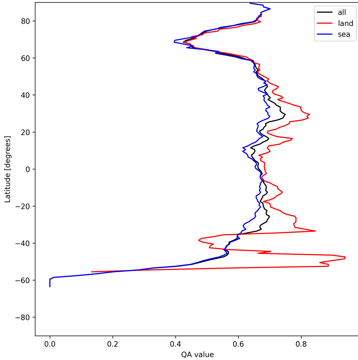
Figure 6: Zonal average of “QA value” for 2025-07-19 to 2025-07-20.
