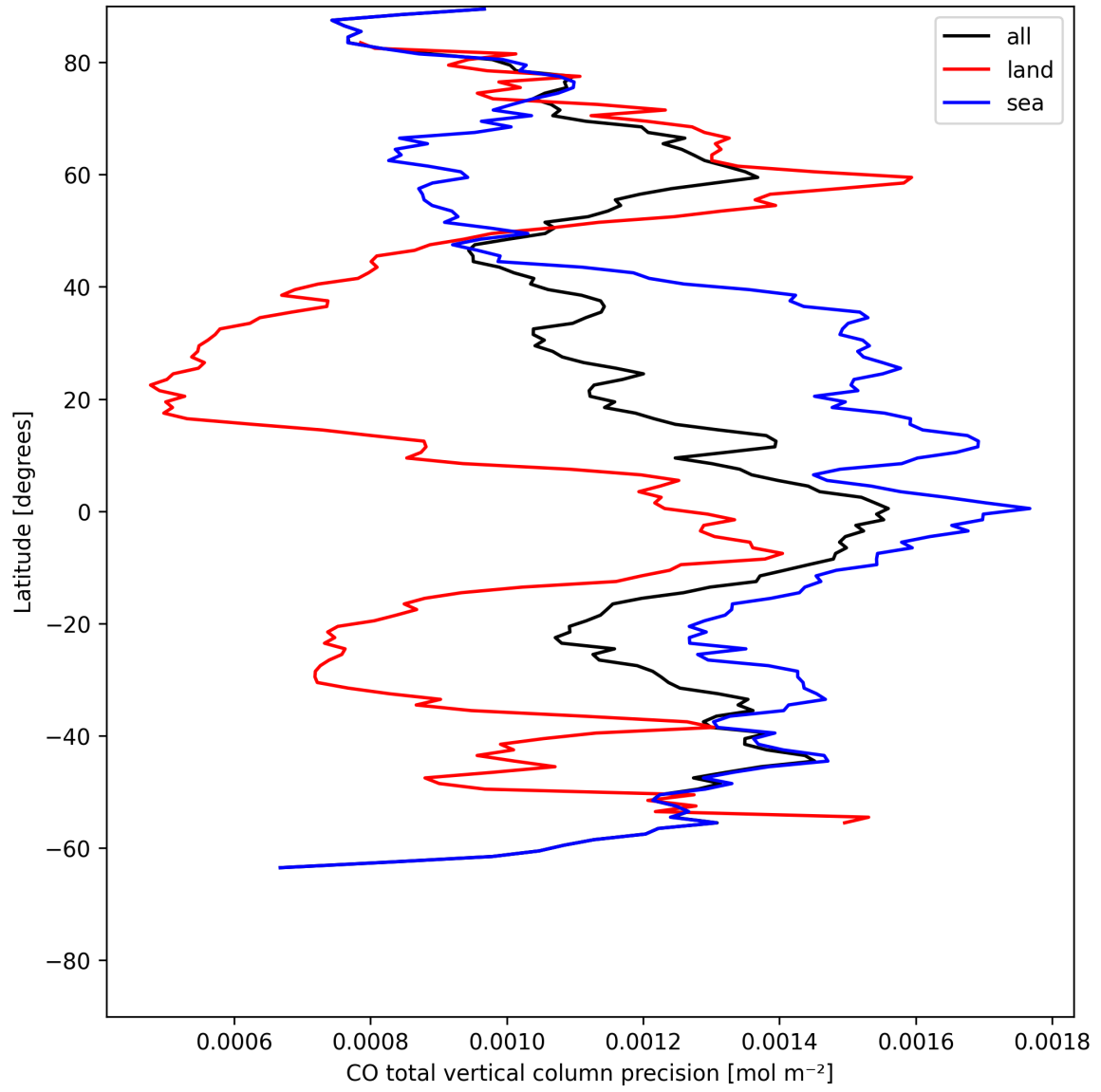
Figure 8: Zonal average of “CO total vertical column precision” for 2025-07-19 to 2025-07-20.
