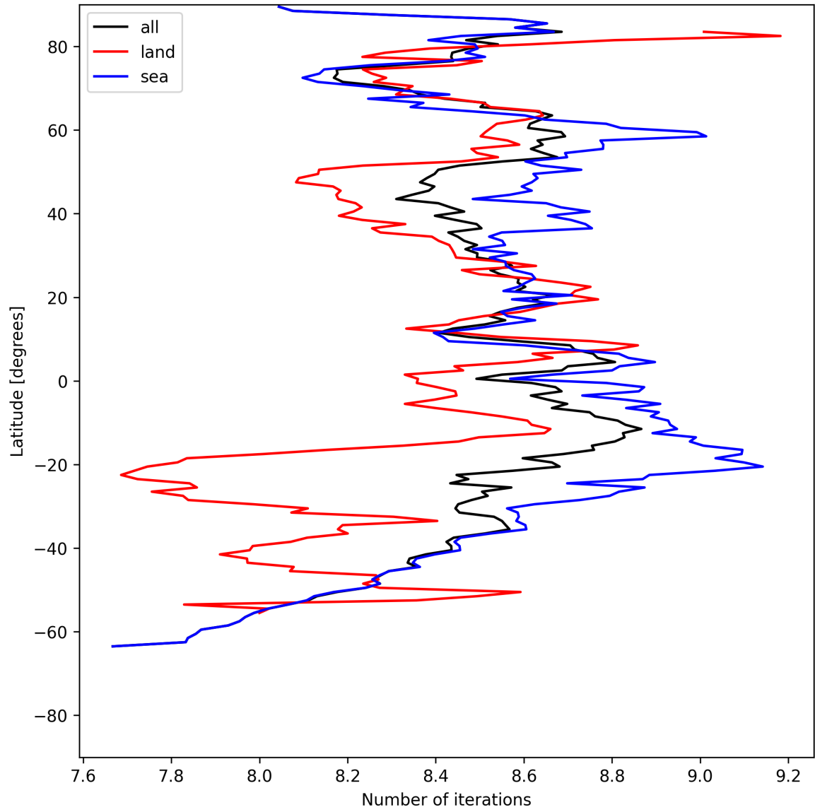
Figure 12: Zonal average of “Number of iterations” for 2025-07-19 to 2025-07-20.
