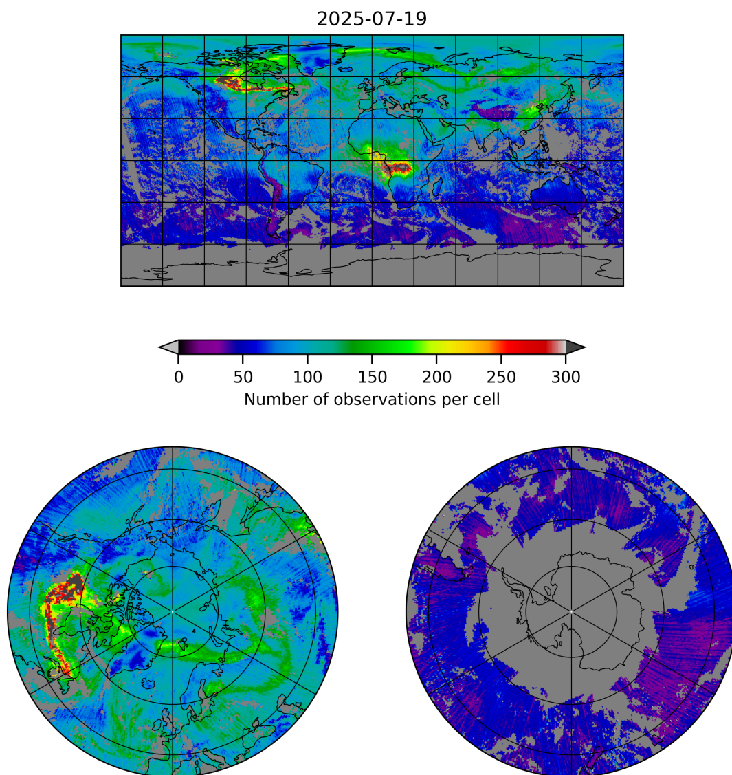
Figure 5: Map of the number of observations for 2025-07-19 to 2025-07-20
