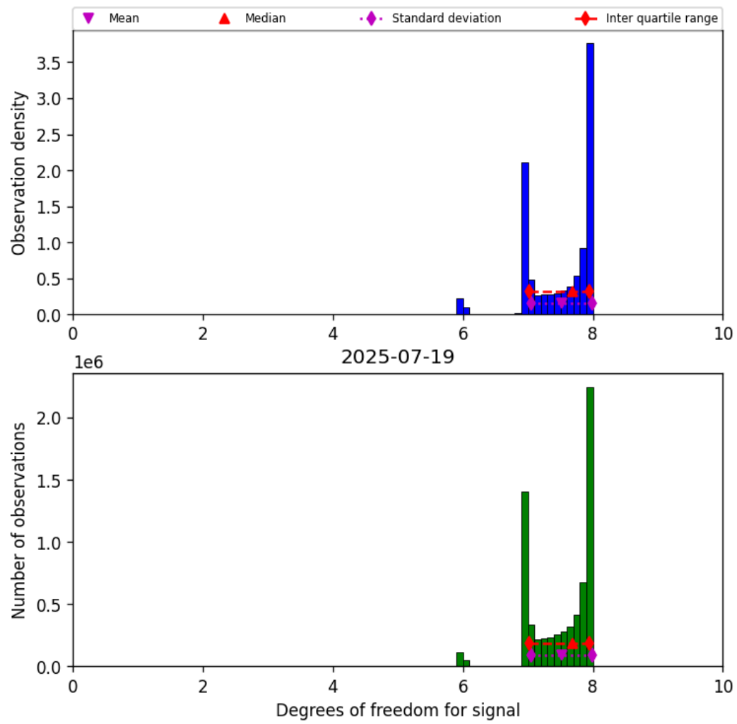
Figure 18: Histogram of “Degrees of freedom for signal” for 2025-07-19 to 2025-07-20
