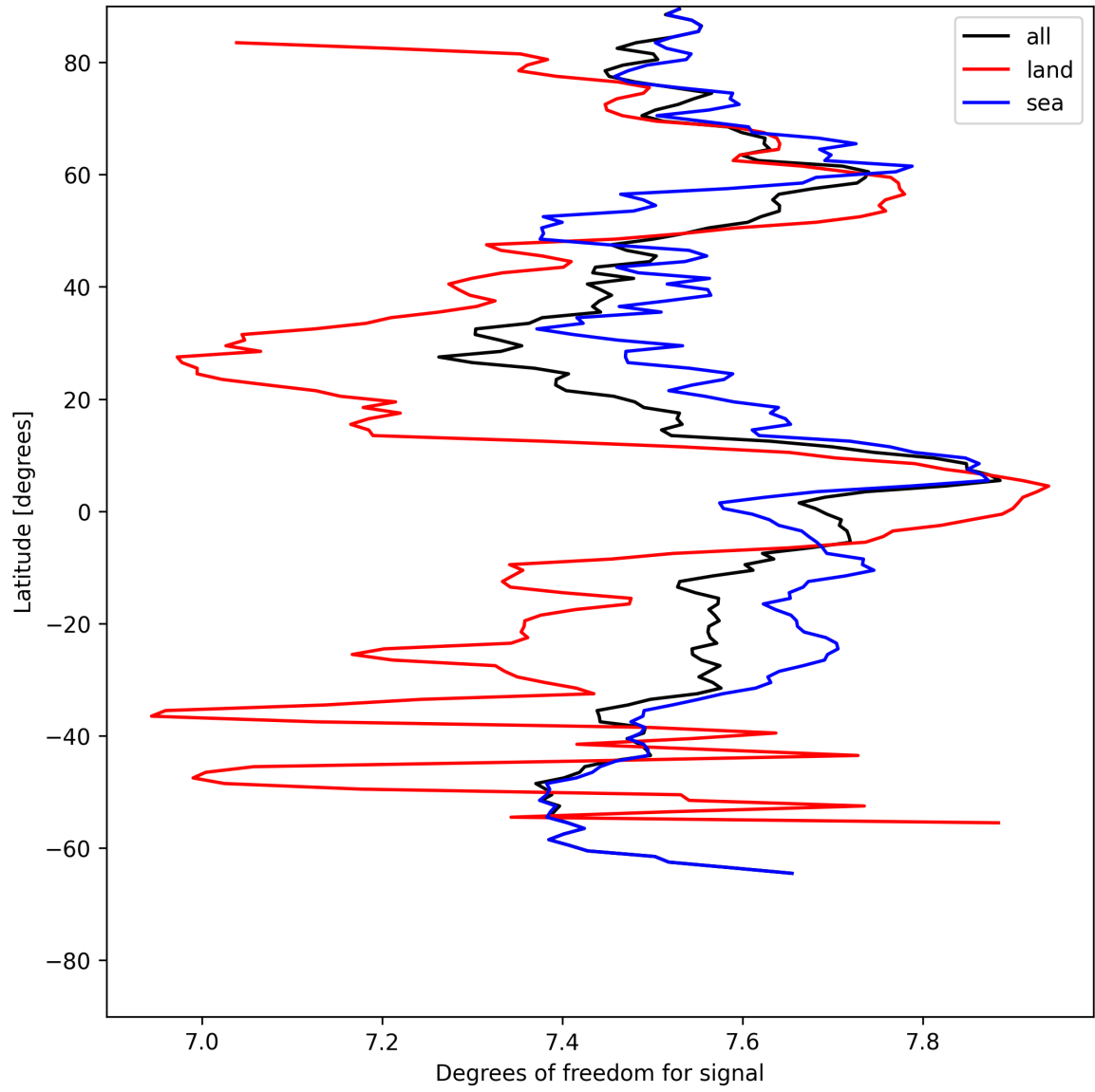
Figure 11: Zonal average of “Degrees of freedom for signal” for 2025-07-21 to 2025-07-22.
