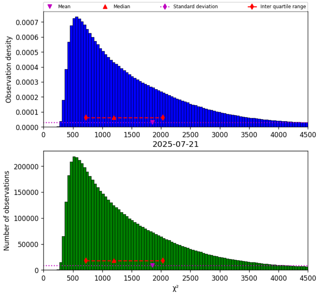
Figure 17: Histogram of “ \chi^2 ” for 2025-07-21 to 2025-07-22
