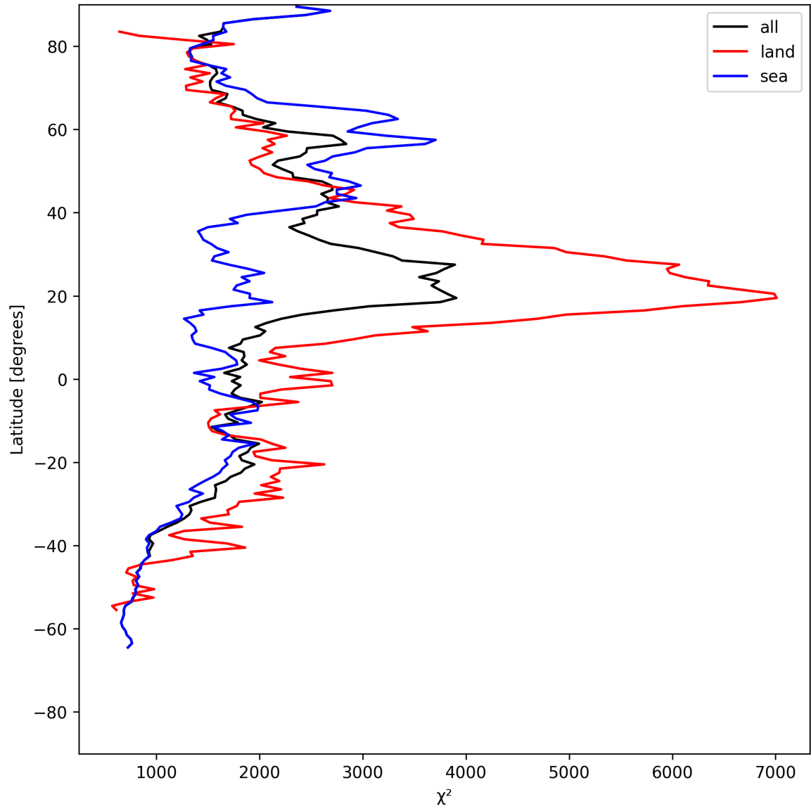
Figure 10: Zonal average of “ \chi^2 ” for 2025-07-21 to 2025-07-22.
