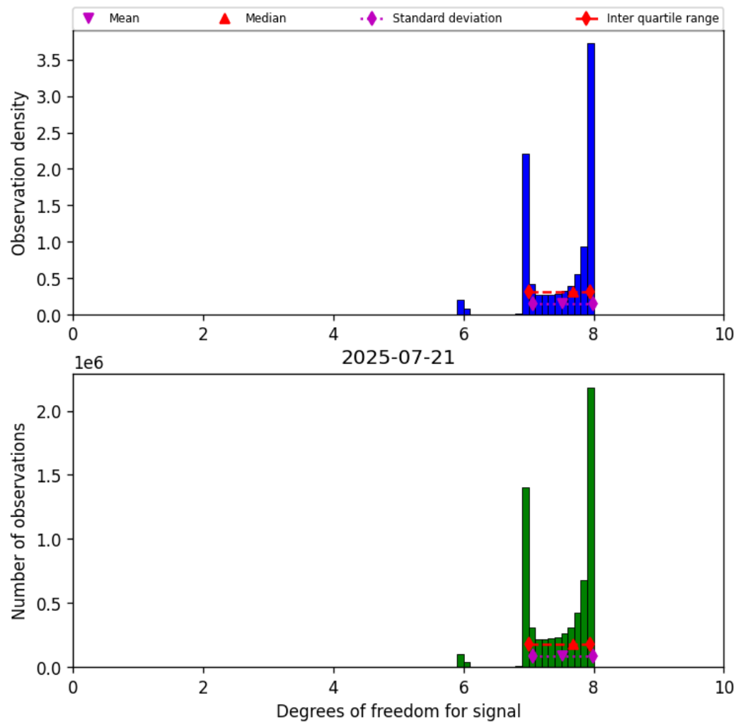
Figure 18: Histogram of “Degrees of freedom for signal” for 2025-07-21 to 2025-07-22
