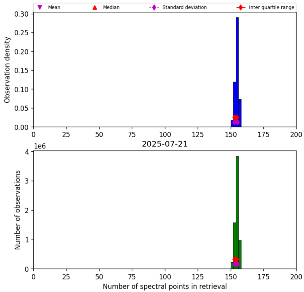
Figure 16: Histogram of “Number of spectral points in retrieval” for 2025-07-21 to 2025-07-22
