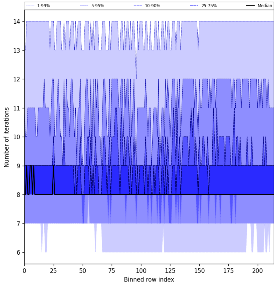
Figure 26: Along track statistics of “Number of iterations” for 2025-07-21 to 2025-07-22
