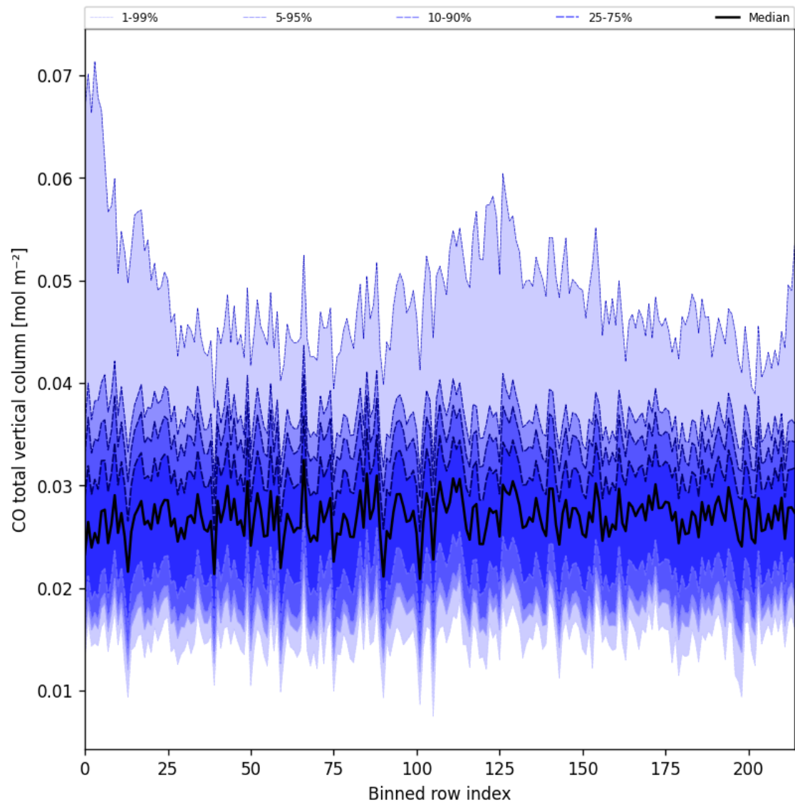
Figure 21: Along track statistics of “CO total vertical column” for 2025-07-21 to 2025-07-22
