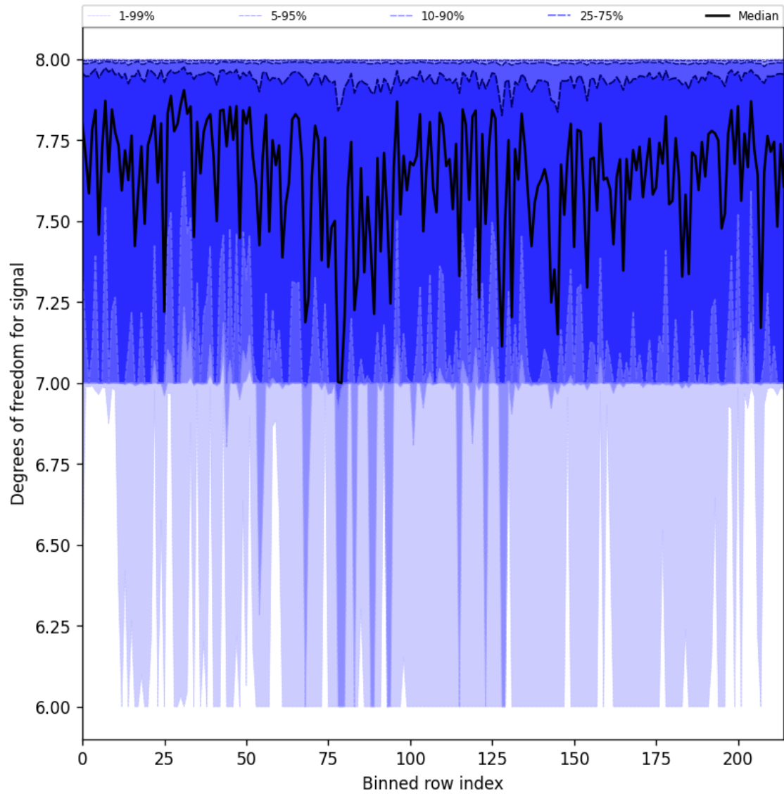
Figure 25: Along track statistics of “Degrees of freedom for signal” for 2025-07-21 to 2025-07-22
