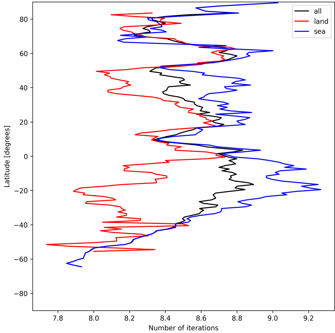
Figure 12: Zonal average of “Number of iterations” for 2025-07-21 to 2025-07-22.
