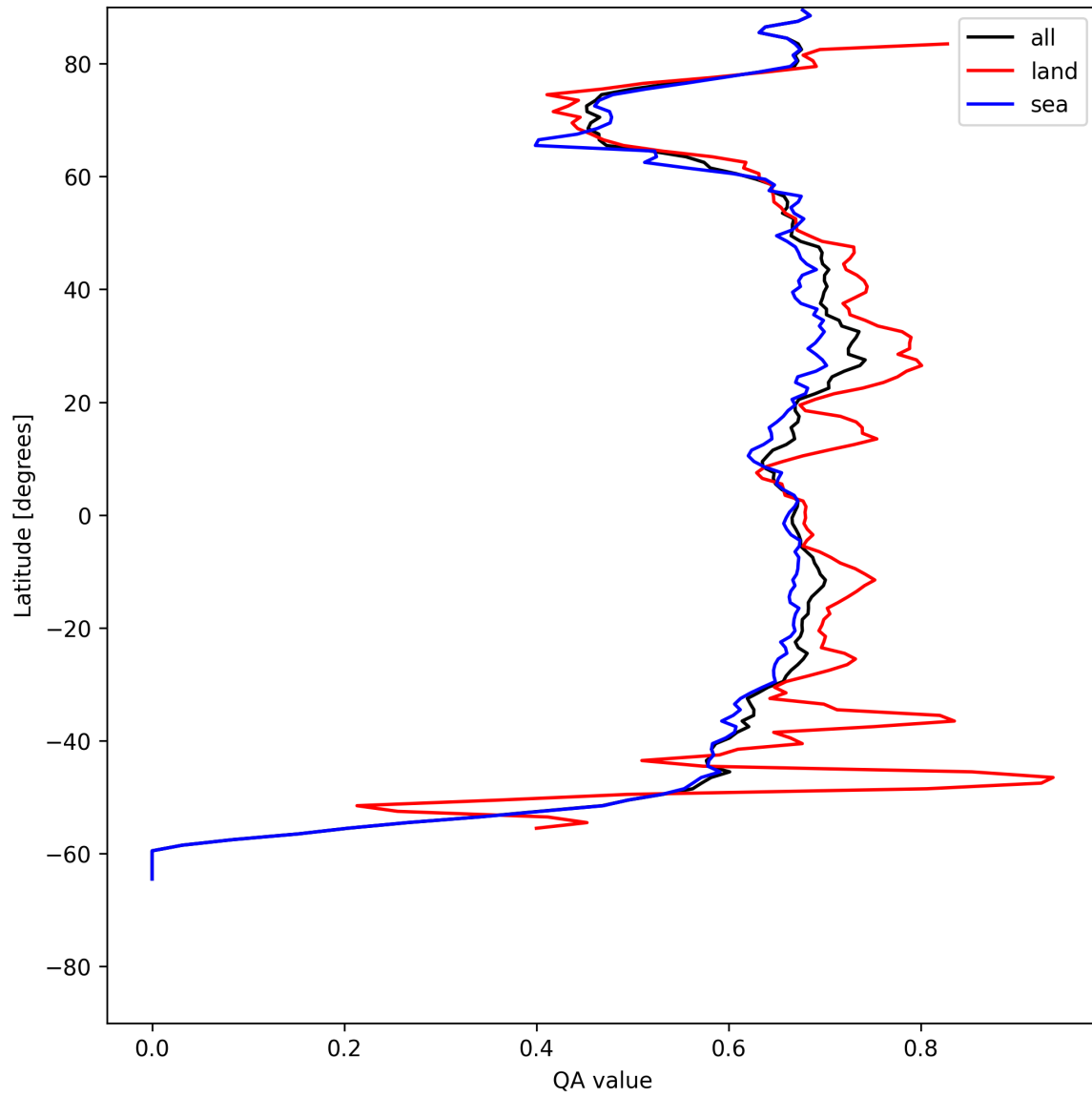
Figure 6: Zonal average of “QA value” for 2025-07-21 to 2025-07-22.
