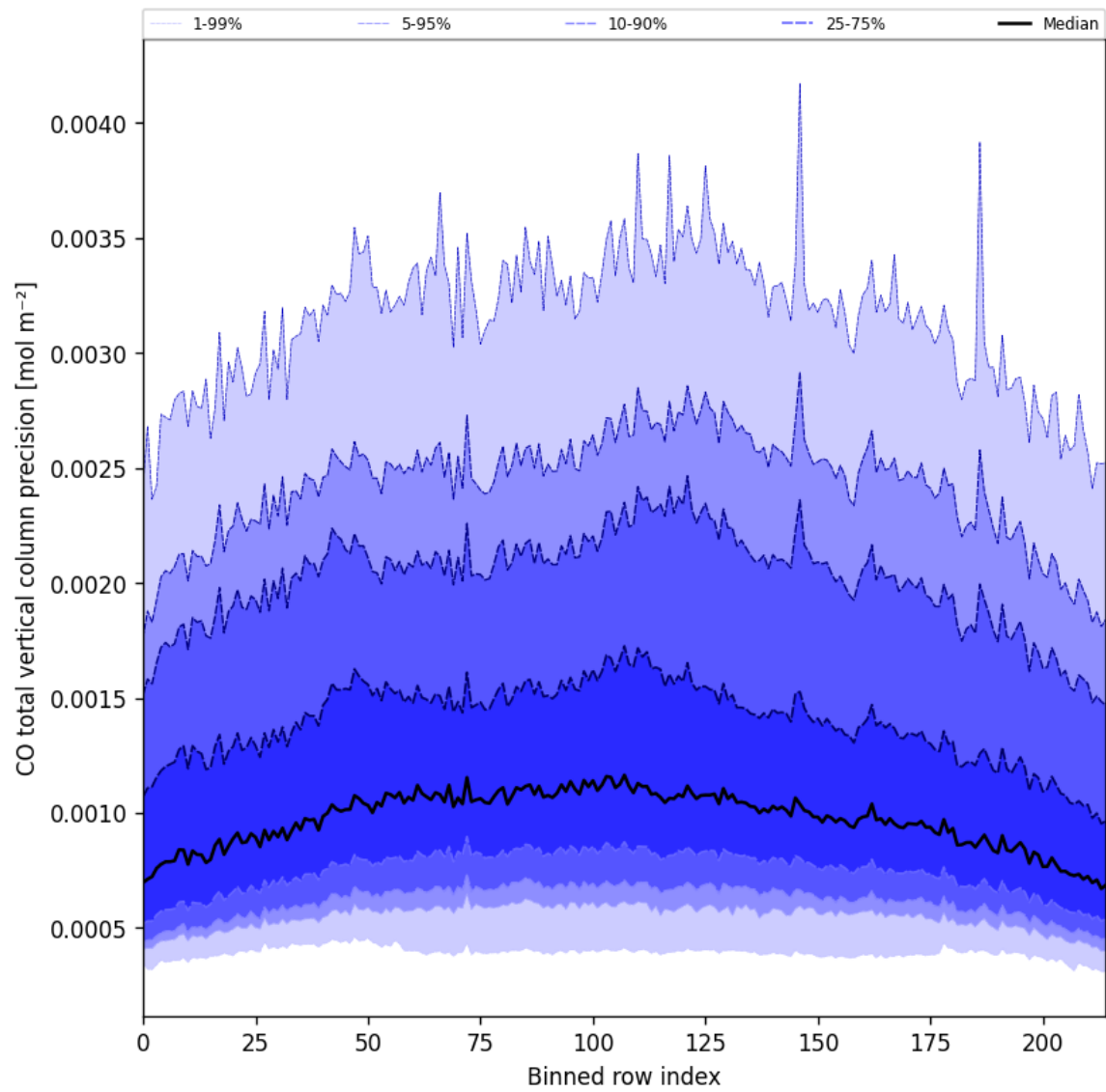
Figure 22: Along track statistics of “CO total vertical column precision” for 2025-07-21 to 2025-07-22
