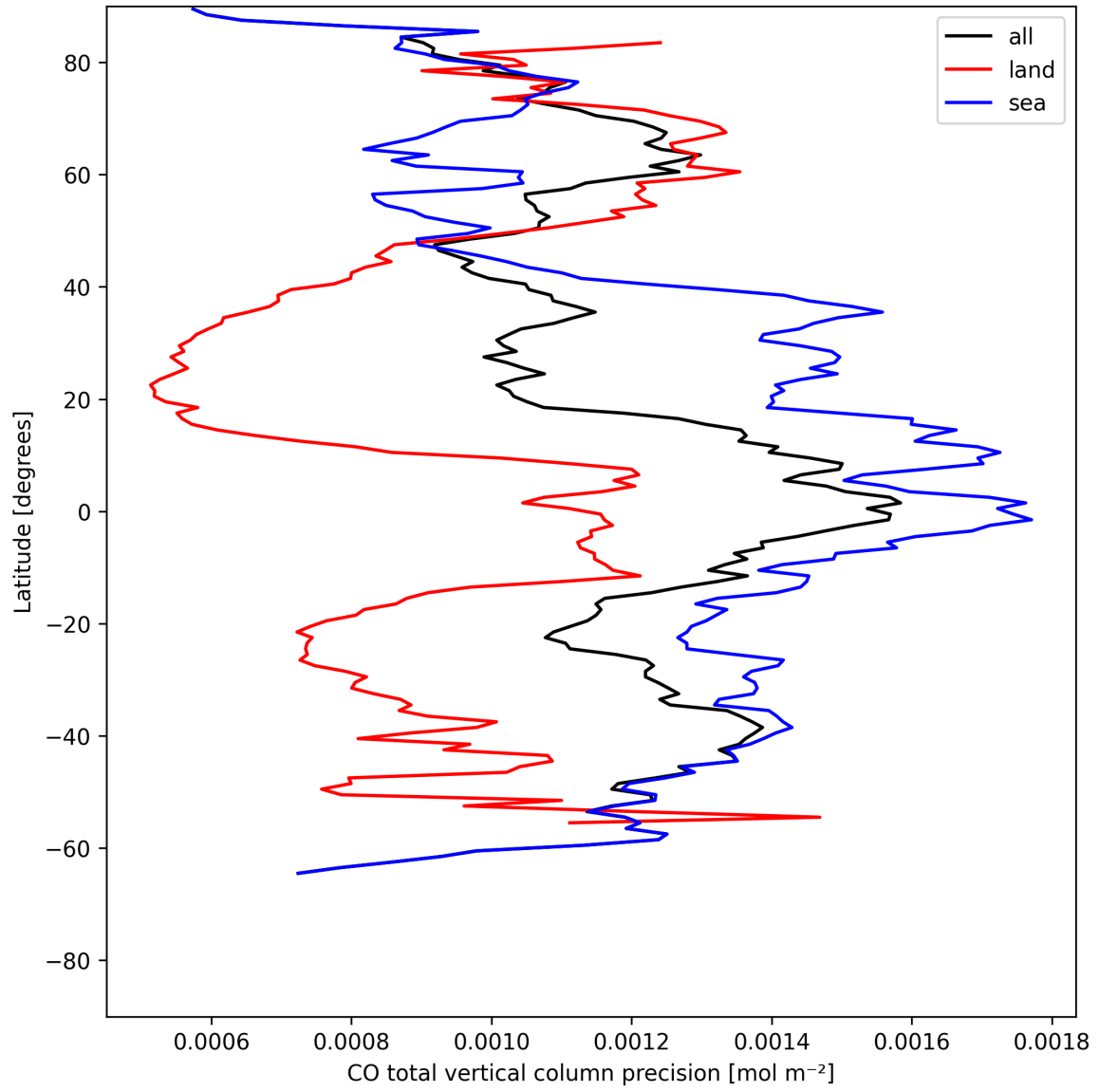
Figure 8: Zonal average of “CO total vertical column precision” for 2025-07-21 to 2025-07-22.
