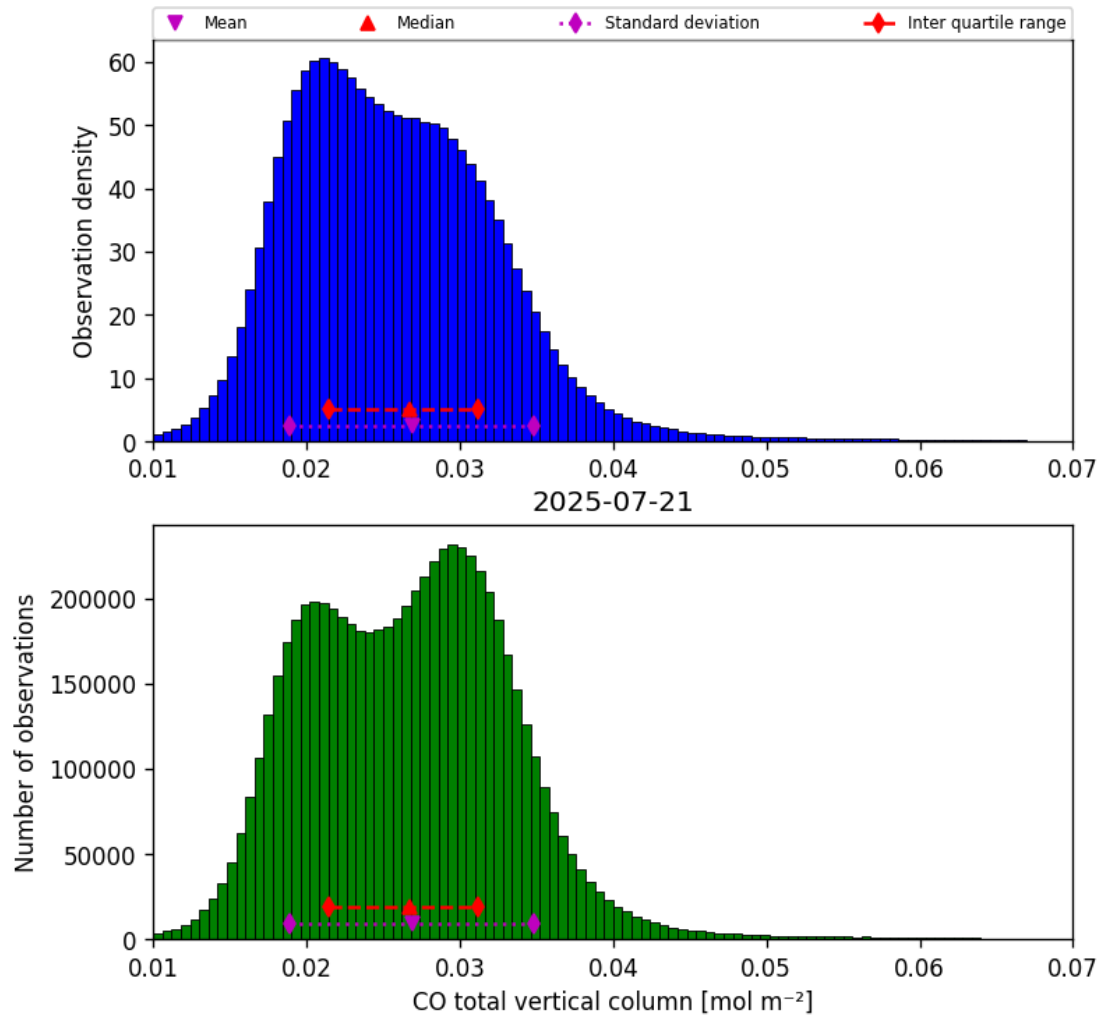
Figure 14: Histogram of “CO total vertical column” for 2025-07-21 to 2025-07-22
