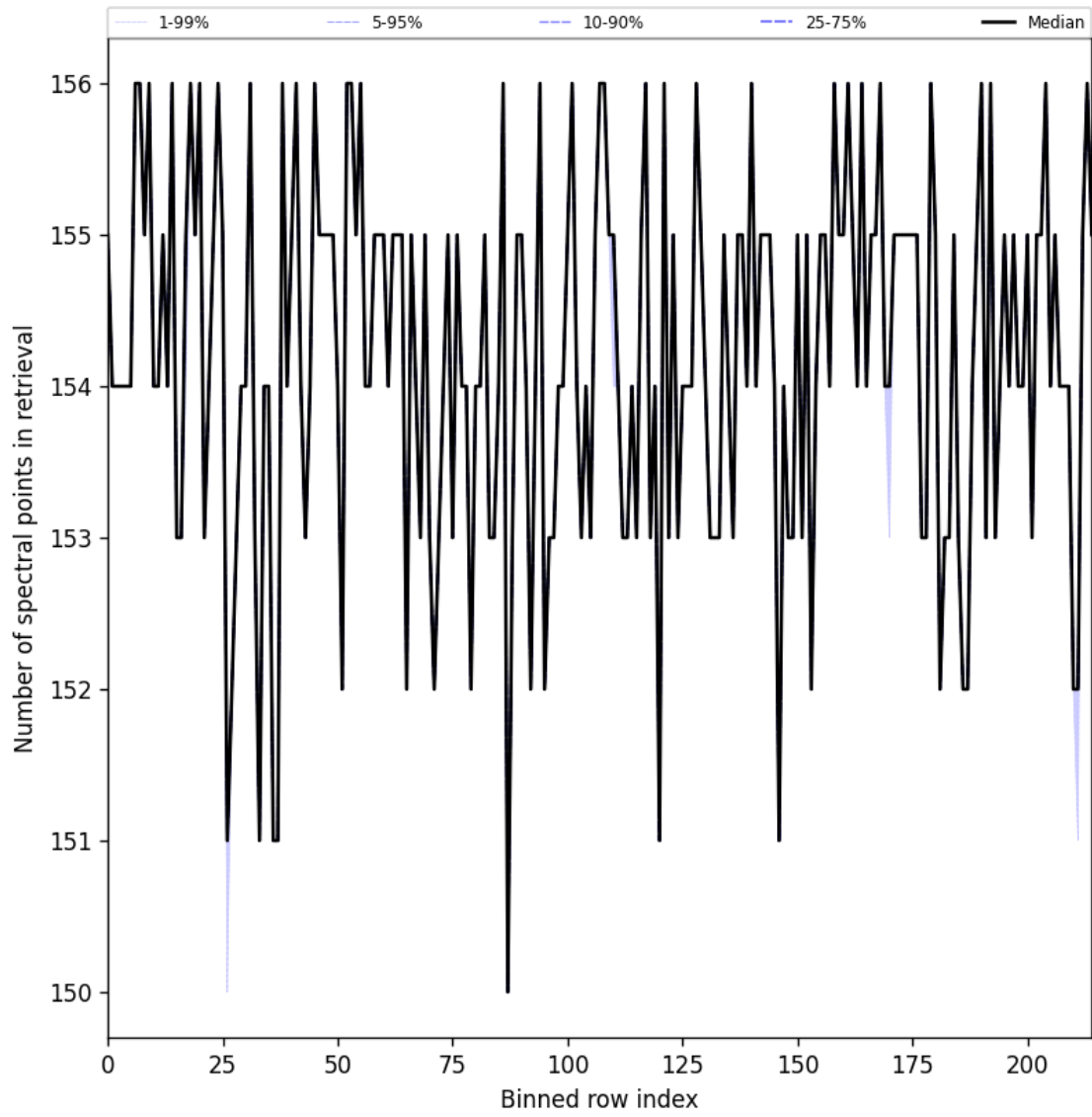
Figure 23: Along track statistics of “Number of spectral points in retrieval” for 2025-07-21 to 2025-07-22
