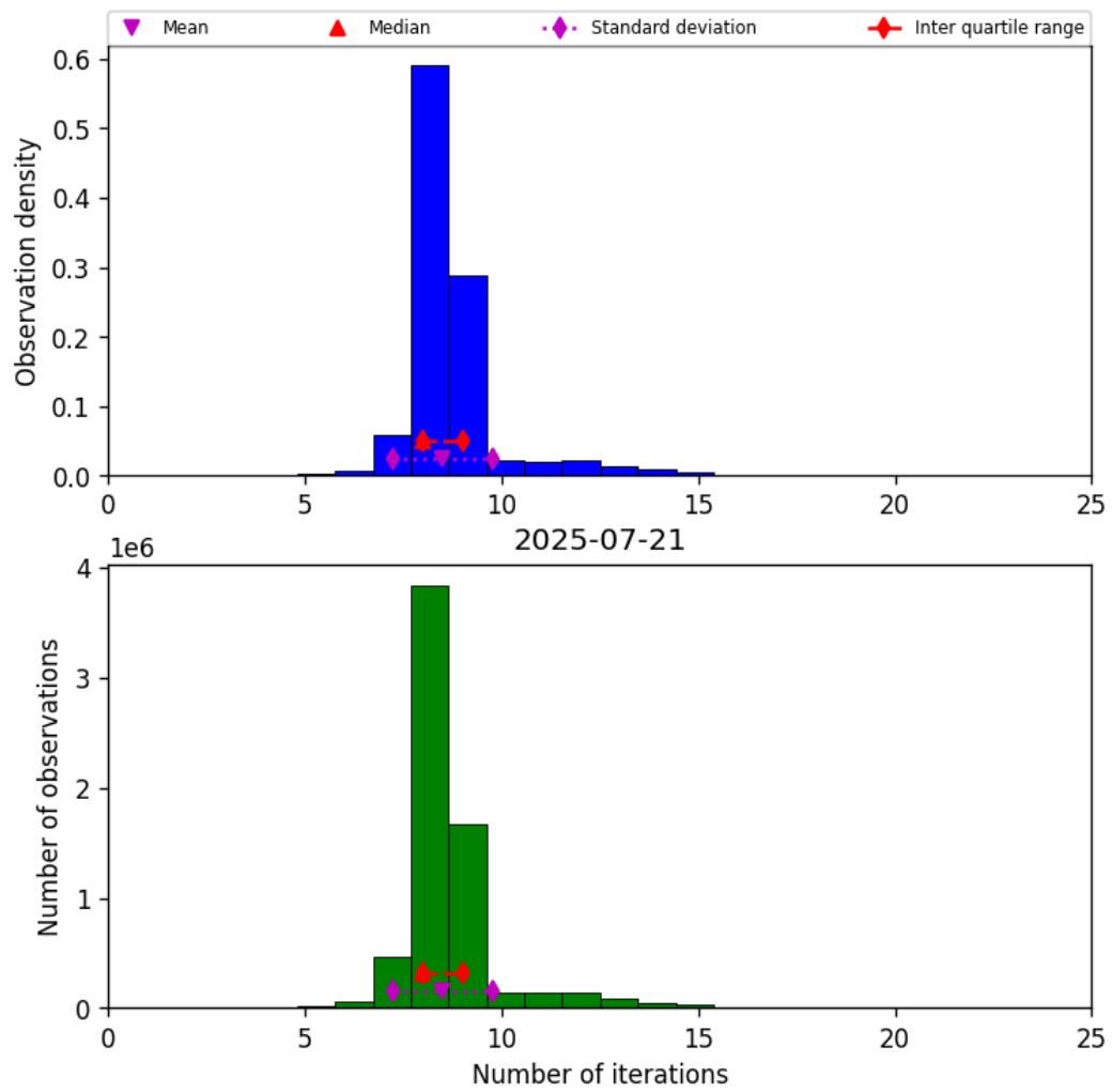
Figure 19: Histogram of “Number of iterations” for 2025-07-21 to 2025-07-22
