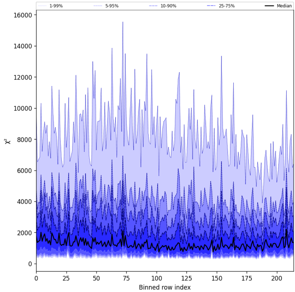
Figure 24: Along track statistics of “ \chi^2 ” for 2025-07-21 to 2025-07-22
