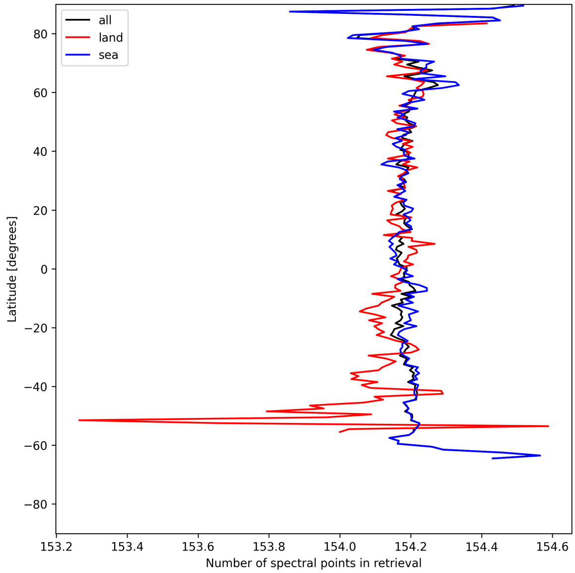
Figure 9: Zonal average of “Number of spectral points in retrieval” for 2025-07-21 to 2025-07-22.
