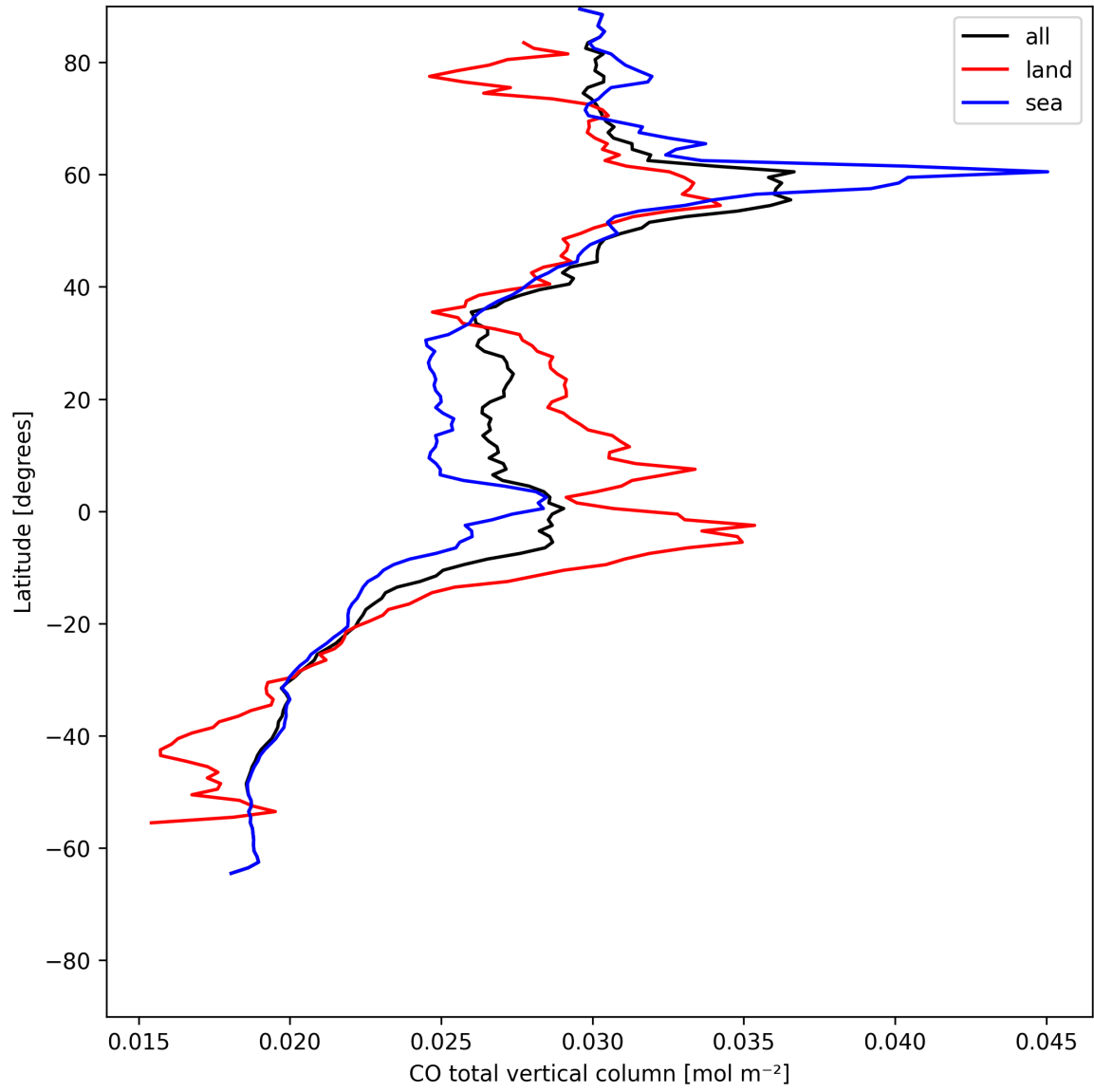
Figure 7: Zonal average of “CO total vertical column” for 2025-07-21 to 2025-07-22.
