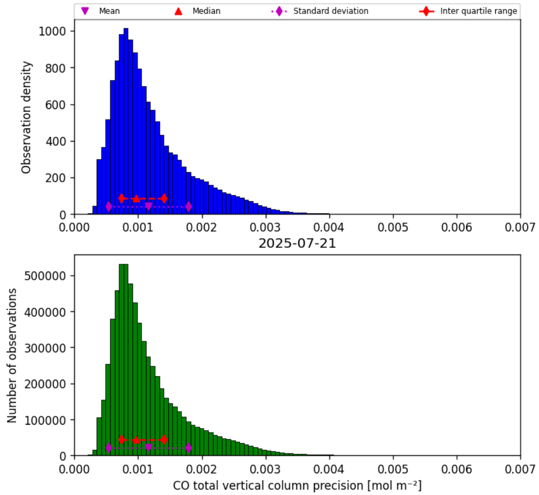
Figure 15: Histogram of “CO total vertical column precision” for 2025-07-21 to 2025-07-22
