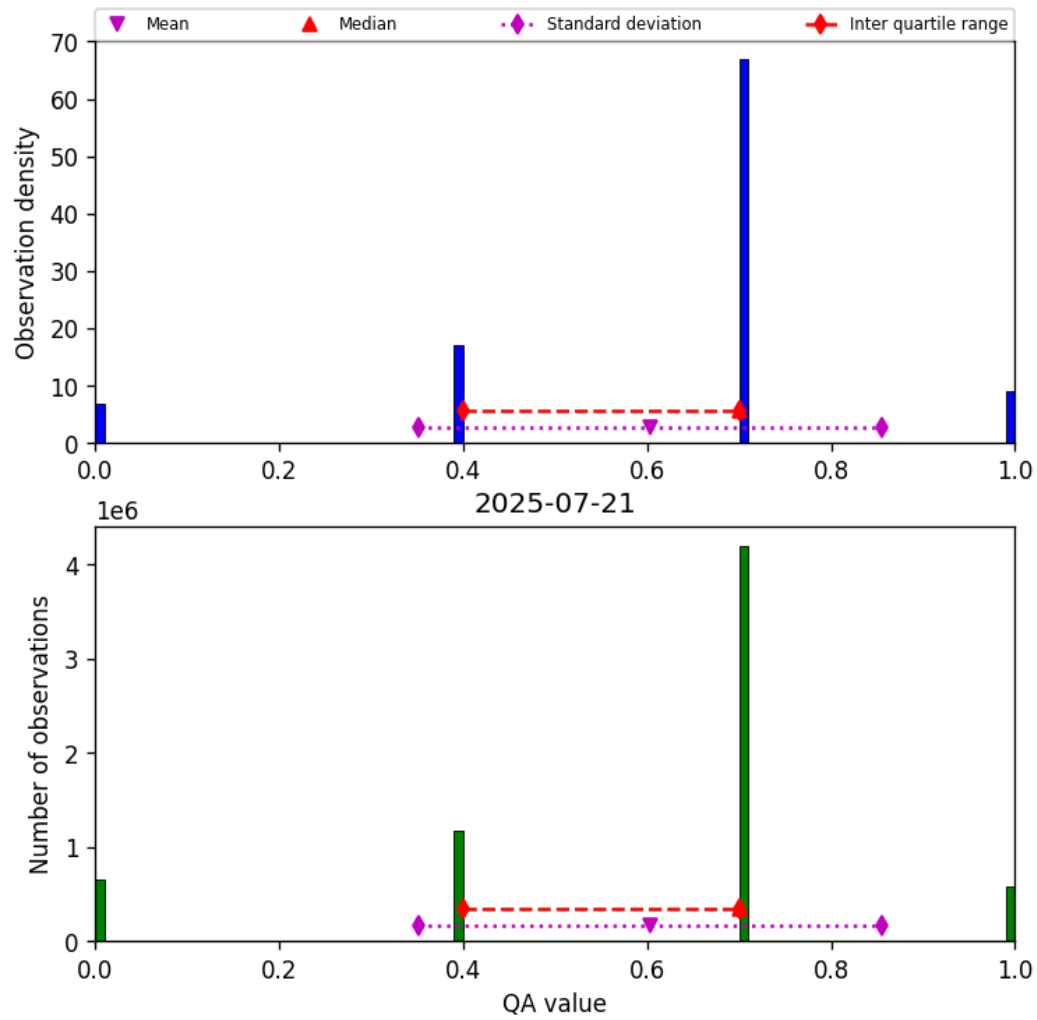
Figure 13: Histogram of “QA value” for 2025-07-21 to 2025-07-22
