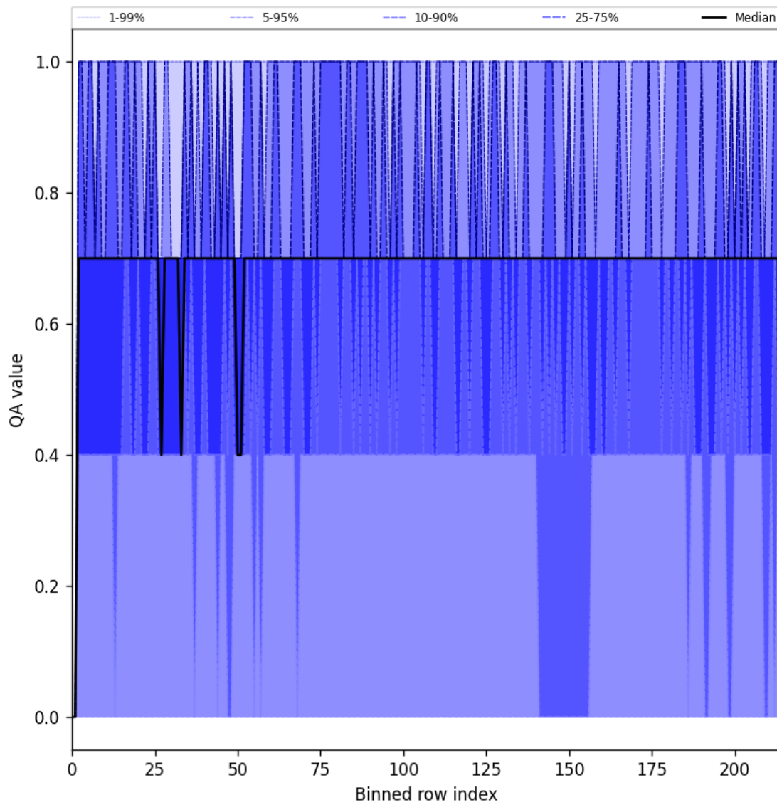
Figure 20: Along track statistics of “QA value” for 2025-07-21 to 2025-07-22
