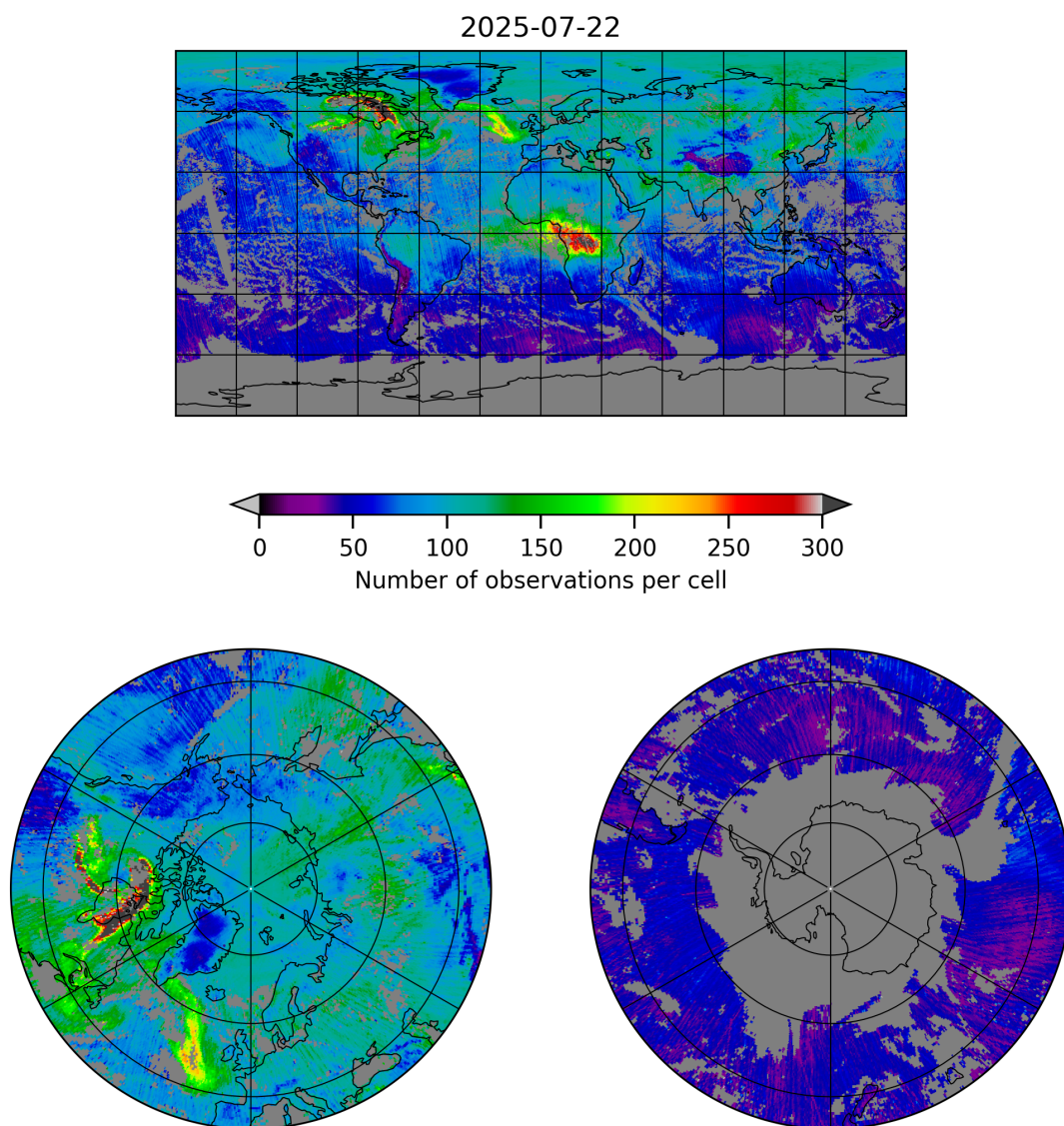
Figure 5: Map of the number of observations for 2025-07-22 to 2025-07-22
