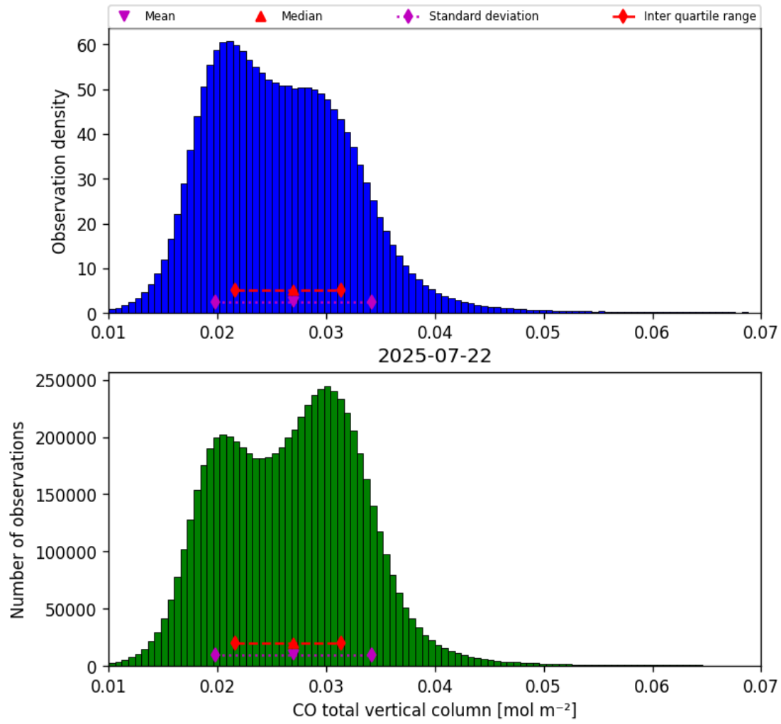
Figure 14: Histogram of “CO total vertical column” for 2025-07-22 to 2025-07-22
