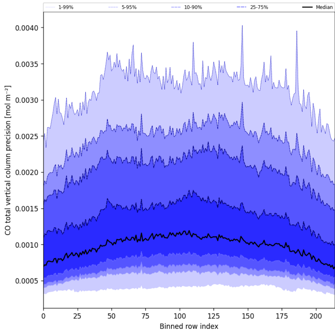
Figure 22: Along track statistics of “CO total vertical column precision” for 2025-07-22 to 2025-07-22
