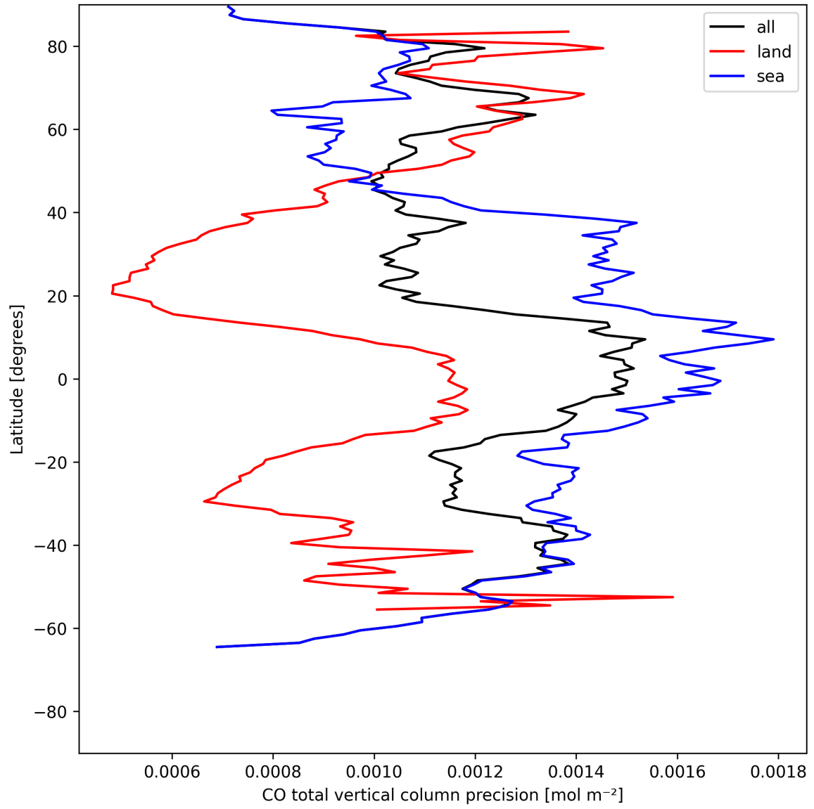
Figure 8: Zonal average of “CO total vertical column precision” for 2025-07-22 to 2025-07-22.
