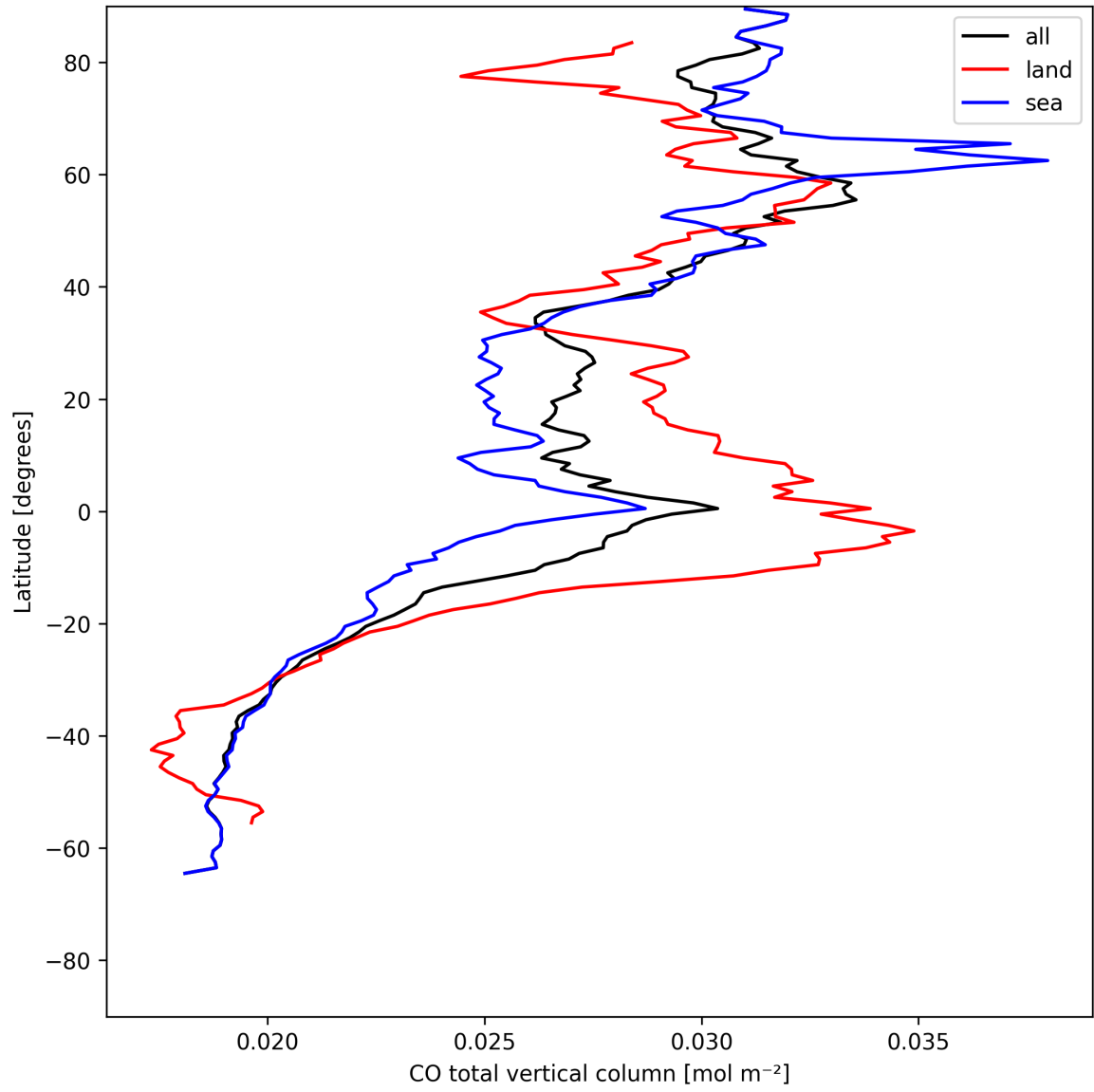
Figure 7: Zonal average of “CO total vertical column” for 2025-07-22 to 2025-07-22.
