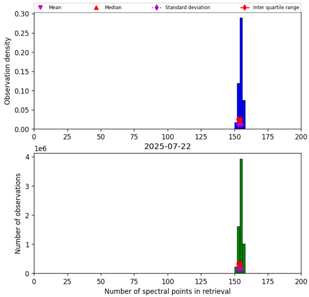
Figure 16: Histogram of “Number of spectral points in retrieval” for 2025-07-22 to 2025-07-22
