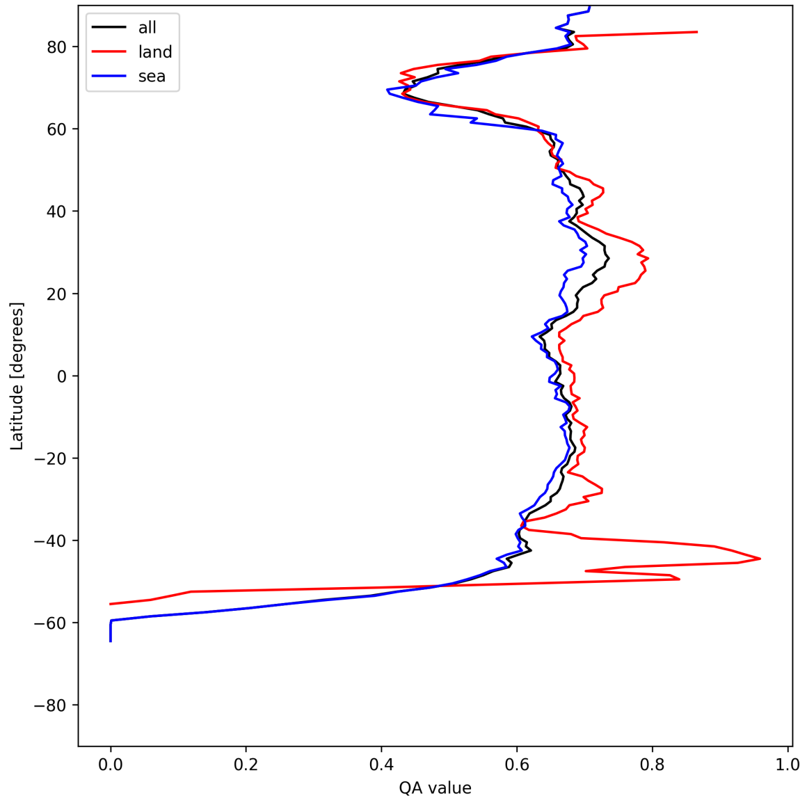
Figure 6: Zonal average of “QA value” for 2025-07-22 to 2025-07-22.
