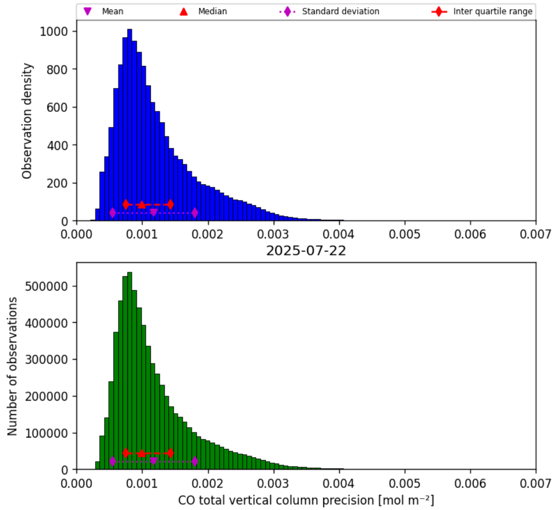
Figure 15: Histogram of “CO total vertical column precision” for 2025-07-22 to 2025-07-22
