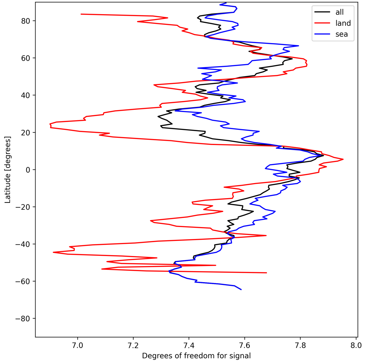
Figure 11: Zonal average of “Degrees of freedom for signal” for 2025-07-22 to 2025-07-22.
