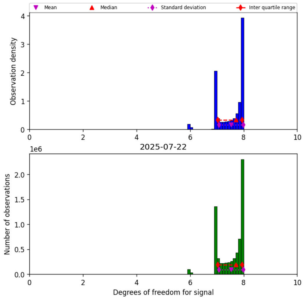
Figure 18: Histogram of “Degrees of freedom for signal” for 2025-07-22 to 2025-07-22
