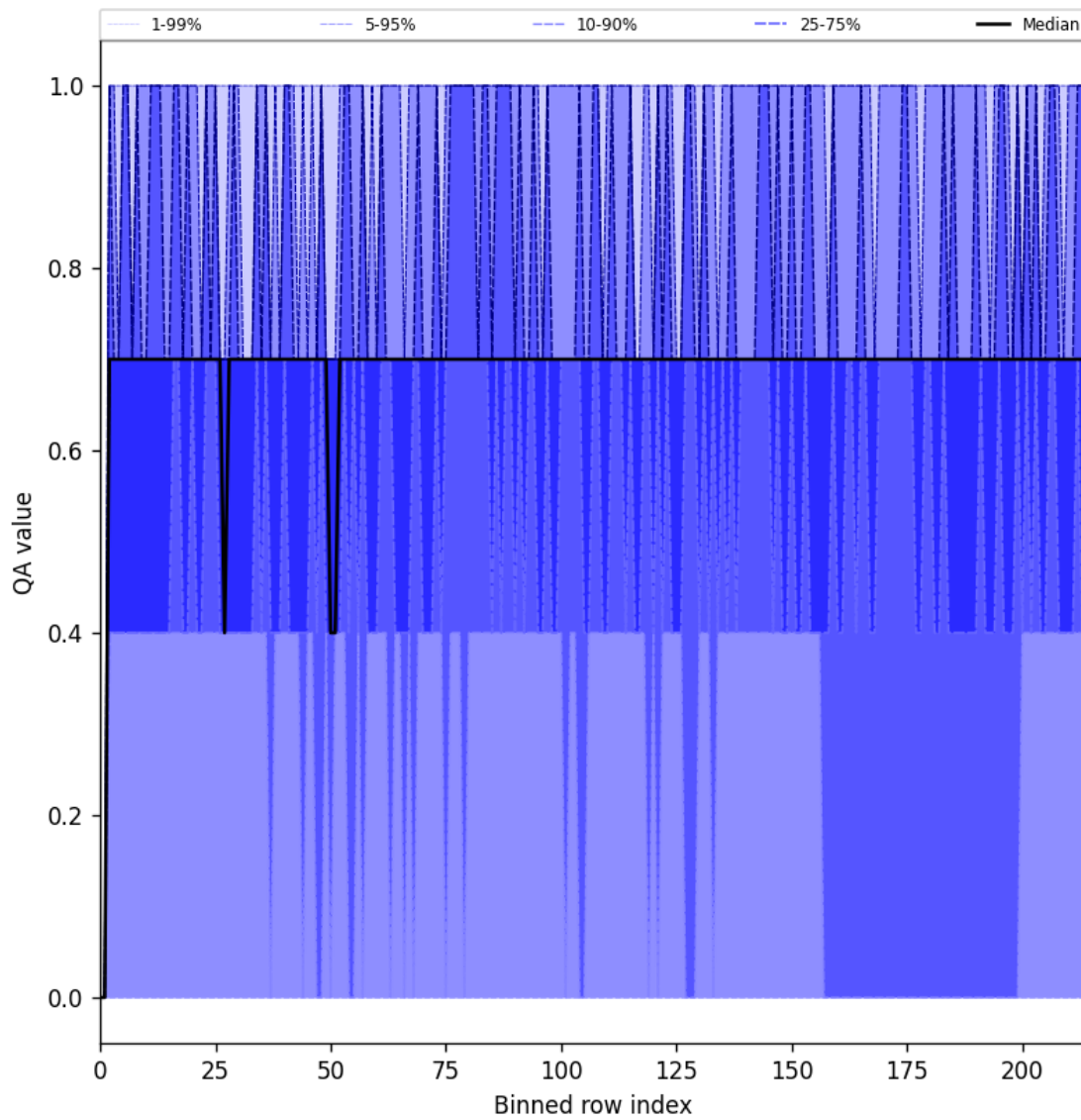
Figure 20: Along track statistics of “QA value” for 2025-07-22 to 2025-07-22
