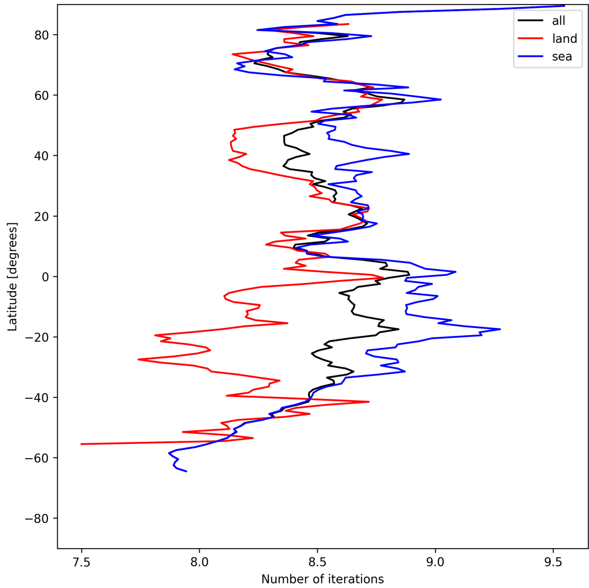
Figure 12: Zonal average of “Number of iterations” for 2025-07-22 to 2025-07-22.
