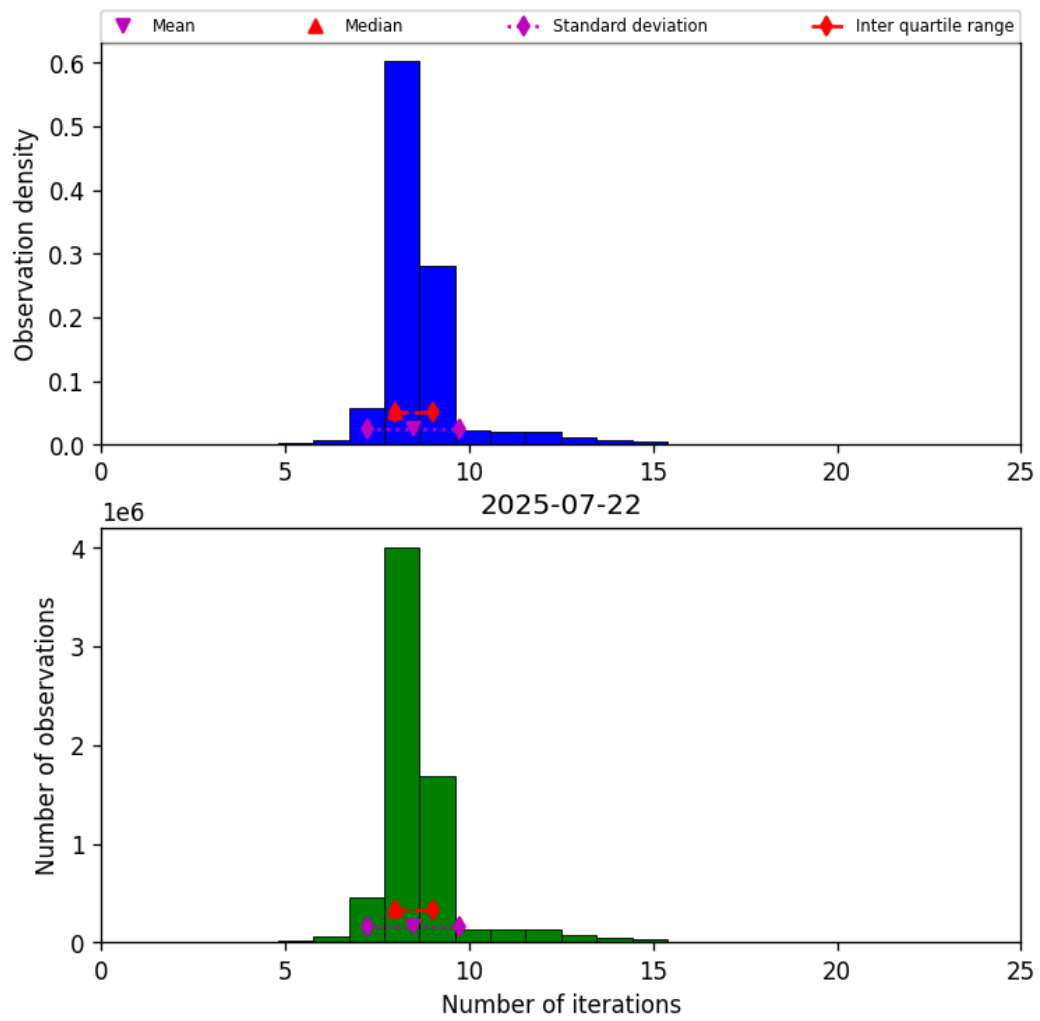
Figure 19: Histogram of “Number of iterations” for 2025-07-22 to 2025-07-22
