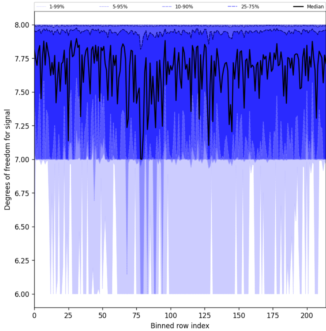
Figure 25: Along track statistics of “Degrees of freedom for signal” for 2025-07-22 to 2025-07-22
