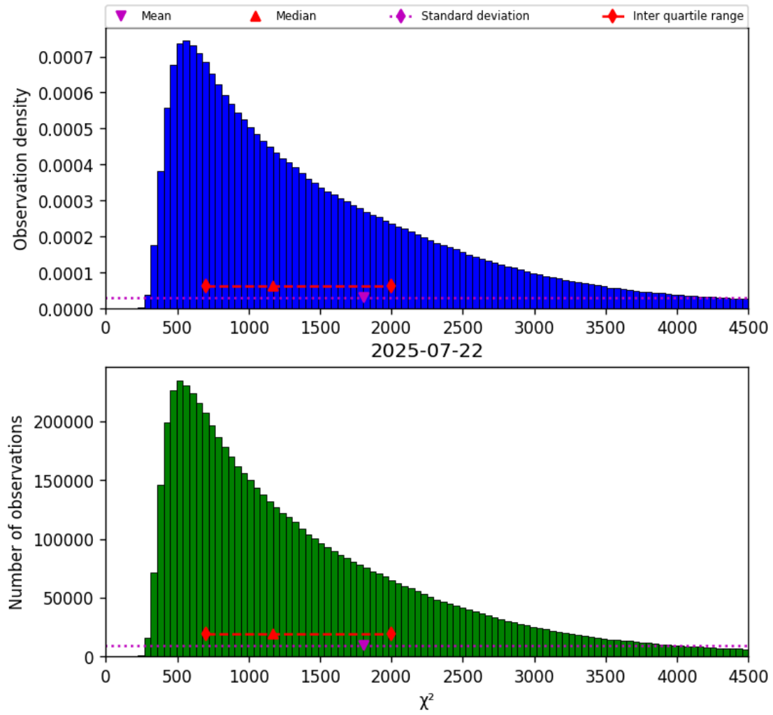
Figure 17: Histogram of “ \chi^2 ” for 2025-07-22 to 2025-07-22
