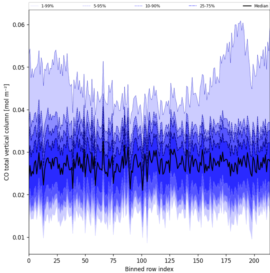
Figure 21: Along track statistics of “CO total vertical column” for 2025-07-22 to 2025-07-22
