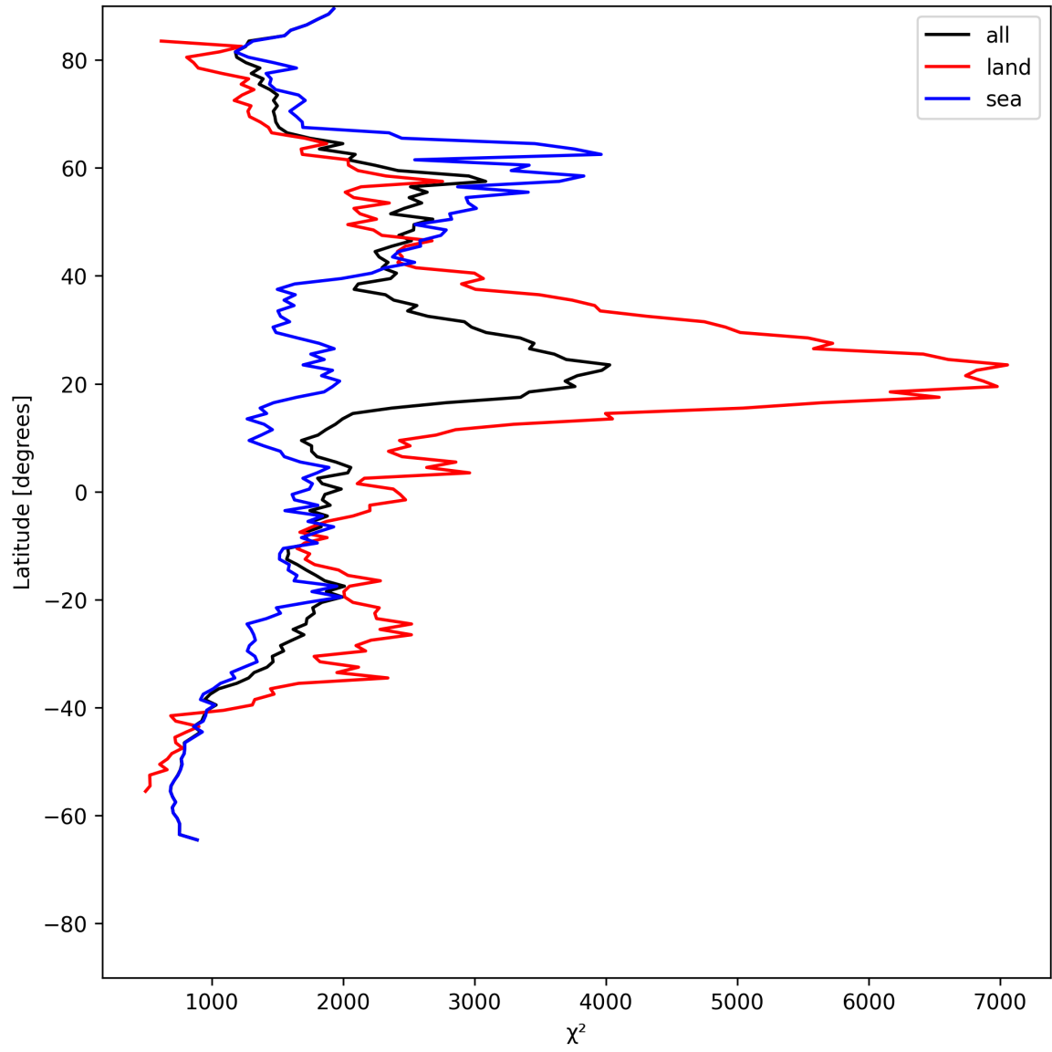
Figure 10: Zonal average of “ \chi^2 ” for 2025-07-22 to 2025-07-22.
