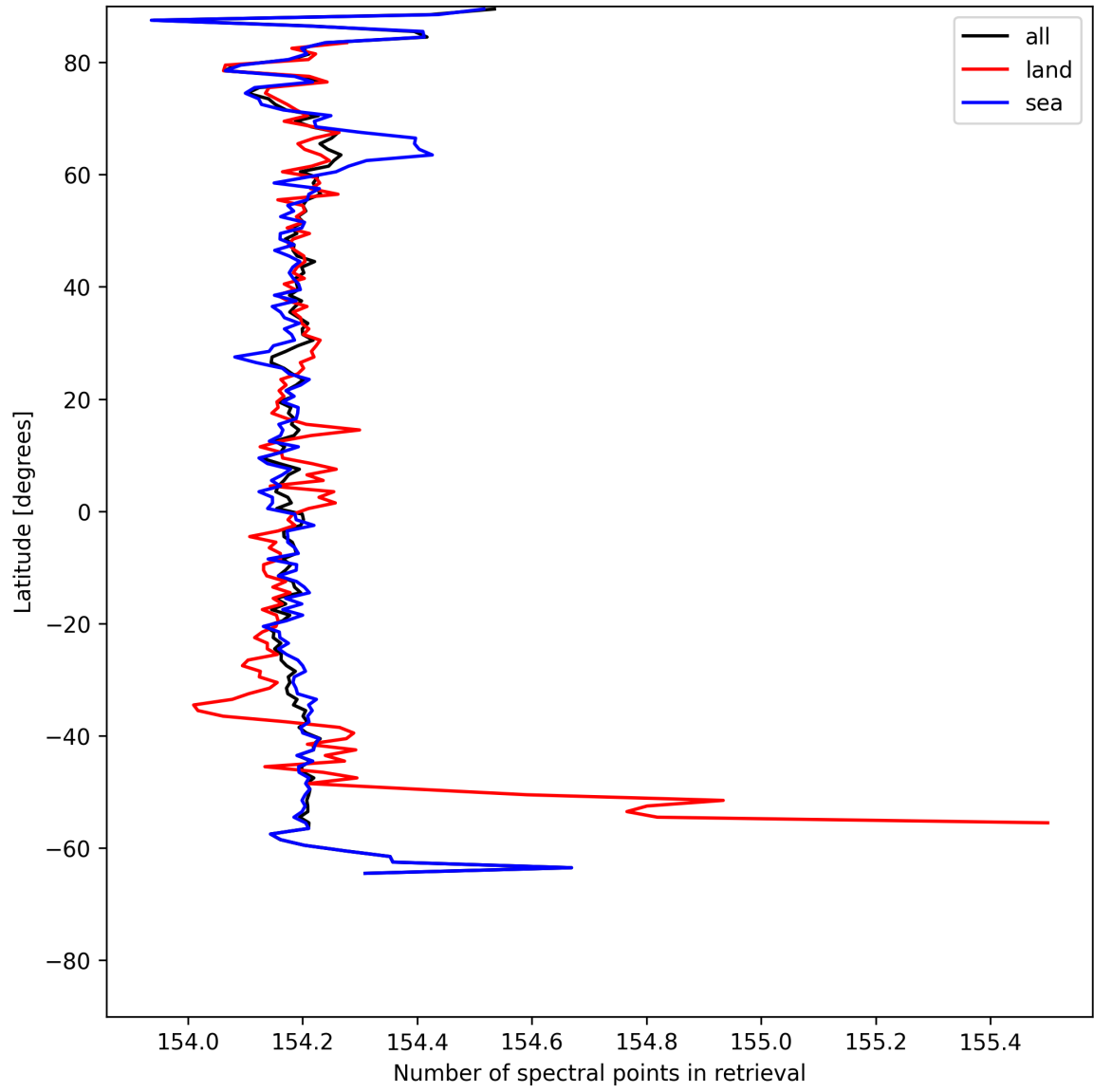
Figure 9: Zonal average of “Number of spectral points in retrieval” for 2025-07-22 to 2025-07-22.
