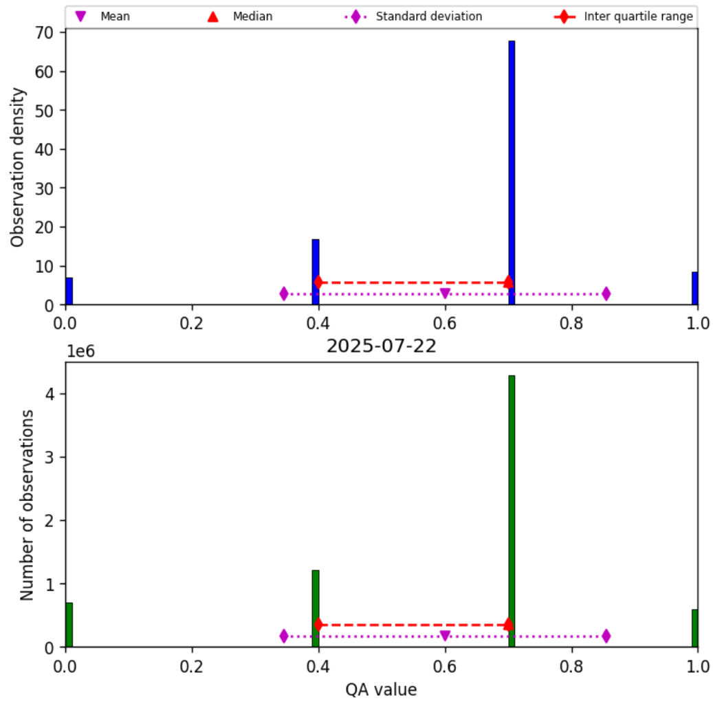
Figure 13: Histogram of “QA value” for 2025-07-22 to 2025-07-22
