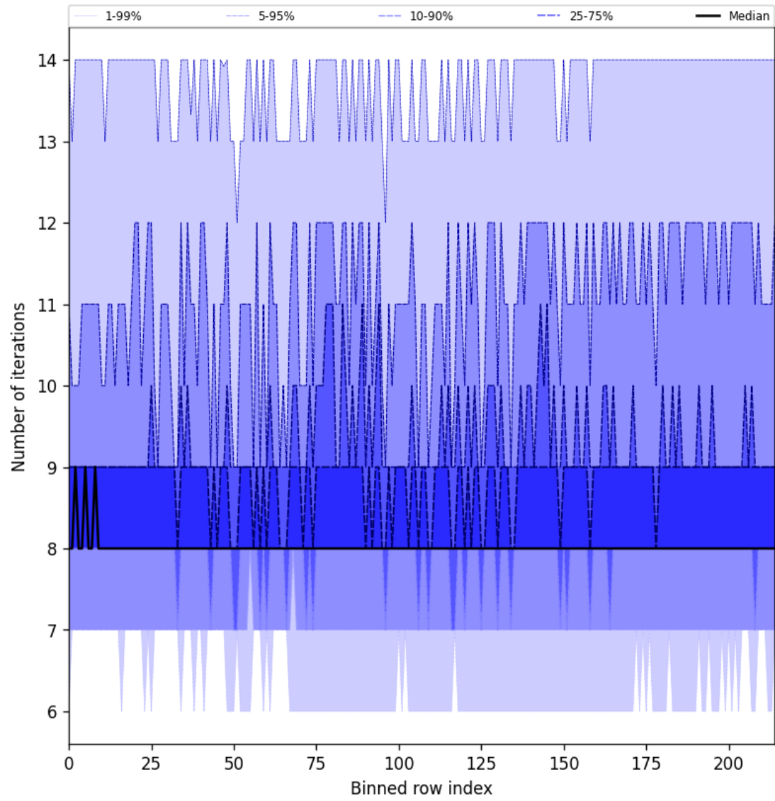
Figure 26: Along track statistics of “Number of iterations” for 2025-07-22 to 2025-07-22
