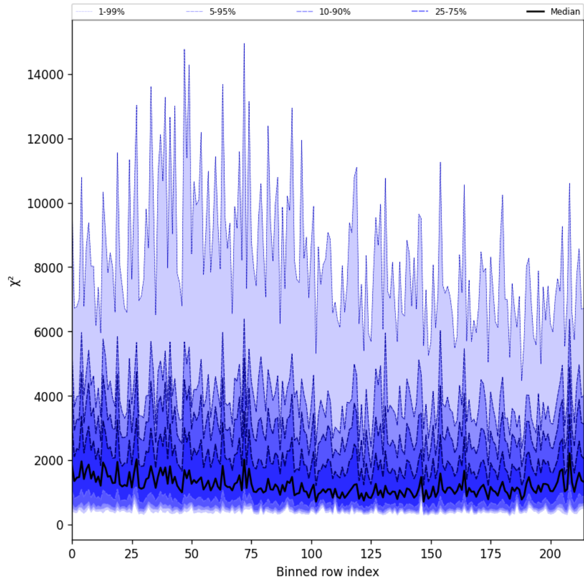
Figure 24: Along track statistics of “ \chi^2 ” for 2025-07-22 to 2025-07-22
