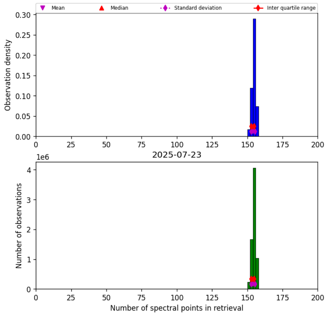
Figure 16: Histogram of “Number of spectral points in retrieval” for 2025-07-23 to 2025-07-24
