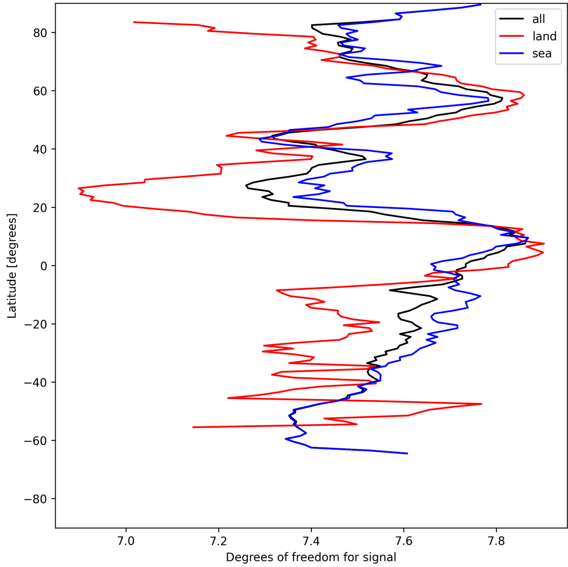
Figure 11: Zonal average of “Degrees of freedom for signal” for 2025-07-23 to 2025-07-24.
