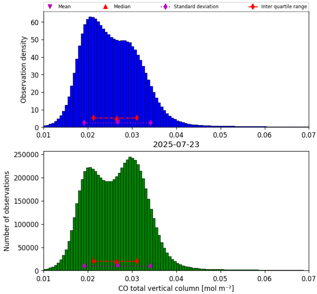
Figure 14: Histogram of “CO total vertical column” for 2025-07-23 to 2025-07-24
