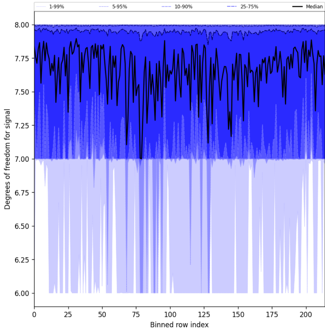
Figure 25: Along track statistics of “Degrees of freedom for signal” for 2025-07-23 to 2025-07-24
