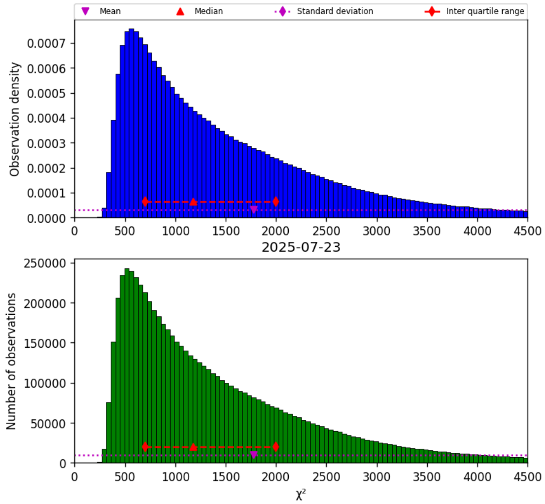
Figure 17: Histogram of “ \chi^2 ” for 2025-07-23 to 2025-07-24
