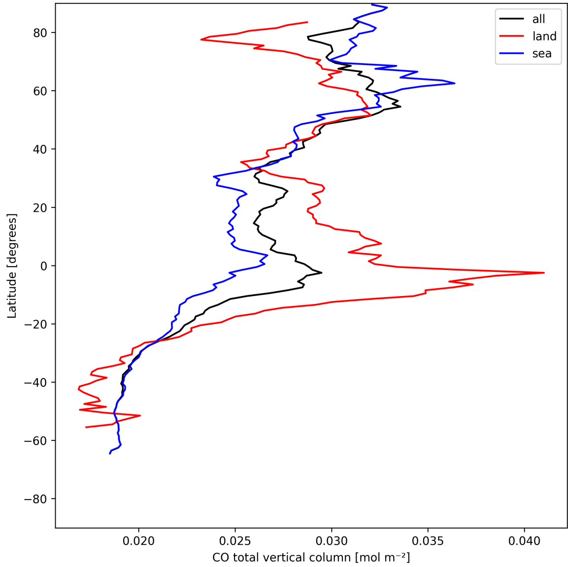
Figure 7: Zonal average of “CO total vertical column” for 2025-07-23 to 2025-07-24.
