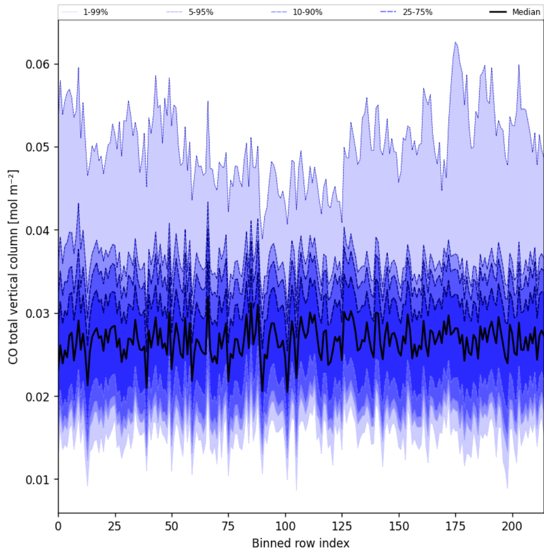
Figure 21: Along track statistics of "CO total vertical column" for 2025-07-23 to 2025-07-24
