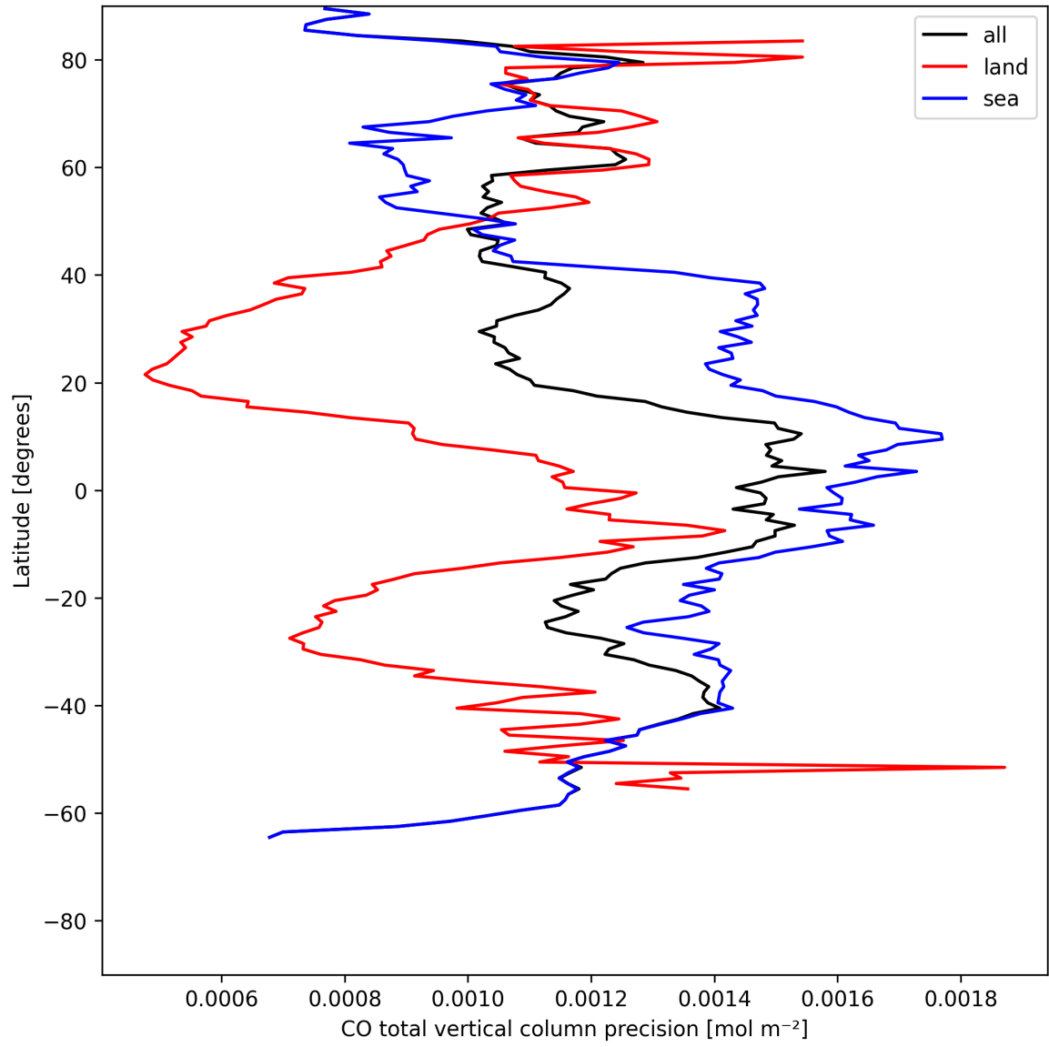
Figure 8: Zonal average of "CO total vertical column precision" for 2025-07-23 to 2025-07-24.
