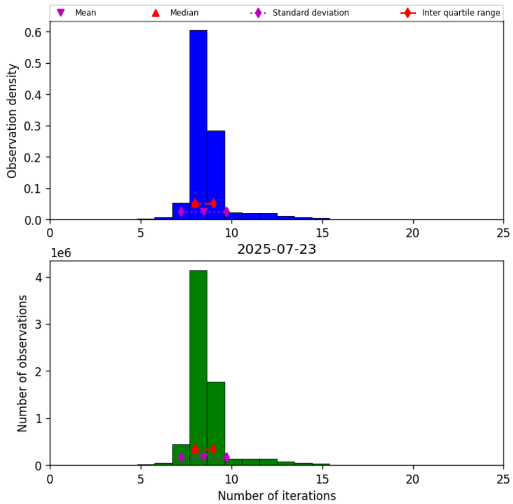
Figure 19: Histogram of “Number of iterations” for 2025-07-23 to 2025-07-24
