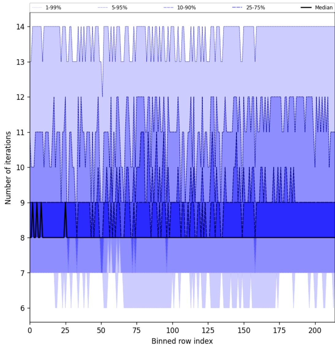
Figure 26: Along track statistics of “Number of iterations” for 2025-07-23 to 2025-07-24
