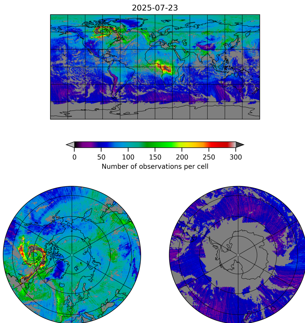
Figure 5: Map of the number of observations for 2025-07-23 to 2025-07-24
