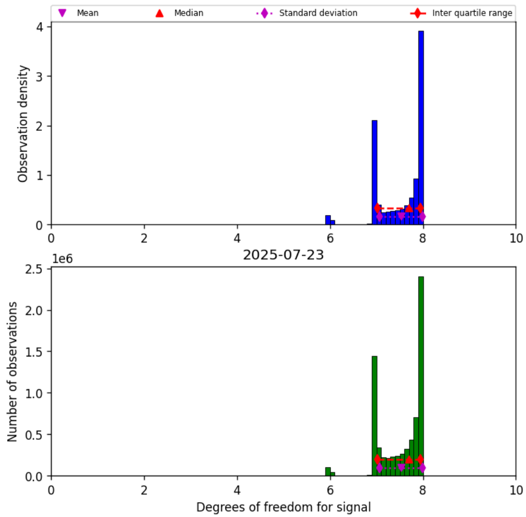
Figure 18: Histogram of “Degrees of freedom for signal” for 2025-07-23 to 2025-07-24
