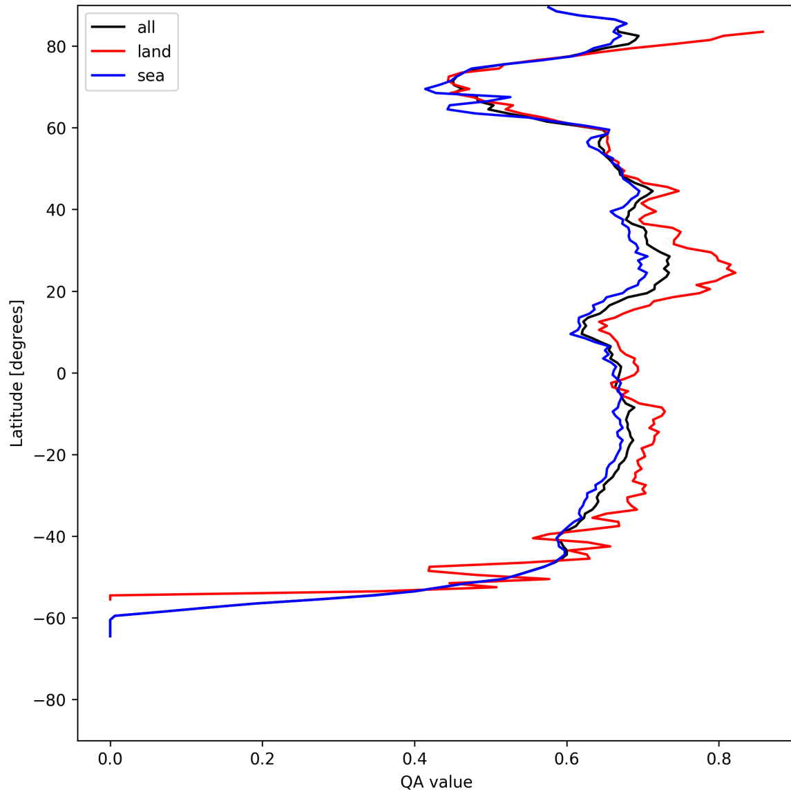
Figure 6: Zonal average of “QA value” for 2025-07-23 to 2025-07-24.
