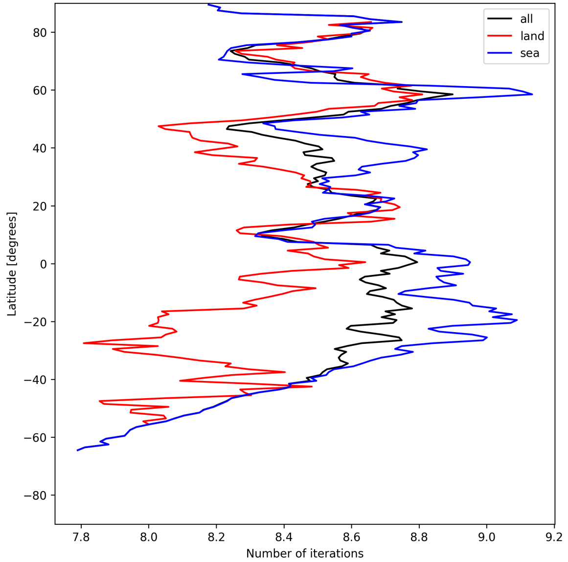
Figure 12: Zonal average of “Number of iterations” for 2025-07-23 to 2025-07-24.
