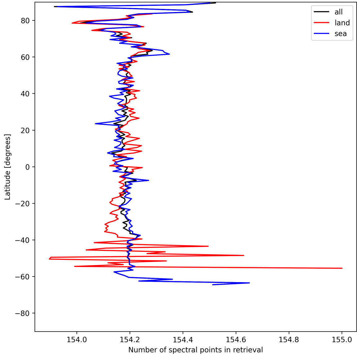
Figure 9: Zonal average of “Number of spectral points in retrieval” for 2025-07-23 to 2025-07-24.
