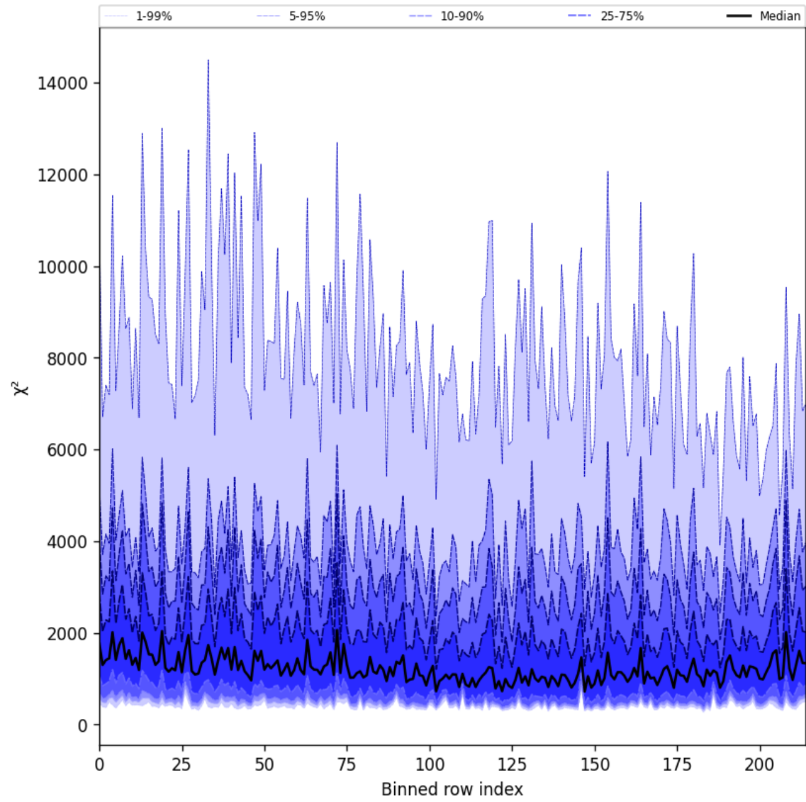
Figure 24: Along track statistics of “ \chi^2 ” for 2025-07-23 to 2025-07-24
