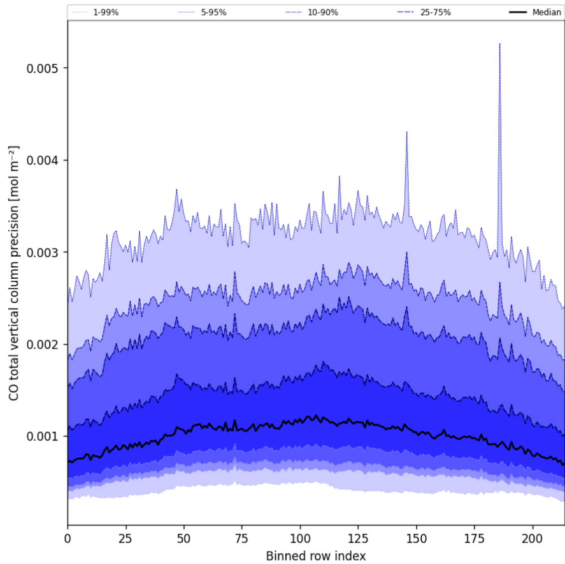
Figure 22: Along track statistics of “CO total vertical column precision” for 2025-07-23 to 2025-07-24
