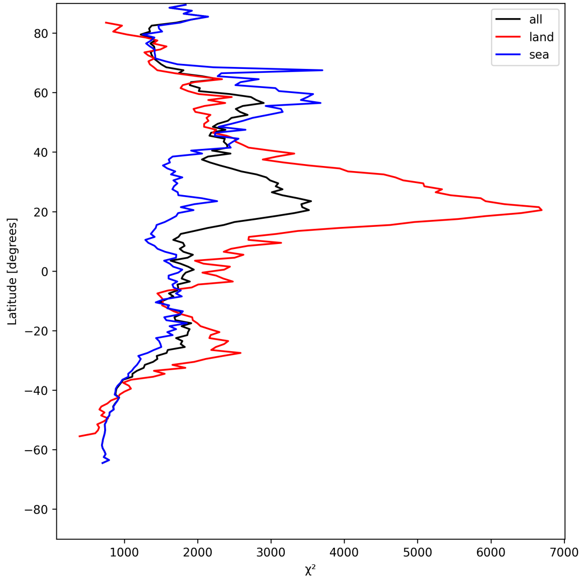
Figure 10: Zonal average of “ \chi^2 ” for 2025-07-23 to 2025-07-24.
