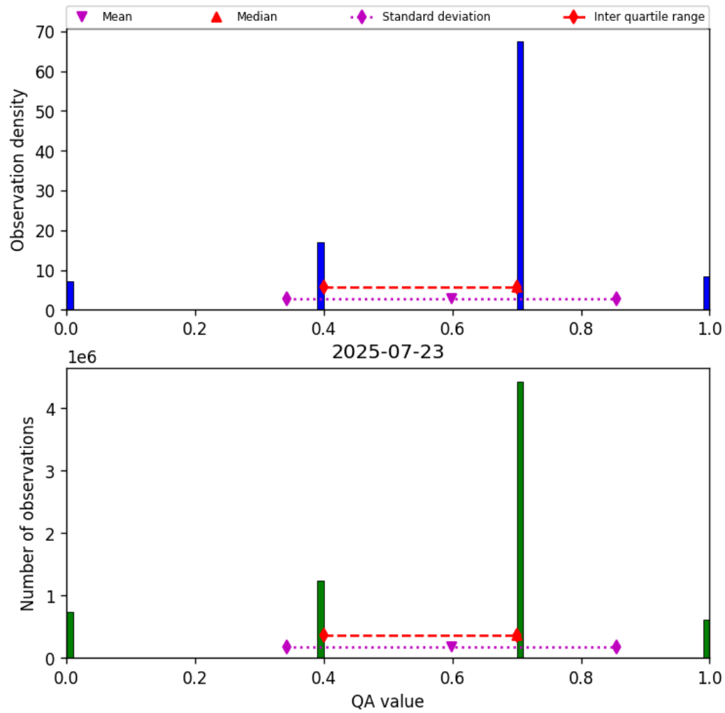
Figure 13: Histogram of “QA value” for 2025-07-23 to 2025-07-24
