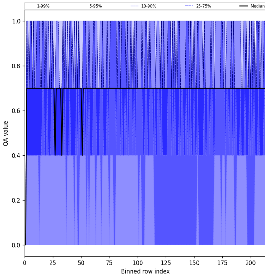
Figure 20: Along track statistics of “QA value” for 2025-07-23 to 2025-07-24
