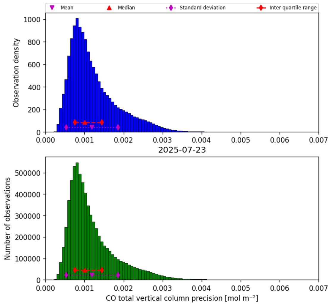
Figure 15: Histogram of “CO total vertical column precision” for 2025-07-23 to 2025-07-24
