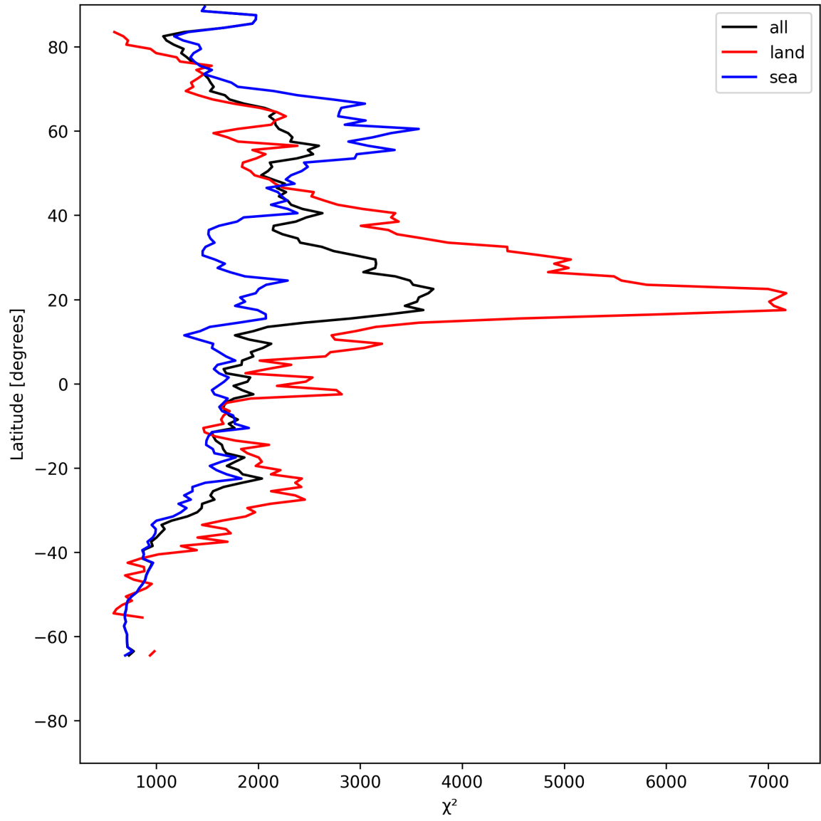
Figure 10: Zonal average of “ \chi^2 ” for 2025-07-24 to 2025-07-25.
