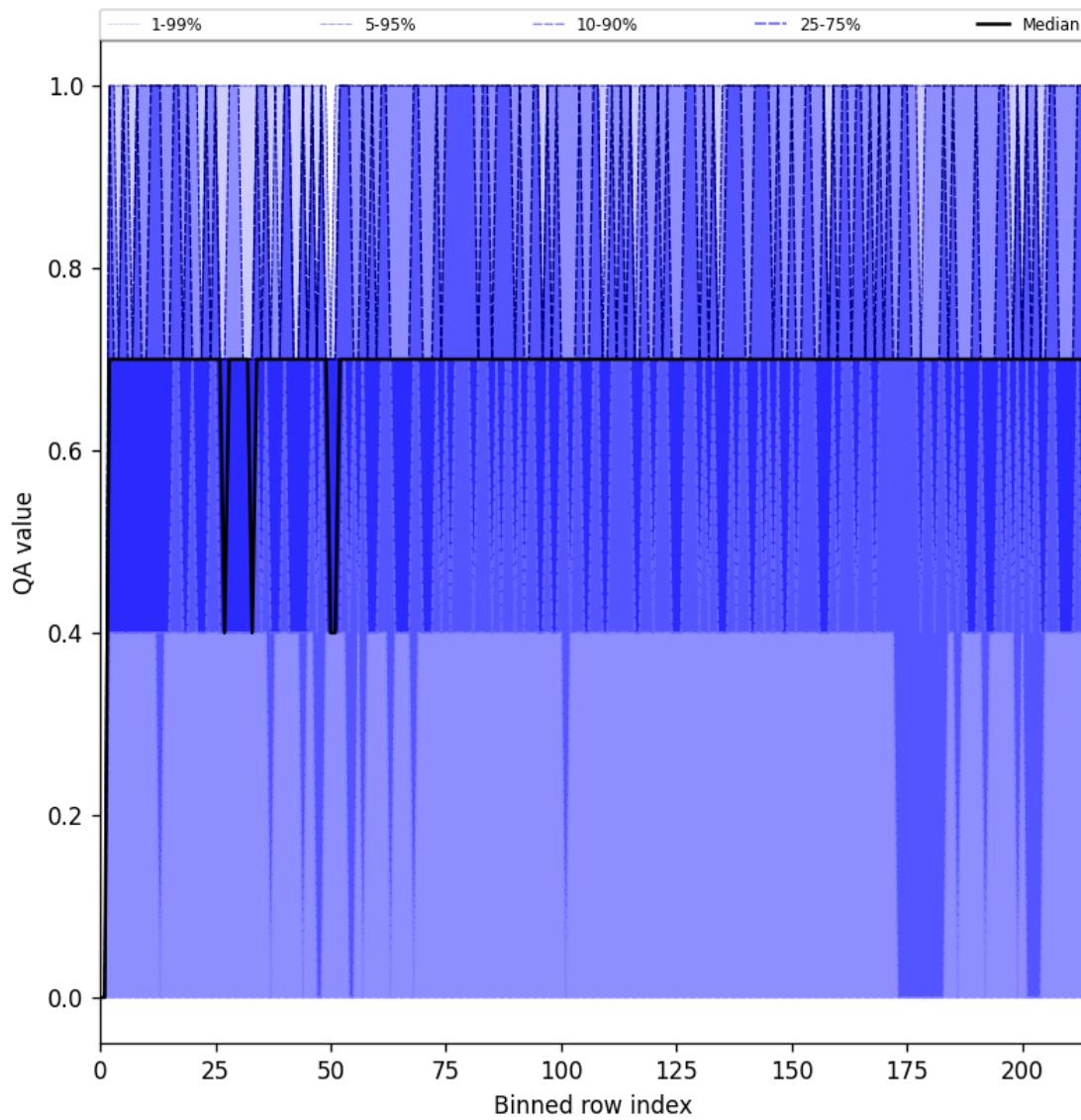
Figure 20: Along track statistics of “QA value” for 2025-07-24 to 2025-07-25
