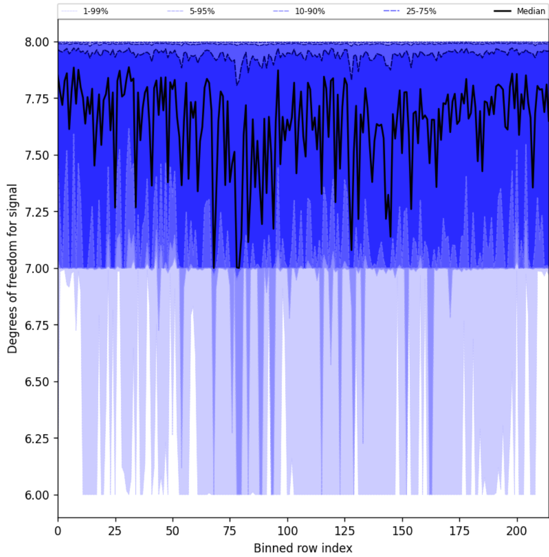
Figure 25: Along track statistics of “Degrees of freedom for signal” for 2025-07-24 to 2025-07-25
