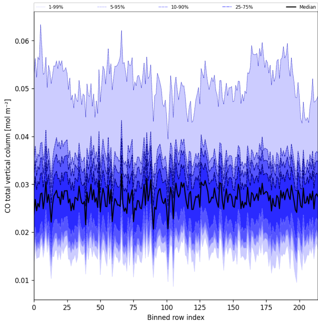
Figure 21: Along track statistics of “CO total vertical column” for 2025-07-24 to 2025-07-25
