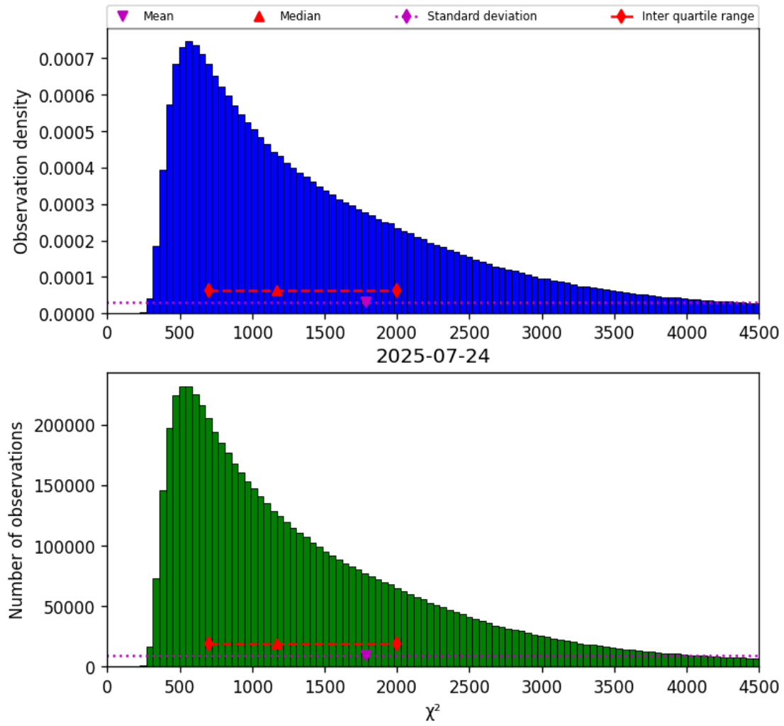
Figure 17: Histogram of “ \chi^2 ” for 2025-07-24 to 2025-07-25
