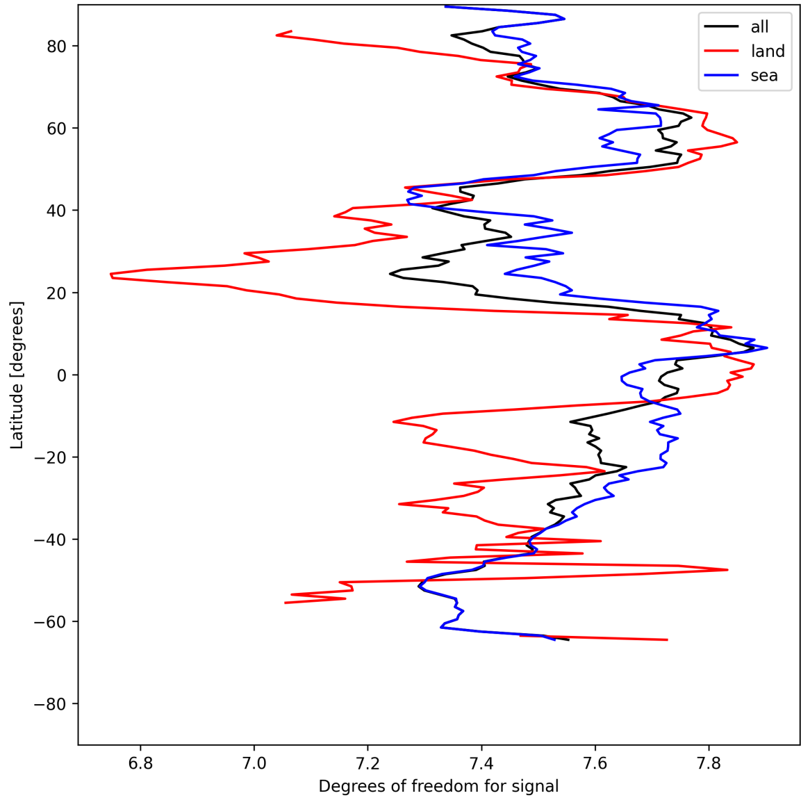
Figure 11: Zonal average of “Degrees of freedom for signal” for 2025-07-24 to 2025-07-25.
