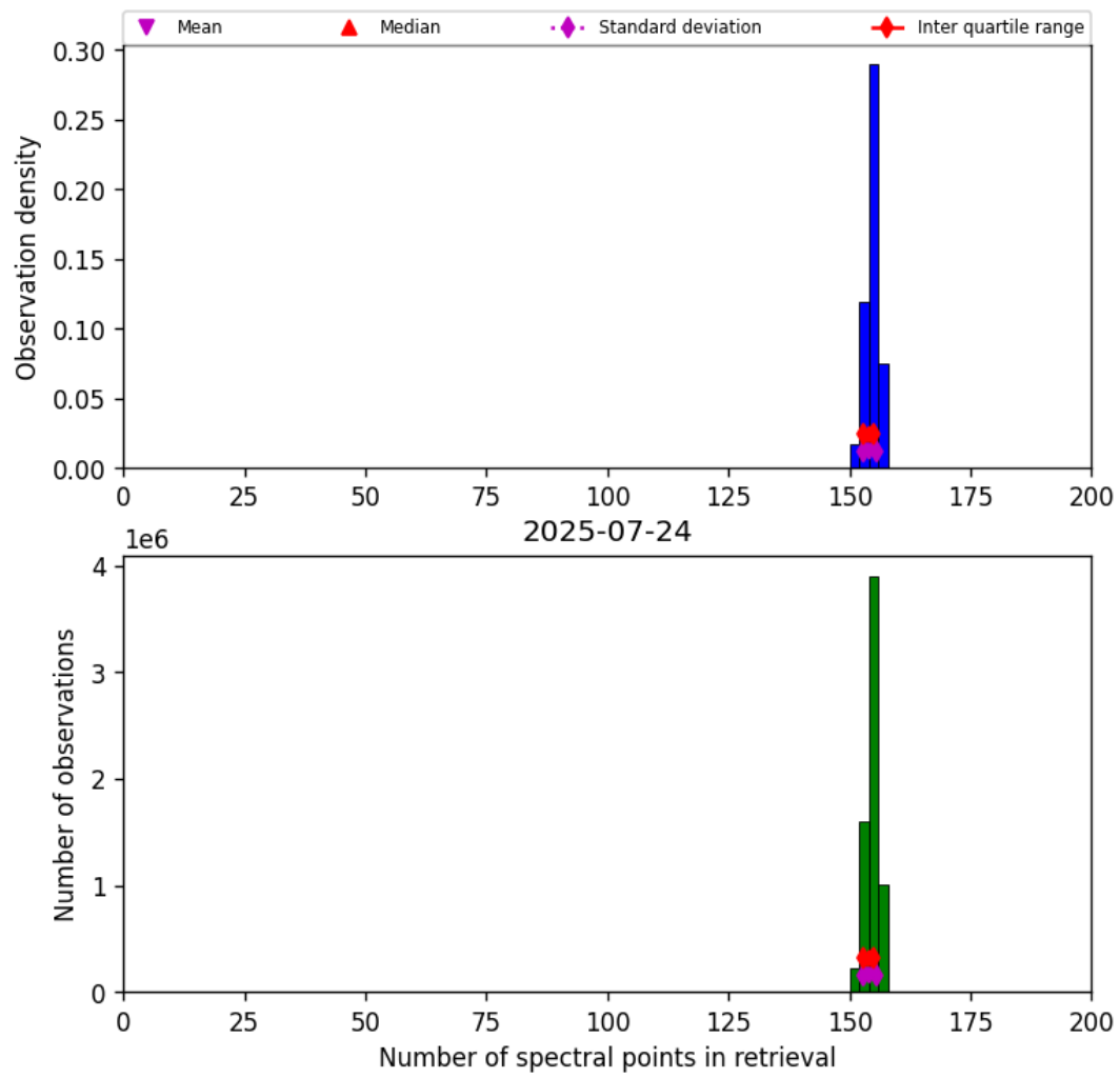
Figure 16: Histogram of “Number of spectral points in retrieval” for 2025-07-24 to 2025-07-25
