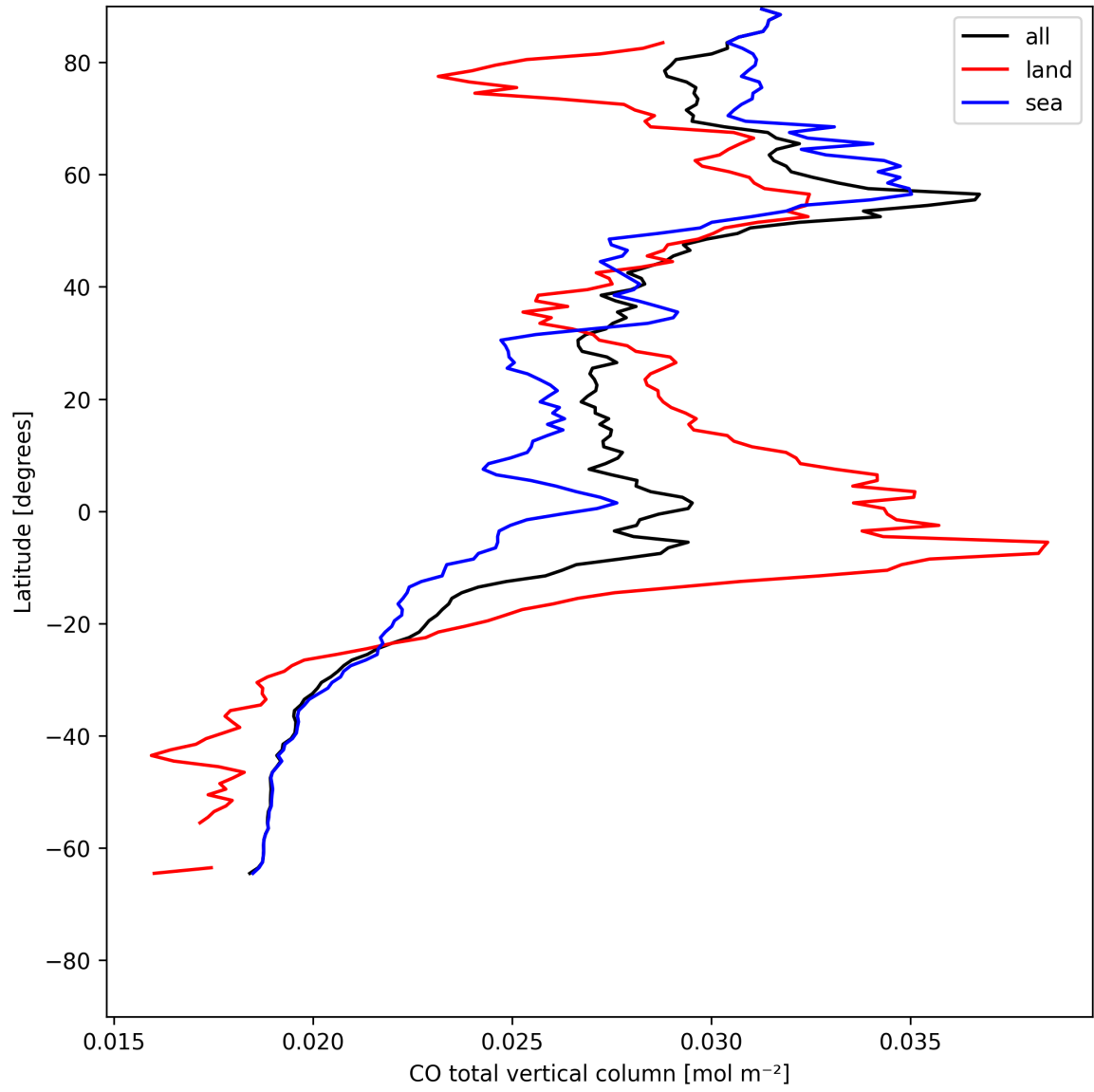
Figure 7: Zonal average of “CO total vertical column” for 2025-07-24 to 2025-07-25.
