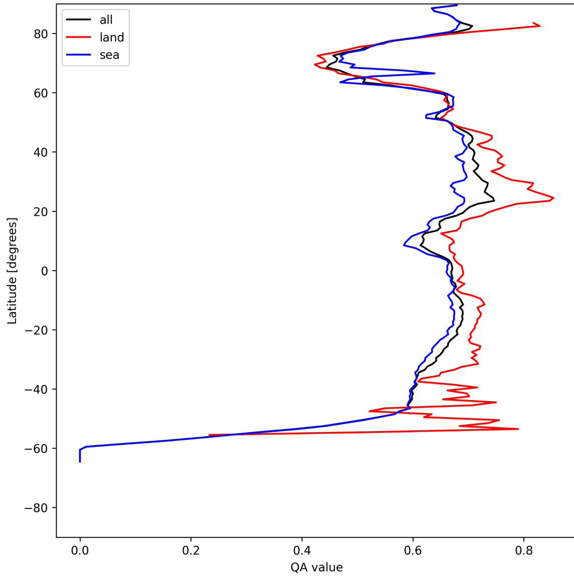
Figure 6: Zonal average of “QA value” for 2025-07-24 to 2025-07-25.
