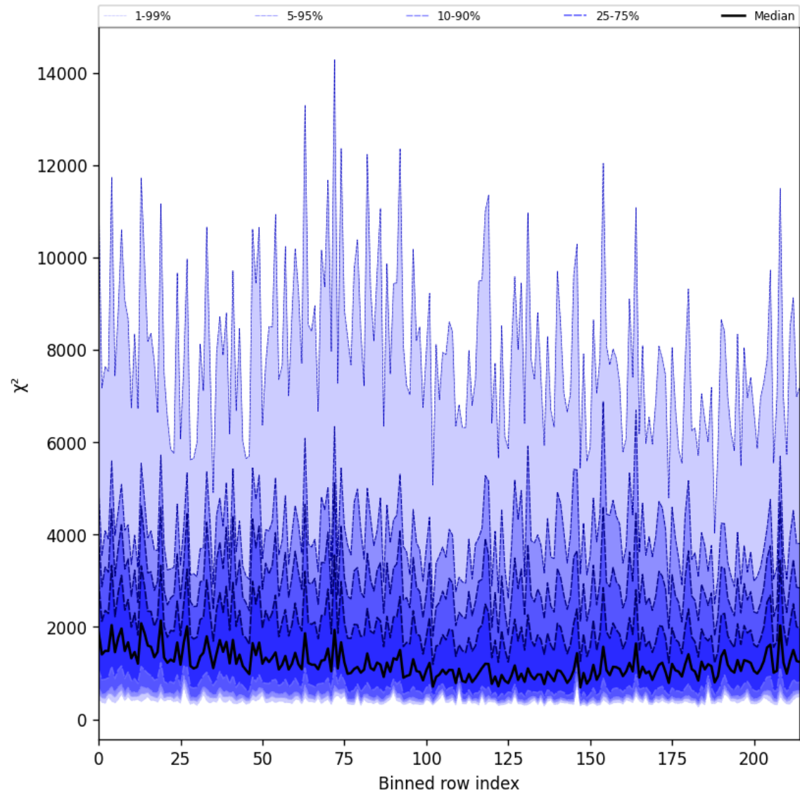
Figure 24: Along track statistics of “ \chi^2 ” for 2025-07-24 to 2025-07-25
