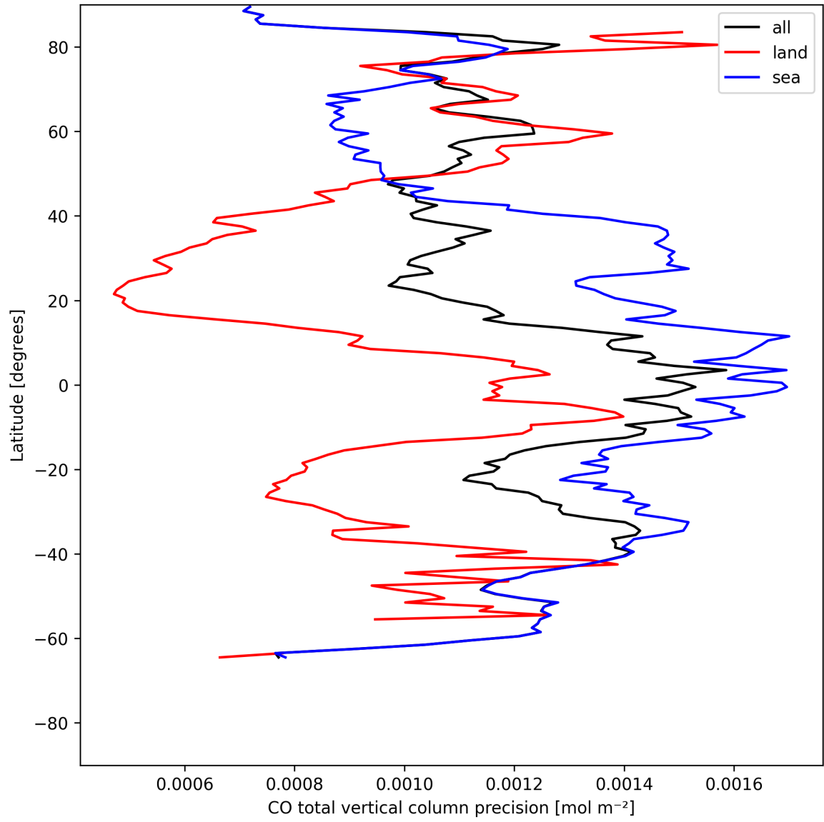
Figure 8: Zonal average of "CO total vertical column precision" for 2025-07-24 to 2025-07-25.
