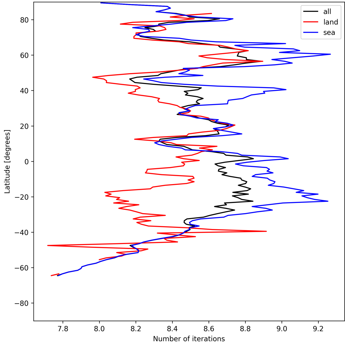
Figure 12: Zonal average of “Number of iterations” for 2025-07-24 to 2025-07-25.
