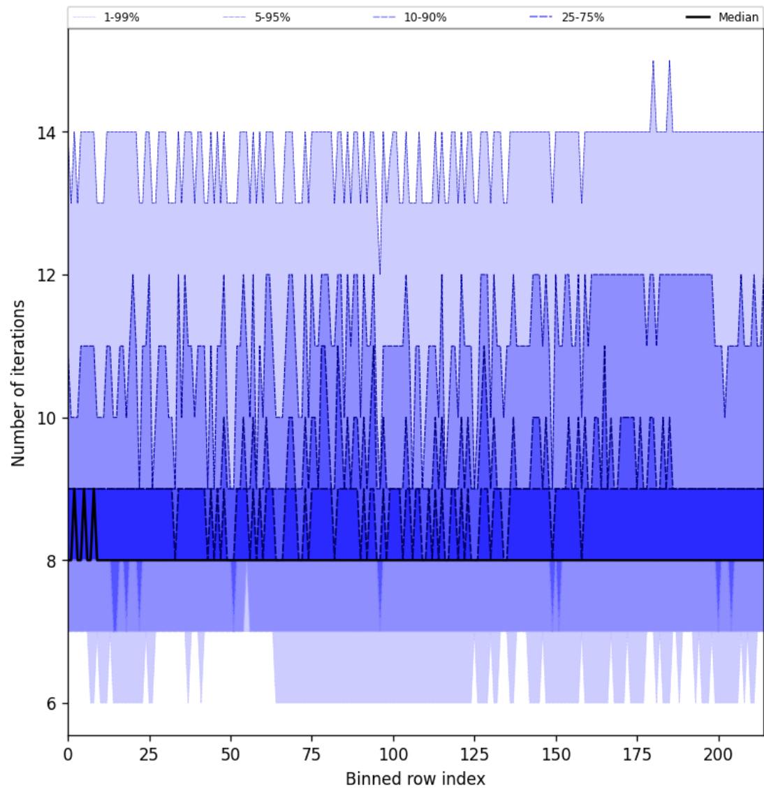
Figure 26: Along track statistics of “Number of iterations” for 2025-07-24 to 2025-07-25
