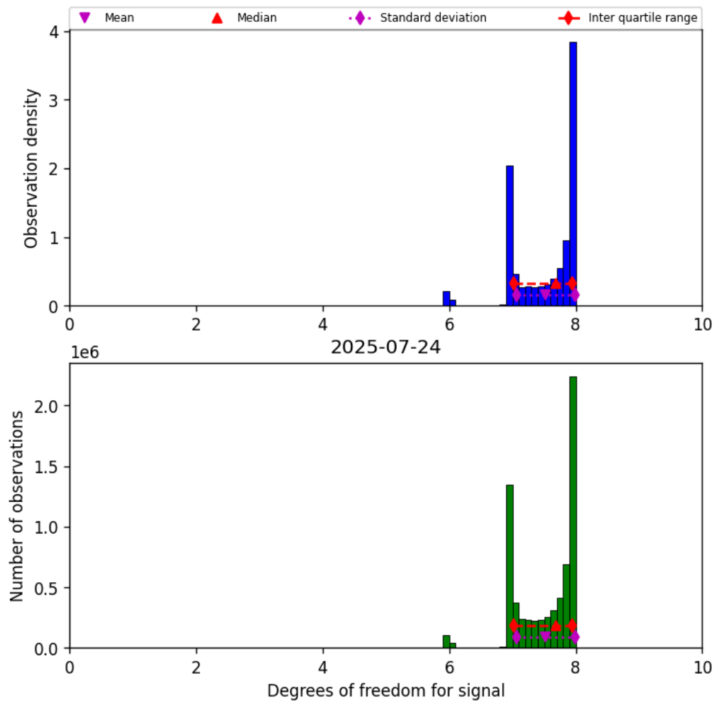
Figure 18: Histogram of “Degrees of freedom for signal” for 2025-07-24 to 2025-07-25
