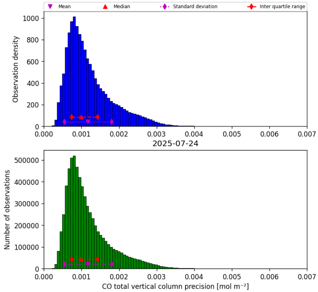
Figure 15: Histogram of “CO total vertical column precision” for 2025-07-24 to 2025-07-25
