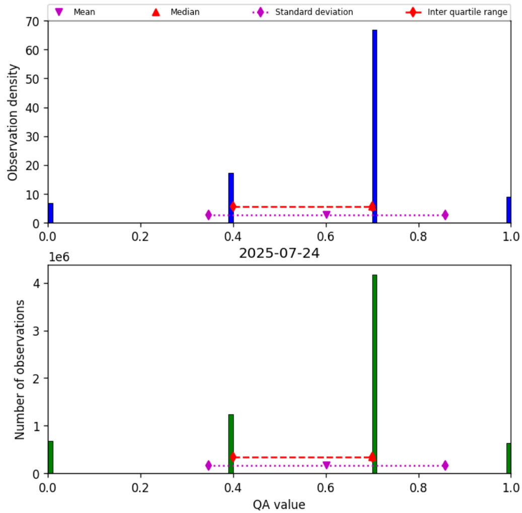
Figure 13: Histogram of “QA value” for 2025-07-24 to 2025-07-25
