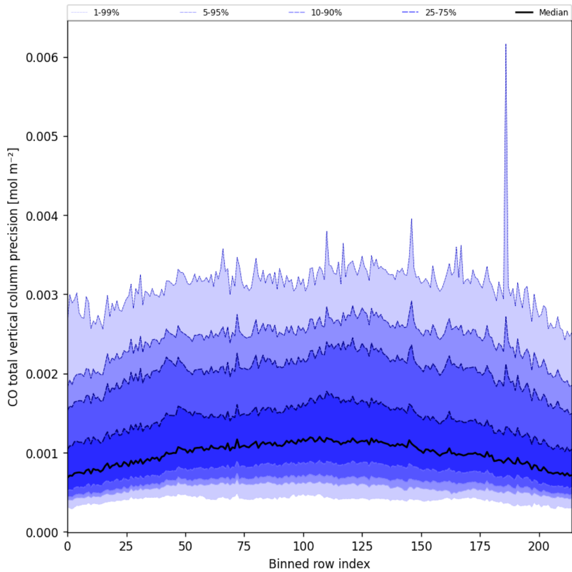
Figure 22: Along track statistics of “CO total vertical column precision” for 2025-07-24 to 2025-07-25
