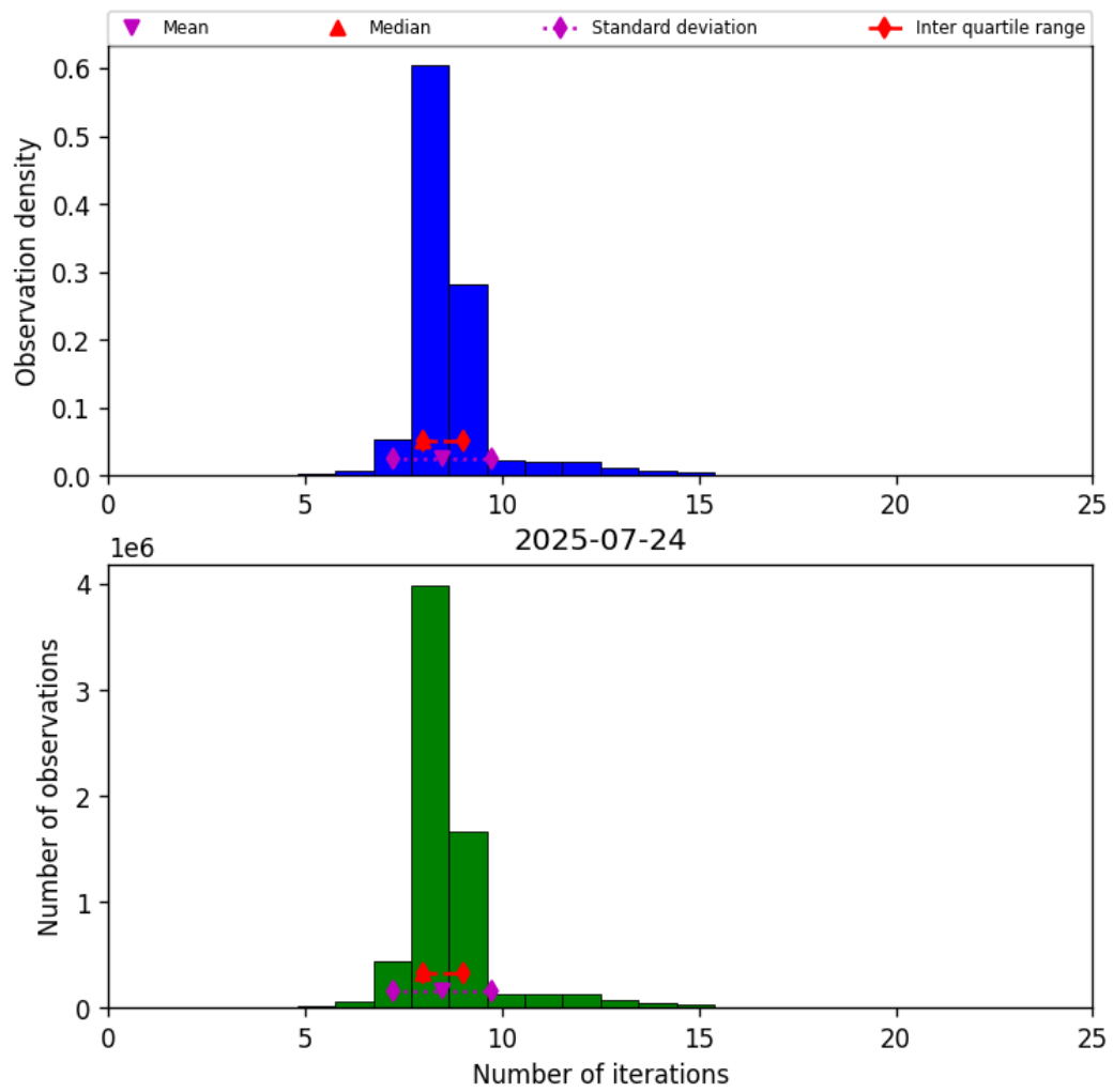
Figure 19: Histogram of “Number of iterations” for 2025-07-24 to 2025-07-25
