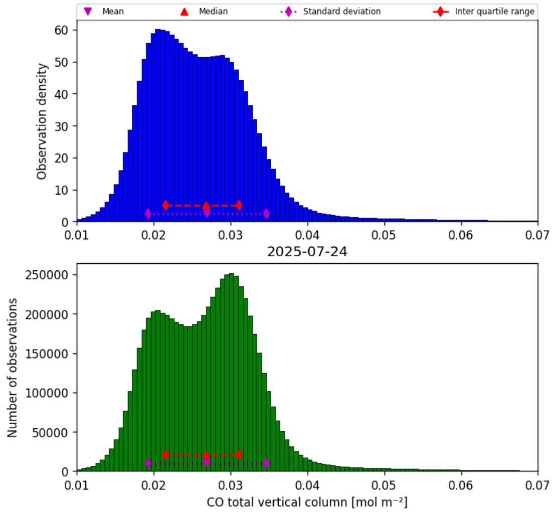
Figure 14: Histogram of “CO total vertical column” for 2025-07-24 to 2025-07-25
