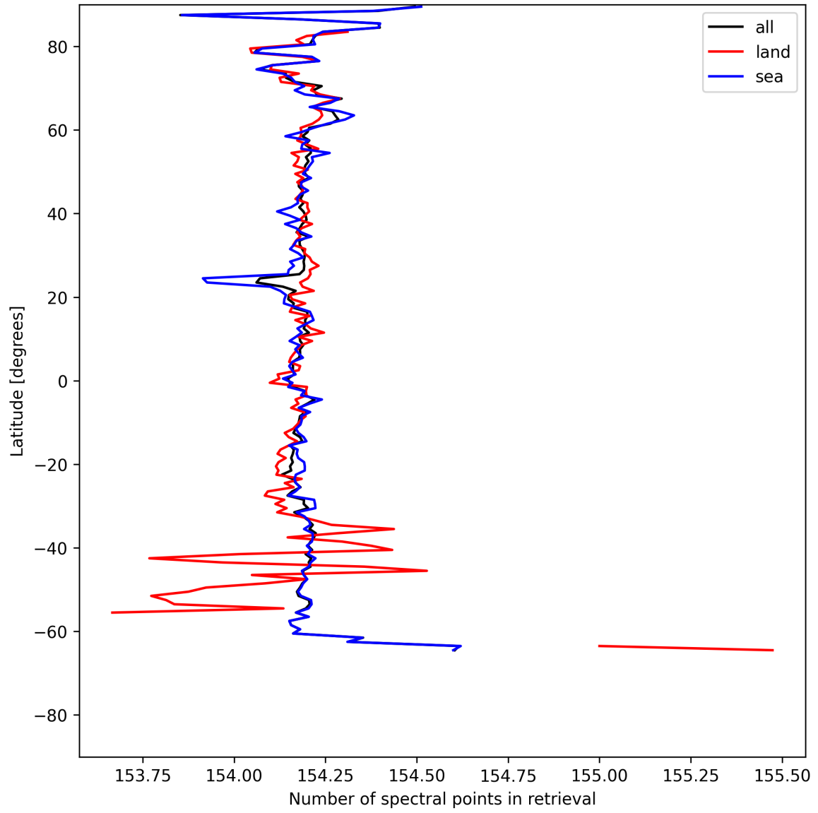
Figure 9: Zonal average of “Number of spectral points in retrieval” for 2025-07-24 to 2025-07-25.
