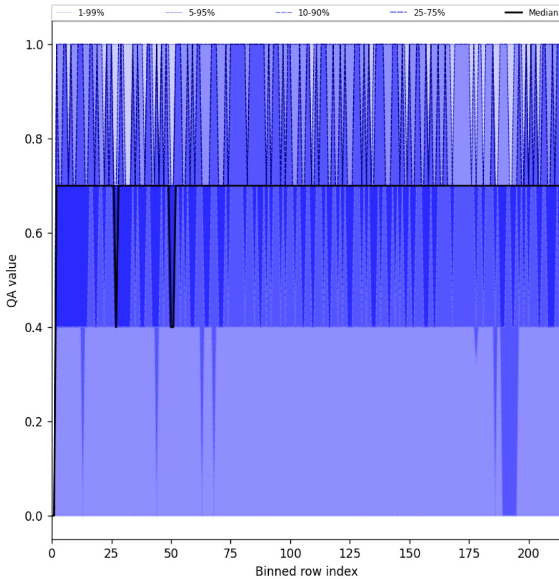
Figure 20: Along track statistics of “QA value” for 2025-07-25 to 2025-07-26
