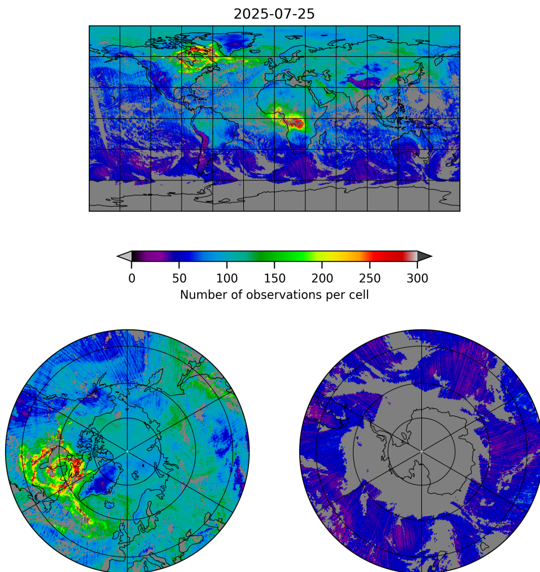
Figure 5: Map of the number of observations for 2025-07-25 to 2025-07-26
