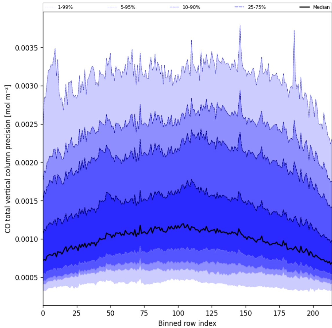
Figure 22: Along track statistics of “CO total vertical column precision” for 2025-07-25 to 2025-07-26
