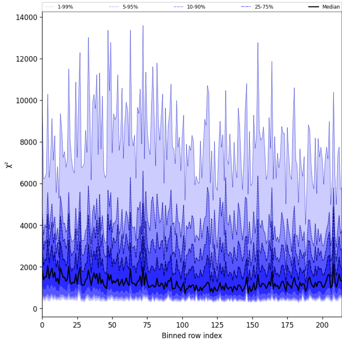
Figure 24: Along track statistics of “ \chi^2 ” for 2025-07-25 to 2025-07-26
