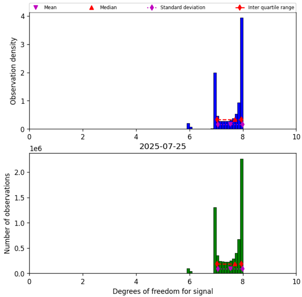
Figure 18: Histogram of “Degrees of freedom for signal” for 2025-07-25 to 2025-07-26
