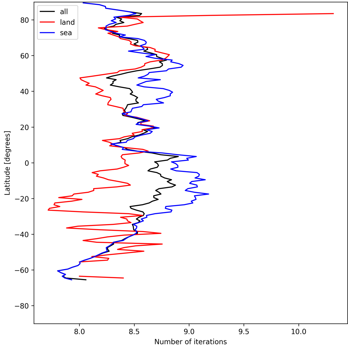
Figure 12: Zonal average of “Number of iterations” for 2025-07-25 to 2025-07-26.
