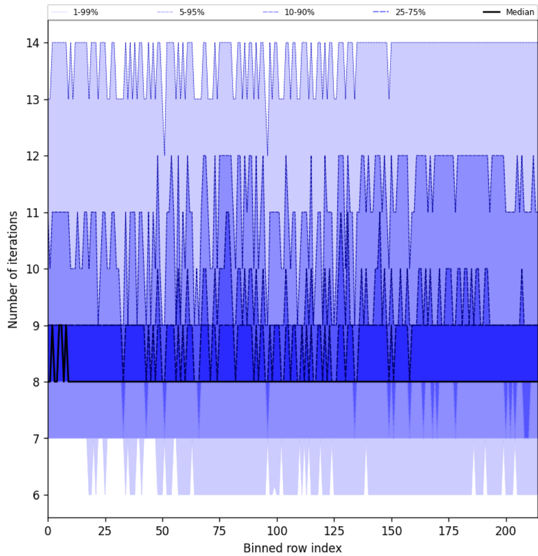
Figure 26: Along track statistics of “Number of iterations” for 2025-07-25 to 2025-07-26
