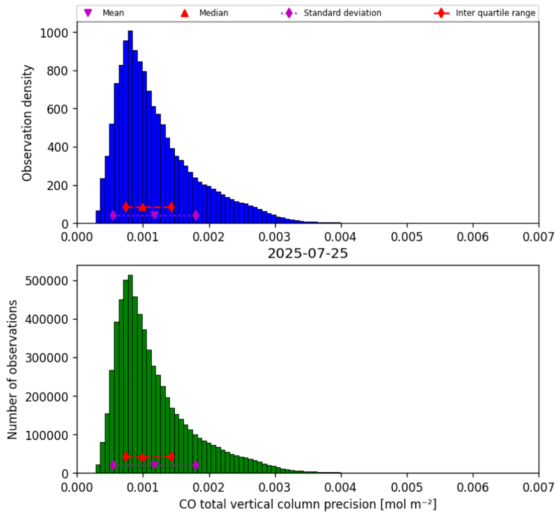
Figure 15: Histogram of “CO total vertical column precision” for 2025-07-25 to 2025-07-26
