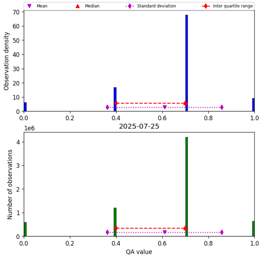
Figure 13: Histogram of “QA value” for 2025-07-25 to 2025-07-26
