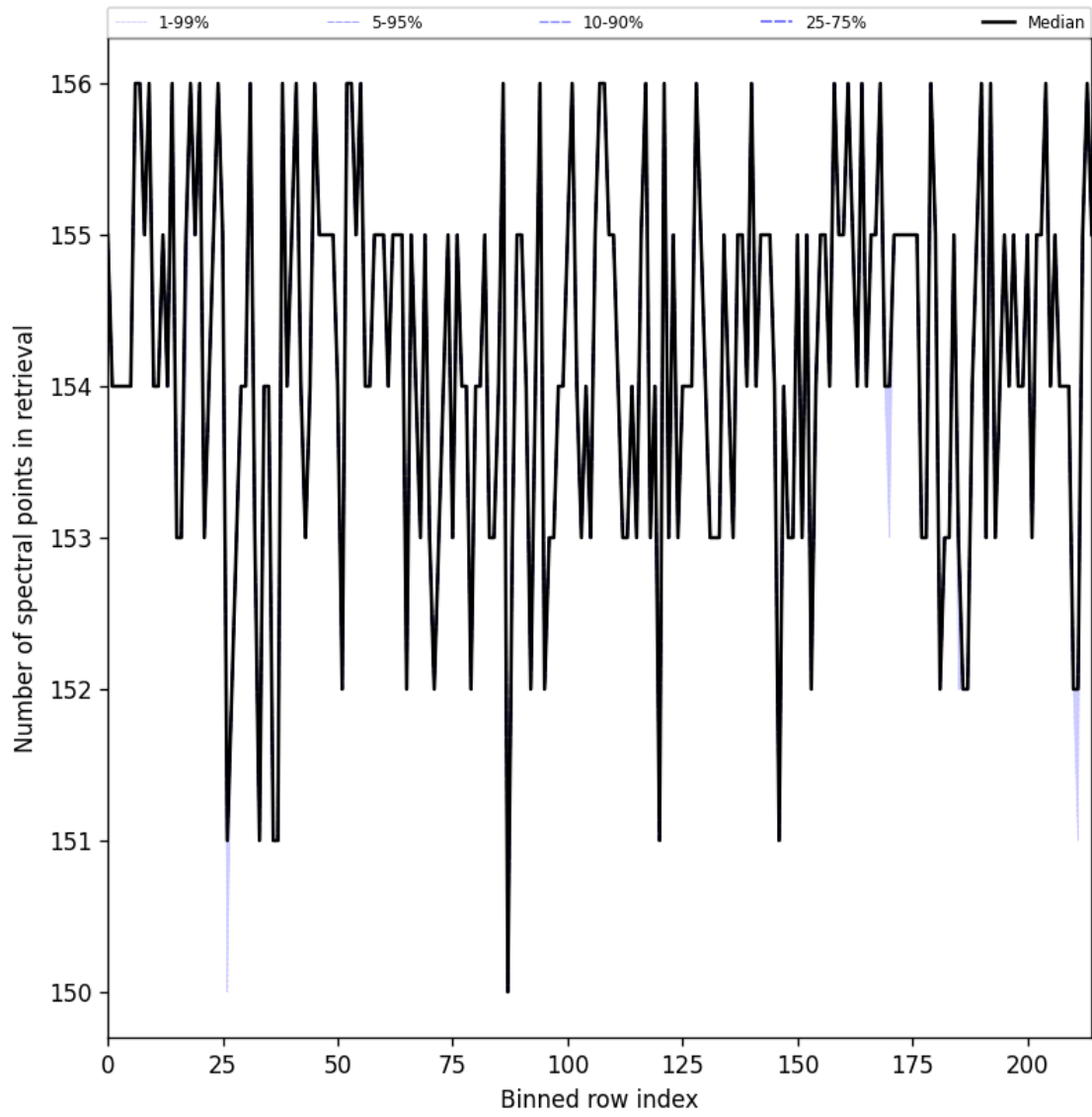
Figure 23: Along track statistics of “Number of spectral points in retrieval” for 2025-07-25 to 2025-07-26
