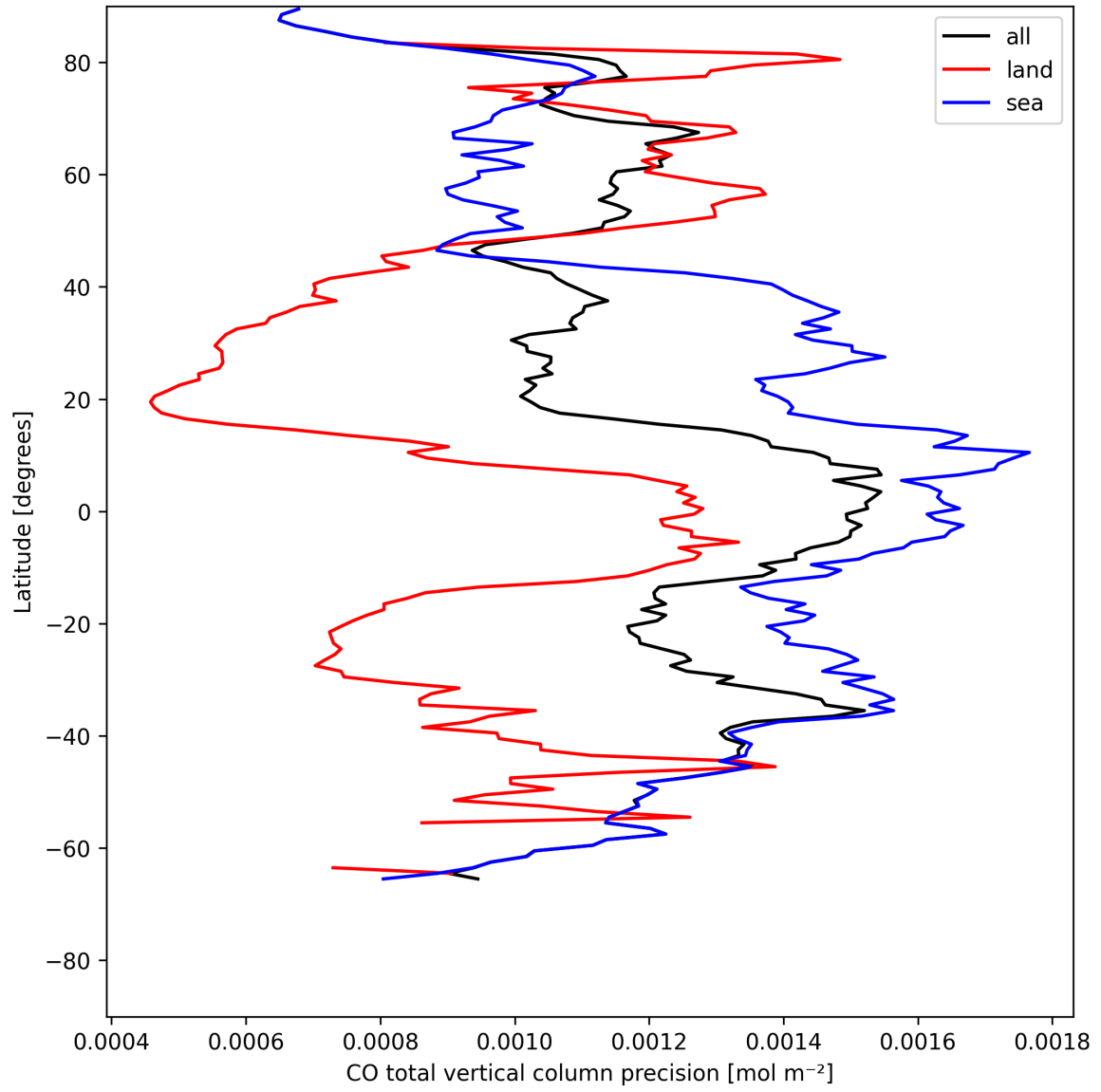
Figure 8: Zonal average of “CO total vertical column precision” for 2025-07-25 to 2025-07-26.
