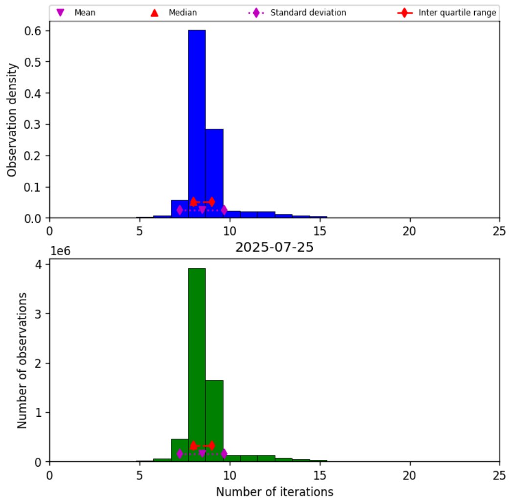
Figure 19: Histogram of “Number of iterations” for 2025-07-25 to 2025-07-26
