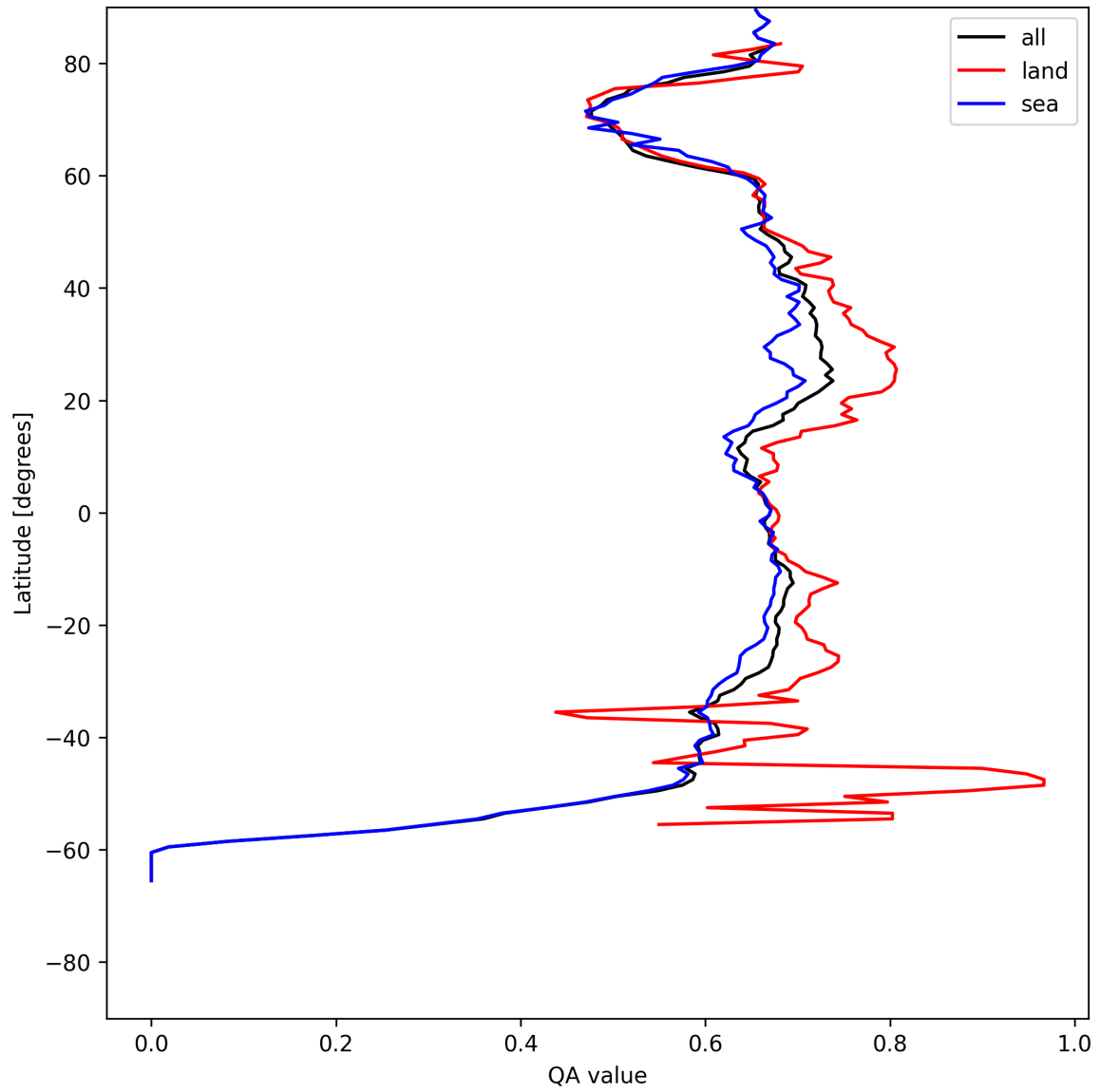
Figure 6: Zonal average of “QA value” for 2025-07-25 to 2025-07-26.
