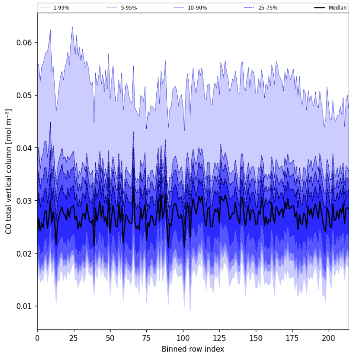
Figure 21: Along track statistics of “CO total vertical column” for 2025-07-25 to 2025-07-26
