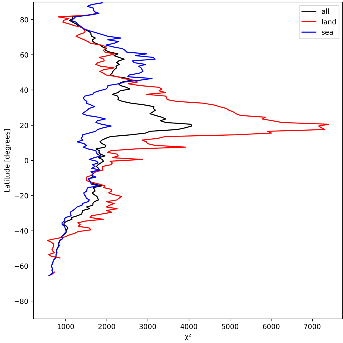
Figure 10: Zonal average of “ \chi^2 ” for 2025-07-25 to 2025-07-26.
