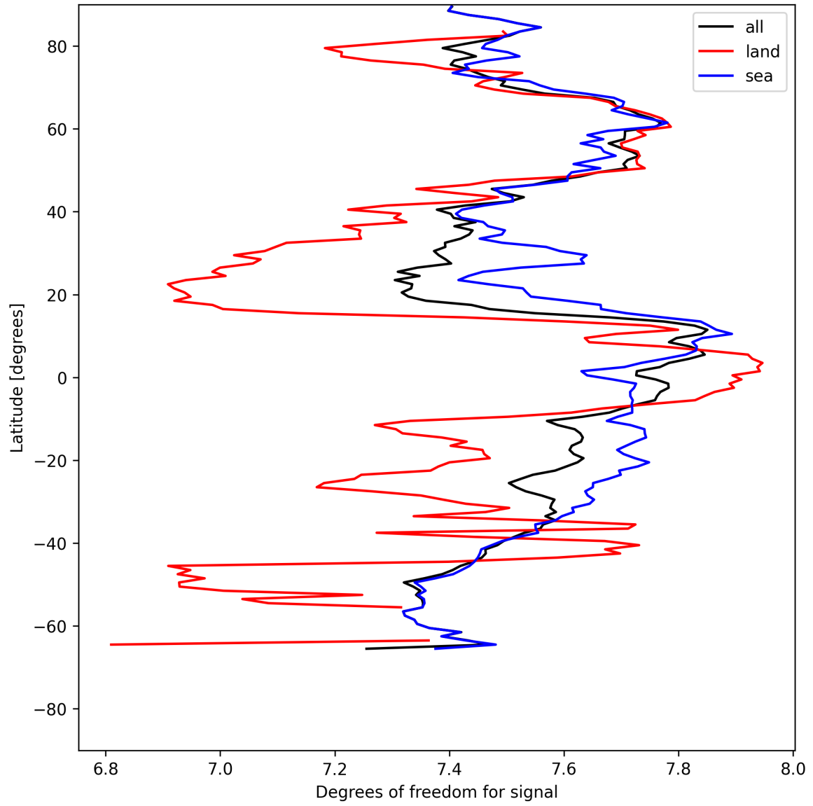
Figure 11: Zonal average of “Degrees of freedom for signal” for 2025-07-25 to 2025-07-26.
