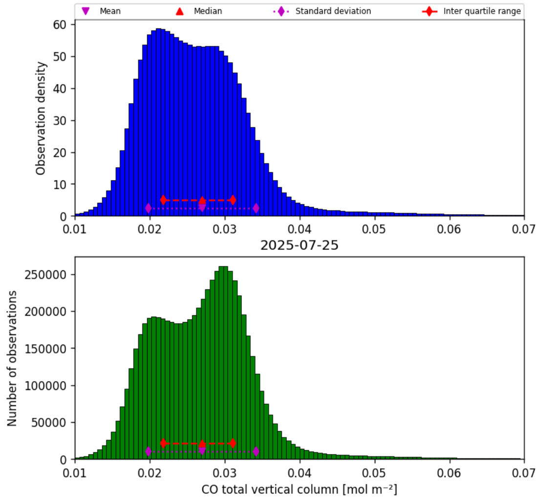
Figure 14: Histogram of “CO total vertical column” for 2025-07-25 to 2025-07-26
