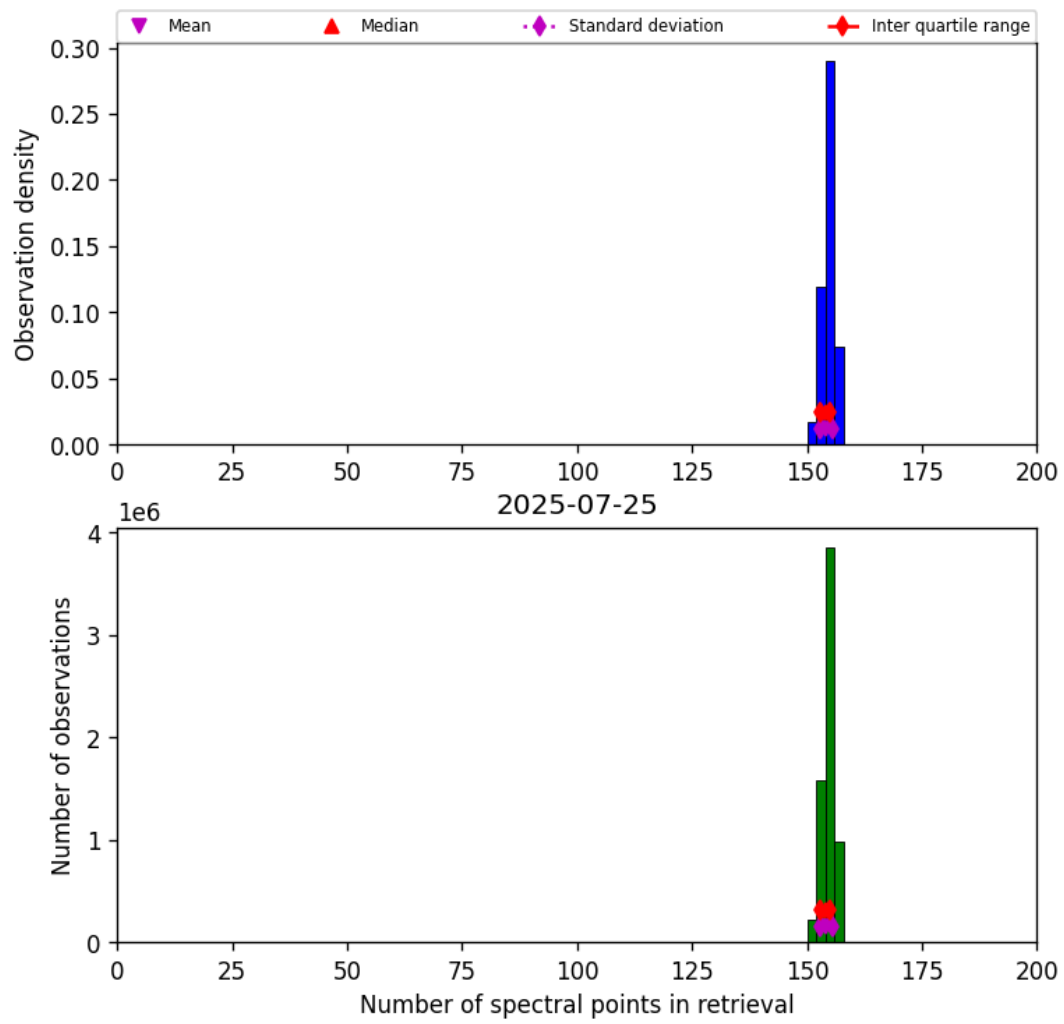
Figure 16: Histogram of “Number of spectral points in retrieval” for 2025-07-25 to 2025-07-26
