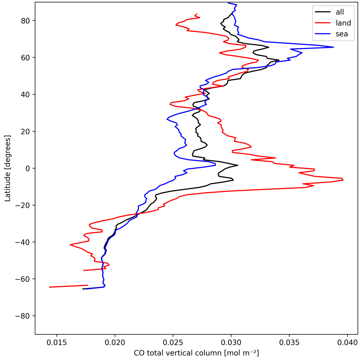
Figure 7: Zonal average of “CO total vertical column” for 2025-07-25 to 2025-07-26.
