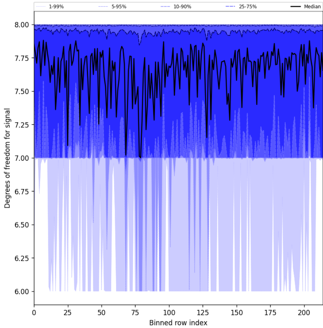
Figure 25: Along track statistics of “Degrees of freedom for signal” for 2025-07-25 to 2025-07-26
