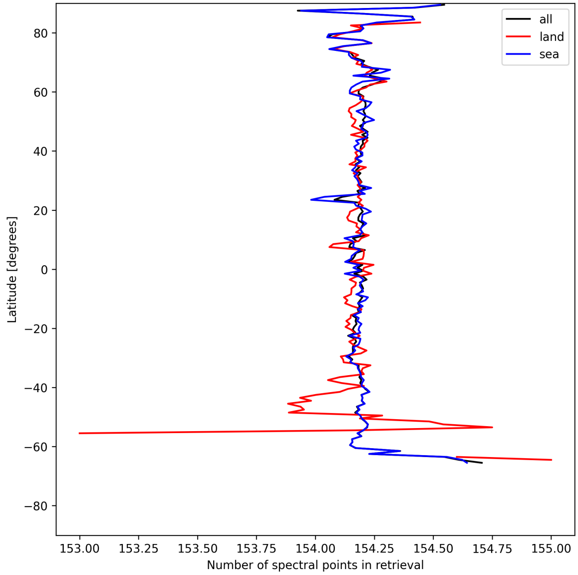
Figure 9: Zonal average of “Number of spectral points in retrieval” for 2025-07-25 to 2025-07-26.
