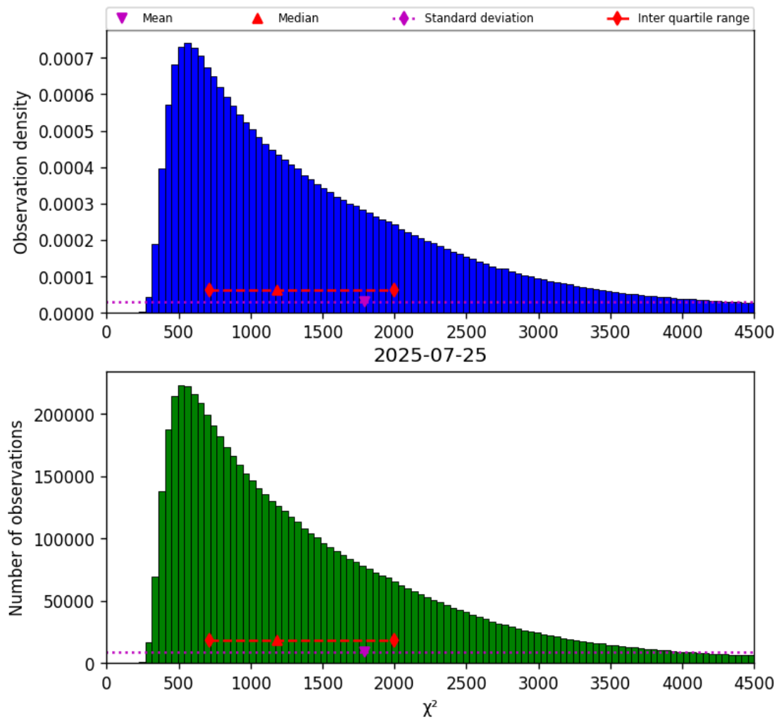
Figure 17: Histogram of “ \chi^2 ” for 2025-07-25 to 2025-07-26
