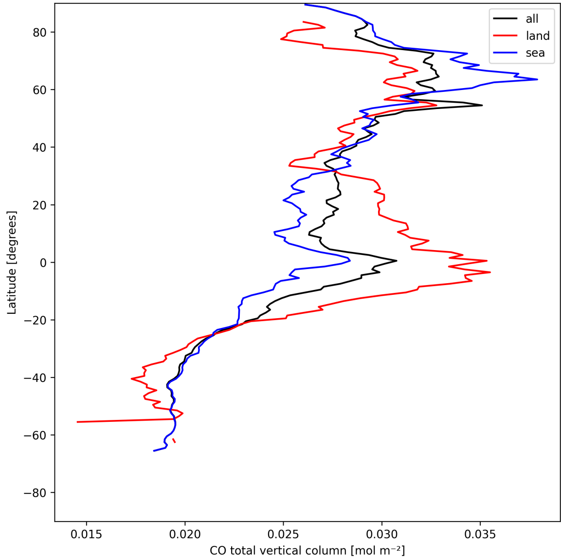
Figure 7: Zonal average of “CO total vertical column” for 2025-07-27 to 2025-07-27.
