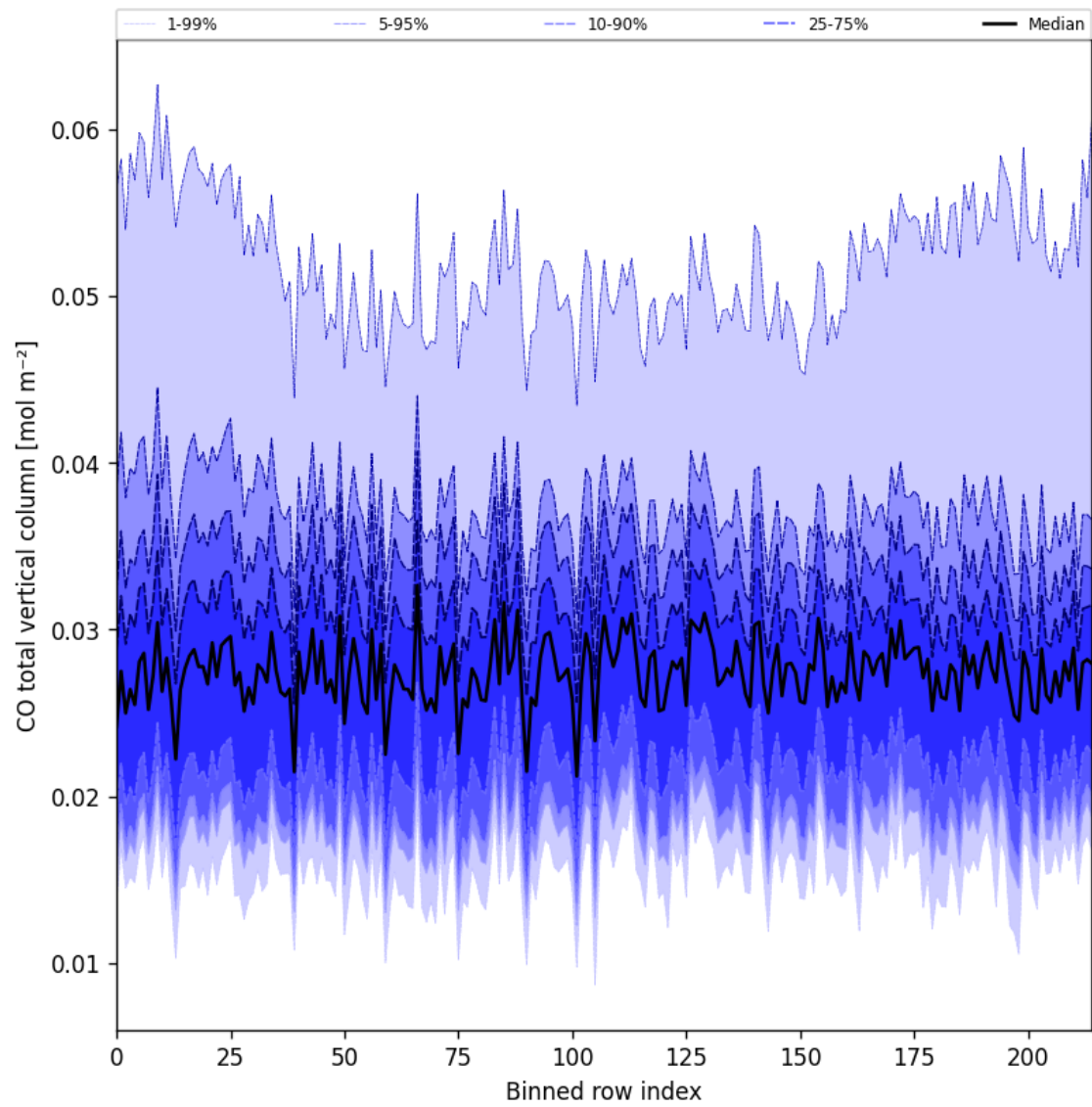
Figure 21: Along track statistics of “CO total vertical column” for 2025-07-27 to 2025-07-27
