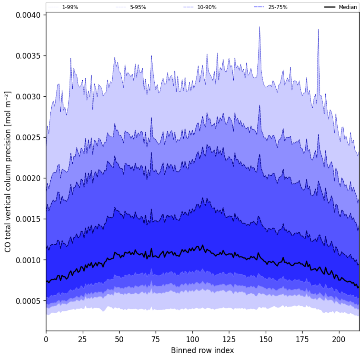
Figure 22: Along track statistics of “CO total vertical column precision” for 2025-07-27 to 2025-07-27
