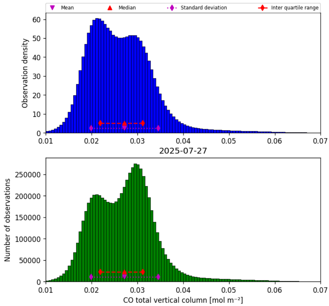
Figure 14: Histogram of “CO total vertical column” for 2025-07-27 to 2025-07-27
