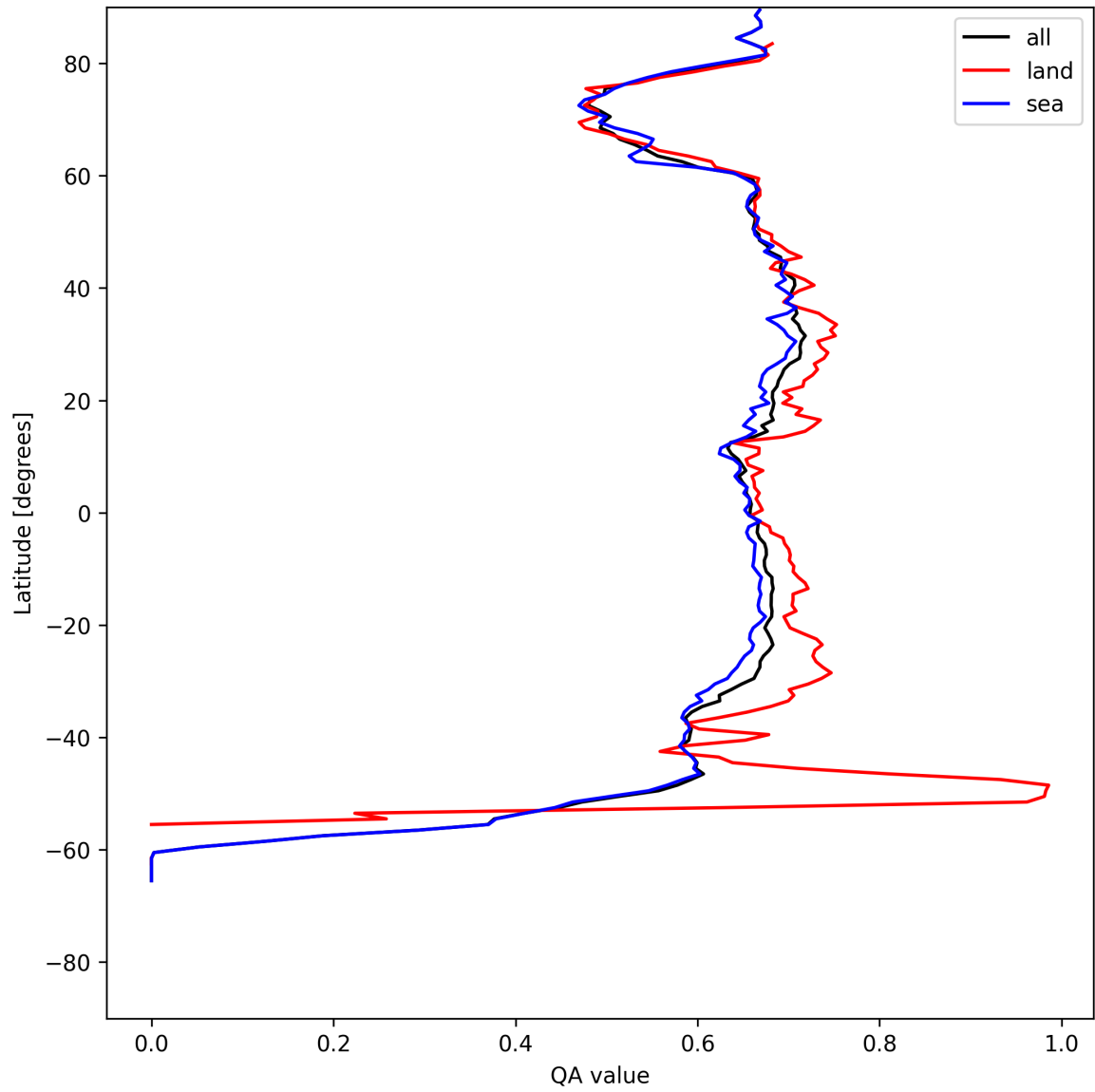
Figure 6: Zonal average of “QA value” for 2025-07-27 to 2025-07-27.
