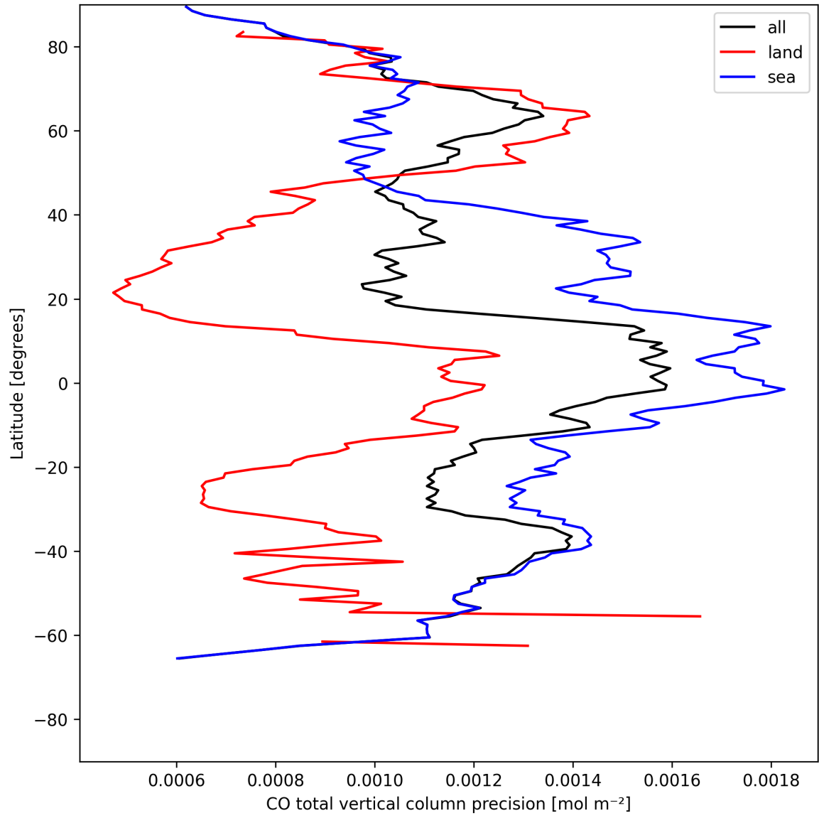
Figure 8: Zonal average of “CO total vertical column precision” for 2025-07-27 to 2025-07-27.
