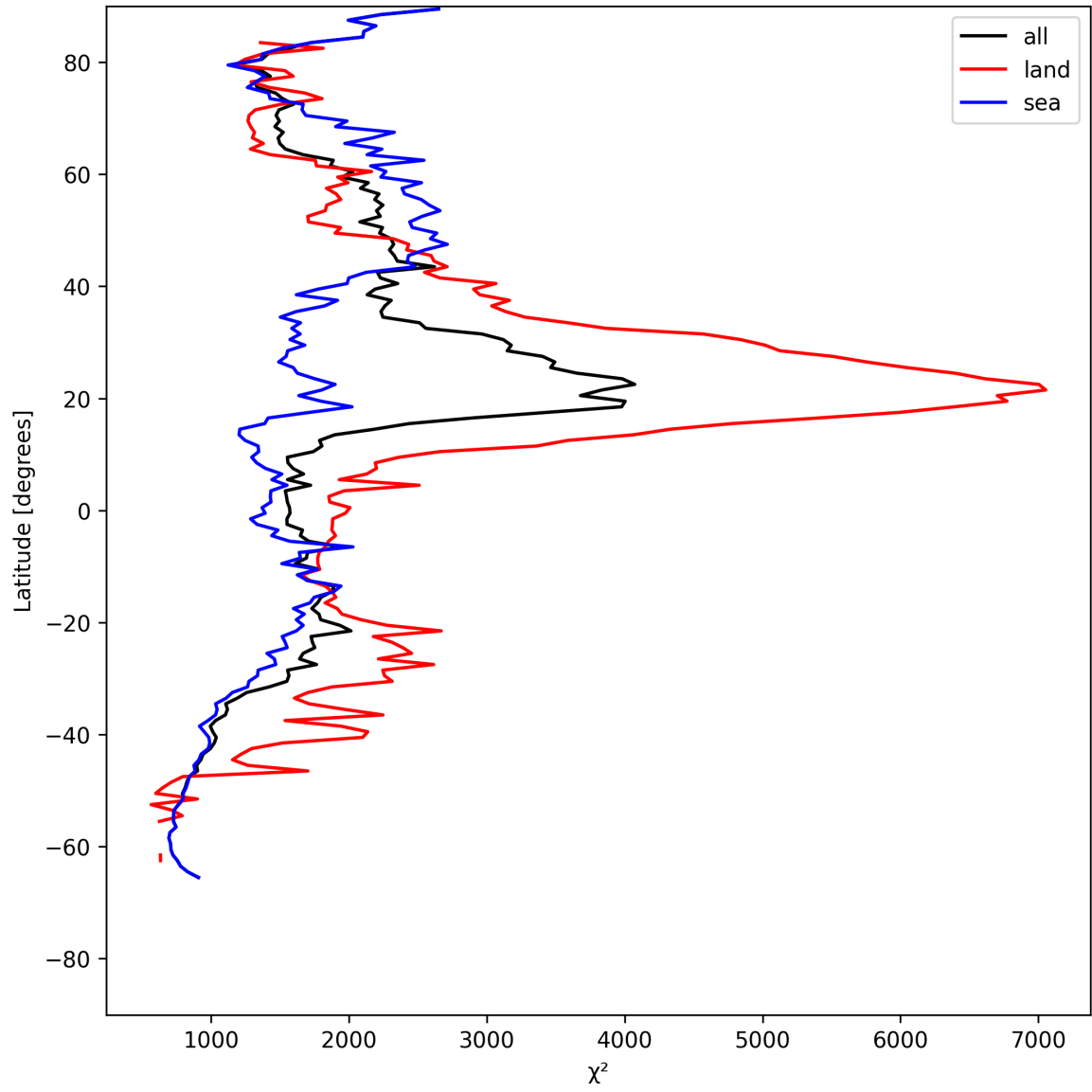
Figure 10: Zonal average of “ \chi^2 ” for 2025-07-27 to 2025-07-27.
