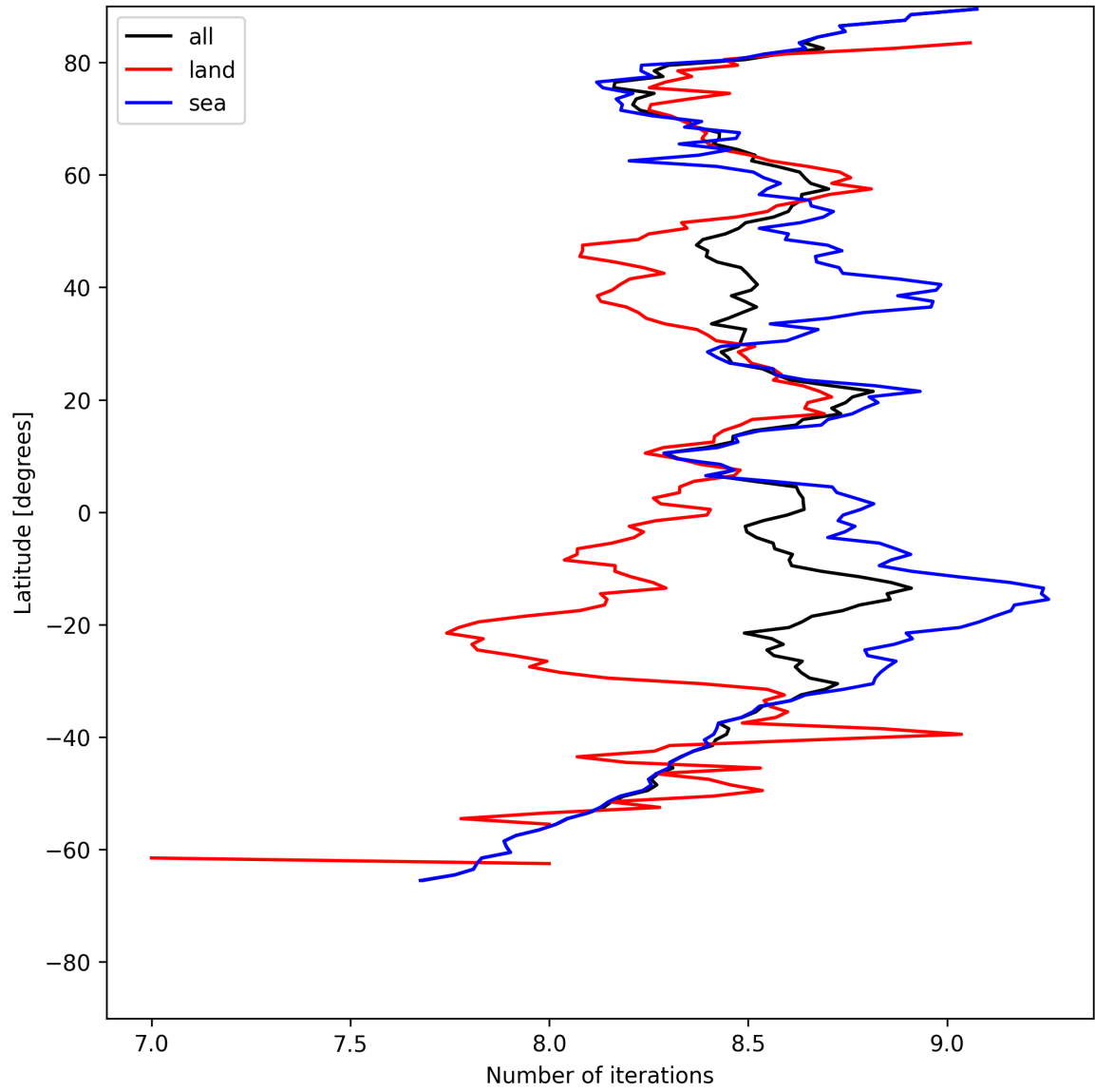
Figure 12: Zonal average of “Number of iterations” for 2025-07-27 to 2025-07-27.
