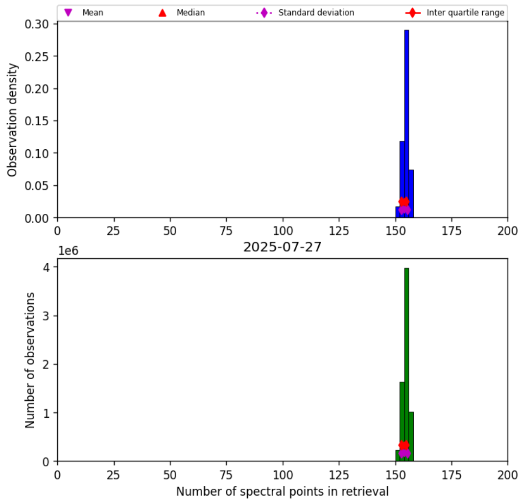
Figure 16: Histogram of “Number of spectral points in retrieval” for 2025-07-27 to 2025-07-27
