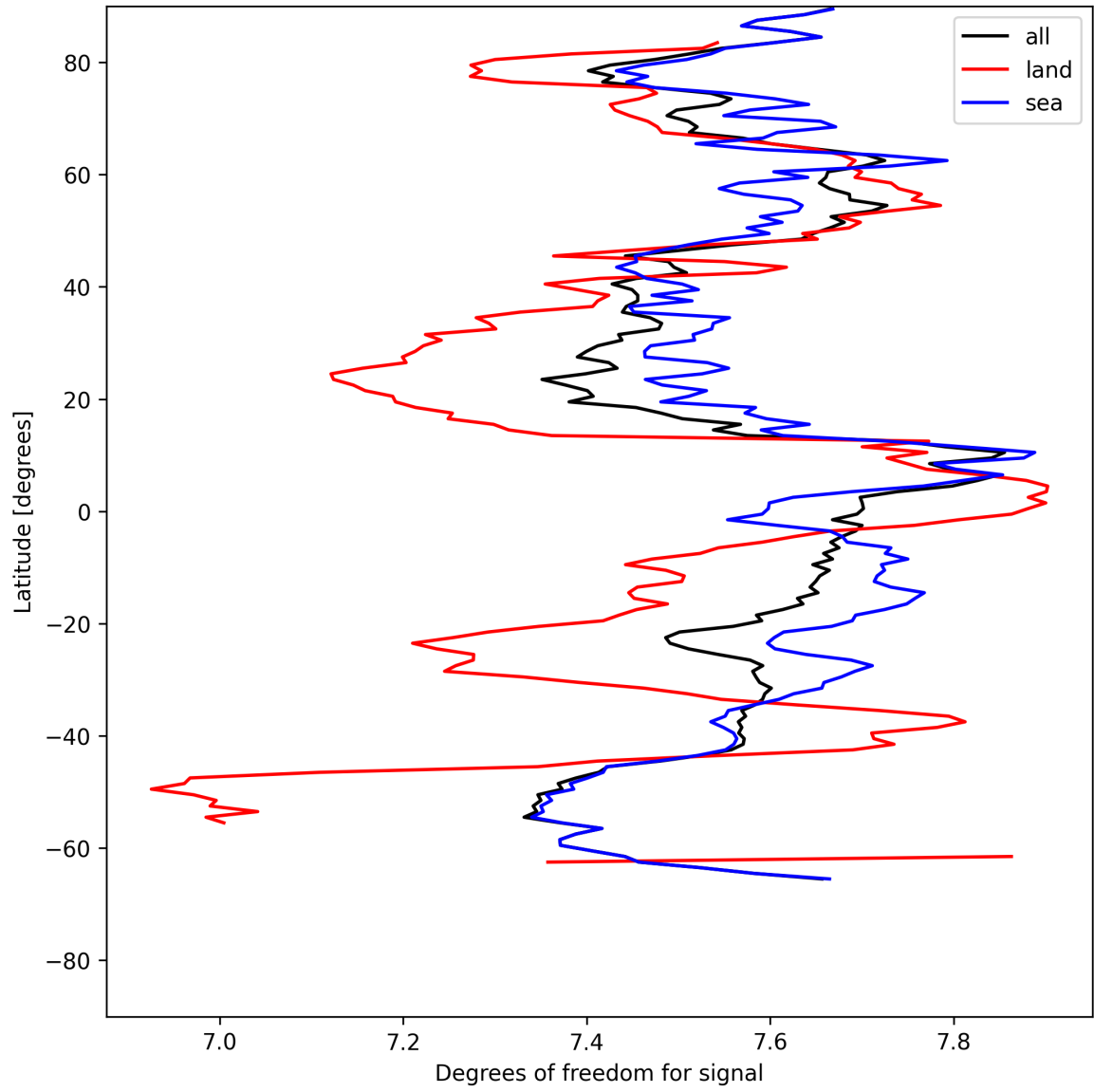
Figure 11: Zonal average of “Degrees of freedom for signal” for 2025-07-27 to 2025-07-27.
