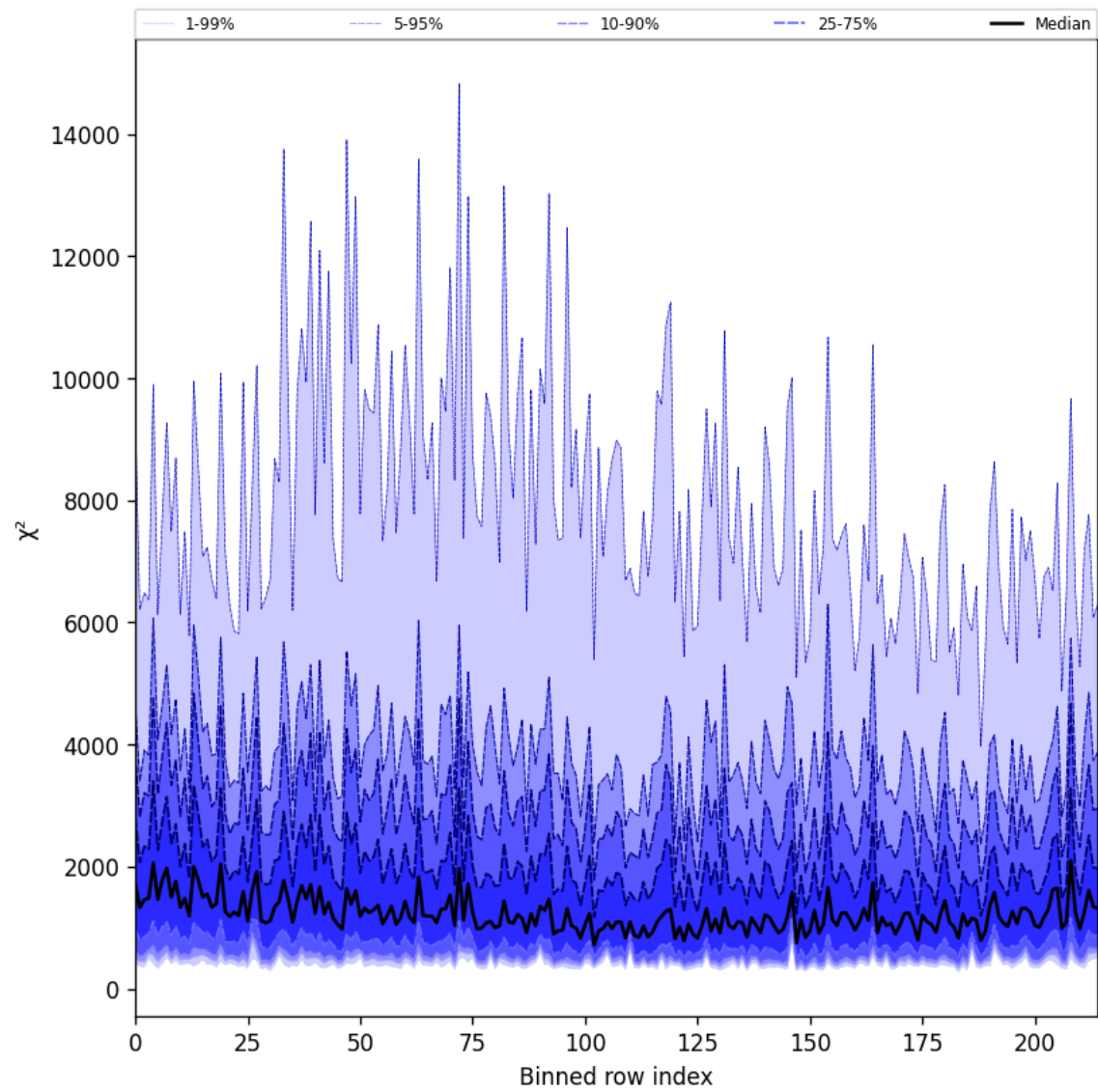
Figure 24: Along track statistics of “ \chi^2 ” for 2025-07-27 to 2025-07-27
