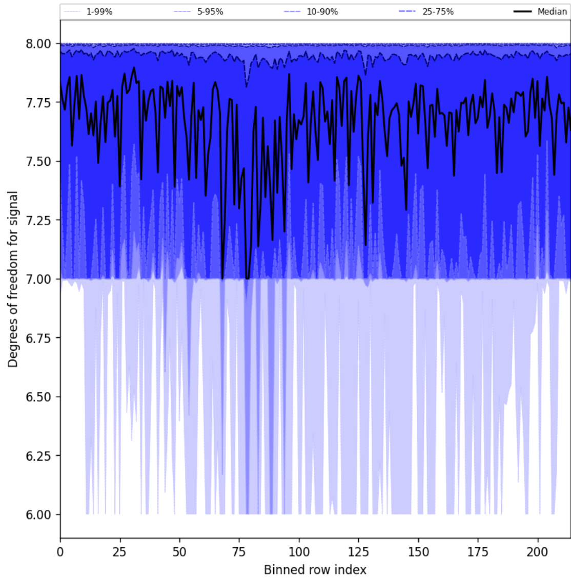
Figure 25: Along track statistics of “Degrees of freedom for signal” for 2025-07-27 to 2025-07-27
