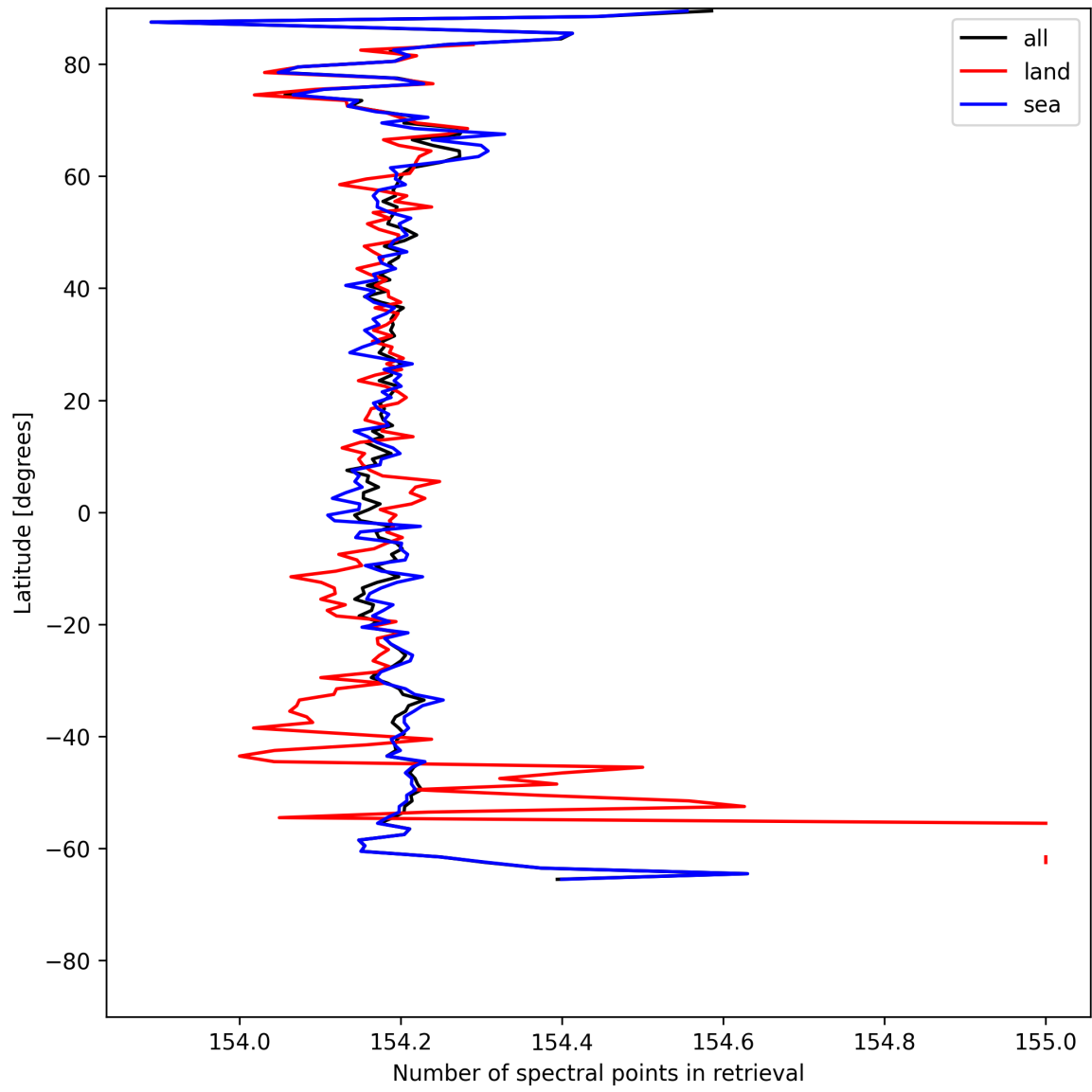
Figure 9: Zonal average of “Number of spectral points in retrieval” for 2025-07-27 to 2025-07-27.
