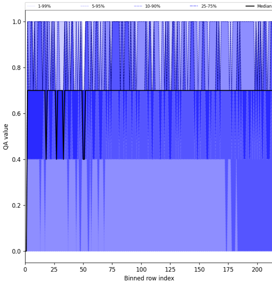
Figure 20: Along track statistics of “QA value” for 2025-07-27 to 2025-07-27
