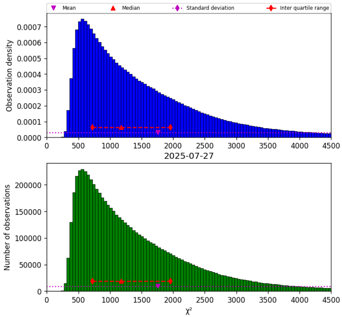
Figure 17: Histogram of “ \chi^2 ” for 2025-07-27 to 2025-07-27
