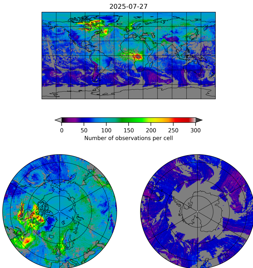
Figure 5: Map of the number of observations for 2025-07-27 to 2025-07-27
