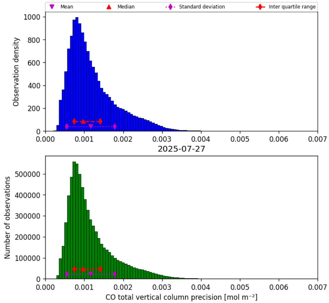
Figure 15: Histogram of “CO total vertical column precision” for 2025-07-27 to 2025-07-27
