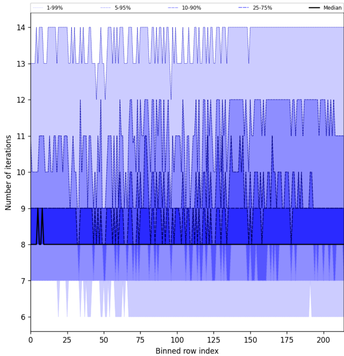
Figure 26: Along track statistics of “Number of iterations” for 2025-07-27 to 2025-07-27
