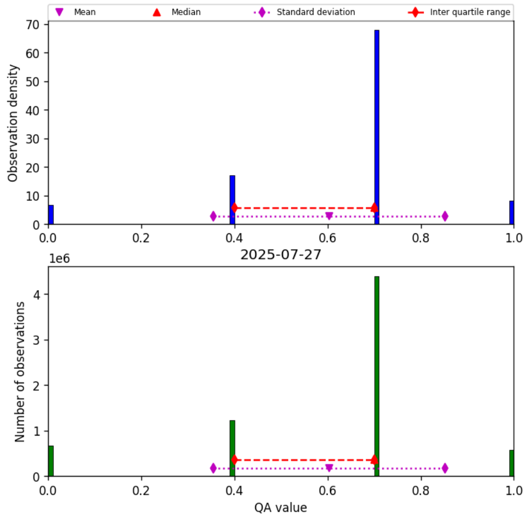
Figure 13: Histogram of “QA value” for 2025-07-27 to 2025-07-27
