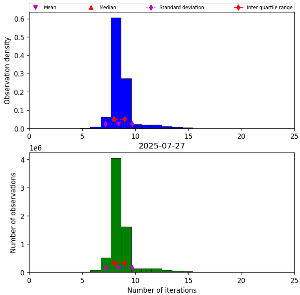
Figure 19: Histogram of “Number of iterations” for 2025-07-27 to 2025-07-27
