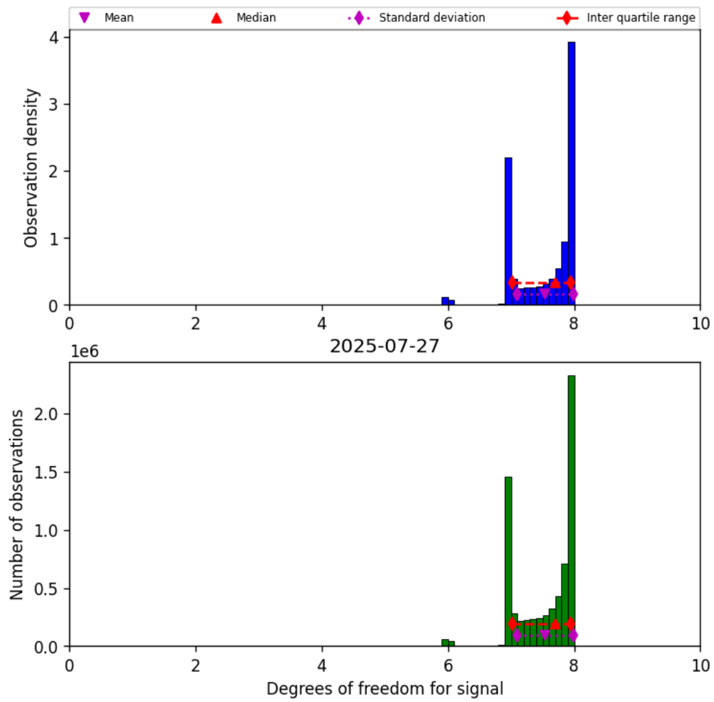
Figure 18: Histogram of “Degrees of freedom for signal” for 2025-07-27 to 2025-07-27
