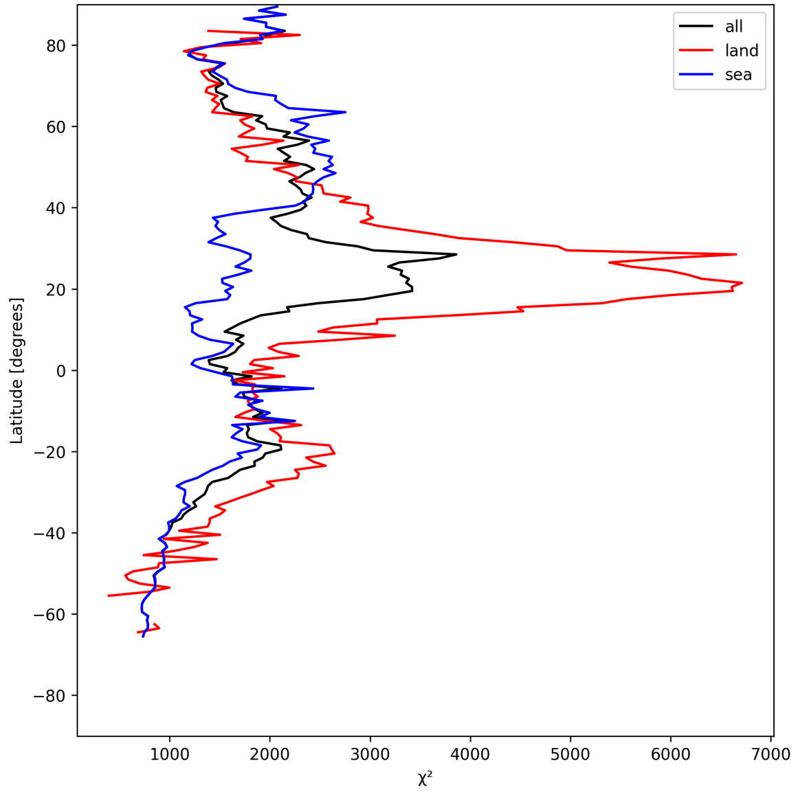
Figure 10: Zonal average of “ \chi^2 ” for 2025-07-28 to 2025-07-29.
