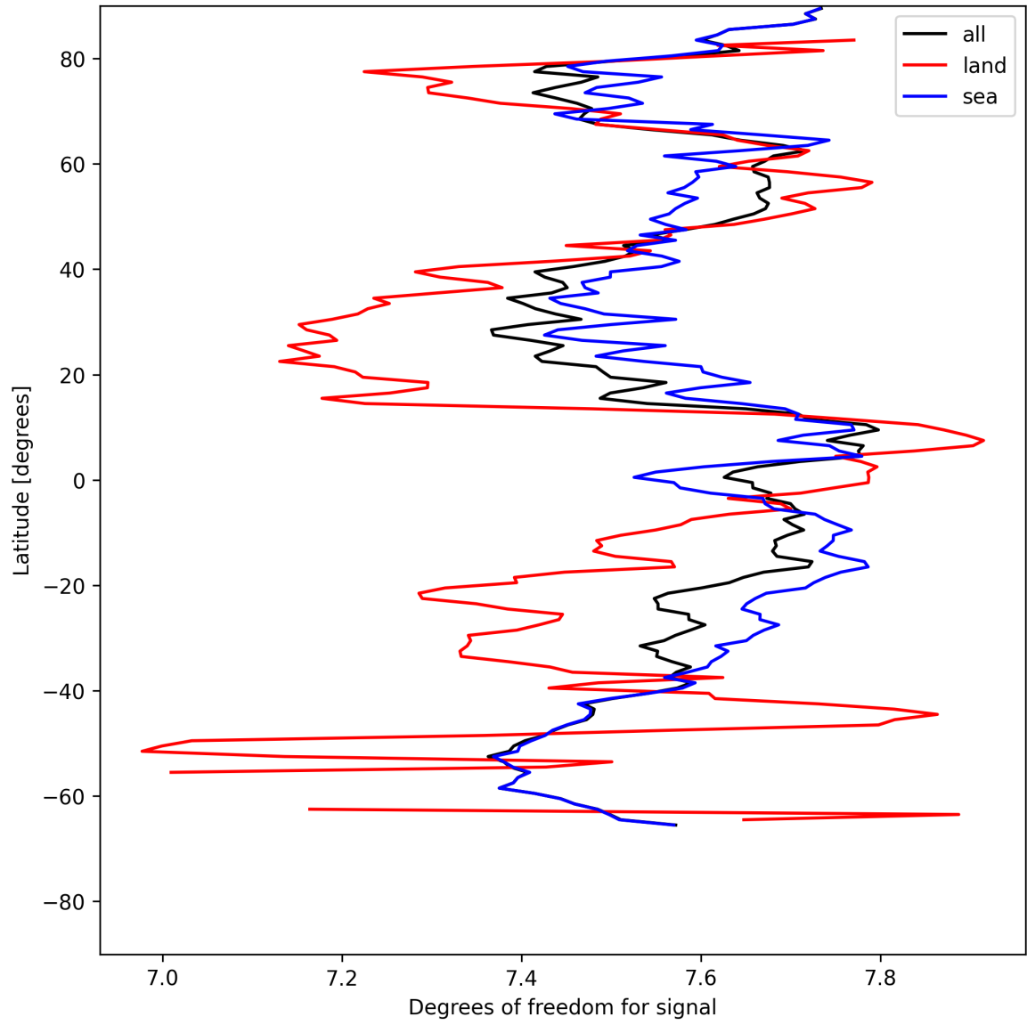
Figure 11: Zonal average of “Degrees of freedom for signal” for 2025-07-28 to 2025-07-29.
