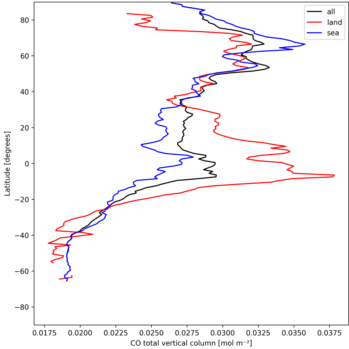
Figure 7: Zonal average of “CO total vertical column” for 2025-07-28 to 2025-07-29.
