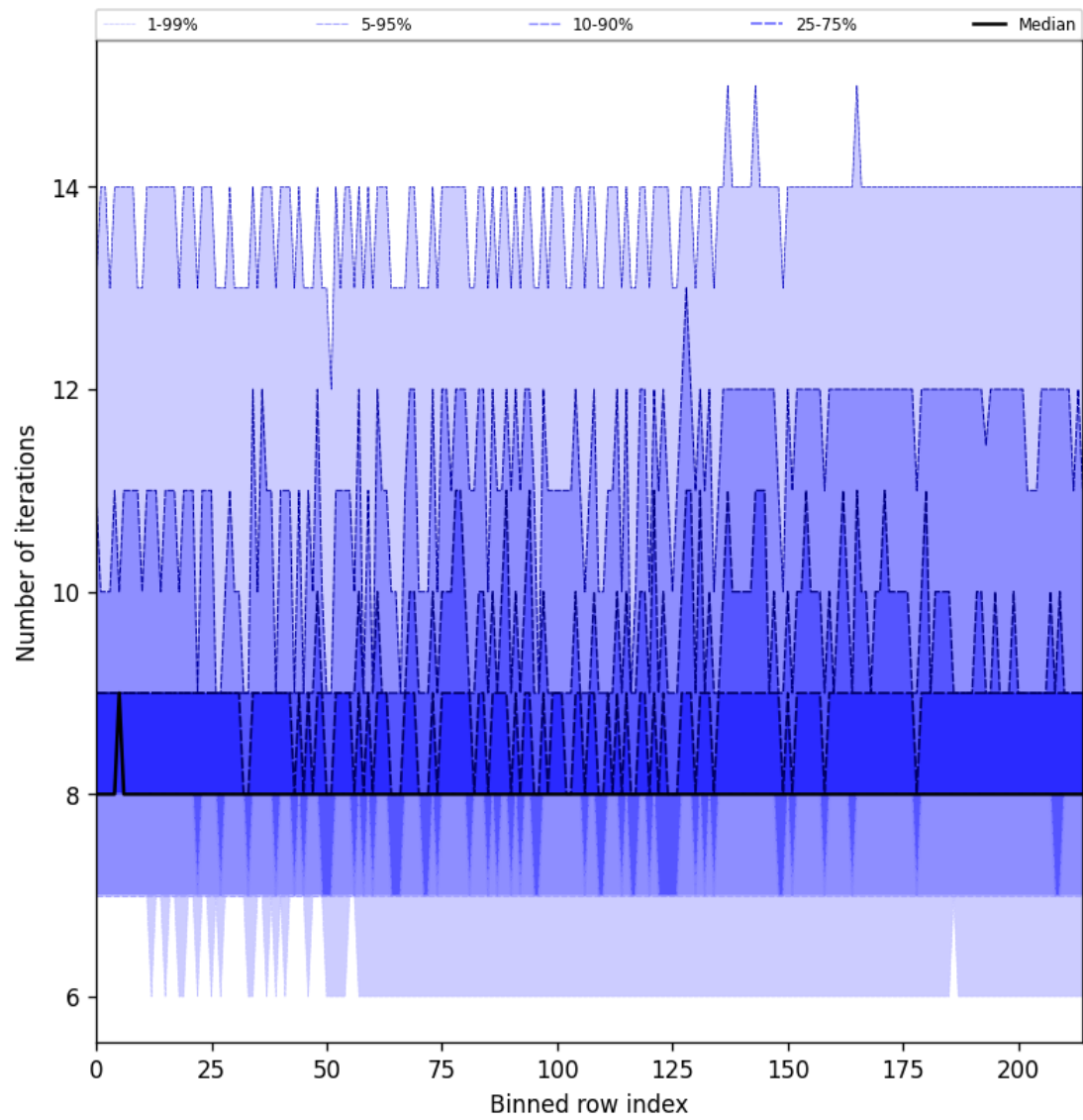
Figure 26: Along track statistics of “Number of iterations” for 2025-07-28 to 2025-07-29
