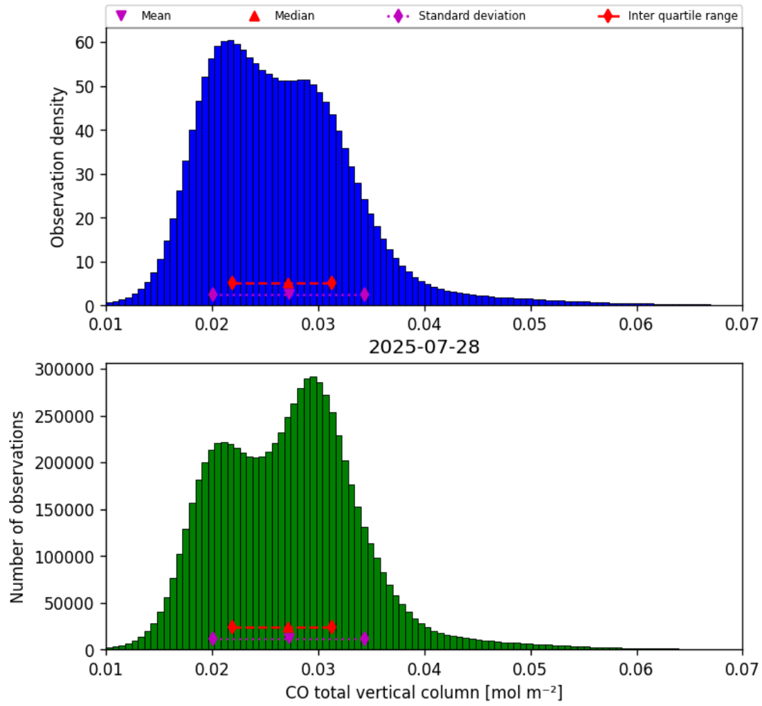
Figure 14: Histogram of “CO total vertical column” for 2025-07-28 to 2025-07-29
