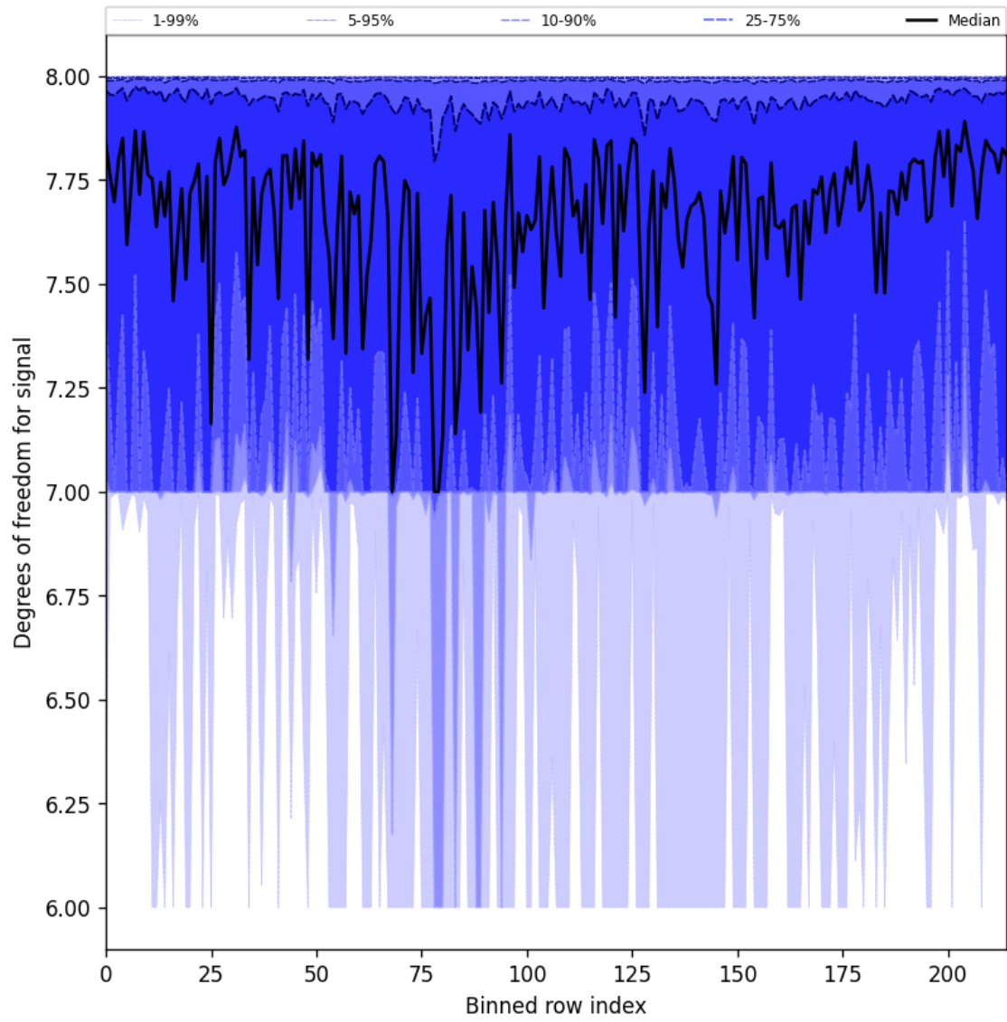
Figure 25: Along track statistics of “Degrees of freedom for signal” for 2025-07-28 to 2025-07-29
