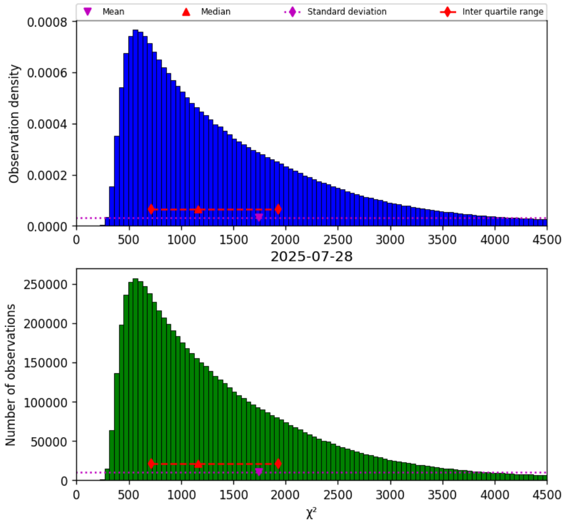
Figure 17: Histogram of “ \chi^2 ” for 2025-07-28 to 2025-07-29
