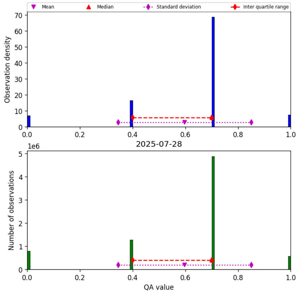
Figure 13: Histogram of “QA value” for 2025-07-28 to 2025-07-29
