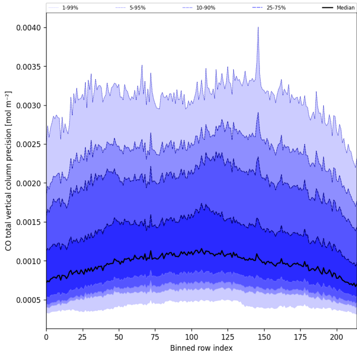
Figure 22: Along track statistics of “CO total vertical column precision” for 2025-07-28 to 2025-07-29
