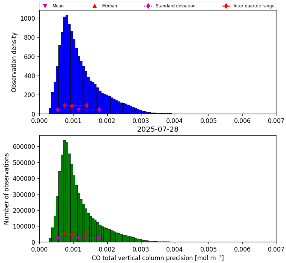
Figure 15: Histogram of “CO total vertical column precision” for 2025-07-28 to 2025-07-29
