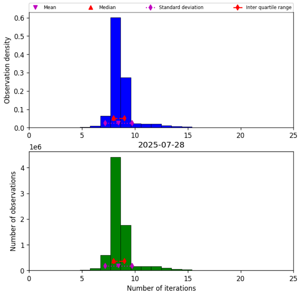
Figure 19: Histogram of “Number of iterations” for 2025-07-28 to 2025-07-29
