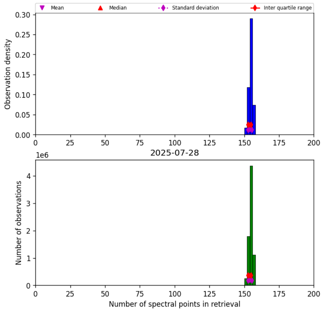
Figure 16: Histogram of “Number of spectral points in retrieval” for 2025-07-28 to 2025-07-29
