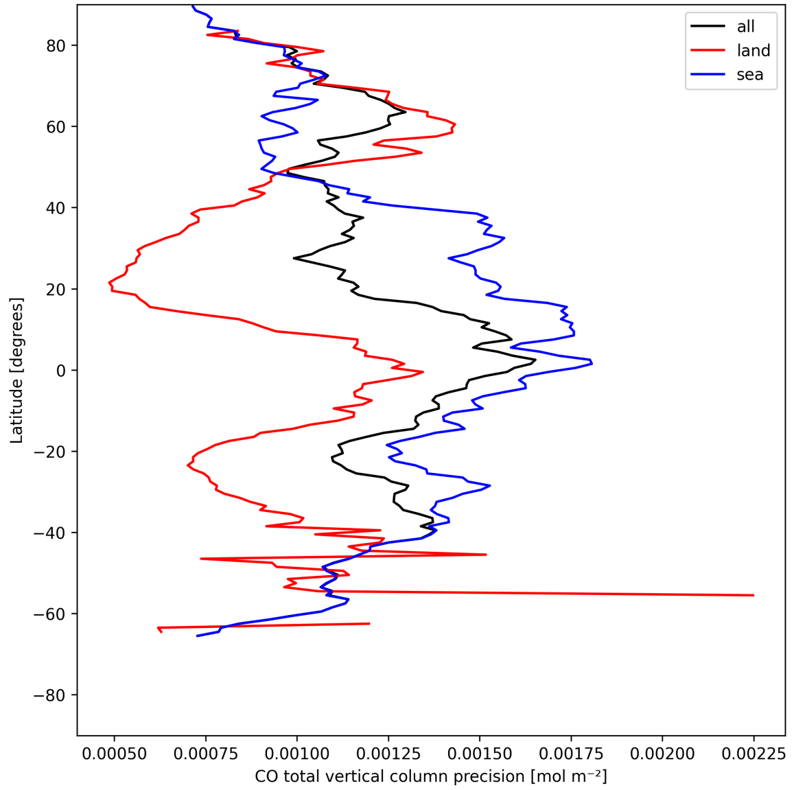
Figure 8: Zonal average of “CO total vertical column precision” for 2025-07-28 to 2025-07-29.
