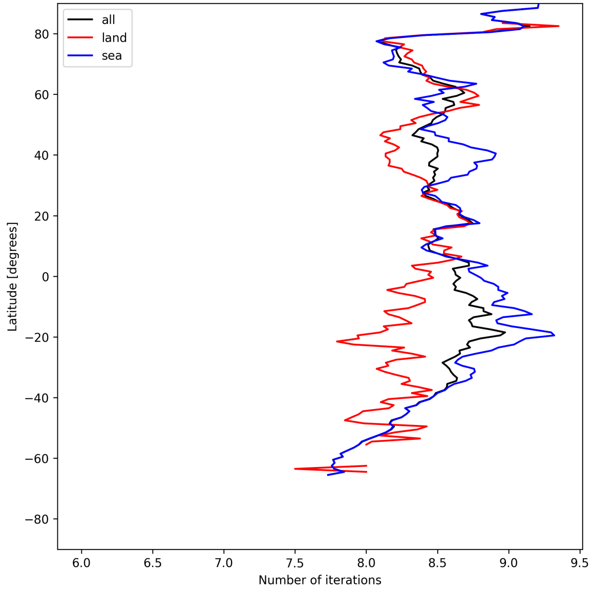
Figure 12: Zonal average of “Number of iterations” for 2025-07-28 to 2025-07-29.
