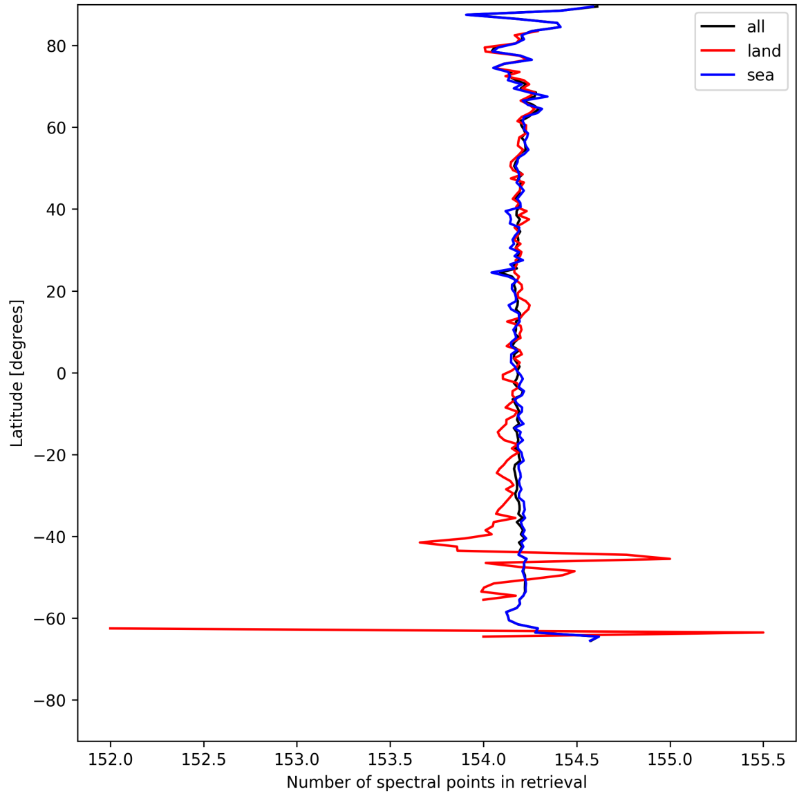
Figure 9: Zonal average of “Number of spectral points in retrieval” for 2025-07-28 to 2025-07-29.
