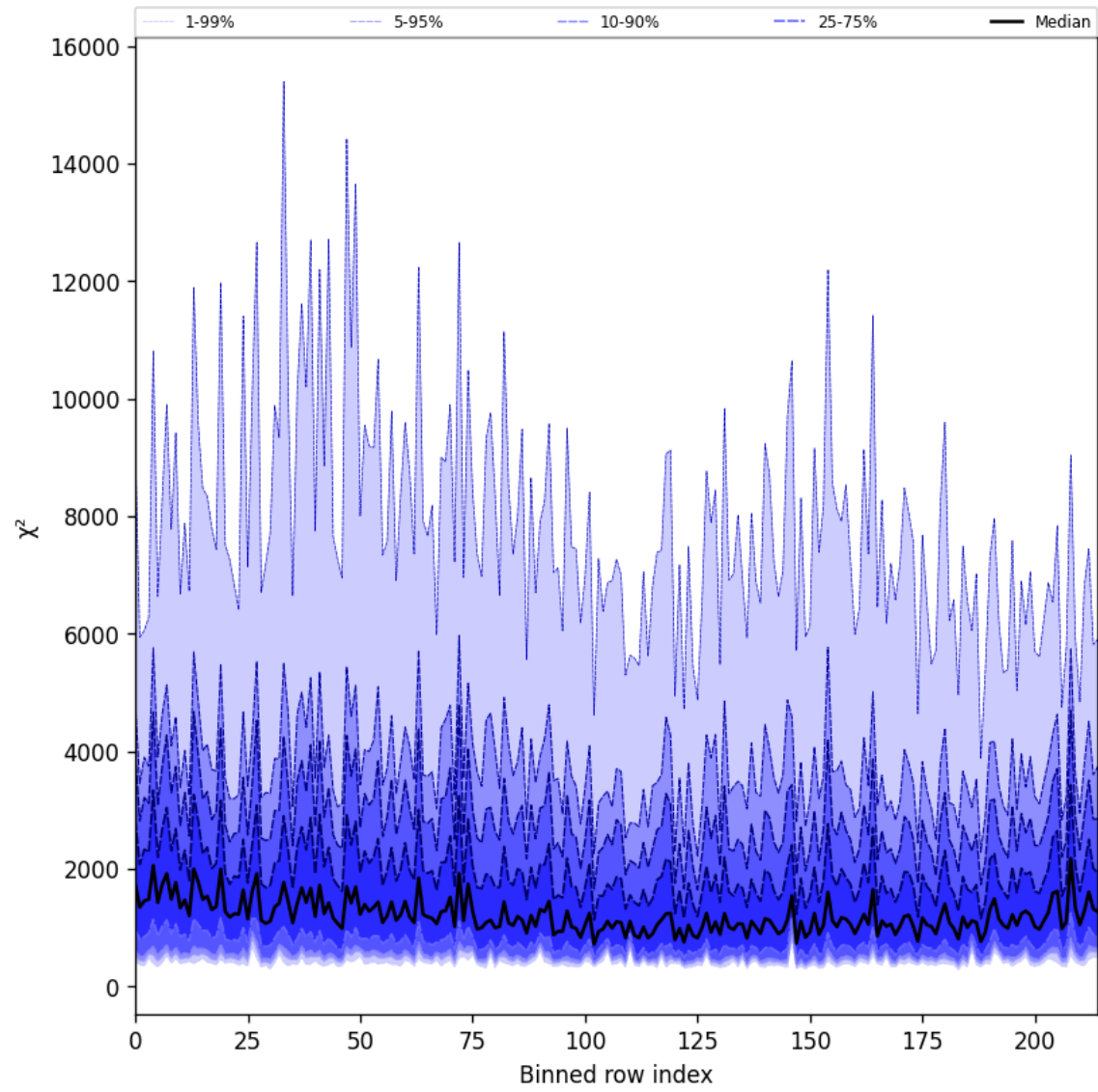
Figure 24: Along track statistics of “ \chi^2 ” for 2025-07-28 to 2025-07-29
