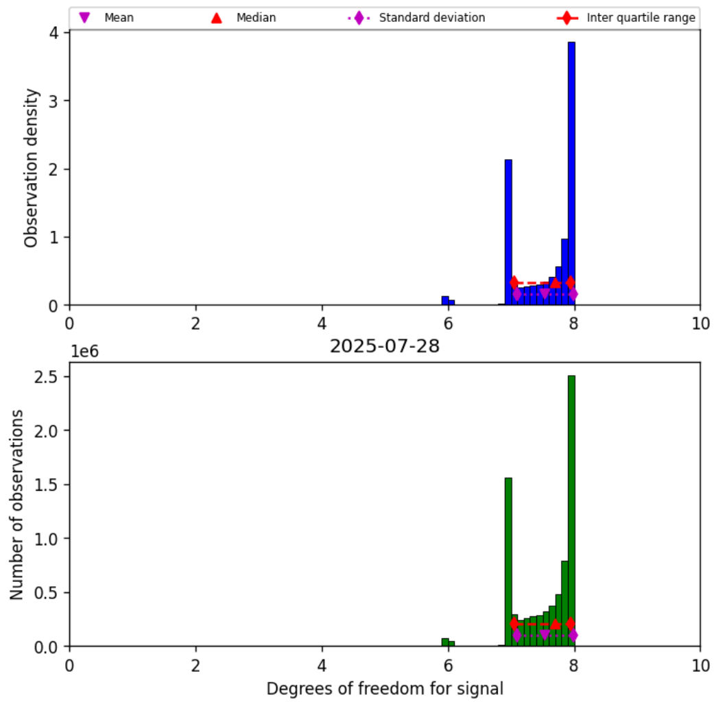
Figure 18: Histogram of “Degrees of freedom for signal” for 2025-07-28 to 2025-07-29
