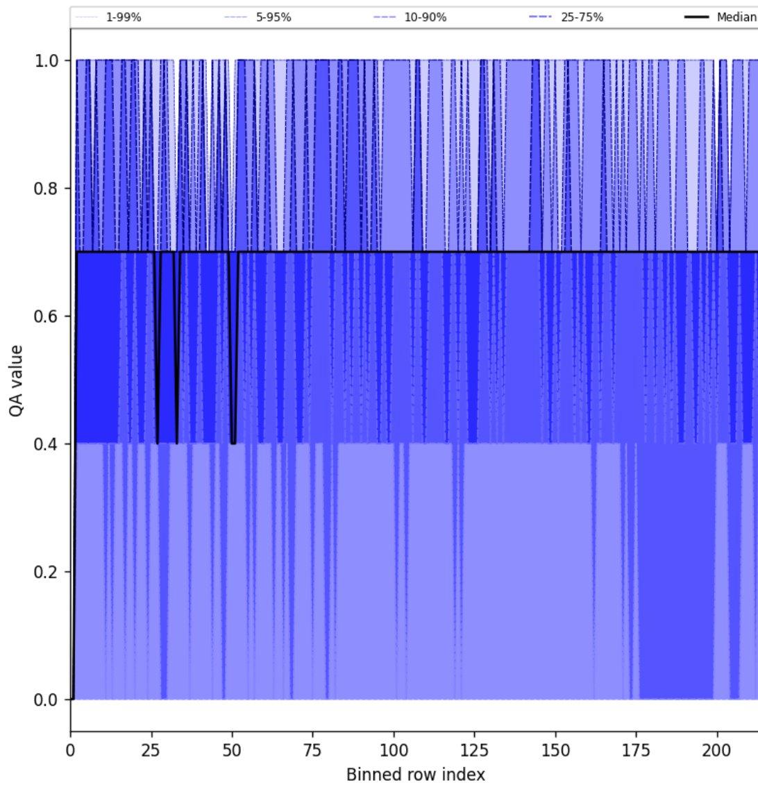
Figure 20: Along track statistics of “QA value” for 2025-07-28 to 2025-07-29
