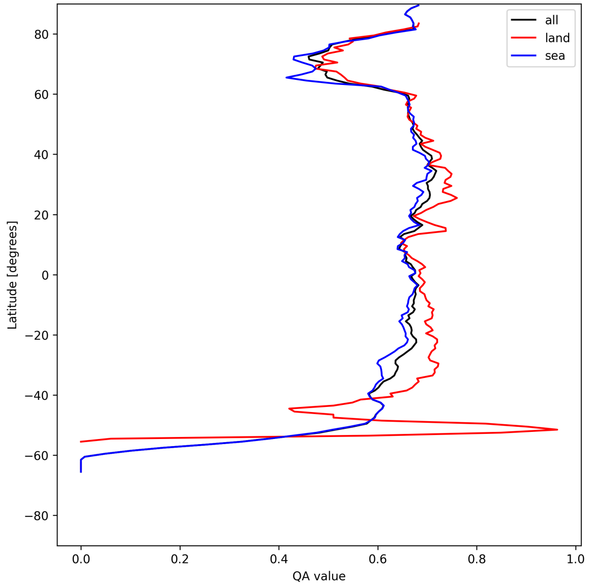
Figure 6: Zonal average of “QA value” for 2025-07-28 to 2025-07-29.
