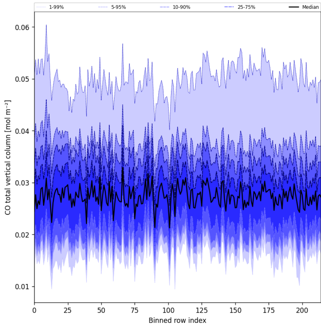
Figure 21: Along track statistics of “CO total vertical column” for 2025-07-28 to 2025-07-29
