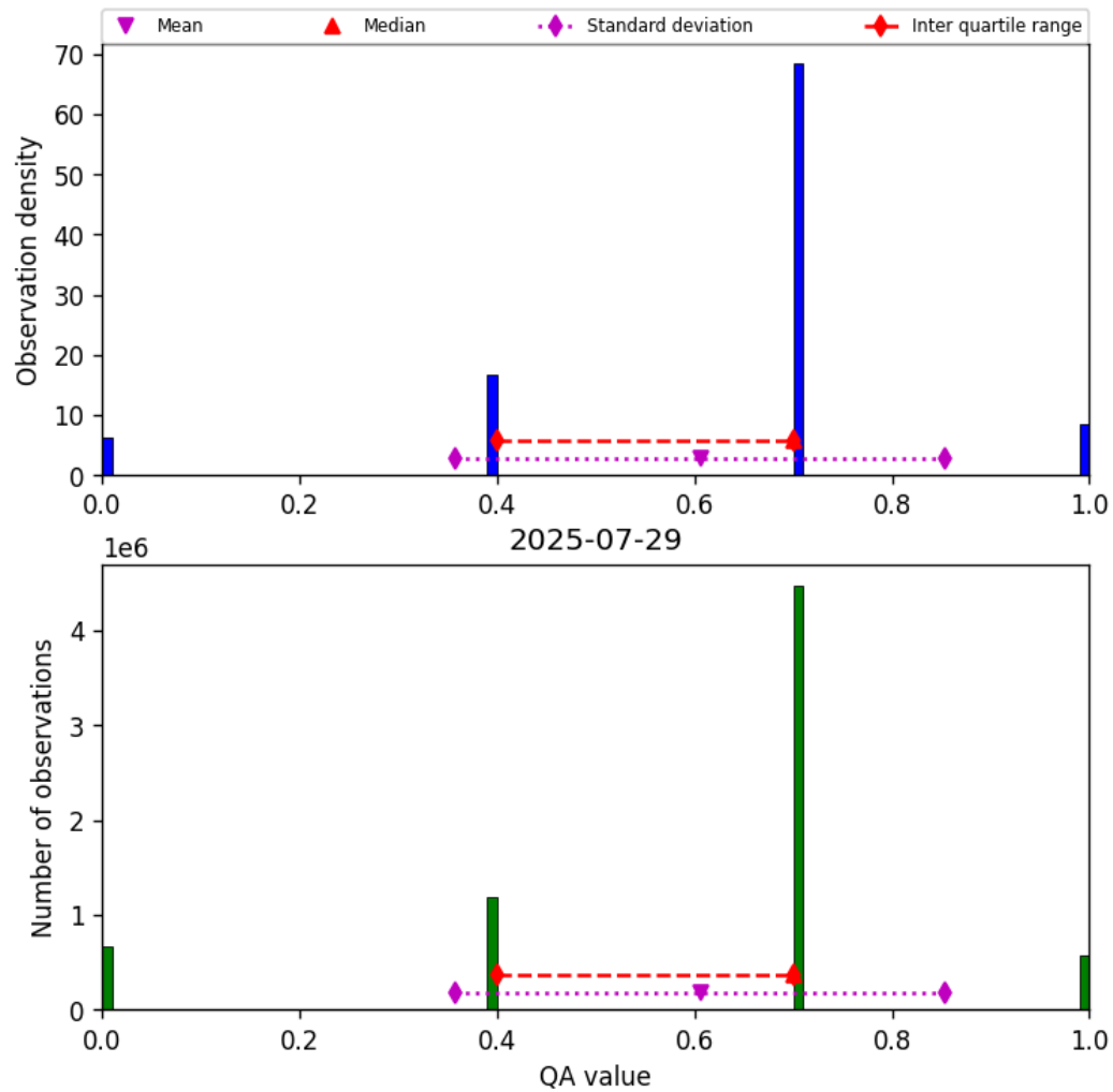
Figure 13: Histogram of “QA value” for 2025-07-29 to 2025-07-30
