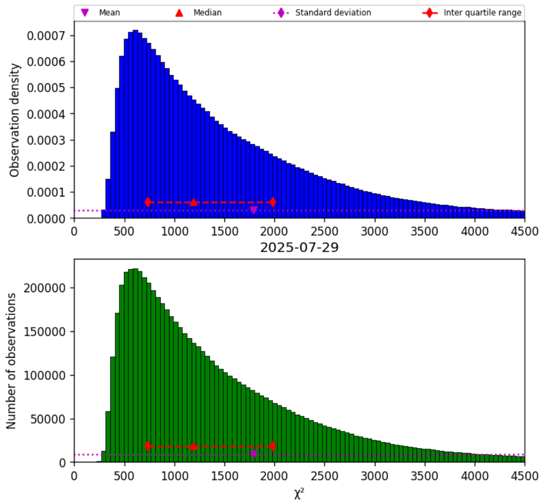
Figure 17: Histogram of “ \chi^2 ” for 2025-07-29 to 2025-07-30
