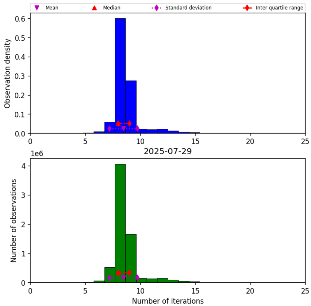
Figure 19: Histogram of “Number of iterations” for 2025-07-29 to 2025-07-30
