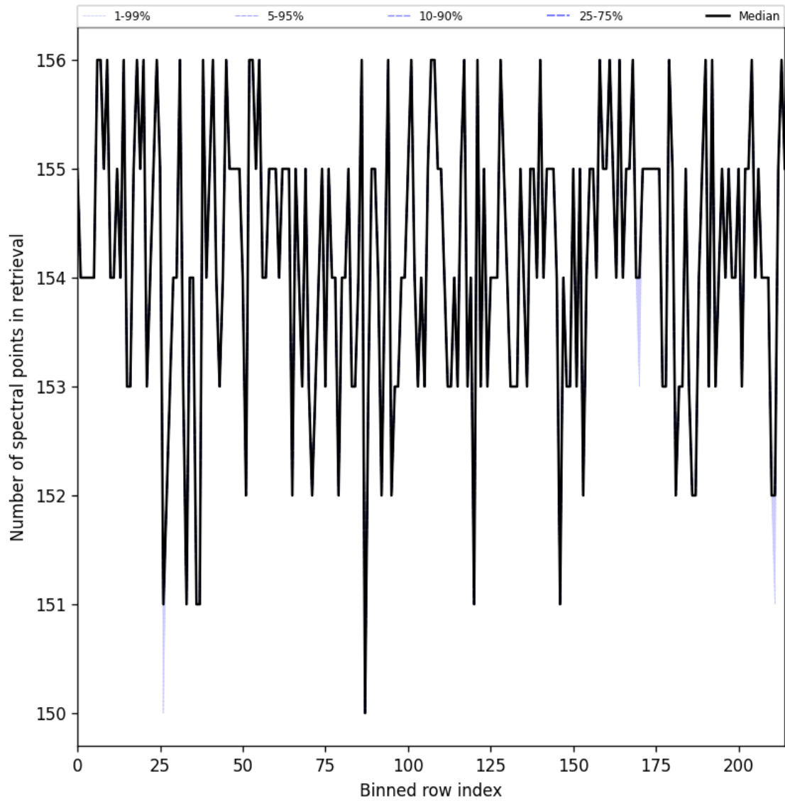
Figure 23: Along track statistics of “Number of spectral points in retrieval” for 2025-07-29 to 2025-07-30
