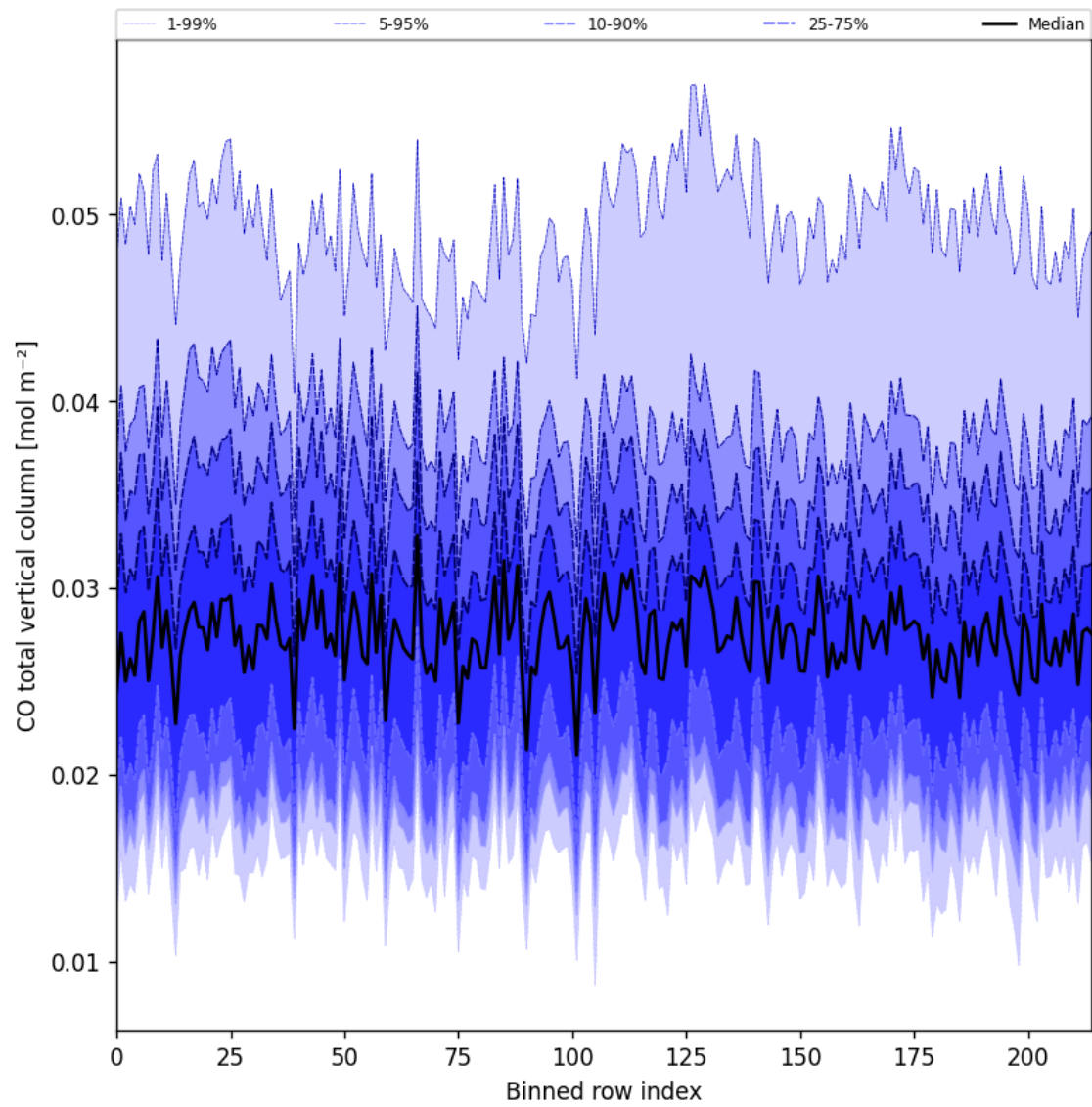
Figure 21: Along track statistics of “CO total vertical column” for 2025-07-29 to 2025-07-30
