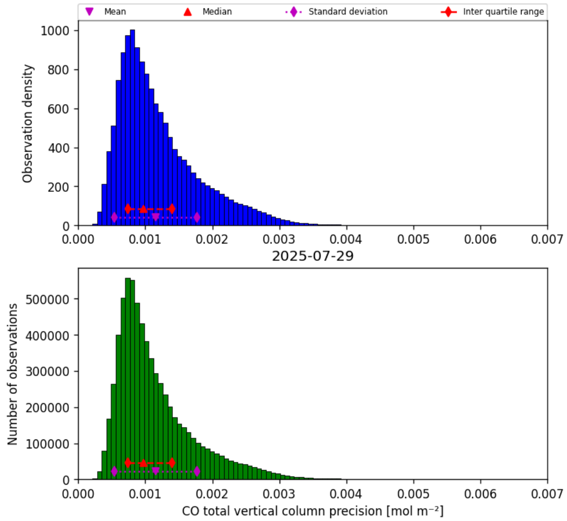
Figure 15: Histogram of “CO total vertical column precision” for 2025-07-29 to 2025-07-30
