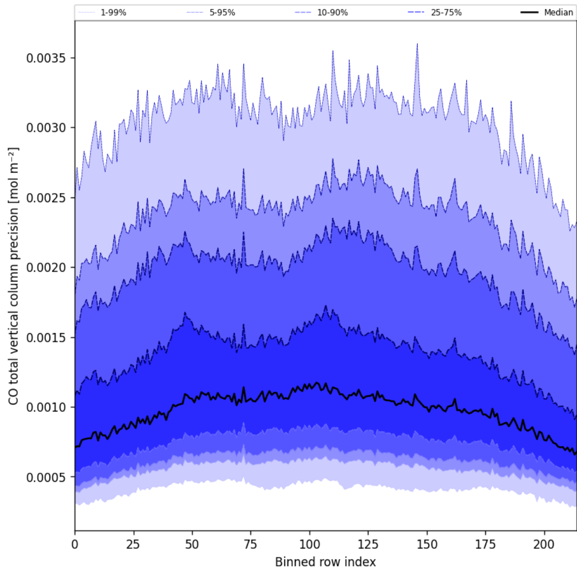
Figure 22: Along track statistics of “CO total vertical column precision” for 2025-07-29 to 2025-07-30
