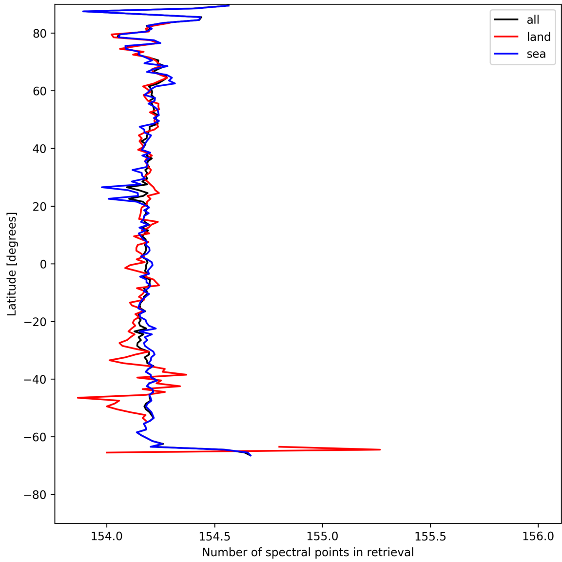
Figure 9: Zonal average of “Number of spectral points in retrieval” for 2025-07-29 to 2025-07-30.
