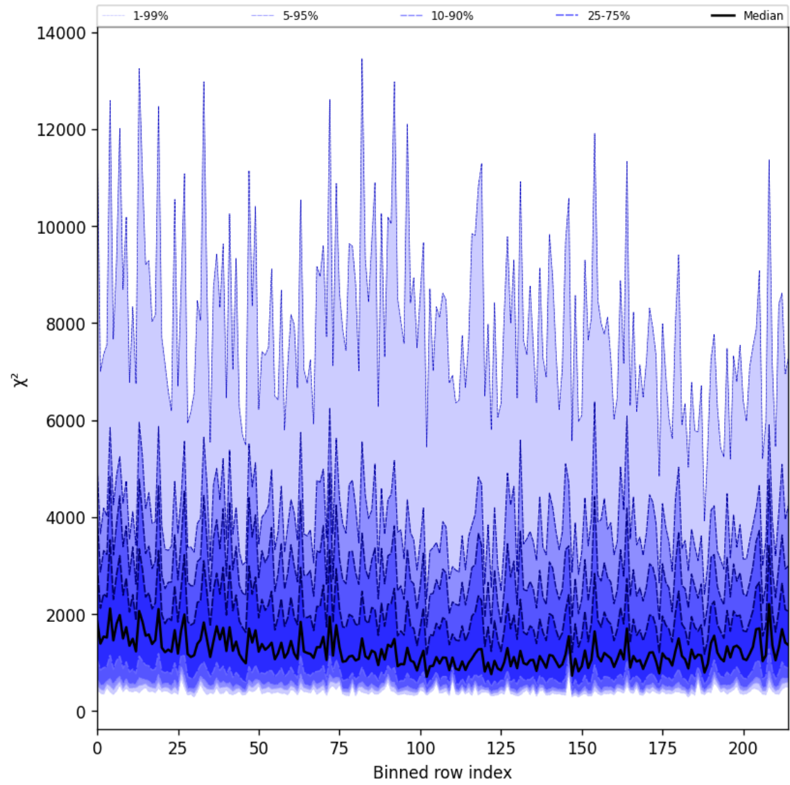
Figure 24: Along track statistics of “ \chi^2 ” for 2025-07-29 to 2025-07-30
