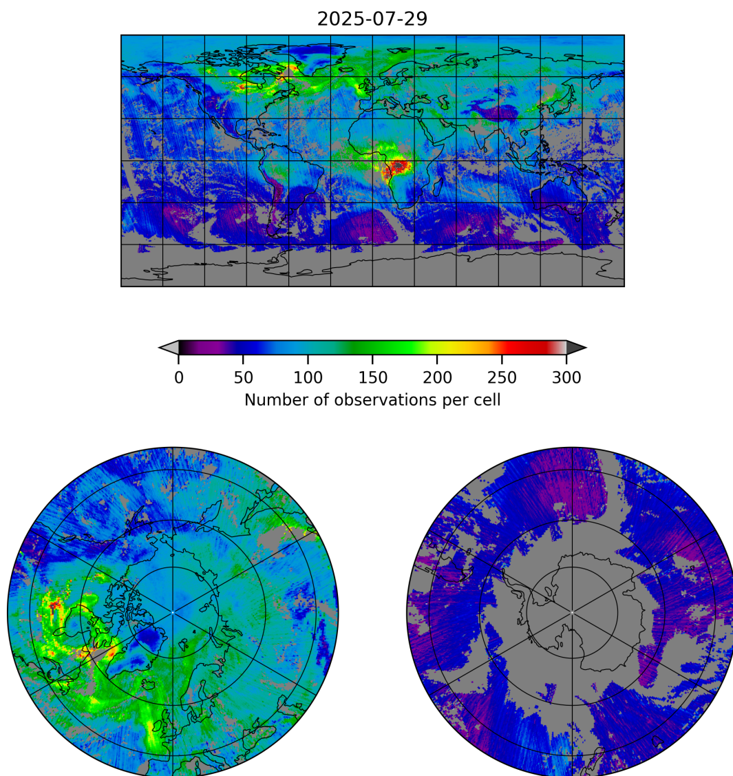
Figure 5: Map of the number of observations for 2025-07-29 to 2025-07-30
