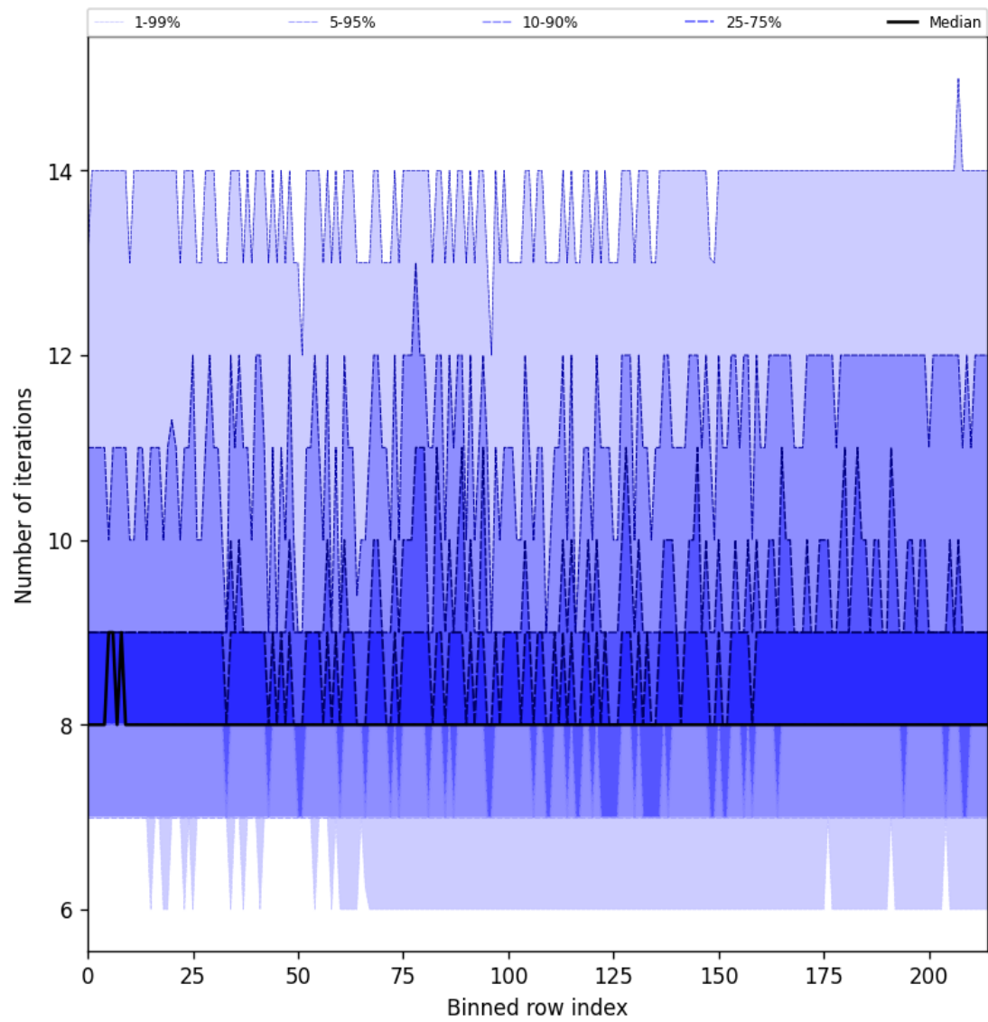
Figure 26: Along track statistics of “Number of iterations” for 2025-07-29 to 2025-07-30
