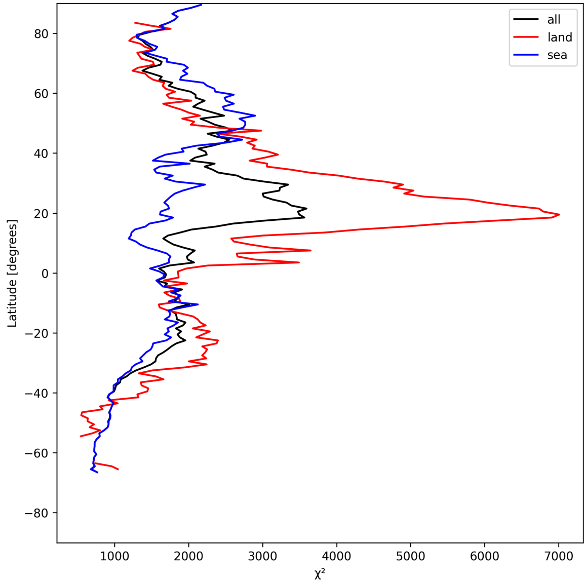
Figure 10: Zonal average of “ \chi^2 ” for 2025-07-29 to 2025-07-30.
