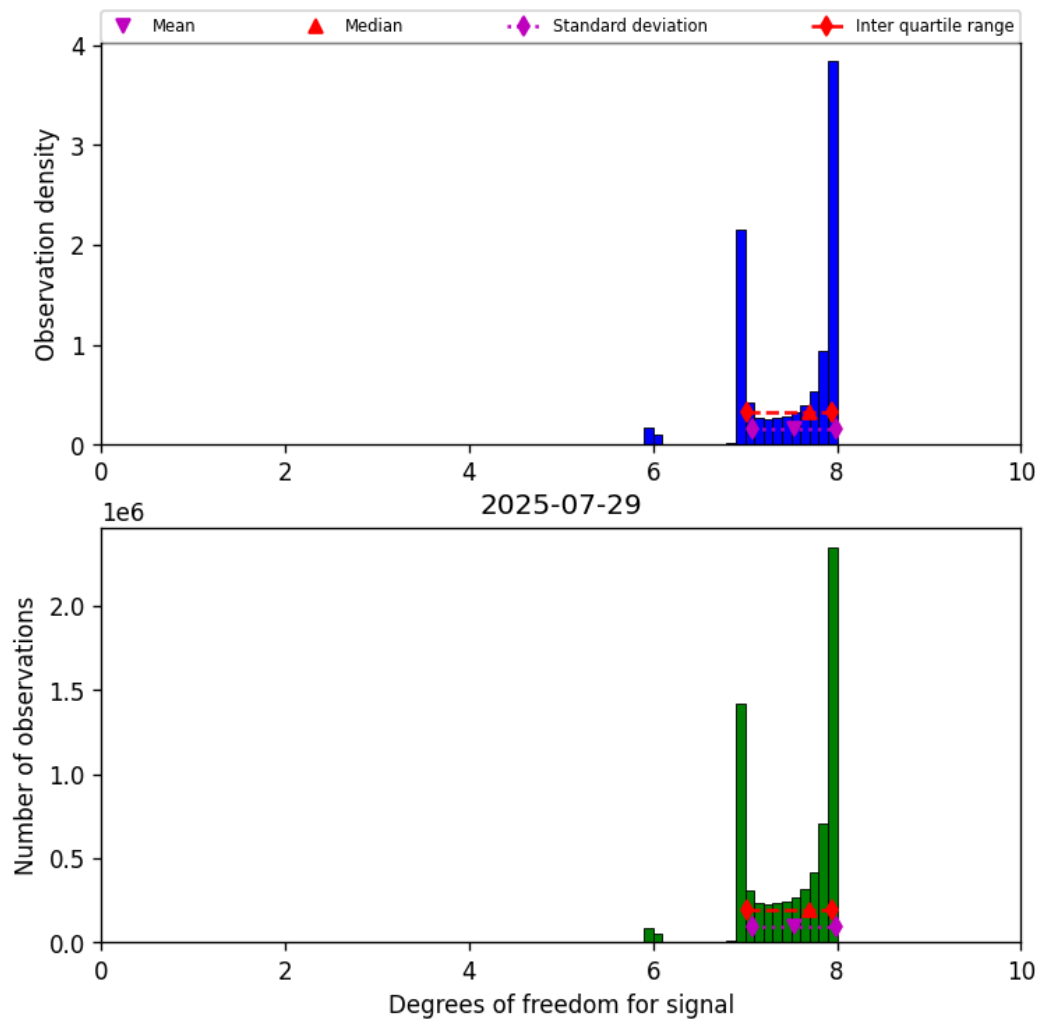
Figure 18: Histogram of “Degrees of freedom for signal” for 2025-07-29 to 2025-07-30
