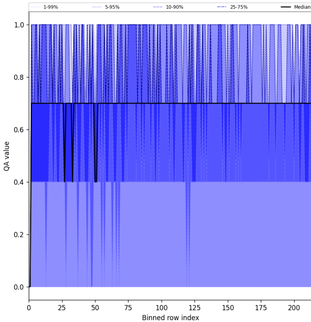
Figure 20: Along track statistics of “QA value” for 2025-07-29 to 2025-07-30
