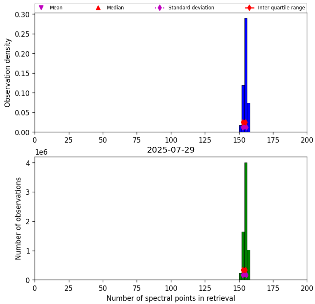
Figure 16: Histogram of “Number of spectral points in retrieval” for 2025-07-29 to 2025-07-30
