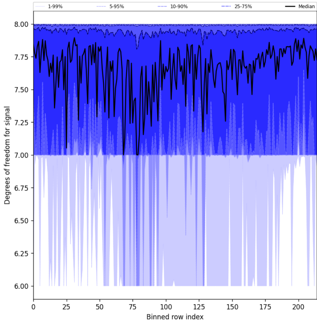
Figure 25: Along track statistics of “Degrees of freedom for signal” for 2025-07-29 to 2025-07-30
