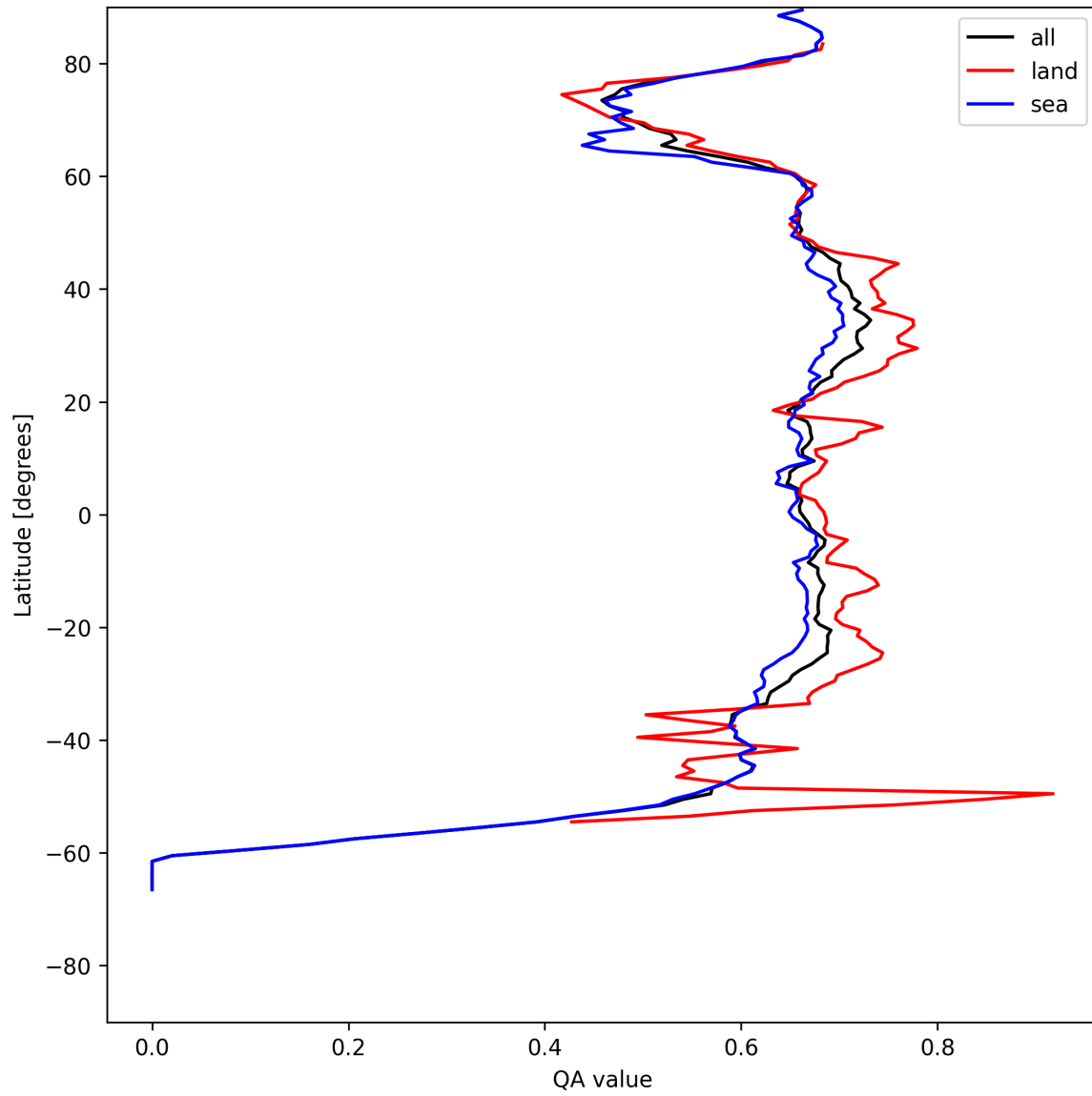
Figure 6: Zonal average of “QA value” for 2025-07-29 to 2025-07-30.
