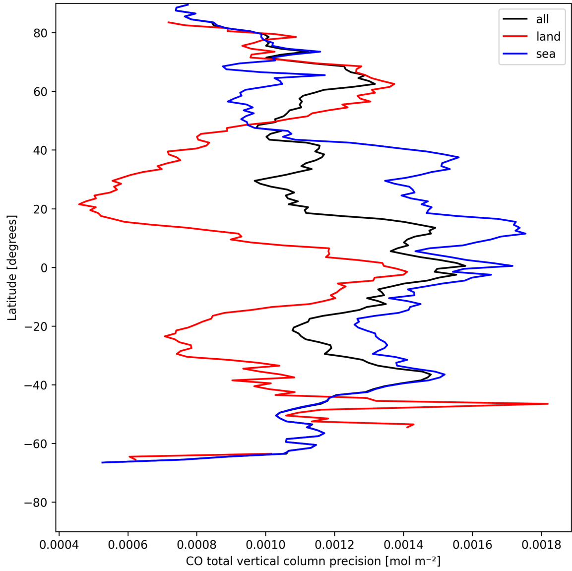
Figure 8: Zonal average of “CO total vertical column precision” for 2025-07-29 to 2025-07-30.
