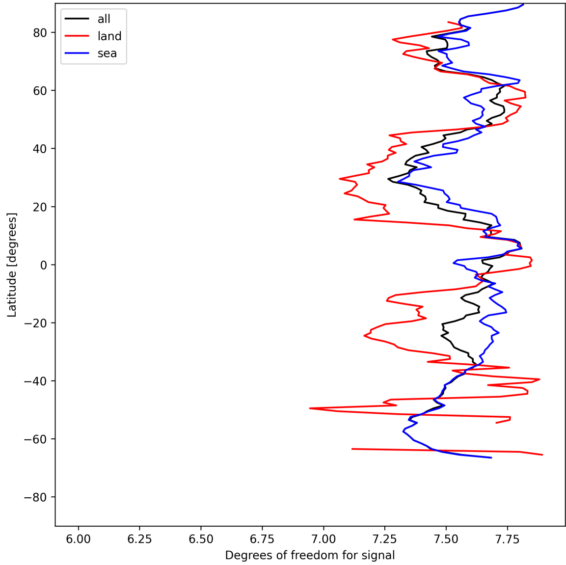
Figure 11: Zonal average of “Degrees of freedom for signal” for 2025-07-29 to 2025-07-30.
