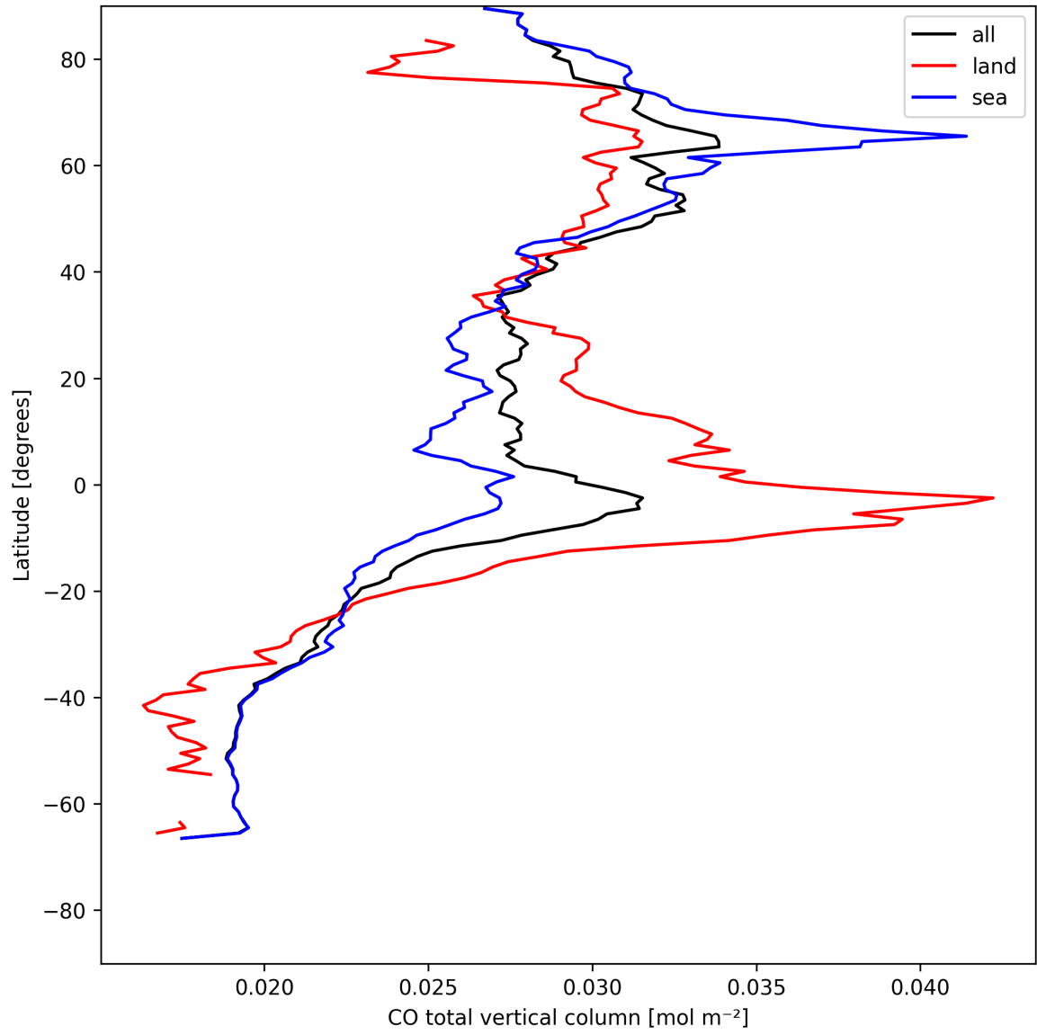
Figure 7: Zonal average of “CO total vertical column” for 2025-07-29 to 2025-07-30.
