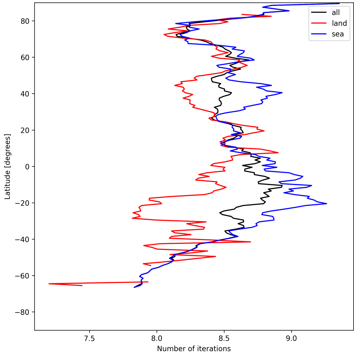
Figure 12: Zonal average of “Number of iterations” for 2025-07-29 to 2025-07-30.
