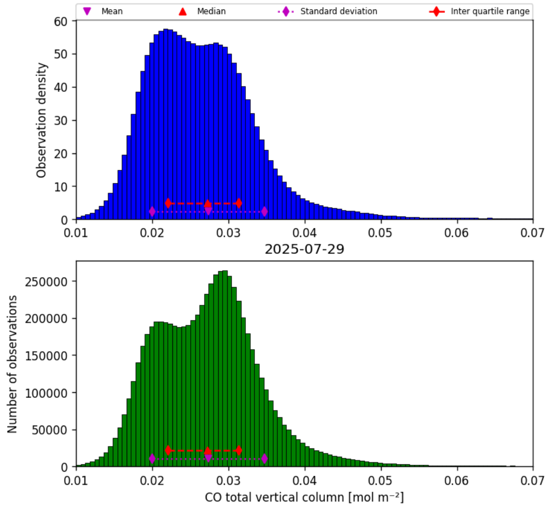
Figure 14: Histogram of “CO total vertical column” for 2025-07-29 to 2025-07-30
