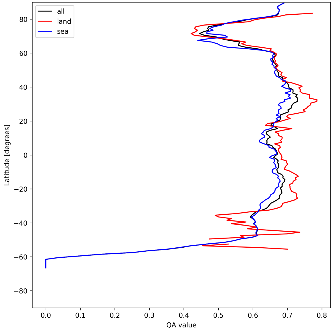
Figure 6: Zonal average of “QA value” for 2025-07-30 to 2025-07-31.
