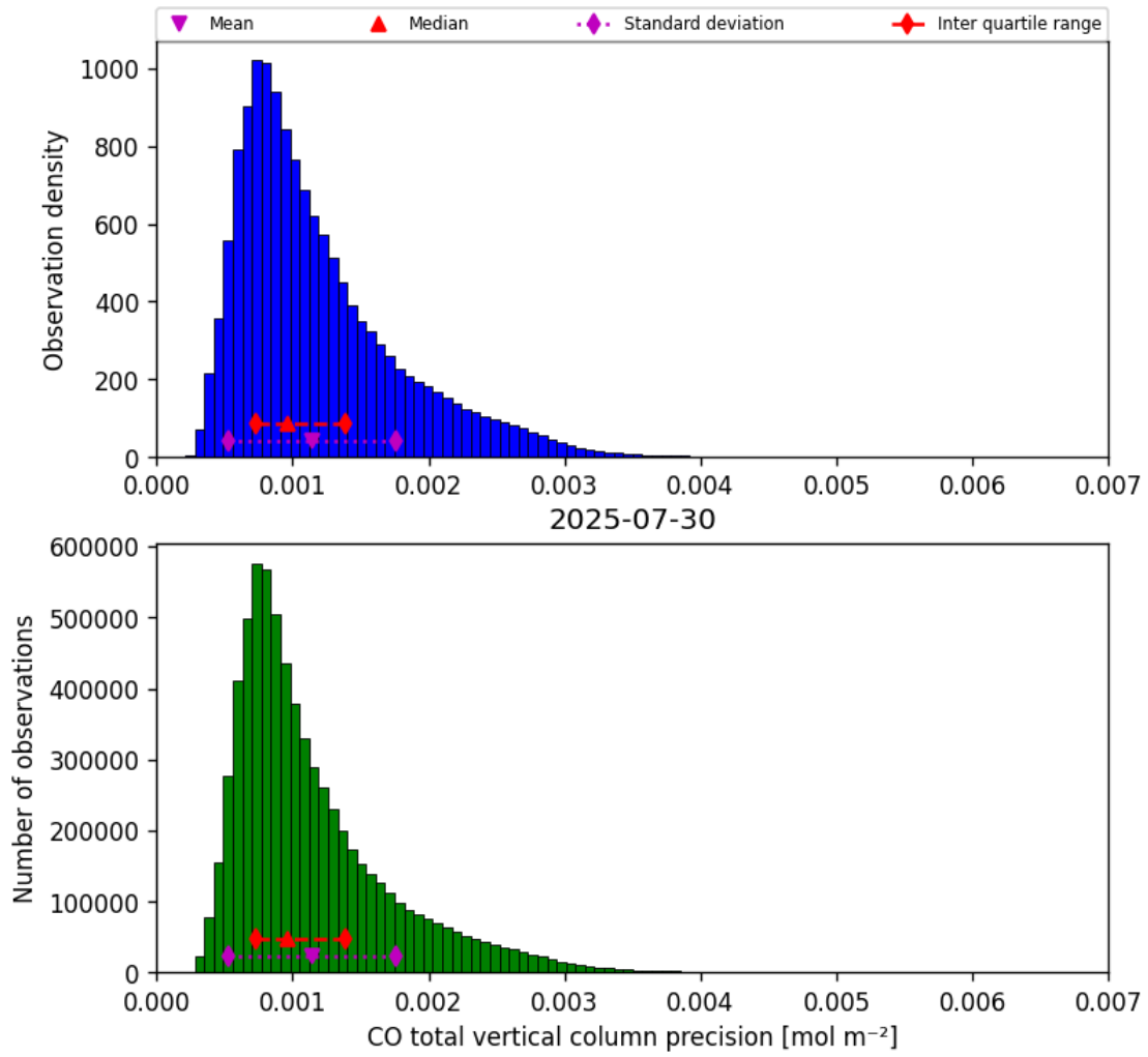
Figure 15: Histogram of “CO total vertical column precision” for 2025-07-30 to 2025-07-31
