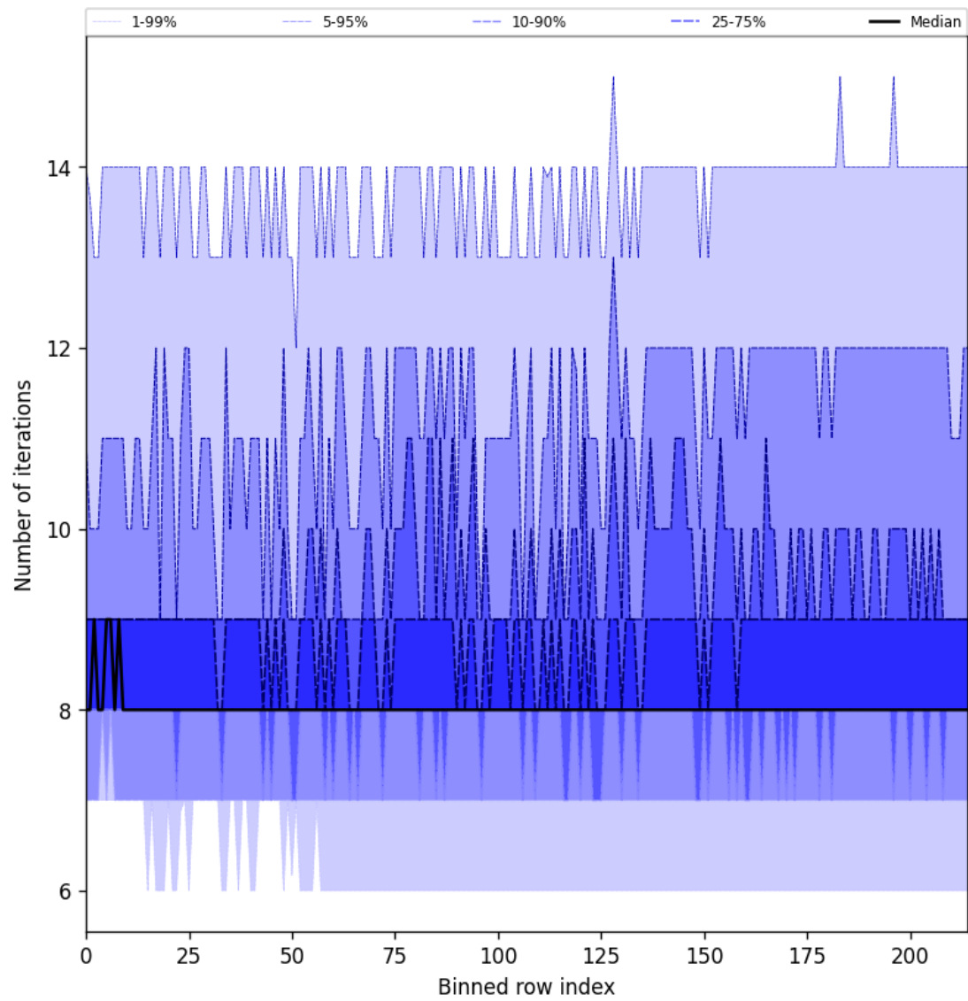
Figure 26: Along track statistics of “Number of iterations” for 2025-07-30 to 2025-07-31
