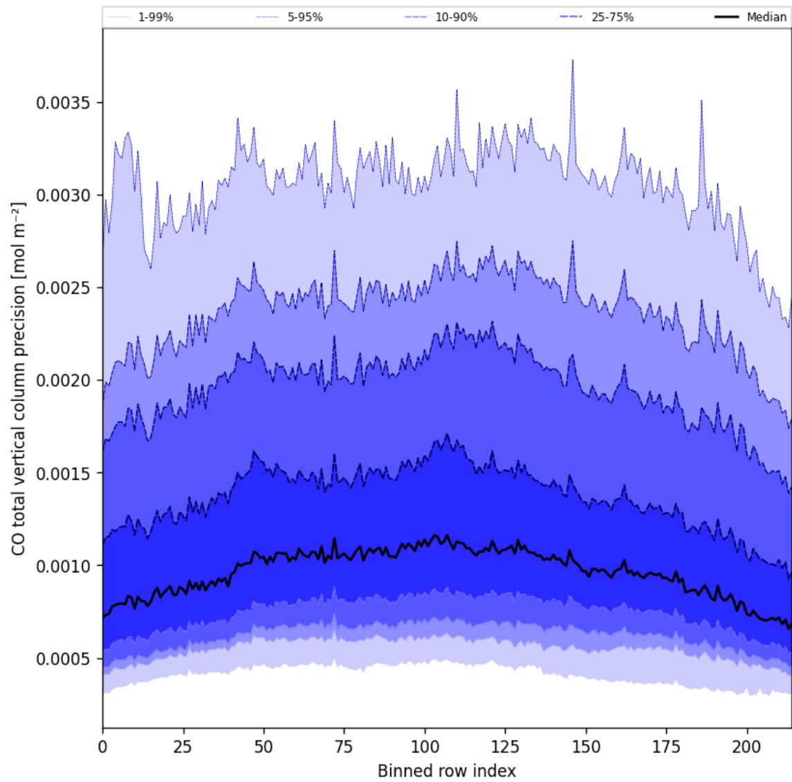
Figure 22: Along track statistics of “CO total vertical column precision” for 2025-07-30 to 2025-07-31
