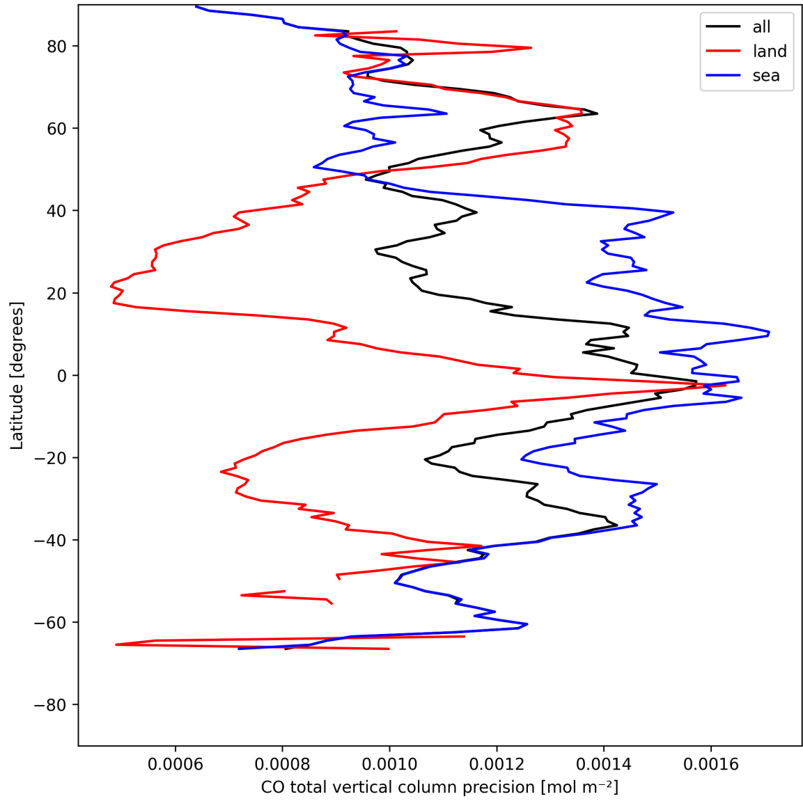
Figure 8: Zonal average of “CO total vertical column precision” for 2025-07-30 to 2025-07-31.
