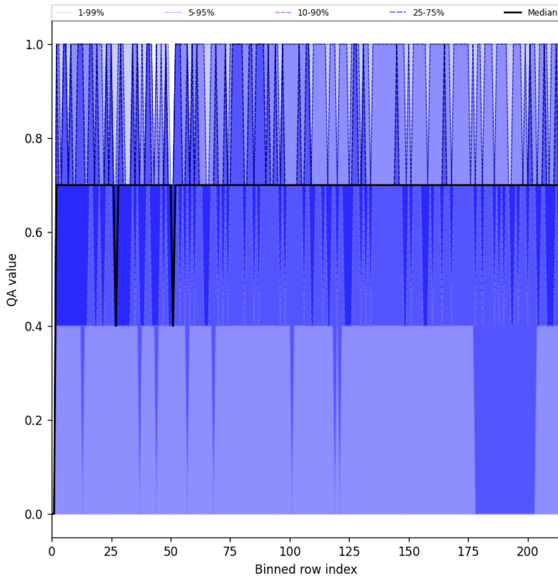
Figure 20: Along track statistics of “QA value” for 2025-07-30 to 2025-07-31
