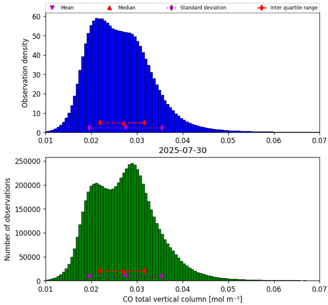
Figure 14: Histogram of “CO total vertical column” for 2025-07-30 to 2025-07-31
