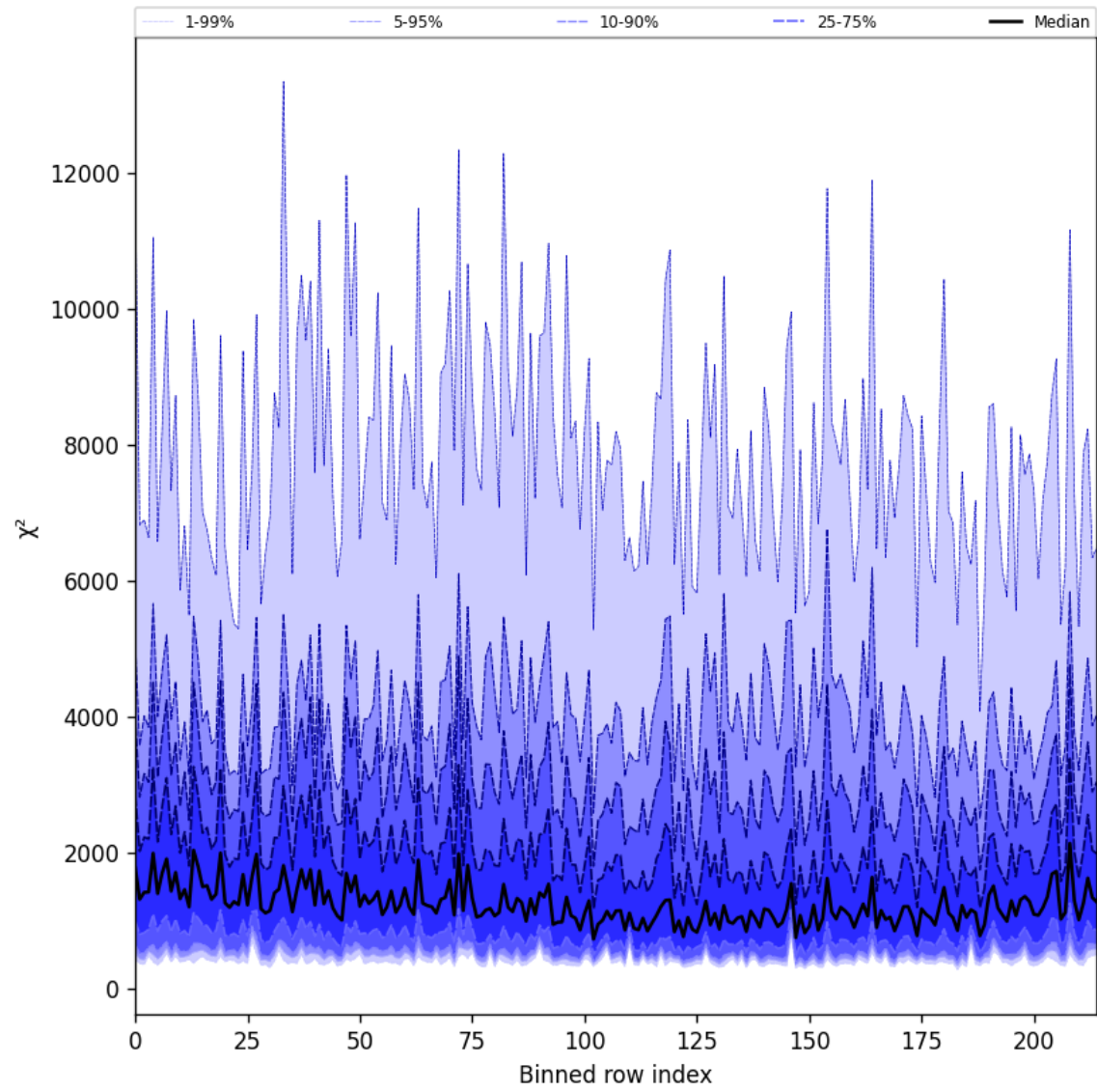
Figure 24: Along track statistics of “ \chi^2 ” for 2025-07-30 to 2025-07-31
