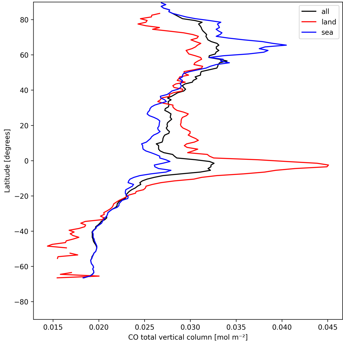
Figure 7: Zonal average of “CO total vertical column” for 2025-07-30 to 2025-07-31.
