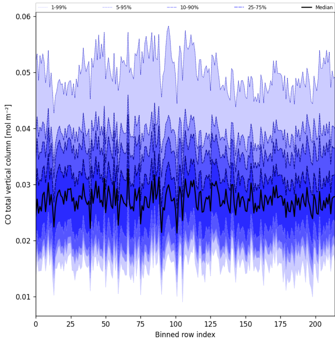
Figure 21: Along track statistics of “CO total vertical column” for 2025-07-30 to 2025-07-31
