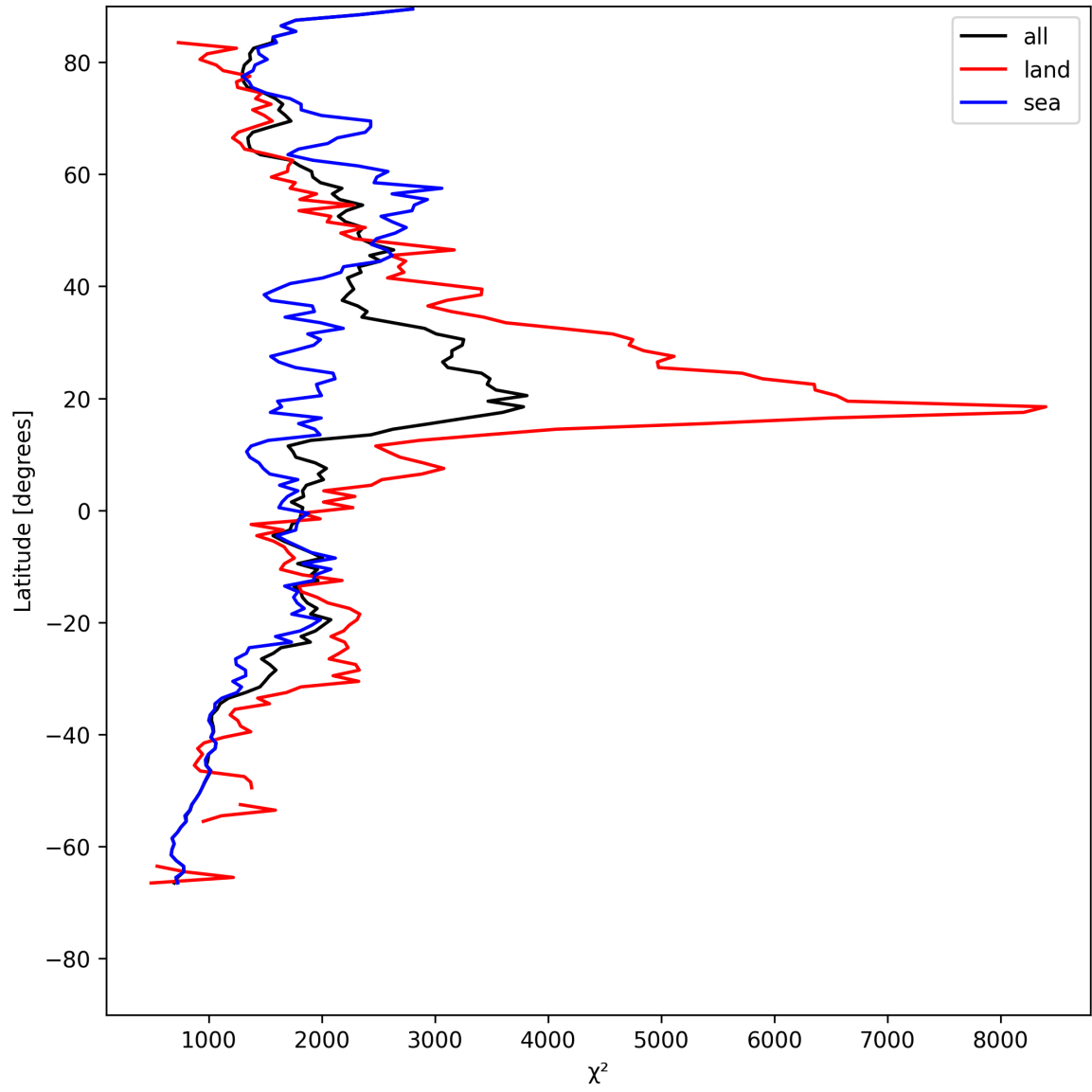
Figure 10: Zonal average of “ \chi^2 ” for 2025-07-30 to 2025-07-31.
