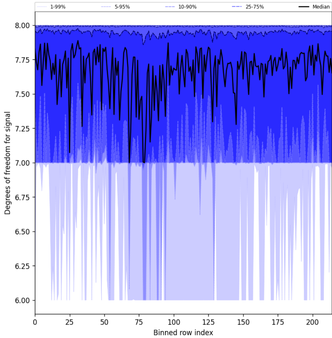
Figure 25: Along track statistics of “Degrees of freedom for signal” for 2025-07-30 to 2025-07-31
