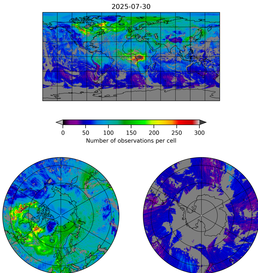
Figure 5: Map of the number of observations for 2025-07-30 to 2025-07-31
