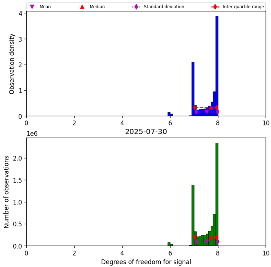
Figure 18: Histogram of “Degrees of freedom for signal” for 2025-07-30 to 2025-07-31
