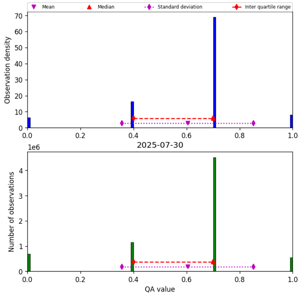
Figure 13: Histogram of “QA value” for 2025-07-30 to 2025-07-31
