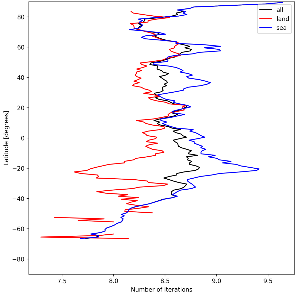
Figure 12: Zonal average of “Number of iterations” for 2025-07-30 to 2025-07-31.
