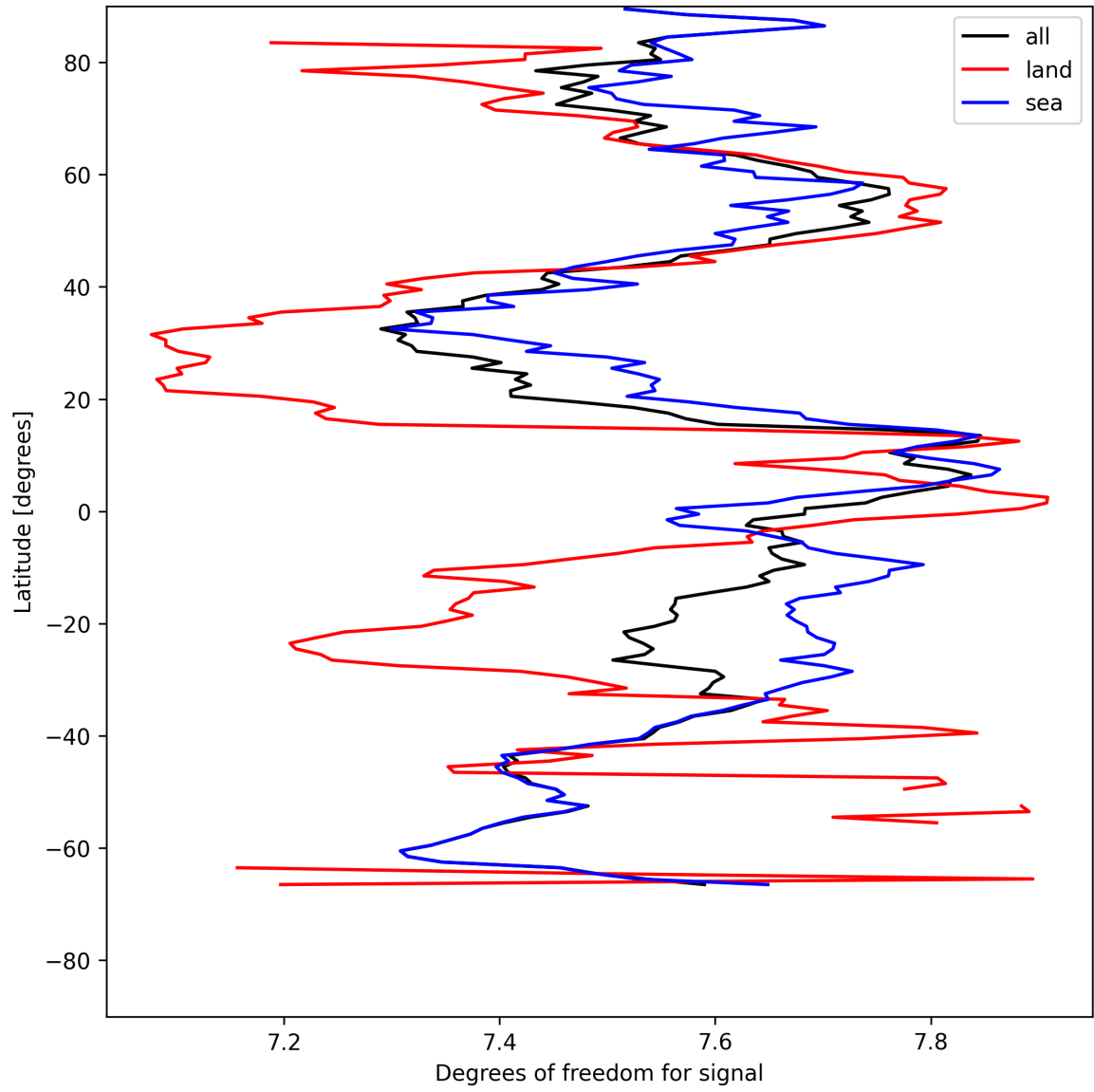
Figure 11: Zonal average of “Degrees of freedom for signal” for 2025-07-30 to 2025-07-31.
