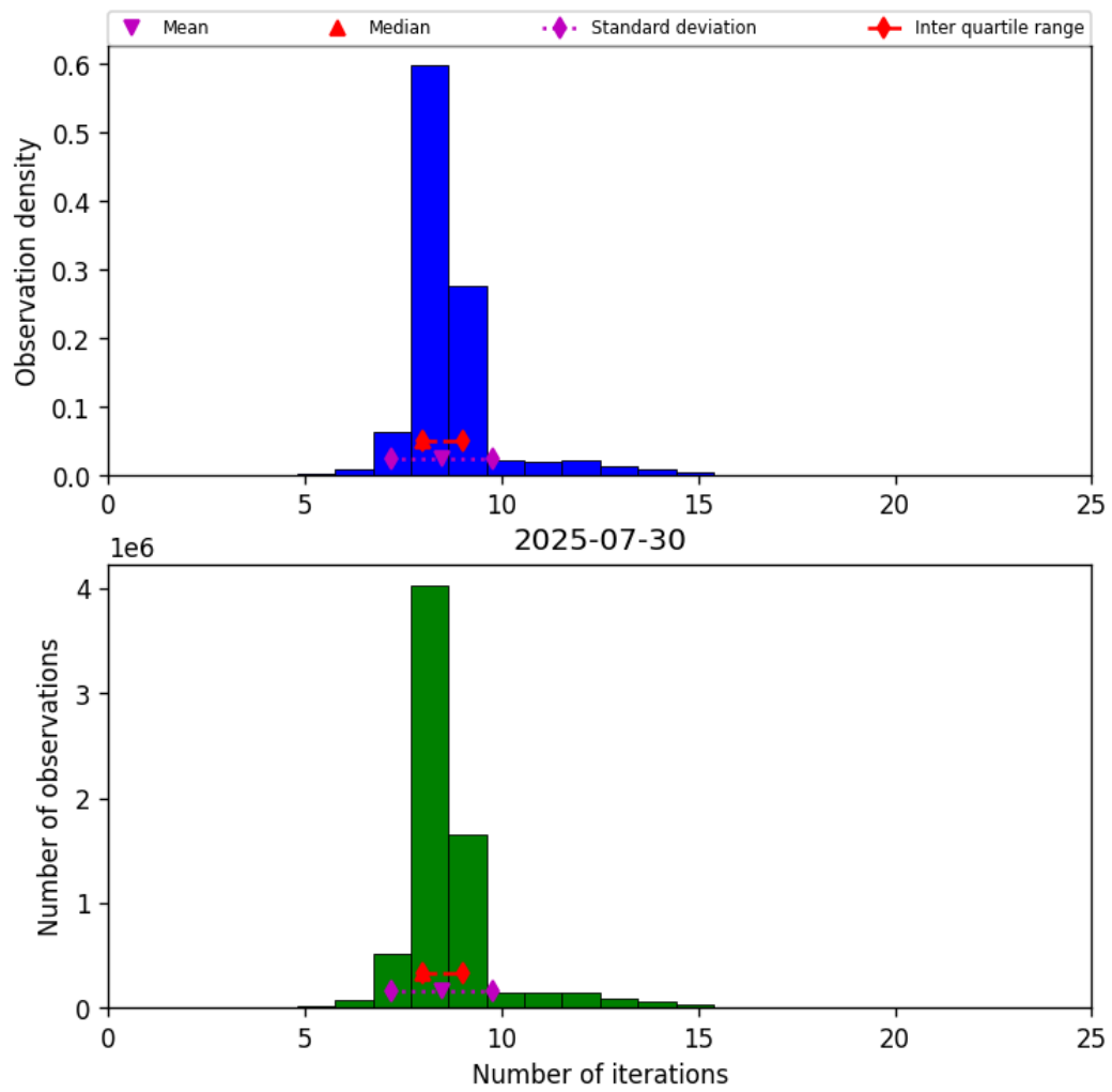
Figure 19: Histogram of “Number of iterations” for 2025-07-30 to 2025-07-31
