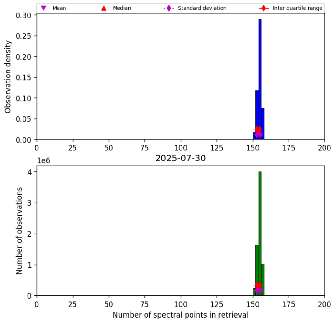
Figure 16: Histogram of “Number of spectral points in retrieval” for 2025-07-30 to 2025-07-31
