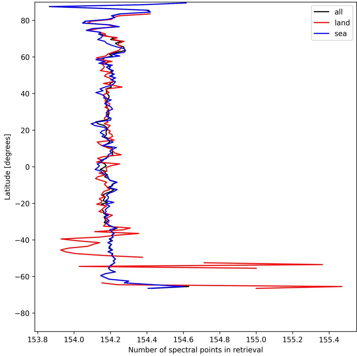
Figure 9: Zonal average of “Number of spectral points in retrieval” for 2025-07-30 to 2025-07-31.
