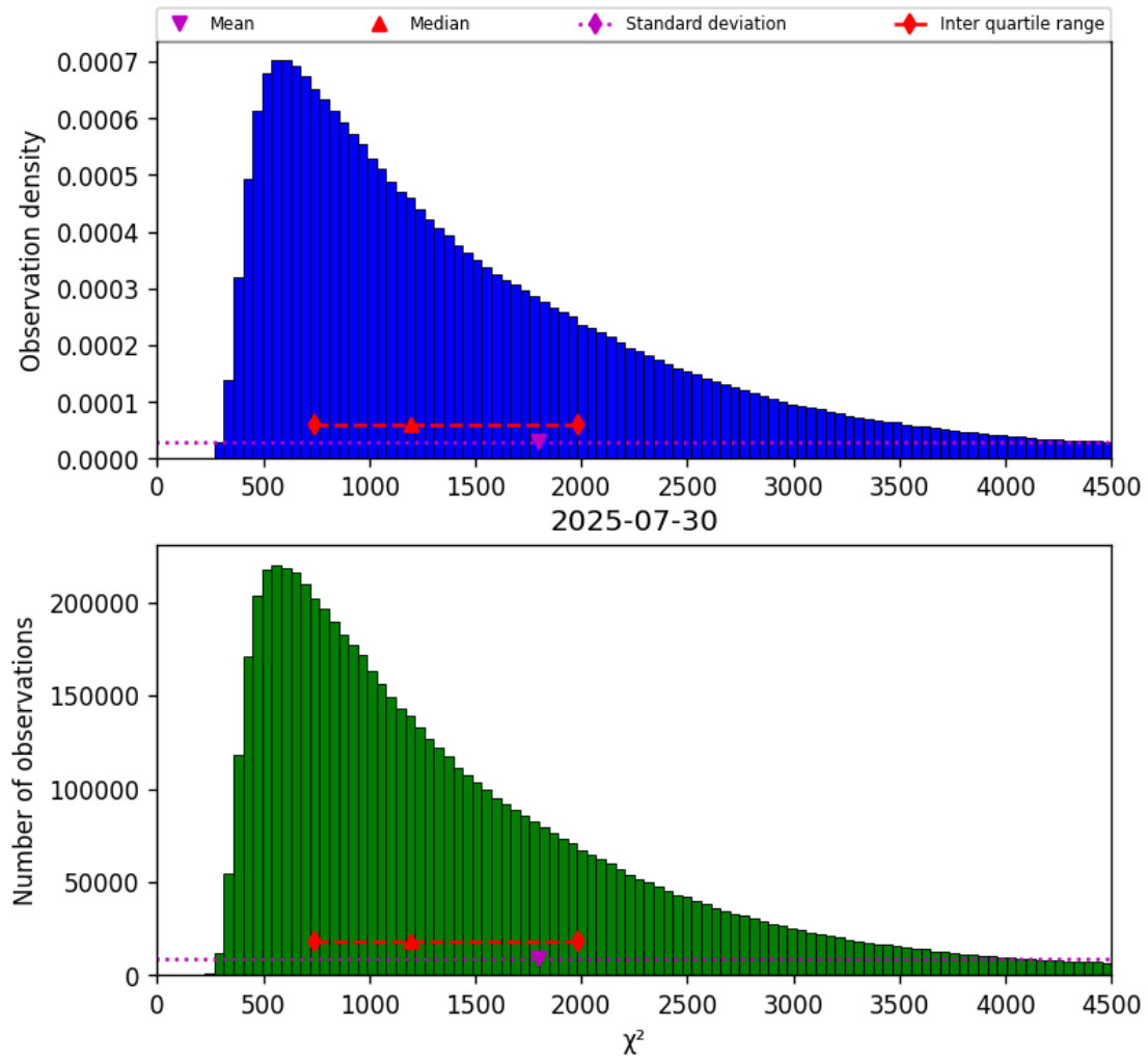
Figure 17: Histogram of “ \chi^2 ” for 2025-07-30 to 2025-07-31
