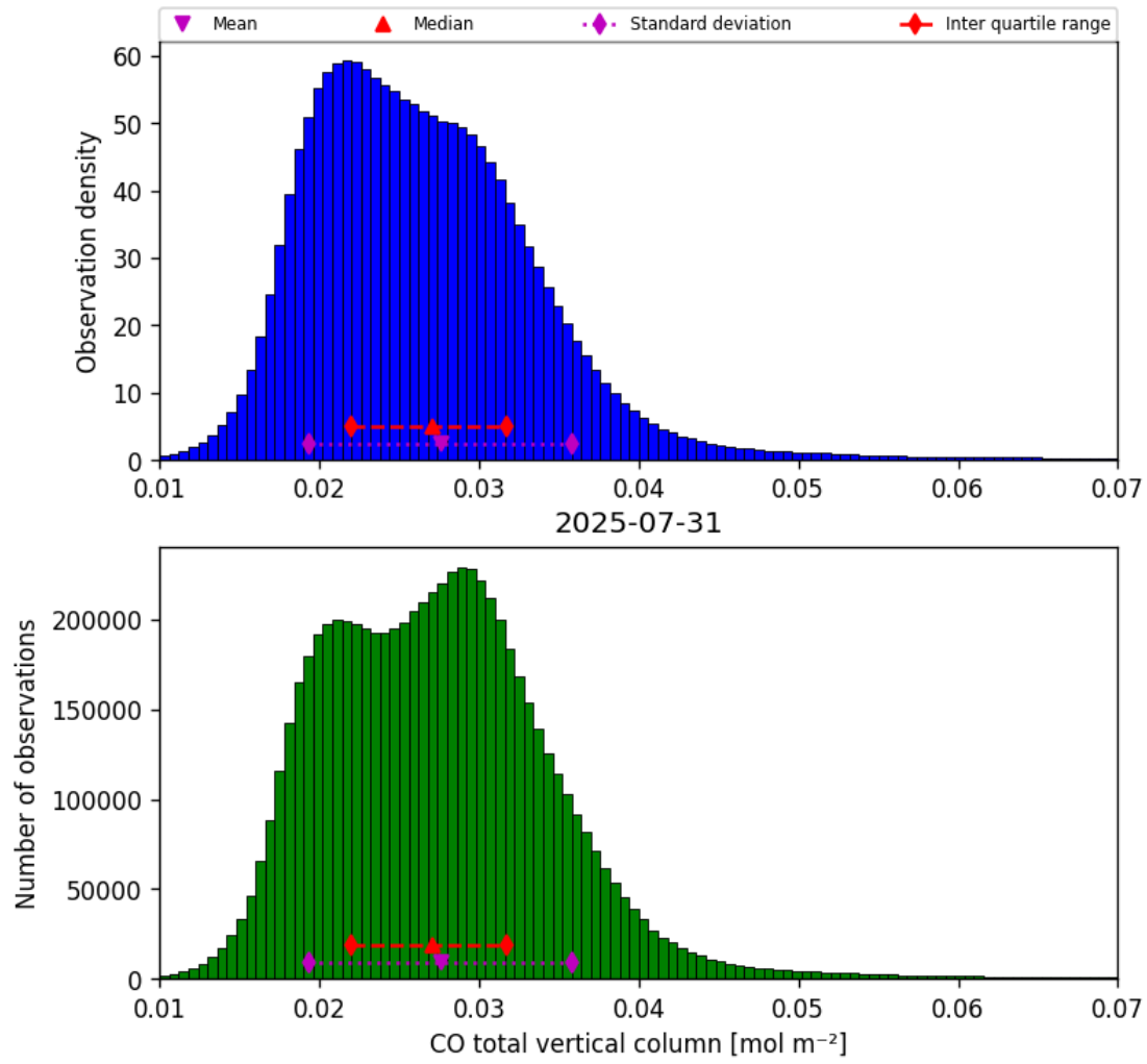
Figure 14: Histogram of “CO total vertical column” for 2025-07-31 to 2025-08-01
