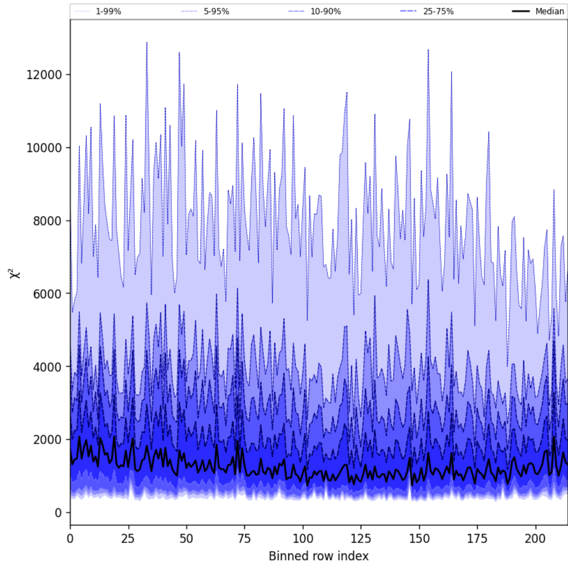
Figure 24: Along track statistics of “ \chi^2 ” for 2025-07-31 to 2025-08-01
