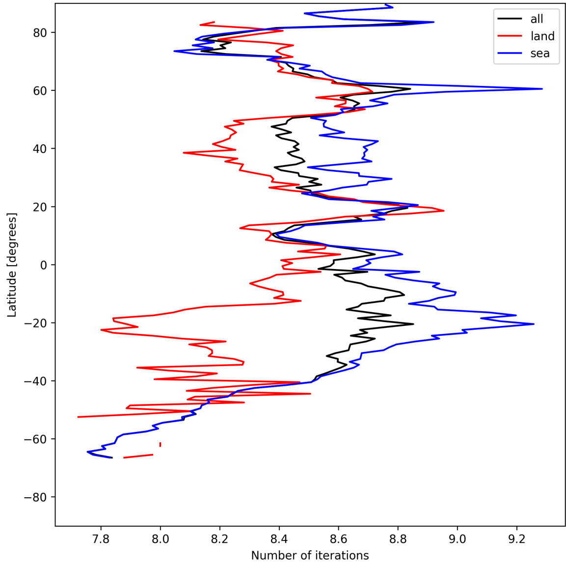
Figure 12: Zonal average of “Number of iterations” for 2025-07-31 to 2025-08-01.
