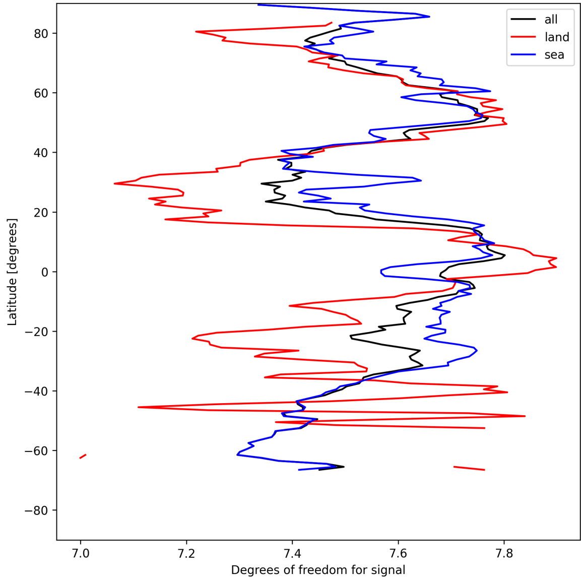
Figure 11: Zonal average of “Degrees of freedom for signal” for 2025-07-31 to 2025-08-01.
