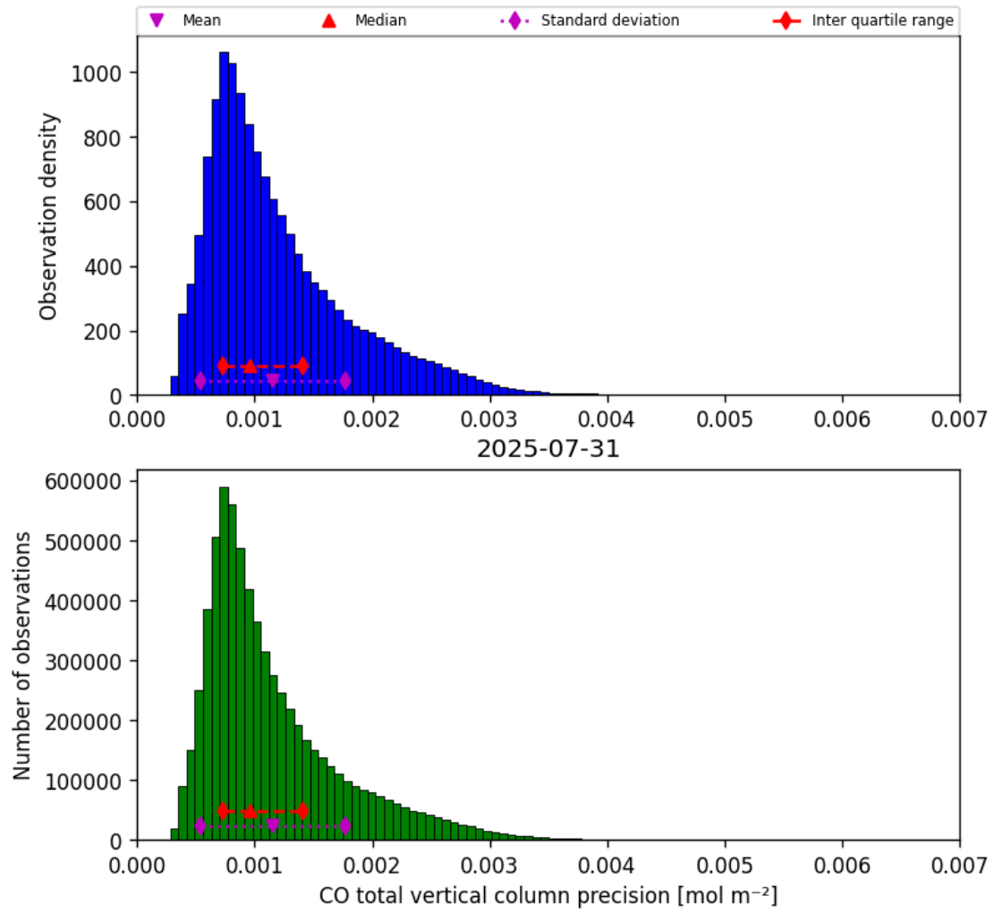
Figure 15: Histogram of “CO total vertical column precision” for 2025-07-31 to 2025-08-01
