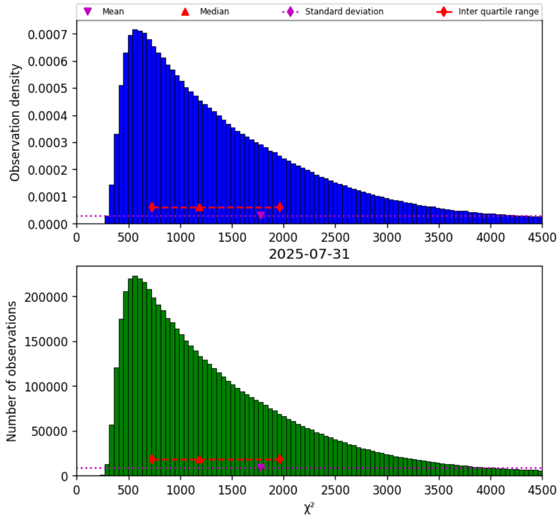
Figure 17: Histogram of " \chi^2 " for 2025-07-31 to 2025-08-01
