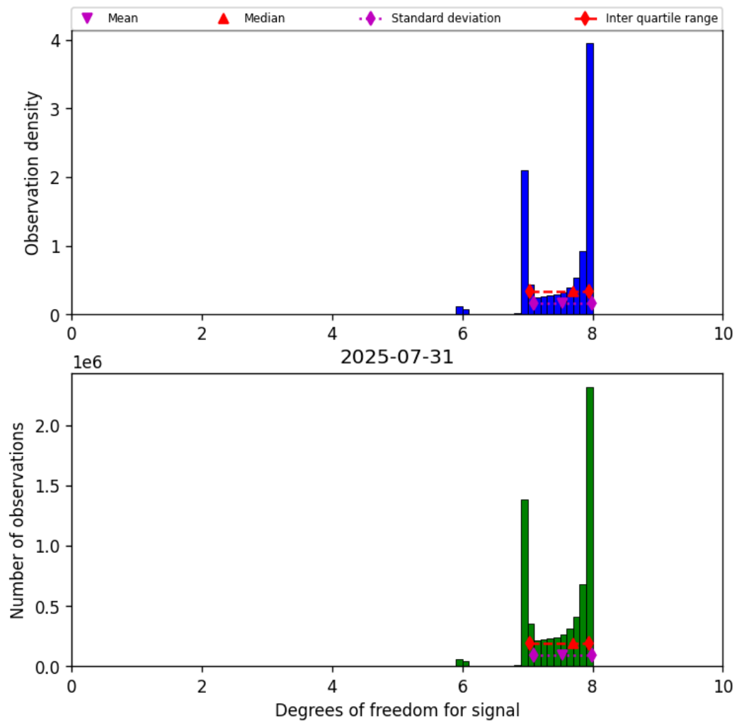
Figure 18: Histogram of “Degrees of freedom for signal” for 2025-07-31 to 2025-08-01
