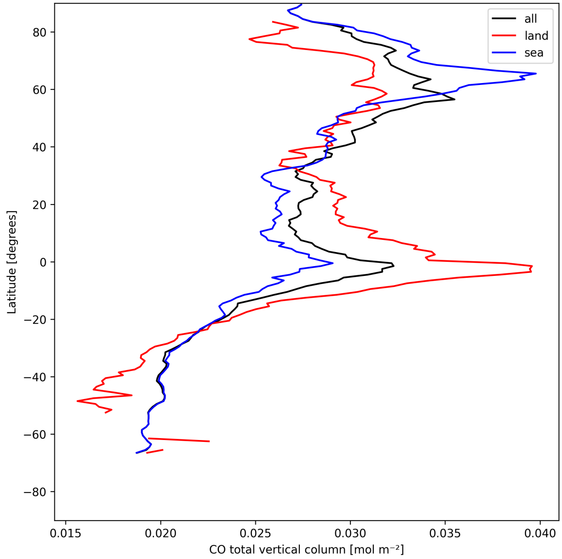
Figure 7: Zonal average of “CO total vertical column” for 2025-07-31 to 2025-08-01.
