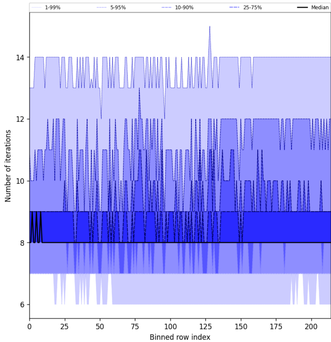
Figure 26: Along track statistics of “Number of iterations” for 2025-07-31 to 2025-08-01
