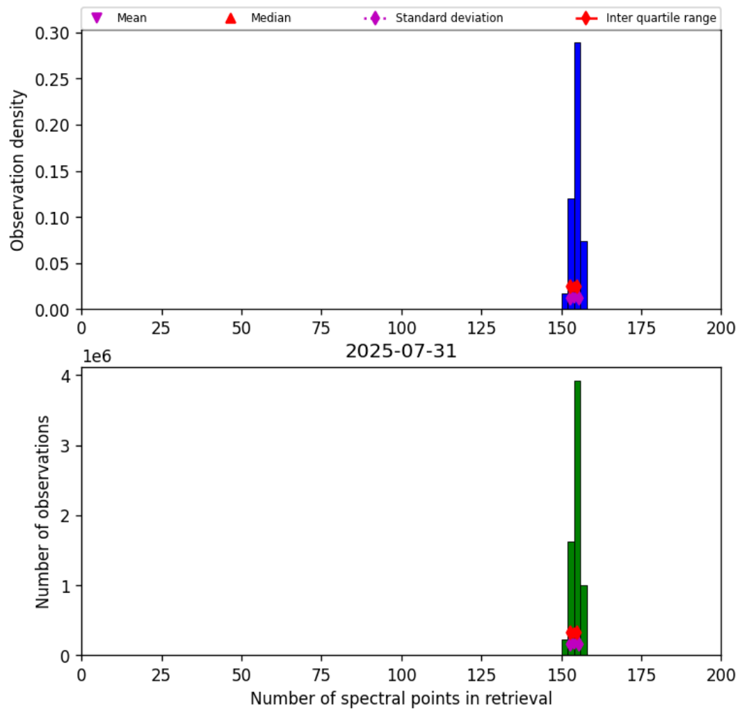
Figure 16: Histogram of “Number of spectral points in retrieval” for 2025-07-31 to 2025-08-01
