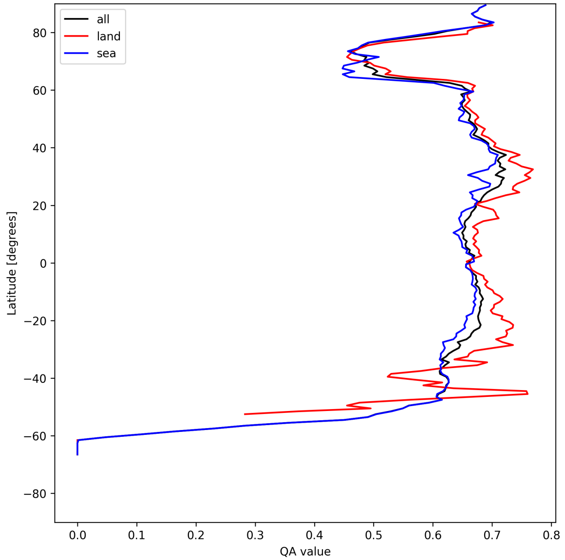
Figure 6: Zonal average of “QA value” for 2025-07-31 to 2025-08-01.
