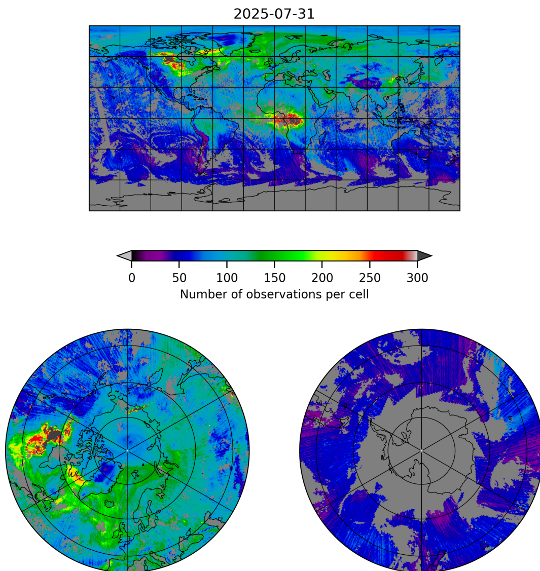
Figure 5: Map of the number of observations for 2025-07-31 to 2025-08-01
