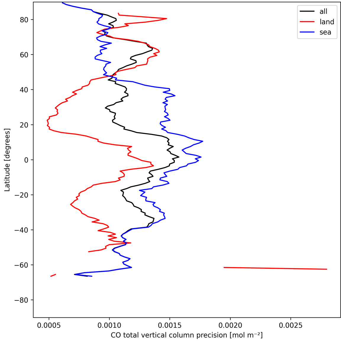
Figure 8: Zonal average of "CO total vertical column precision" for 2025-07-31 to 2025-08-01.
