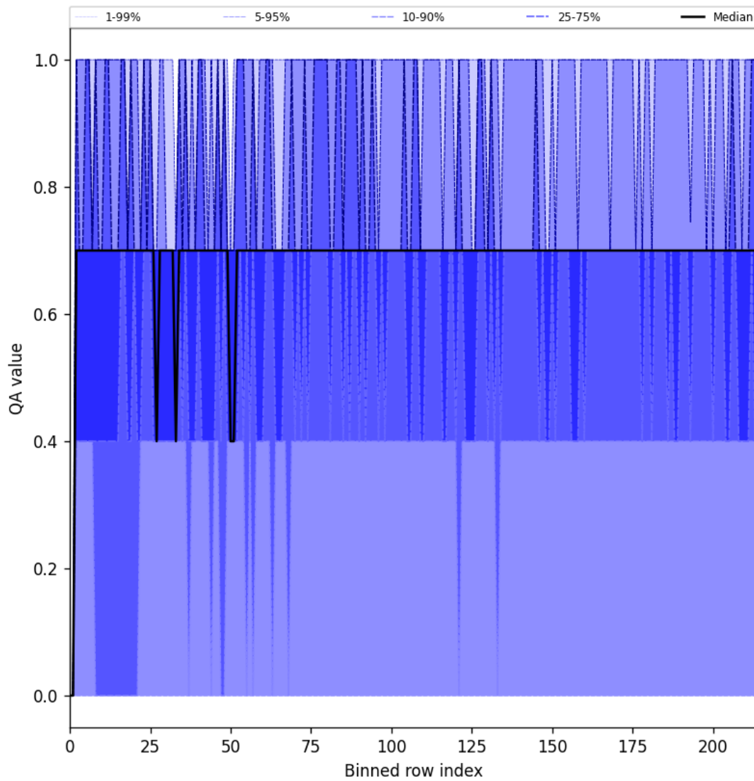
Figure 20: Along track statistics of “QA value” for 2025-07-31 to 2025-08-01
