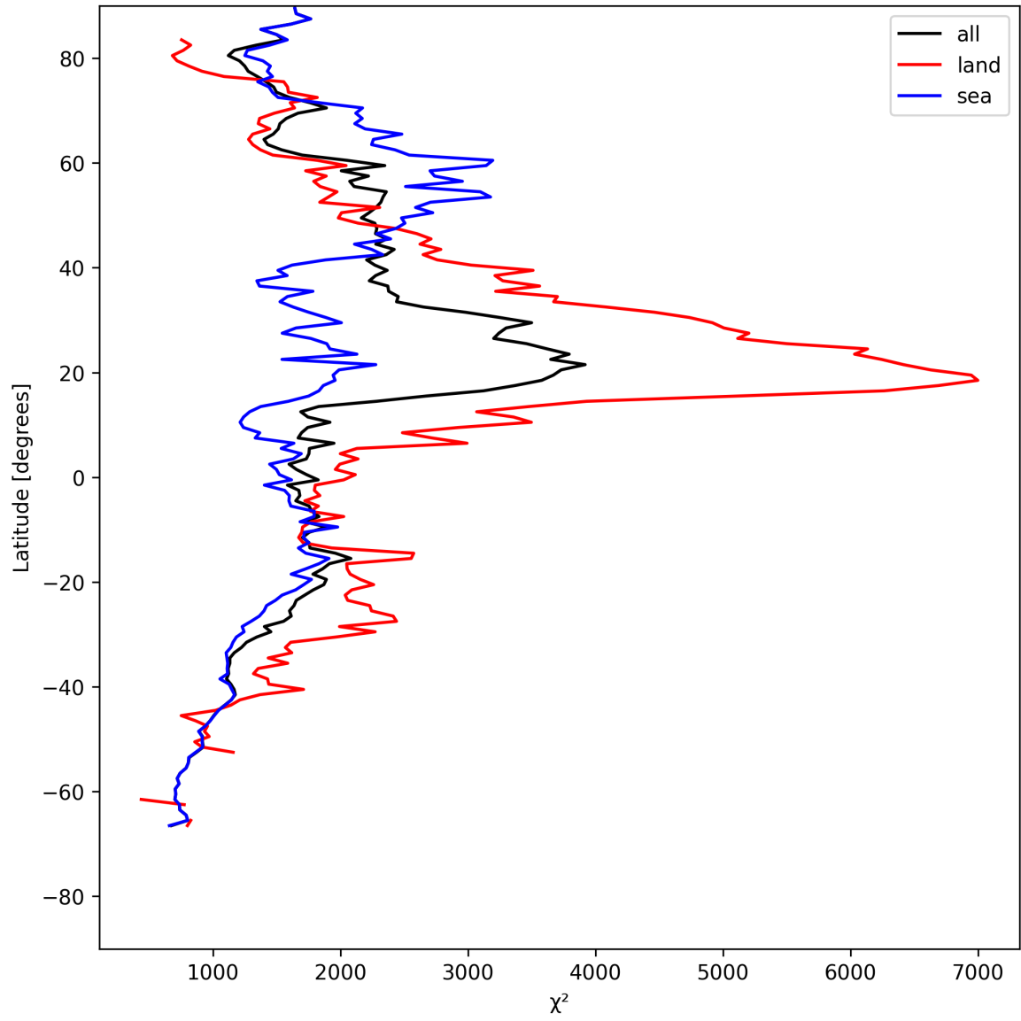
Figure 10: Zonal average of “ \chi^2 ” for 2025-07-31 to 2025-08-01.
