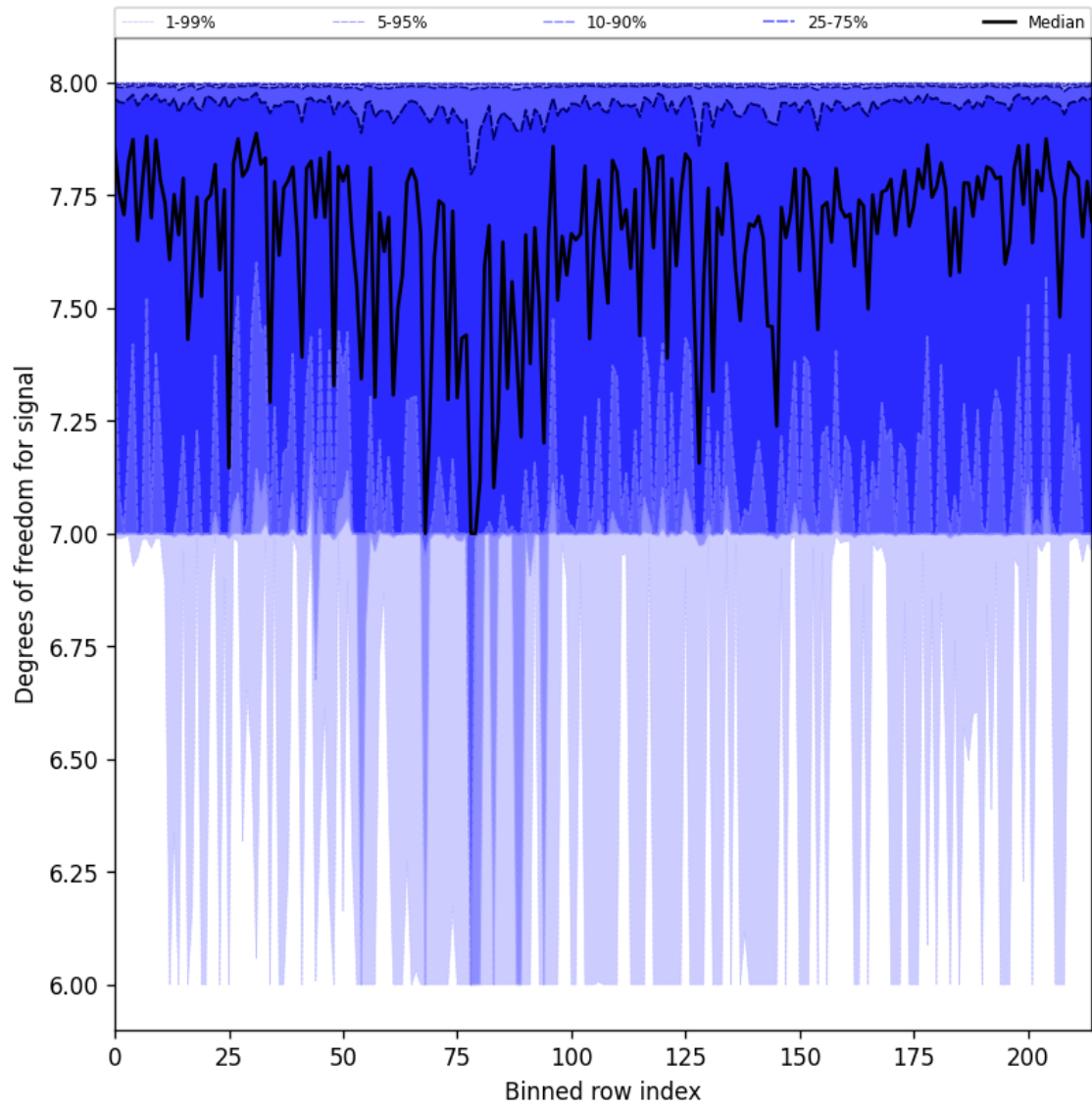
Figure 25: Along track statistics of “Degrees of freedom for signal” for 2025-07-31 to 2025-08-01
