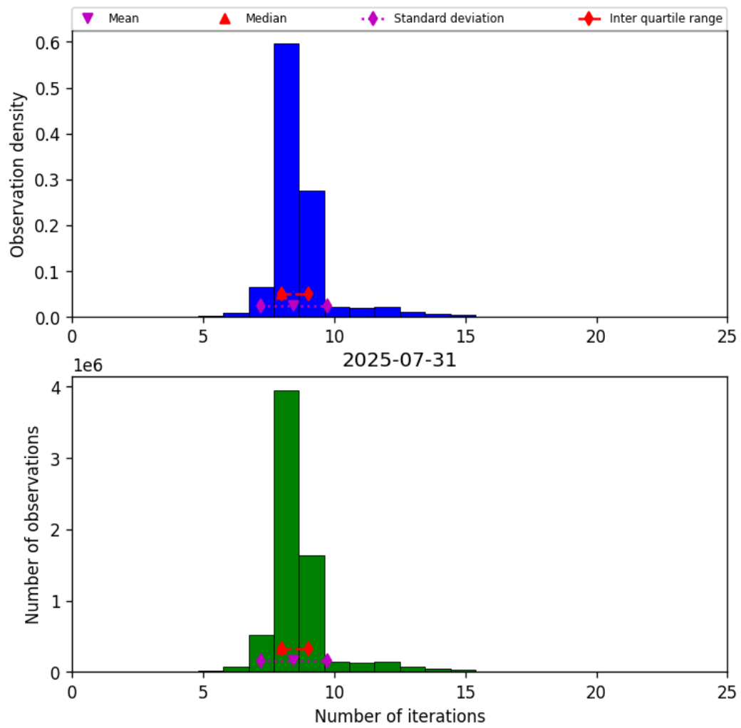
Figure 19: Histogram of “Number of iterations” for 2025-07-31 to 2025-08-01
