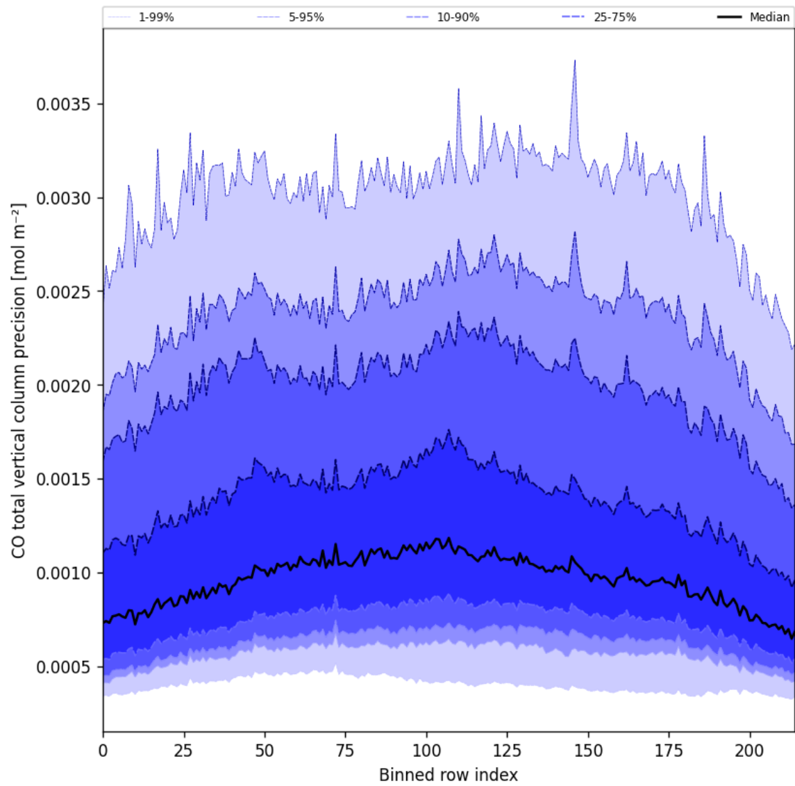
Figure 22: Along track statistics of “CO total vertical column precision” for 2025-07-31 to 2025-08-01
