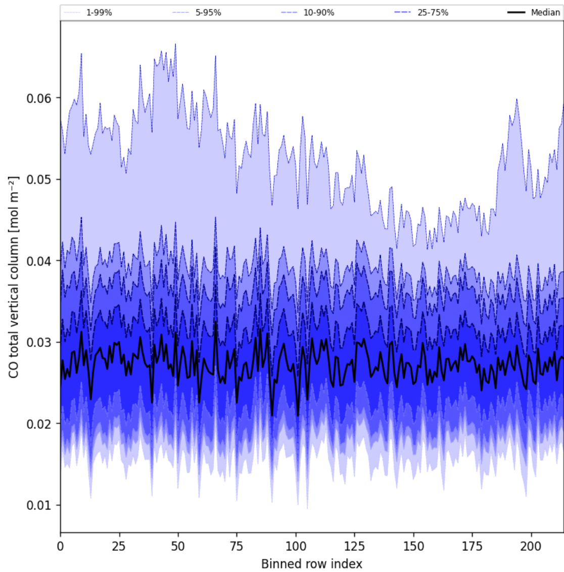
Figure 21: Along track statistics of “CO total vertical column” for 2025-07-31 to 2025-08-01
