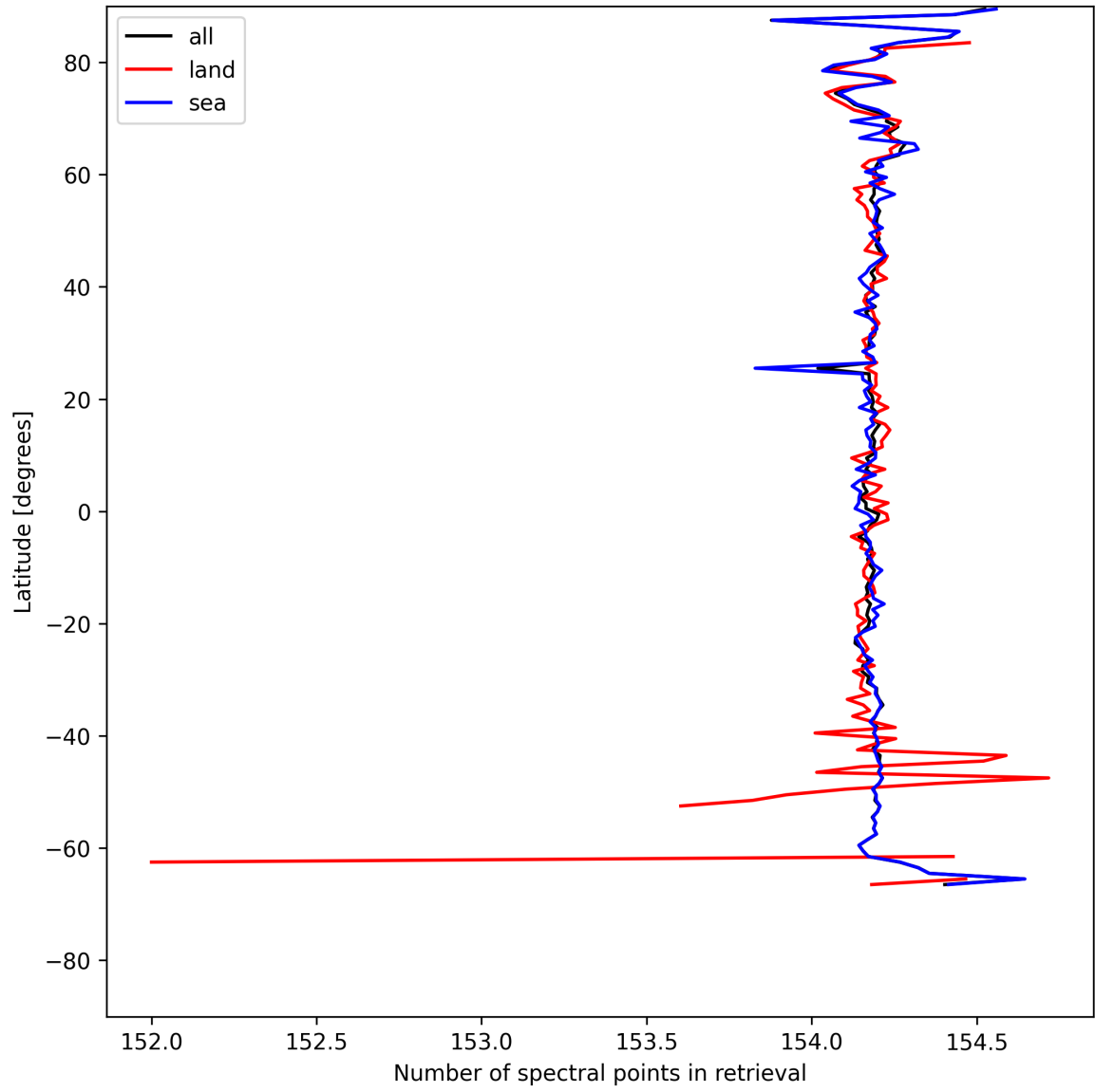
Figure 9: Zonal average of “Number of spectral points in retrieval” for 2025-07-31 to 2025-08-01.
