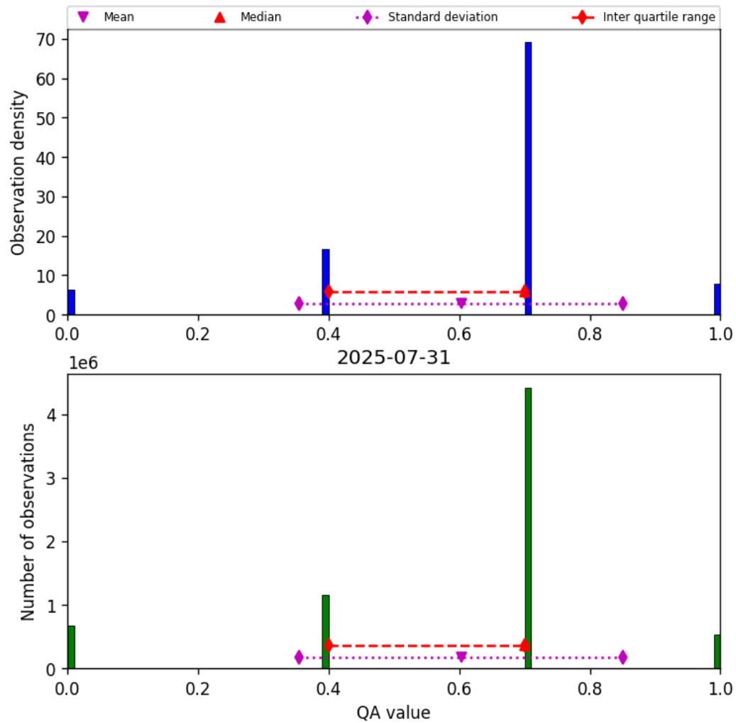
Figure 13: Histogram of “QA value” for 2025-07-31 to 2025-08-01
