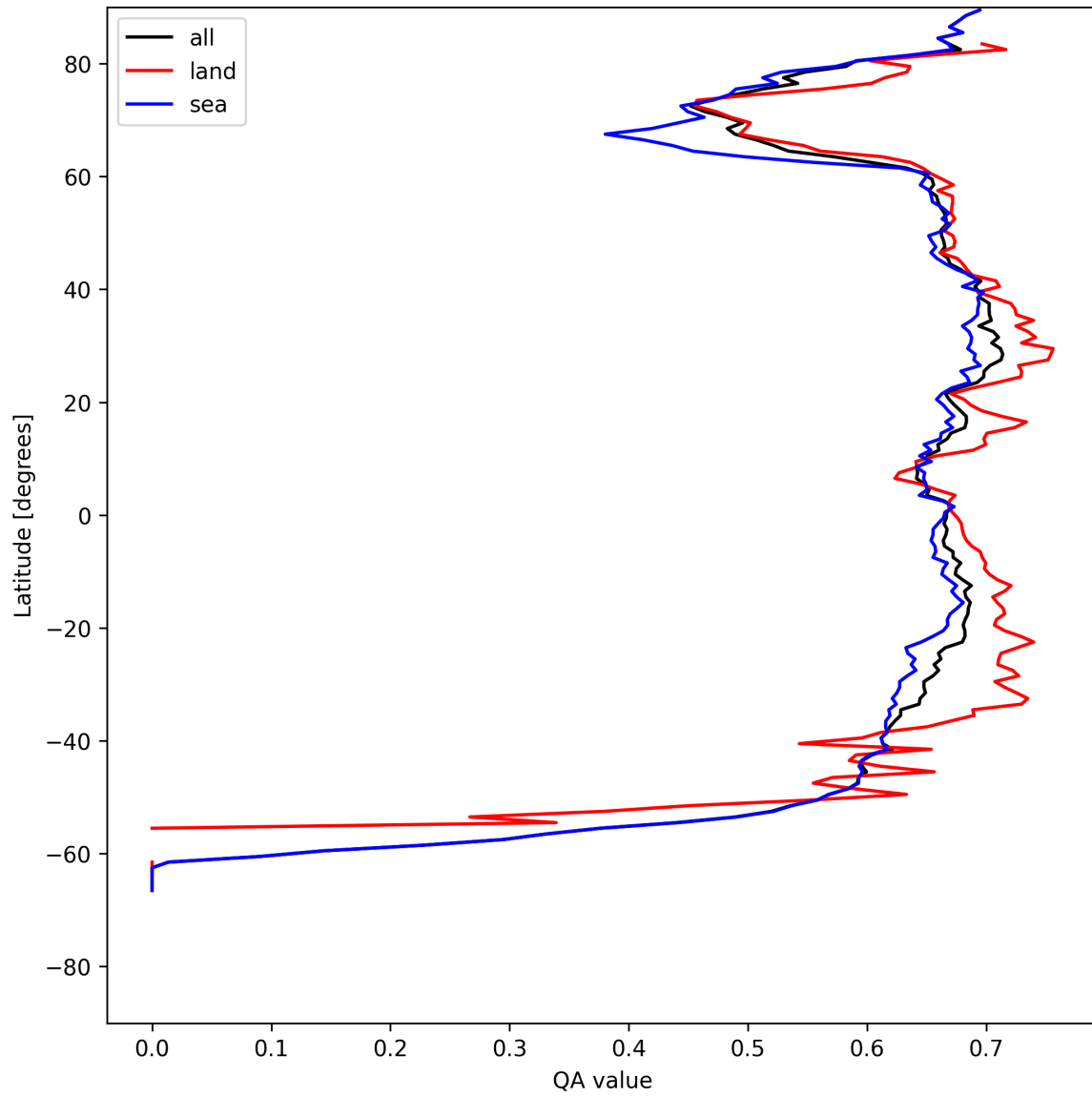
Figure 6: Zonal average of “QA value” for 2025-08-01 to 2025-08-01.
