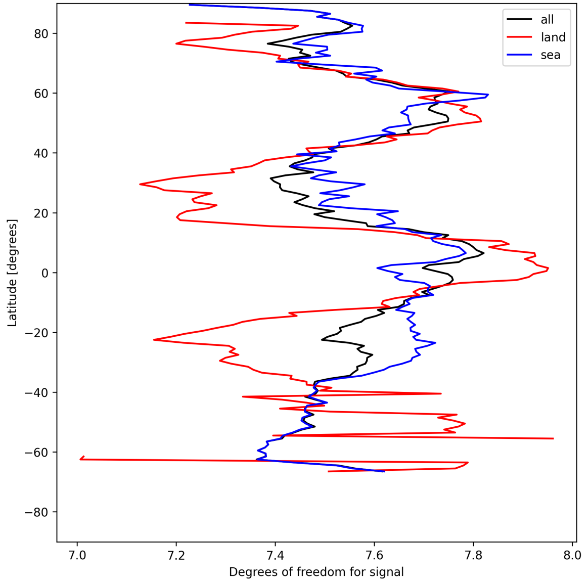
Figure 11: Zonal average of “Degrees of freedom for signal” for 2025-08-01 to 2025-08-01.
