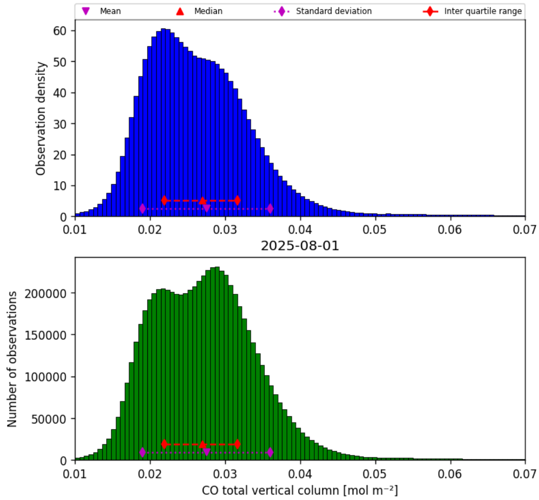
Figure 14: Histogram of “CO total vertical column” for 2025-08-01 to 2025-08-01
