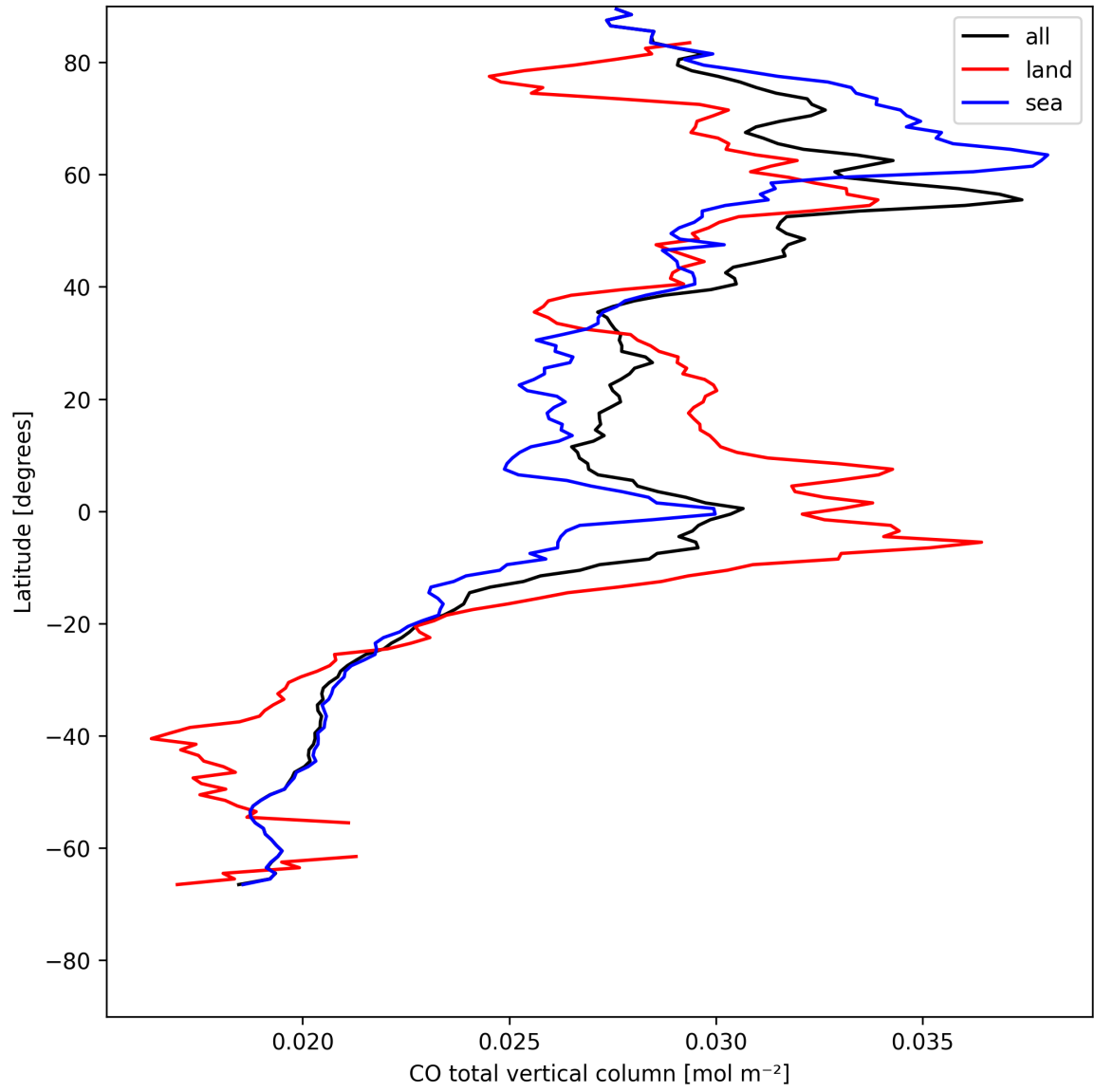
Figure 7: Zonal average of “CO total vertical column” for 2025-08-01 to 2025-08-01.
