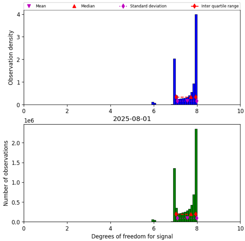
Figure 18: Histogram of “Degrees of freedom for signal” for 2025-08-01 to 2025-08-01
