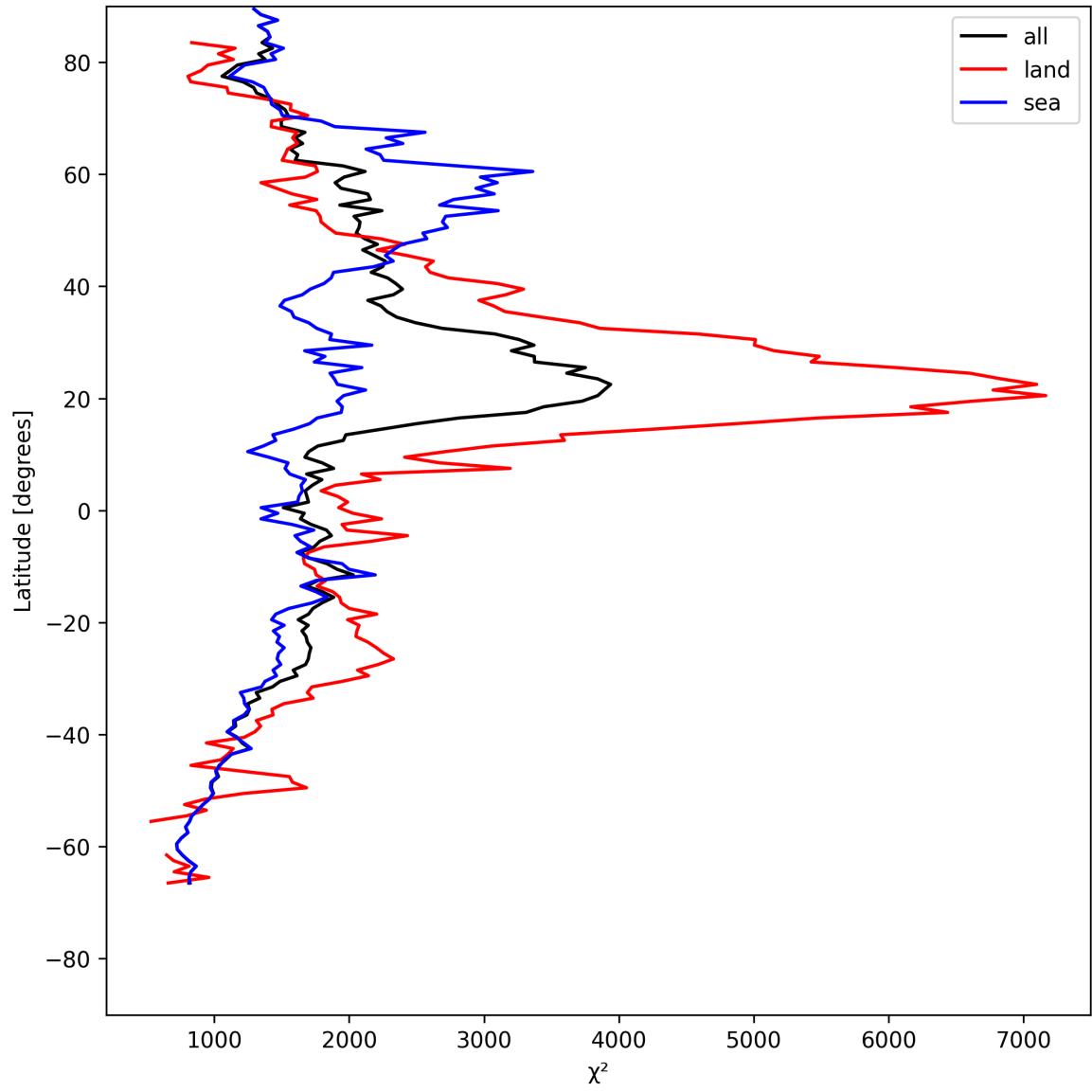
Figure 10: Zonal average of “ \chi^2 ” for 2025-08-01 to 2025-08-01.
