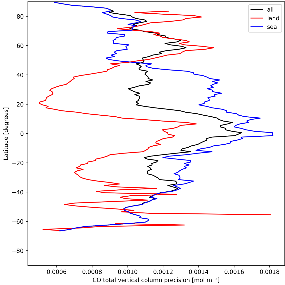
Figure 8: Zonal average of “CO total vertical column precision” for 2025-08-01 to 2025-08-01.
