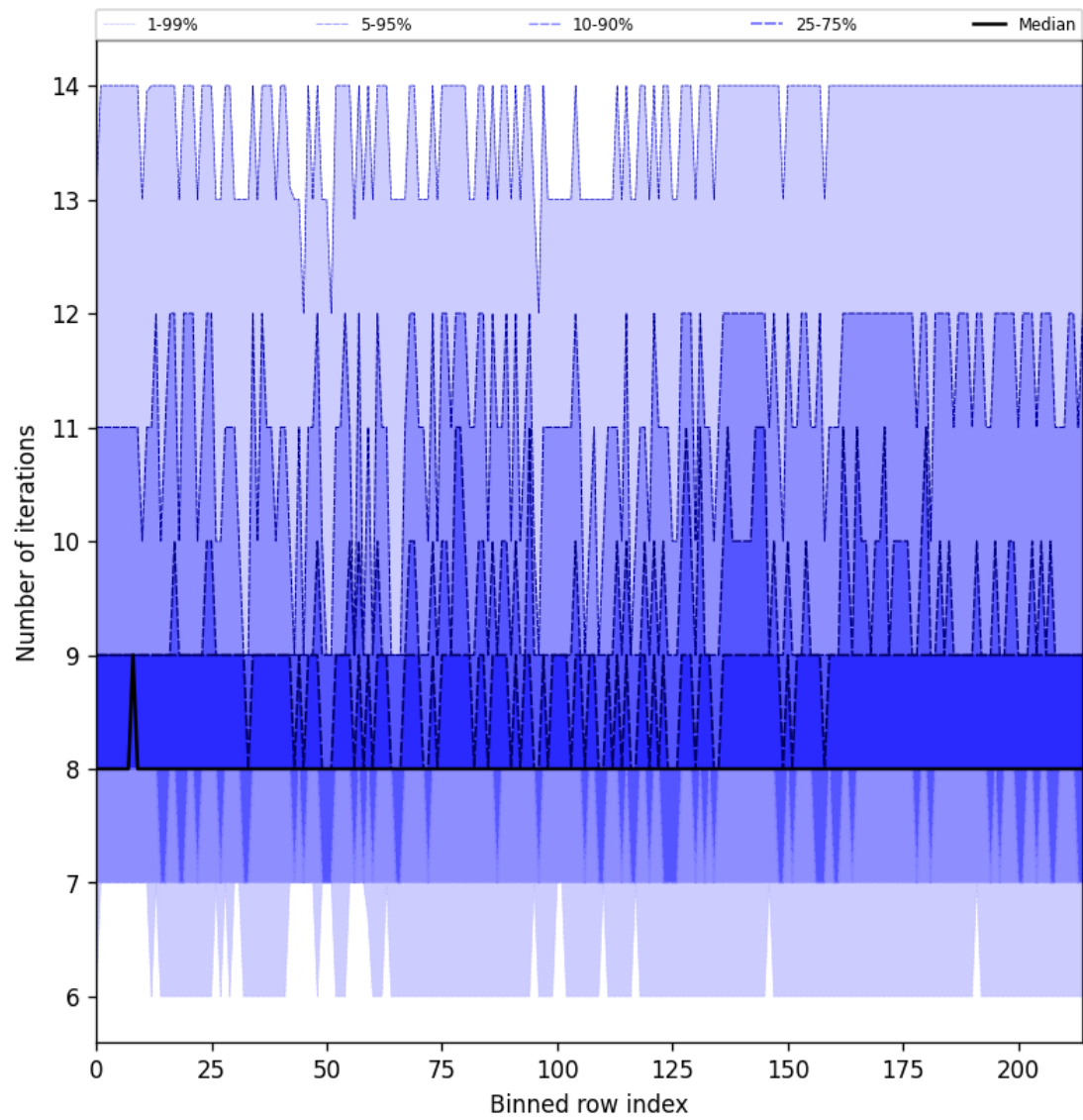
Figure 26: Along track statistics of “Number of iterations” for 2025-08-01 to 2025-08-01
