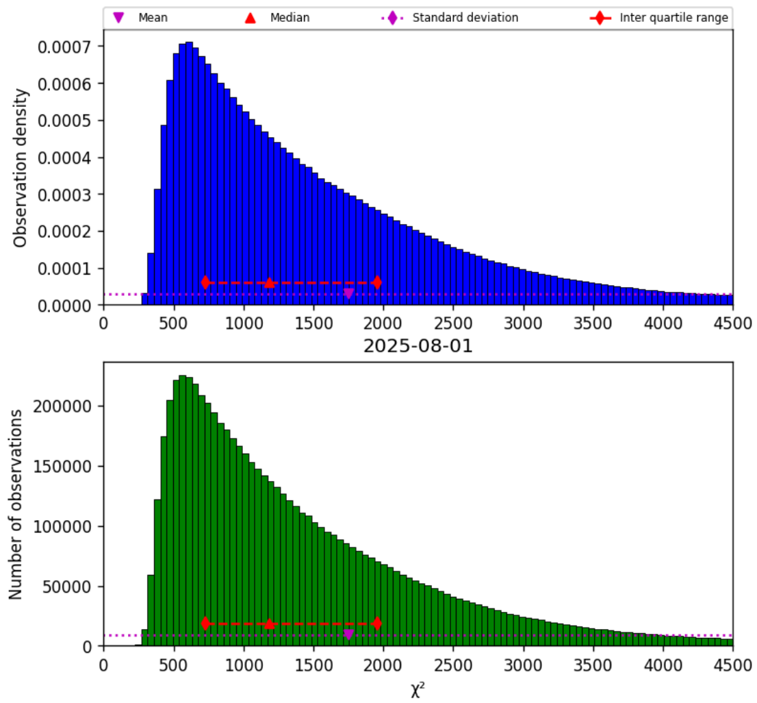
Figure 17: Histogram of " \chi^2 " for 2025-08-01 to 2025-08-01
