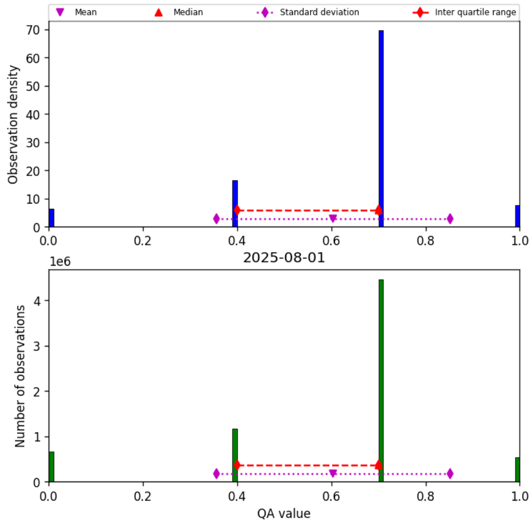
Figure 13: Histogram of “QA value” for 2025-08-01 to 2025-08-01
