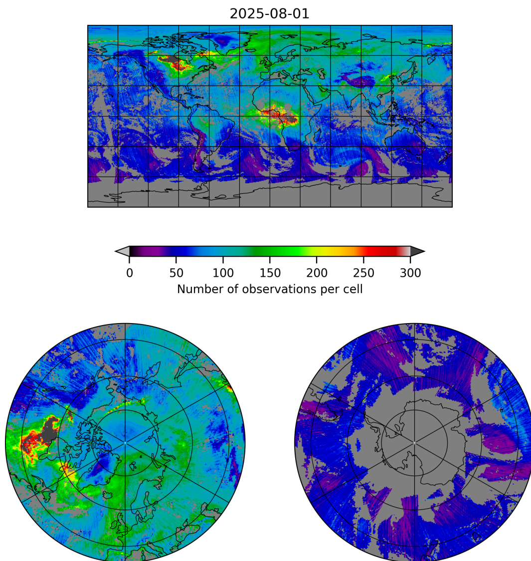
Figure 5: Map of the number of observations for 2025-08-01 to 2025-08-01
