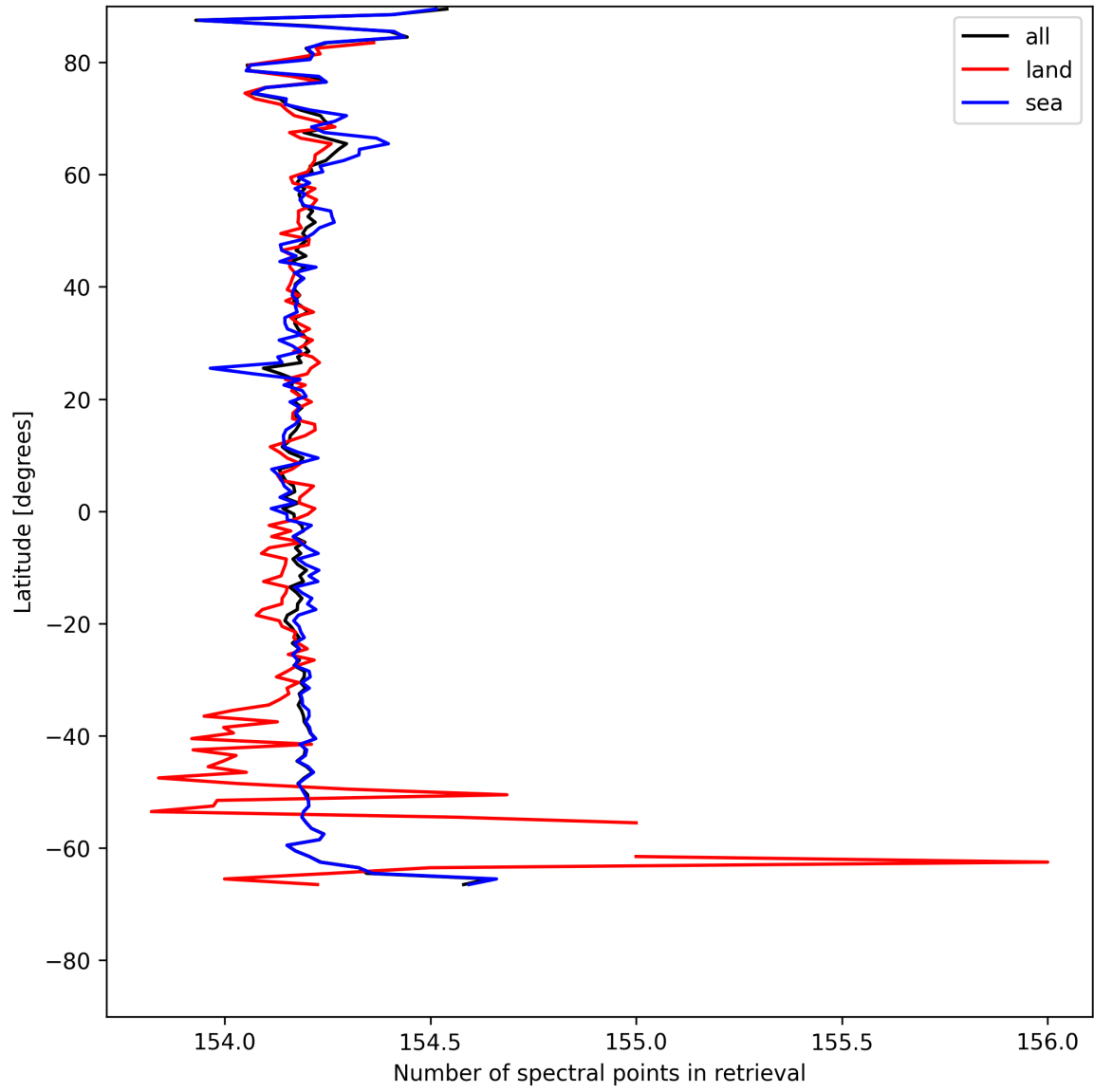
Figure 9: Zonal average of “Number of spectral points in retrieval” for 2025-08-01 to 2025-08-01.
