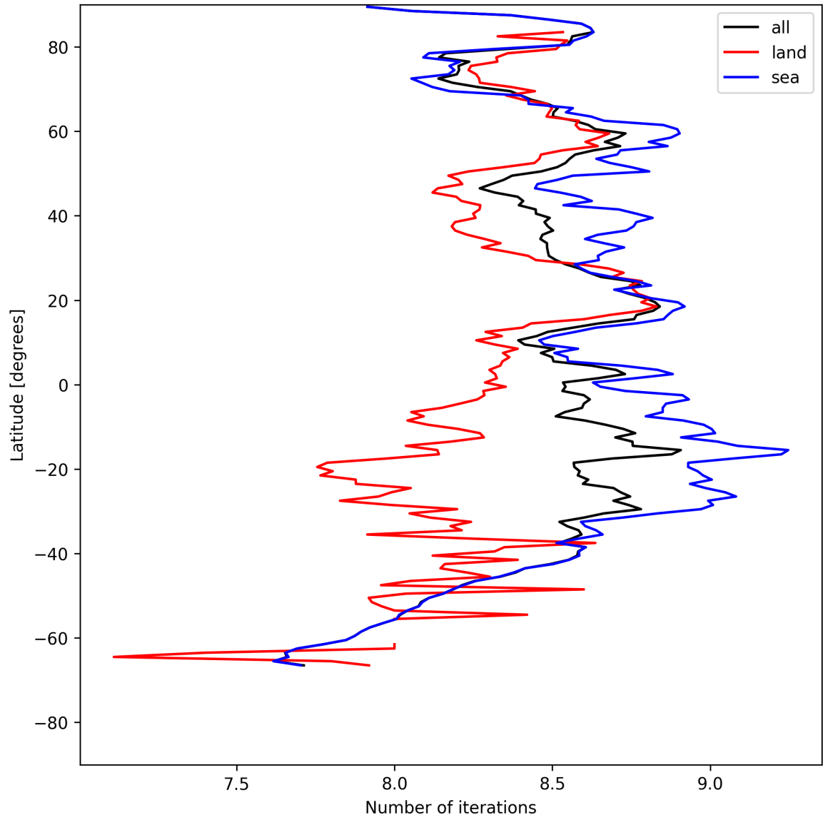
Figure 12: Zonal average of “Number of iterations” for 2025-08-01 to 2025-08-01.
