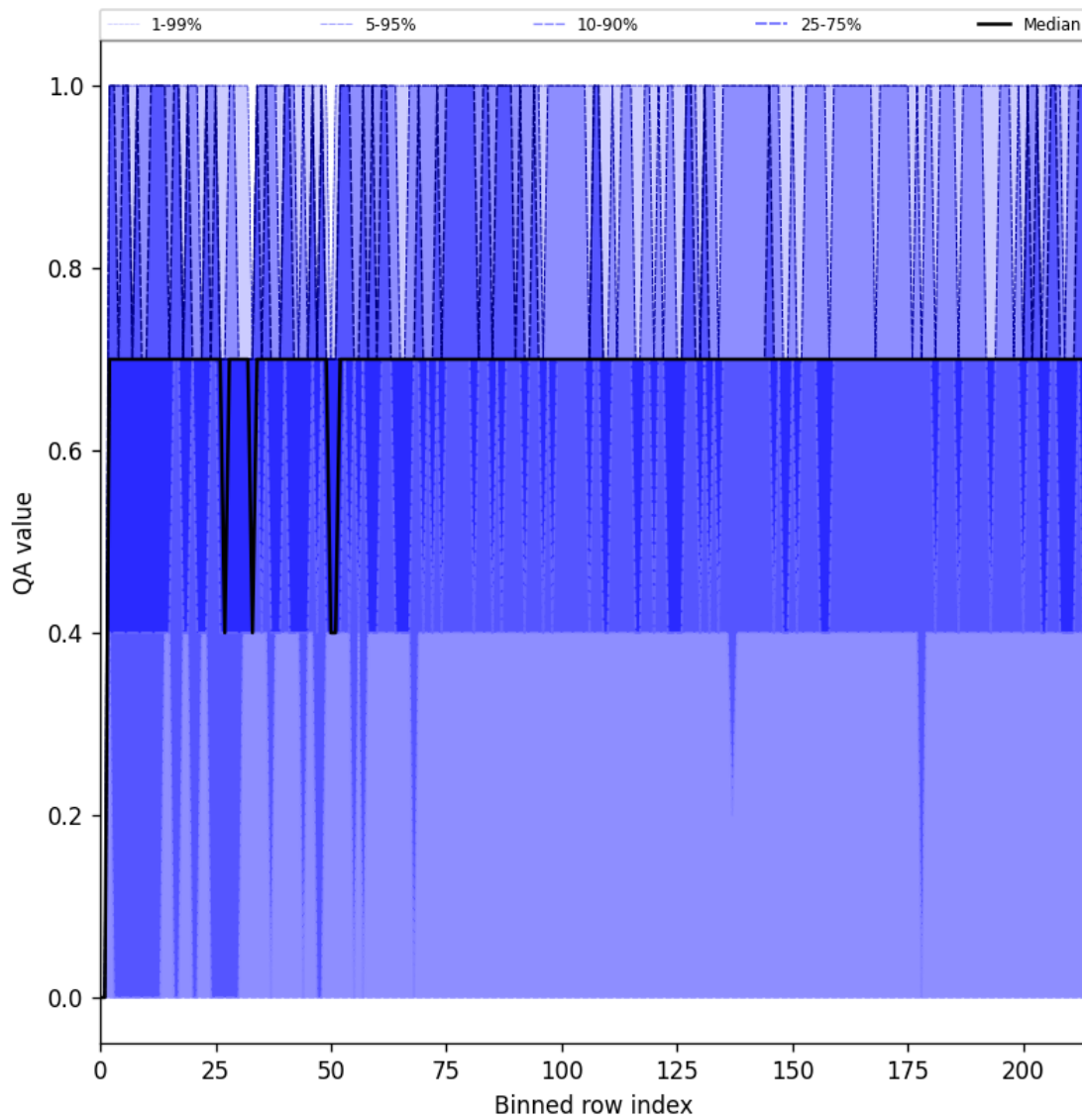
Figure 20: Along track statistics of “QA value” for 2025-08-01 to 2025-08-01
