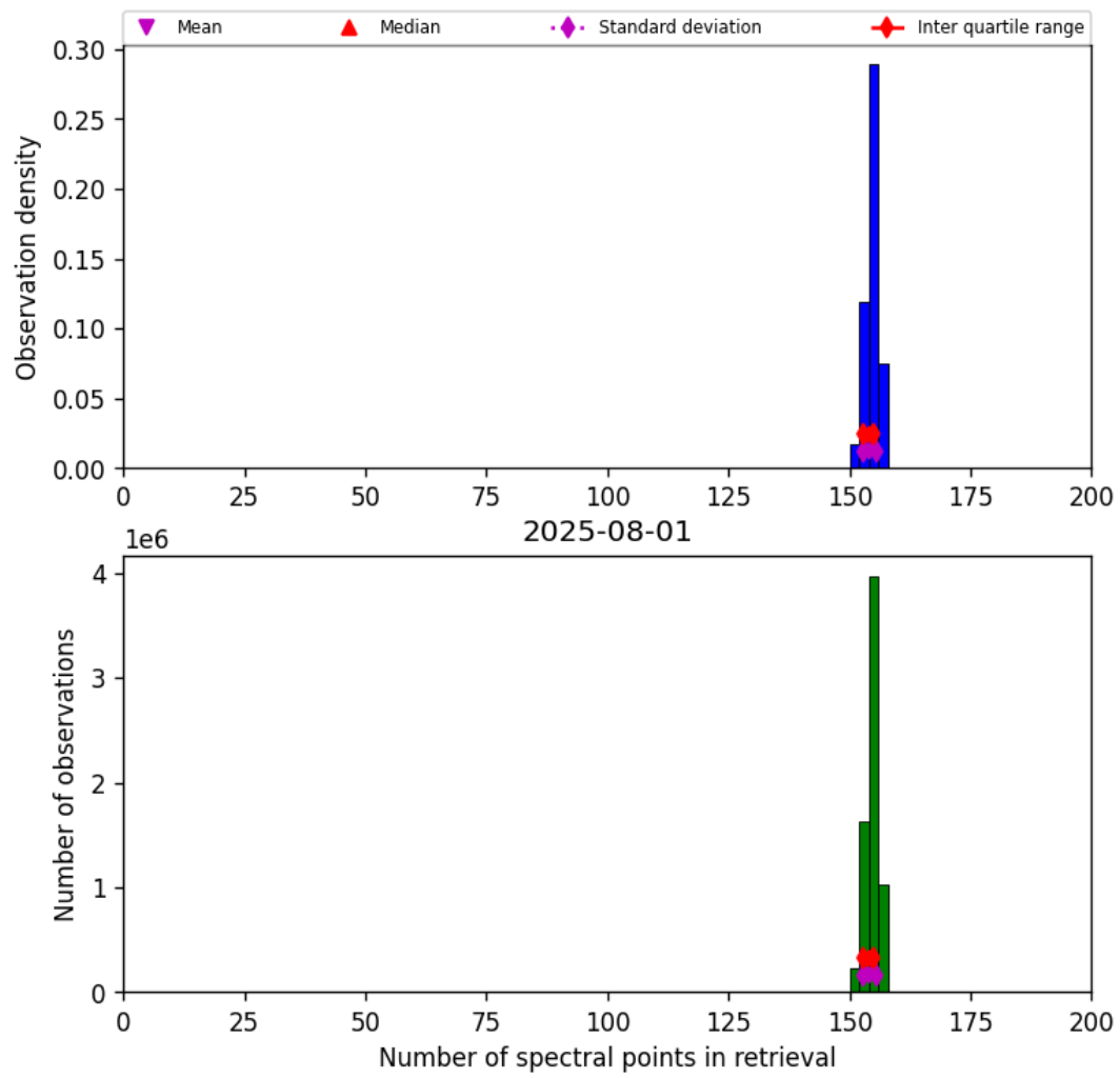
Figure 16: Histogram of “Number of spectral points in retrieval” for 2025-08-01 to 2025-08-01
