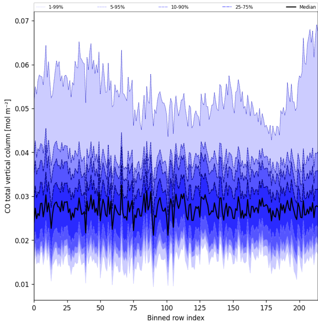
Figure 21: Along track statistics of “CO total vertical column” for 2025-08-01 to 2025-08-01
