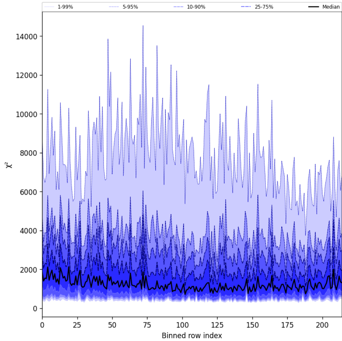
Figure 24: Along track statistics of “ \chi^2 ” for 2025-08-01 to 2025-08-01
