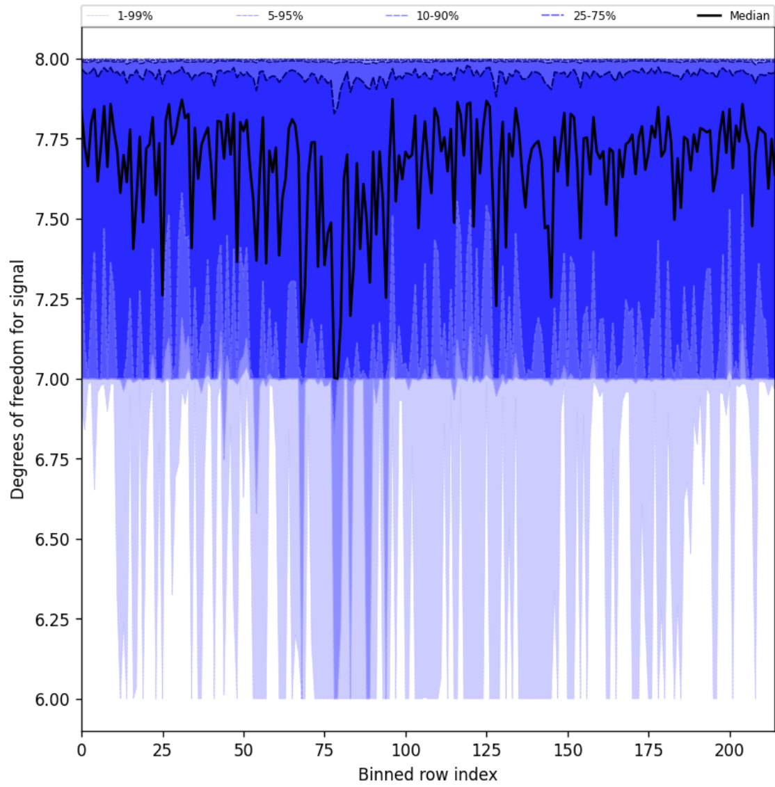
Figure 25: Along track statistics of “Degrees of freedom for signal” for 2025-08-01 to 2025-08-01
