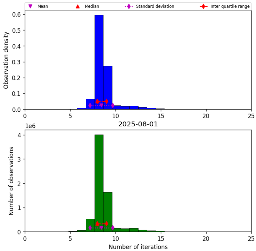
Figure 19: Histogram of “Number of iterations” for 2025-08-01 to 2025-08-01
