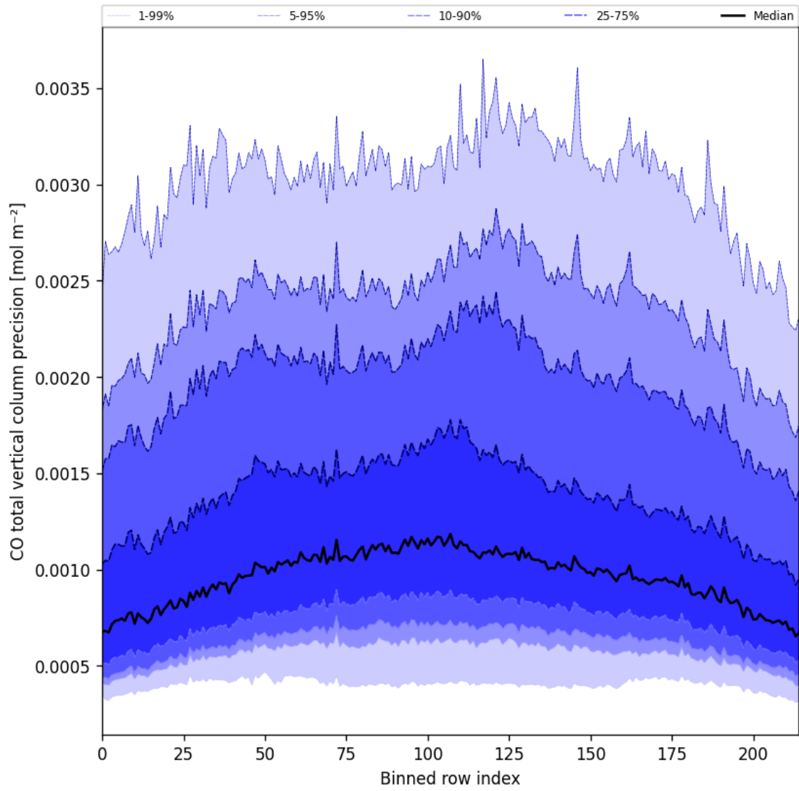
Figure 22: Along track statistics of “CO total vertical column precision” for 2025-08-01 to 2025-08-01
