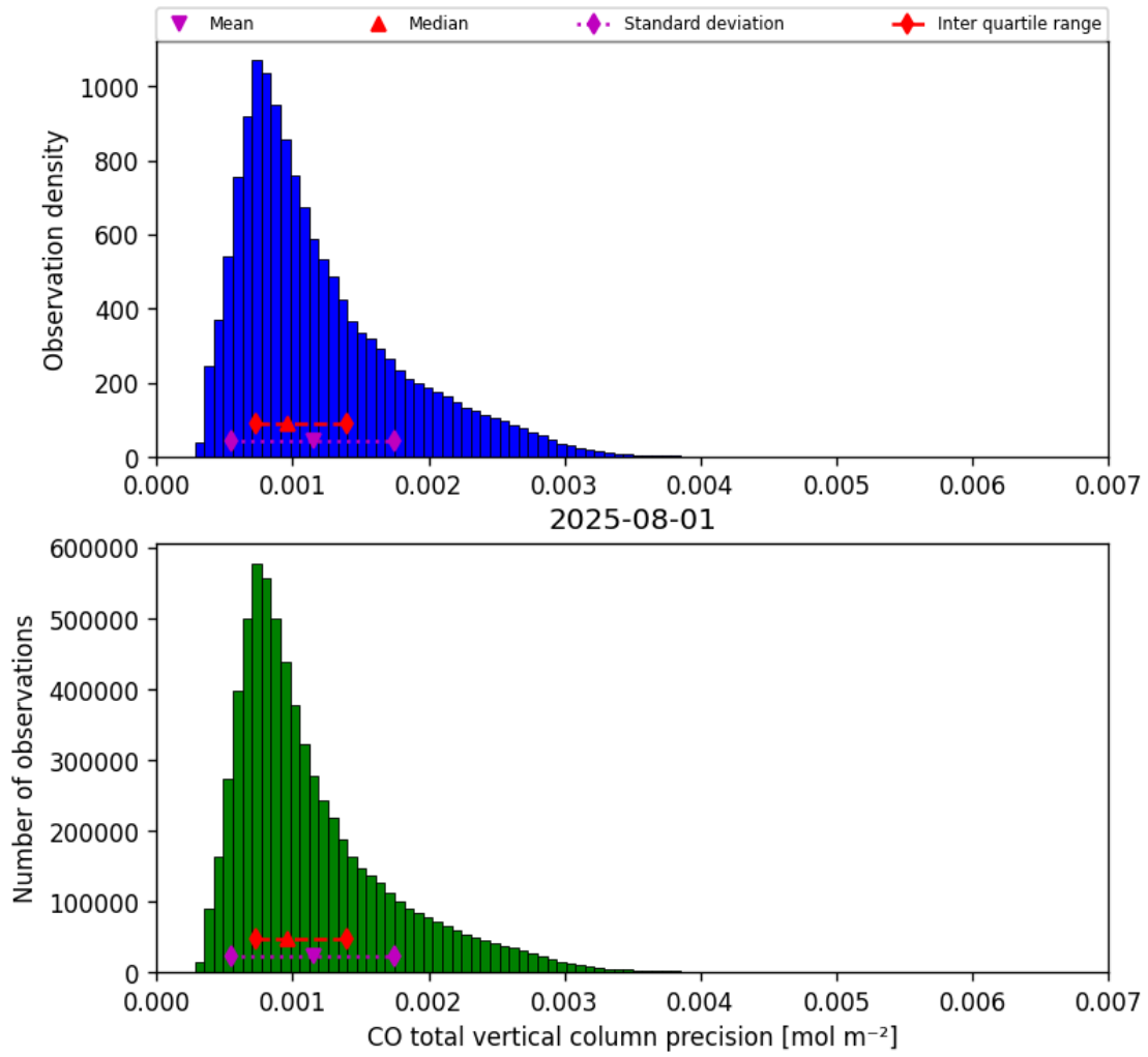
Figure 15: Histogram of “CO total vertical column precision” for 2025-08-01 to 2025-08-01
