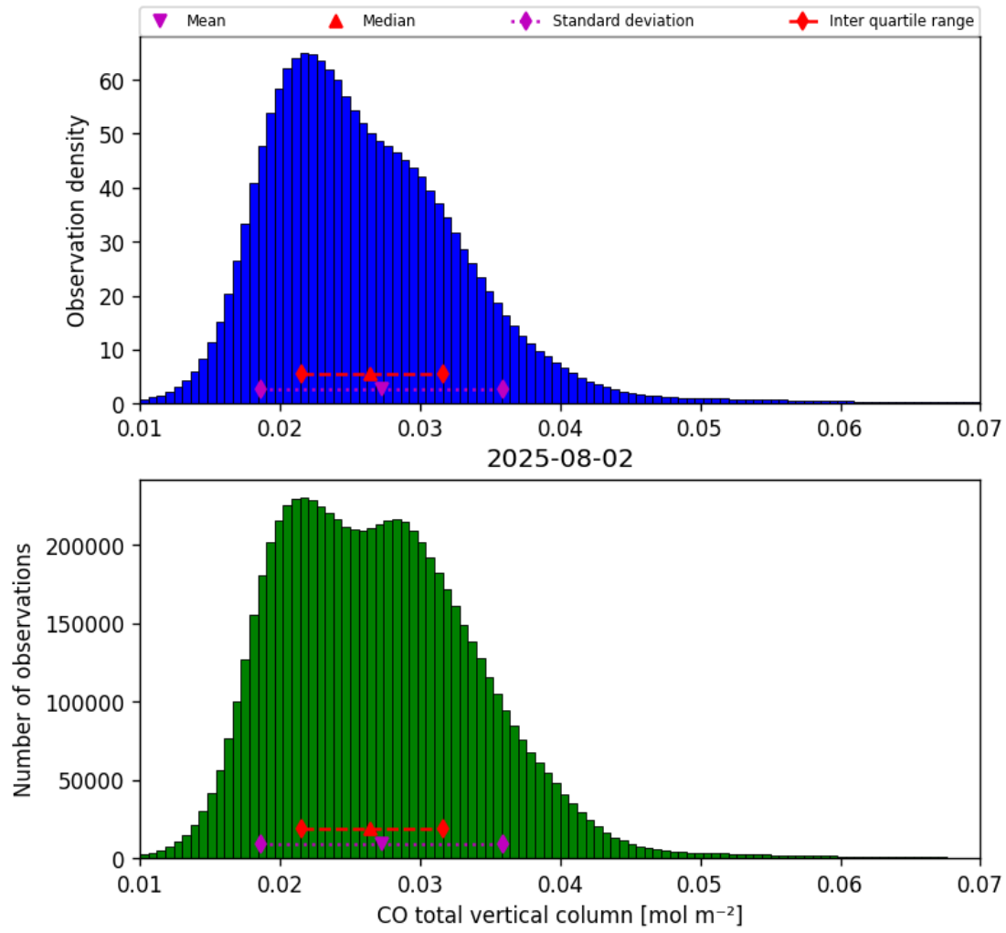
Figure 14: Histogram of “CO total vertical column” for 2025-08-02 to 2025-08-03
