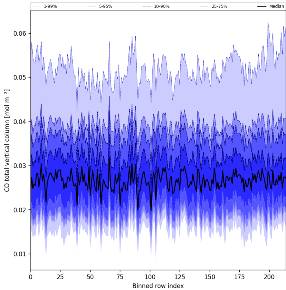
Figure 21: Along track statistics of “CO total vertical column” for 2025-08-02 to 2025-08-03
