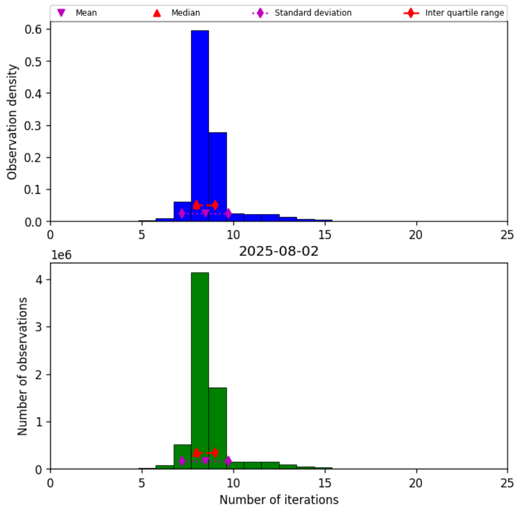
Figure 19: Histogram of “Number of iterations” for 2025-08-02 to 2025-08-03
