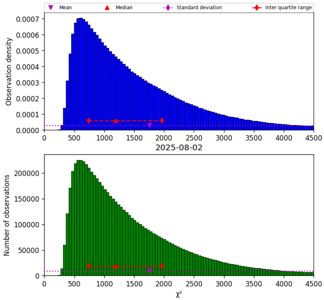
Figure 17: Histogram of " \chi^2 " for 2025-08-02 to 2025-08-03
