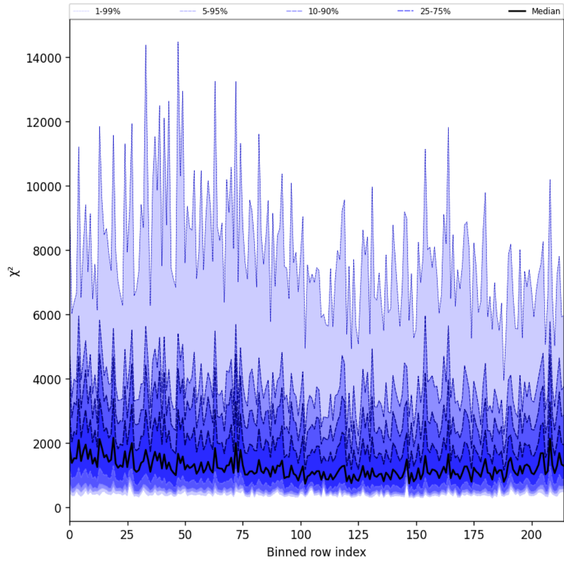
Figure 24: Along track statistics of “ \chi^2 ” for 2025-08-02 to 2025-08-03
