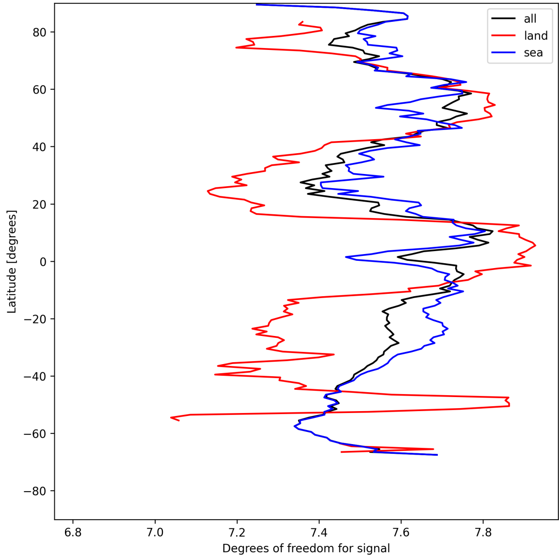
Figure 11: Zonal average of “Degrees of freedom for signal” for 2025-08-02 to 2025-08-03.
