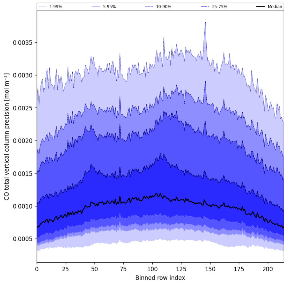
Figure 22: Along track statistics of “CO total vertical column precision” for 2025-08-02 to 2025-08-03
