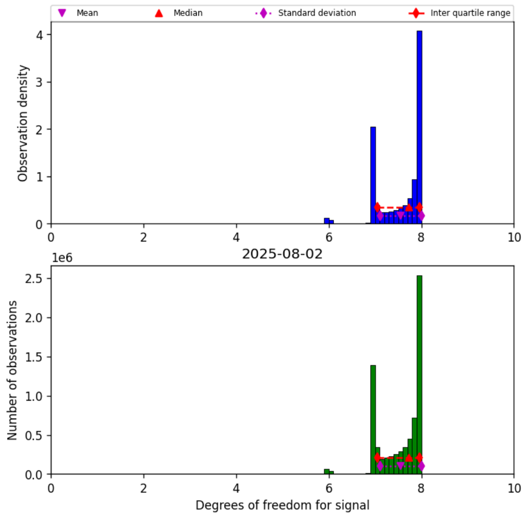
Figure 18: Histogram of “Degrees of freedom for signal” for 2025-08-02 to 2025-08-03
