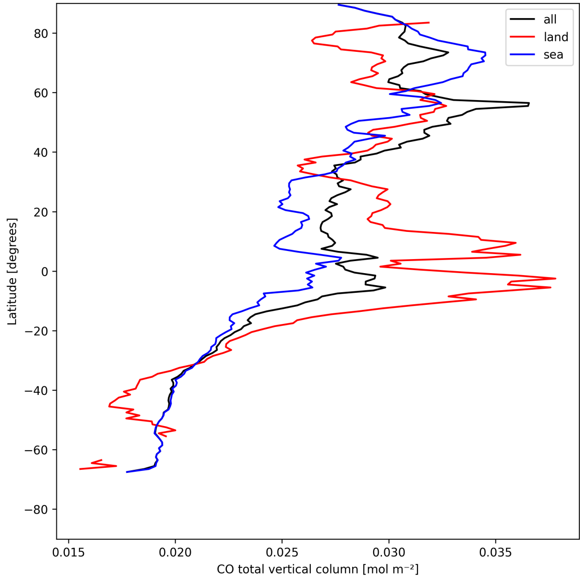
Figure 7: Zonal average of “CO total vertical column” for 2025-08-02 to 2025-08-03.
