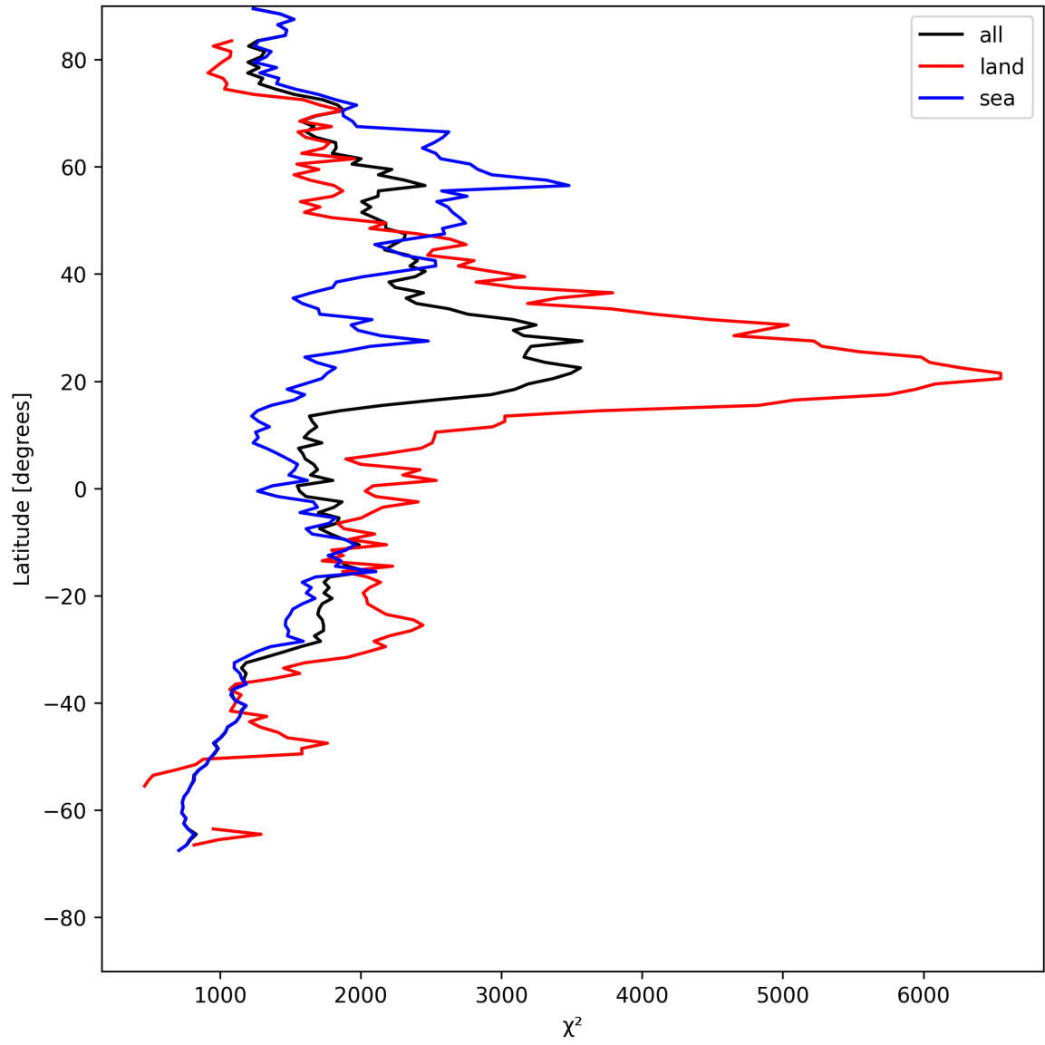
Figure 10: Zonal average of “ \chi^2 ” for 2025-08-02 to 2025-08-03.
