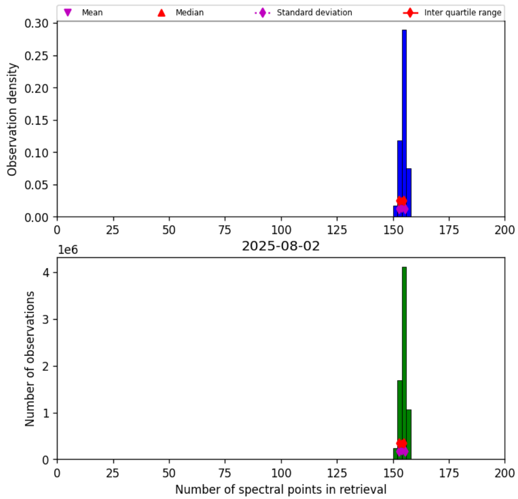
Figure 16: Histogram of “Number of spectral points in retrieval” for 2025-08-02 to 2025-08-03
