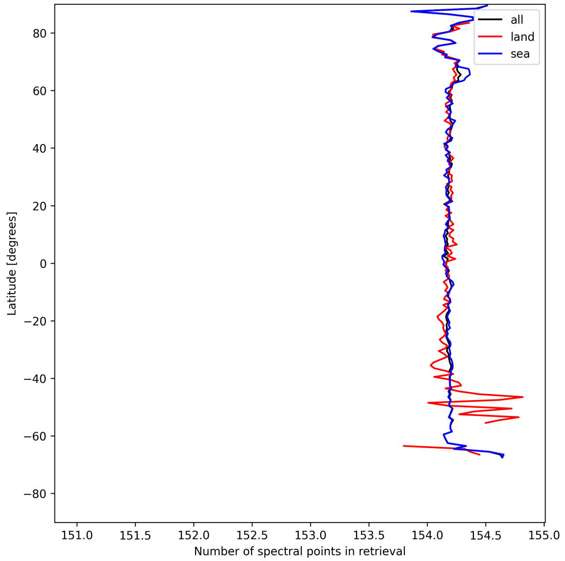
Figure 9: Zonal average of “Number of spectral points in retrieval” for 2025-08-02 to 2025-08-03.
