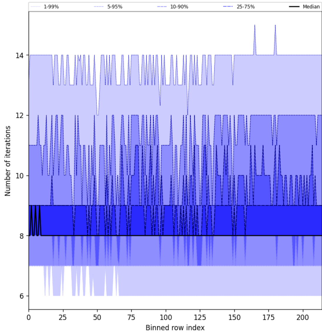
Figure 26: Along track statistics of “Number of iterations” for 2025-08-02 to 2025-08-03
