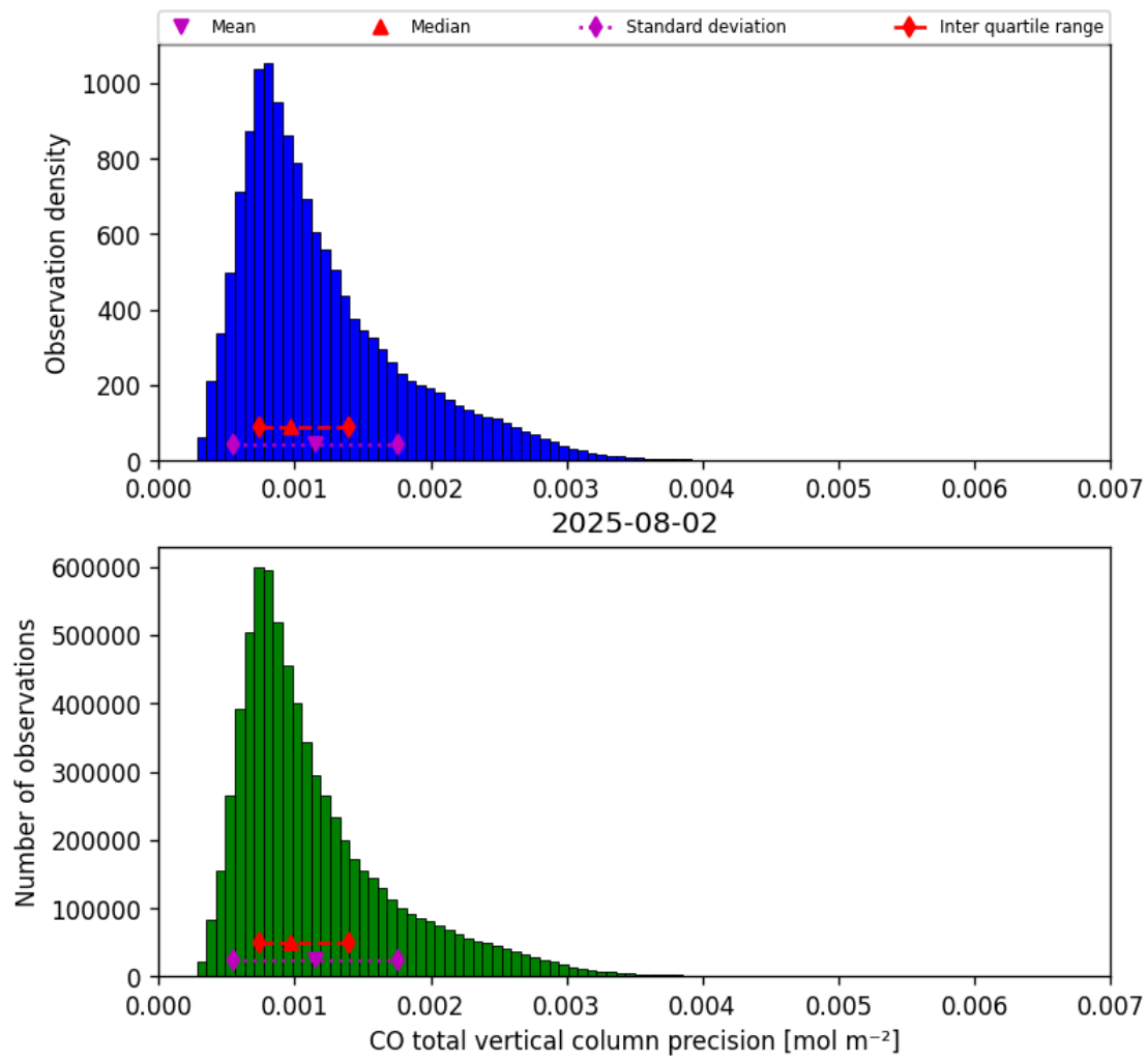
Figure 15: Histogram of “CO total vertical column precision” for 2025-08-02 to 2025-08-03
