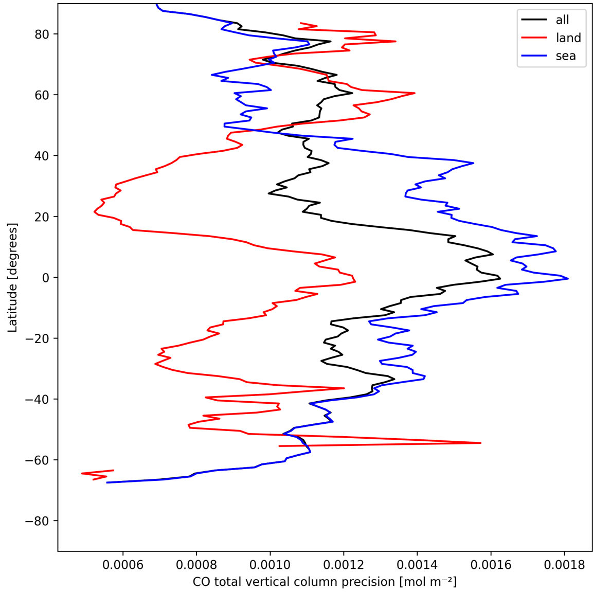
Figure 8: Zonal average of “CO total vertical column precision” for 2025-08-02 to 2025-08-03.
