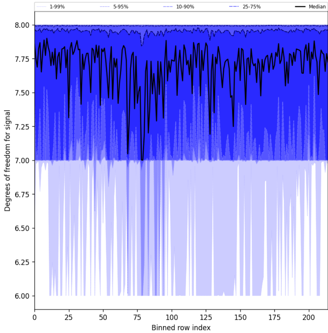
Figure 25: Along track statistics of “Degrees of freedom for signal” for 2025-08-02 to 2025-08-03
