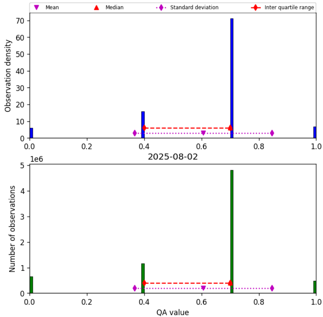
Figure 13: Histogram of “QA value” for 2025-08-02 to 2025-08-03
