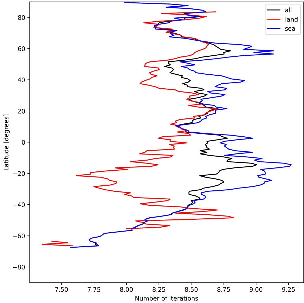
Figure 12: Zonal average of “Number of iterations” for 2025-08-02 to 2025-08-03.
