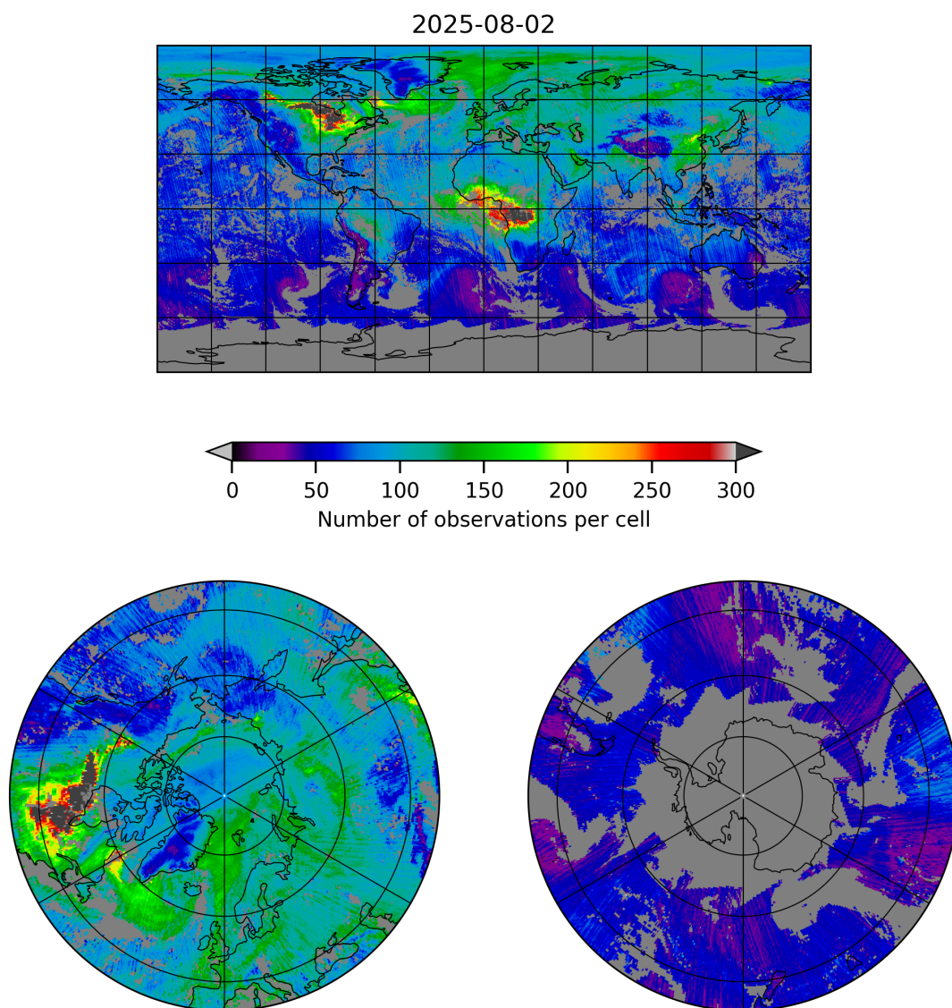
Figure 5: Map of the number of observations for 2025-08-02 to 2025-08-03
