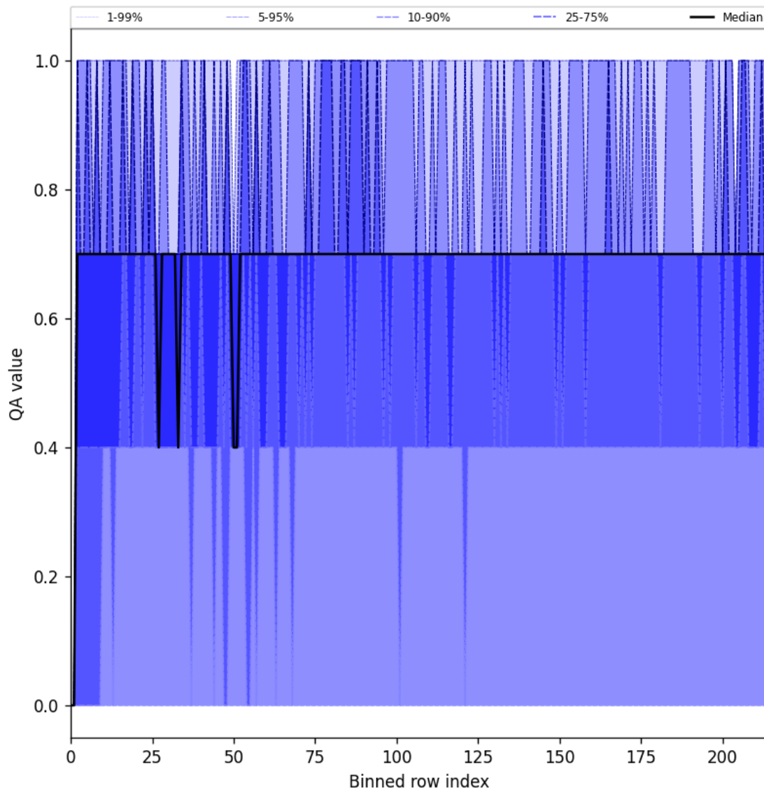
Figure 20: Along track statistics of “QA value” for 2025-08-02 to 2025-08-03
