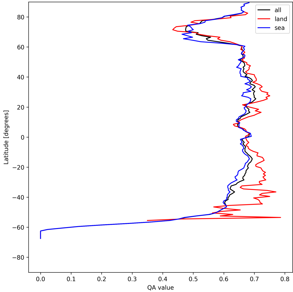
Figure 6: Zonal average of “QA value” for 2025-08-02 to 2025-08-03.
