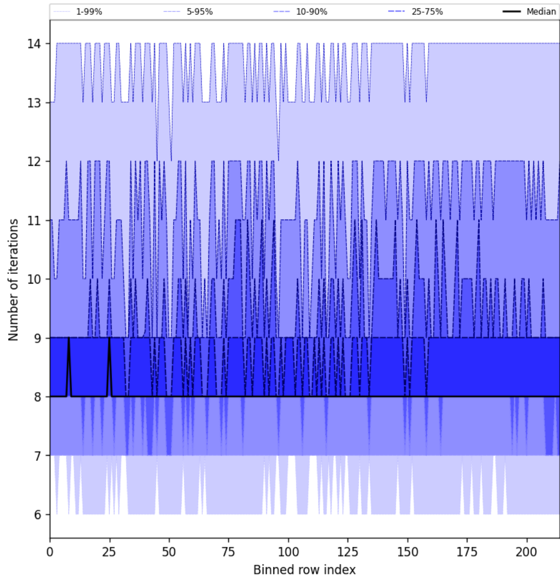
Figure 26: Along track statistics of “Number of iterations” for 2025-08-03 to 2025-08-04
