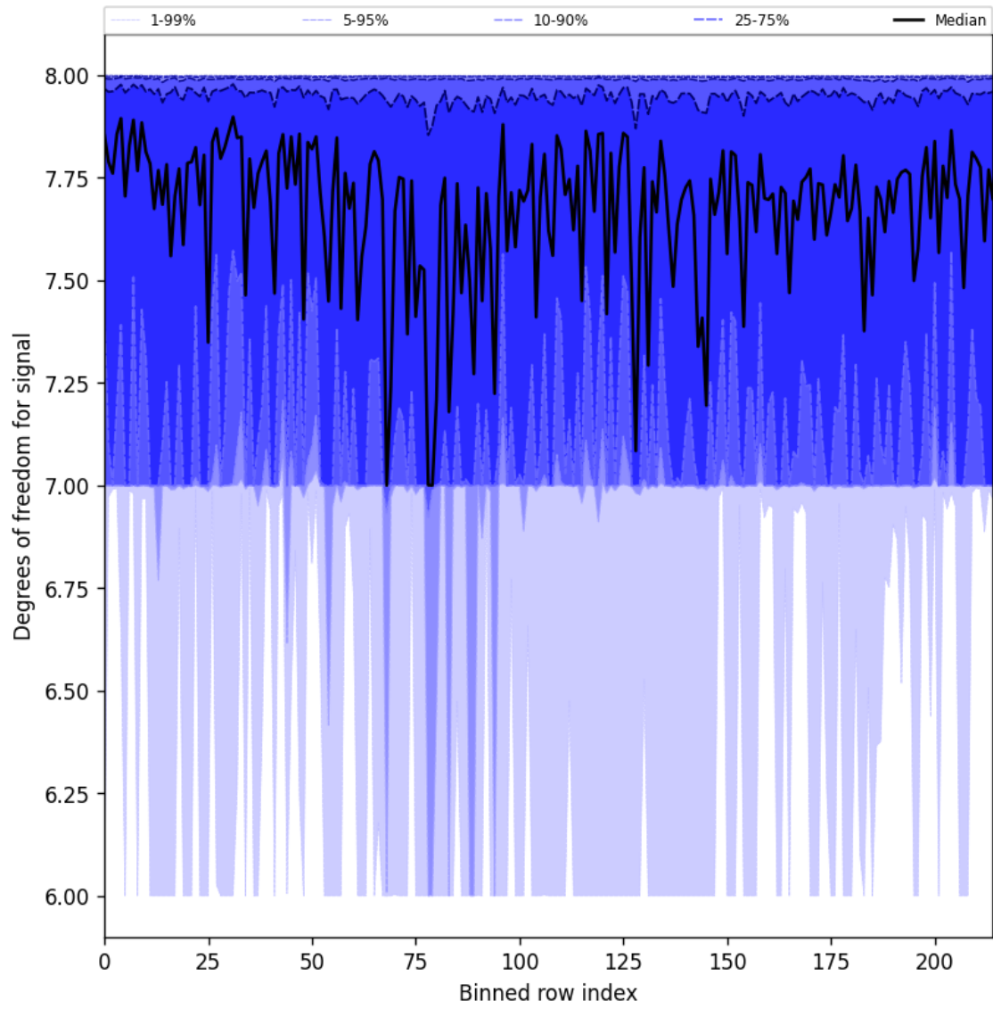
Figure 25: Along track statistics of “Degrees of freedom for signal” for 2025-08-03 to 2025-08-04
