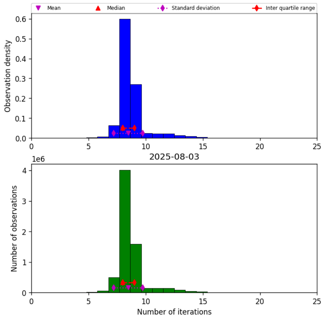
Figure 19: Histogram of “Number of iterations” for 2025-08-03 to 2025-08-04
