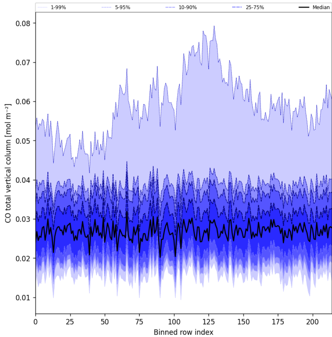
Figure 21: Along track statistics of “CO total vertical column” for 2025-08-03 to 2025-08-04
