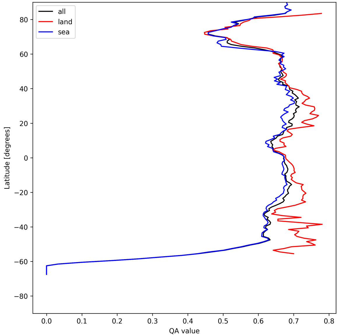
Figure 6: Zonal average of “QA value” for 2025-08-03 to 2025-08-04.
