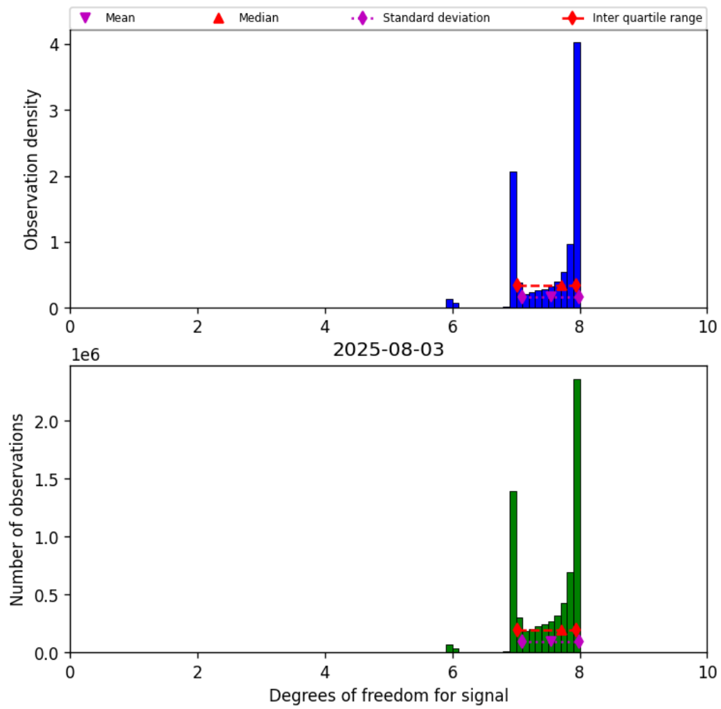
Figure 18: Histogram of “Degrees of freedom for signal” for 2025-08-03 to 2025-08-04
