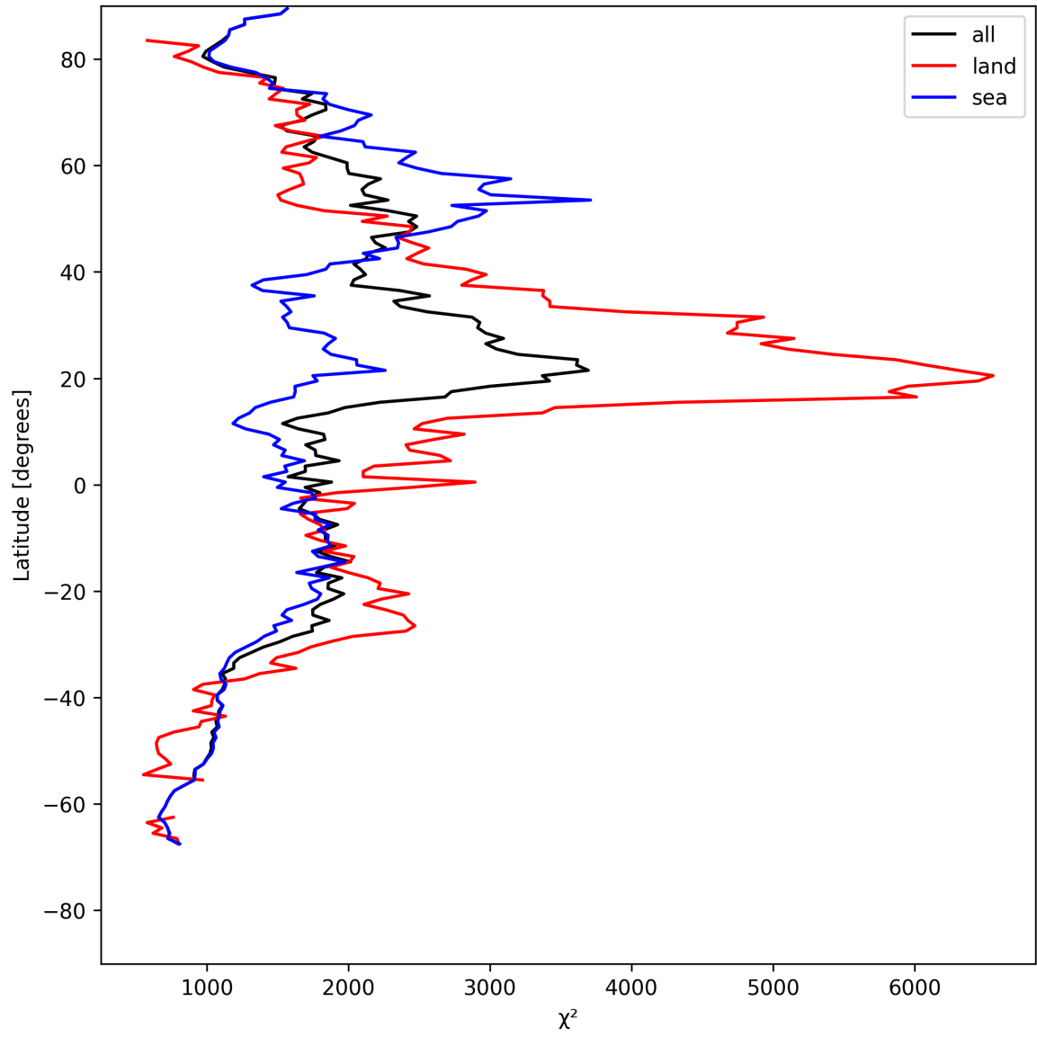
Figure 10: Zonal average of “ \chi^2 ” for 2025-08-03 to 2025-08-04.
