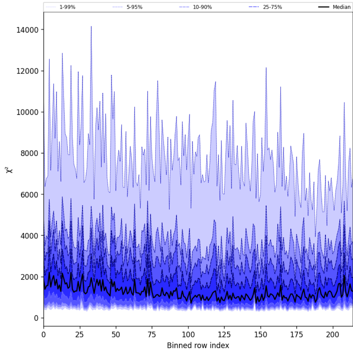
Figure 24: Along track statistics of “ \chi^2 ” for 2025-08-03 to 2025-08-04
