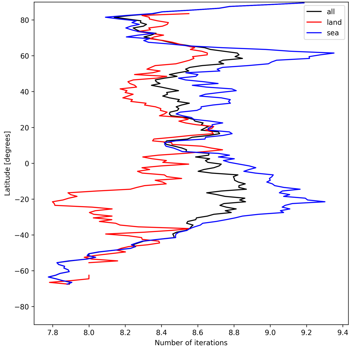
Figure 12: Zonal average of “Number of iterations” for 2025-08-03 to 2025-08-04.
