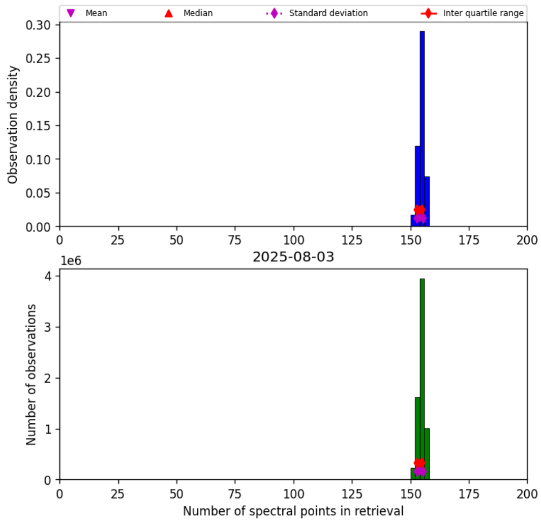
Figure 16: Histogram of “Number of spectral points in retrieval” for 2025-08-03 to 2025-08-04
