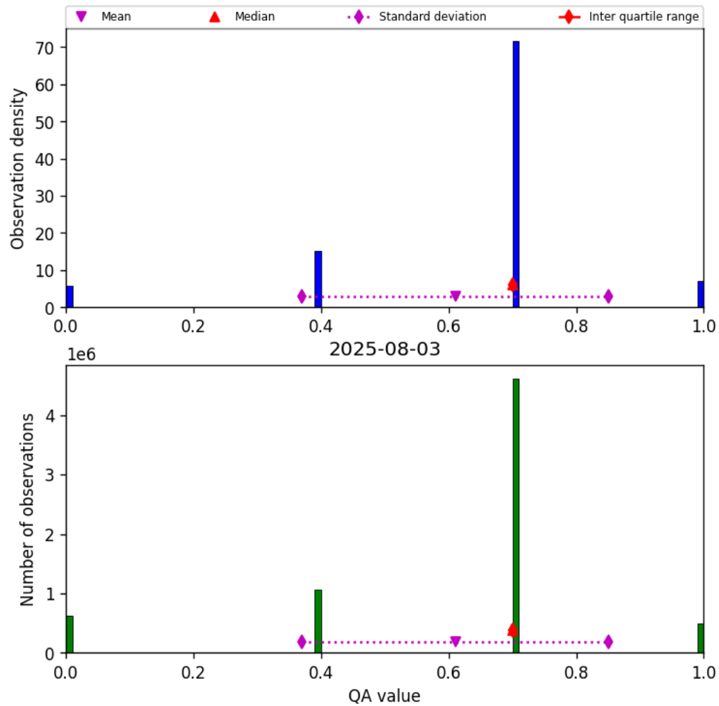
Figure 13: Histogram of “QA value” for 2025-08-03 to 2025-08-04
