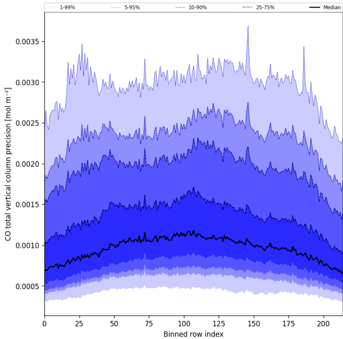
Figure 22: Along track statistics of “CO total vertical column precision” for 2025-08-03 to 2025-08-04
