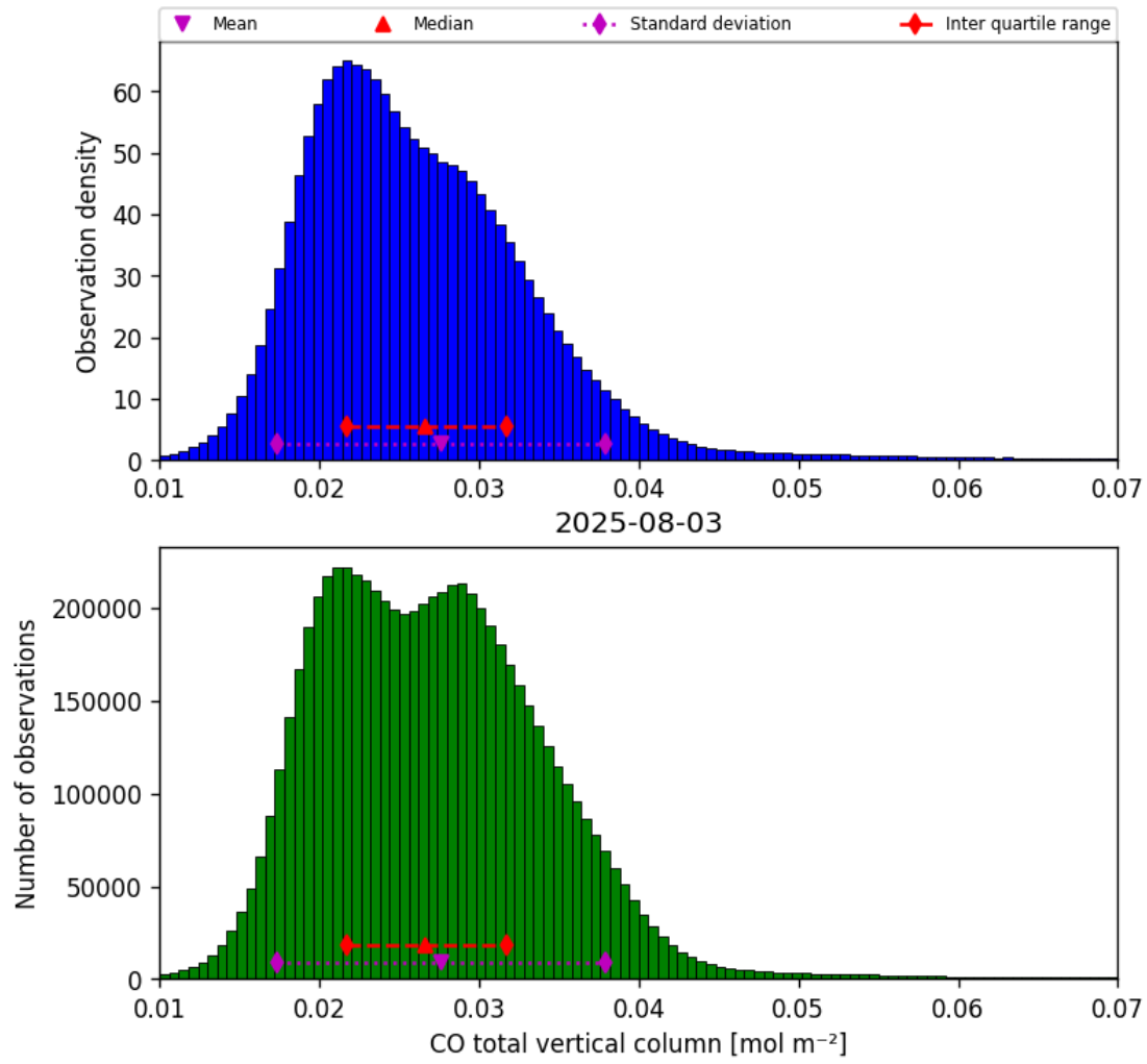
Figure 14: Histogram of “CO total vertical column” for 2025-08-03 to 2025-08-04
