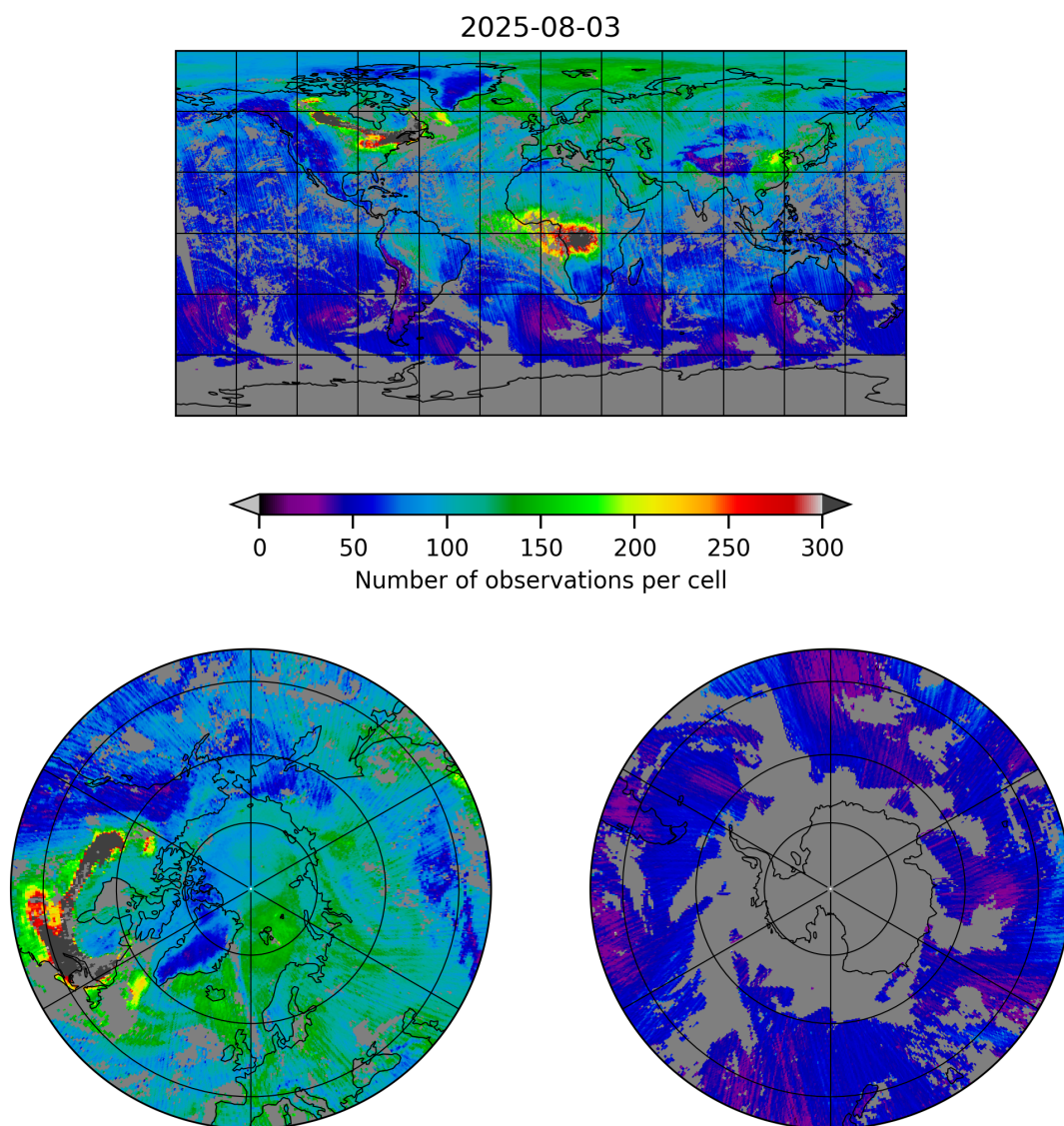
Figure 5: Map of the number of observations for 2025-08-03 to 2025-08-04
