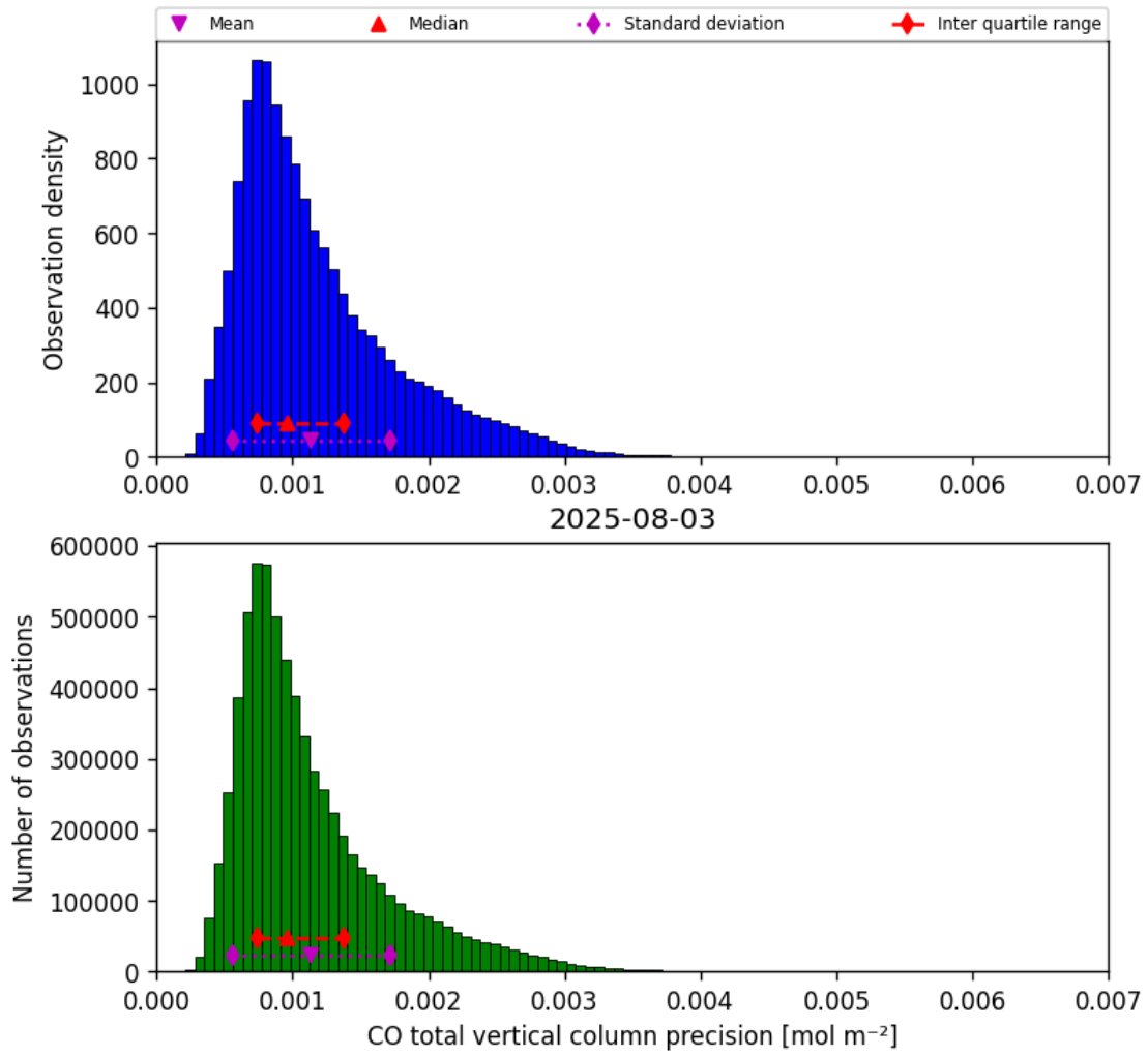
Figure 15: Histogram of “CO total vertical column precision” for 2025-08-03 to 2025-08-04
