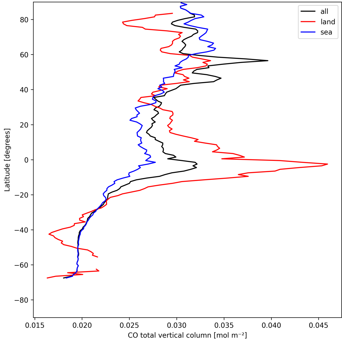
Figure 7: Zonal average of “CO total vertical column” for 2025-08-03 to 2025-08-04.
