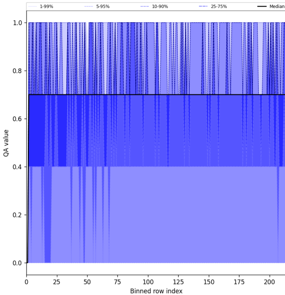
Figure 20: Along track statistics of “QA value” for 2025-08-03 to 2025-08-04
