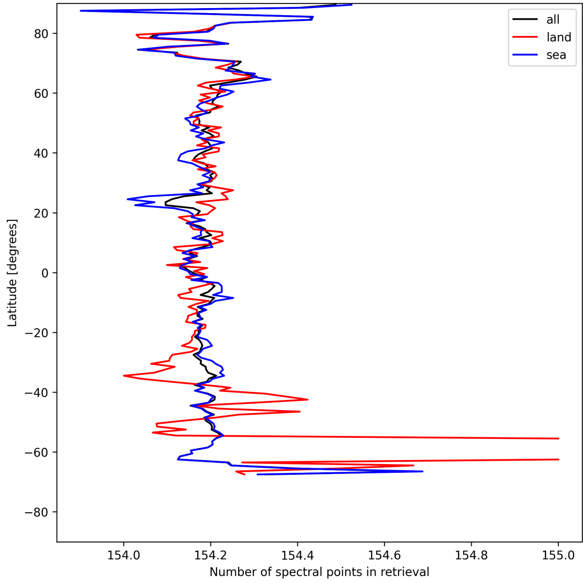
Figure 9: Zonal average of “Number of spectral points in retrieval” for 2025-08-03 to 2025-08-04.
