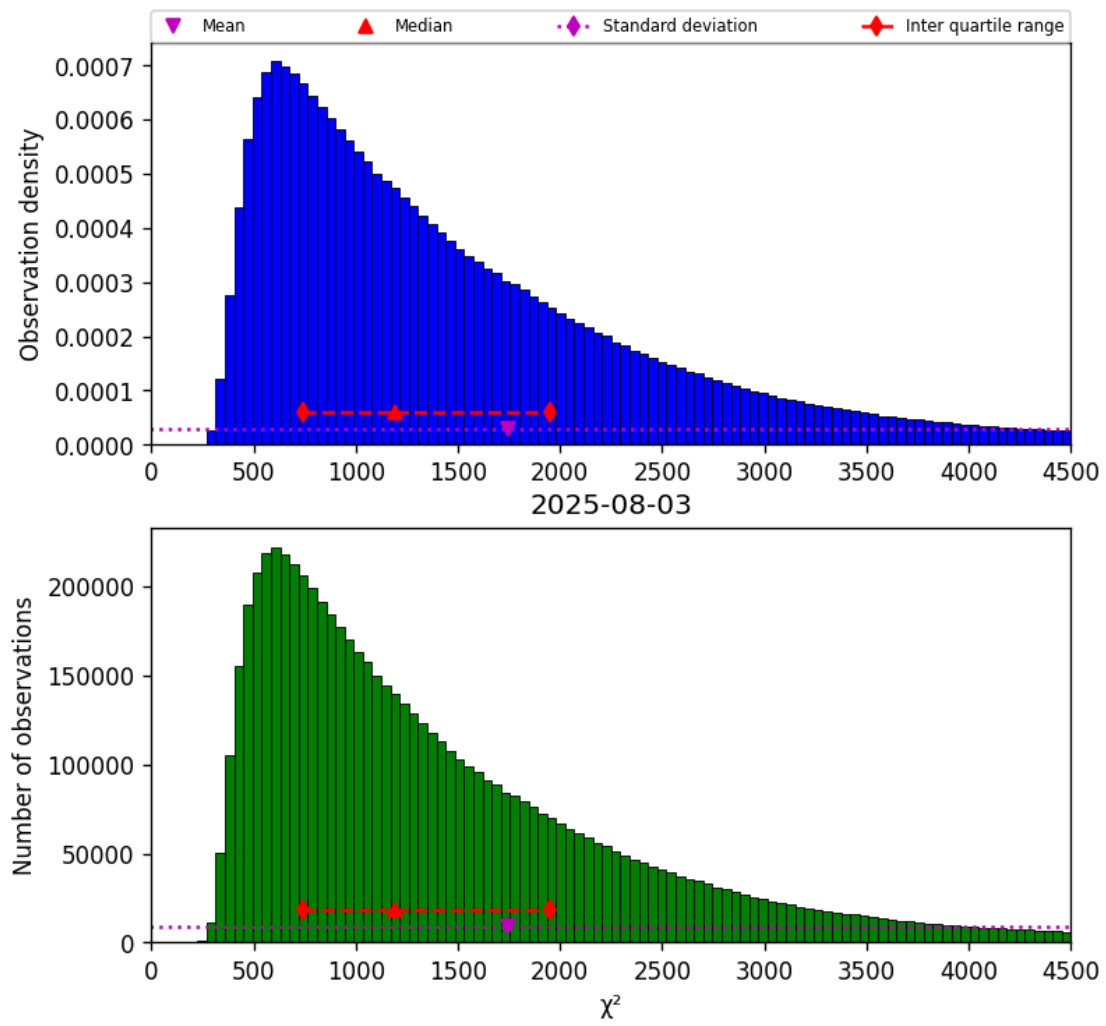
Figure 17: Histogram of “ \chi^2 ” for 2025-08-03 to 2025-08-04
