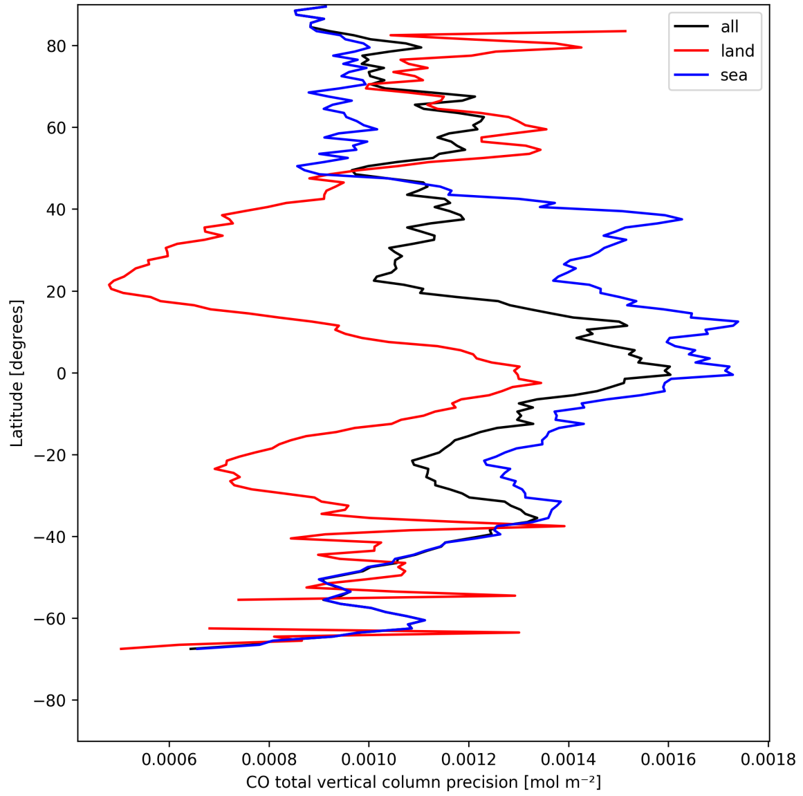
Figure 8: Zonal average of “CO total vertical column precision” for 2025-08-03 to 2025-08-04.
