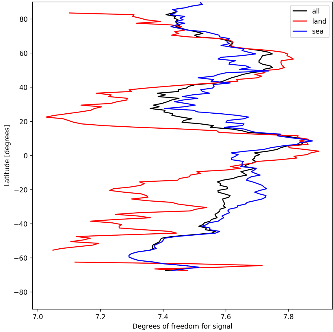
Figure 11: Zonal average of “Degrees of freedom for signal” for 2025-08-03 to 2025-08-04.
