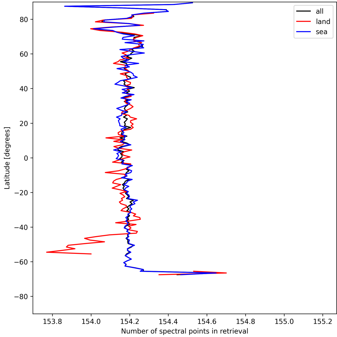
Figure 9: Zonal average of “Number of spectral points in retrieval” for 2025-08-04 to 2025-08-05.
