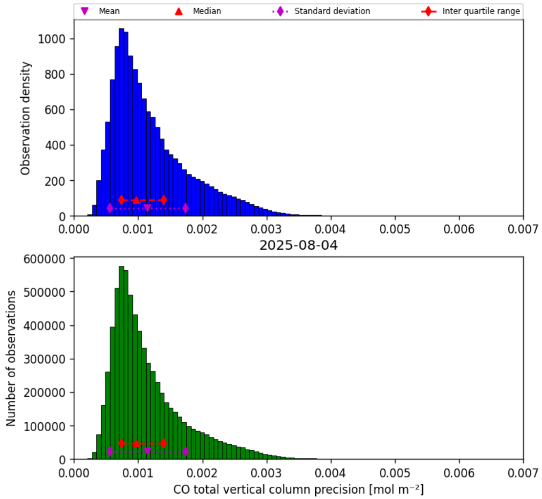
Figure 15: Histogram of “CO total vertical column precision” for 2025-08-04 to 2025-08-05
