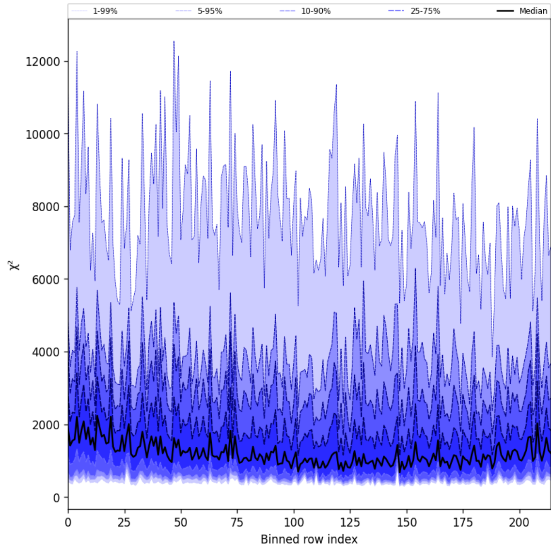
Figure 24: Along track statistics of “ \chi^2 ” for 2025-08-04 to 2025-08-05
