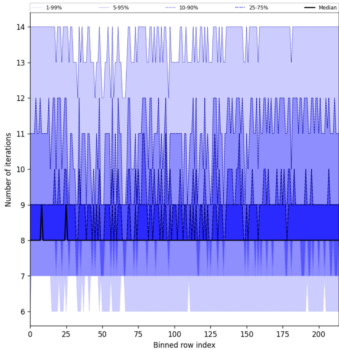
Figure 26: Along track statistics of “Number of iterations” for 2025-08-04 to 2025-08-05
