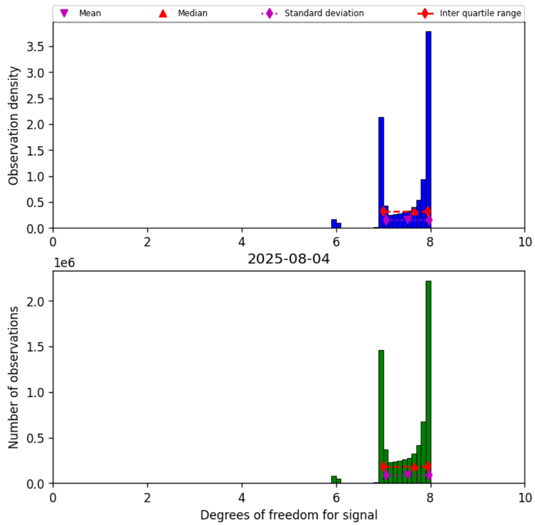
Figure 18: Histogram of “Degrees of freedom for signal” for 2025-08-04 to 2025-08-05
