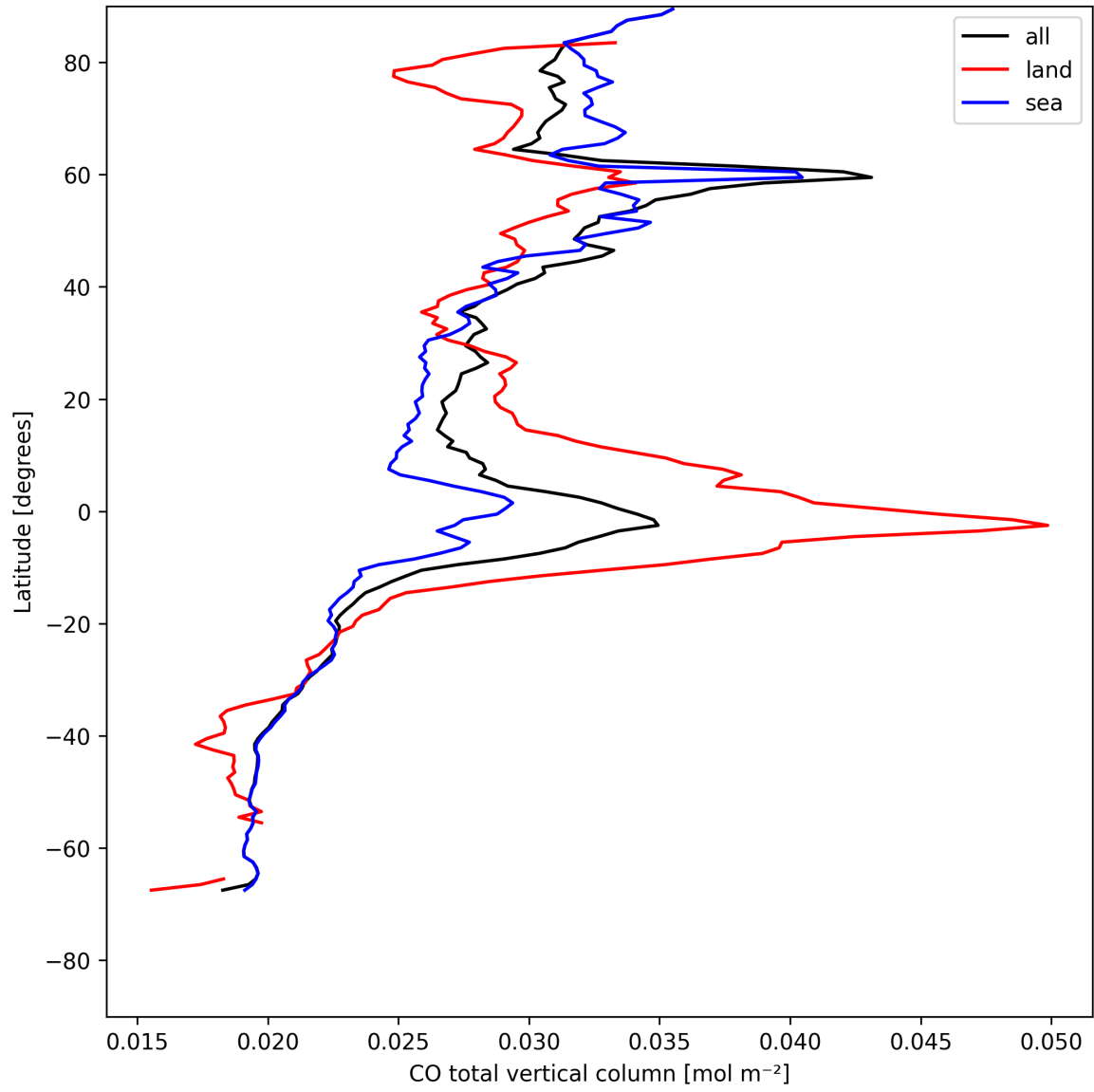
Figure 7: Zonal average of “CO total vertical column” for 2025-08-04 to 2025-08-05.
