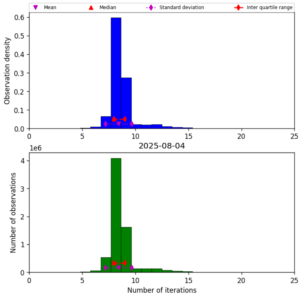
Figure 19: Histogram of “Number of iterations” for 2025-08-04 to 2025-08-05
