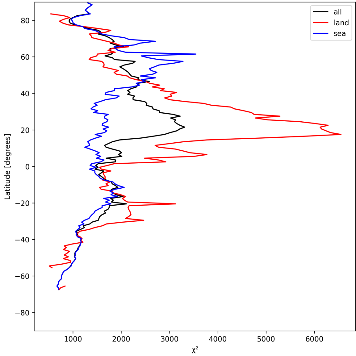
Figure 10: Zonal average of “ \chi^2 ” for 2025-08-04 to 2025-08-05.
