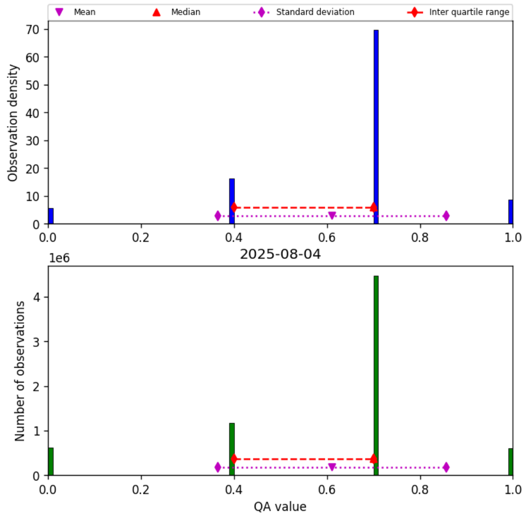
Figure 13: Histogram of “QA value” for 2025-08-04 to 2025-08-05
