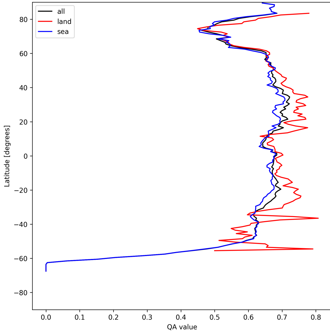
Figure 6: Zonal average of “QA value” for 2025-08-04 to 2025-08-05.
