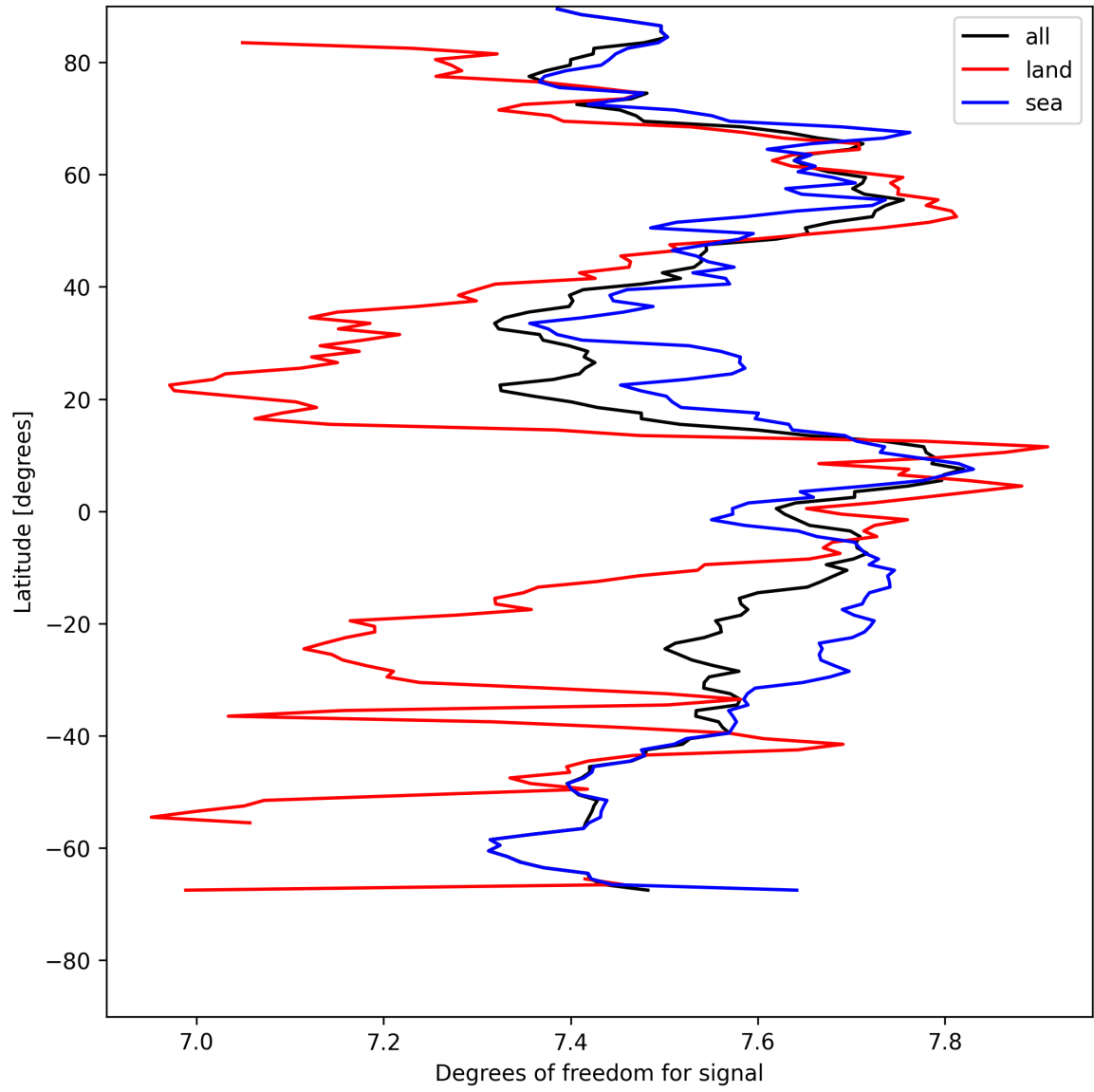
Figure 11: Zonal average of “Degrees of freedom for signal” for 2025-08-04 to 2025-08-05.
