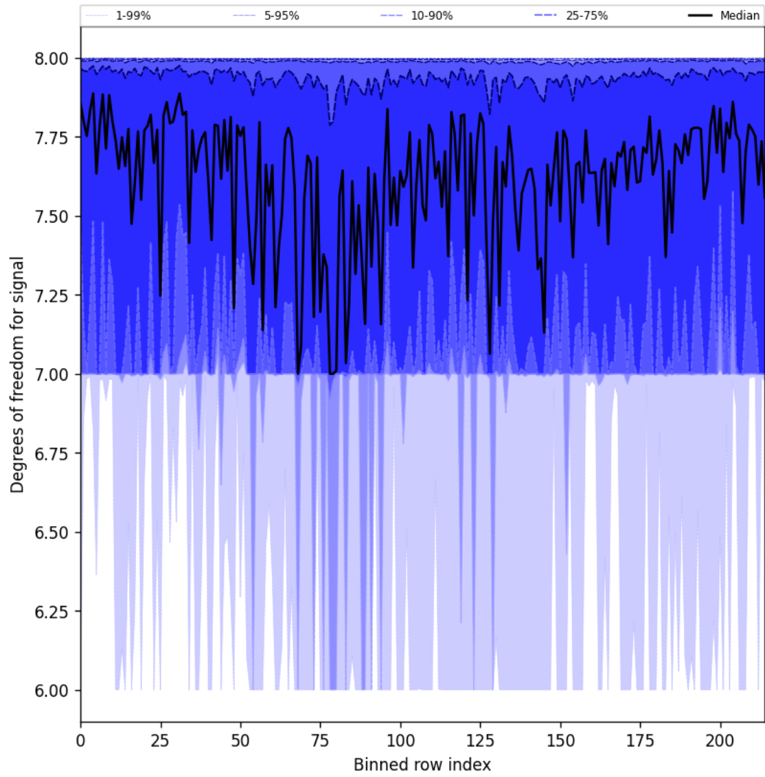
Figure 25: Along track statistics of “Degrees of freedom for signal” for 2025-08-04 to 2025-08-05
