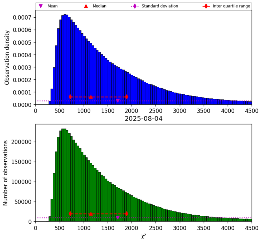
Figure 17: Histogram of “ \chi^2 ” for 2025-08-04 to 2025-08-05
