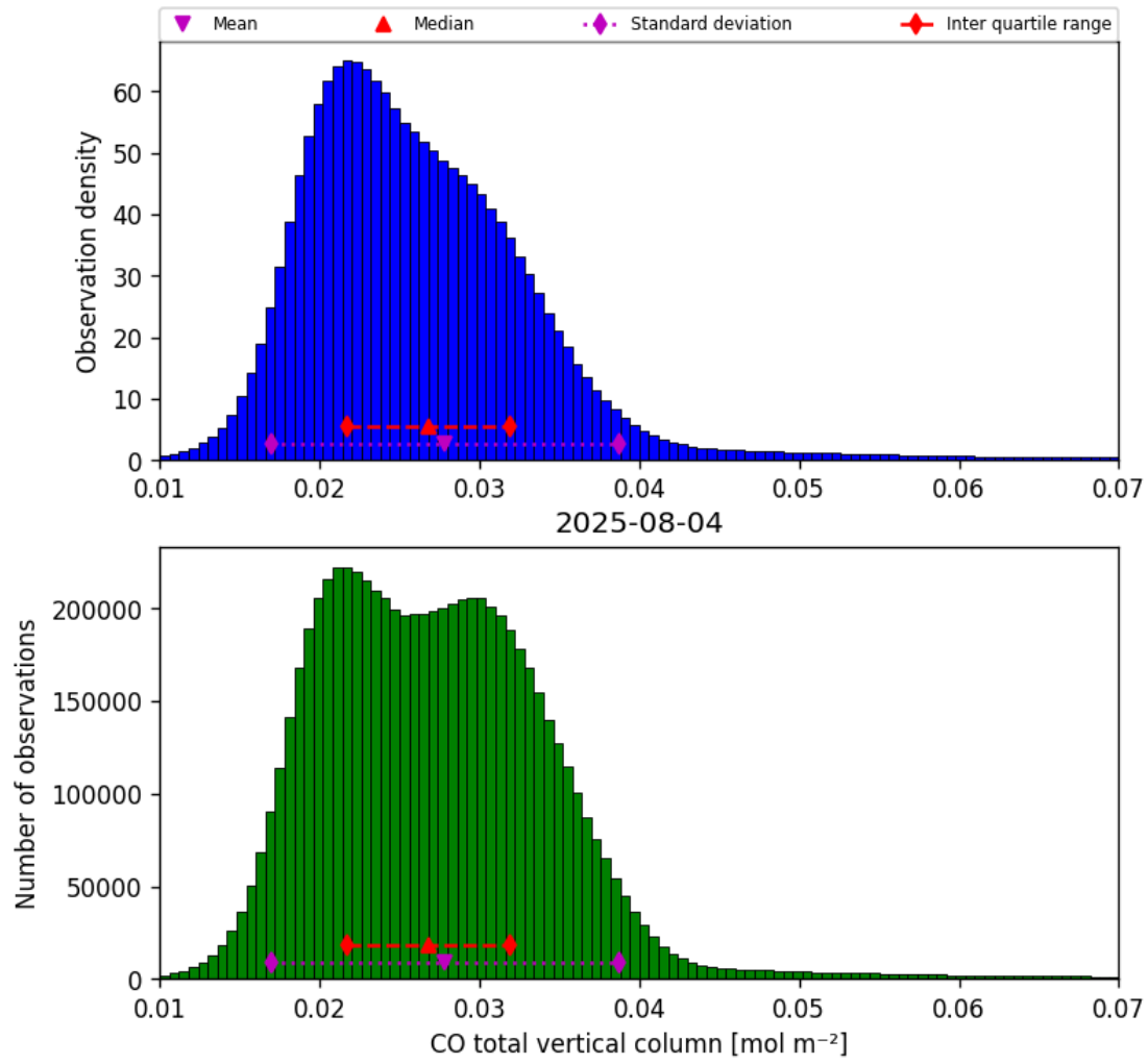
Figure 14: Histogram of “CO total vertical column” for 2025-08-04 to 2025-08-05
