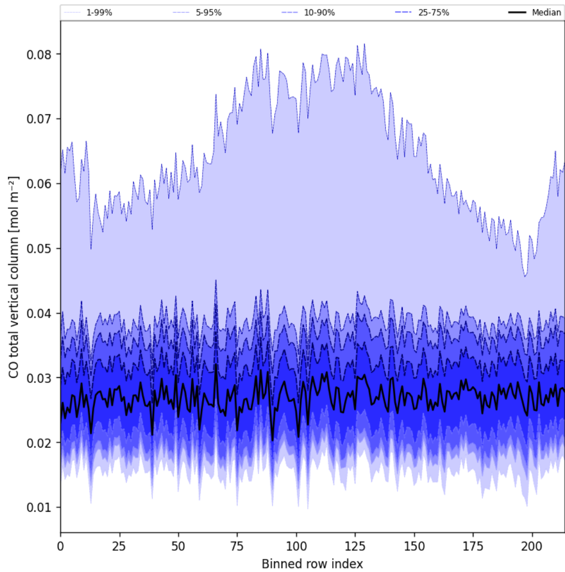
Figure 21: Along track statistics of “CO total vertical column” for 2025-08-04 to 2025-08-05
