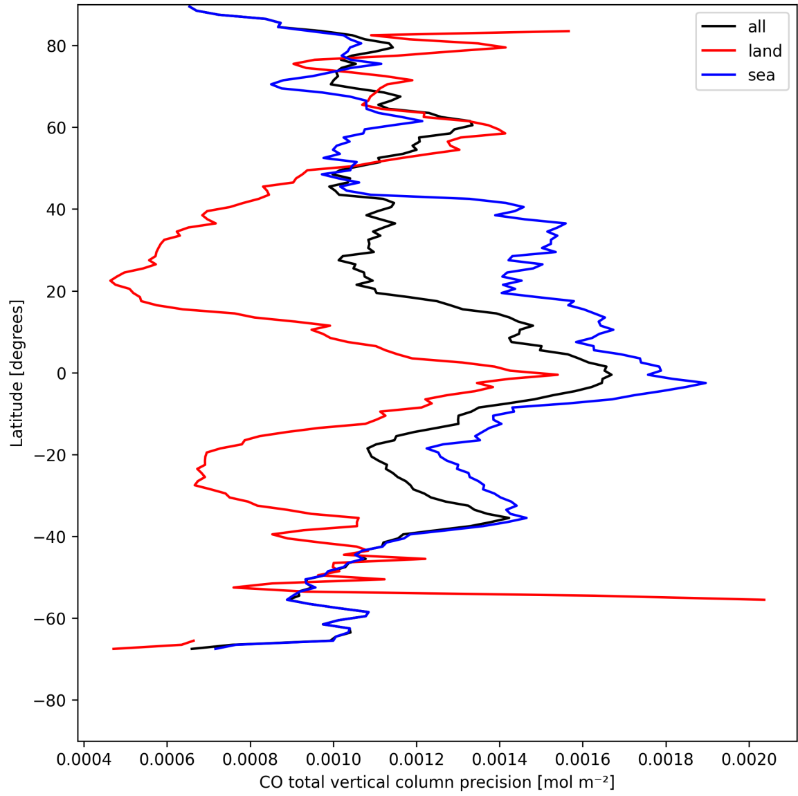
Figure 8: Zonal average of "CO total vertical column precision" for 2025-08-04 to 2025-08-05.
