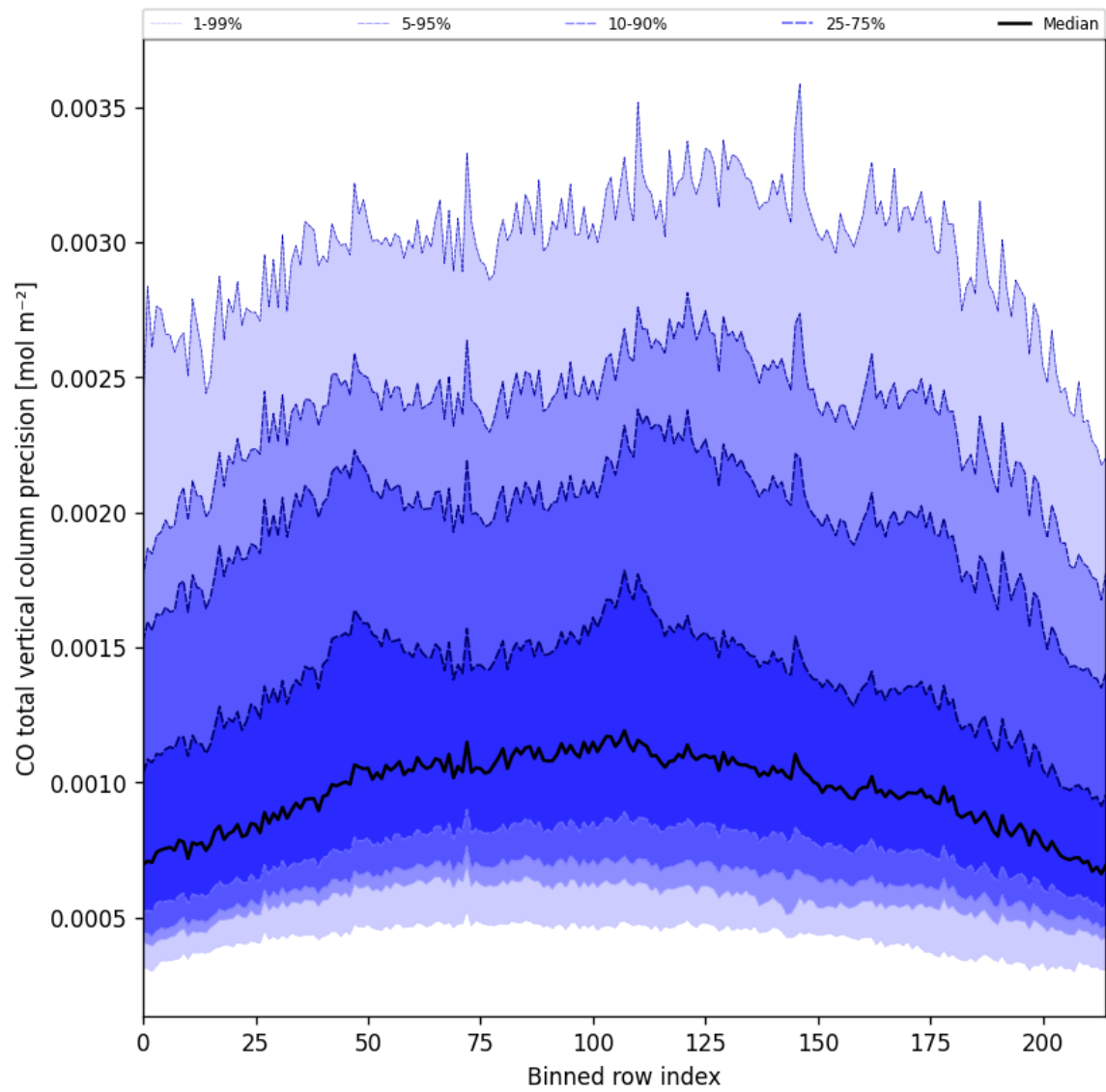
Figure 22: Along track statistics of “CO total vertical column precision” for 2025-08-04 to 2025-08-05
