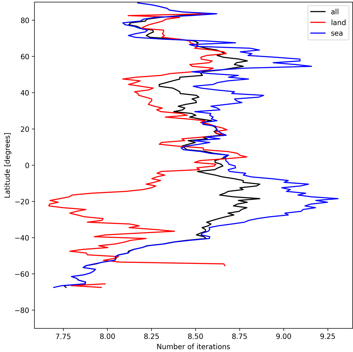
Figure 12: Zonal average of “Number of iterations” for 2025-08-04 to 2025-08-05.
