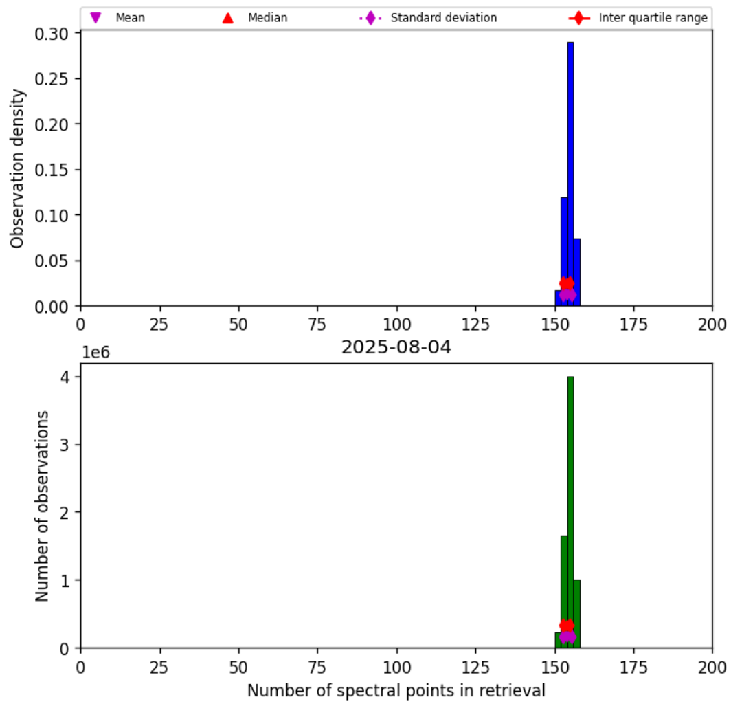
Figure 16: Histogram of “Number of spectral points in retrieval” for 2025-08-04 to 2025-08-05
