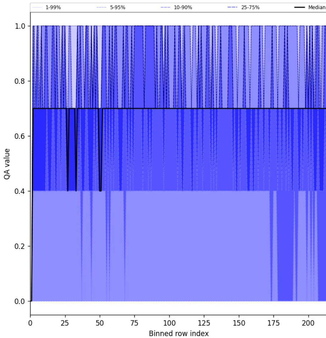
Figure 20: Along track statistics of “QA value” for 2025-08-04 to 2025-08-05
