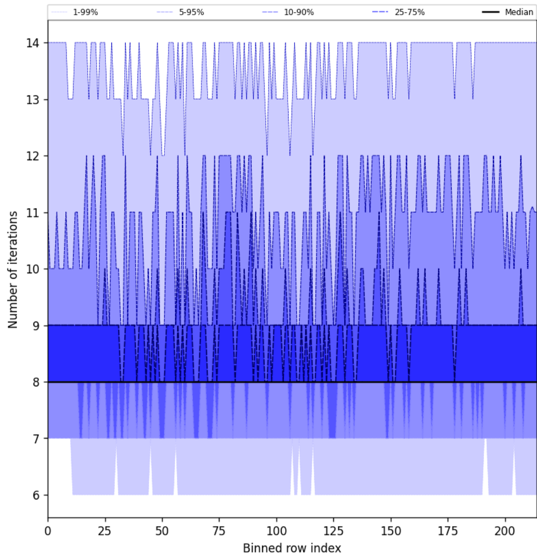
Figure 26: Along track statistics of “Number of iterations” for 2025-08-05 to 2025-08-06
