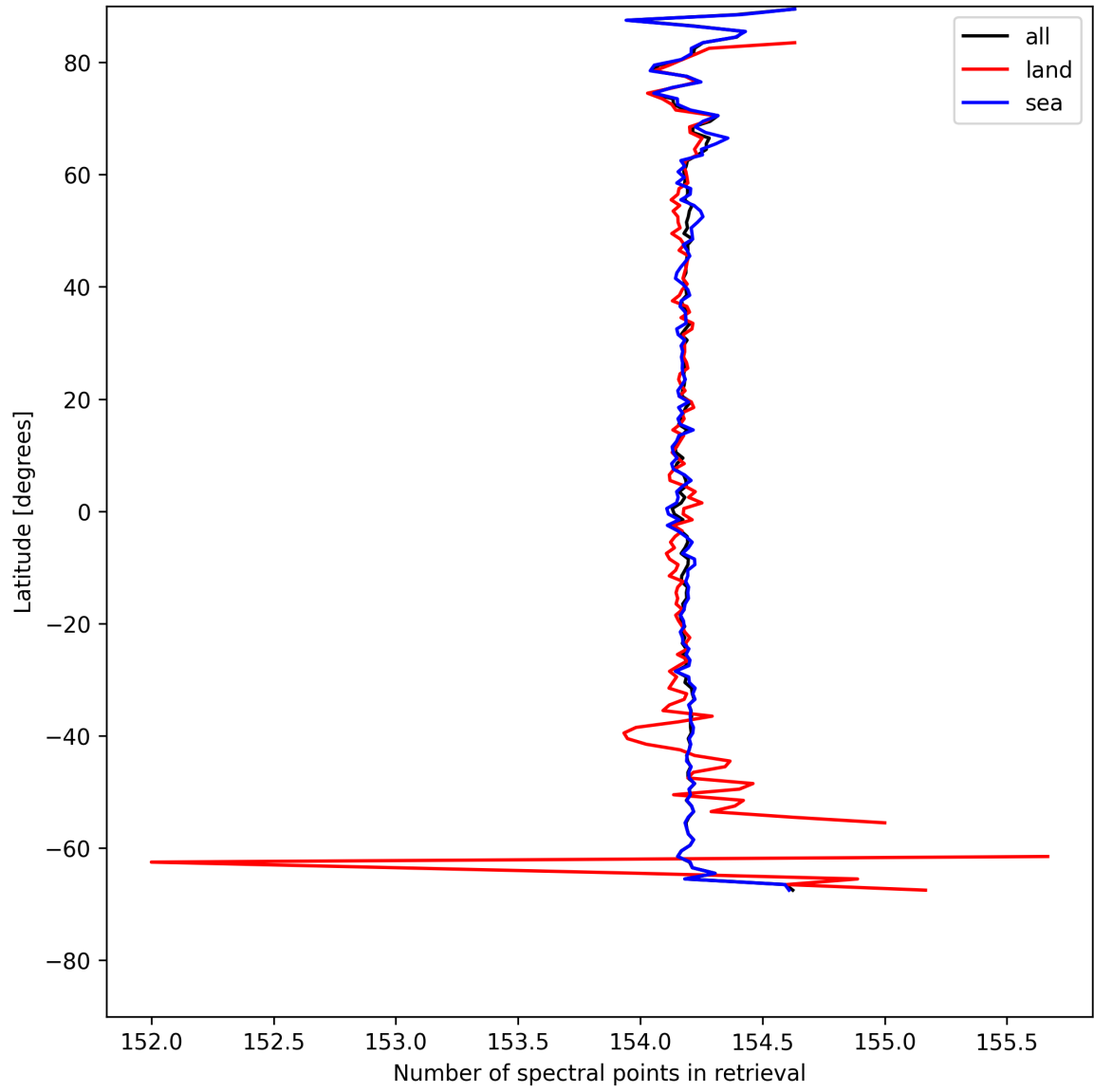
Figure 9: Zonal average of “Number of spectral points in retrieval” for 2025-08-05 to 2025-08-06.
