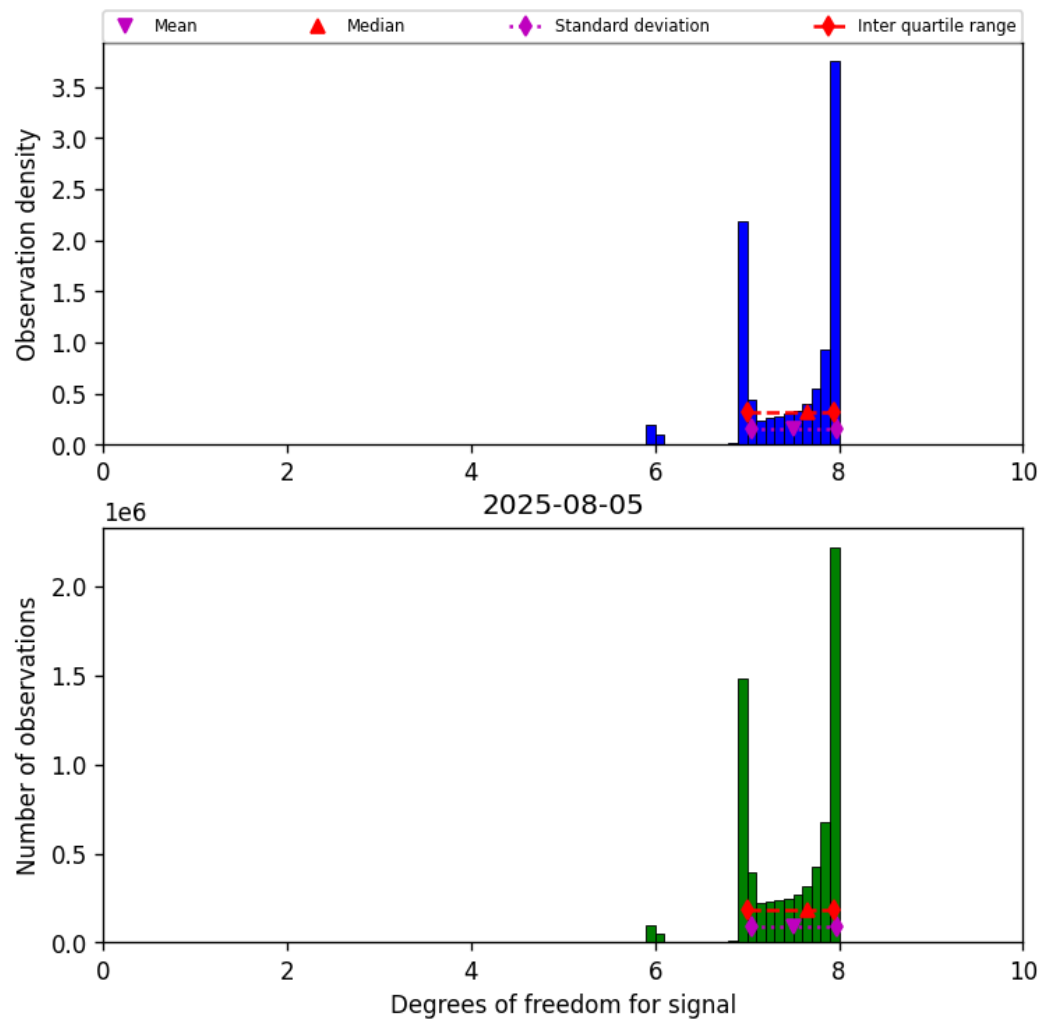
Figure 18: Histogram of “Degrees of freedom for signal” for 2025-08-05 to 2025-08-06
