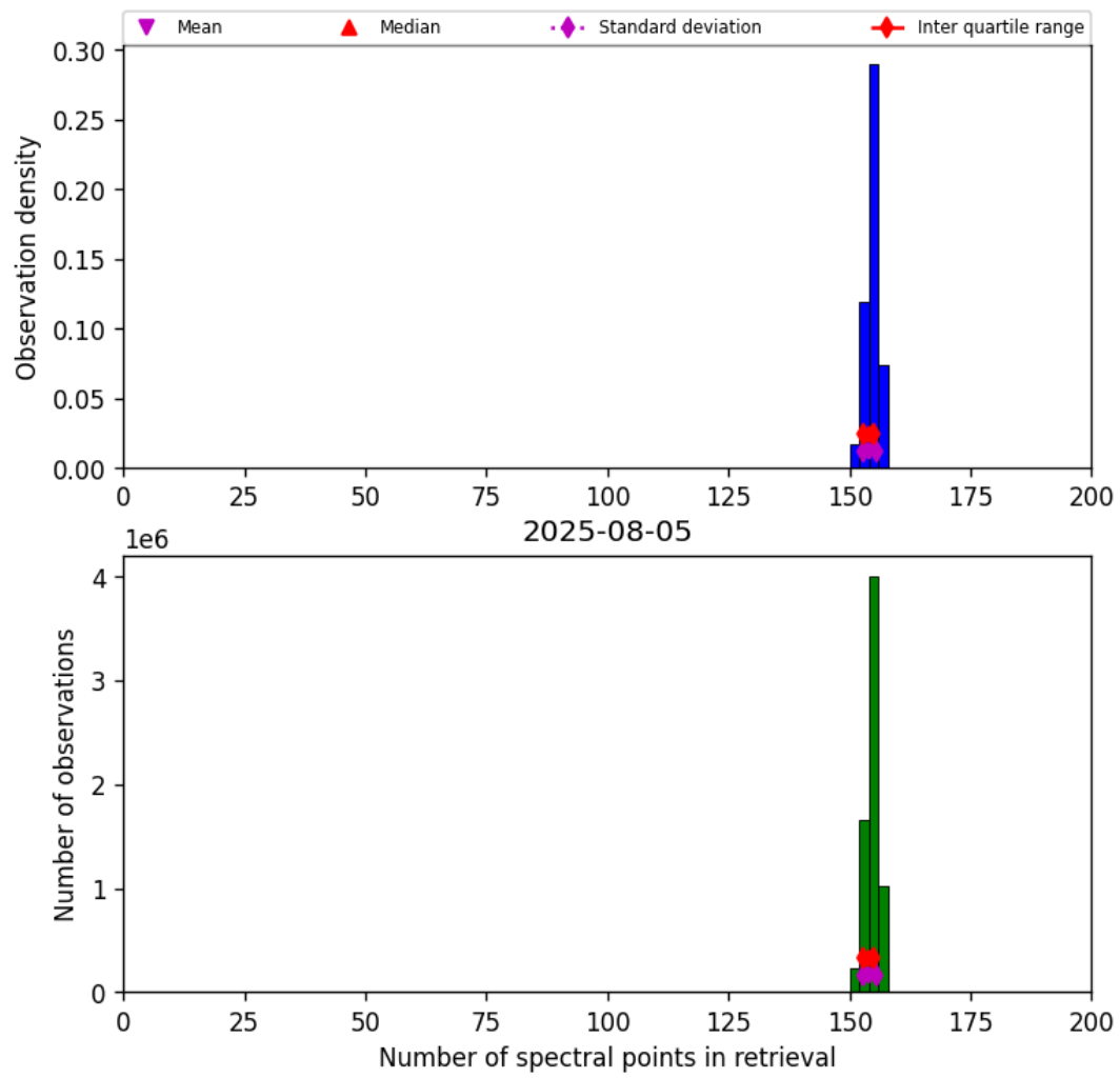
Figure 16: Histogram of “Number of spectral points in retrieval” for 2025-08-05 to 2025-08-06
