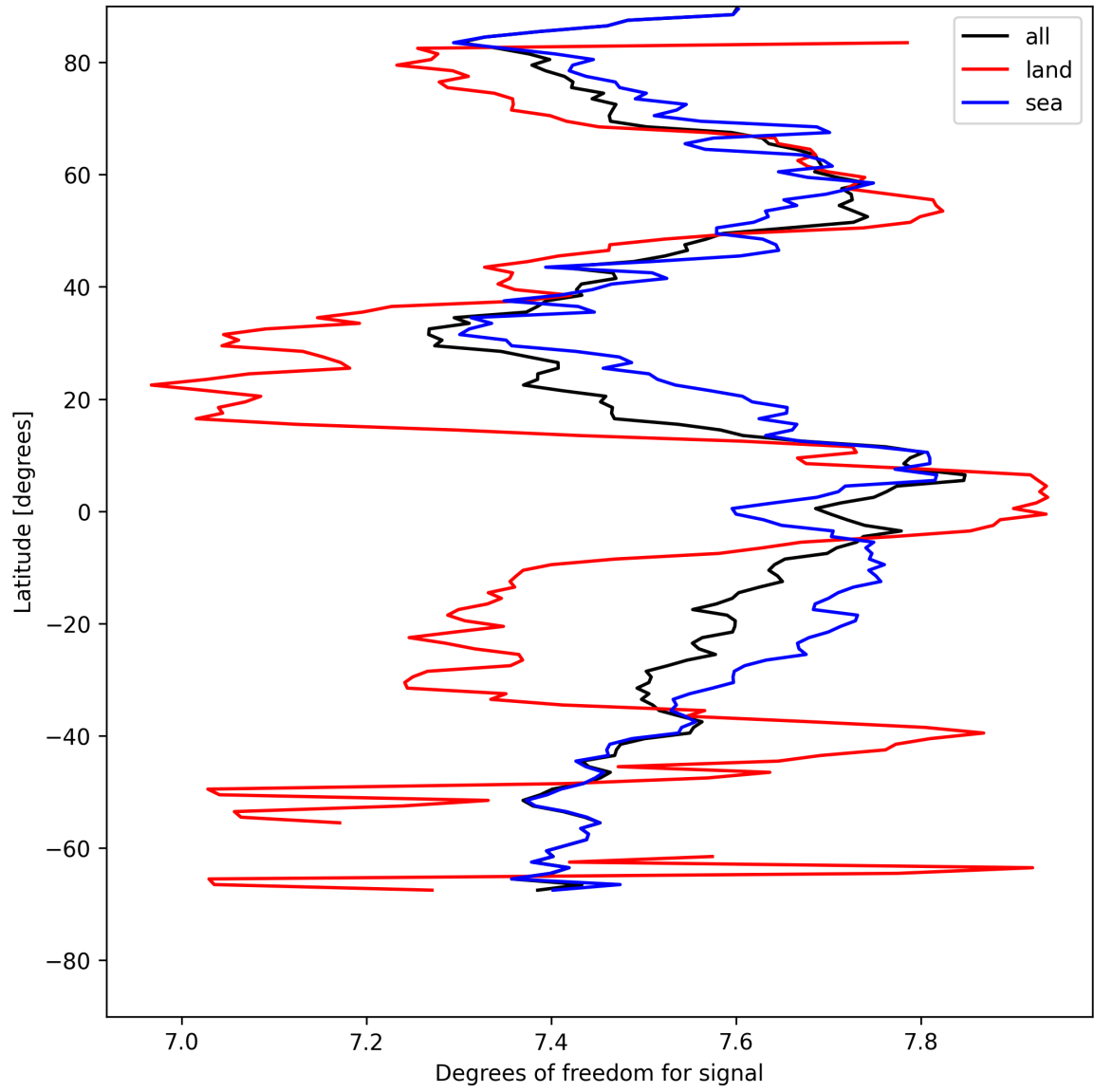
Figure 11: Zonal average of “Degrees of freedom for signal” for 2025-08-05 to 2025-08-06.
