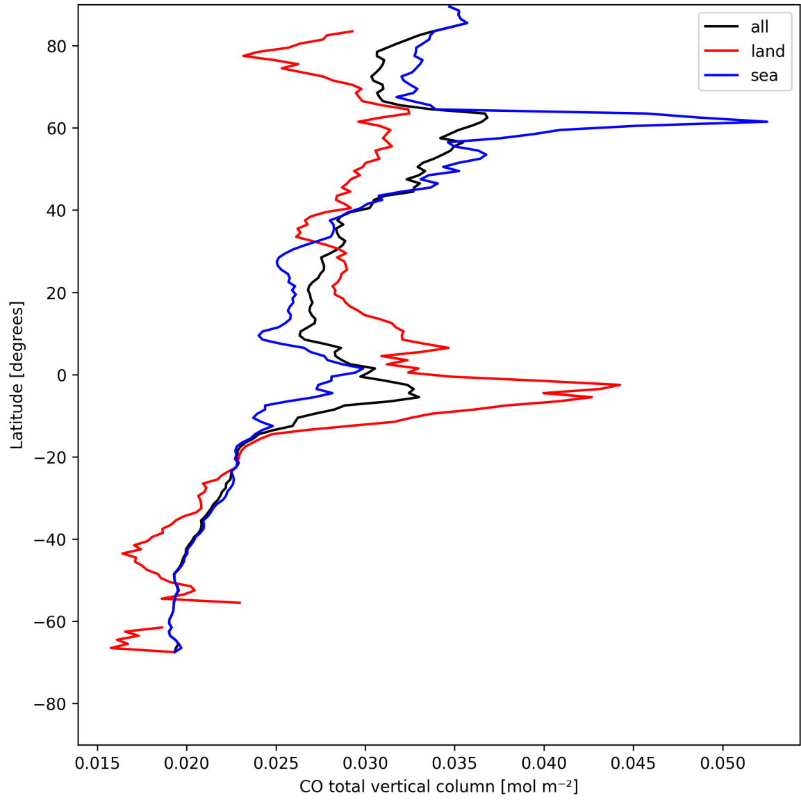
Figure 7: Zonal average of “CO total vertical column” for 2025-08-05 to 2025-08-06.
