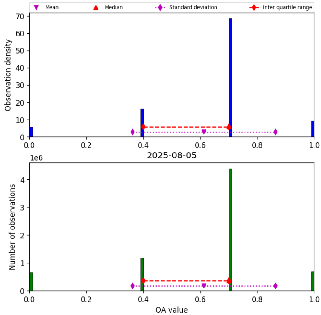
Figure 13: Histogram of “QA value” for 2025-08-05 to 2025-08-06
