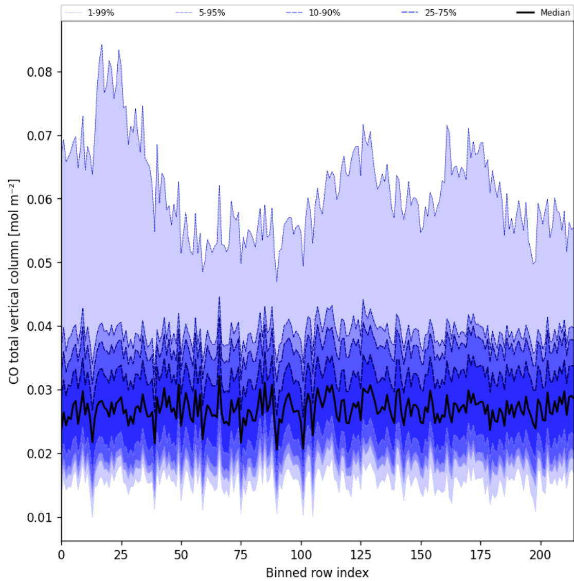
Figure 21: Along track statistics of “CO total vertical column” for 2025-08-05 to 2025-08-06
