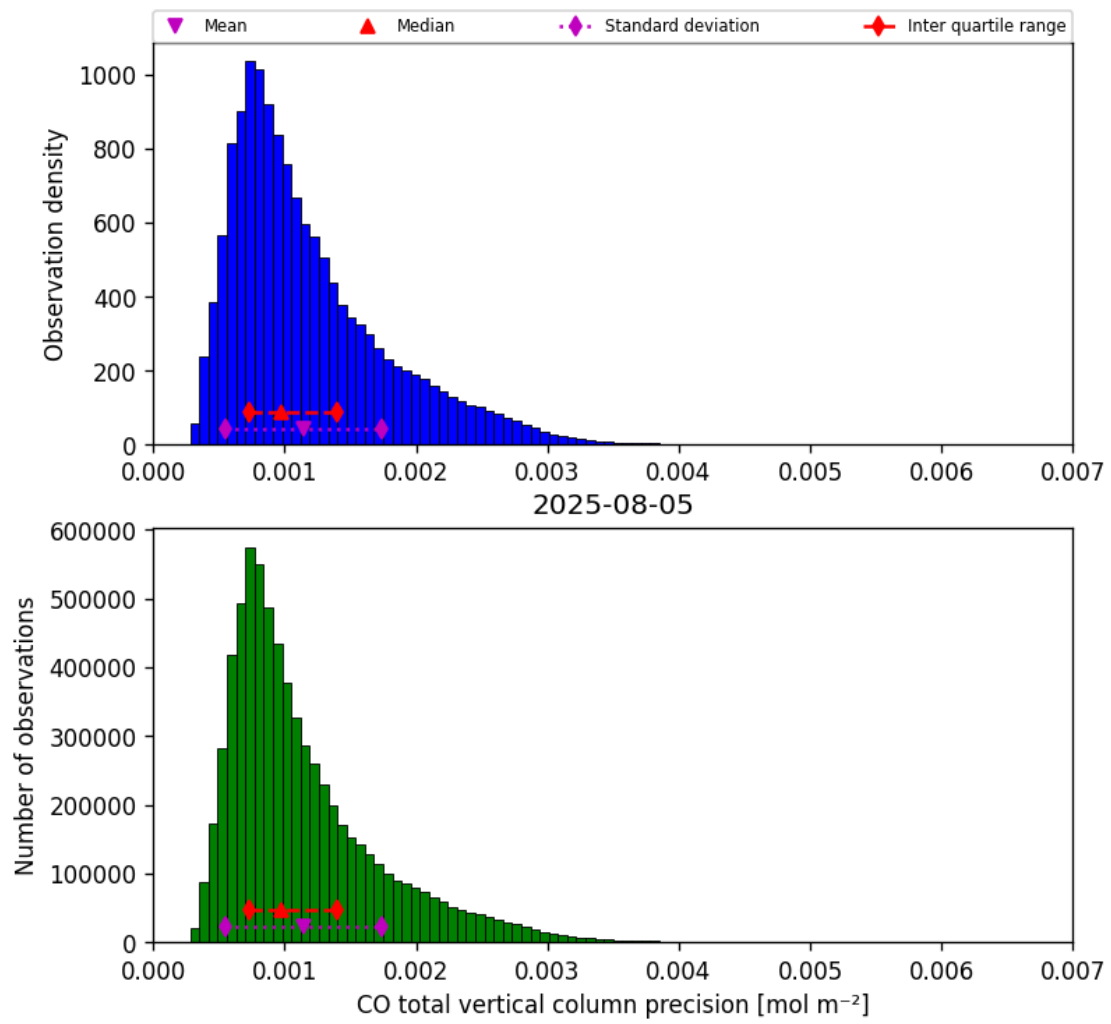
Figure 15: Histogram of “CO total vertical column precision” for 2025-08-05 to 2025-08-06
