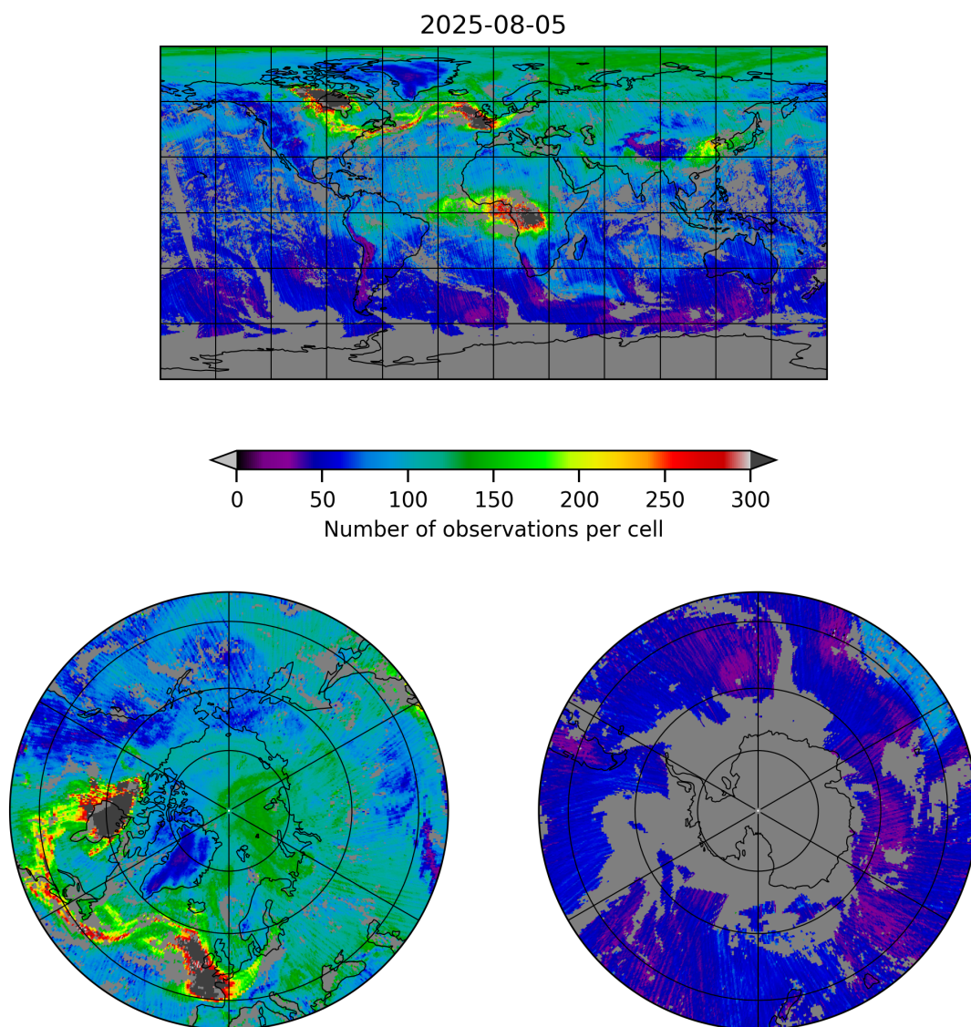
Figure 5: Map of the number of observations for 2025-08-05 to 2025-08-06
