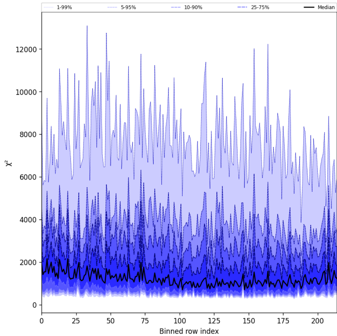
Figure 24: Along track statistics of “ \chi^2 ” for 2025-08-05 to 2025-08-06
