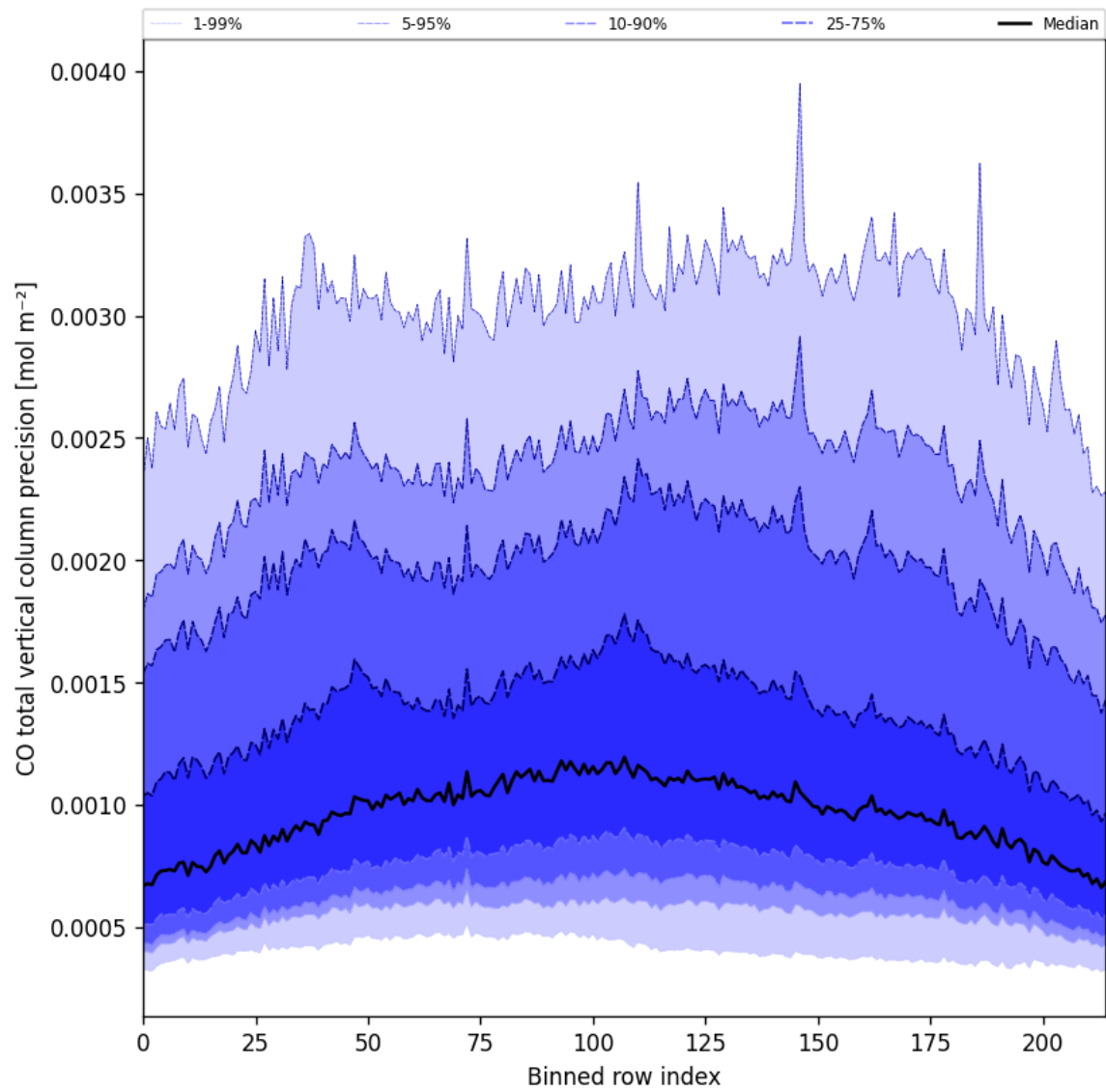
Figure 22: Along track statistics of “CO total vertical column precision” for 2025-08-05 to 2025-08-06
