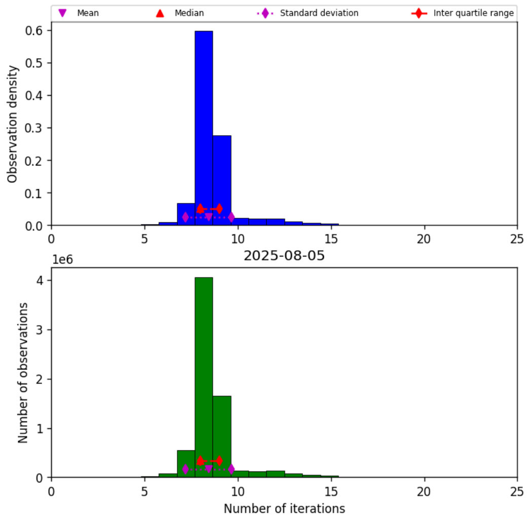
Figure 19: Histogram of “Number of iterations” for 2025-08-05 to 2025-08-06
