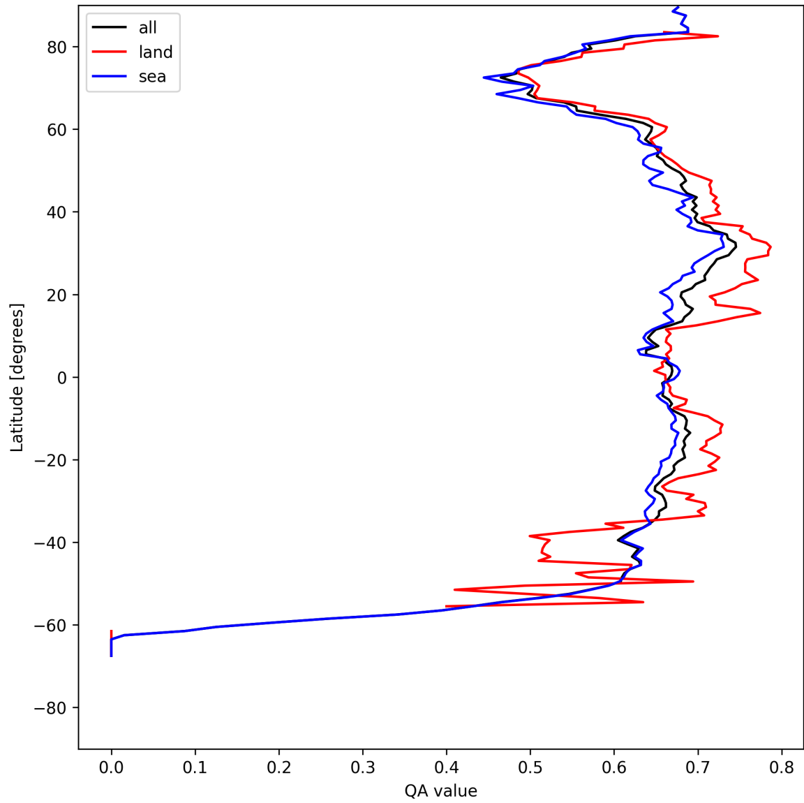
Figure 6: Zonal average of “QA value” for 2025-08-05 to 2025-08-06.
