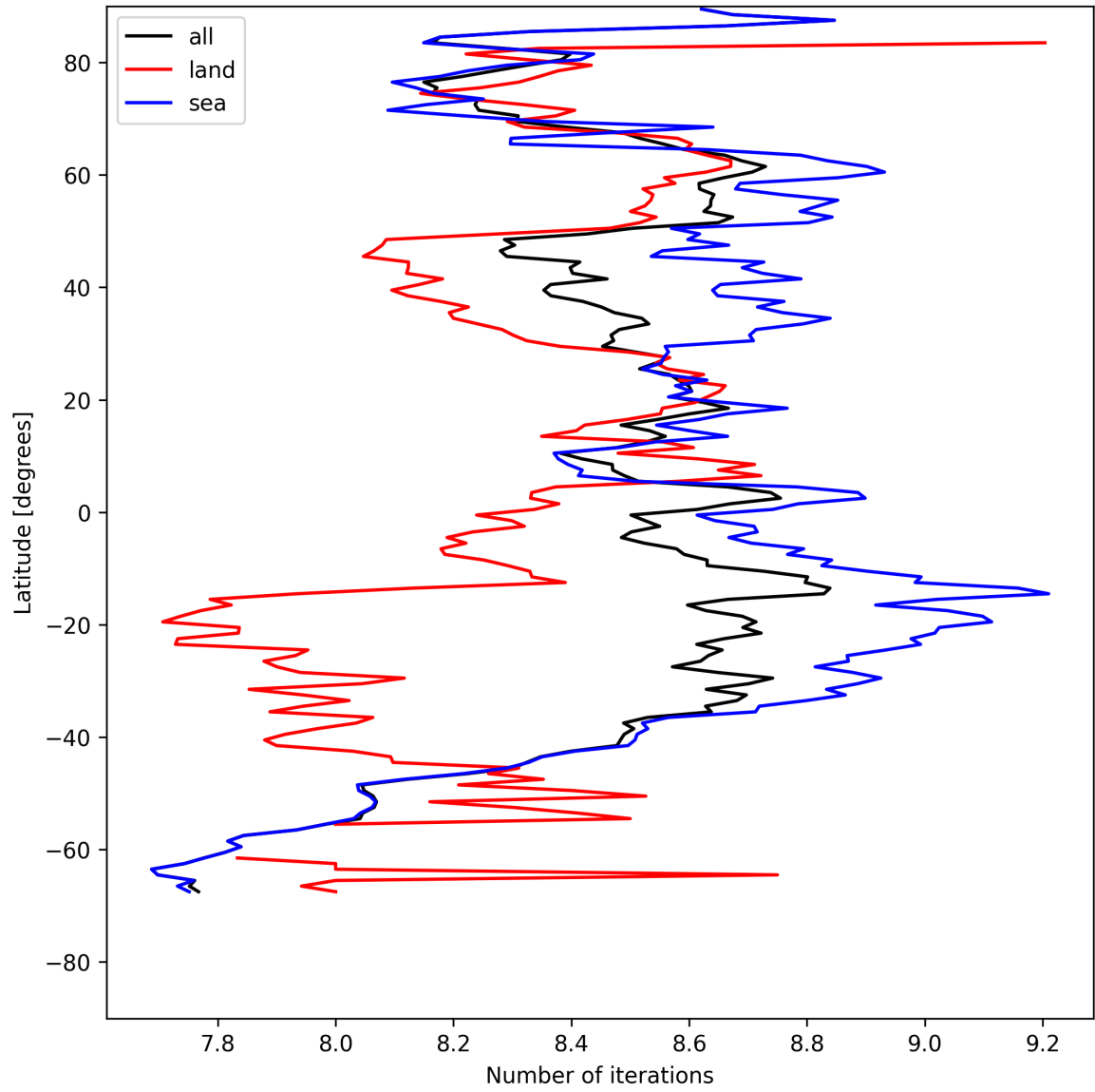
Figure 12: Zonal average of “Number of iterations” for 2025-08-05 to 2025-08-06.
