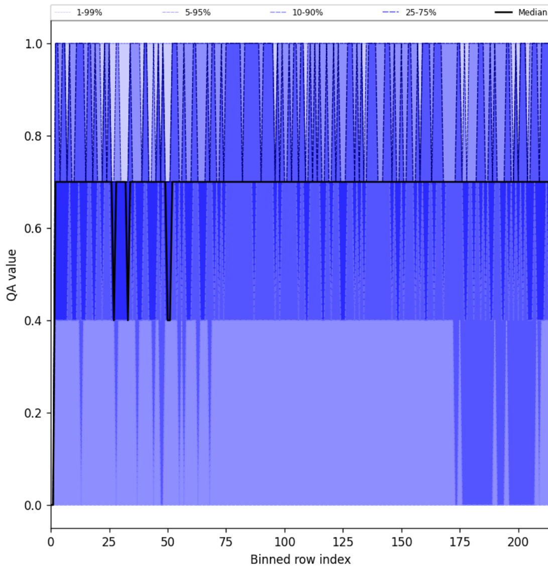
Figure 20: Along track statistics of “QA value” for 2025-08-05 to 2025-08-06
