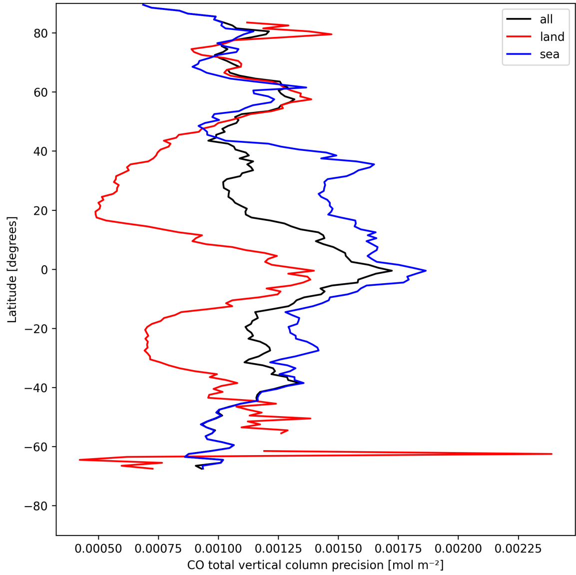
Figure 8: Zonal average of “CO total vertical column precision” for 2025-08-05 to 2025-08-06.
