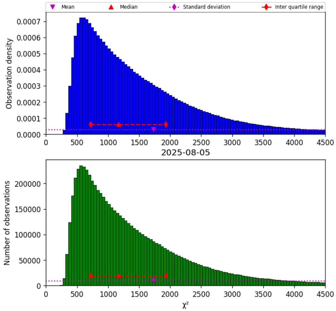
Figure 17: Histogram of “ \chi^2 ” for 2025-08-05 to 2025-08-06
