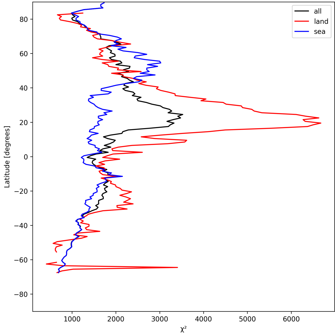
Figure 10: Zonal average of “ \chi^2 ” for 2025-08-05 to 2025-08-06.
