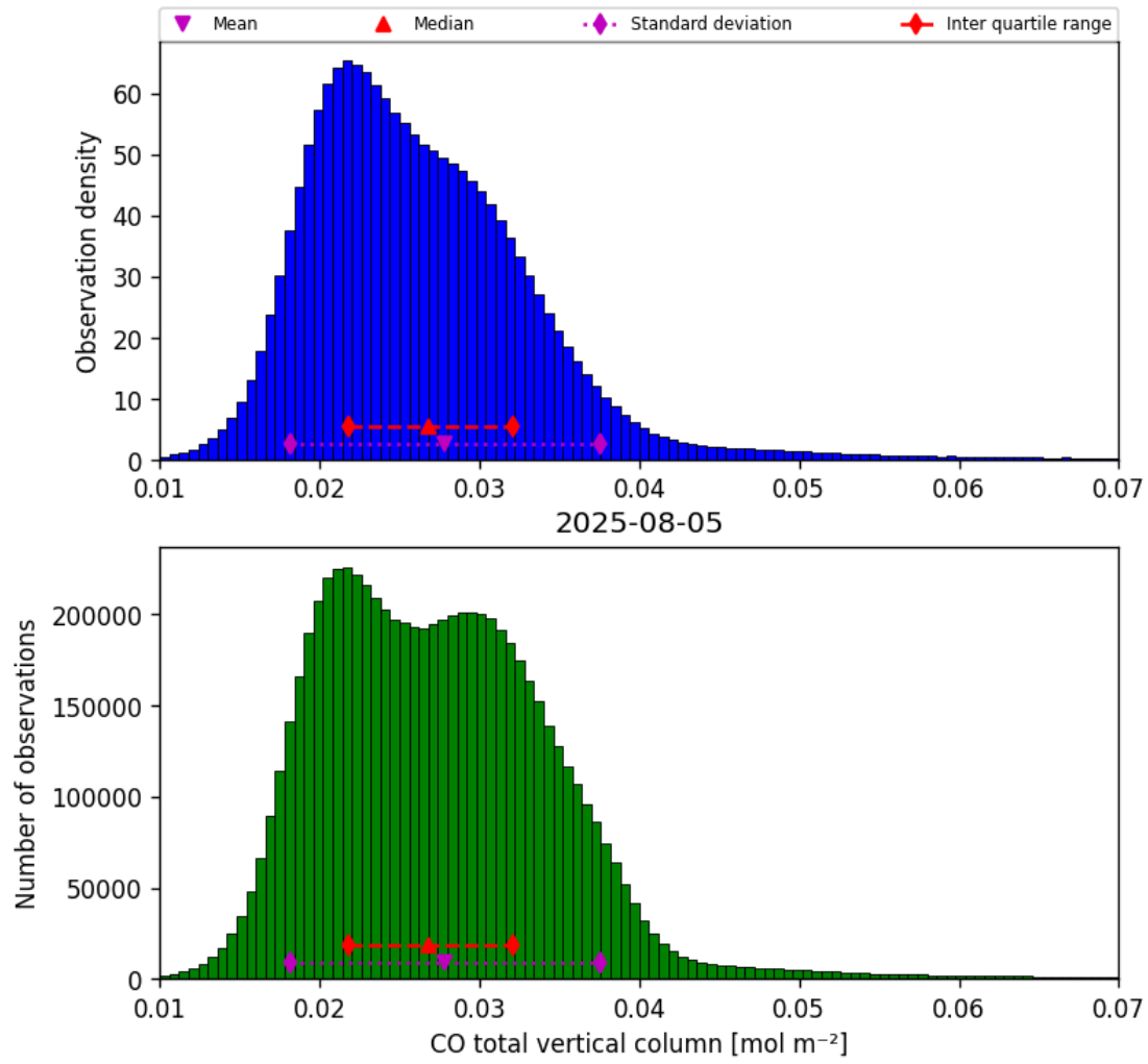
Figure 14: Histogram of “CO total vertical column” for 2025-08-05 to 2025-08-06
