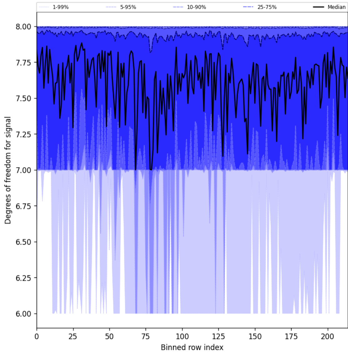
Figure 25: Along track statistics of “Degrees of freedom for signal” for 2025-08-05 to 2025-08-06
