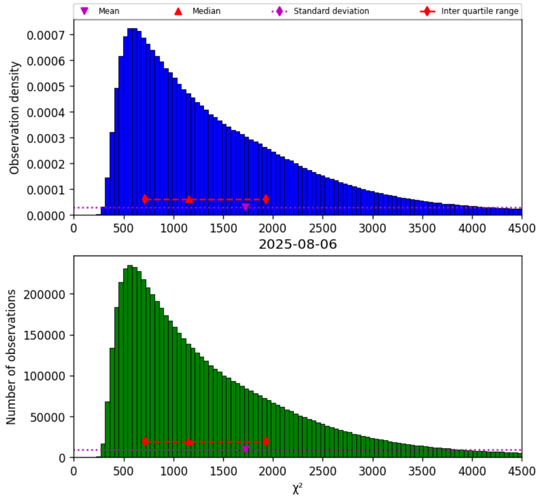
Figure 17: Histogram of " \chi^2 " for 2025-08-06 to 2025-08-07
