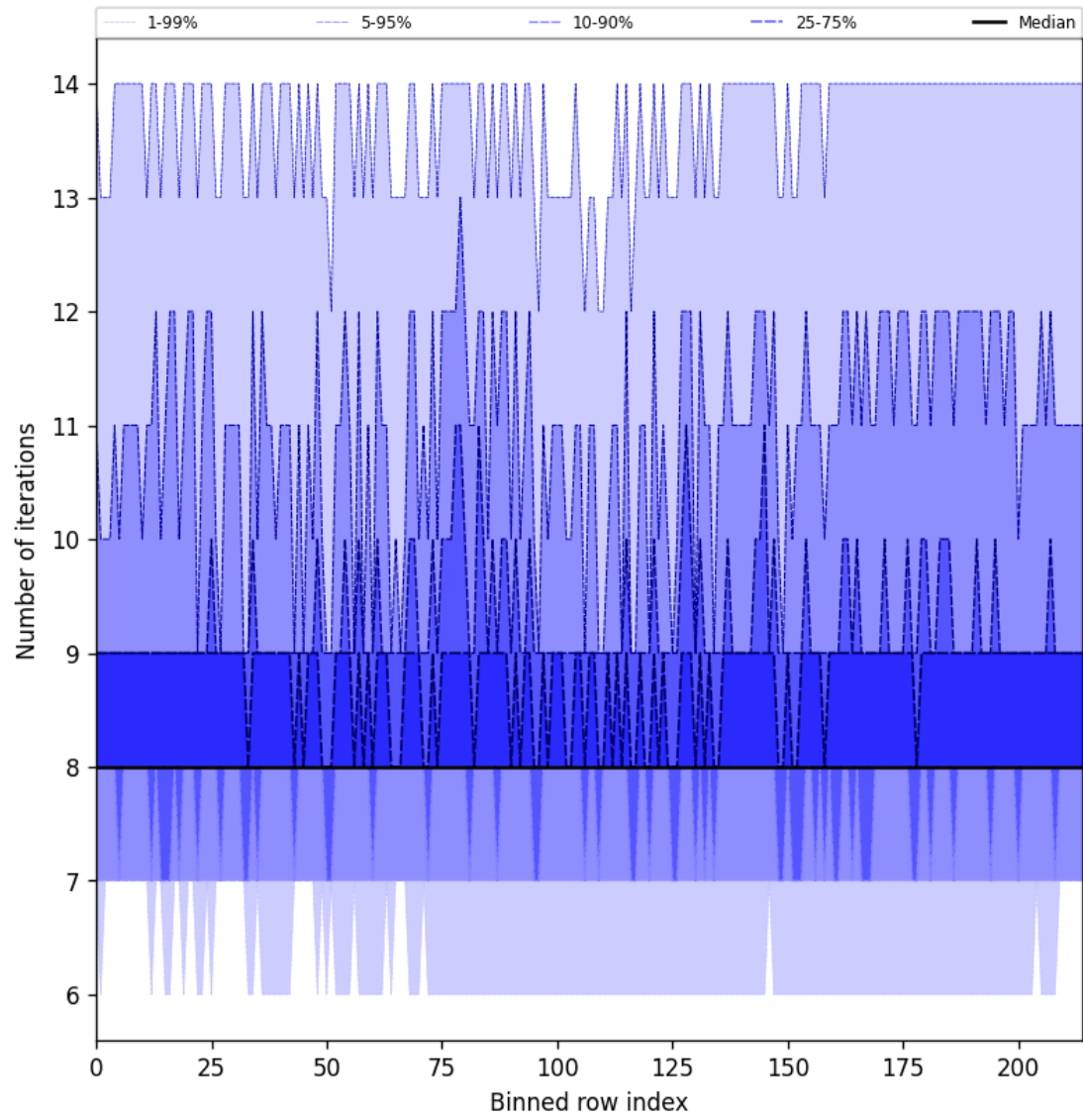
Figure 26: Along track statistics of “Number of iterations” for 2025-08-06 to 2025-08-07
