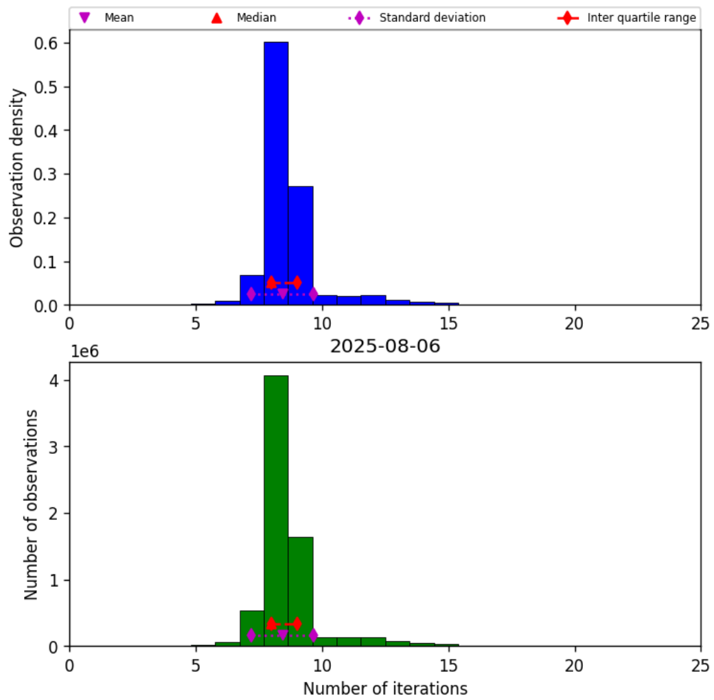
Figure 19: Histogram of “Number of iterations” for 2025-08-06 to 2025-08-07
