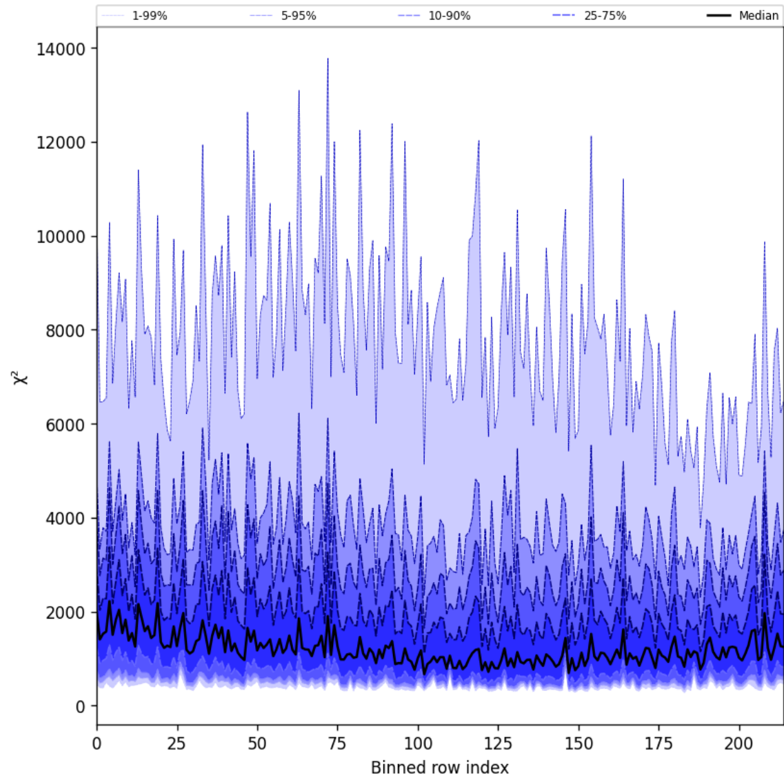
Figure 24: Along track statistics of “ \chi^2 ” for 2025-08-06 to 2025-08-07
