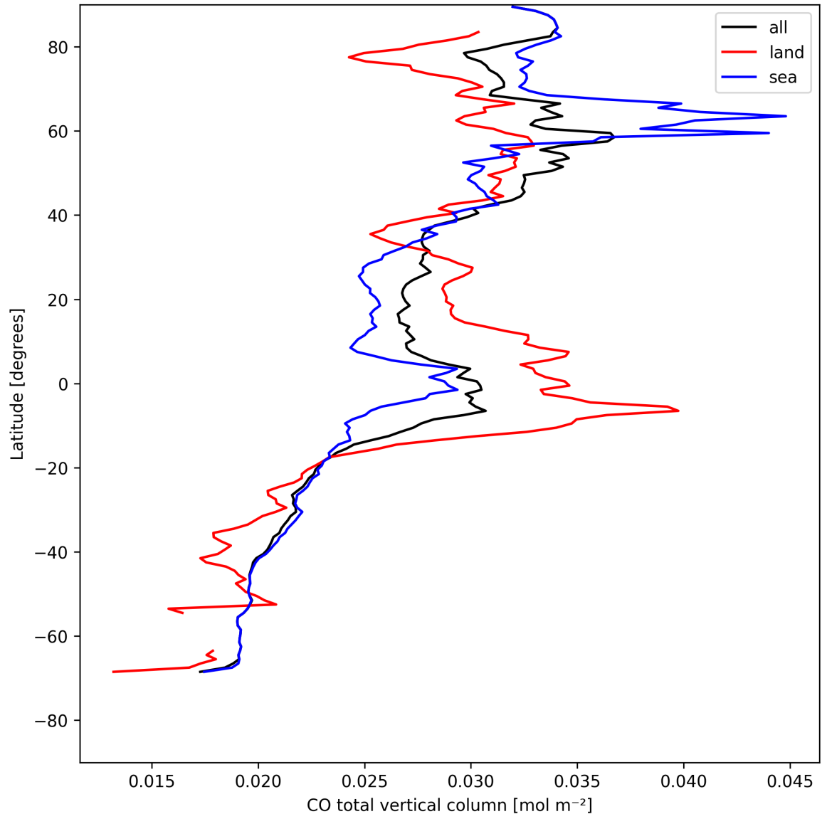
Figure 7: Zonal average of “CO total vertical column” for 2025-08-06 to 2025-08-07.
