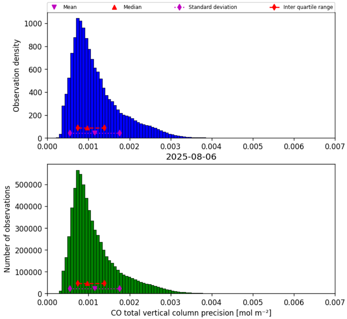
Figure 15: Histogram of “CO total vertical column precision” for 2025-08-06 to 2025-08-07
