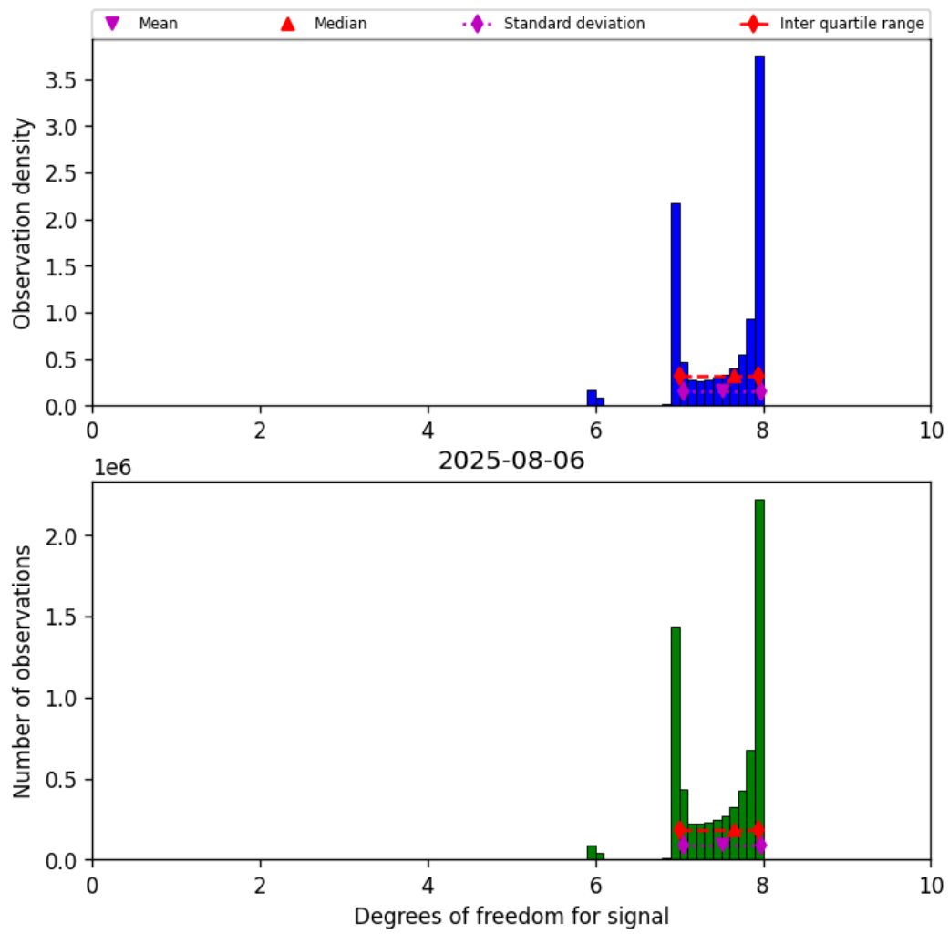
Figure 18: Histogram of “Degrees of freedom for signal” for 2025-08-06 to 2025-08-07
