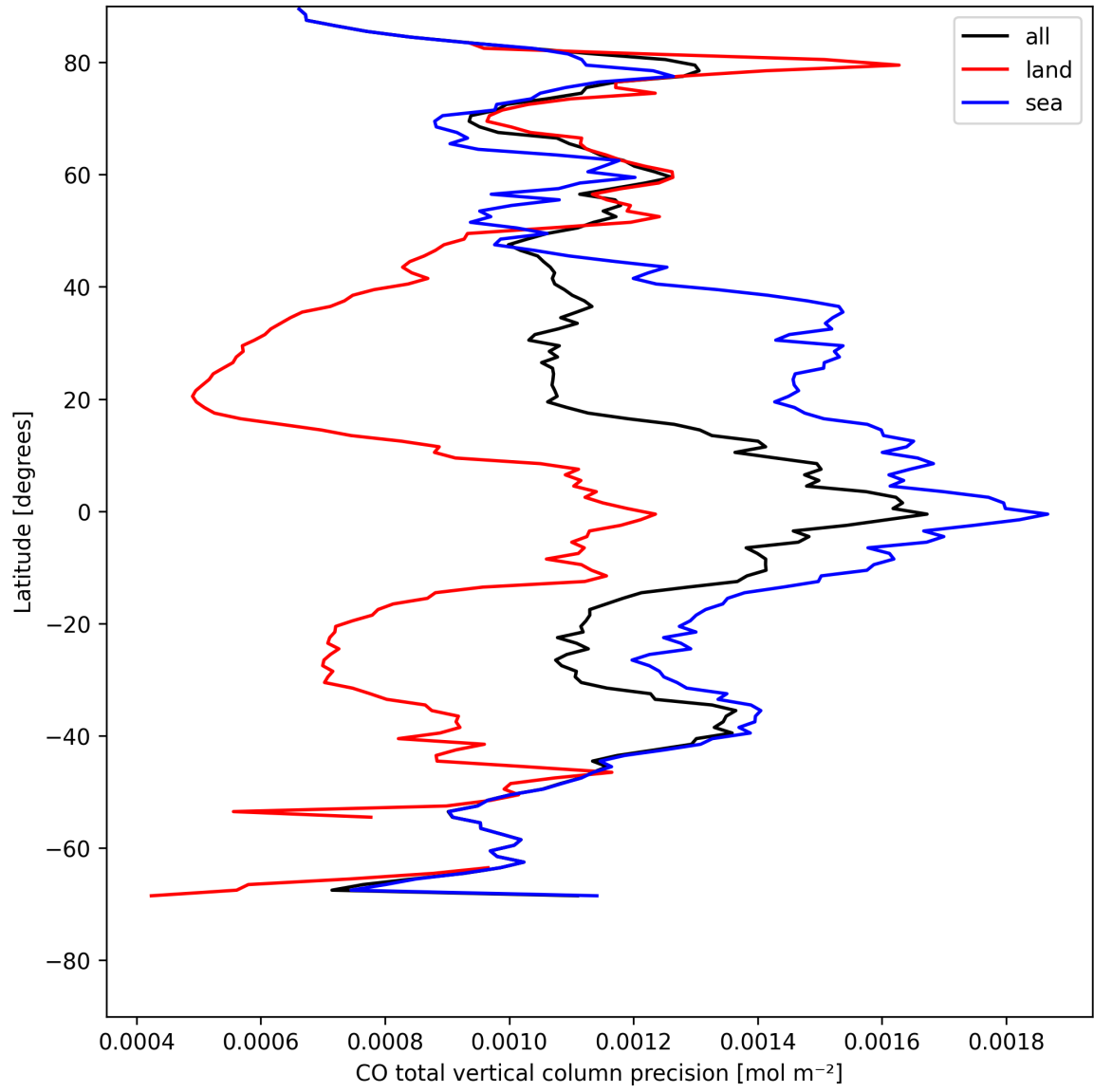
Figure 8: Zonal average of “CO total vertical column precision” for 2025-08-06 to 2025-08-07.
