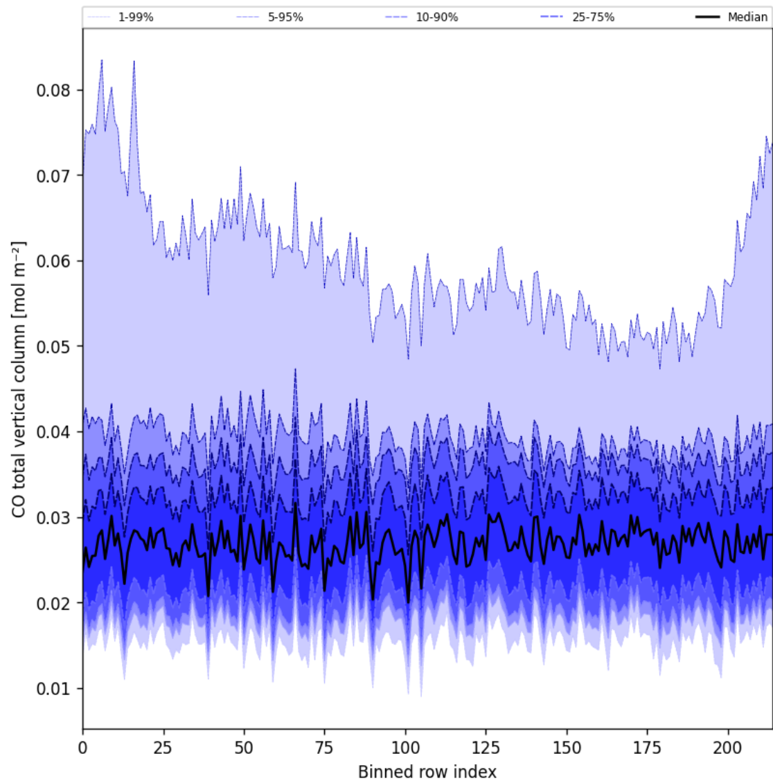
Figure 21: Along track statistics of “CO total vertical column” for 2025-08-06 to 2025-08-07
