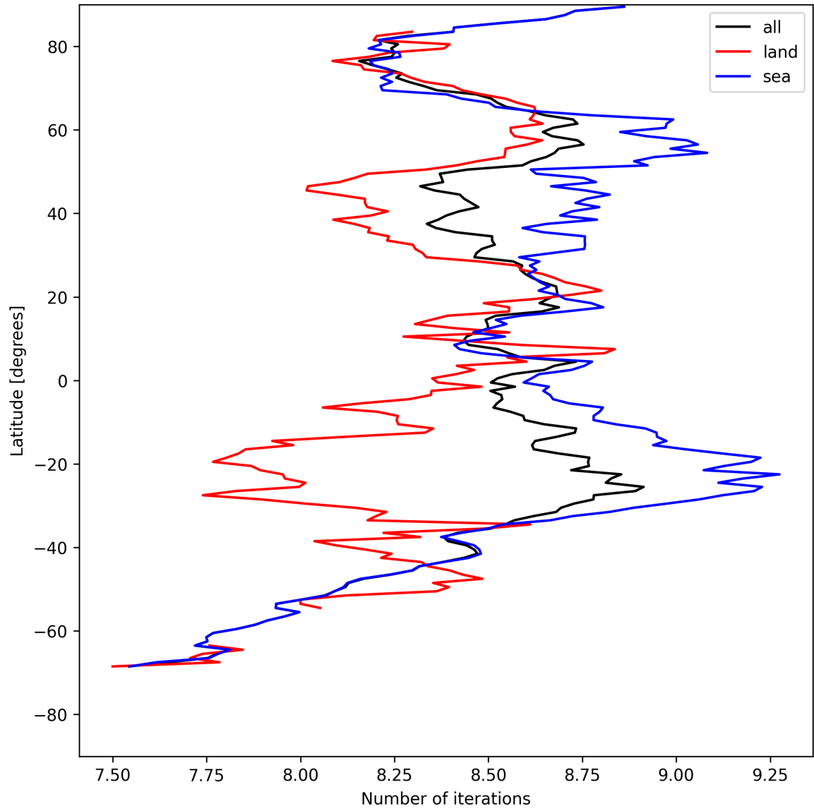
Figure 12: Zonal average of “Number of iterations” for 2025-08-06 to 2025-08-07.
