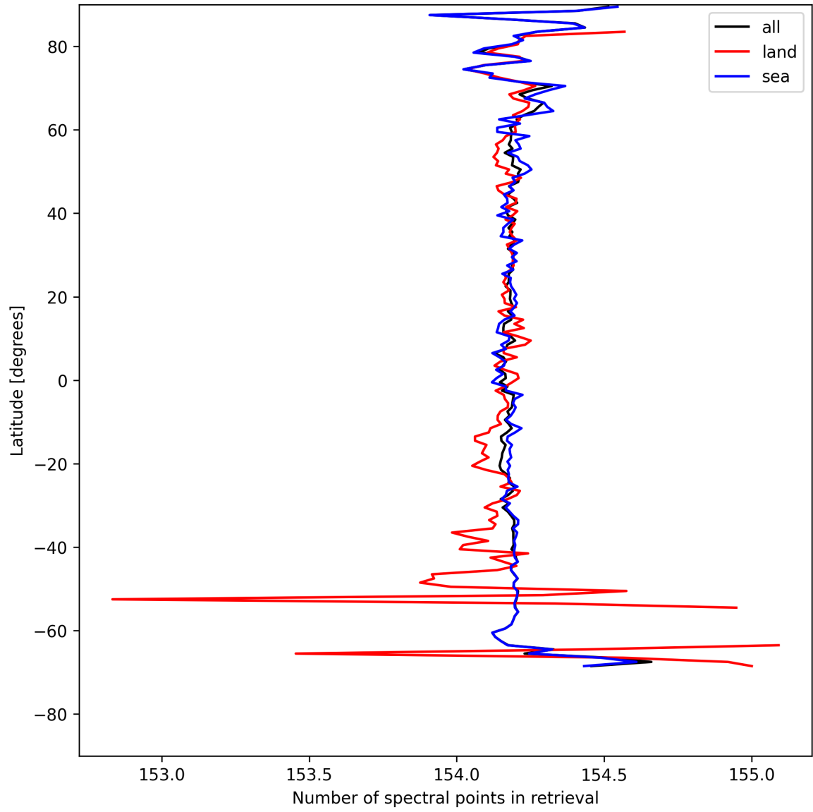
Figure 9: Zonal average of “Number of spectral points in retrieval” for 2025-08-06 to 2025-08-07.
