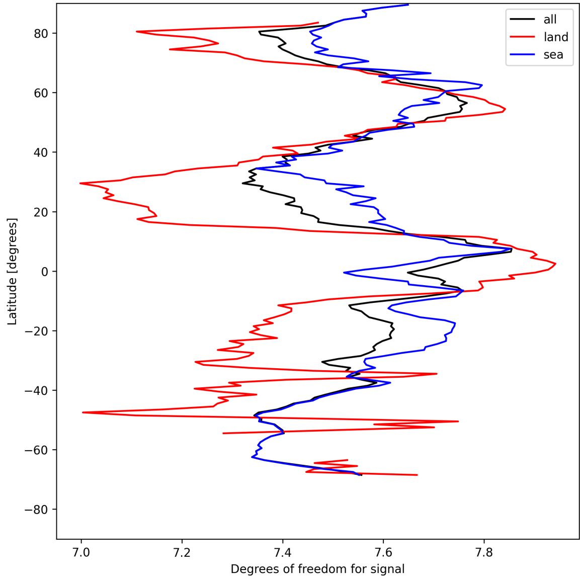
Figure 11: Zonal average of “Degrees of freedom for signal” for 2025-08-06 to 2025-08-07.
