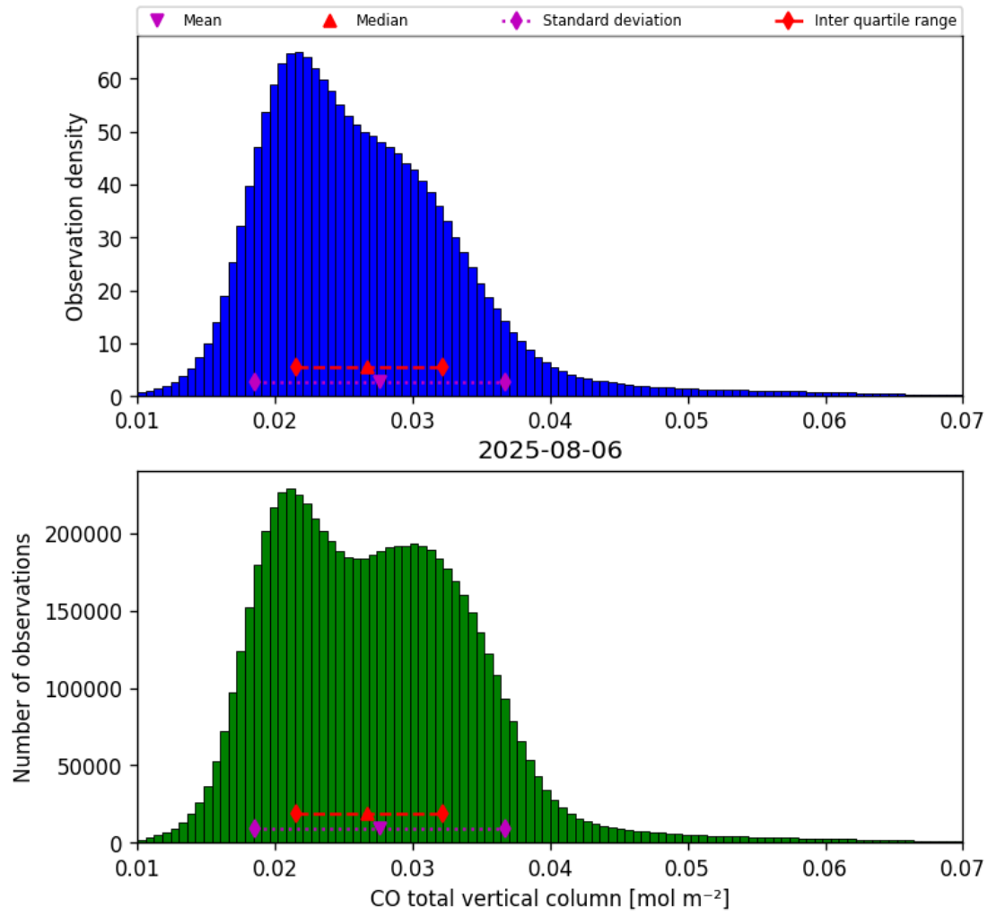
Figure 14: Histogram of “CO total vertical column” for 2025-08-06 to 2025-08-07
