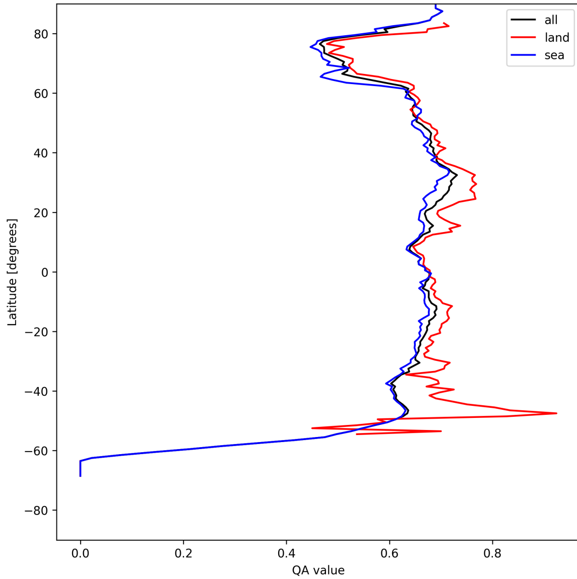
Figure 6: Zonal average of “QA value” for 2025-08-06 to 2025-08-07.
