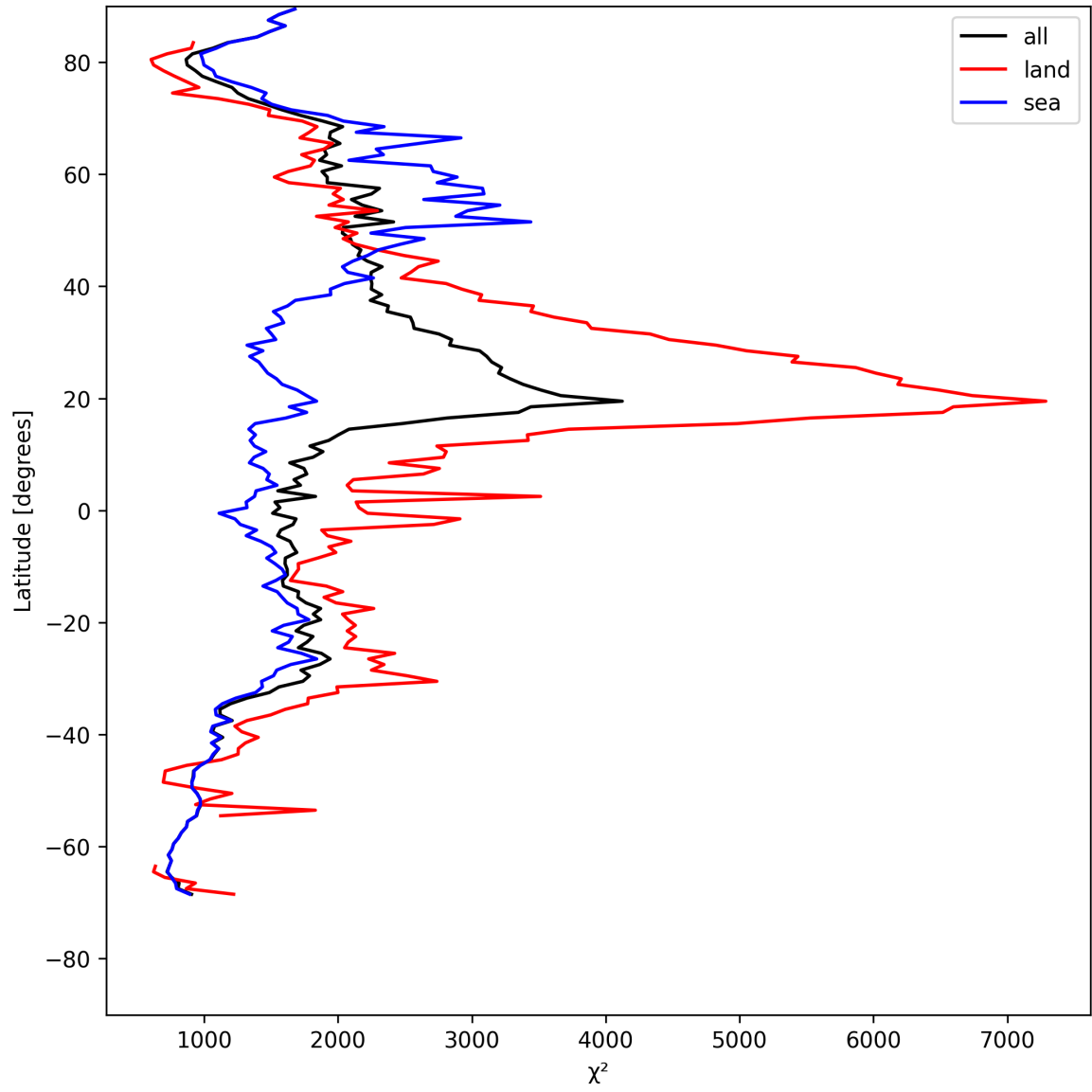
Figure 10: Zonal average of “ \chi^2 ” for 2025-08-06 to 2025-08-07.
