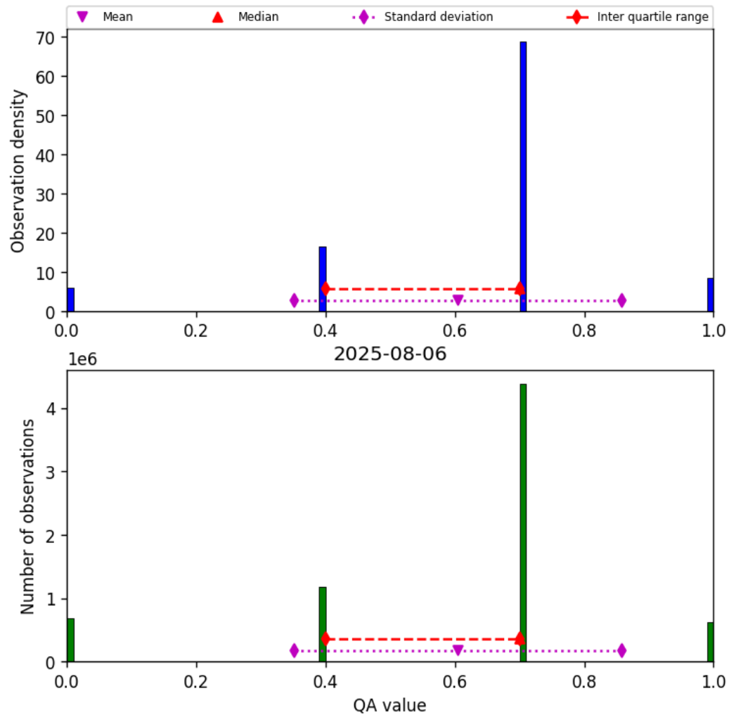
Figure 13: Histogram of “QA value” for 2025-08-06 to 2025-08-07
