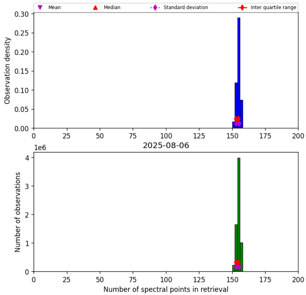
Figure 16: Histogram of “Number of spectral points in retrieval” for 2025-08-06 to 2025-08-07
