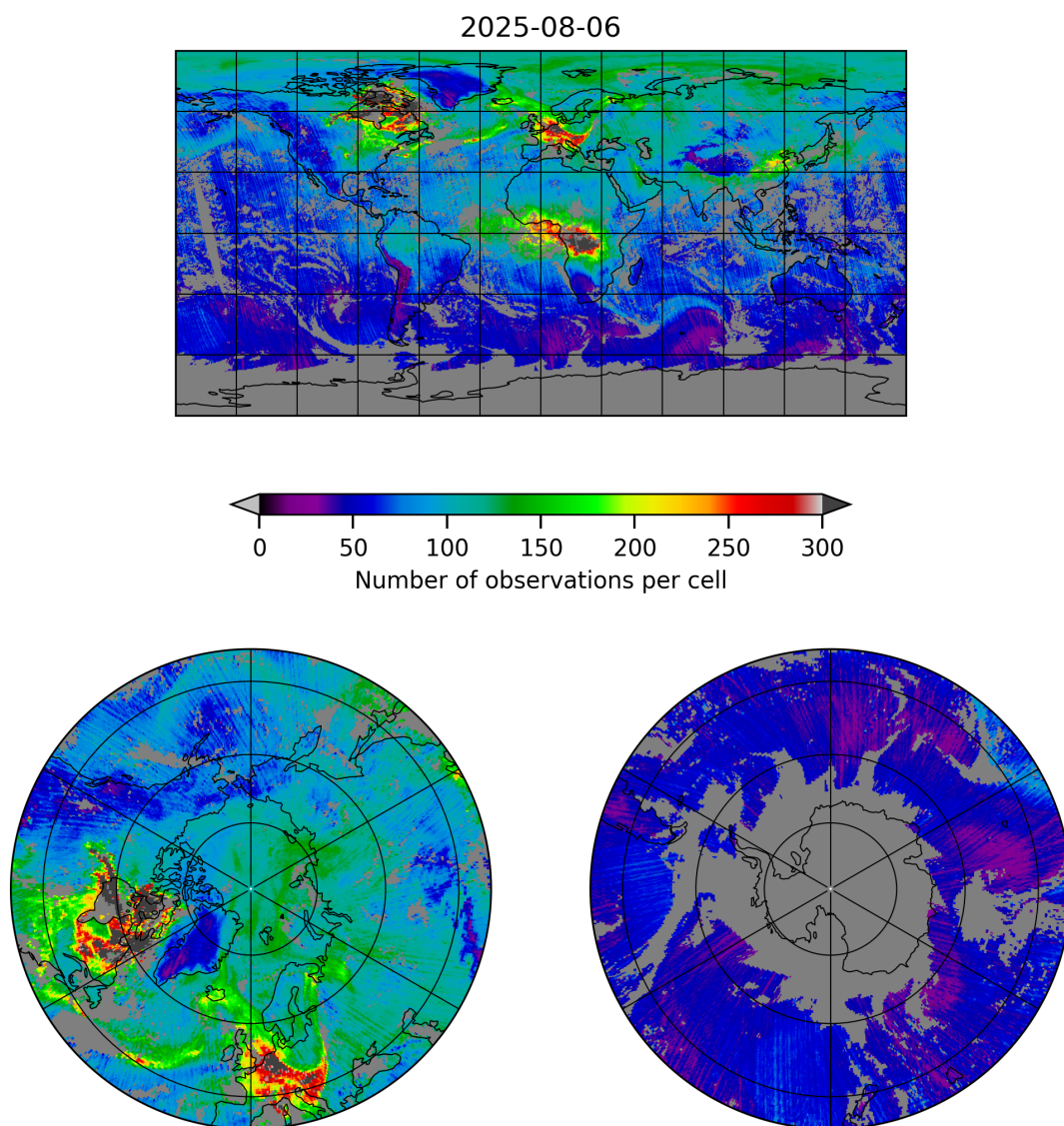
Figure 5: Map of the number of observations for 2025-08-06 to 2025-08-07
