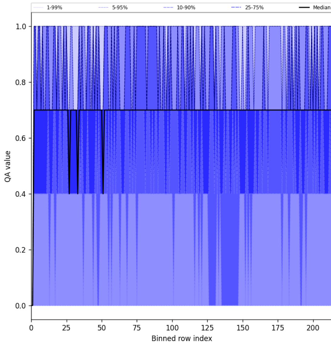
Figure 20: Along track statistics of “QA value” for 2025-08-06 to 2025-08-07
