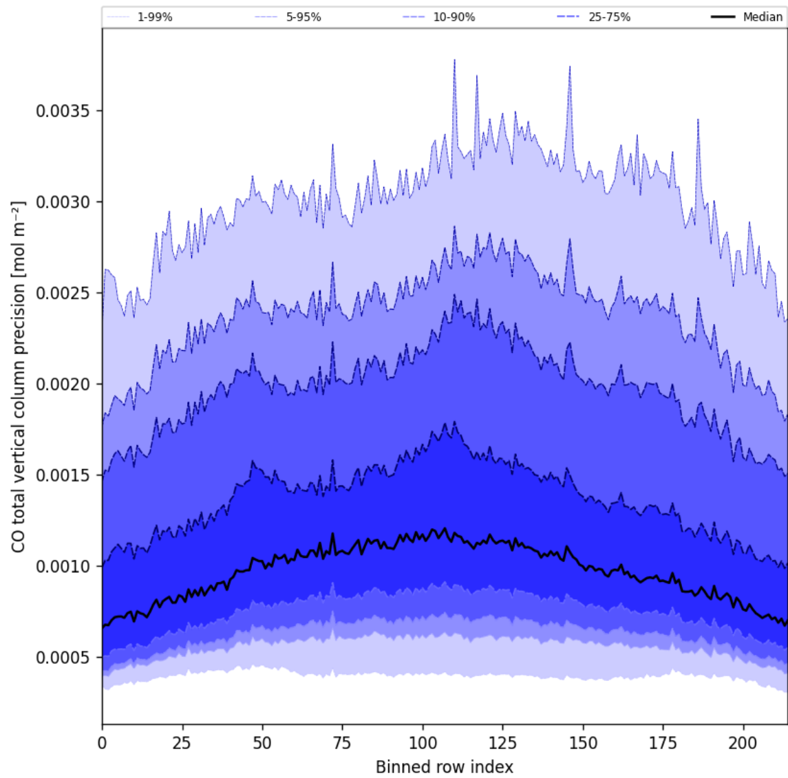
Figure 22: Along track statistics of “CO total vertical column precision” for 2025-08-06 to 2025-08-07
