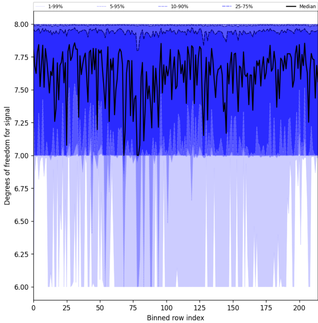
Figure 25: Along track statistics of “Degrees of freedom for signal” for 2025-08-06 to 2025-08-07
