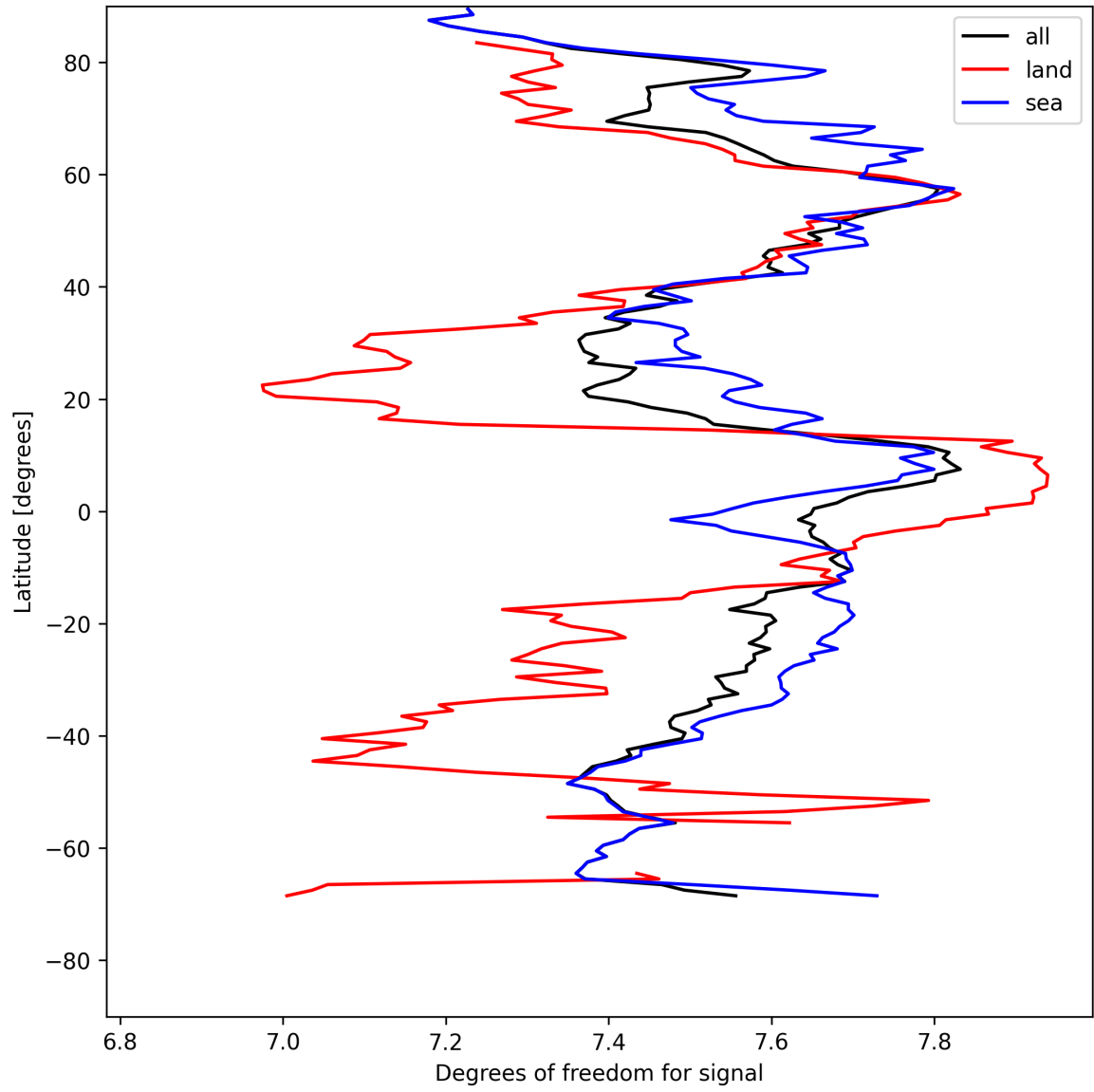
Figure 11: Zonal average of “Degrees of freedom for signal” for 2025-08-07 to 2025-08-07.
