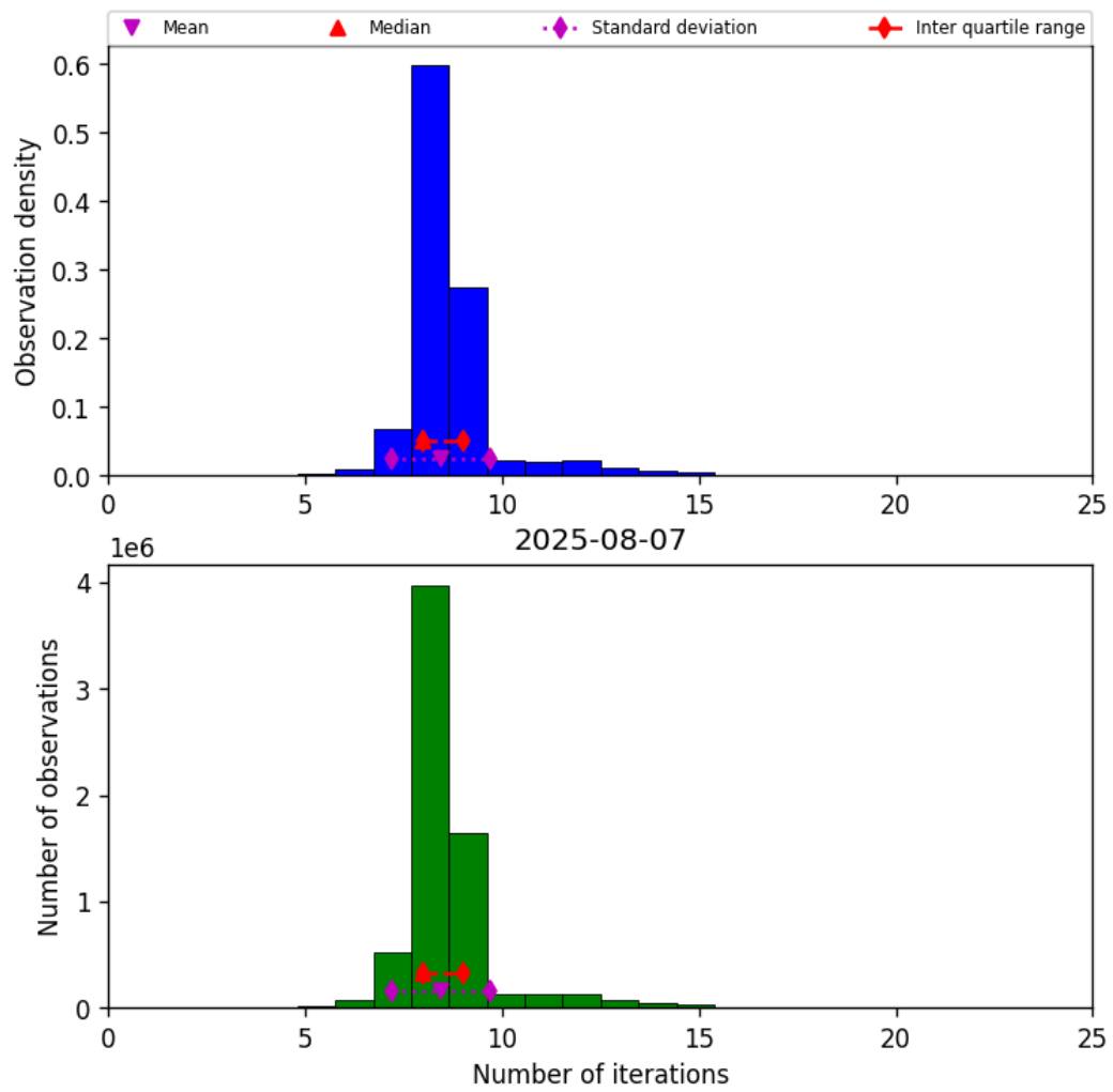
Figure 19: Histogram of “Number of iterations” for 2025-08-07 to 2025-08-07
