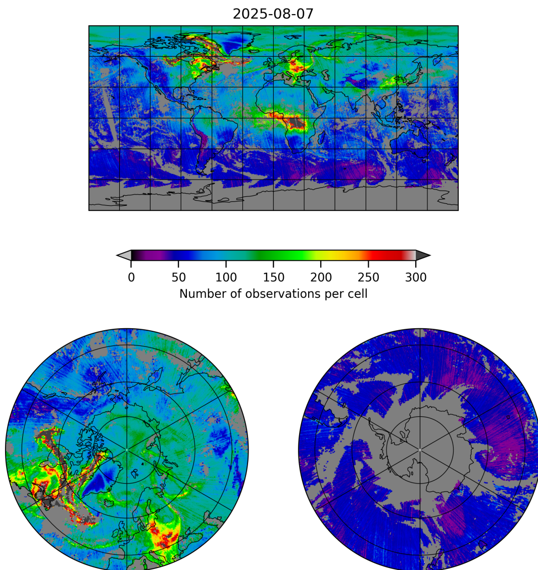
Figure 5: Map of the number of observations for 2025-08-07 to 2025-08-07
