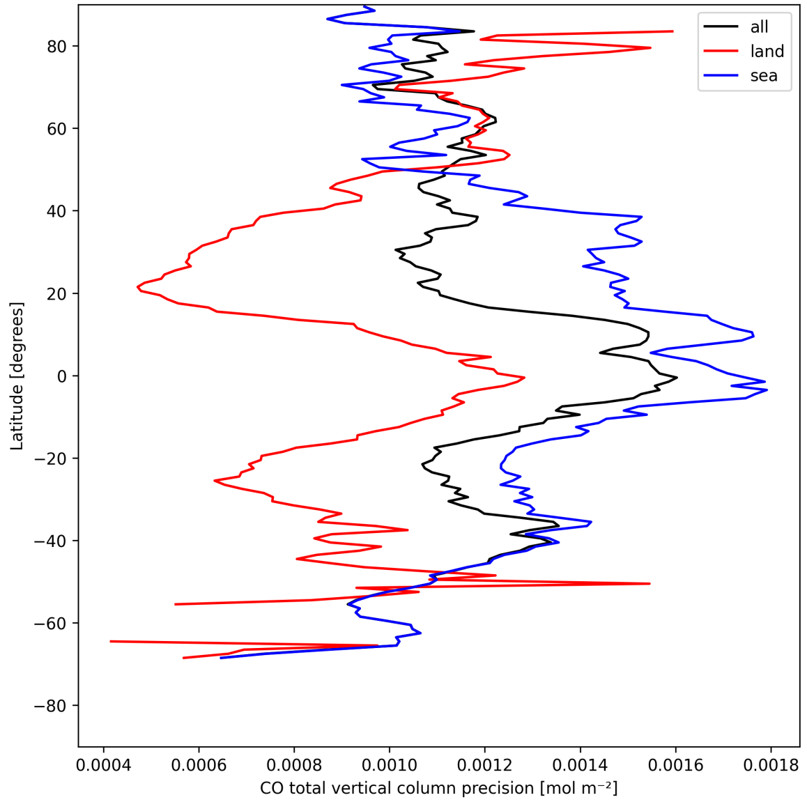
Figure 8: Zonal average of “CO total vertical column precision” for 2025-08-07 to 2025-08-07.
