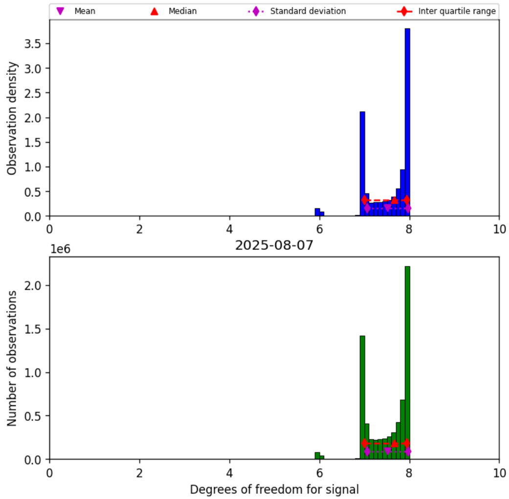
Figure 18: Histogram of “Degrees of freedom for signal” for 2025-08-07 to 2025-08-07
