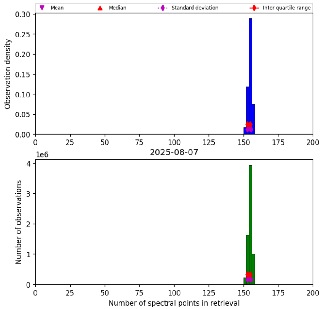
Figure 16: Histogram of “Number of spectral points in retrieval” for 2025-08-07 to 2025-08-07
