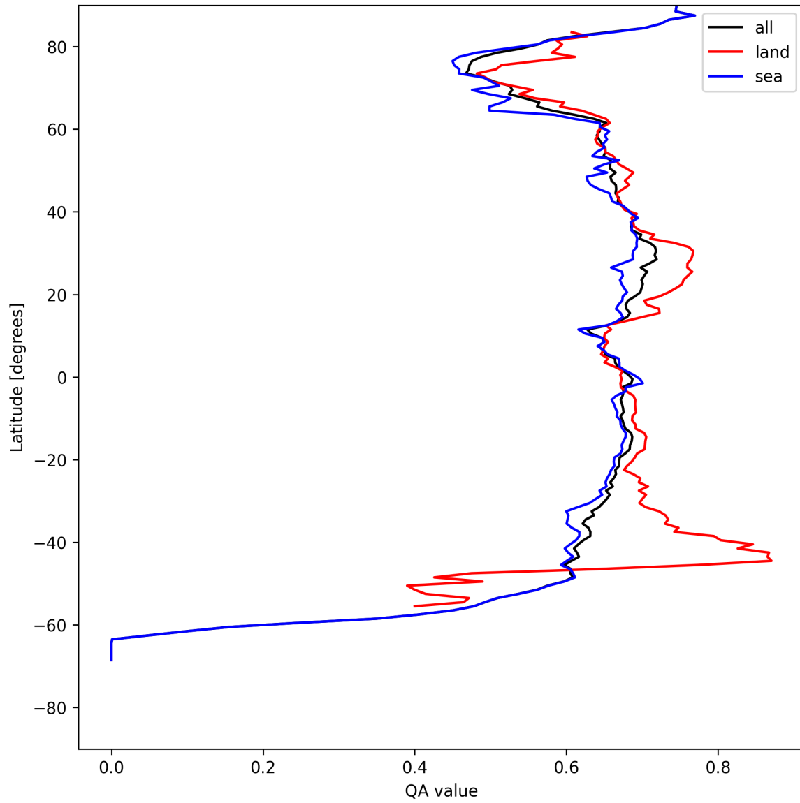
Figure 6: Zonal average of “QA value” for 2025-08-07 to 2025-08-07.
