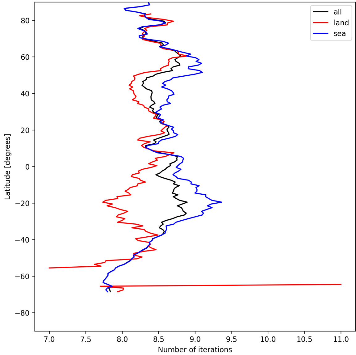
Figure 12: Zonal average of “Number of iterations” for 2025-08-07 to 2025-08-07.
