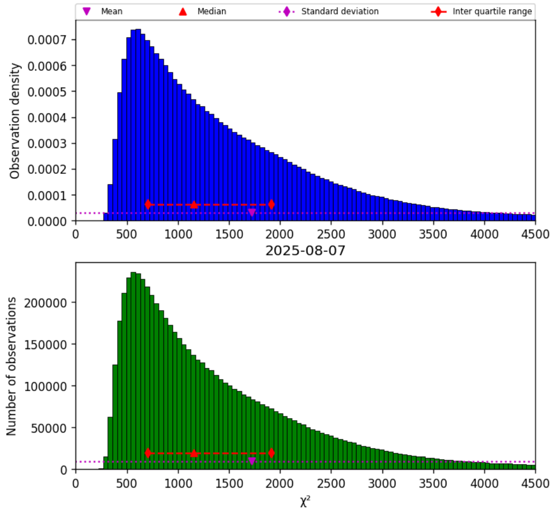
Figure 17: Histogram of “ \chi^2 ” for 2025-08-07 to 2025-08-07
