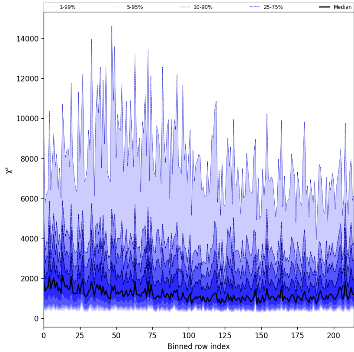
Figure 24: Along track statistics of “ \chi^2 ” for 2025-08-07 to 2025-08-07
