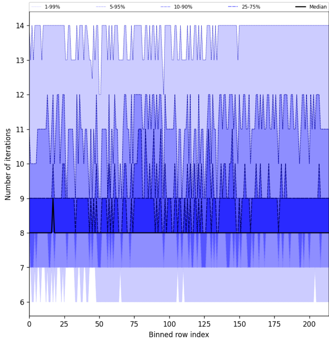
Figure 26: Along track statistics of “Number of iterations” for 2025-08-07 to 2025-08-07
