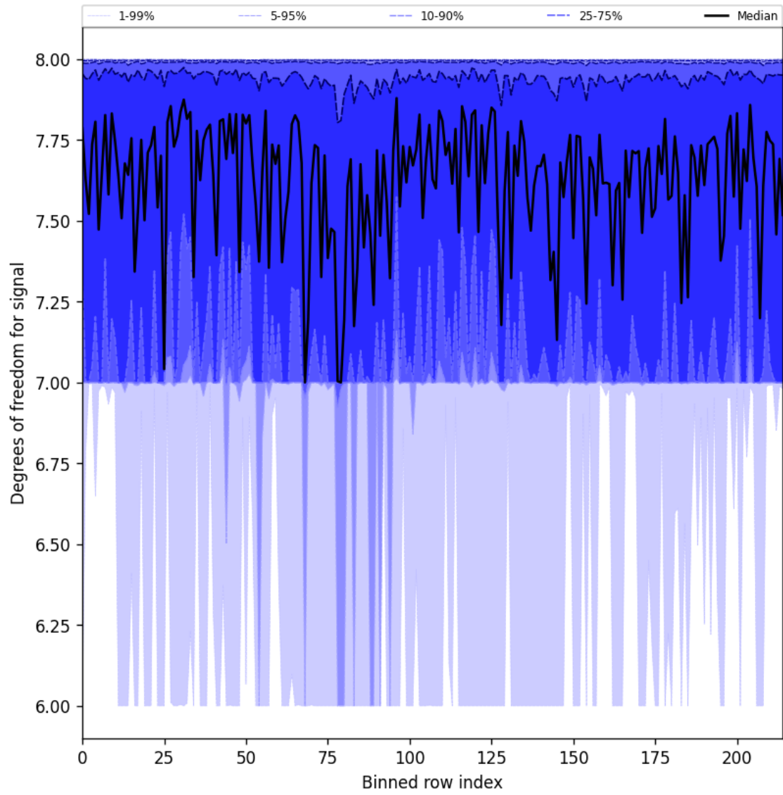
Figure 25: Along track statistics of “Degrees of freedom for signal” for 2025-08-07 to 2025-08-07
