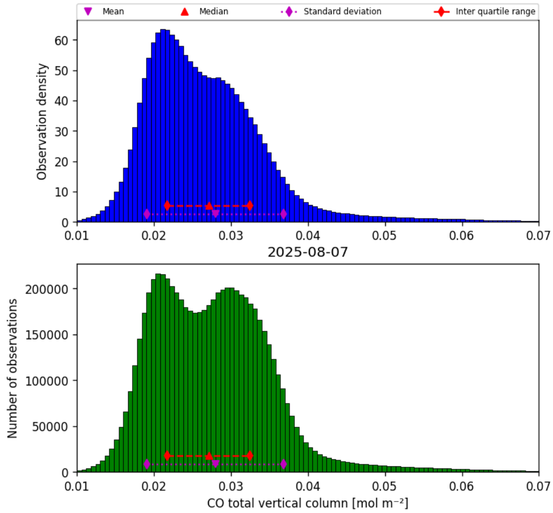
Figure 14: Histogram of “CO total vertical column” for 2025-08-07 to 2025-08-07
