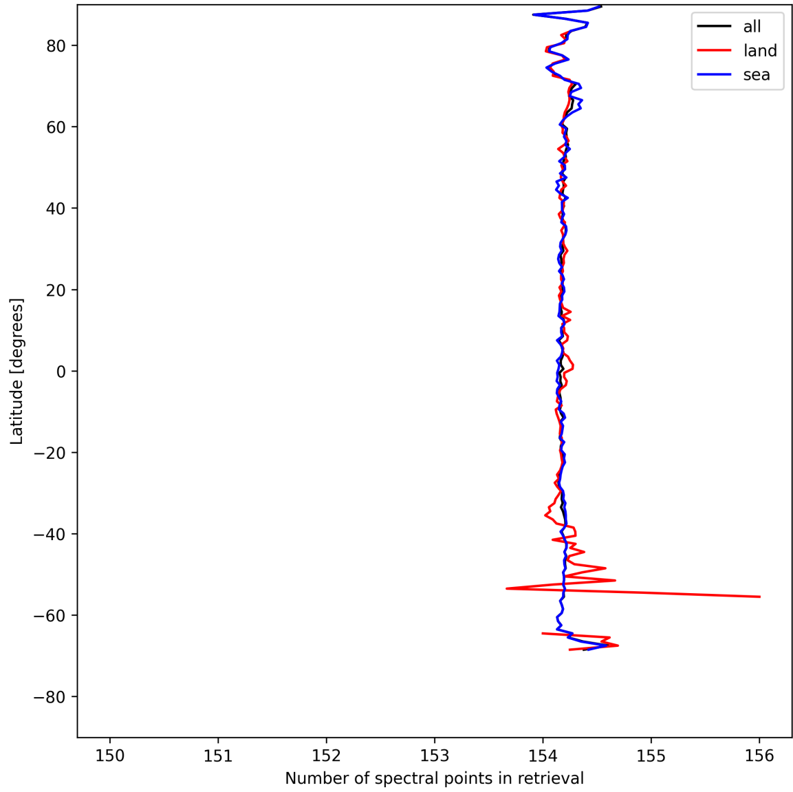
Figure 9: Zonal average of “Number of spectral points in retrieval” for 2025-08-07 to 2025-08-07.
