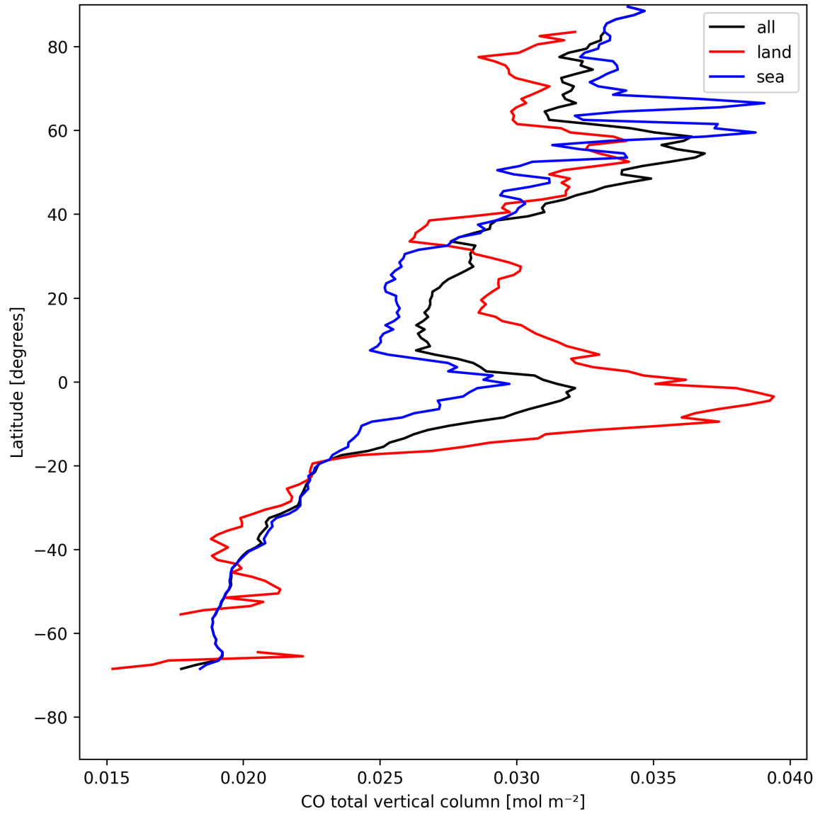
Figure 7: Zonal average of “CO total vertical column” for 2025-08-07 to 2025-08-07.
