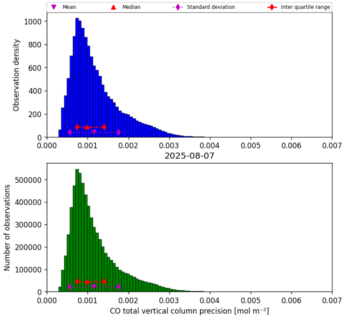
Figure 15: Histogram of “CO total vertical column precision” for 2025-08-07 to 2025-08-07
