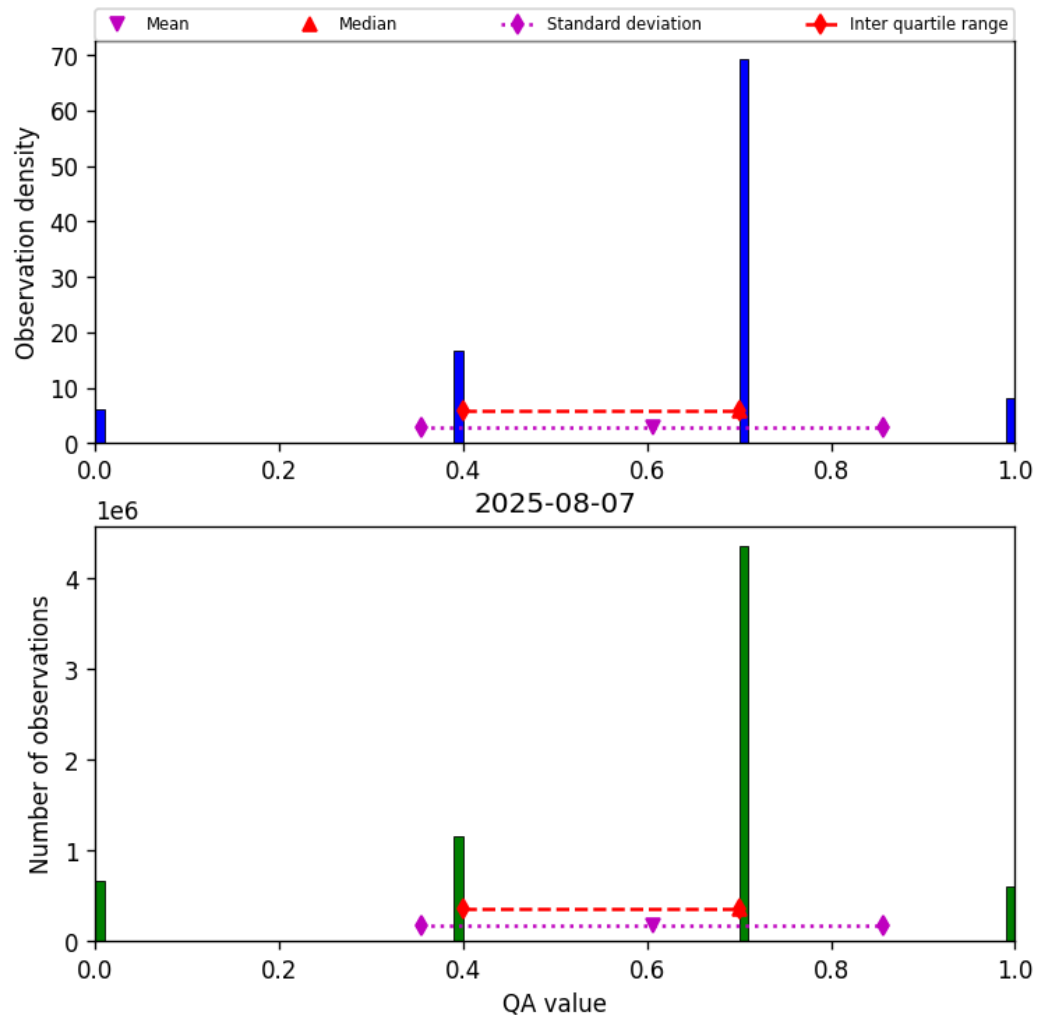
Figure 13: Histogram of “QA value” for 2025-08-07 to 2025-08-07
