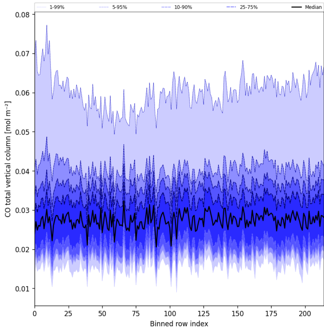
Figure 21: Along track statistics of "CO total vertical column" for 2025-08-07 to 2025-08-07
