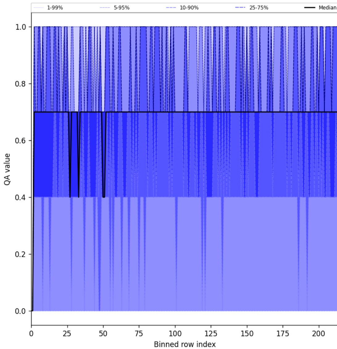
Figure 20: Along track statistics of “QA value” for 2025-08-07 to 2025-08-07
