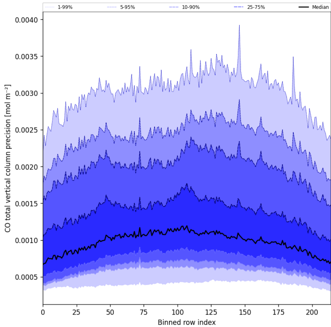
Figure 22: Along track statistics of “CO total vertical column precision” for 2025-08-07 to 2025-08-07
