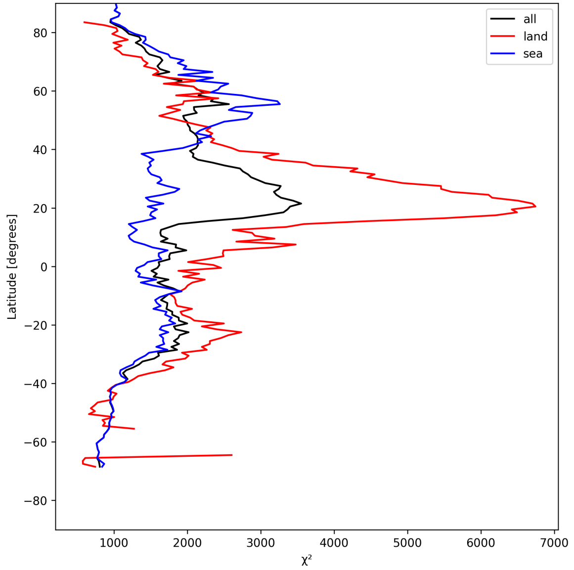
Figure 10: Zonal average of “ \chi^2 ” for 2025-08-07 to 2025-08-07.
