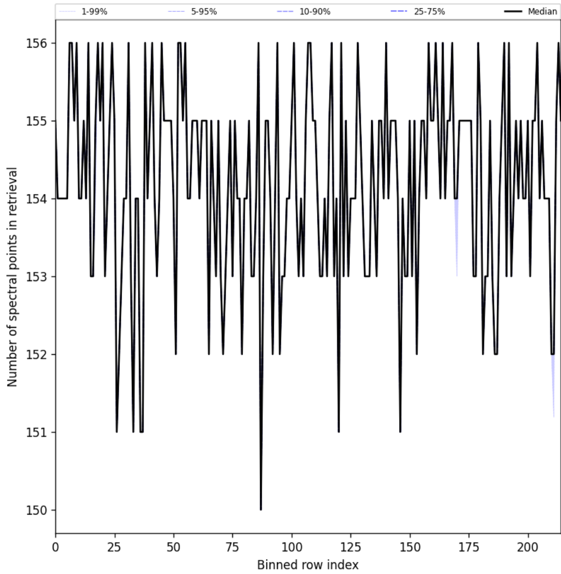
Figure 23: Along track statistics of “Number of spectral points in retrieval” for 2025-08-09 to 2025-08-10
