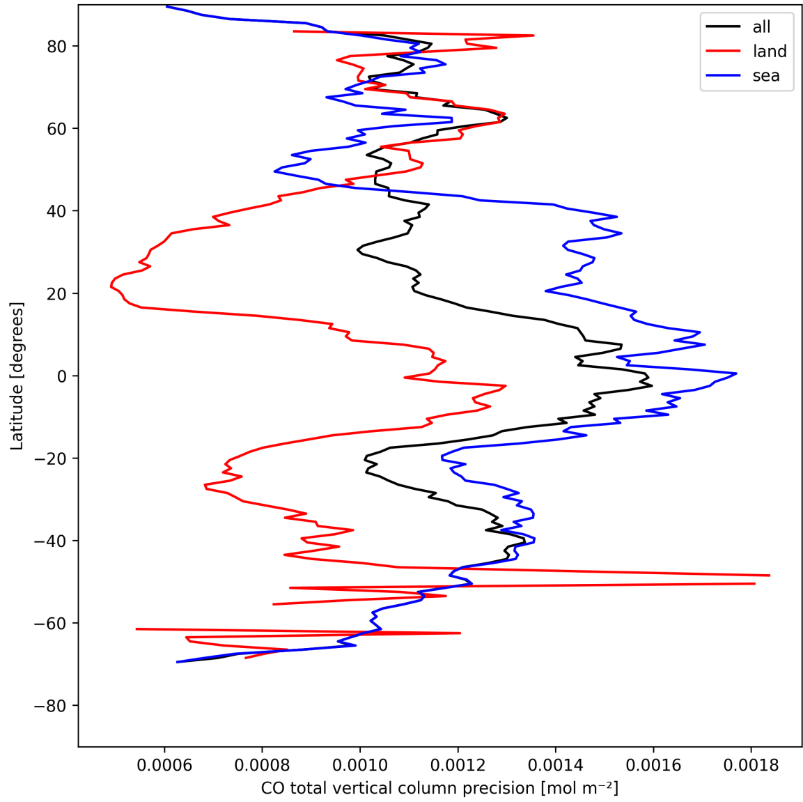
Figure 8: Zonal average of "CO total vertical column precision" for 2025-08-09 to 2025-08-10.
