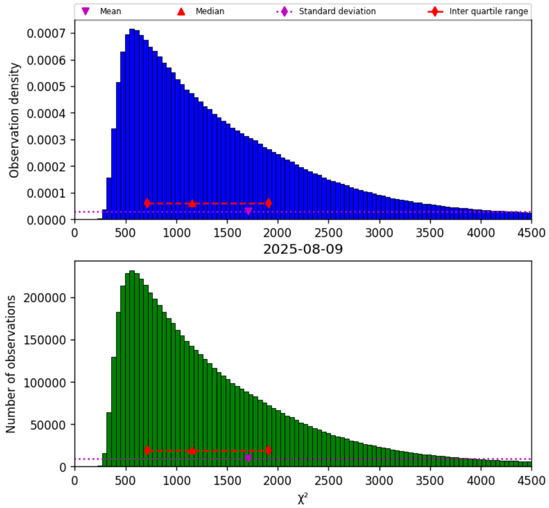
Figure 17: Histogram of “ \chi^2 ” for 2025-08-09 to 2025-08-10
