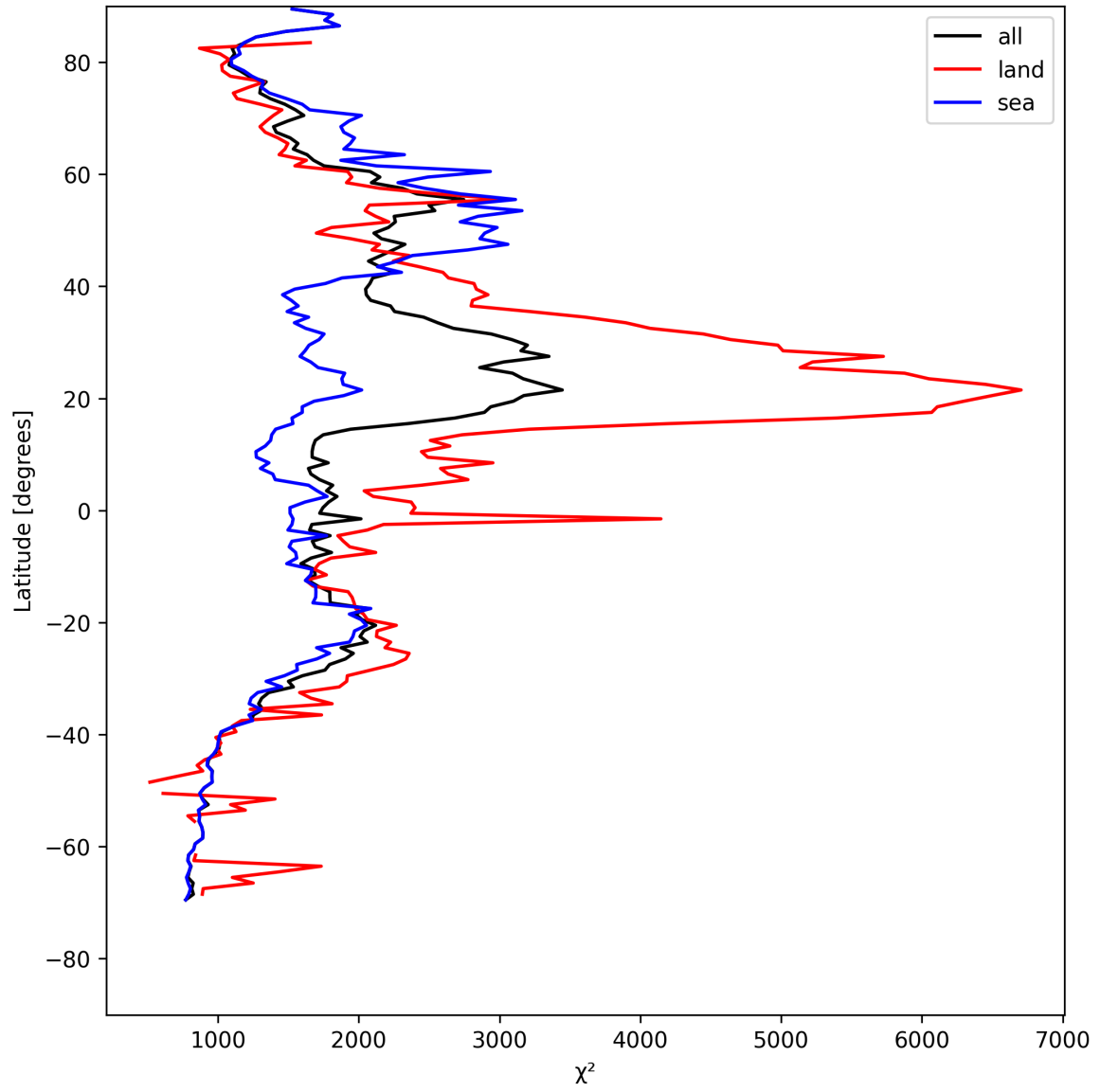
Figure 10: Zonal average of “ \chi^2 ” for 2025-08-09 to 2025-08-10.
