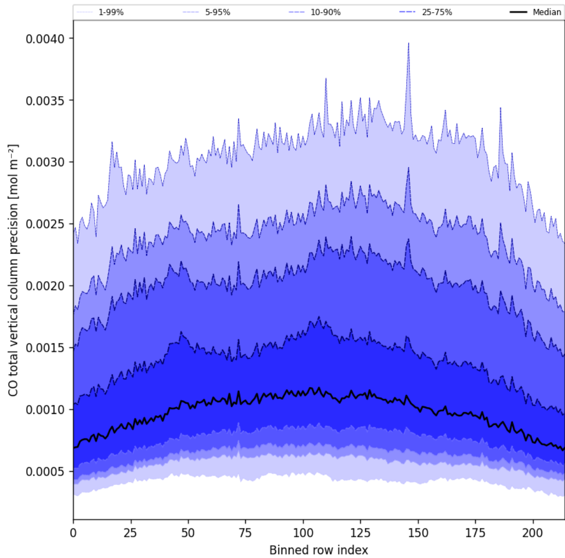
Figure 22: Along track statistics of “CO total vertical column precision” for 2025-08-09 to 2025-08-10
