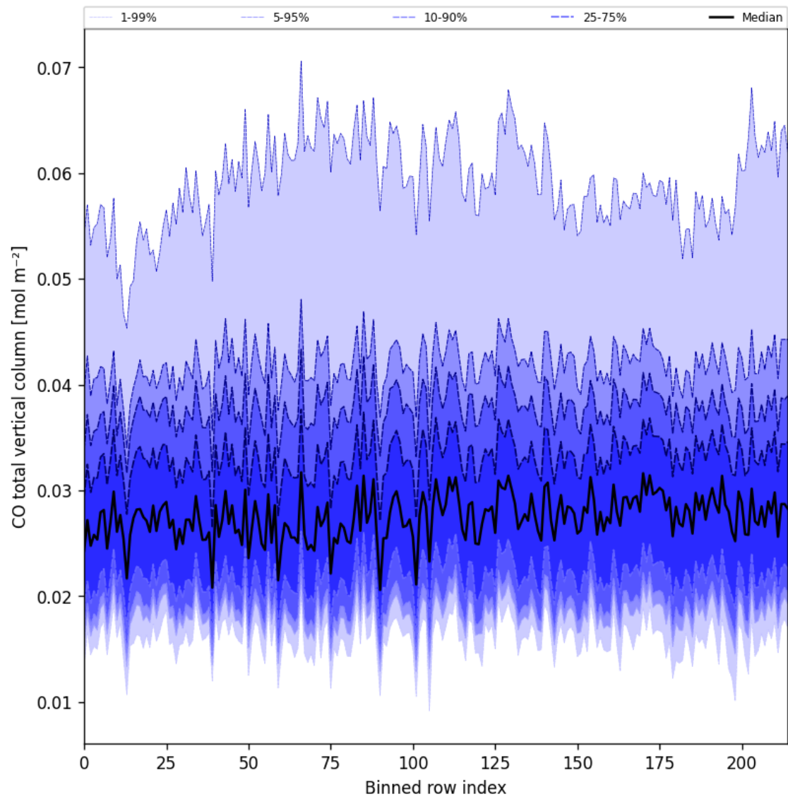
Figure 21: Along track statistics of “CO total vertical column” for 2025-08-09 to 2025-08-10
