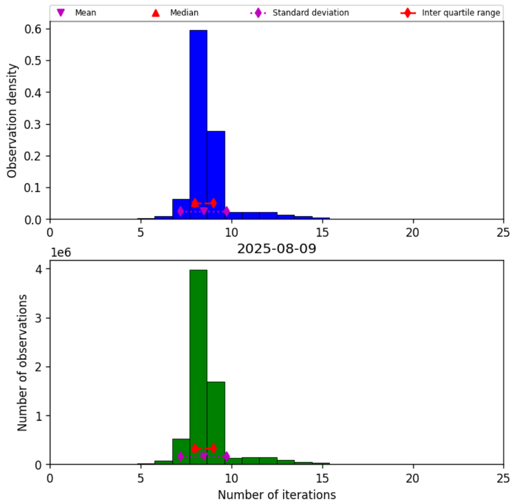
Figure 19: Histogram of “Number of iterations” for 2025-08-09 to 2025-08-10
