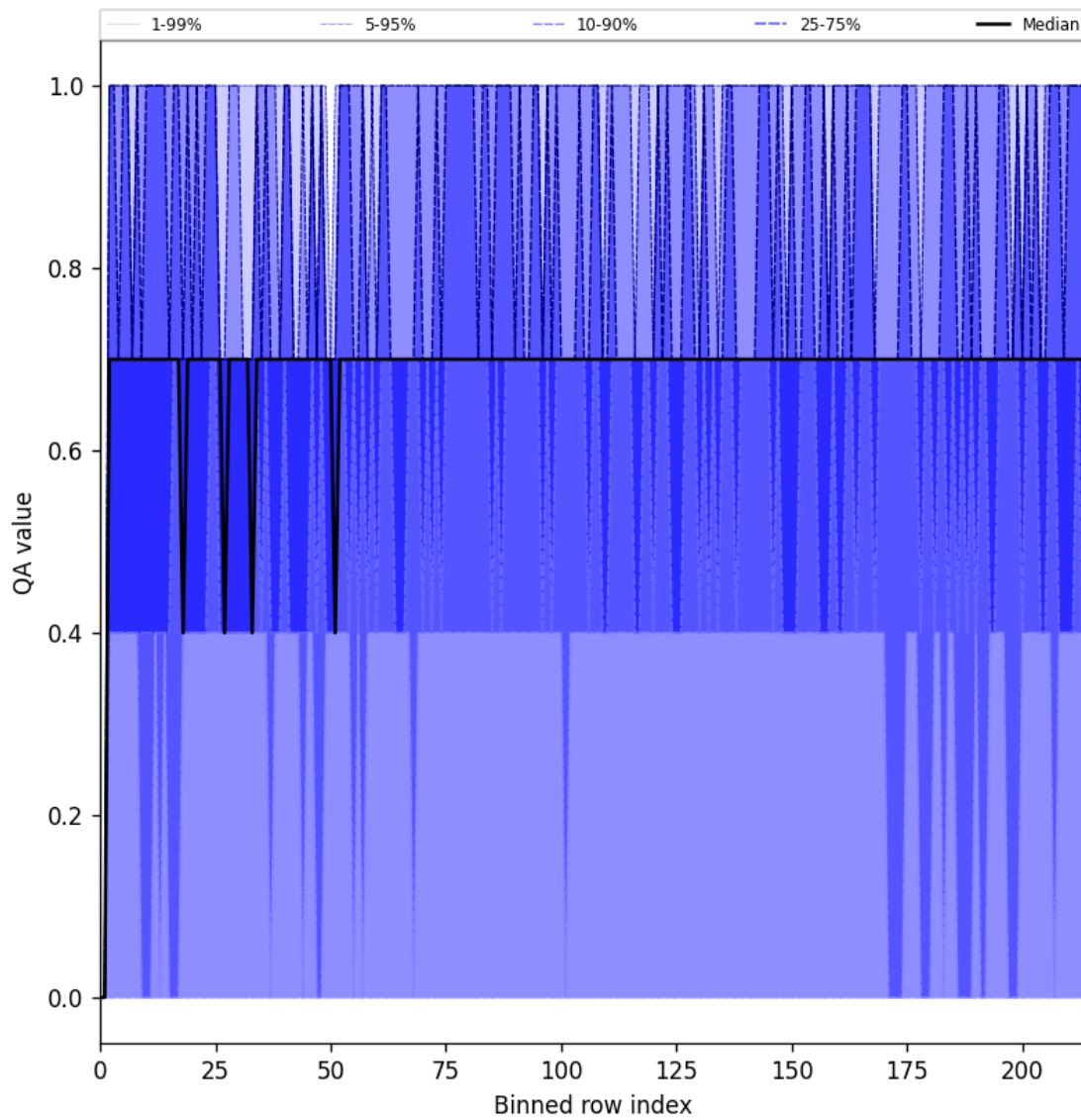
Figure 20: Along track statistics of “QA value” for 2025-08-09 to 2025-08-10
