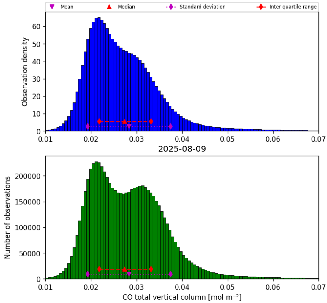
Figure 14: Histogram of “CO total vertical column” for 2025-08-09 to 2025-08-10
