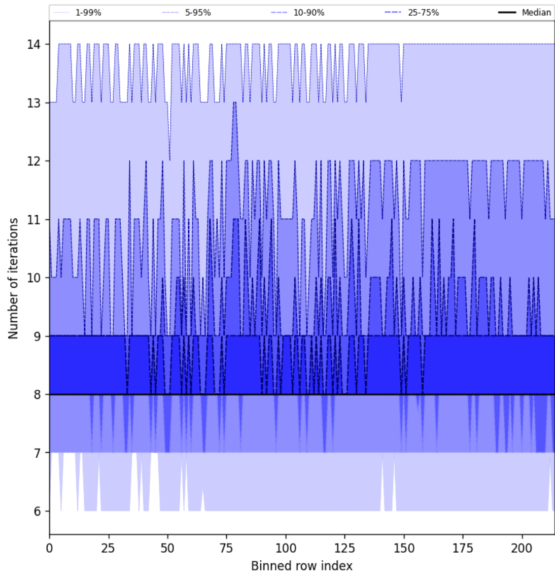
Figure 26: Along track statistics of “Number of iterations” for 2025-08-09 to 2025-08-10
