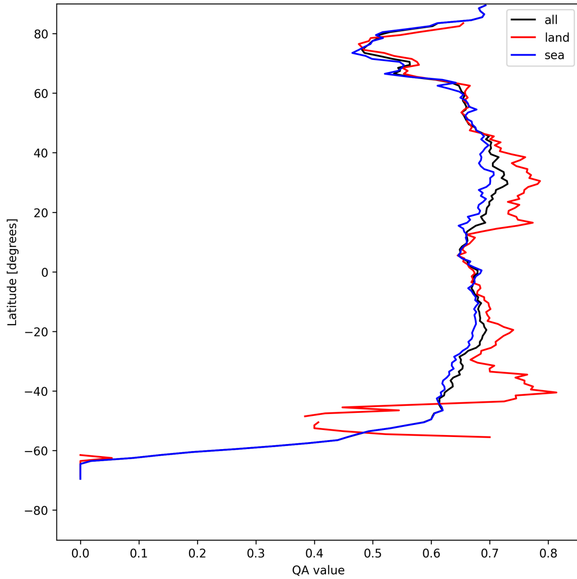
Figure 6: Zonal average of “QA value” for 2025-08-09 to 2025-08-10.
