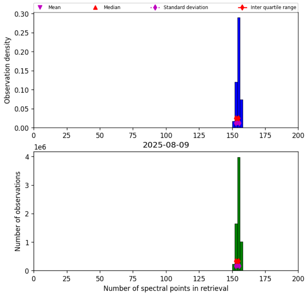
Figure 16: Histogram of "Number of spectral points in retrieval" for 2025-08-09 to 2025-08-10
