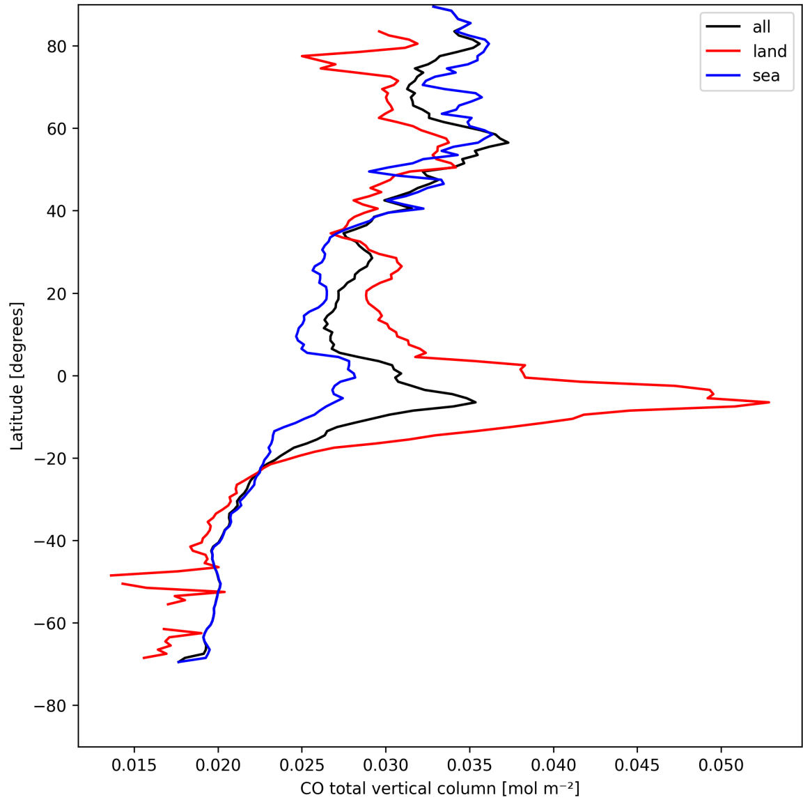
Figure 7: Zonal average of “CO total vertical column” for 2025-08-09 to 2025-08-10.
