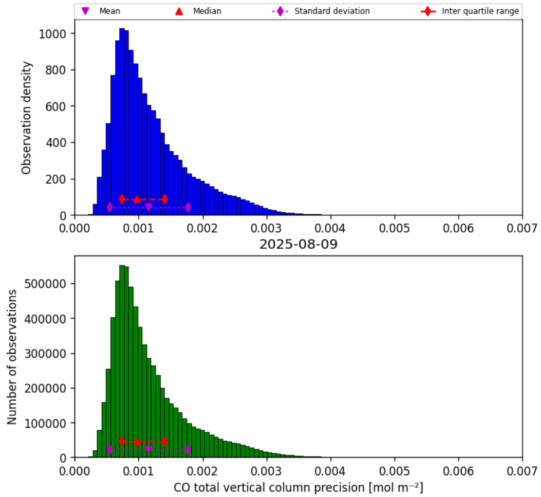
Figure 15: Histogram of “CO total vertical column precision” for 2025-08-09 to 2025-08-10
