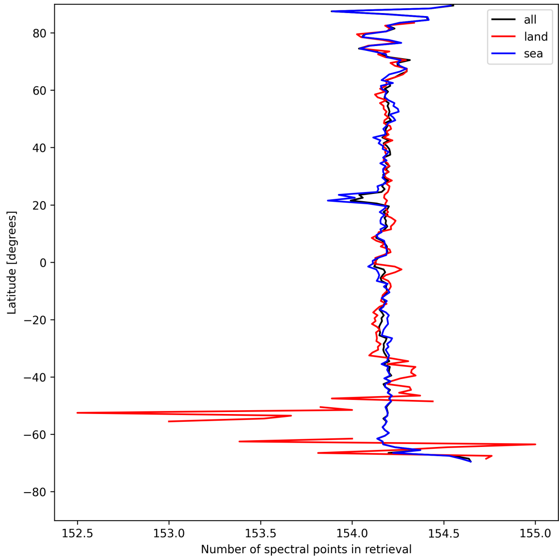
Figure 9: Zonal average of “Number of spectral points in retrieval” for 2025-08-09 to 2025-08-10.
