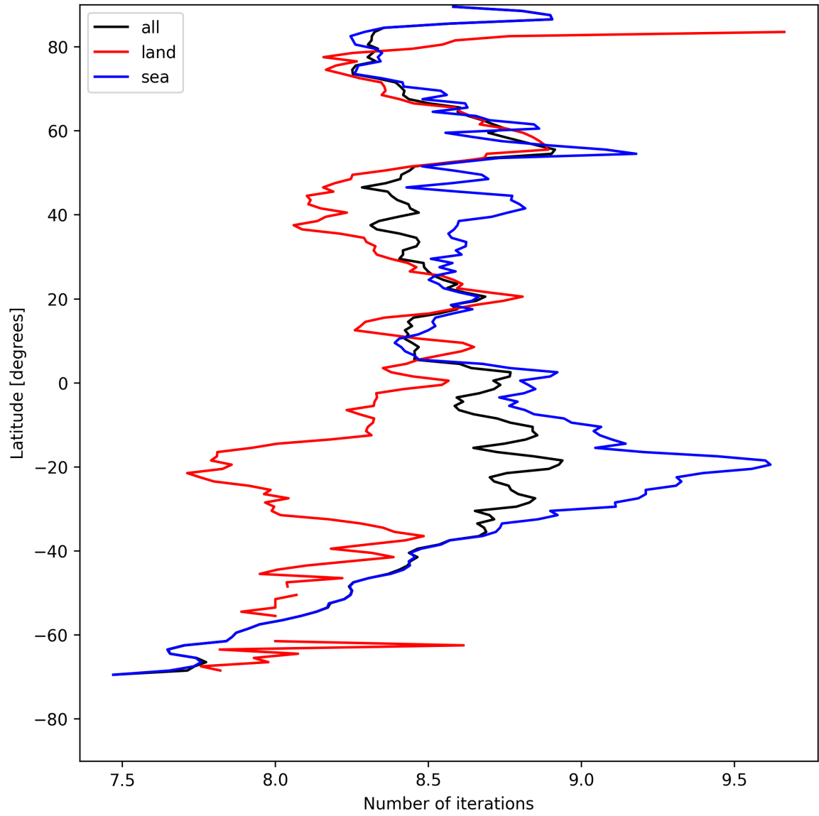
Figure 12: Zonal average of “Number of iterations” for 2025-08-09 to 2025-08-10.
