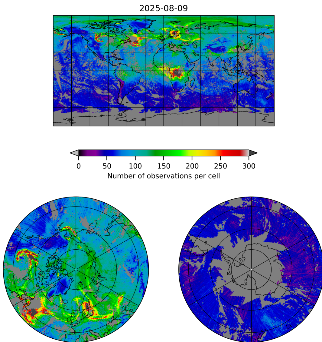
Figure 5: Map of the number of observations for 2025-08-09 to 2025-08-10
