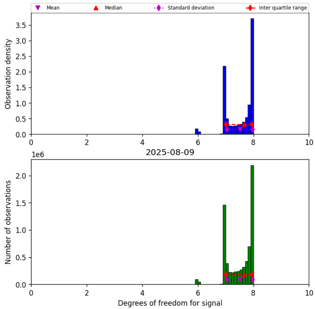
Figure 18: Histogram of “Degrees of freedom for signal” for 2025-08-09 to 2025-08-10
