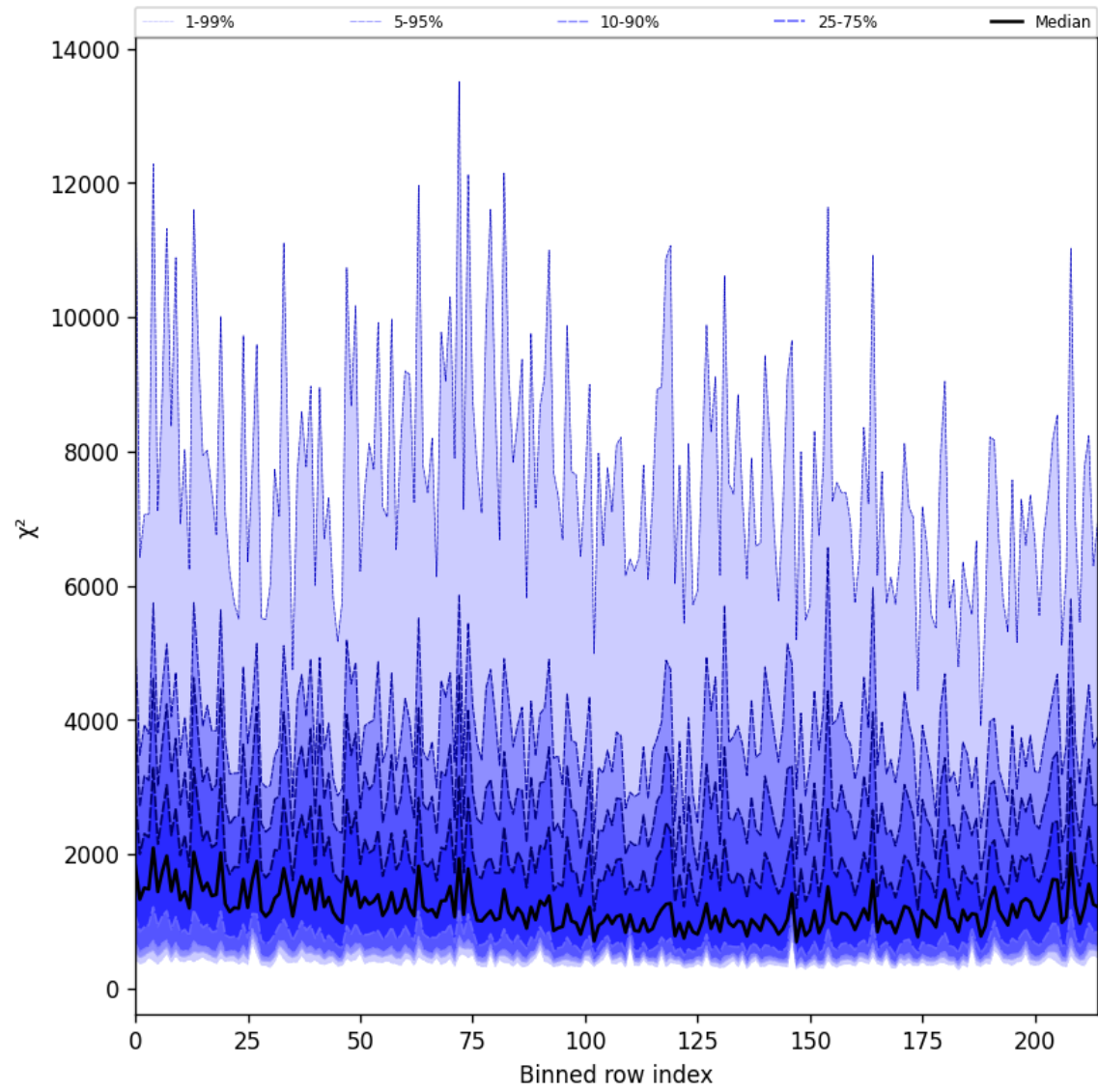
Figure 24: Along track statistics of “ \chi^2 ” for 2025-08-09 to 2025-08-10
