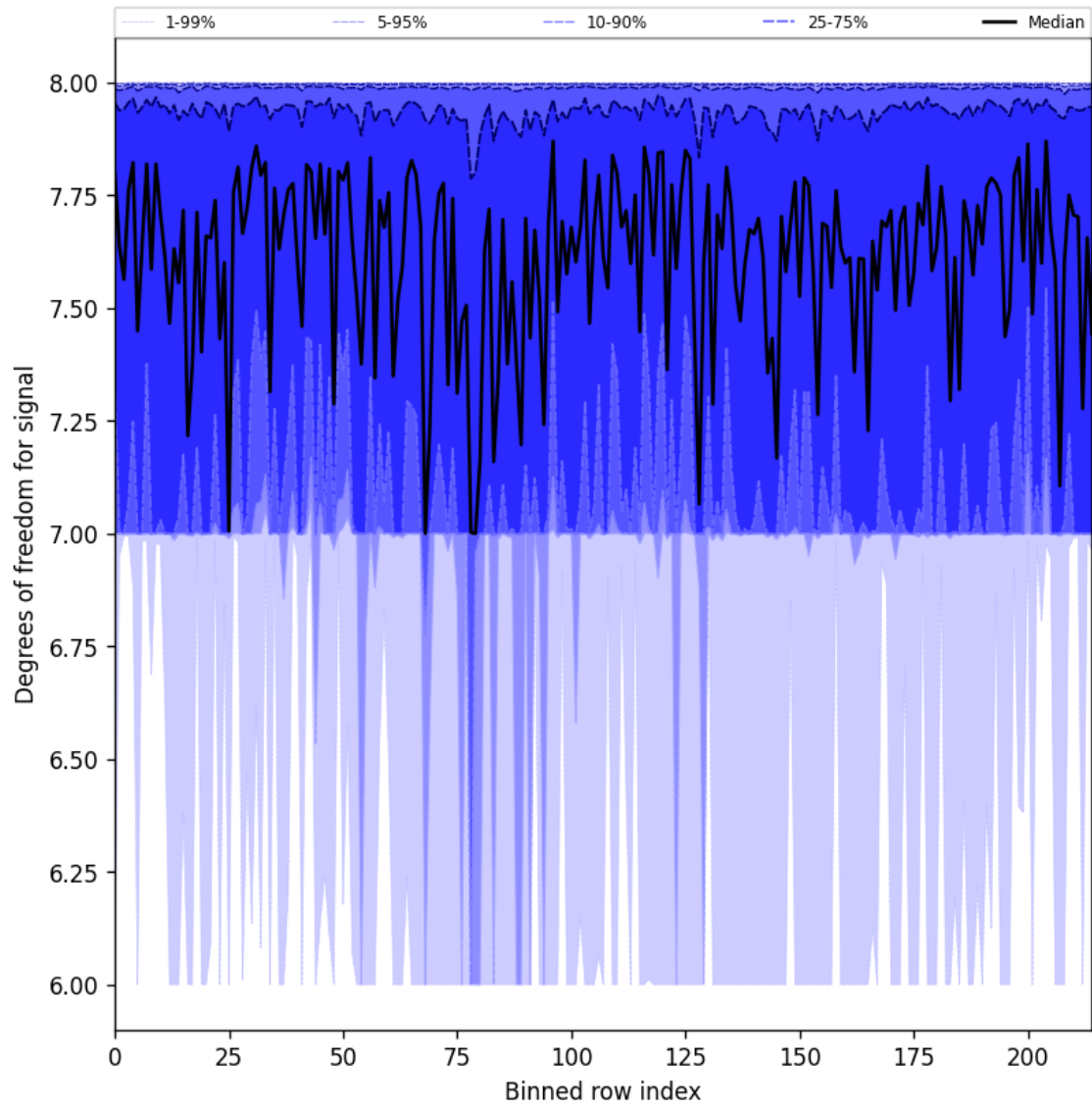
Figure 25: Along track statistics of “Degrees of freedom for signal” for 2025-08-09 to 2025-08-10
