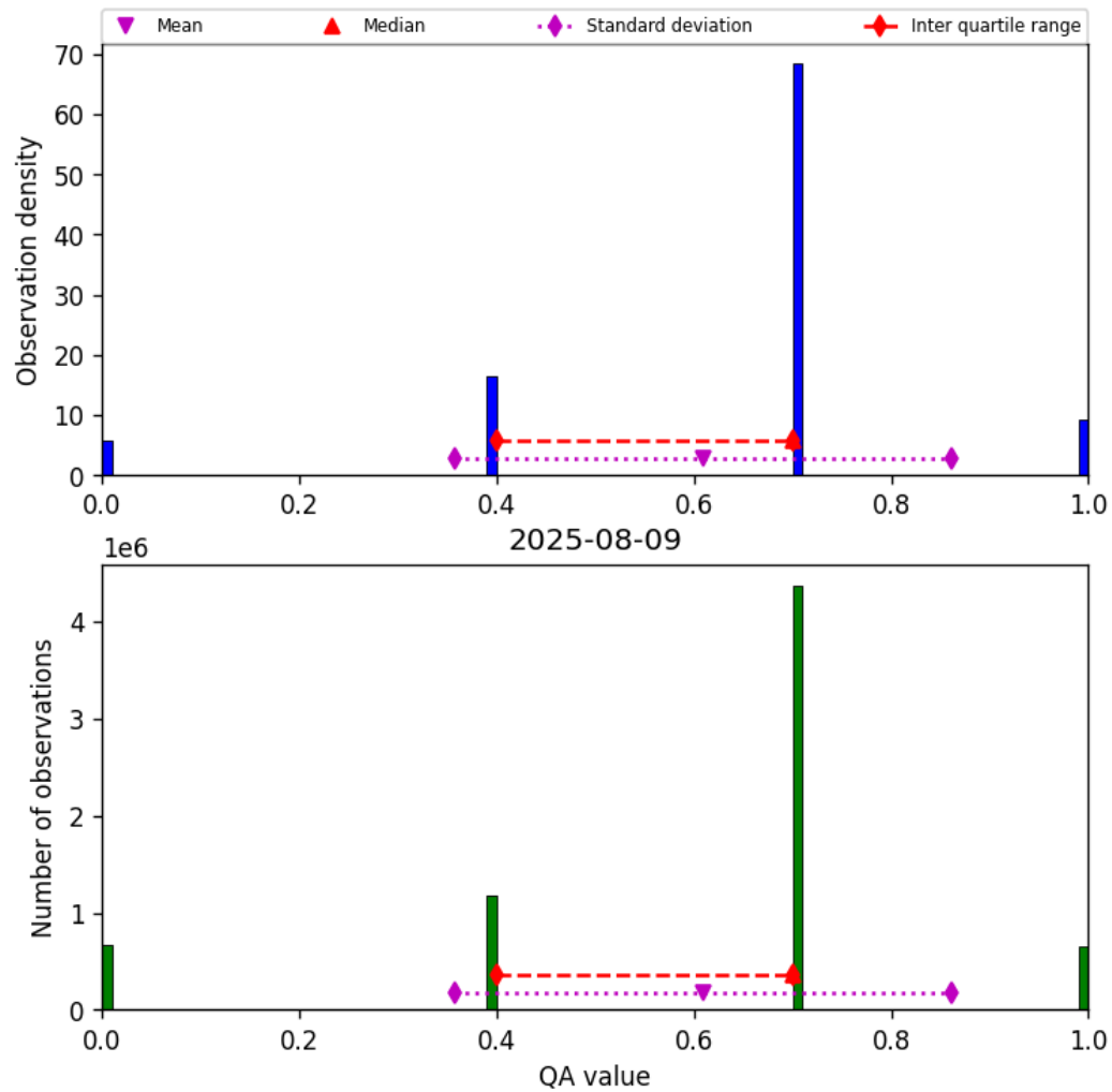
Figure 13: Histogram of “QA value” for 2025-08-09 to 2025-08-10
