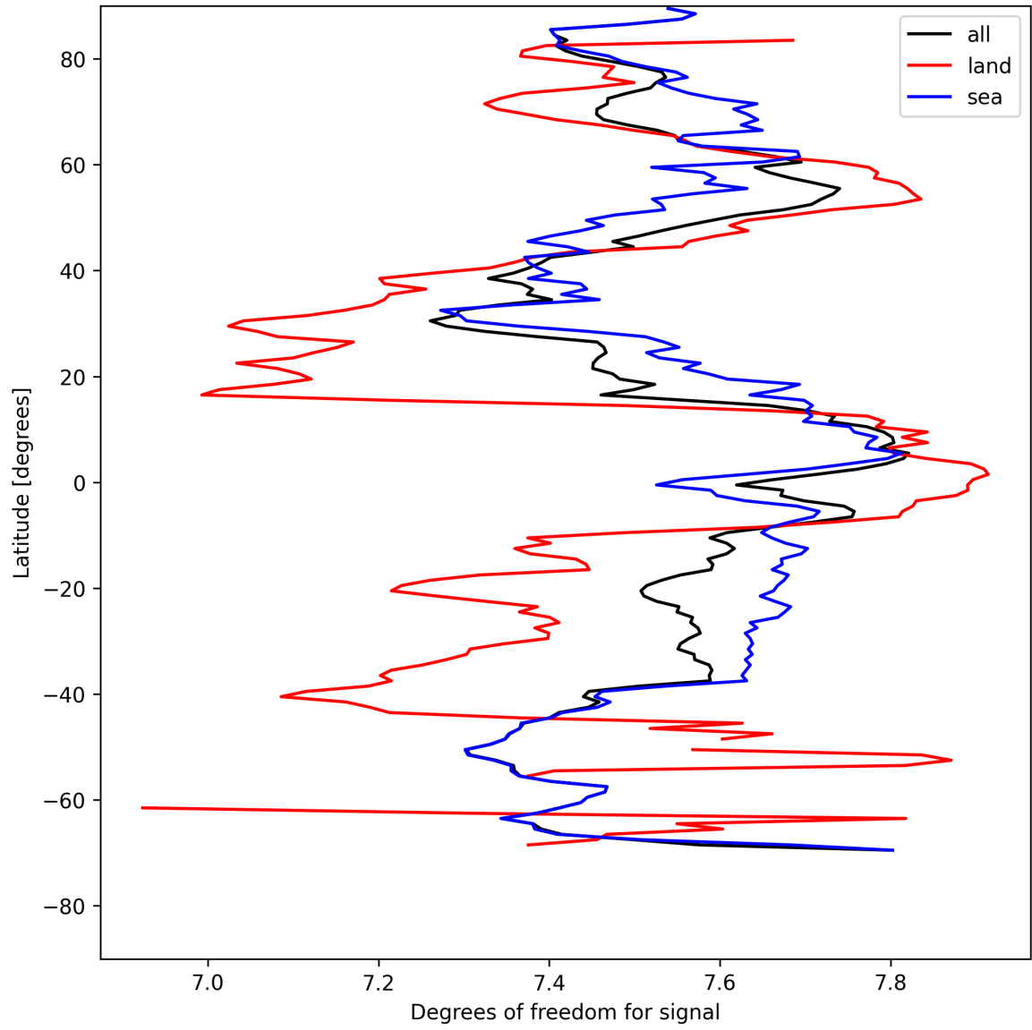
Figure 11: Zonal average of “Degrees of freedom for signal” for 2025-08-09 to 2025-08-10.
