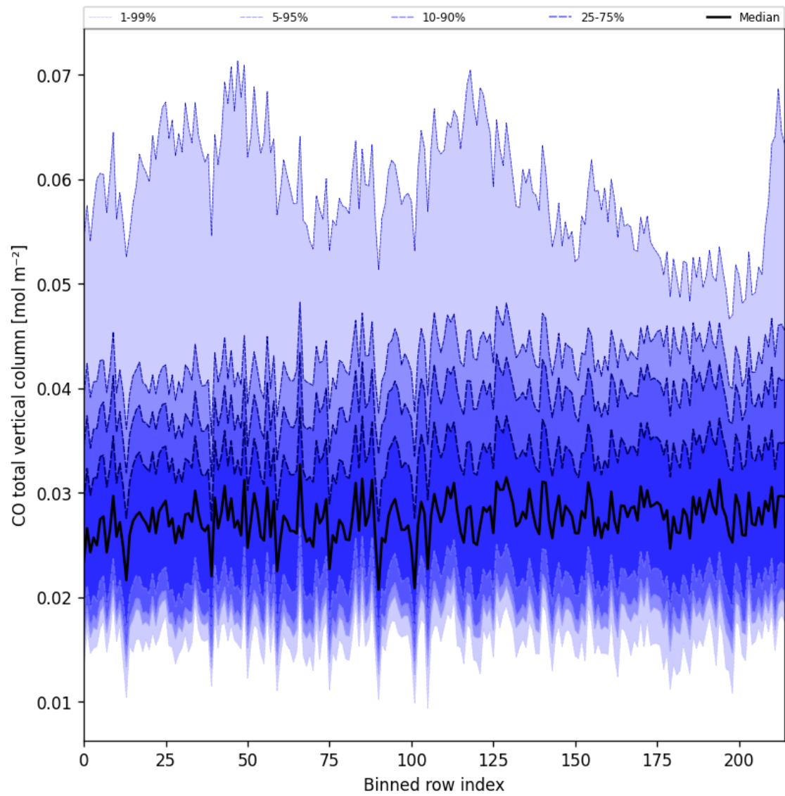
Figure 21: Along track statistics of “CO total vertical column” for 2025-08-10 to 2025-08-11
