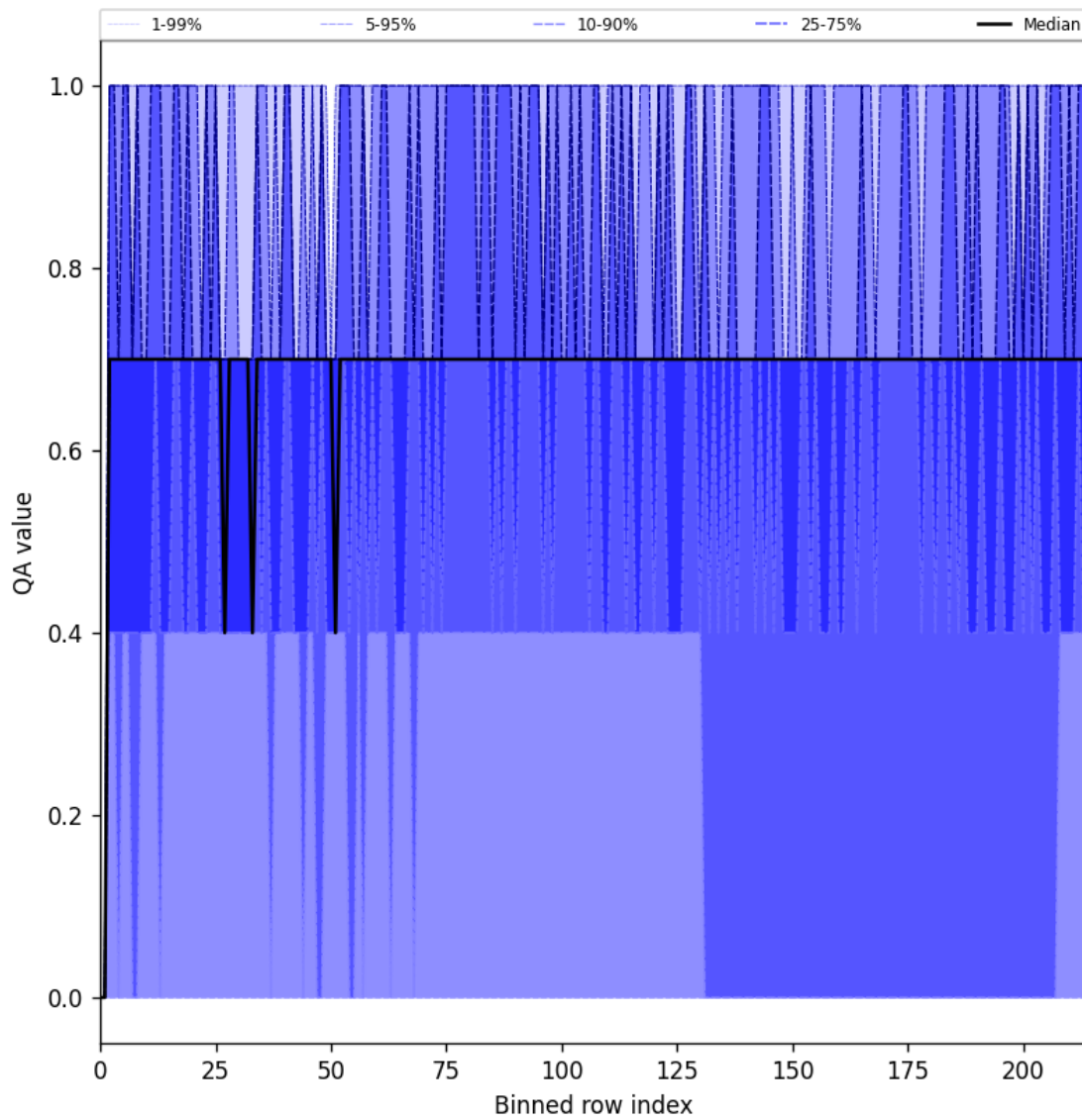
Figure 20: Along track statistics of “QA value” for 2025-08-10 to 2025-08-11
