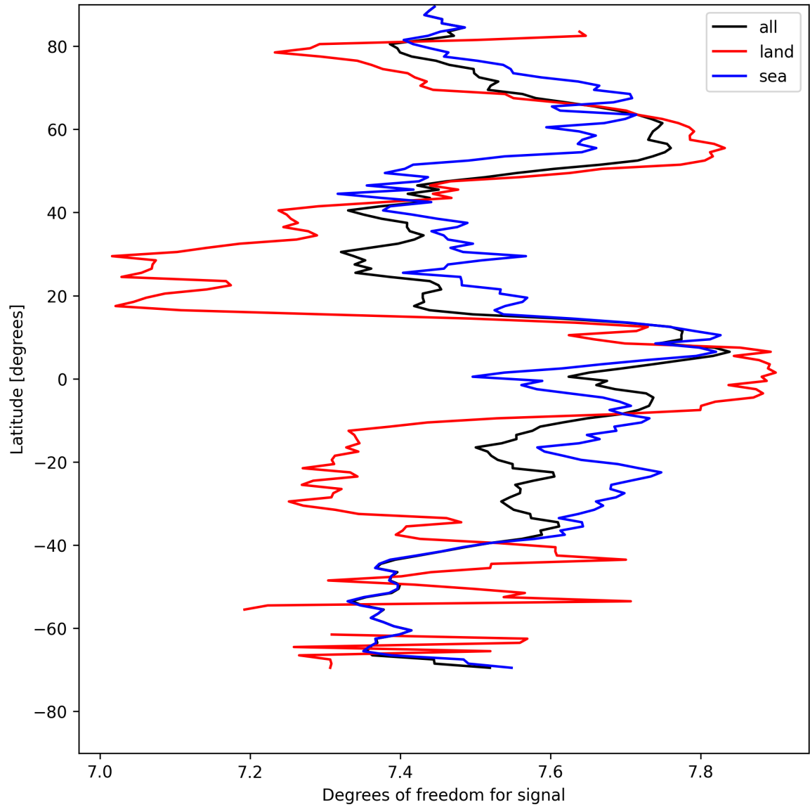
Figure 11: Zonal average of “Degrees of freedom for signal” for 2025-08-10 to 2025-08-11.
