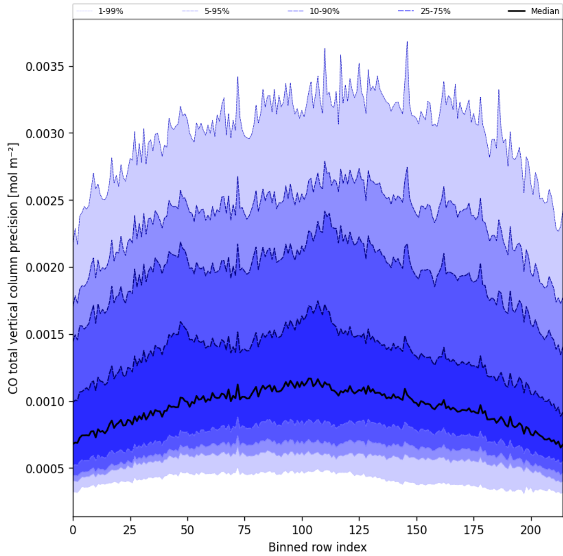
Figure 22: Along track statistics of “CO total vertical column precision” for 2025-08-10 to 2025-08-11
