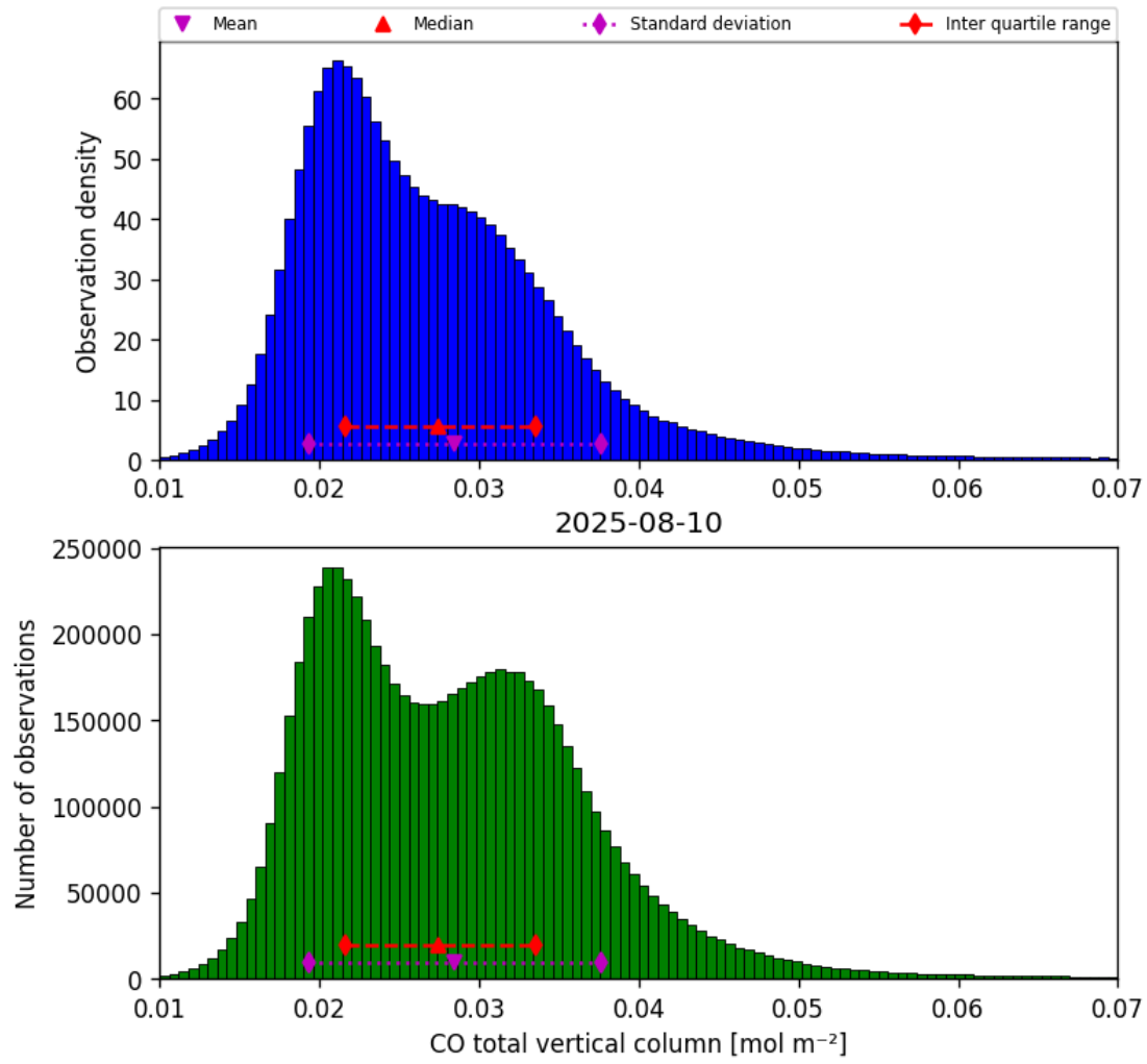
Figure 14: Histogram of “CO total vertical column” for 2025-08-10 to 2025-08-11
