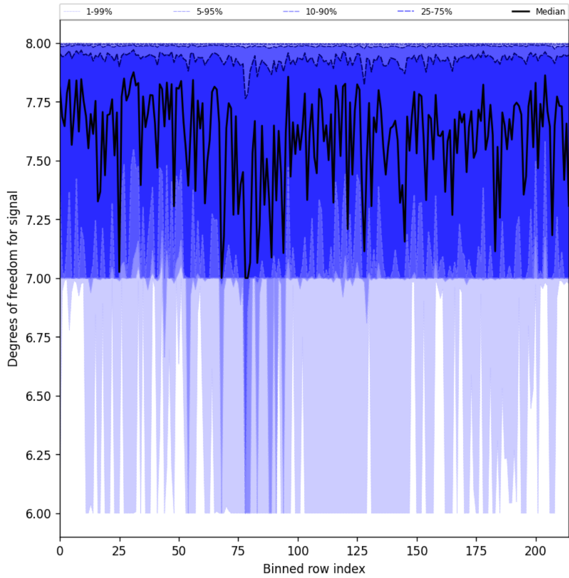
Figure 25: Along track statistics of “Degrees of freedom for signal” for 2025-08-10 to 2025-08-11
