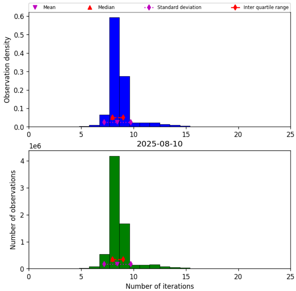
Figure 19: Histogram of “Number of iterations” for 2025-08-10 to 2025-08-11
