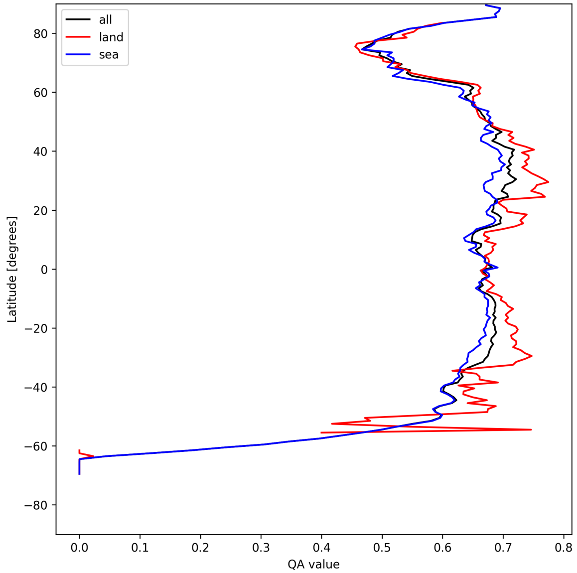
Figure 6: Zonal average of “QA value” for 2025-08-10 to 2025-08-11.
