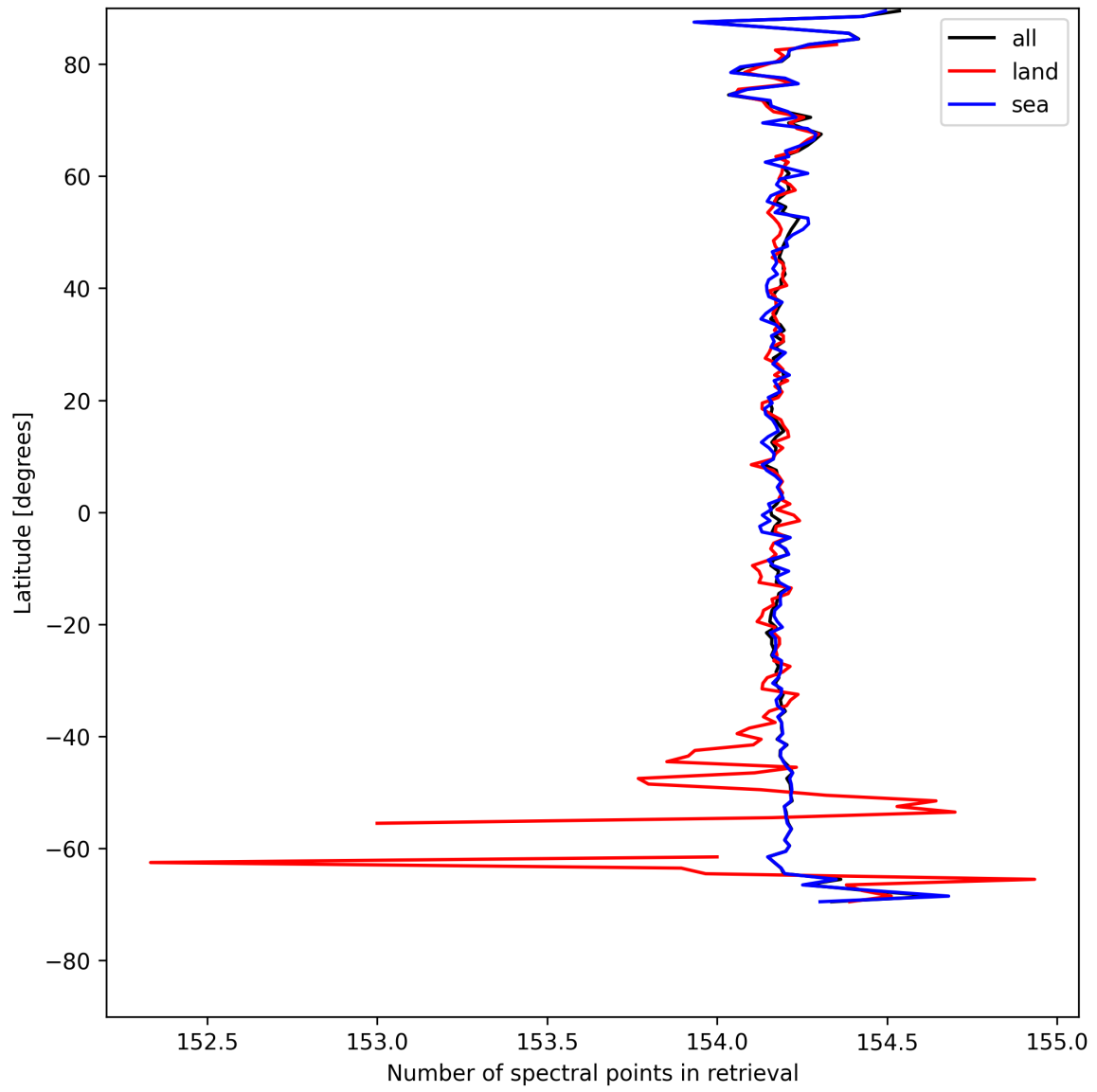
Figure 9: Zonal average of “Number of spectral points in retrieval” for 2025-08-10 to 2025-08-11.
