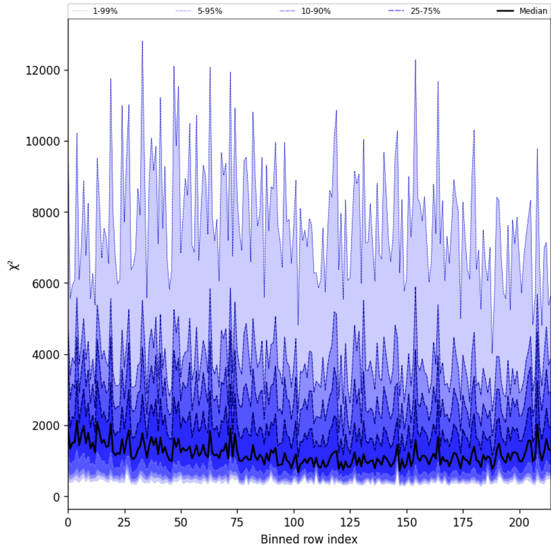
Figure 24: Along track statistics of “ \chi^2 ” for 2025-08-10 to 2025-08-11
