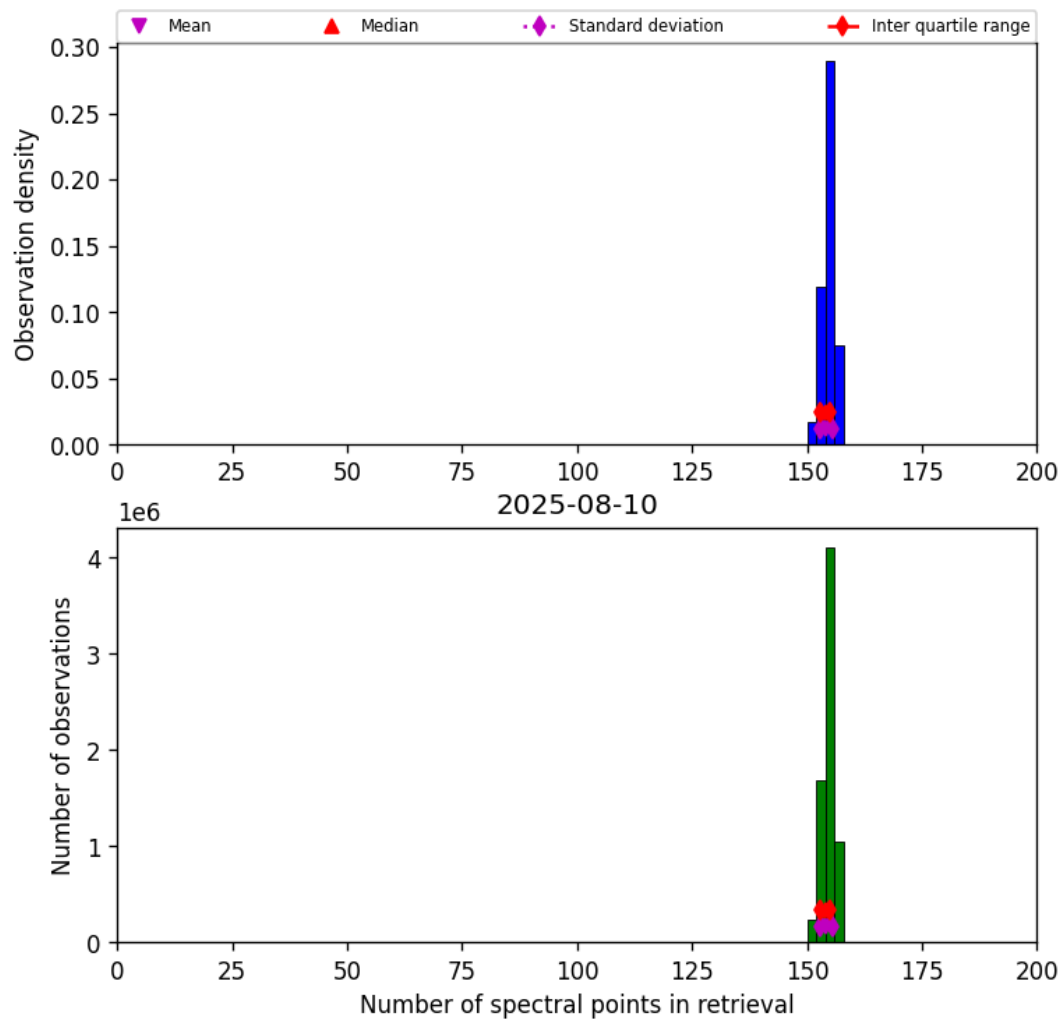
Figure 16: Histogram of “Number of spectral points in retrieval” for 2025-08-10 to 2025-08-11
