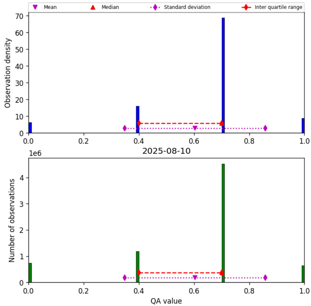
Figure 13: Histogram of “QA value” for 2025-08-10 to 2025-08-11
