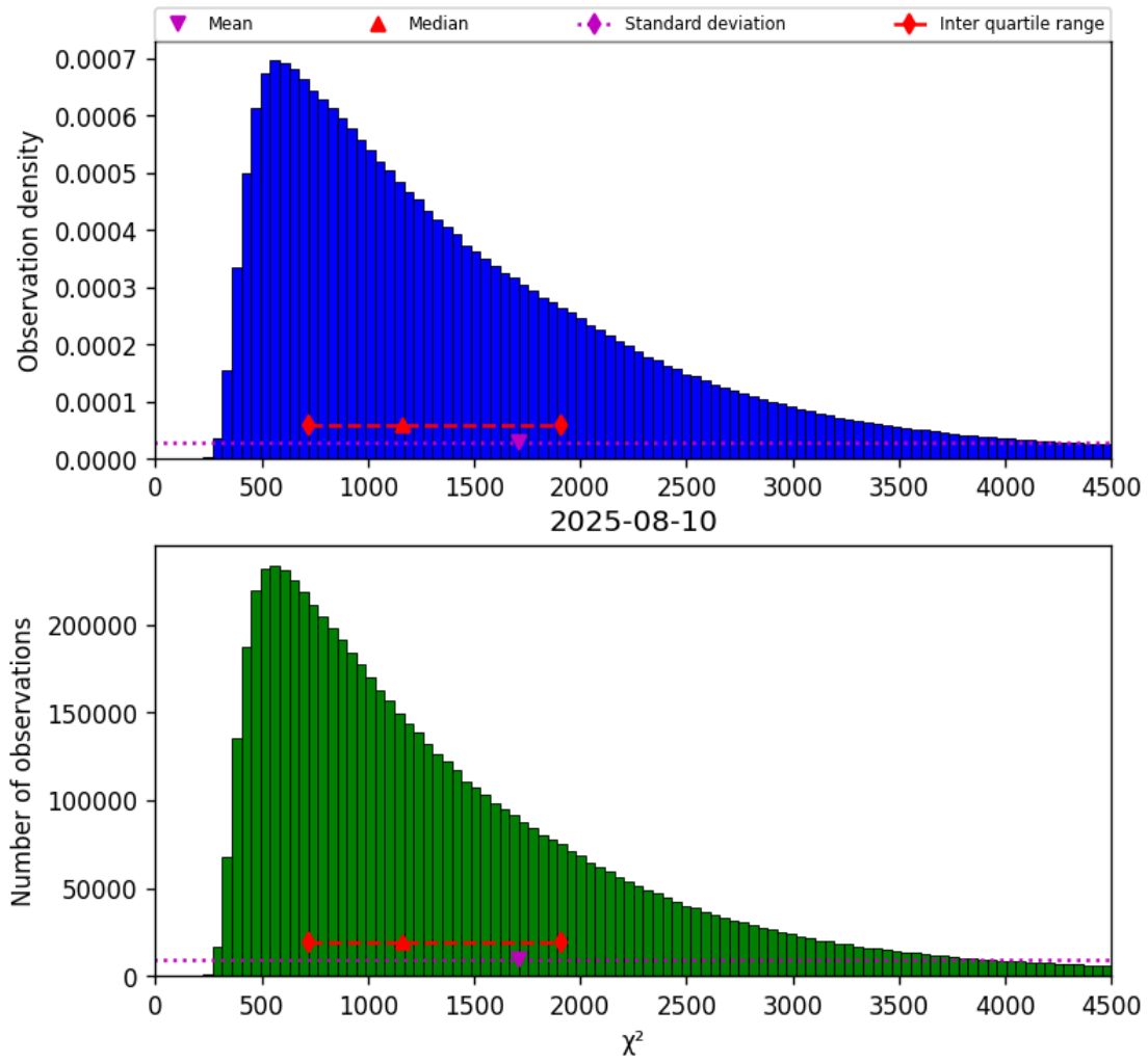
Figure 17: Histogram of “ \chi^2 ” for 2025-08-10 to 2025-08-11
