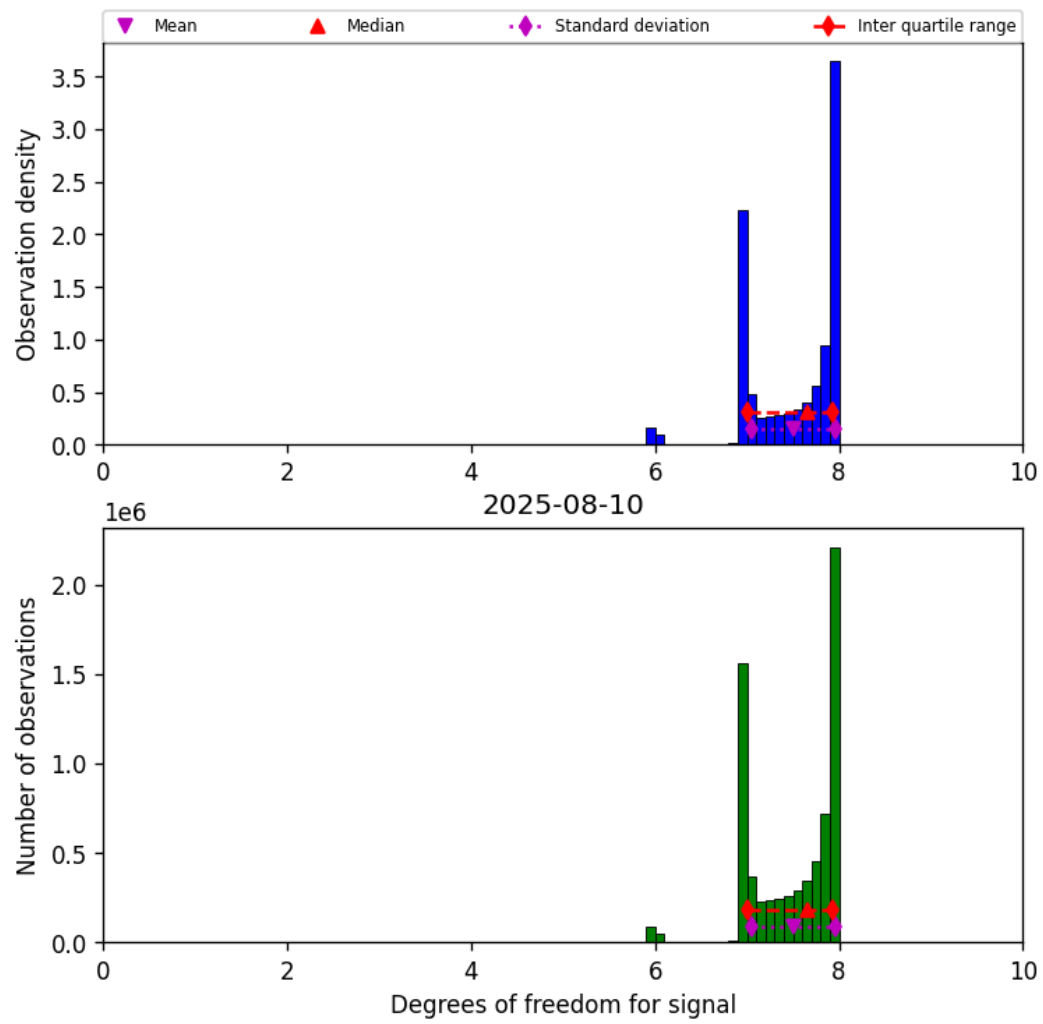
Figure 18: Histogram of “Degrees of freedom for signal” for 2025-08-10 to 2025-08-11
