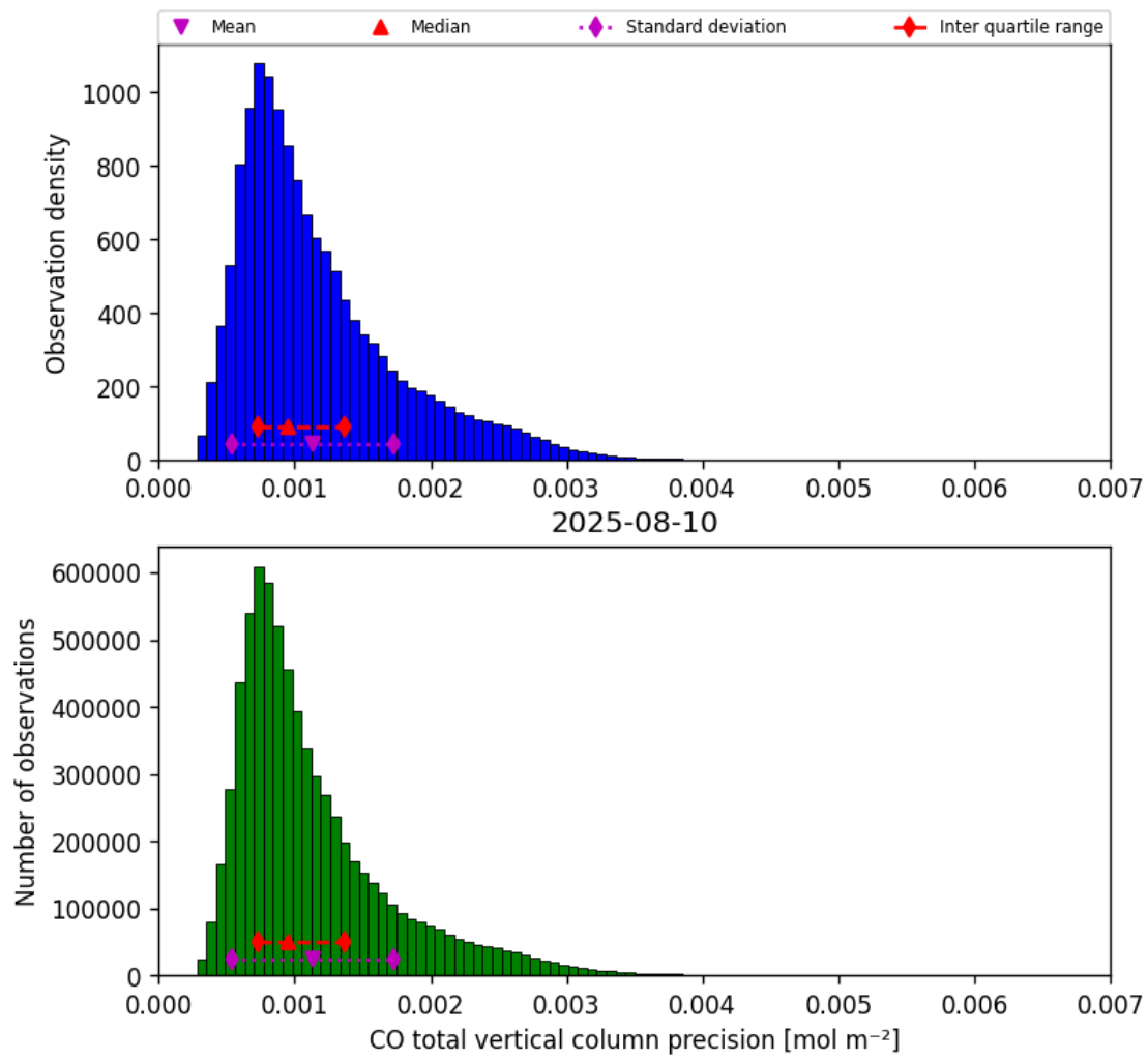
Figure 15: Histogram of “CO total vertical column precision” for 2025-08-10 to 2025-08-11
