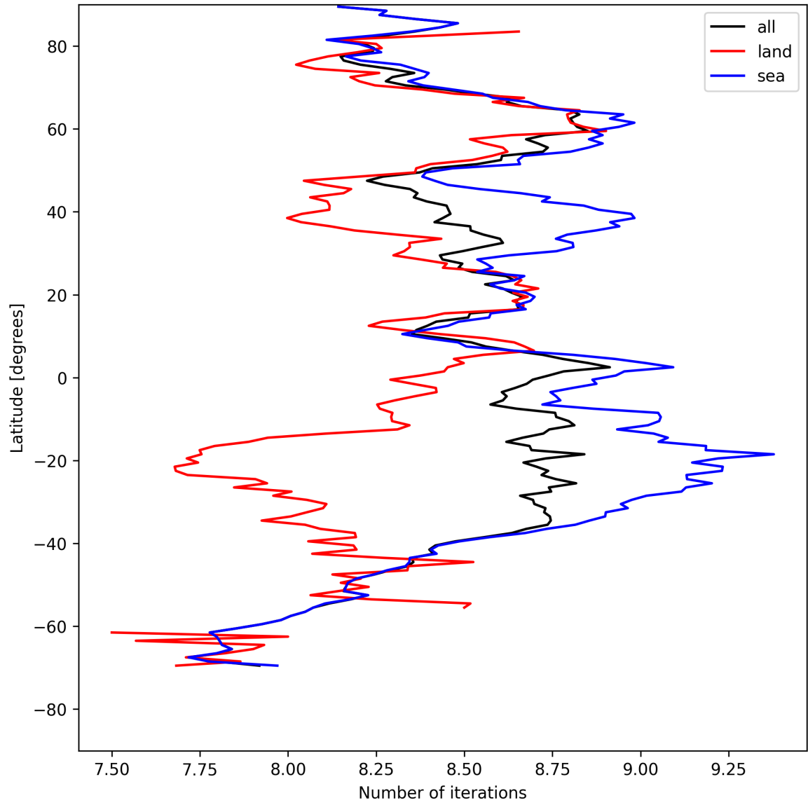
Figure 12: Zonal average of “Number of iterations” for 2025-08-10 to 2025-08-11.
