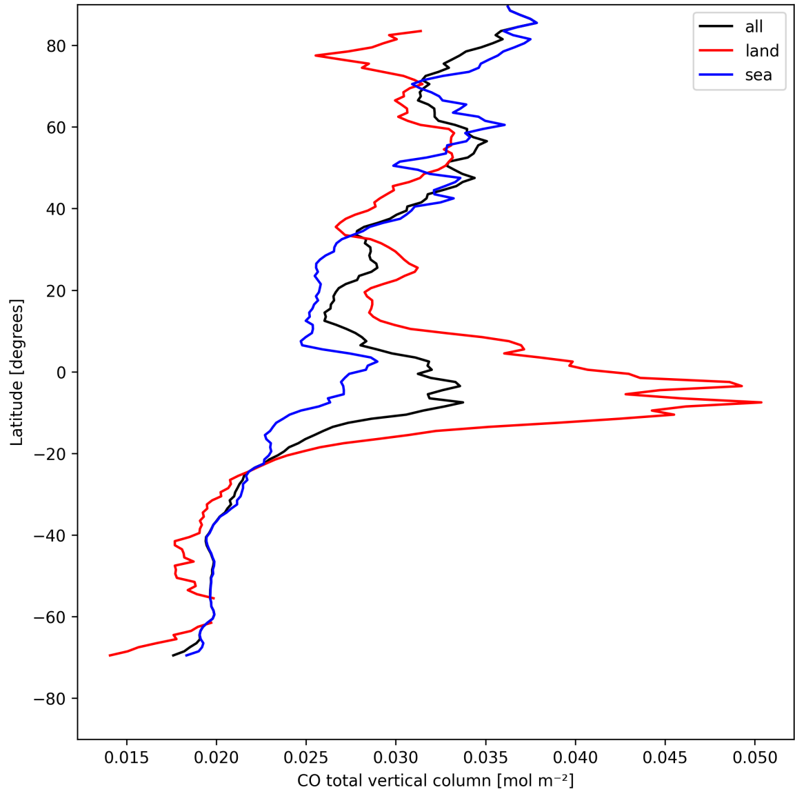
Figure 7: Zonal average of “CO total vertical column” for 2025-08-10 to 2025-08-11.
