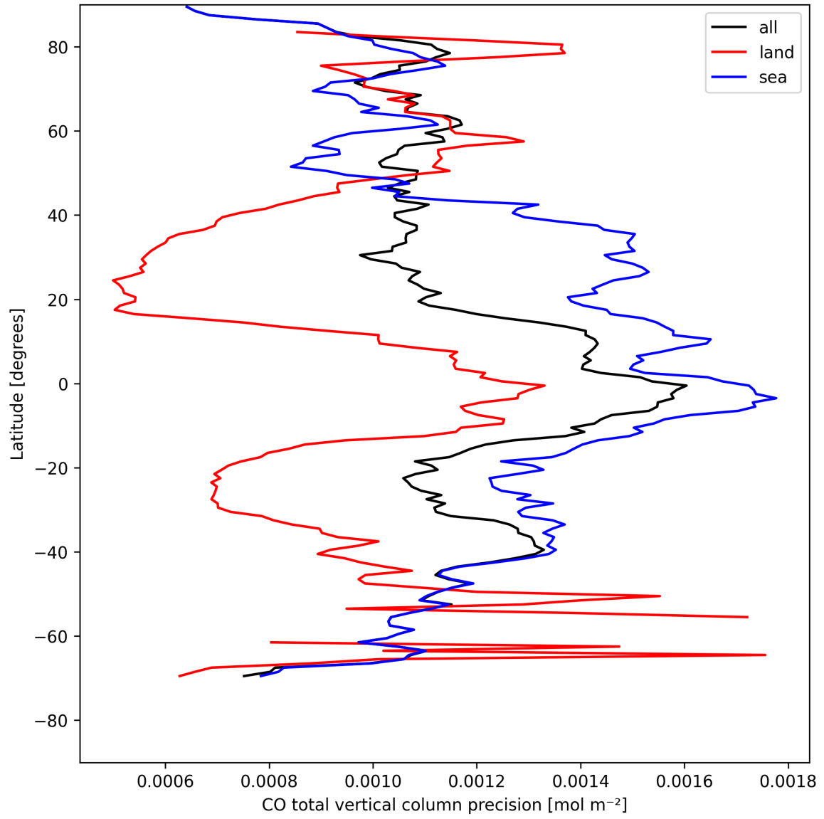
Figure 8: Zonal average of “CO total vertical column precision” for 2025-08-10 to 2025-08-11.
