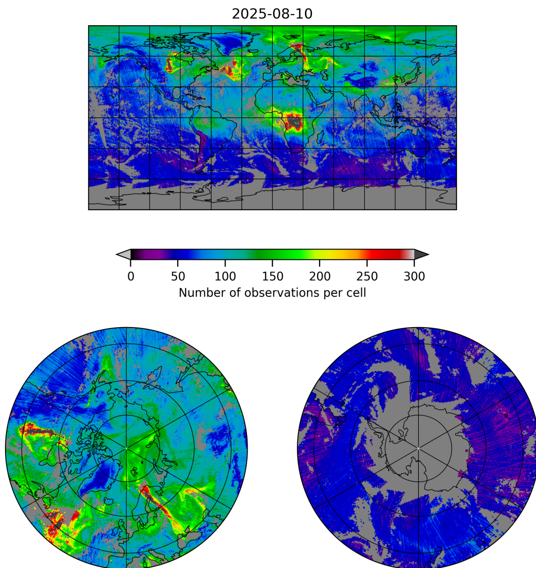
Figure 5: Map of the number of observations for 2025-08-10 to 2025-08-11
