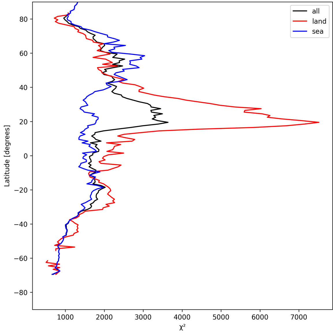
Figure 10: Zonal average of “ \chi^2 ” for 2025-08-10 to 2025-08-11.
