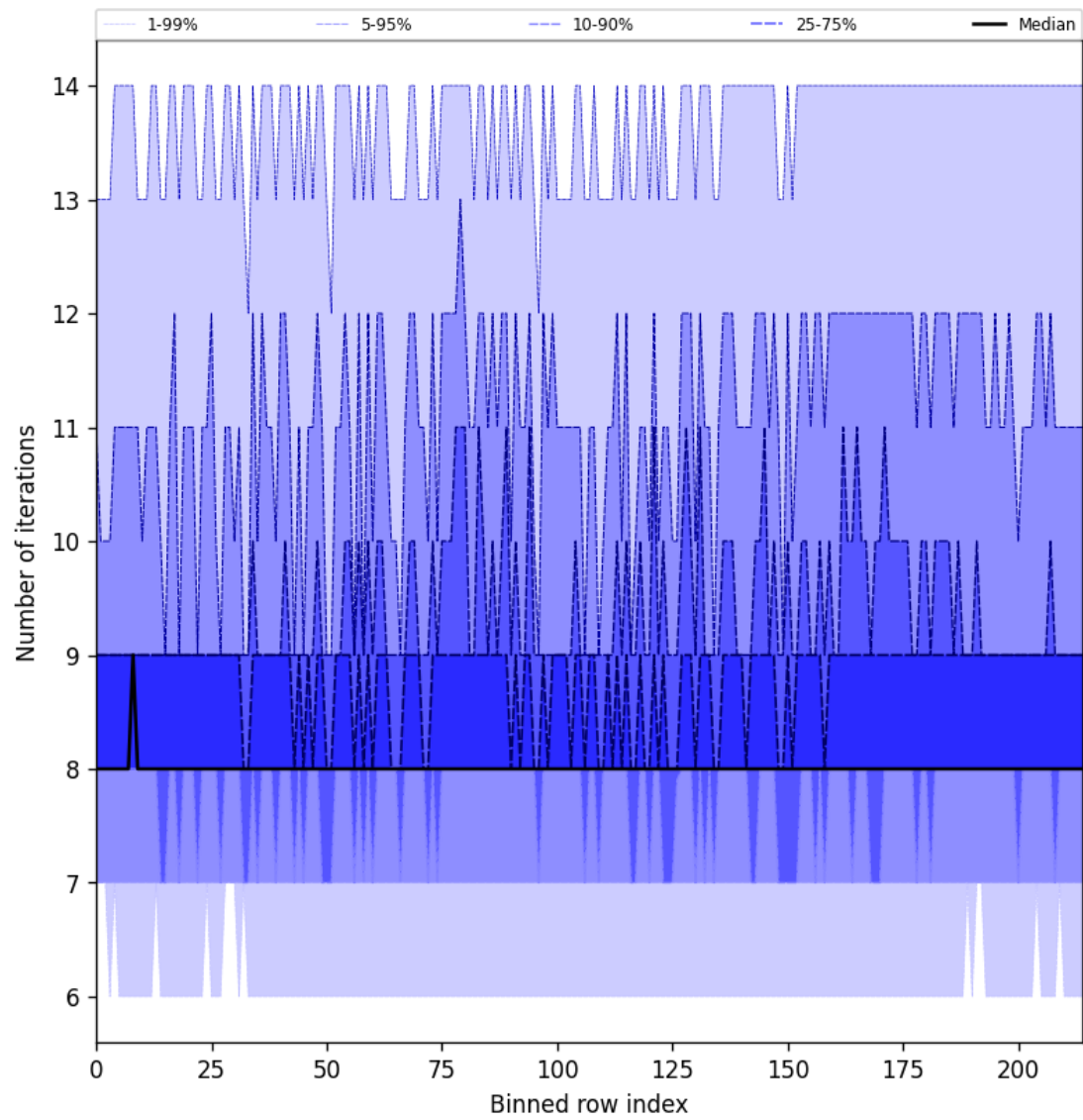
Figure 26: Along track statistics of “Number of iterations” for 2025-08-10 to 2025-08-11
