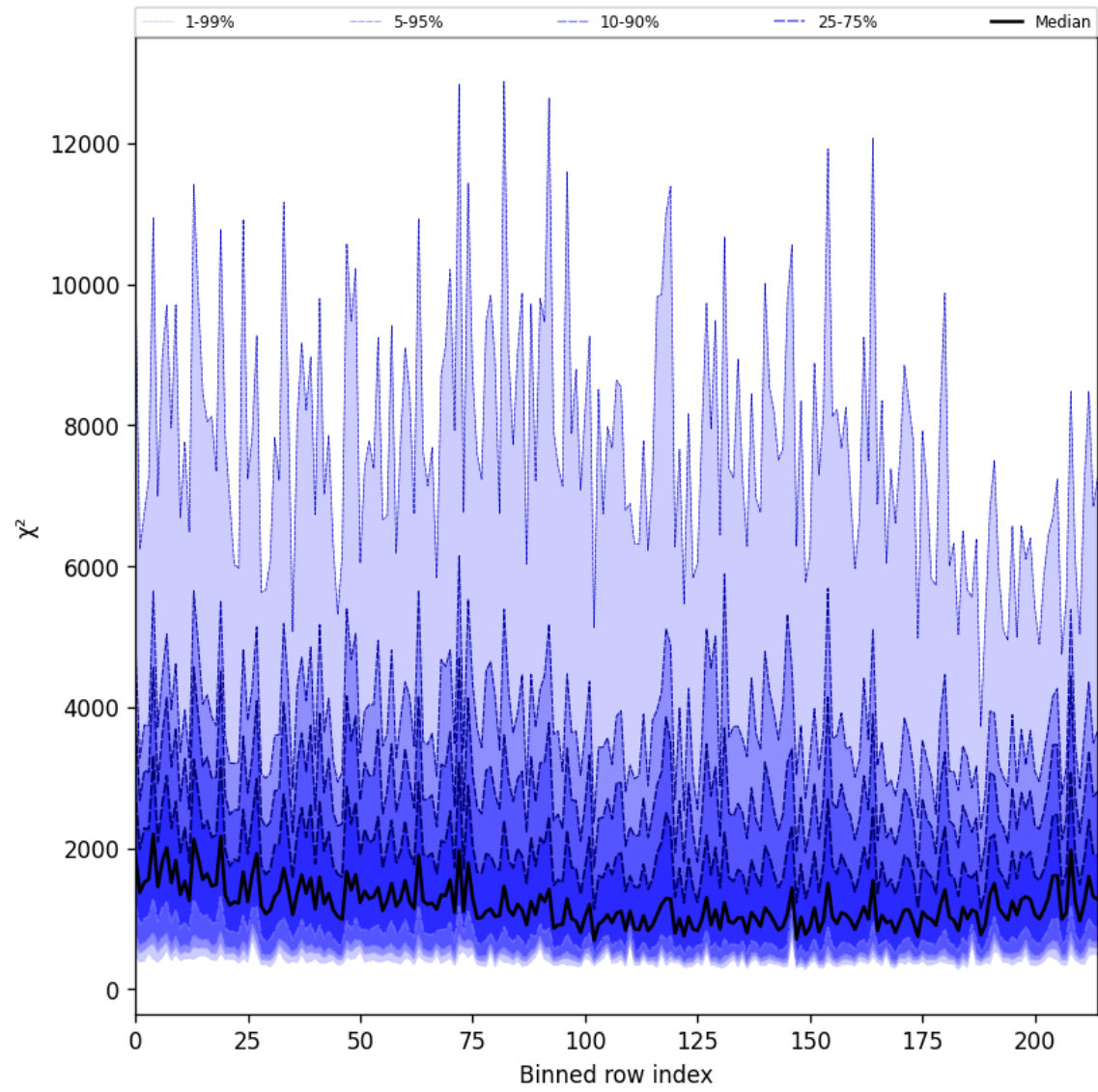
Figure 24: Along track statistics of “ \chi^2 ” for 2025-08-11 to 2025-08-12
