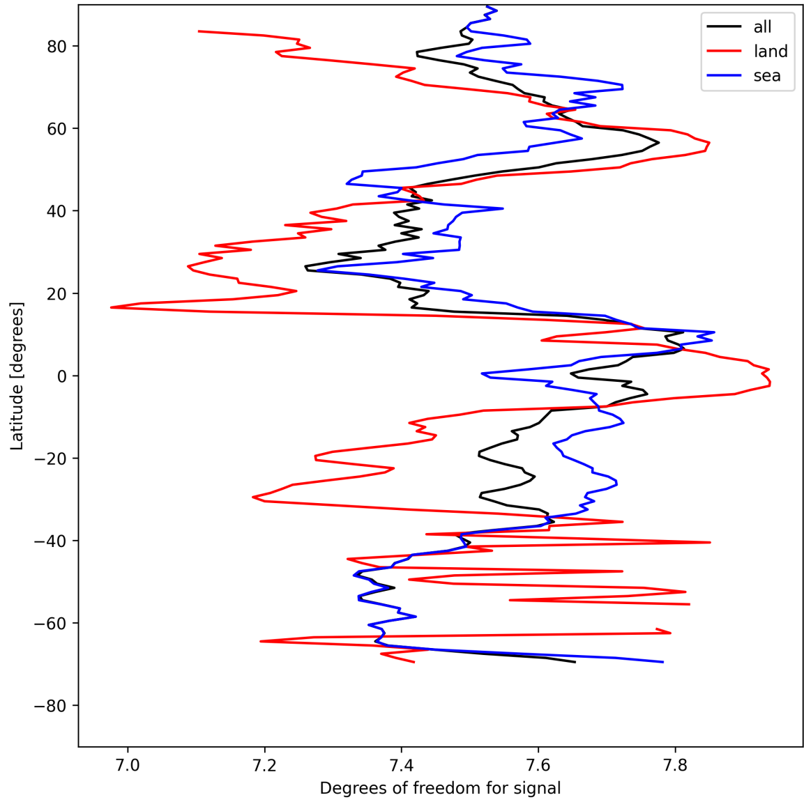
Figure 11: Zonal average of “Degrees of freedom for signal” for 2025-08-11 to 2025-08-12.
