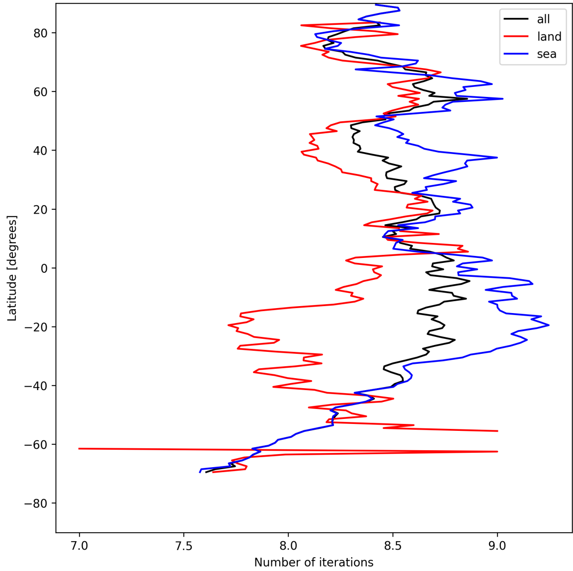
Figure 12: Zonal average of “Number of iterations” for 2025-08-11 to 2025-08-12.
