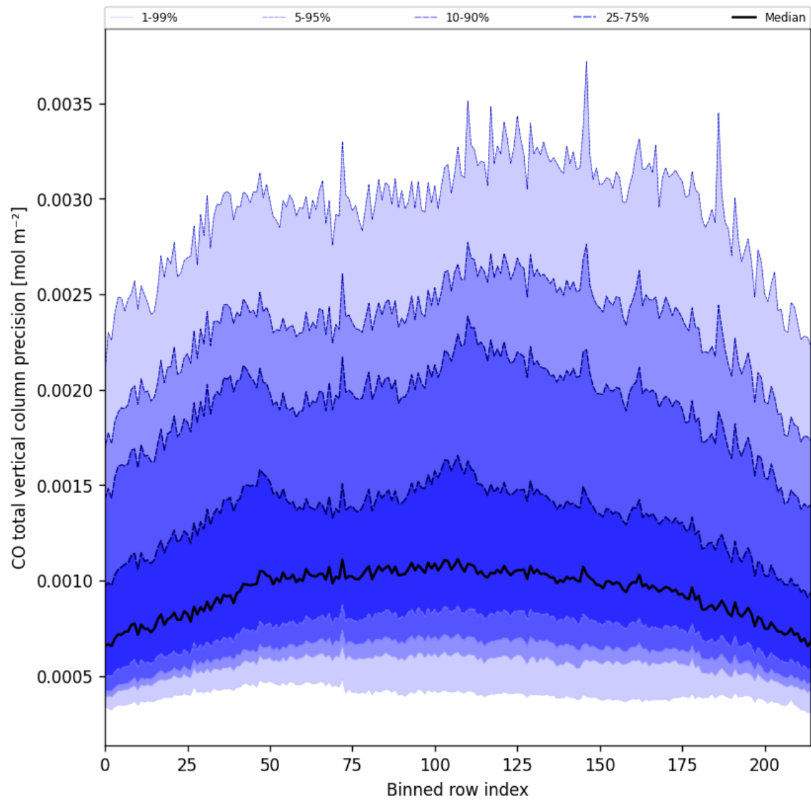
Figure 22: Along track statistics of “CO total vertical column precision” for 2025-08-11 to 2025-08-12
