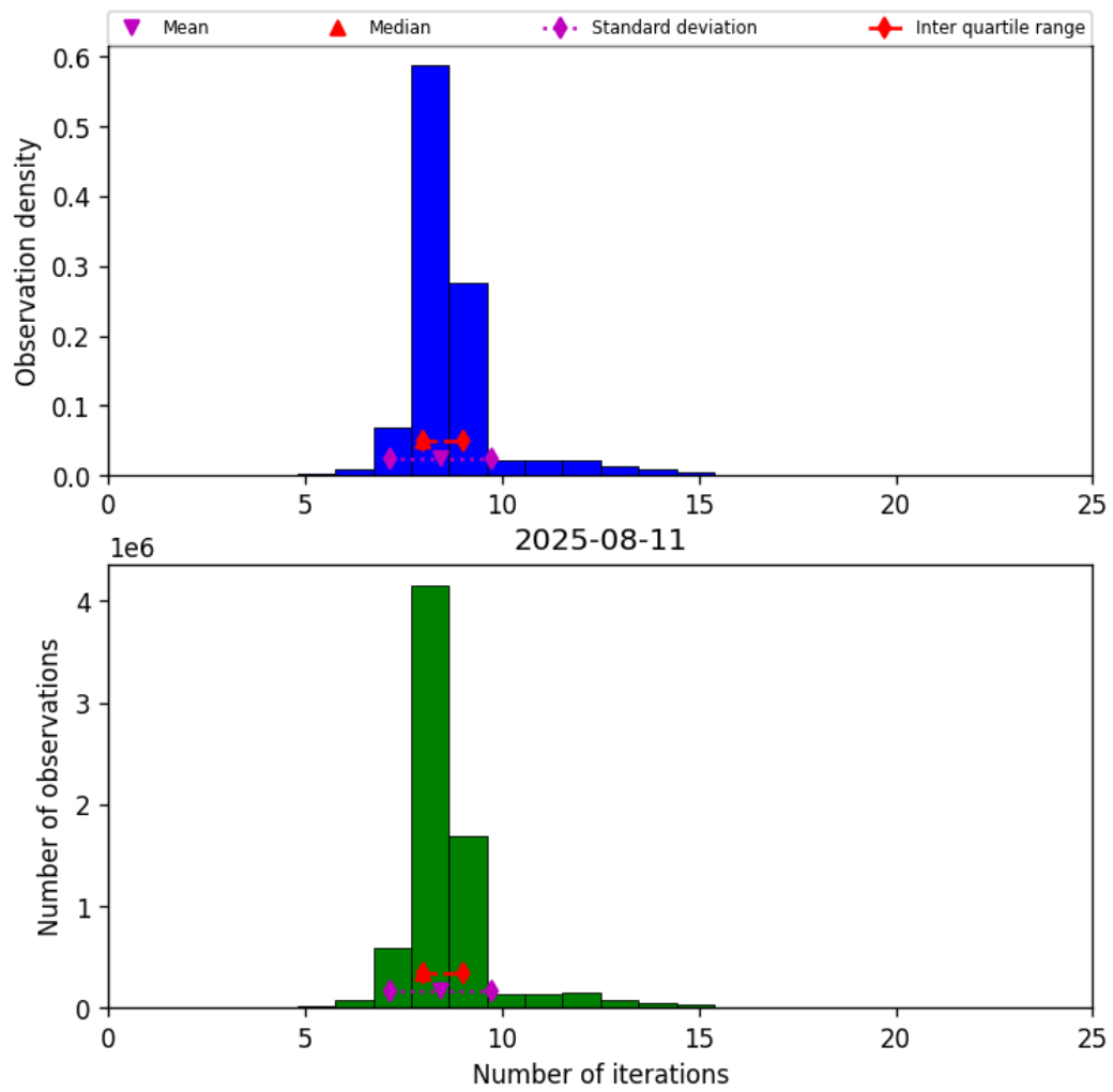
Figure 19: Histogram of “Number of iterations” for 2025-08-11 to 2025-08-12
