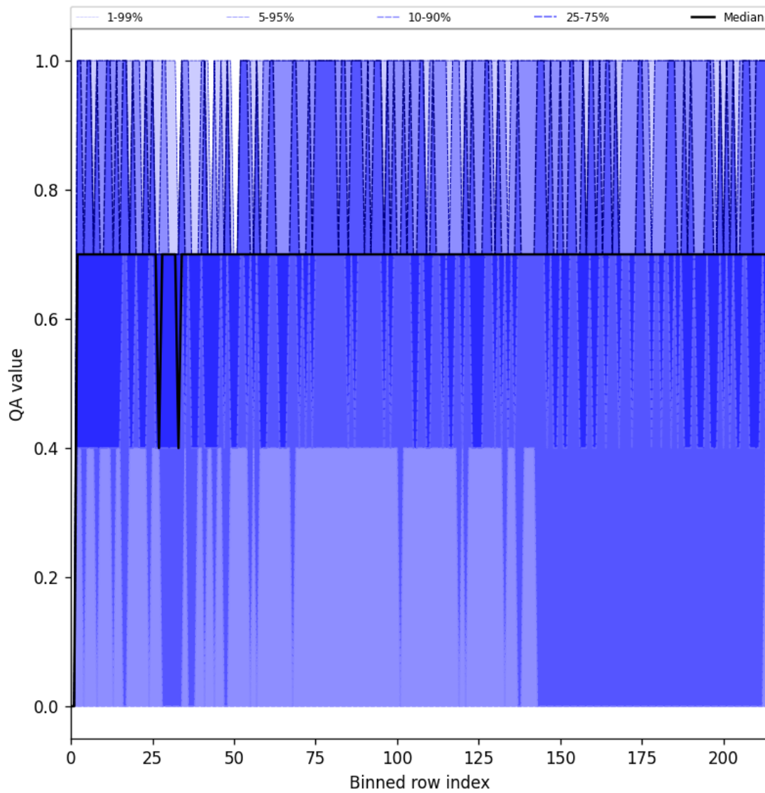
Figure 20: Along track statistics of “QA value” for 2025-08-11 to 2025-08-12
