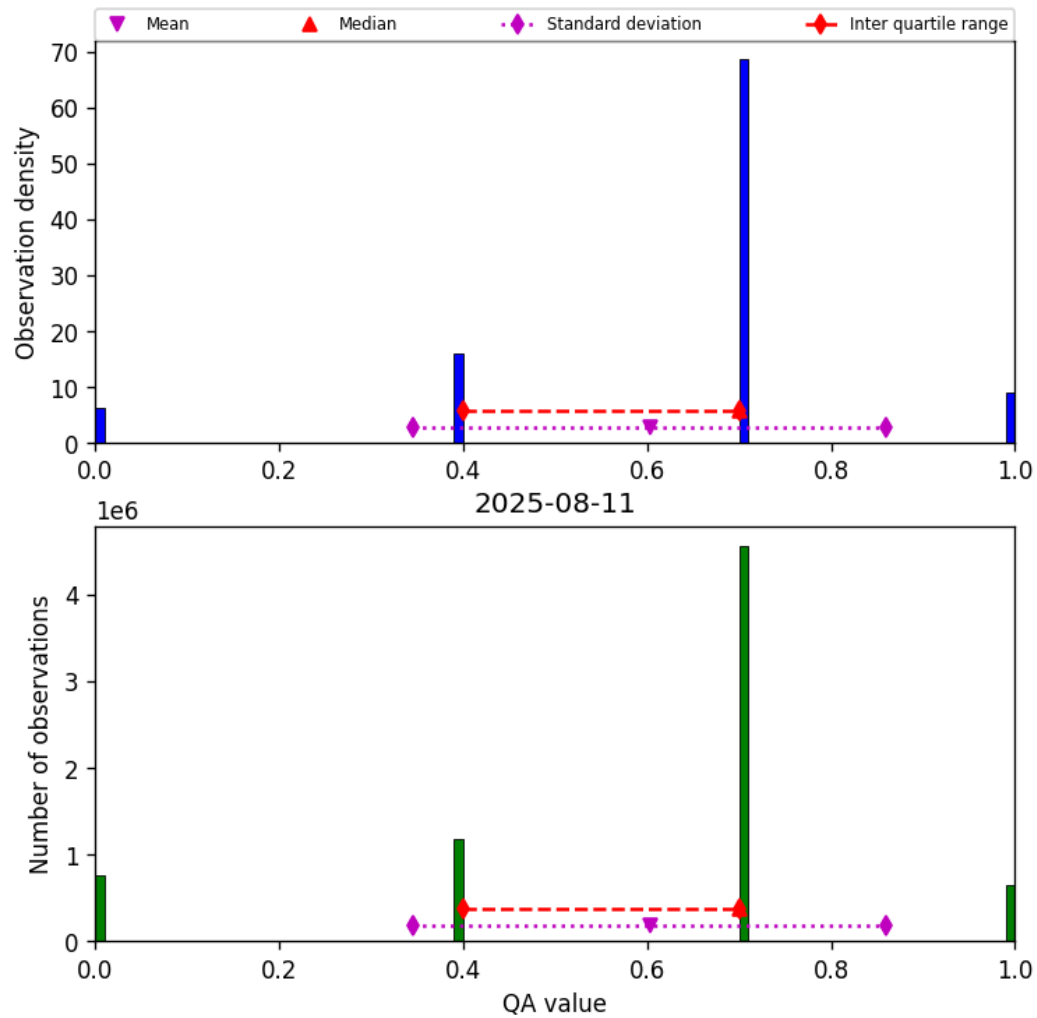
Figure 13: Histogram of “QA value” for 2025-08-11 to 2025-08-12
