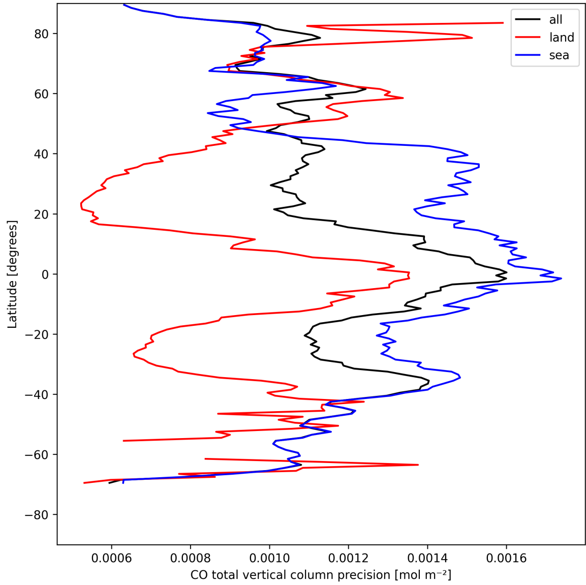
Figure 8: Zonal average of "CO total vertical column precision" for 2025-08-11 to 2025-08-12.
