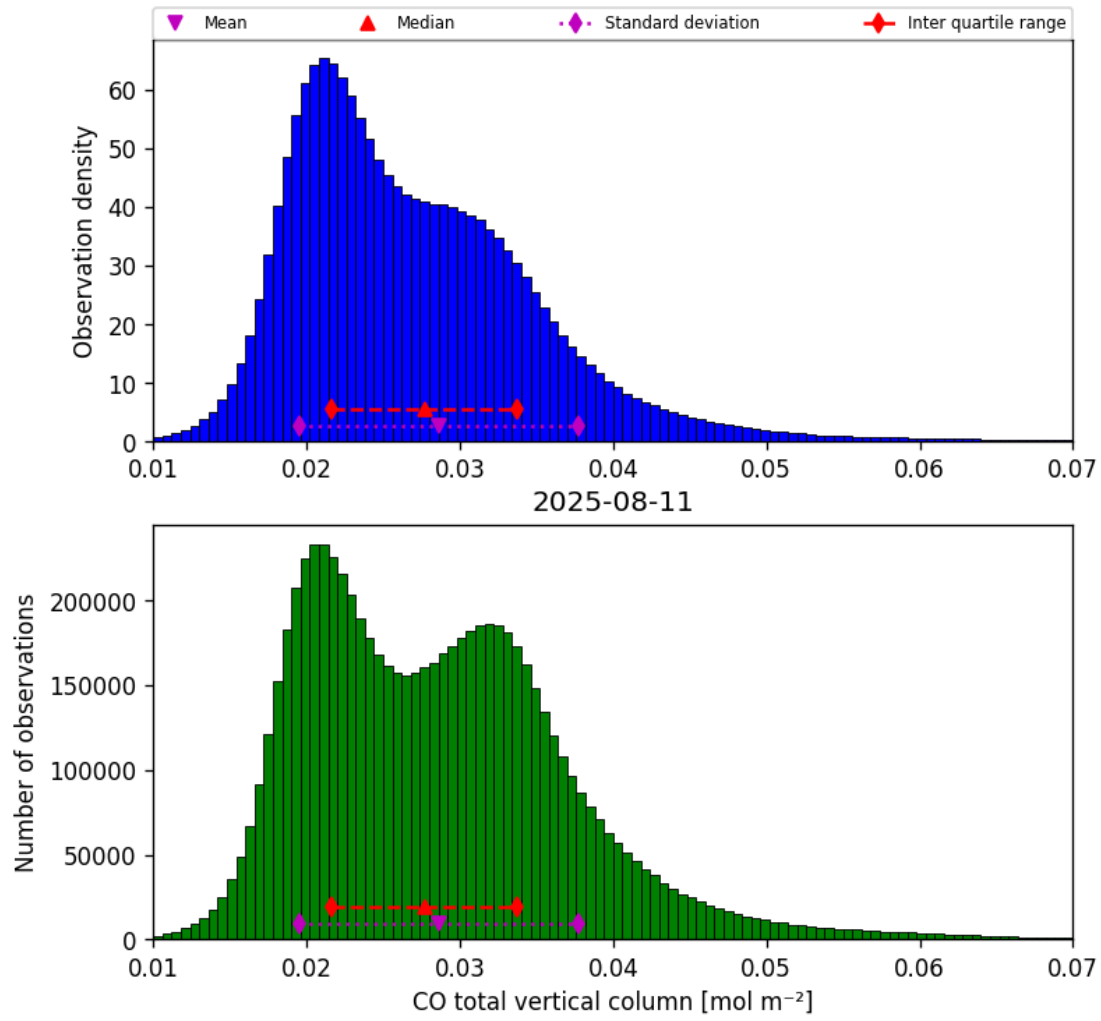
Figure 14: Histogram of “CO total vertical column” for 2025-08-11 to 2025-08-12
