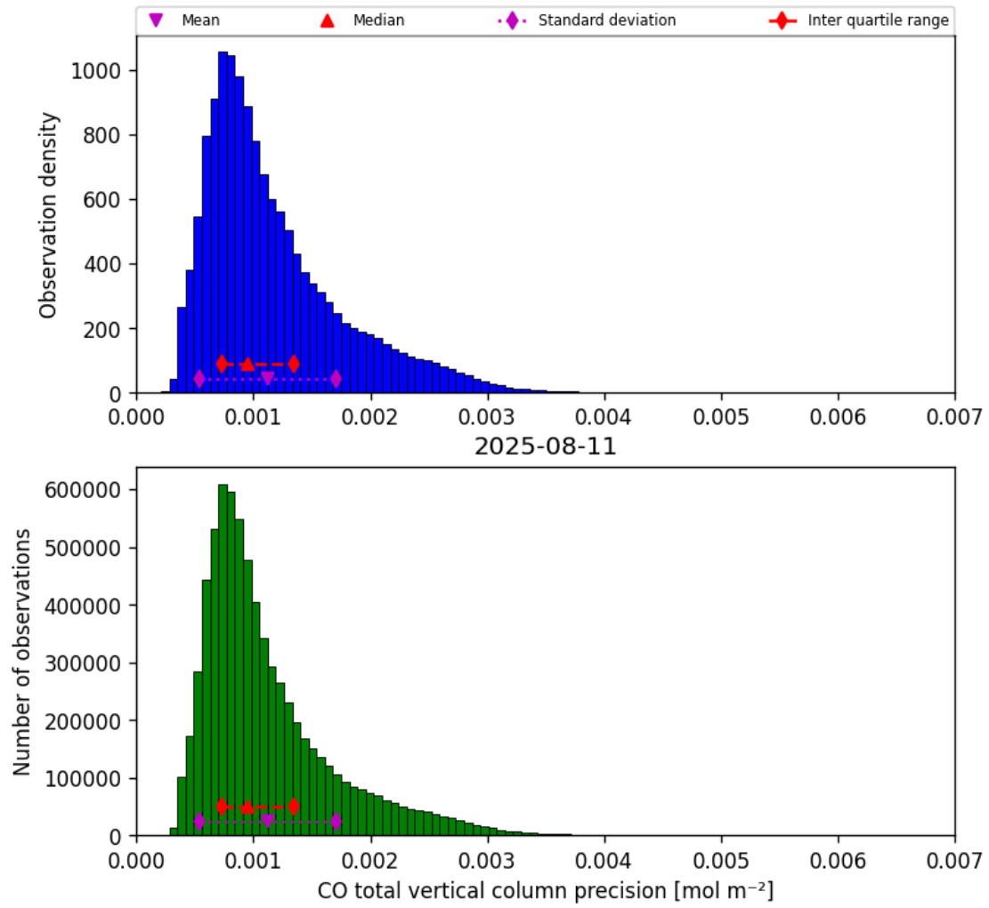
Figure 15: Histogram of “CO total vertical column precision” for 2025-08-11 to 2025-08-12
