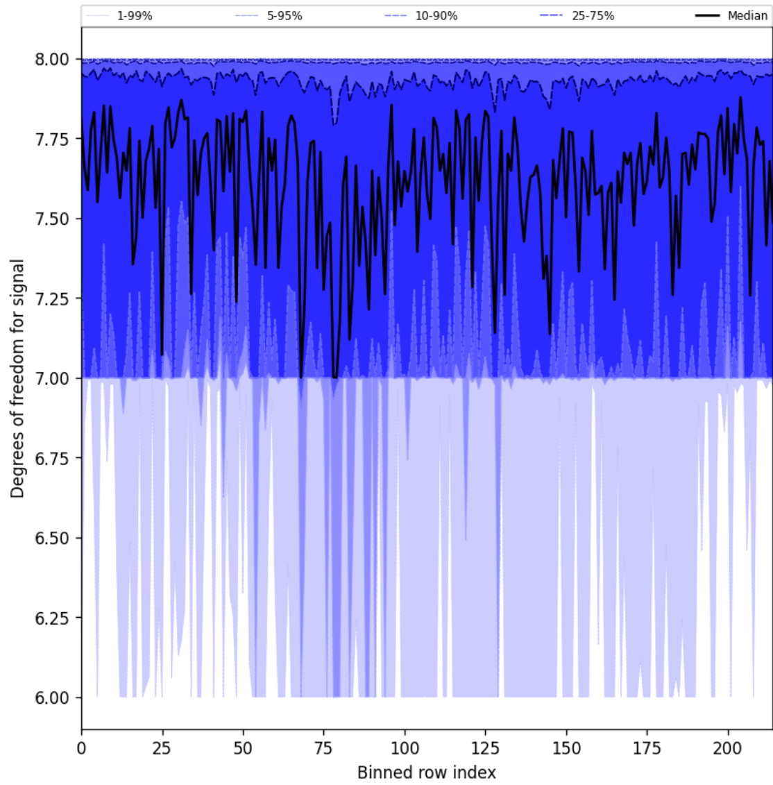
Figure 25: Along track statistics of “Degrees of freedom for signal” for 2025-08-11 to 2025-08-12
