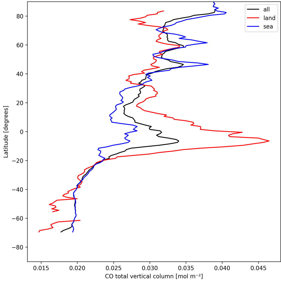
Figure 7: Zonal average of “CO total vertical column” for 2025-08-11 to 2025-08-12.
