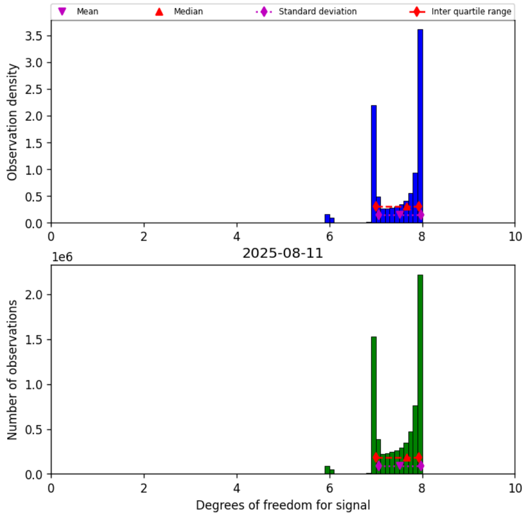
Figure 18: Histogram of “Degrees of freedom for signal” for 2025-08-11 to 2025-08-12
