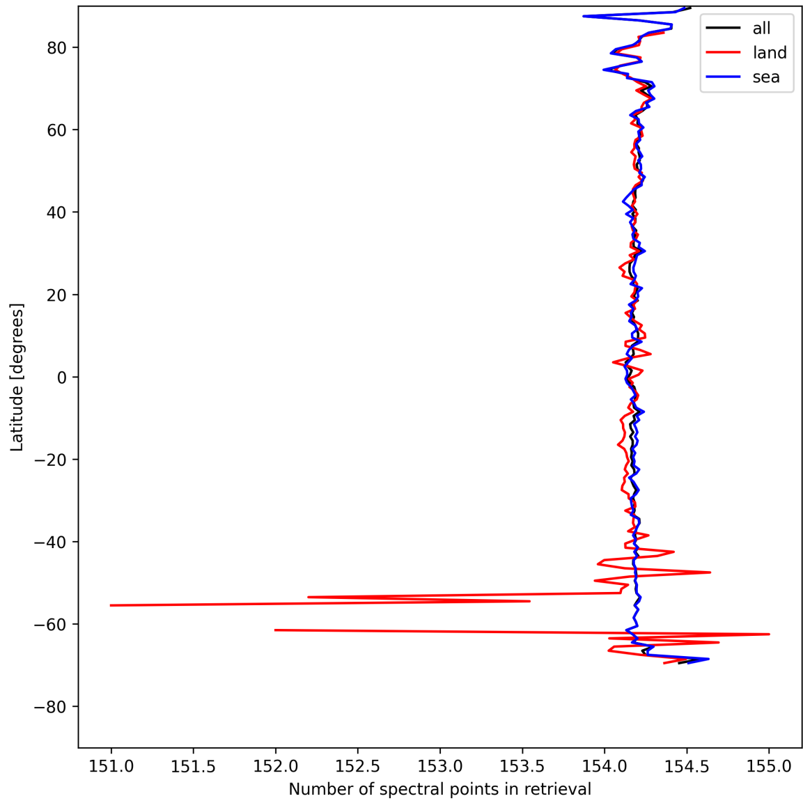
Figure 9: Zonal average of “Number of spectral points in retrieval” for 2025-08-11 to 2025-08-12.
