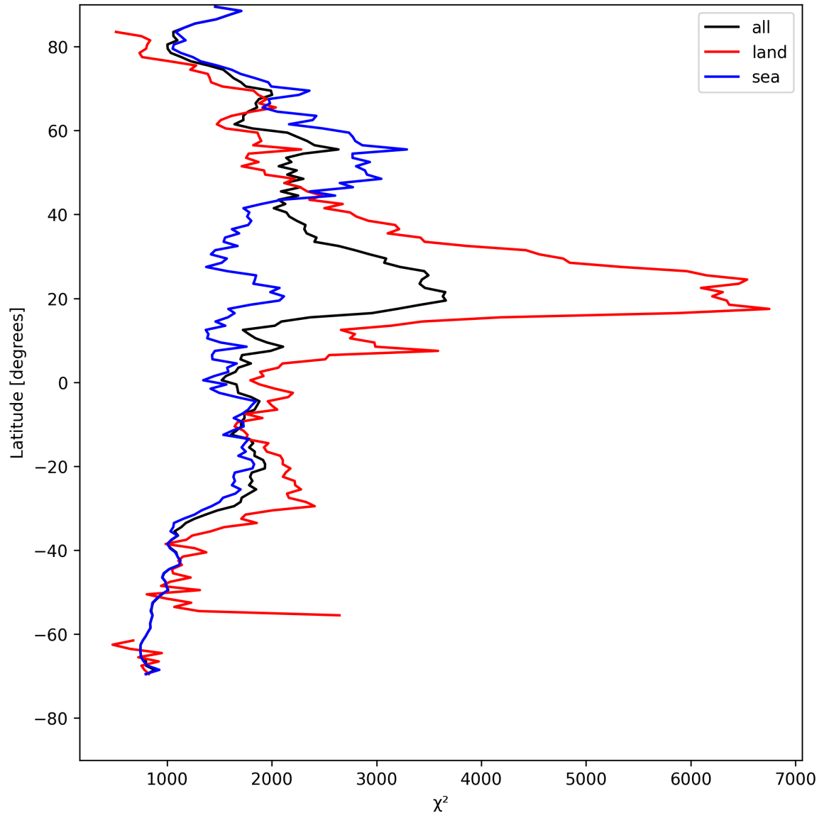
Figure 10: Zonal average of “ \chi^2 ” for 2025-08-11 to 2025-08-12.
