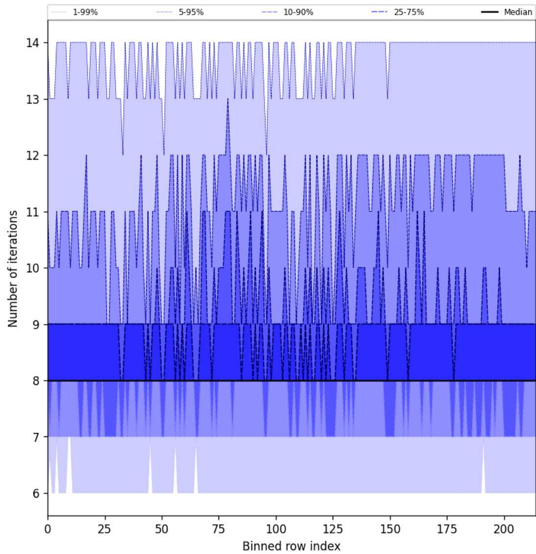
Figure 26: Along track statistics of “Number of iterations” for 2025-08-11 to 2025-08-12
