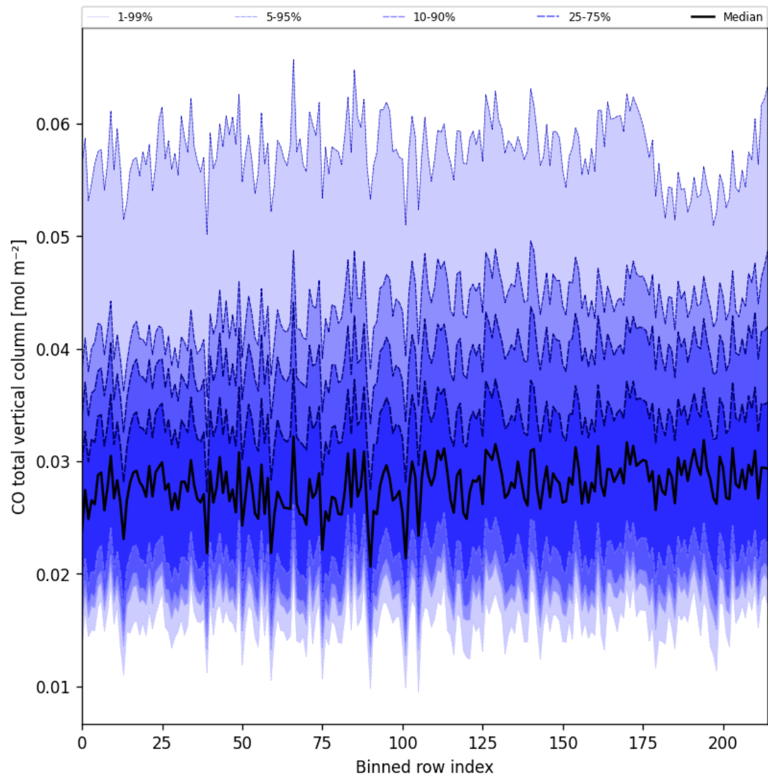
Figure 21: Along track statistics of “CO total vertical column” for 2025-08-11 to 2025-08-12
