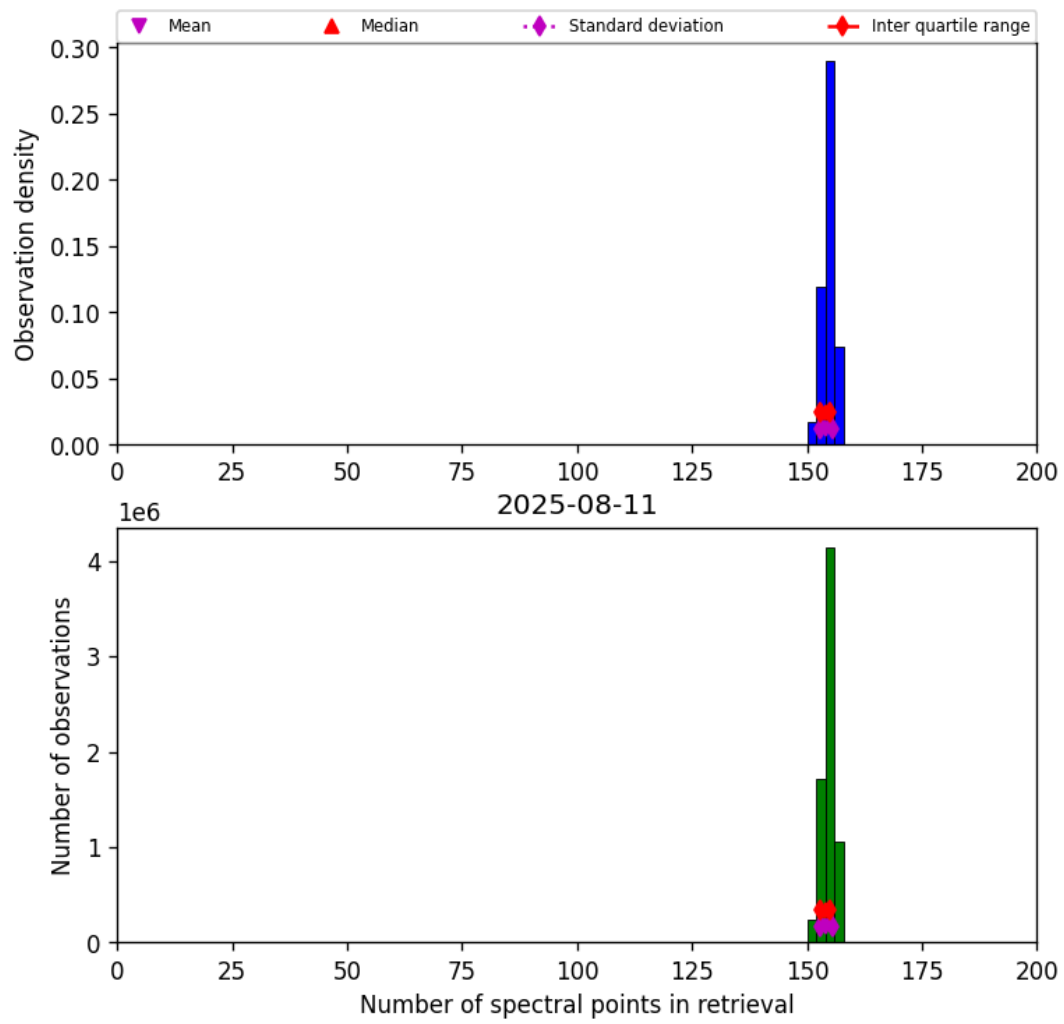
Figure 16: Histogram of “Number of spectral points in retrieval” for 2025-08-11 to 2025-08-12
