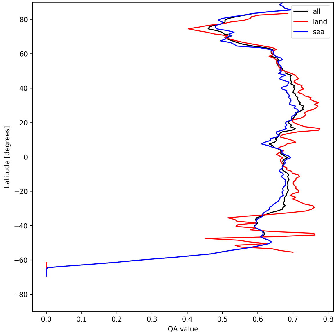
Figure 6: Zonal average of “QA value” for 2025-08-11 to 2025-08-12.
