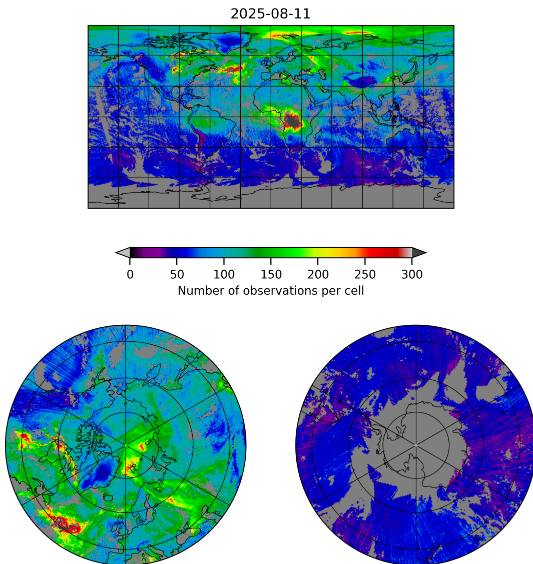
Figure 5: Map of the number of observations for 2025-08-11 to 2025-08-12
