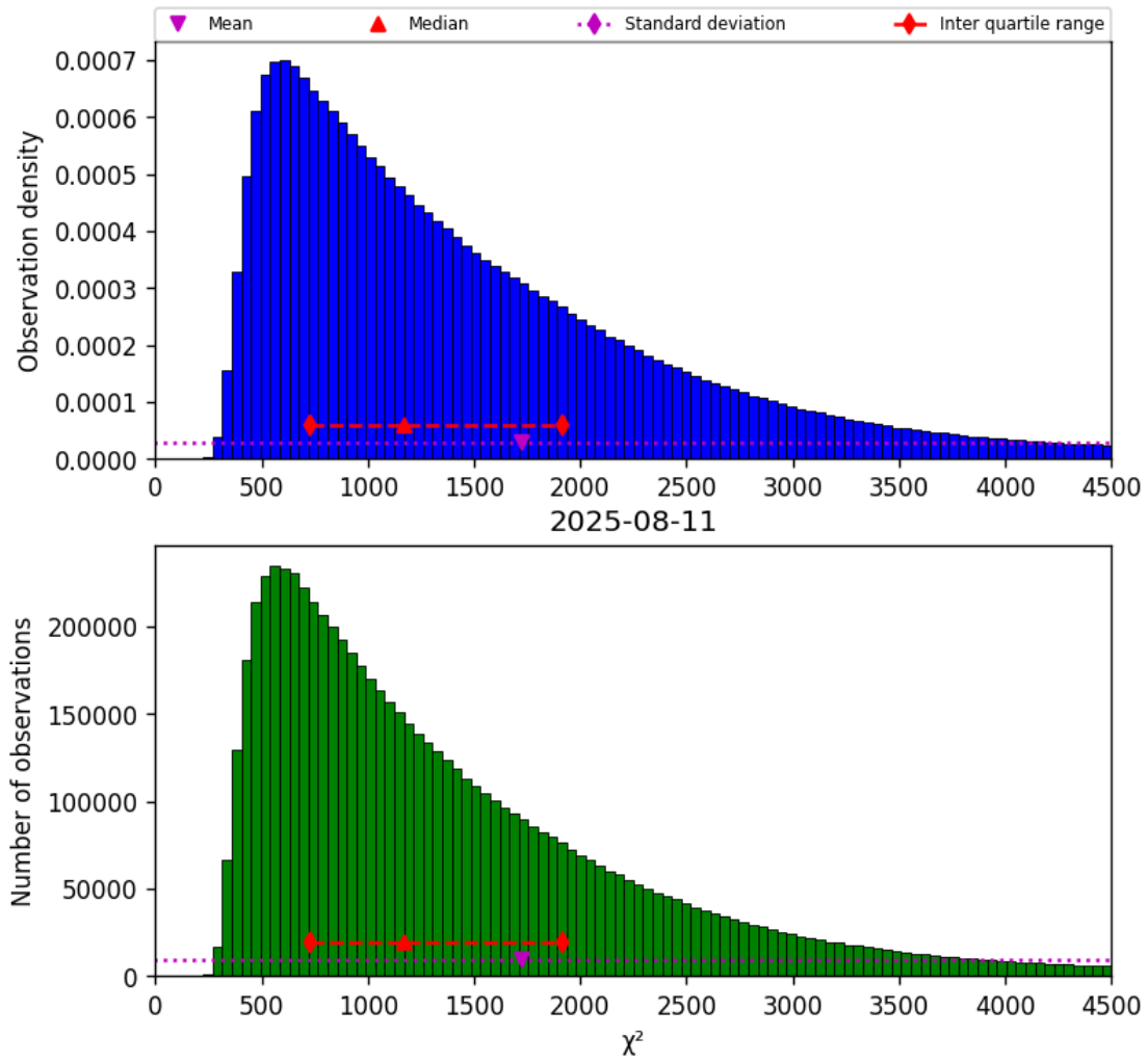
Figure 17: Histogram of “ \chi^2 ” for 2025-08-11 to 2025-08-12
