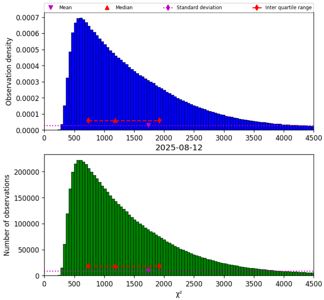
Figure 17: Histogram of “ \chi^2 ” for 2025-08-12 to 2025-08-12
