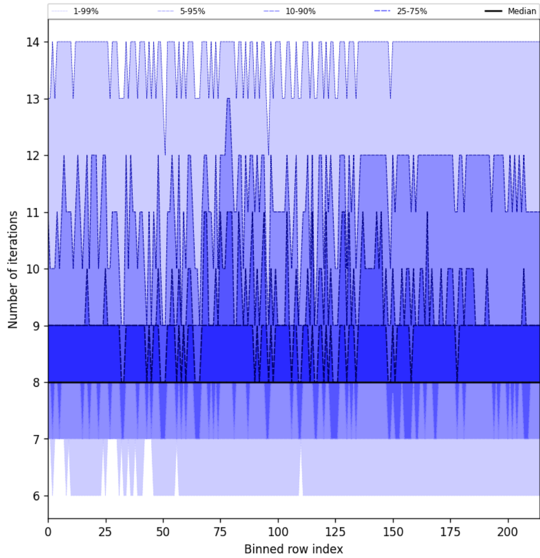
Figure 26: Along track statistics of “Number of iterations” for 2025-08-12 to 2025-08-12
