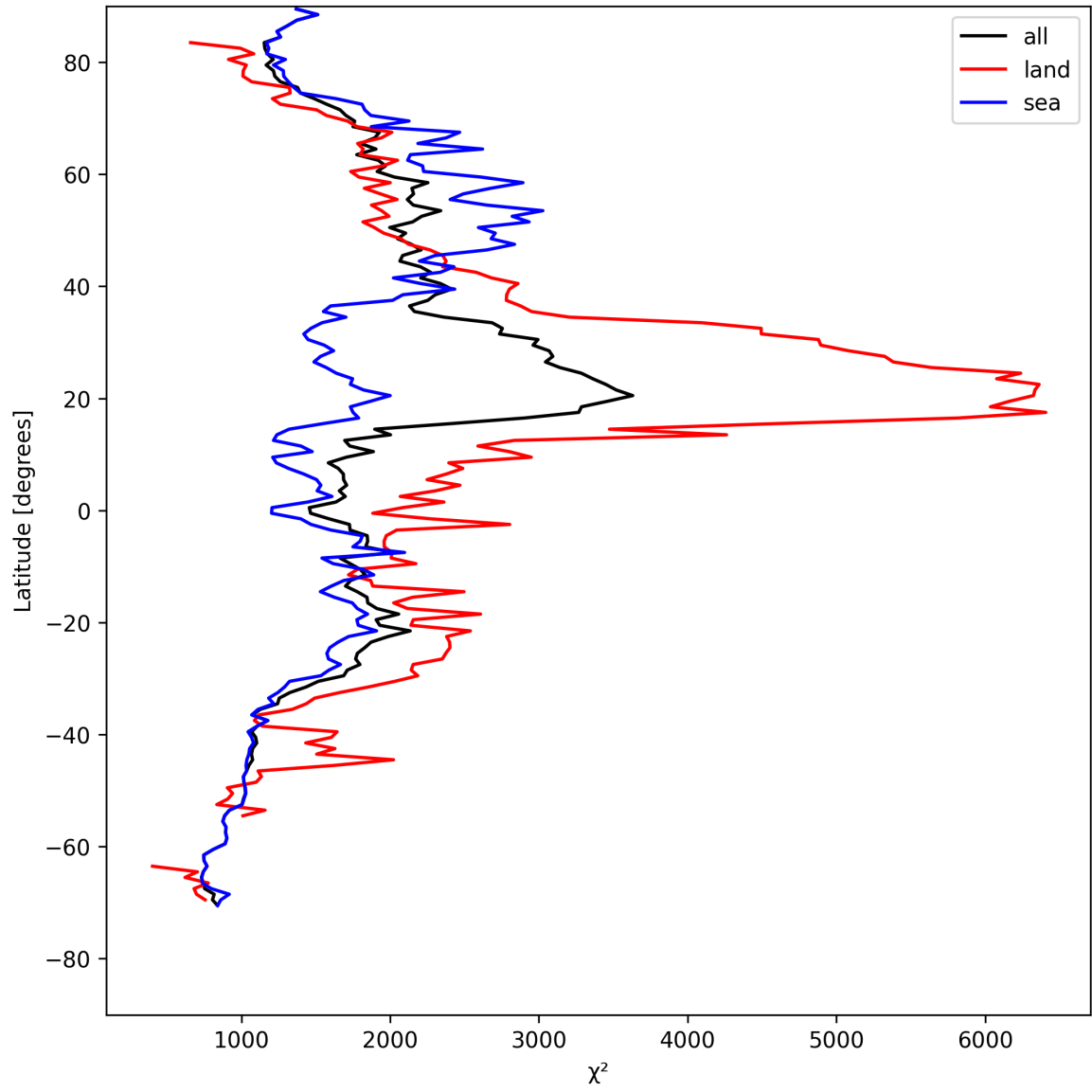
Figure 10: Zonal average of “ \chi^2 ” for 2025-08-12 to 2025-08-12.
