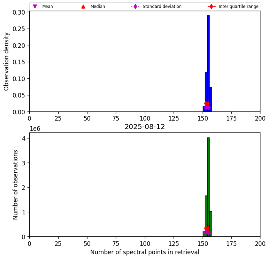
Figure 16: Histogram of “Number of spectral points in retrieval” for 2025-08-12 to 2025-08-12
