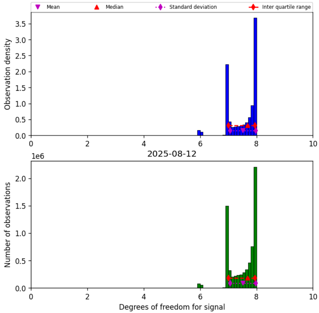
Figure 18: Histogram of “Degrees of freedom for signal” for 2025-08-12 to 2025-08-12
