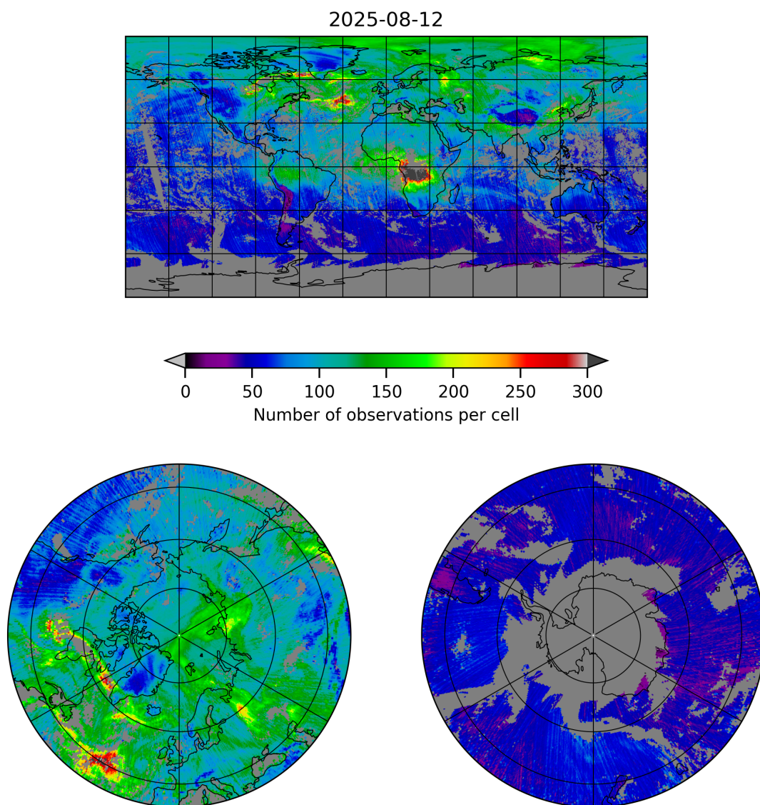
Figure 5: Map of the number of observations for 2025-08-12 to 2025-08-12
