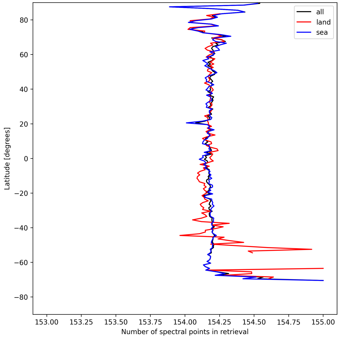
Figure 9: Zonal average of “Number of spectral points in retrieval” for 2025-08-12 to 2025-08-12.
