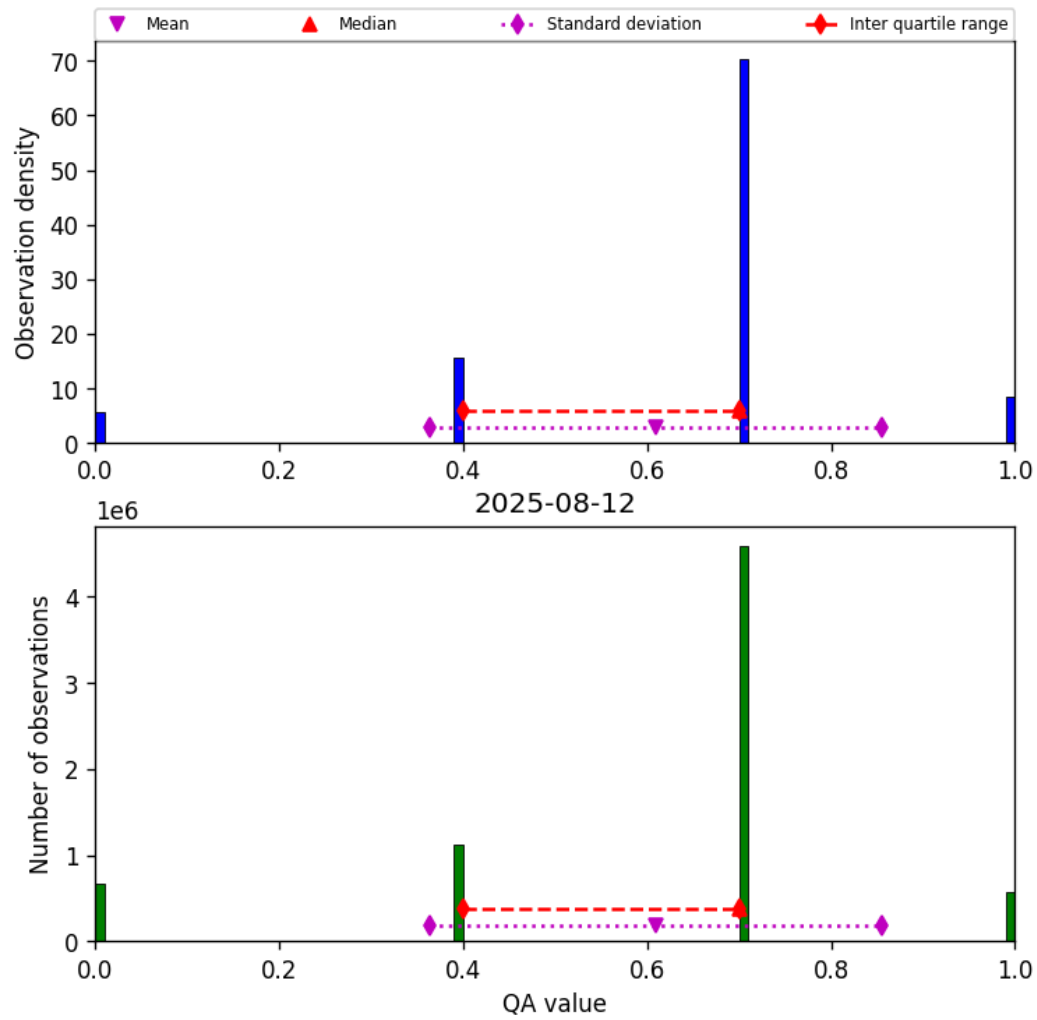
Figure 13: Histogram of “QA value” for 2025-08-12 to 2025-08-12
