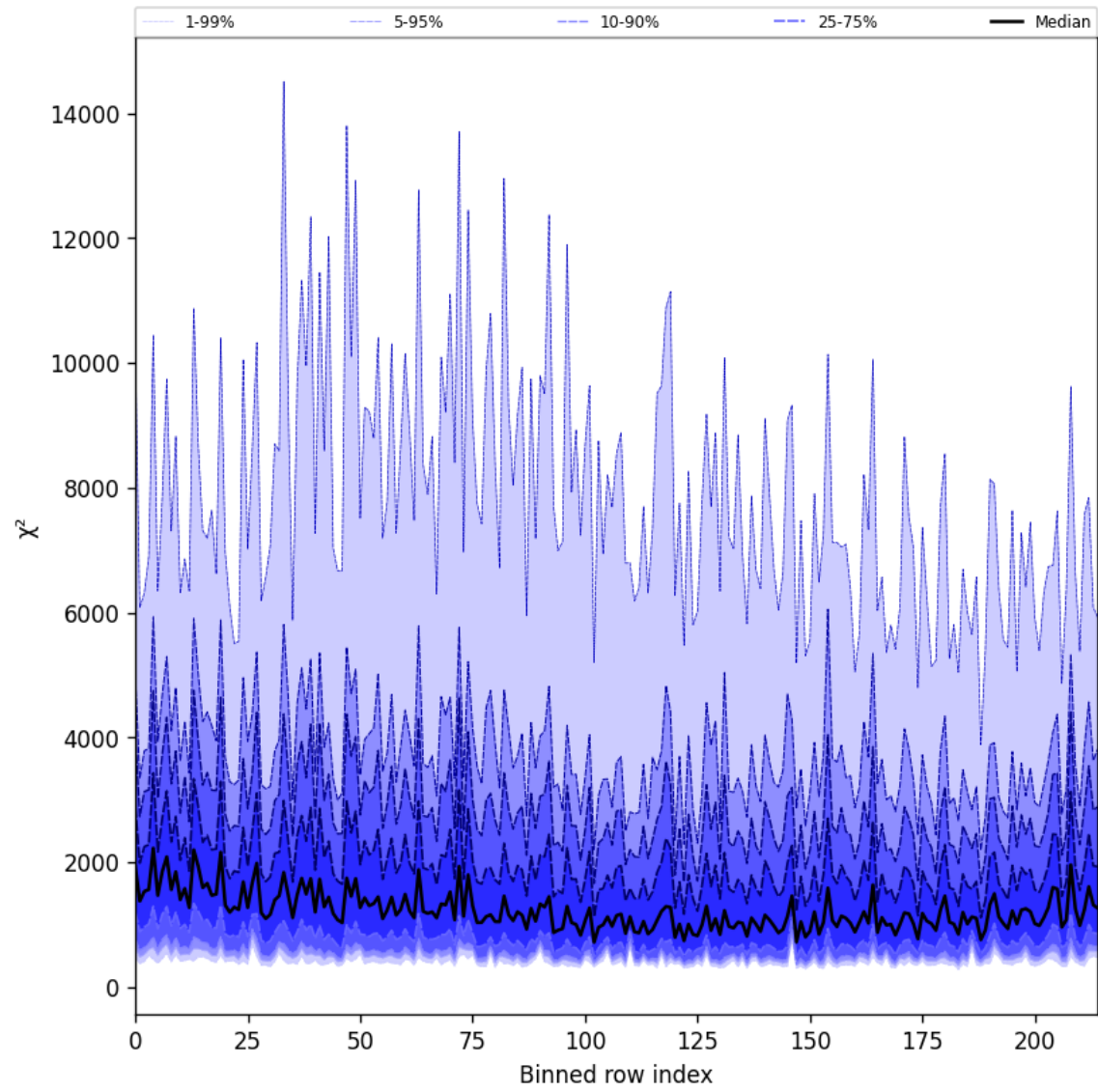
Figure 24: Along track statistics of “ \chi^2 ” for 2025-08-12 to 2025-08-12
