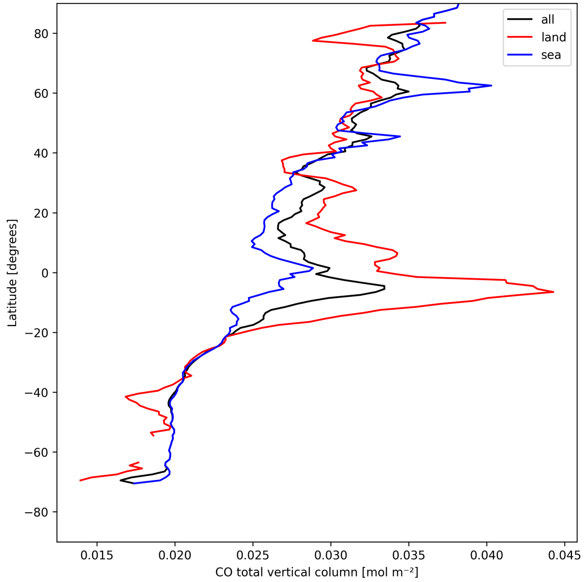
Figure 7: Zonal average of “CO total vertical column” for 2025-08-12 to 2025-08-12.
