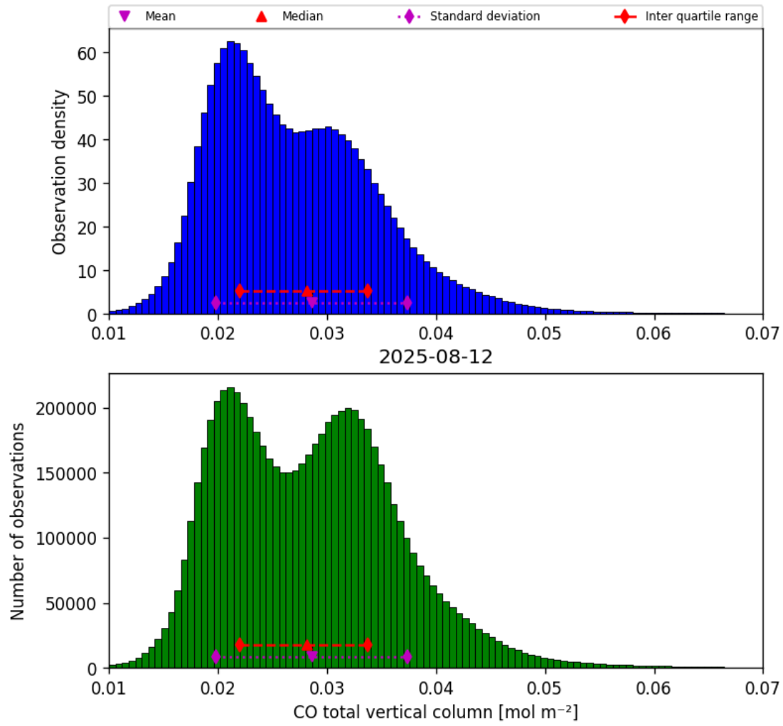
Figure 14: Histogram of “CO total vertical column” for 2025-08-12 to 2025-08-12
