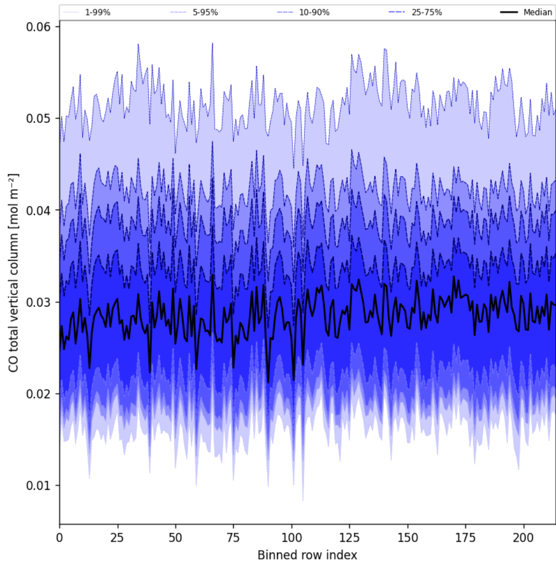
Figure 21: Along track statistics of “CO total vertical column” for 2025-08-12 to 2025-08-12
