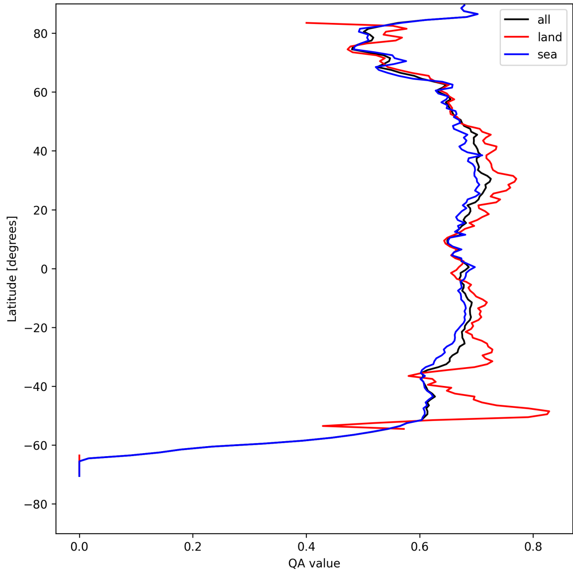
Figure 6: Zonal average of “QA value” for 2025-08-12 to 2025-08-12.
