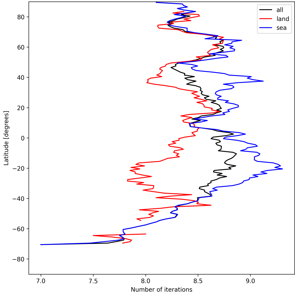
Figure 12: Zonal average of “Number of iterations” for 2025-08-12 to 2025-08-12.
