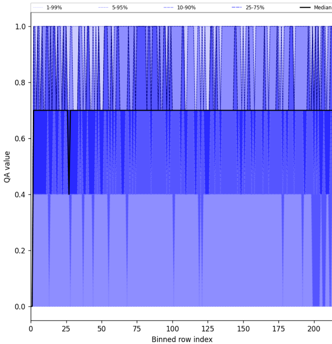
Figure 20: Along track statistics of “QA value” for 2025-08-12 to 2025-08-12
