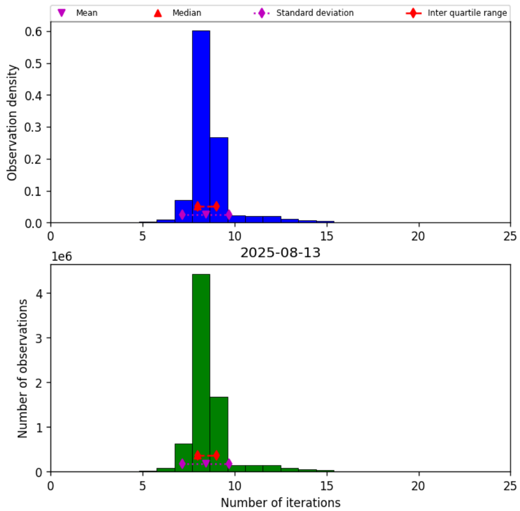
Figure 19: Histogram of “Number of iterations” for 2025-08-13 to 2025-08-14
