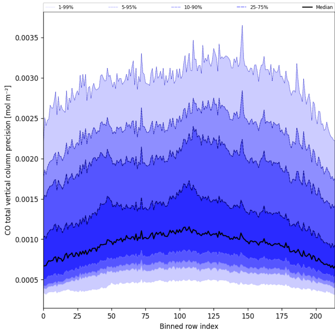
Figure 22: Along track statistics of “CO total vertical column precision” for 2025-08-13 to 2025-08-14
