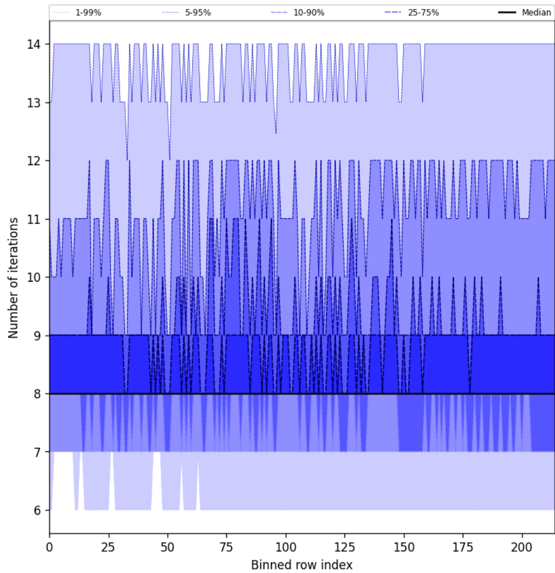
Figure 26: Along track statistics of “Number of iterations” for 2025-08-13 to 2025-08-14
