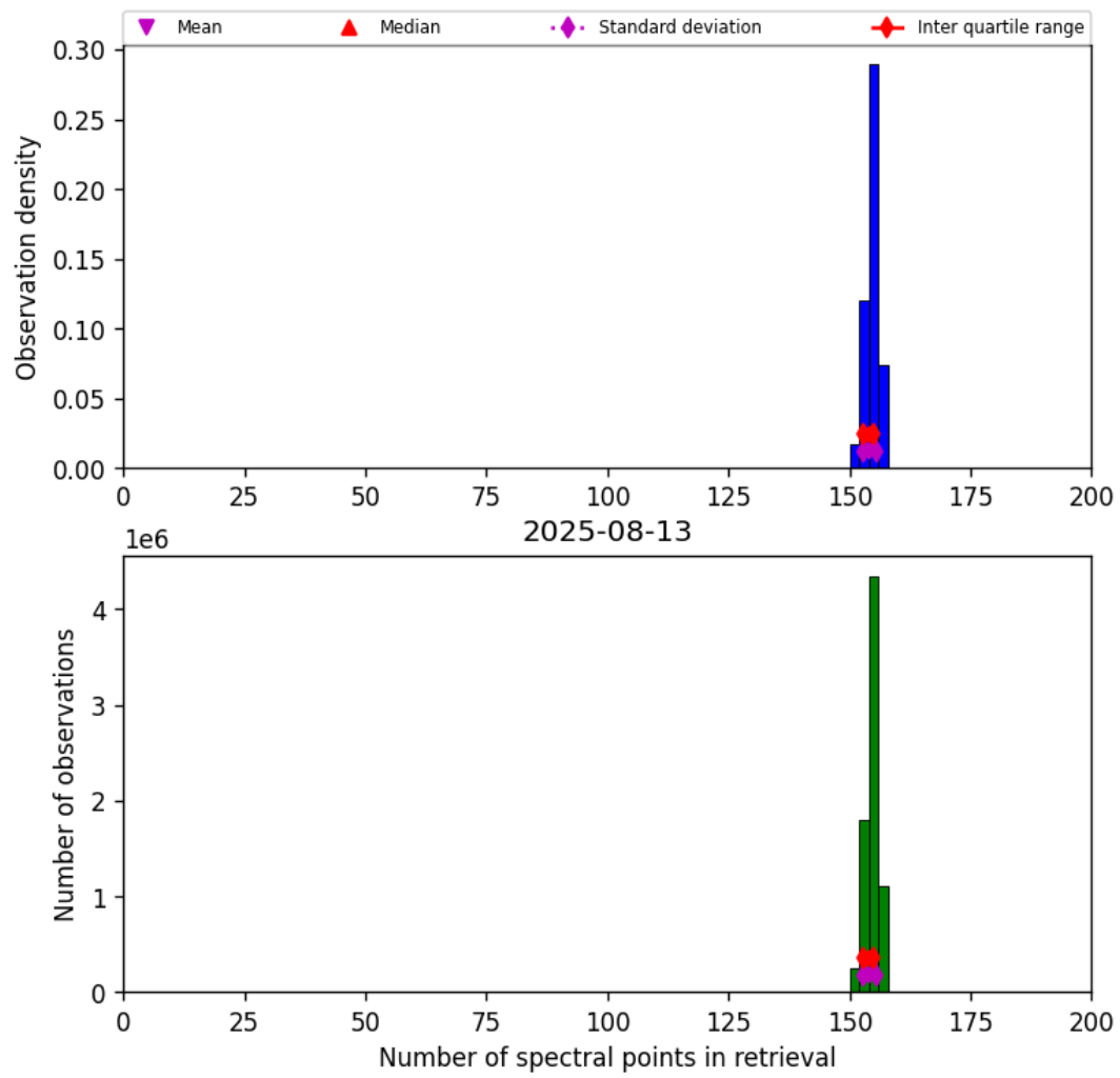
Figure 16: Histogram of “Number of spectral points in retrieval” for 2025-08-13 to 2025-08-14
