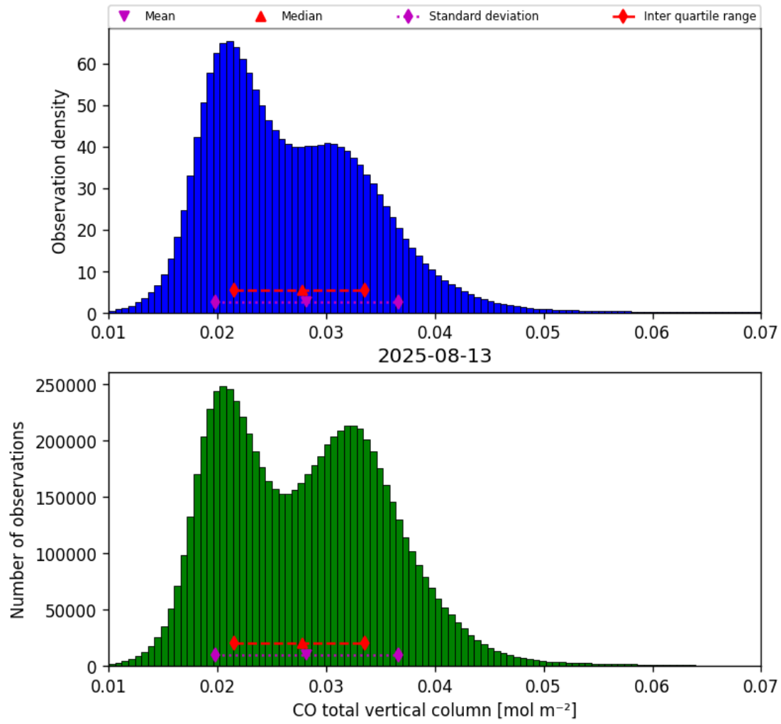
Figure 14: Histogram of “CO total vertical column” for 2025-08-13 to 2025-08-14
