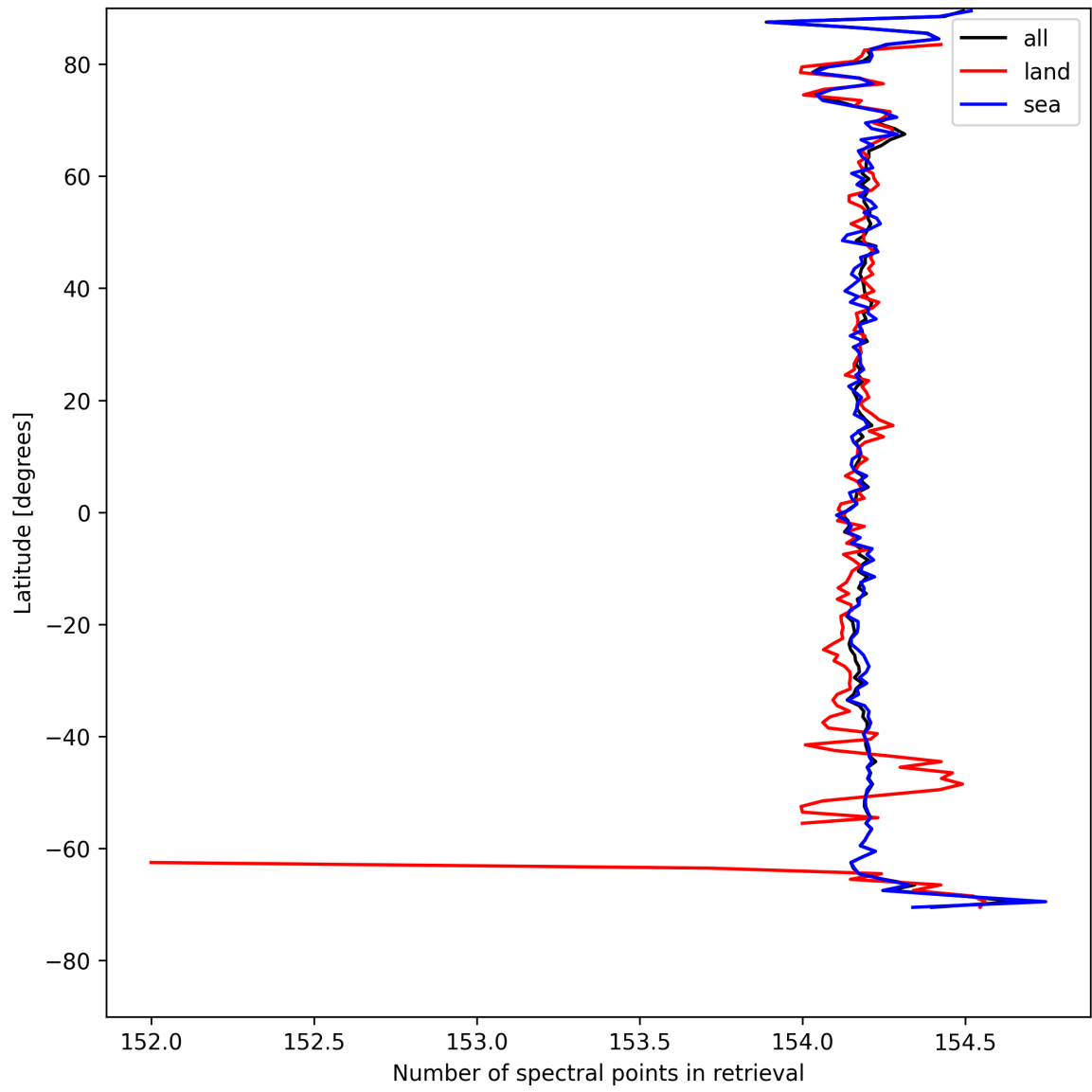
Figure 9: Zonal average of “Number of spectral points in retrieval” for 2025-08-13 to 2025-08-14.
