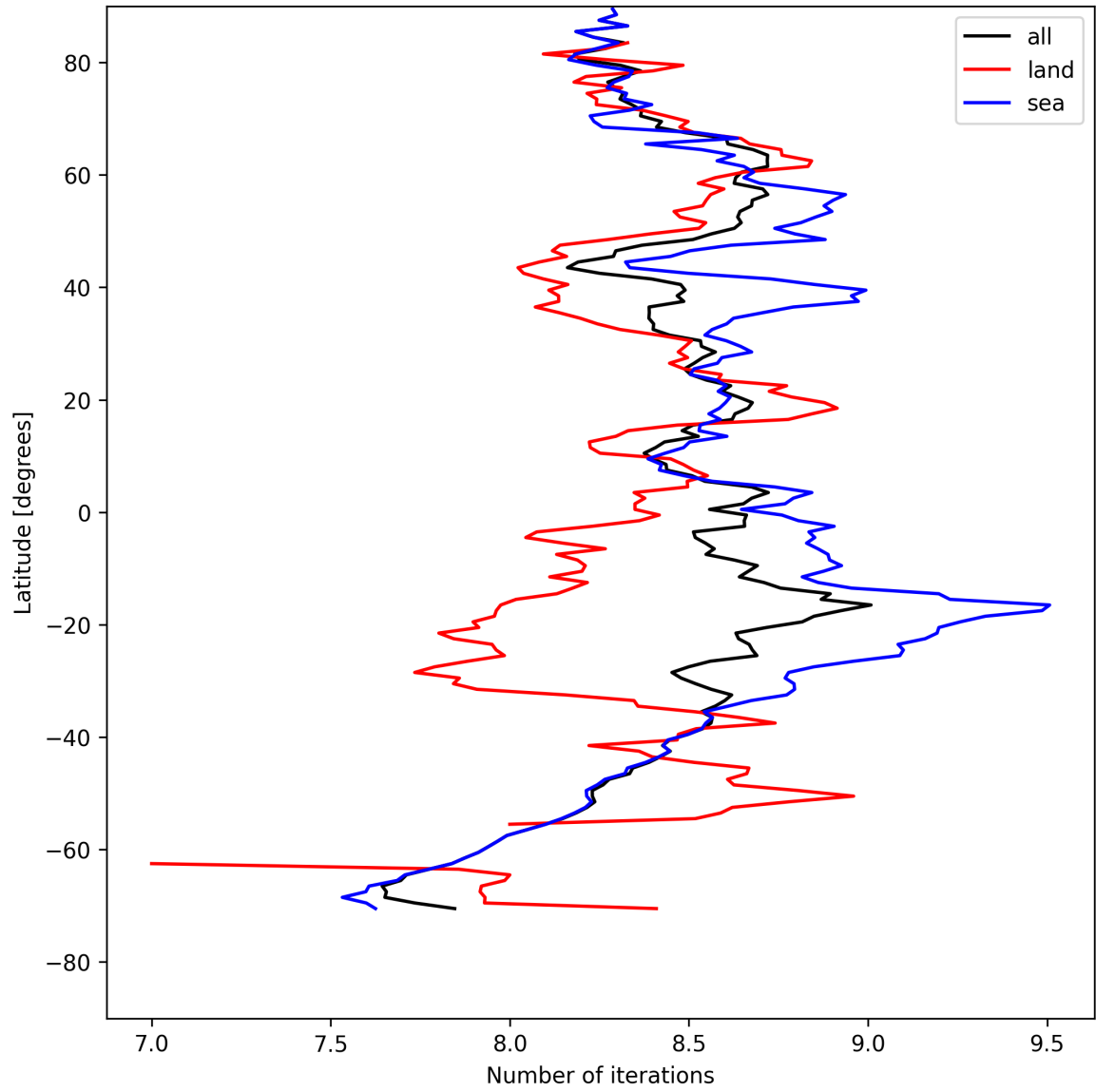
Figure 12: Zonal average of “Number of iterations” for 2025-08-13 to 2025-08-14.
