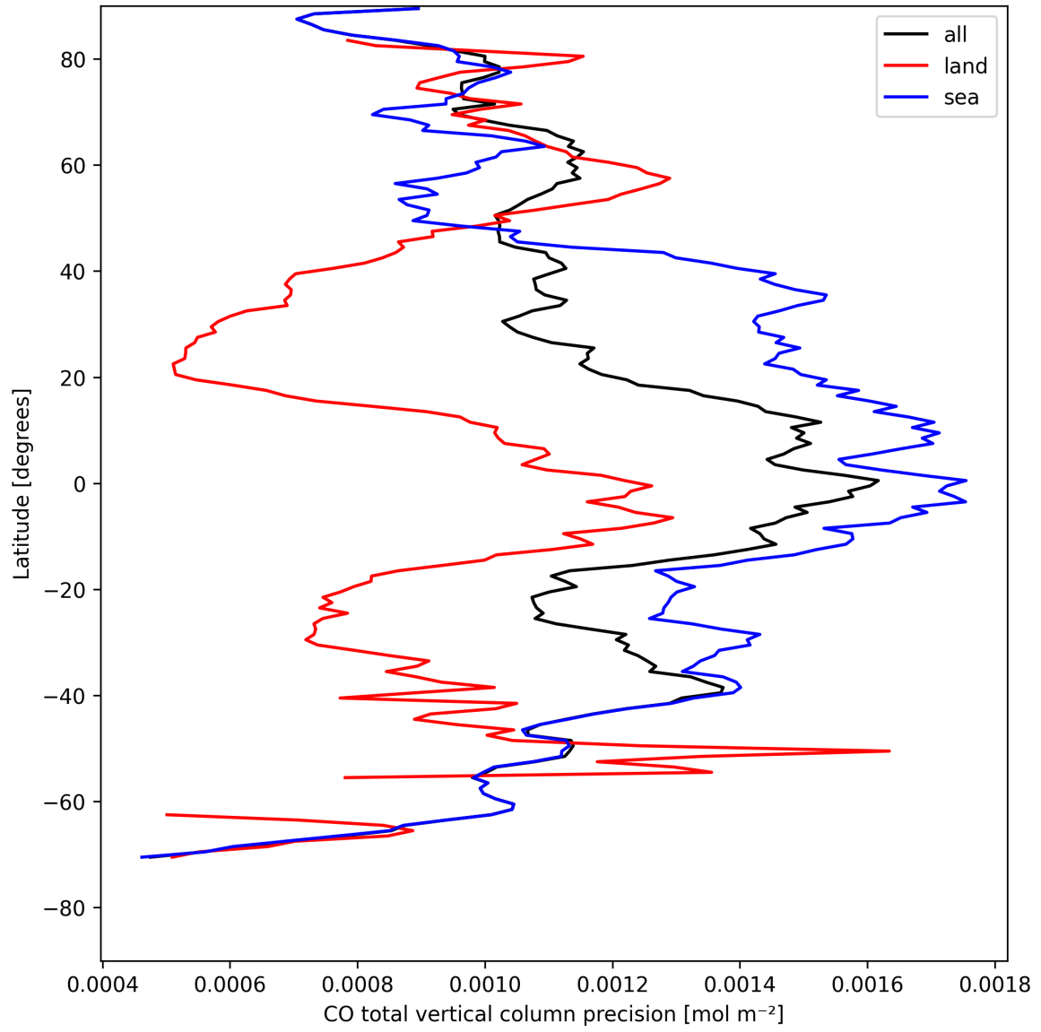
Figure 8: Zonal average of "CO total vertical column precision" for 2025-08-13 to 2025-08-14.
