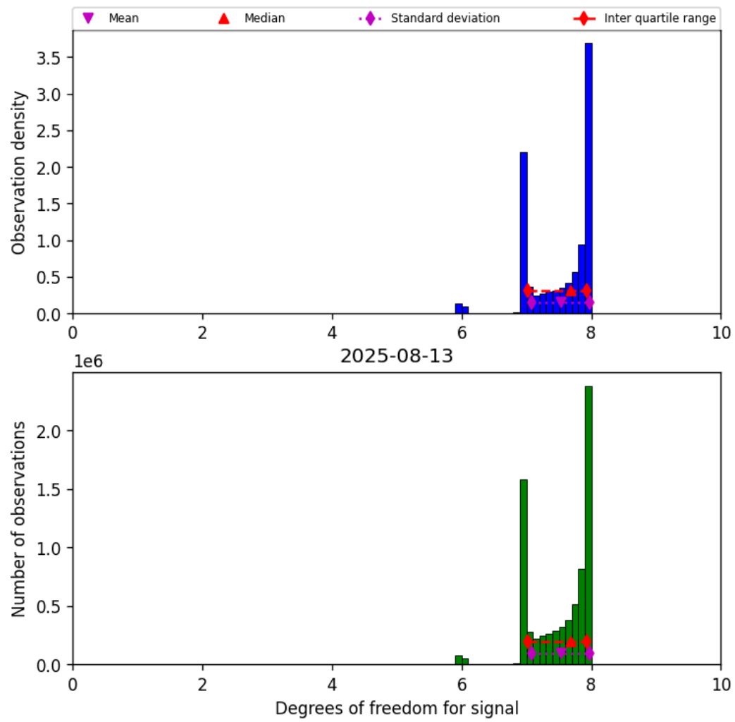
Figure 18: Histogram of “Degrees of freedom for signal” for 2025-08-13 to 2025-08-14
