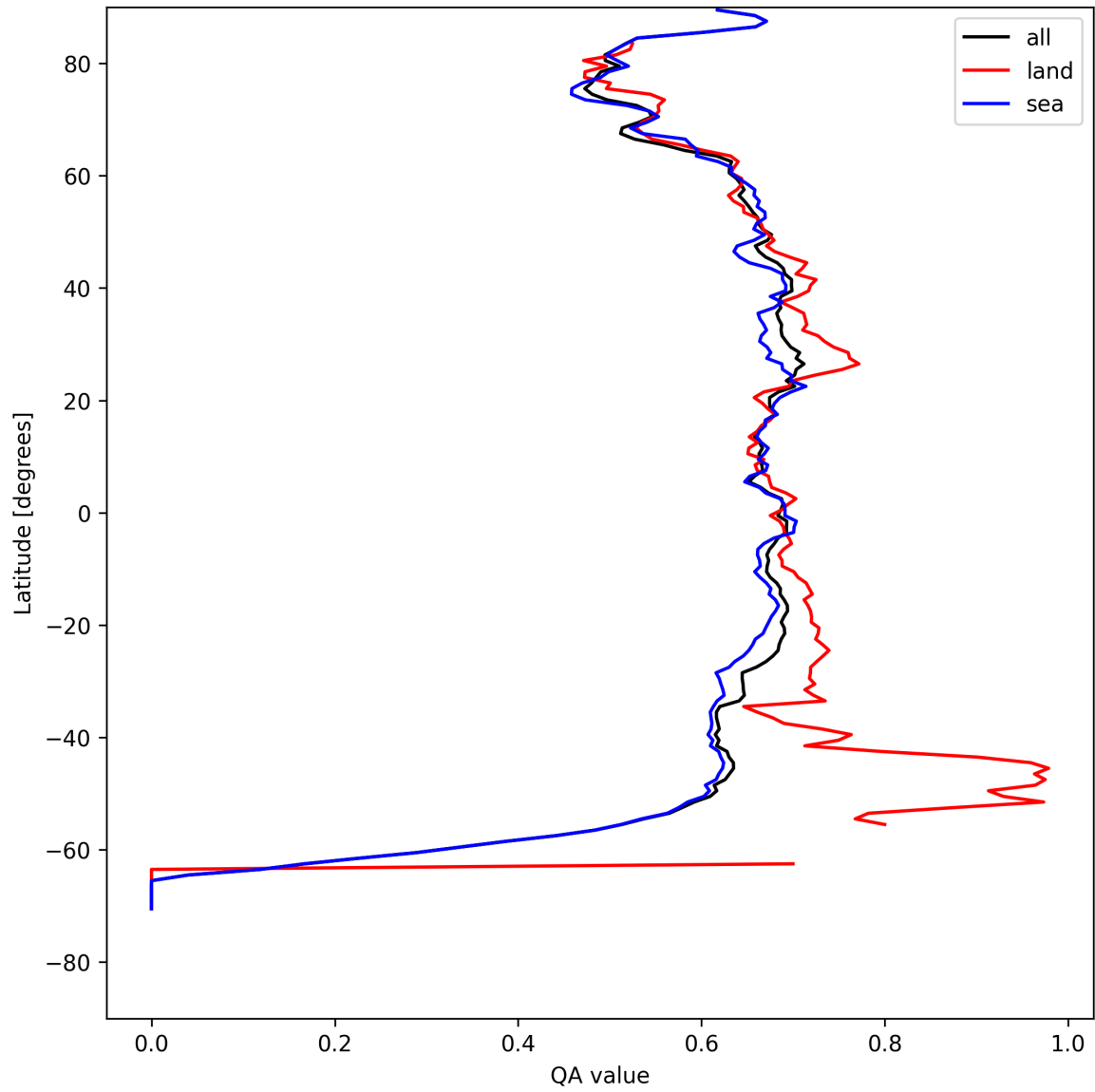
Figure 6: Zonal average of “QA value” for 2025-08-13 to 2025-08-14.
