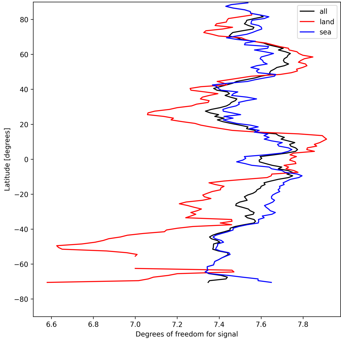
Figure 11: Zonal average of “Degrees of freedom for signal” for 2025-08-13 to 2025-08-14.
