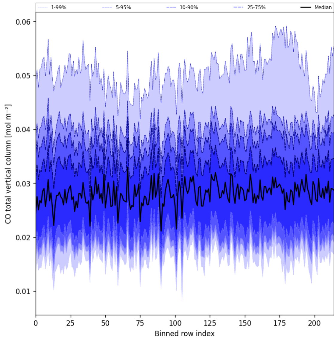
Figure 21: Along track statistics of “CO total vertical column” for 2025-08-13 to 2025-08-14
