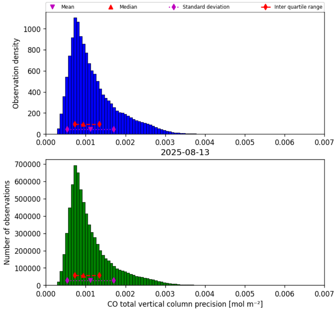
Figure 15: Histogram of “CO total vertical column precision” for 2025-08-13 to 2025-08-14
