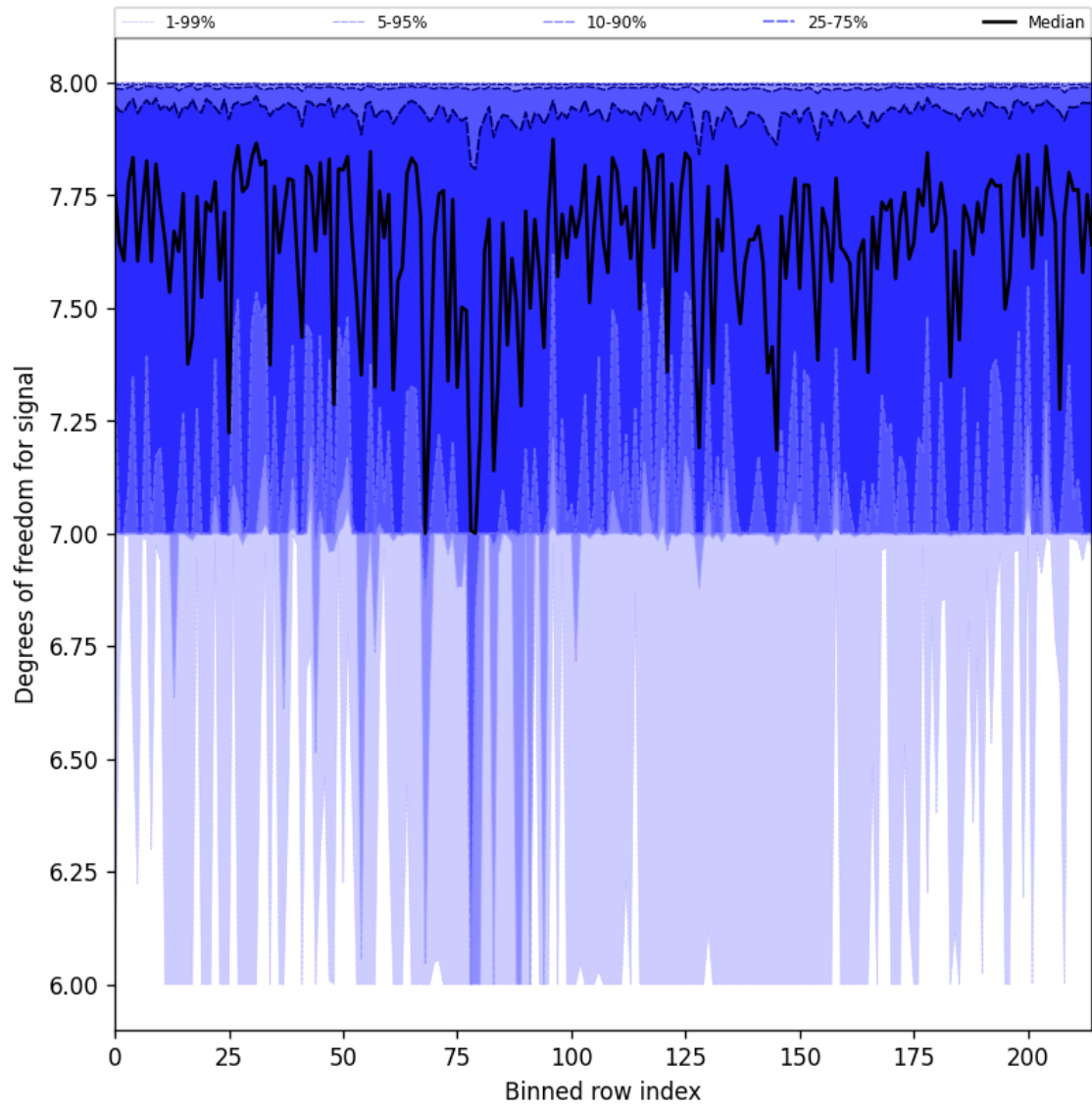
Figure 25: Along track statistics of “Degrees of freedom for signal” for 2025-08-13 to 2025-08-14
