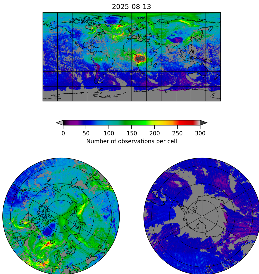
Figure 5: Map of the number of observations for 2025-08-13 to 2025-08-14
