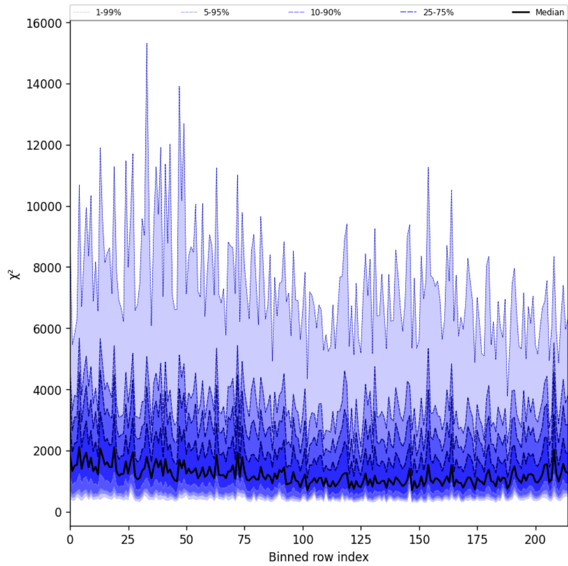
Figure 24: Along track statistics of “ \chi^2 ” for 2025-08-13 to 2025-08-14
