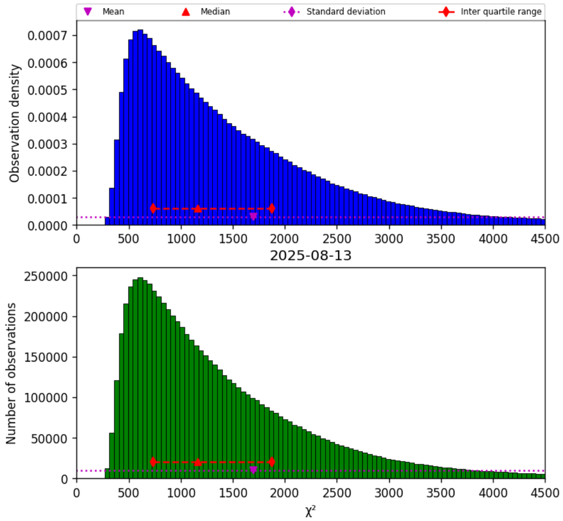
Figure 17: Histogram of “ \chi^2 ” for 2025-08-13 to 2025-08-14
