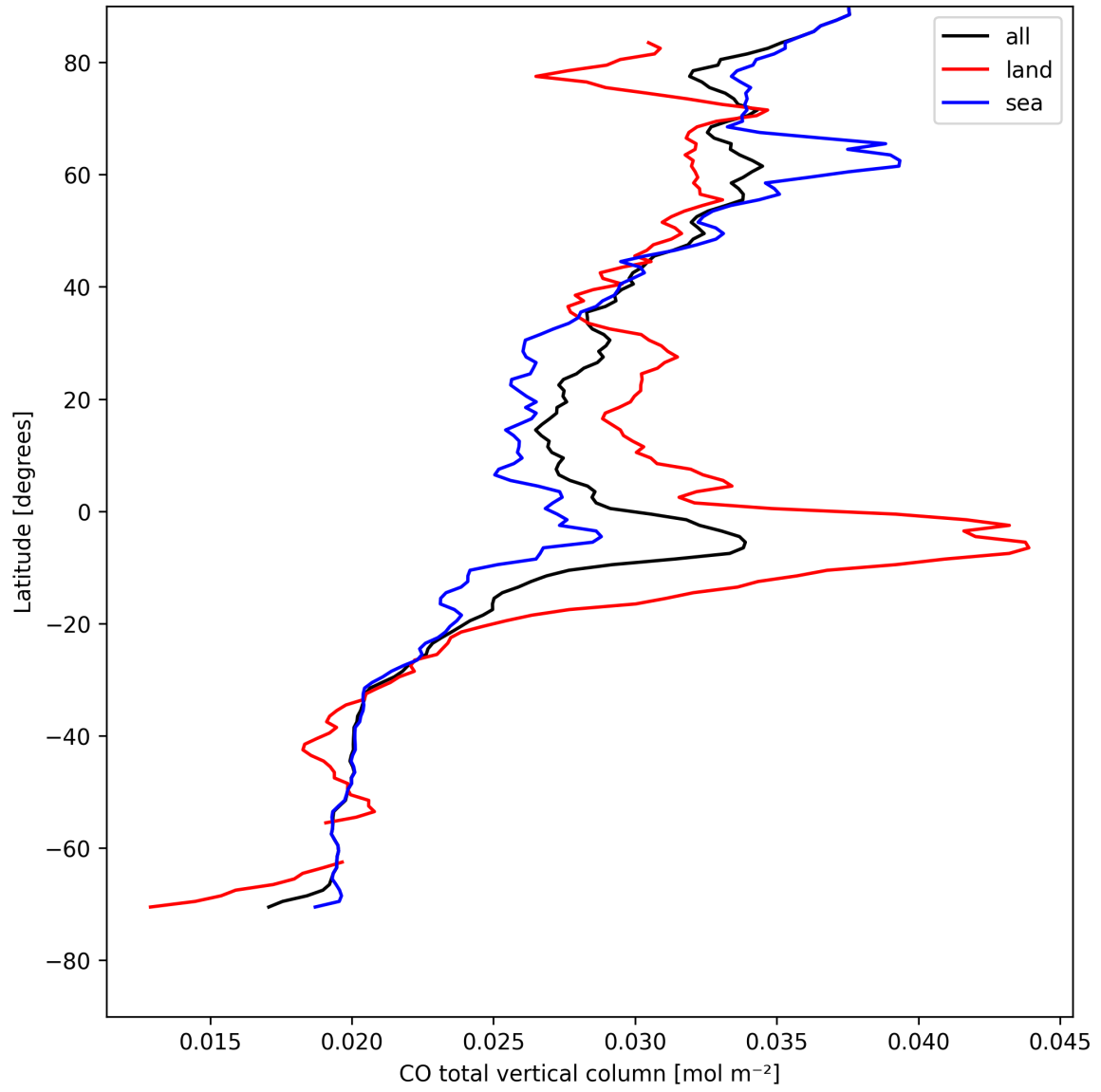
Figure 7: Zonal average of “CO total vertical column” for 2025-08-13 to 2025-08-14.
