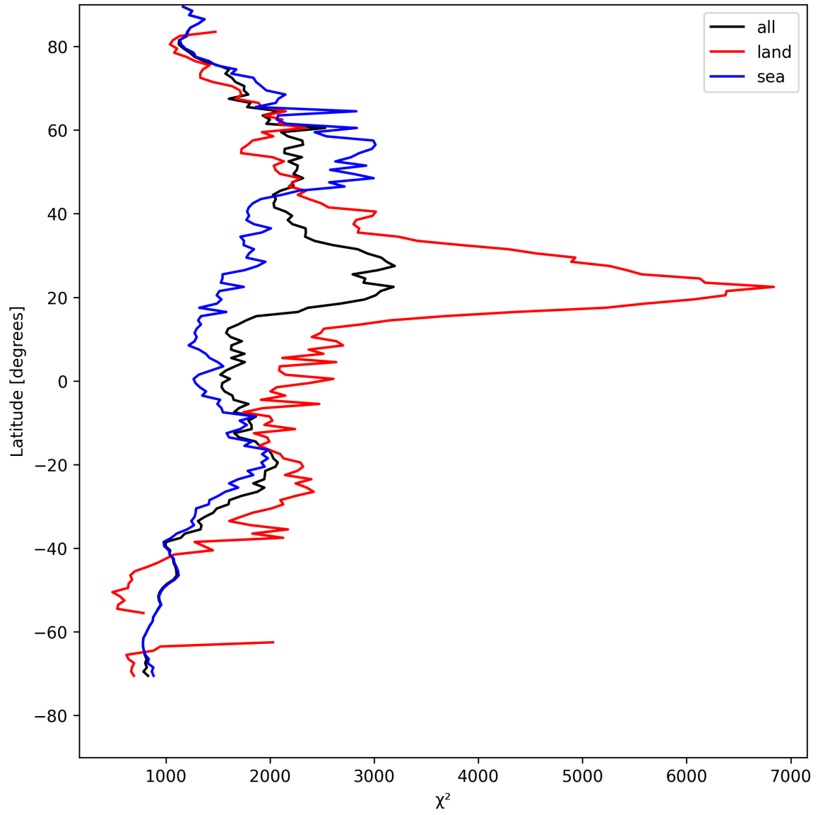
Figure 10: Zonal average of “ \chi^2 ” for 2025-08-13 to 2025-08-14.
