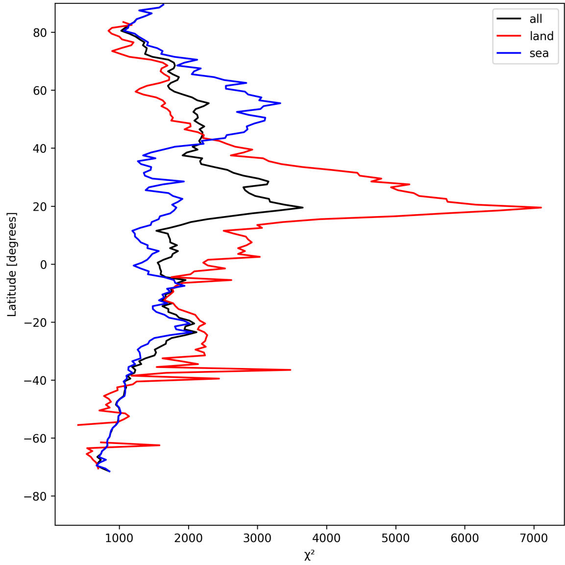
Figure 10: Zonal average of “ \chi^2 ” for 2025-08-15 to 2025-08-16.
