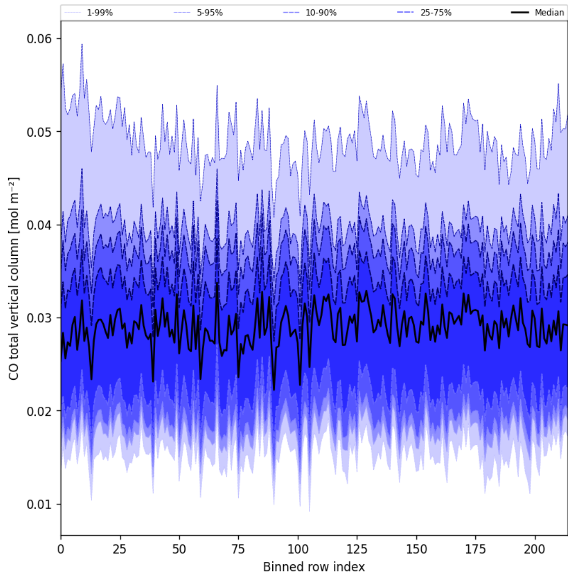
Figure 21: Along track statistics of “CO total vertical column” for 2025-08-15 to 2025-08-16
