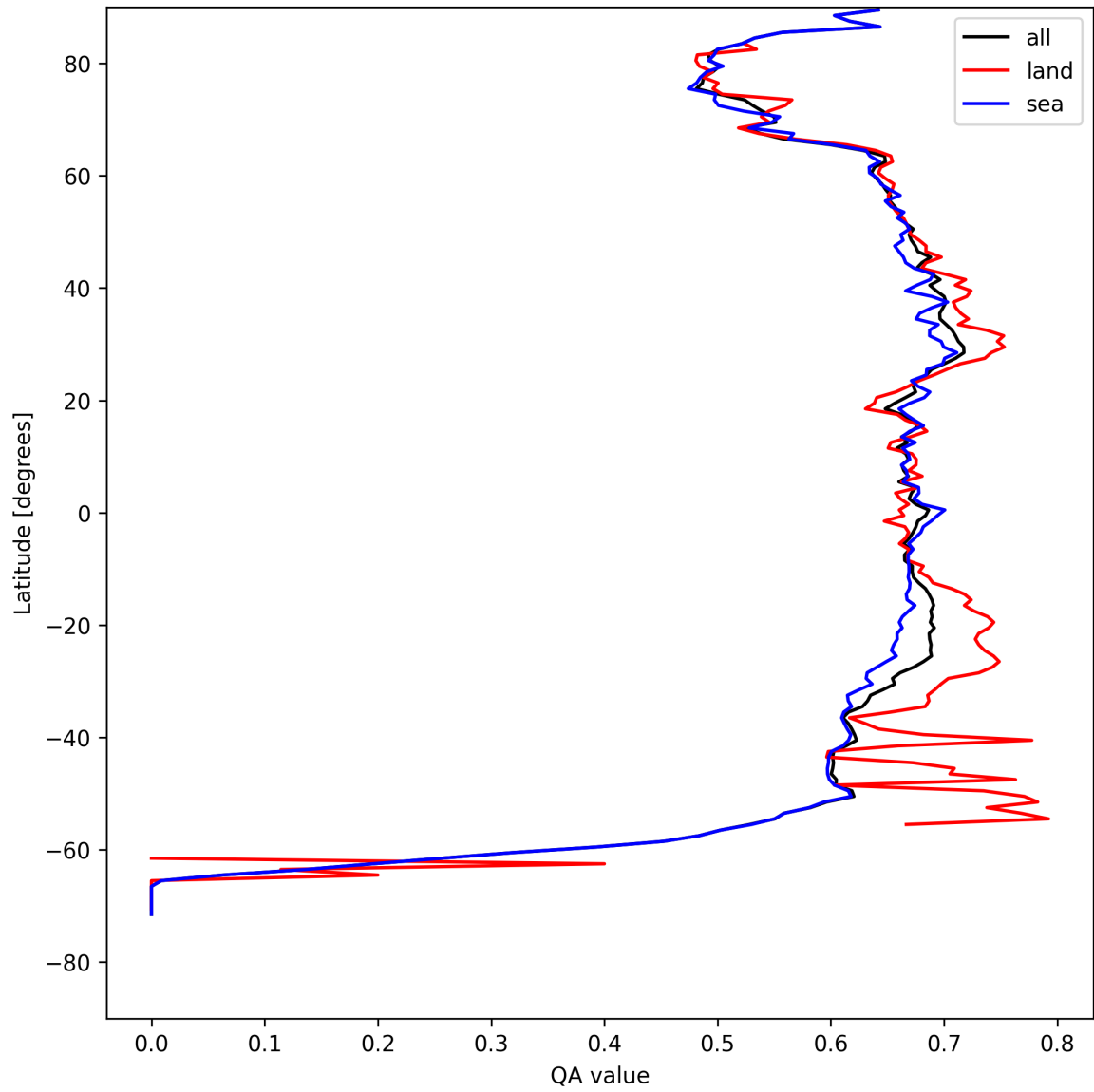
Figure 6: Zonal average of “QA value” for 2025-08-15 to 2025-08-16.
