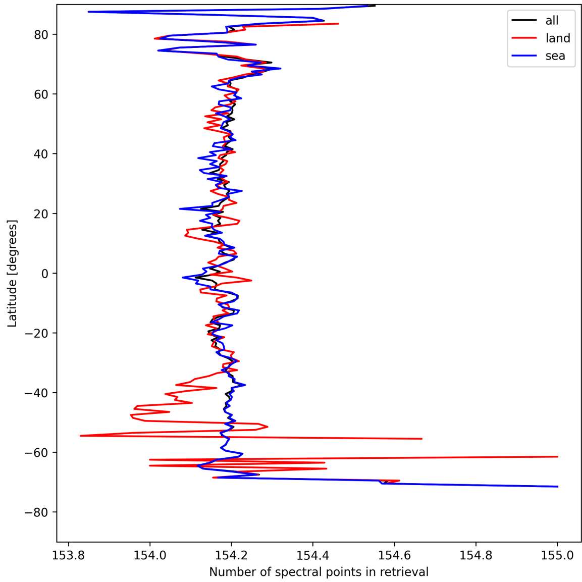
Figure 9: Zonal average of “Number of spectral points in retrieval” for 2025-08-15 to 2025-08-16.
