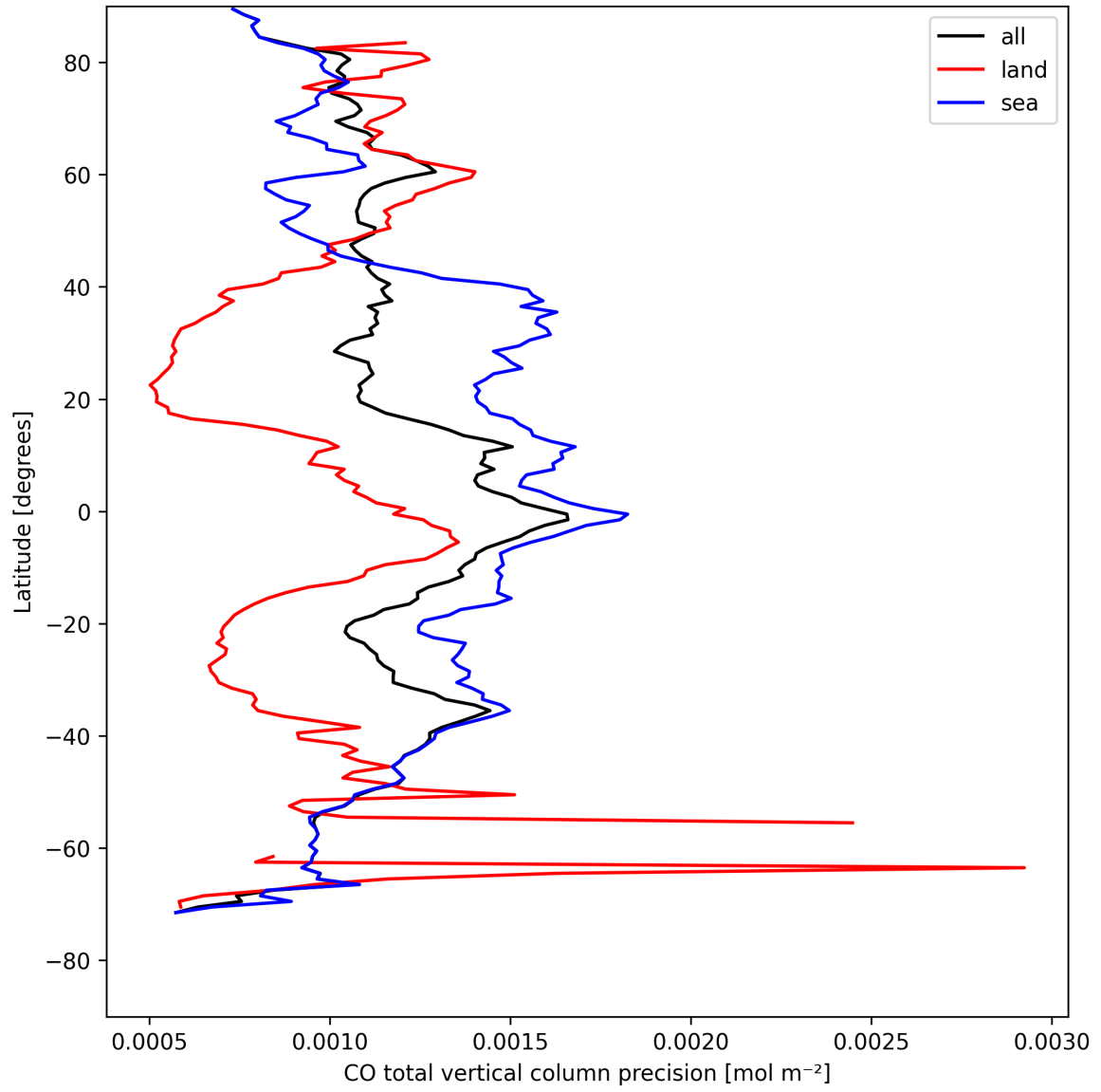
Figure 8: Zonal average of “CO total vertical column precision” for 2025-08-15 to 2025-08-16.
