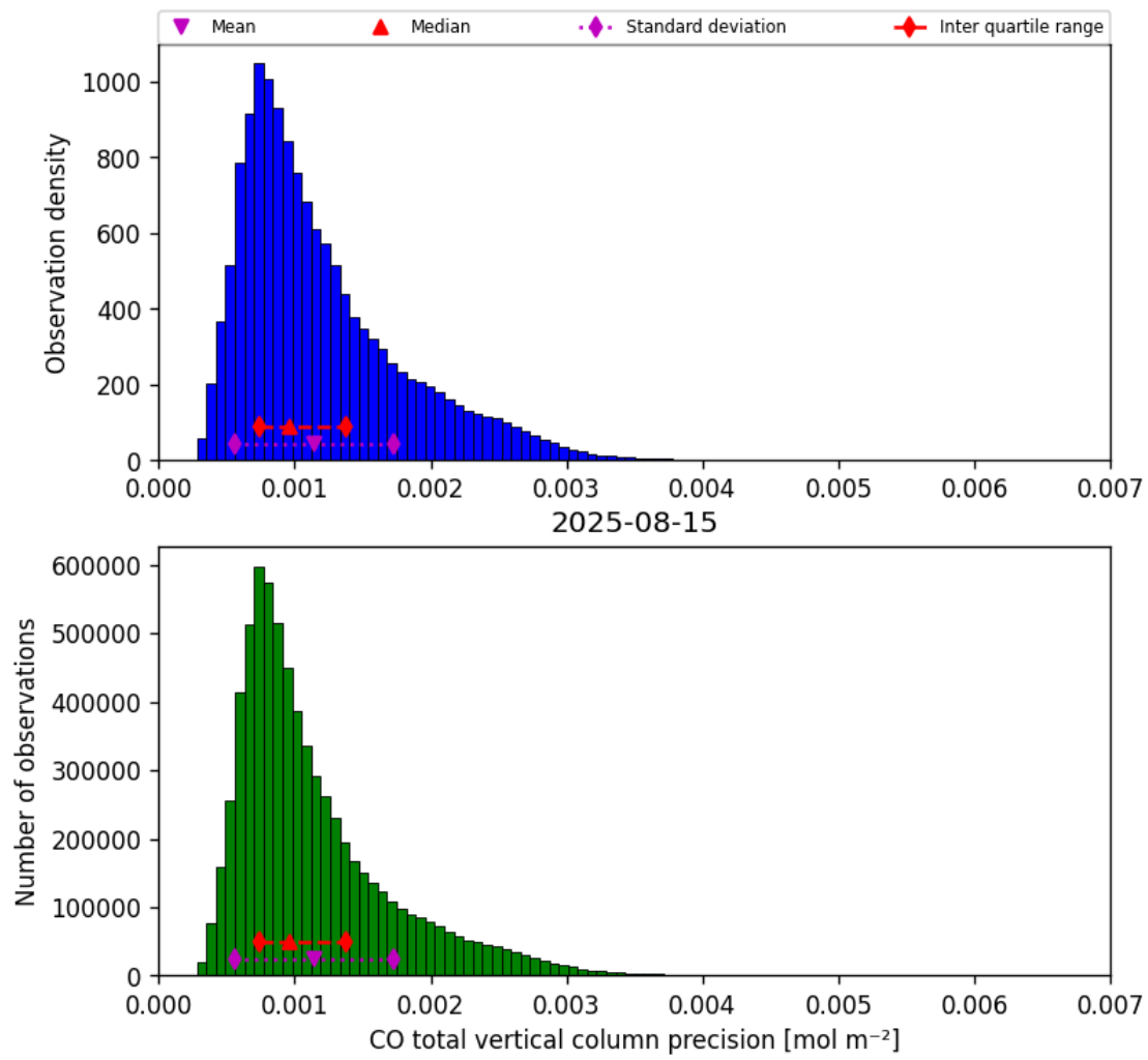
Figure 15: Histogram of “CO total vertical column precision” for 2025-08-15 to 2025-08-16
