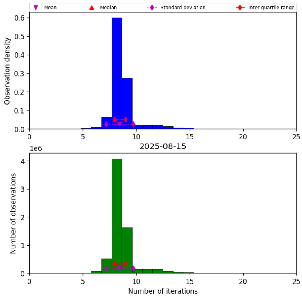
Figure 19: Histogram of “Number of iterations” for 2025-08-15 to 2025-08-16
