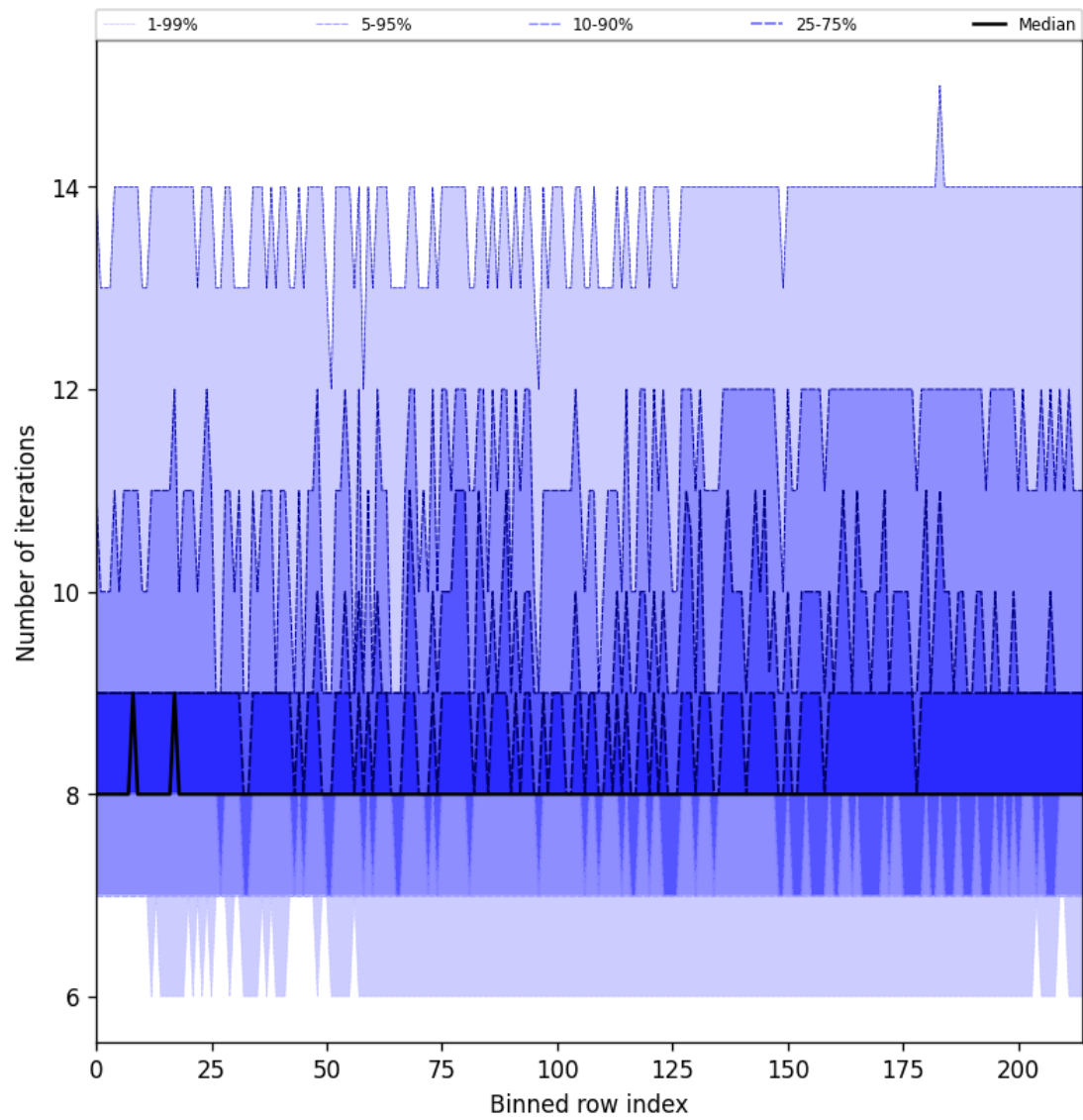
Figure 26: Along track statistics of “Number of iterations” for 2025-08-15 to 2025-08-16
