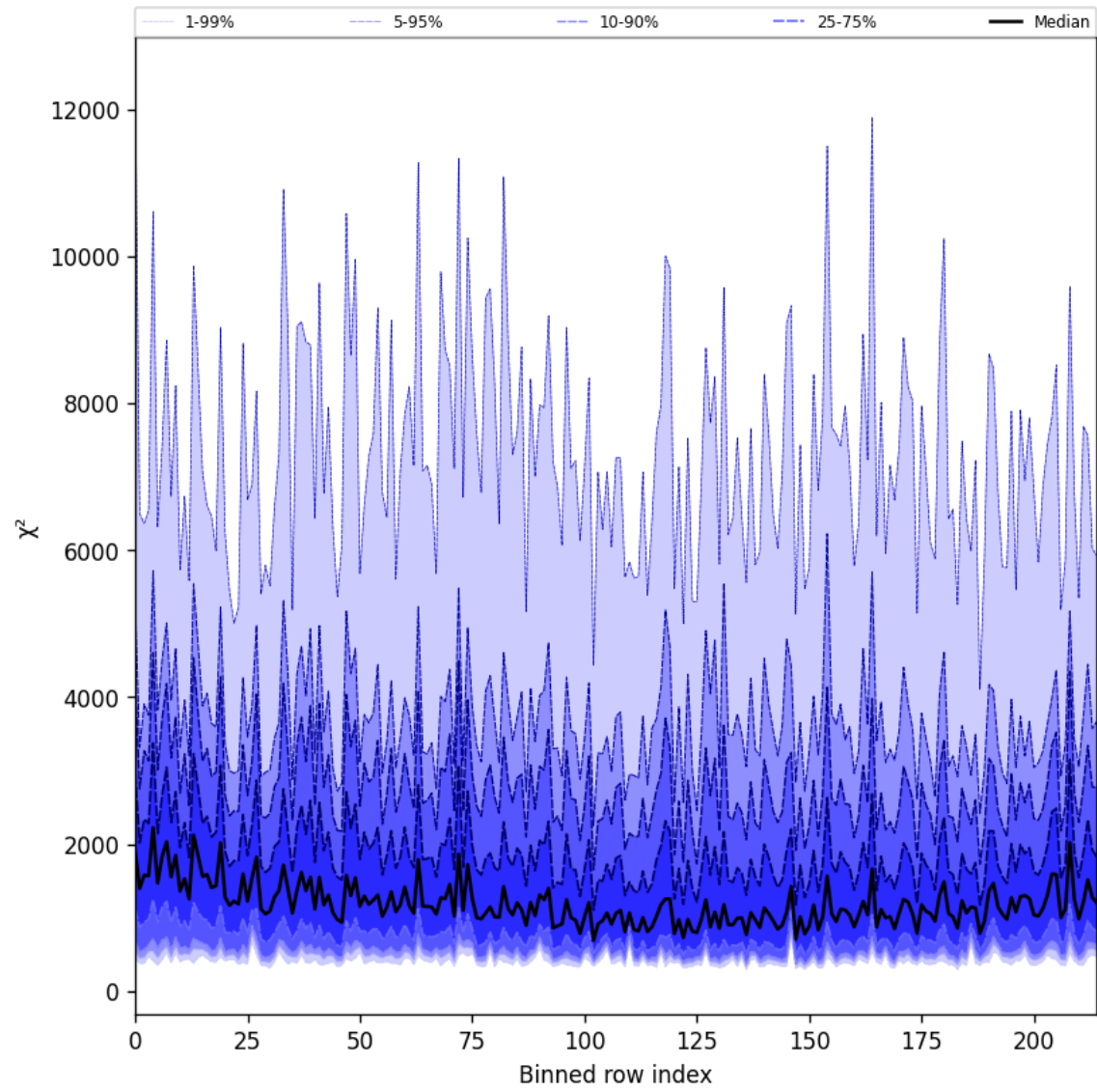
Figure 24: Along track statistics of “ \chi^2 ” for 2025-08-15 to 2025-08-16
