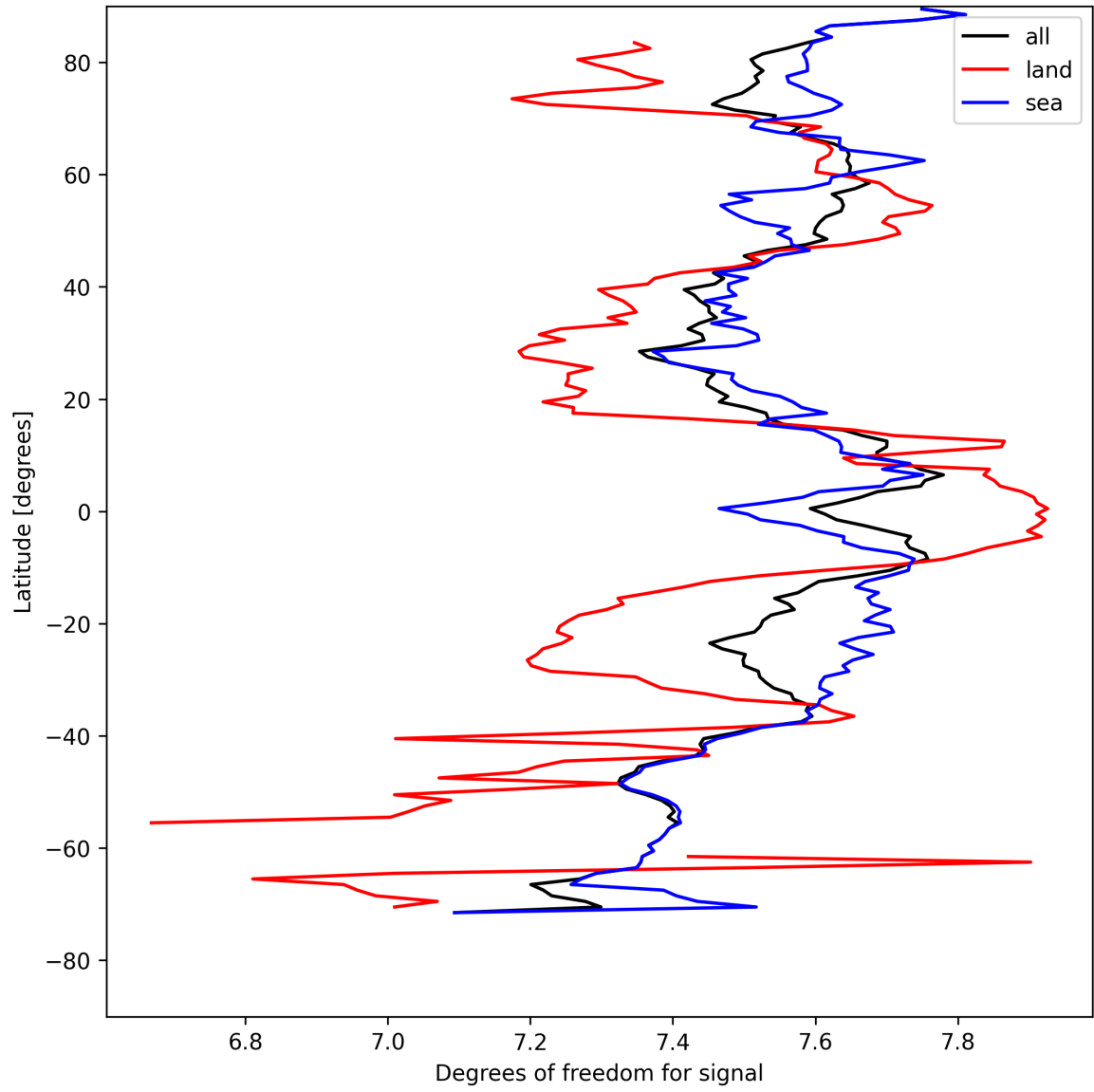
Figure 11: Zonal average of “Degrees of freedom for signal” for 2025-08-15 to 2025-08-16.
