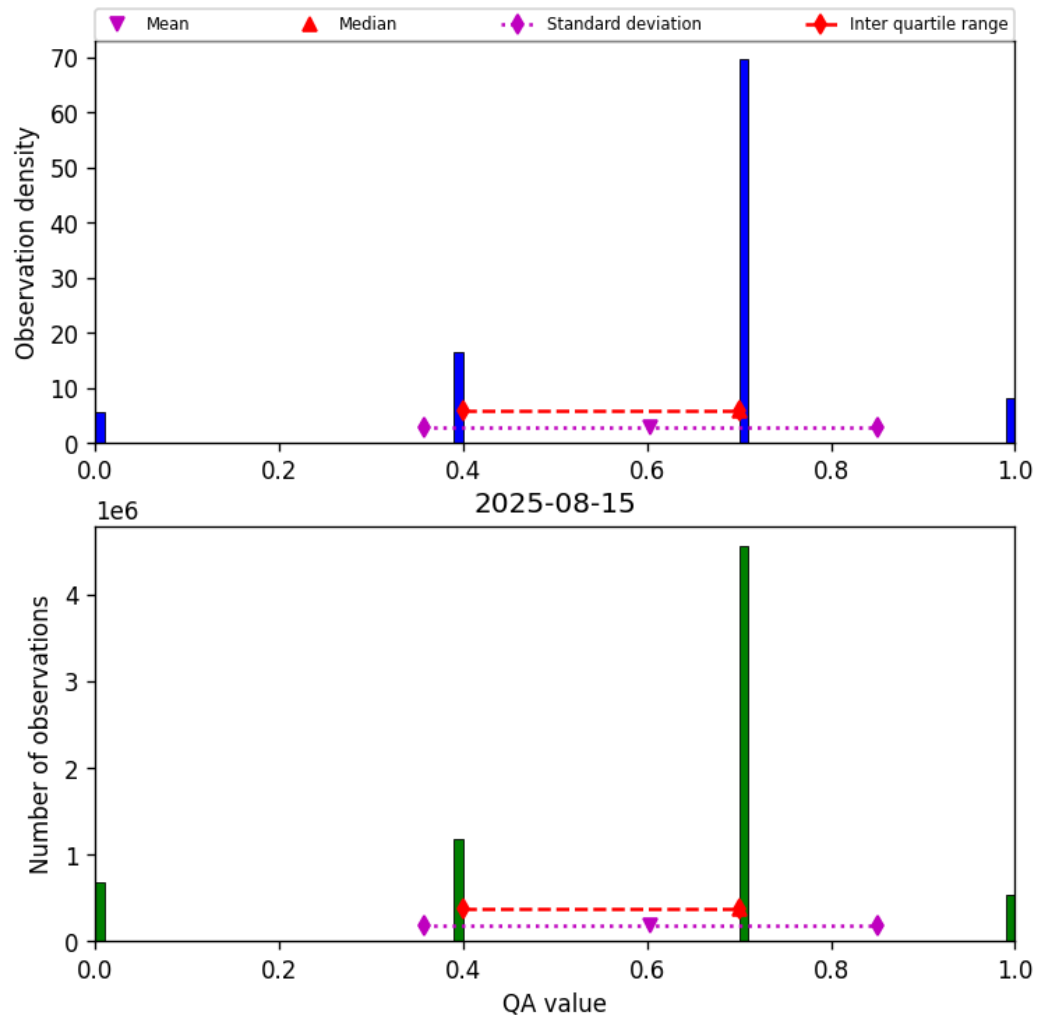
Figure 13: Histogram of “QA value” for 2025-08-15 to 2025-08-16
