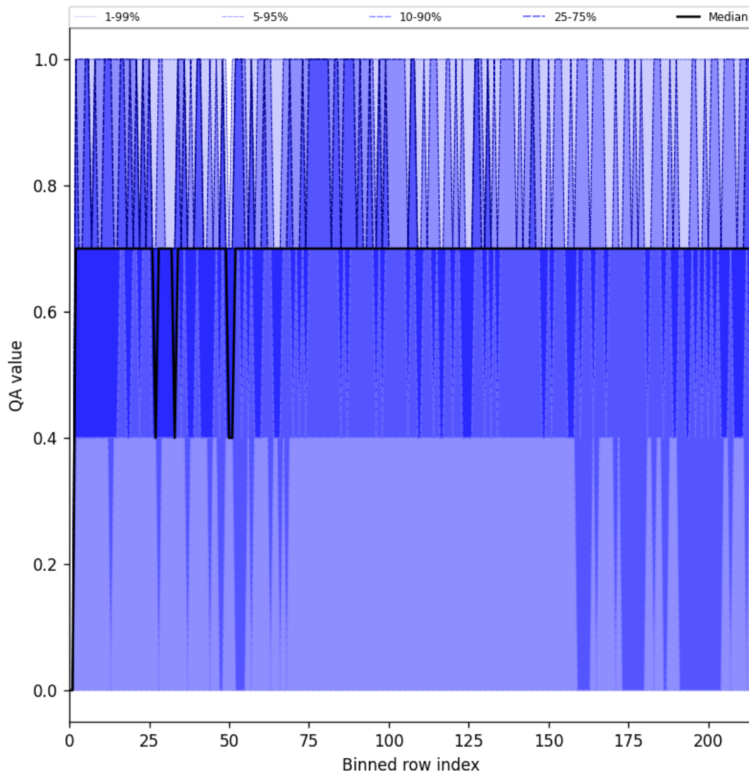
Figure 20: Along track statistics of “QA value” for 2025-08-15 to 2025-08-16
