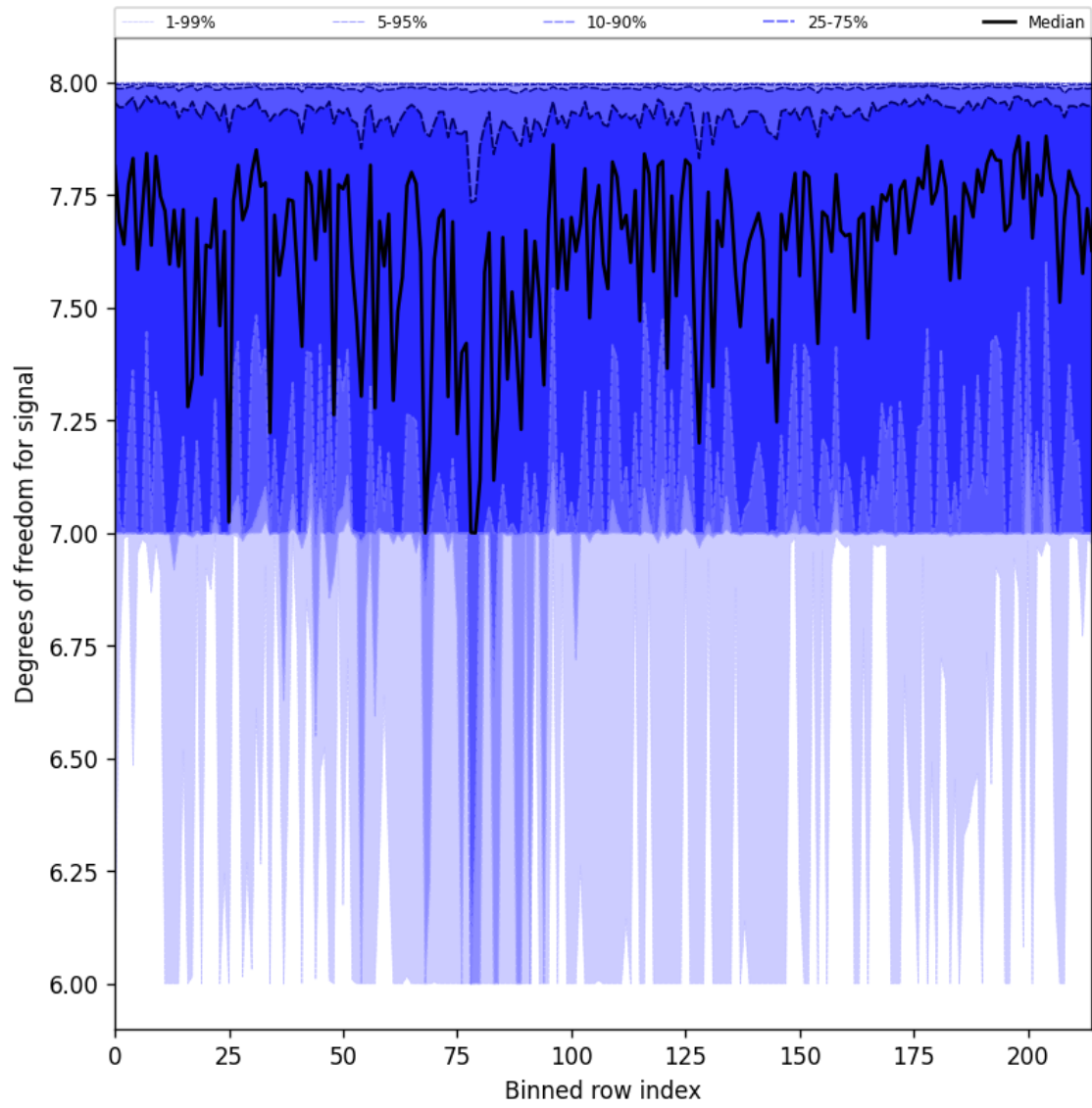
Figure 25: Along track statistics of “Degrees of freedom for signal” for 2025-08-15 to 2025-08-16
