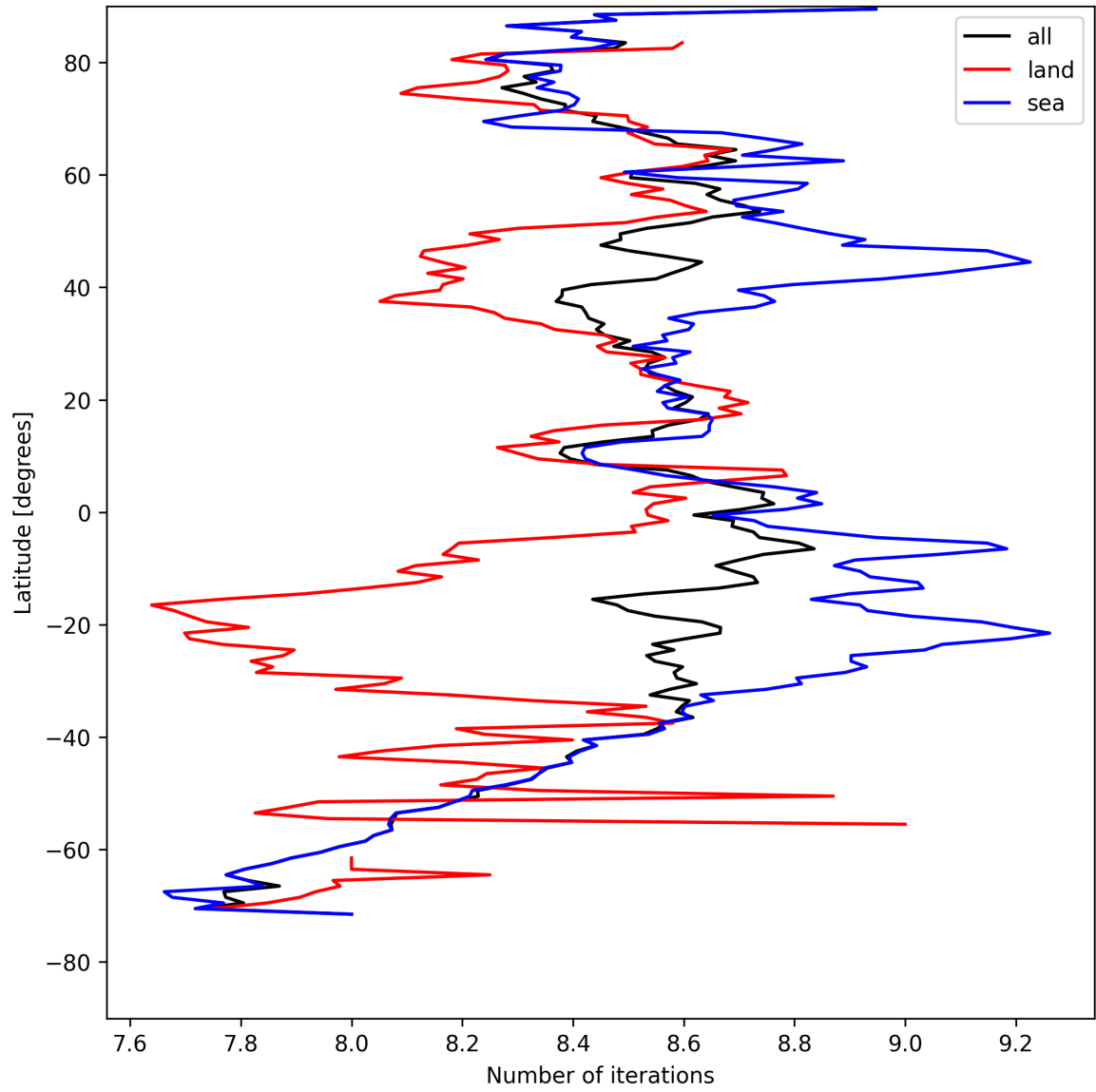
Figure 12: Zonal average of “Number of iterations” for 2025-08-15 to 2025-08-16.
