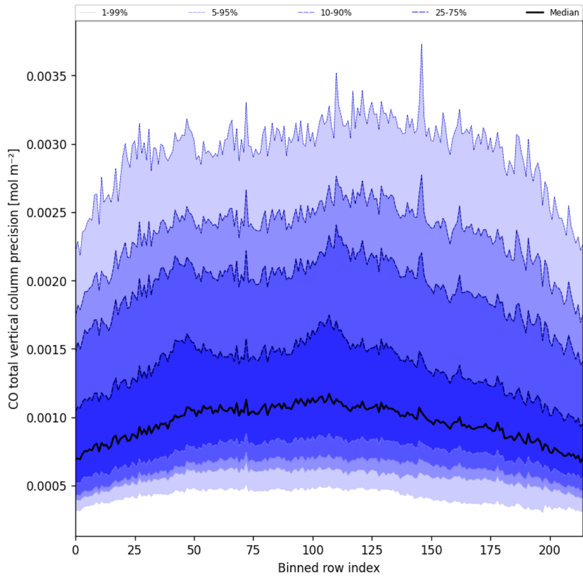
Figure 22: Along track statistics of “CO total vertical column precision” for 2025-08-15 to 2025-08-16
