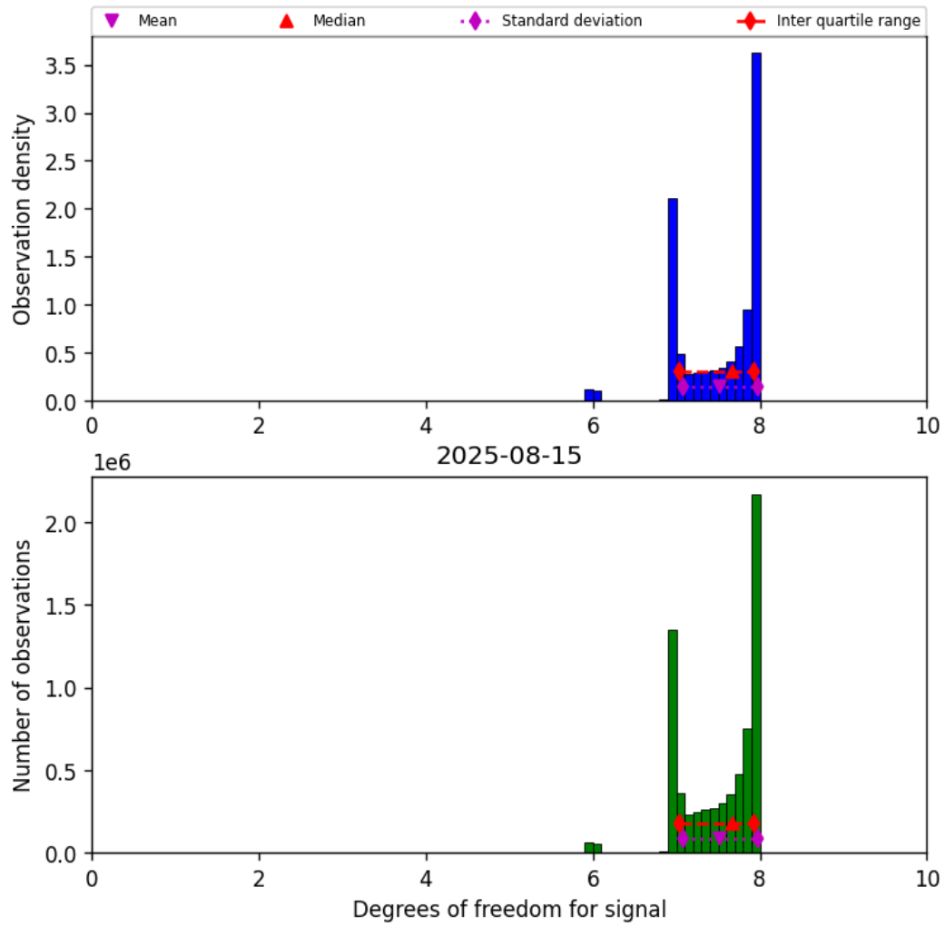
Figure 18: Histogram of “Degrees of freedom for signal” for 2025-08-15 to 2025-08-16
