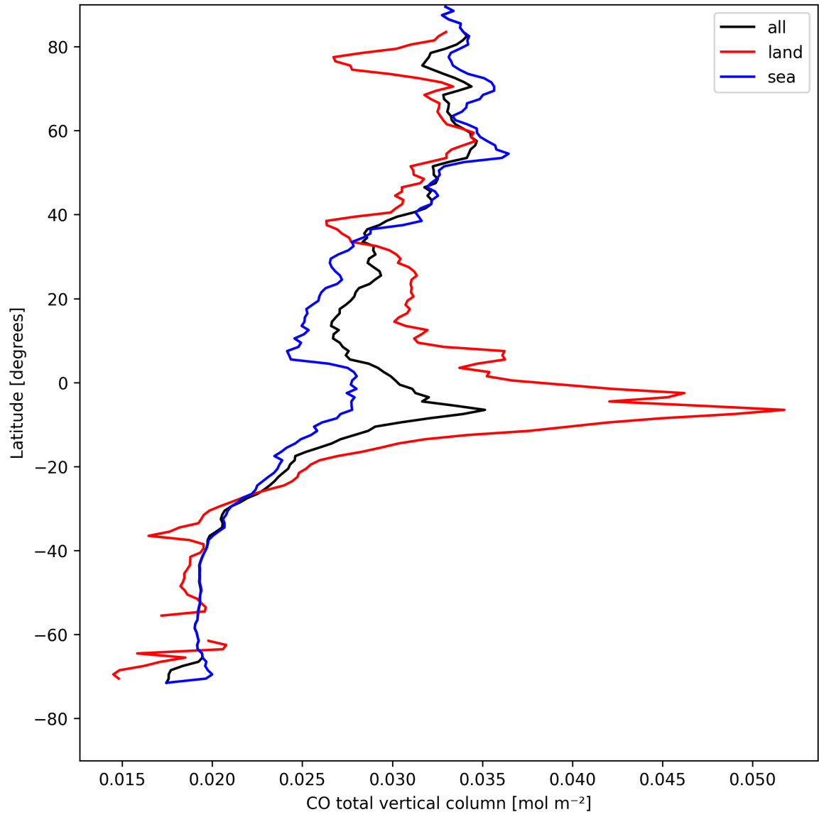
Figure 7: Zonal average of “CO total vertical column” for 2025-08-15 to 2025-08-16.
