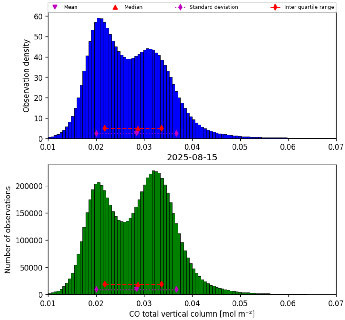
Figure 14: Histogram of “CO total vertical column” for 2025-08-15 to 2025-08-16
