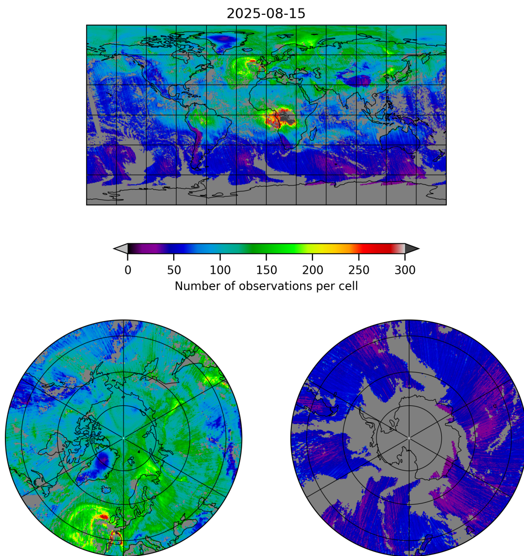
Figure 5: Map of the number of observations for 2025-08-15 to 2025-08-16
