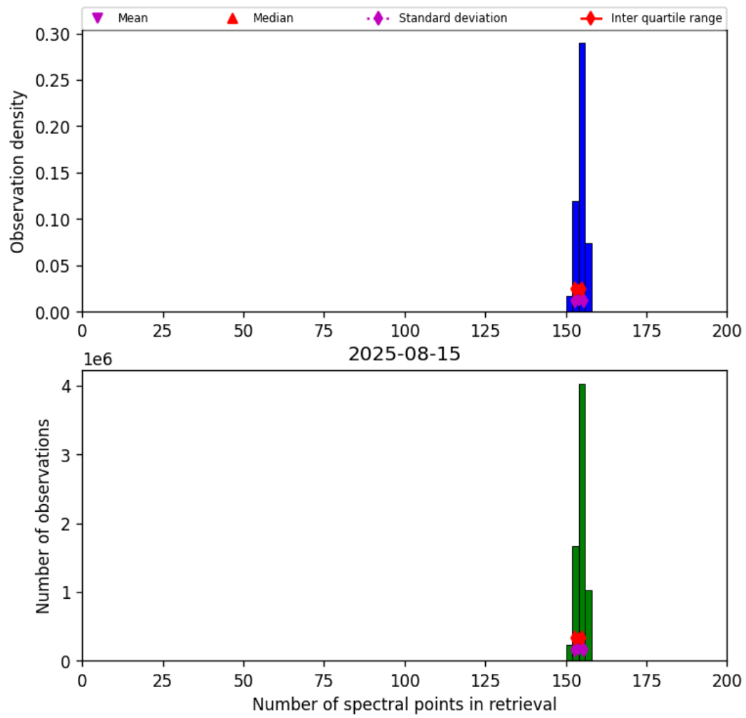
Figure 16: Histogram of “Number of spectral points in retrieval” for 2025-08-15 to 2025-08-16
