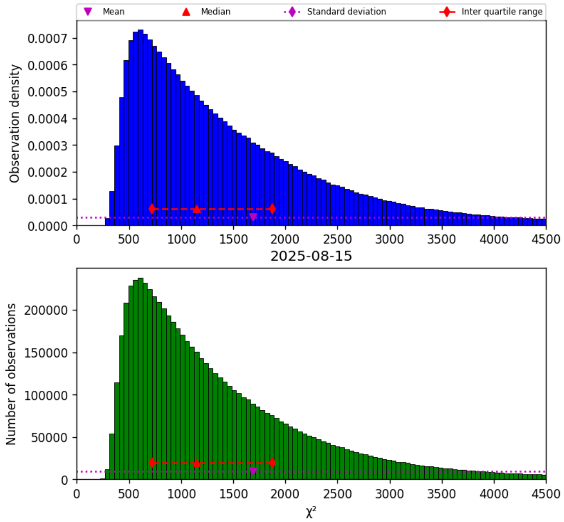
Figure 17: Histogram of “ \chi^2 ” for 2025-08-15 to 2025-08-16
