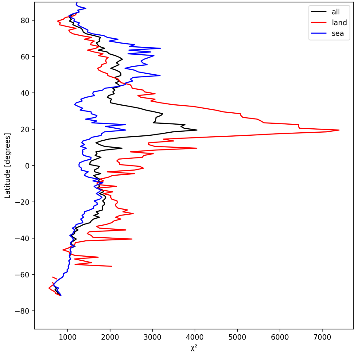
Figure 10: Zonal average of “ \chi^2 ” for 2025-08-16 to 2025-08-17.
