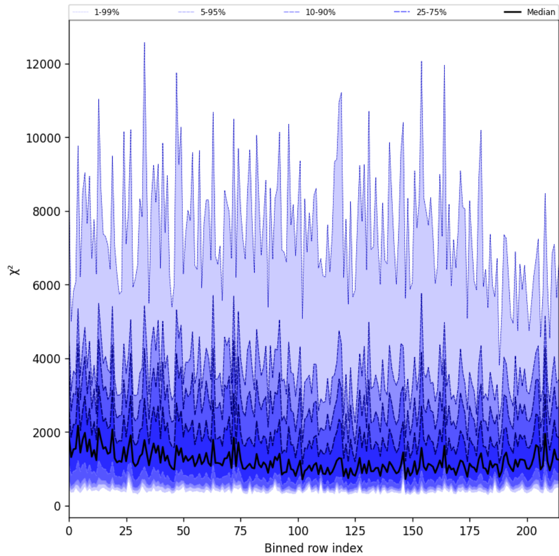
Figure 24: Along track statistics of “ \chi^2 ” for 2025-08-16 to 2025-08-17
