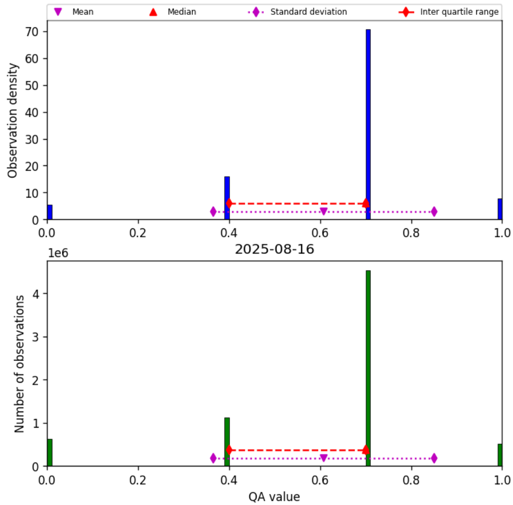
Figure 13: Histogram of “QA value” for 2025-08-16 to 2025-08-17
