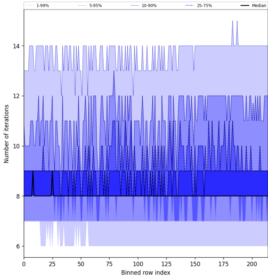
Figure 26: Along track statistics of “Number of iterations” for 2025-08-16 to 2025-08-17
