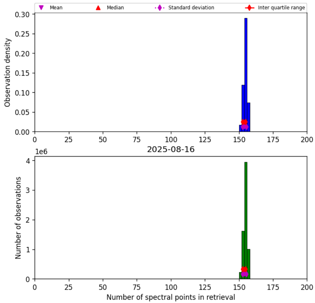
Figure 16: Histogram of “Number of spectral points in retrieval” for 2025-08-16 to 2025-08-17
