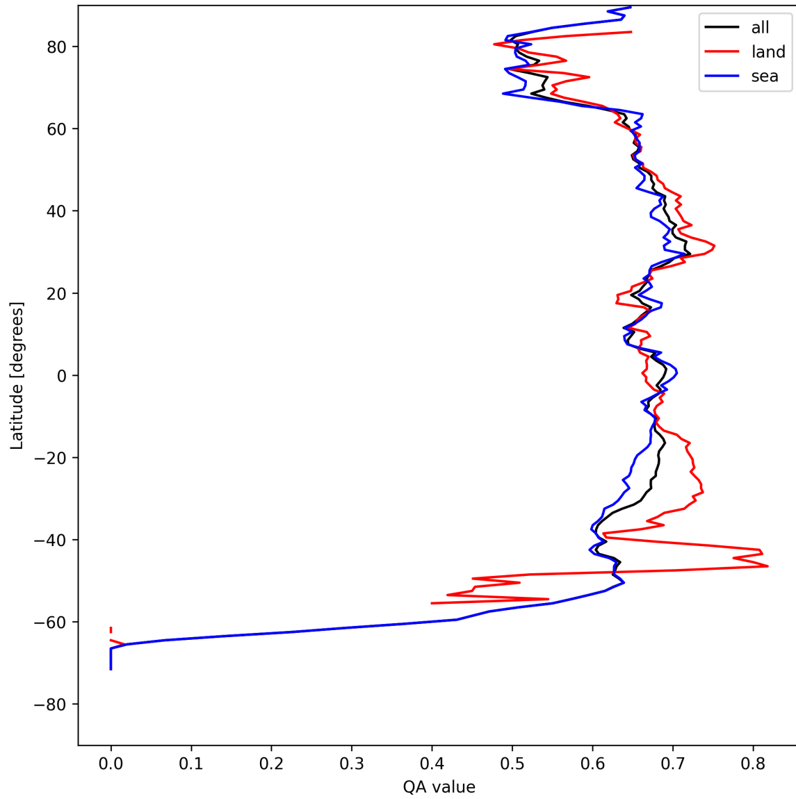
Figure 6: Zonal average of “QA value” for 2025-08-16 to 2025-08-17.
