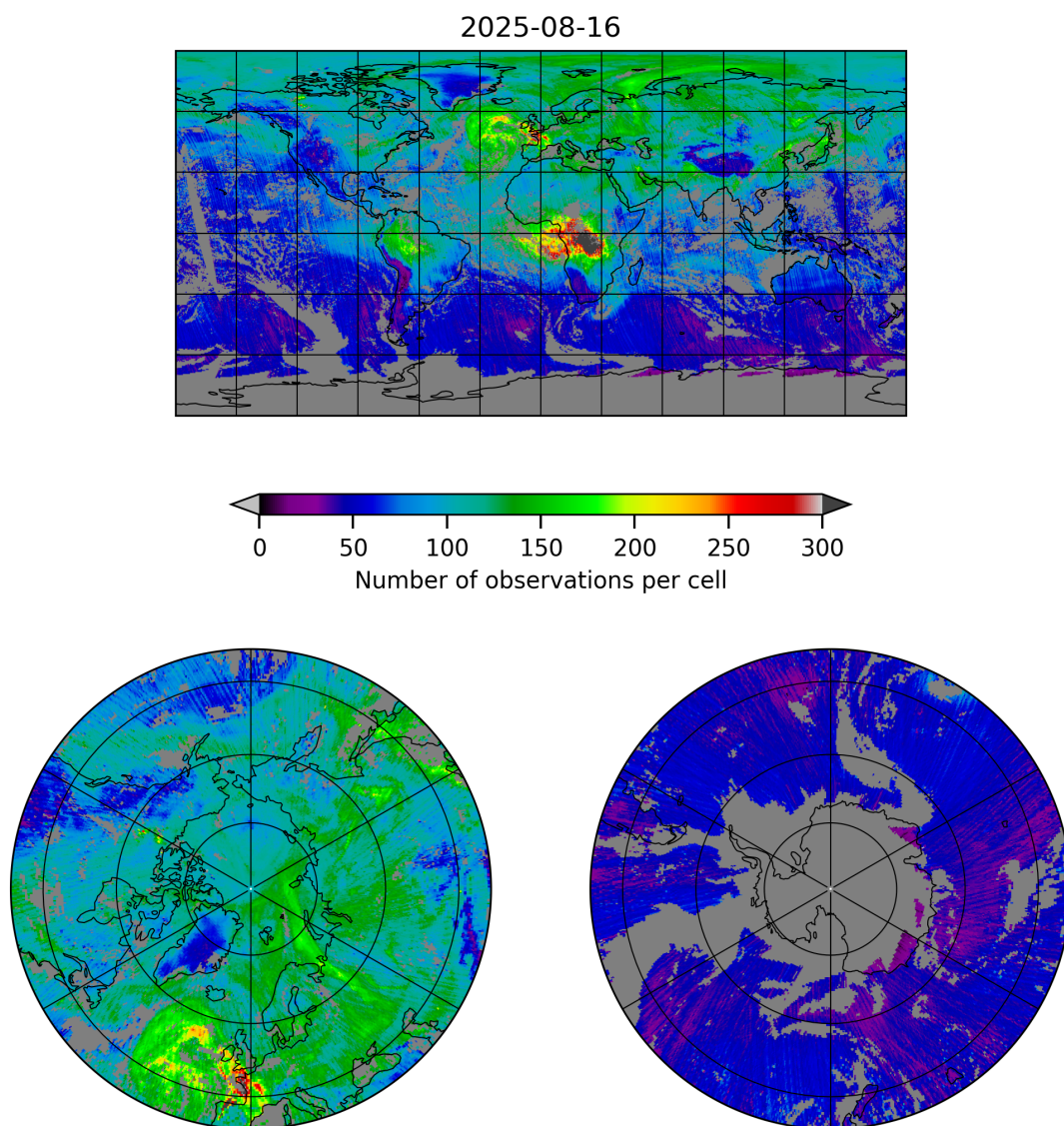
Figure 5: Map of the number of observations for 2025-08-16 to 2025-08-17
