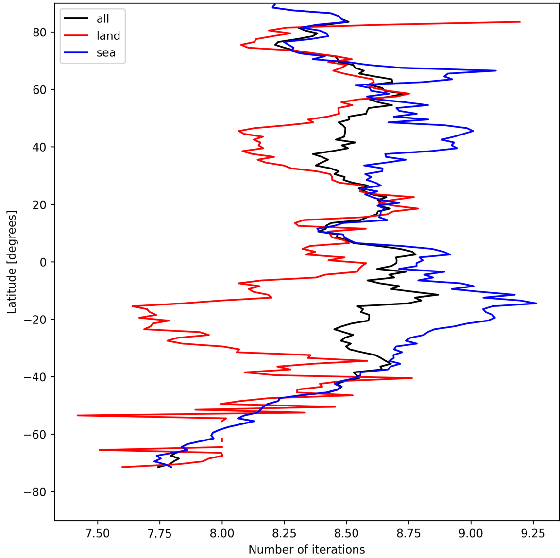
Figure 12: Zonal average of “Number of iterations” for 2025-08-16 to 2025-08-17.
