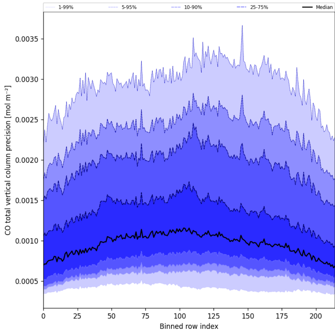
Figure 22: Along track statistics of “CO total vertical column precision” for 2025-08-16 to 2025-08-17
