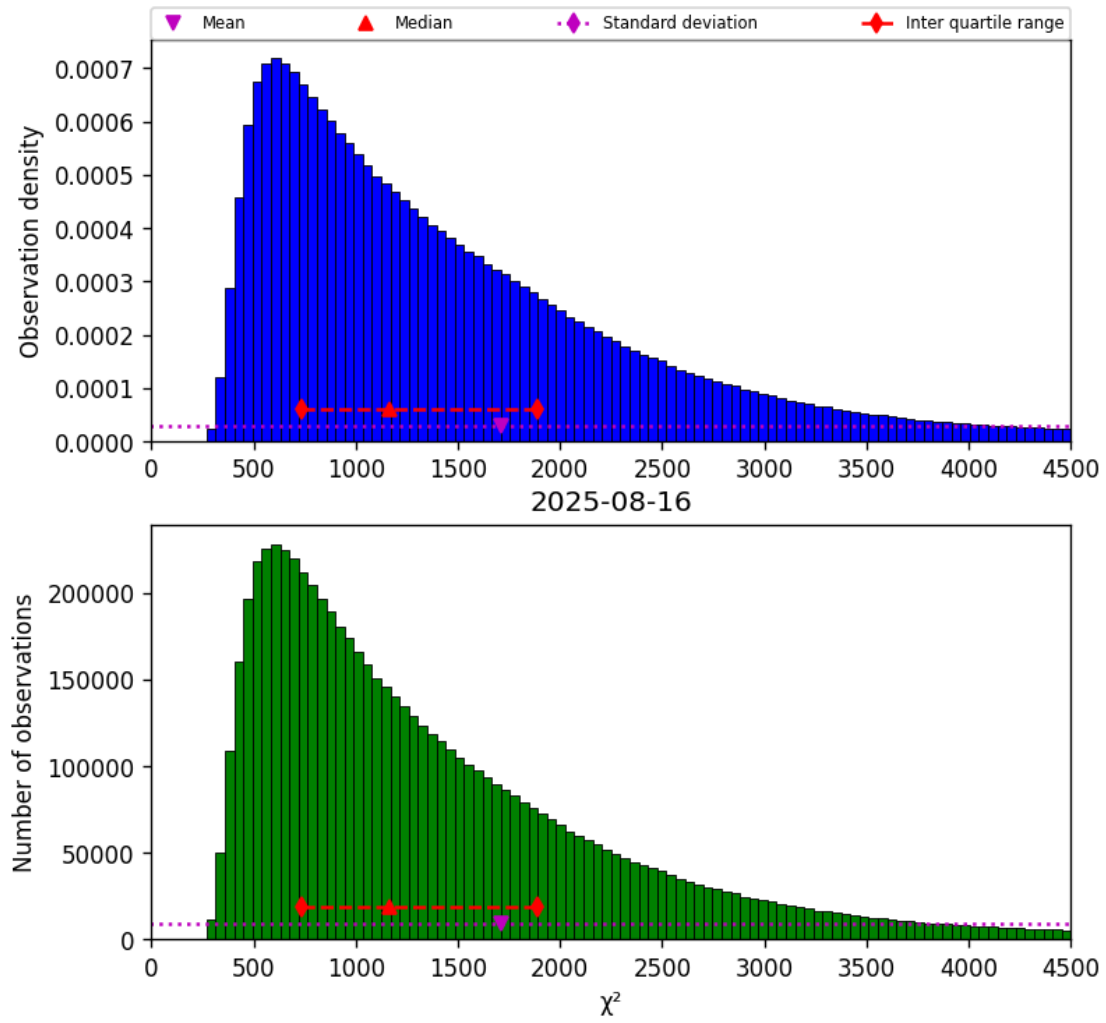
Figure 17: Histogram of “ \chi^2 ” for 2025-08-16 to 2025-08-17
