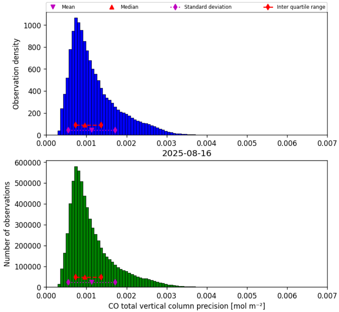
Figure 15: Histogram of “CO total vertical column precision” for 2025-08-16 to 2025-08-17
