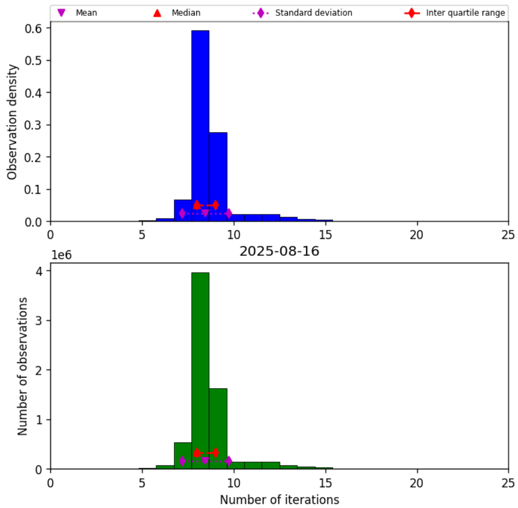
Figure 19: Histogram of “Number of iterations” for 2025-08-16 to 2025-08-17
