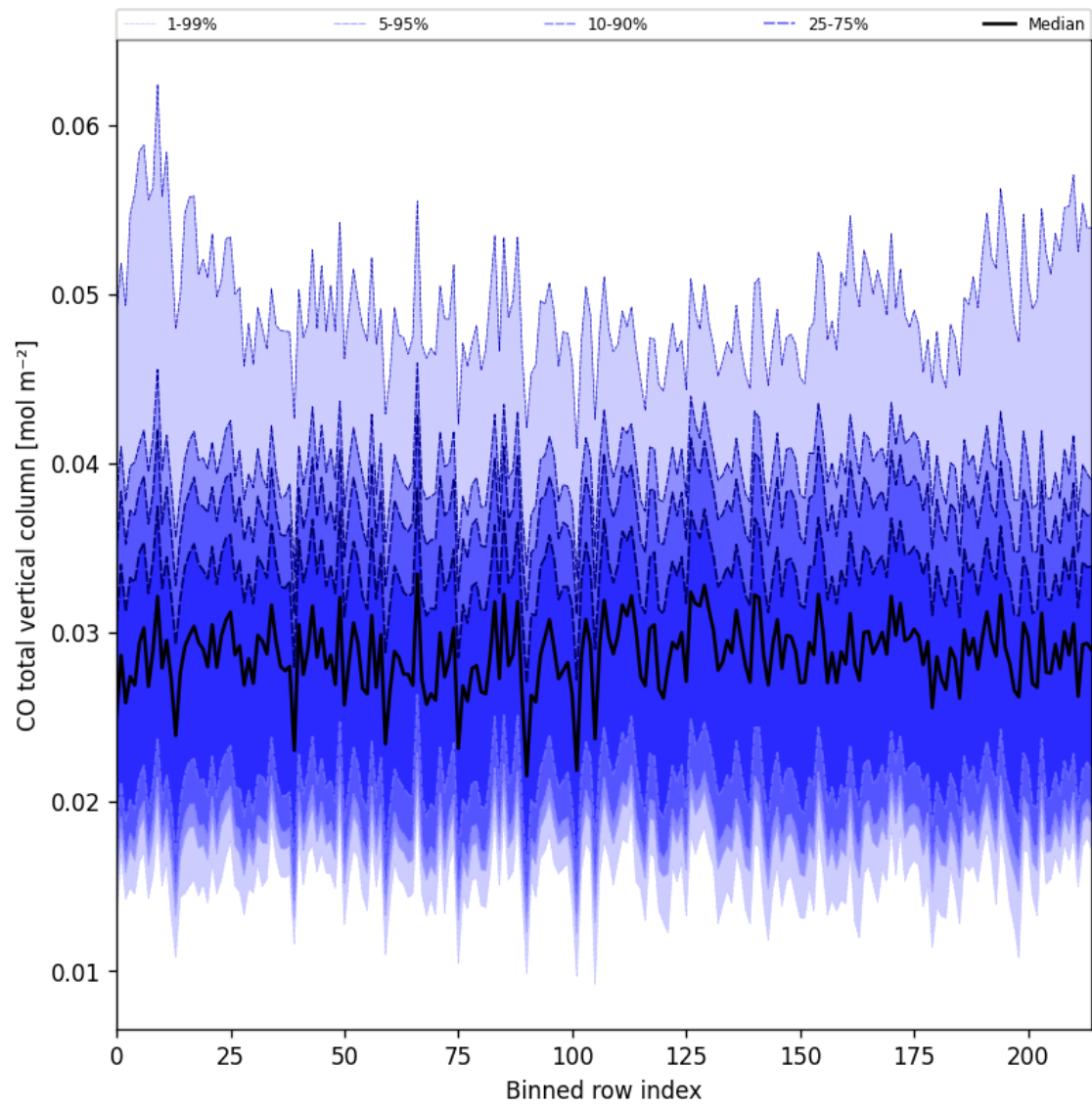
Figure 21: Along track statistics of “CO total vertical column” for 2025-08-16 to 2025-08-17
