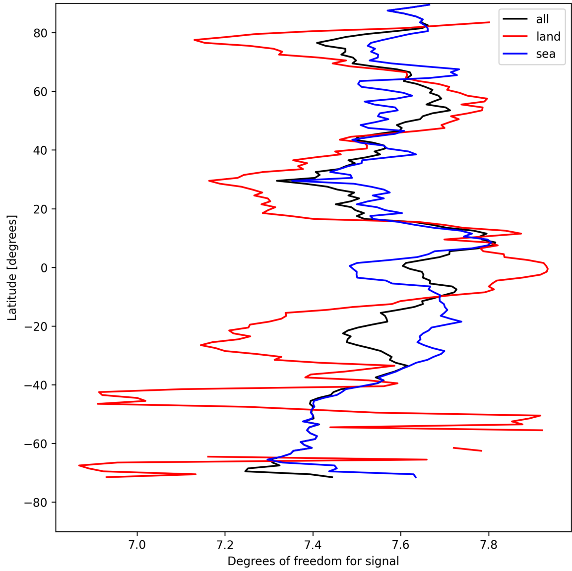
Figure 11: Zonal average of “Degrees of freedom for signal” for 2025-08-16 to 2025-08-17.
