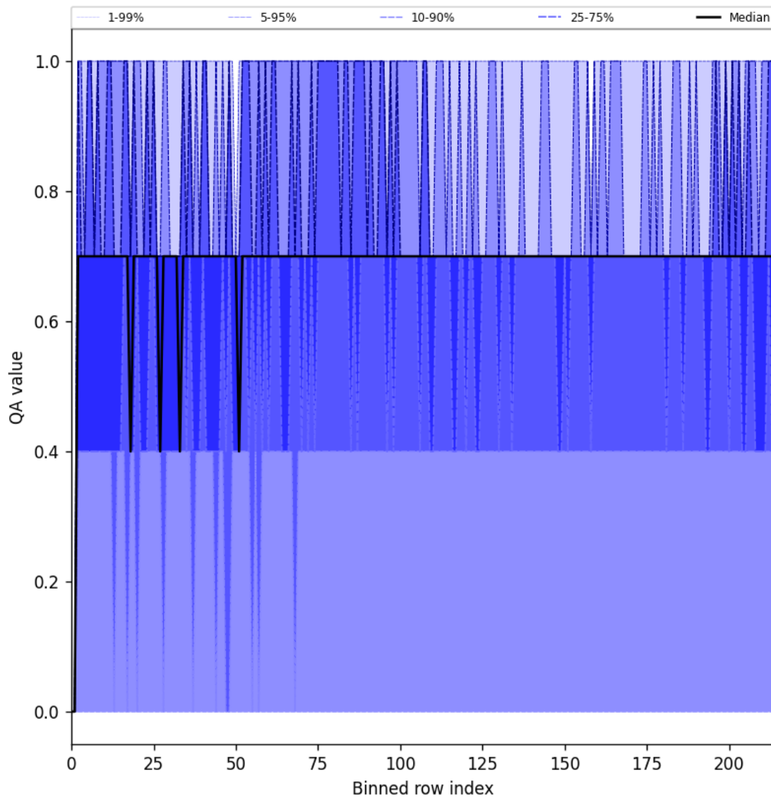
Figure 20: Along track statistics of “QA value” for 2025-08-16 to 2025-08-17
