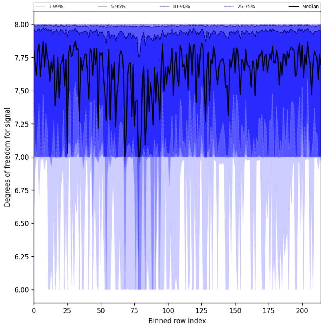
Figure 25: Along track statistics of “Degrees of freedom for signal” for 2025-08-16 to 2025-08-17
