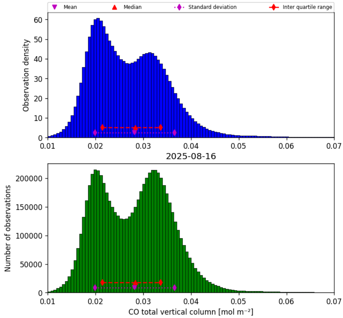
Figure 14: Histogram of “CO total vertical column” for 2025-08-16 to 2025-08-17
