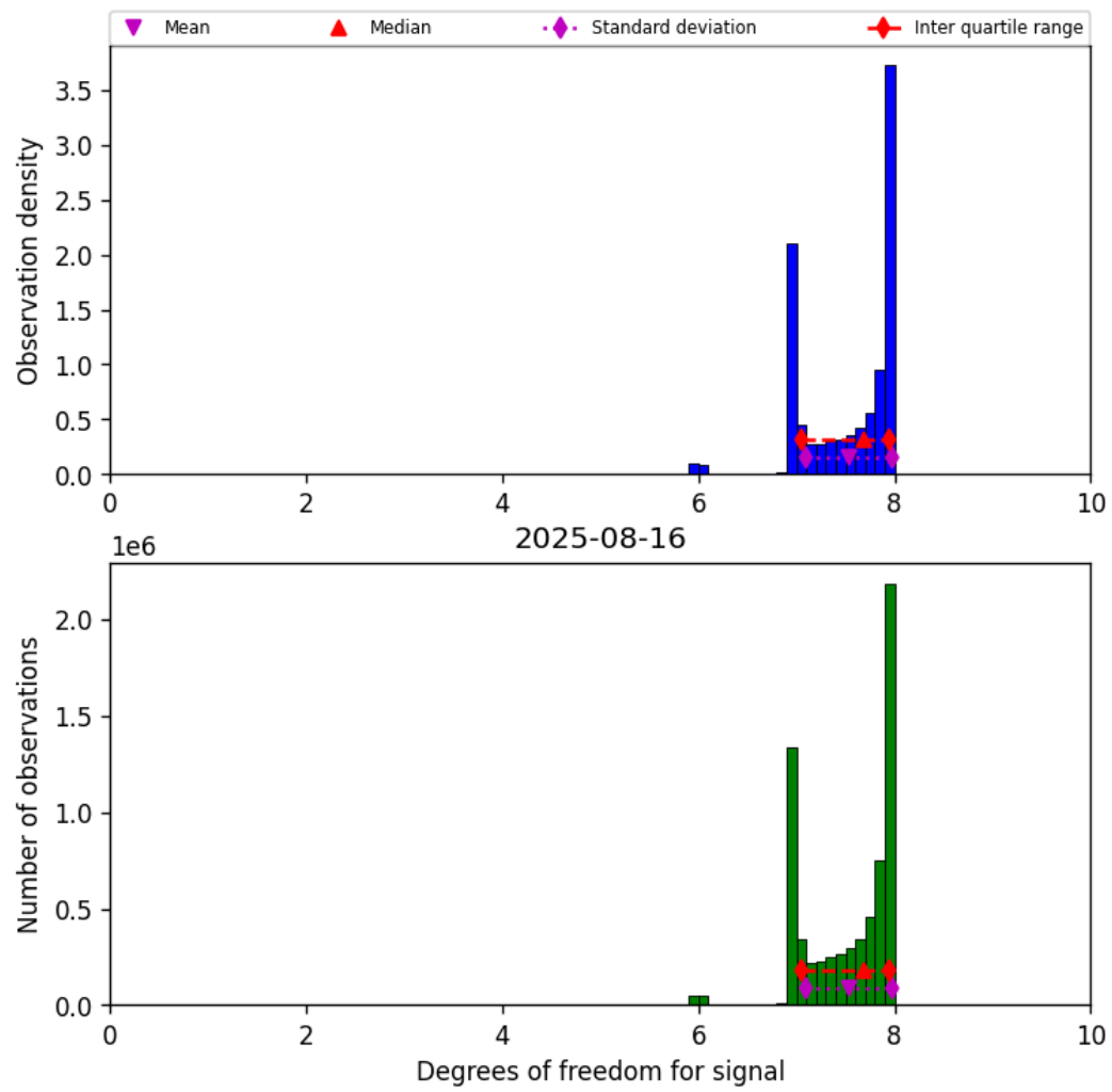
Figure 18: Histogram of “Degrees of freedom for signal” for 2025-08-16 to 2025-08-17
