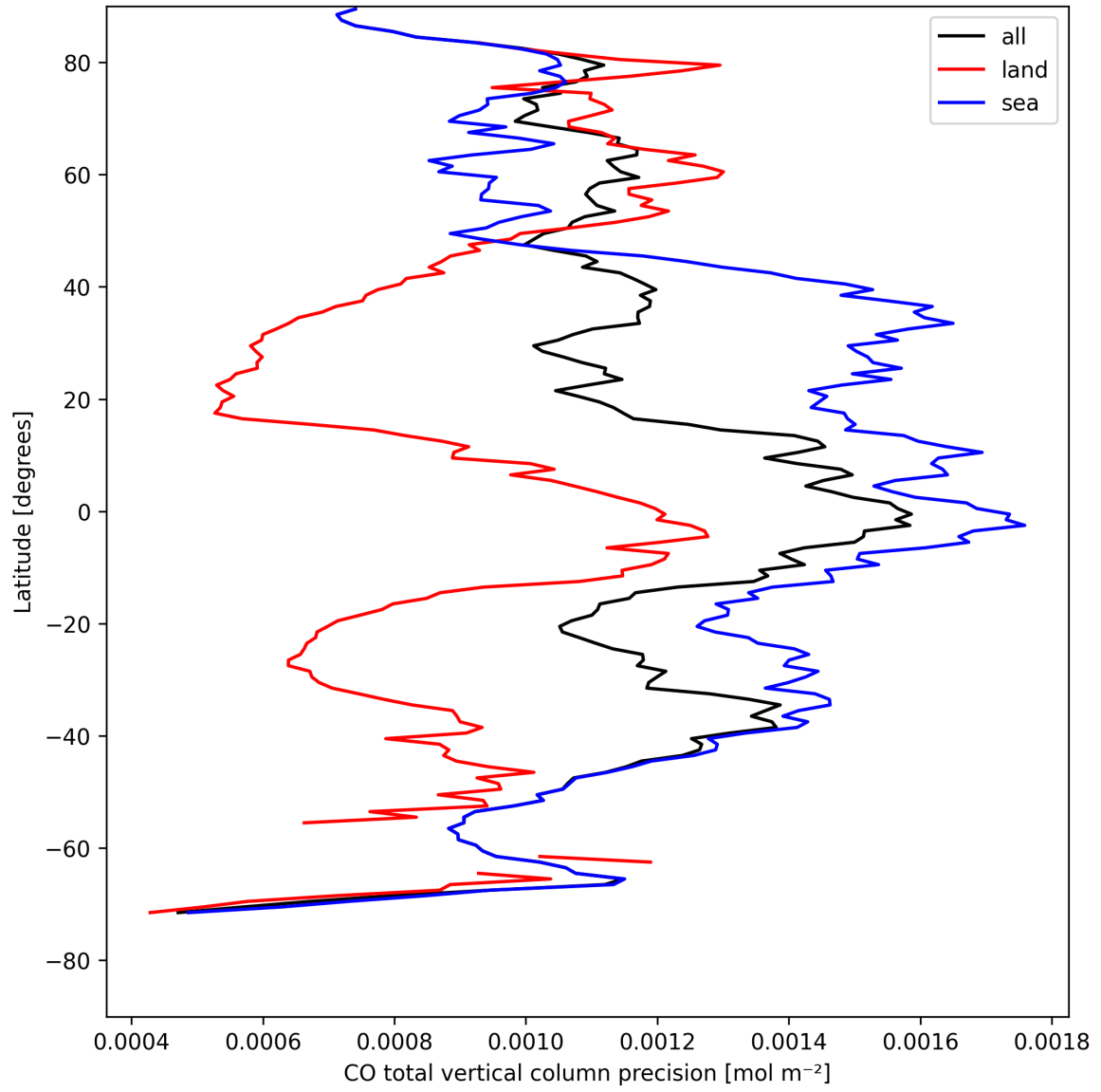
Figure 8: Zonal average of “CO total vertical column precision” for 2025-08-16 to 2025-08-17.
