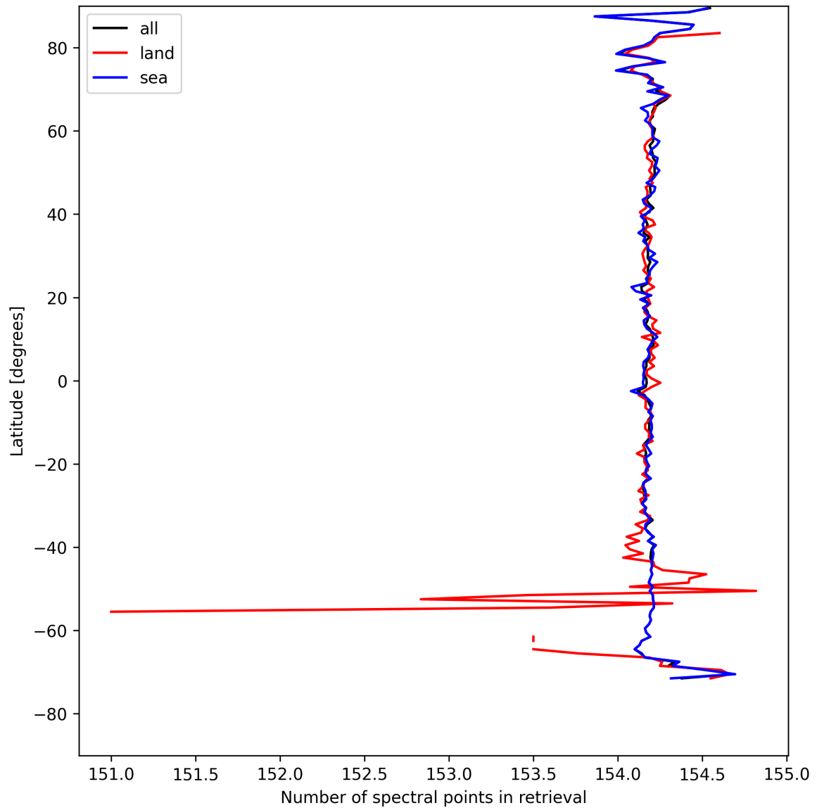
Figure 9: Zonal average of “Number of spectral points in retrieval” for 2025-08-16 to 2025-08-17.
