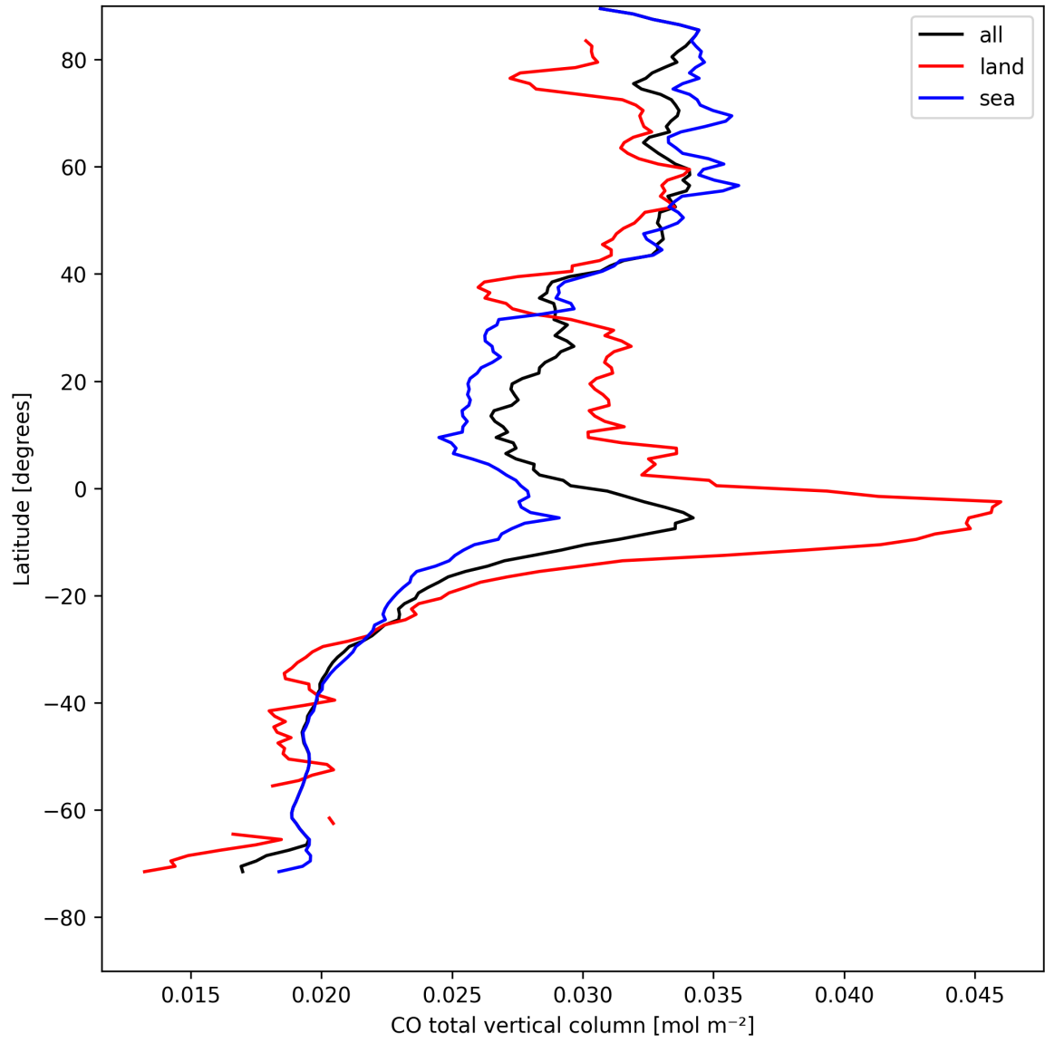
Figure 7: Zonal average of “CO total vertical column” for 2025-08-16 to 2025-08-17.
