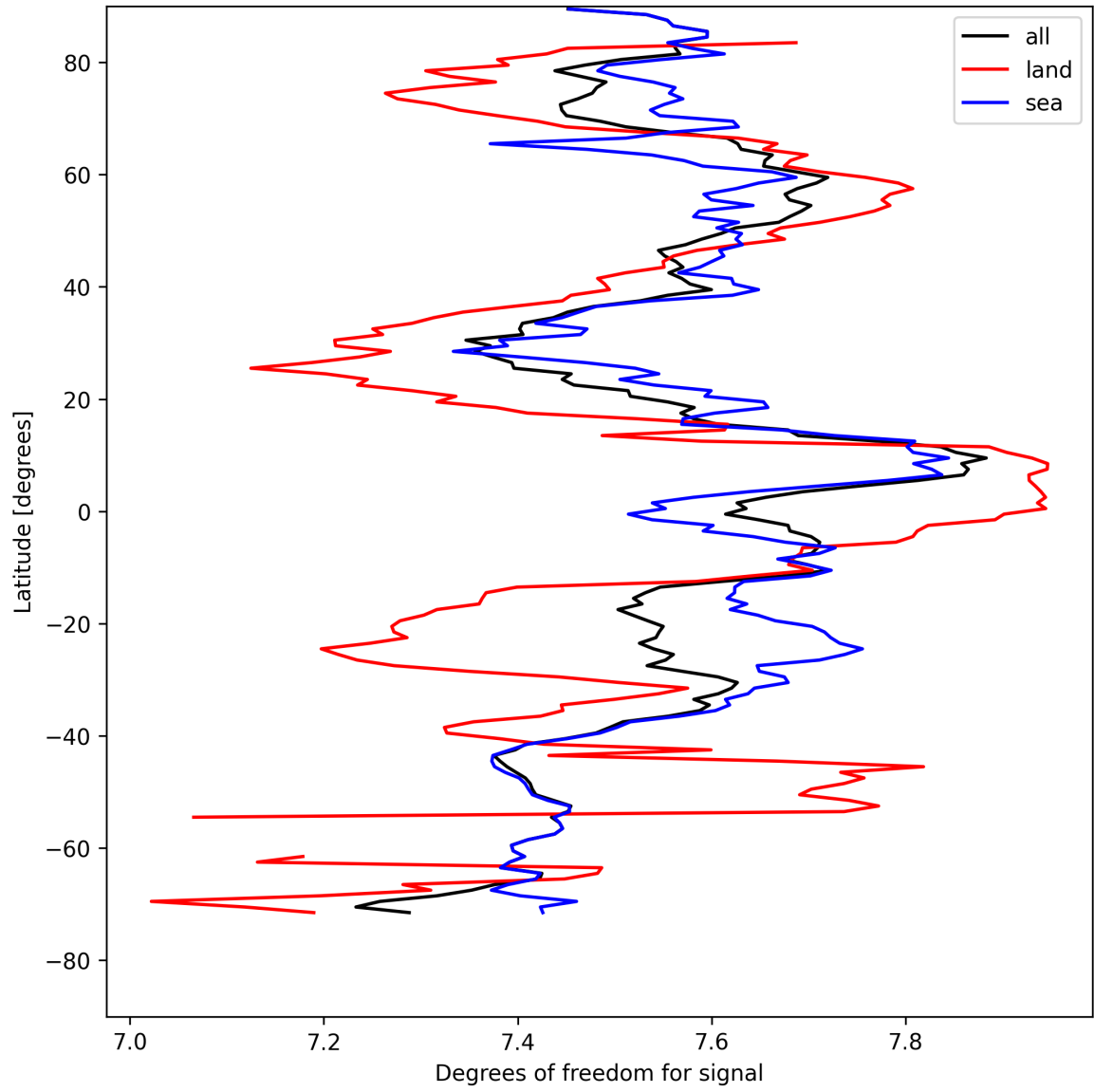
Figure 11: Zonal average of “Degrees of freedom for signal” for 2025-08-17 to 2025-08-17.
