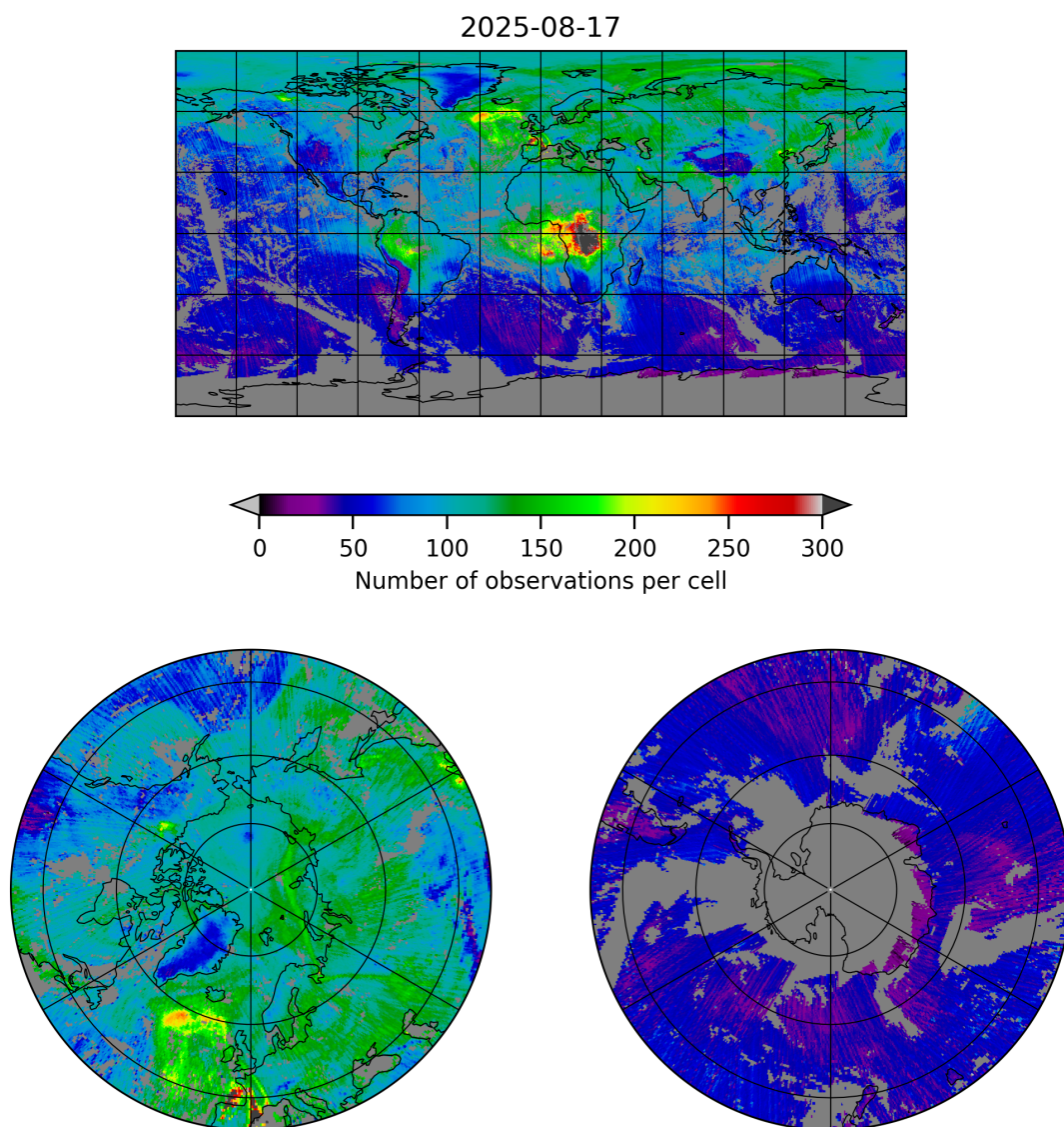
Figure 5: Map of the number of observations for 2025-08-17 to 2025-08-17
