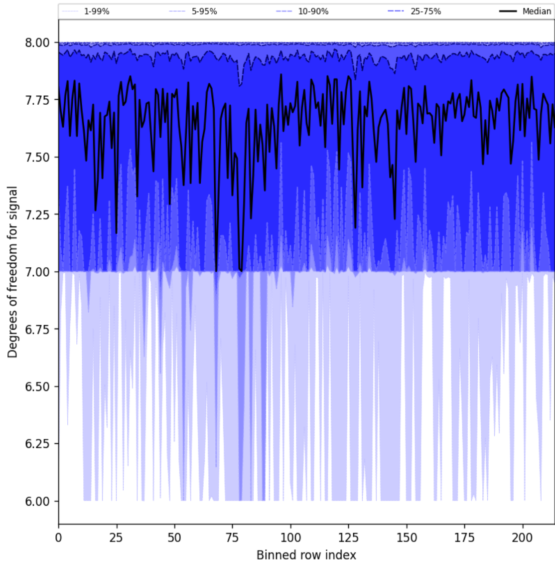
Figure 25: Along track statistics of “Degrees of freedom for signal” for 2025-08-17 to 2025-08-17
