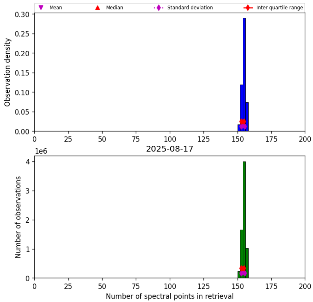
Figure 16: Histogram of “Number of spectral points in retrieval” for 2025-08-17 to 2025-08-17
