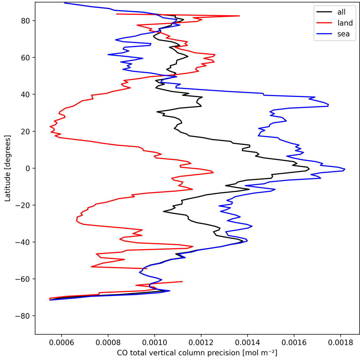
Figure 8: Zonal average of “CO total vertical column precision” for 2025-08-17 to 2025-08-17.
