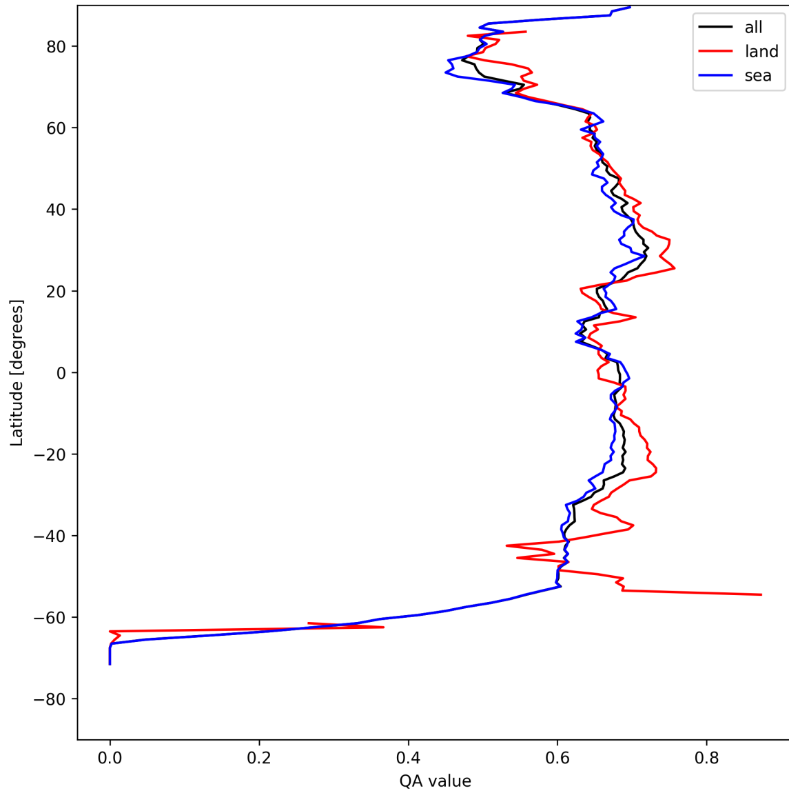
Figure 6: Zonal average of “QA value” for 2025-08-17 to 2025-08-17.
