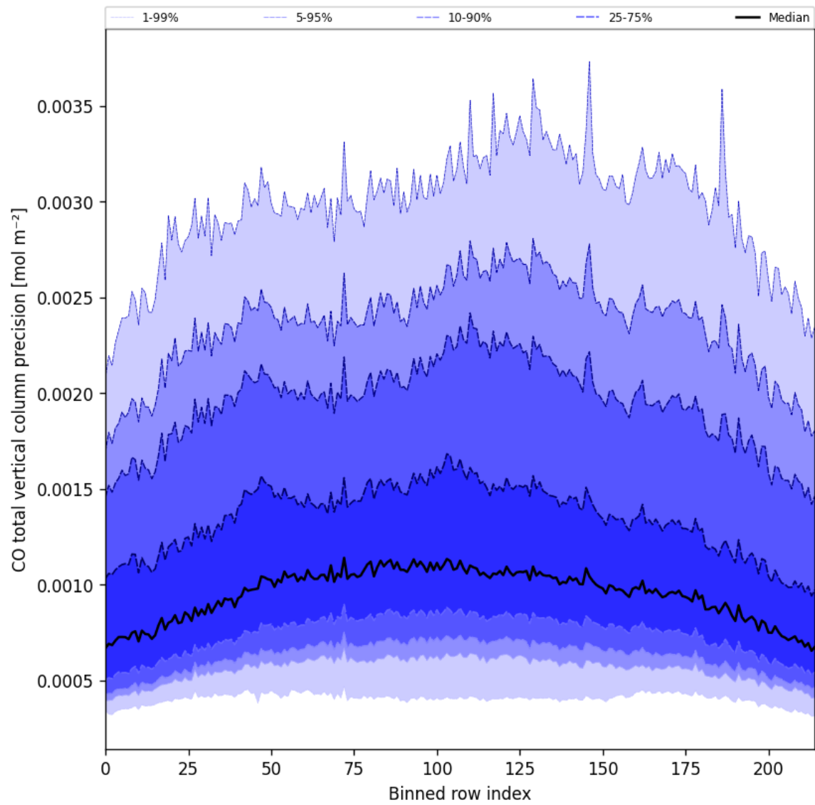
Figure 22: Along track statistics of “CO total vertical column precision” for 2025-08-17 to 2025-08-17
