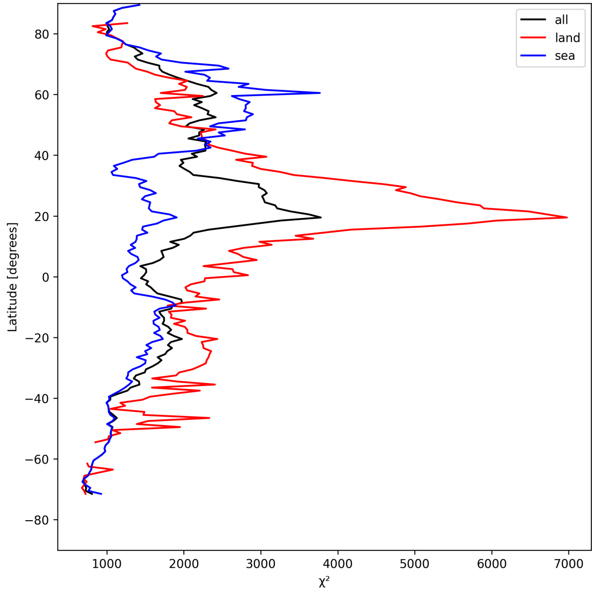
Figure 10: Zonal average of “ \chi^2 ” for 2025-08-17 to 2025-08-17.
