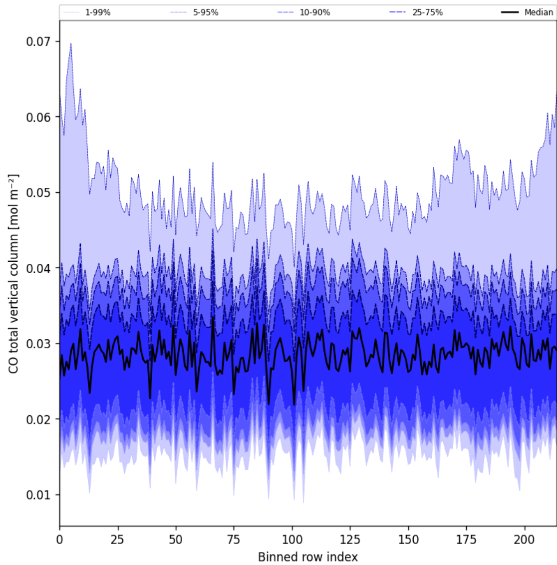
Figure 21: Along track statistics of “CO total vertical column” for 2025-08-17 to 2025-08-17
