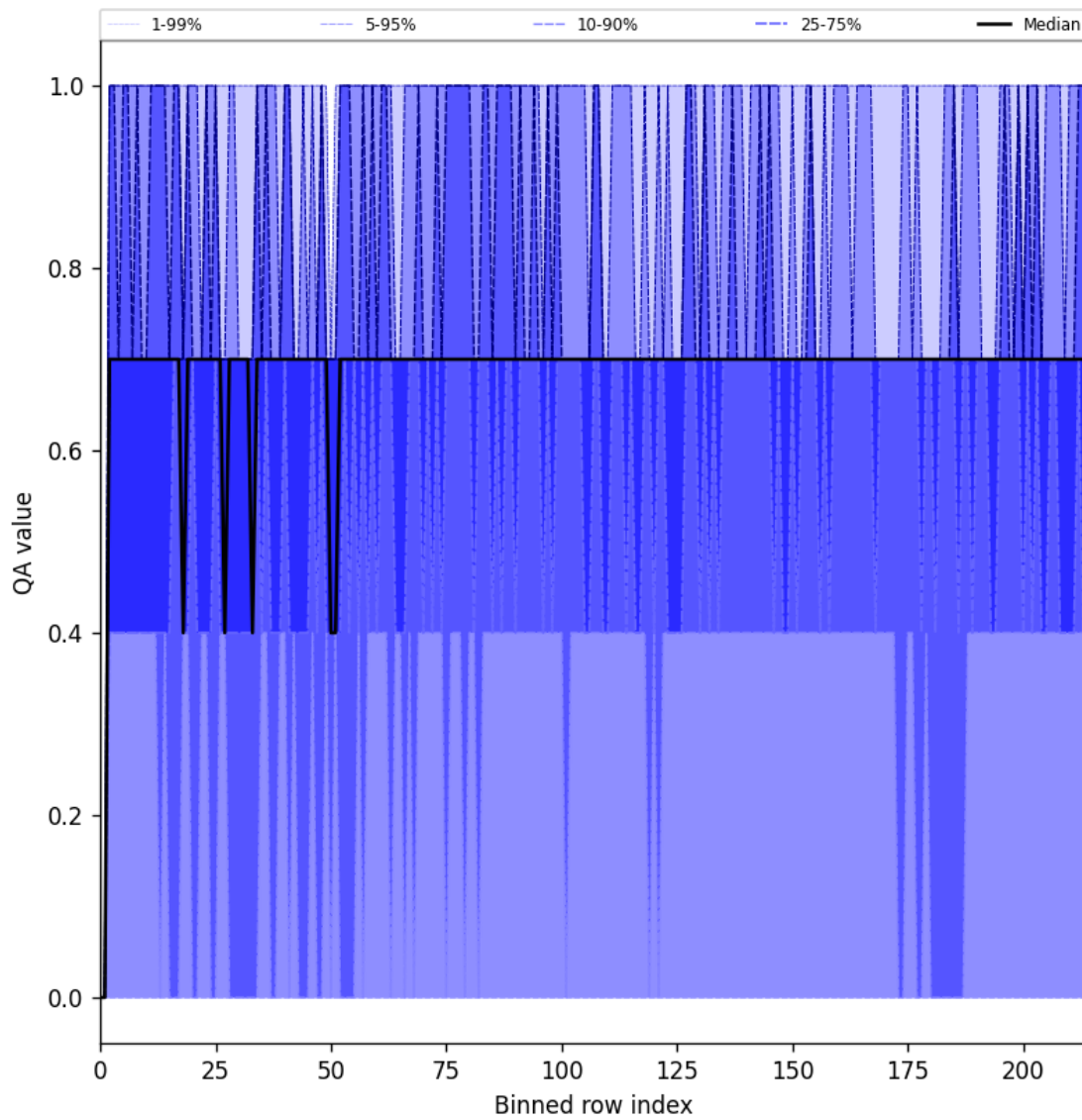
Figure 20: Along track statistics of “QA value” for 2025-08-17 to 2025-08-17
