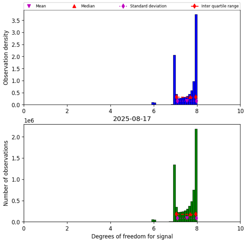
Figure 18: Histogram of “Degrees of freedom for signal” for 2025-08-17 to 2025-08-17
