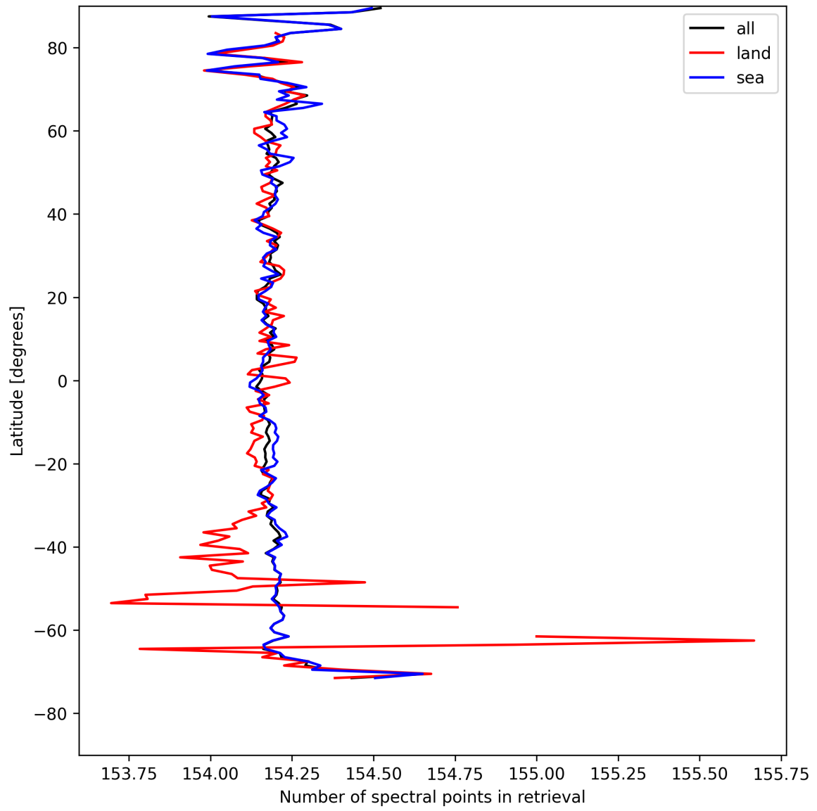
Figure 9: Zonal average of “Number of spectral points in retrieval” for 2025-08-17 to 2025-08-17.
