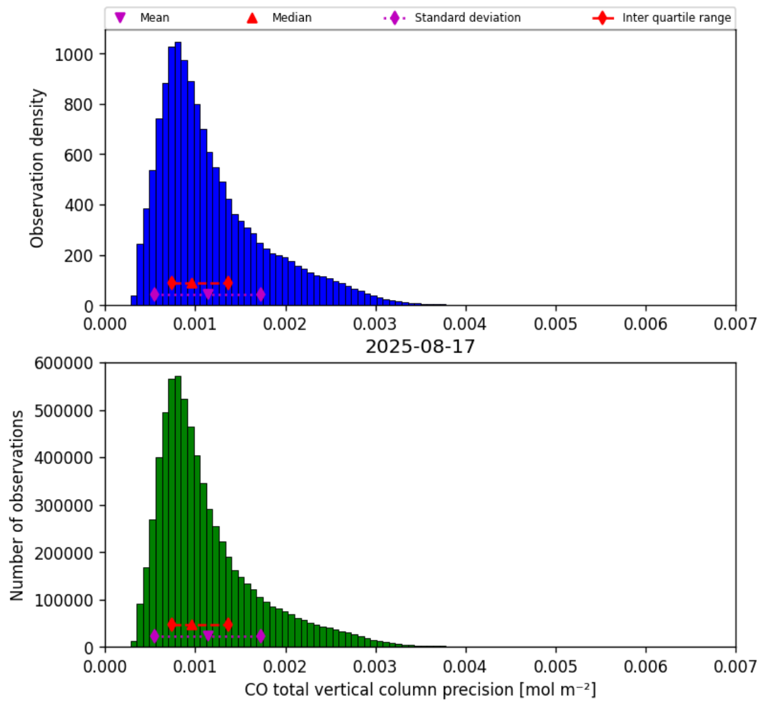
Figure 15: Histogram of “CO total vertical column precision” for 2025-08-17 to 2025-08-17
