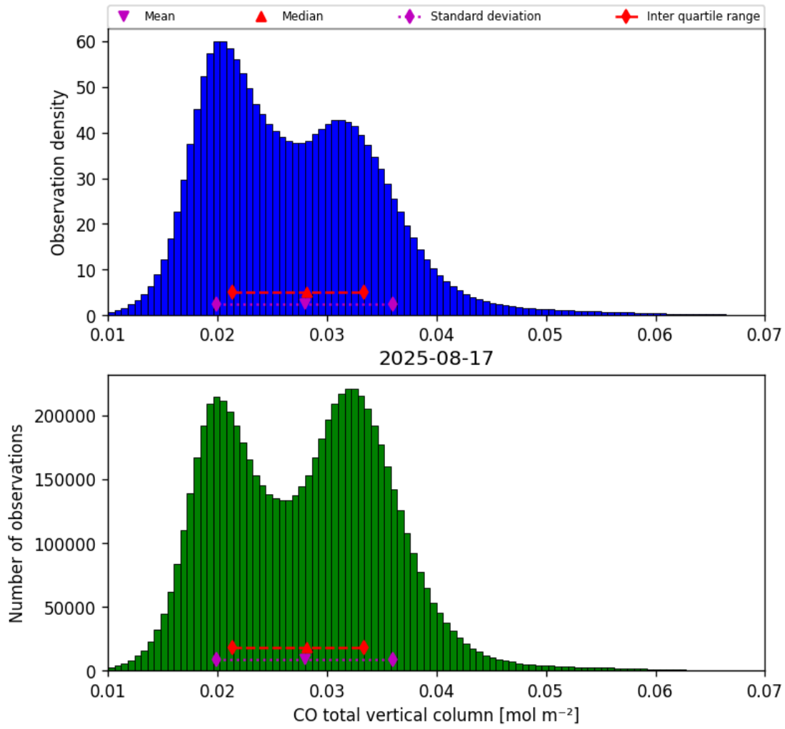
Figure 14: Histogram of “CO total vertical column” for 2025-08-17 to 2025-08-17
