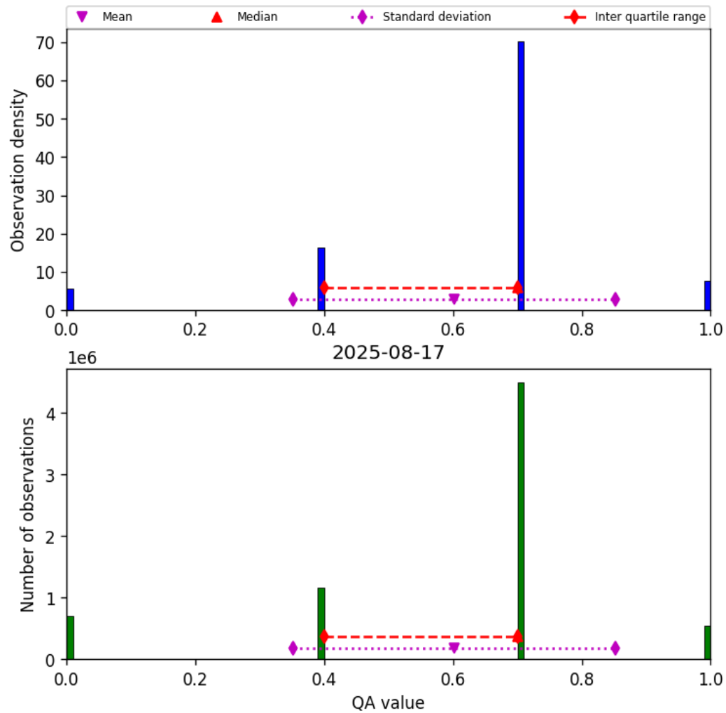
Figure 13: Histogram of “QA value” for 2025-08-17 to 2025-08-17
