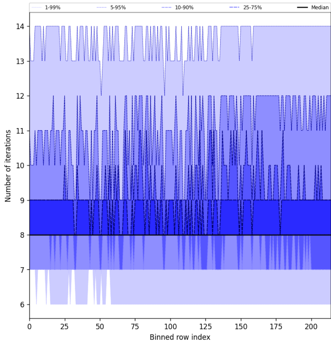
Figure 26: Along track statistics of “Number of iterations” for 2025-08-17 to 2025-08-17
