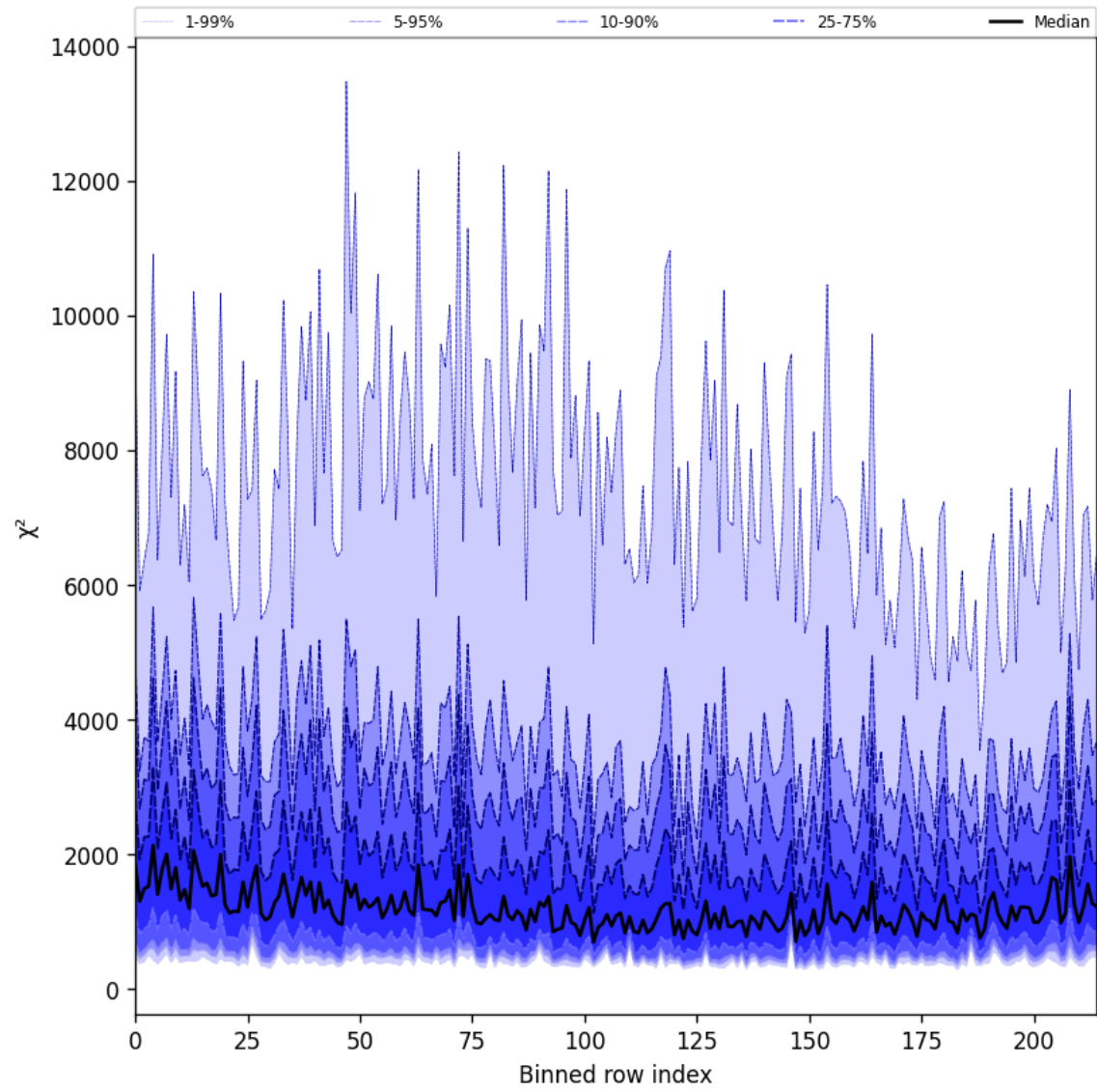
Figure 24: Along track statistics of “ \chi^2 ” for 2025-08-17 to 2025-08-17
