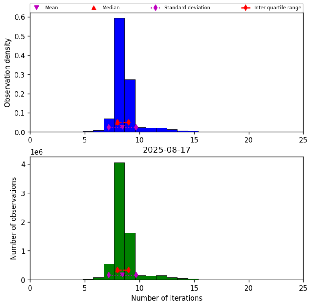
Figure 19: Histogram of “Number of iterations” for 2025-08-17 to 2025-08-17
