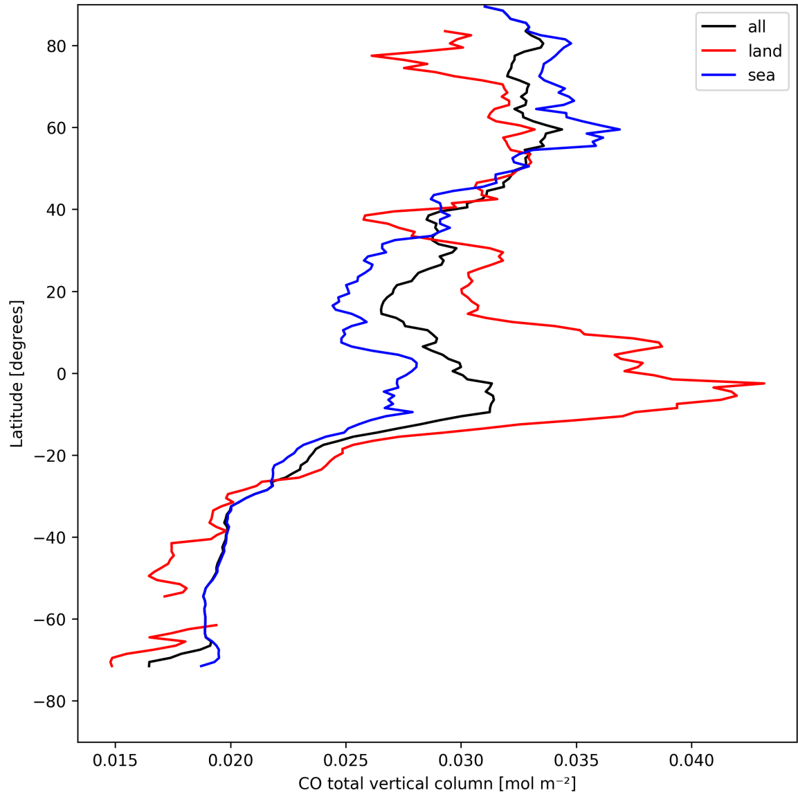
Figure 7: Zonal average of “CO total vertical column” for 2025-08-17 to 2025-08-17.
