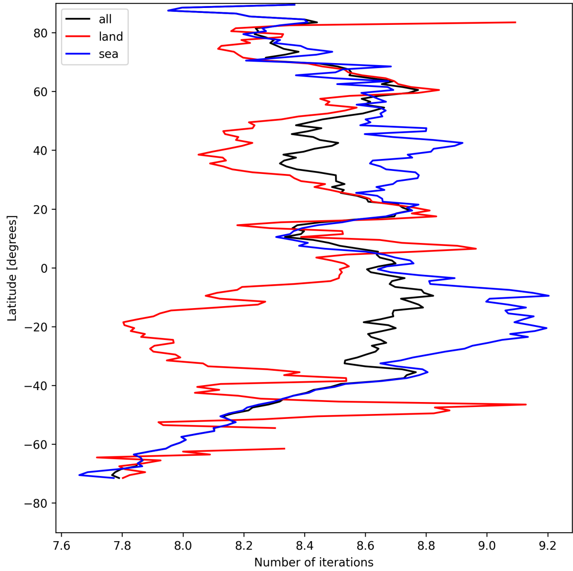
Figure 12: Zonal average of “Number of iterations” for 2025-08-17 to 2025-08-17.
