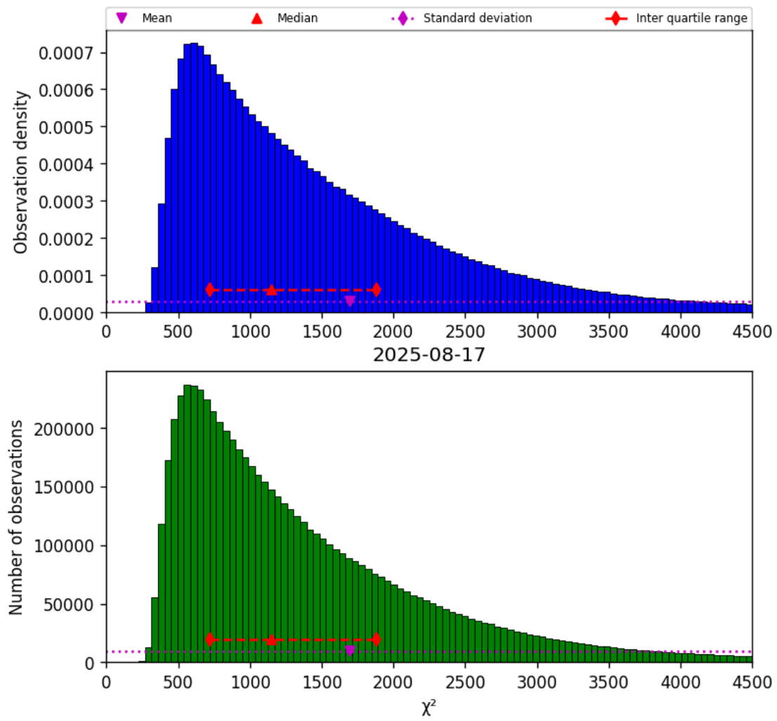
Figure 17: Histogram of " \chi^2 " for 2025-08-17 to 2025-08-17
