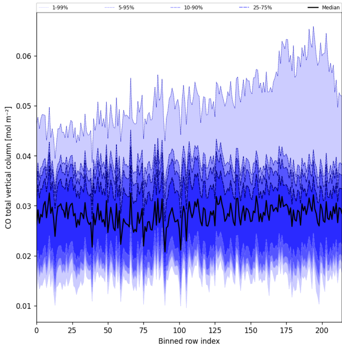
Figure 21: Along track statistics of “CO total vertical column” for 2025-08-18 to 2025-08-19
