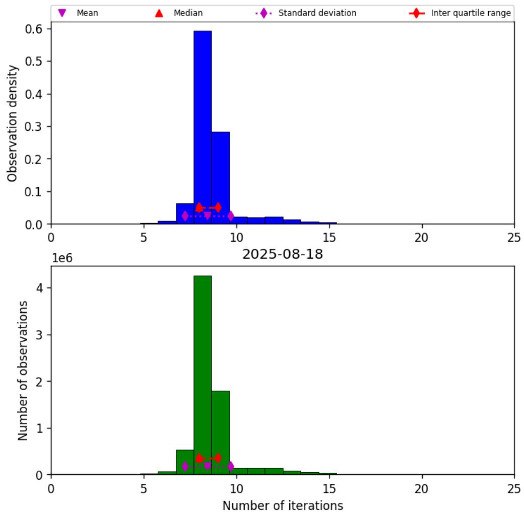
Figure 19: Histogram of “Number of iterations” for 2025-08-18 to 2025-08-19
