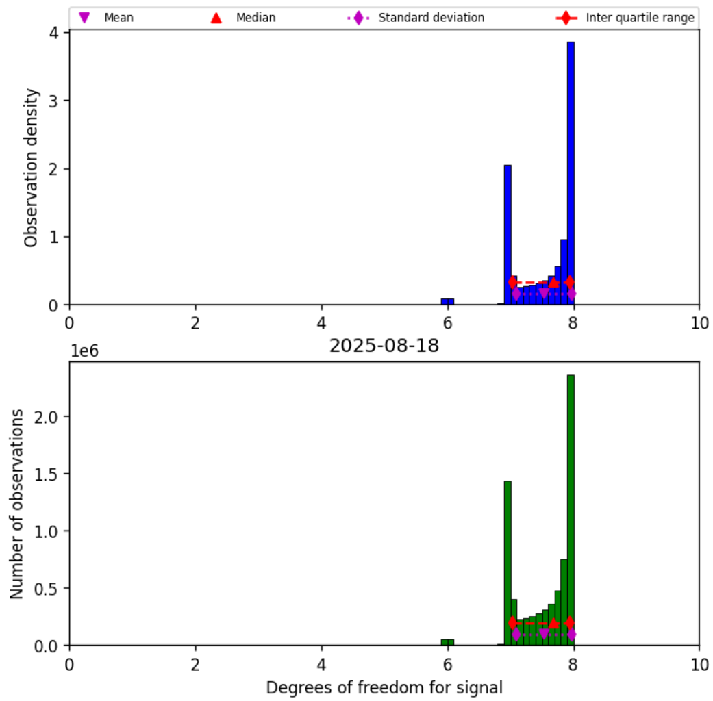
Figure 18: Histogram of “Degrees of freedom for signal” for 2025-08-18 to 2025-08-19
