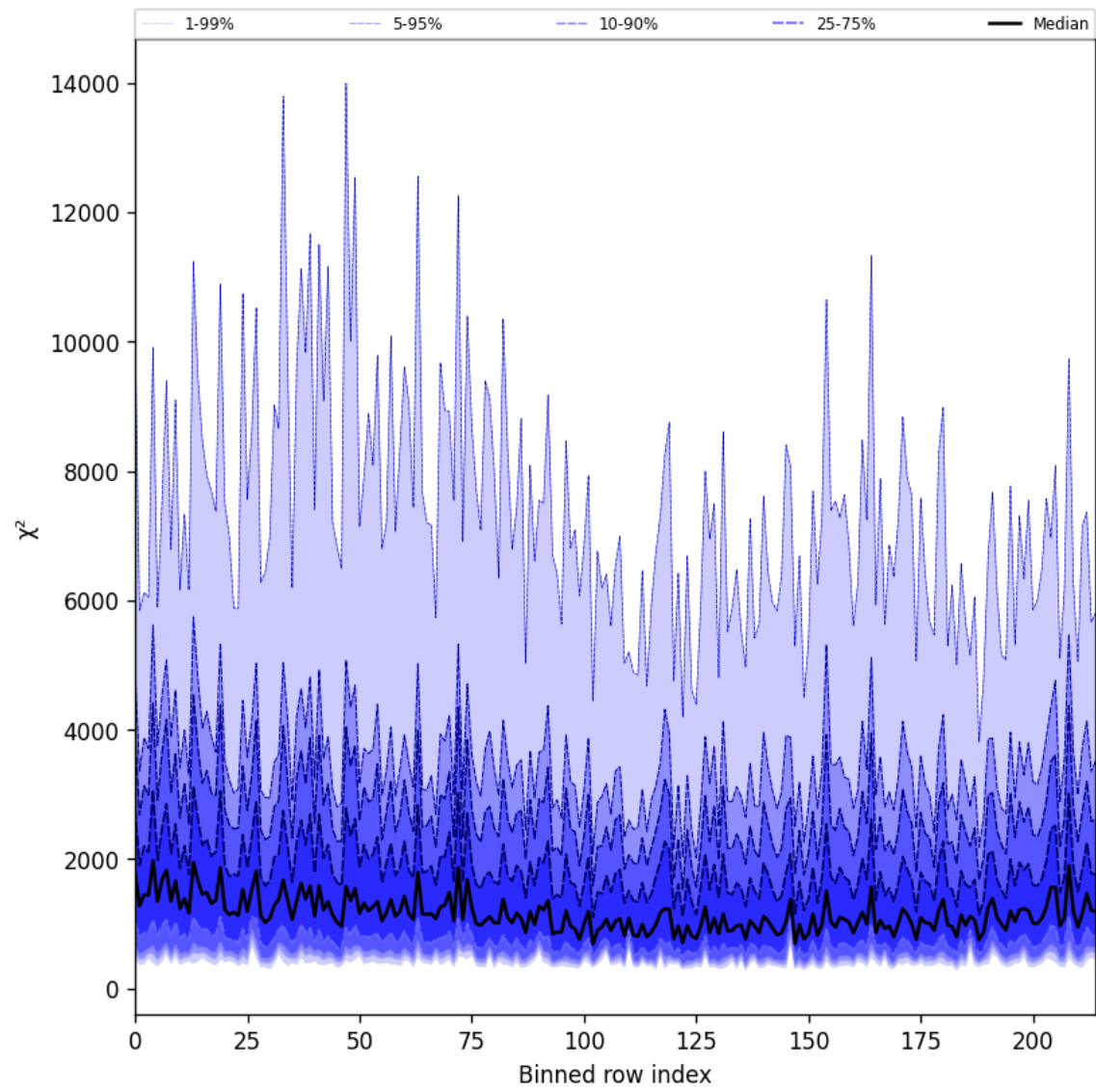
Figure 24: Along track statistics of “ \chi^2 ” for 2025-08-18 to 2025-08-19
