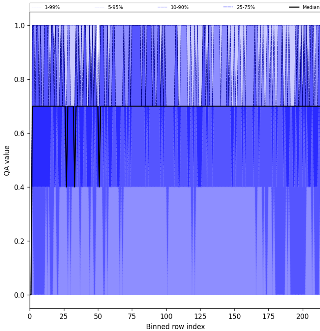
Figure 20: Along track statistics of “QA value” for 2025-08-18 to 2025-08-19
