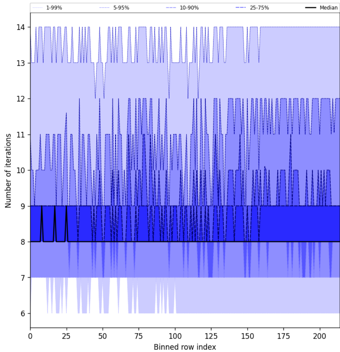
Figure 26: Along track statistics of “Number of iterations” for 2025-08-18 to 2025-08-19
