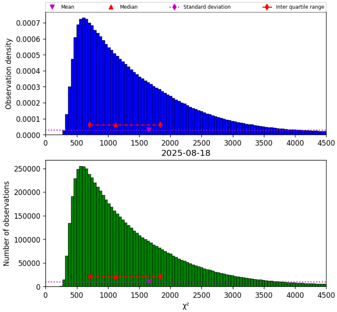
Figure 17: Histogram of “ \chi^2 ” for 2025-08-18 to 2025-08-19
