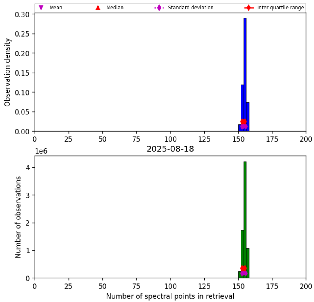
Figure 16: Histogram of “Number of spectral points in retrieval” for 2025-08-18 to 2025-08-19
