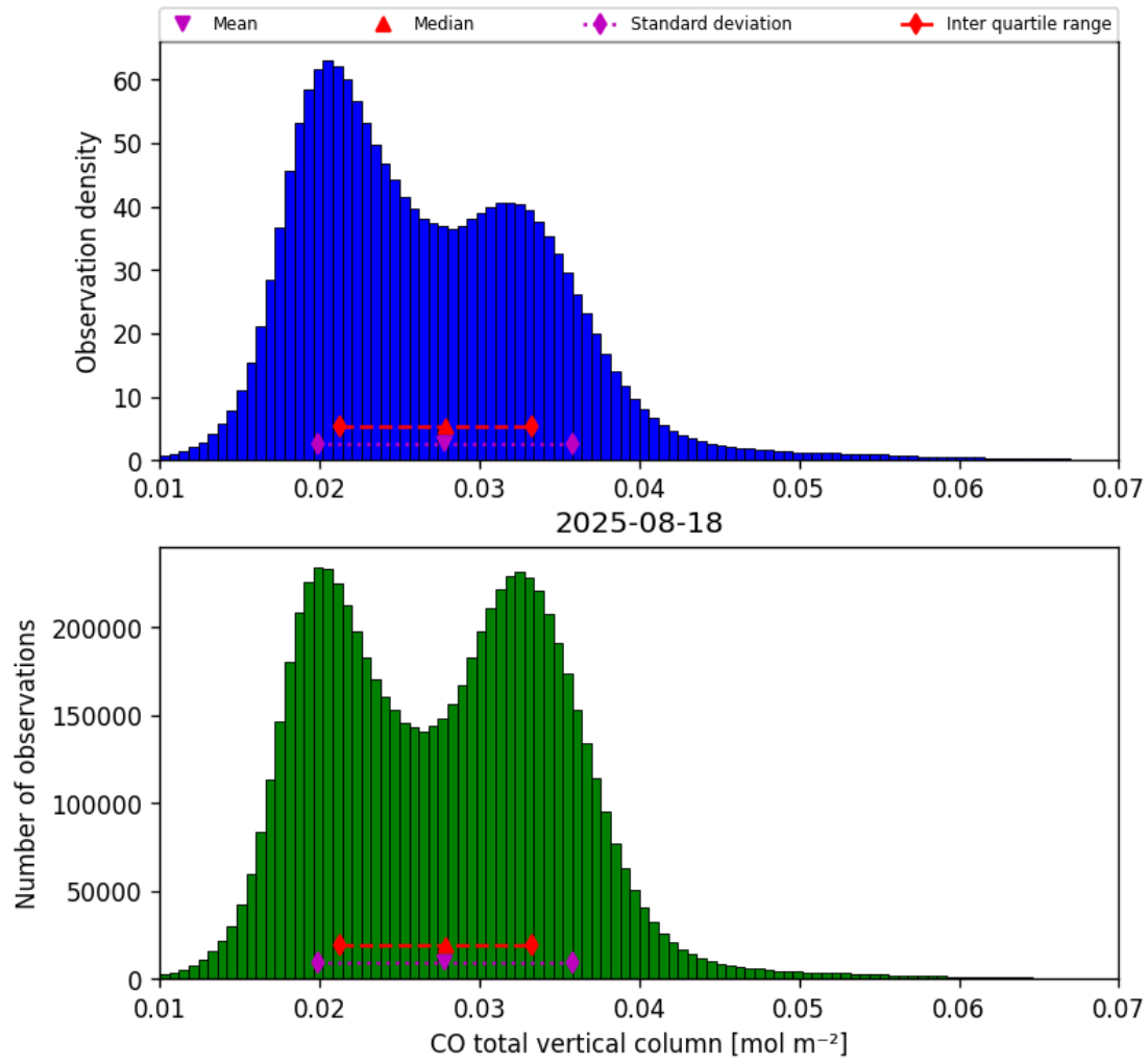
Figure 14: Histogram of “CO total vertical column” for 2025-08-18 to 2025-08-19
