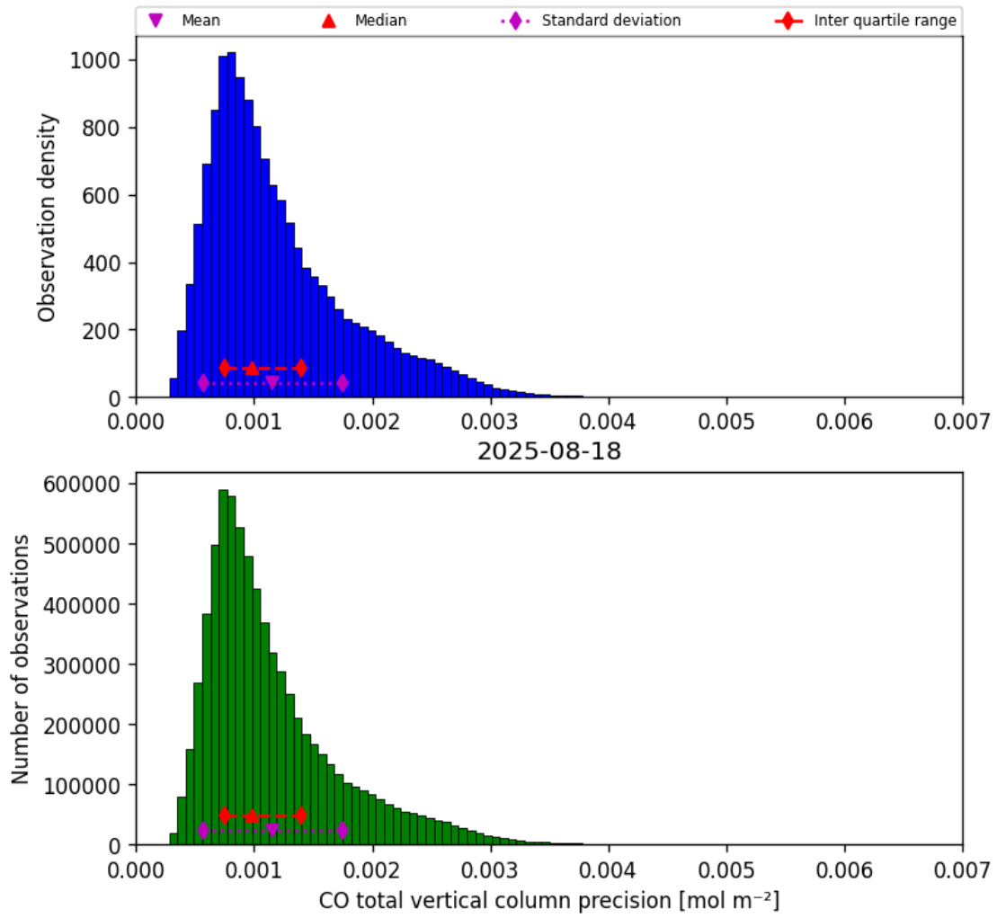
Figure 15: Histogram of “CO total vertical column precision” for 2025-08-18 to 2025-08-19
