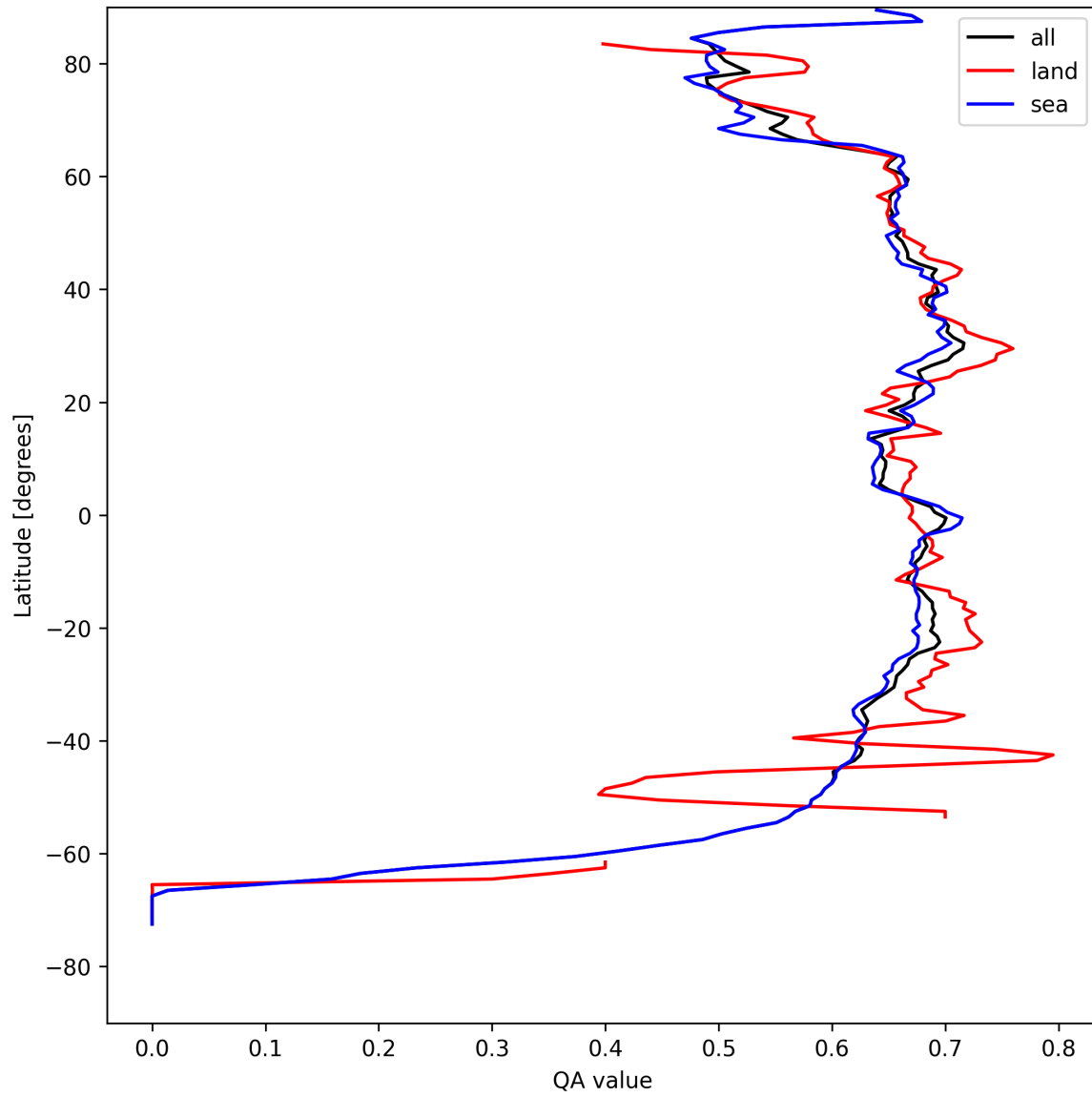
Figure 6: Zonal average of “QA value” for 2025-08-18 to 2025-08-19.
