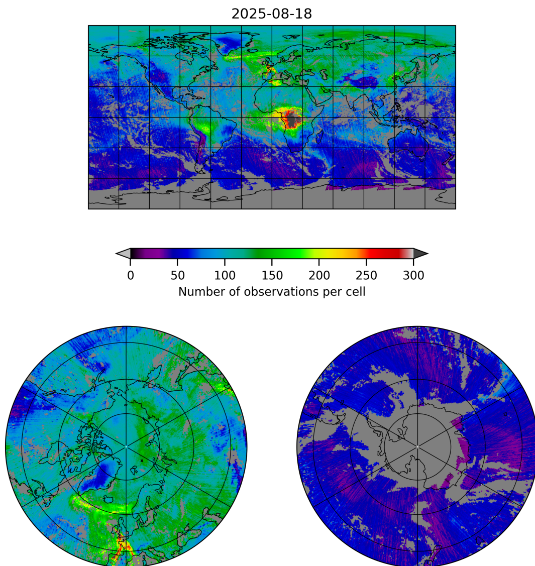
Figure 5: Map of the number of observations for 2025-08-18 to 2025-08-19
