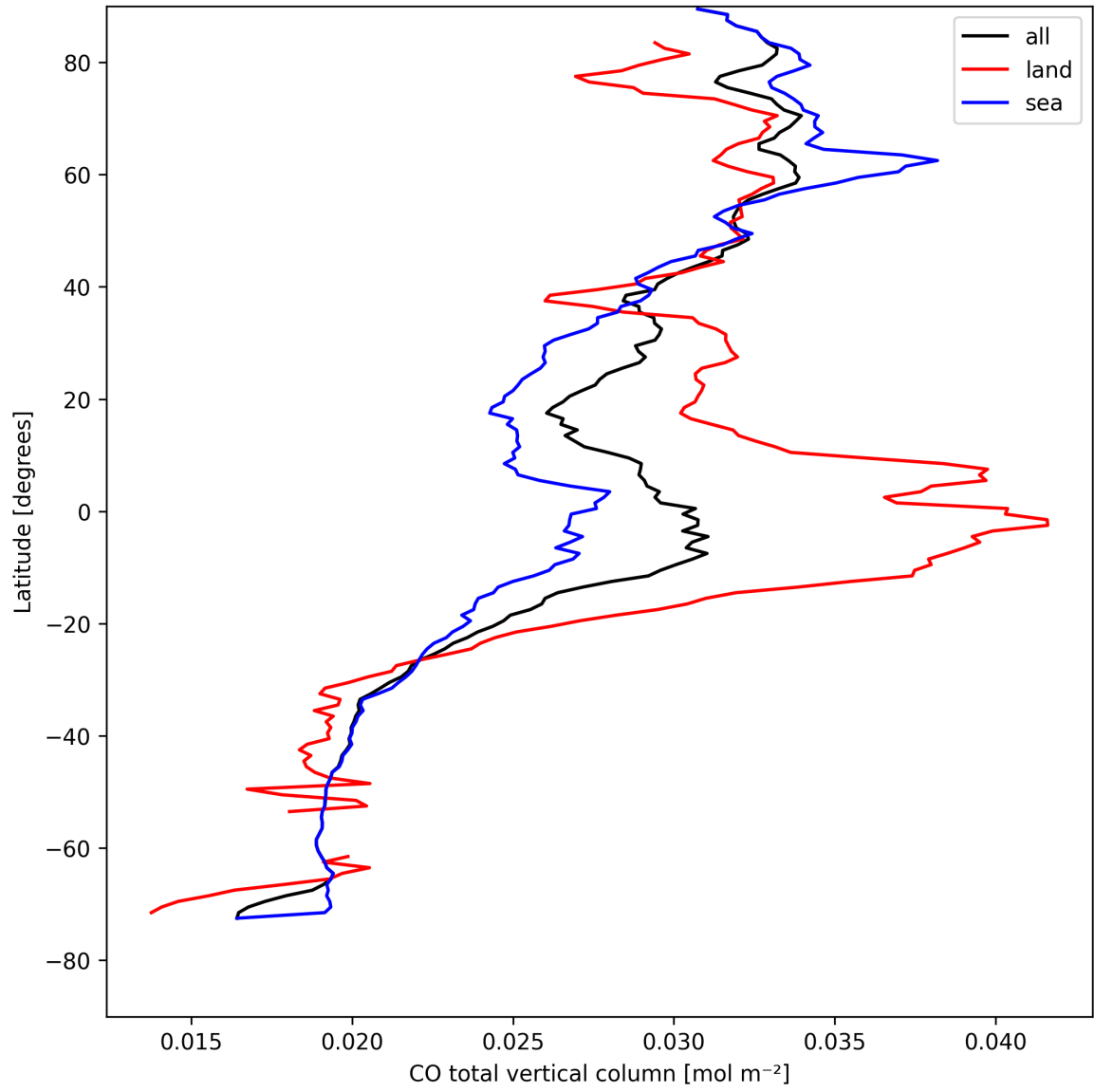
Figure 7: Zonal average of “CO total vertical column” for 2025-08-18 to 2025-08-19.
