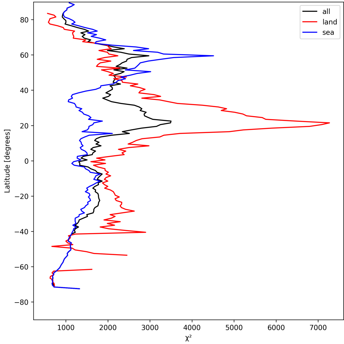
Figure 10: Zonal average of “ \chi^2 ” for 2025-08-18 to 2025-08-19.
