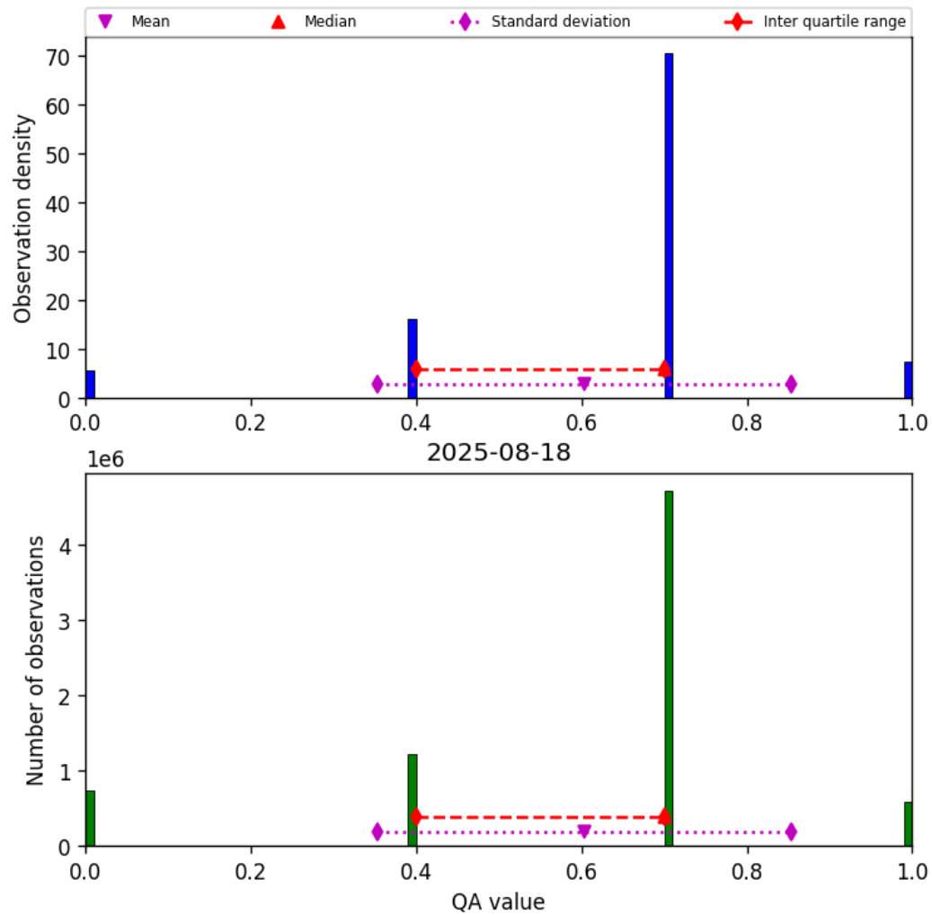
Figure 13: Histogram of “QA value” for 2025-08-18 to 2025-08-19
