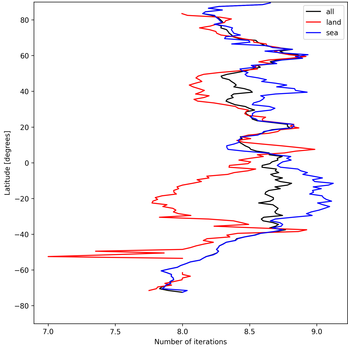
Figure 12: Zonal average of “Number of iterations” for 2025-08-18 to 2025-08-19.
