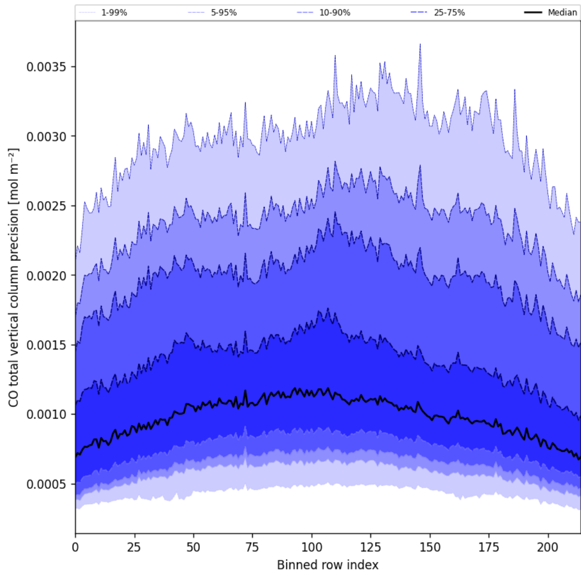
Figure 22: Along track statistics of “CO total vertical column precision” for 2025-08-18 to 2025-08-19
