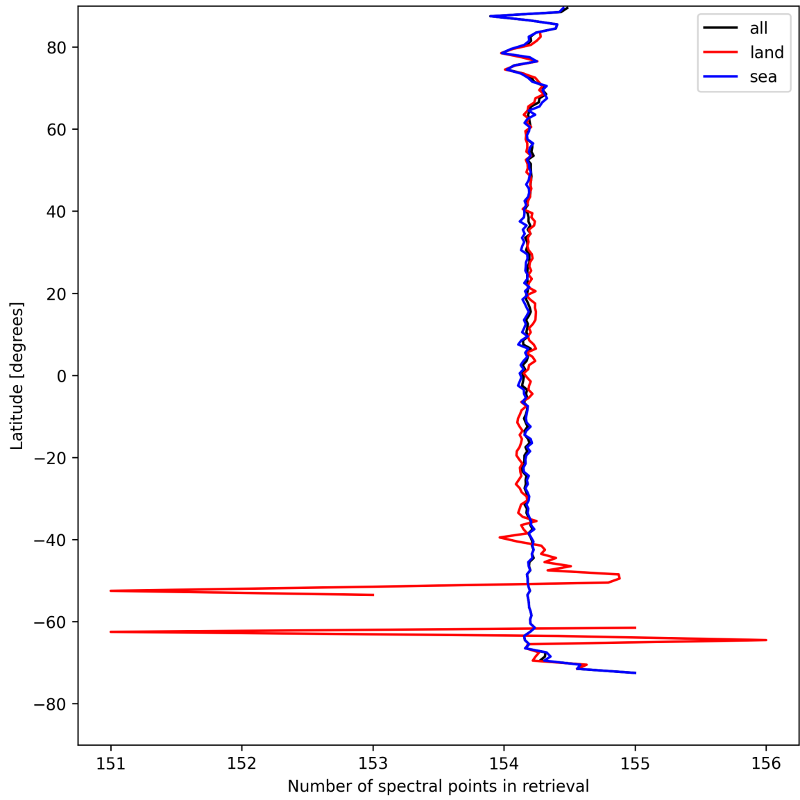
Figure 9: Zonal average of “Number of spectral points in retrieval” for 2025-08-18 to 2025-08-19.
