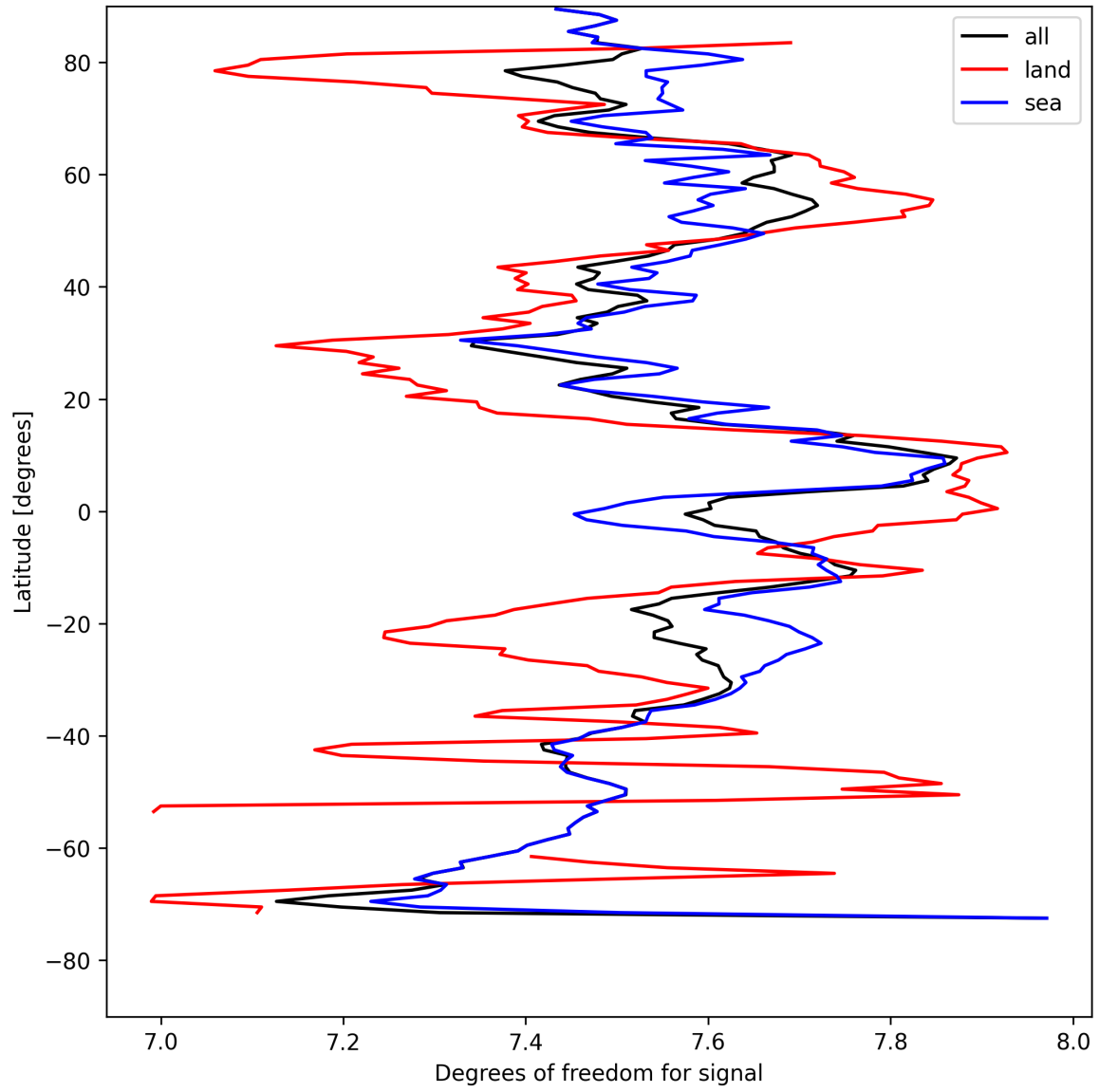
Figure 11: Zonal average of “Degrees of freedom for signal” for 2025-08-18 to 2025-08-19.
