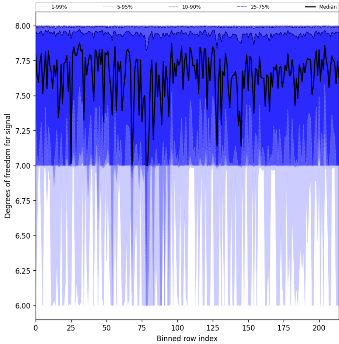
Figure 25: Along track statistics of “Degrees of freedom for signal” for 2025-08-18 to 2025-08-19
