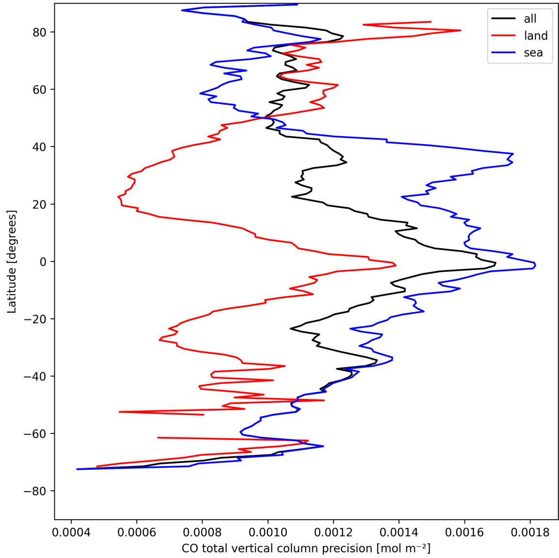
Figure 8: Zonal average of “CO total vertical column precision” for 2025-08-18 to 2025-08-19.
