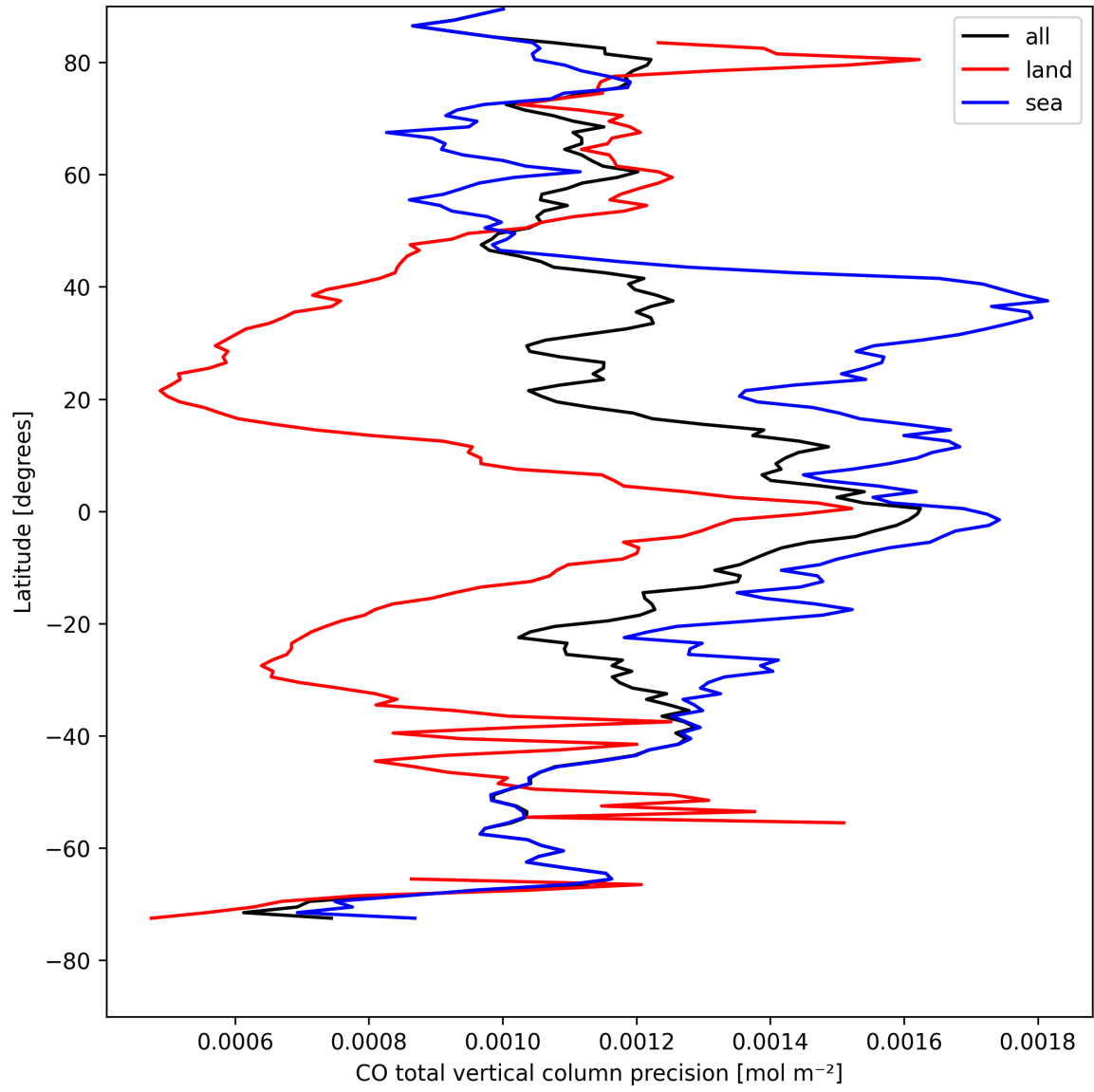
Figure 8: Zonal average of “CO total vertical column precision” for 2025-08-19 to 2025-08-20.
