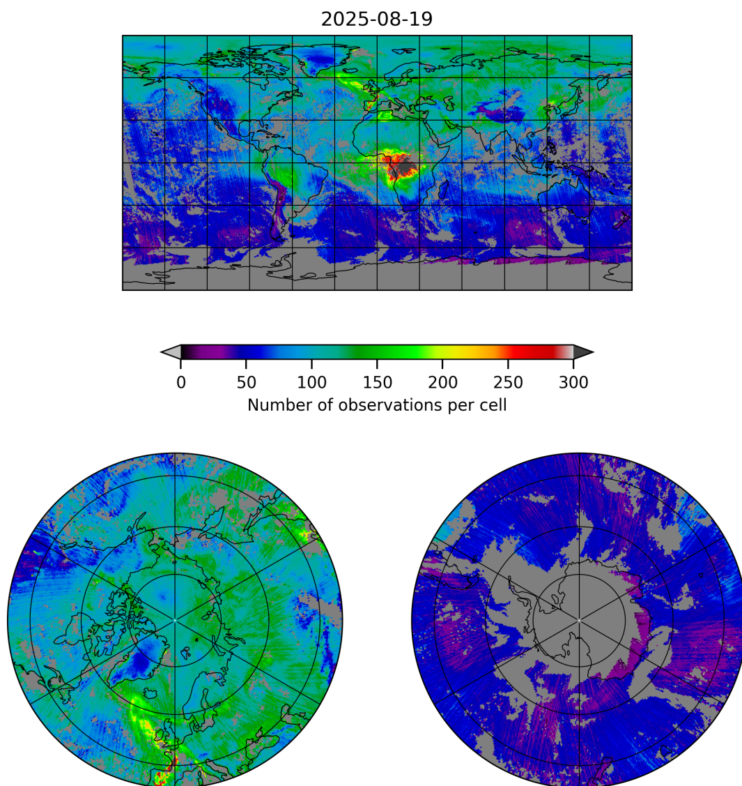
Figure 5: Map of the number of observations for 2025-08-19 to 2025-08-20
