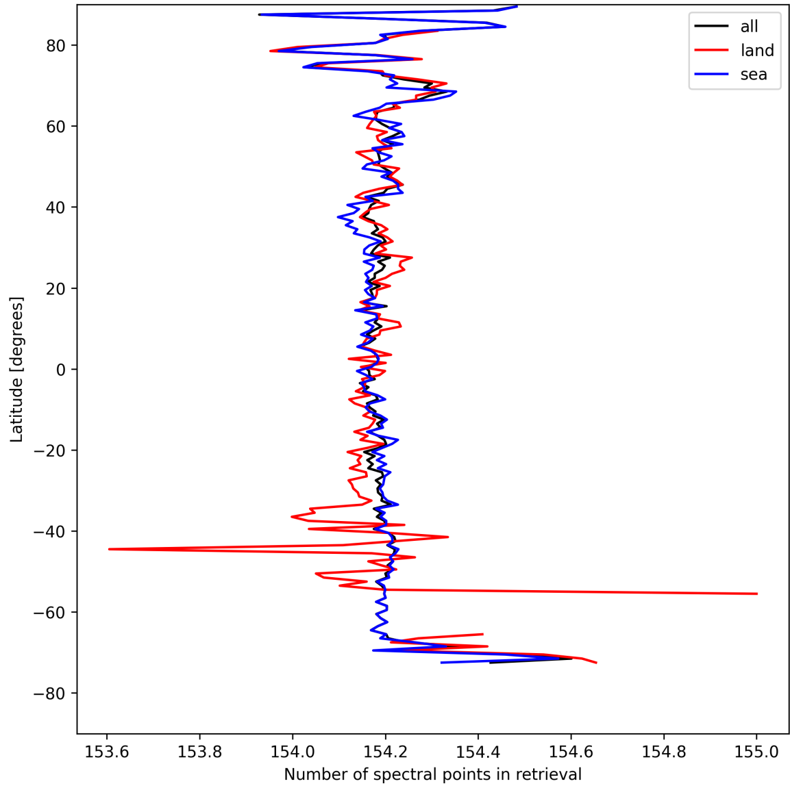
Figure 9: Zonal average of “Number of spectral points in retrieval” for 2025-08-19 to 2025-08-20.
