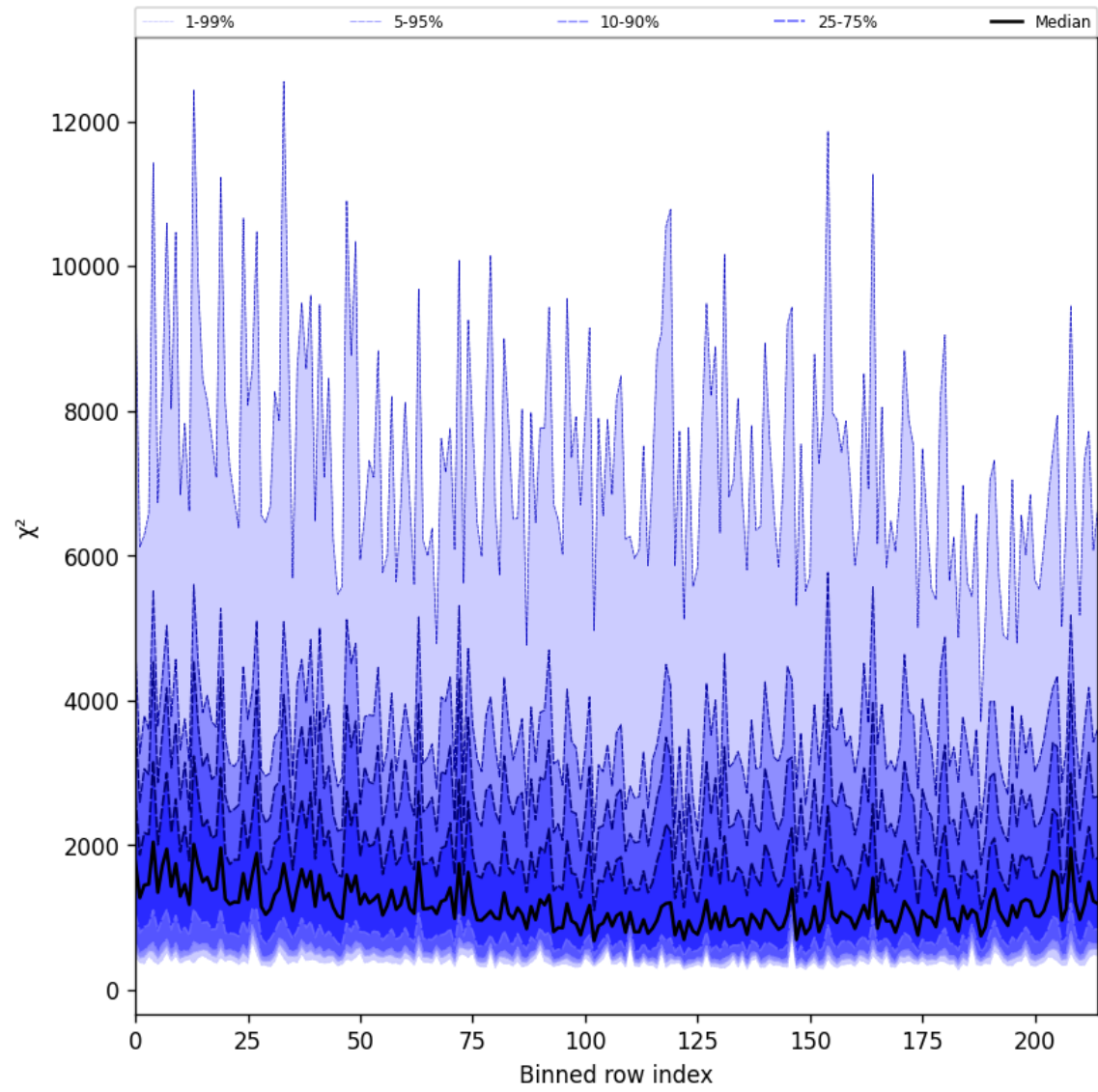
Figure 24: Along track statistics of “ \chi^2 ” for 2025-08-19 to 2025-08-20
