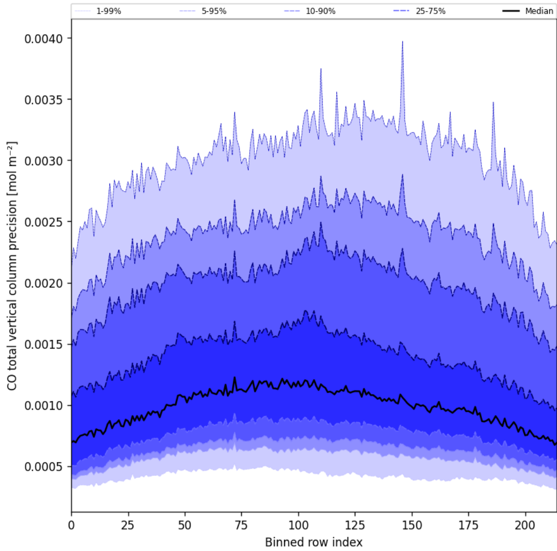
Figure 22: Along track statistics of “CO total vertical column precision” for 2025-08-19 to 2025-08-20
