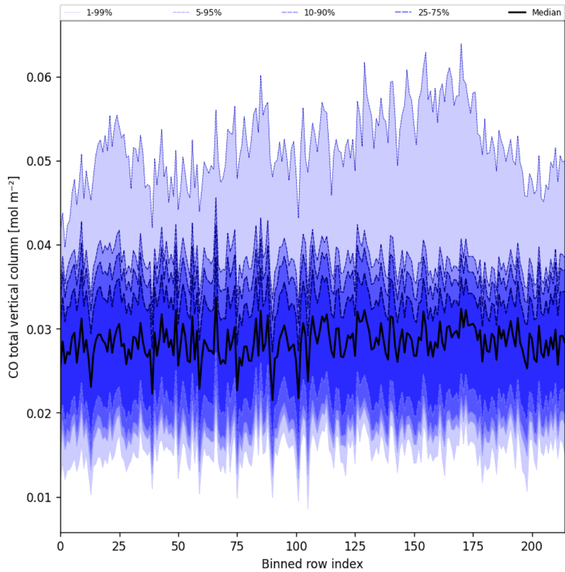
Figure 21: Along track statistics of “CO total vertical column” for 2025-08-19 to 2025-08-20
