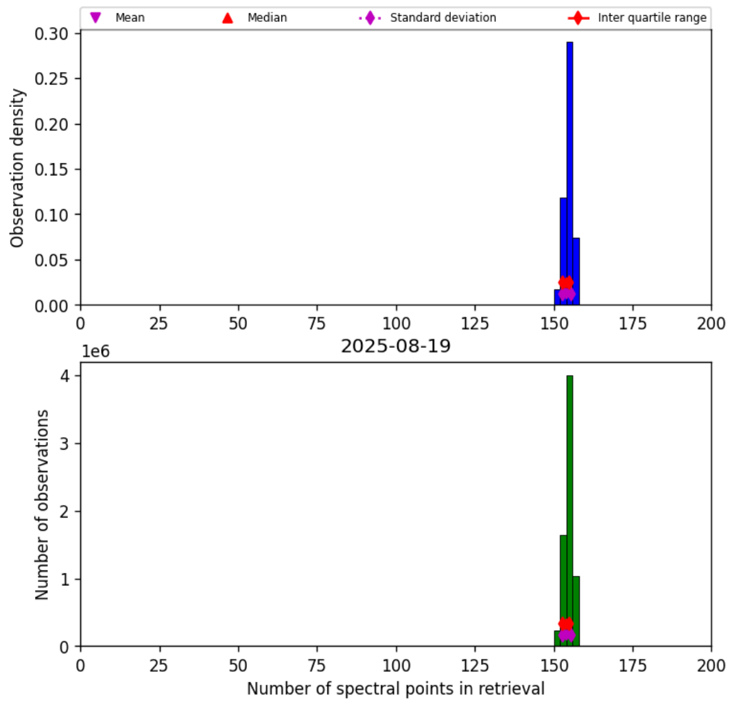
Figure 16: Histogram of “Number of spectral points in retrieval” for 2025-08-19 to 2025-08-20
