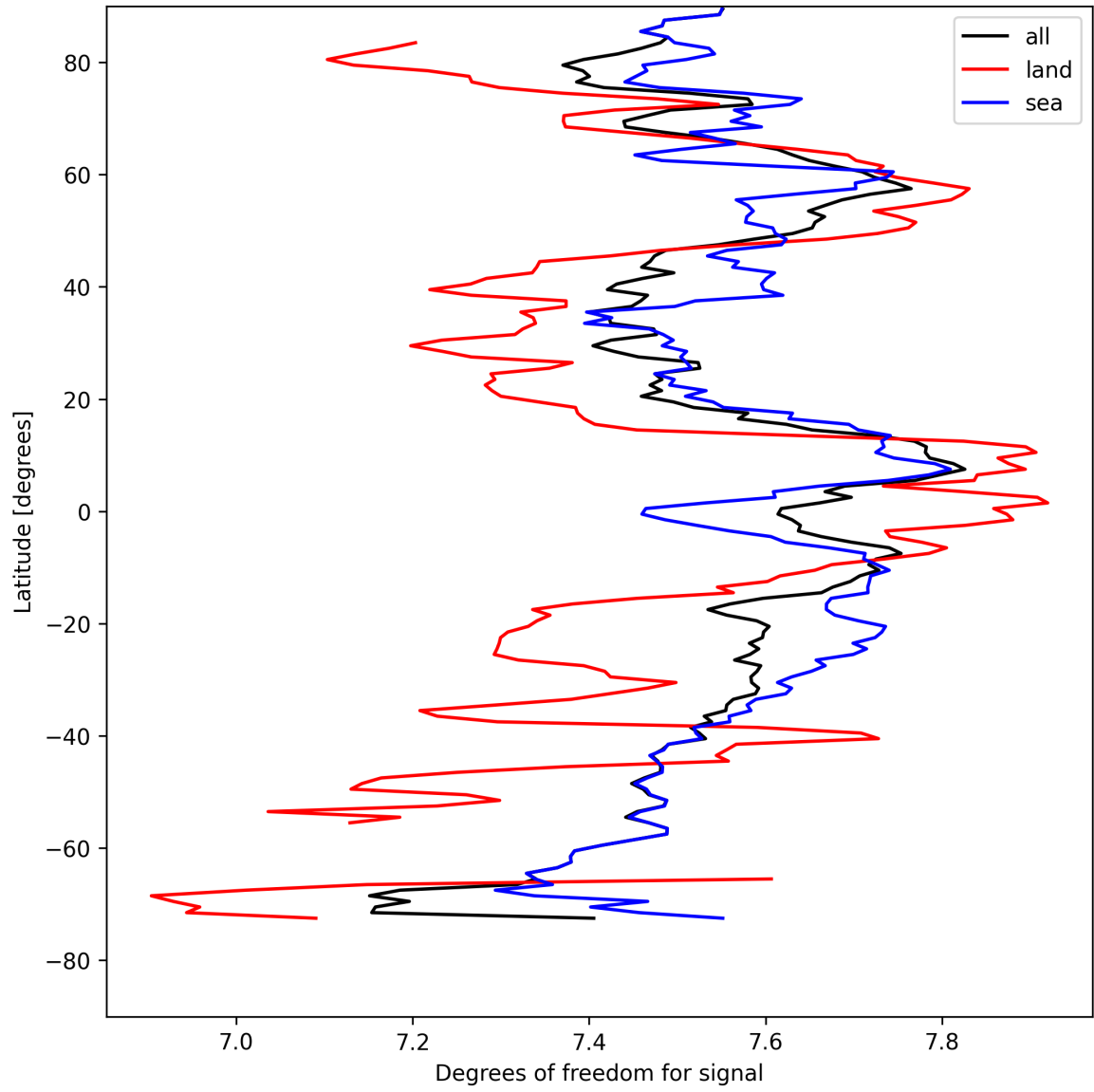
Figure 11: Zonal average of “Degrees of freedom for signal” for 2025-08-19 to 2025-08-20.
