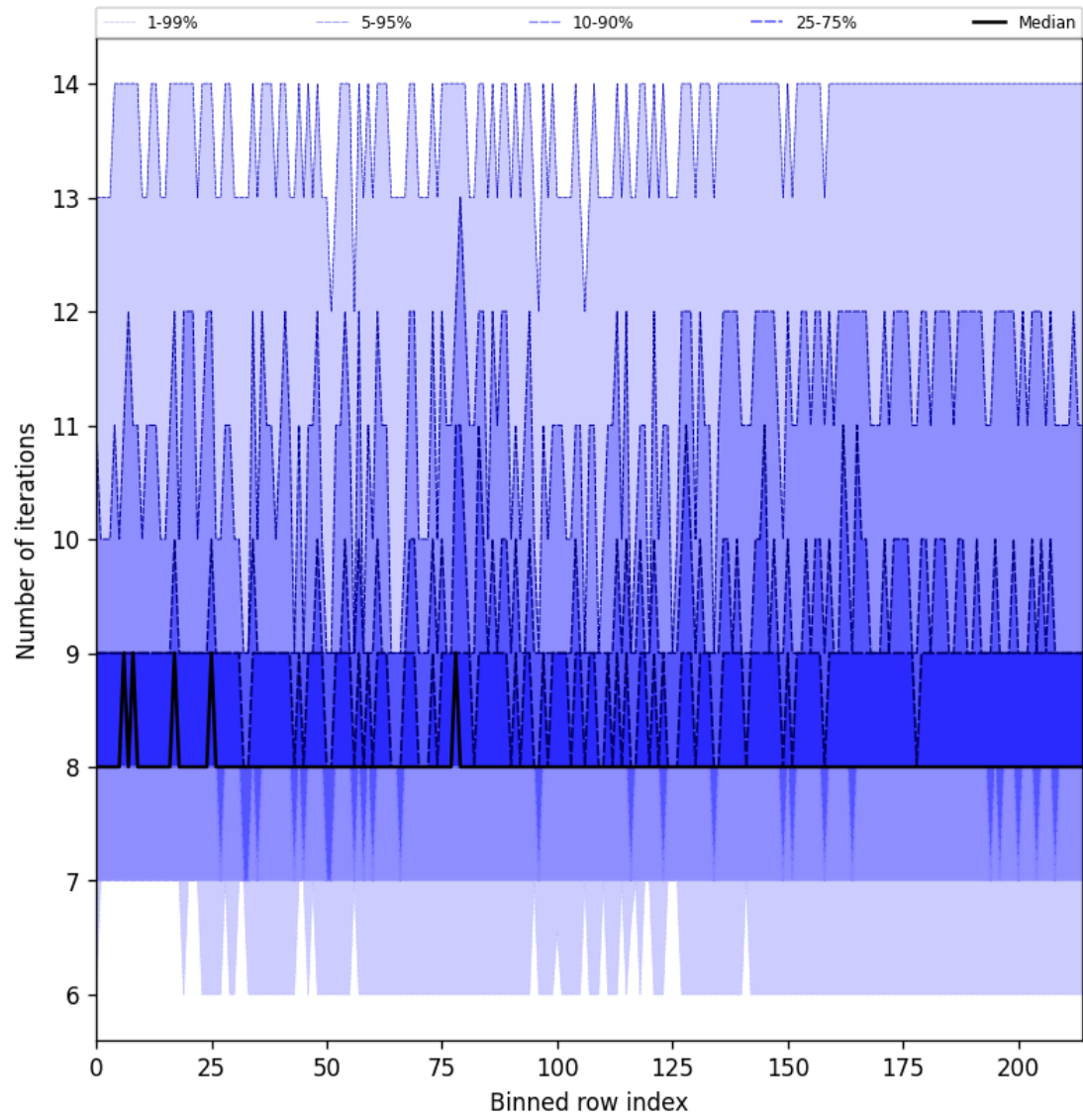
Figure 26: Along track statistics of “Number of iterations” for 2025-08-19 to 2025-08-20
