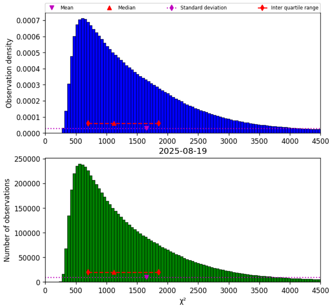
Figure 17: Histogram of “ \chi^2 ” for 2025-08-19 to 2025-08-20
