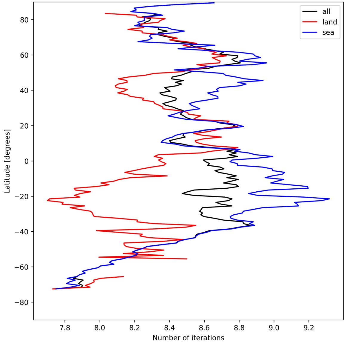
Figure 12: Zonal average of “Number of iterations” for 2025-08-19 to 2025-08-20.
