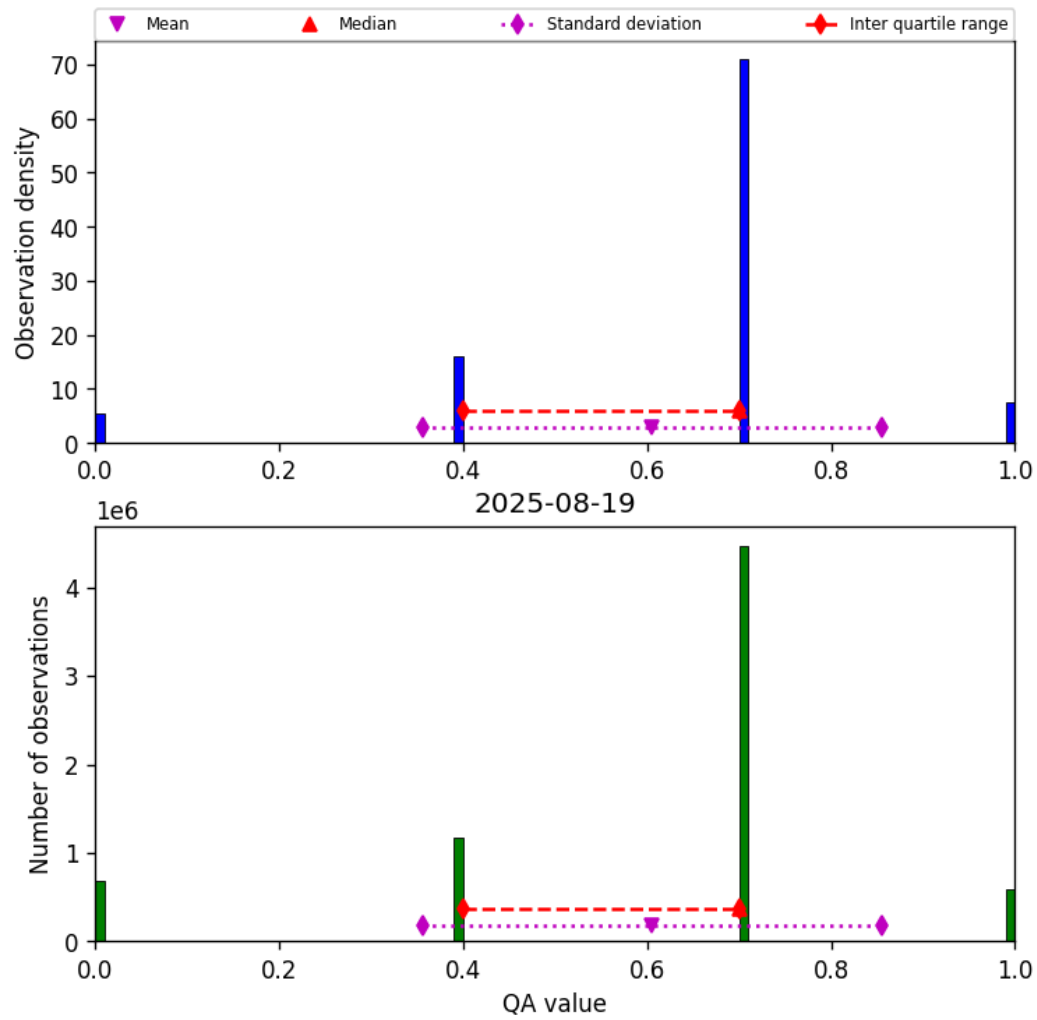
Figure 13: Histogram of “QA value” for 2025-08-19 to 2025-08-20
