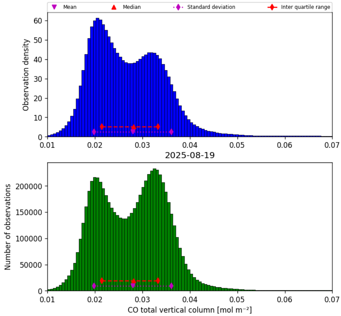
Figure 14: Histogram of “CO total vertical column” for 2025-08-19 to 2025-08-20
