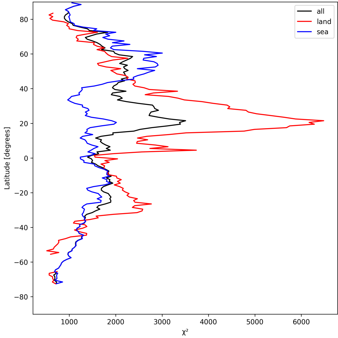
Figure 10: Zonal average of “ \chi^2 ” for 2025-08-19 to 2025-08-20.
