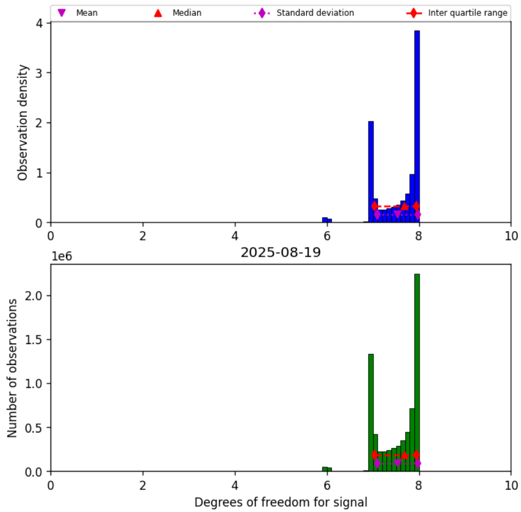
Figure 18: Histogram of “Degrees of freedom for signal” for 2025-08-19 to 2025-08-20
