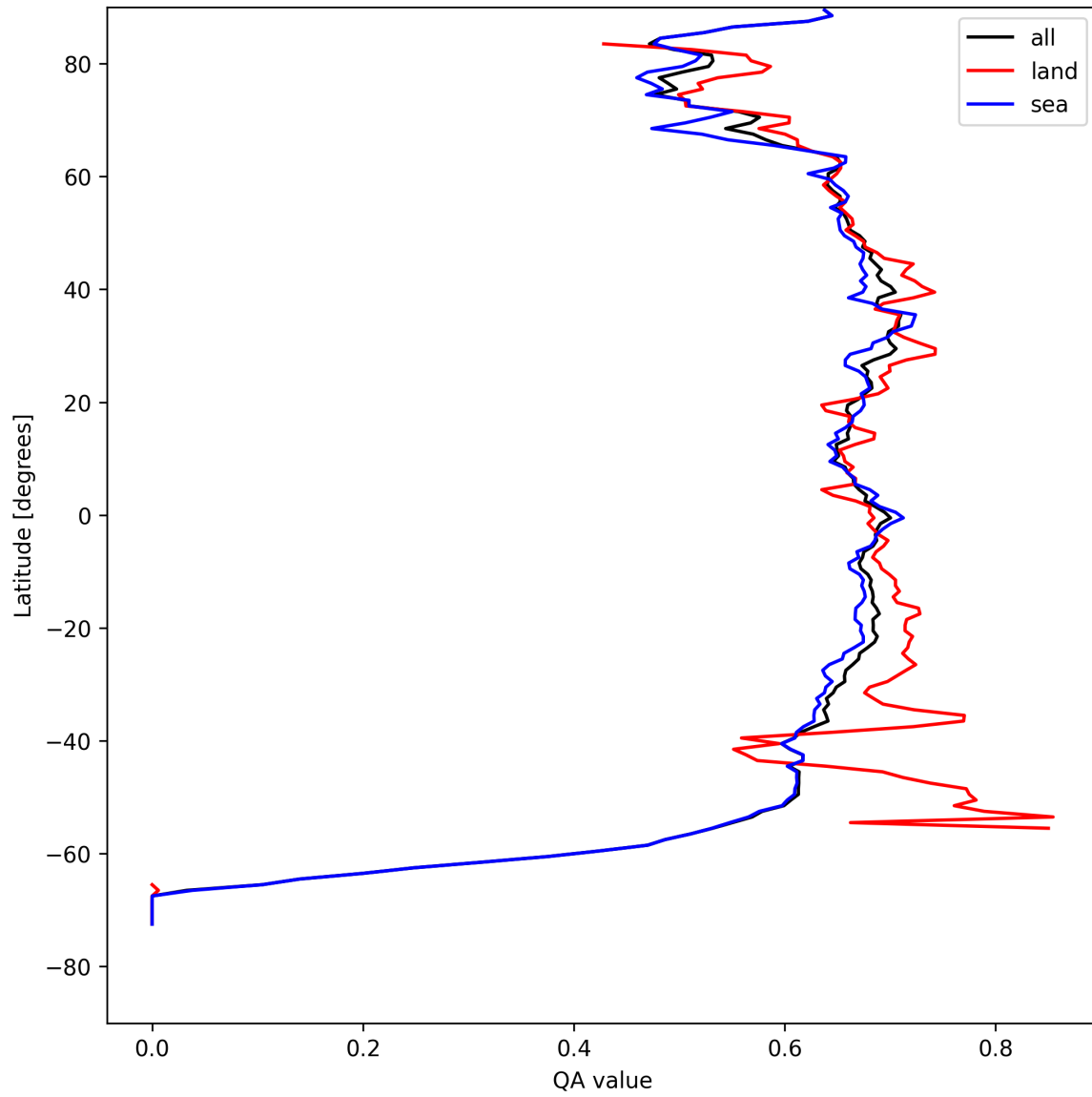
Figure 6: Zonal average of “QA value” for 2025-08-19 to 2025-08-20.
