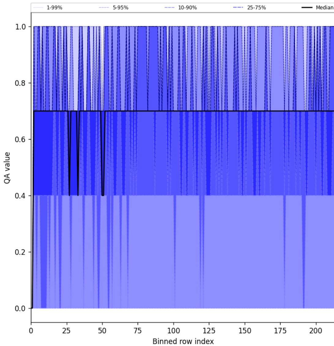
Figure 20: Along track statistics of “QA value” for 2025-08-19 to 2025-08-20
