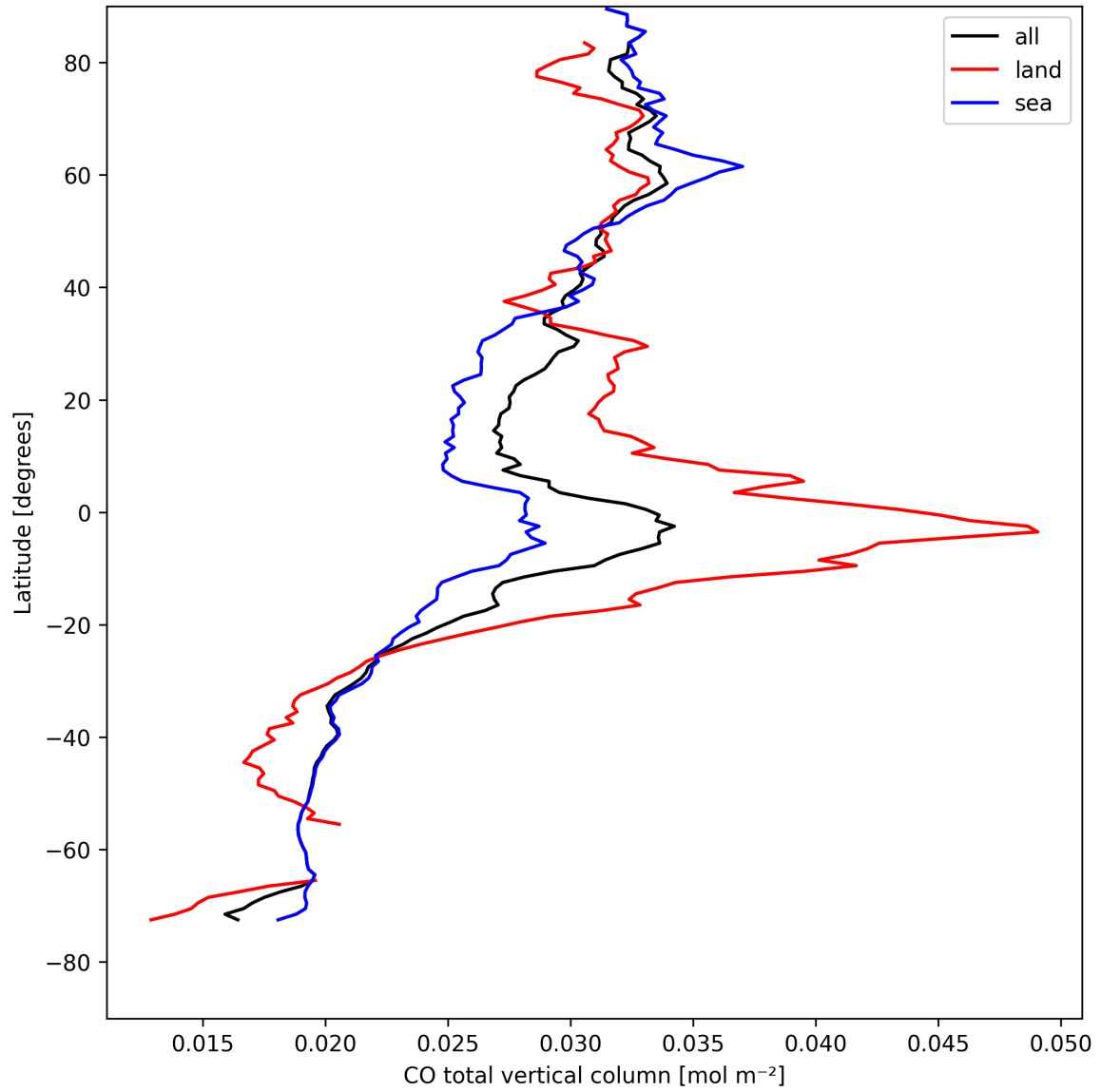
Figure 7: Zonal average of “CO total vertical column” for 2025-08-19 to 2025-08-20.
