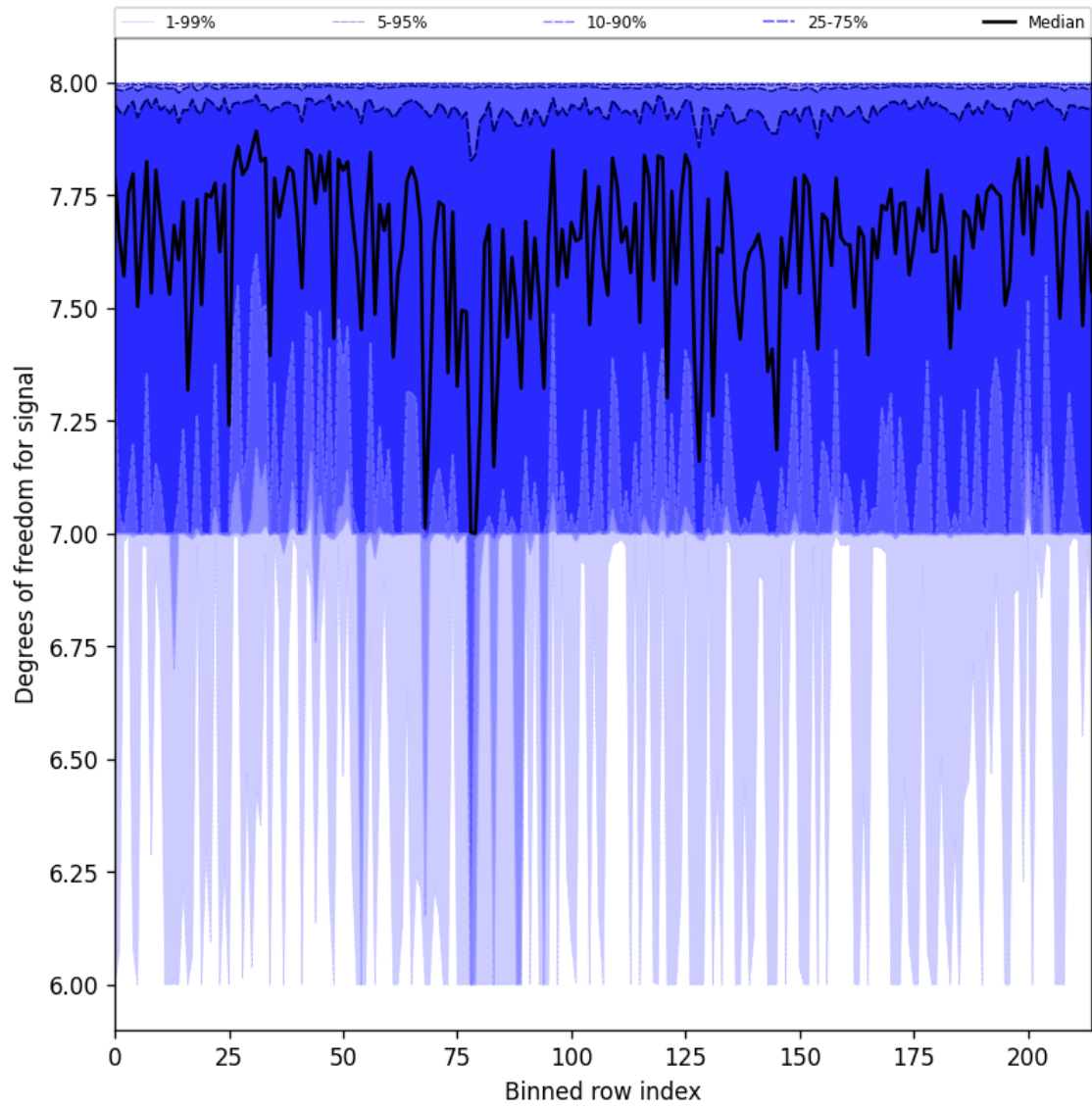
Figure 25: Along track statistics of “Degrees of freedom for signal” for 2025-08-19 to 2025-08-20
