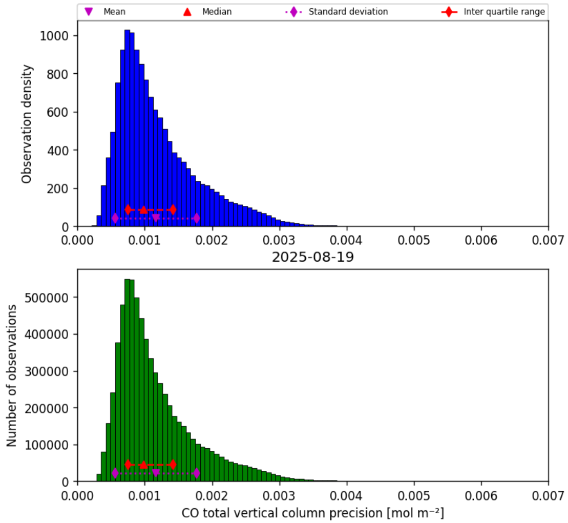
Figure 15: Histogram of “CO total vertical column precision” for 2025-08-19 to 2025-08-20
