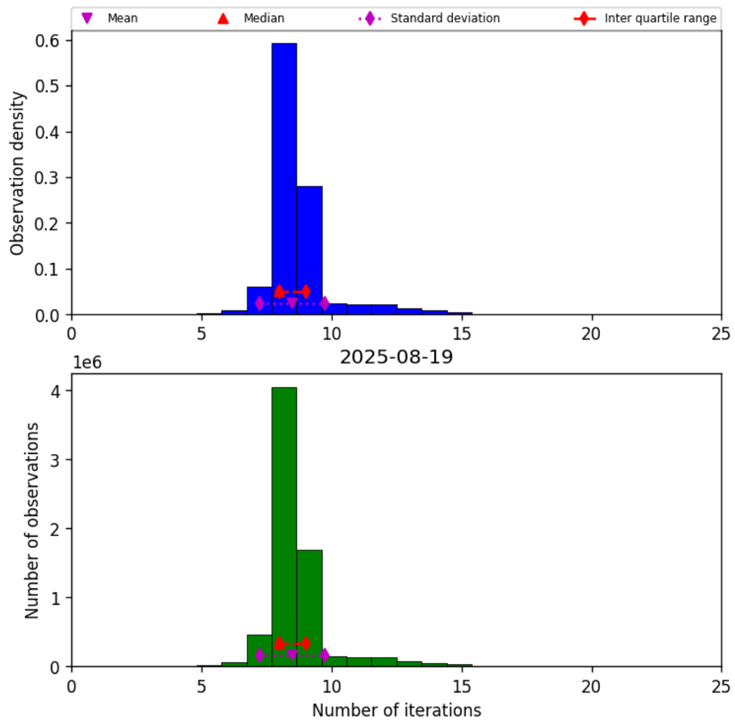
Figure 19: Histogram of “Number of iterations” for 2025-08-19 to 2025-08-20
