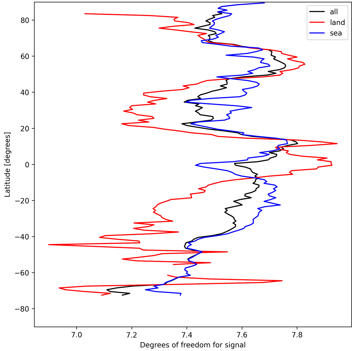
Figure 11: Zonal average of “Degrees of freedom for signal” for 2025-08-20 to 2025-08-21.
