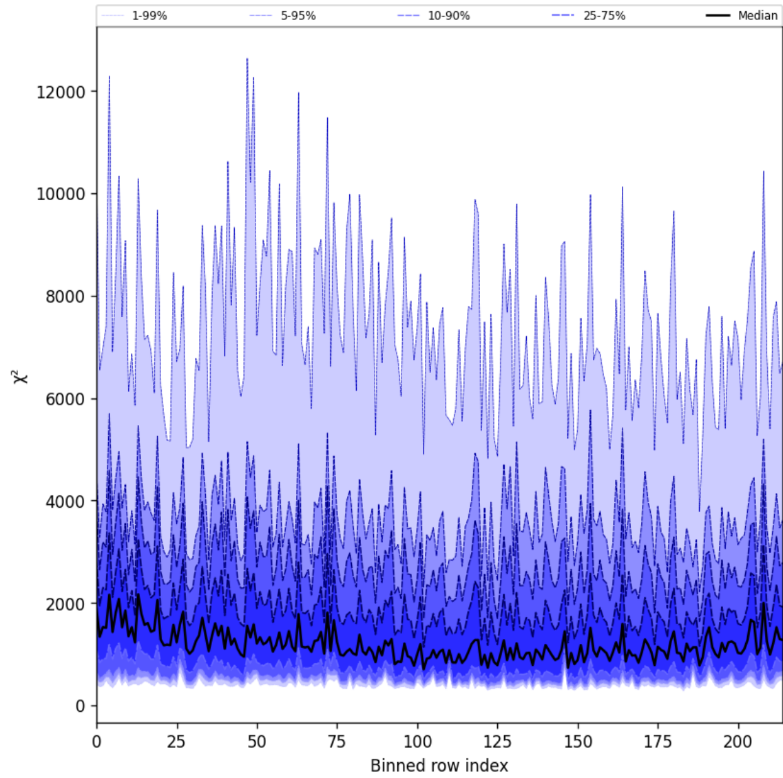
Figure 24: Along track statistics of “ \chi^2 ” for 2025-08-20 to 2025-08-21
