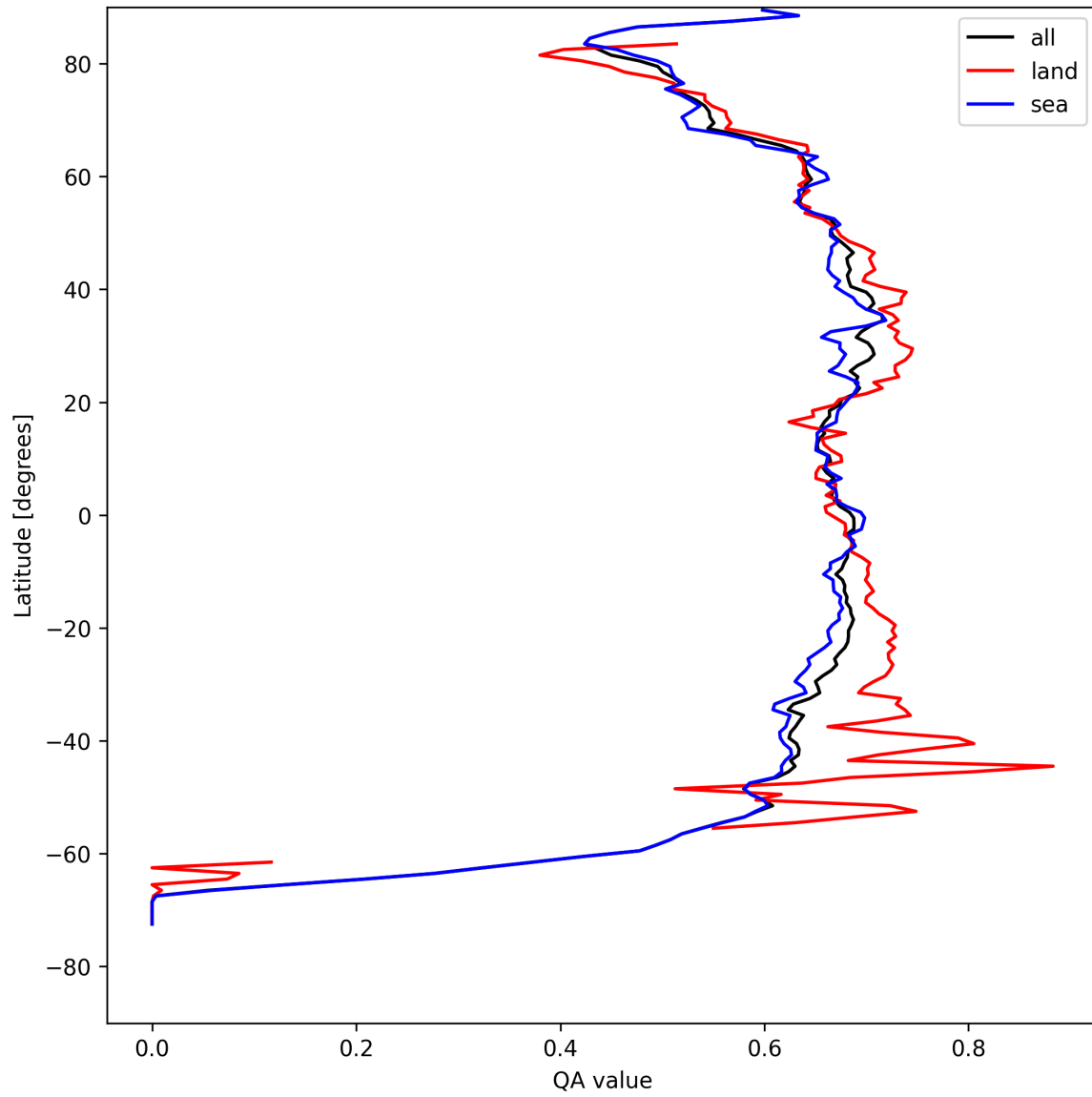
Figure 6: Zonal average of “QA value” for 2025-08-20 to 2025-08-21.
