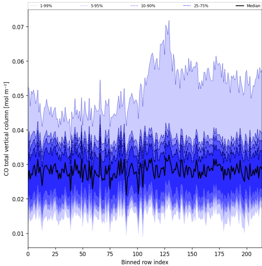
Figure 21: Along track statistics of “CO total vertical column” for 2025-08-20 to 2025-08-21
