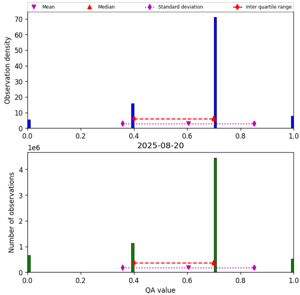
Figure 13: Histogram of “QA value” for 2025-08-20 to 2025-08-21
