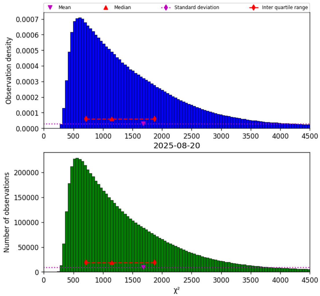
Figure 17: Histogram of “ \chi^2 ” for 2025-08-20 to 2025-08-21
