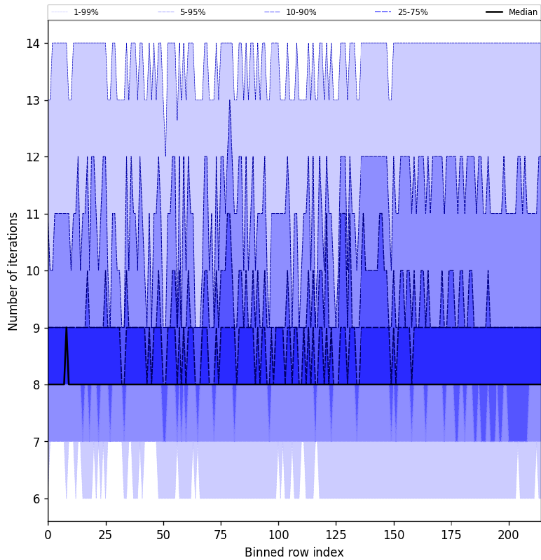
Figure 26: Along track statistics of “Number of iterations” for 2025-08-20 to 2025-08-21
