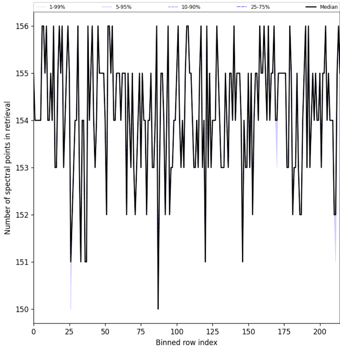
Figure 23: Along track statistics of “Number of spectral points in retrieval” for 2025-08-20 to 2025-08-21
