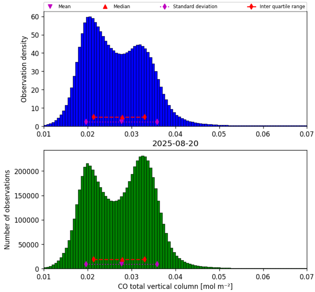
Figure 14: Histogram of “CO total vertical column” for 2025-08-20 to 2025-08-21
