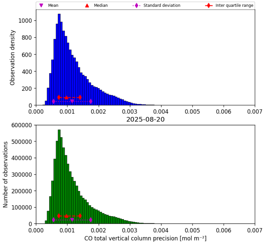
Figure 15: Histogram of “CO total vertical column precision” for 2025-08-20 to 2025-08-21
