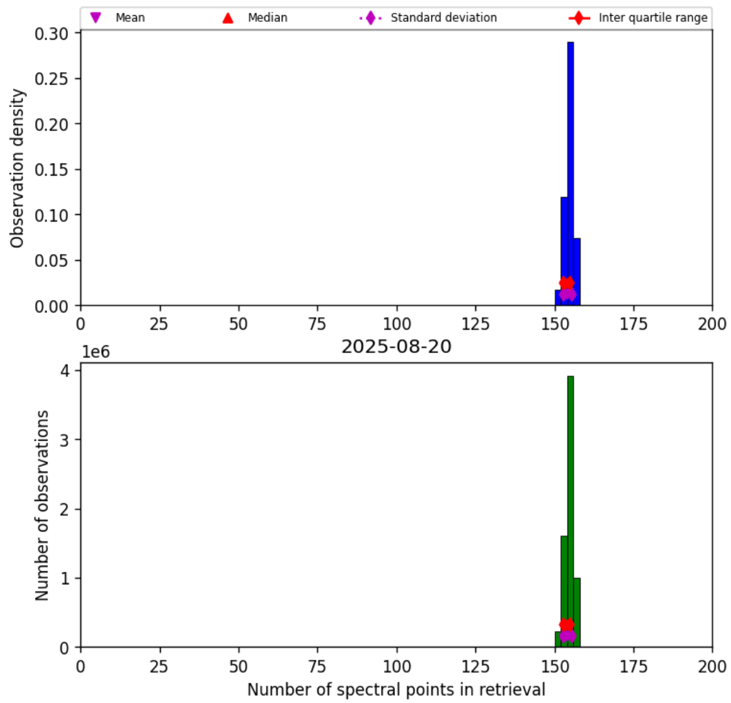
Figure 16: Histogram of “Number of spectral points in retrieval” for 2025-08-20 to 2025-08-21
