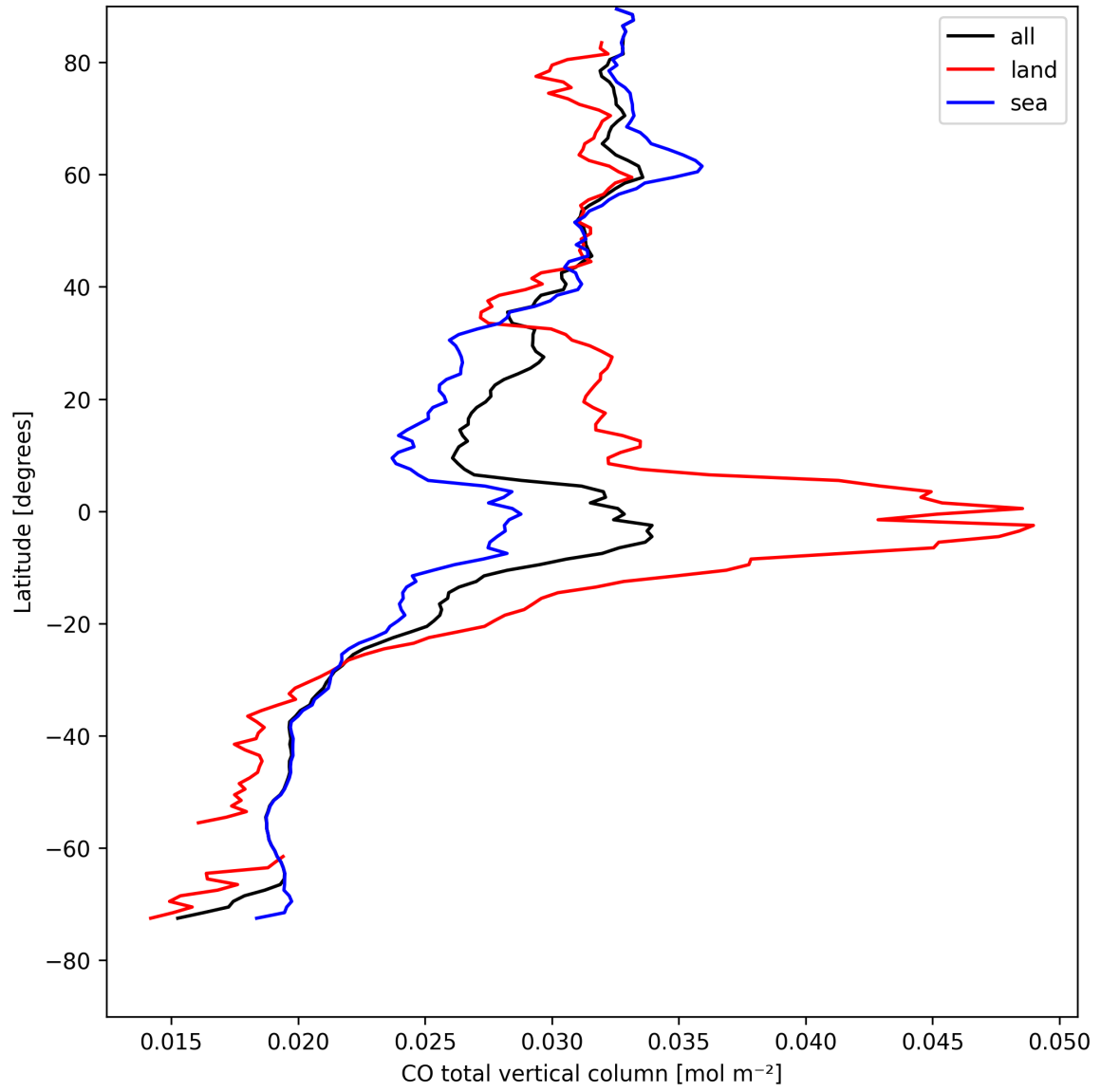
Figure 7: Zonal average of “CO total vertical column” for 2025-08-20 to 2025-08-21.
