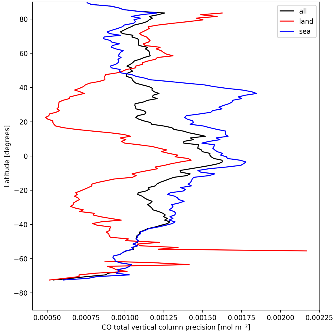
Figure 8: Zonal average of “CO total vertical column precision” for 2025-08-20 to 2025-08-21.
