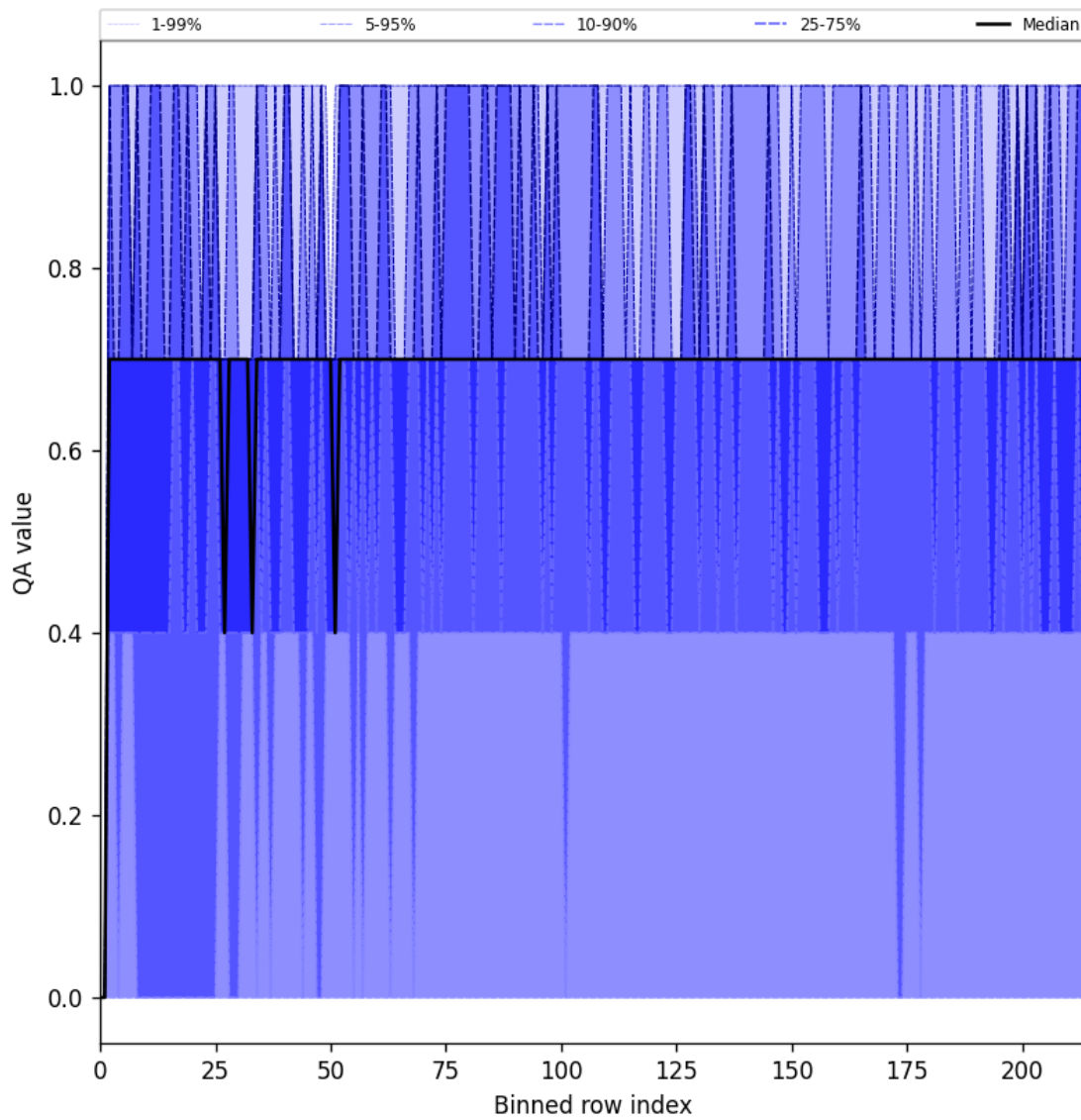
Figure 20: Along track statistics of “QA value” for 2025-08-20 to 2025-08-21
