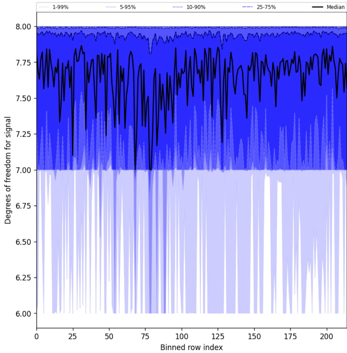
Figure 25: Along track statistics of “Degrees of freedom for signal” for 2025-08-20 to 2025-08-21
