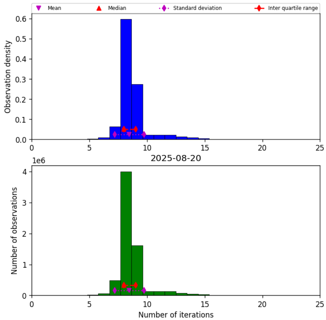
Figure 19: Histogram of “Number of iterations” for 2025-08-20 to 2025-08-21
