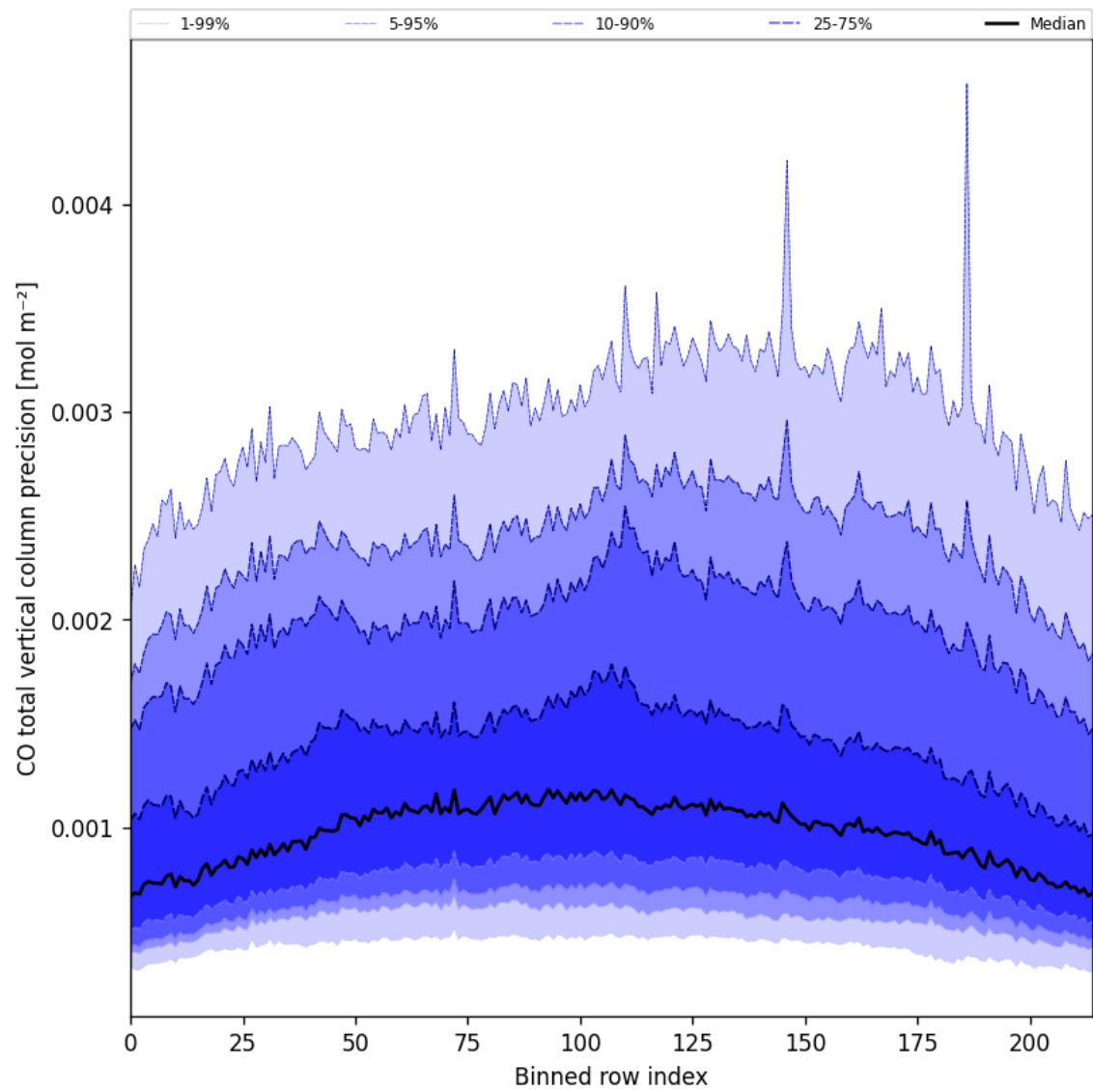
Figure 22: Along track statistics of “CO total vertical column precision” for 2025-08-20 to 2025-08-21
