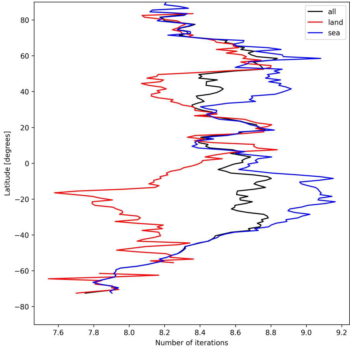
Figure 12: Zonal average of “Number of iterations” for 2025-08-20 to 2025-08-21.
