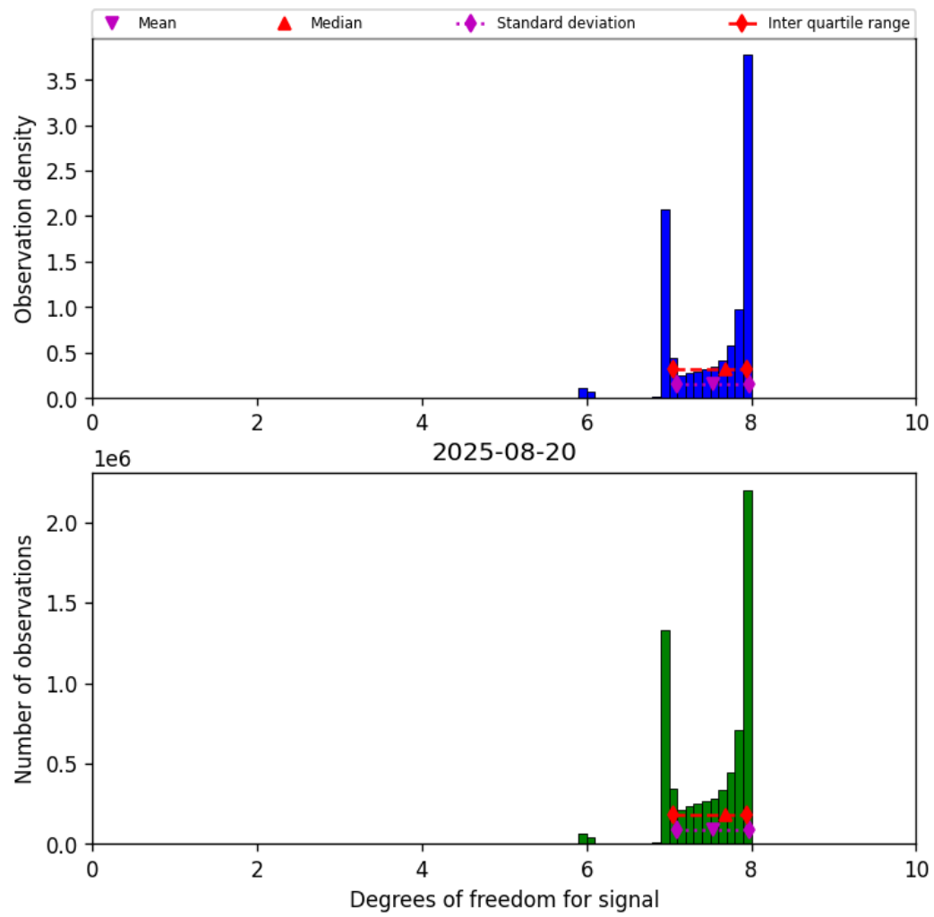
Figure 18: Histogram of “Degrees of freedom for signal” for 2025-08-20 to 2025-08-21
