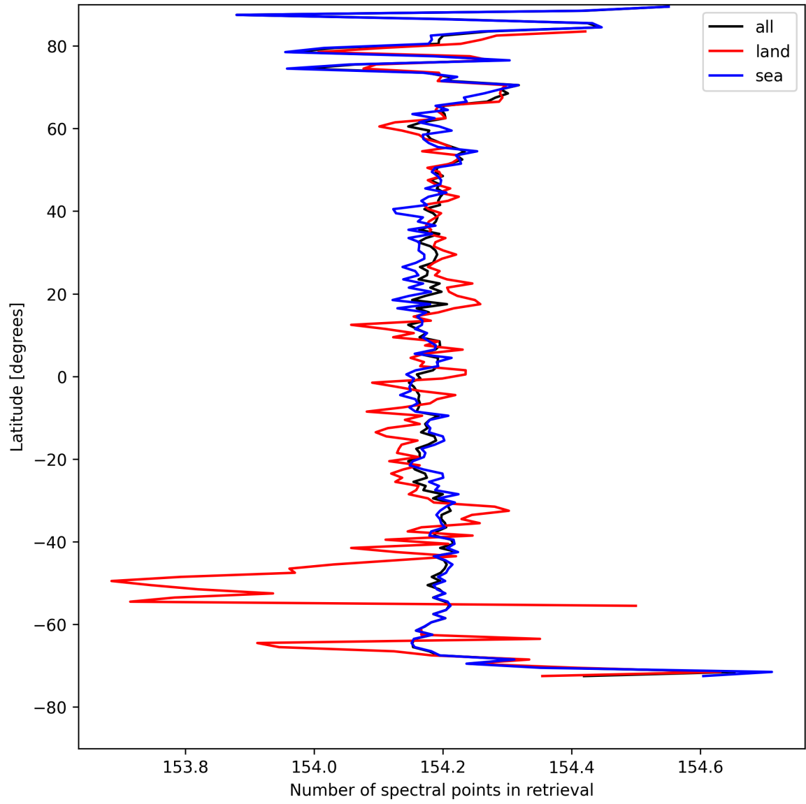
Figure 9: Zonal average of “Number of spectral points in retrieval” for 2025-08-20 to 2025-08-21.
