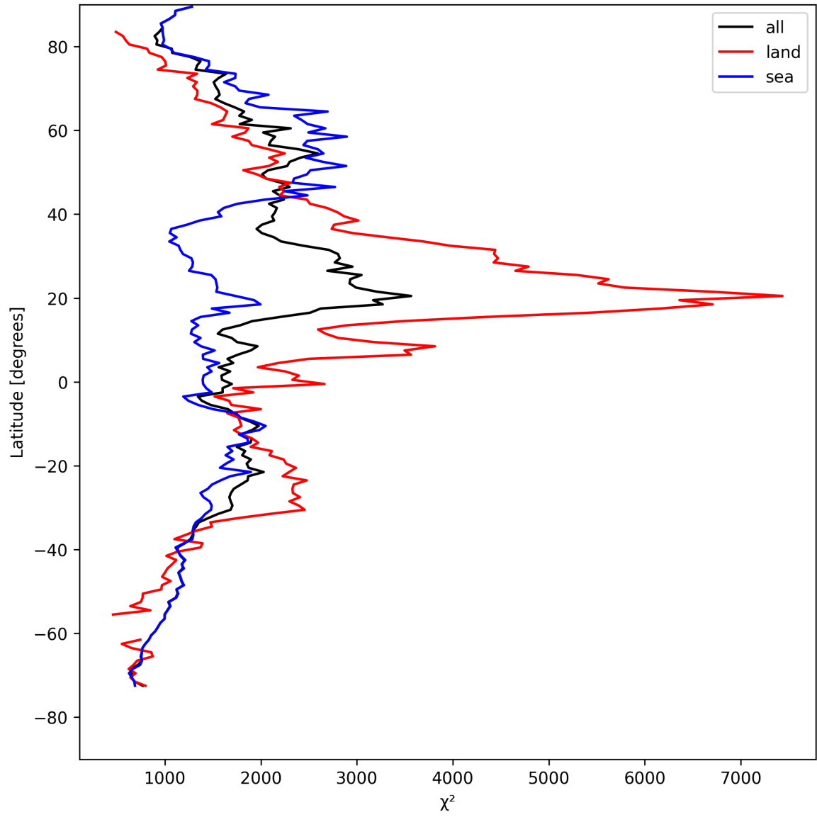
Figure 10: Zonal average of “ \chi^2 ” for 2025-08-20 to 2025-08-21.
