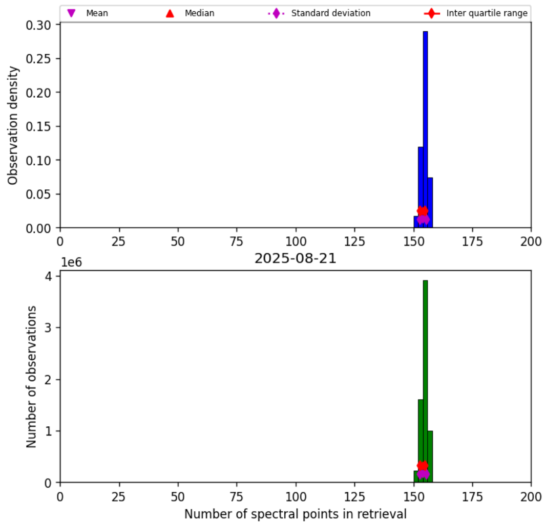
Figure 16: Histogram of “Number of spectral points in retrieval” for 2025-08-21 to 2025-08-22
