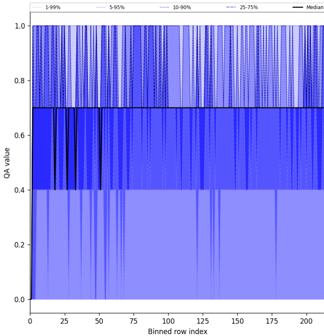
Figure 20: Along track statistics of “QA value” for 2025-08-21 to 2025-08-22
