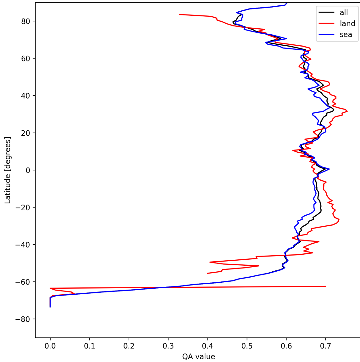
Figure 6: Zonal average of “QA value” for 2025-08-21 to 2025-08-22.
