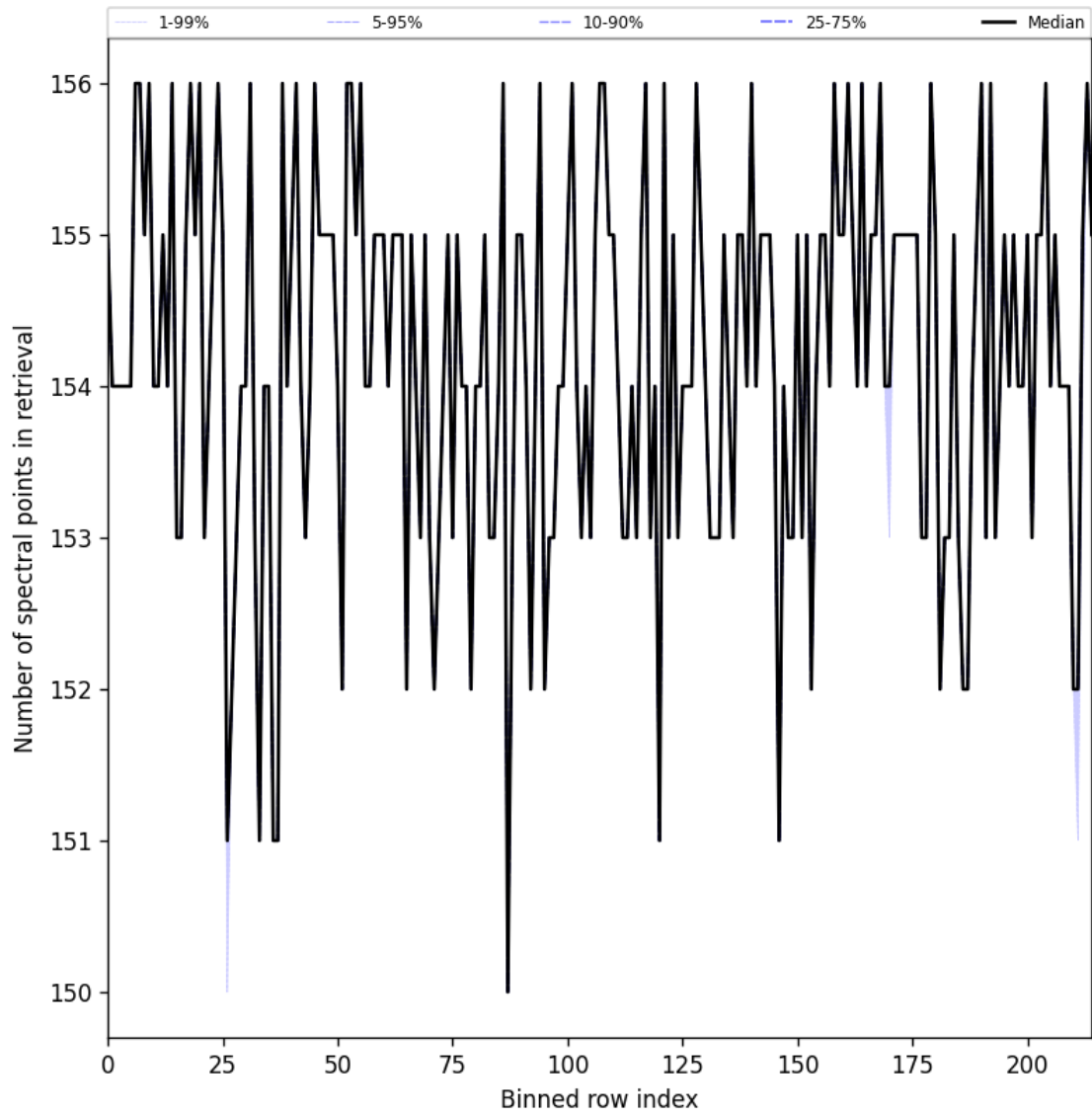
Figure 23: Along track statistics of “Number of spectral points in retrieval” for 2025-08-21 to 2025-08-22
