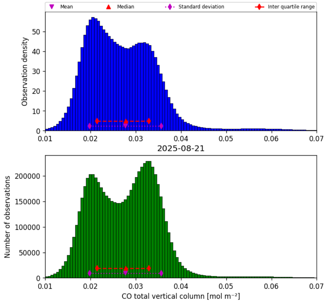
Figure 14: Histogram of “CO total vertical column” for 2025-08-21 to 2025-08-22
