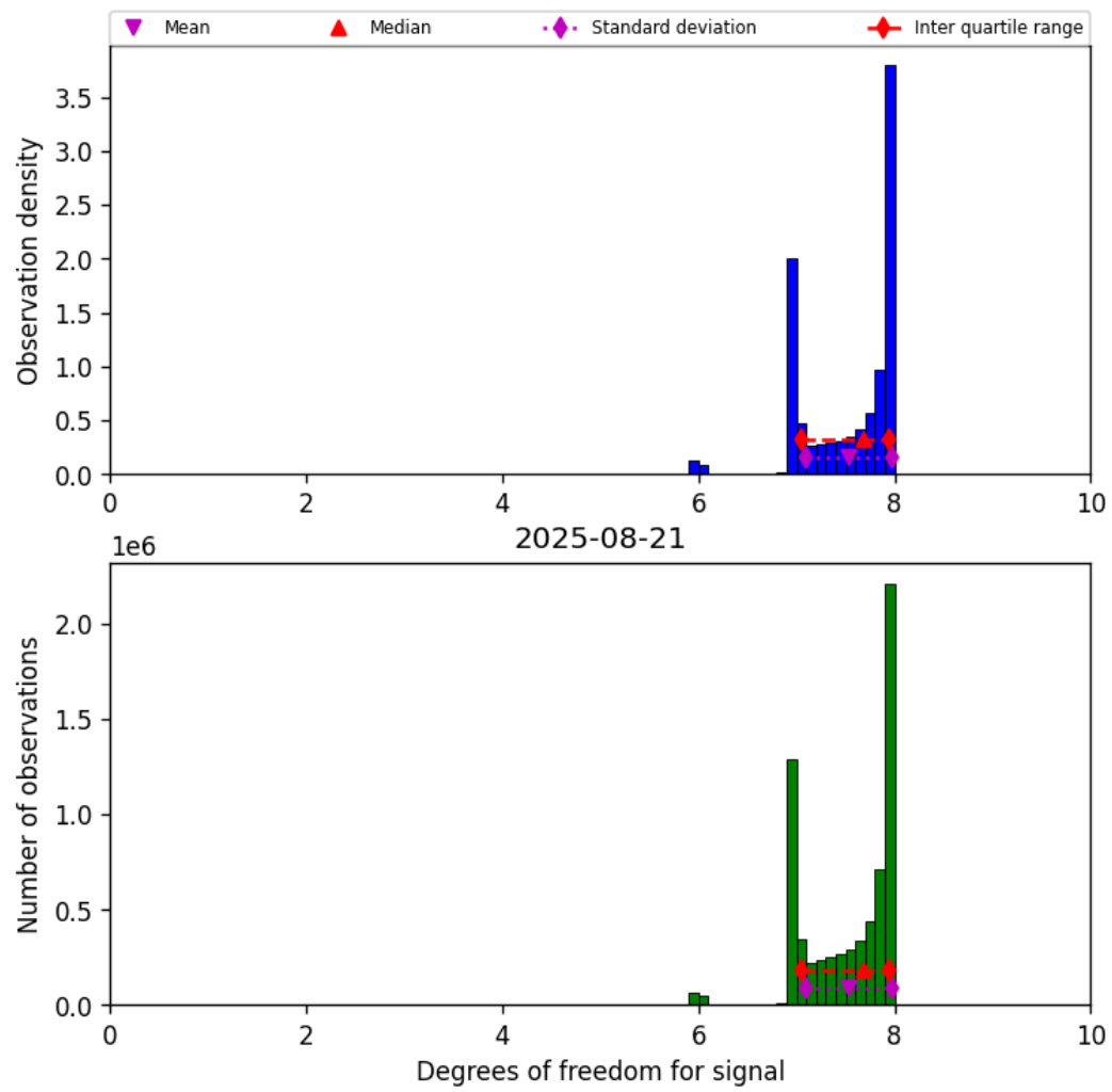
Figure 18: Histogram of “Degrees of freedom for signal” for 2025-08-21 to 2025-08-22
