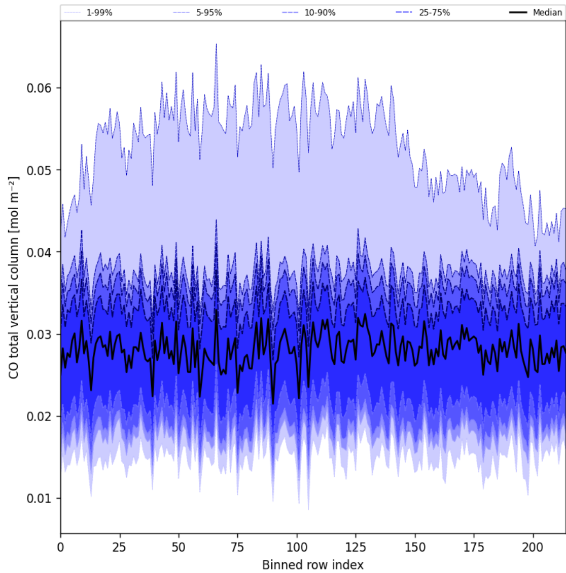
Figure 21: Along track statistics of “CO total vertical column” for 2025-08-21 to 2025-08-22
