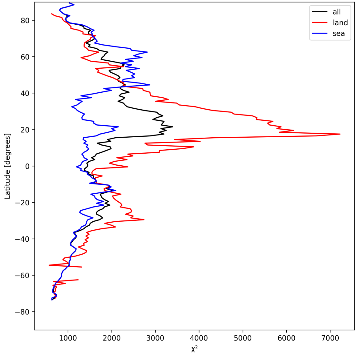
Figure 10: Zonal average of “ \chi^2 ” for 2025-08-21 to 2025-08-22.
