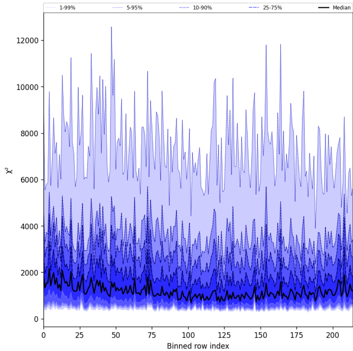
Figure 24: Along track statistics of “ \chi^2 ” for 2025-08-21 to 2025-08-22
