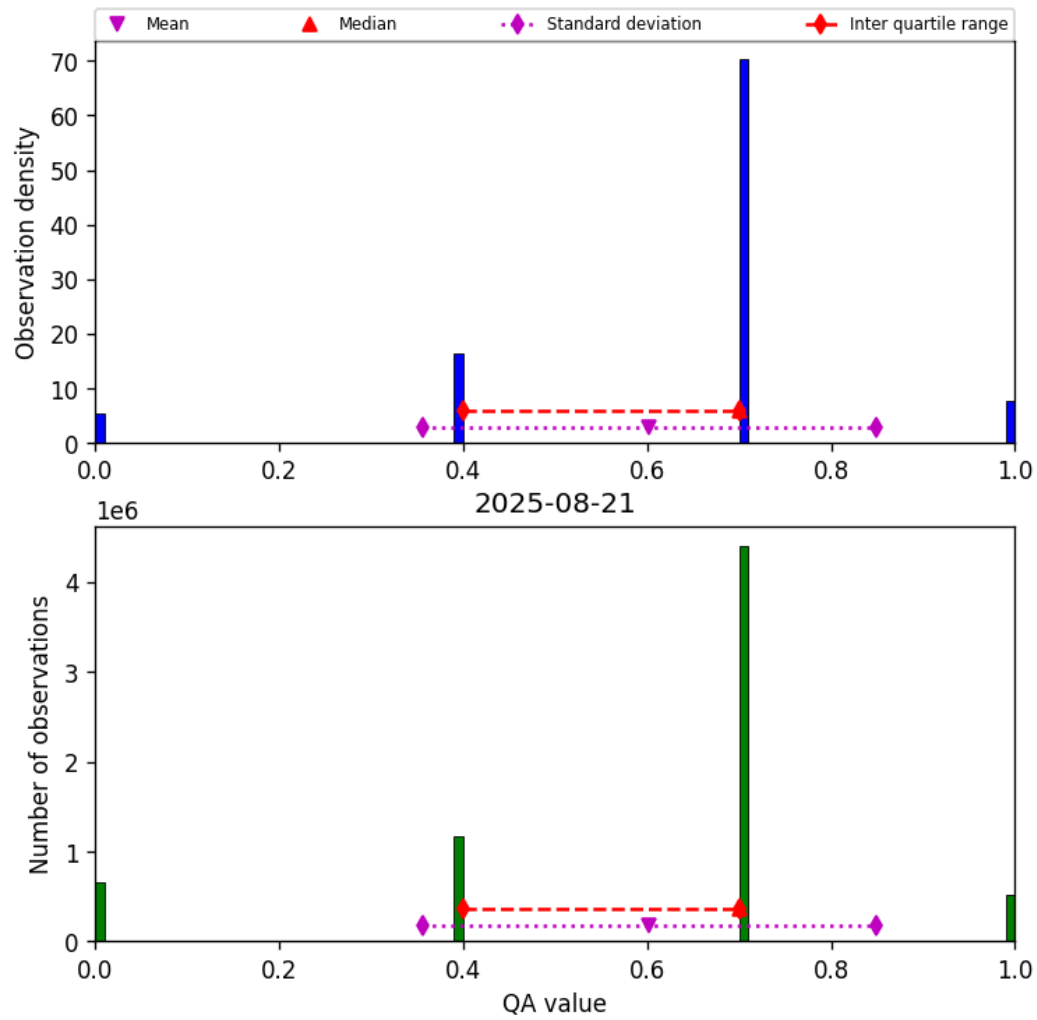
Figure 13: Histogram of “QA value” for 2025-08-21 to 2025-08-22
