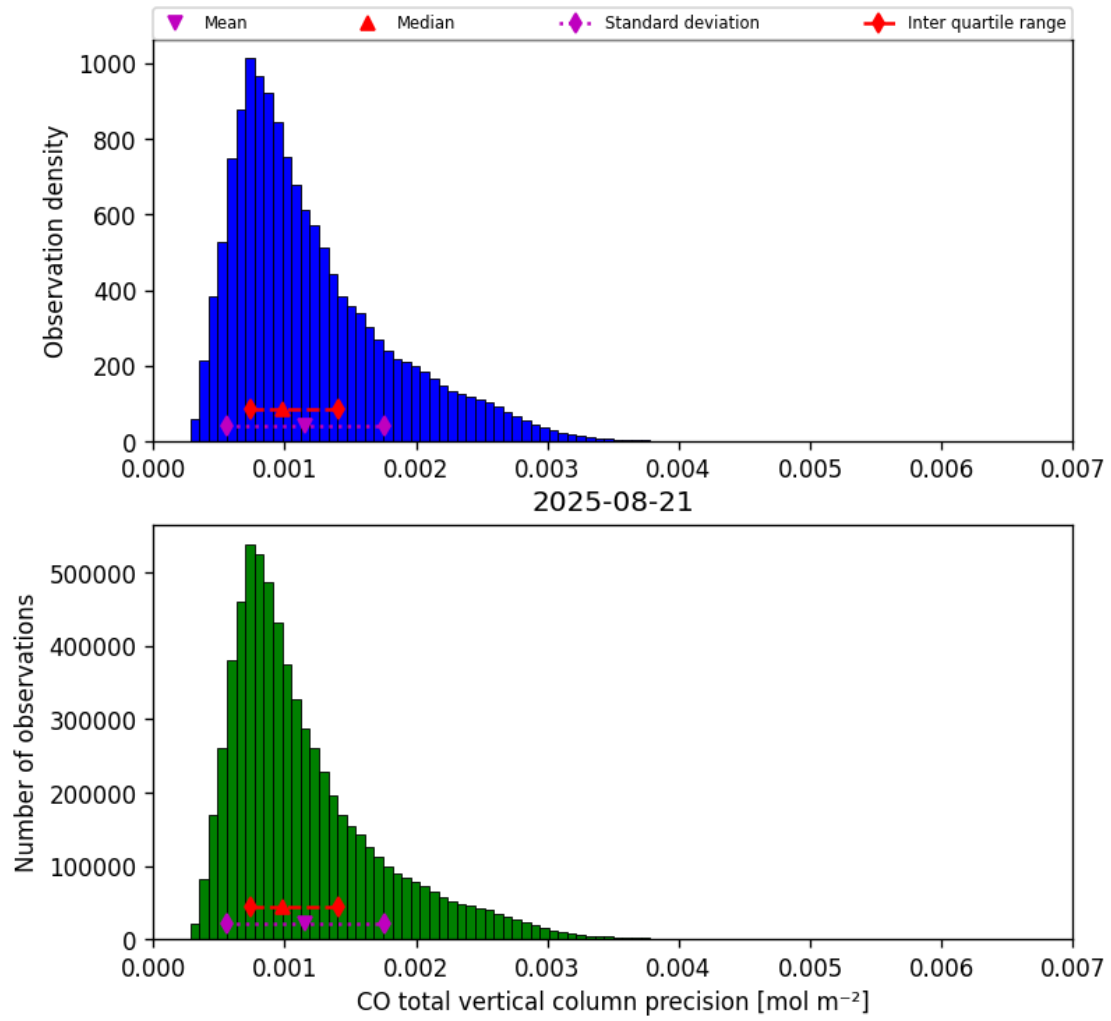
Figure 15: Histogram of “CO total vertical column precision” for 2025-08-21 to 2025-08-22
