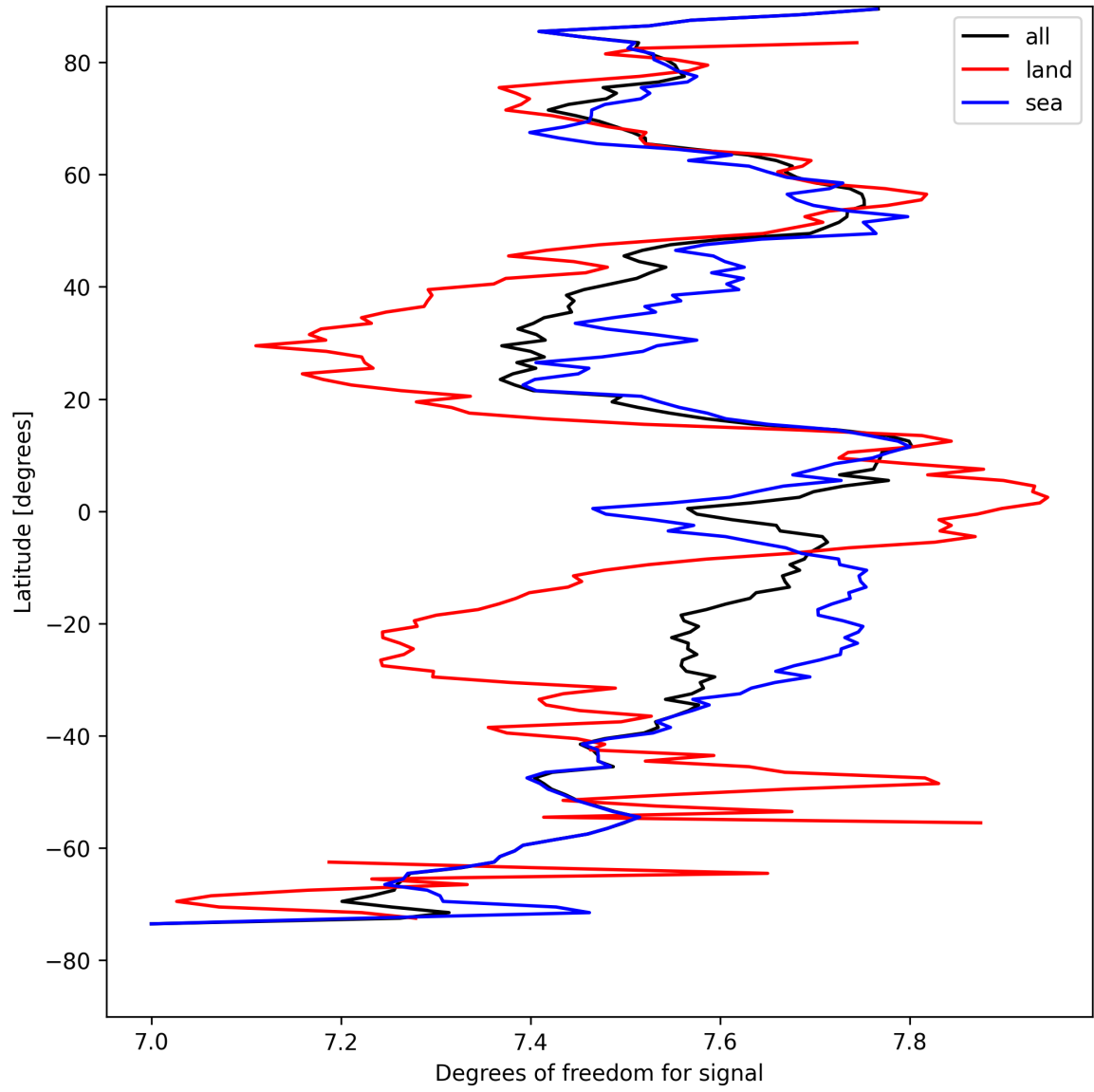
Figure 11: Zonal average of “Degrees of freedom for signal” for 2025-08-21 to 2025-08-22.
