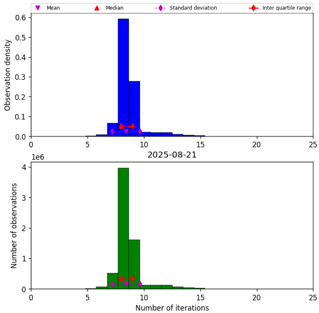
Figure 19: Histogram of “Number of iterations” for 2025-08-21 to 2025-08-22
