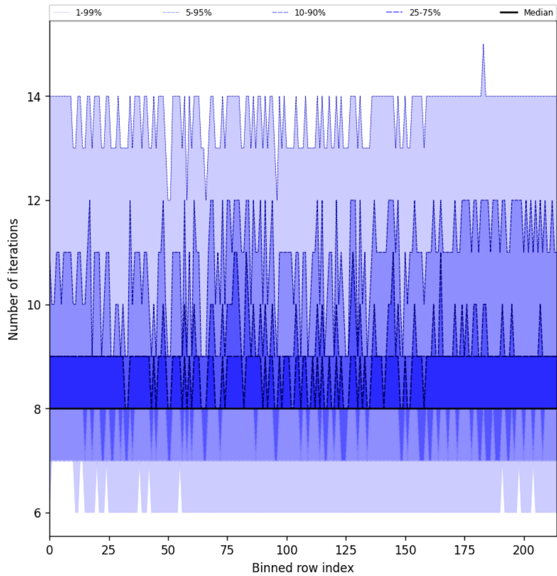
Figure 26: Along track statistics of “Number of iterations” for 2025-08-21 to 2025-08-22
