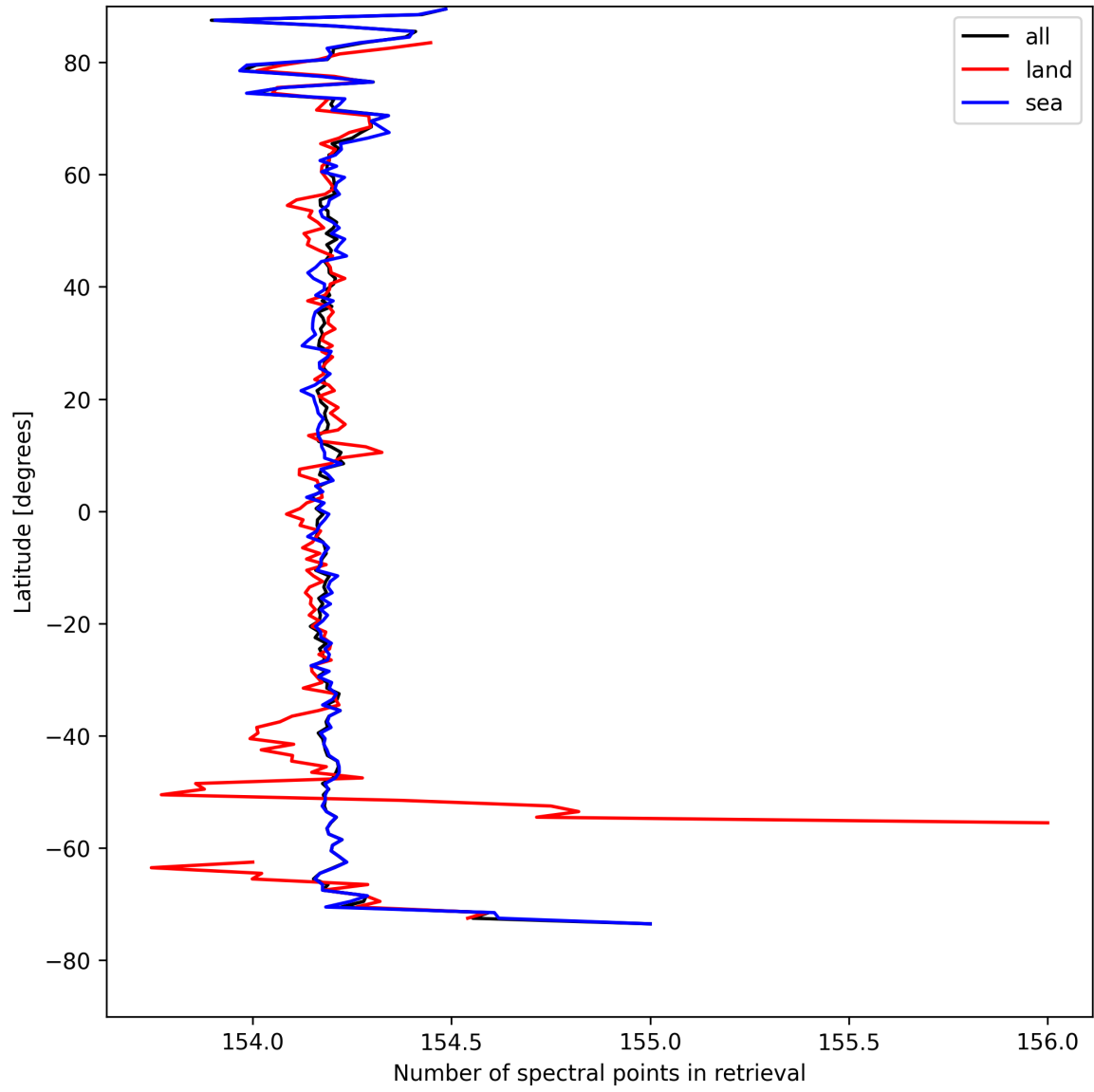
Figure 9: Zonal average of “Number of spectral points in retrieval” for 2025-08-21 to 2025-08-22.
