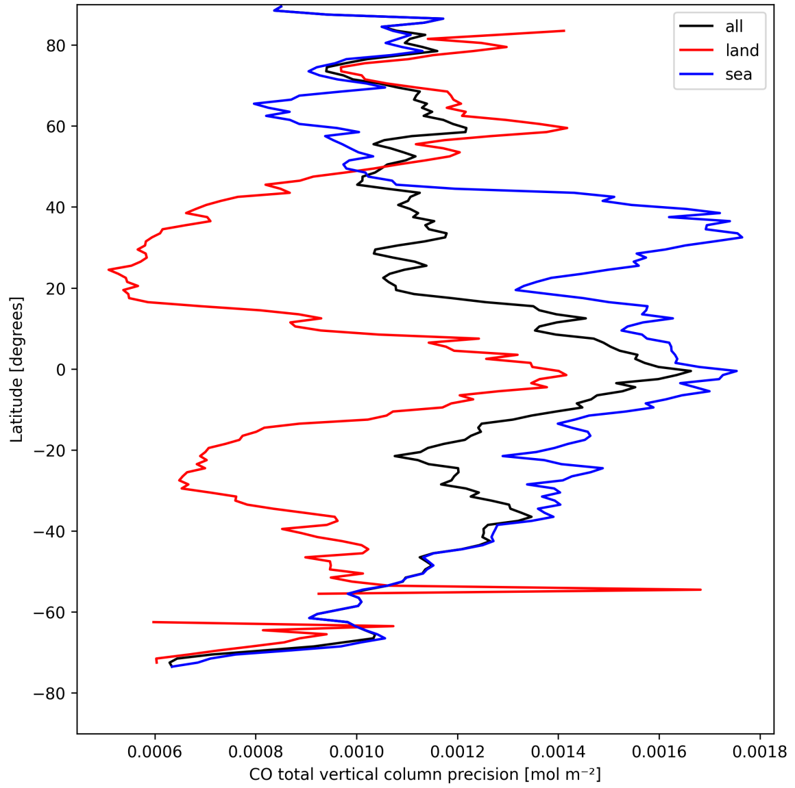
Figure 8: Zonal average of “CO total vertical column precision” for 2025-08-21 to 2025-08-22.
