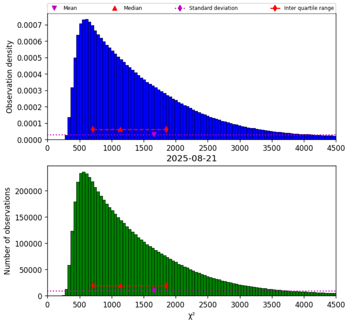
Figure 17: Histogram of “ \chi^2 ” for 2025-08-21 to 2025-08-22
