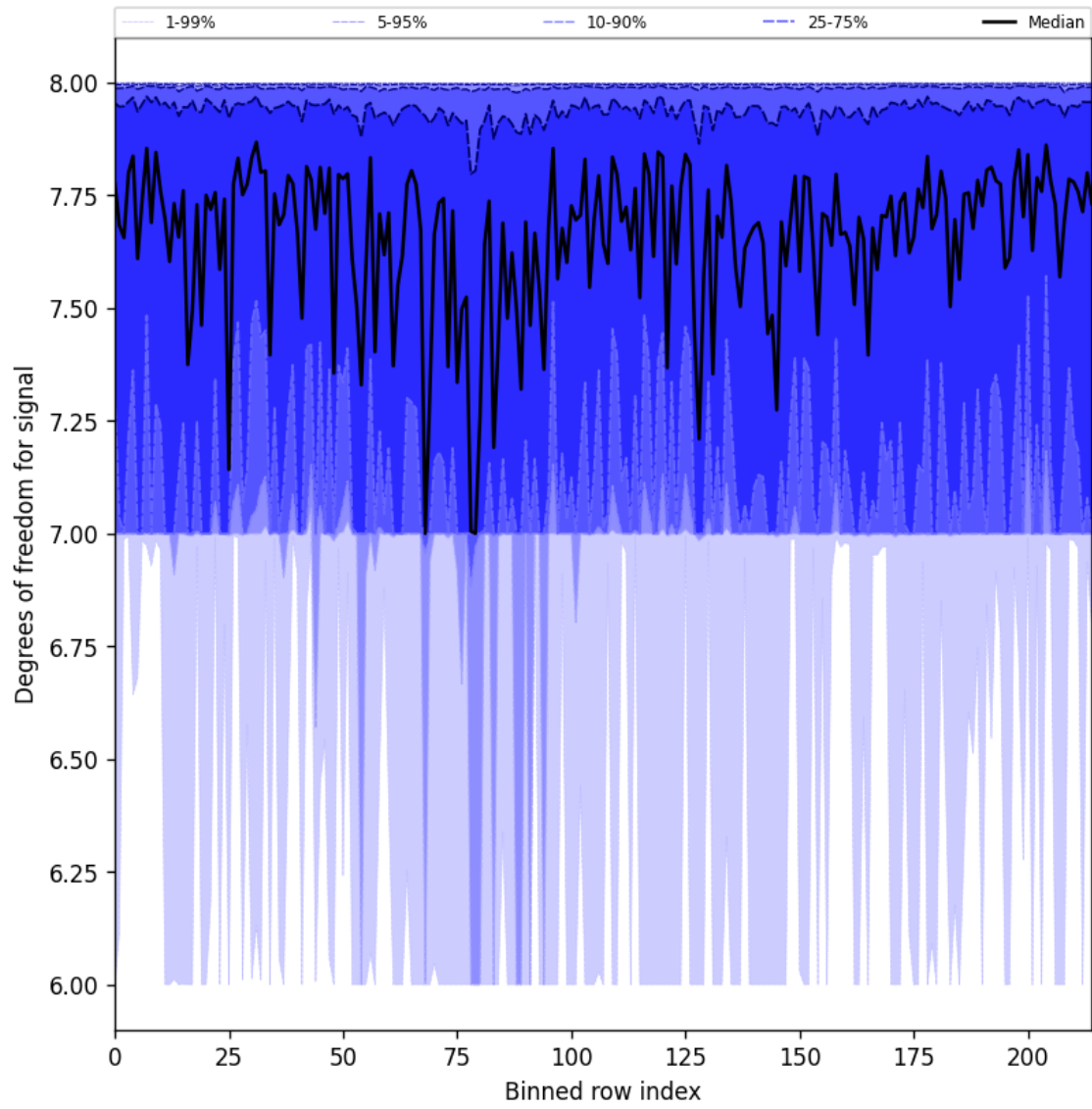
Figure 25: Along track statistics of “Degrees of freedom for signal” for 2025-08-21 to 2025-08-22
