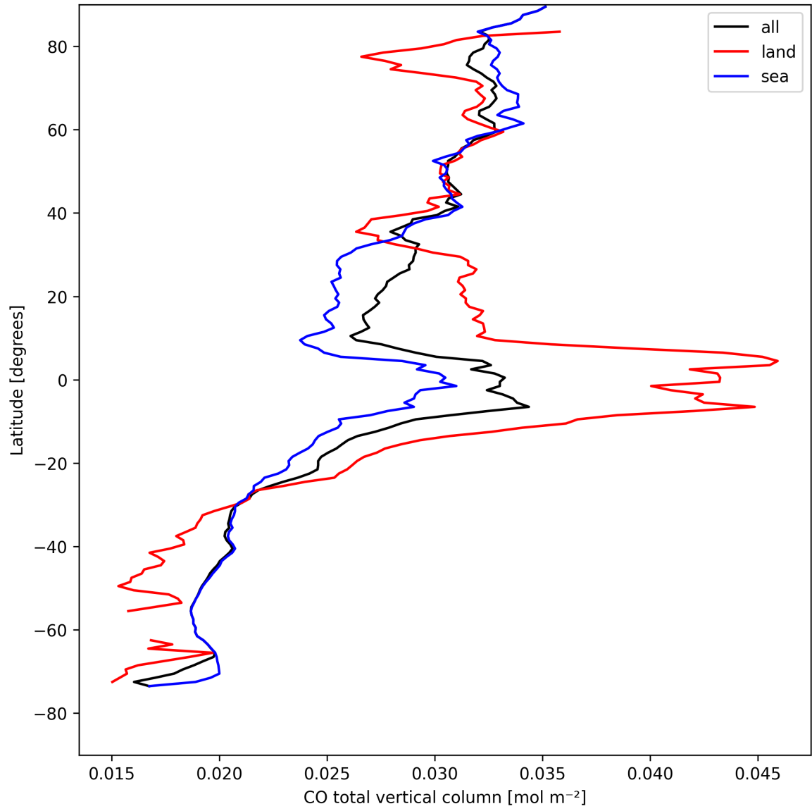
Figure 7: Zonal average of “CO total vertical column” for 2025-08-21 to 2025-08-22.
