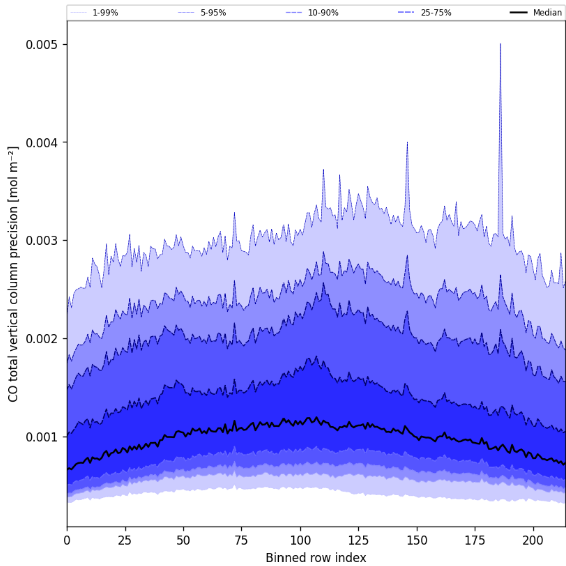
Figure 22: Along track statistics of “CO total vertical column precision” for 2025-08-21 to 2025-08-22
