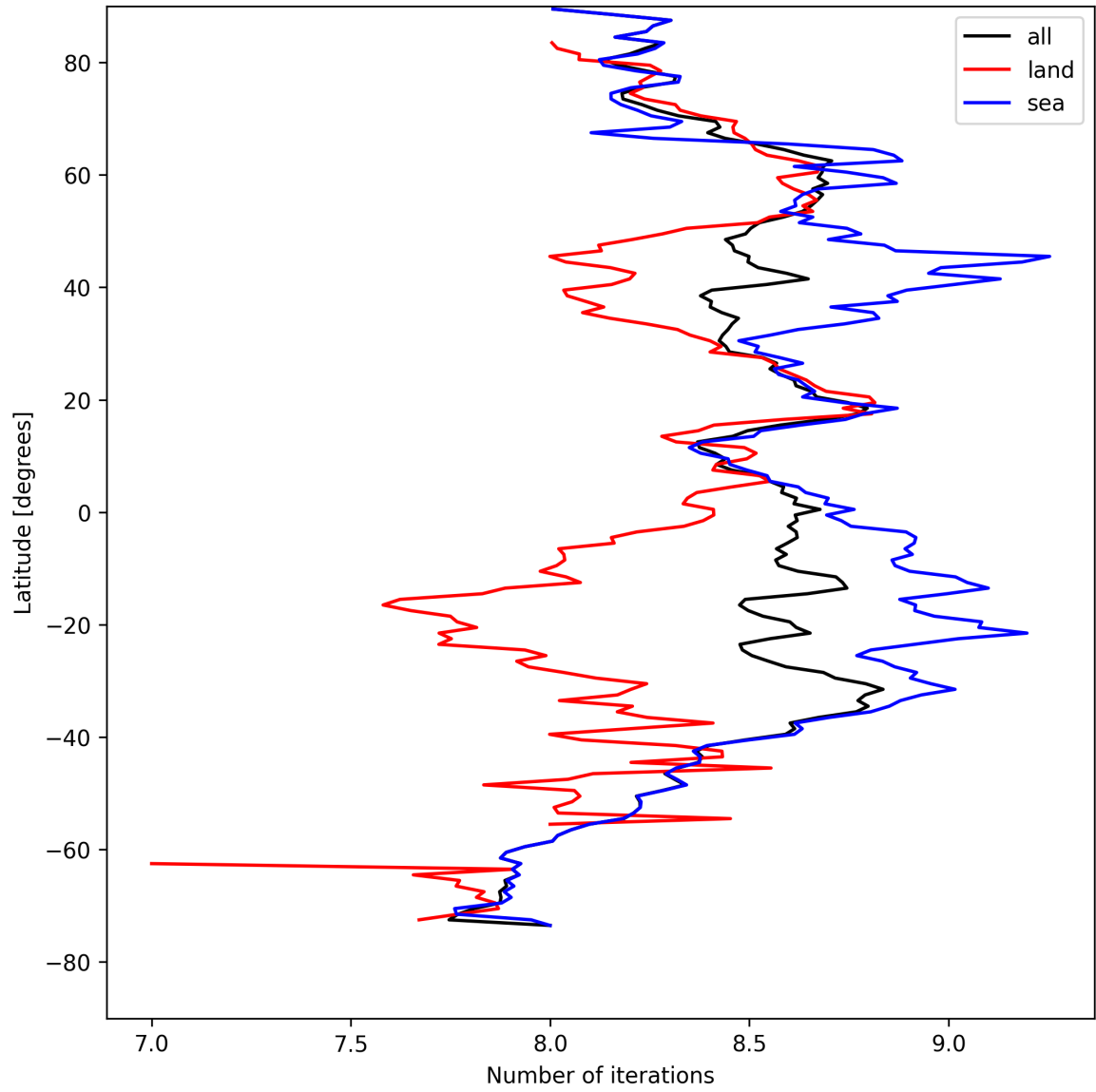
Figure 12: Zonal average of “Number of iterations” for 2025-08-21 to 2025-08-22.
