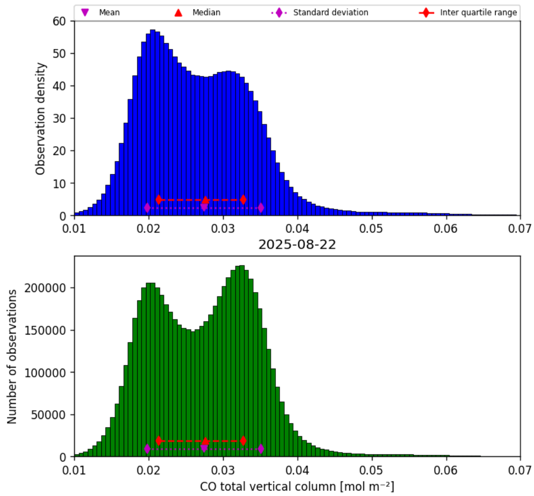
Figure 14: Histogram of “CO total vertical column” for 2025-08-22 to 2025-08-23
