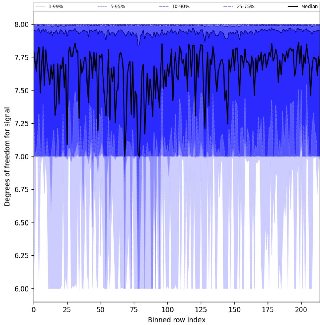
Figure 25: Along track statistics of “Degrees of freedom for signal” for 2025-08-22 to 2025-08-23
