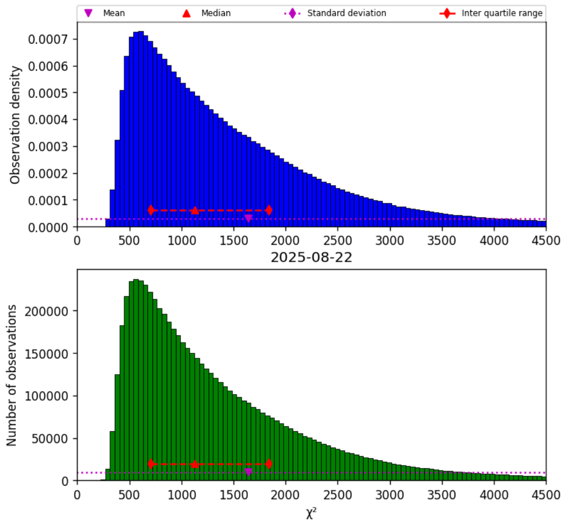
Figure 17: Histogram of “ \chi^2 ” for 2025-08-22 to 2025-08-23
