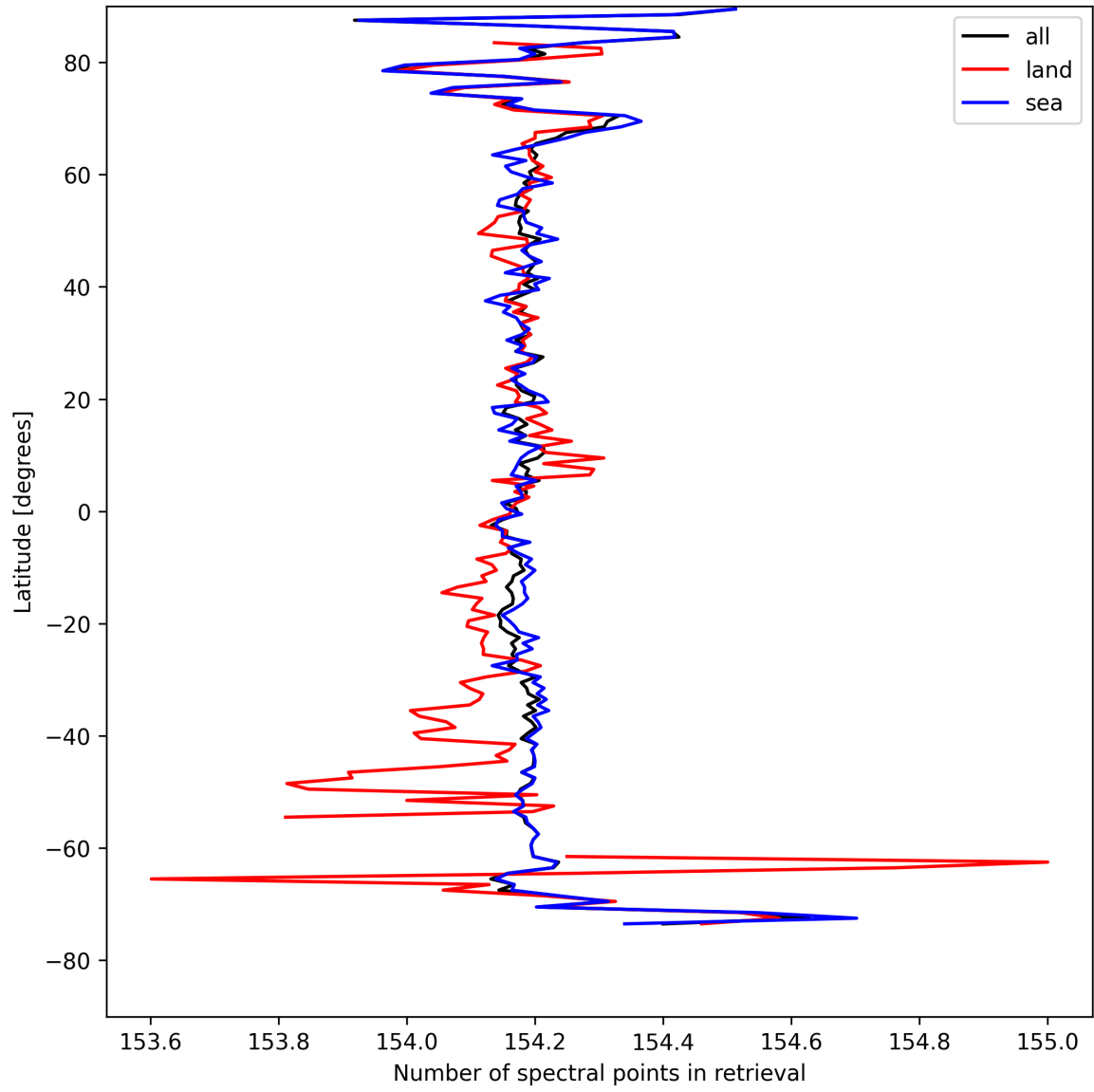
Figure 9: Zonal average of “Number of spectral points in retrieval” for 2025-08-22 to 2025-08-23.
