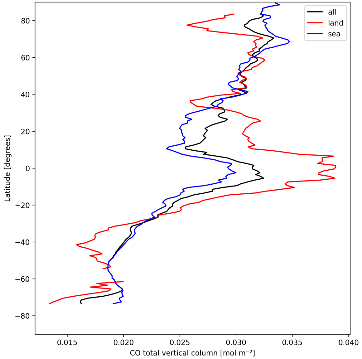
Figure 7: Zonal average of “CO total vertical column” for 2025-08-22 to 2025-08-23.
