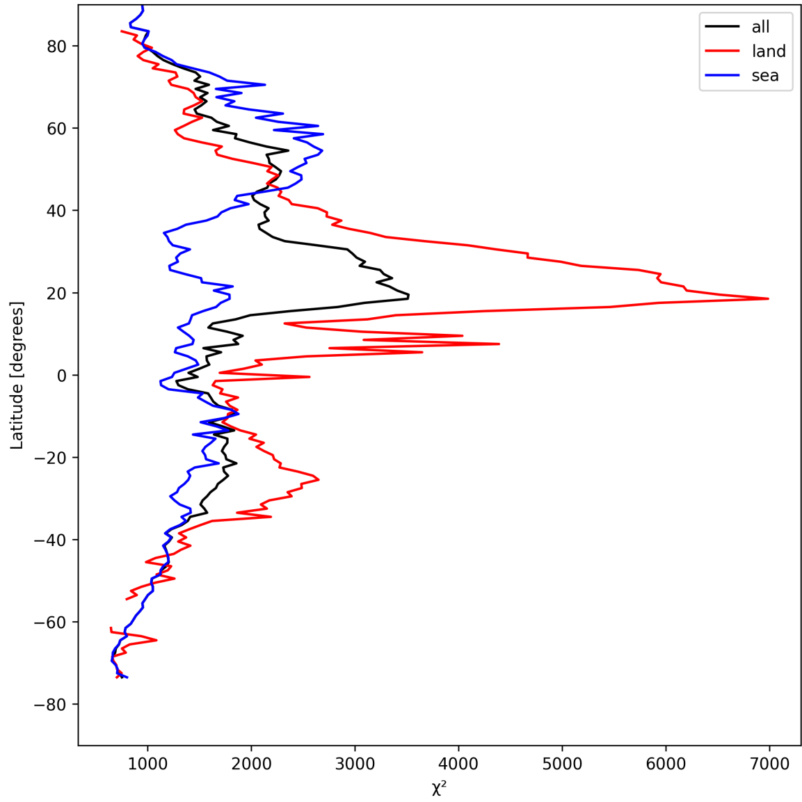
Figure 10: Zonal average of “ \chi^2 ” for 2025-08-22 to 2025-08-23.
