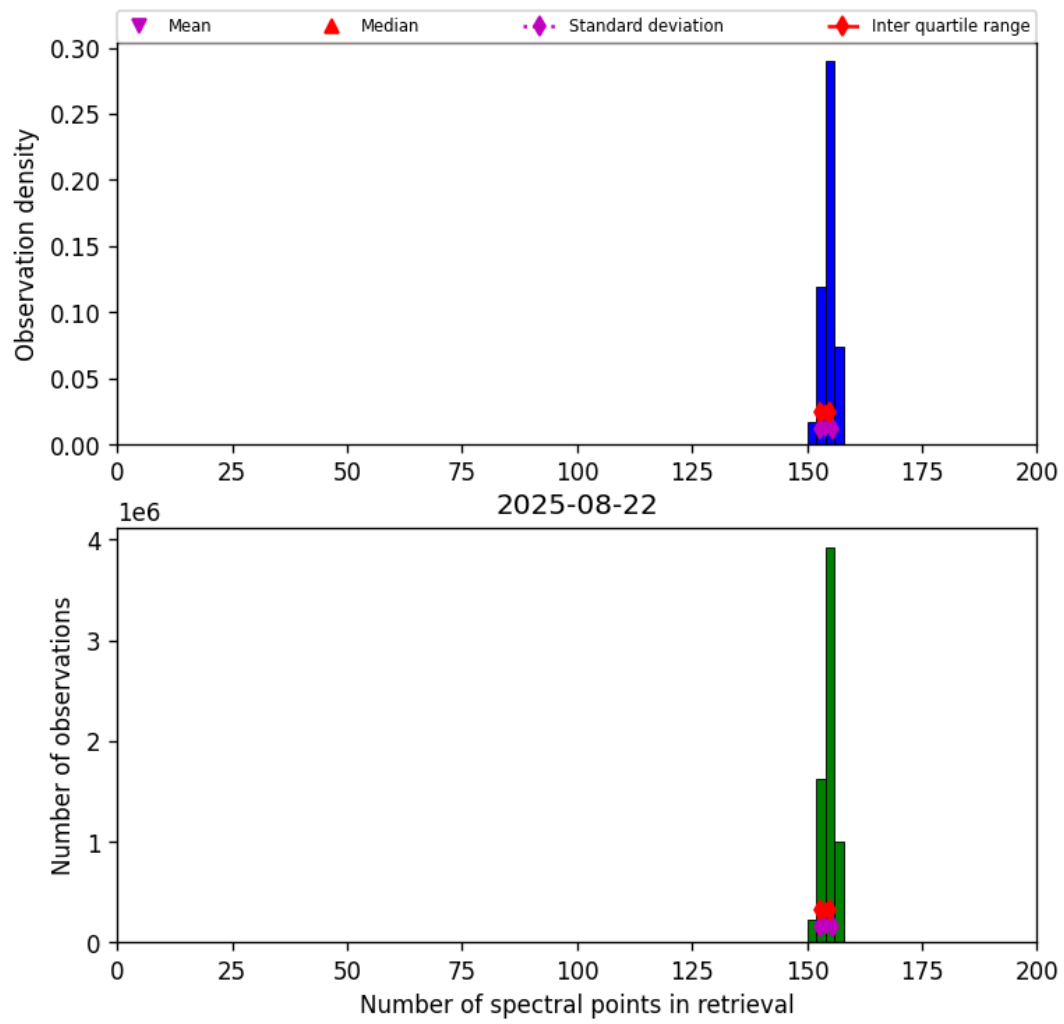
Figure 16: Histogram of “Number of spectral points in retrieval” for 2025-08-22 to 2025-08-23
