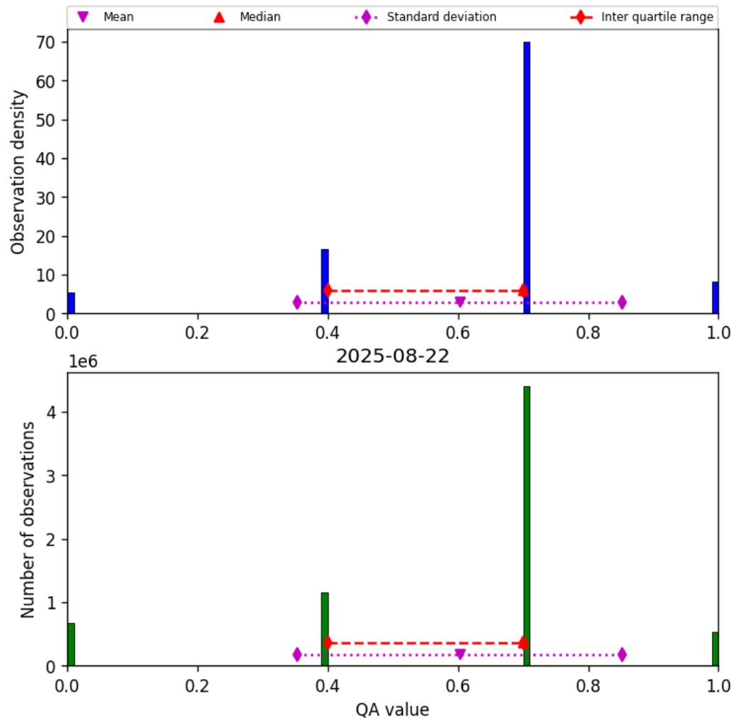
Figure 13: Histogram of “QA value” for 2025-08-22 to 2025-08-23
