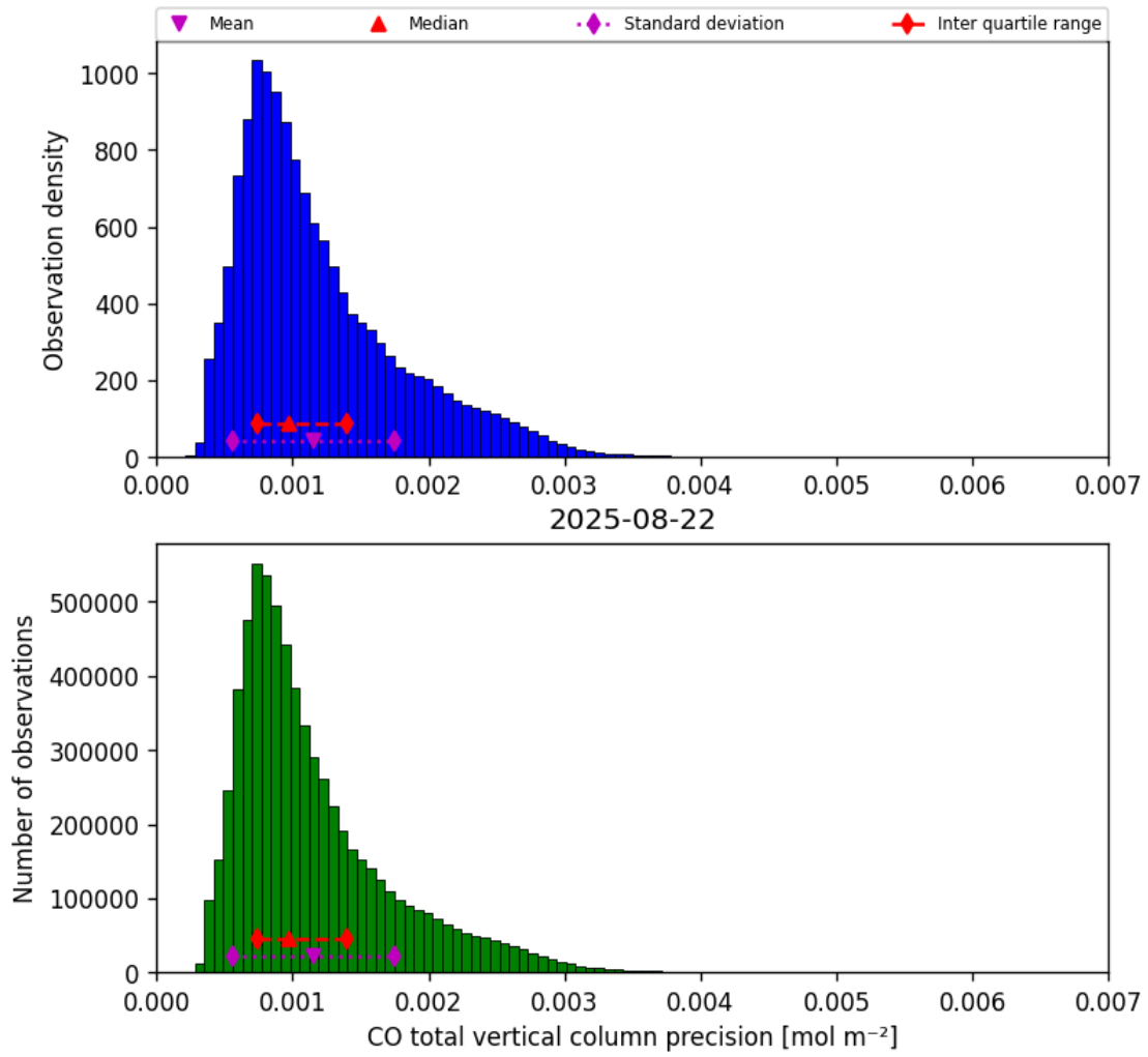
Figure 15: Histogram of “CO total vertical column precision” for 2025-08-22 to 2025-08-23
