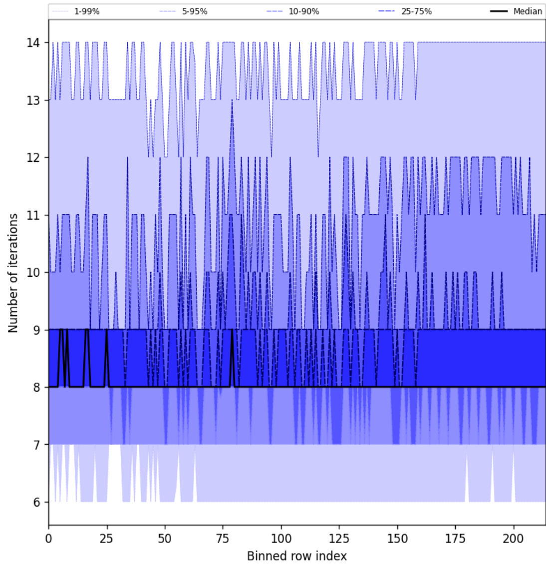
Figure 26: Along track statistics of “Number of iterations” for 2025-08-22 to 2025-08-23
