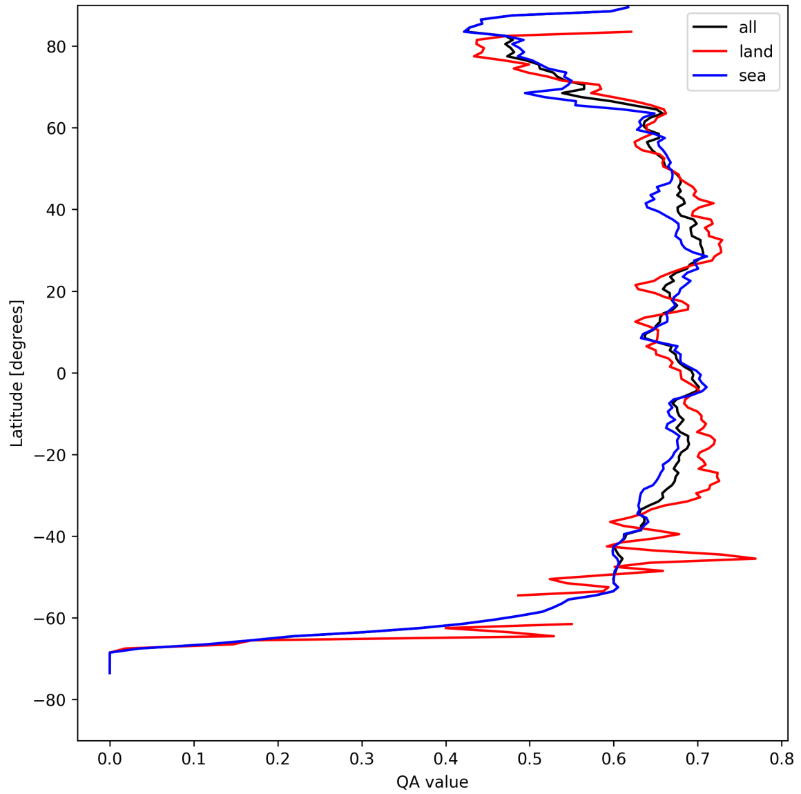
Figure 6: Zonal average of “QA value” for 2025-08-22 to 2025-08-23.
