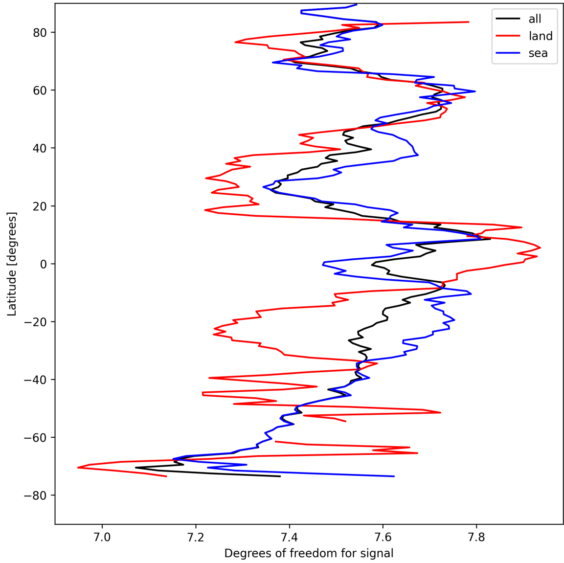
Figure 11: Zonal average of “Degrees of freedom for signal” for 2025-08-22 to 2025-08-23.
