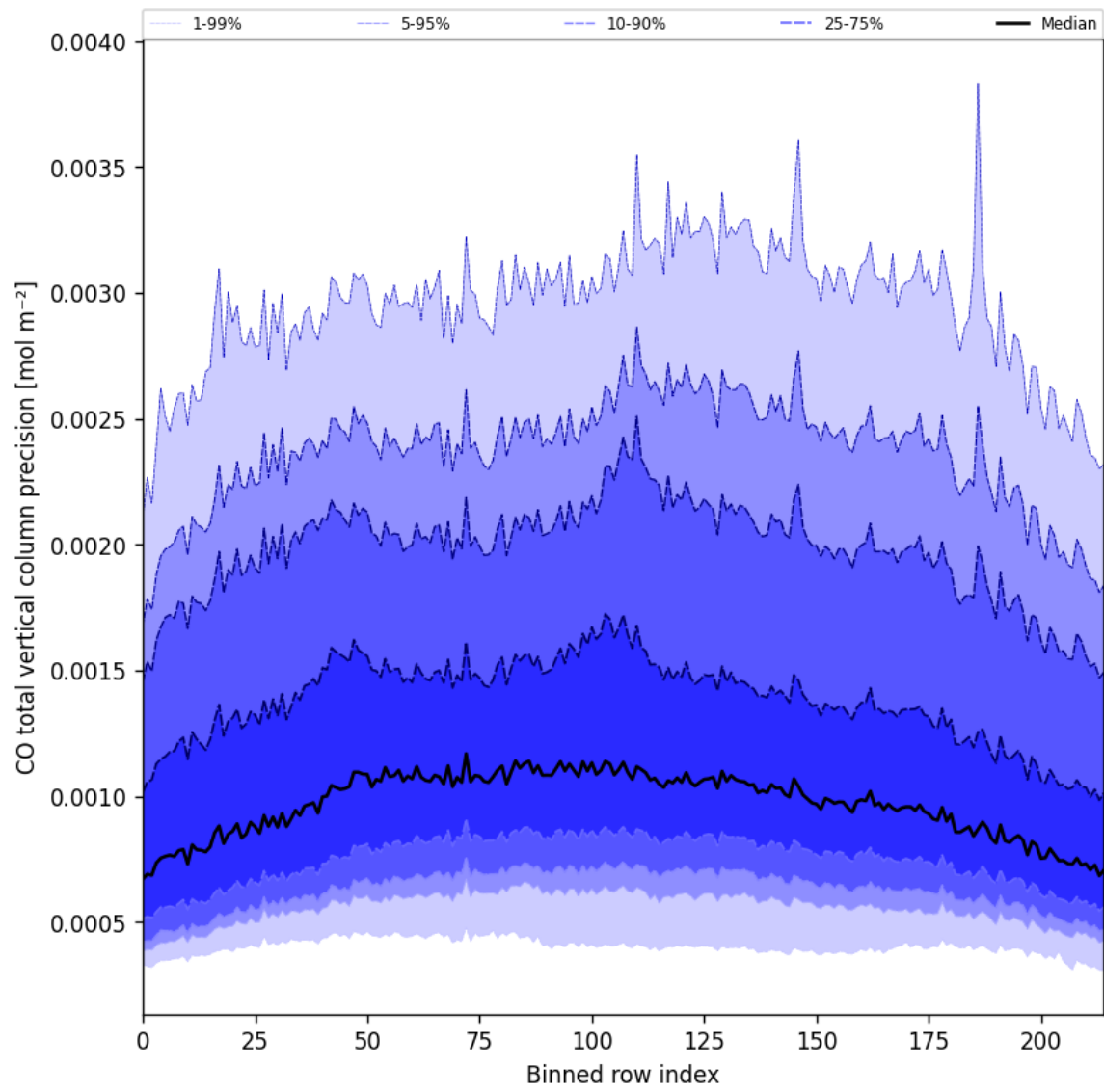
Figure 22: Along track statistics of “CO total vertical column precision” for 2025-08-22 to 2025-08-23
