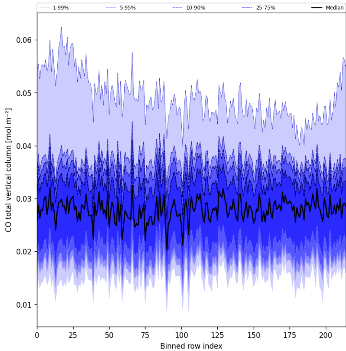
Figure 21: Along track statistics of “CO total vertical column” for 2025-08-22 to 2025-08-23
