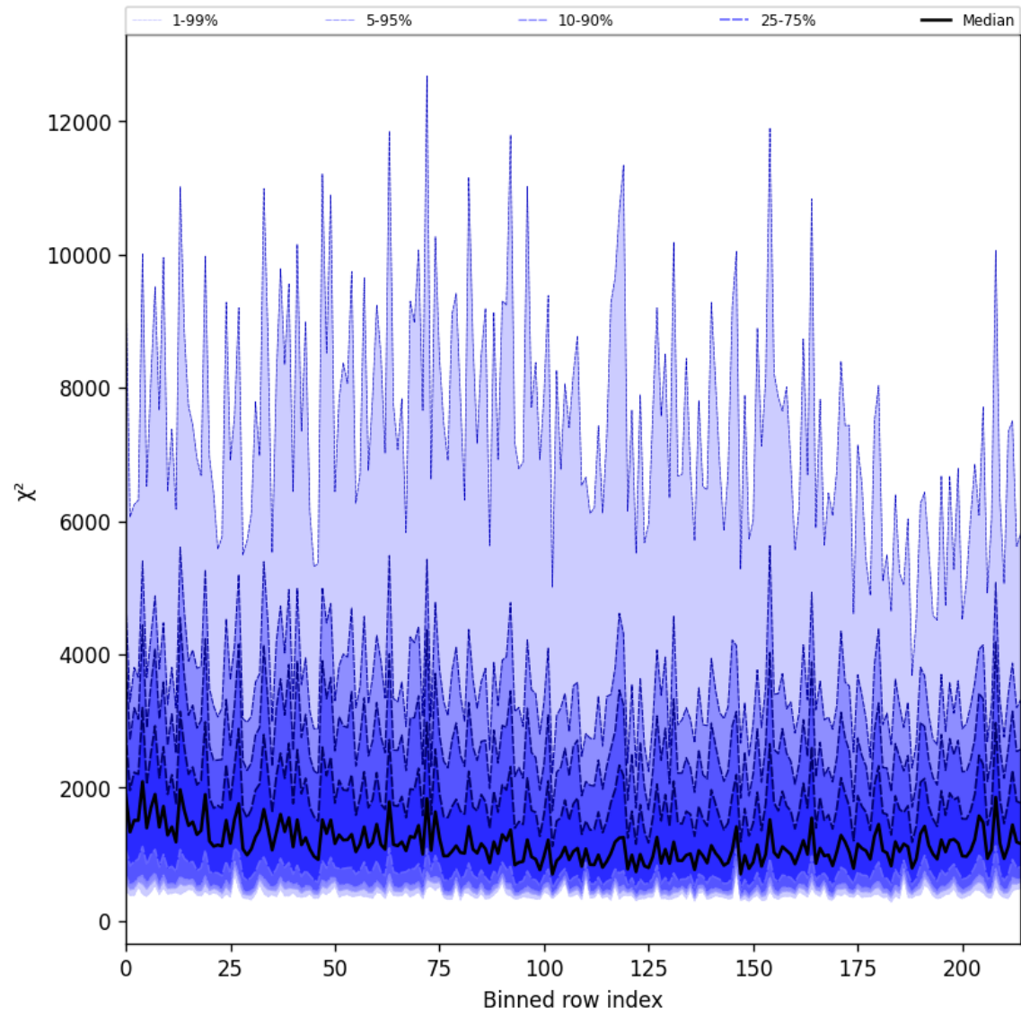
Figure 24: Along track statistics of “ \chi^2 ” for 2025-08-22 to 2025-08-23
