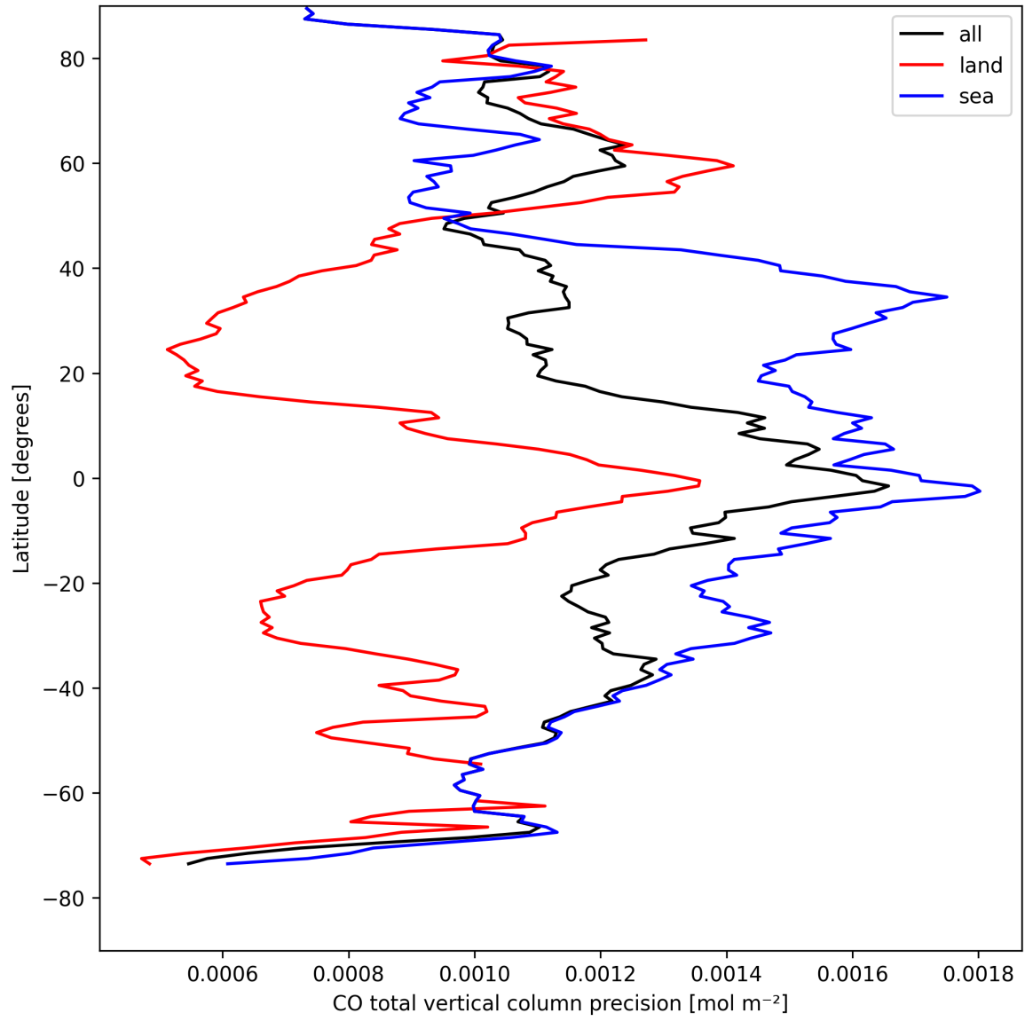
Figure 8: Zonal average of "CO total vertical column precision" for 2025-08-22 to 2025-08-23.
