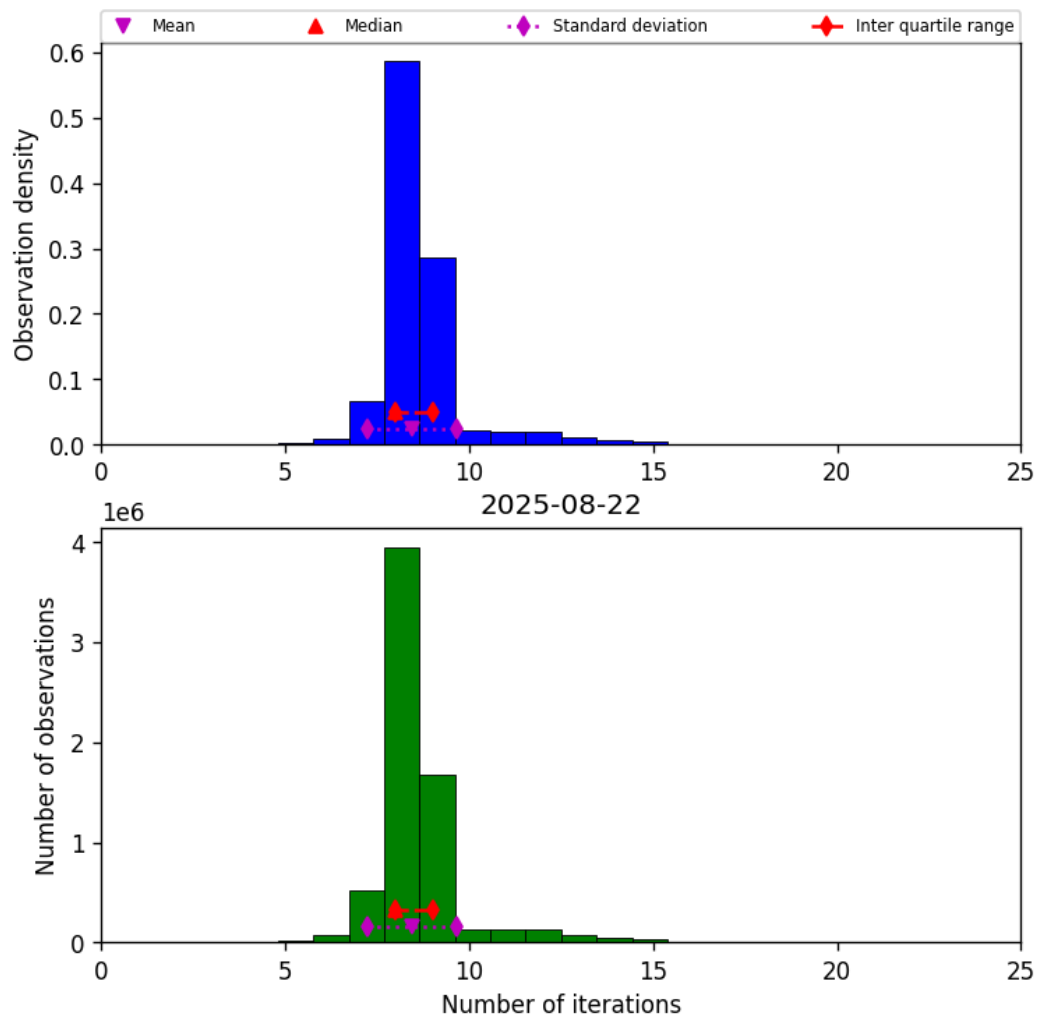
Figure 19: Histogram of “Number of iterations” for 2025-08-22 to 2025-08-23
