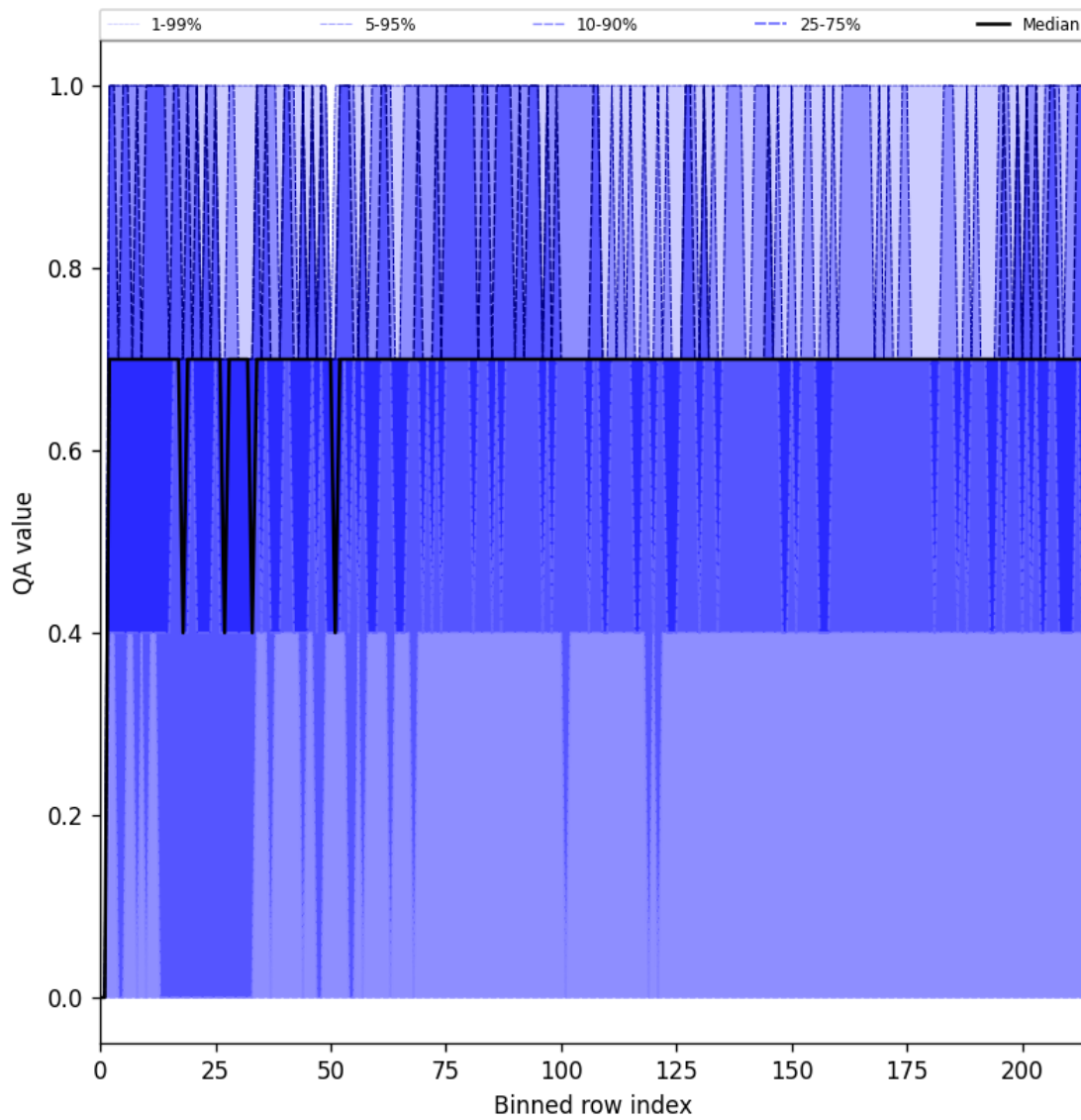
Figure 20: Along track statistics of “QA value” for 2025-08-22 to 2025-08-23
