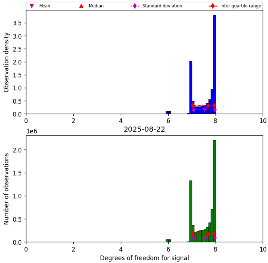
Figure 18: Histogram of “Degrees of freedom for signal” for 2025-08-22 to 2025-08-23
