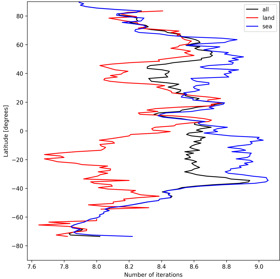
Figure 12: Zonal average of “Number of iterations” for 2025-08-22 to 2025-08-23.
