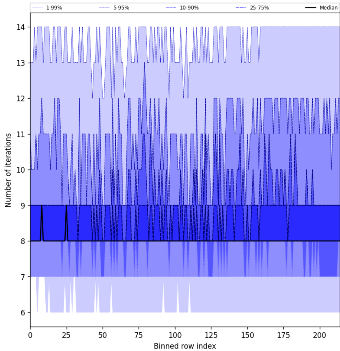
Figure 26: Along track statistics of “Number of iterations” for 2025-08-23 to 2025-08-23
