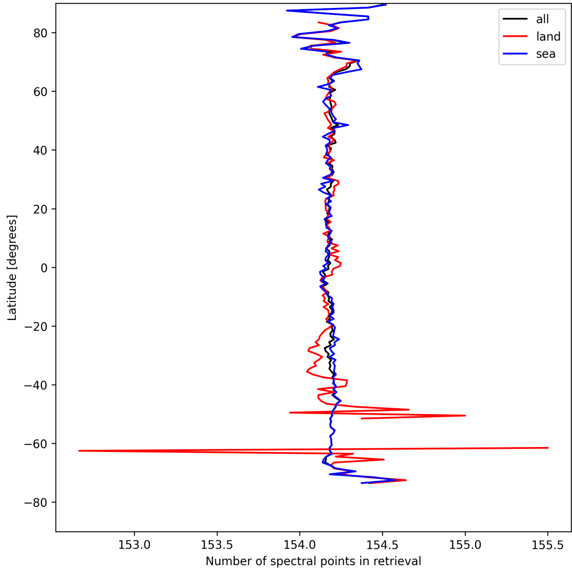
Figure 9: Zonal average of “Number of spectral points in retrieval” for 2025-08-23 to 2025-08-23.
