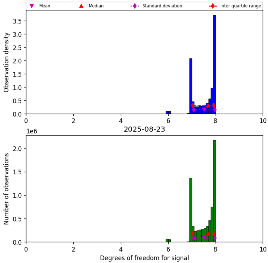
Figure 18: Histogram of “Degrees of freedom for signal” for 2025-08-23 to 2025-08-23
