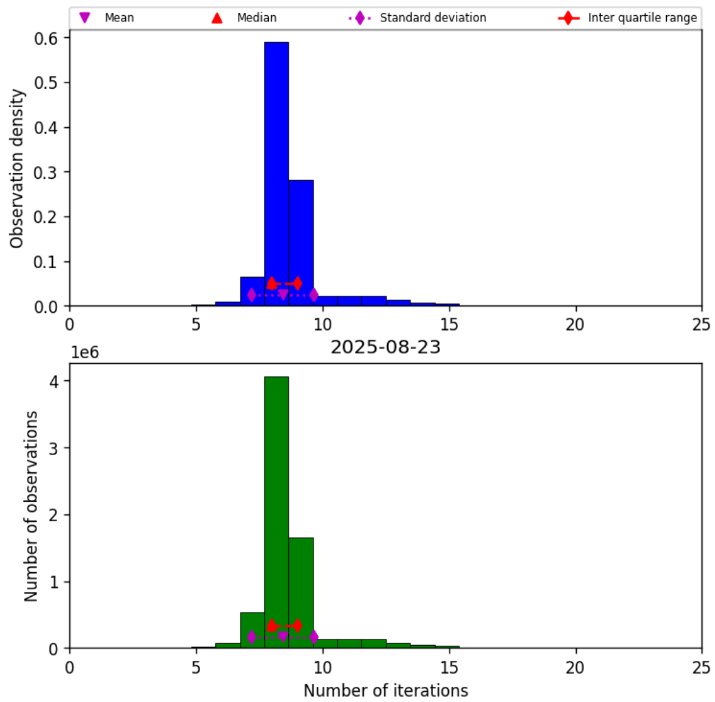
Figure 19: Histogram of “Number of iterations” for 2025-08-23 to 2025-08-23
