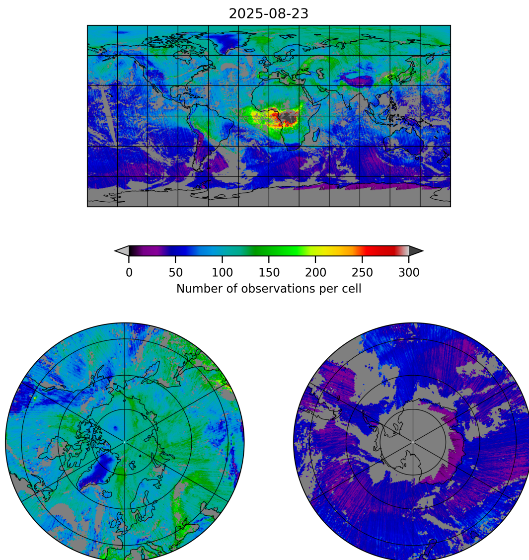
Figure 5: Map of the number of observations for 2025-08-23 to 2025-08-23
