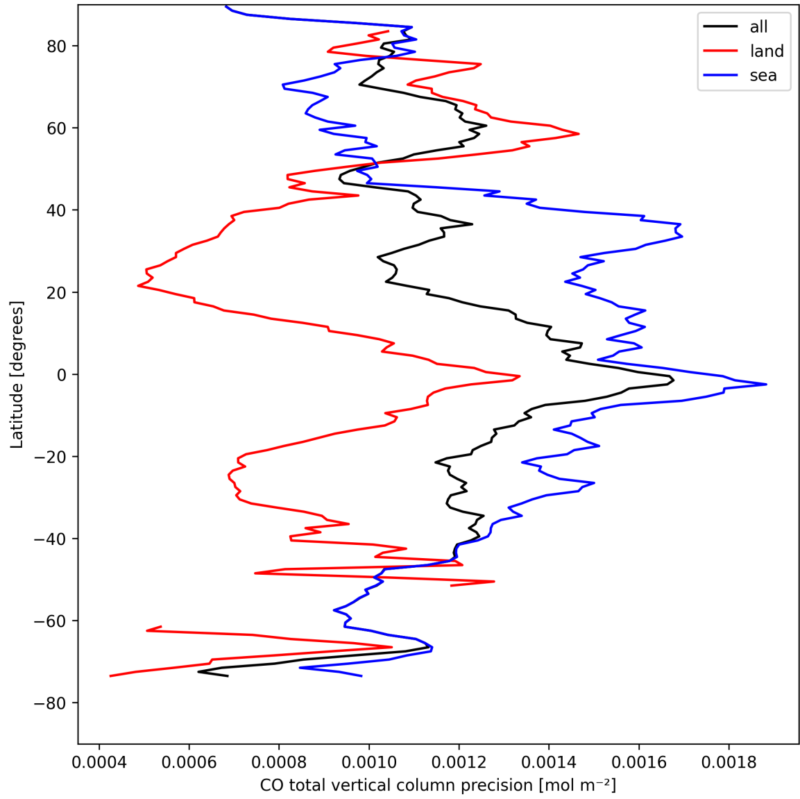
Figure 8: Zonal average of “CO total vertical column precision” for 2025-08-23 to 2025-08-23.
