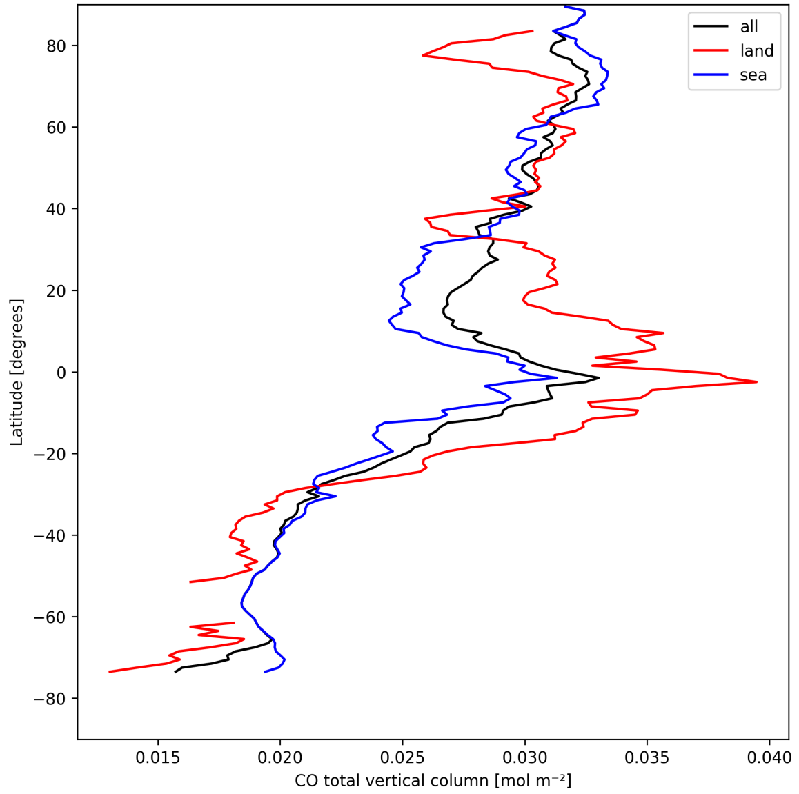
Figure 7: Zonal average of “CO total vertical column” for 2025-08-23 to 2025-08-23.
