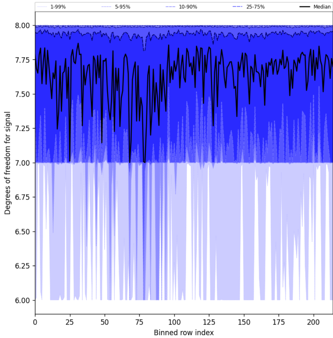
Figure 25: Along track statistics of “Degrees of freedom for signal” for 2025-08-23 to 2025-08-23
