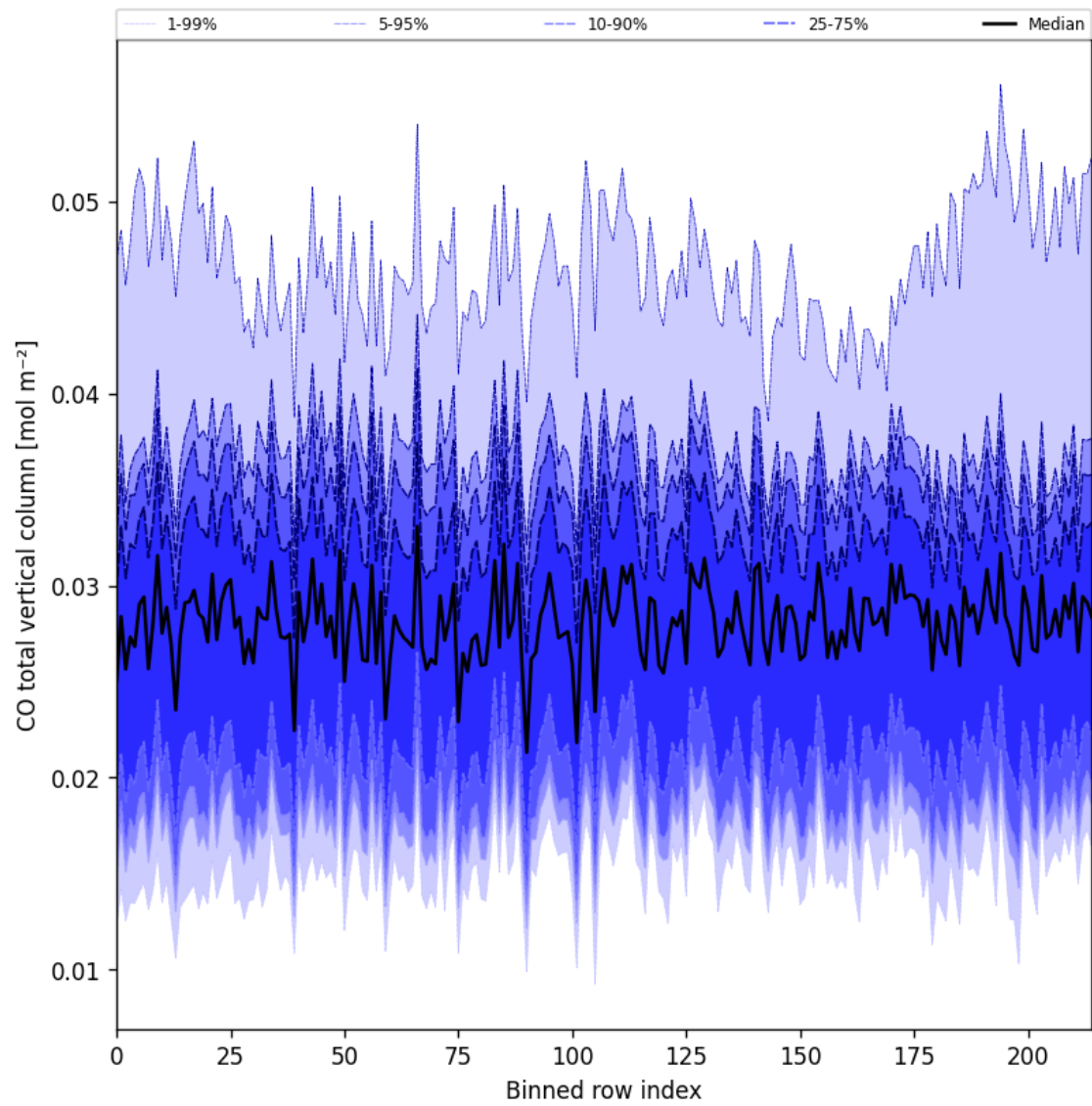
Figure 21: Along track statistics of “CO total vertical column” for 2025-08-23 to 2025-08-23
