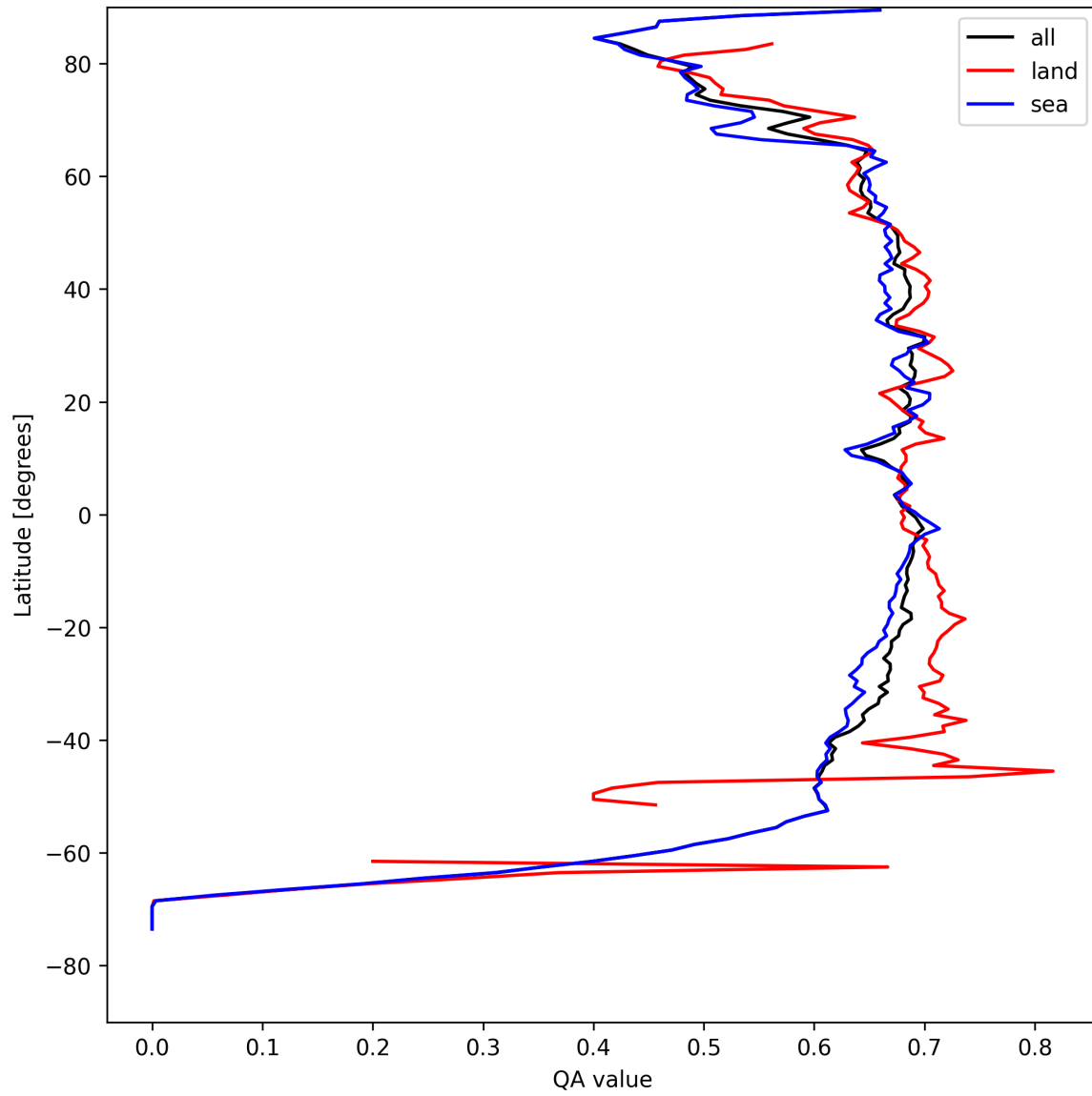
Figure 6: Zonal average of “QA value” for 2025-08-23 to 2025-08-23.
