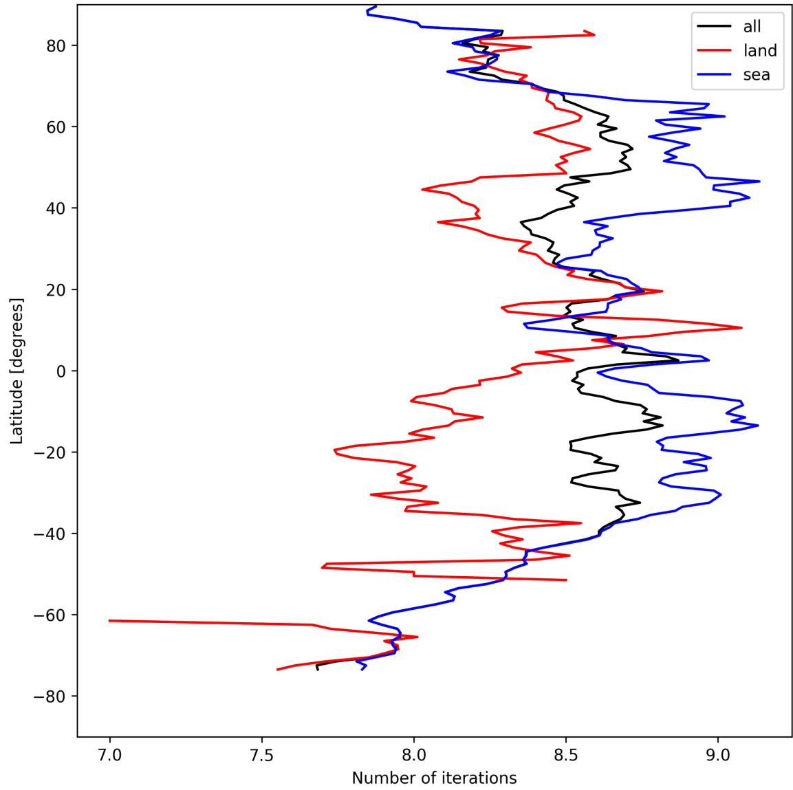
Figure 12: Zonal average of “Number of iterations” for 2025-08-23 to 2025-08-23.
