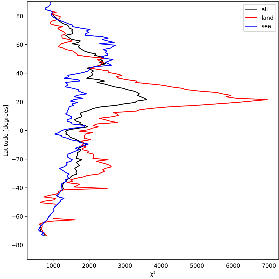
Figure 10: Zonal average of “ \chi^2 ” for 2025-08-23 to 2025-08-23.
