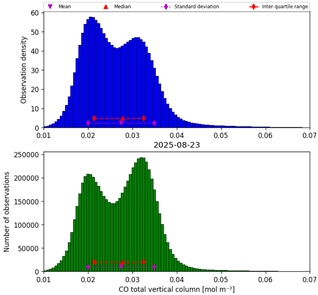
Figure 14: Histogram of “CO total vertical column” for 2025-08-23 to 2025-08-23
