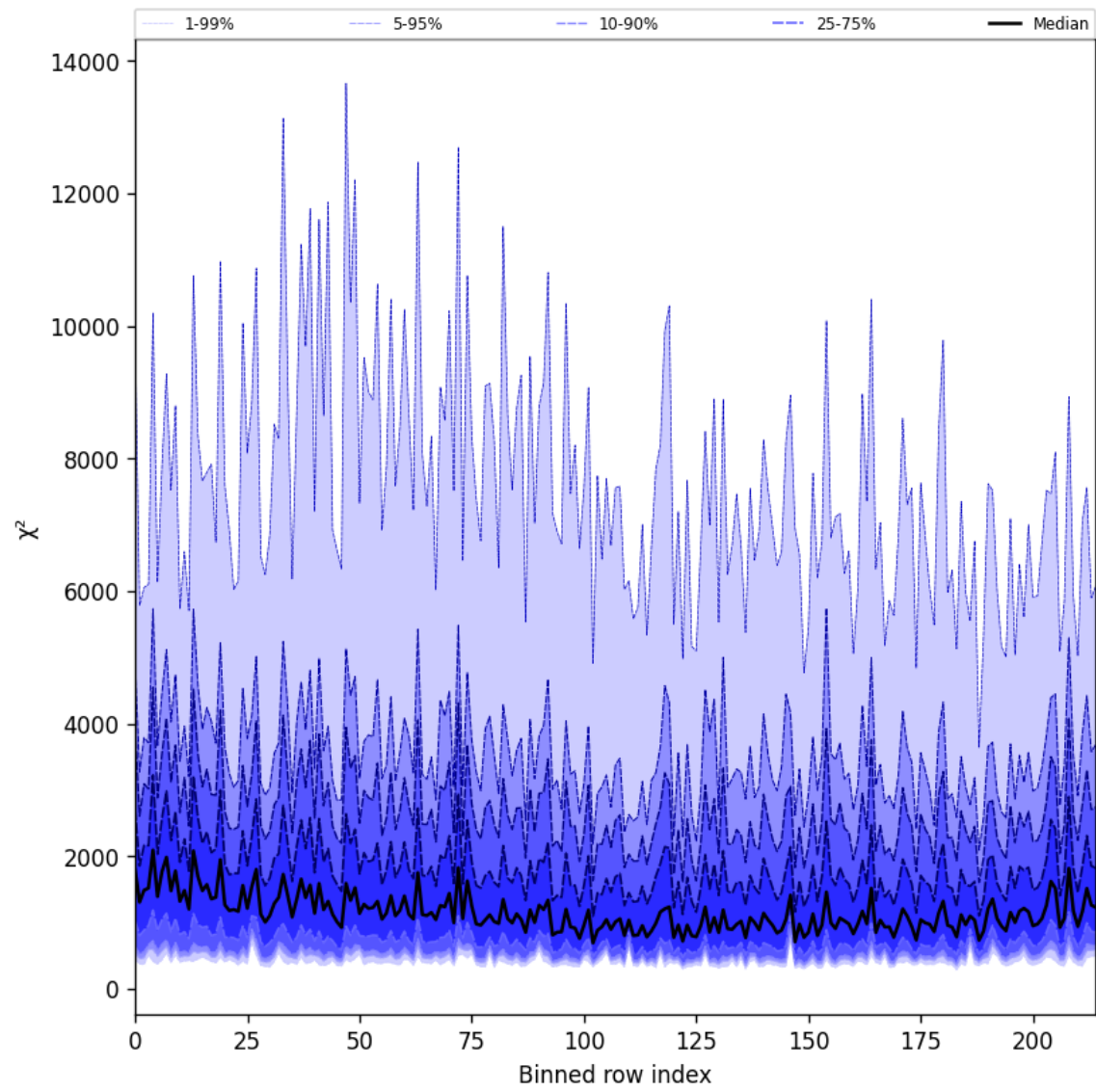
Figure 24: Along track statistics of “ \chi^2 ” for 2025-08-23 to 2025-08-23
