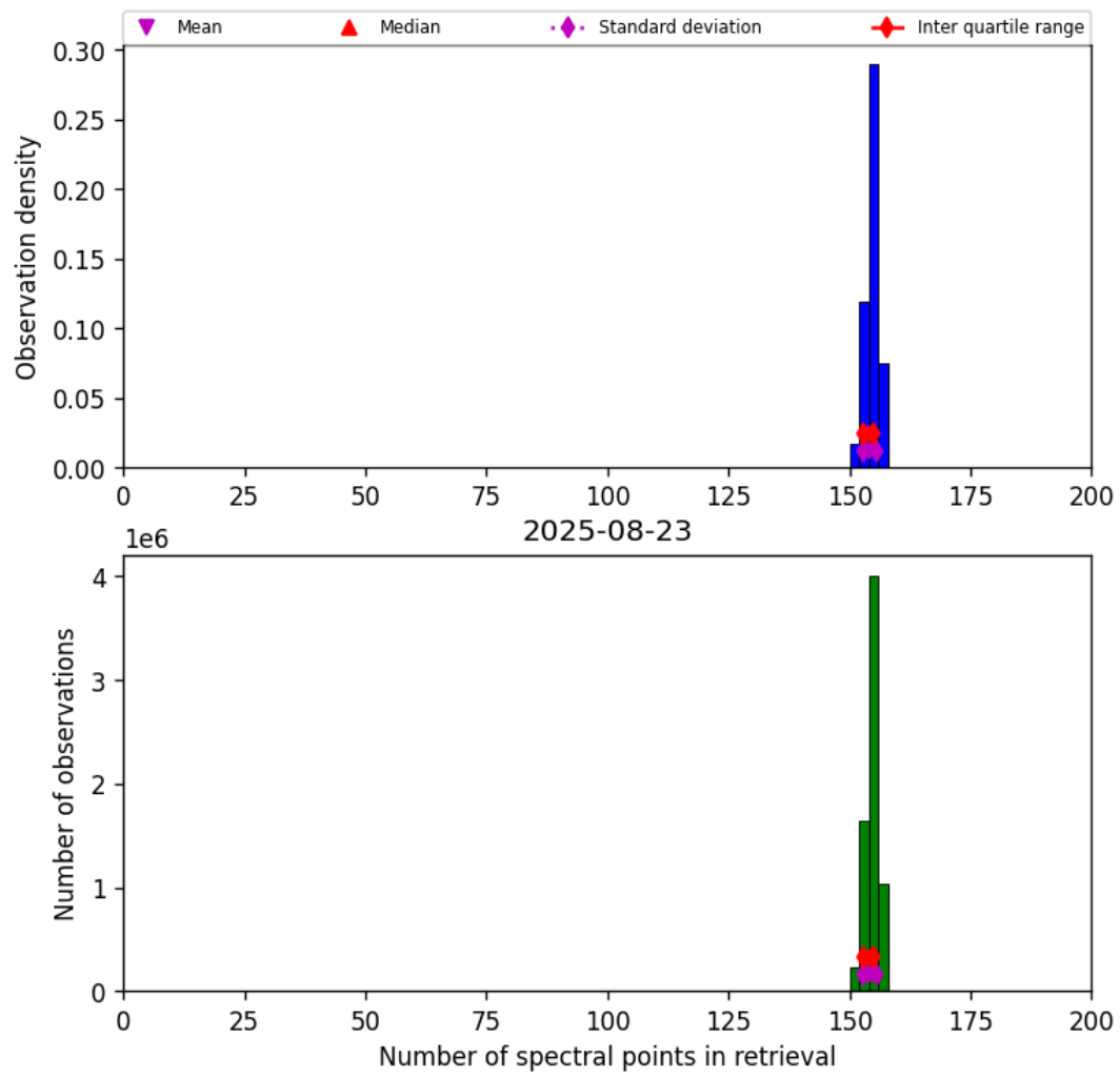
Figure 16: Histogram of “Number of spectral points in retrieval” for 2025-08-23 to 2025-08-23
