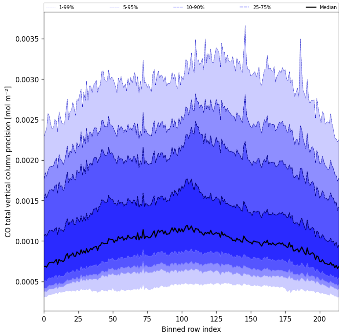
Figure 22: Along track statistics of “CO total vertical column precision” for 2025-08-23 to 2025-08-23
