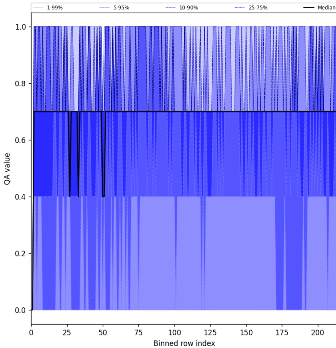
Figure 20: Along track statistics of “QA value” for 2025-08-23 to 2025-08-23
