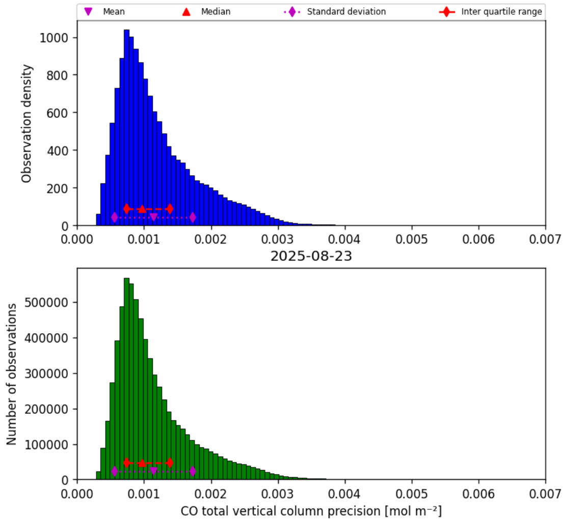
Figure 15: Histogram of “CO total vertical column precision” for 2025-08-23 to 2025-08-23
