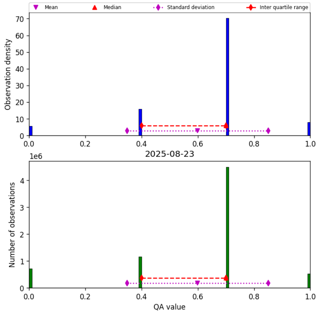
Figure 13: Histogram of “QA value” for 2025-08-23 to 2025-08-23
