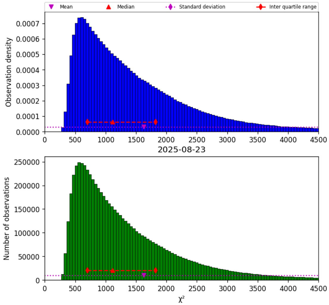
Figure 17: Histogram of “ \chi^2 ” for 2025-08-23 to 2025-08-23
