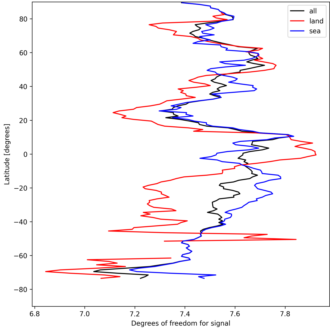
Figure 11: Zonal average of “Degrees of freedom for signal” for 2025-08-23 to 2025-08-23.
