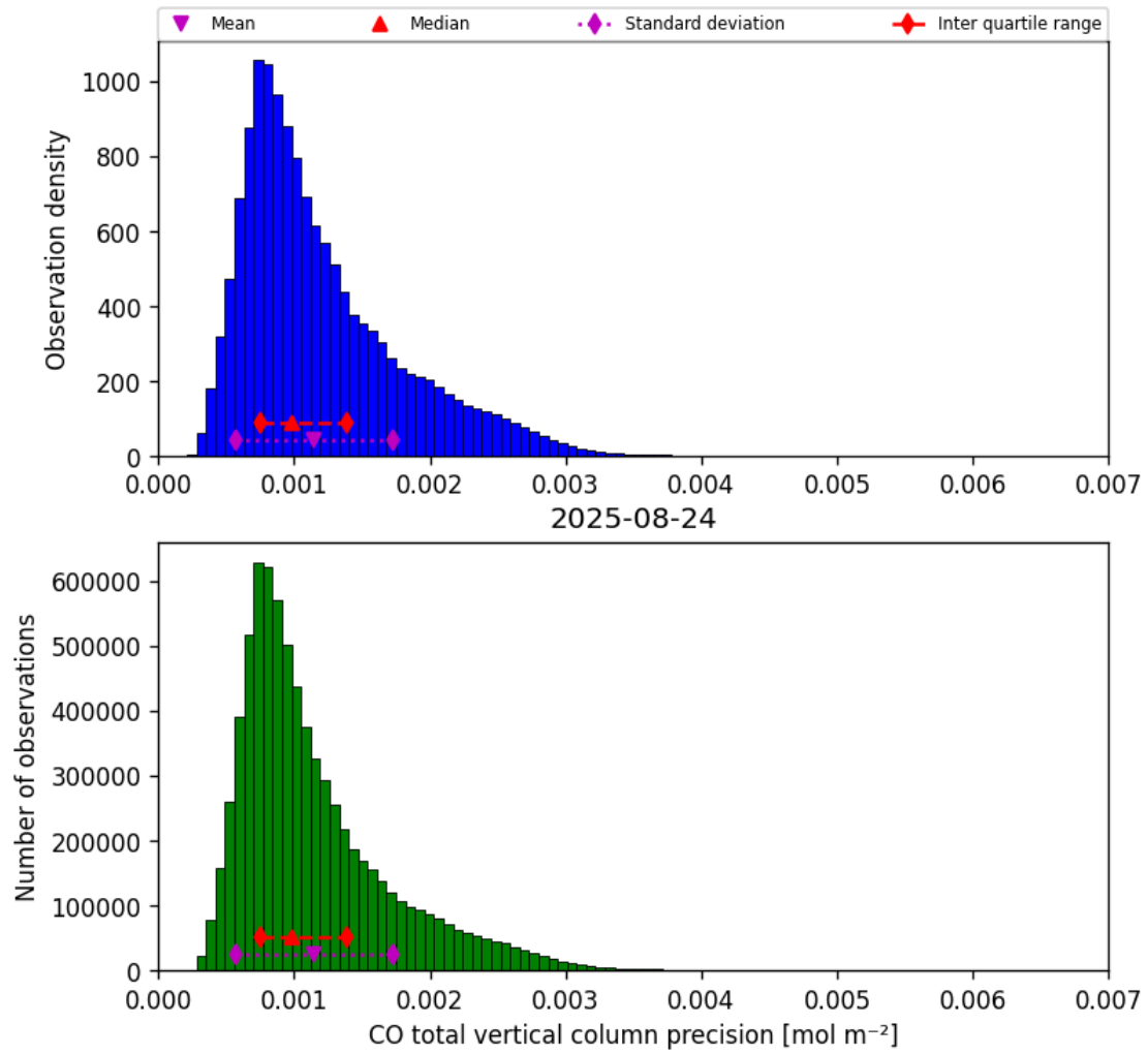
Figure 15: Histogram of “CO total vertical column precision” for 2025-08-24 to 2025-08-25
