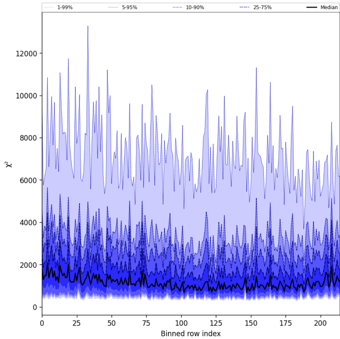
Figure 24: Along track statistics of “ \chi^2 ” for 2025-08-24 to 2025-08-25
