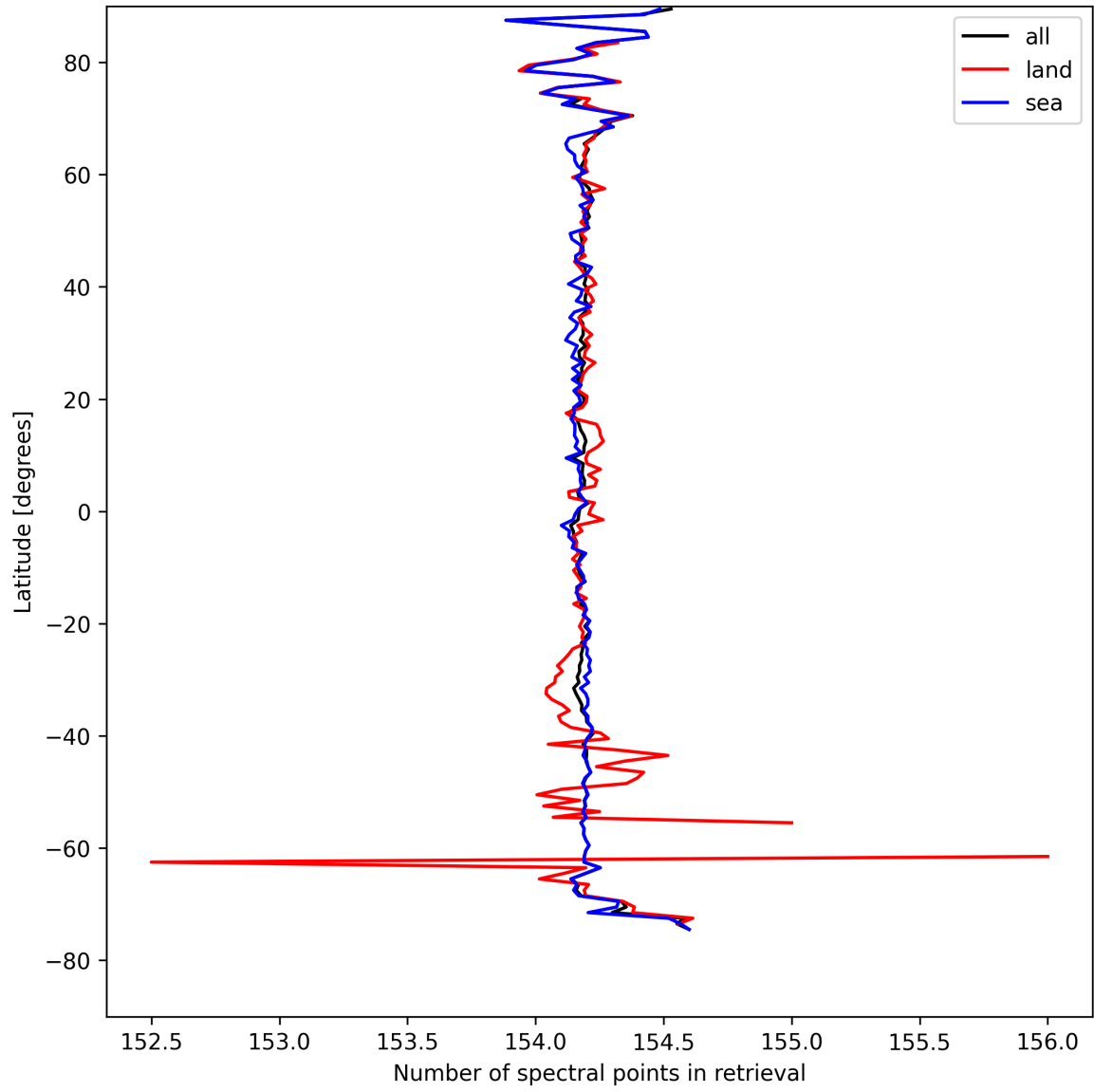
Figure 9: Zonal average of “Number of spectral points in retrieval” for 2025-08-24 to 2025-08-25.
