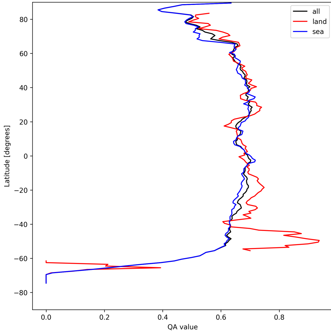
Figure 6: Zonal average of “QA value” for 2025-08-24 to 2025-08-25.
