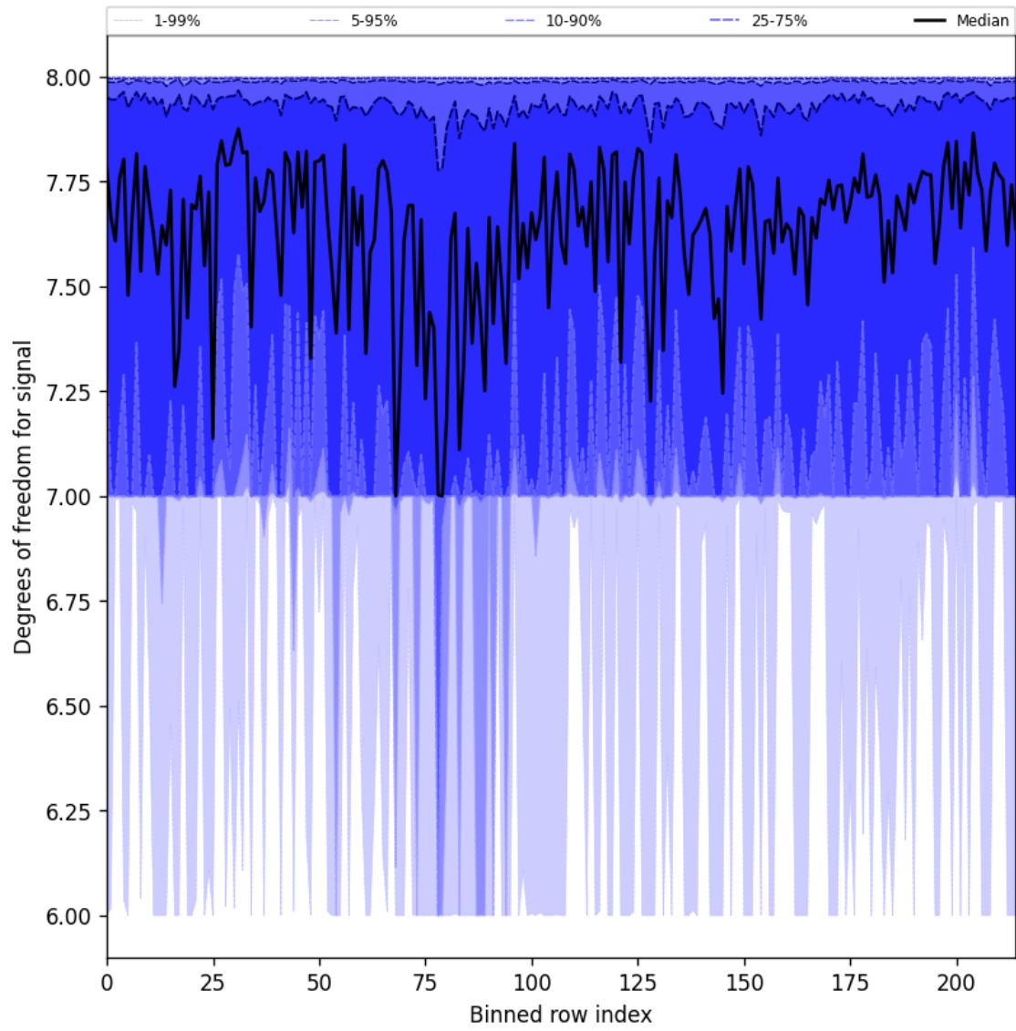
Figure 25: Along track statistics of “Degrees of freedom for signal” for 2025-08-24 to 2025-08-25
