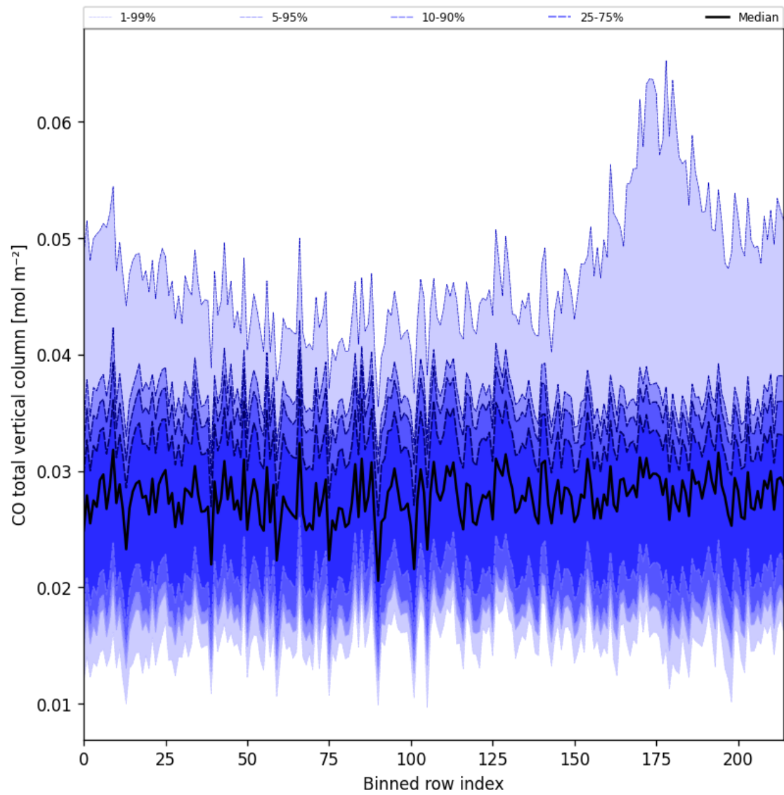
Figure 21: Along track statistics of “CO total vertical column” for 2025-08-24 to 2025-08-25
