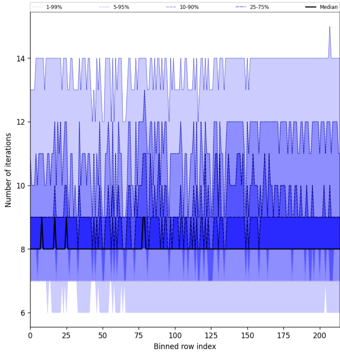
Figure 26: Along track statistics of “Number of iterations” for 2025-08-24 to 2025-08-25
