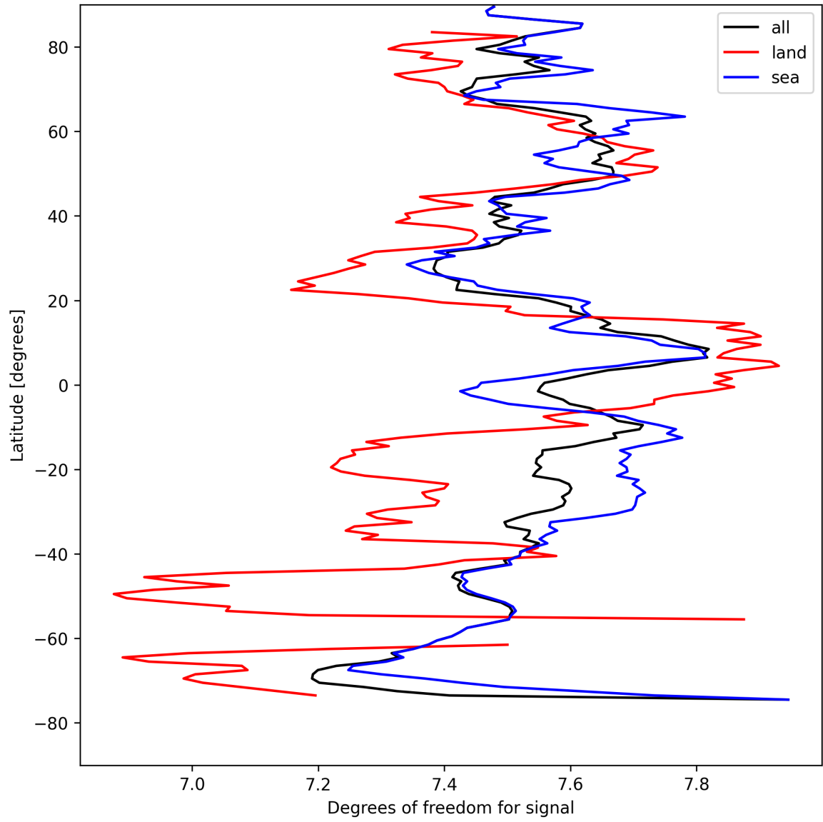
Figure 11: Zonal average of “Degrees of freedom for signal” for 2025-08-24 to 2025-08-25.
