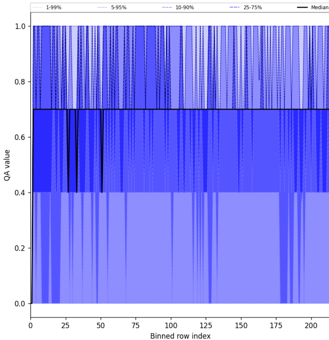
Figure 20: Along track statistics of “QA value” for 2025-08-24 to 2025-08-25
