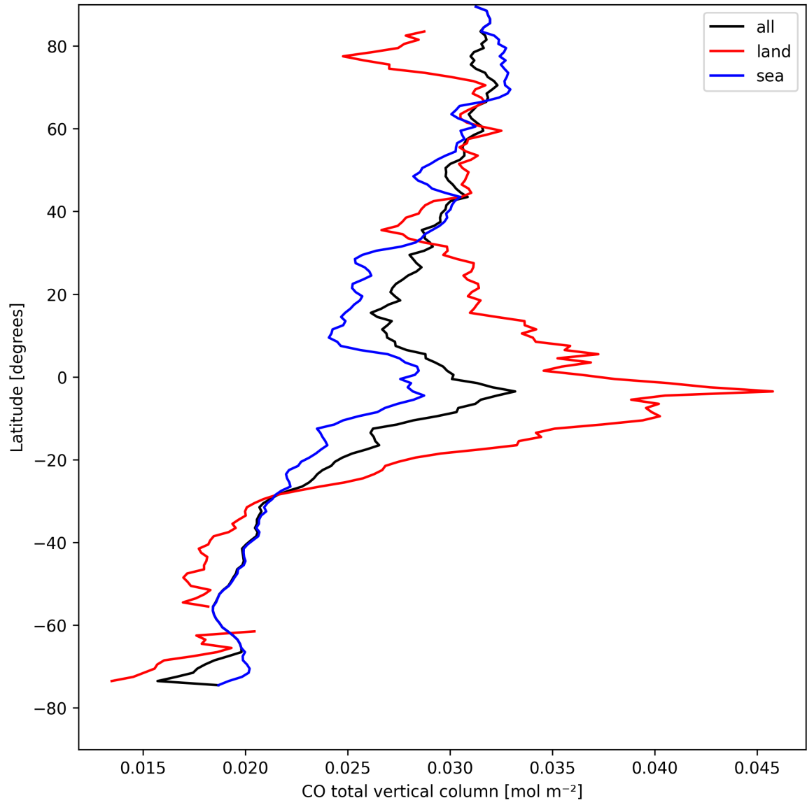
Figure 7: Zonal average of “CO total vertical column” for 2025-08-24 to 2025-08-25.
