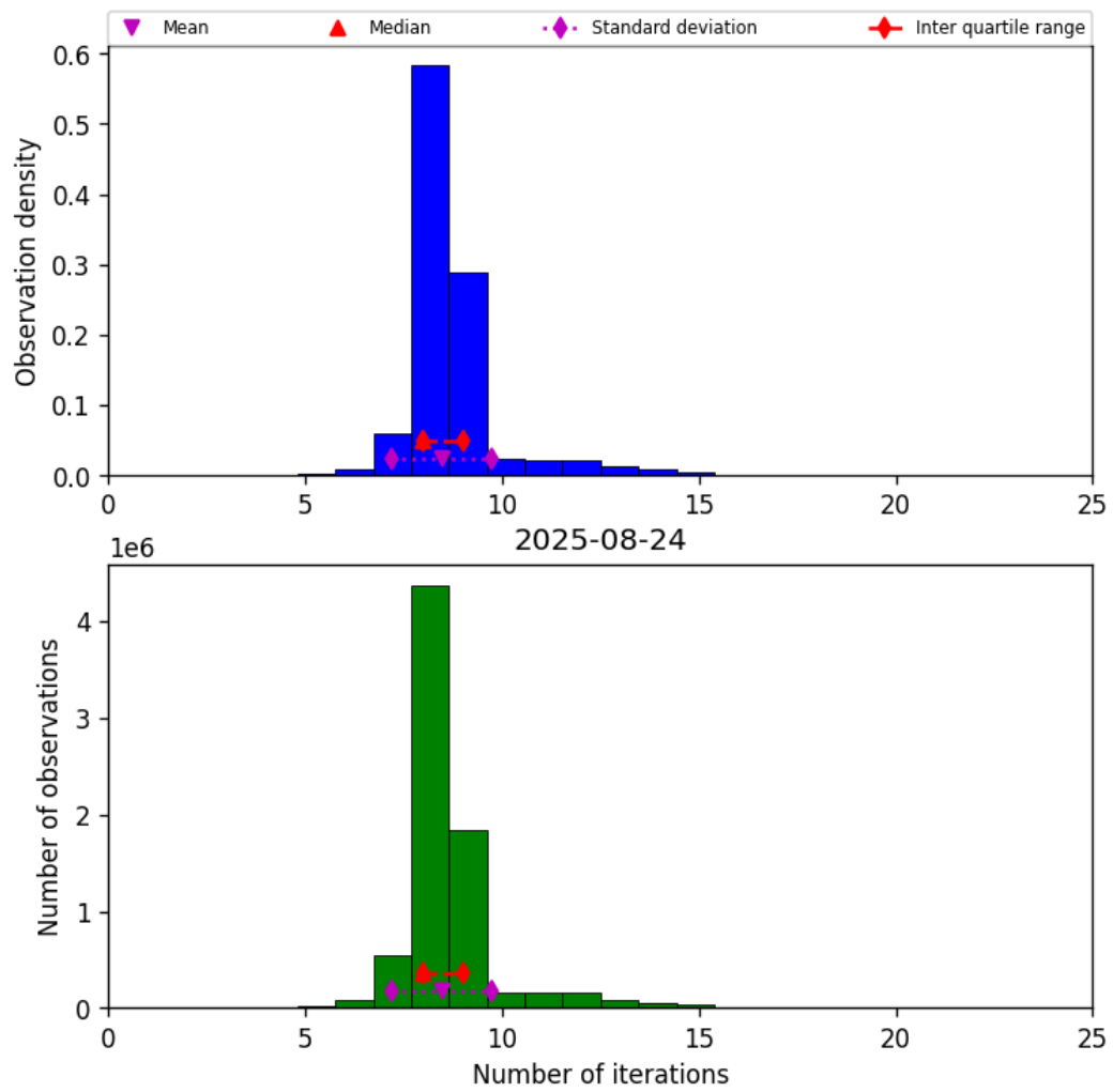
Figure 19: Histogram of “Number of iterations” for 2025-08-24 to 2025-08-25
