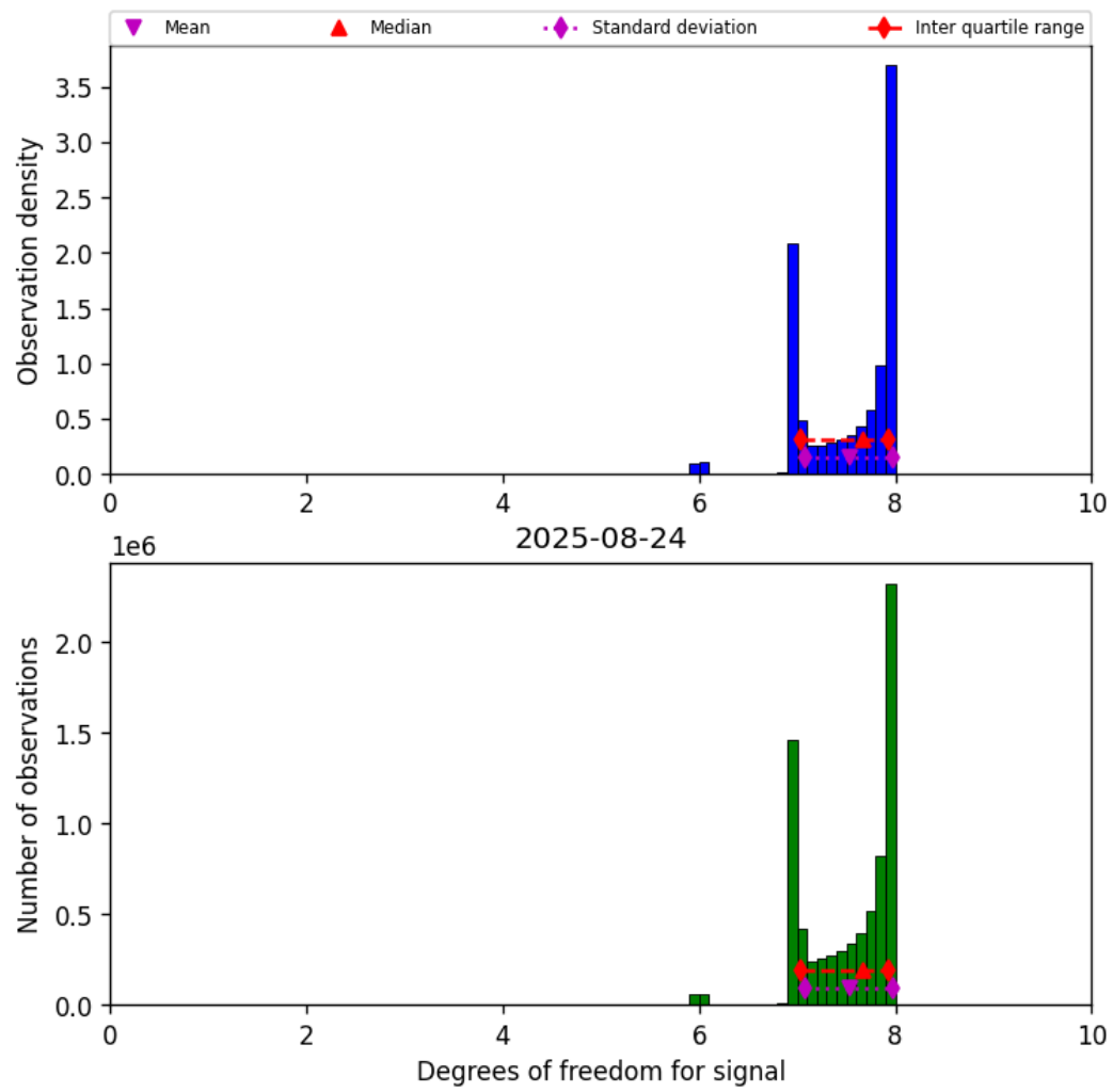
Figure 18: Histogram of “Degrees of freedom for signal” for 2025-08-24 to 2025-08-25
