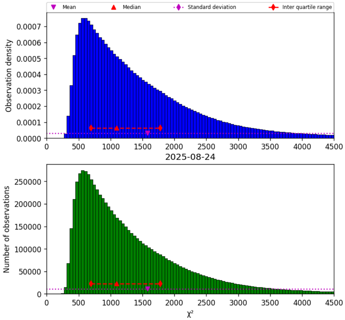
Figure 17: Histogram of “ \chi^2 ” for 2025-08-24 to 2025-08-25
