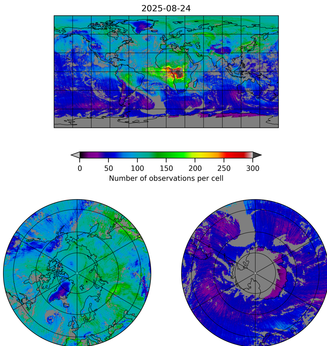
Figure 5: Map of the number of observations for 2025-08-24 to 2025-08-25
