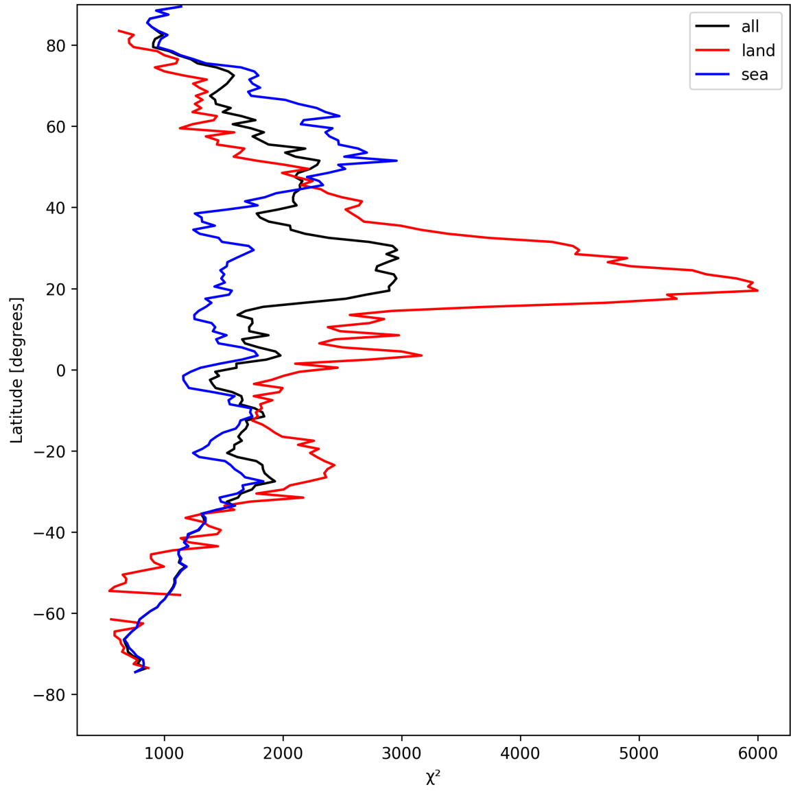
Figure 10: Zonal average of “ \chi^2 ” for 2025-08-24 to 2025-08-25.
