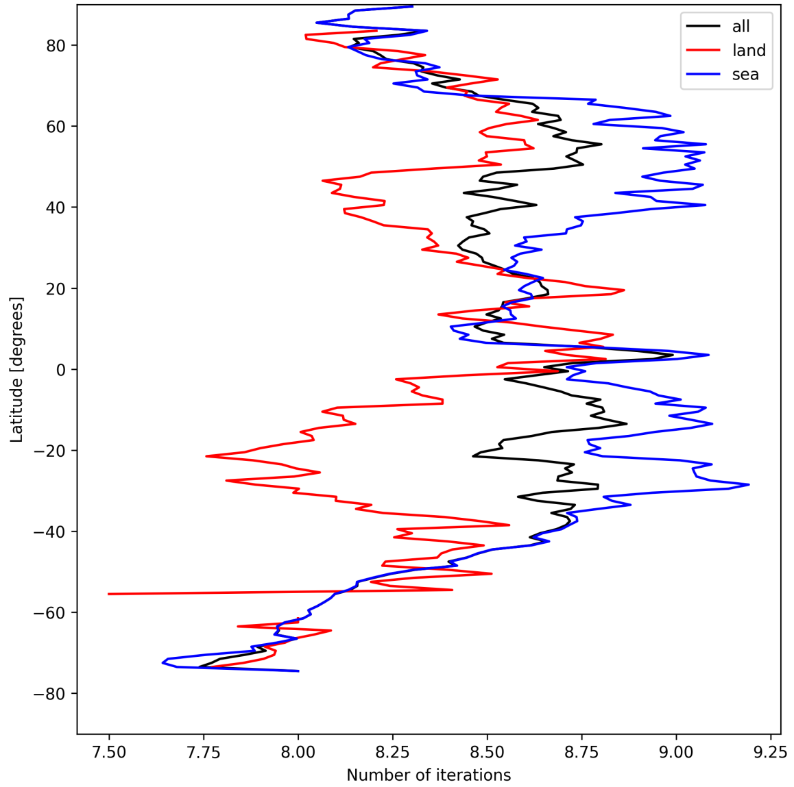
Figure 12: Zonal average of “Number of iterations” for 2025-08-24 to 2025-08-25.
