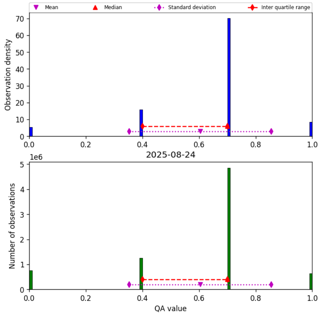
Figure 13: Histogram of “QA value” for 2025-08-24 to 2025-08-25
