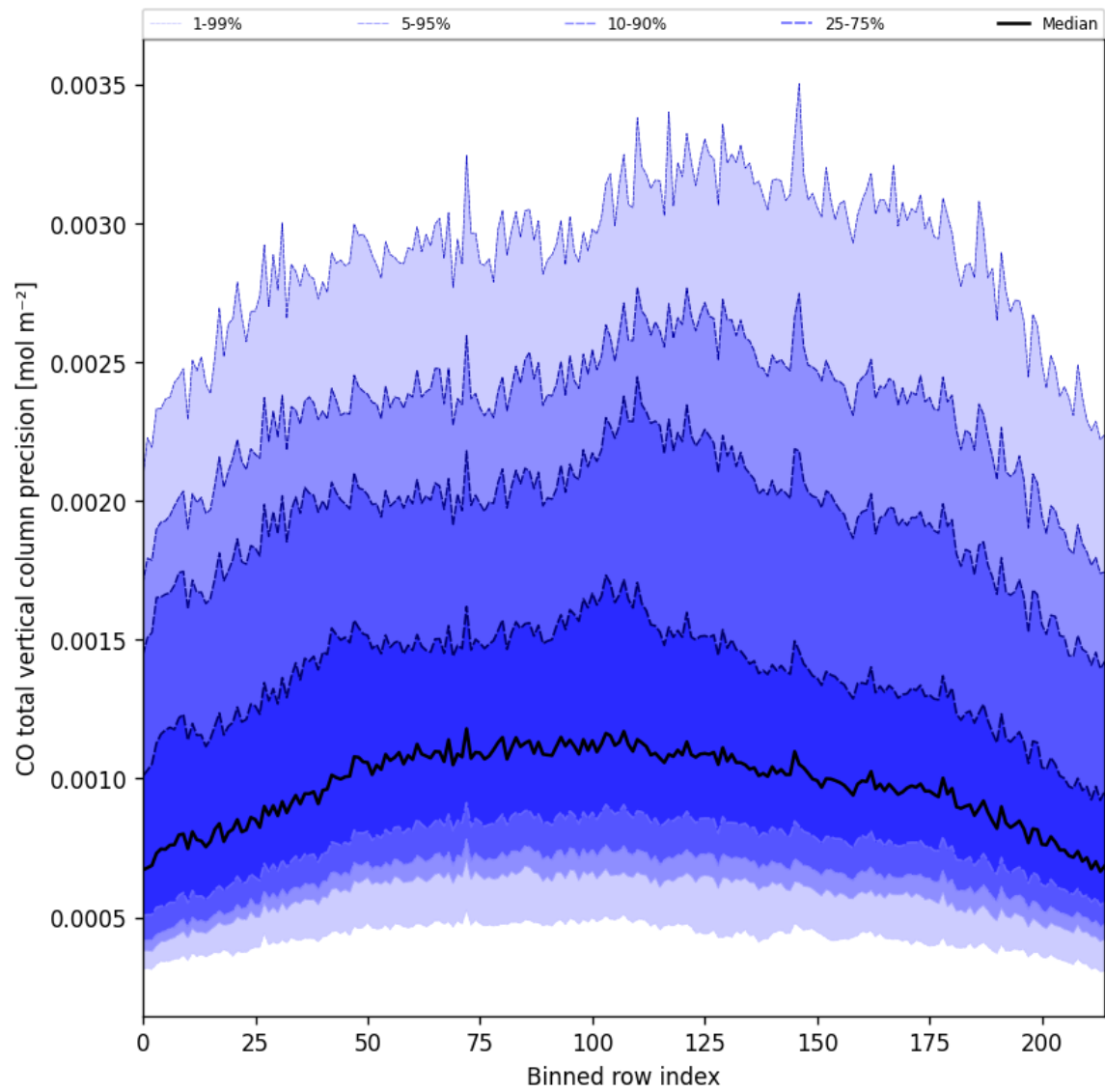
Figure 22: Along track statistics of “CO total vertical column precision” for 2025-08-24 to 2025-08-25
