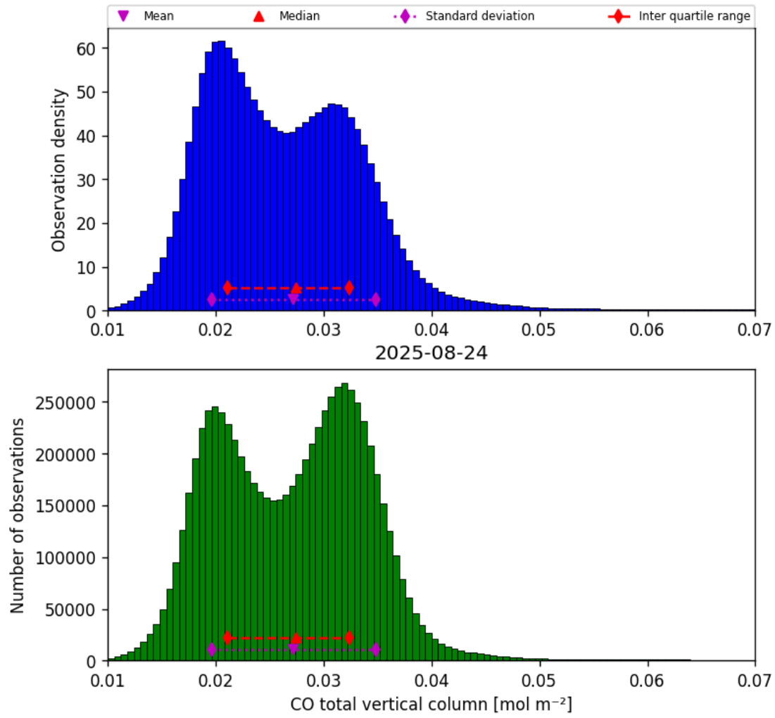
Figure 14: Histogram of “CO total vertical column” for 2025-08-24 to 2025-08-25
