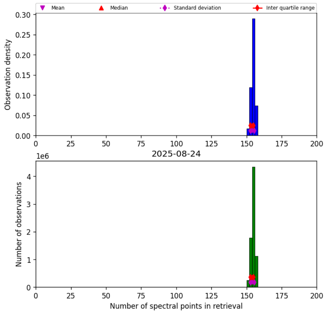
Figure 16: Histogram of “Number of spectral points in retrieval” for 2025-08-24 to 2025-08-25
