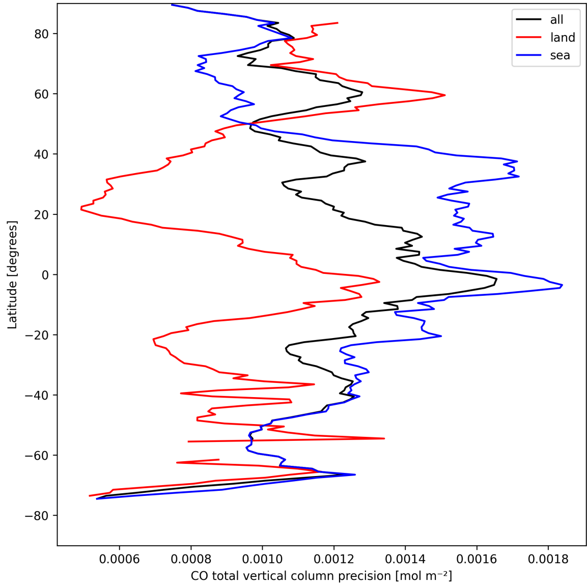
Figure 8: Zonal average of "CO total vertical column precision" for 2025-08-24 to 2025-08-25.
