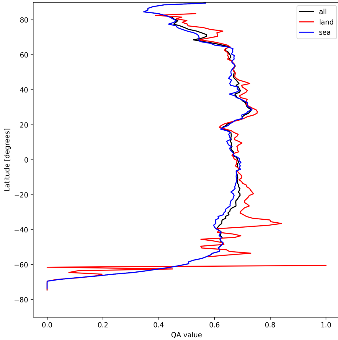
Figure 6: Zonal average of “QA value” for 2025-08-25 to 2025-08-26.
