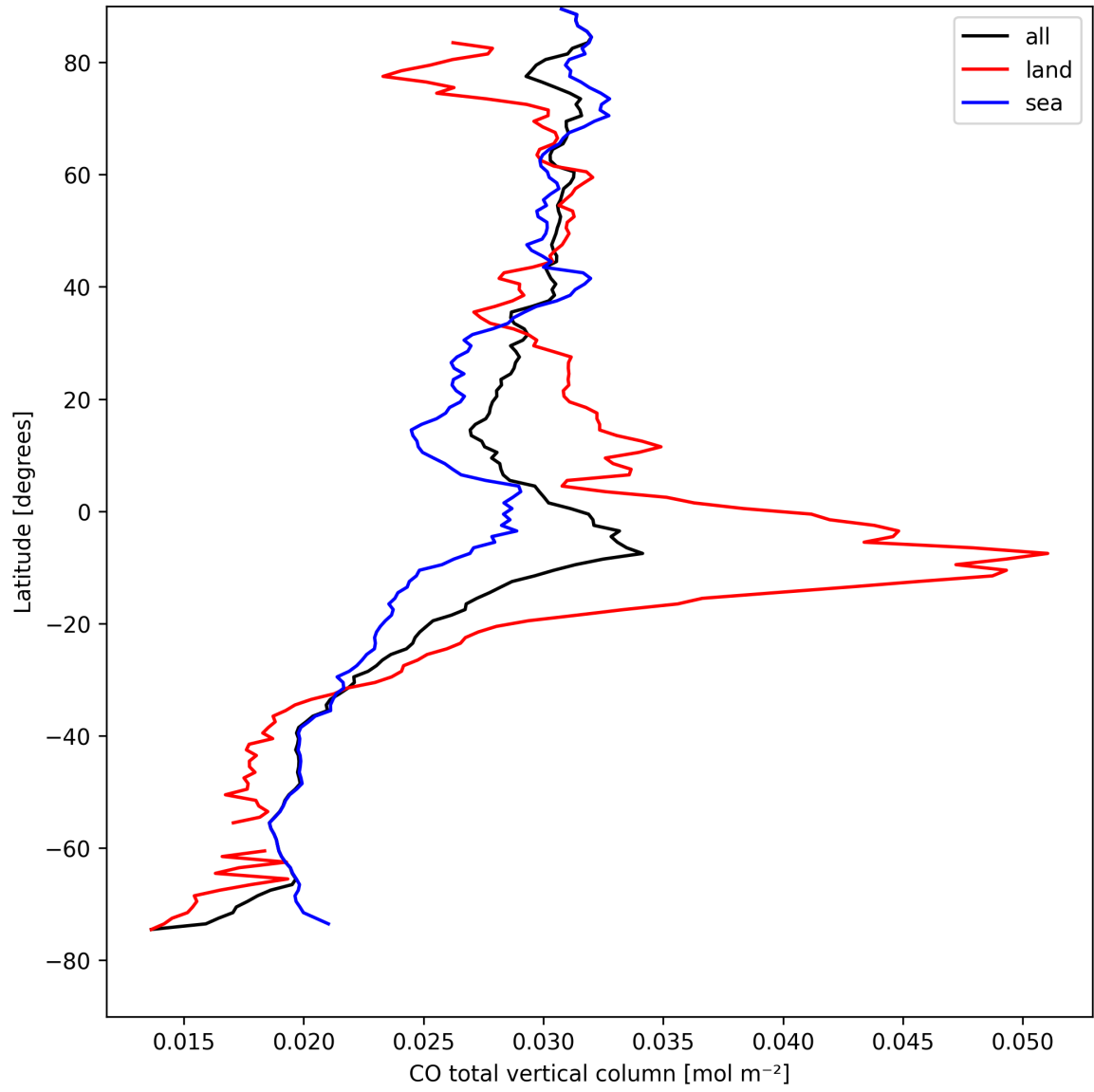
Figure 7: Zonal average of “CO total vertical column” for 2025-08-25 to 2025-08-26.
