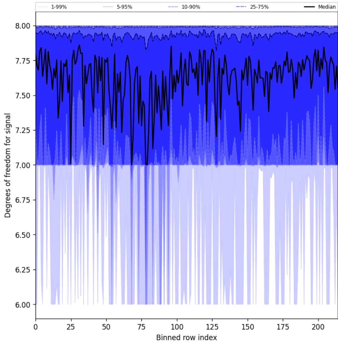
Figure 25: Along track statistics of “Degrees of freedom for signal” for 2025-08-25 to 2025-08-26
