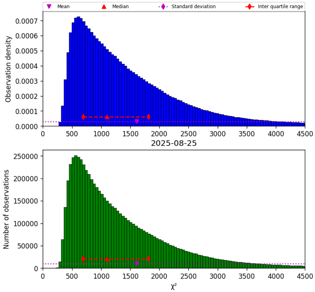
Figure 17: Histogram of “ \chi^2 ” for 2025-08-25 to 2025-08-26
