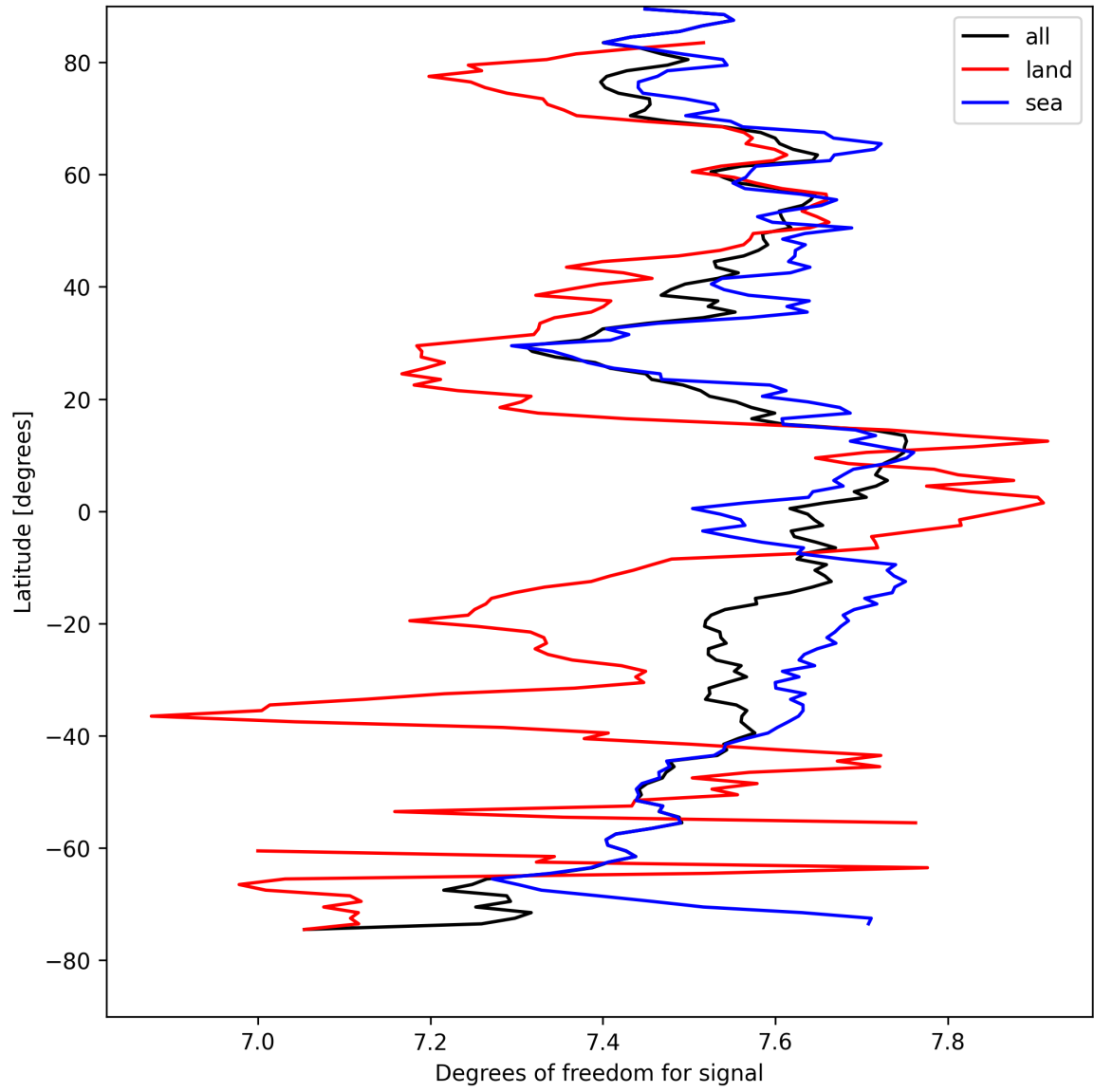
Figure 11: Zonal average of “Degrees of freedom for signal” for 2025-08-25 to 2025-08-26.
