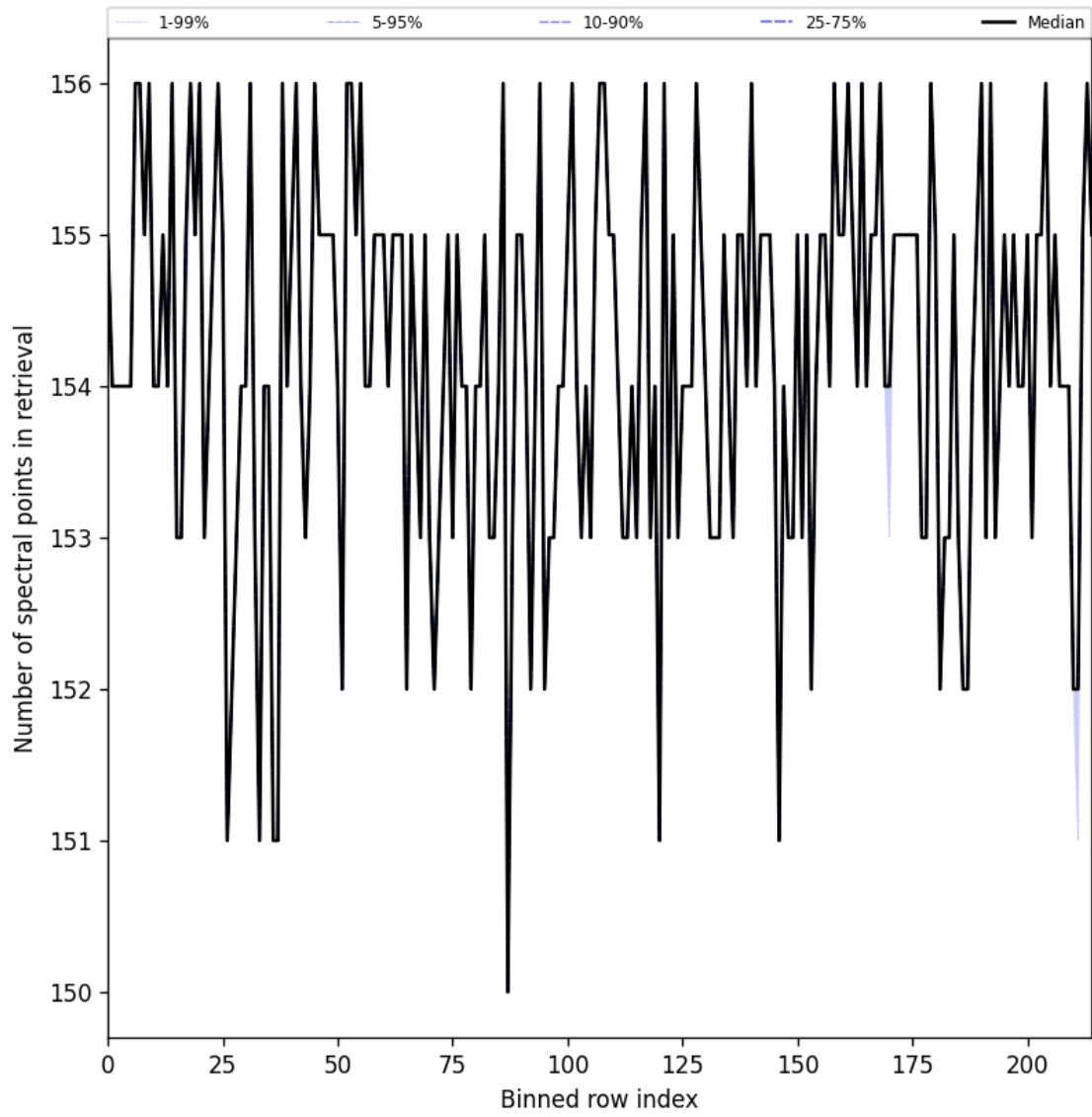
Figure 23: Along track statistics of “Number of spectral points in retrieval” for 2025-08-25 to 2025-08-26
