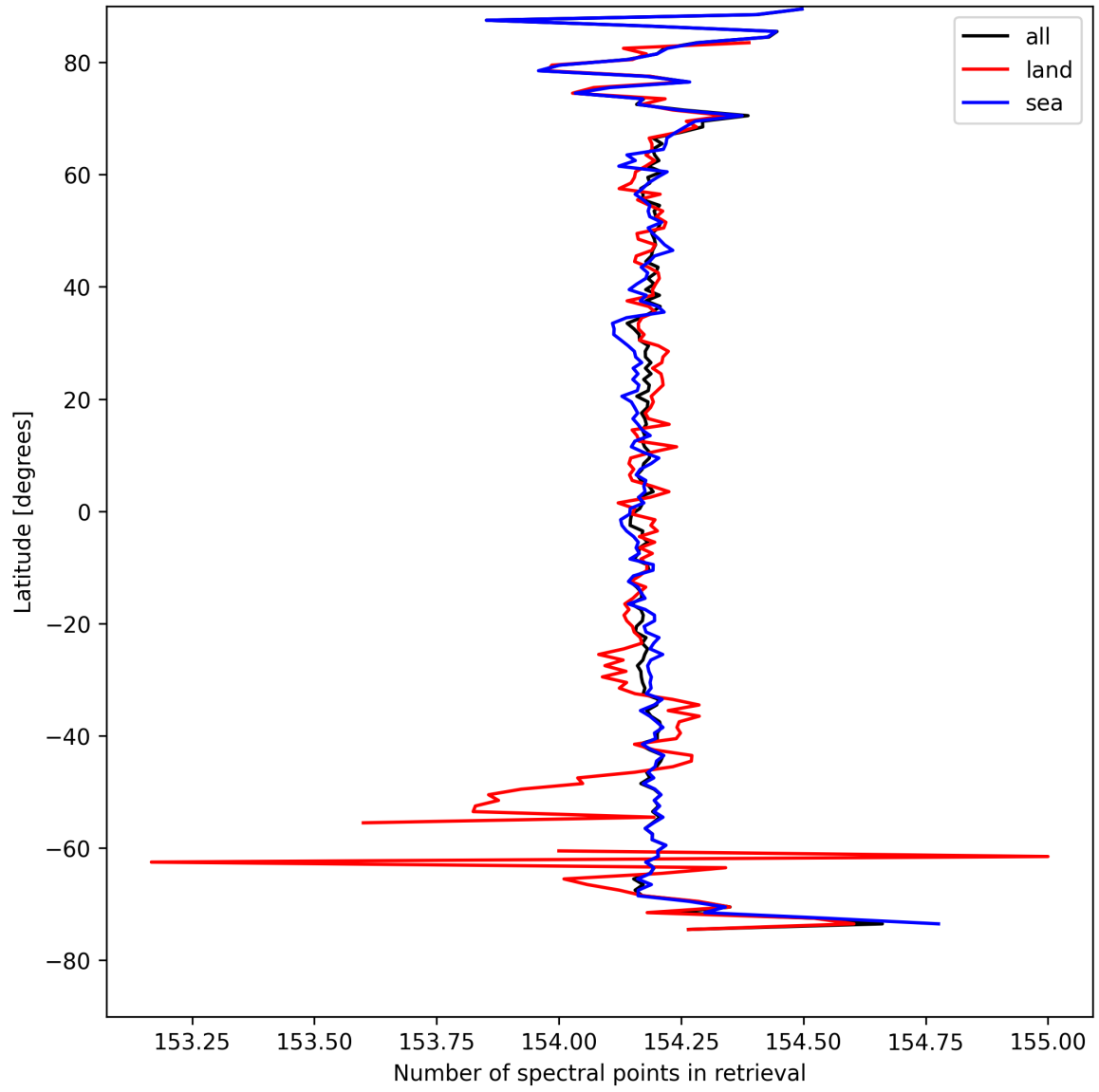
Figure 9: Zonal average of “Number of spectral points in retrieval” for 2025-08-25 to 2025-08-26.
