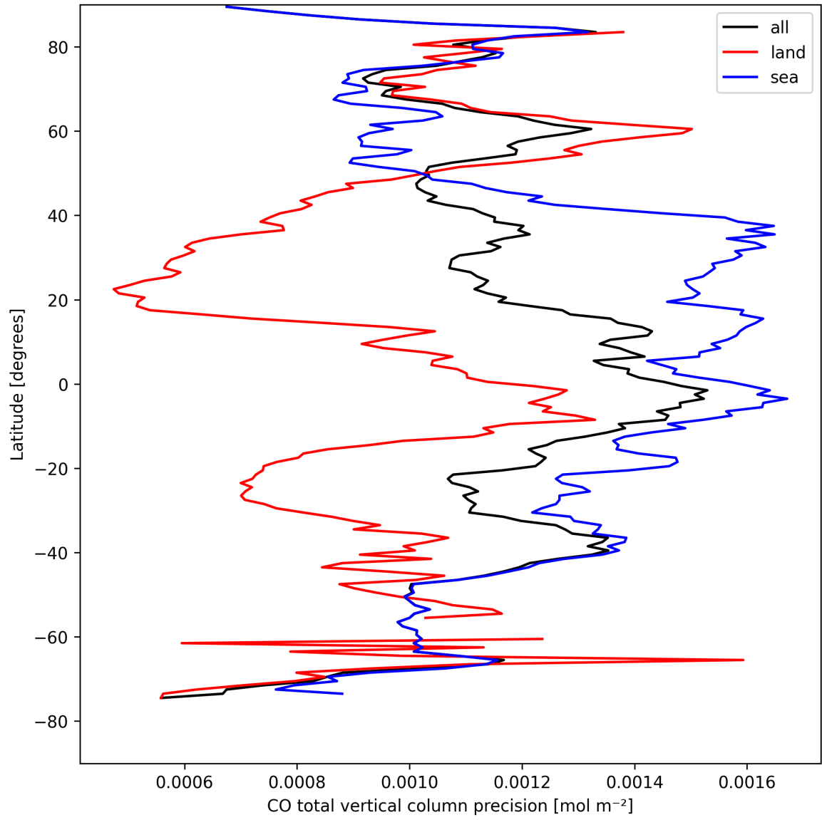
Figure 8: Zonal average of "CO total vertical column precision" for 2025-08-25 to 2025-08-26.
