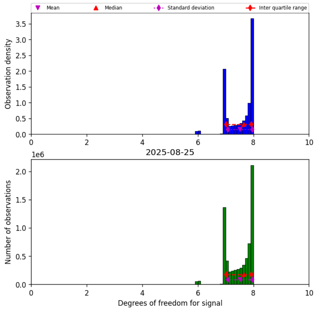
Figure 18: Histogram of “Degrees of freedom for signal” for 2025-08-25 to 2025-08-26
