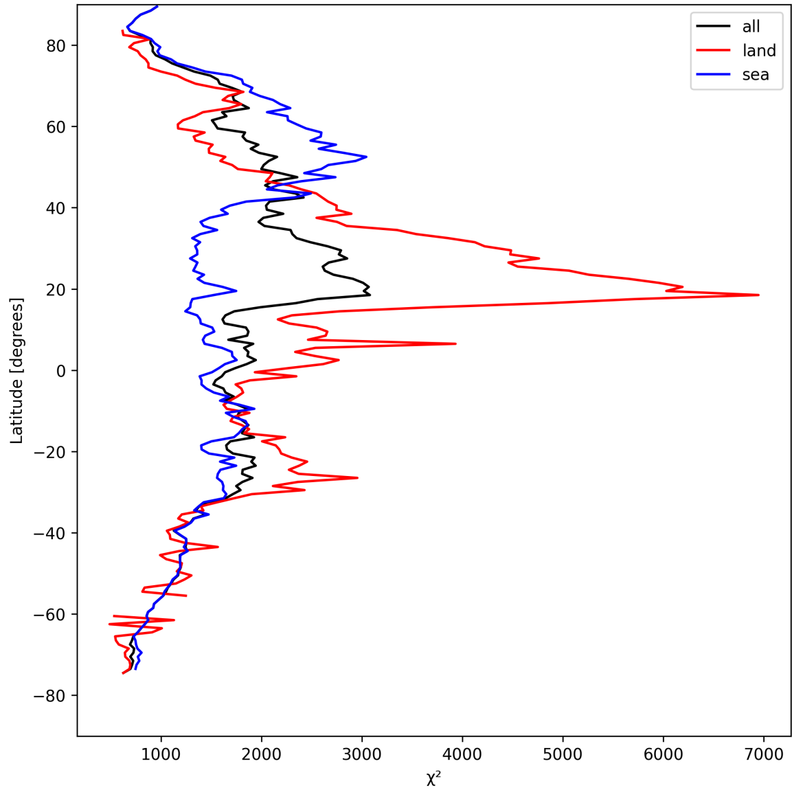
Figure 10: Zonal average of “ \chi^2 ” for 2025-08-25 to 2025-08-26.
