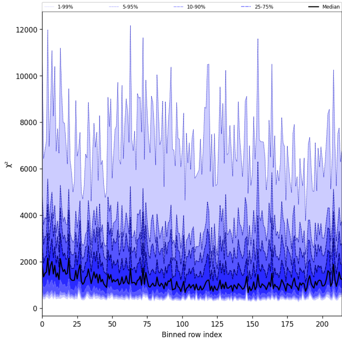
Figure 24: Along track statistics of “ \chi^2 ” for 2025-08-25 to 2025-08-26
