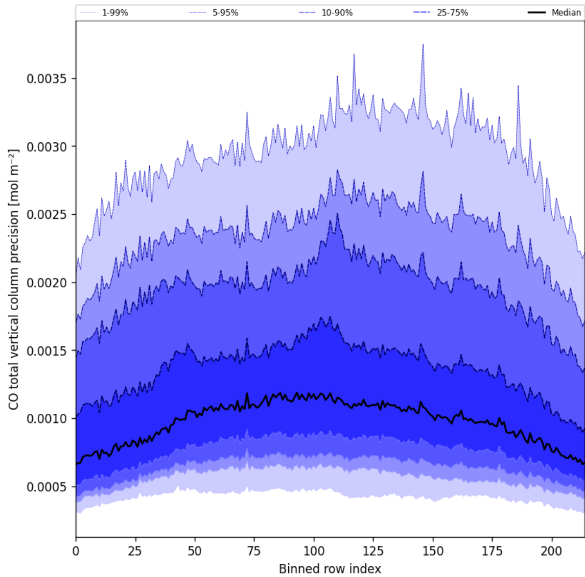
Figure 22: Along track statistics of “CO total vertical column precision” for 2025-08-25 to 2025-08-26
