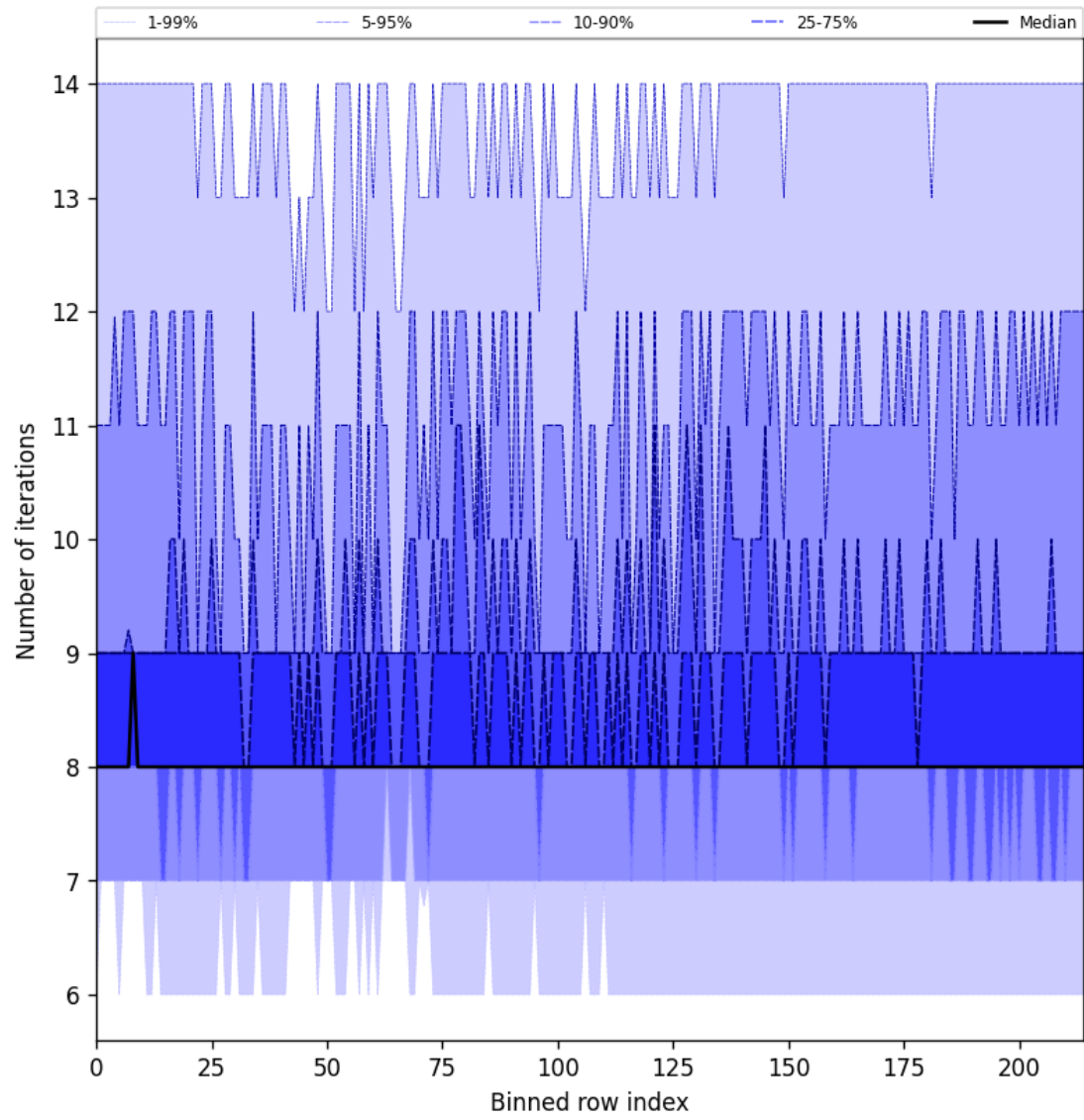
Figure 26: Along track statistics of “Number of iterations” for 2025-08-25 to 2025-08-26
