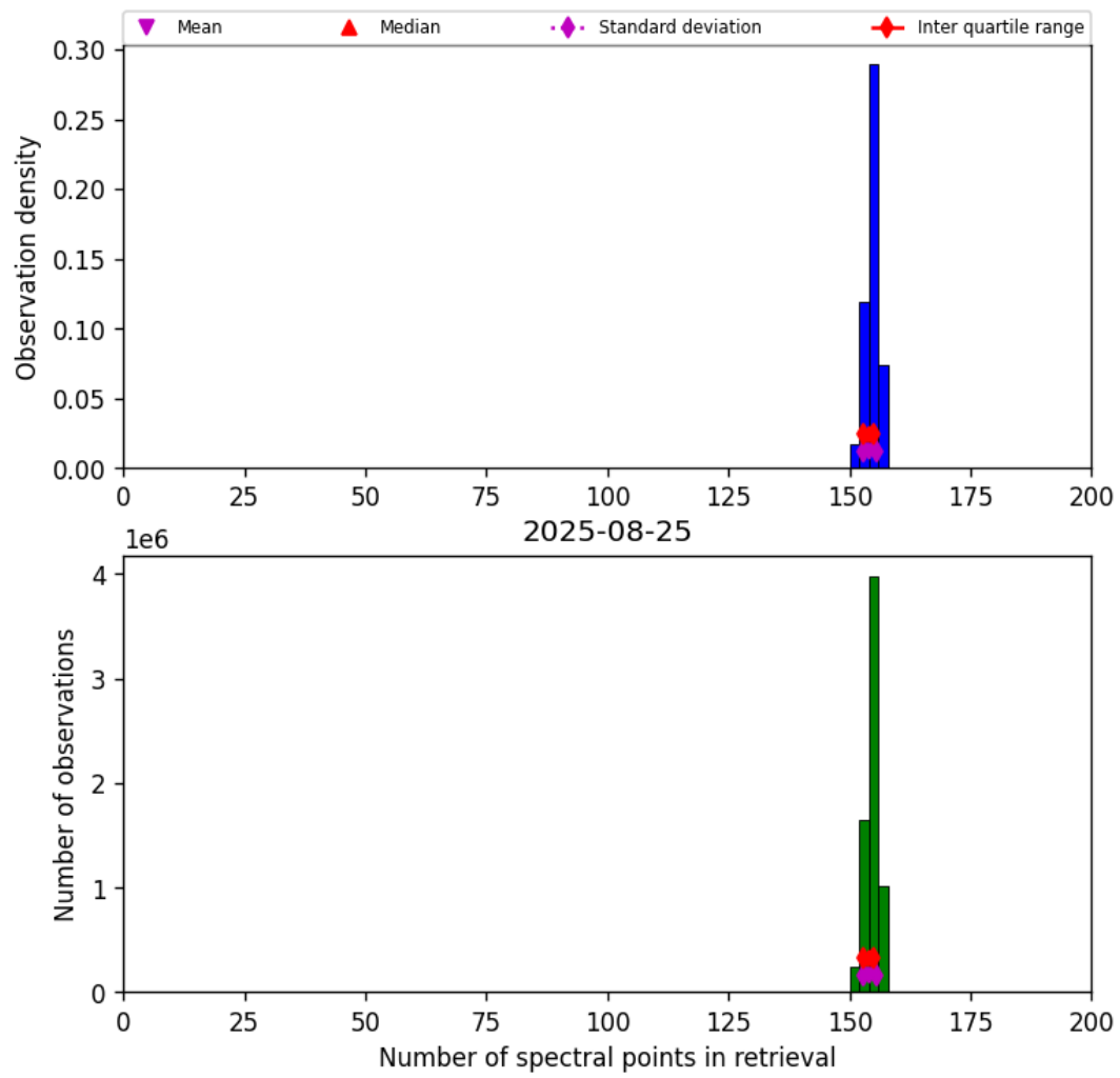
Figure 16: Histogram of “Number of spectral points in retrieval” for 2025-08-25 to 2025-08-26
