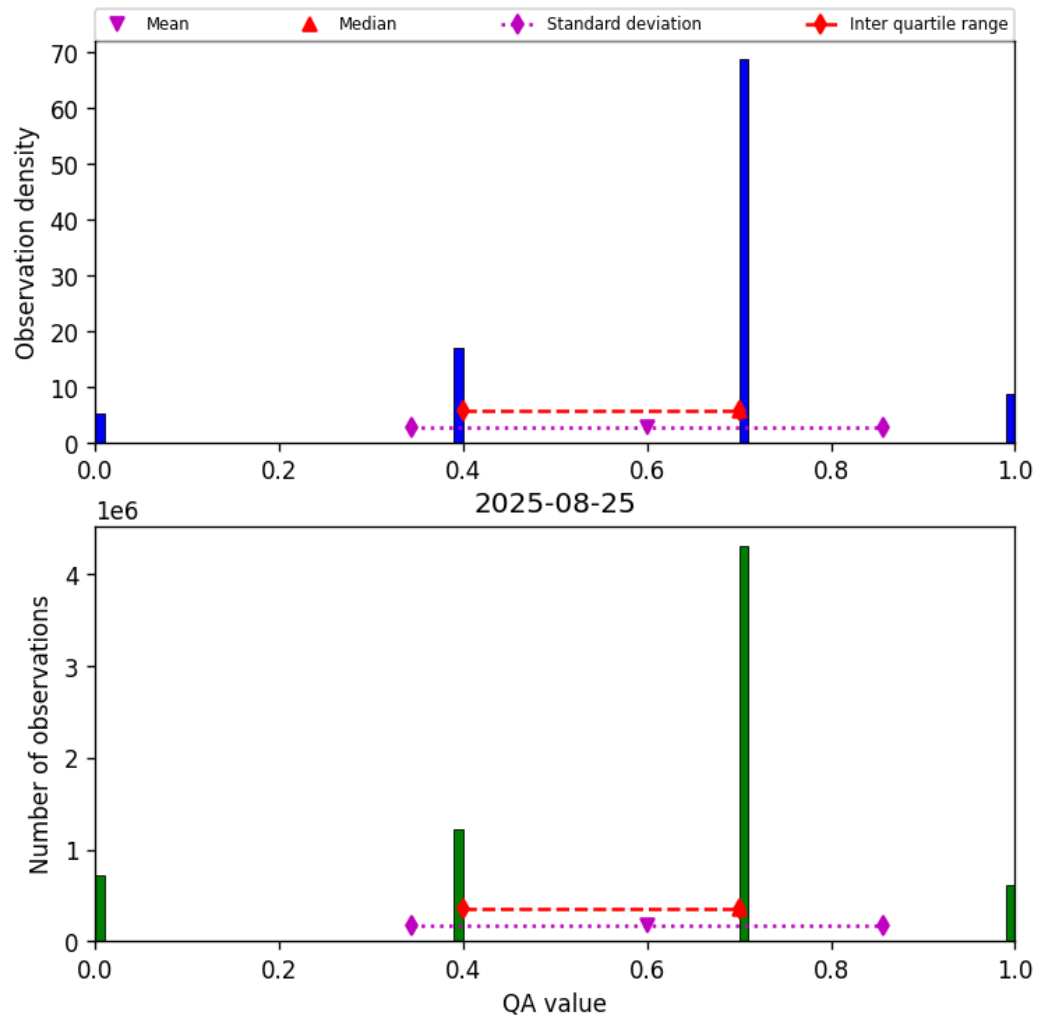
Figure 13: Histogram of “QA value” for 2025-08-25 to 2025-08-26
