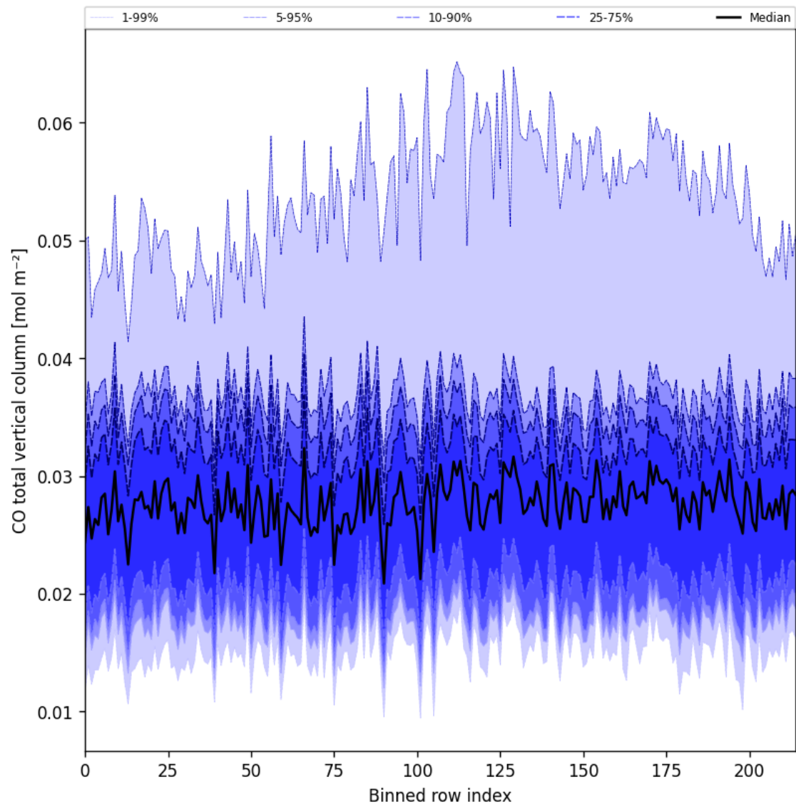
Figure 21: Along track statistics of “CO total vertical column” for 2025-08-25 to 2025-08-26
