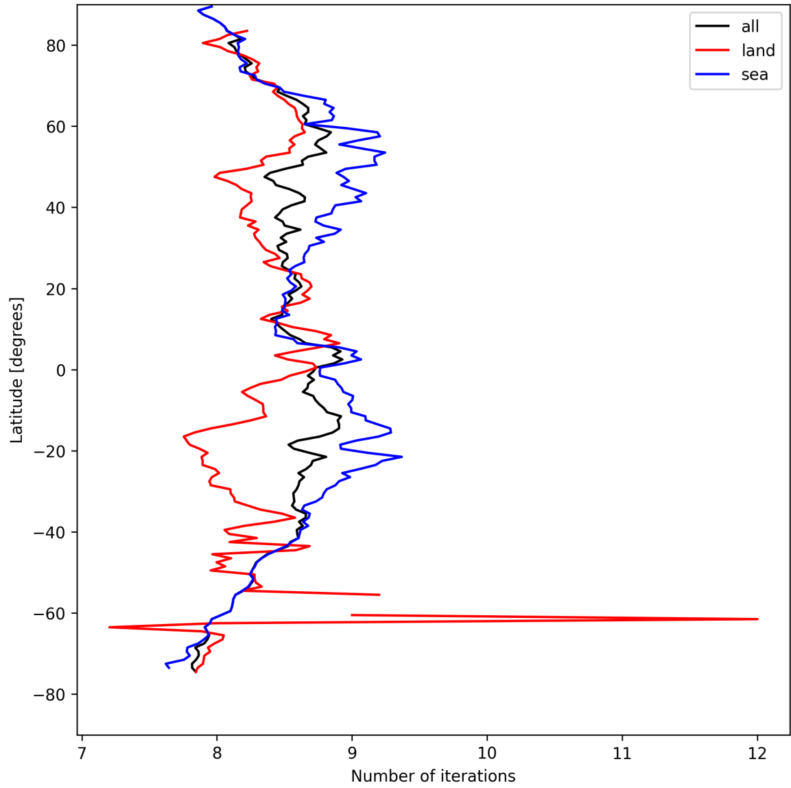
Figure 12: Zonal average of “Number of iterations” for 2025-08-25 to 2025-08-26.
