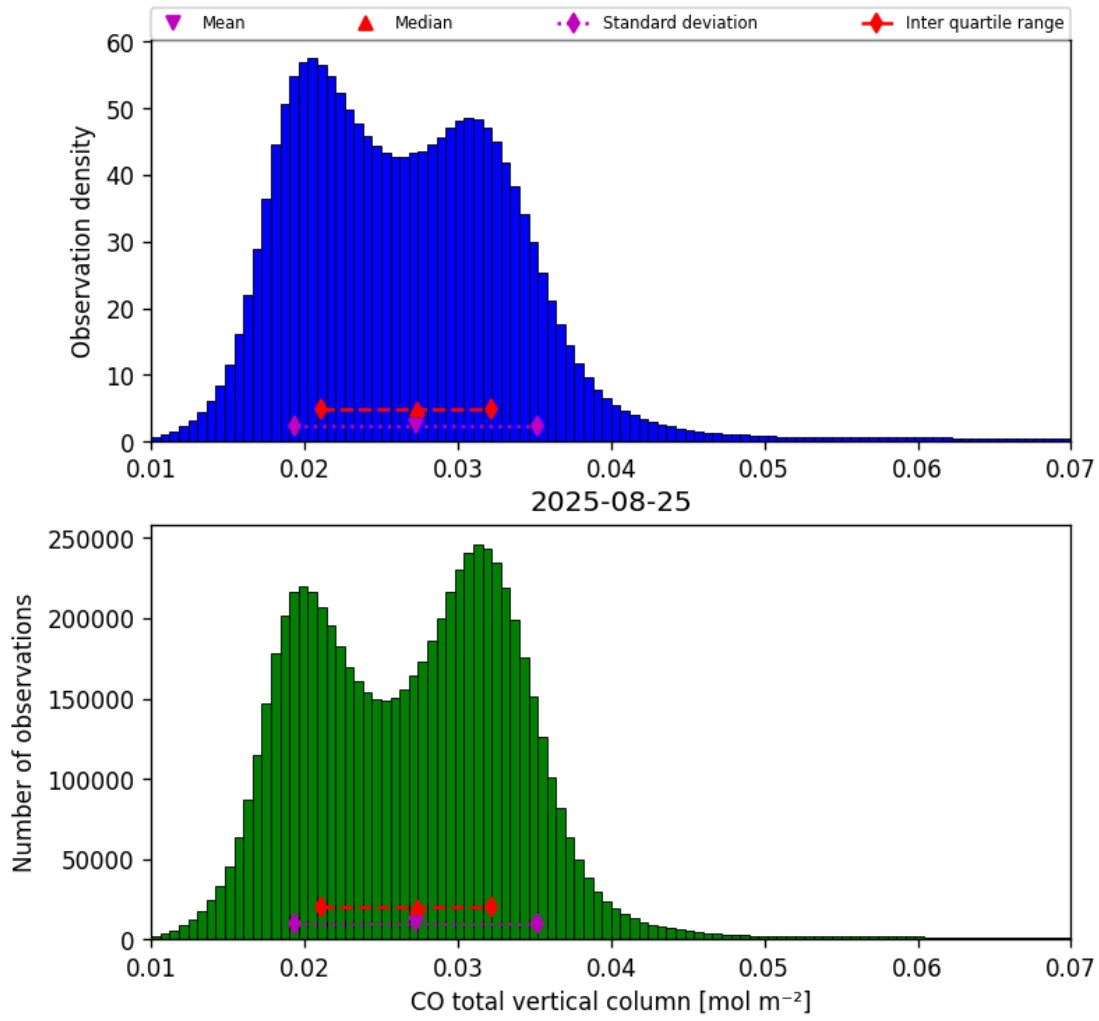
Figure 14: Histogram of “CO total vertical column” for 2025-08-25 to 2025-08-26
