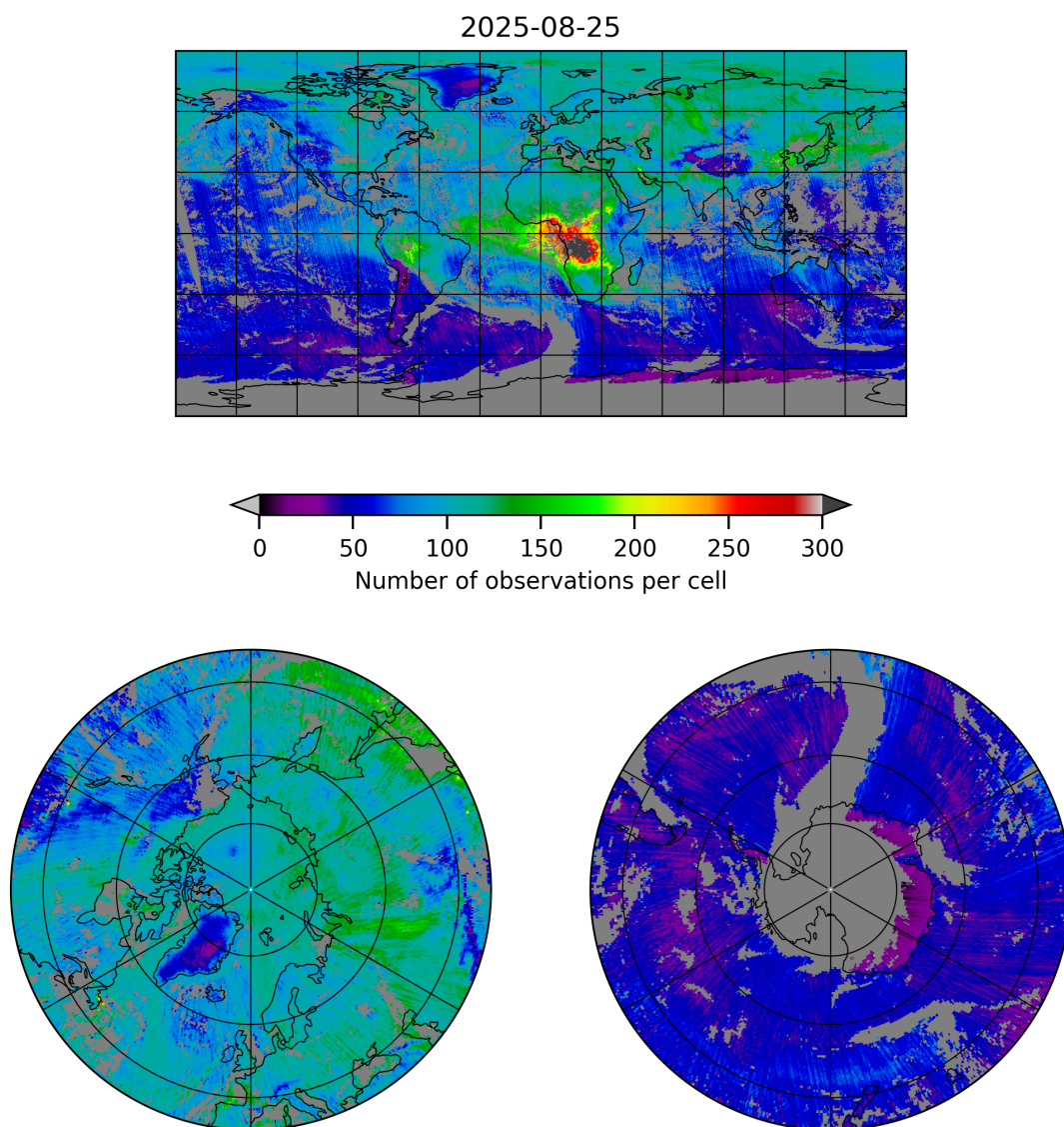
Figure 5: Map of the number of observations for 2025-08-25 to 2025-08-26
