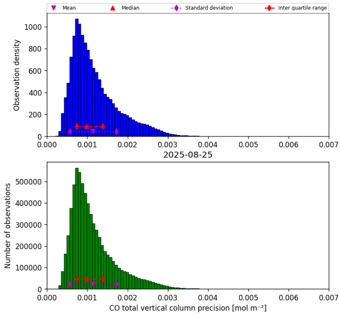
Figure 15: Histogram of “CO total vertical column precision” for 2025-08-25 to 2025-08-26
