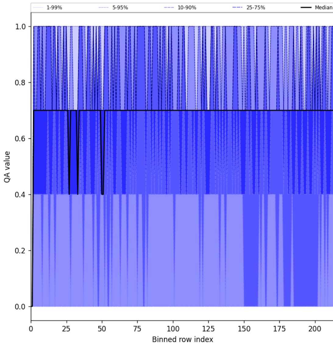
Figure 20: Along track statistics of “QA value” for 2025-08-25 to 2025-08-26
