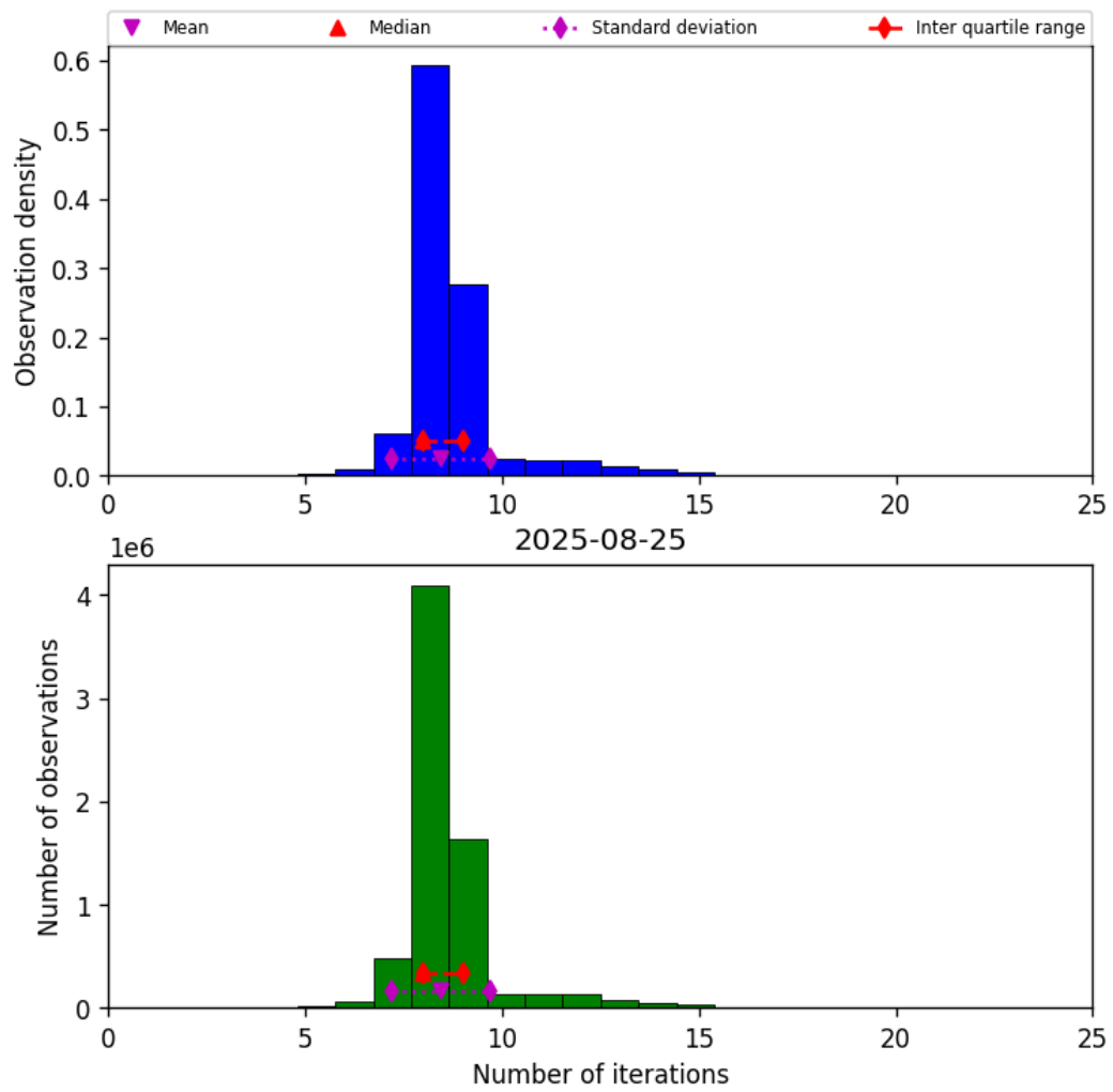
Figure 19: Histogram of “Number of iterations” for 2025-08-25 to 2025-08-26
