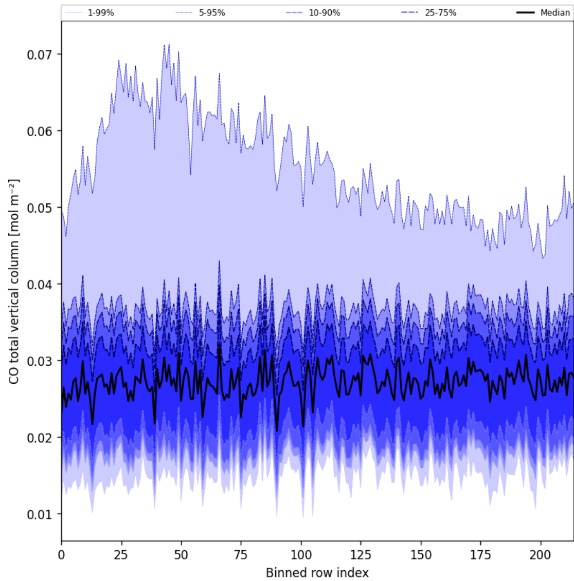
Figure 21: Along track statistics of “CO total vertical column” for 2025-08-26 to 2025-08-27
