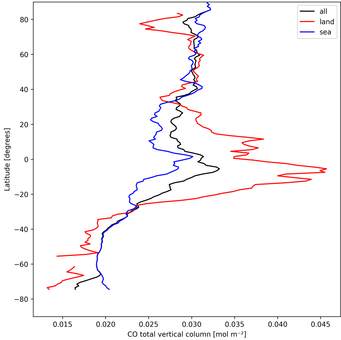
Figure 7: Zonal average of “CO total vertical column” for 2025-08-26 to 2025-08-27.
