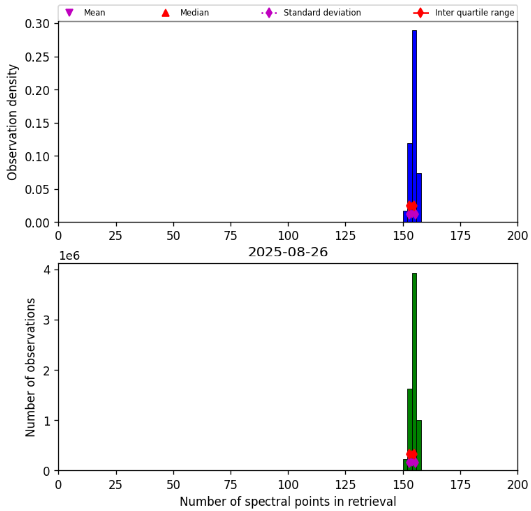
Figure 16: Histogram of "Number of spectral points in retrieval" for 2025-08-26 to 2025-08-27
