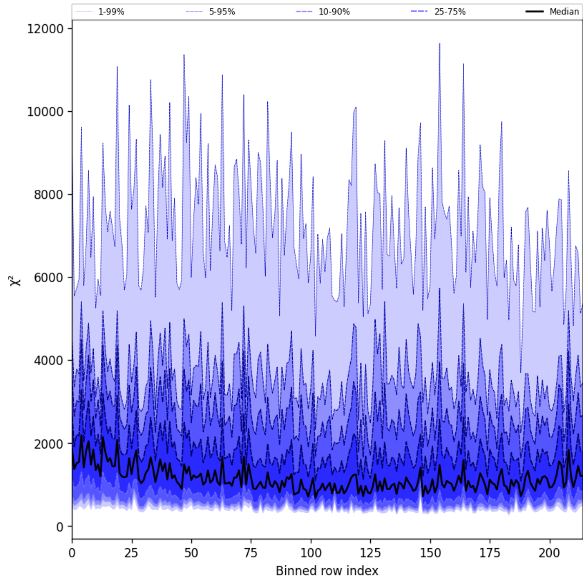
Figure 24: Along track statistics of “ \chi^2 ” for 2025-08-26 to 2025-08-27
