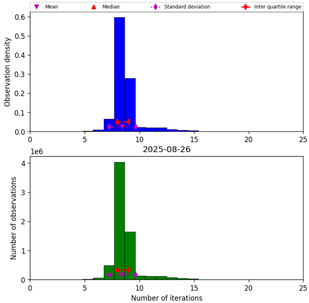
Figure 19: Histogram of “Number of iterations” for 2025-08-26 to 2025-08-27
