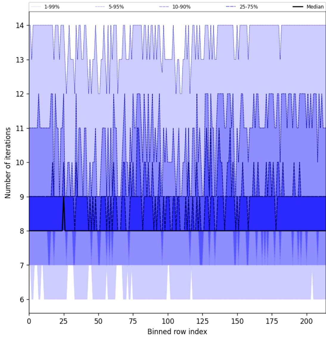
Figure 26: Along track statistics of “Number of iterations” for 2025-08-26 to 2025-08-27
