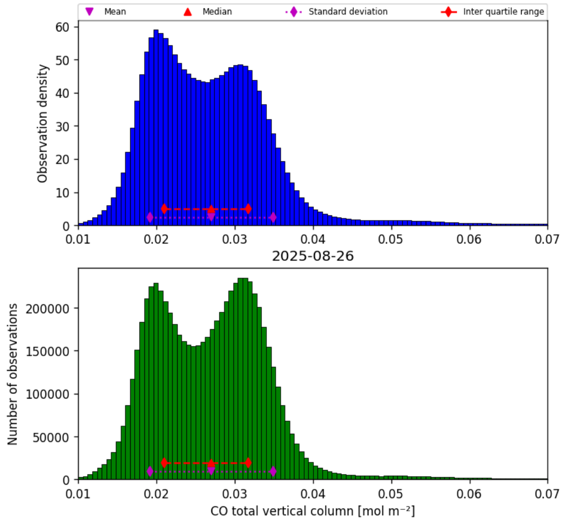
Figure 14: Histogram of “CO total vertical column” for 2025-08-26 to 2025-08-27
