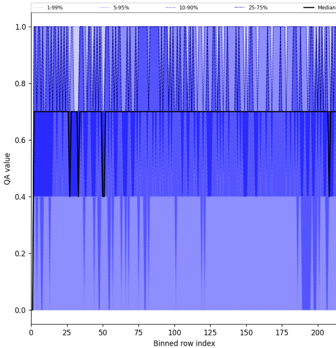
Figure 20: Along track statistics of “QA value” for 2025-08-26 to 2025-08-27
