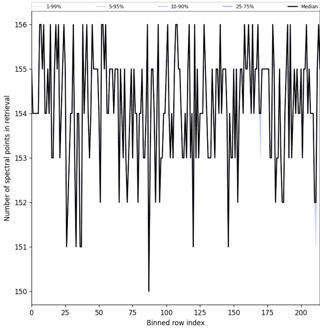
Figure 23: Along track statistics of “Number of spectral points in retrieval” for 2025-08-26 to 2025-08-27
