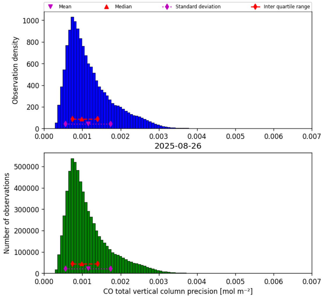
Figure 15: Histogram of “CO total vertical column precision” for 2025-08-26 to 2025-08-27
