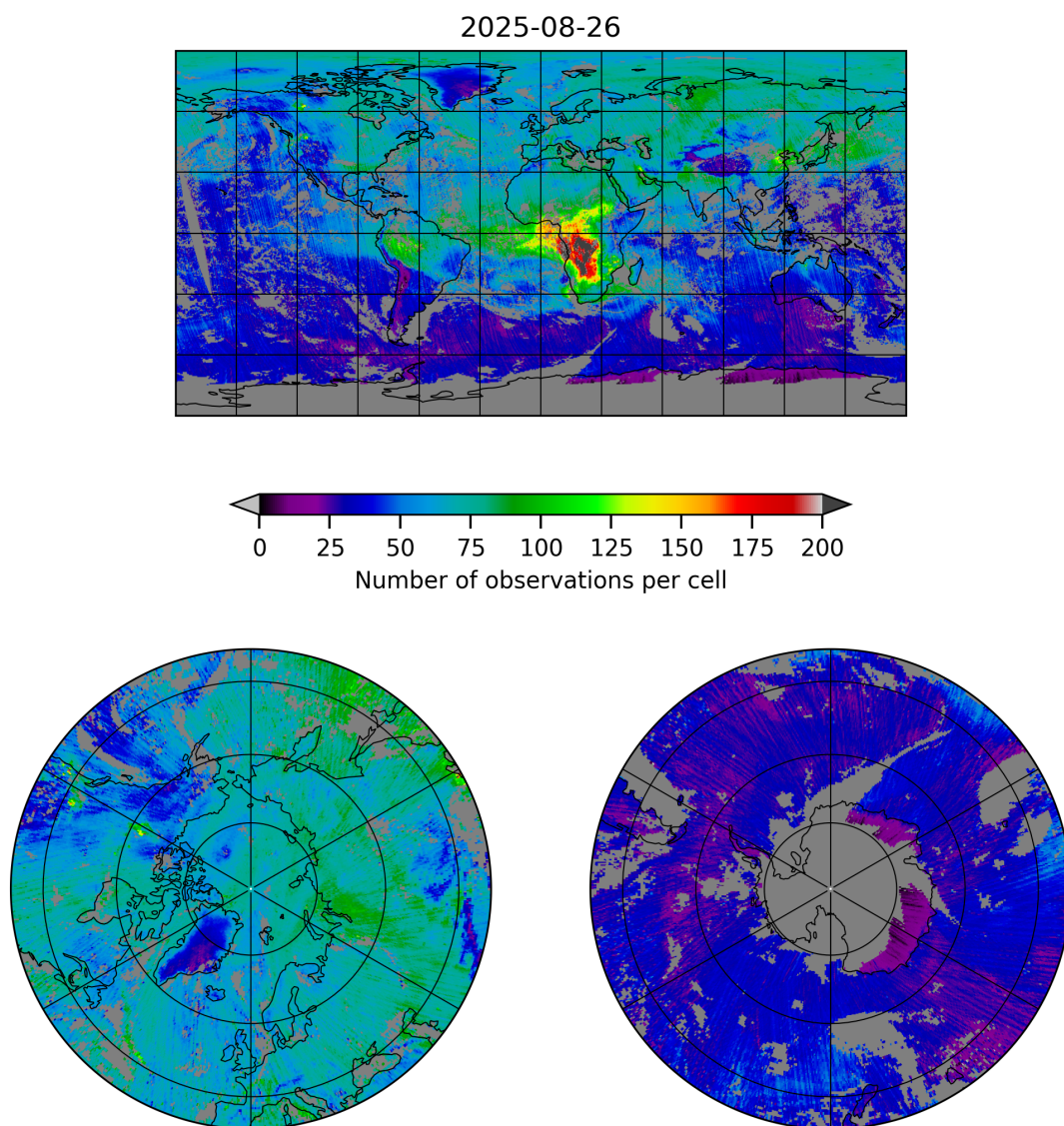
Figure 5: Map of the number of observations for 2025-08-26 to 2025-08-27
