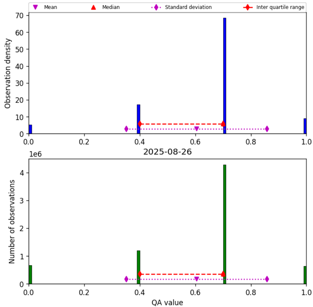
Figure 13: Histogram of “QA value” for 2025-08-26 to 2025-08-27
