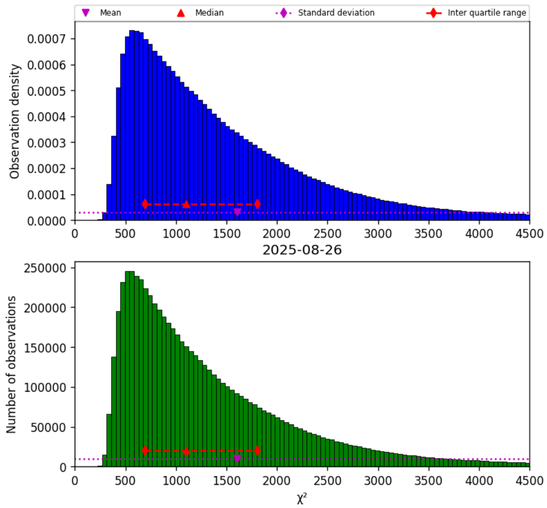
Figure 17: Histogram of " \chi^2 " for 2025-08-26 to 2025-08-27
