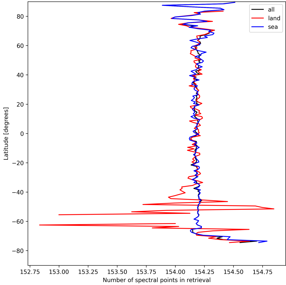
Figure 9: Zonal average of “Number of spectral points in retrieval” for 2025-08-26 to 2025-08-27.
