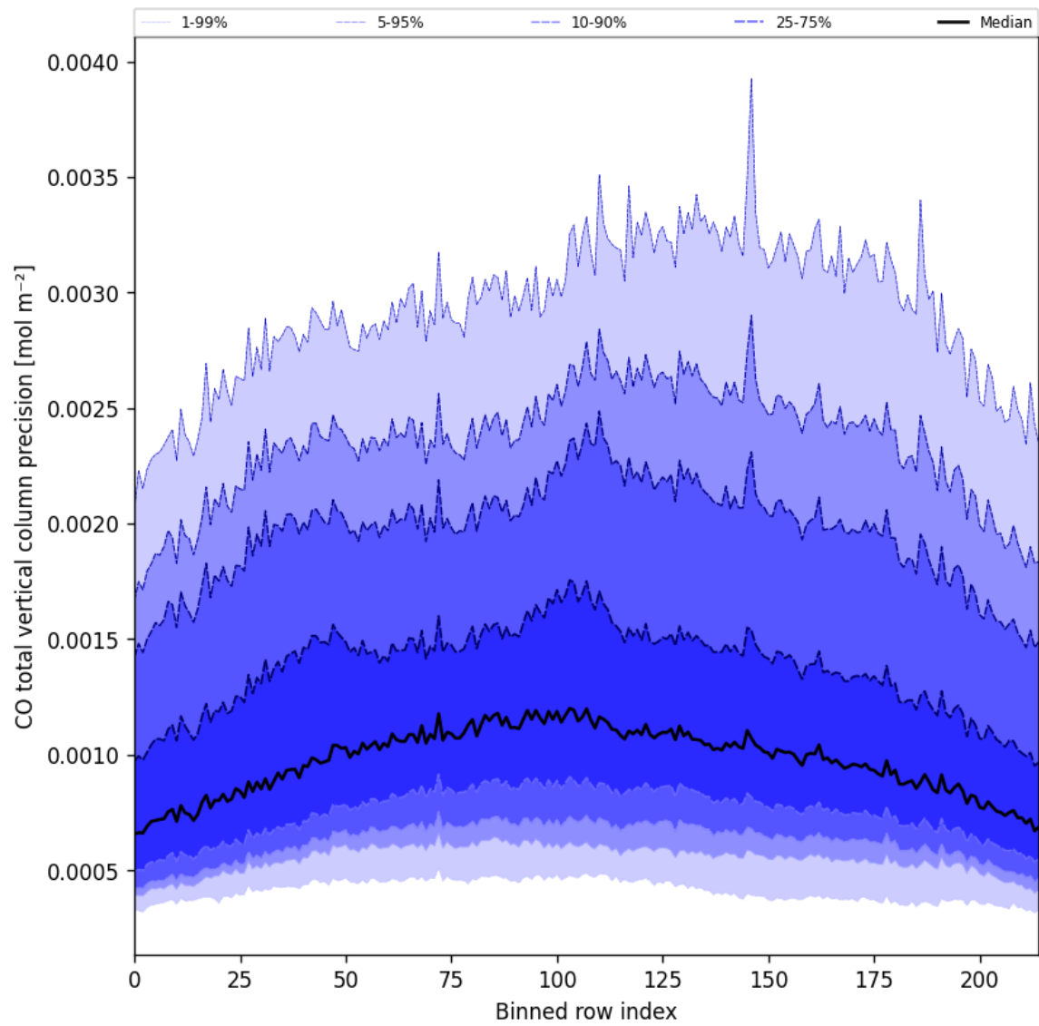
Figure 22: Along track statistics of “CO total vertical column precision” for 2025-08-26 to 2025-08-27
