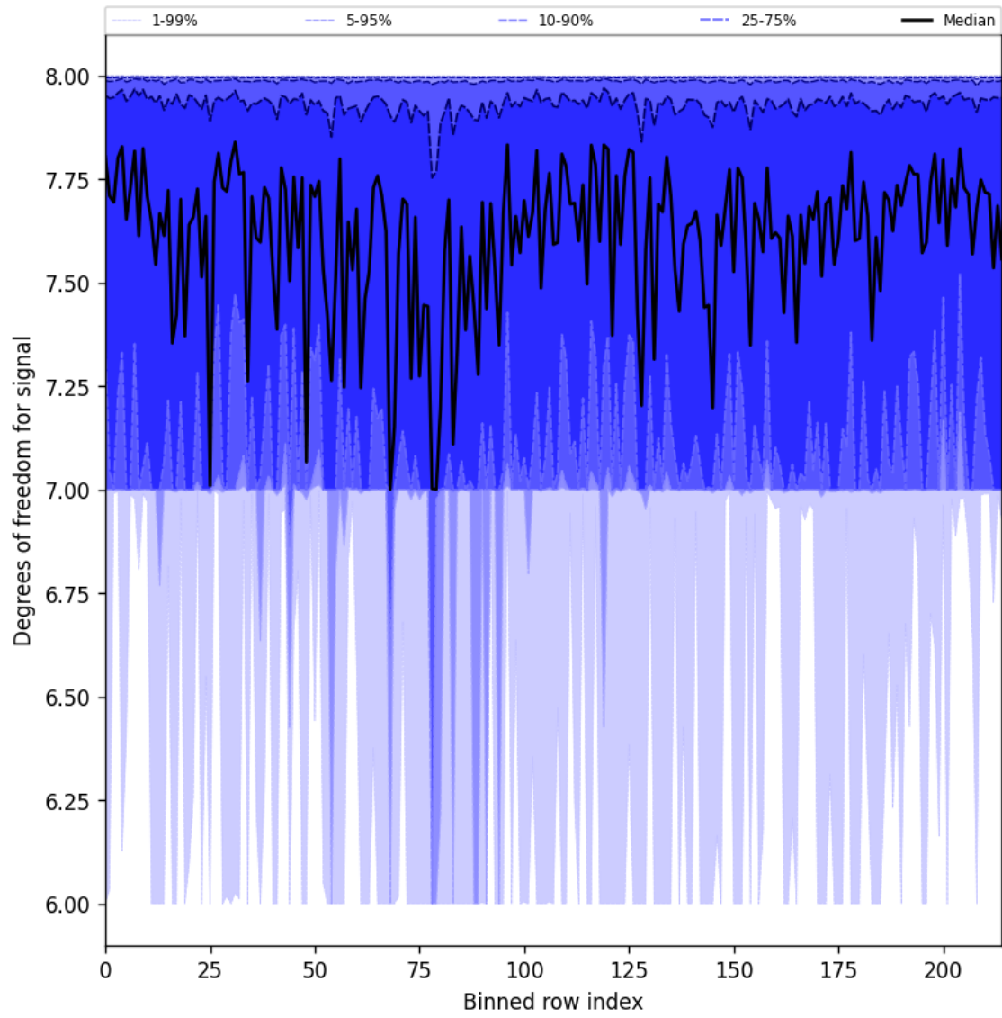
Figure 25: Along track statistics of “Degrees of freedom for signal” for 2025-08-26 to 2025-08-27
