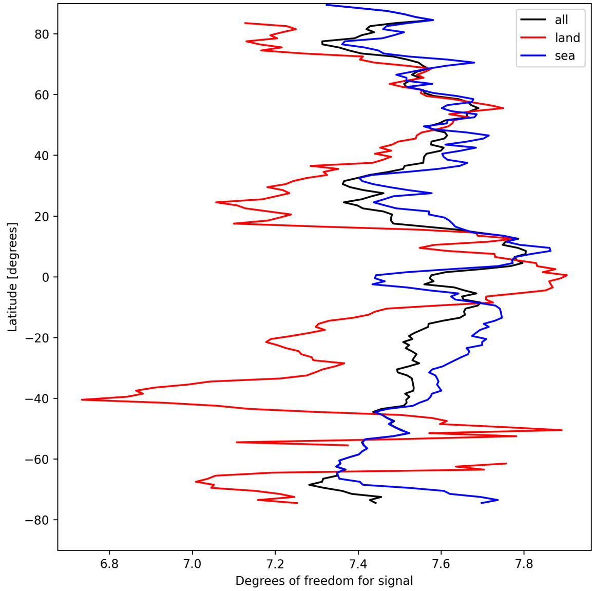
Figure 11: Zonal average of “Degrees of freedom for signal” for 2025-08-26 to 2025-08-27.
