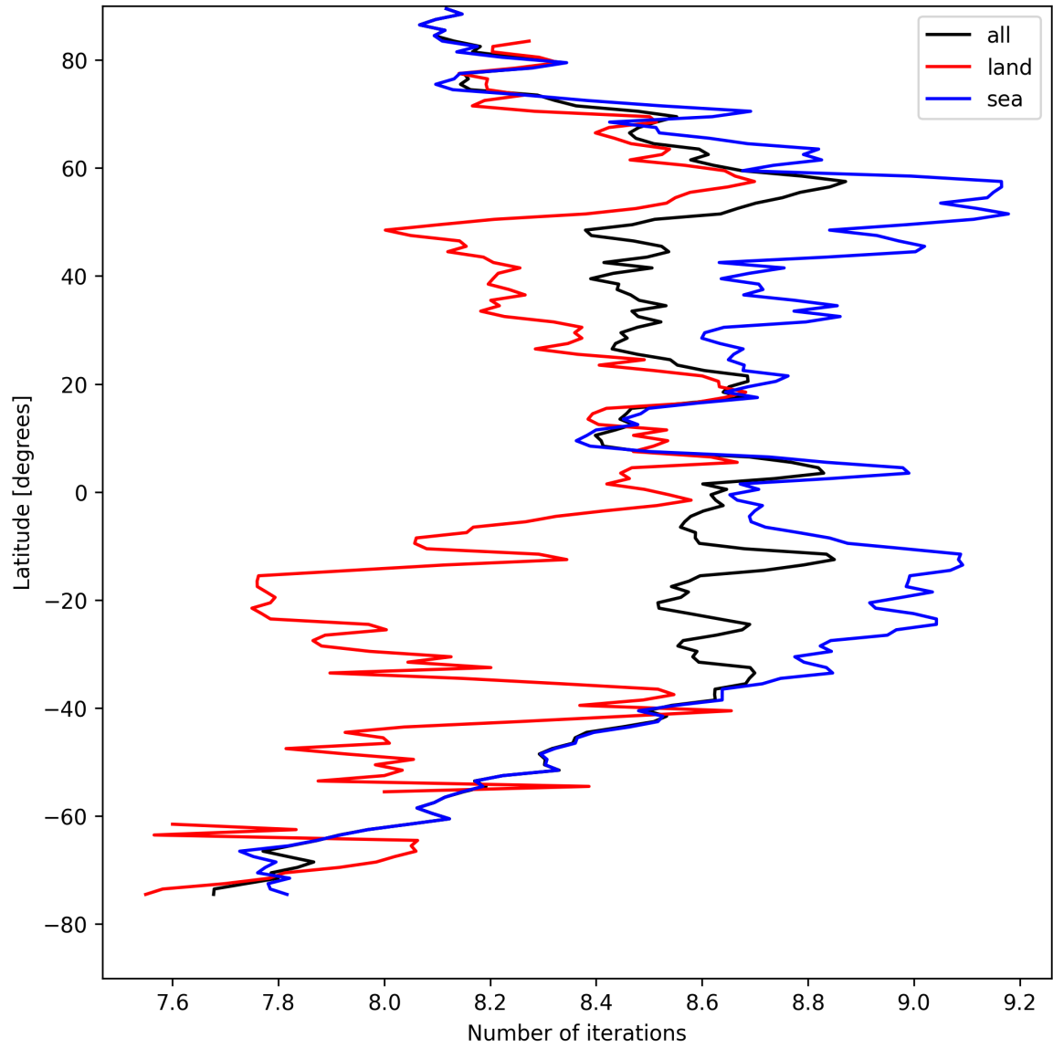
Figure 12: Zonal average of “Number of iterations” for 2025-08-26 to 2025-08-27.
