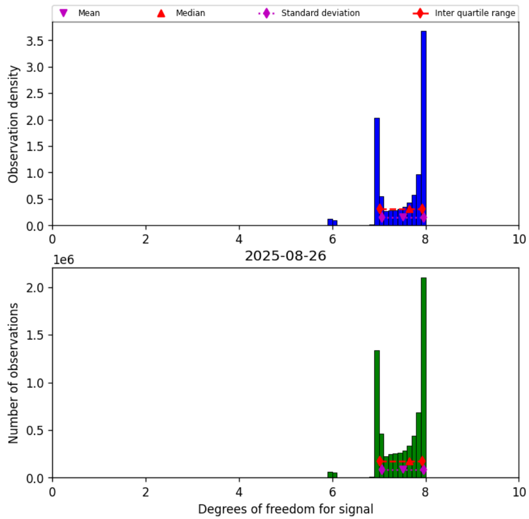
Figure 18: Histogram of “Degrees of freedom for signal” for 2025-08-26 to 2025-08-27
