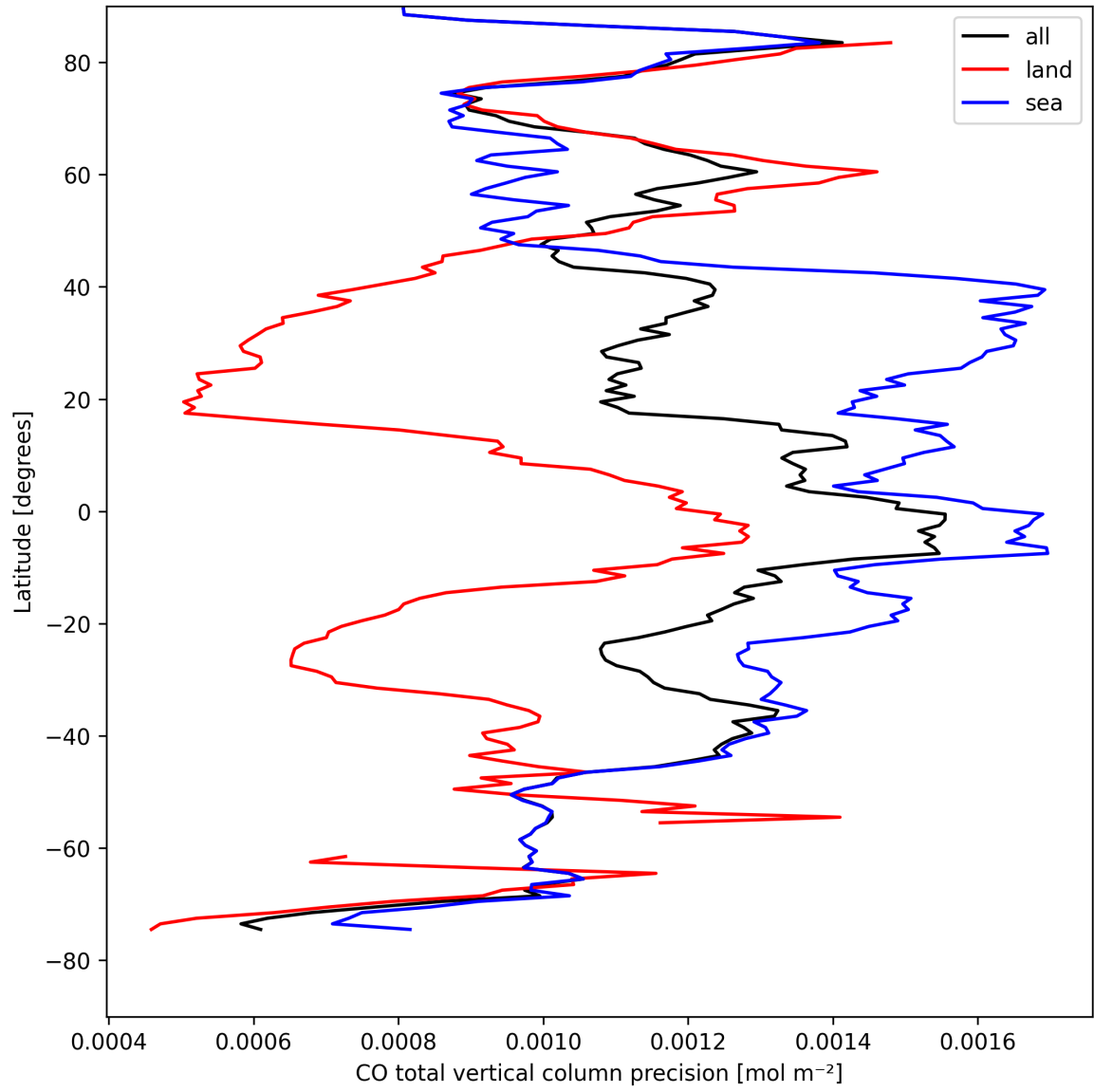
Figure 8: Zonal average of "CO total vertical column precision" for 2025-08-26 to 2025-08-27.
