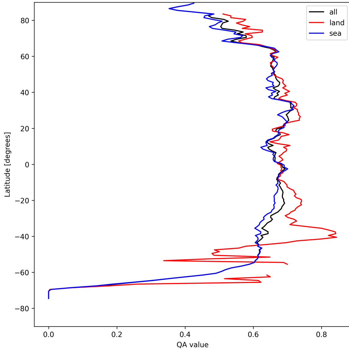
Figure 6: Zonal average of “QA value” for 2025-08-26 to 2025-08-27.
