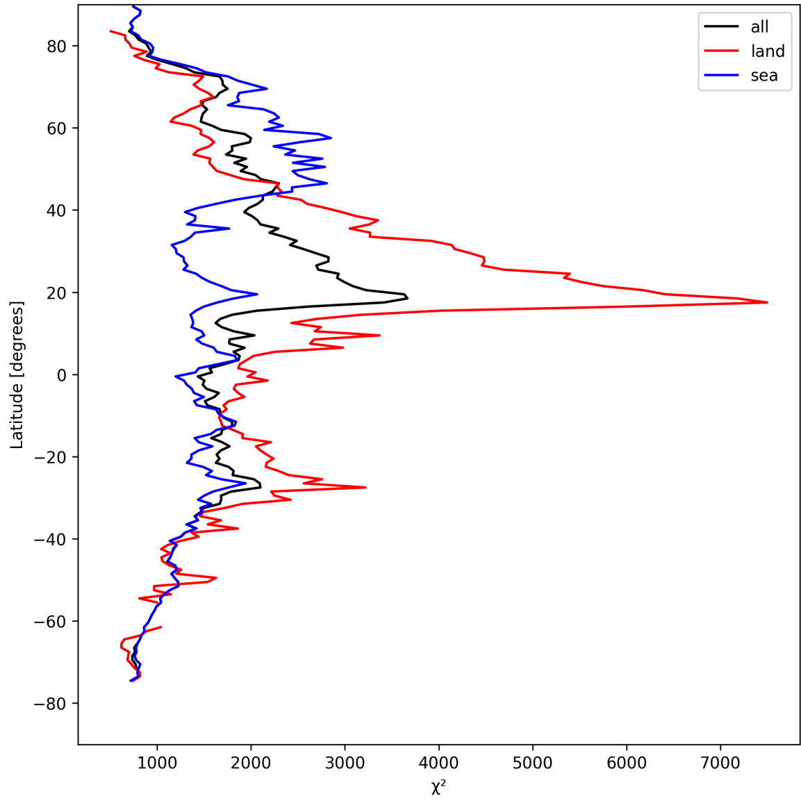
Figure 10: Zonal average of “ \chi^2 ” for 2025-08-26 to 2025-08-27.
