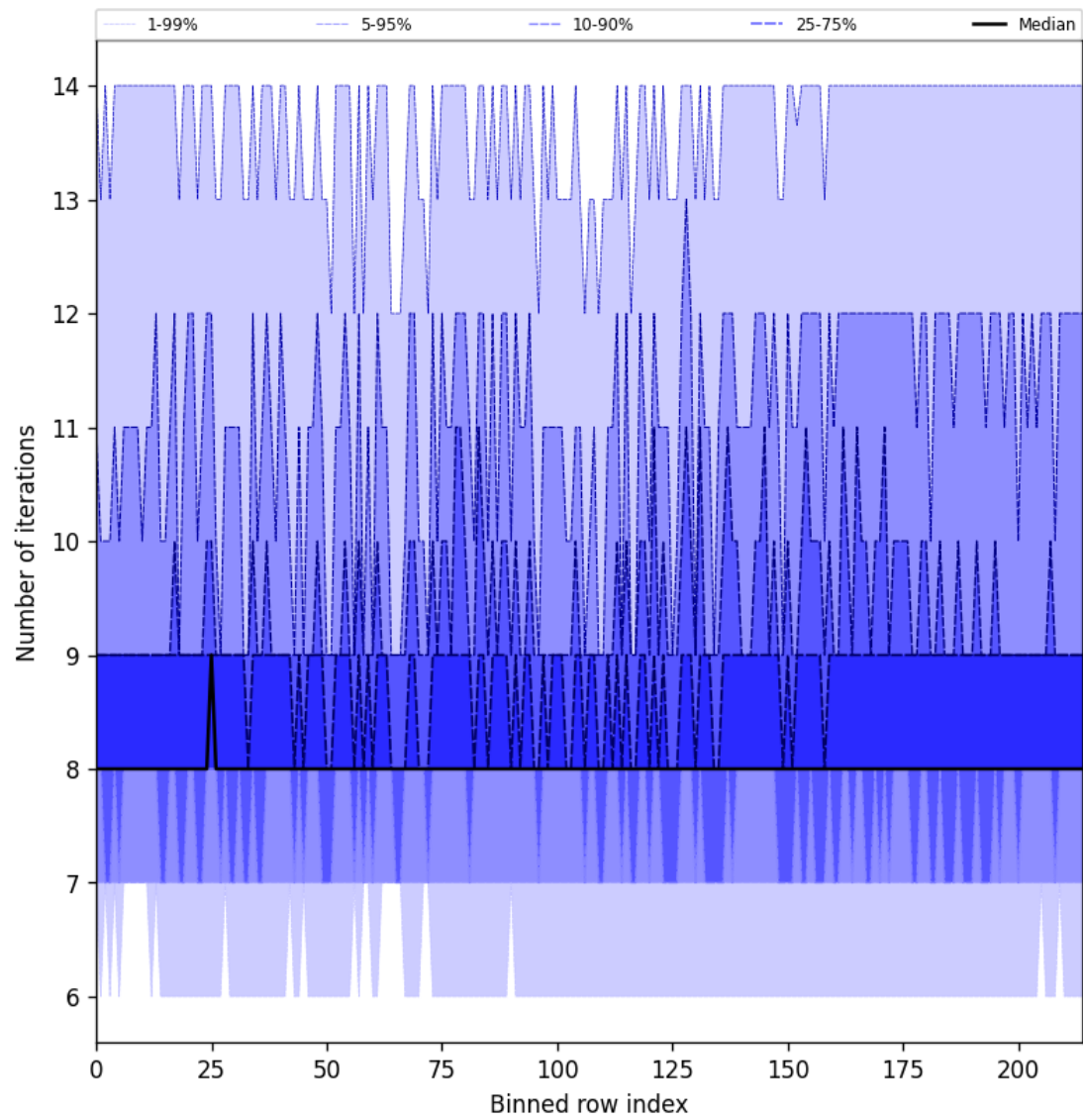
Figure 26: Along track statistics of “Number of iterations” for 2025-08-27 to 2025-08-28
