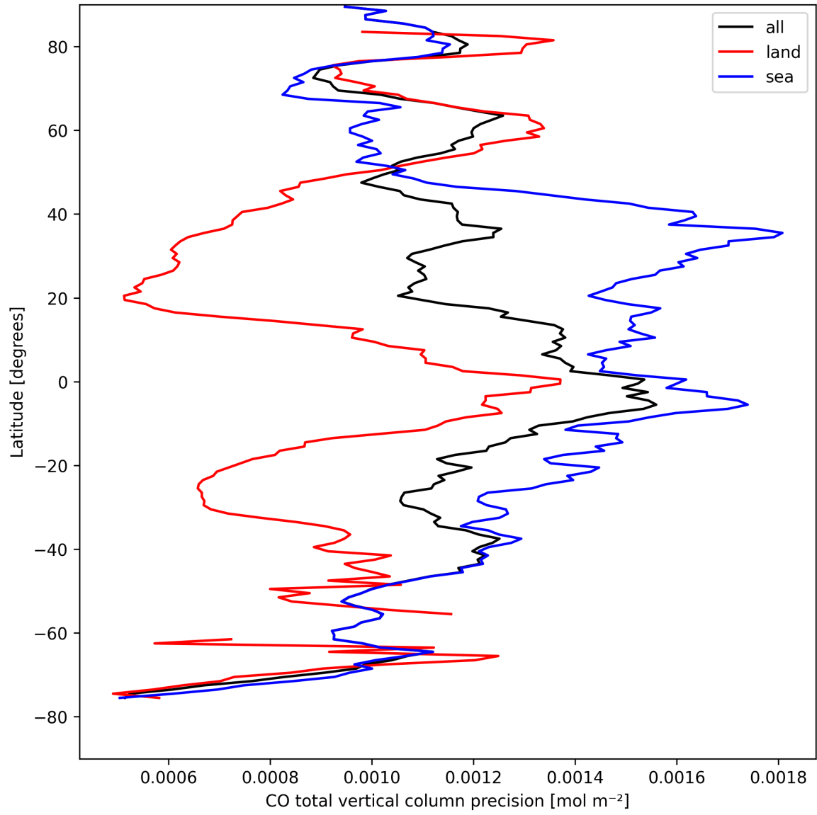
Figure 8: Zonal average of “CO total vertical column precision” for 2025-08-27 to 2025-08-28.
