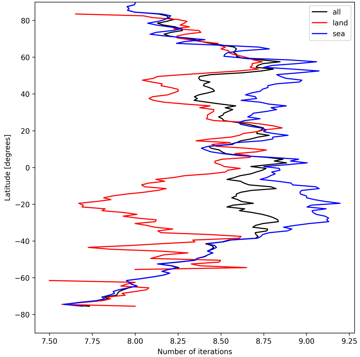
Figure 12: Zonal average of “Number of iterations” for 2025-08-27 to 2025-08-28.
