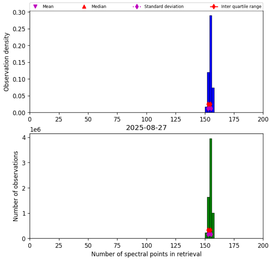
Figure 16: Histogram of “Number of spectral points in retrieval” for 2025-08-27 to 2025-08-28
