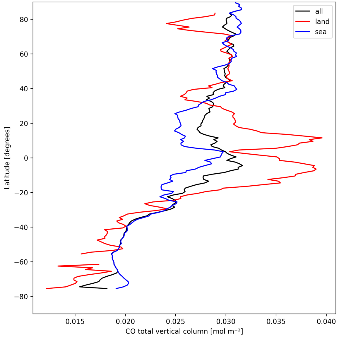
Figure 7: Zonal average of “CO total vertical column” for 2025-08-27 to 2025-08-28.
