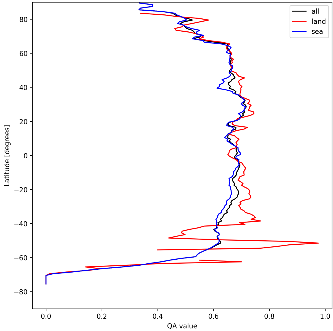
Figure 6: Zonal average of “QA value” for 2025-08-27 to 2025-08-28.
