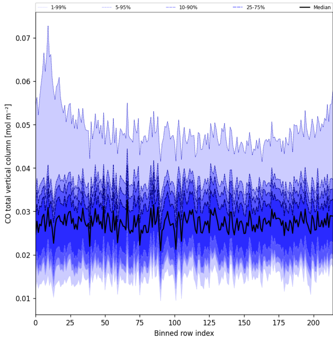
Figure 21: Along track statistics of “CO total vertical column” for 2025-08-27 to 2025-08-28
