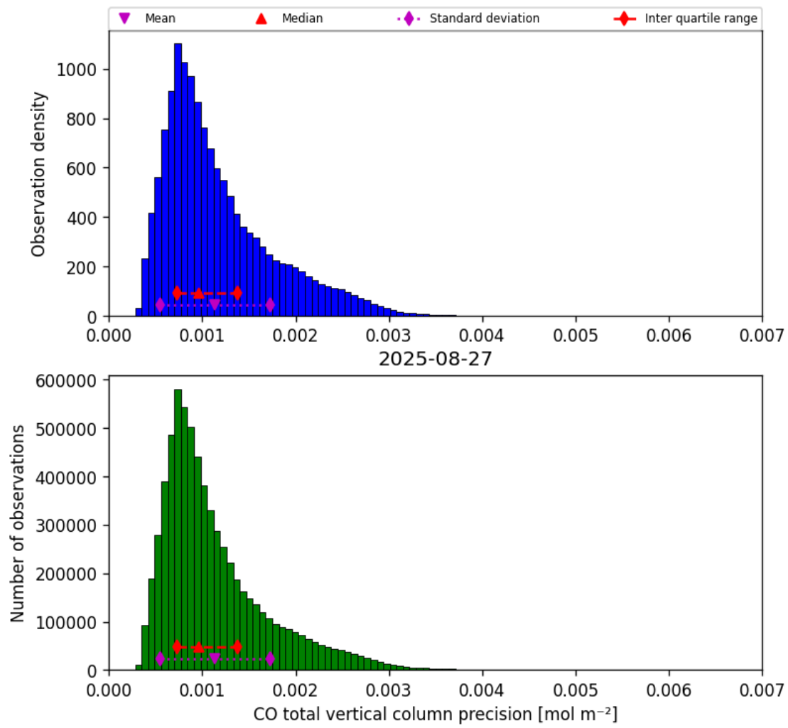
Figure 15: Histogram of “CO total vertical column precision” for 2025-08-27 to 2025-08-28
