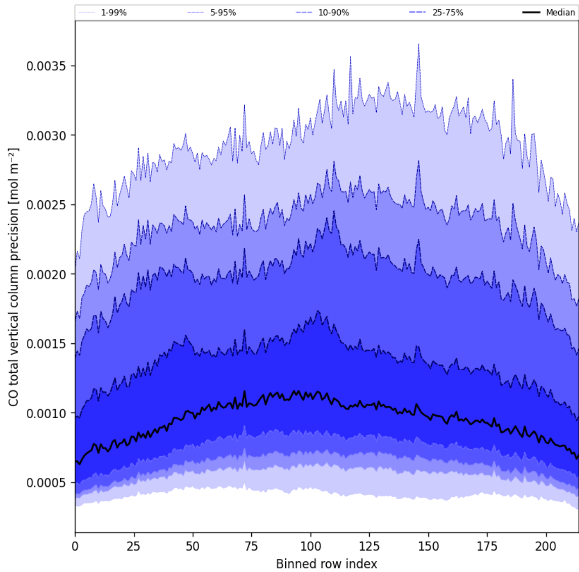
Figure 22: Along track statistics of “CO total vertical column precision” for 2025-08-27 to 2025-08-28
