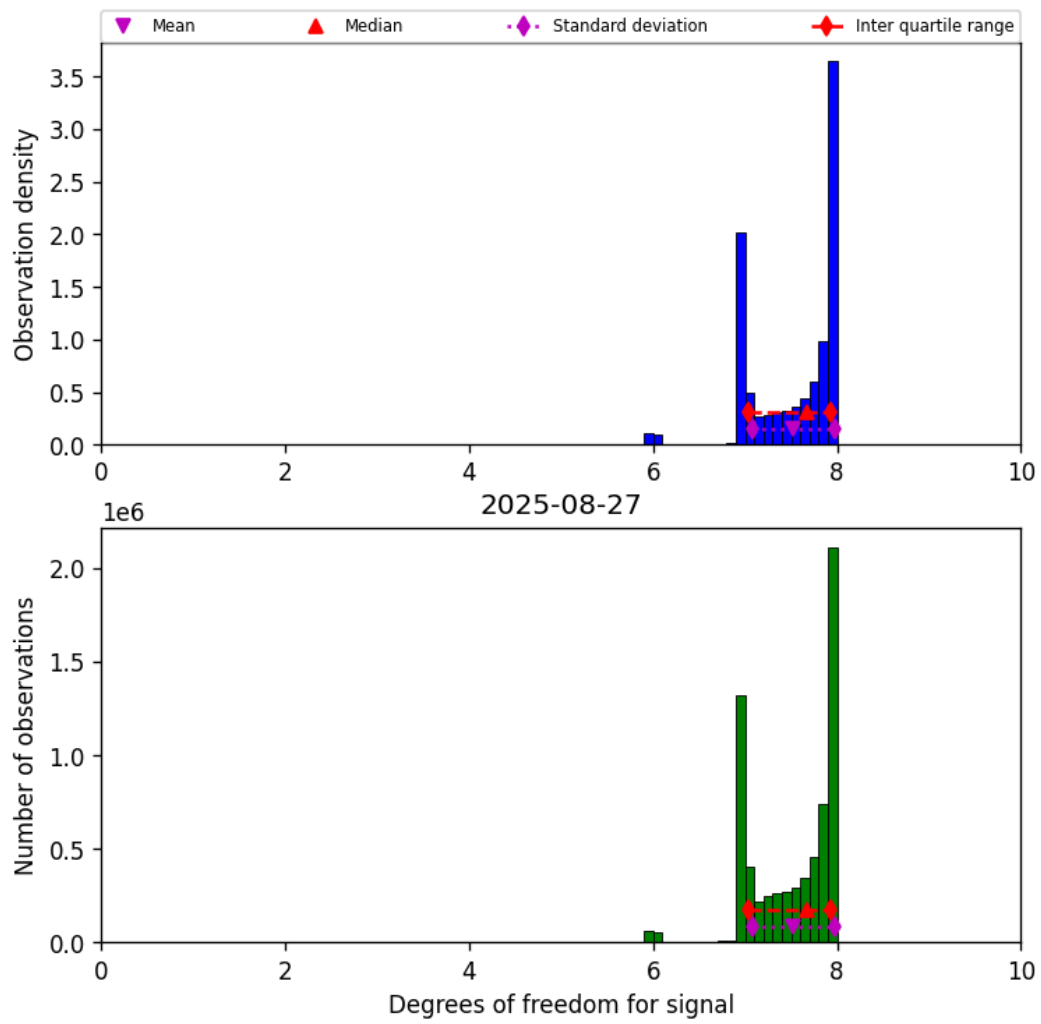
Figure 18: Histogram of “Degrees of freedom for signal” for 2025-08-27 to 2025-08-28
