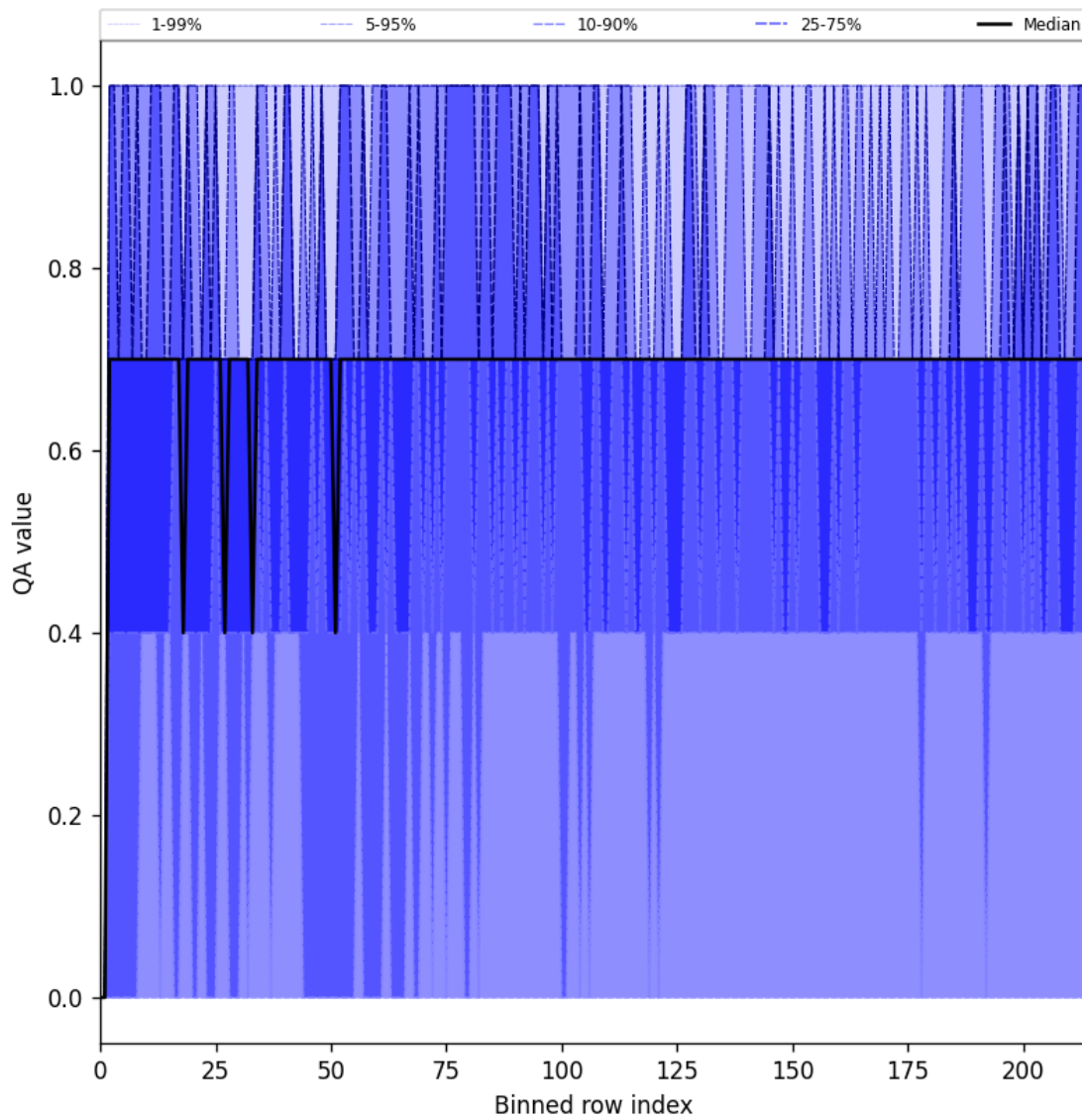
Figure 20: Along track statistics of “QA value” for 2025-08-27 to 2025-08-28
