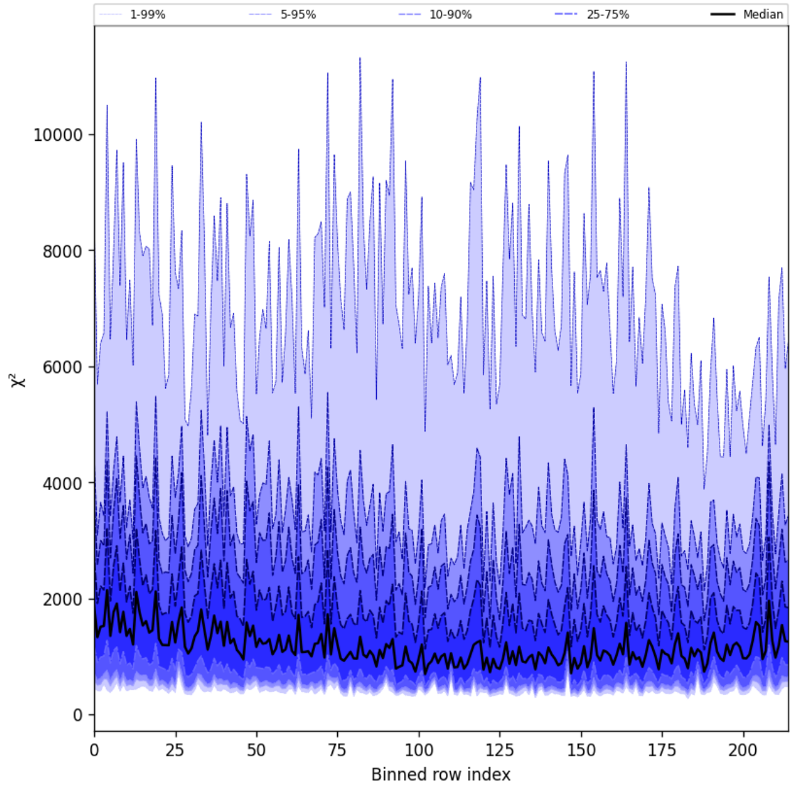
Figure 24: Along track statistics of “ \chi^2 ” for 2025-08-27 to 2025-08-28
