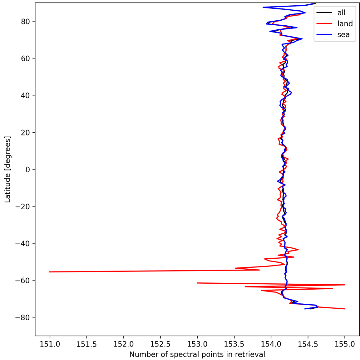
Figure 9: Zonal average of “Number of spectral points in retrieval” for 2025-08-27 to 2025-08-28.
