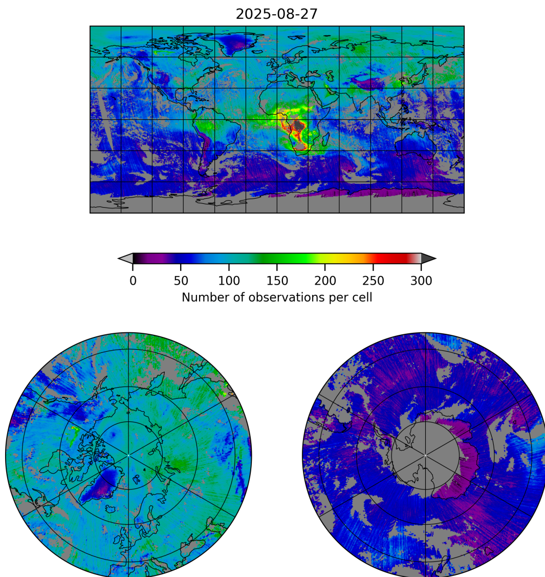
Figure 5: Map of the number of observations for 2025-08-27 to 2025-08-28
