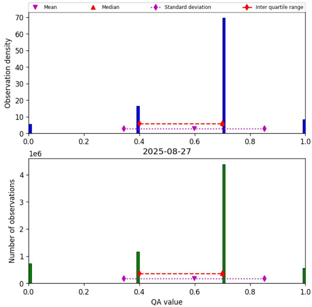
Figure 13: Histogram of “QA value” for 2025-08-27 to 2025-08-28
