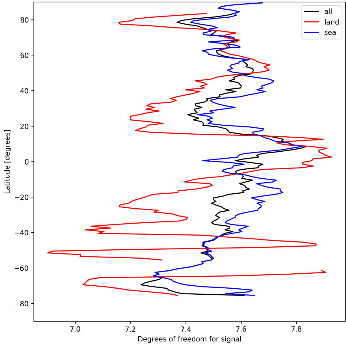
Figure 11: Zonal average of “Degrees of freedom for signal” for 2025-08-27 to 2025-08-28.
