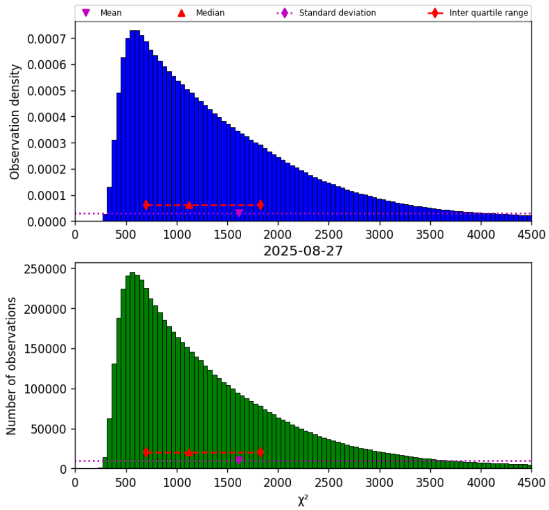
Figure 17: Histogram of “ \chi^2 ” for 2025-08-27 to 2025-08-28
