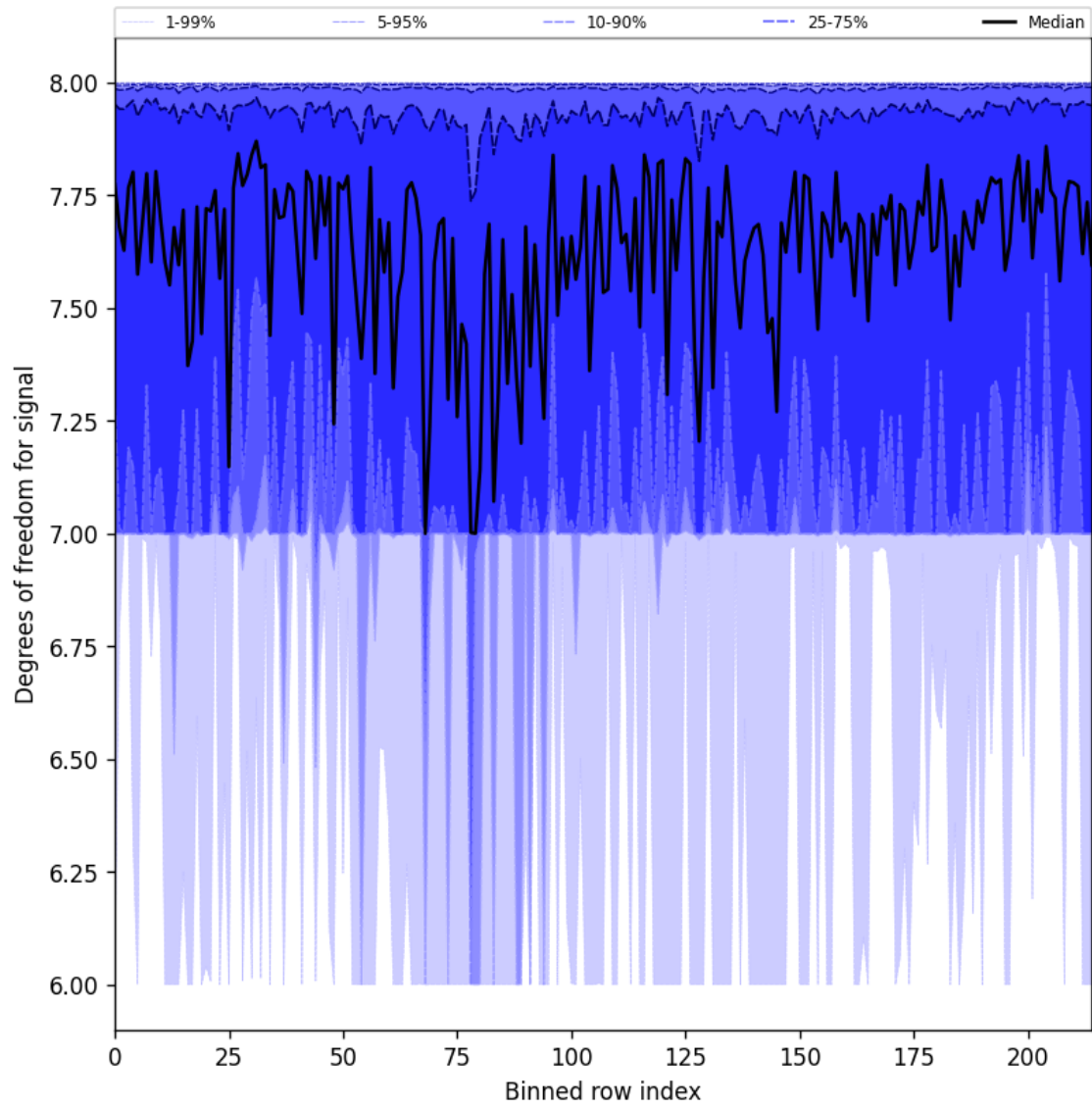
Figure 25: Along track statistics of “Degrees of freedom for signal” for 2025-08-27 to 2025-08-28
