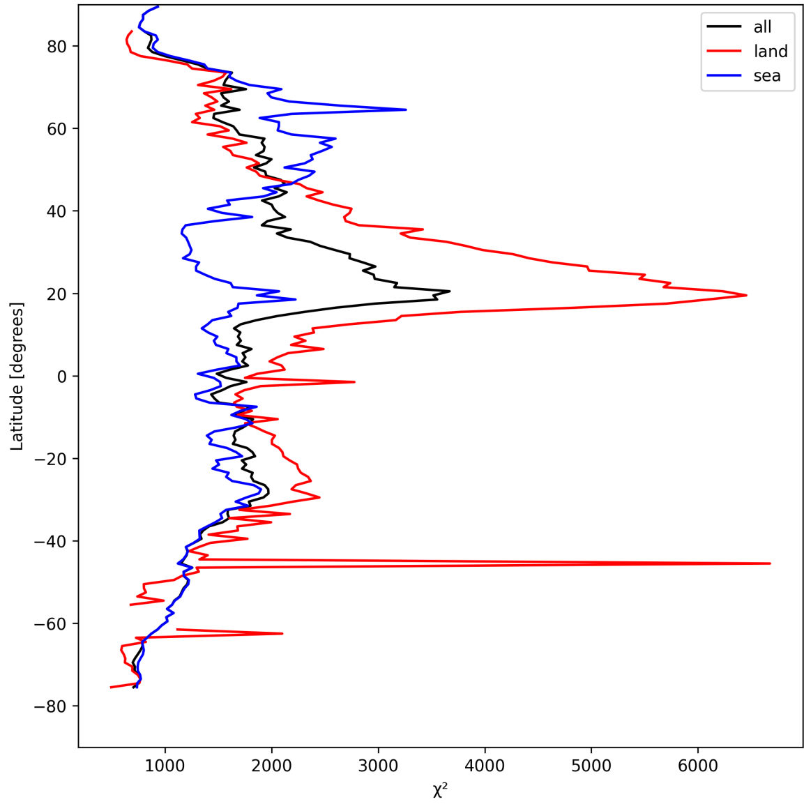
Figure 10: Zonal average of “ \chi^2 ” for 2025-08-27 to 2025-08-28.
