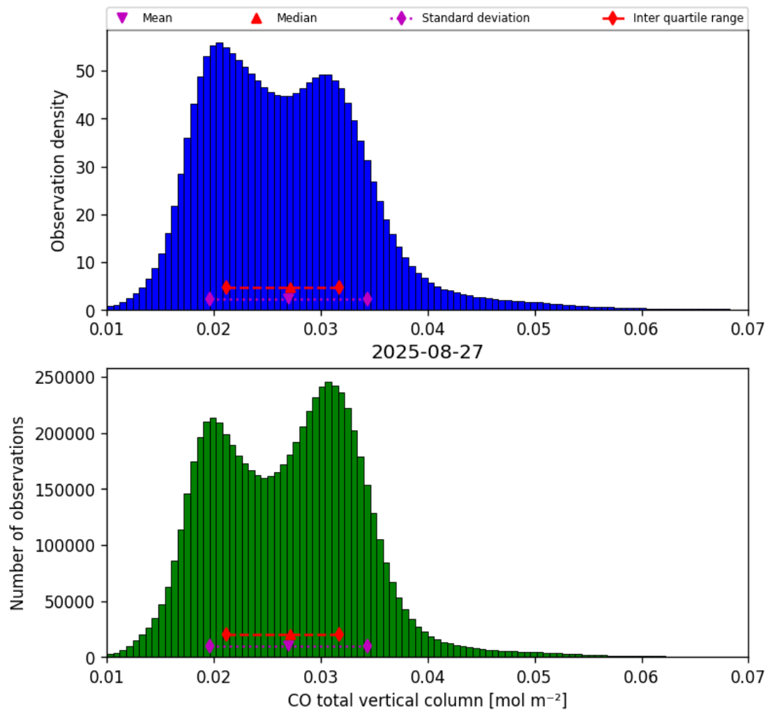
Figure 14: Histogram of “CO total vertical column” for 2025-08-27 to 2025-08-28
