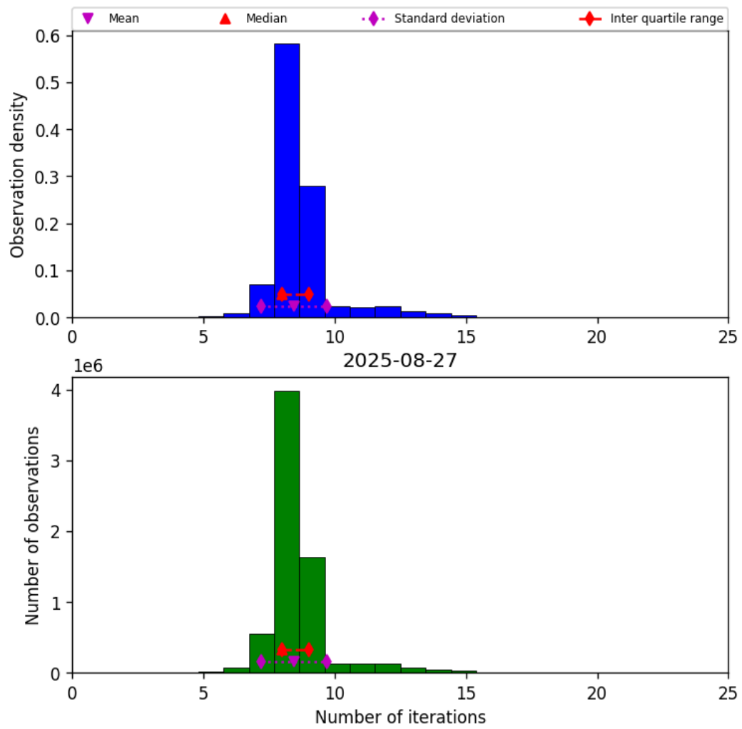
Figure 19: Histogram of “Number of iterations” for 2025-08-27 to 2025-08-28
