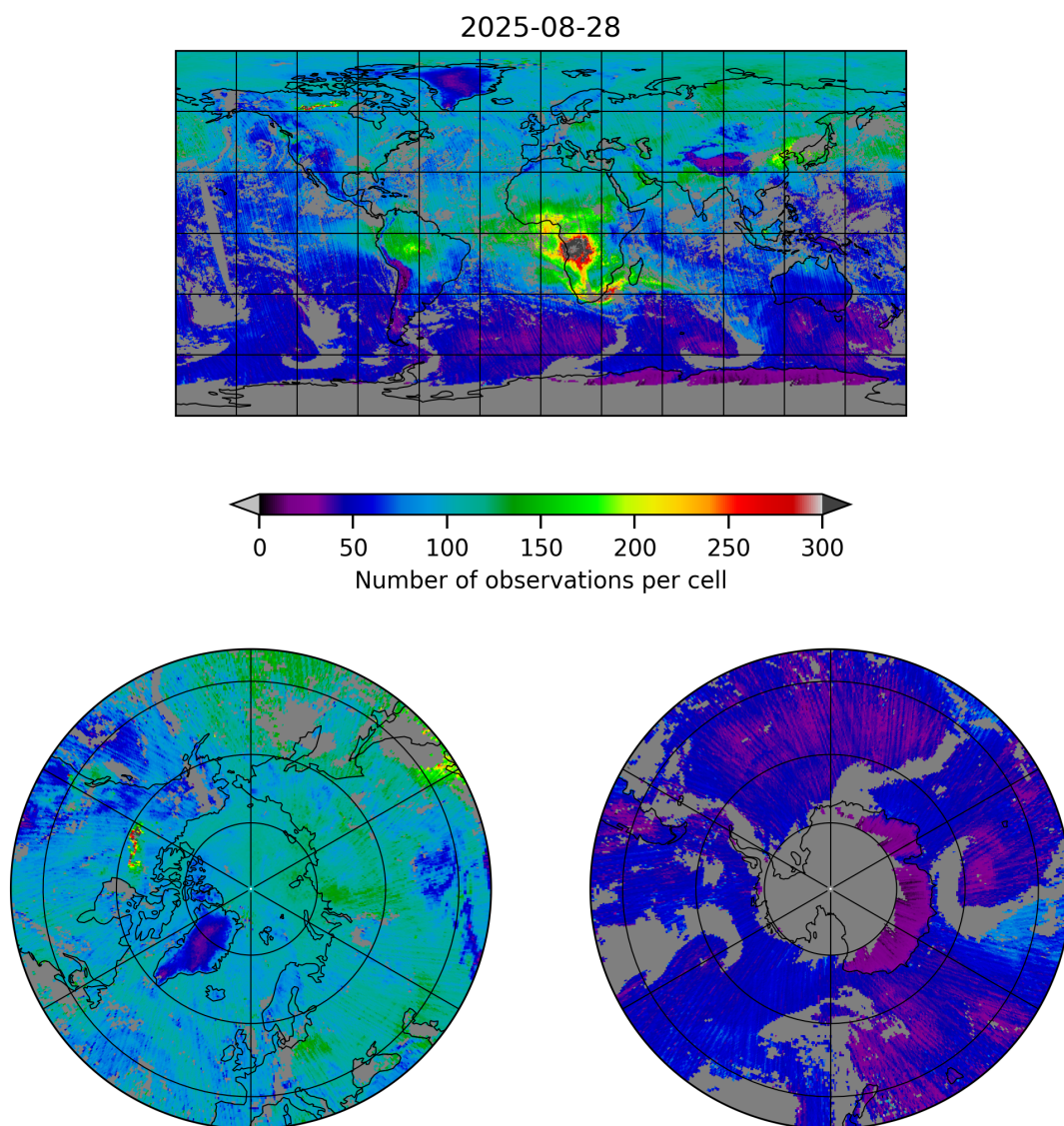
Figure 5: Map of the number of observations for 2025-08-28 to 2025-08-28
