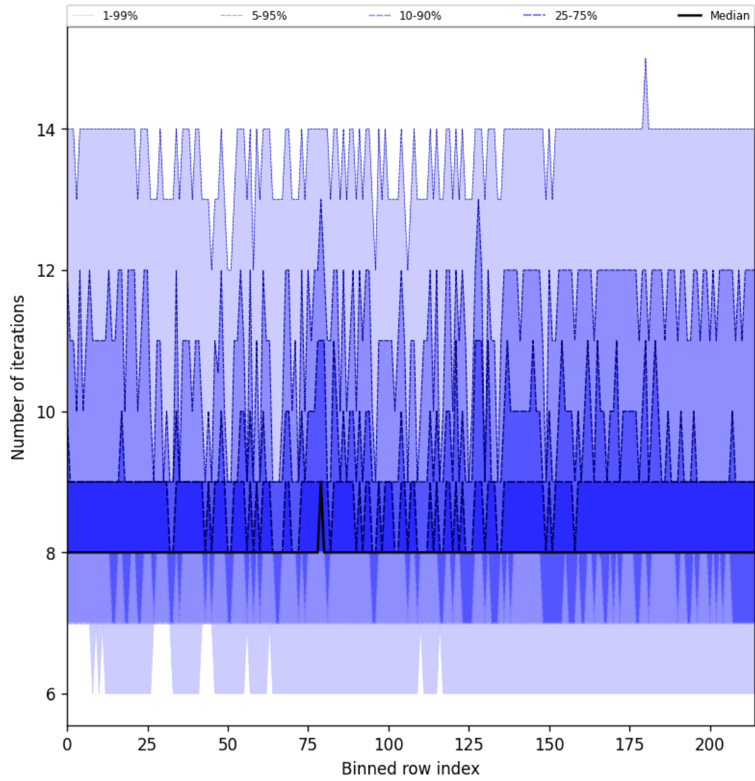
Figure 26: Along track statistics of “Number of iterations” for 2025-08-28 to 2025-08-28
