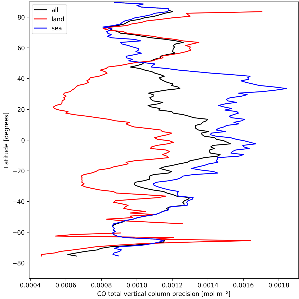
Figure 8: Zonal average of “CO total vertical column precision” for 2025-08-28 to 2025-08-28.
