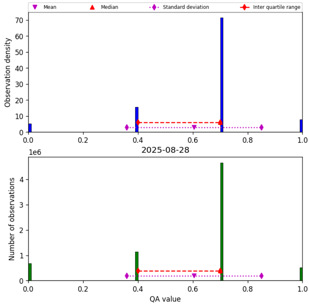
Figure 13: Histogram of “QA value” for 2025-08-28 to 2025-08-28
