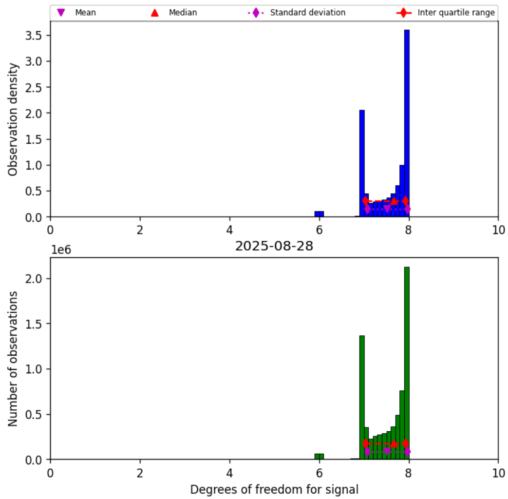
Figure 18: Histogram of “Degrees of freedom for signal” for 2025-08-28 to 2025-08-28
