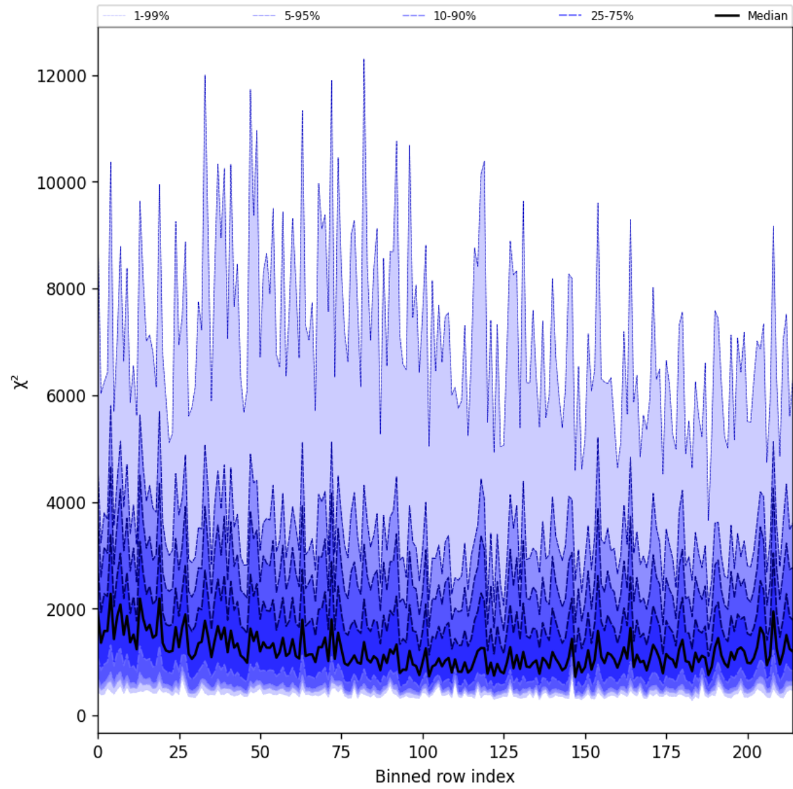
Figure 24: Along track statistics of “ \chi^2 ” for 2025-08-28 to 2025-08-28
