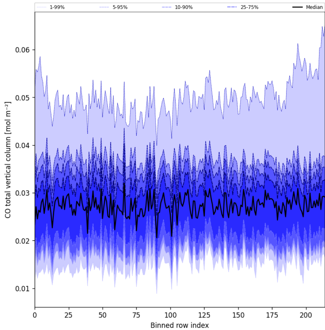
Figure 21: Along track statistics of “CO total vertical column” for 2025-08-28 to 2025-08-28
