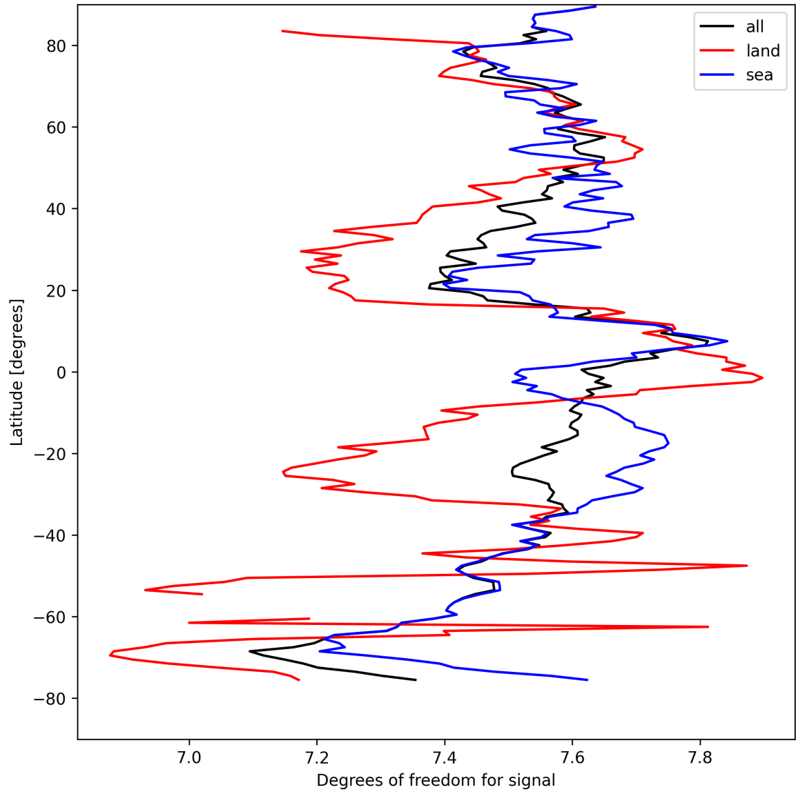
Figure 11: Zonal average of “Degrees of freedom for signal” for 2025-08-28 to 2025-08-28.
