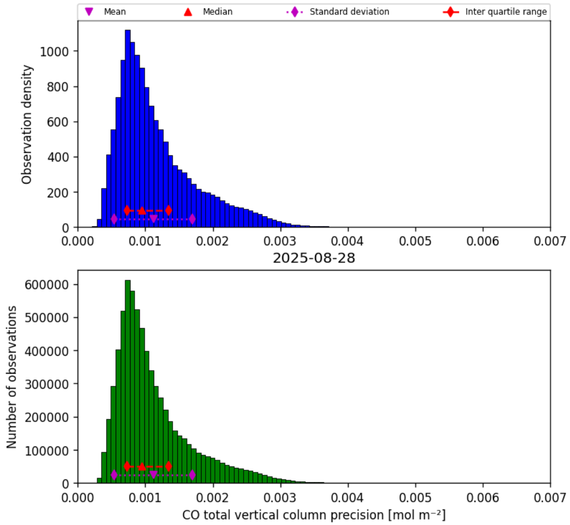
Figure 15: Histogram of “CO total vertical column precision” for 2025-08-28 to 2025-08-28
