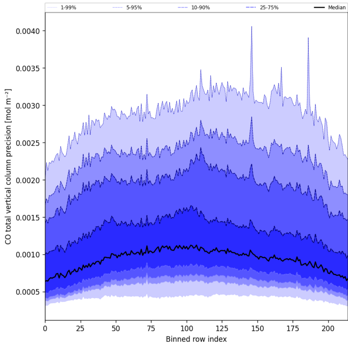
Figure 22: Along track statistics of “CO total vertical column precision” for 2025-08-28 to 2025-08-28
