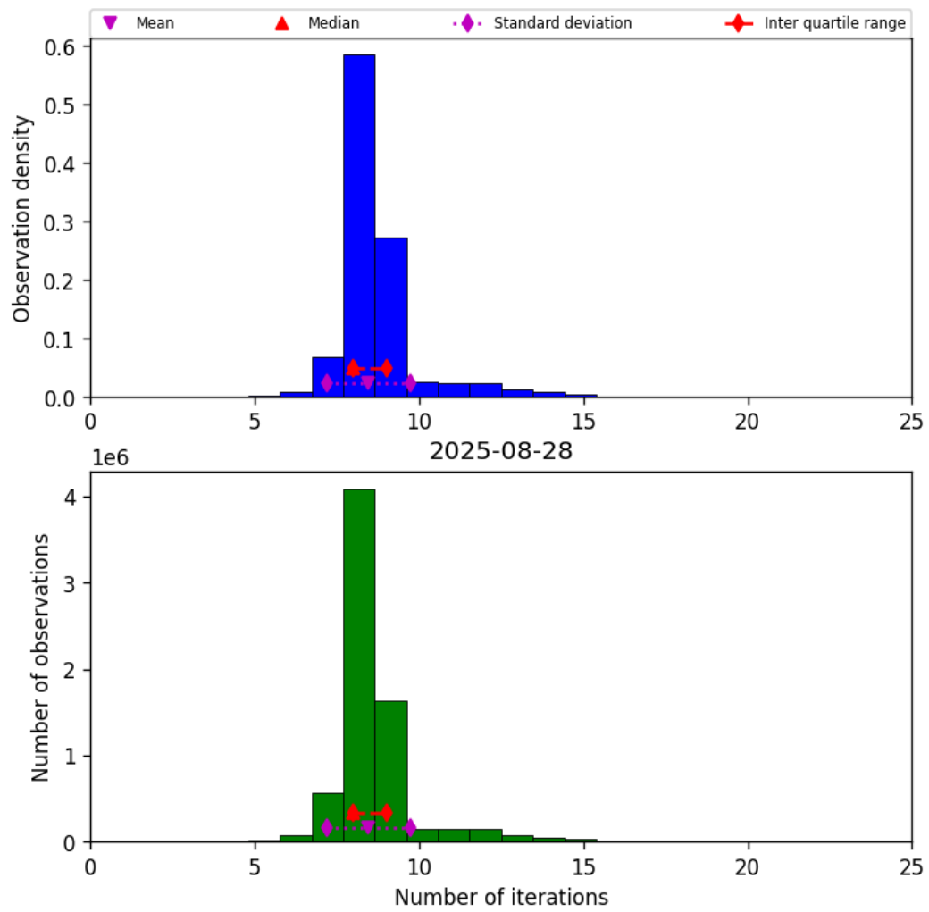
Figure 19: Histogram of “Number of iterations” for 2025-08-28 to 2025-08-28
