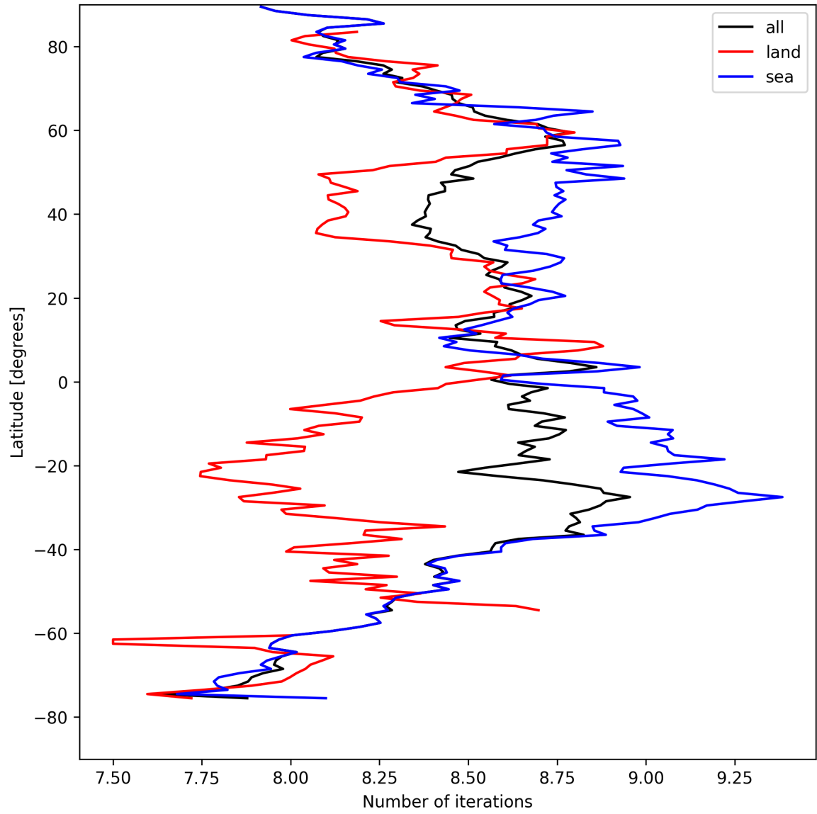
Figure 12: Zonal average of “Number of iterations” for 2025-08-28 to 2025-08-28.
