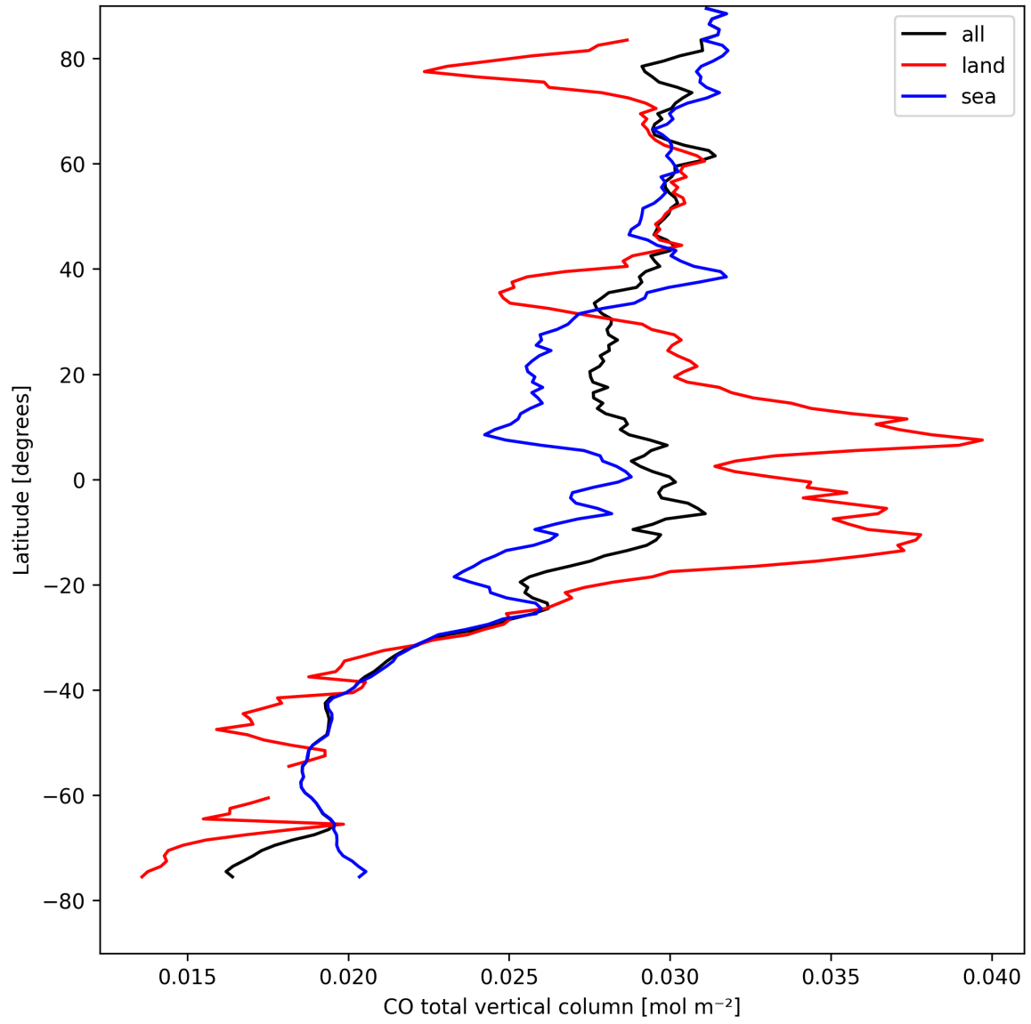
Figure 7: Zonal average of “CO total vertical column” for 2025-08-28 to 2025-08-28.
