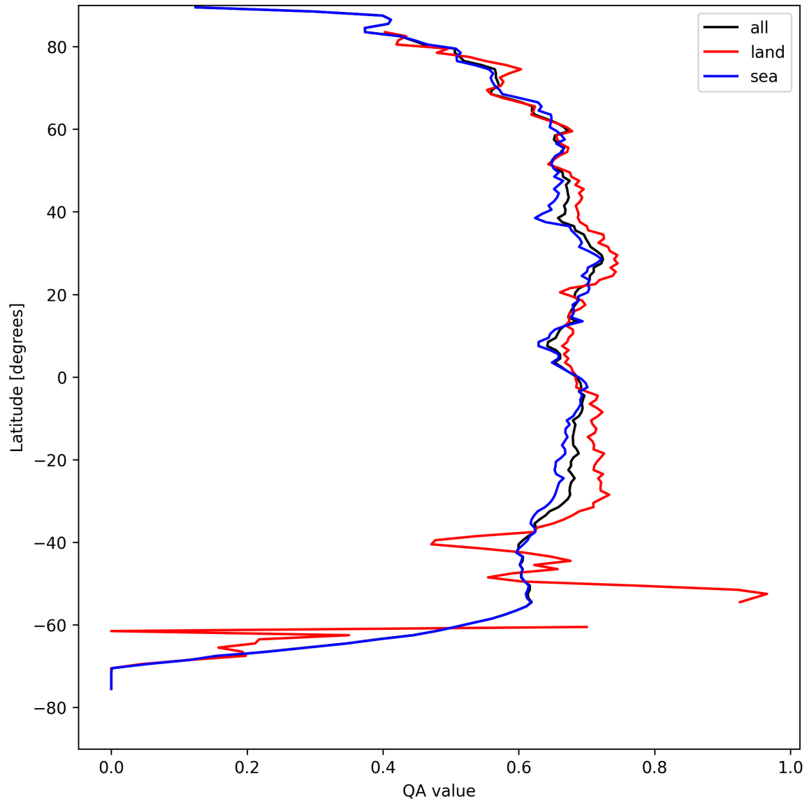
Figure 6: Zonal average of “QA value” for 2025-08-28 to 2025-08-28.
