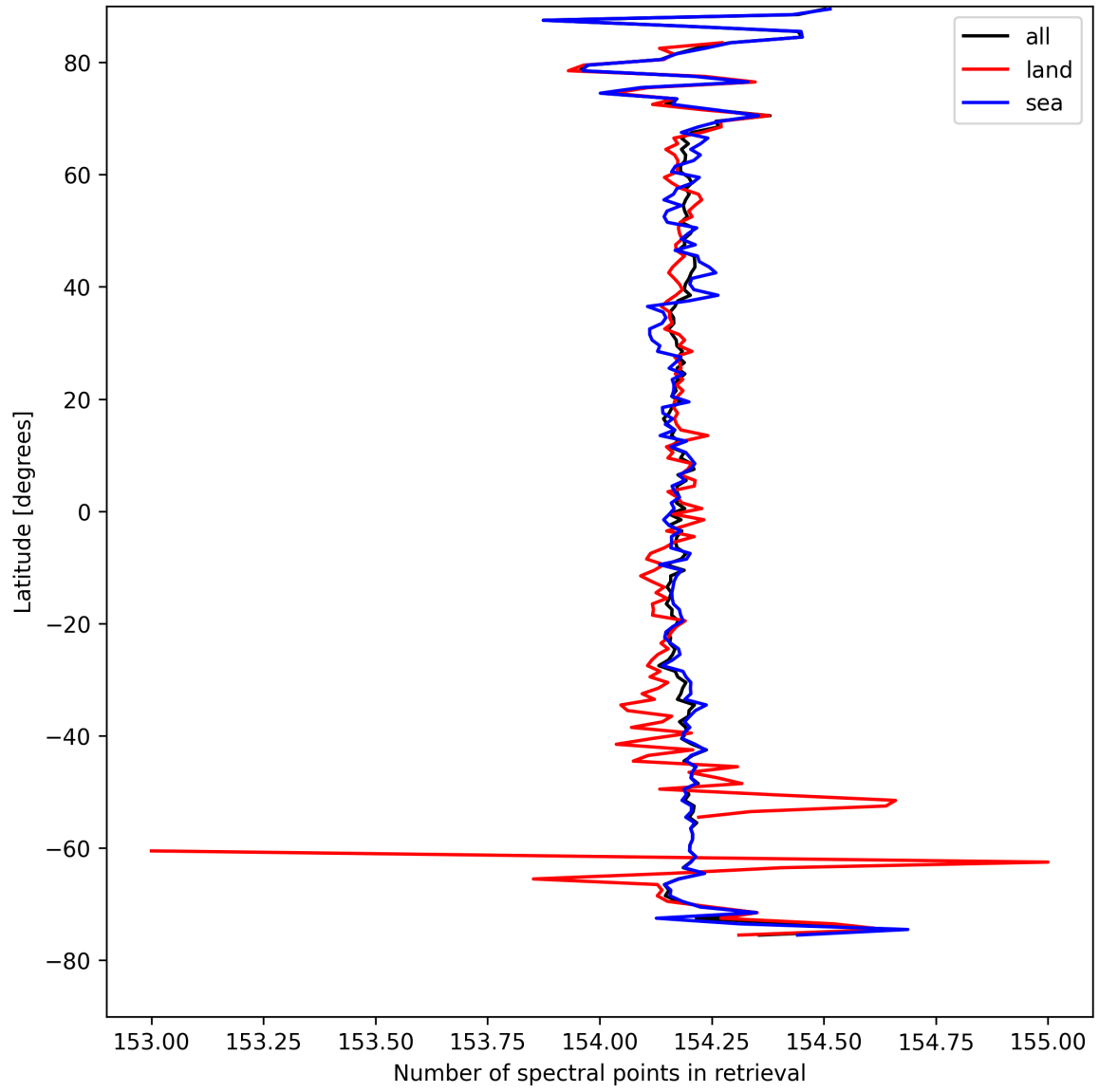
Figure 9: Zonal average of “Number of spectral points in retrieval” for 2025-08-28 to 2025-08-28.
