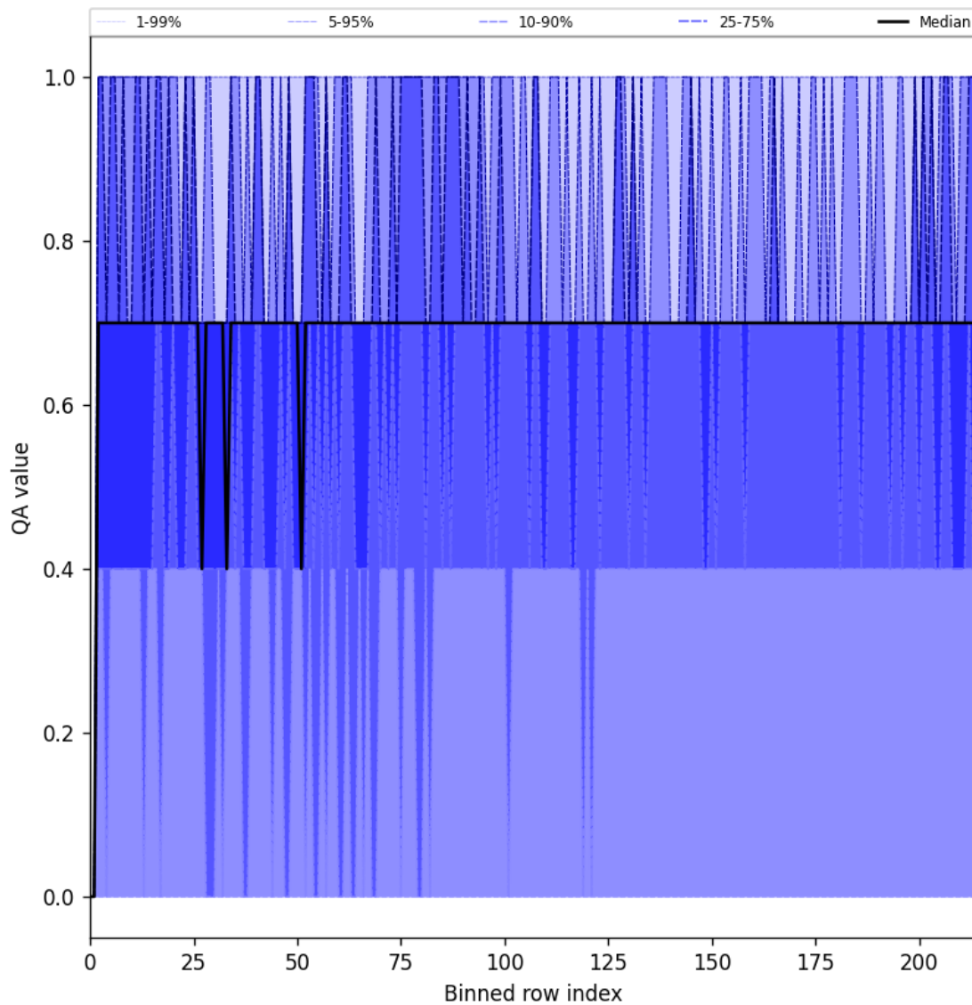
Figure 20: Along track statistics of “QA value” for 2025-08-28 to 2025-08-28
