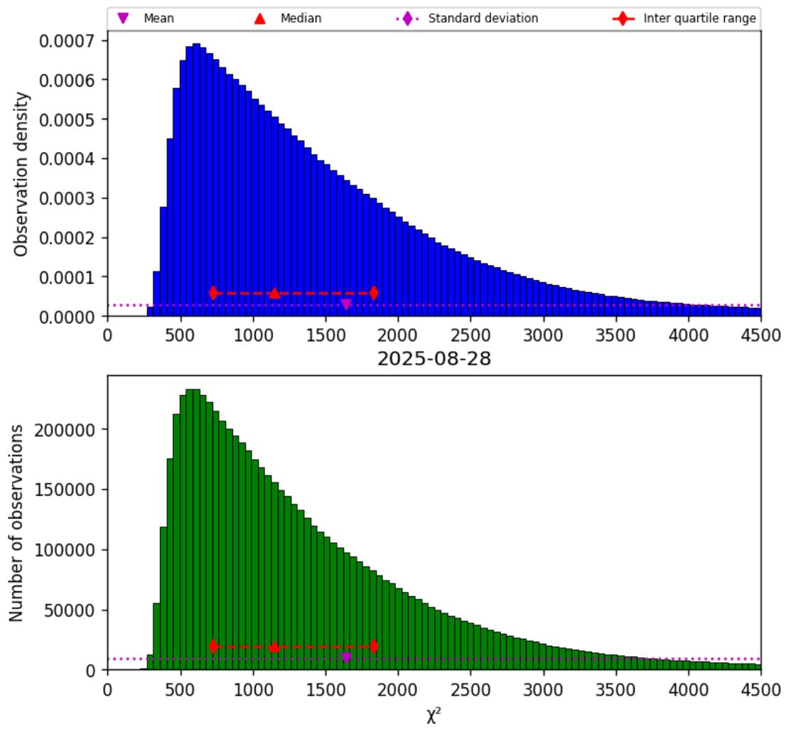
Figure 17: Histogram of " \chi^2 " for 2025-08-28 to 2025-08-28
