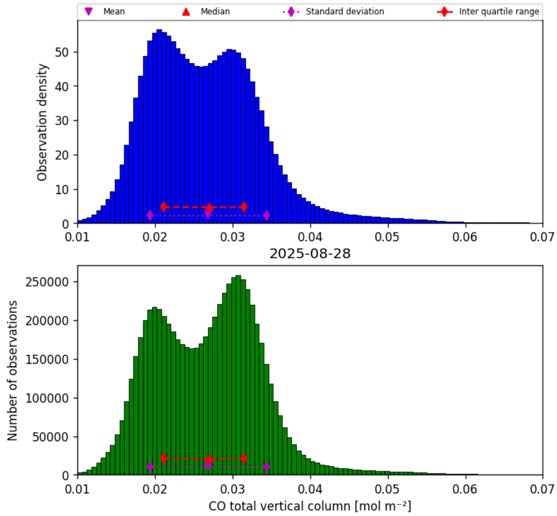
Figure 14: Histogram of “CO total vertical column” for 2025-08-28 to 2025-08-28
