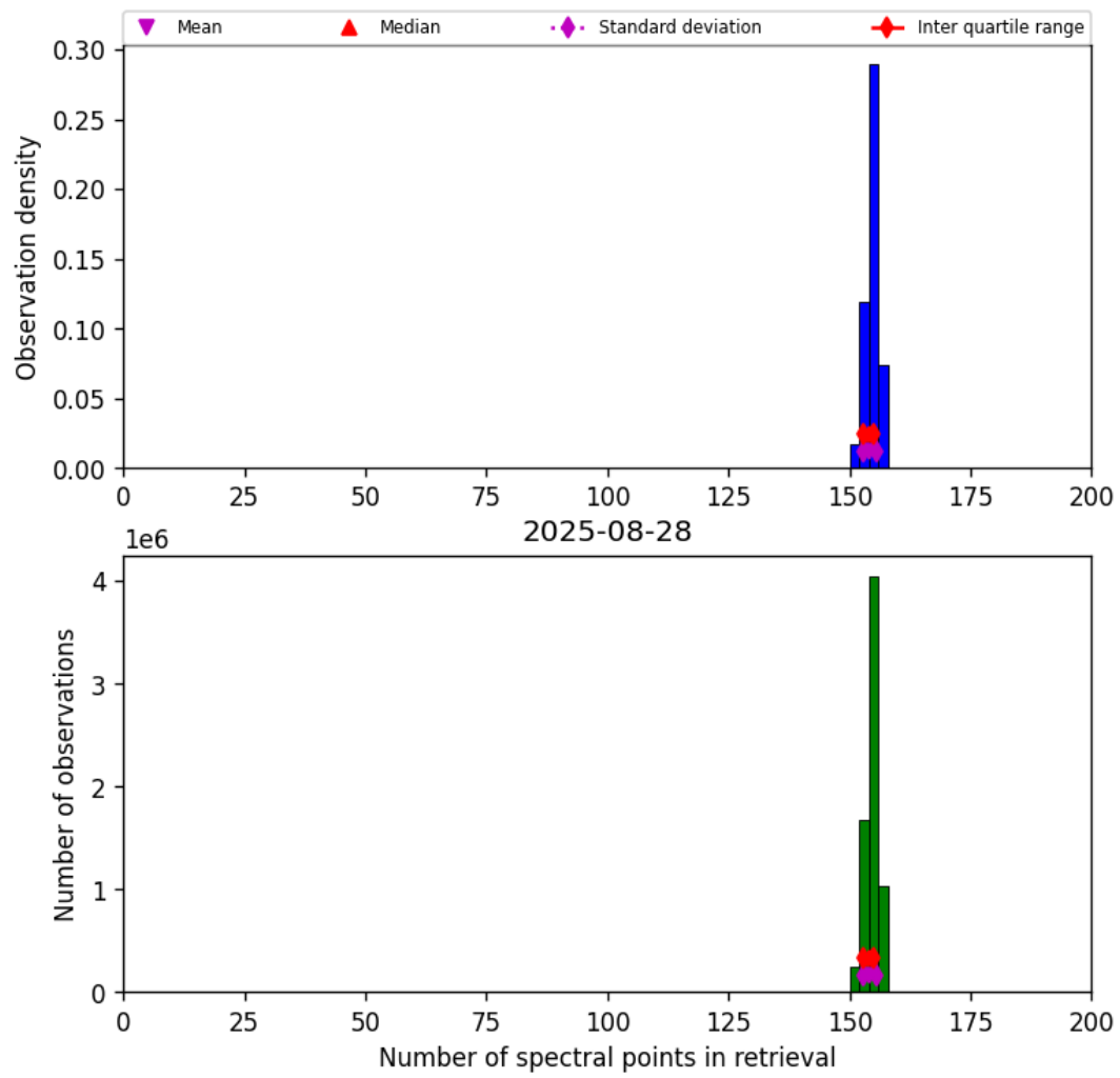
Figure 16: Histogram of “Number of spectral points in retrieval” for 2025-08-28 to 2025-08-28
