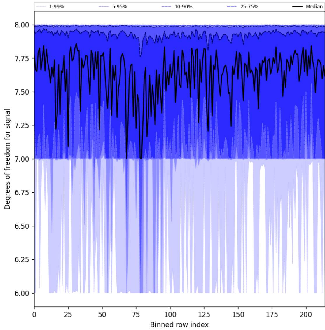
Figure 25: Along track statistics of “Degrees of freedom for signal” for 2025-08-28 to 2025-08-28
