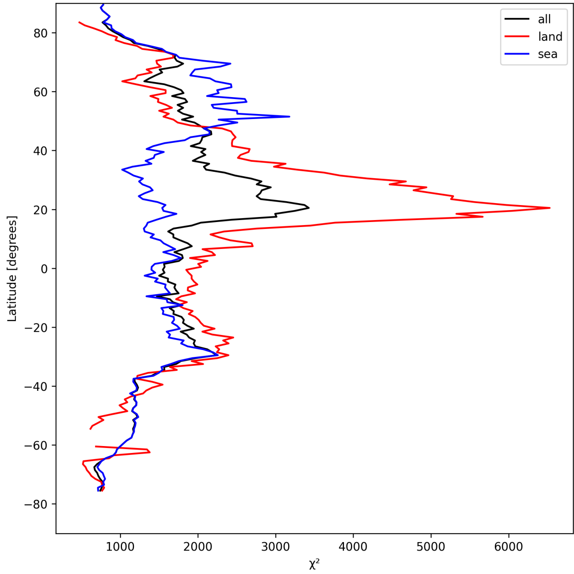
Figure 10: Zonal average of “ \chi^2 ” for 2025-08-28 to 2025-08-28.
