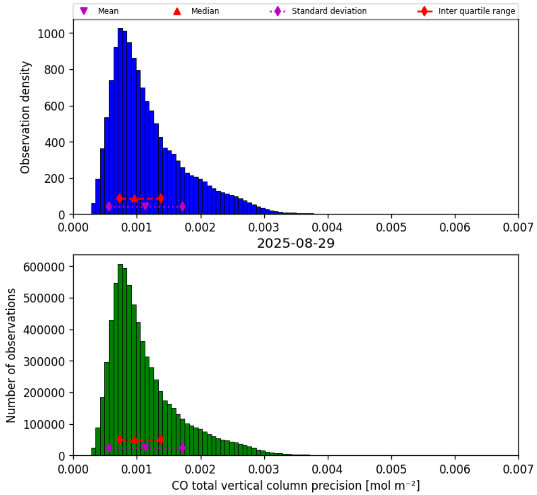
Figure 15: Histogram of “CO total vertical column precision” for 2025-08-29 to 2025-08-30
