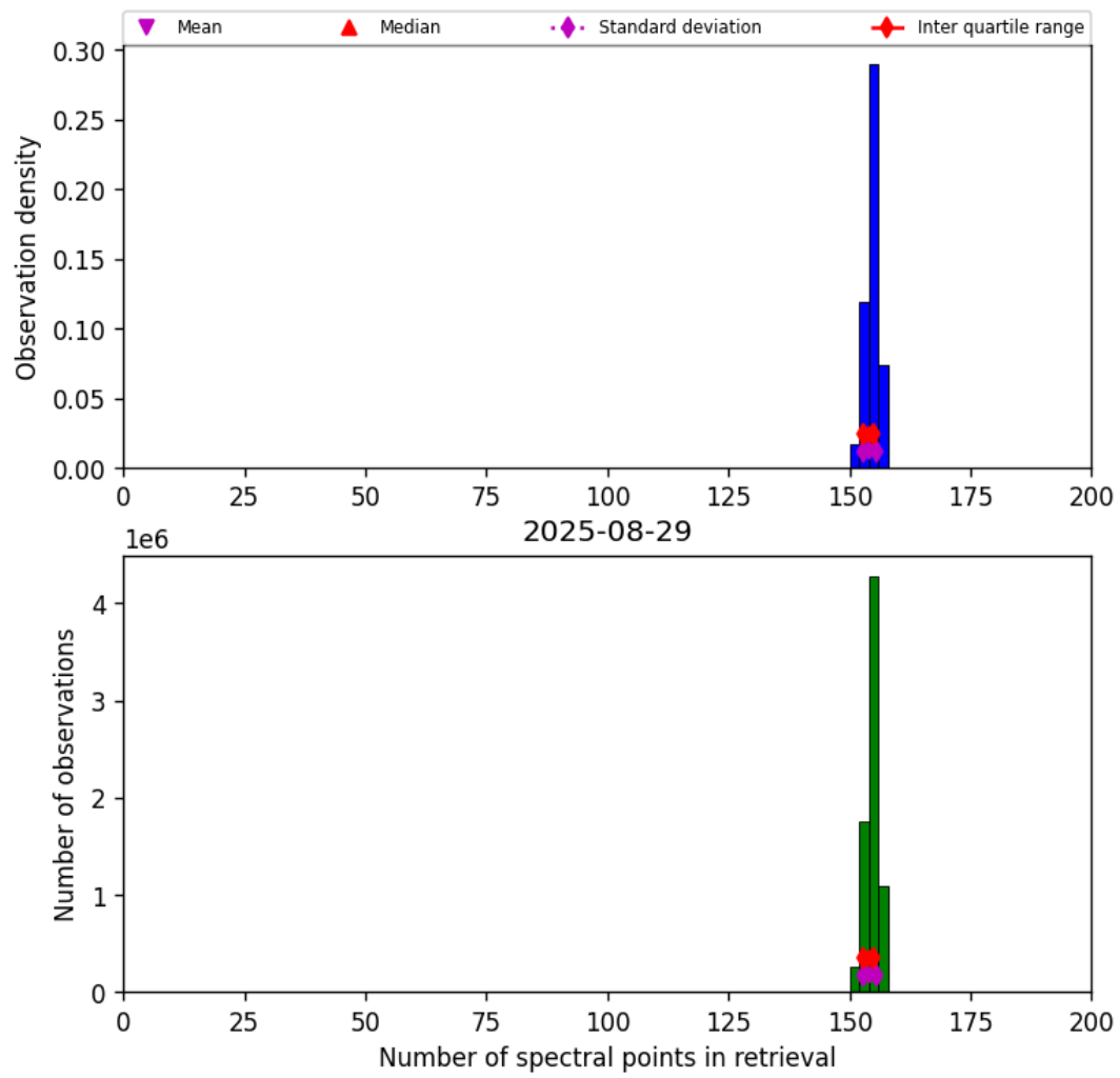
Figure 16: Histogram of “Number of spectral points in retrieval” for 2025-08-29 to 2025-08-30
