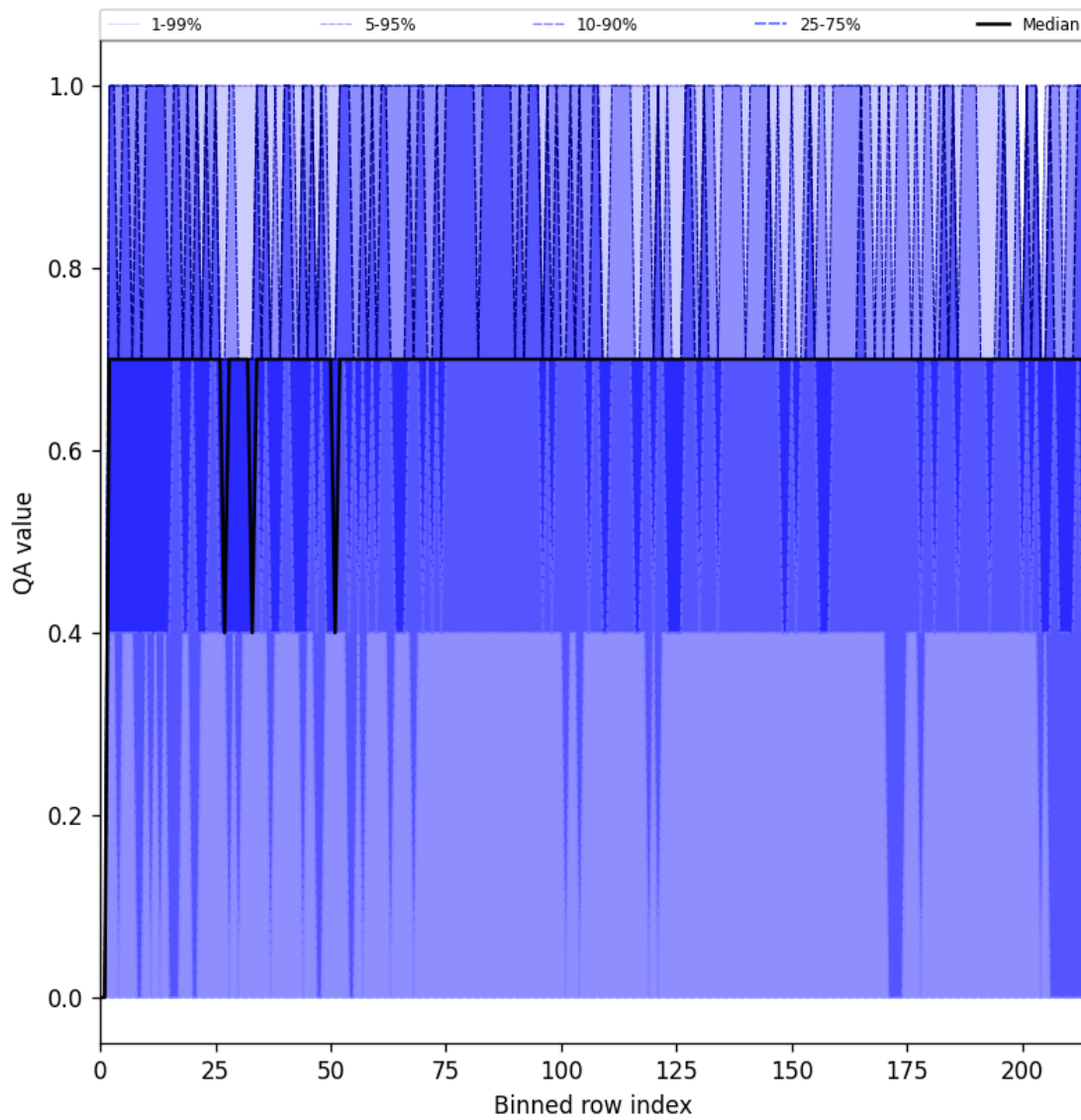
Figure 20: Along track statistics of “QA value” for 2025-08-29 to 2025-08-30
