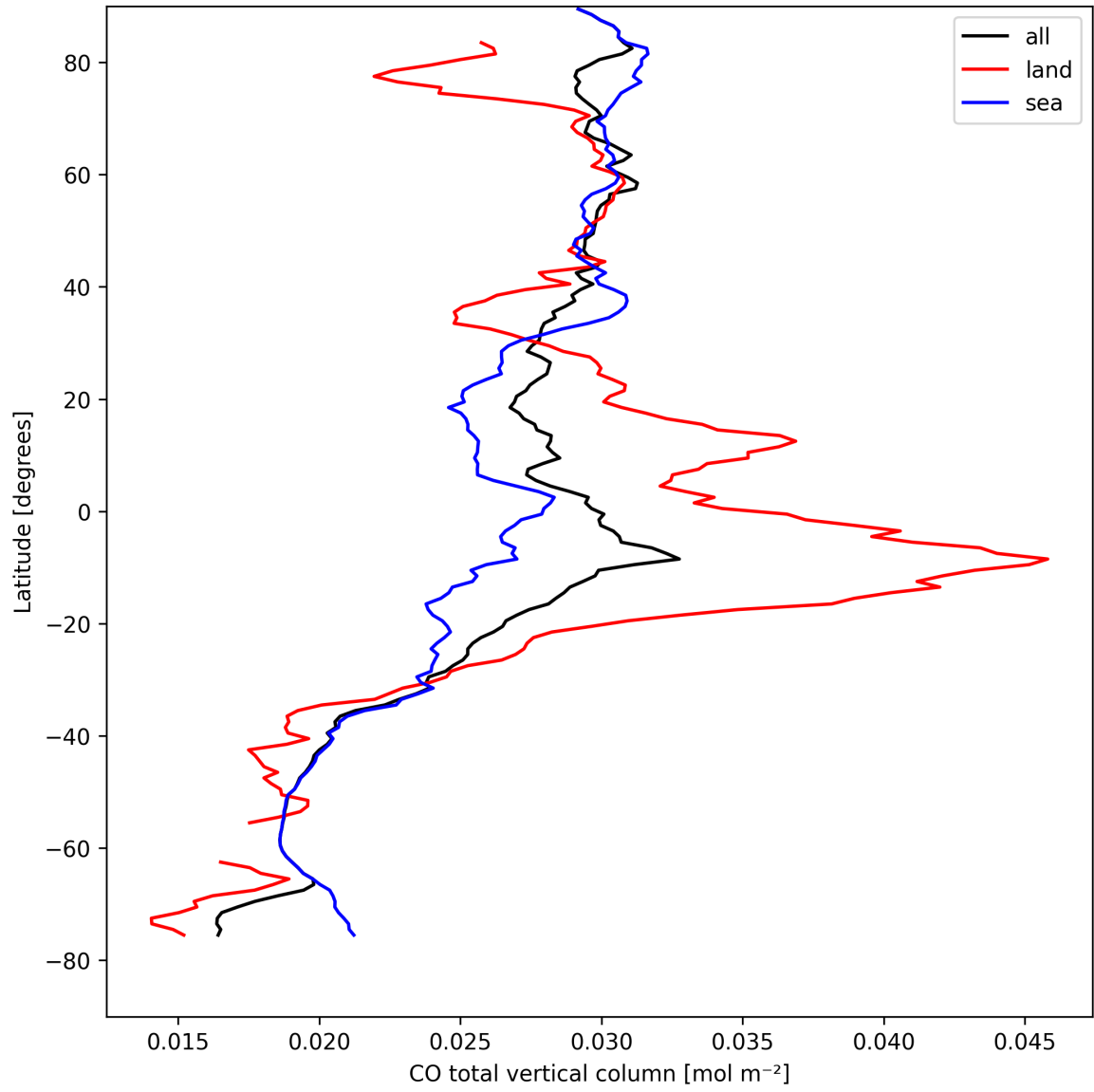
Figure 7: Zonal average of “CO total vertical column” for 2025-08-29 to 2025-08-30.
