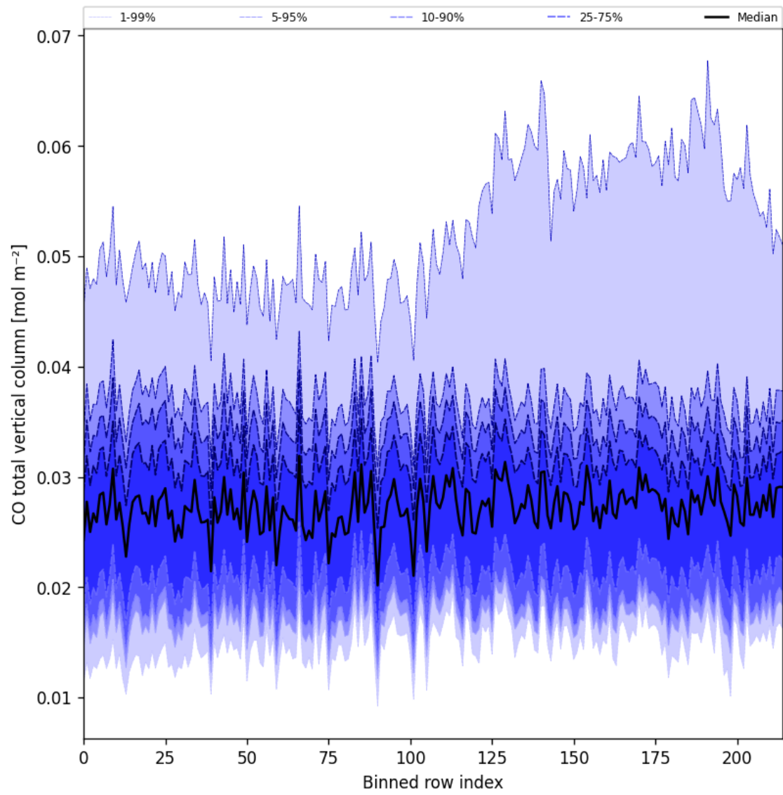
Figure 21: Along track statistics of “CO total vertical column” for 2025-08-29 to 2025-08-30
