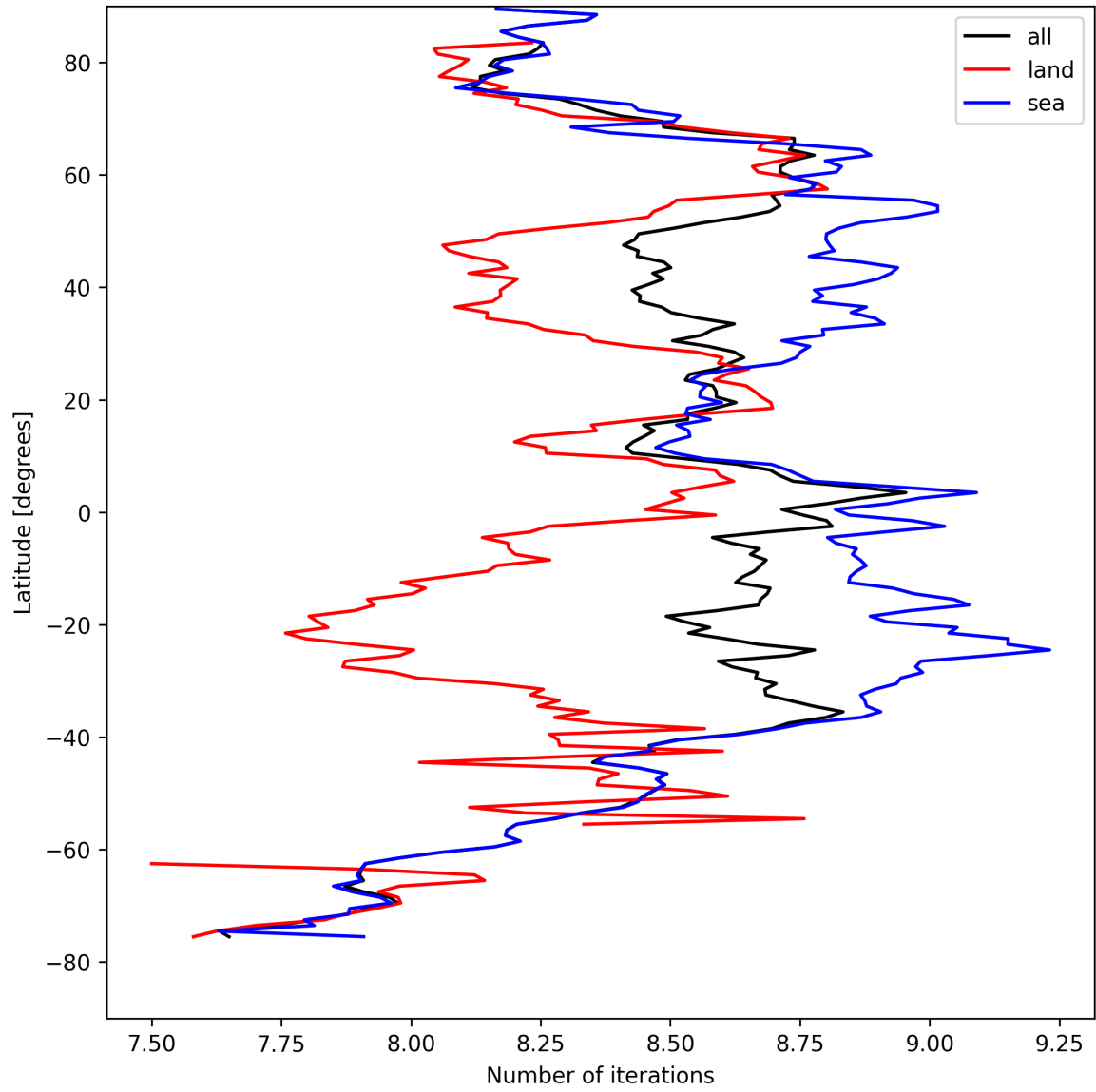
Figure 12: Zonal average of “Number of iterations” for 2025-08-29 to 2025-08-30.
