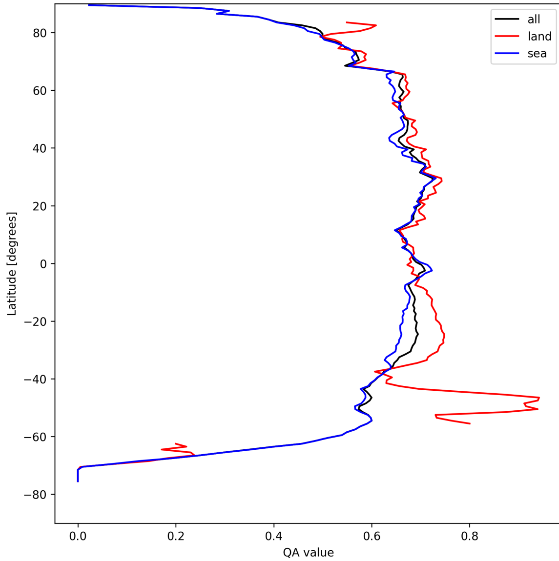
Figure 6: Zonal average of “QA value” for 2025-08-29 to 2025-08-30.
