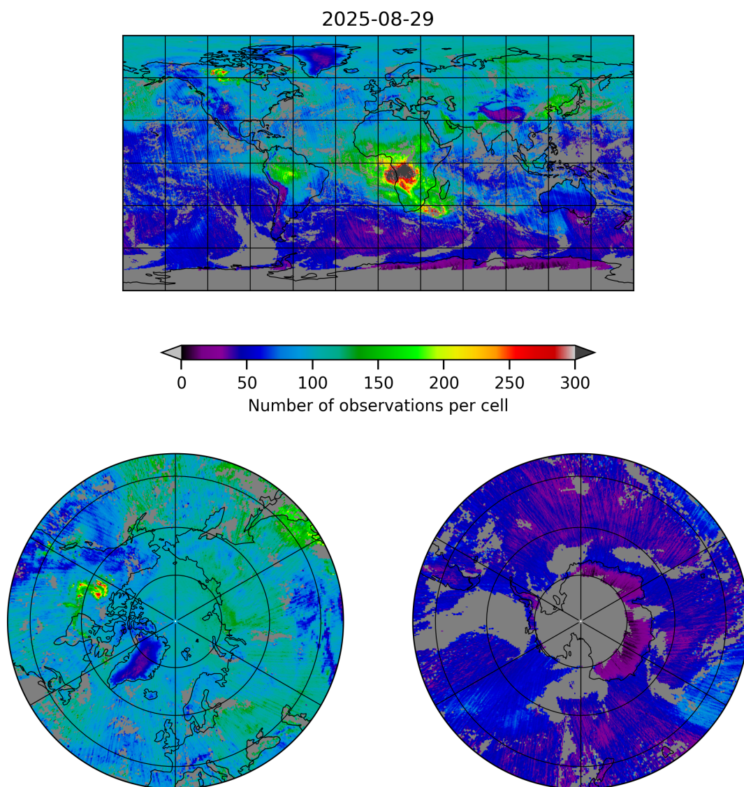
Figure 5: Map of the number of observations for 2025-08-29 to 2025-08-30
