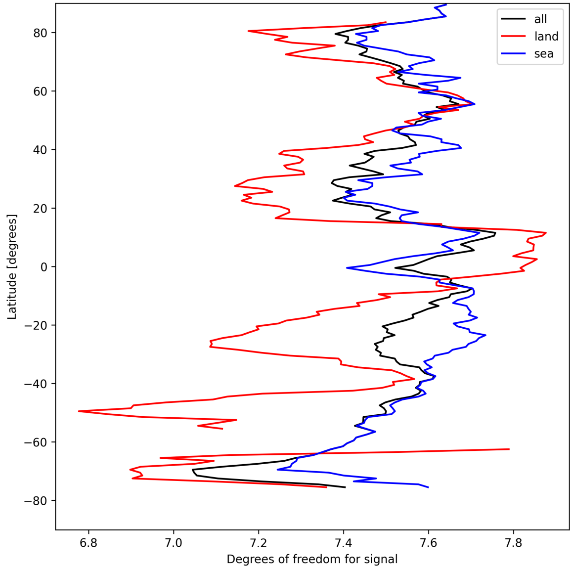
Figure 11: Zonal average of “Degrees of freedom for signal” for 2025-08-29 to 2025-08-30.
