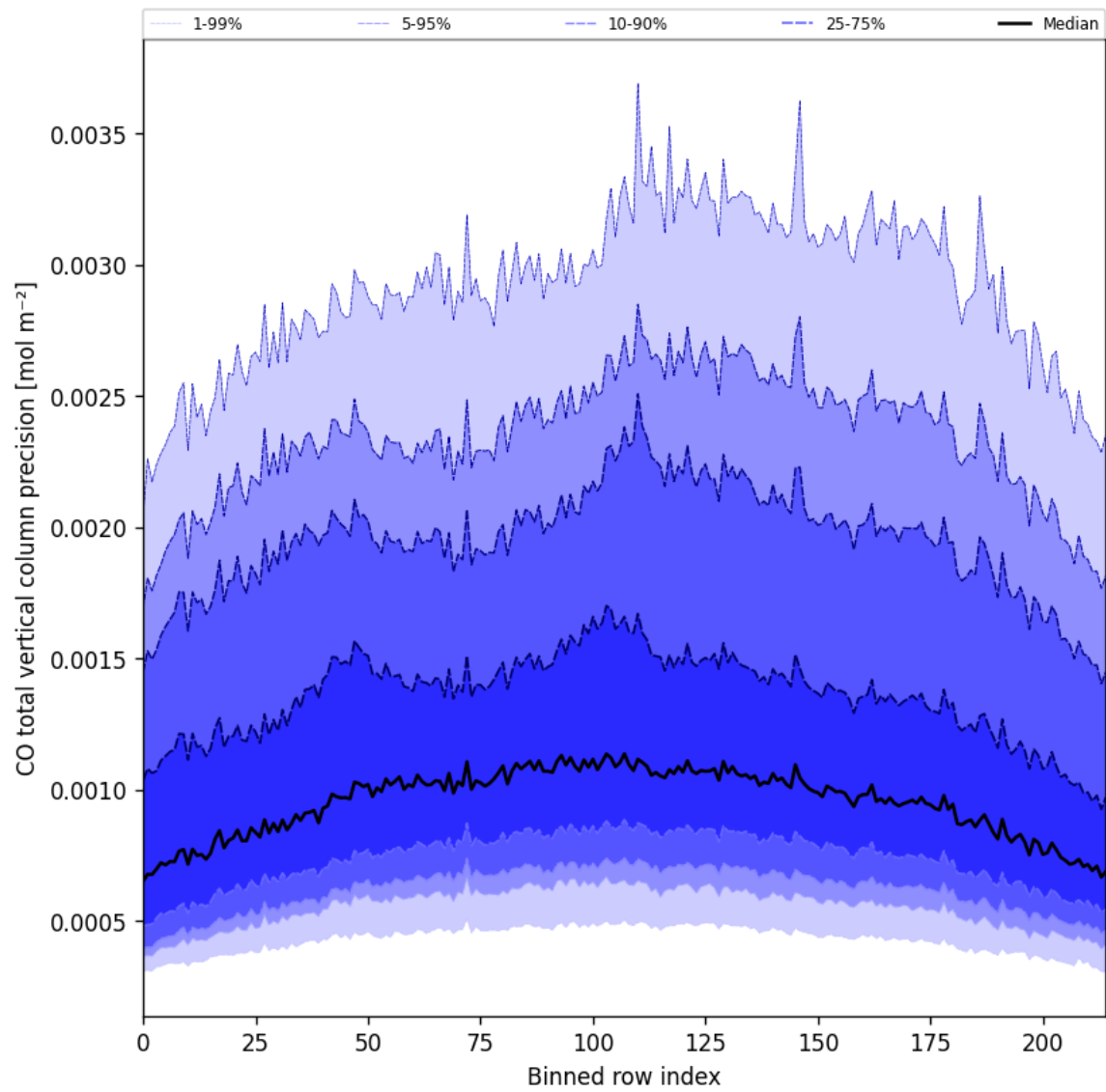
Figure 22: Along track statistics of “CO total vertical column precision” for 2025-08-29 to 2025-08-30
