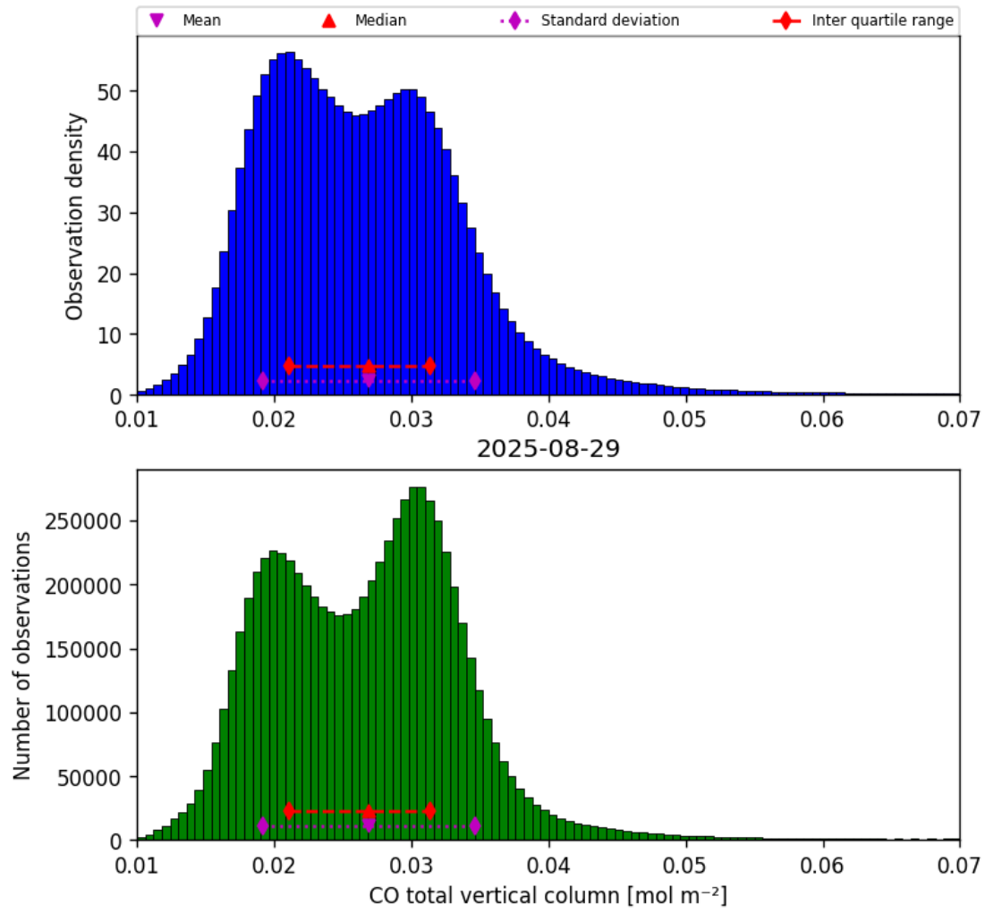
Figure 14: Histogram of “CO total vertical column” for 2025-08-29 to 2025-08-30
