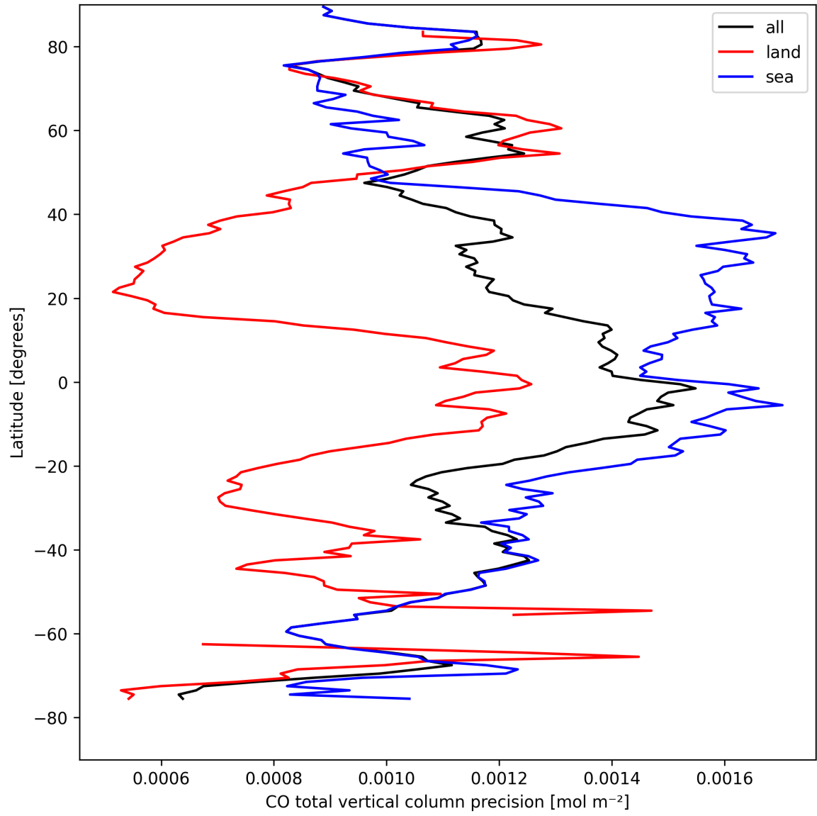
Figure 8: Zonal average of “CO total vertical column precision” for 2025-08-29 to 2025-08-30.
