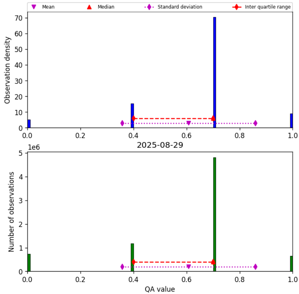
Figure 13: Histogram of “QA value” for 2025-08-29 to 2025-08-30
