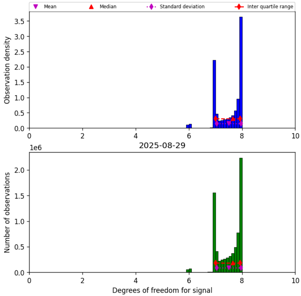
Figure 18: Histogram of “Degrees of freedom for signal” for 2025-08-29 to 2025-08-30
