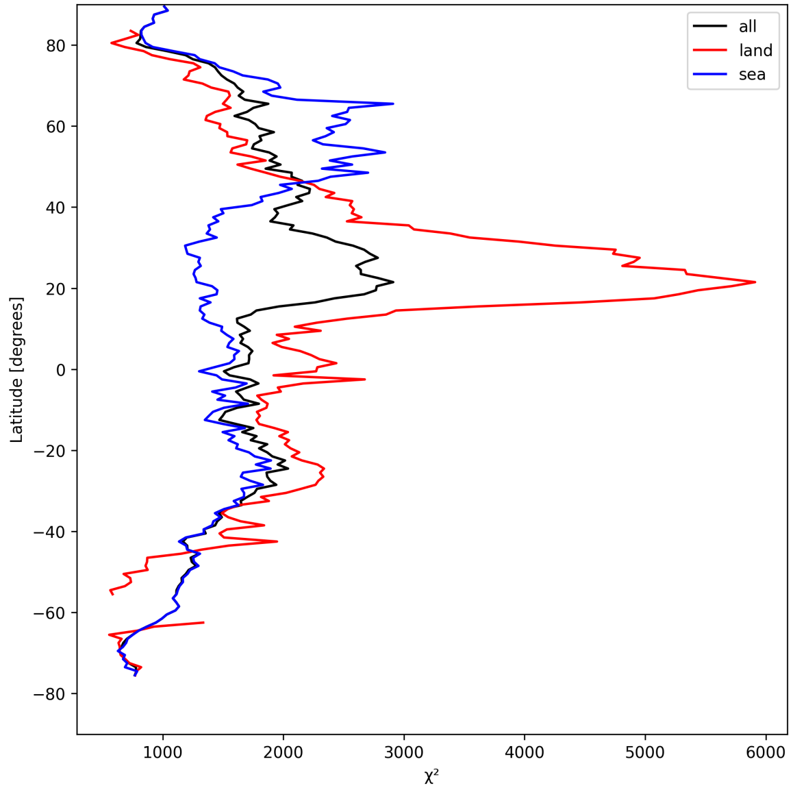
Figure 10: Zonal average of “ \chi^2 ” for 2025-08-29 to 2025-08-30.
