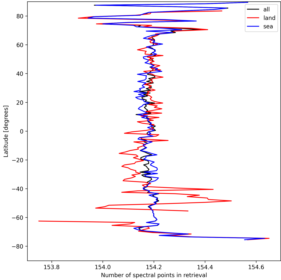
Figure 9: Zonal average of “Number of spectral points in retrieval” for 2025-08-29 to 2025-08-30.
