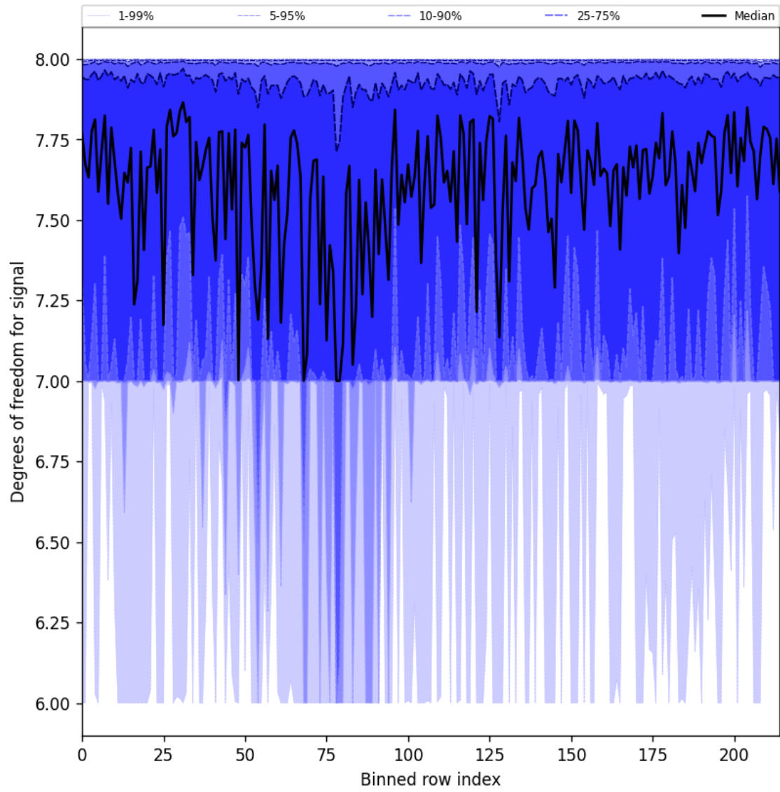
Figure 25: Along track statistics of “Degrees of freedom for signal” for 2025-08-29 to 2025-08-30
