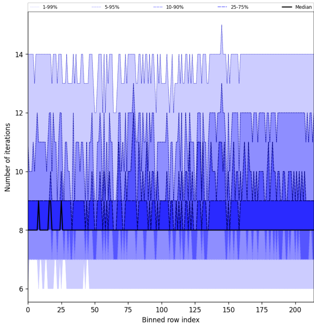
Figure 26: Along track statistics of “Number of iterations” for 2025-08-29 to 2025-08-30
