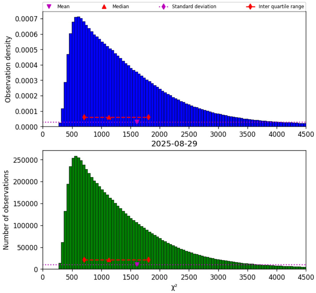
Figure 17: Histogram of “ \chi^2 ” for 2025-08-29 to 2025-08-30
