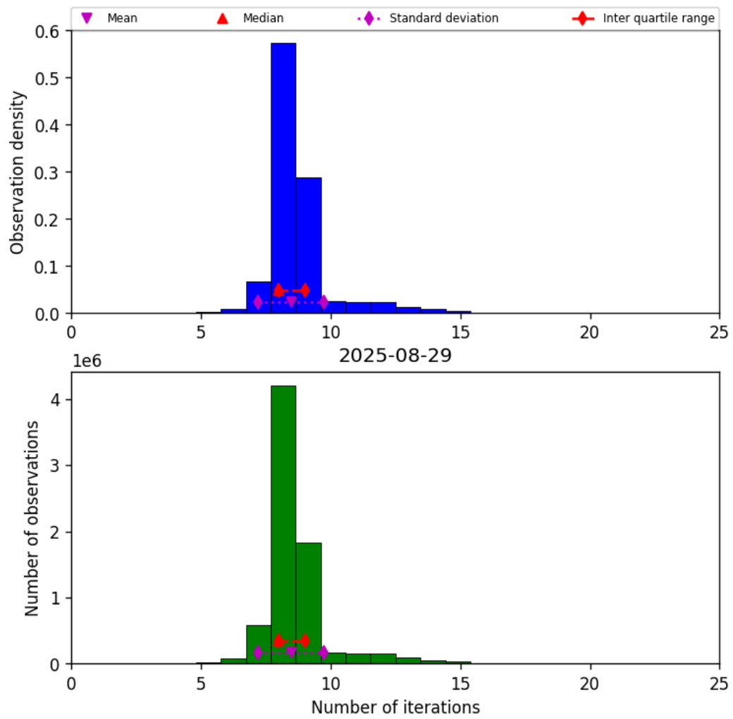
Figure 19: Histogram of “Number of iterations” for 2025-08-29 to 2025-08-30
