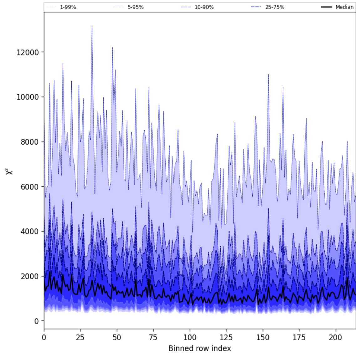
Figure 24: Along track statistics of “ \chi^2 ” for 2025-08-29 to 2025-08-30
