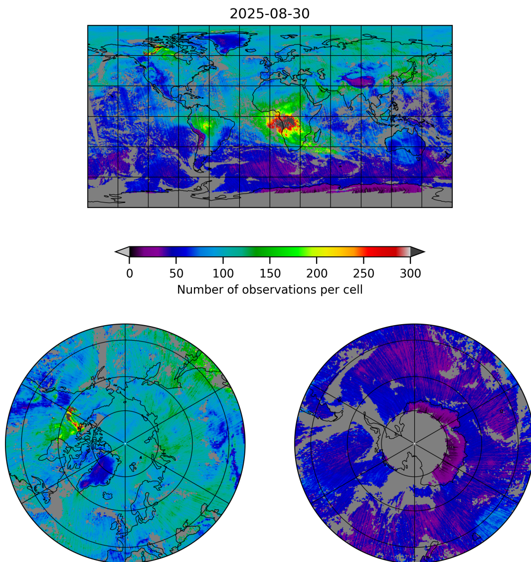
Figure 5: Map of the number of observations for 2025-08-30 to 2025-08-31
