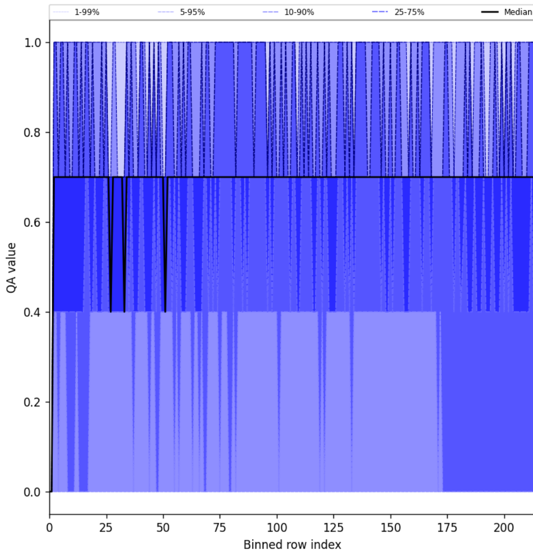
Figure 20: Along track statistics of “QA value” for 2025-08-30 to 2025-08-31
