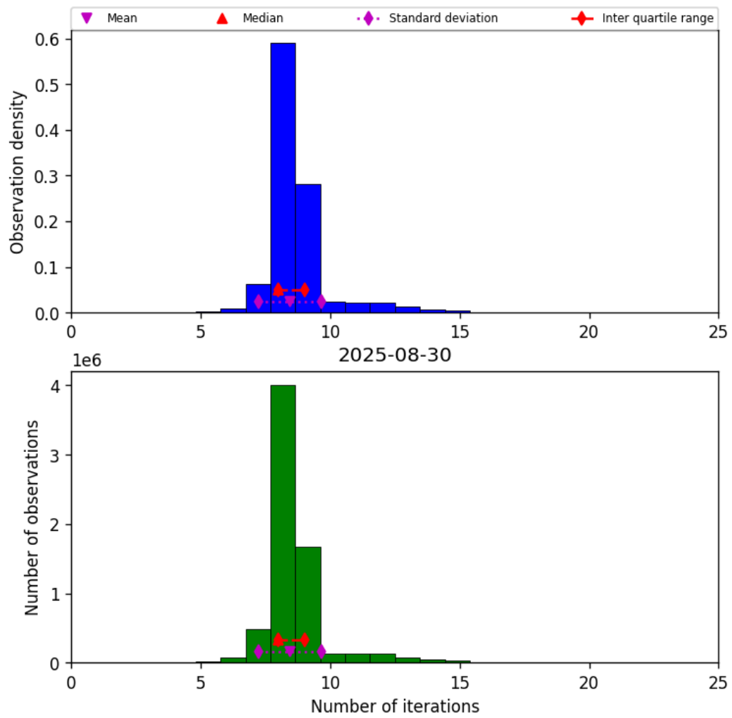
Figure 19: Histogram of “Number of iterations” for 2025-08-30 to 2025-08-31
