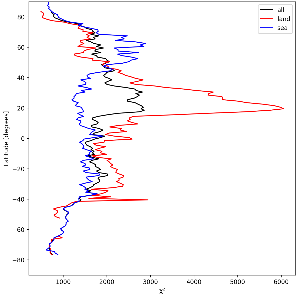
Figure 10: Zonal average of “ \chi^2 ” for 2025-08-30 to 2025-08-31.
