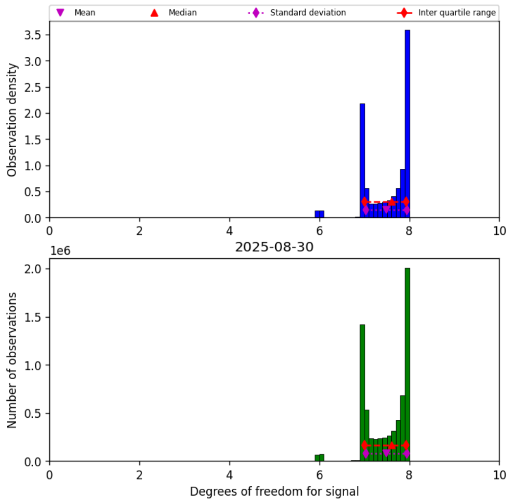
Figure 18: Histogram of “Degrees of freedom for signal” for 2025-08-30 to 2025-08-31
