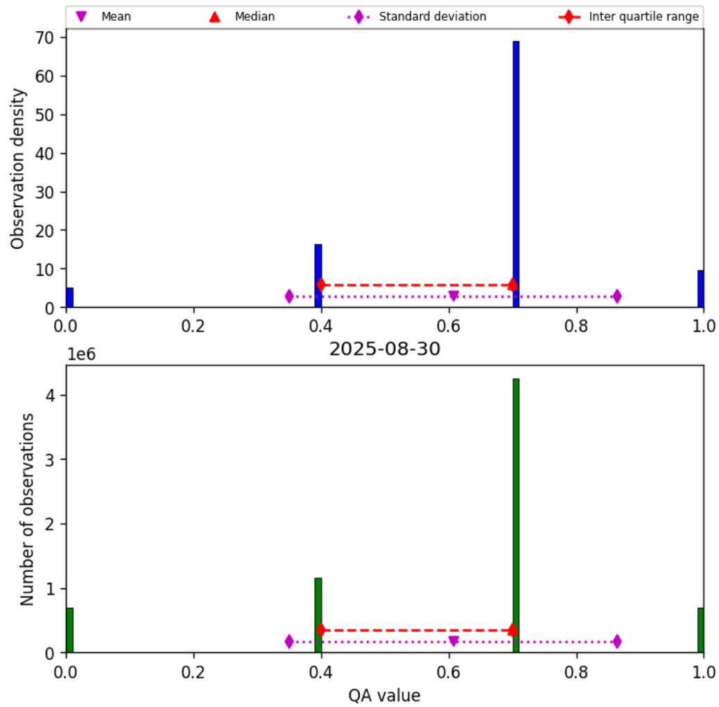
Figure 13: Histogram of “QA value” for 2025-08-30 to 2025-08-31
