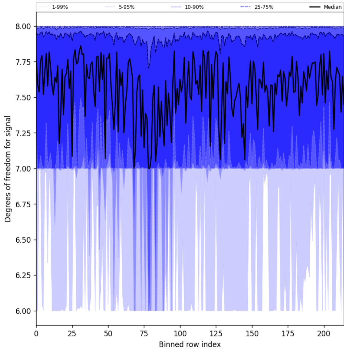
Figure 25: Along track statistics of “Degrees of freedom for signal” for 2025-08-30 to 2025-08-31
