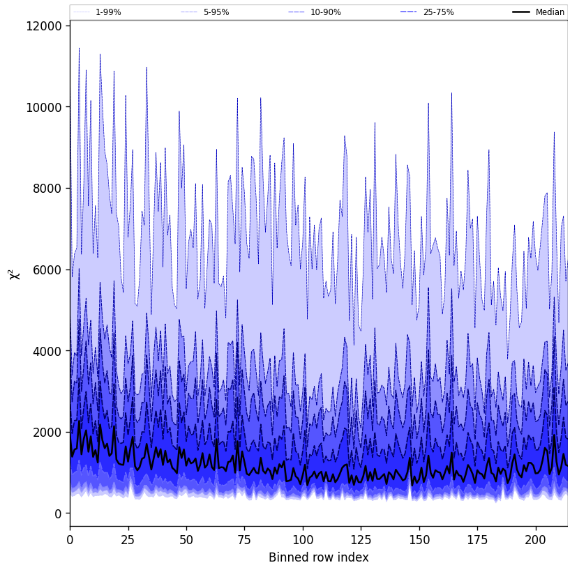
Figure 24: Along track statistics of “ \chi^2 ” for 2025-08-30 to 2025-08-31
