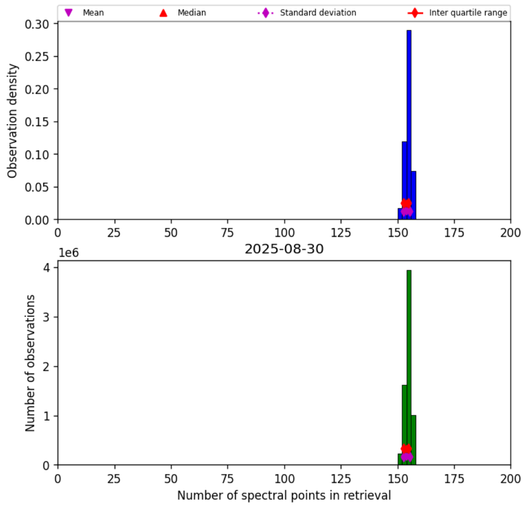
Figure 16: Histogram of “Number of spectral points in retrieval” for 2025-08-30 to 2025-08-31
