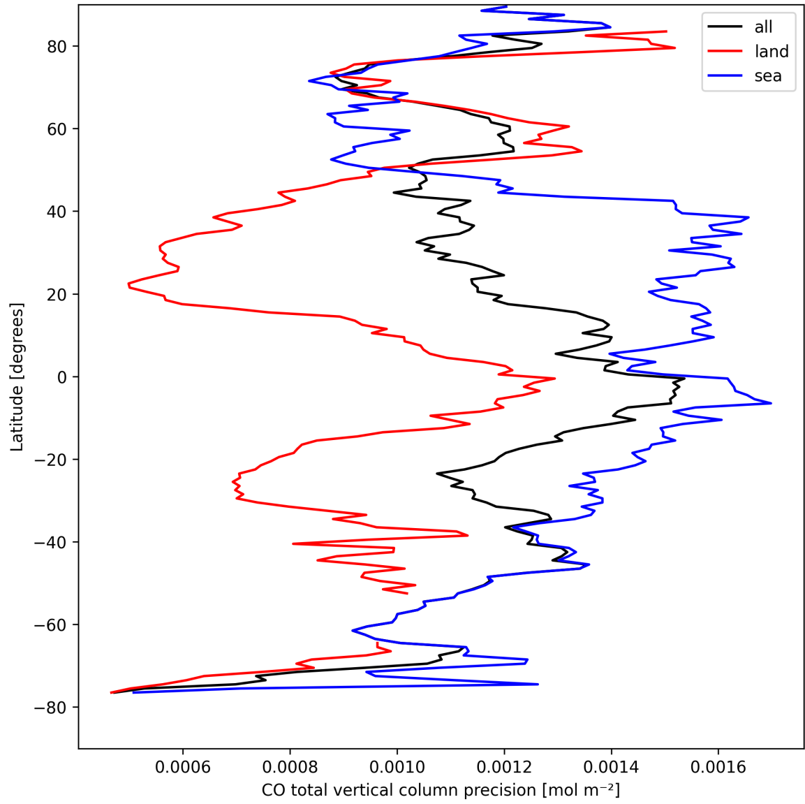
Figure 8: Zonal average of "CO total vertical column precision" for 2025-08-30 to 2025-08-31.
