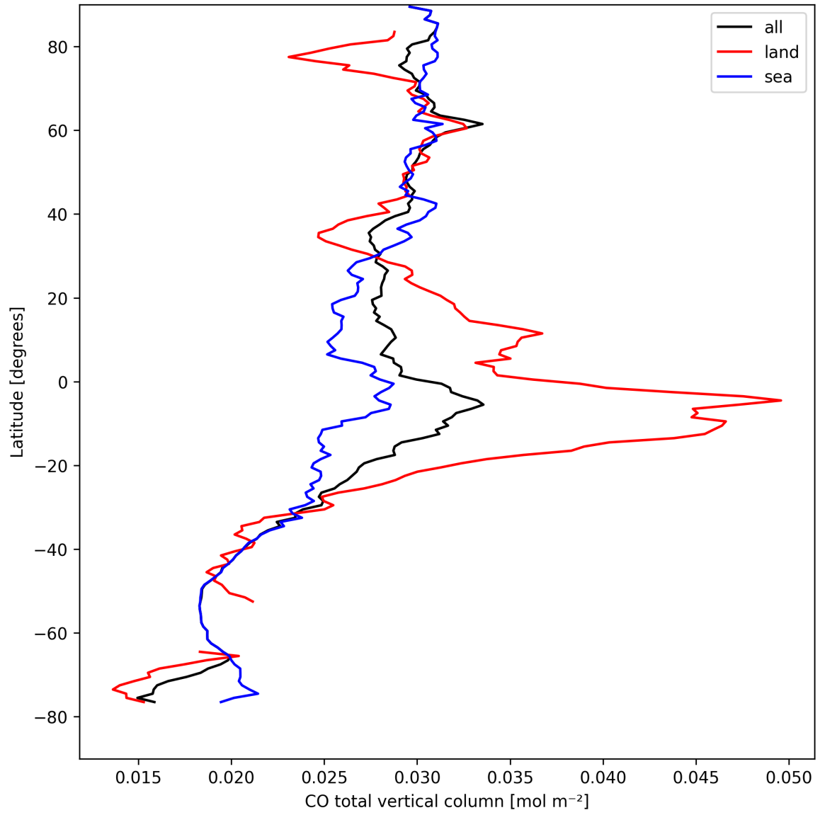
Figure 7: Zonal average of “CO total vertical column” for 2025-08-30 to 2025-08-31.
