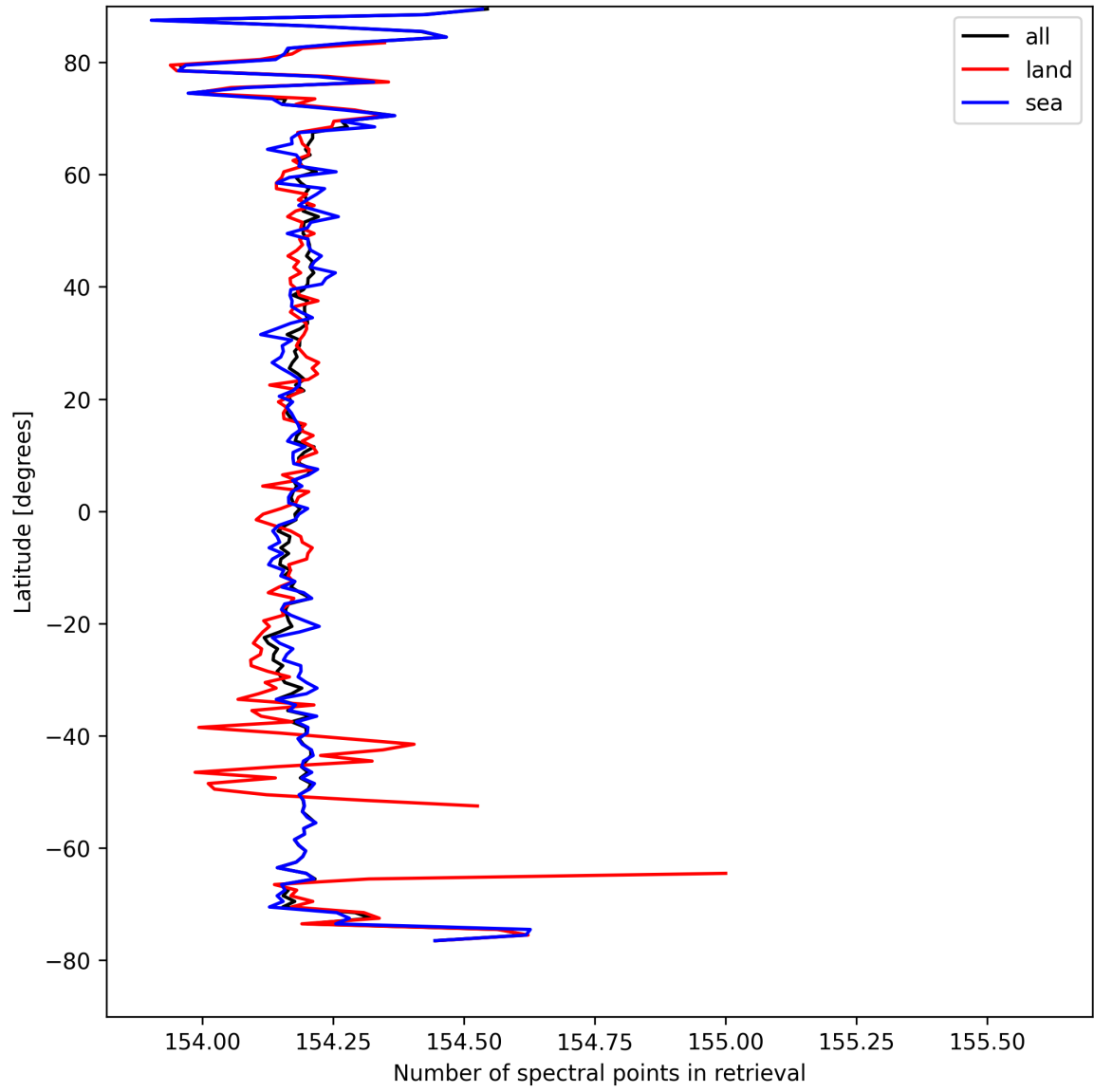
Figure 9: Zonal average of “Number of spectral points in retrieval” for 2025-08-30 to 2025-08-31.
