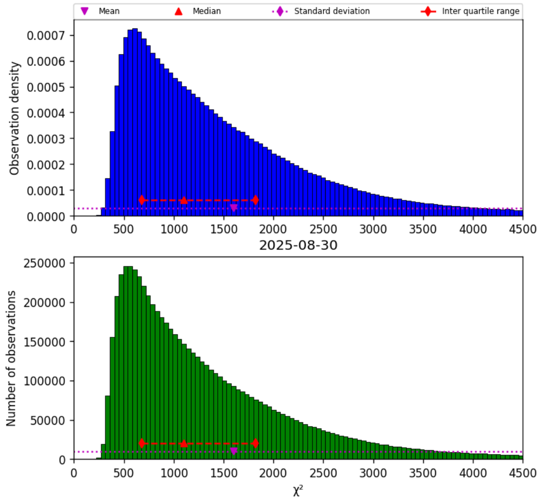
Figure 17: Histogram of " \chi^2 " for 2025-08-30 to 2025-08-31
