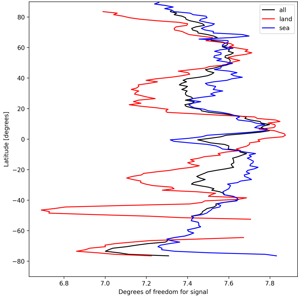
Figure 11: Zonal average of “Degrees of freedom for signal” for 2025-08-30 to 2025-08-31.
