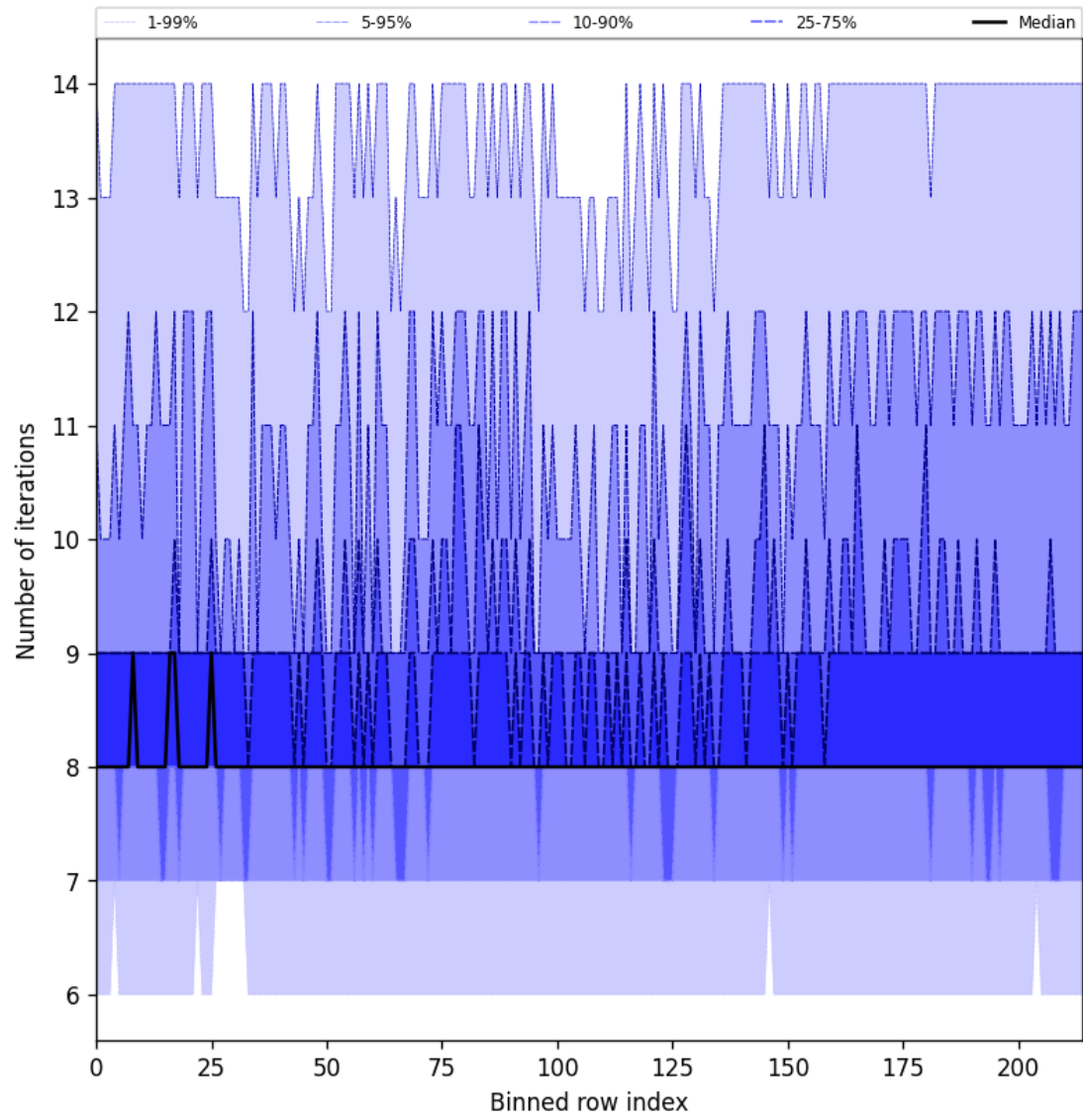
Figure 26: Along track statistics of “Number of iterations” for 2025-08-30 to 2025-08-31
