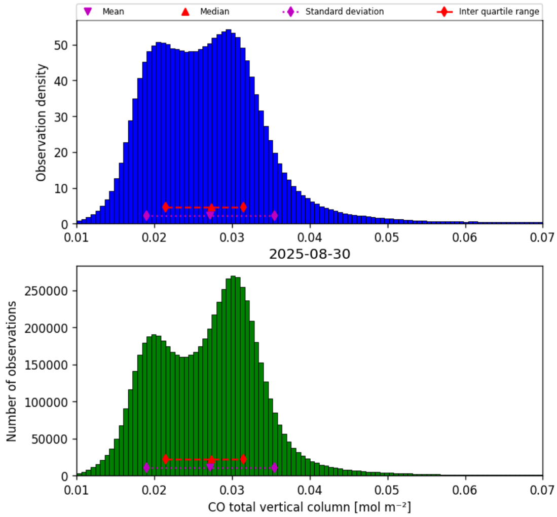
Figure 14: Histogram of “CO total vertical column” for 2025-08-30 to 2025-08-31
