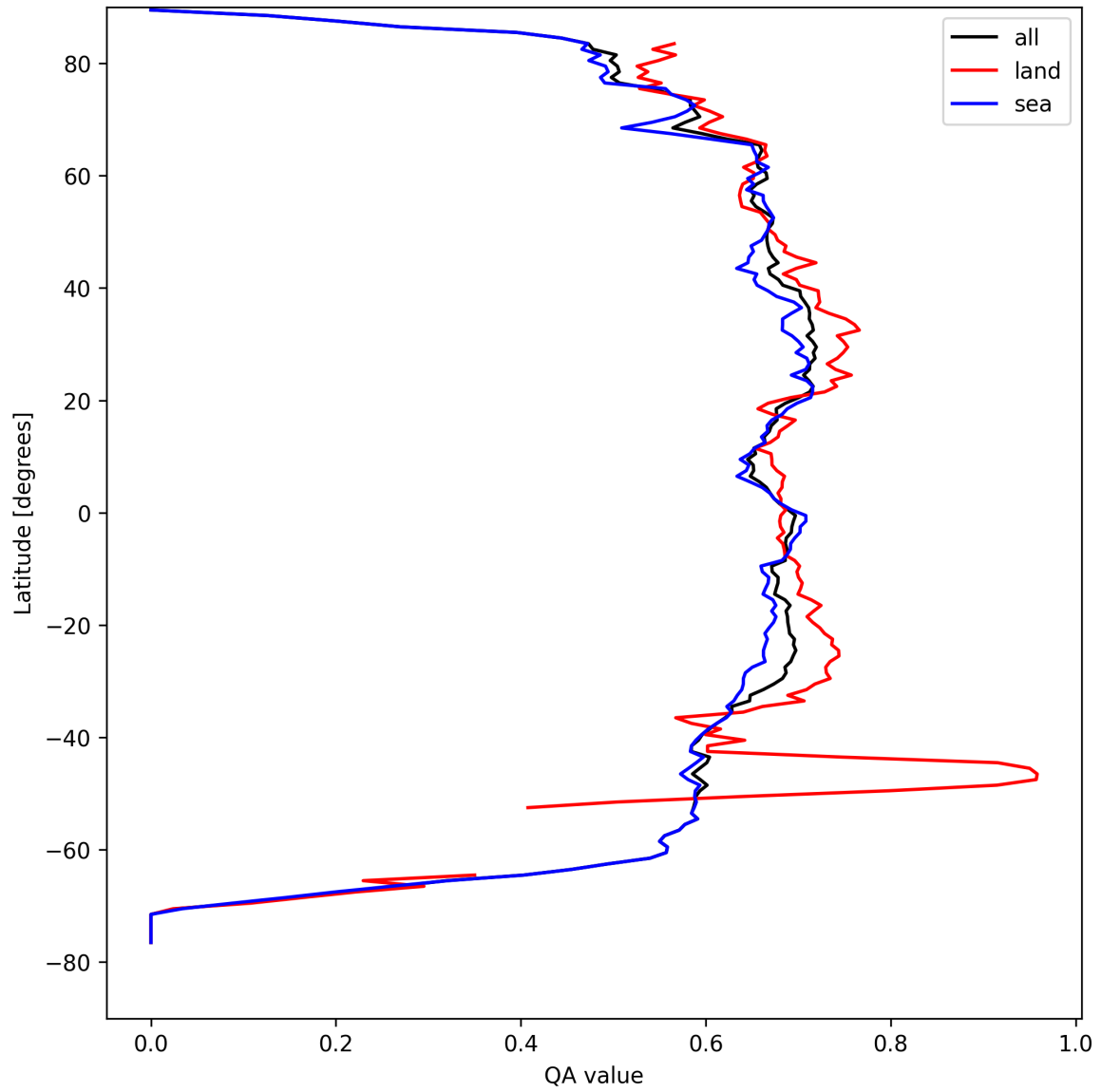
Figure 6: Zonal average of “QA value” for 2025-08-30 to 2025-08-31.
