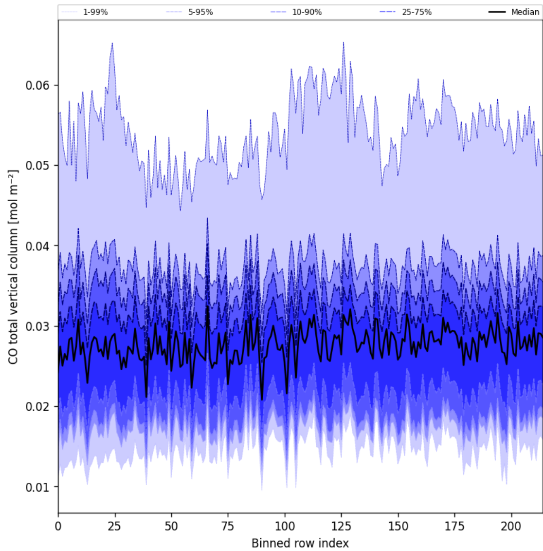
Figure 21: Along track statistics of “CO total vertical column” for 2025-08-30 to 2025-08-31
