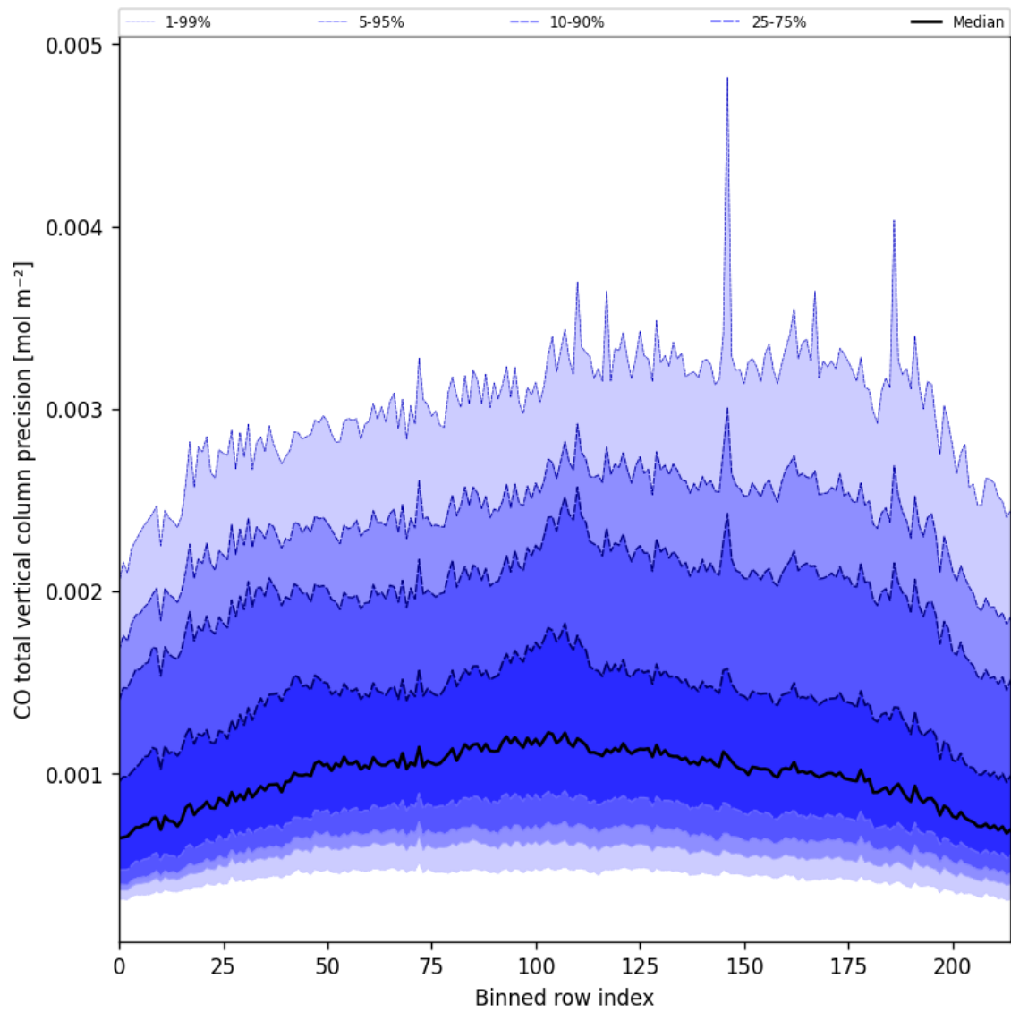
Figure 22: Along track statistics of “CO total vertical column precision” for 2025-08-30 to 2025-08-31
