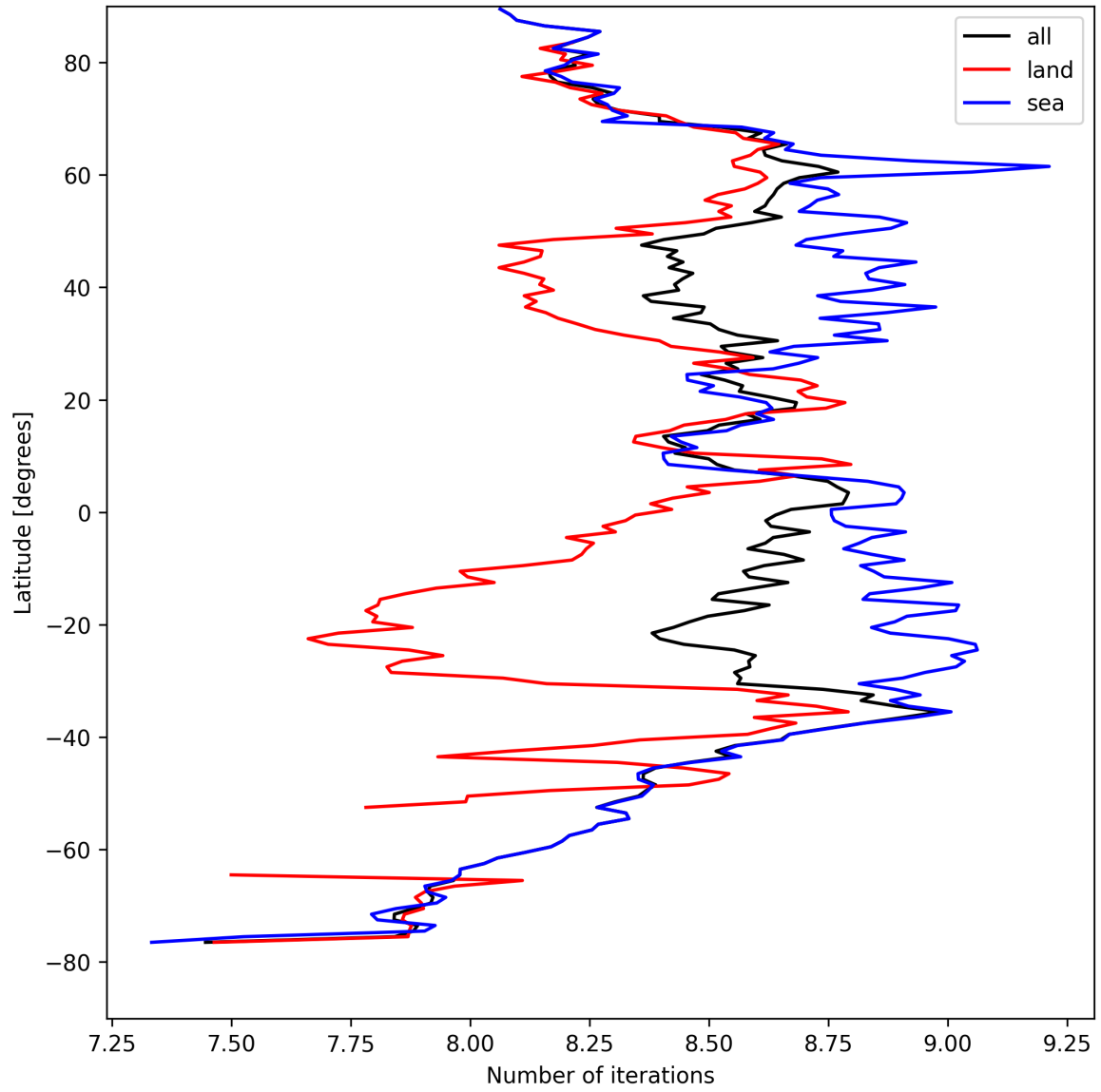
Figure 12: Zonal average of “Number of iterations” for 2025-08-30 to 2025-08-31.
