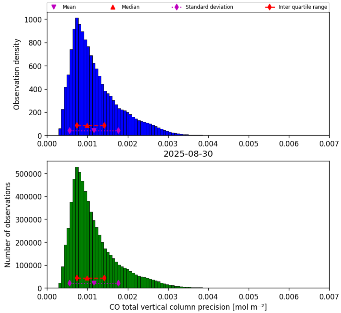
Figure 15: Histogram of “CO total vertical column precision” for 2025-08-30 to 2025-08-31
